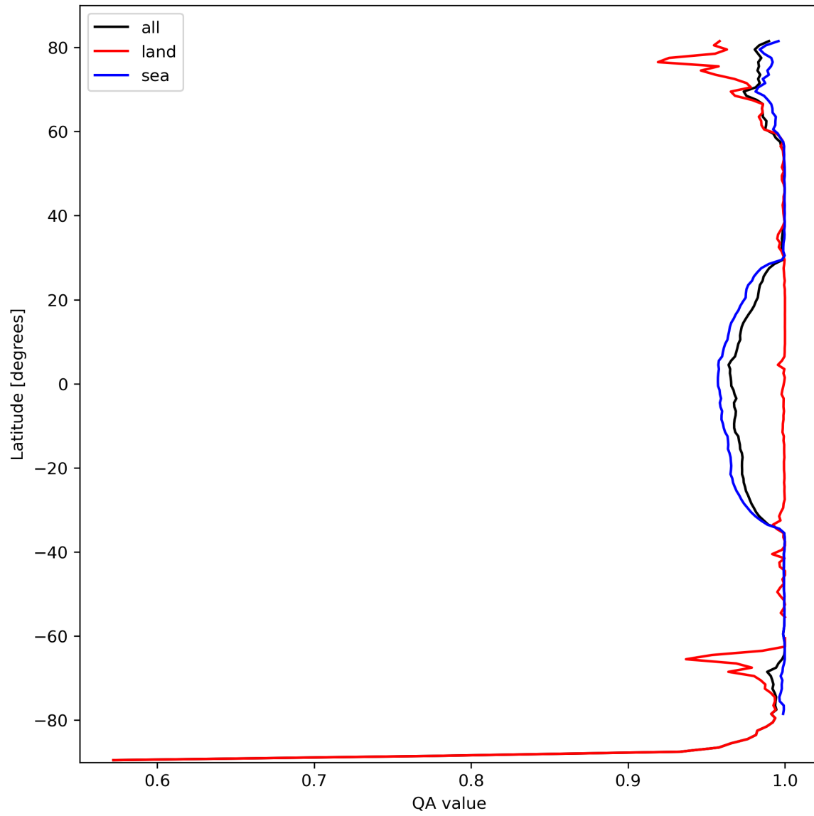
Figure 12: Zonal average of “QA value” for 2024-03-01 to 2024-03-03.
