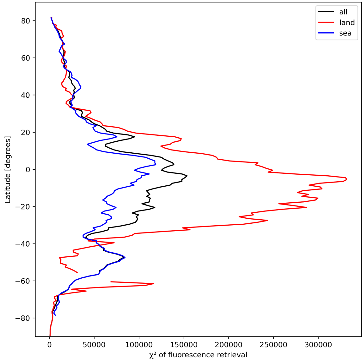
Figure 25: Zonal average of “ \chi^2 of fluorescence retrieval” for 2024-03-01 to 2024-03-03.
