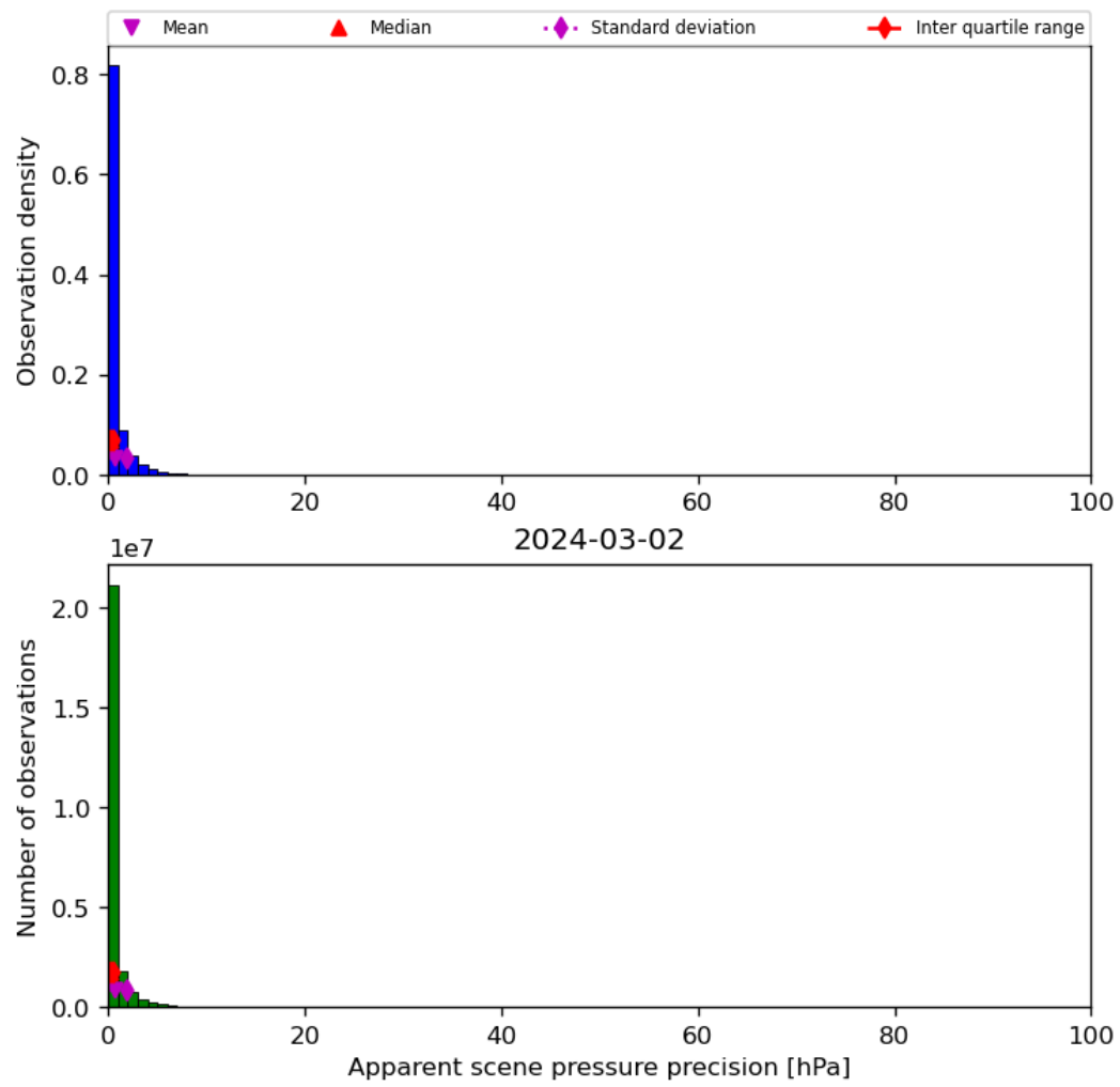
Figure 37: Histogram of "Apparent scene pressure precision" for 2024-03-01 to 2024-03-03
