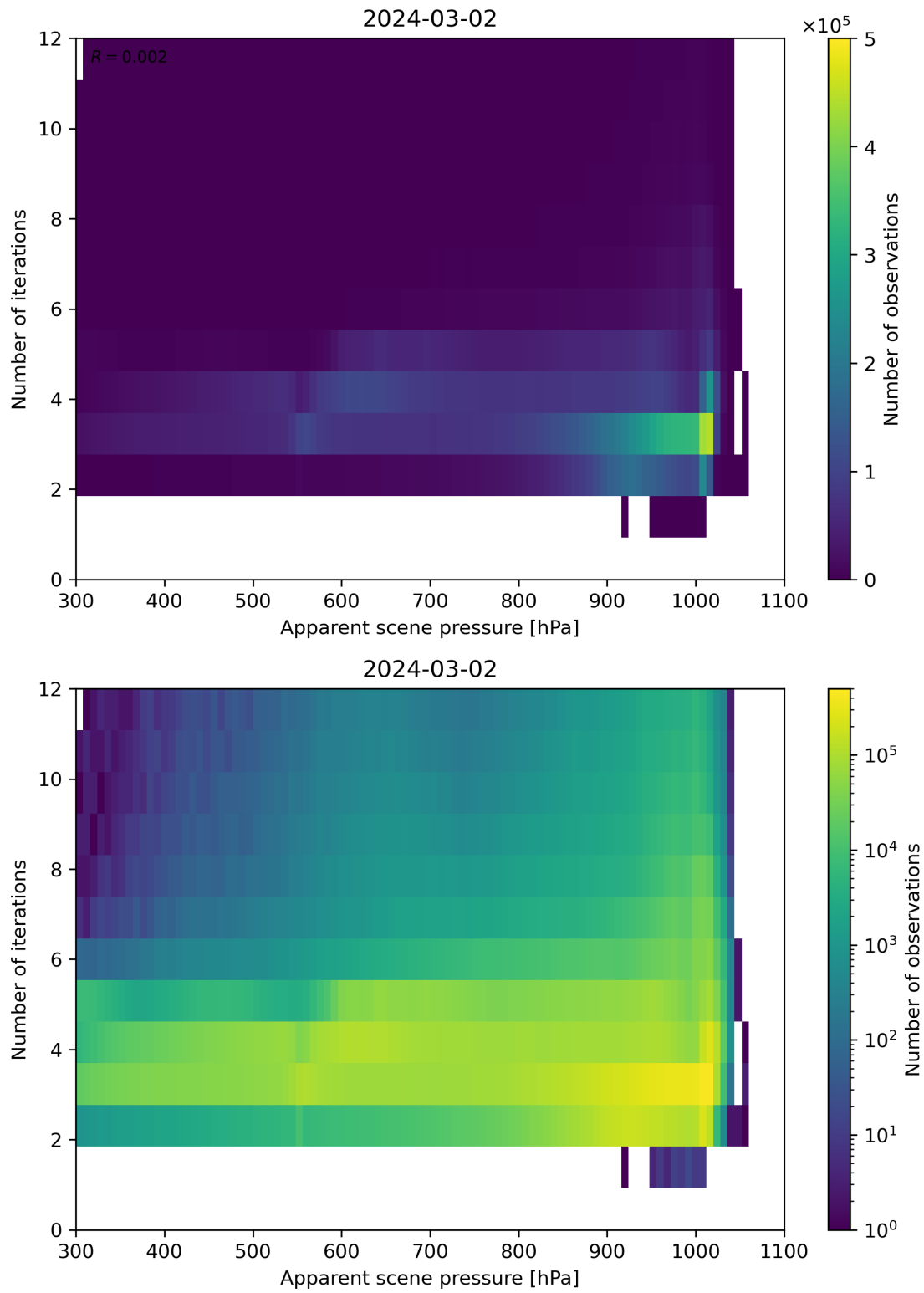
Figure 65: Scatter density plot of “Apparent scene pressure” against “Number of iterations” for 2024-03-01 to 2024-03-03.
