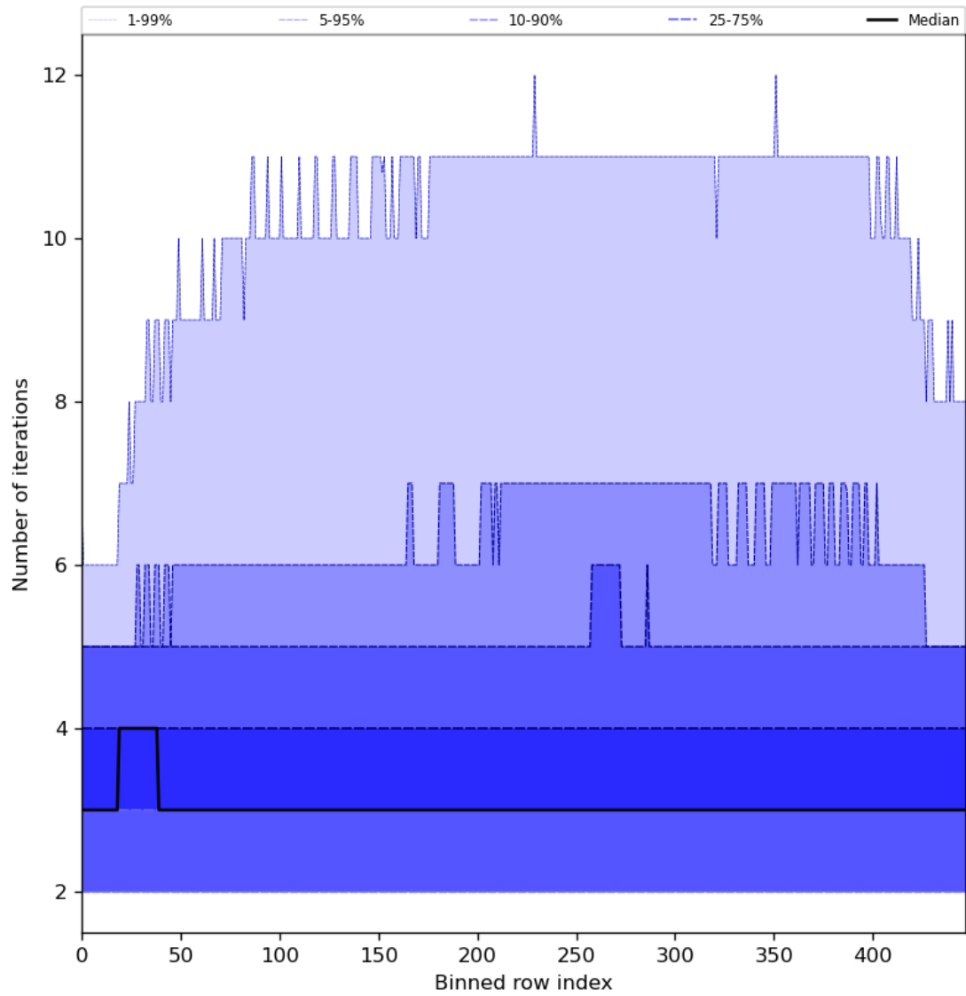
Figure 56: Along track statistics of “Number of iterations” for 2024-03-01 to 2024-03-03
