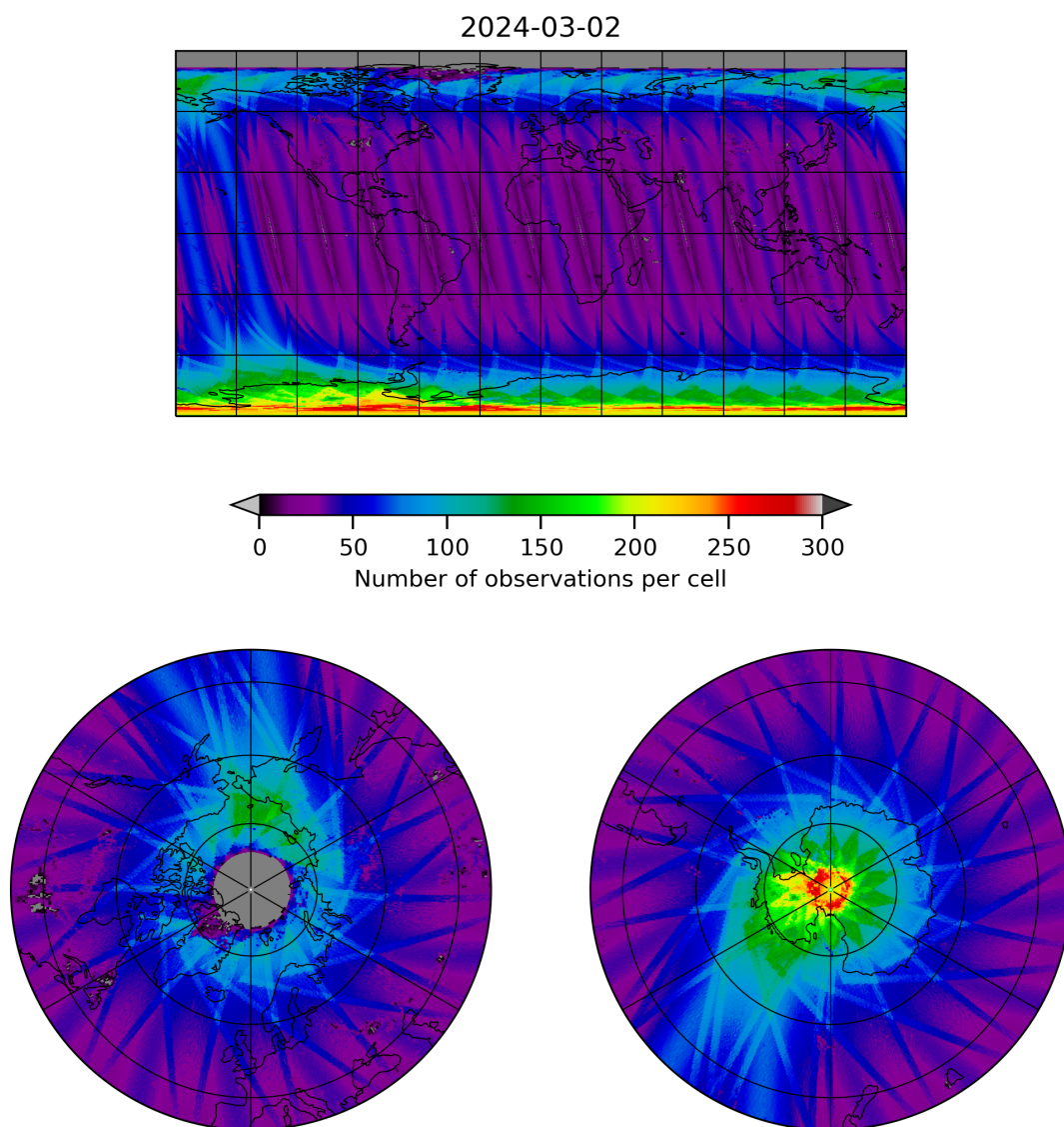
Figure 11: Map of the number of observations for 2024-03-01 to 2024-03-03
