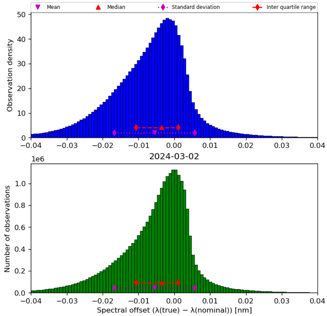
Figure 45: Histogram of “Spectral offset ( \lambda(\text{true}) - \lambda(\text{nominal}) )” for 2024-03-01 to 2024-03-03
