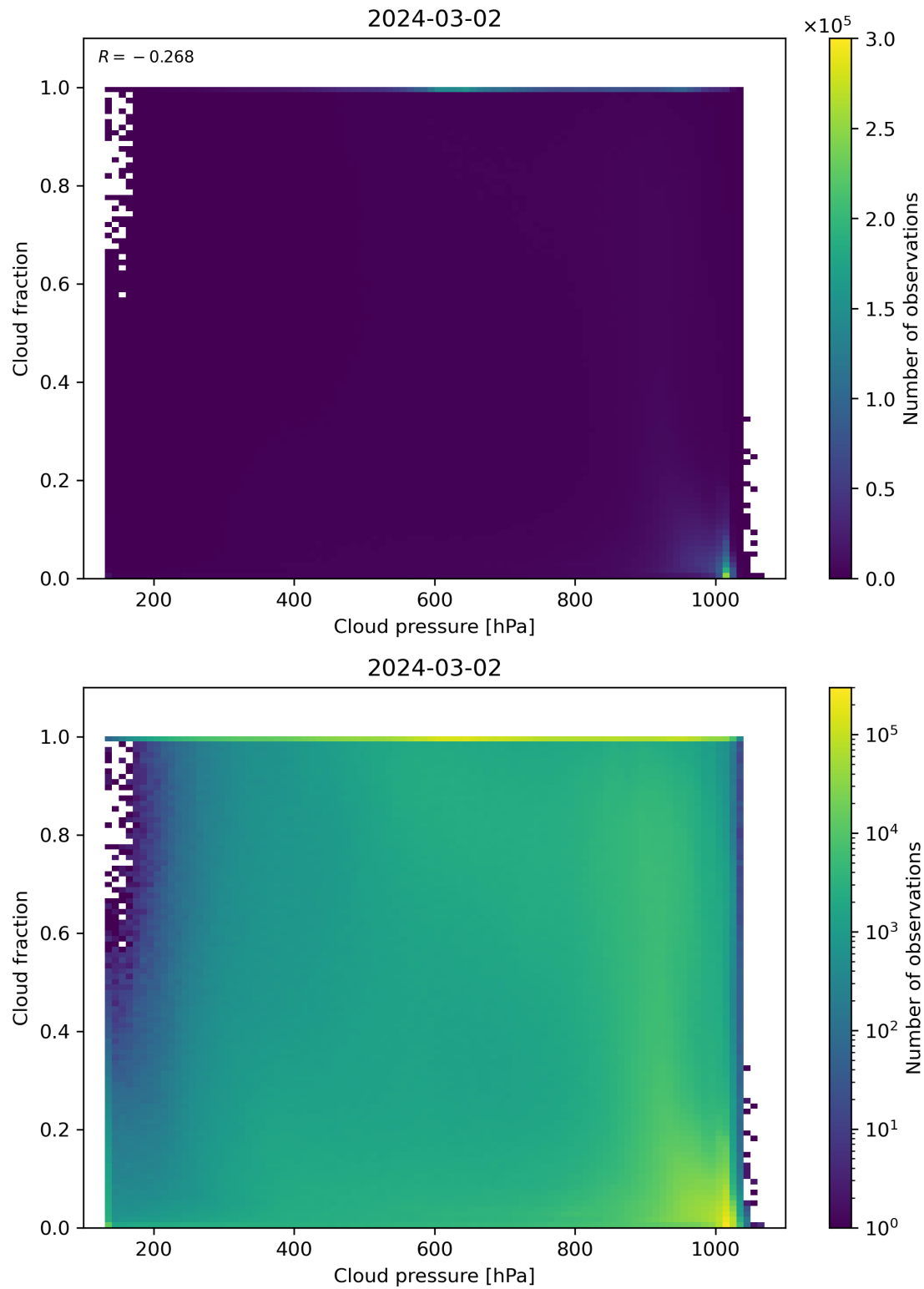
Figure 79: Scatter density plot of “Cloud pressure” against “Cloud fraction” for 2024-03-01 to 2024-03-03.
