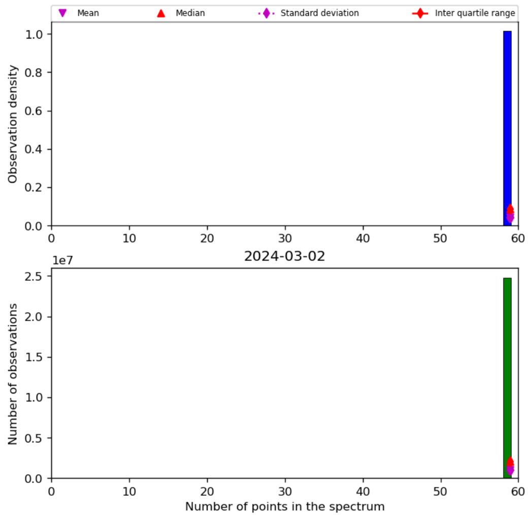
Figure 44: Histogram of “Number of points in the spectrum” for 2024-03-01 to 2024-03-03
