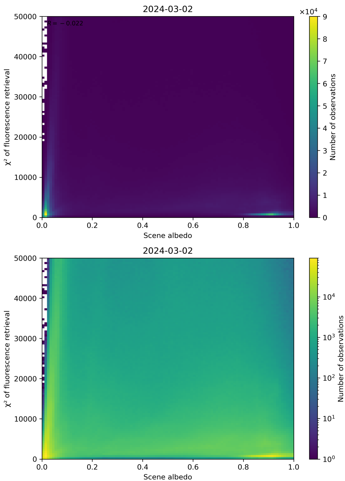
Figure 103: Scatter density plot of “Scene albedo” against “ \chi^2 of fluorescence retrieval” for 2024-03-01 to 2024-03-03.
