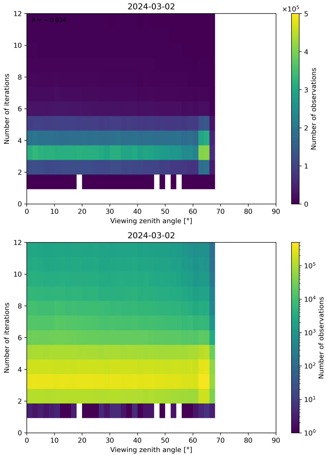
Figure 124: Scatter density plot of “Viewing zenith angle” against “Number of iterations” for 2024-03-01 to 2024-03-03.
