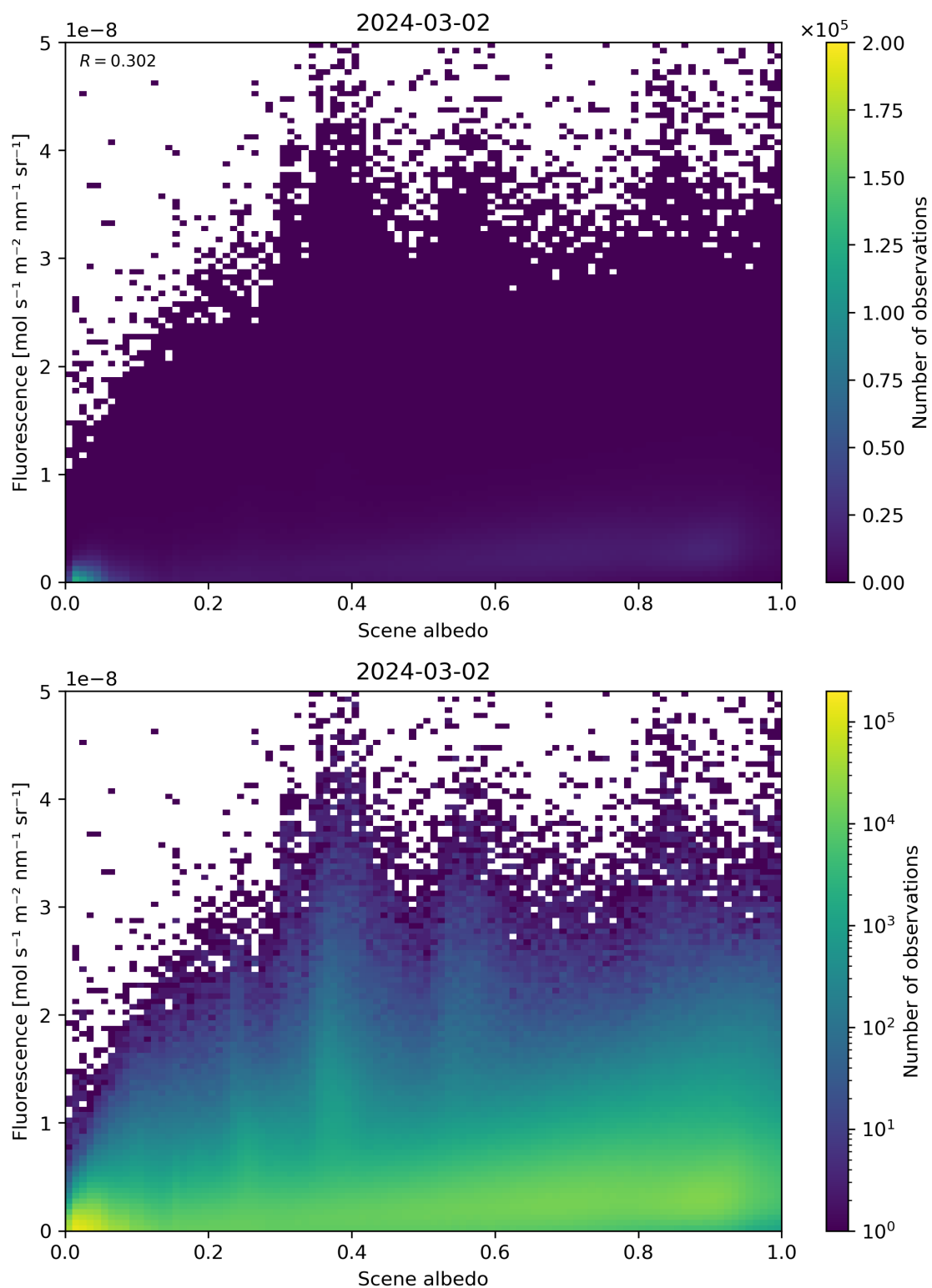
Figure 104: Scatter density plot of “Scene albedo” against “Fluorescence” for 2024-03-01 to 2024-03-03.
