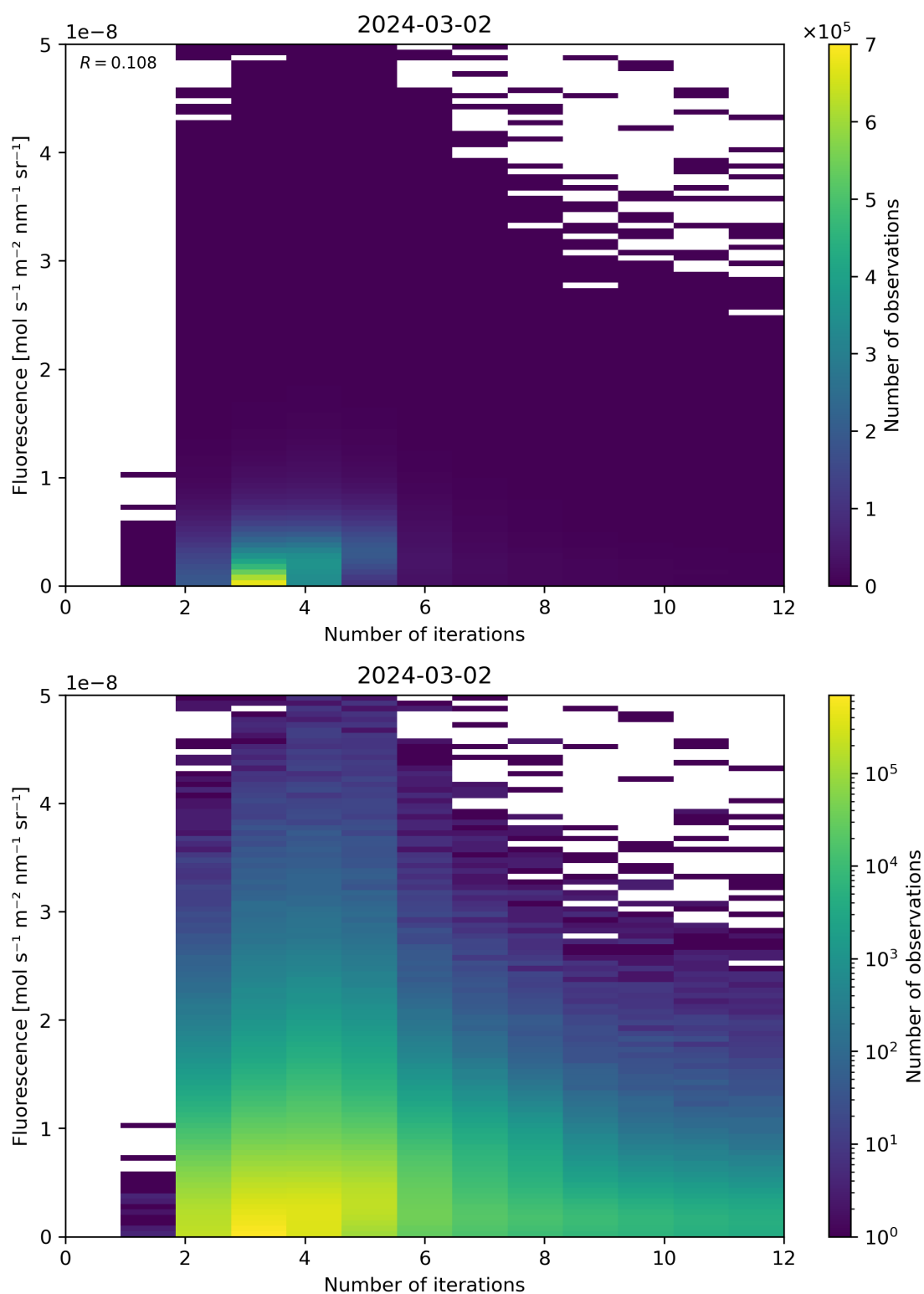
Figure 98: Scatter density plot of “Number of iterations” against “Fluorescence” for 2024-03-01 to 2024-03-03.
