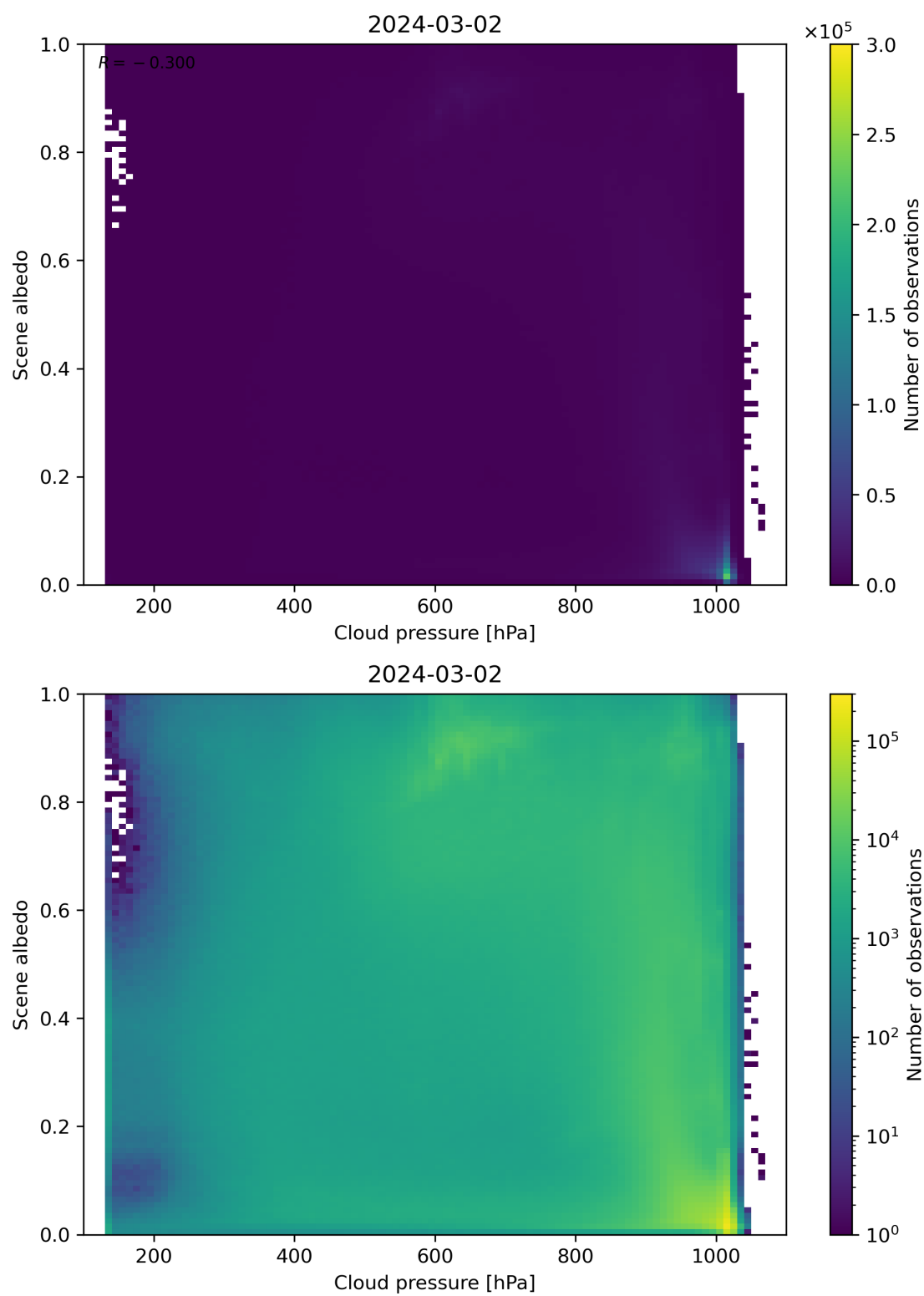
Figure 83: Scatter density plot of “Cloud pressure” against “Scene albedo” for 2024-03-01 to 2024-03-03.
