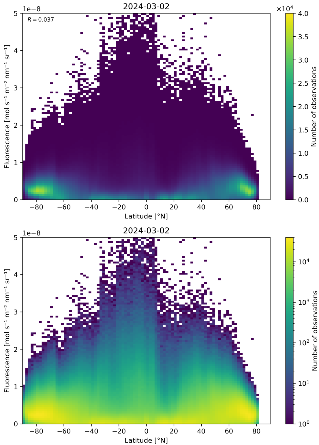
Figure 92: Scatter density plot of “Latitude” against “Fluorescence” for 2024-03-01 to 2024-03-03.
