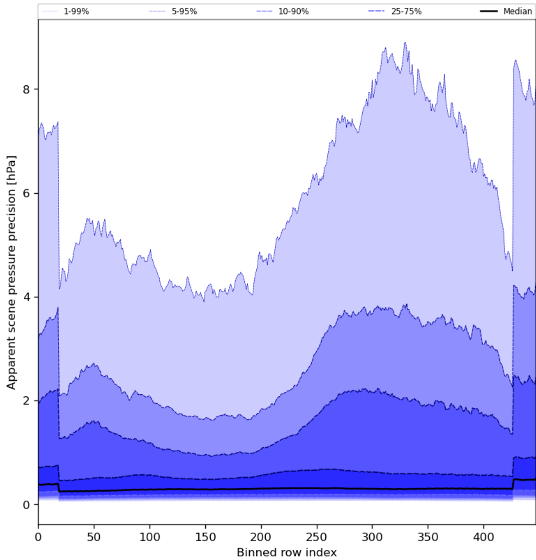
Figure 54: Along track statistics of “Apparent scene pressure precision” for 2024-03-01 to 2024-03-03
