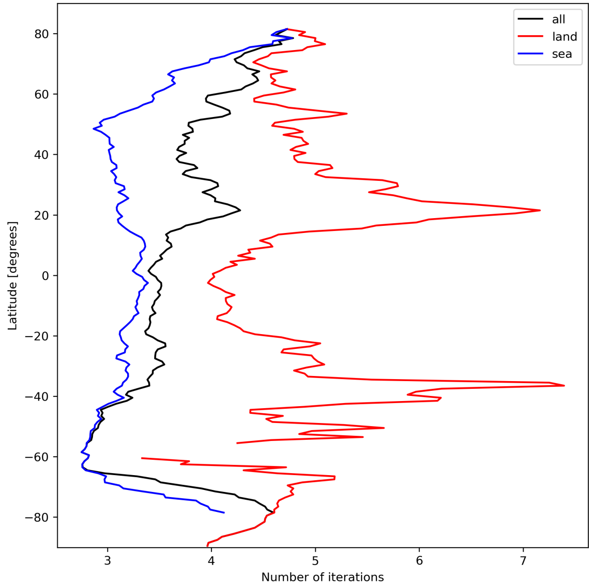
Figure 22: Zonal average of “Number of iterations” for 2024-03-01 to 2024-03-03.
