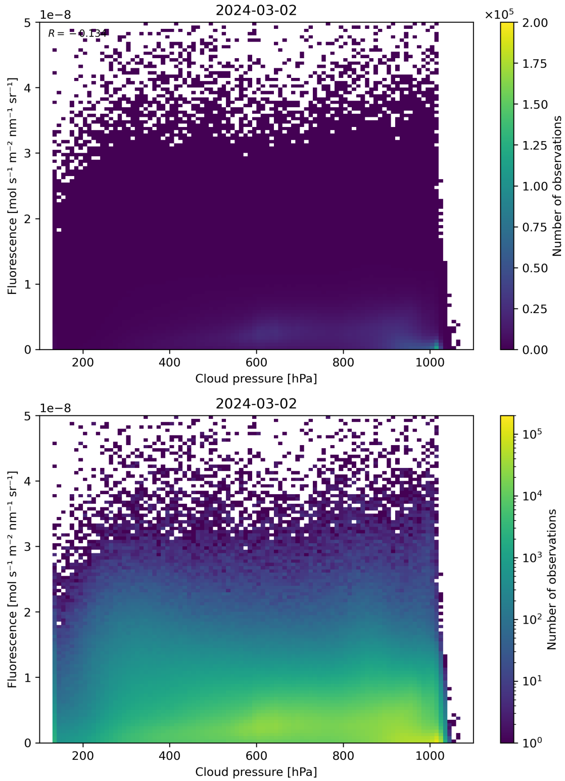
Figure 80: Scatter density plot of “Cloud pressure” against “Fluorescence” for 2024-03-01 to 2024-03-03.
