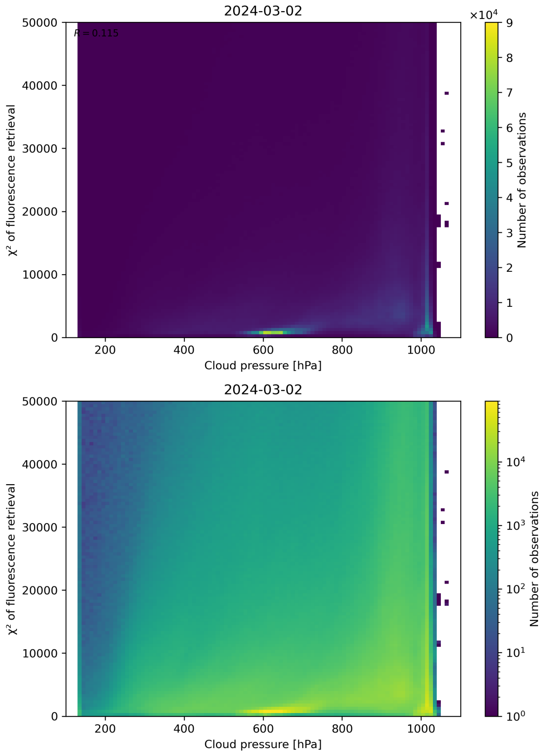
Figure 78: Scatter density plot of “Cloud pressure” against “ \chi^2 of fluorescence retrieval” for 2024-03-01 to 2024-03-03.
