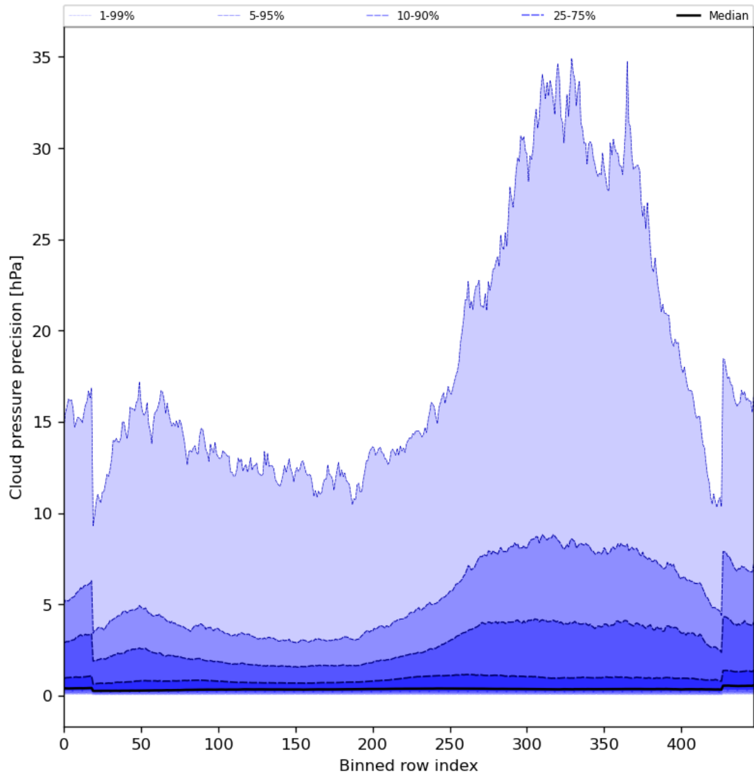
Figure 48: Along track statistics of “Cloud pressure precision” for 2024-03-01 to 2024-03-03
