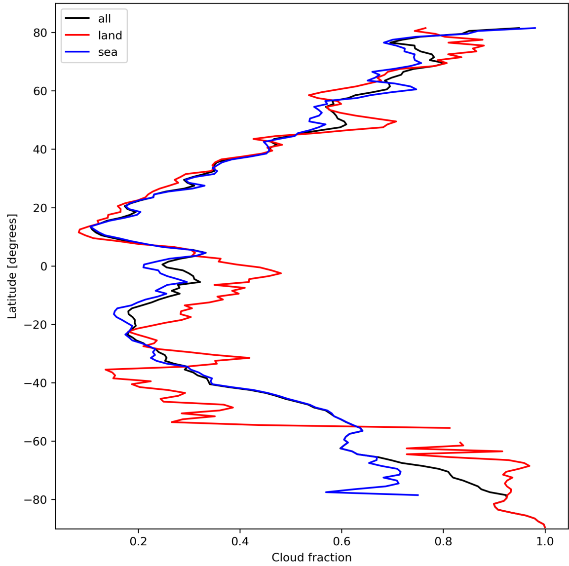
Figure 15: Zonal average of “Cloud fraction” for 2024-03-01 to 2024-03-03.
