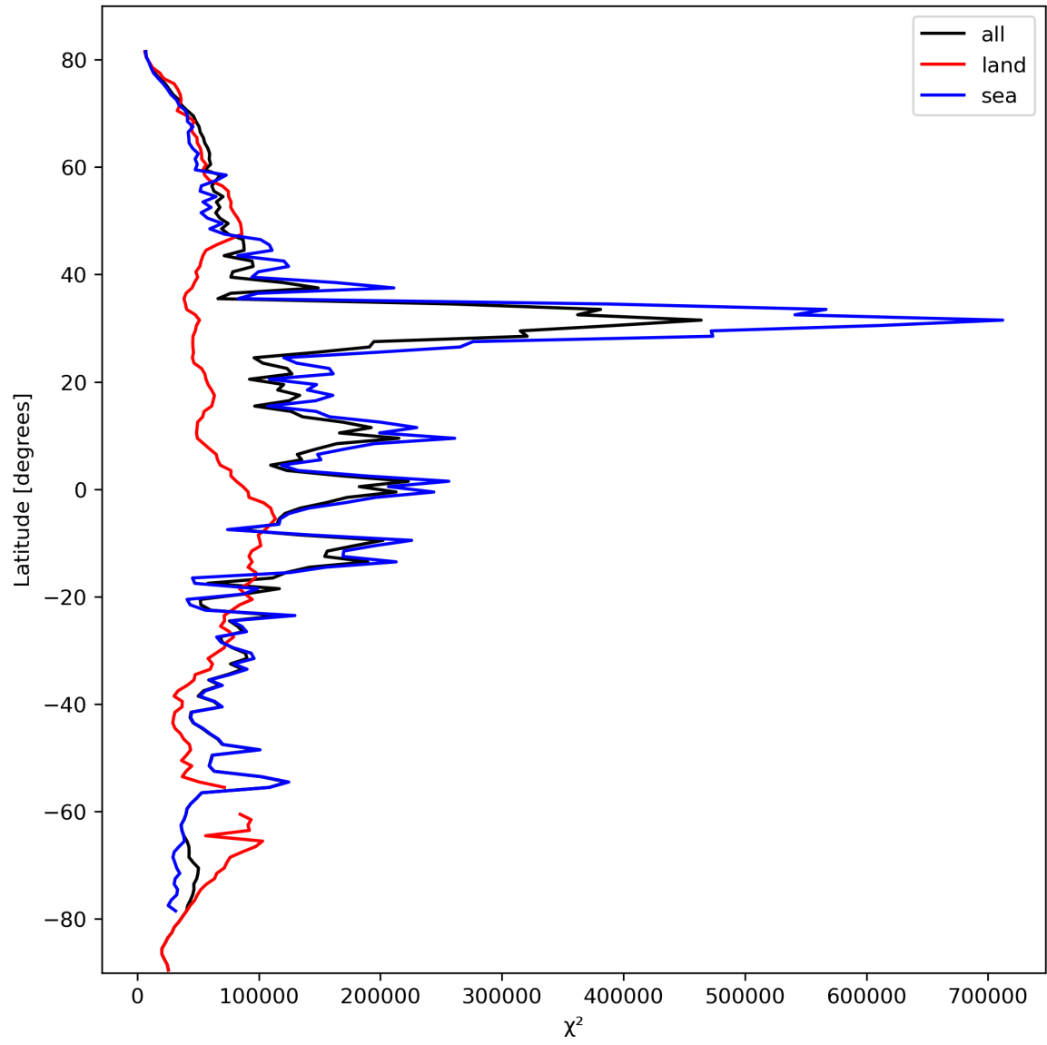
Figure 21: Zonal average of “ \chi^2 ” for 2024-03-01 to 2024-03-03.
