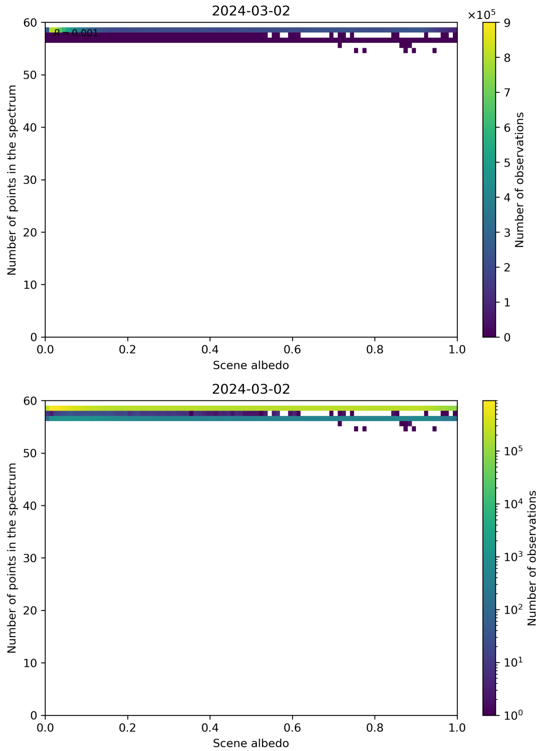
Figure 106: Scatter density plot of “Scene albedo” against “Number of points in the spectrum” for 2024-03-01 to 2024-03-03.
