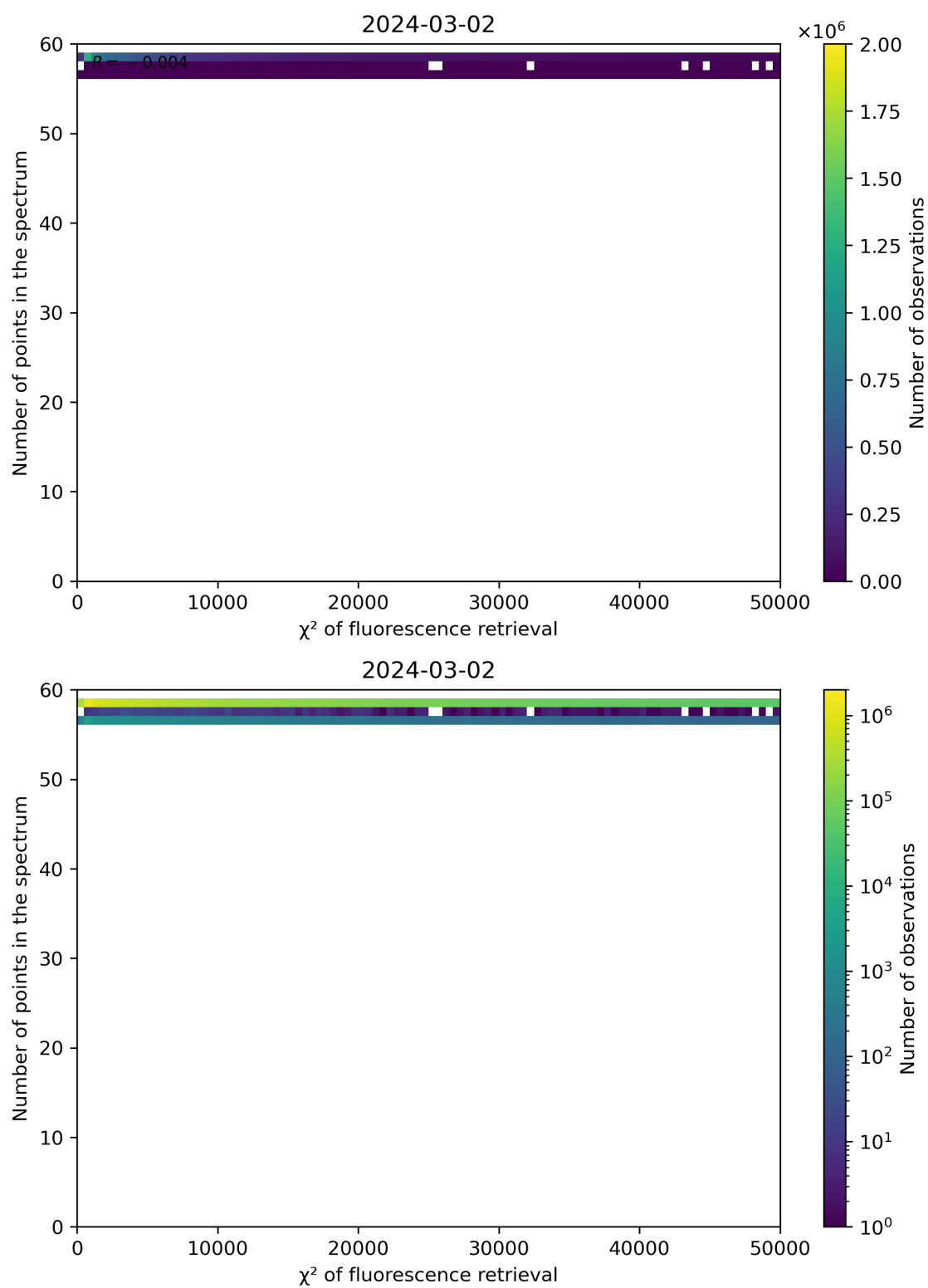
Figure 68: Scatter density plot of " \chi^2 of fluorescence retrieval" against "Number of points in the spectrum" for 2024-03-01 to 2024-03-03.
