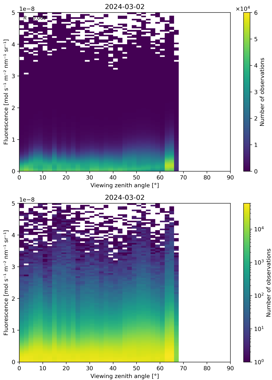
Figure 122: Scatter density plot of “Viewing zenith angle” against “Fluorescence” for 2024-03-01 to 2024-03-03.
