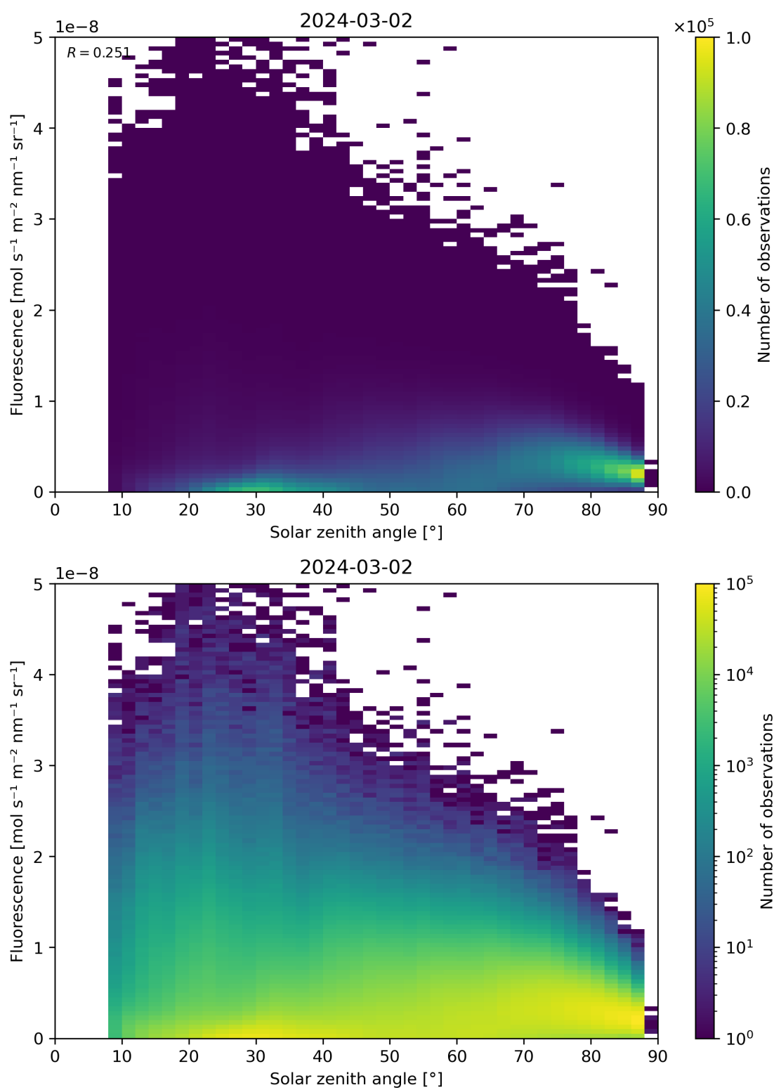
Figure 112: Scatter density plot of “Solar zenith angle” against “Fluorescence” for 2024-03-01 to 2024-03-03.
