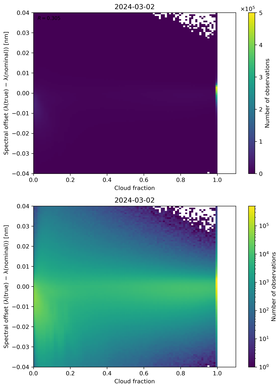
Figure 76: Scatter density plot of “Cloud fraction” against “Spectral offset ( \lambda(\text{true}) - \lambda(\text{nominal}) )” for 2024-03-01 to 2024-03-03.
