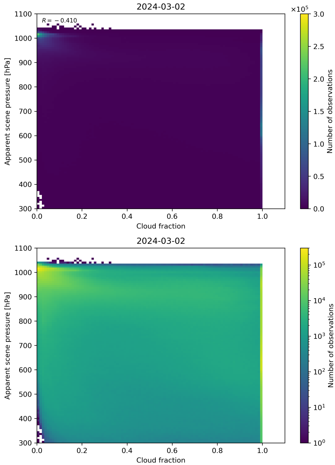
Figure 70: Scatter density plot of “Cloud fraction” against “Apparent scene pressure” for 2024-03-01 to 2024-03-03.
