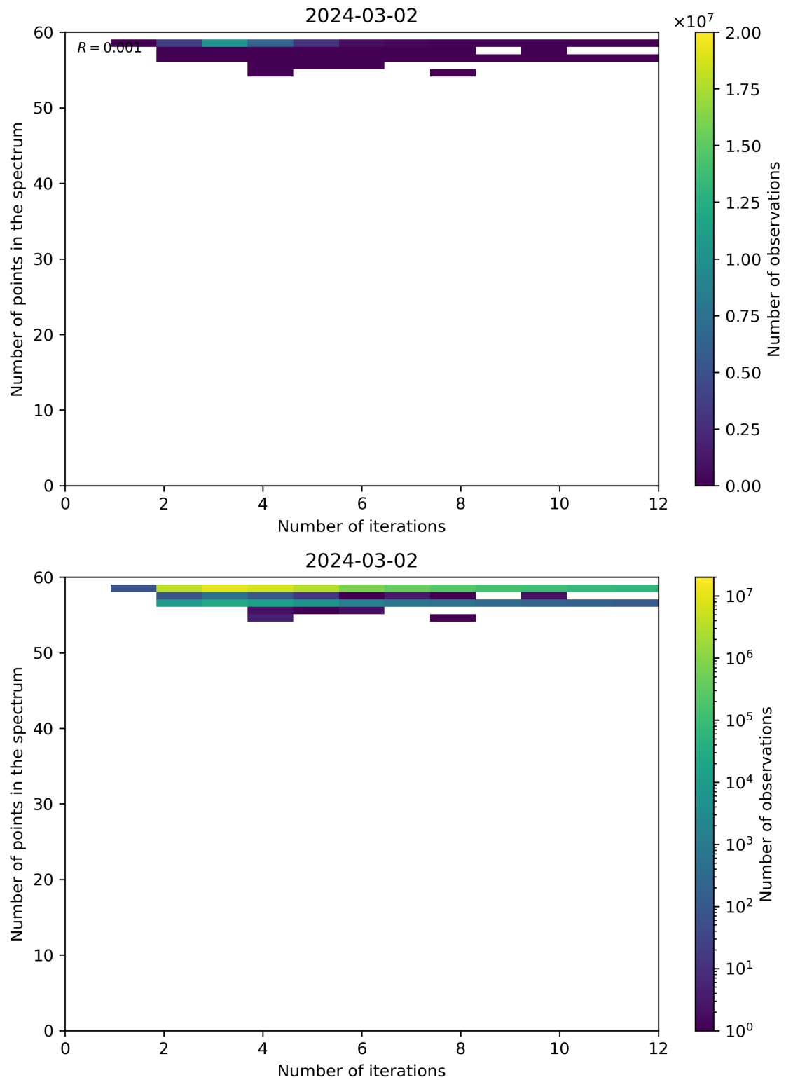
Figure 99: Scatter density plot of “Number of iterations” against “Number of points in the spectrum” for 2024-03-01 to 2024-03-03.
