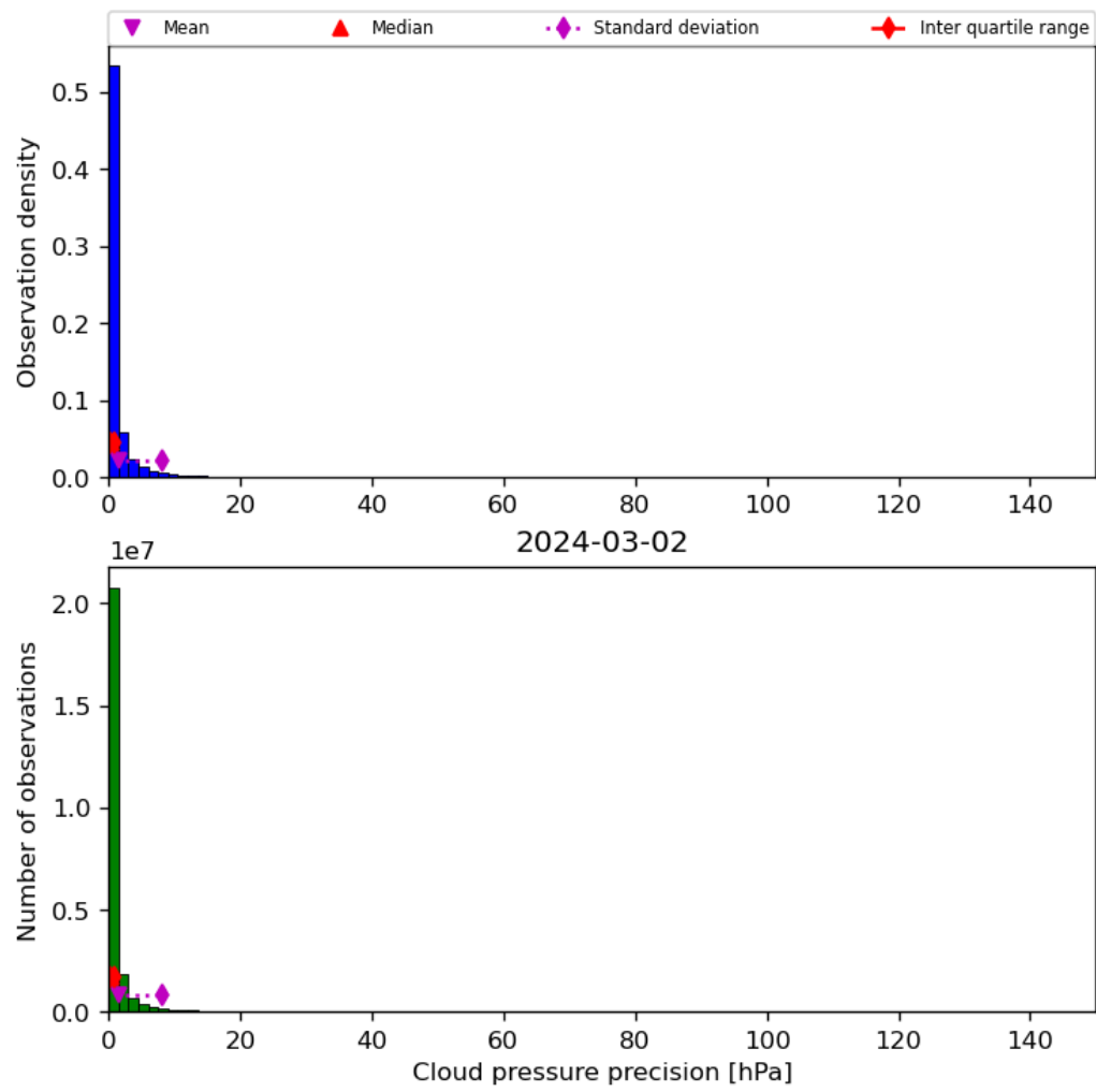
Figure 31: Histogram of “Cloud pressure precision” for 2024-03-01 to 2024-03-03
