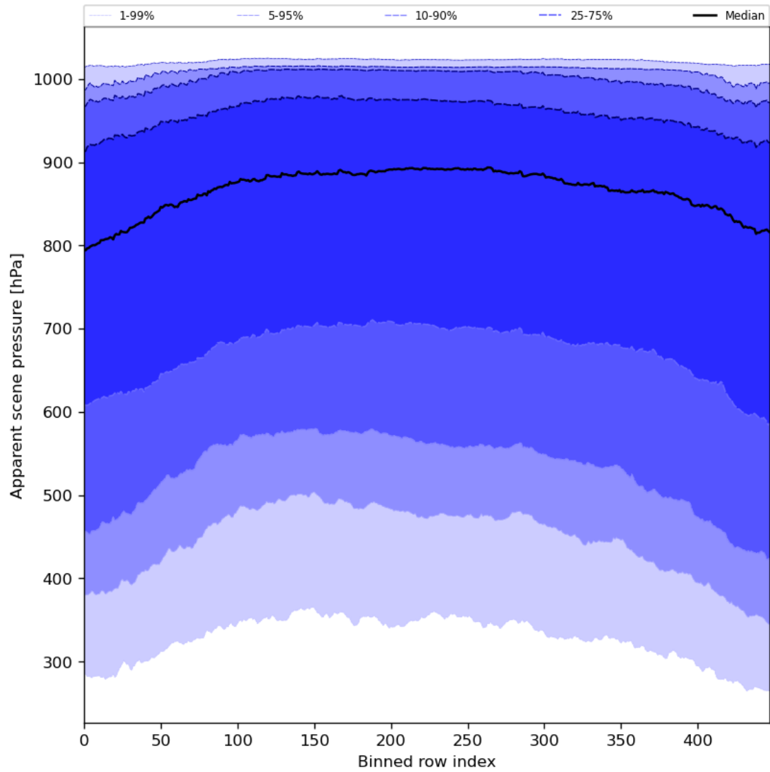
Figure 53: Along track statistics of “Apparent scene pressure” for 2024-03-01 to 2024-03-03
