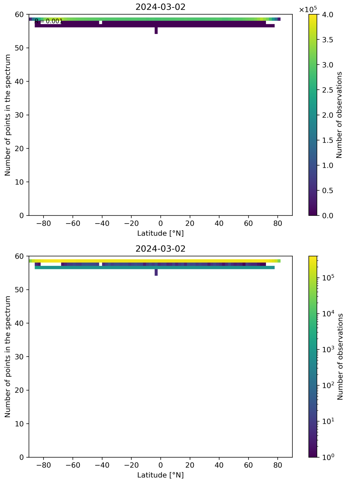
Figure 94: Scatter density plot of “Latitude” against “Number of points in the spectrum” for 2024-03-01 to 2024-03-03.
