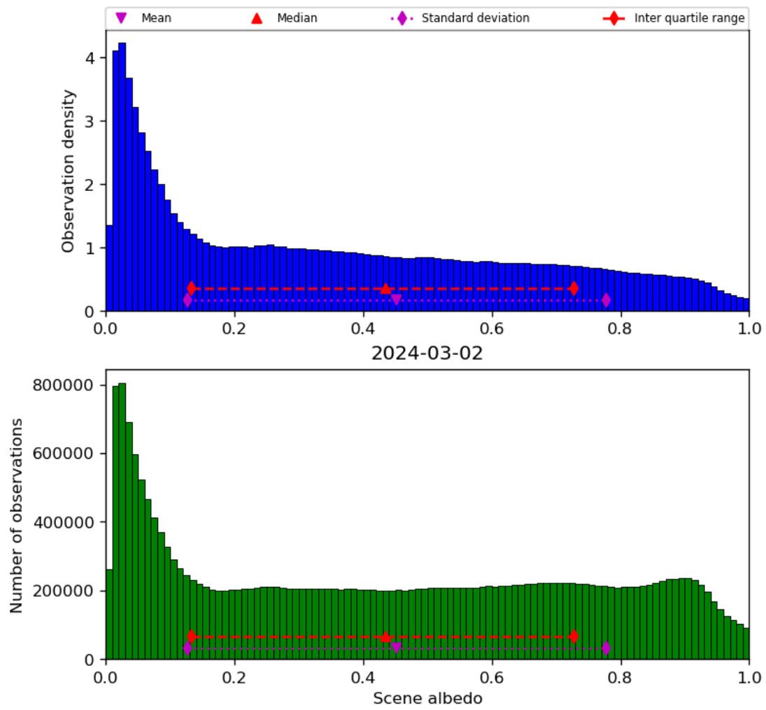
Figure 34: Histogram of “Scene albedo” for 2024-03-01 to 2024-03-03
