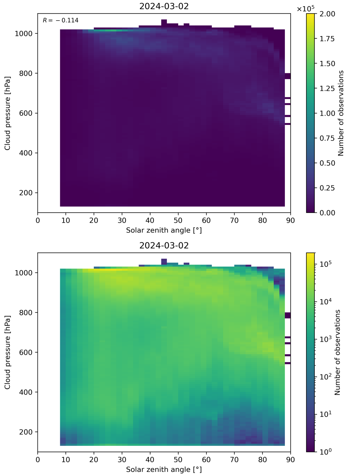
Figure 111: Scatter density plot of “Solar zenith angle” against “Cloud pressure” for 2024-03-01 to 2024-03-03.
