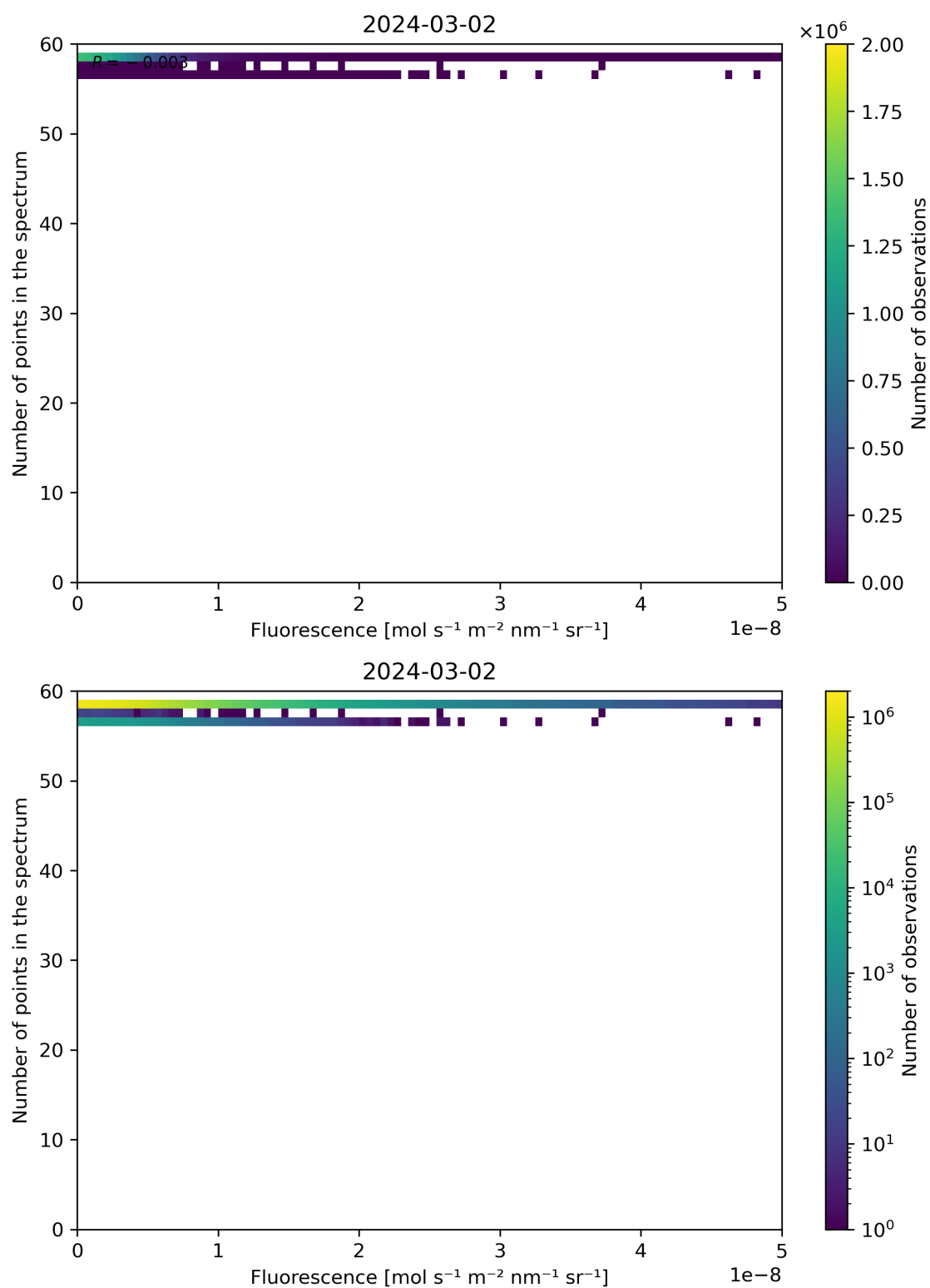
Figure 86: Scatter density plot of “Fluorescence” against “Number of points in the spectrum” for 2024-03-01 to 2024-03-03.
