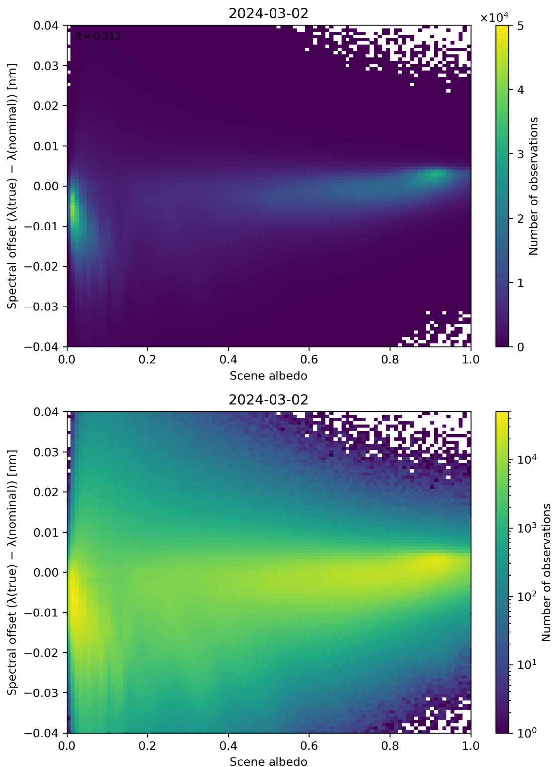
Figure 107: Scatter density plot of “Scene albedo” against “Spectral offset ( \lambda(\text{true}) - \lambda(\text{nominal}) )” for 2024-03-01 to 2024-03-03.
