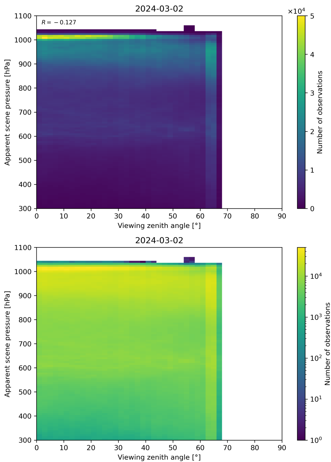
Figure 118: Scatter density plot of “Viewing zenith angle” against “Apparent scene pressure” for 2024-03-01 to 2024-03-03.
