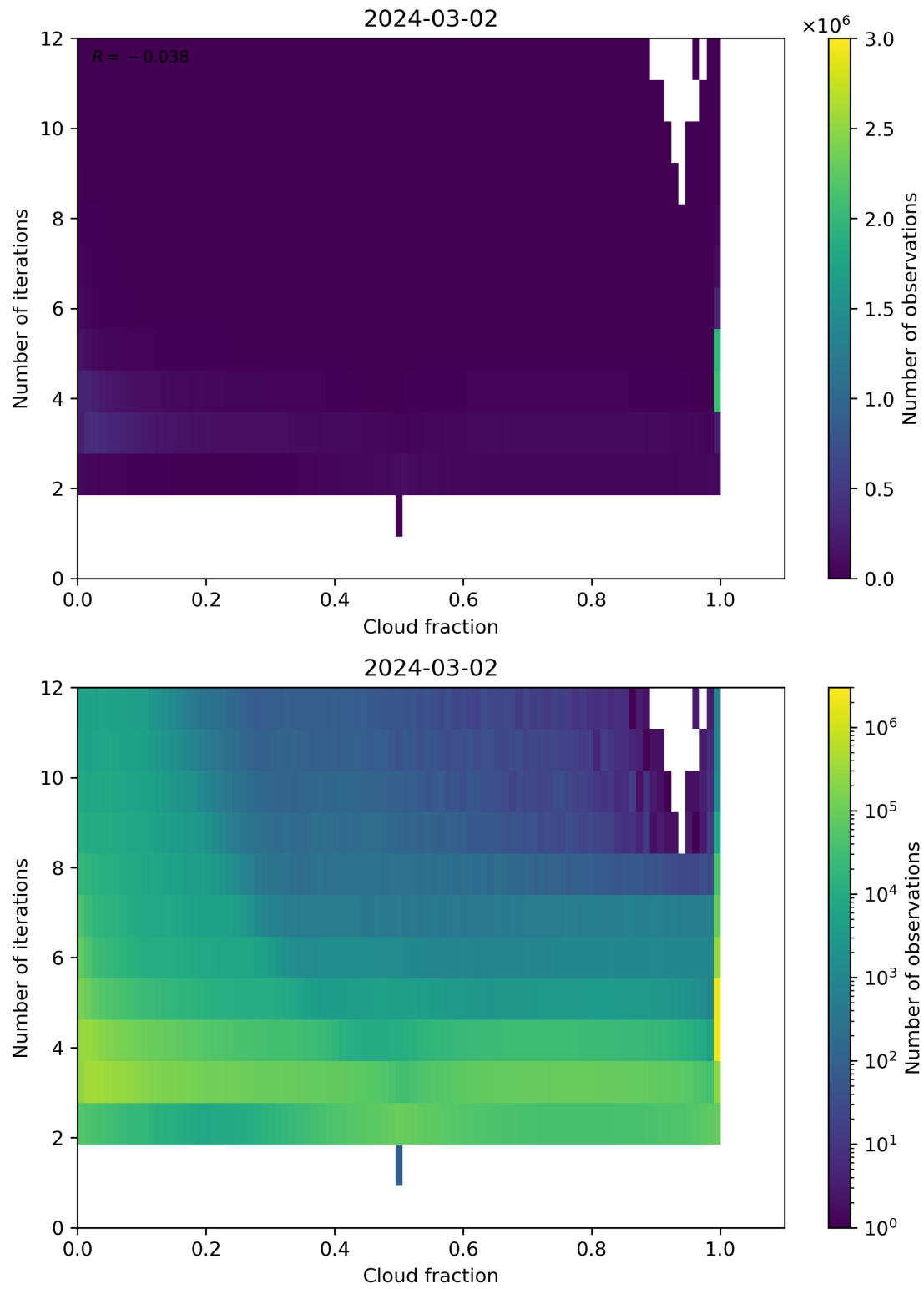
Figure 73: Scatter density plot of “Cloud fraction” against “Number of iterations” for 2024-03-01 to 2024-03-03.
