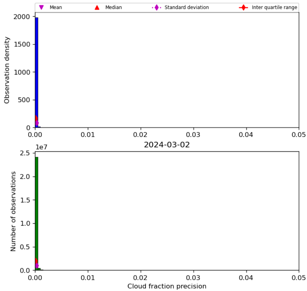
Figure 33: Histogram of “Cloud fraction precision” for 2024-03-01 to 2024-03-03
