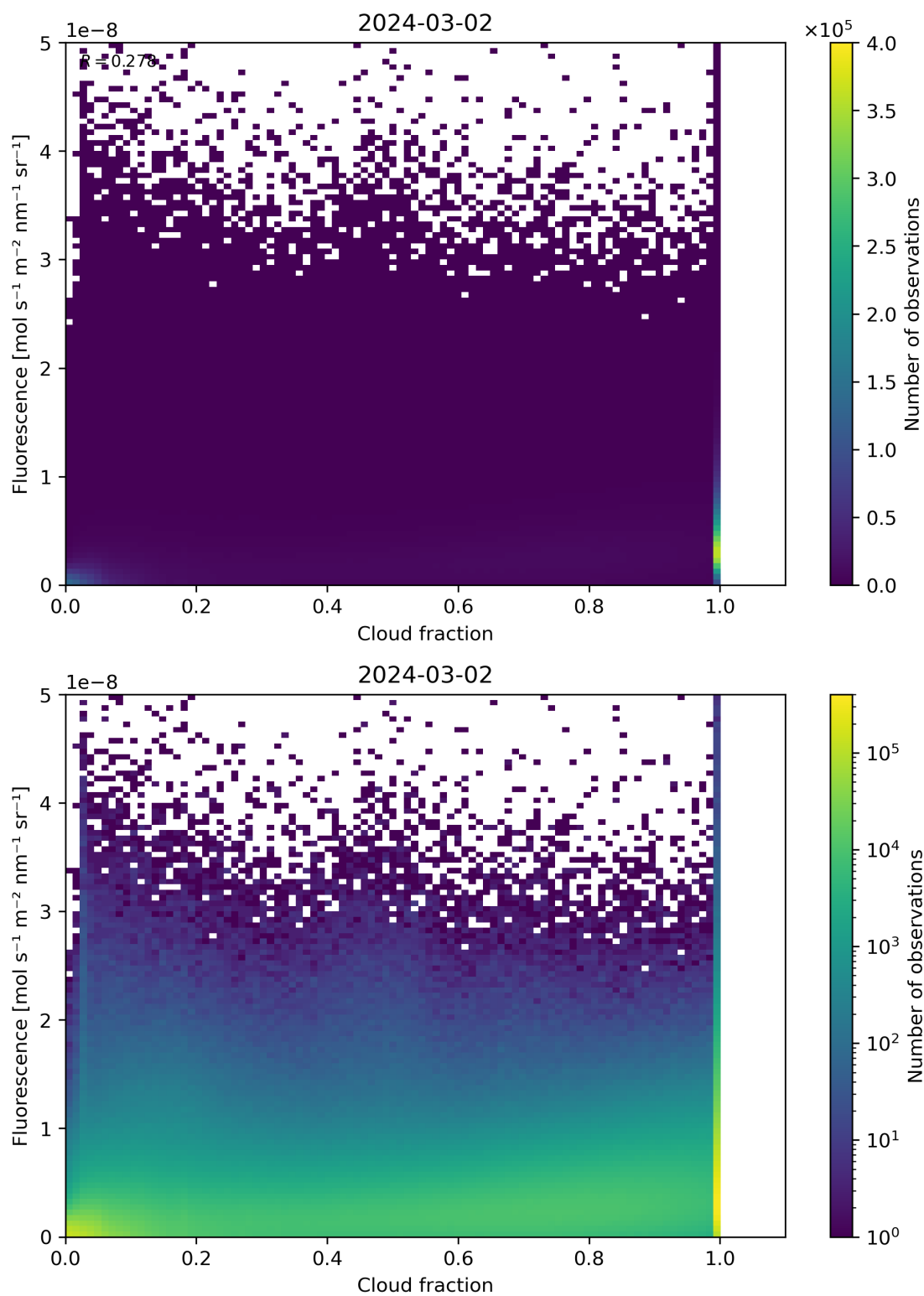
Figure 72: Scatter density plot of “Cloud fraction” against “Fluorescence” for 2024-03-01 to 2024-03-03.
