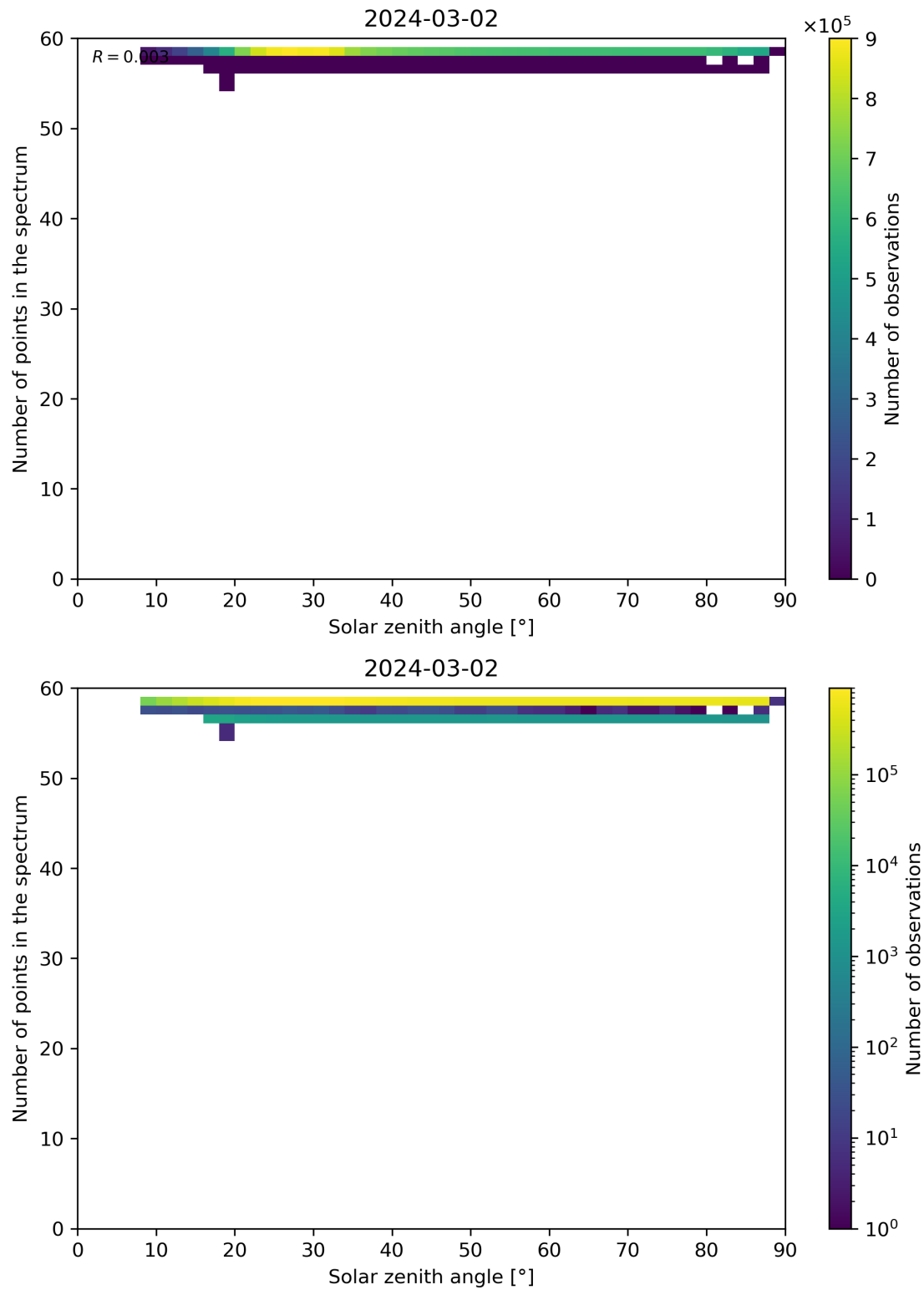
Figure 115: Scatter density plot of “Solar zenith angle” against “Number of points in the spectrum” for 2024-03-01 to 2024-03-03.
