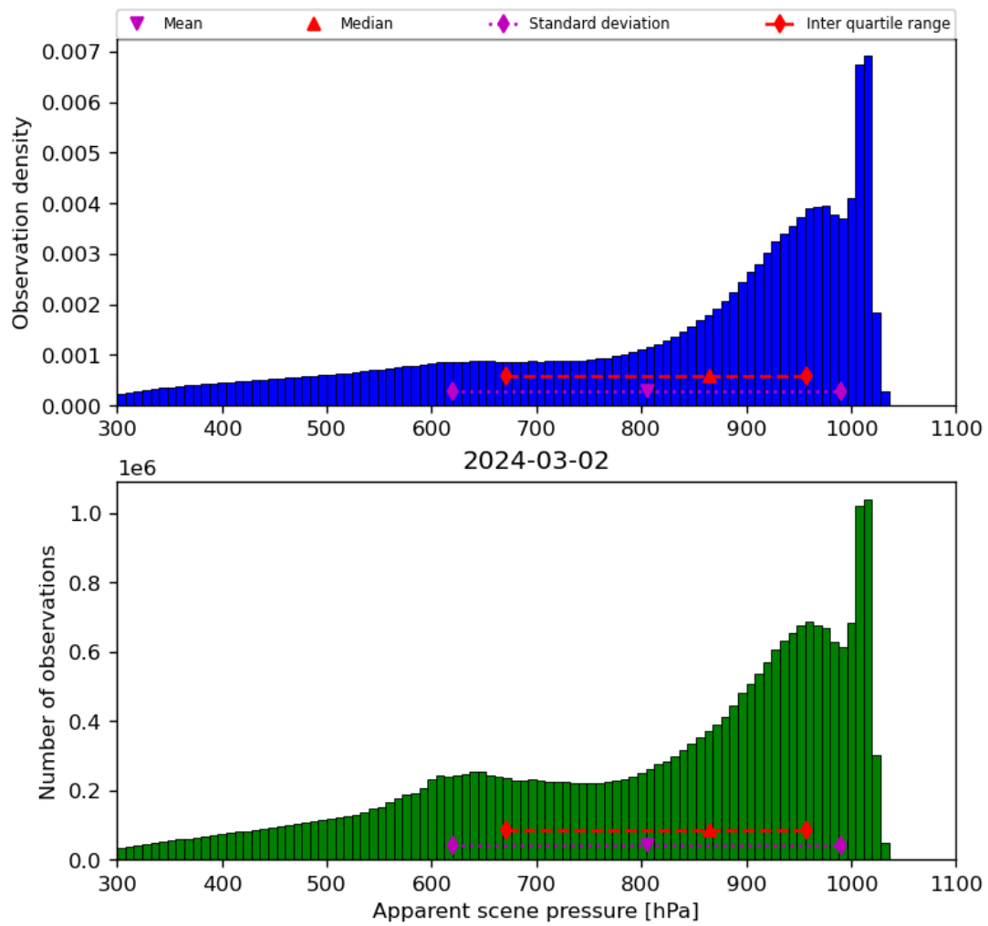
Figure 36: Histogram of “Apparent scene pressure” for 2024-03-01 to 2024-03-03
