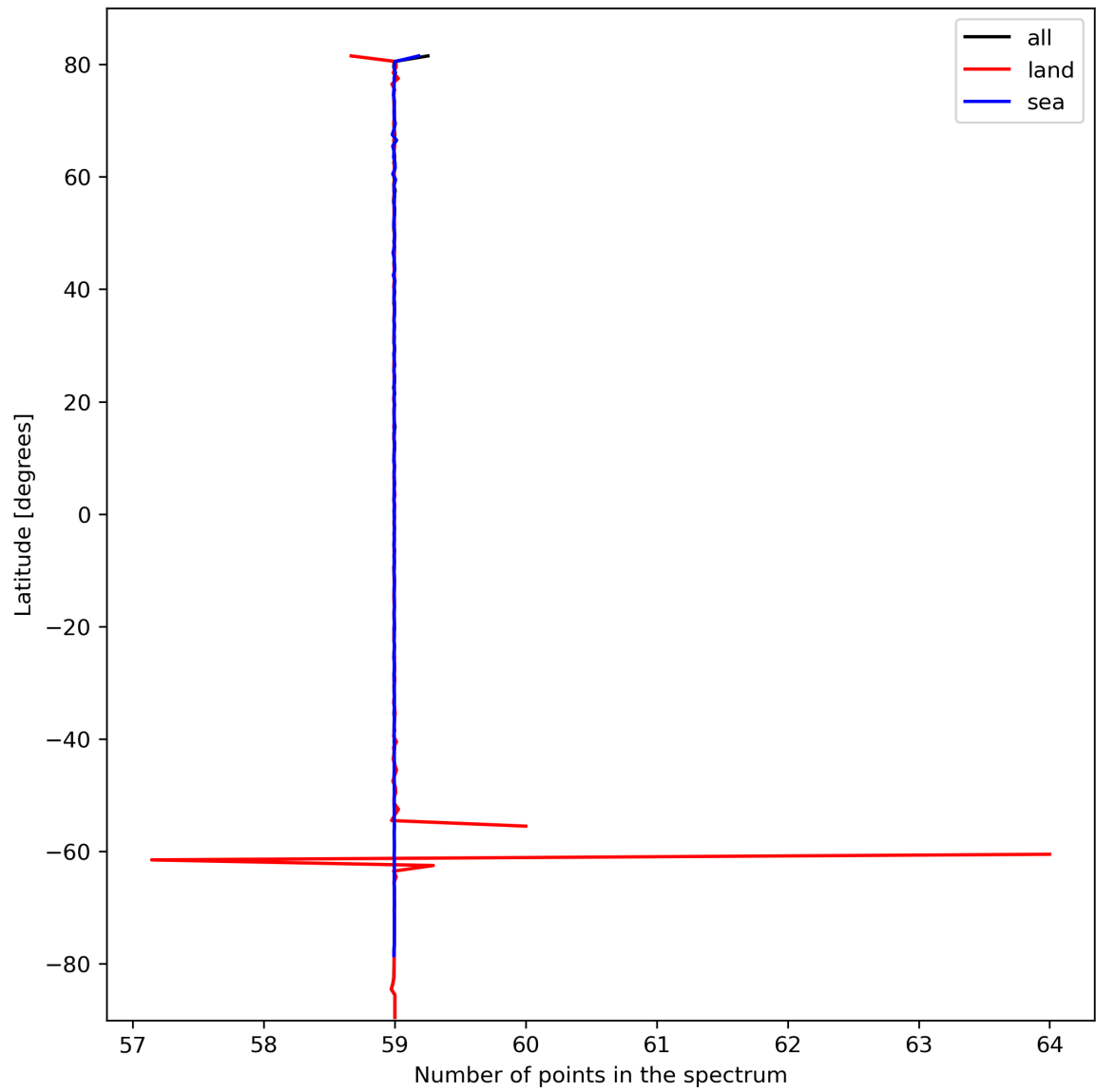
Figure 27: Zonal average of “Number of points in the spectrum” for 2024-03-01 to 2024-03-03.
