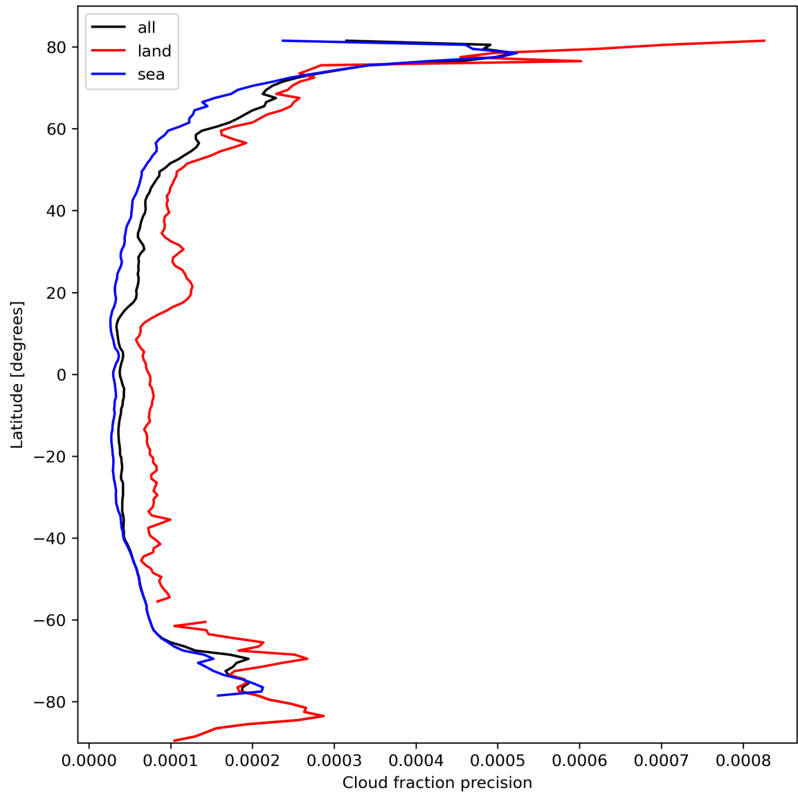
Figure 16: Zonal average of “Cloud fraction precision” for 2024-03-01 to 2024-03-03.
