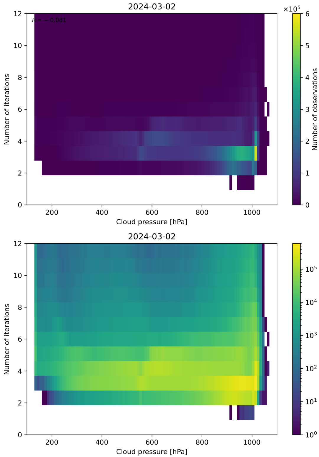
Figure 81: Scatter density plot of “Cloud pressure” against “Number of iterations” for 2024-03-01 to 2024-03-03.
