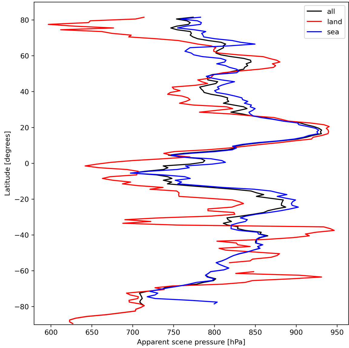
Figure 19: Zonal average of “Apparent scene pressure” for 2024-03-01 to 2024-03-03.
