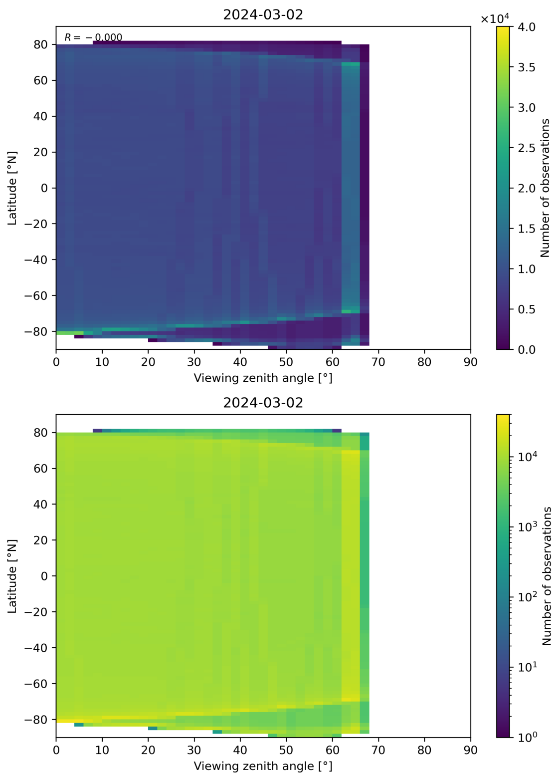
Figure 123: Scatter density plot of “Viewing zenith angle” against “Latitude” for 2024-03-01 to 2024-03-03.
