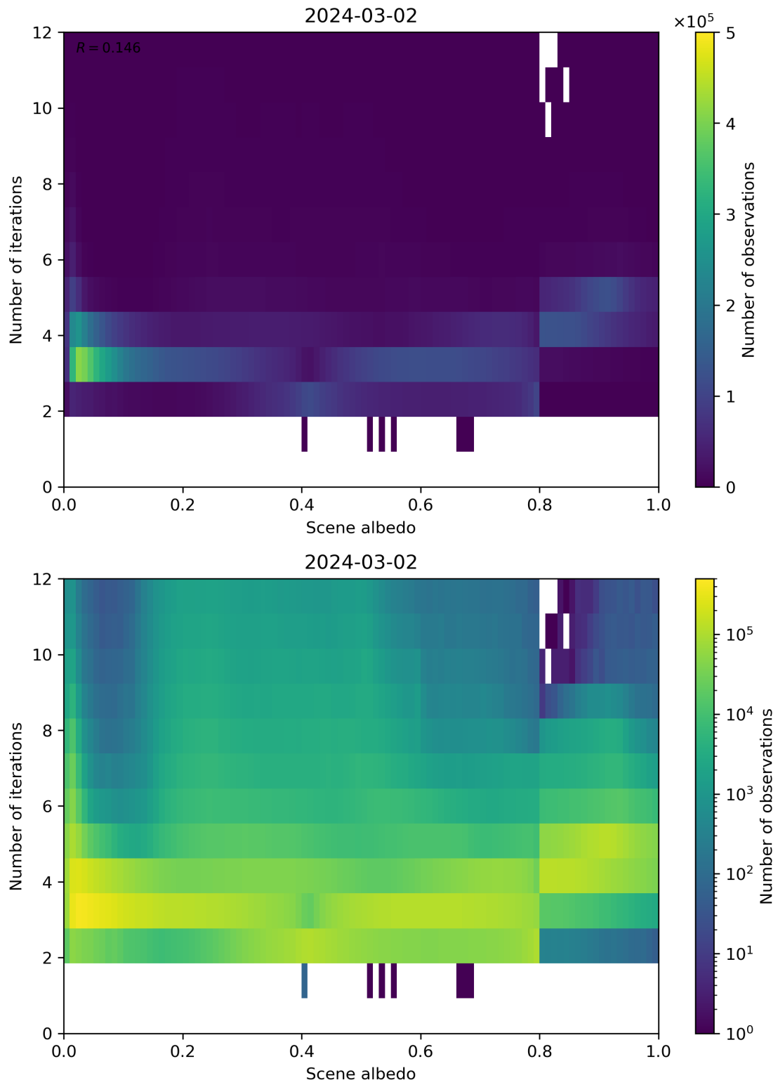
Figure 105: Scatter density plot of “Scene albedo” against “Number of iterations” for 2024-03-01 to 2024-03-03.
