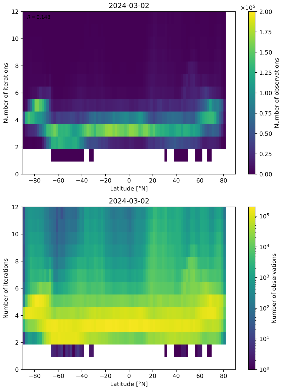
Figure 93: Scatter density plot of “Latitude” against “Number of iterations” for 2024-03-01 to 2024-03-03.
