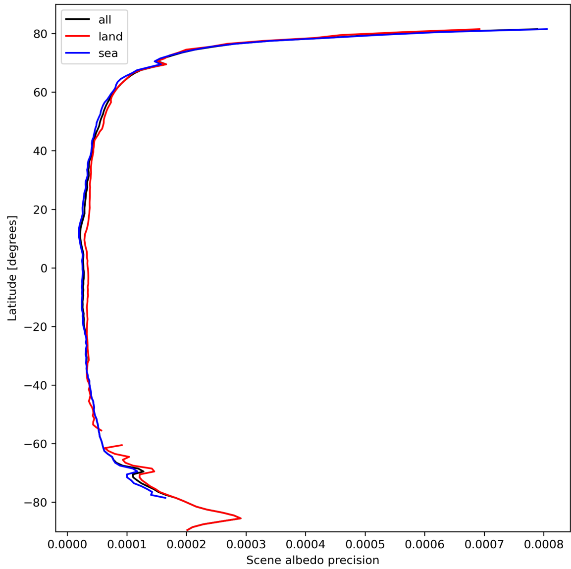
Figure 18: Zonal average of “Scene albedo precision” for 2024-03-01 to 2024-03-03.
