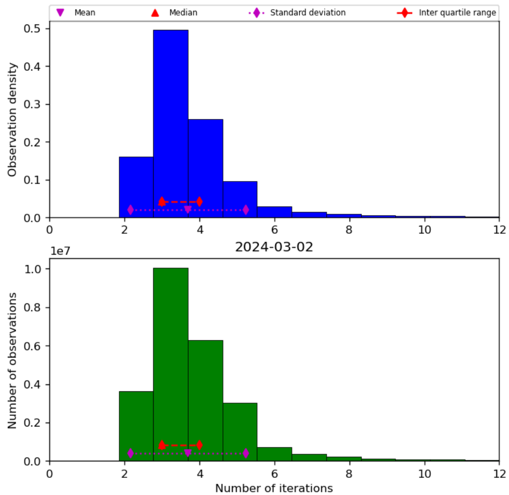
Figure 39: Histogram of “Number of iterations” for 2024-03-01 to 2024-03-03
