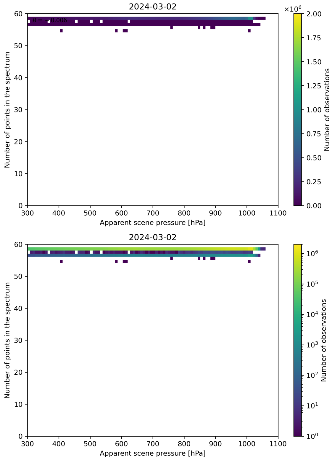
Figure 66: Scatter density plot of “Apparent scene pressure” against “Number of points in the spectrum” for 2024-03-01 to 2024-03-03.
