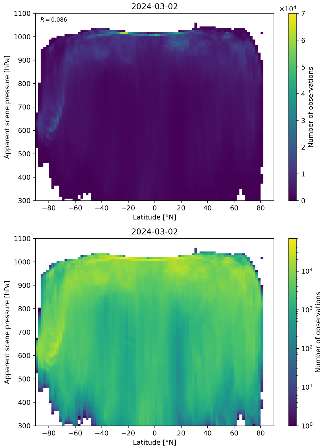
Figure 88: Scatter density plot of “Latitude” against “Apparent scene pressure” for 2024-03-01 to 2024-03-03.
