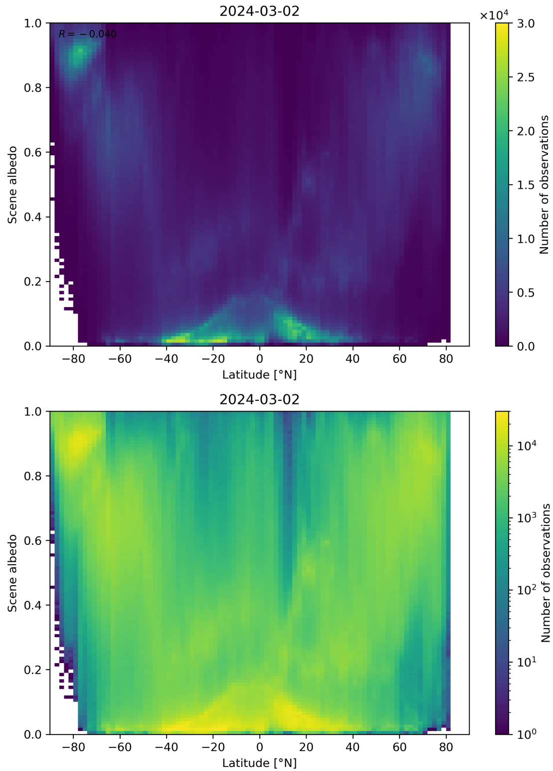
Figure 95: Scatter density plot of “Latitude” against “Scene albedo” for 2024-03-01 to 2024-03-03.
