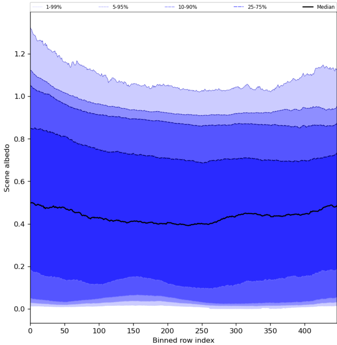
Figure 51: Along track statistics of “Scene albedo” for 2024-03-01 to 2024-03-03
