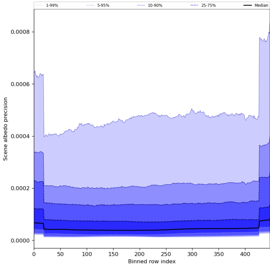
Figure 52: Along track statistics of “Scene albedo precision” for 2024-03-01 to 2024-03-03
