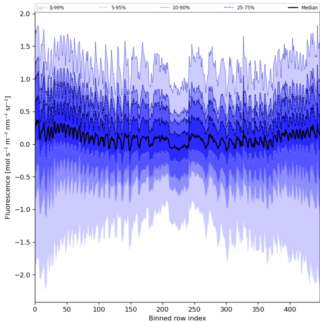
Figure 57: Along track statistics of "Fluorescence" for 2024-03-01 to 2024-03-03
