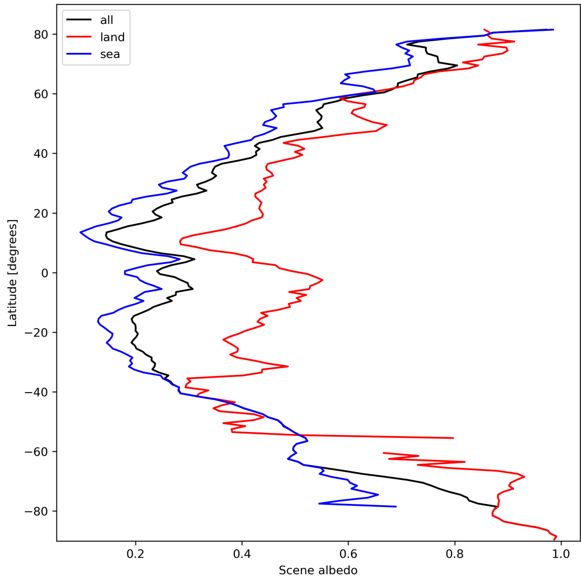
Figure 17: Zonal average of “Scene albedo” for 2024-03-01 to 2024-03-03.
