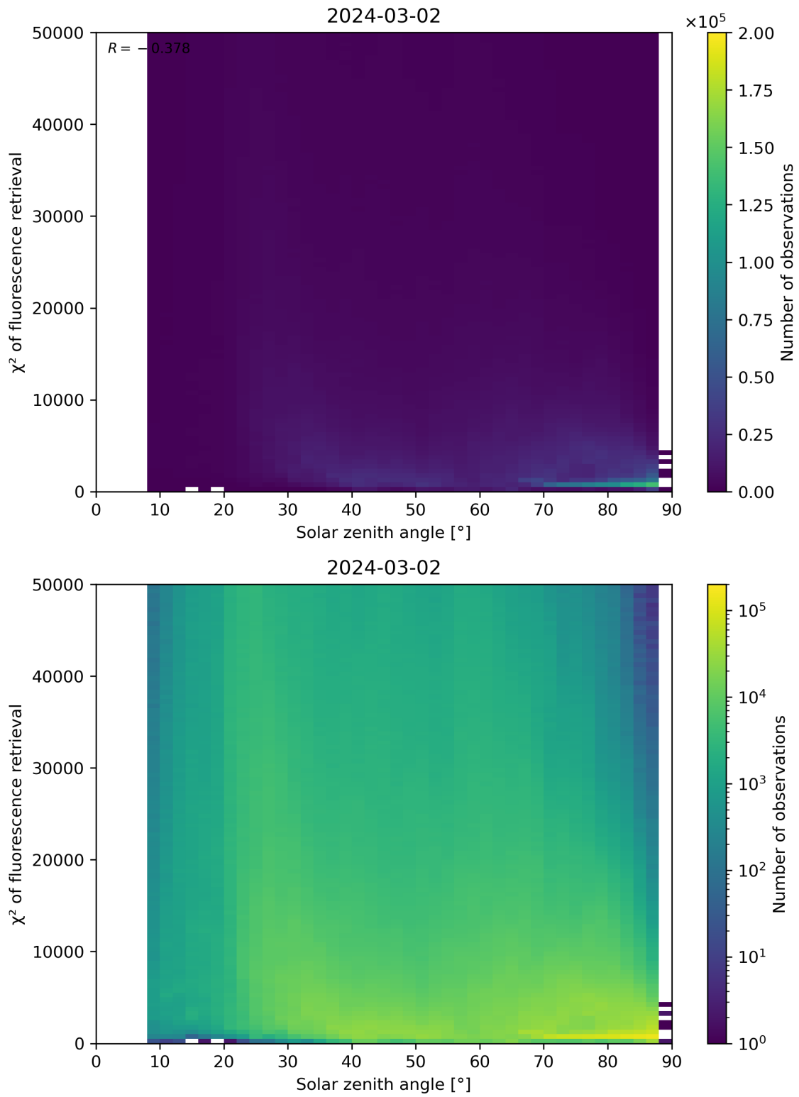
Figure 109: Scatter density plot of “Solar zenith angle” against “ \chi^2 of fluorescence retrieval” for 2024-03-01 to 2024-03-03.
