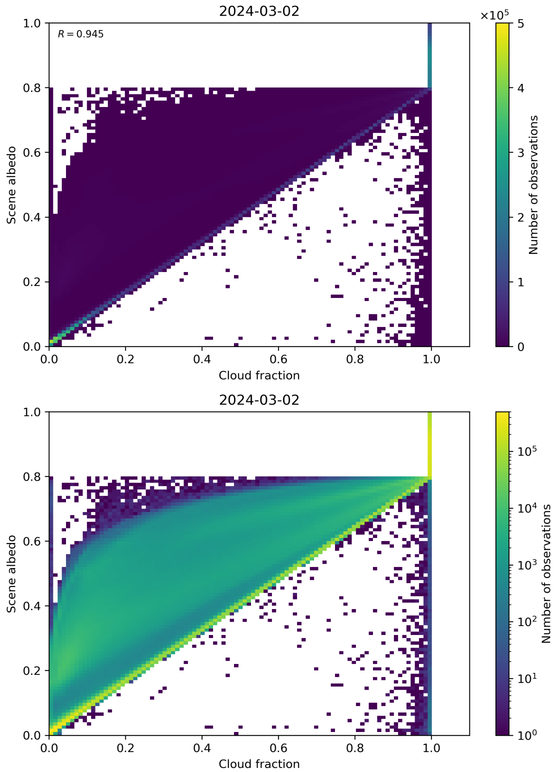
Figure 75: Scatter density plot of “Cloud fraction” against “Scene albedo” for 2024-03-01 to 2024-03-03.
