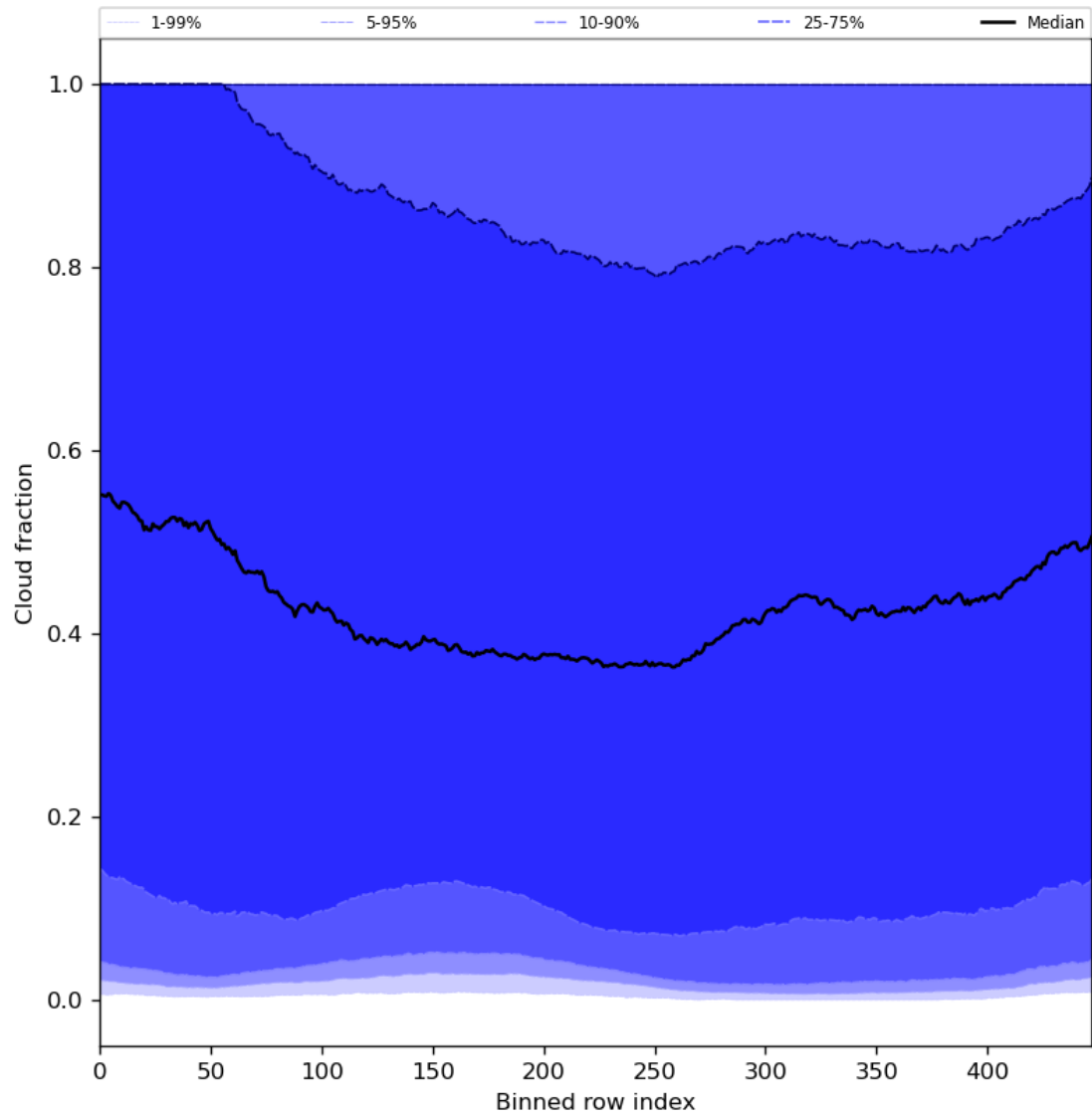
Figure 49: Along track statistics of “Cloud fraction” for 2024-03-01 to 2024-03-03
