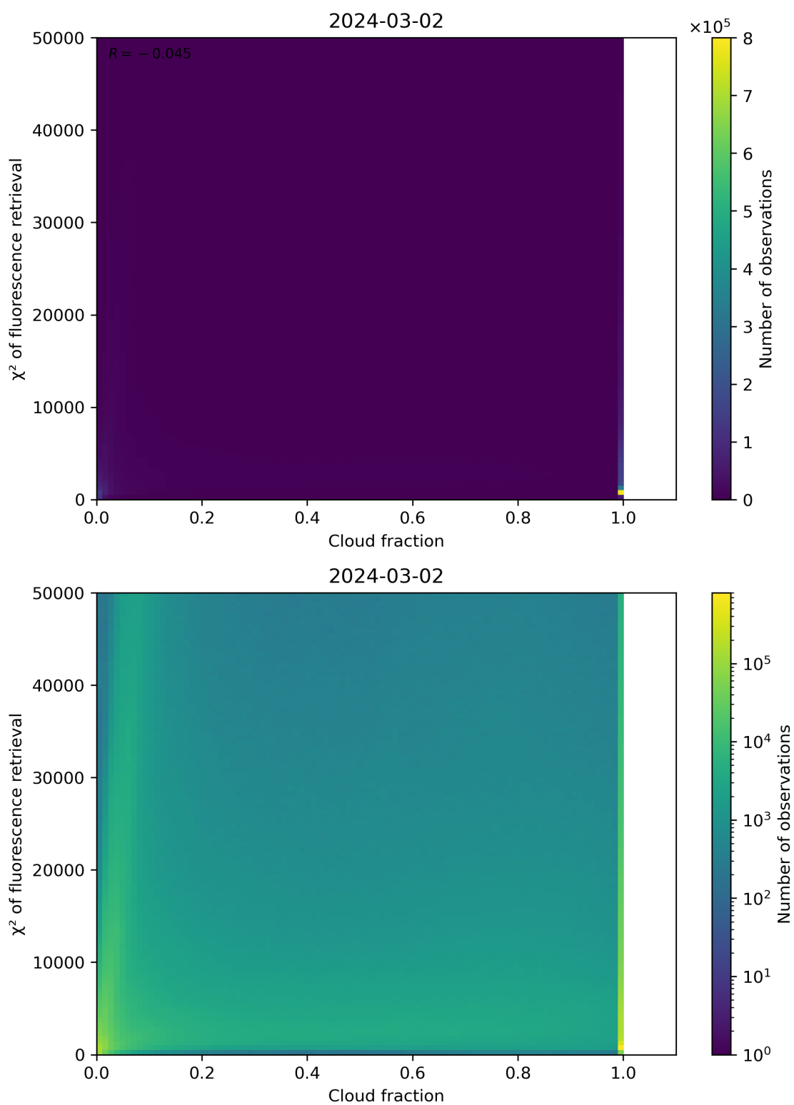
Figure 71: Scatter density plot of “Cloud fraction” against “ \chi^2 of fluorescence retrieval” for 2024-03-01 to 2024-03-03.
