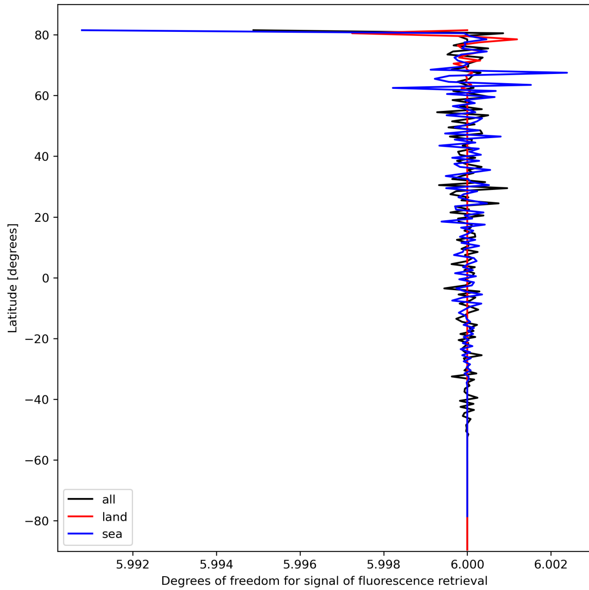
Figure 26: Zonal average of “Degrees of freedom for signal of fluorescence retrieval” for 2024-03-01 to 2024-03-03.
