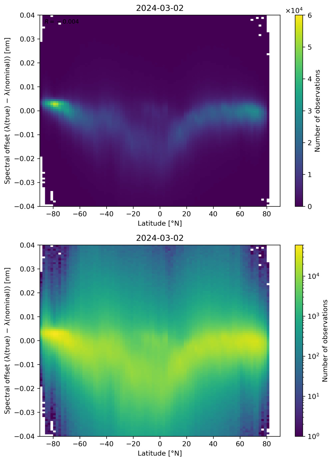
Figure 96: Scatter density plot of “Latitude” against “Spectral offset ( \lambda(\text{true}) - \lambda(\text{nominal}) )” for 2024-03-01 to 2024-03-03.
