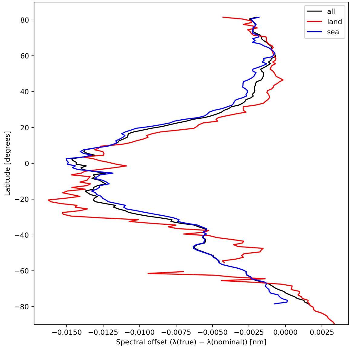
Figure 28: Zonal average of “Spectral offset ( \lambda(\text{true}) - \lambda(\text{nominal}) )” for 2024-03-01 to 2024-03-03.
