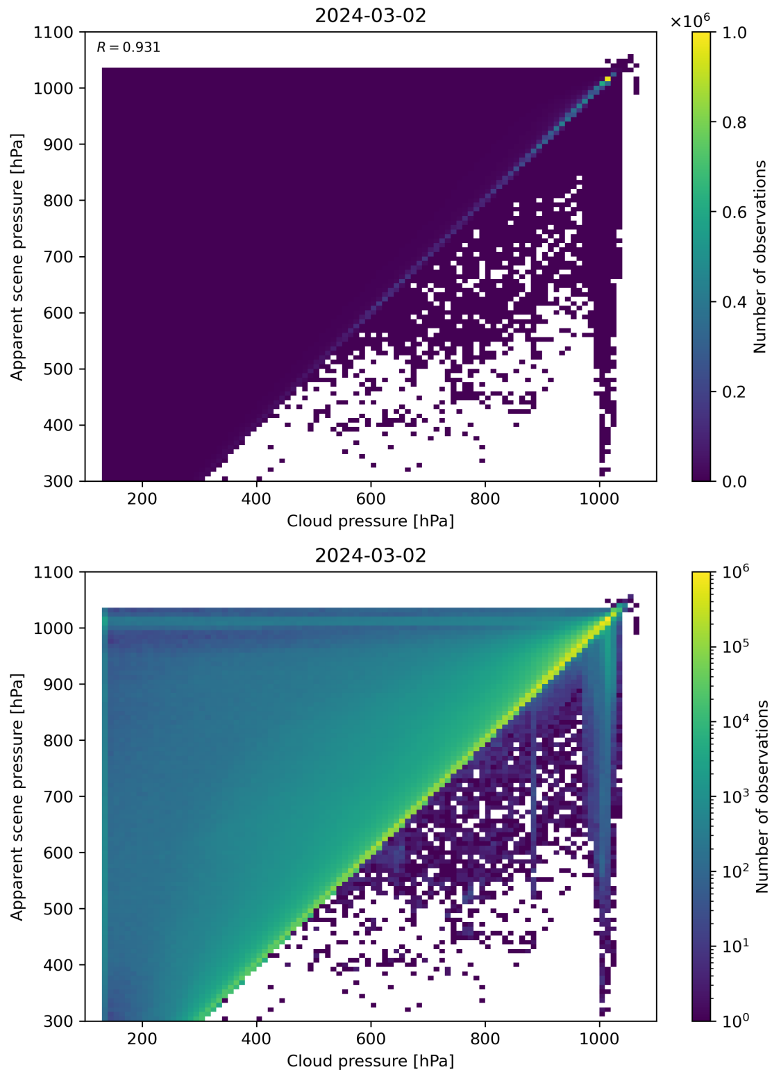
Figure 77: Scatter density plot of “Cloud pressure” against “Apparent scene pressure” for 2024-03-01 to 2024-03-03.
