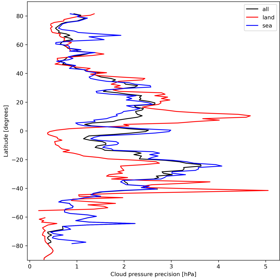
Figure 14: Zonal average of “Cloud pressure precision” for 2024-03-01 to 2024-03-03.
