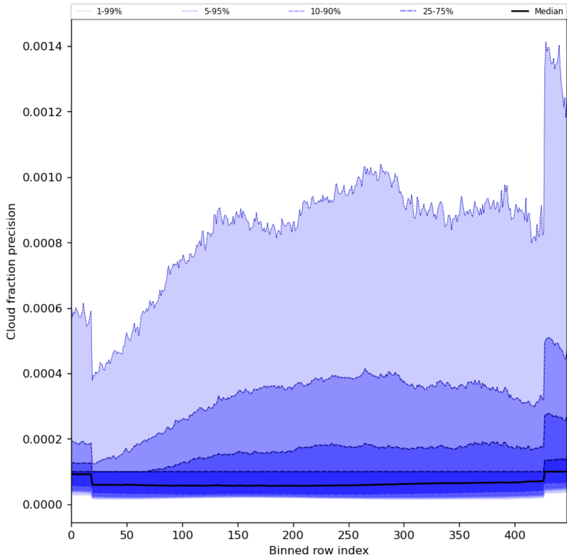
Figure 50: Along track statistics of “Cloud fraction precision” for 2024-03-01 to 2024-03-03
