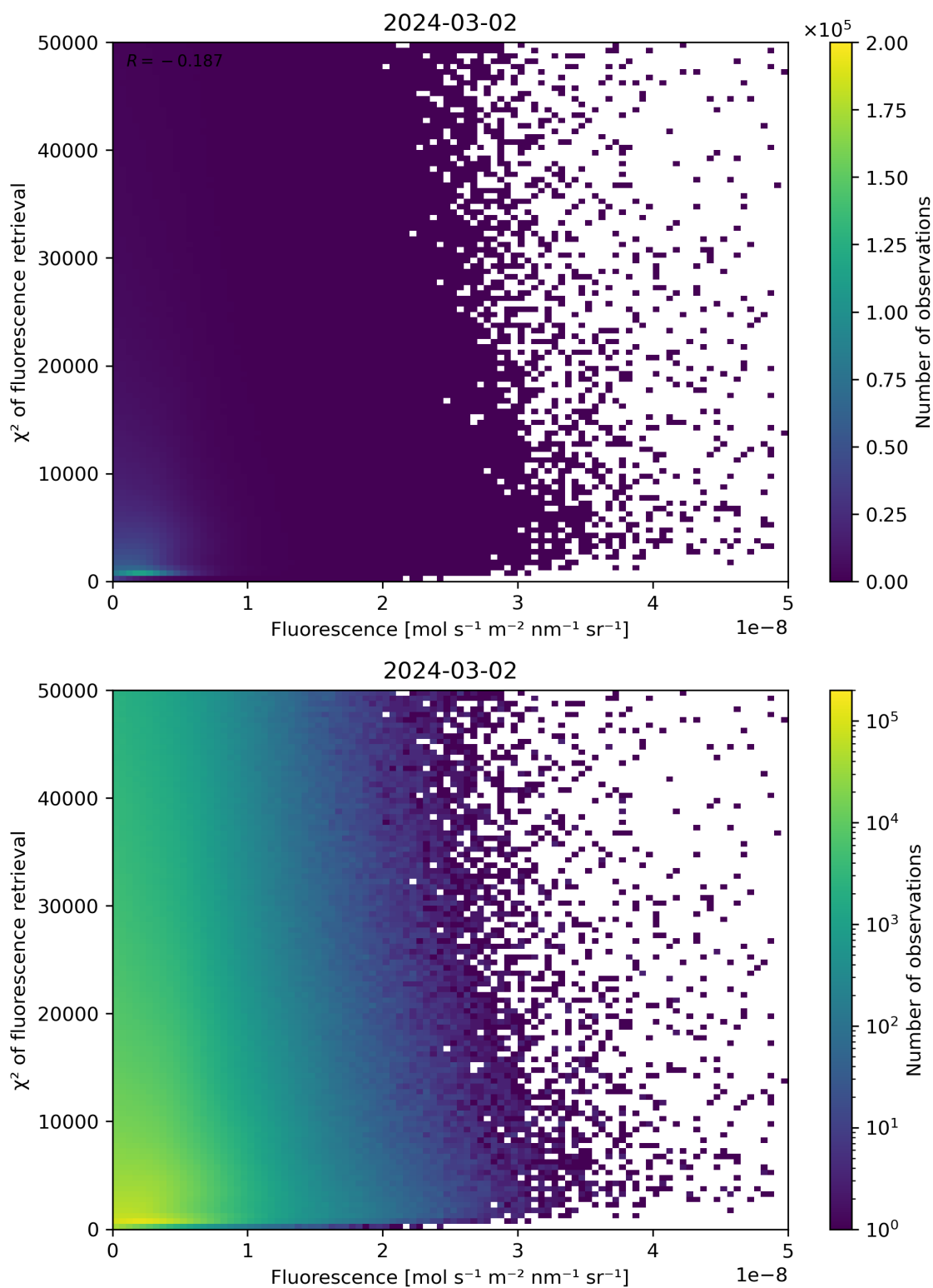
Figure 85: Scatter density plot of “Fluorescence” against “ \chi^2 of fluorescence retrieval” for 2024-03-01 to 2024-03-03.
