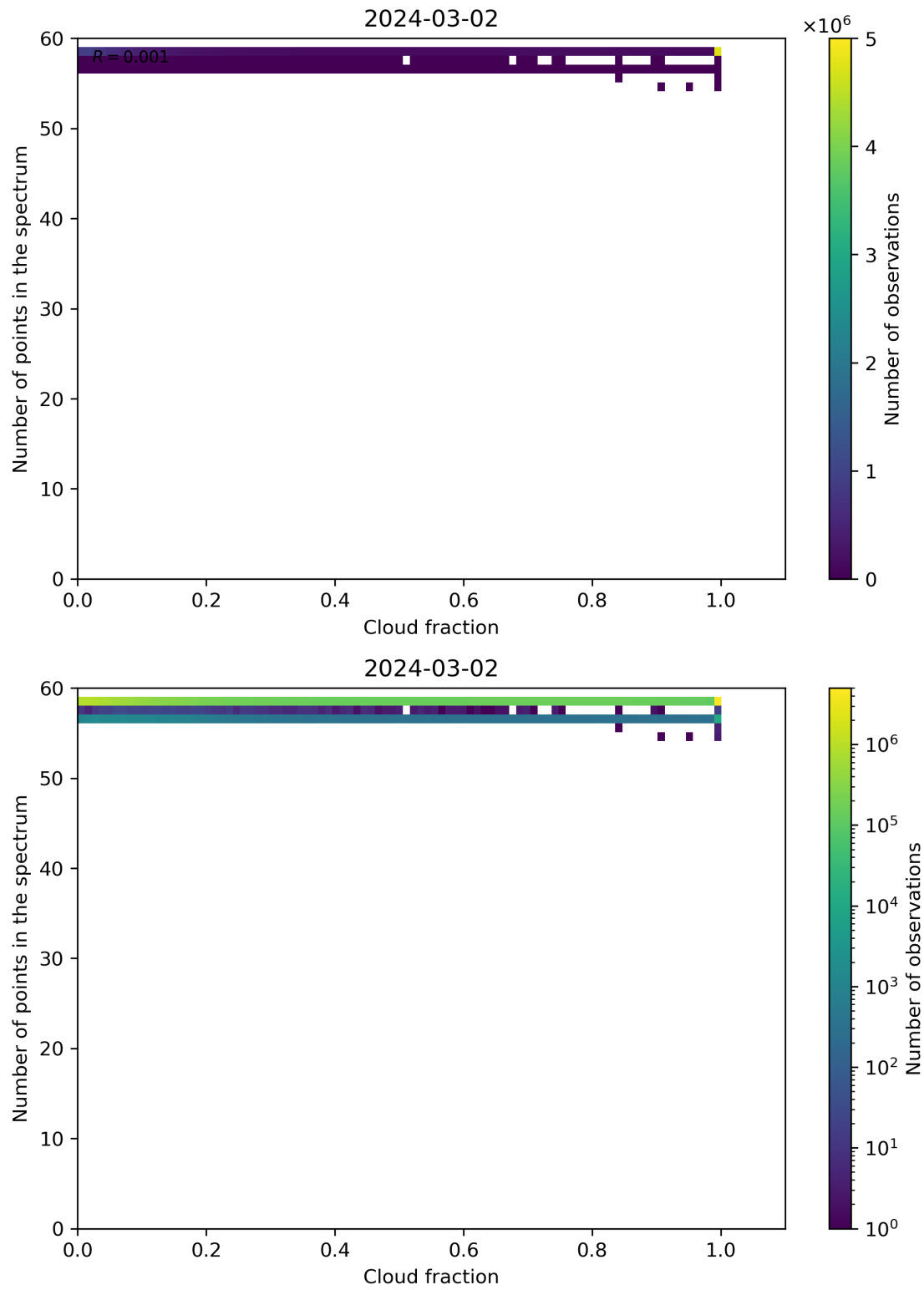
Figure 74: Scatter density plot of “Cloud fraction” against “Number of points in the spectrum” for 2024-03-01 to 2024-03-03.
