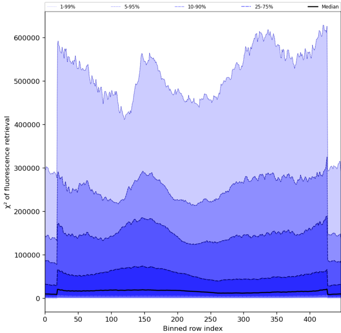
Figure 59: Along track statistics of “ \chi^2 of fluorescence retrieval” for 2024-03-01 to 2024-03-03
