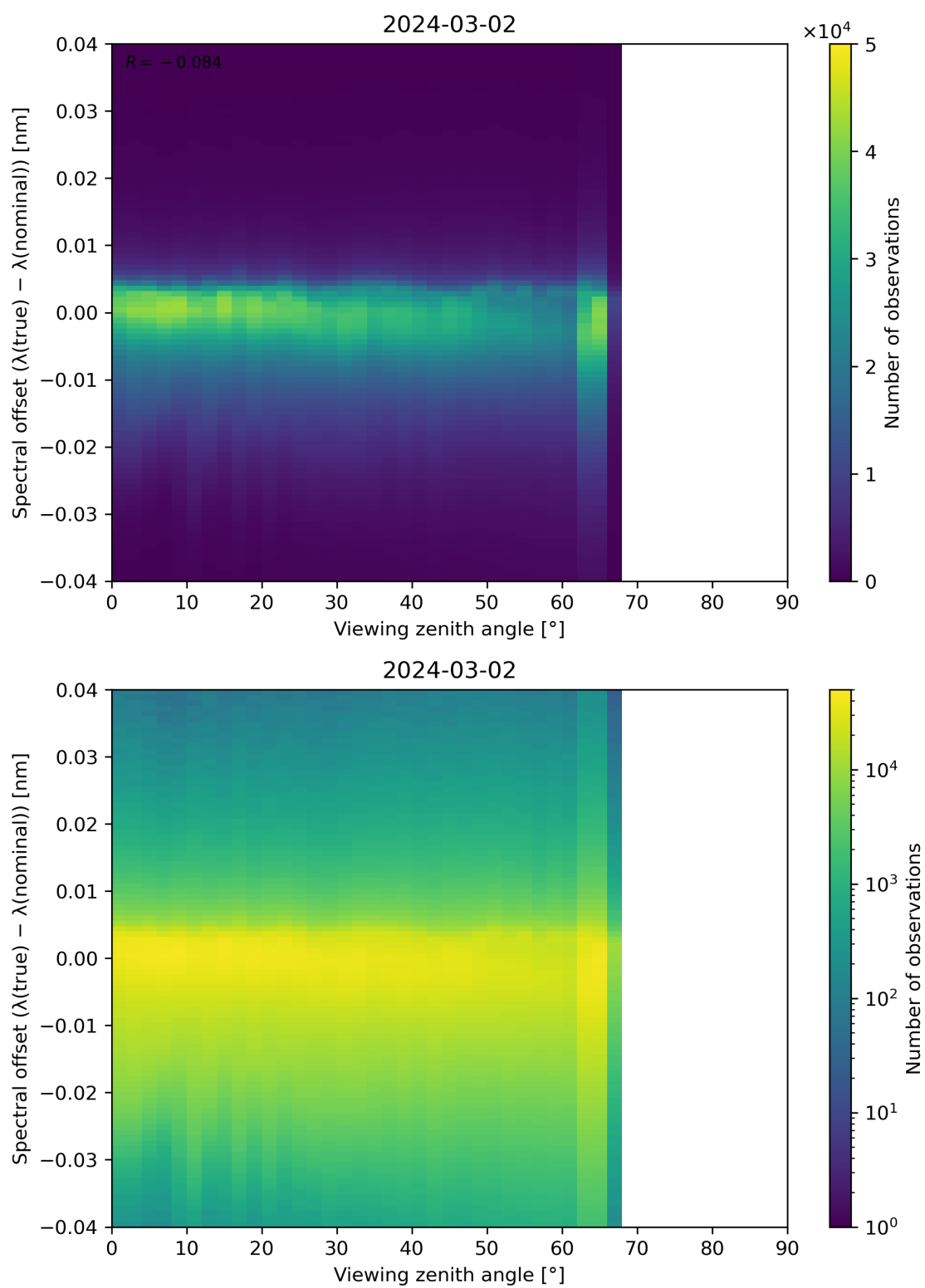
Figure 128: Scatter density plot of “Viewing zenith angle” against “Spectral offset ( \lambda(\text{true}) - \lambda(\text{nominal}) )” for 2024-03-01 to 2024-03-03.
