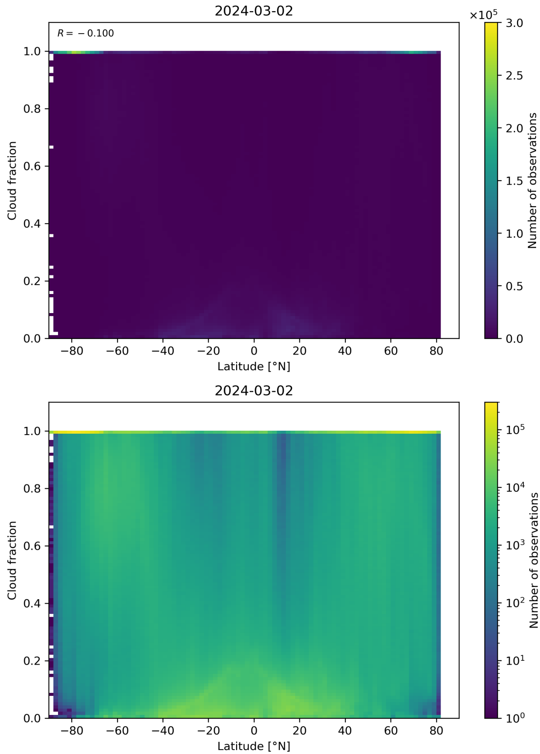
Figure 90: Scatter density plot of “Latitude” against “Cloud fraction” for 2024-03-01 to 2024-03-03.
