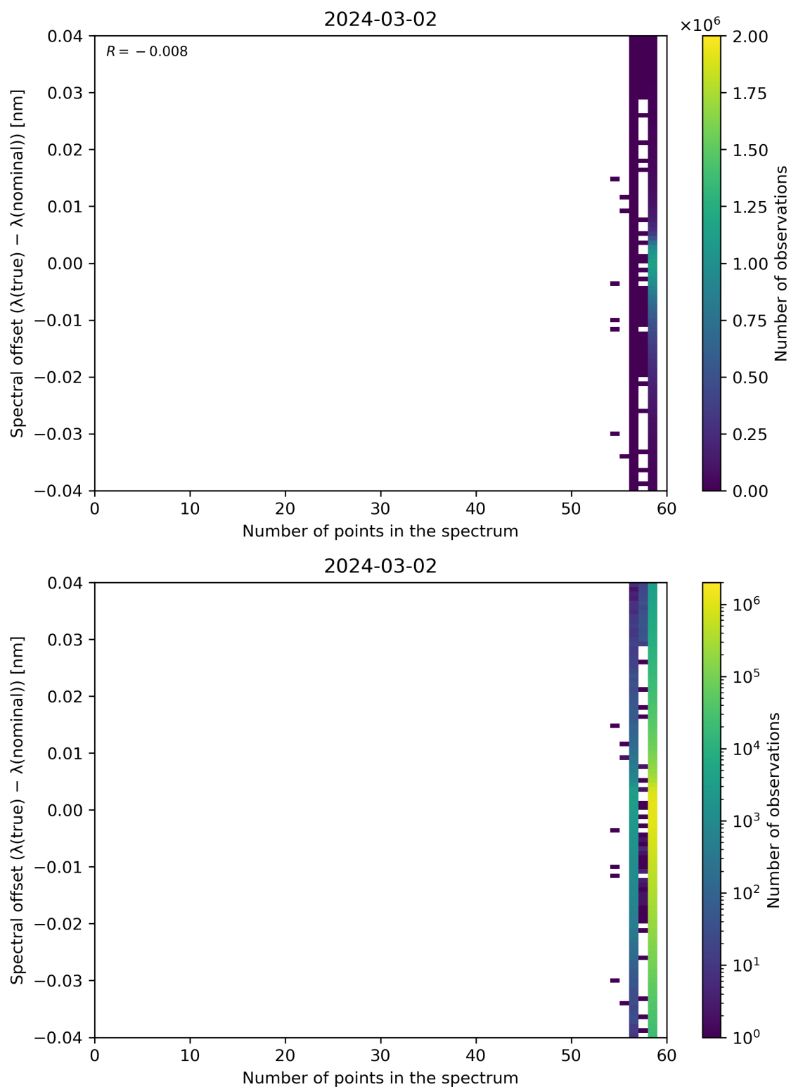
Figure 101: Scatter density plot of “Number of points in the spectrum” against “Spectral offset ( \lambda(\text{true}) - \lambda(\text{nominal}) )” for 2024-03-01 to 2024-03-03.
