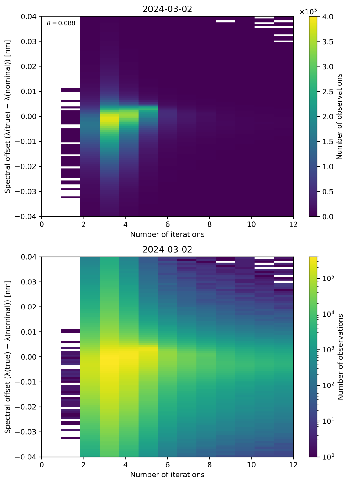
Figure 100: Scatter density plot of “Number of iterations” against “Spectral offset ( \lambda(\text{true}) - \lambda(\text{nominal}) )” for 2024-03-01 to 2024-03-03.
