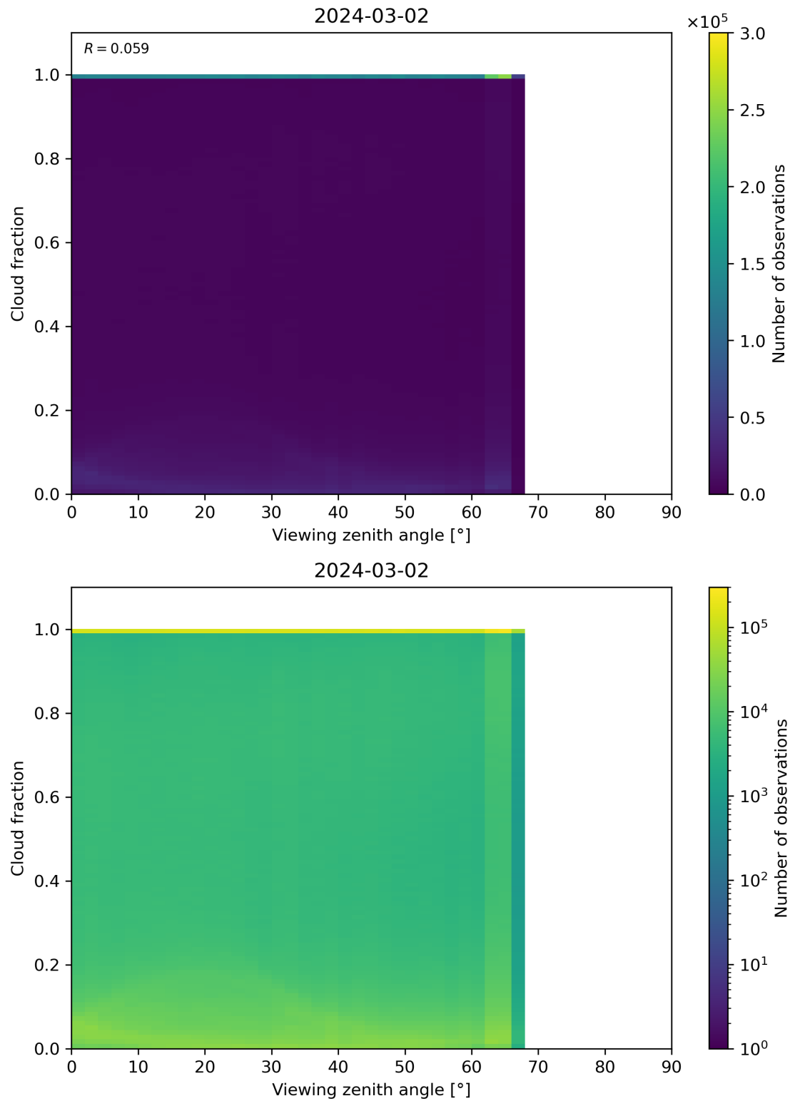
Figure 120: Scatter density plot of “Viewing zenith angle” against “Cloud fraction” for 2024-03-01 to 2024-03-03.
