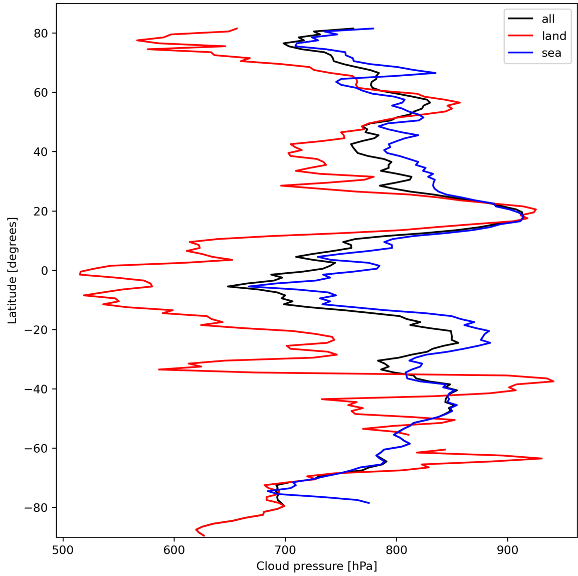
Figure 13: Zonal average of “Cloud pressure” for 2024-03-01 to 2024-03-03.
