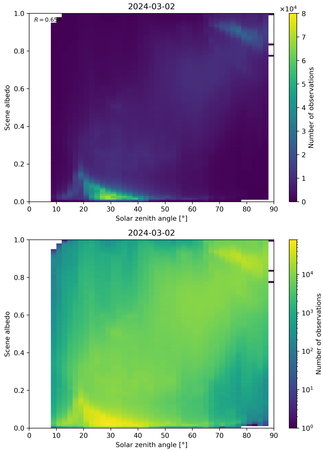
Figure 116: Scatter density plot of “Solar zenith angle” against “Scene albedo” for 2024-03-01 to 2024-03-03.
