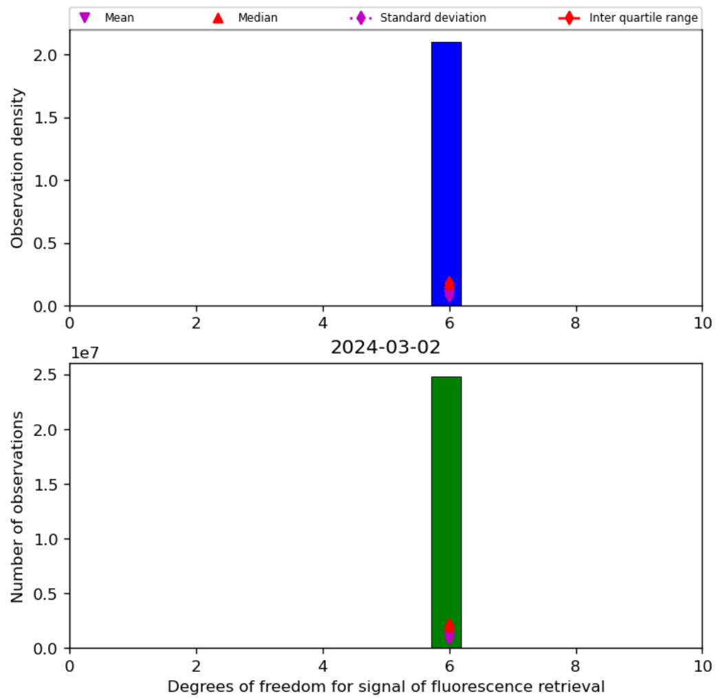
Figure 43: Histogram of “Degrees of freedom for signal of fluorescence retrieval” for 2024-03-01 to 2024-03-03
