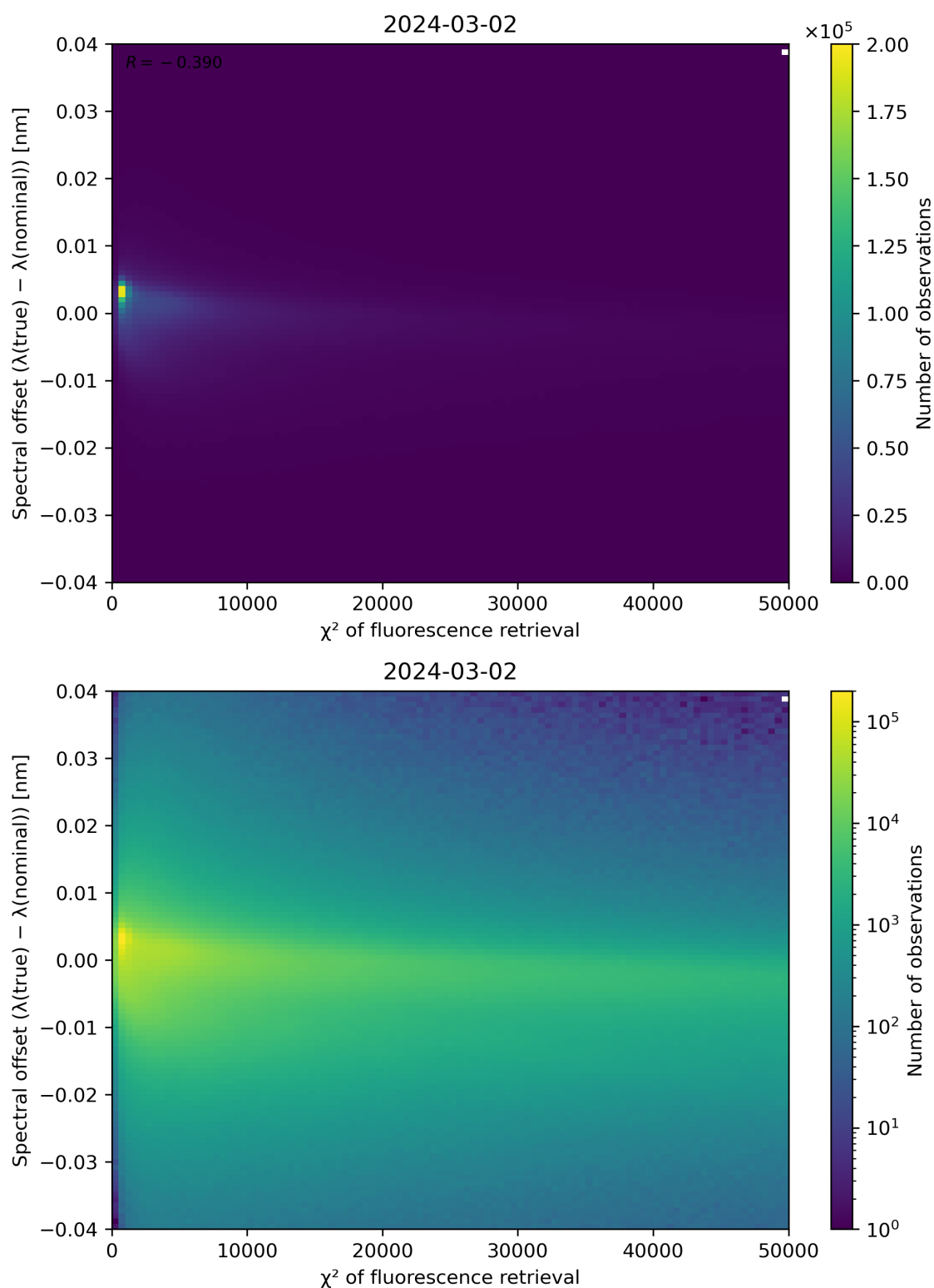
Figure 69: Scatter density plot of " \chi^2 of fluorescence retrieval" against "Spectral offset ( \lambda(\text{true}) - \lambda(\text{nominal}) )" for 2024-03-01 to 2024-03-03.
