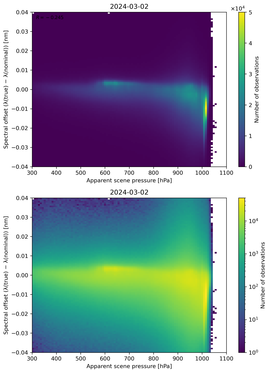
Figure 67: Scatter density plot of “Apparent scene pressure” against “Spectral offset ( \lambda(\text{true}) - \lambda(\text{nominal}) )” for 2024-03-01 to 2024-03-03.
