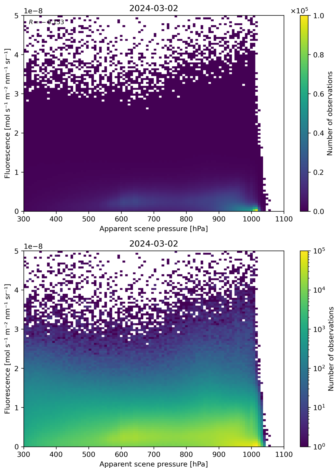
Figure 64: Scatter density plot of “Apparent scene pressure” against “Fluorescence” for 2024-03-01 to 2024-03-03.
