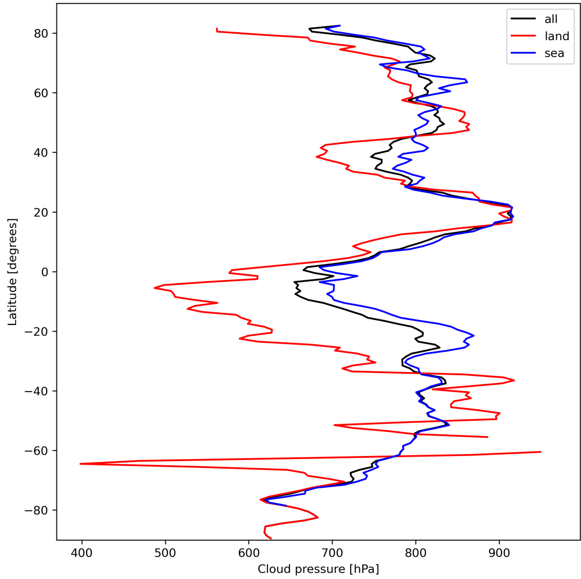
Figure 13: Zonal average of “Cloud pressure” for 2024-03-04 to 2024-03-05.
