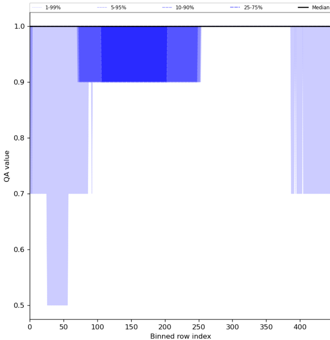
Figure 46: Along track statistics of “QA value” for 2024-03-04 to 2024-03-05
