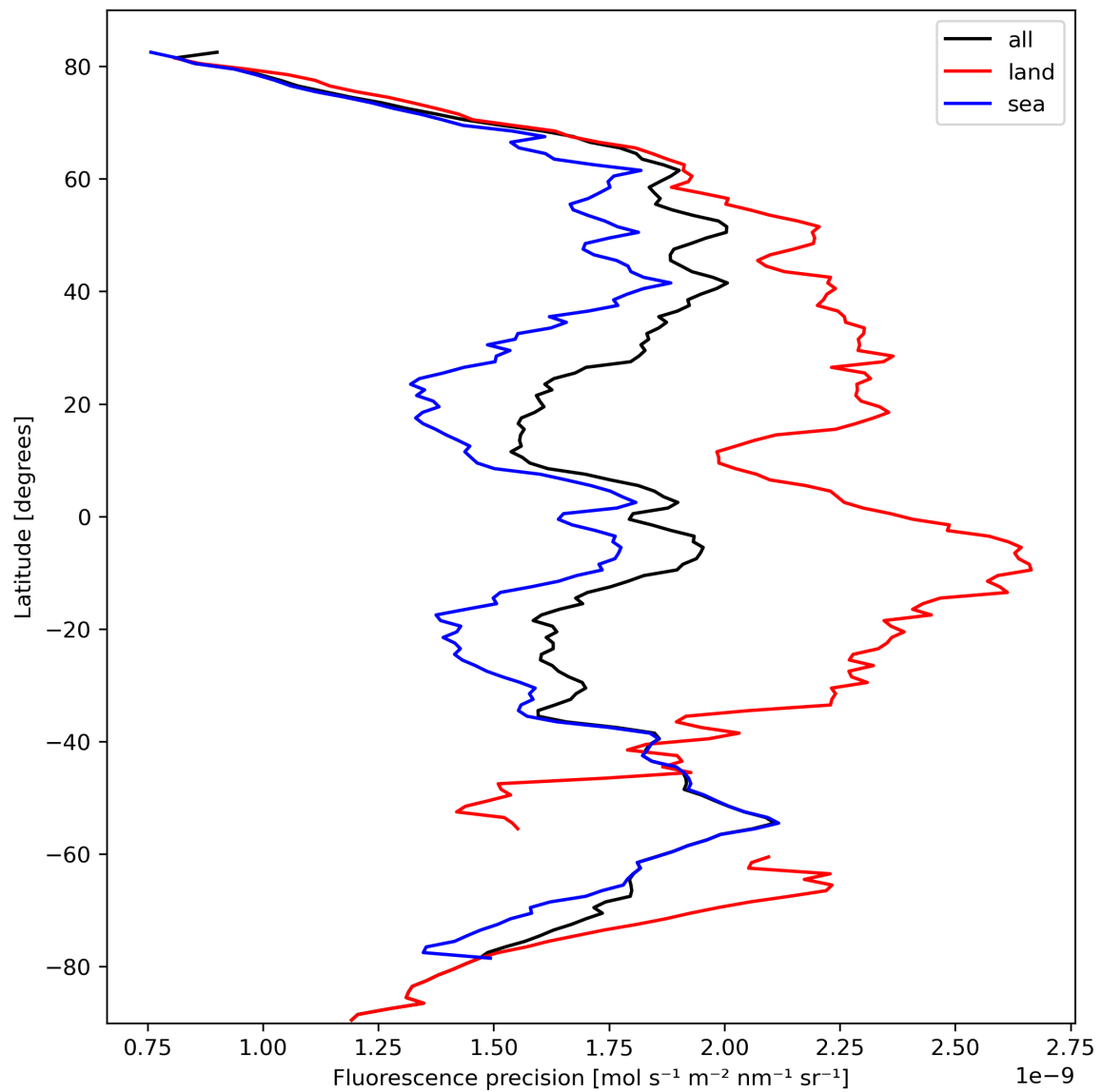
Figure 24: Zonal average of “Fluorescence precision” for 2024-03-04 to 2024-03-05.
