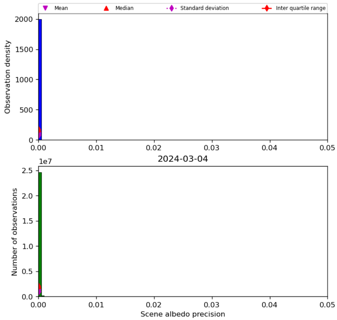
Figure 35: Histogram of “Scene albedo precision” for 2024-03-04 to 2024-03-05
