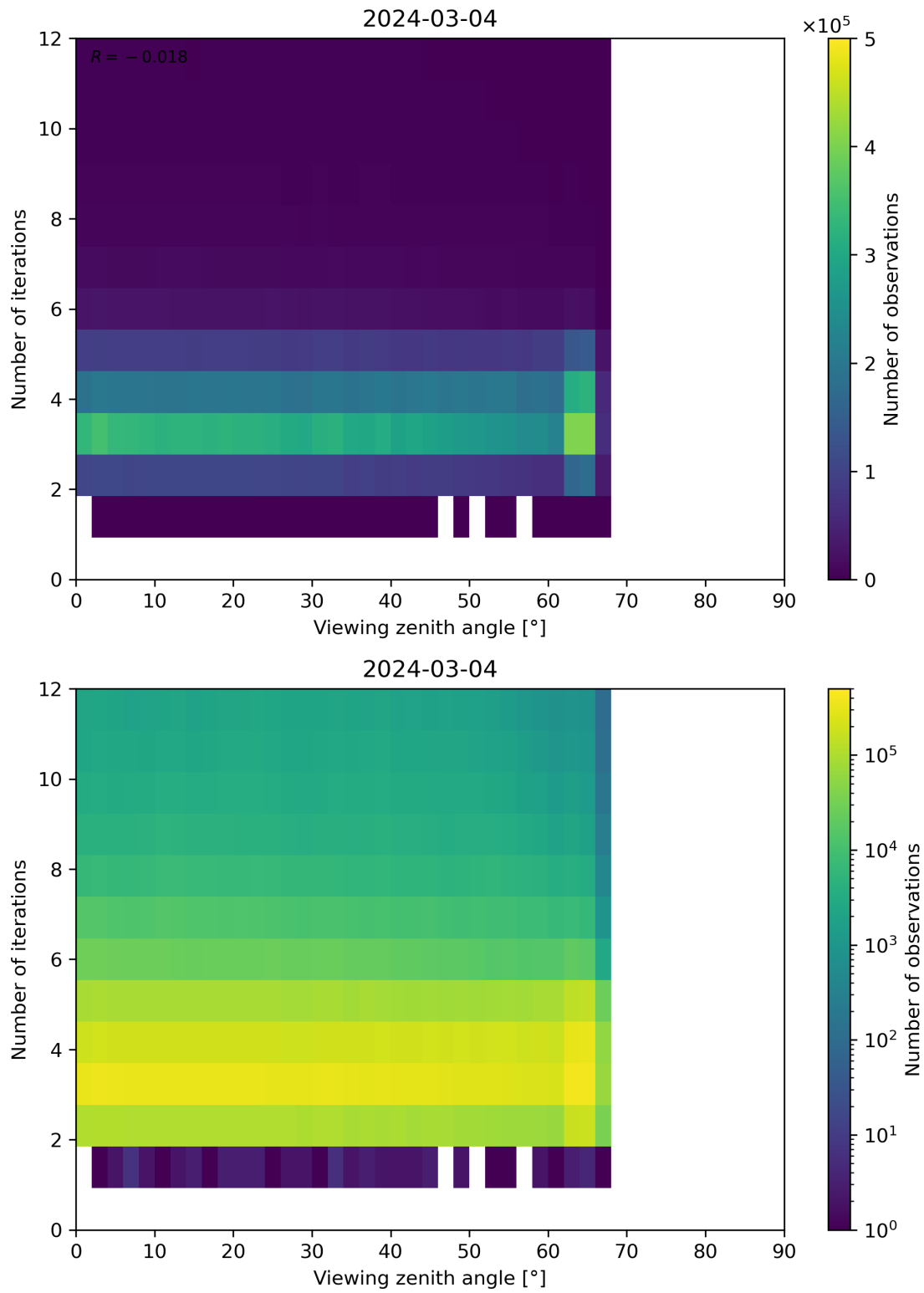
Figure 124: Scatter density plot of “Viewing zenith angle” against “Number of iterations” for 2024-03-04 to 2024-03-05.
