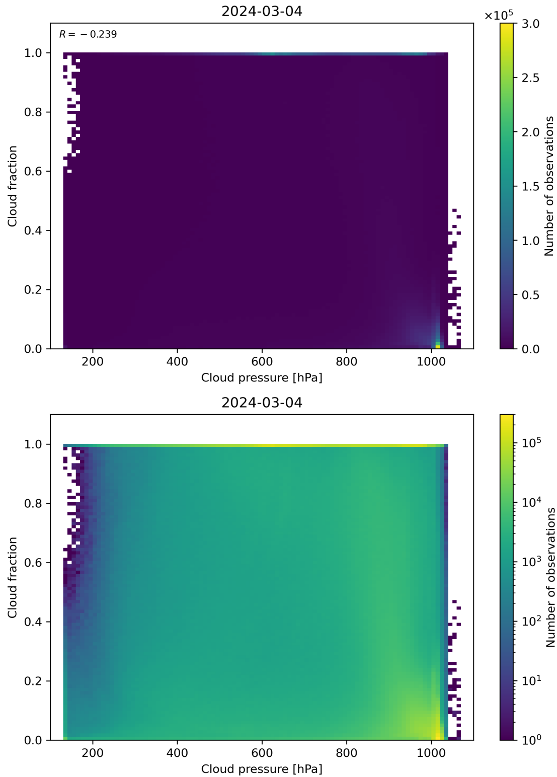
Figure 79: Scatter density plot of “Cloud pressure” against “Cloud fraction” for 2024-03-04 to 2024-03-05.
