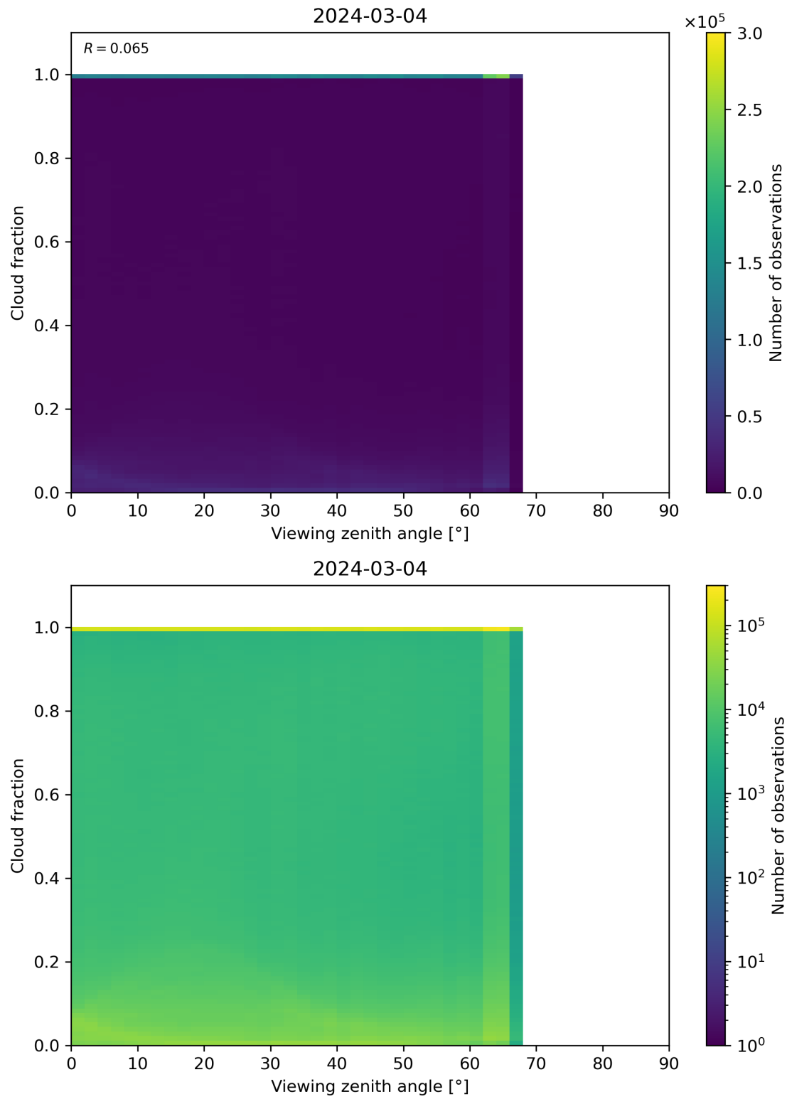
Figure 120: Scatter density plot of “Viewing zenith angle” against “Cloud fraction” for 2024-03-04 to 2024-03-05.
