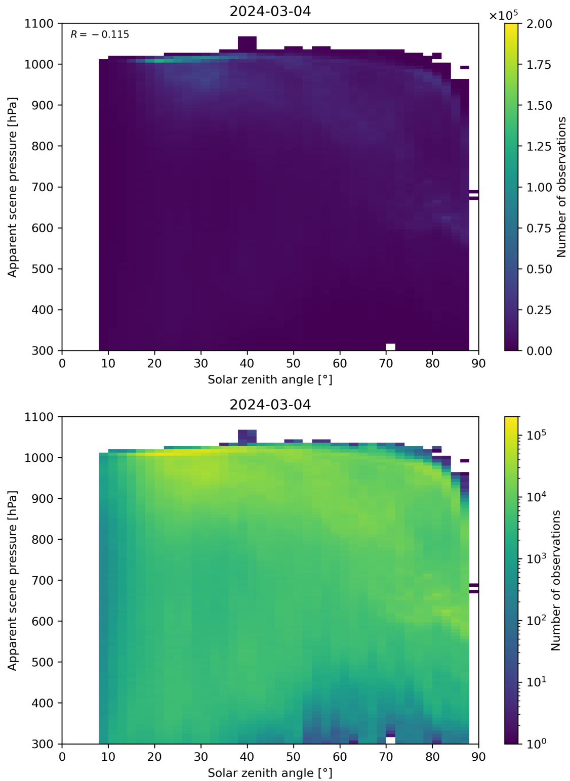
Figure 108: Scatter density plot of “Solar zenith angle” against “Apparent scene pressure” for 2024-03-04 to 2024-03-05.
