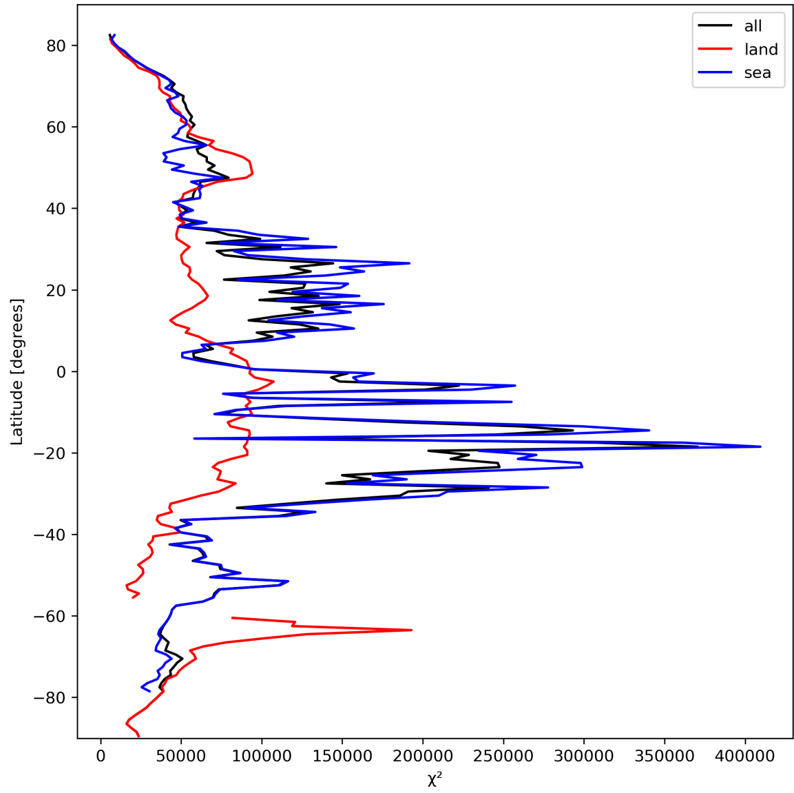
Figure 21: Zonal average of “ \chi^2 ” for 2024-03-04 to 2024-03-05.
