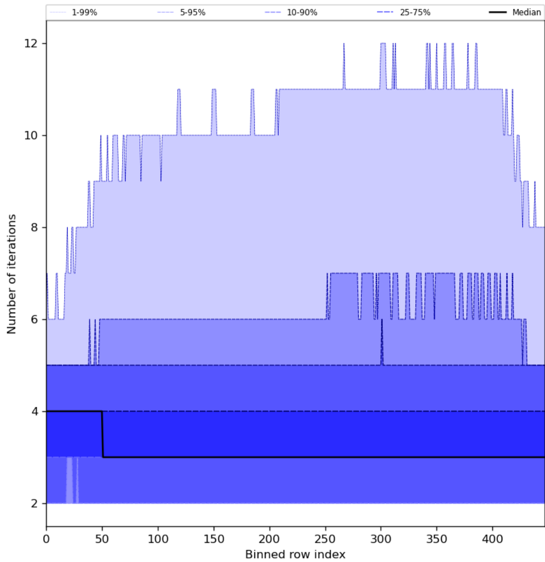
Figure 56: Along track statistics of “Number of iterations” for 2024-03-04 to 2024-03-05
