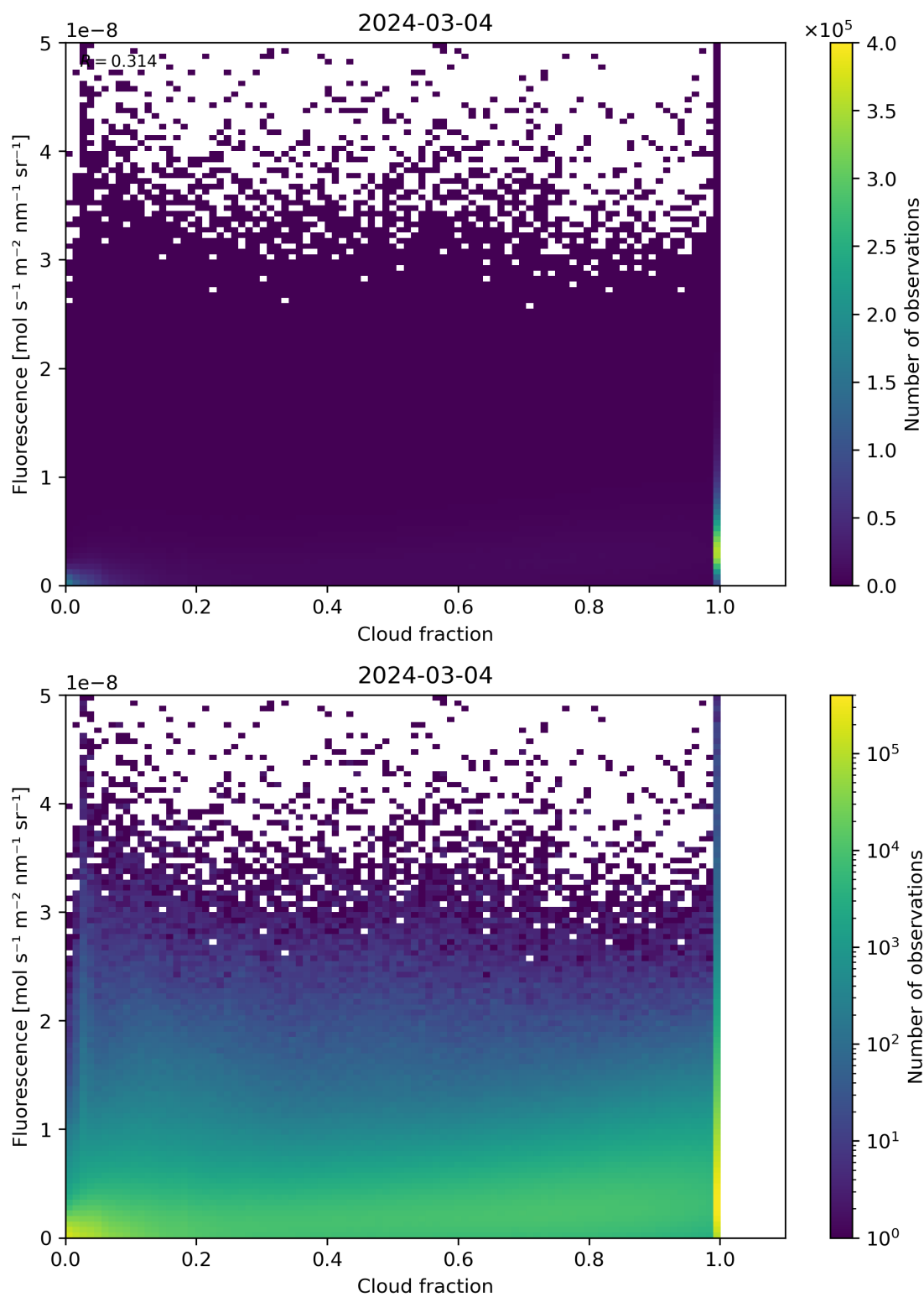
Figure 72: Scatter density plot of “Cloud fraction” against “Fluorescence” for 2024-03-04 to 2024-03-05.
