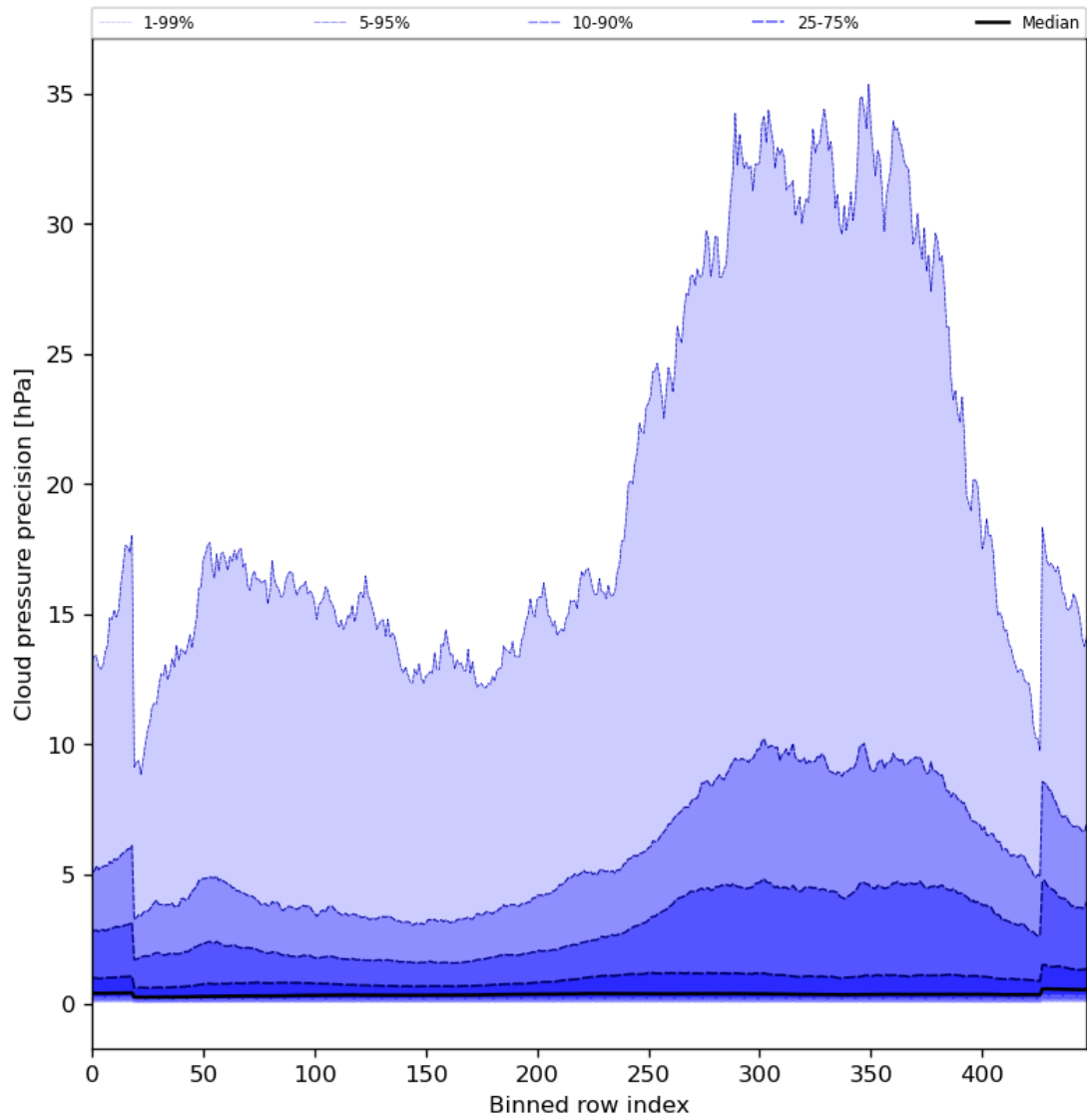
Figure 48: Along track statistics of “Cloud pressure precision” for 2024-03-04 to 2024-03-05
