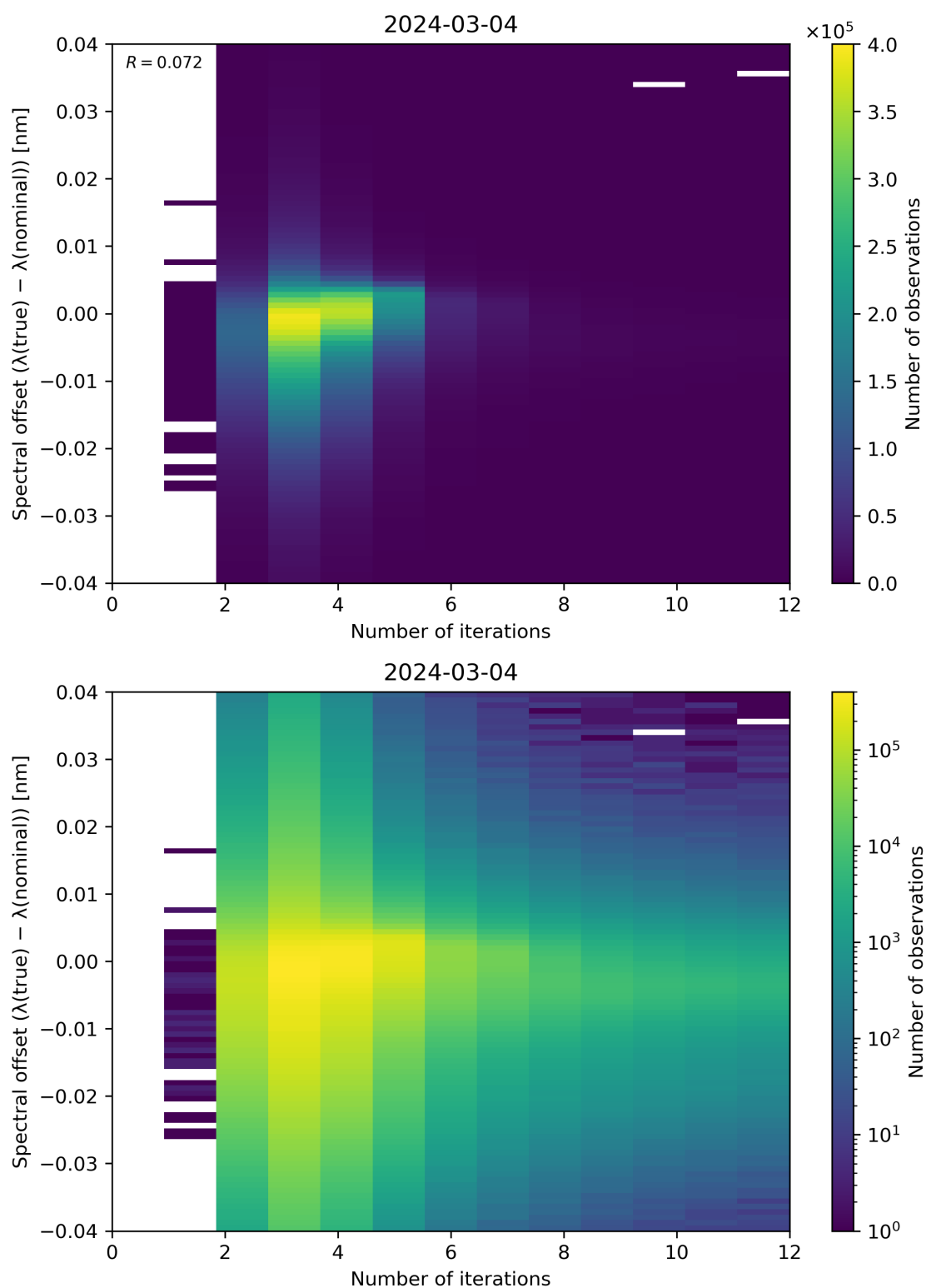
Figure 100: Scatter density plot of “Number of iterations” against “Spectral offset ( \lambda(\text{true}) - \lambda(\text{nominal}) )” for 2024-03-04 to 2024-03-05.
