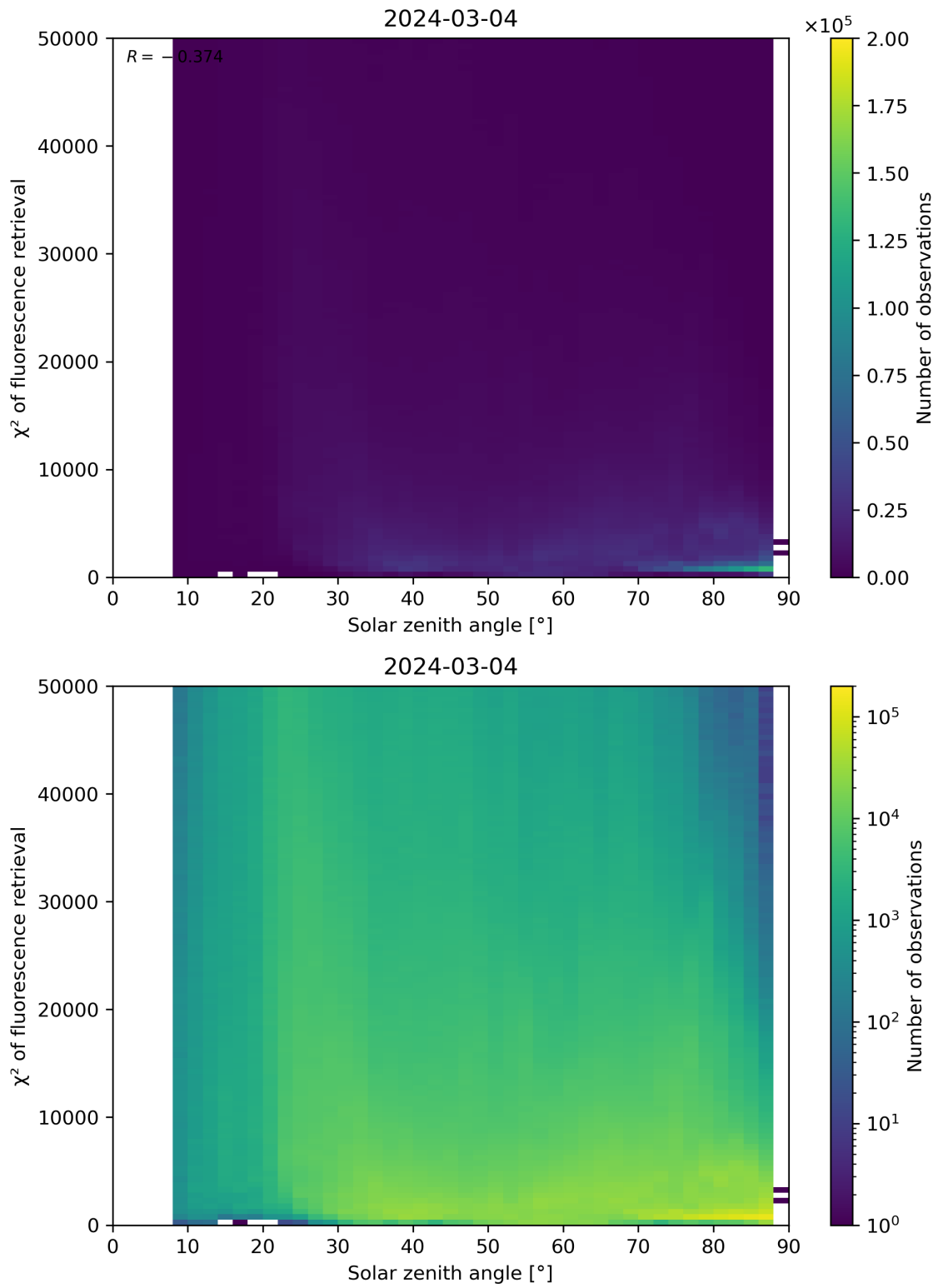
Figure 109: Scatter density plot of “Solar zenith angle” against “ \chi^2 of fluorescence retrieval” for 2024-03-04 to 2024-03-05.
