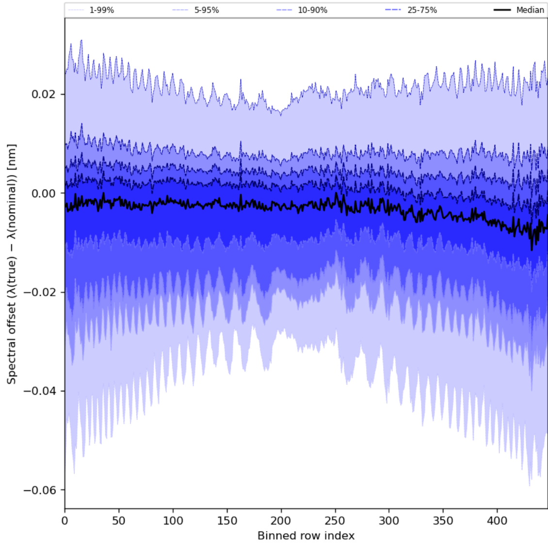
Figure 62: Along track statistics of “Spectral offset ( \lambda(\text{true}) - \lambda(\text{nominal}) )” for 2024-03-04 to 2024-03-05
