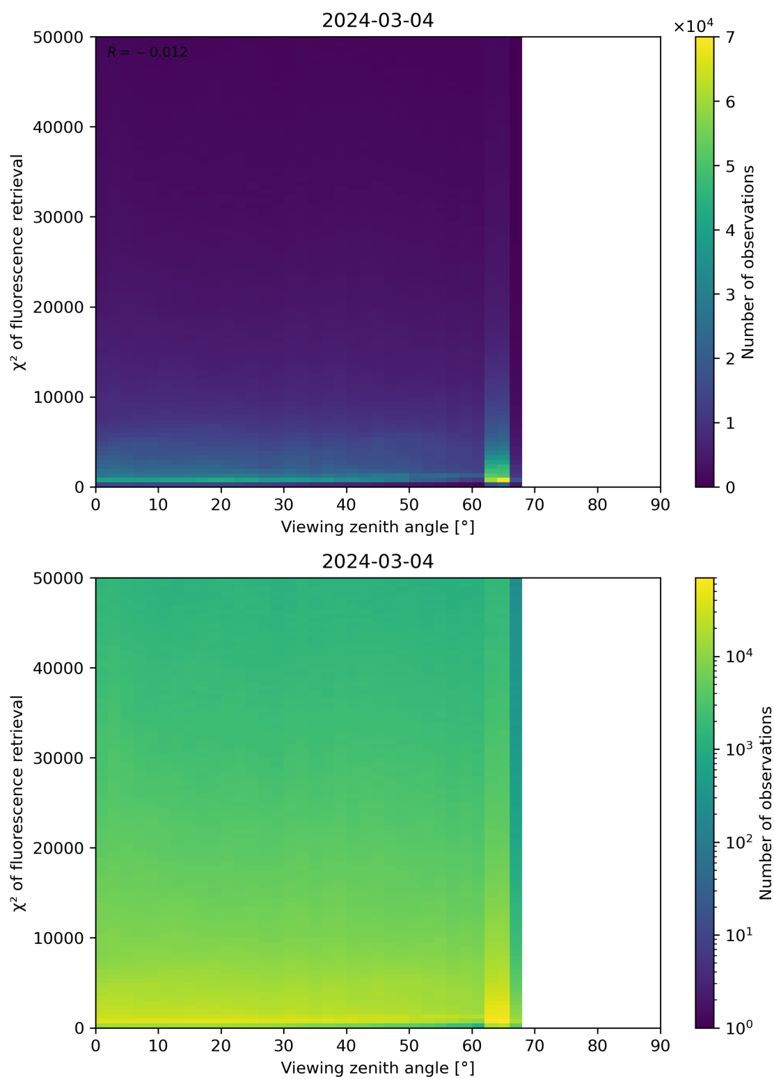
Figure 119: Scatter density plot of “Viewing zenith angle” against “ \chi^2 of fluorescence retrieval” for 2024-03-04 to 2024-03-05.
