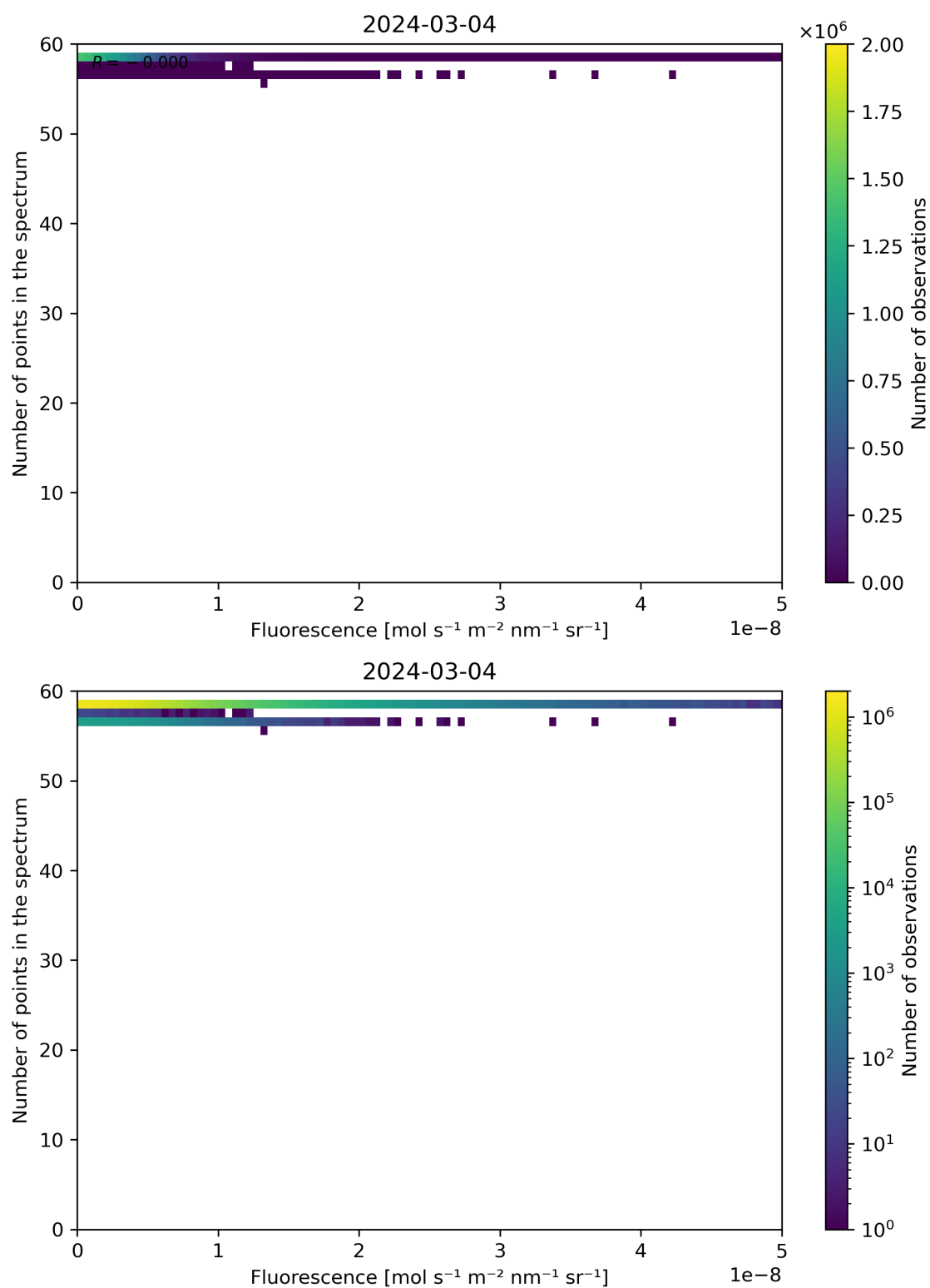
Figure 86: Scatter density plot of “Fluorescence” against “Number of points in the spectrum” for 2024-03-04 to 2024-03-05.
