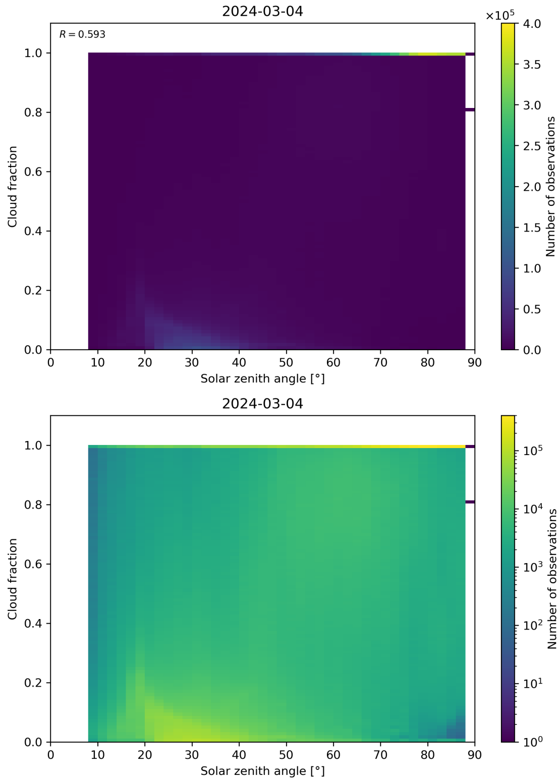
Figure 110: Scatter density plot of “Solar zenith angle” against “Cloud fraction” for 2024-03-04 to 2024-03-05.
