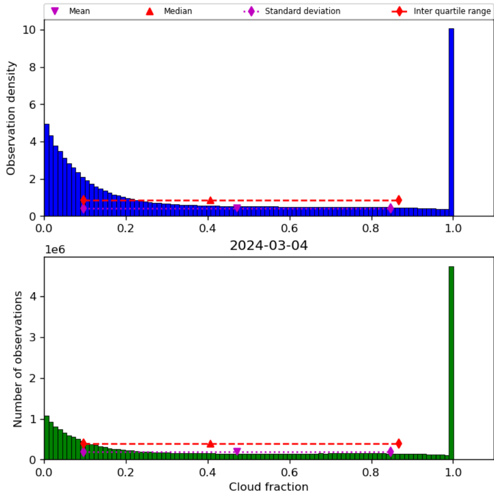
Figure 32: Histogram of “Cloud fraction” for 2024-03-04 to 2024-03-05
