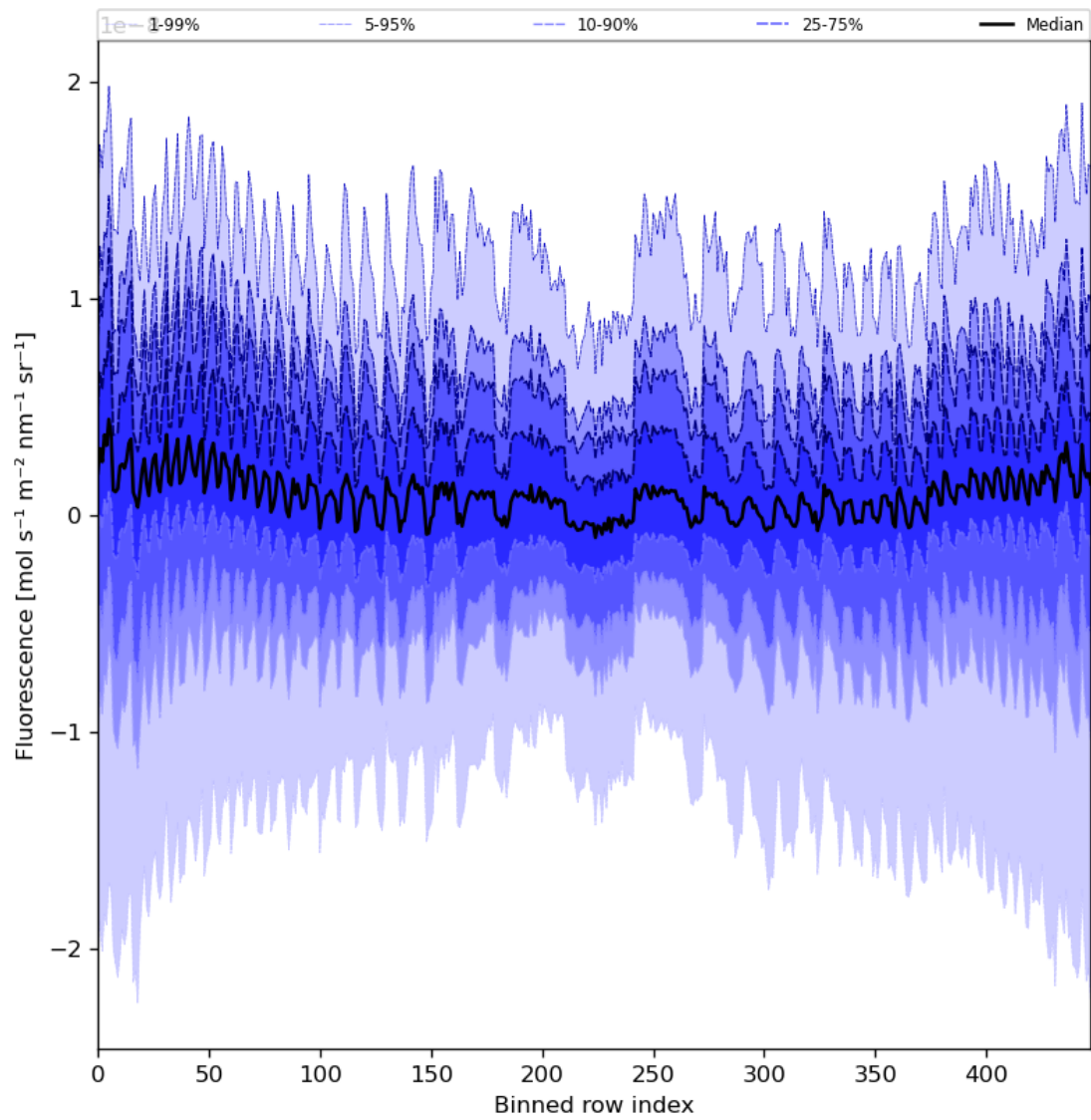
Figure 57: Along track statistics of “Fluorescence” for 2024-03-04 to 2024-03-05
