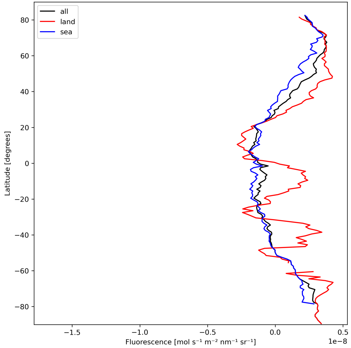
Figure 23: Zonal average of “Fluorescence” for 2024-03-04 to 2024-03-05.
