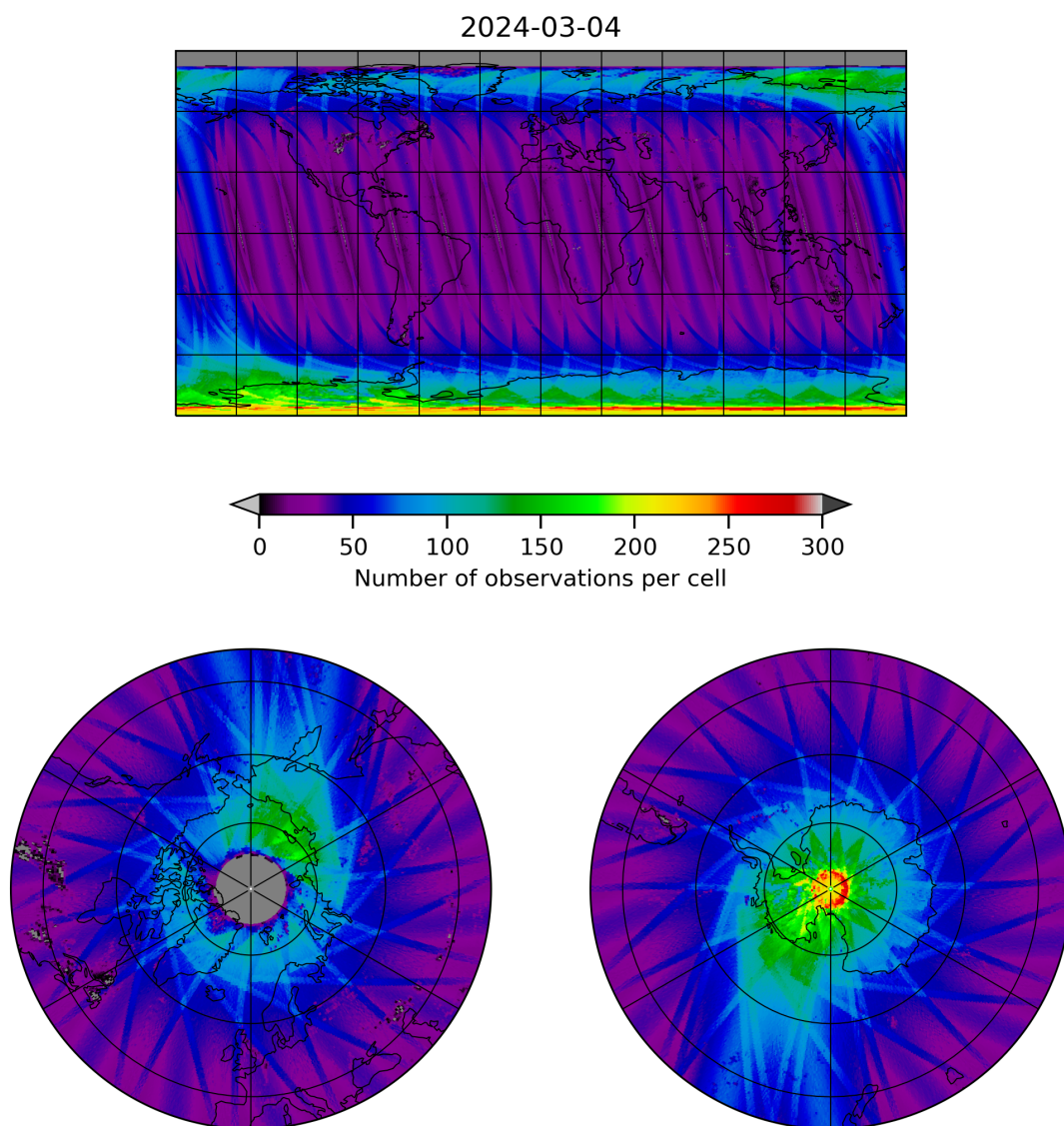
Figure 11: Map of the number of observations for 2024-03-04 to 2024-03-05
