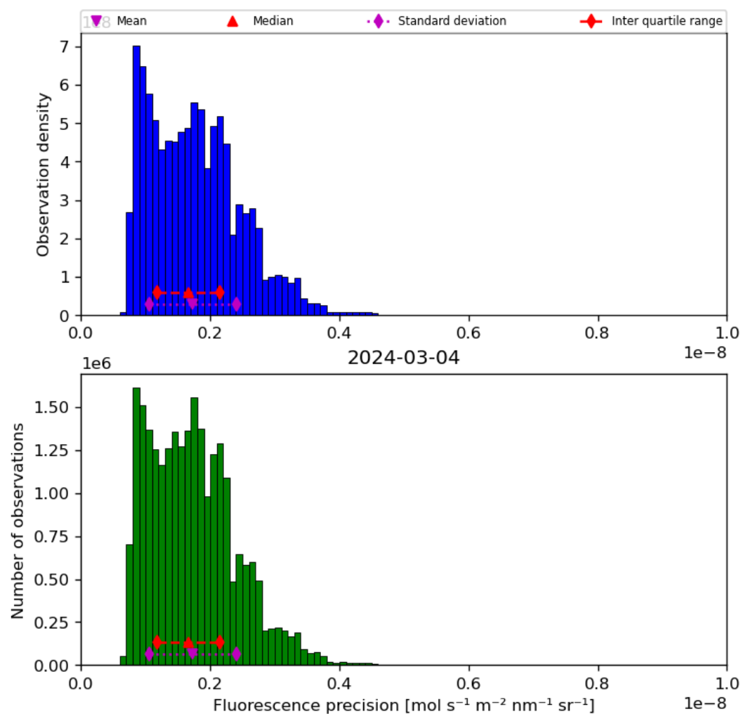
Figure 41: Histogram of “Fluorescence precision” for 2024-03-04 to 2024-03-05
