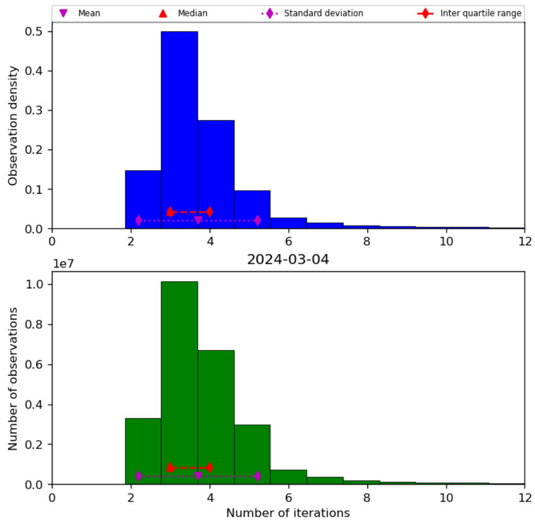
Figure 39: Histogram of “Number of iterations” for 2024-03-04 to 2024-03-05
