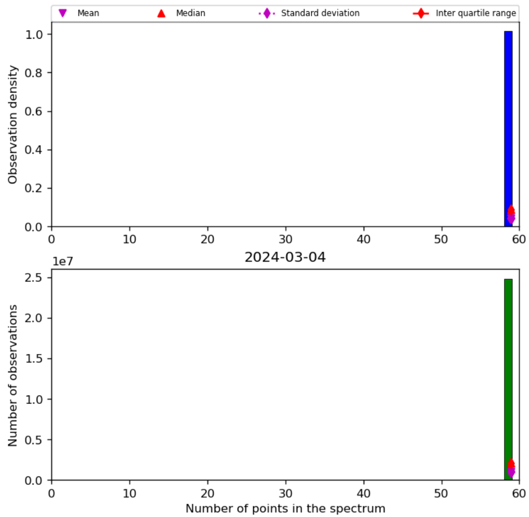
Figure 44: Histogram of “Number of points in the spectrum” for 2024-03-04 to 2024-03-05
