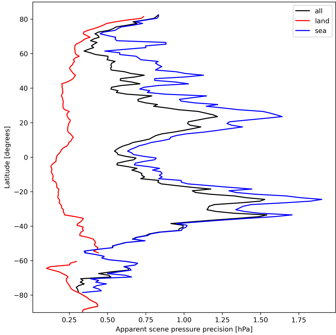
Figure 20: Zonal average of “Apparent scene pressure precision” for 2024-03-04 to 2024-03-05.
