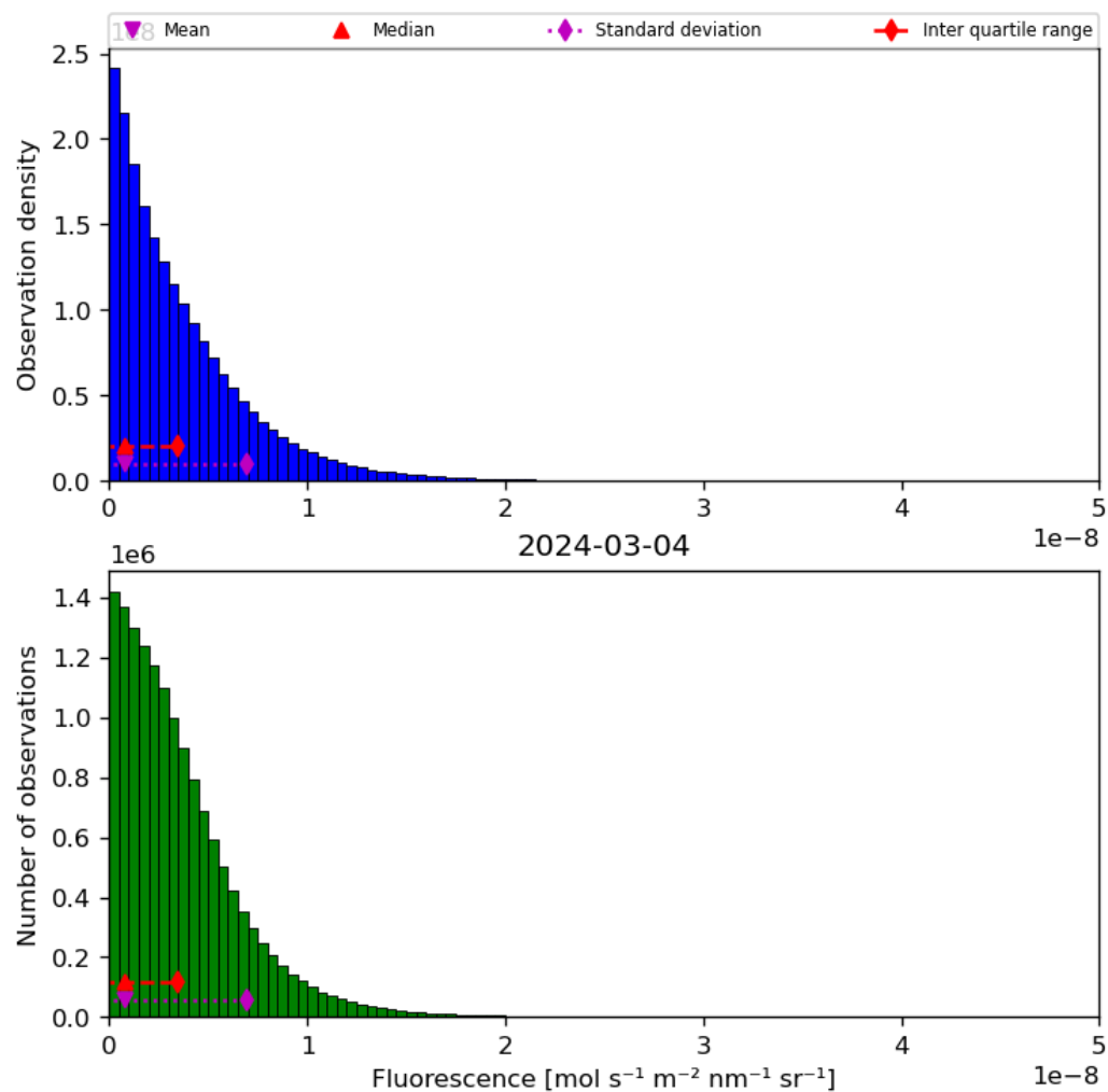
Figure 40: Histogram of “Fluorescence” for 2024-03-04 to 2024-03-05
