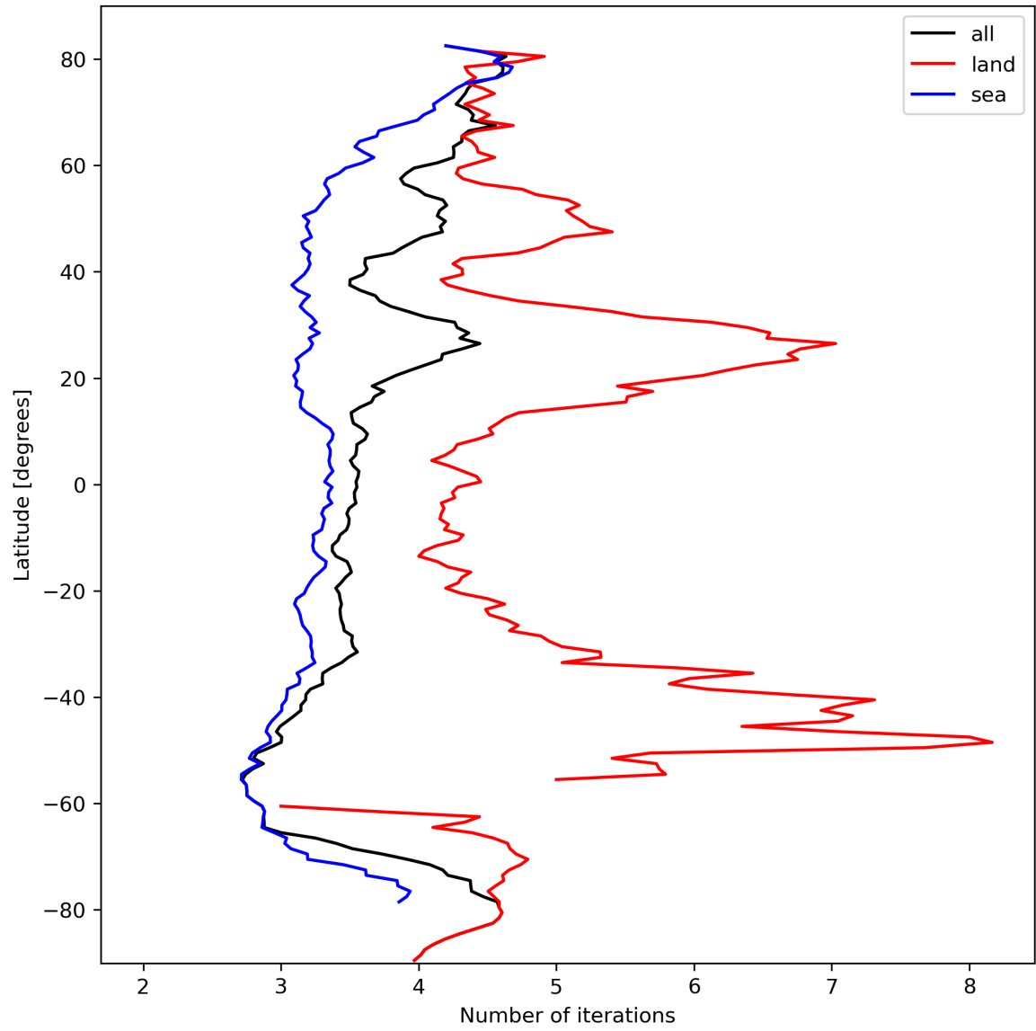
Figure 22: Zonal average of “Number of iterations” for 2024-03-04 to 2024-03-05.
