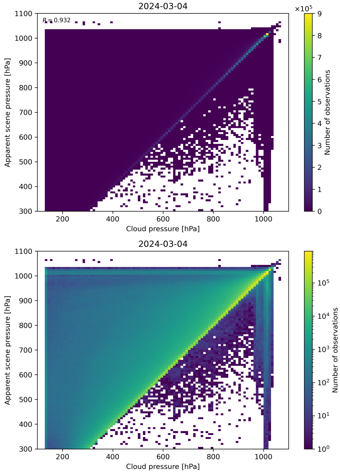
Figure 77: Scatter density plot of “Cloud pressure” against “Apparent scene pressure” for 2024-03-04 to 2024-03-05.
