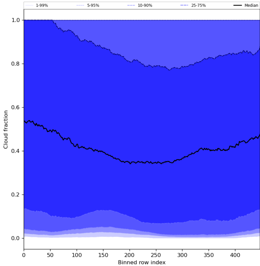
Figure 49: Along track statistics of “Cloud fraction” for 2024-03-04 to 2024-03-05
