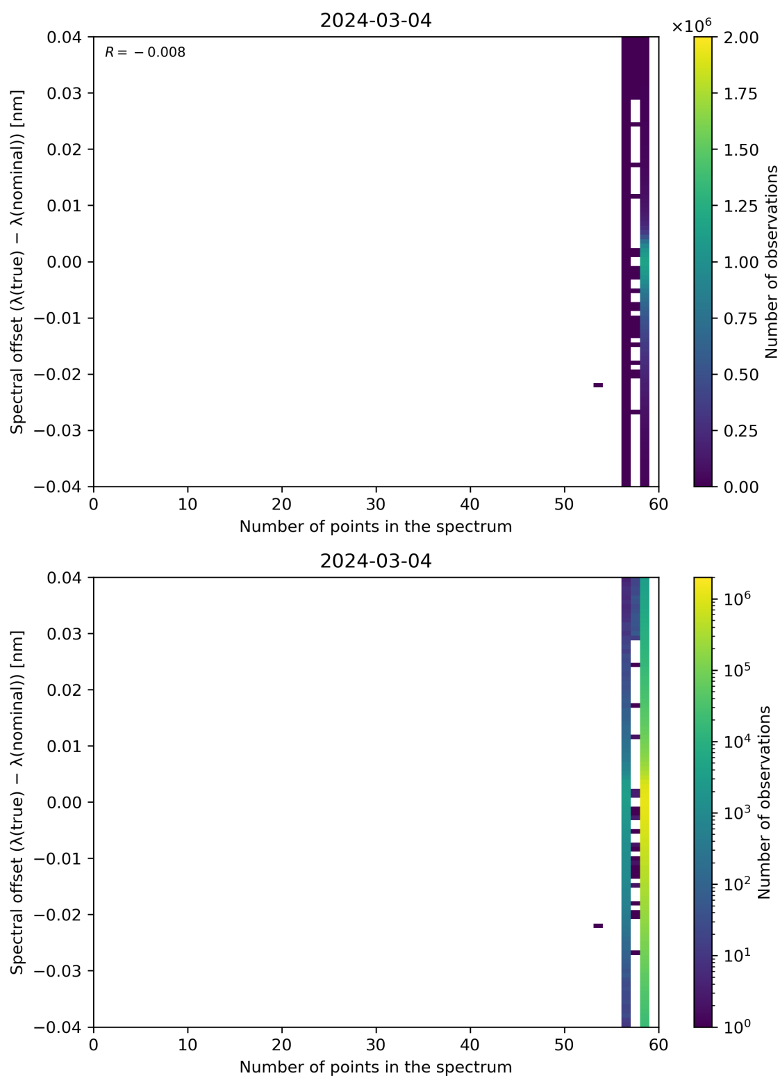
Figure 101: Scatter density plot of “Number of points in the spectrum” against “Spectral offset ( \lambda(\text{true}) - \lambda(\text{nominal}) )” for 2024-03-04 to 2024-03-05.
