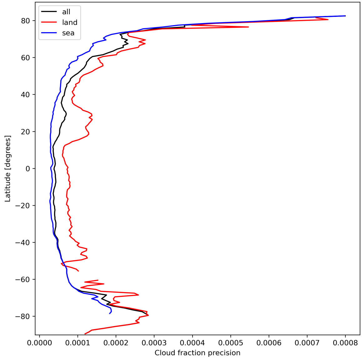
Figure 16: Zonal average of “Cloud fraction precision” for 2024-03-04 to 2024-03-05.
