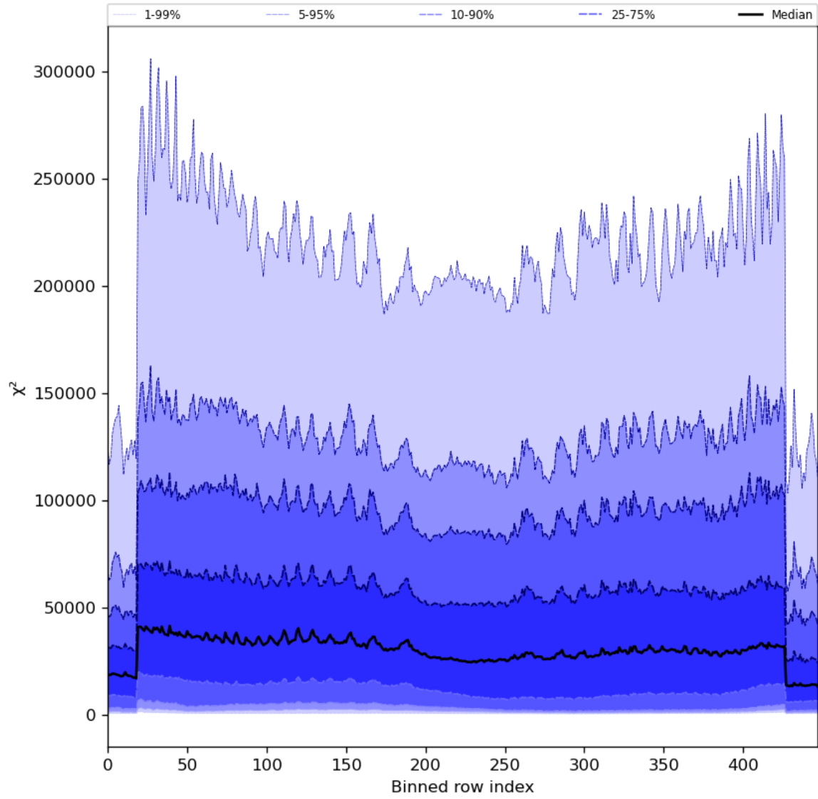
Figure 55: Along track statistics of “ \chi^2 ” for 2024-03-04 to 2024-03-05
