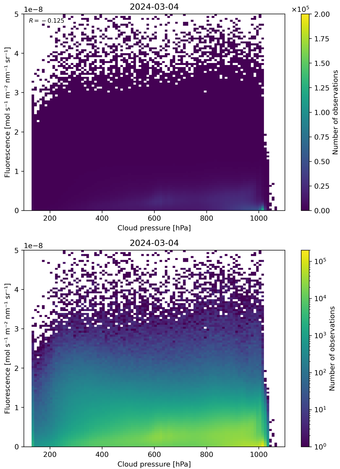
Figure 80: Scatter density plot of “Cloud pressure” against “Fluorescence” for 2024-03-04 to 2024-03-05.
