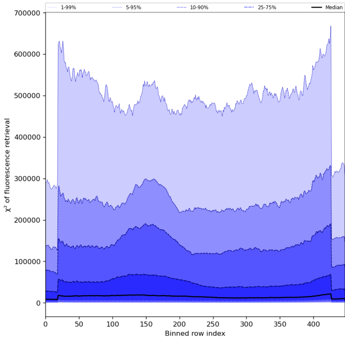
Figure 59: Along track statistics of “ \chi^2 of fluorescence retrieval” for 2024-03-04 to 2024-03-05
