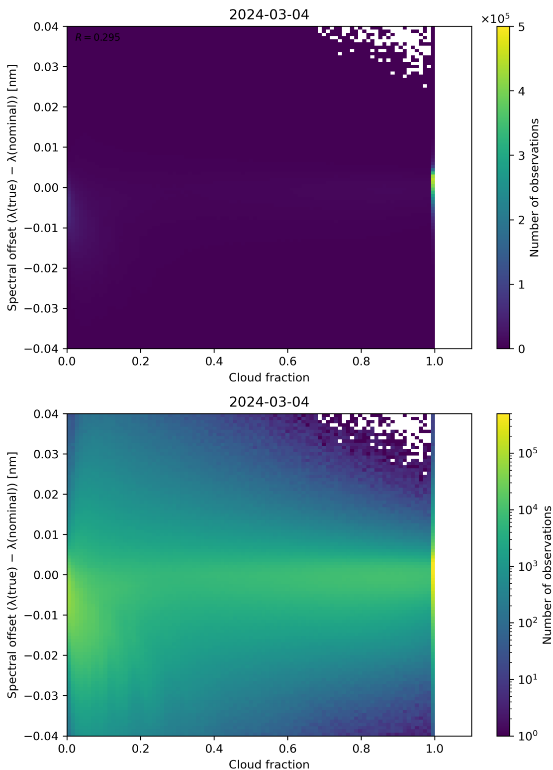
Figure 76: Scatter density plot of “Cloud fraction” against “Spectral offset ( \lambda(\text{true}) - \lambda(\text{nominal}) )” for 2024-03-04 to 2024-03-05.
