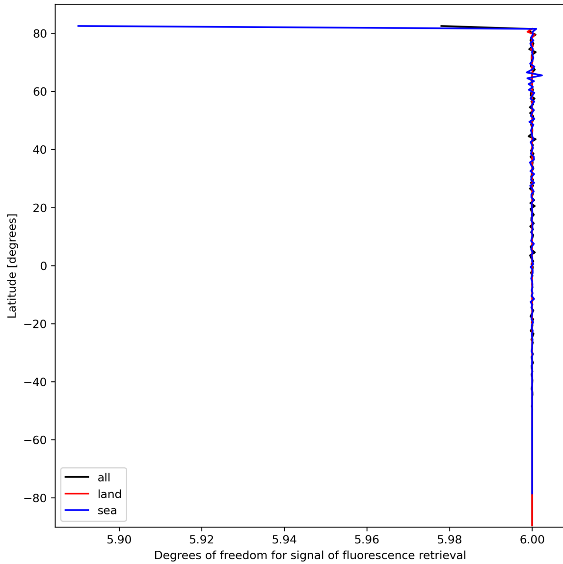
Figure 26: Zonal average of “Degrees of freedom for signal of fluorescence retrieval” for 2024-03-04 to 2024-03-05.
