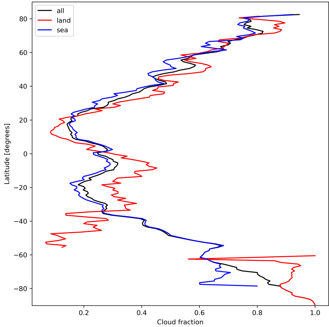
Figure 15: Zonal average of “Cloud fraction” for 2024-03-04 to 2024-03-05.
