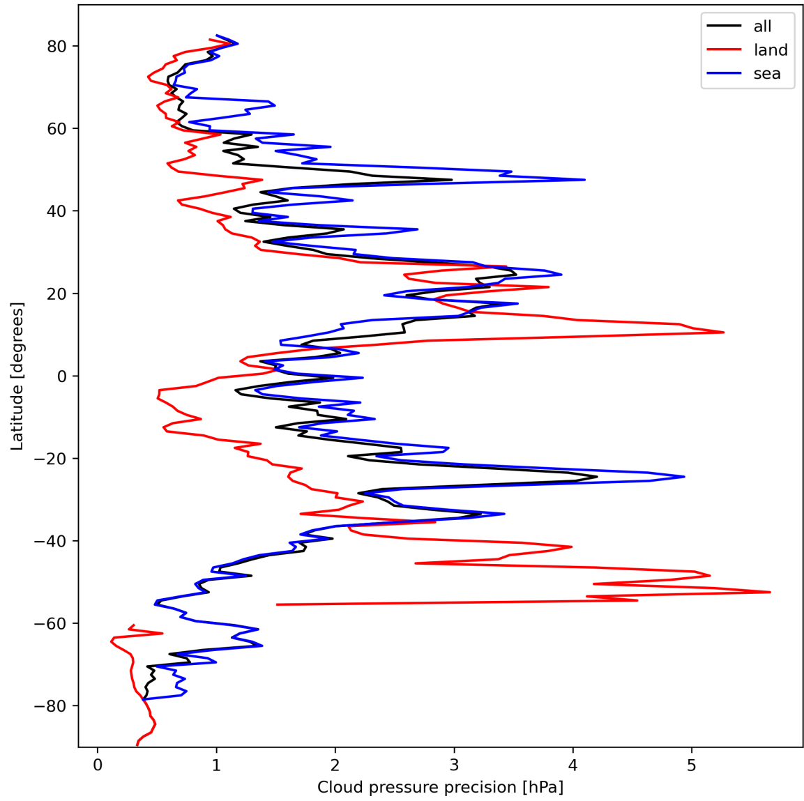
Figure 14: Zonal average of “Cloud pressure precision” for 2024-03-04 to 2024-03-05.
