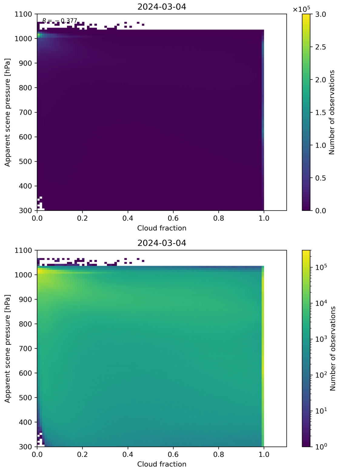
Figure 70: Scatter density plot of “Cloud fraction” against “Apparent scene pressure” for 2024-03-04 to 2024-03-05.
