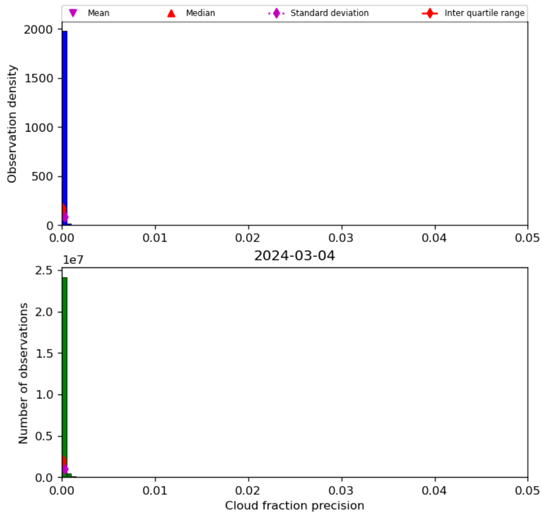
Figure 33: Histogram of “Cloud fraction precision” for 2024-03-04 to 2024-03-05
