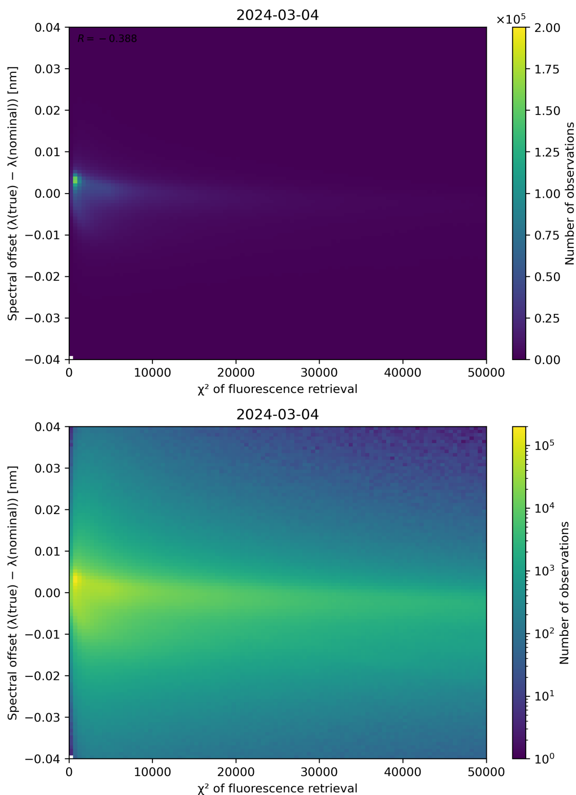
Figure 69: Scatter density plot of " \chi^2 of fluorescence retrieval" against "Spectral offset ( \lambda(\text{true}) - \lambda(\text{nominal}) )" for 2024-03-04 to 2024-03-05.
