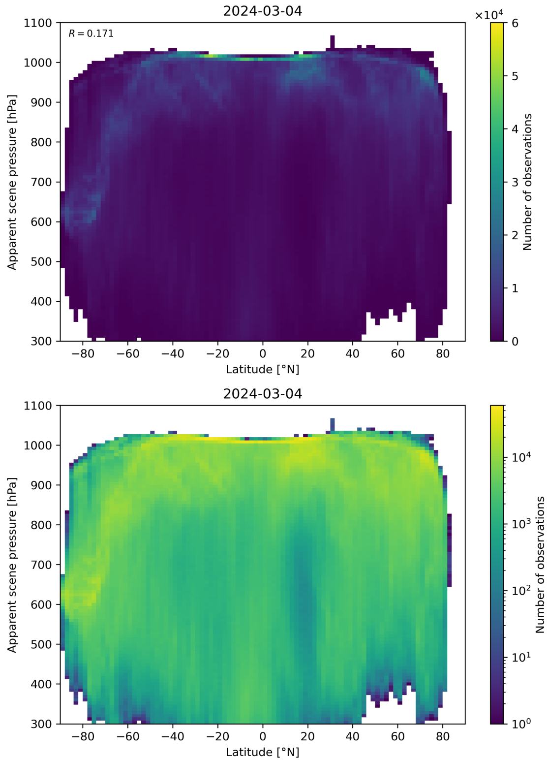
Figure 88: Scatter density plot of “Latitude” against “Apparent scene pressure” for 2024-03-04 to 2024-03-05.
