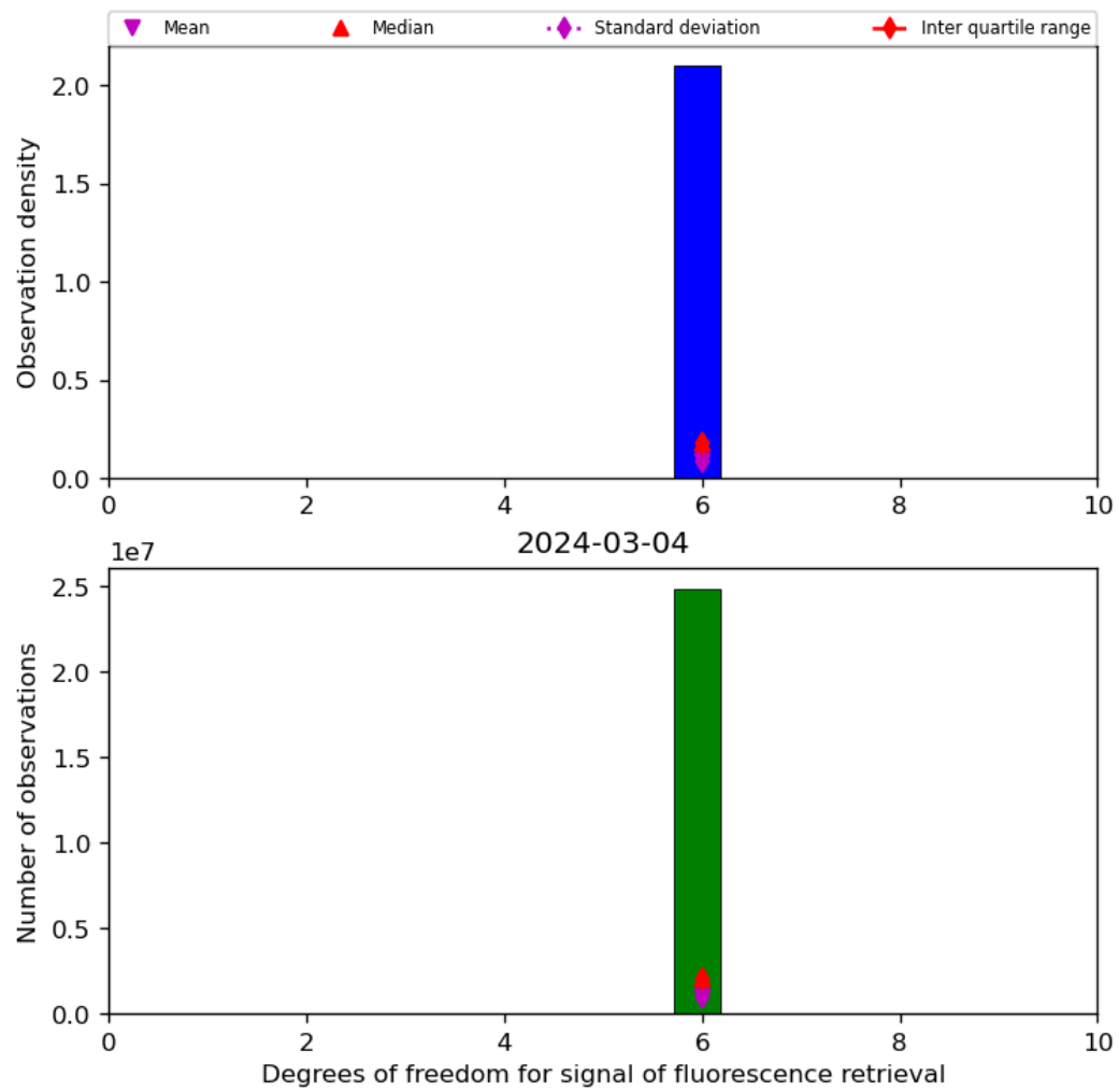
Figure 43: Histogram of “Degrees of freedom for signal of fluorescence retrieval” for 2024-03-04 to 2024-03-05
