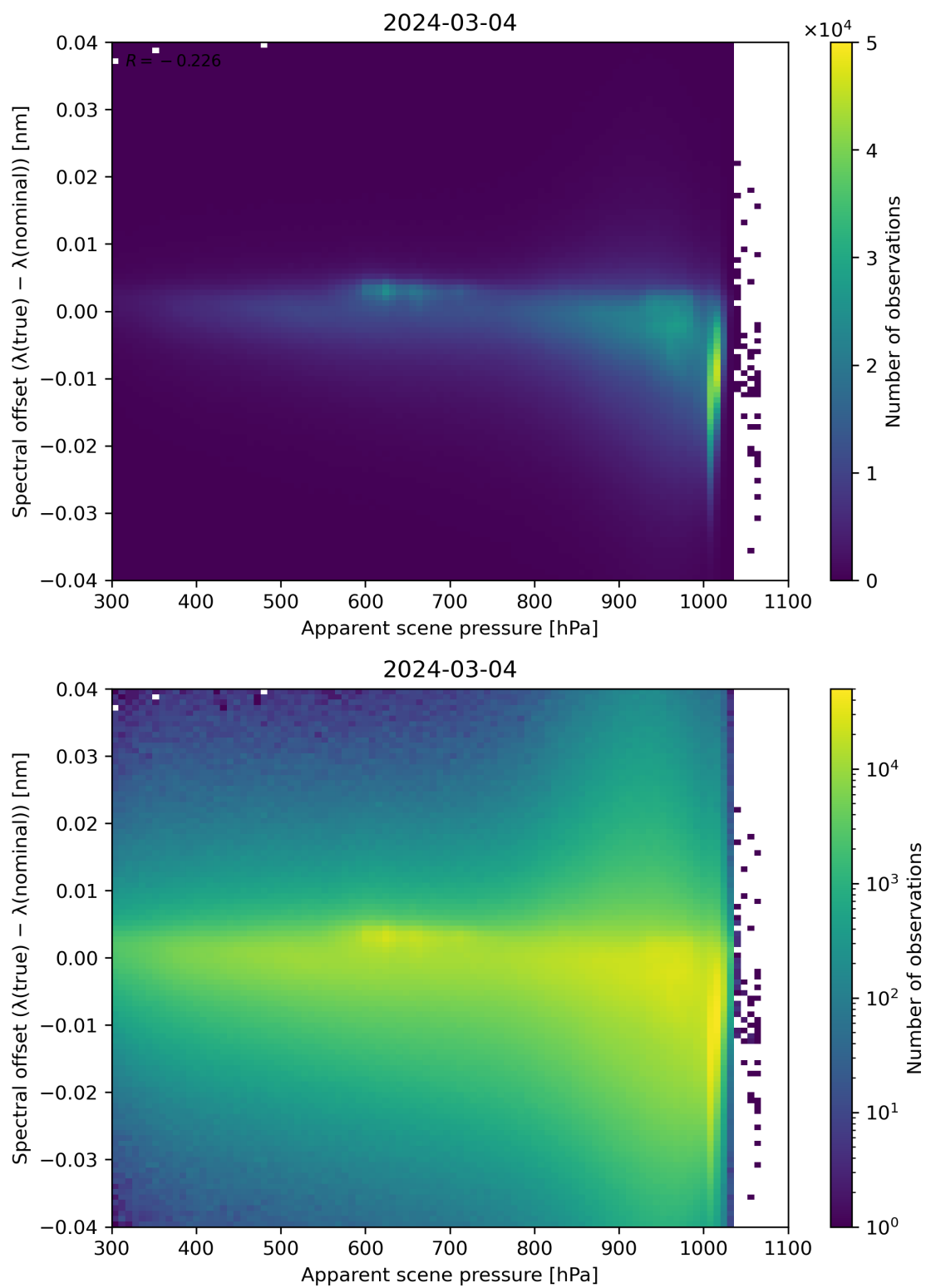
Figure 67: Scatter density plot of “Apparent scene pressure” against “Spectral offset ( \lambda(\text{true}) - \lambda(\text{nominal}) )” for 2024-03-04 to 2024-03-05.
