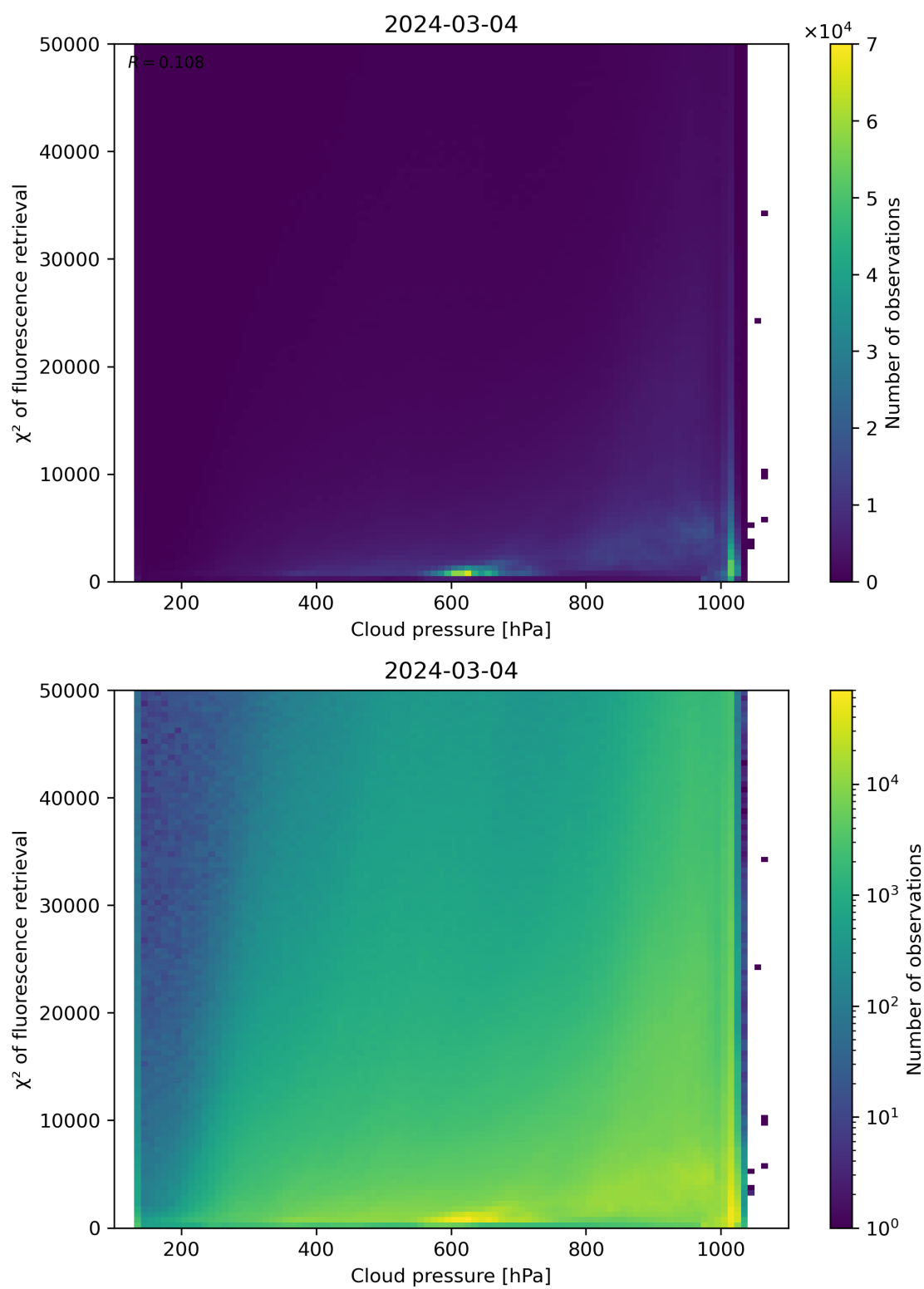
Figure 78: Scatter density plot of “Cloud pressure” against “ \chi^2 of fluorescence retrieval” for 2024-03-04 to 2024-03-05.
