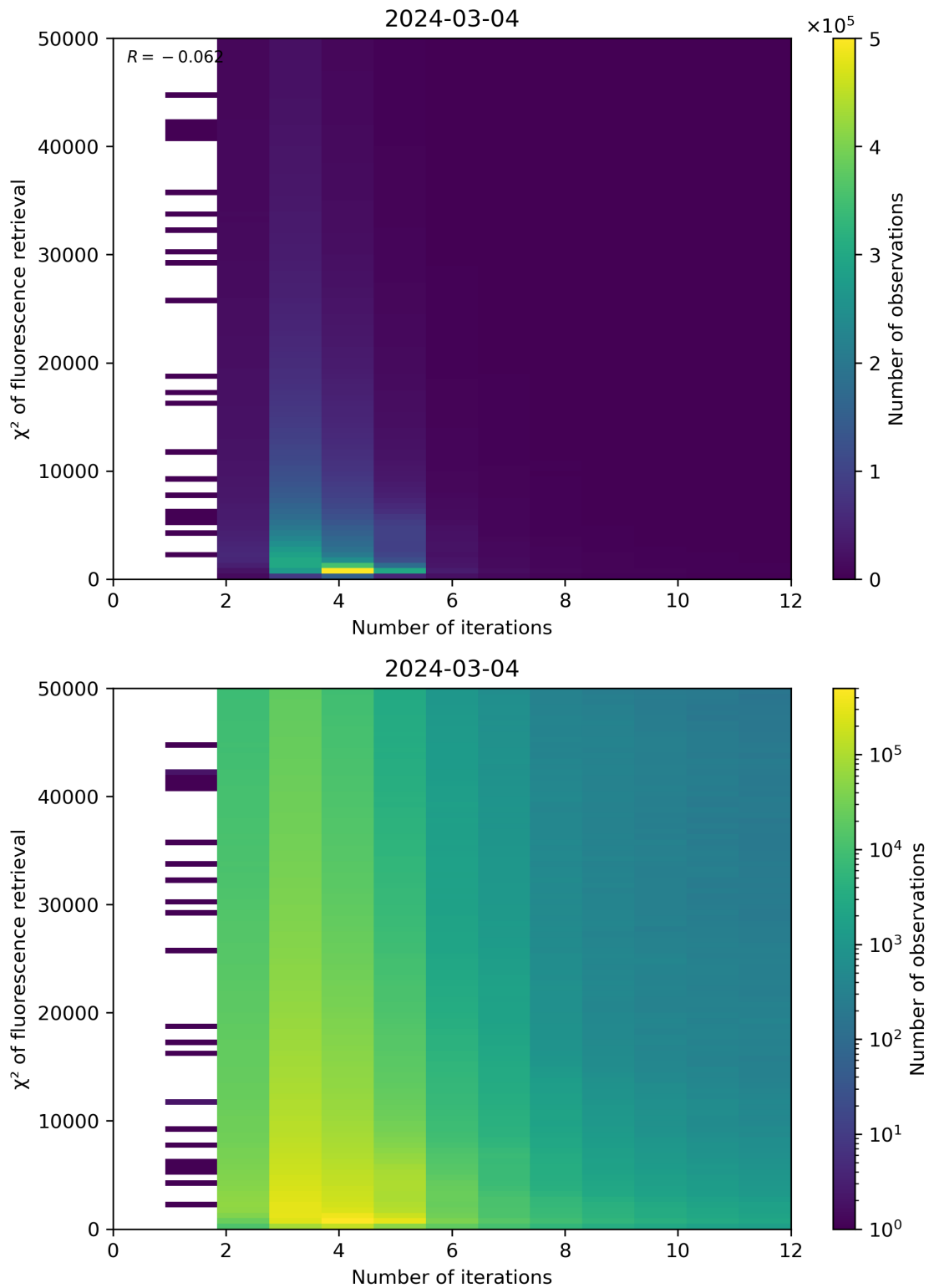
Figure 97: Scatter density plot of “Number of iterations” against “ \chi^2 of fluorescence retrieval” for 2024-03-04 to 2024-03-05.
