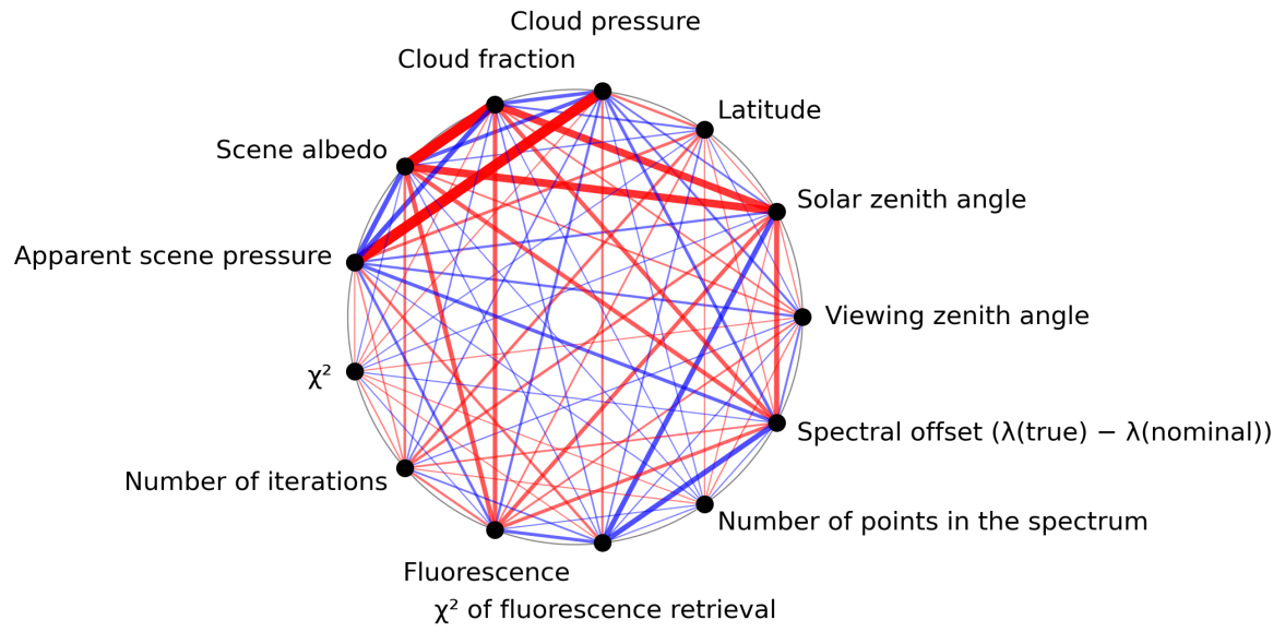
Figure 1: Map of correlation graph for 2024-03-04 to 2024-03-05.
