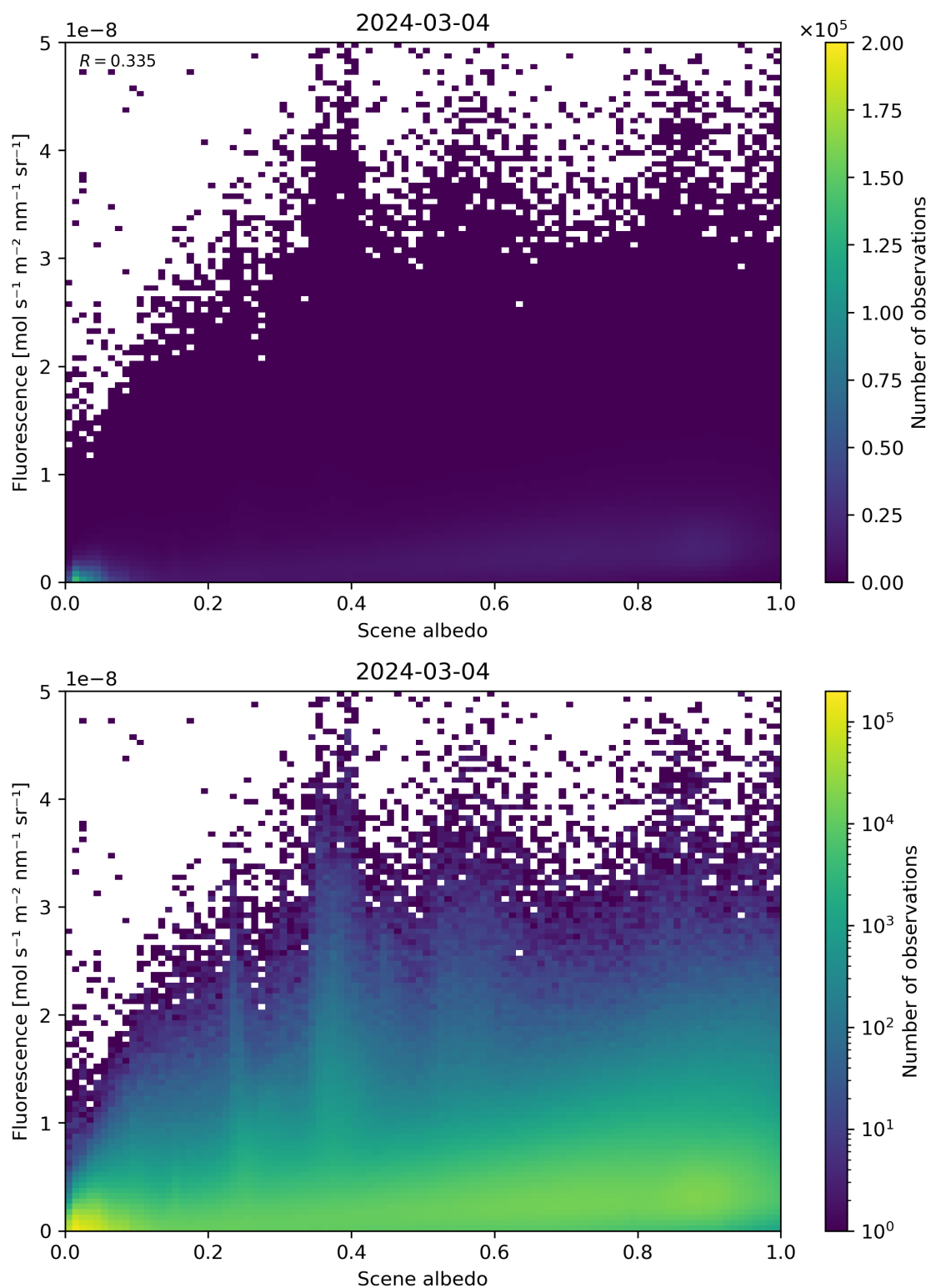
Figure 104: Scatter density plot of “Scene albedo” against “Fluorescence” for 2024-03-04 to 2024-03-05.
