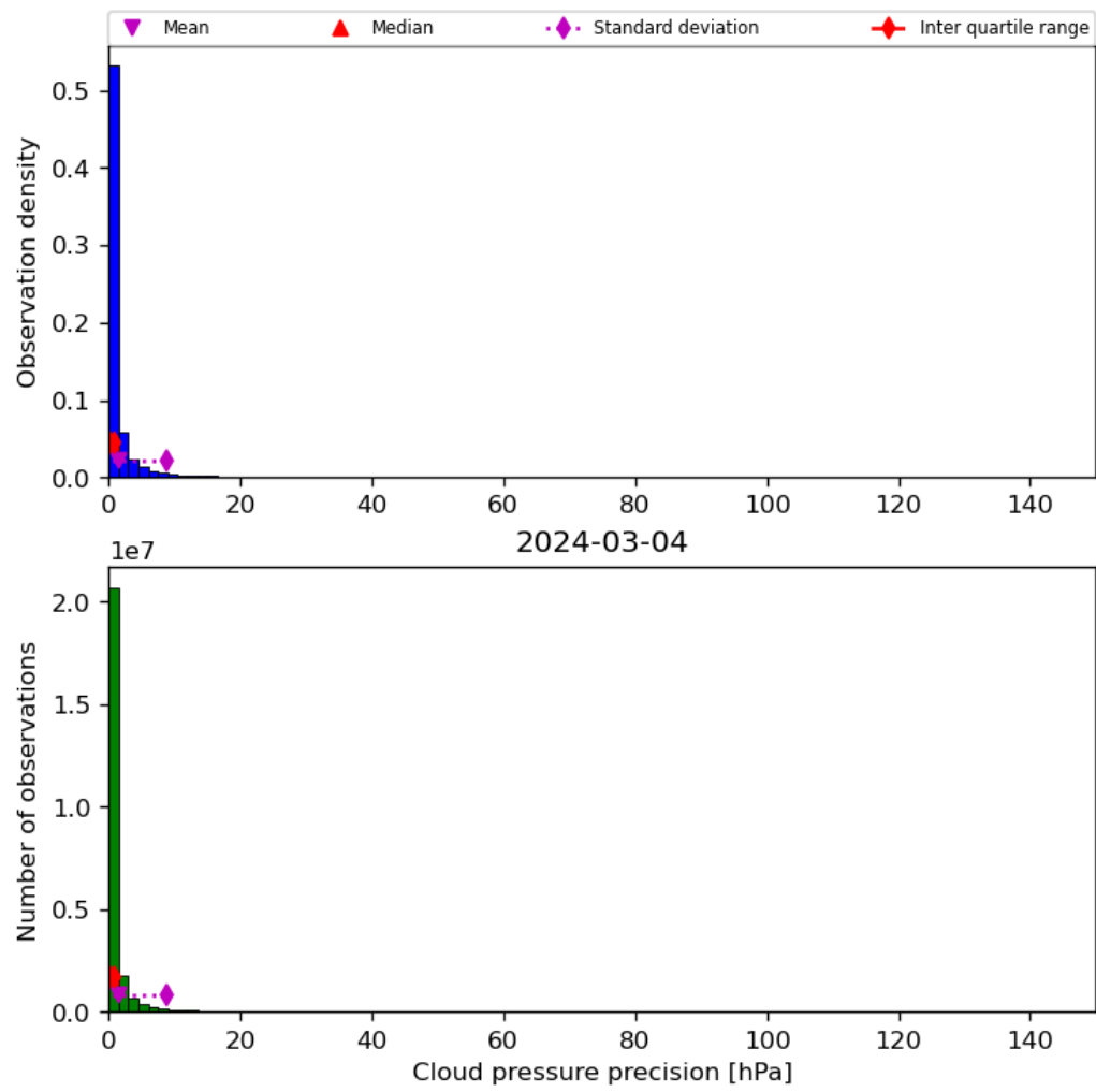
Figure 31: Histogram of “Cloud pressure precision” for 2024-03-04 to 2024-03-05
