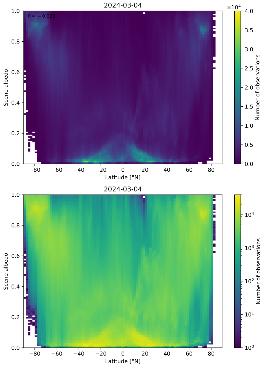
Figure 95: Scatter density plot of “Latitude” against “Scene albedo” for 2024-03-04 to 2024-03-05.
