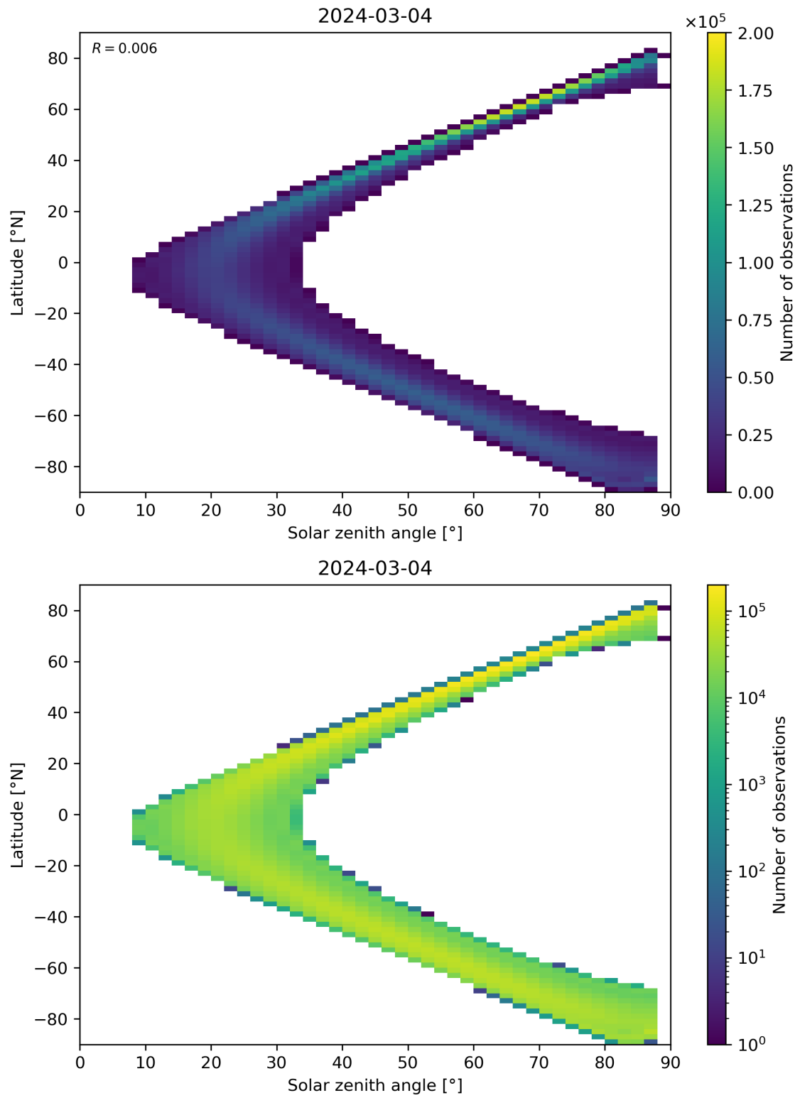
Figure 113: Scatter density plot of “Solar zenith angle” against “Latitude” for 2024-03-04 to 2024-03-05.
