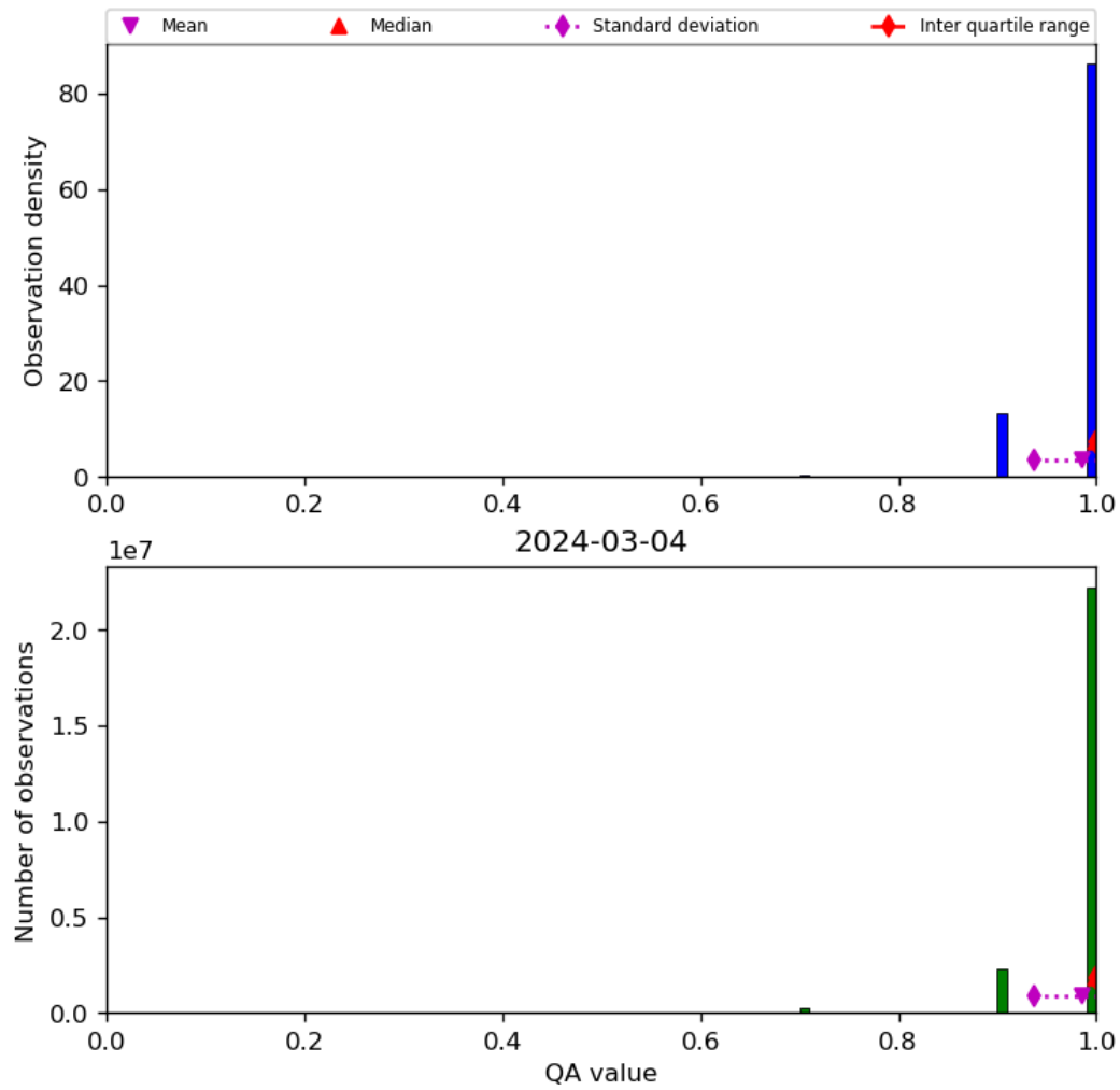
Figure 29: Histogram of “QA value” for 2024-03-04 to 2024-03-05
