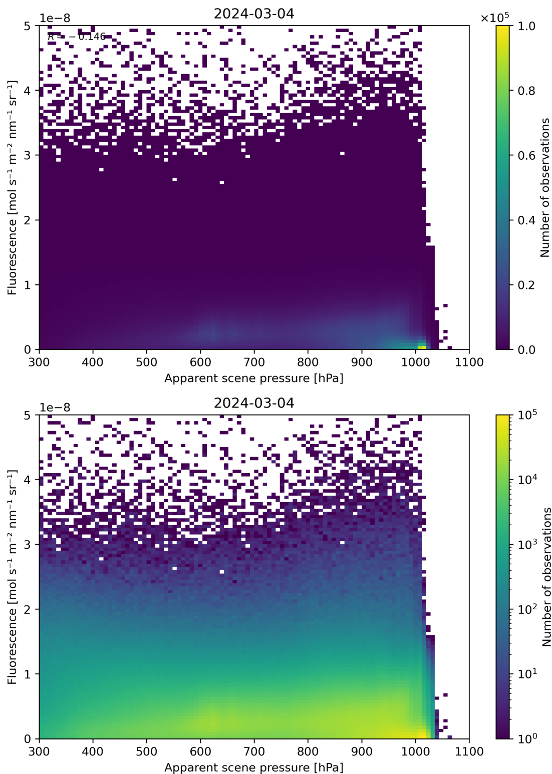
Figure 64: Scatter density plot of “Apparent scene pressure” against “Fluorescence” for 2024-03-04 to 2024-03-05.
