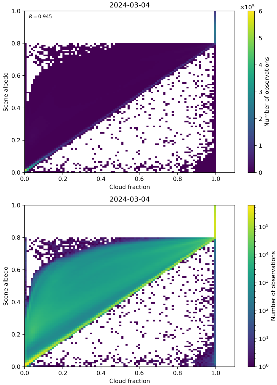
Figure 75: Scatter density plot of “Cloud fraction” against “Scene albedo” for 2024-03-04 to 2024-03-05.
