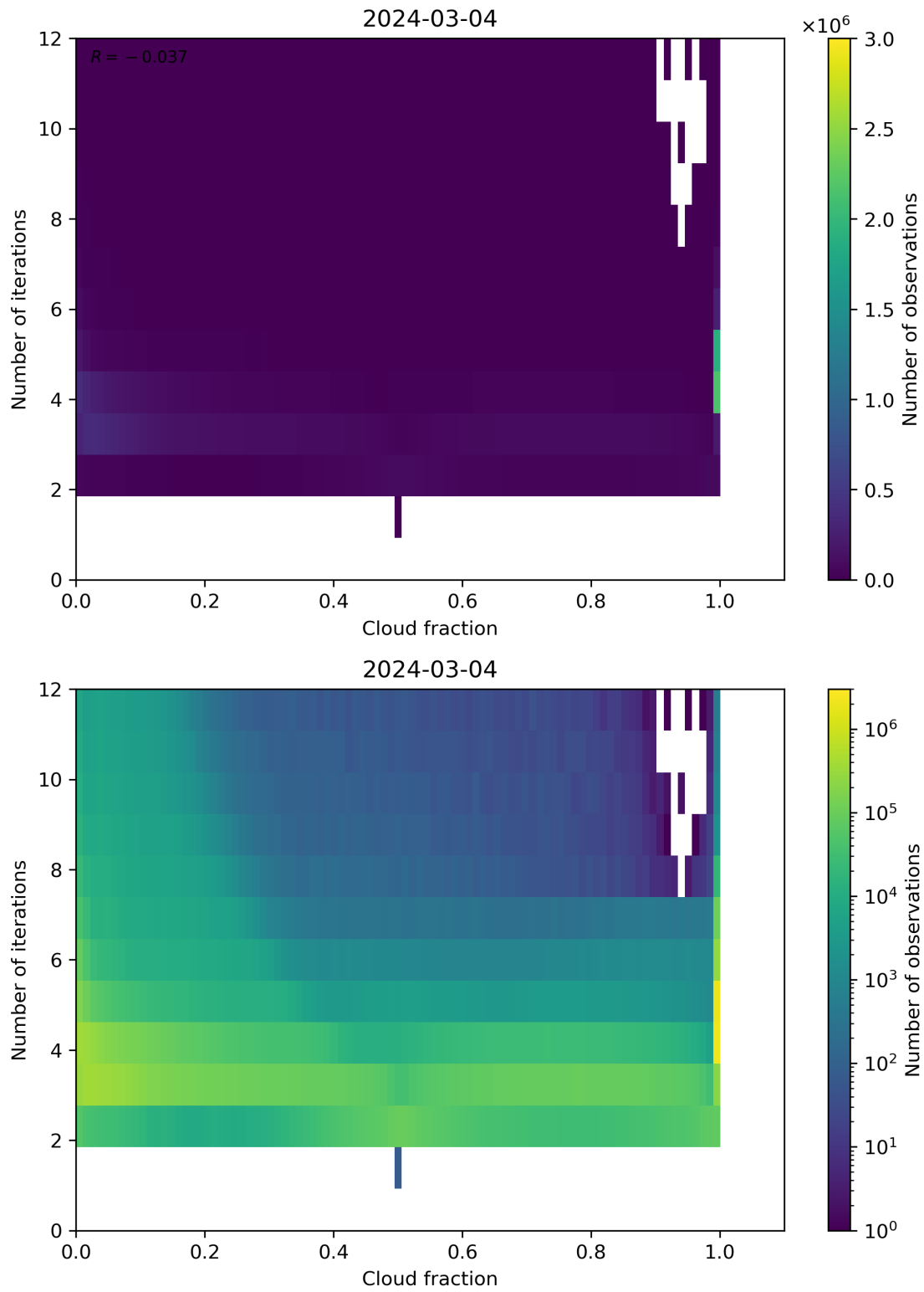
Figure 73: Scatter density plot of “Cloud fraction” against “Number of iterations” for 2024-03-04 to 2024-03-05.
