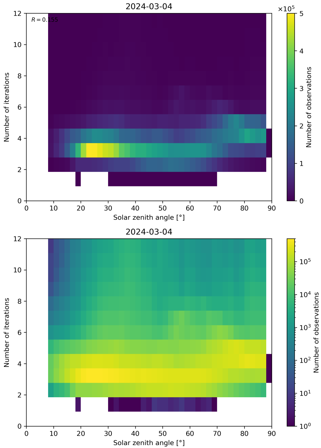
Figure 114: Scatter density plot of “Solar zenith angle” against “Number of iterations” for 2024-03-04 to 2024-03-05.
