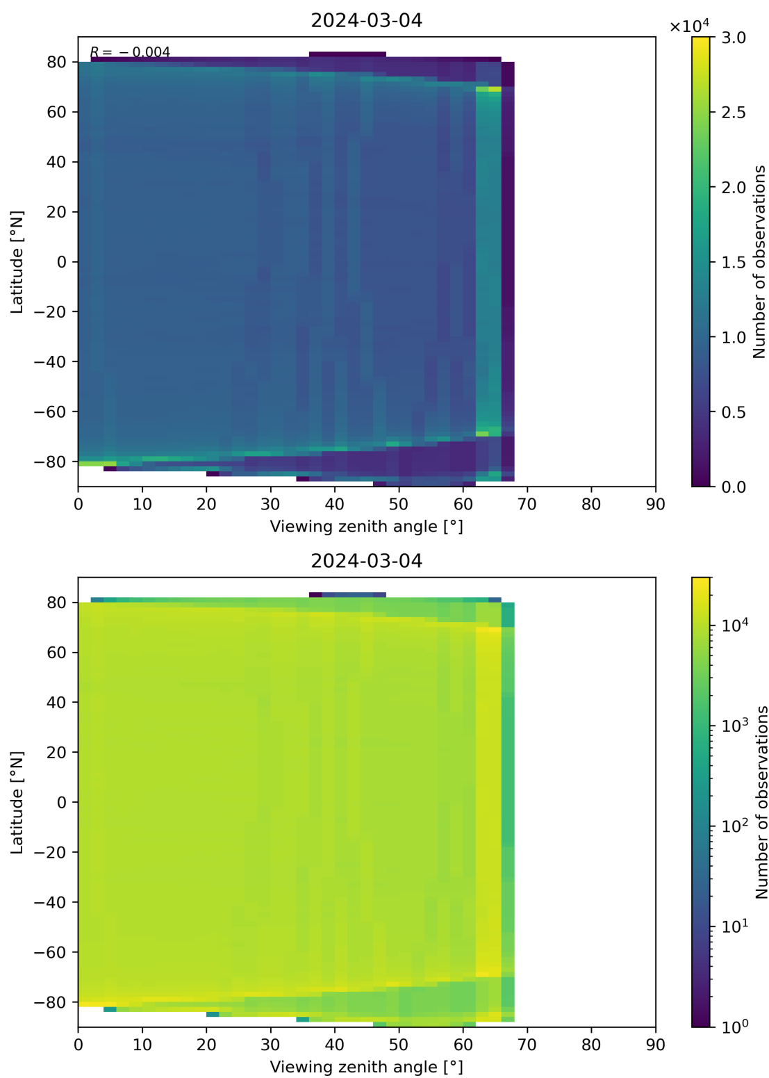
Figure 123: Scatter density plot of “Viewing zenith angle” against “Latitude” for 2024-03-04 to 2024-03-05.
