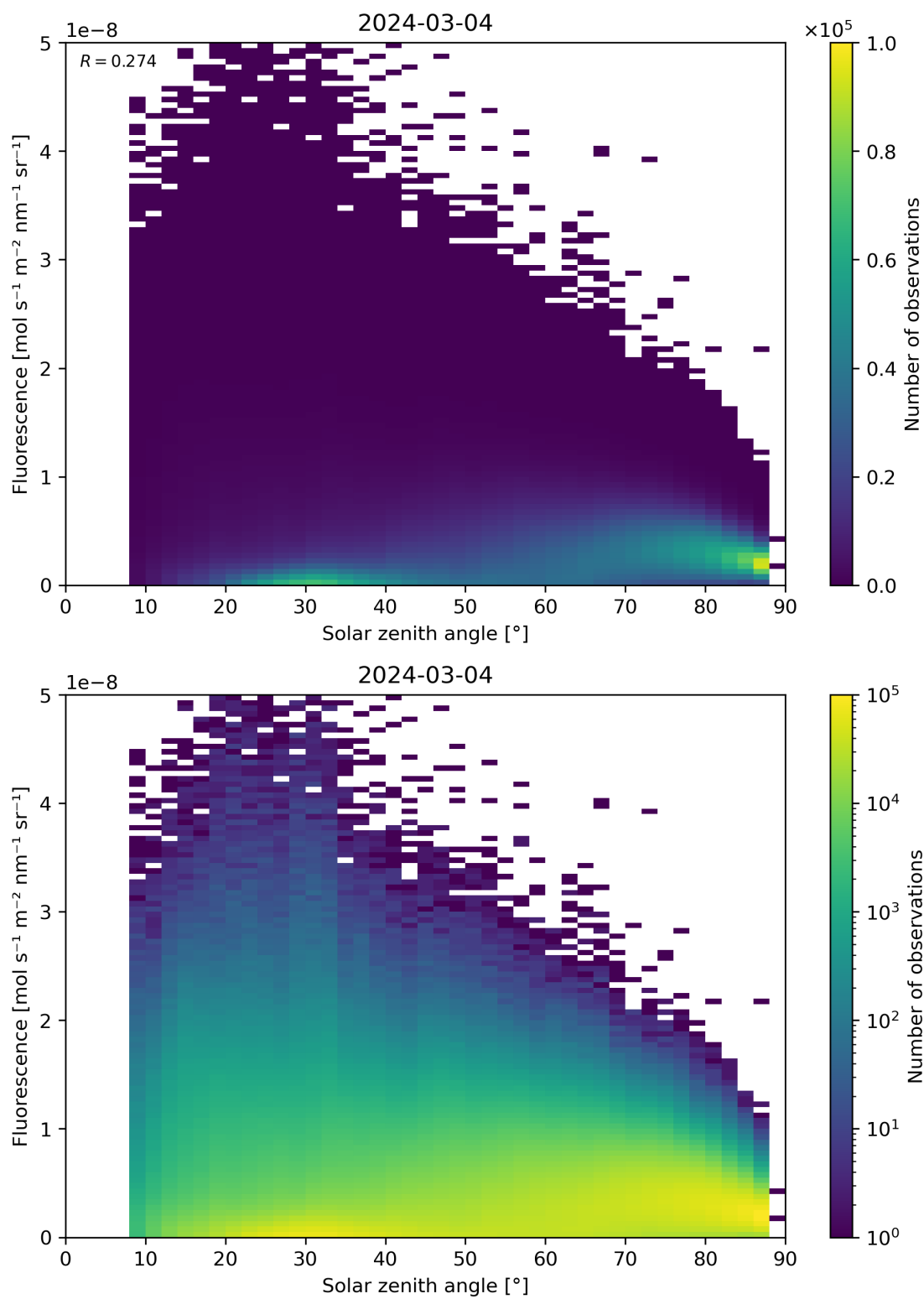
Figure 112: Scatter density plot of “Solar zenith angle” against “Fluorescence” for 2024-03-04 to 2024-03-05.
