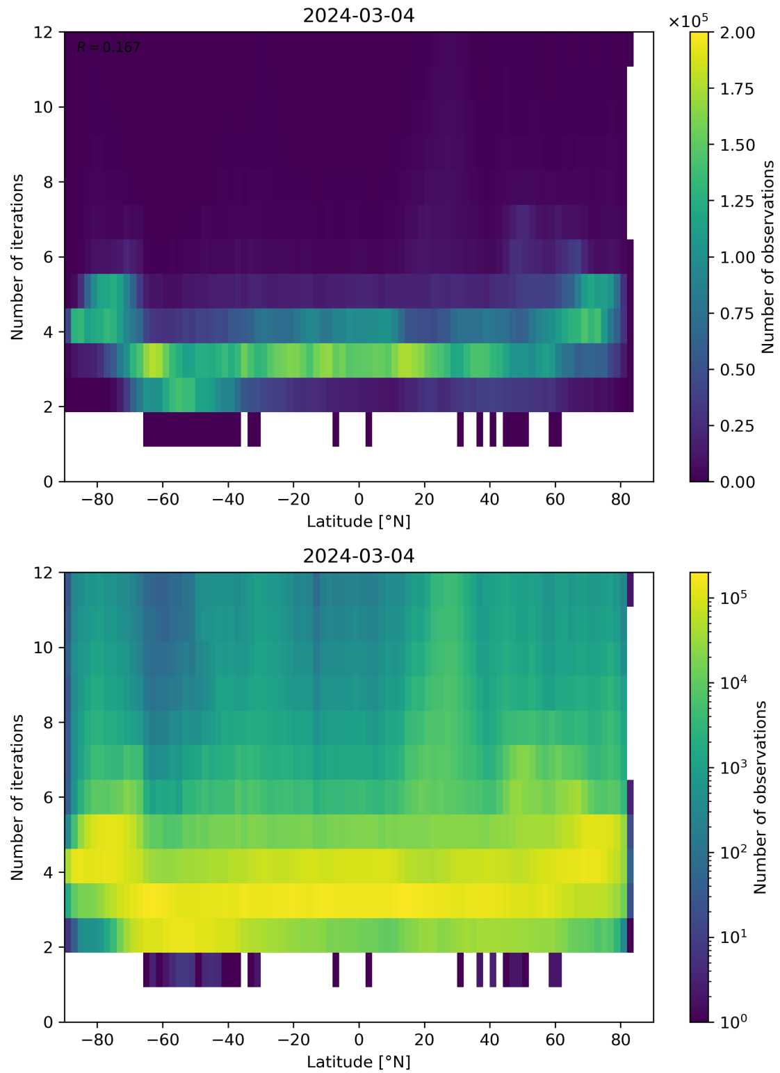
Figure 93: Scatter density plot of “Latitude” against “Number of iterations” for 2024-03-04 to 2024-03-05.
