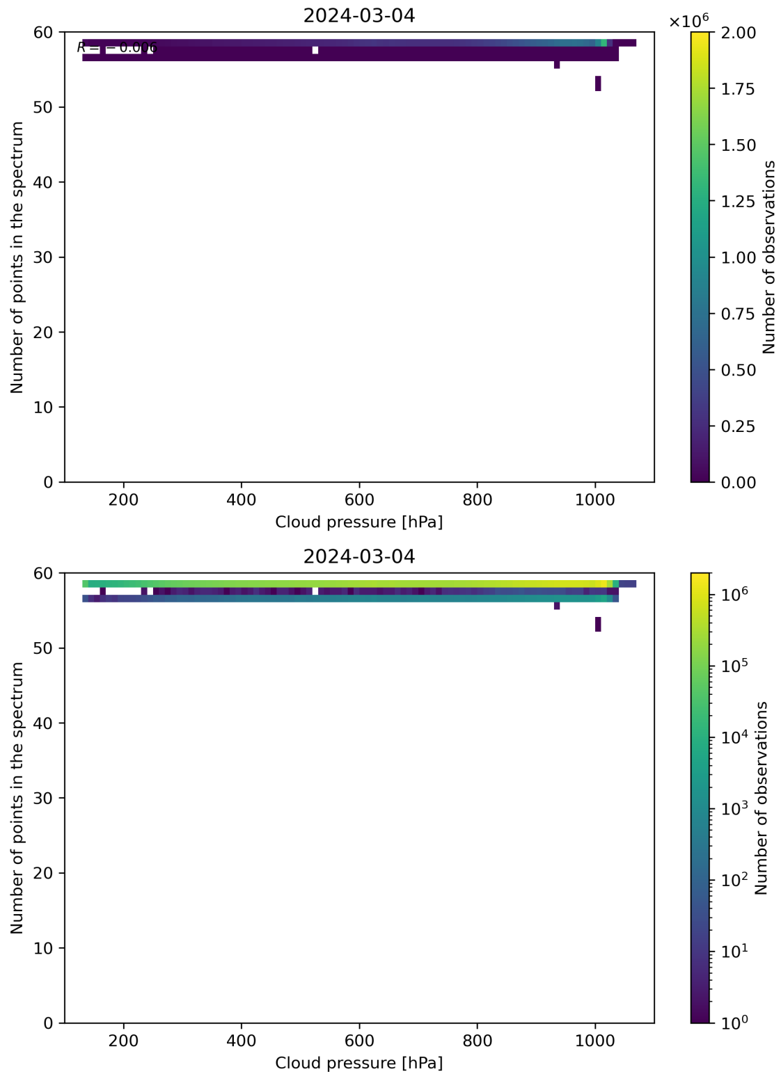
Figure 82: Scatter density plot of “Cloud pressure” against “Number of points in the spectrum” for 2024-03-04 to 2024-03-05.
