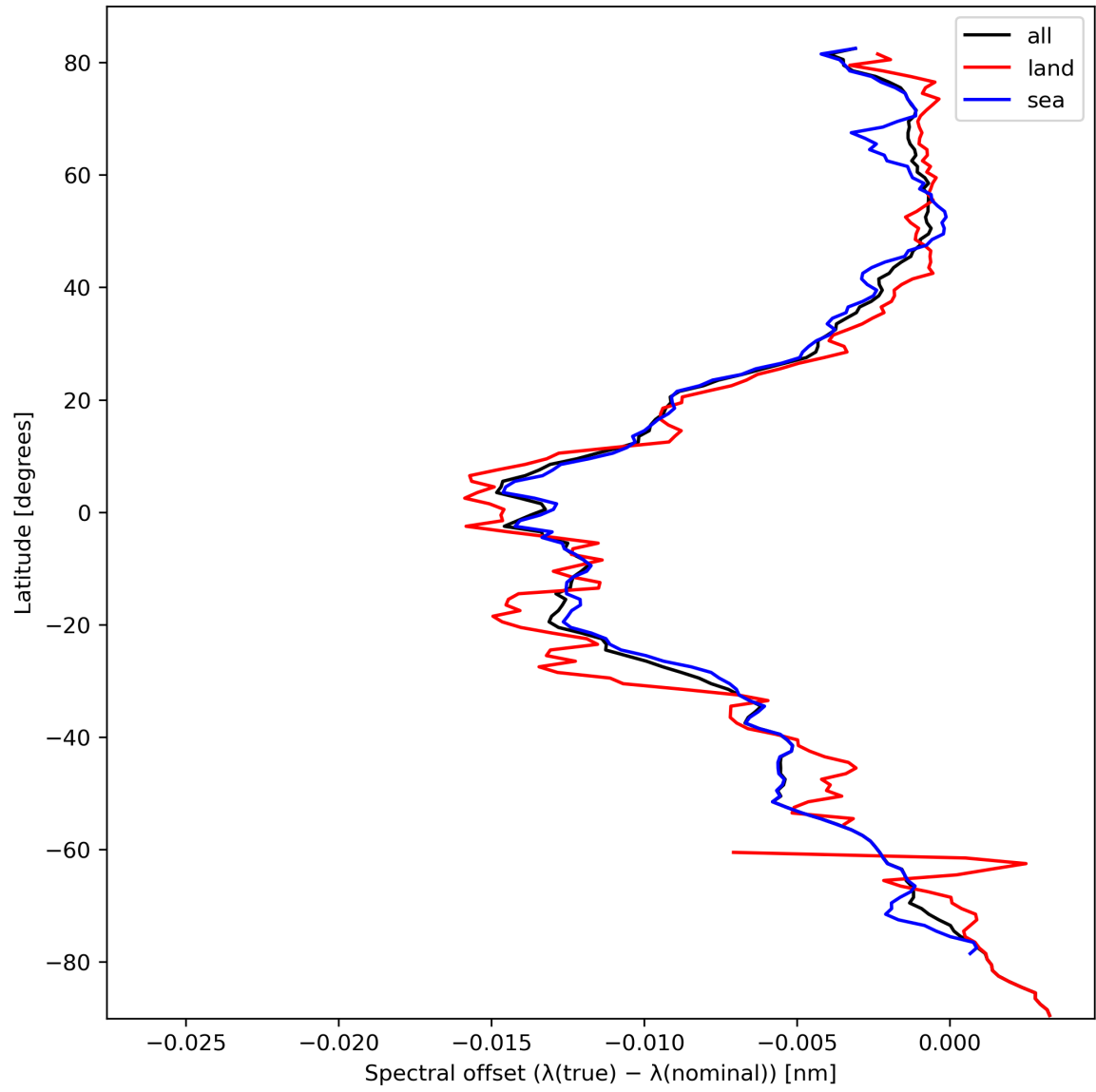
Figure 28: Zonal average of “Spectral offset ( \lambda(\text{true}) - \lambda(\text{nominal}) )” for 2024-03-04 to 2024-03-05.
