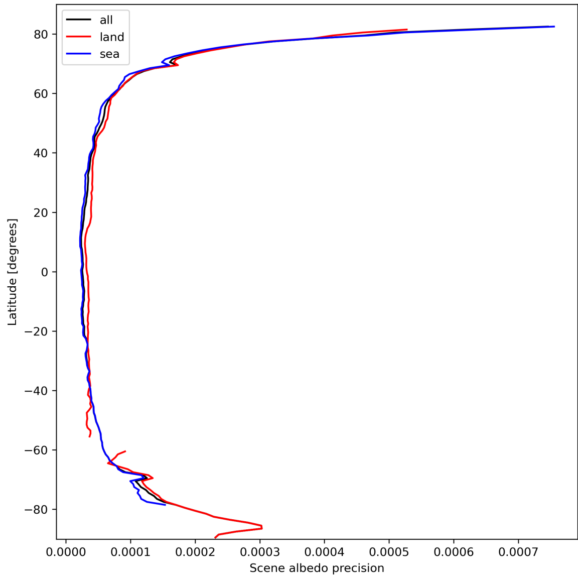
Figure 18: Zonal average of “Scene albedo precision” for 2024-03-04 to 2024-03-05.
