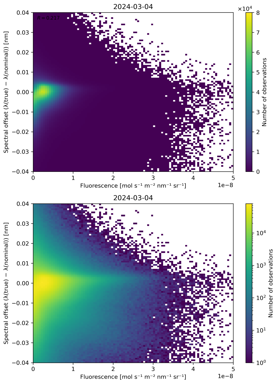
Figure 87: Scatter density plot of “Fluorescence” against “Spectral offset ( \lambda(\text{true}) - \lambda(\text{nominal}) )” for 2024-03-04 to 2024-03-05.
