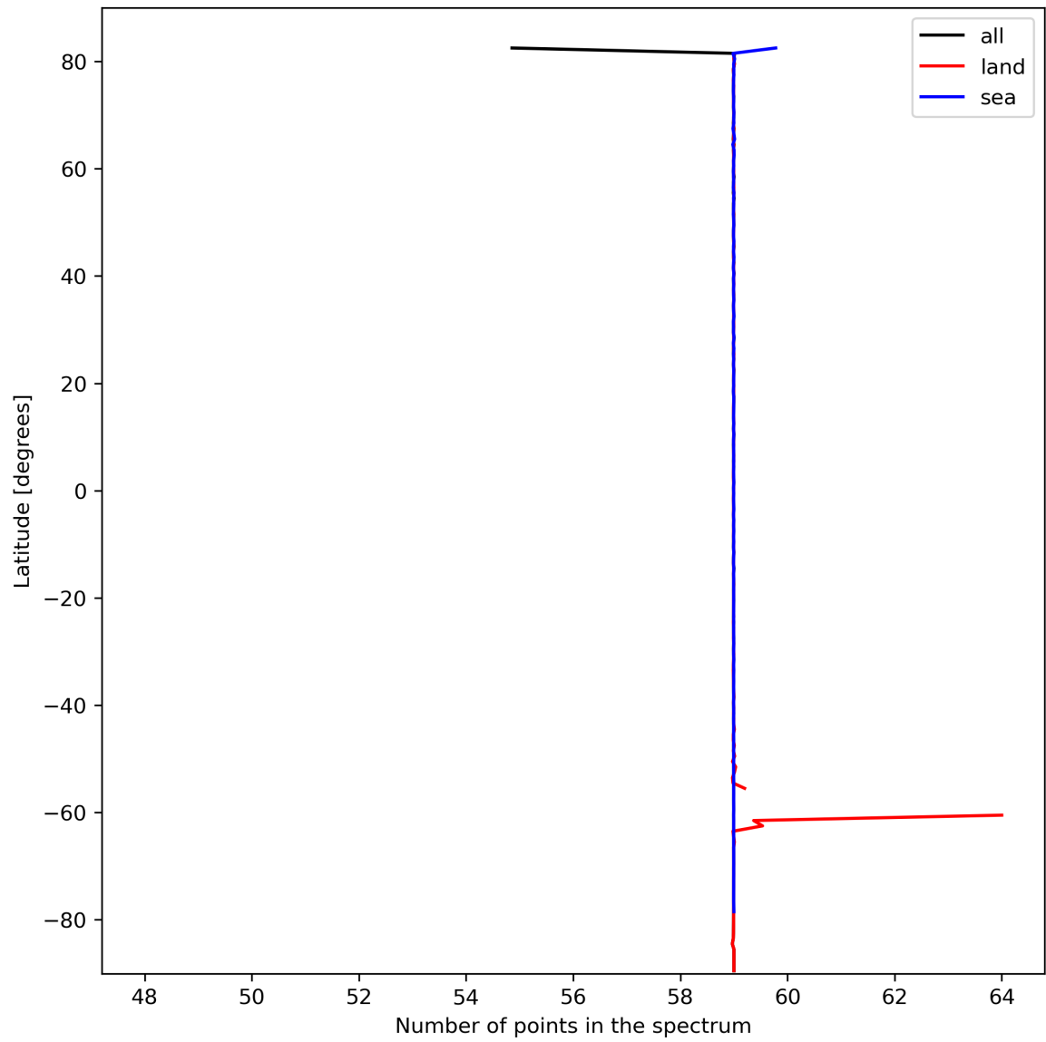
Figure 27: Zonal average of “Number of points in the spectrum” for 2024-03-04 to 2024-03-05.
