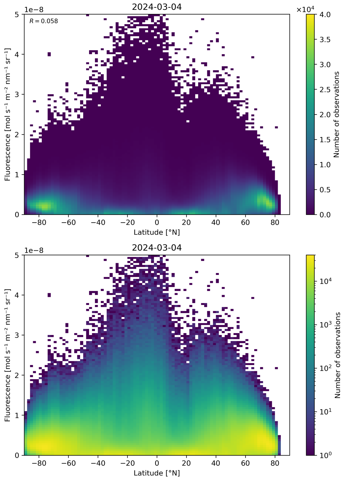
Figure 92: Scatter density plot of “Latitude” against “Fluorescence” for 2024-03-04 to 2024-03-05.
