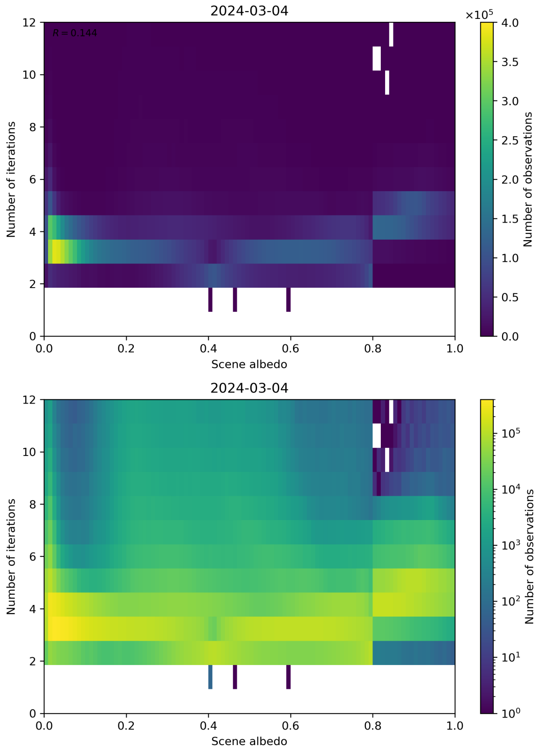
Figure 105: Scatter density plot of “Scene albedo” against “Number of iterations” for 2024-03-04 to 2024-03-05.
