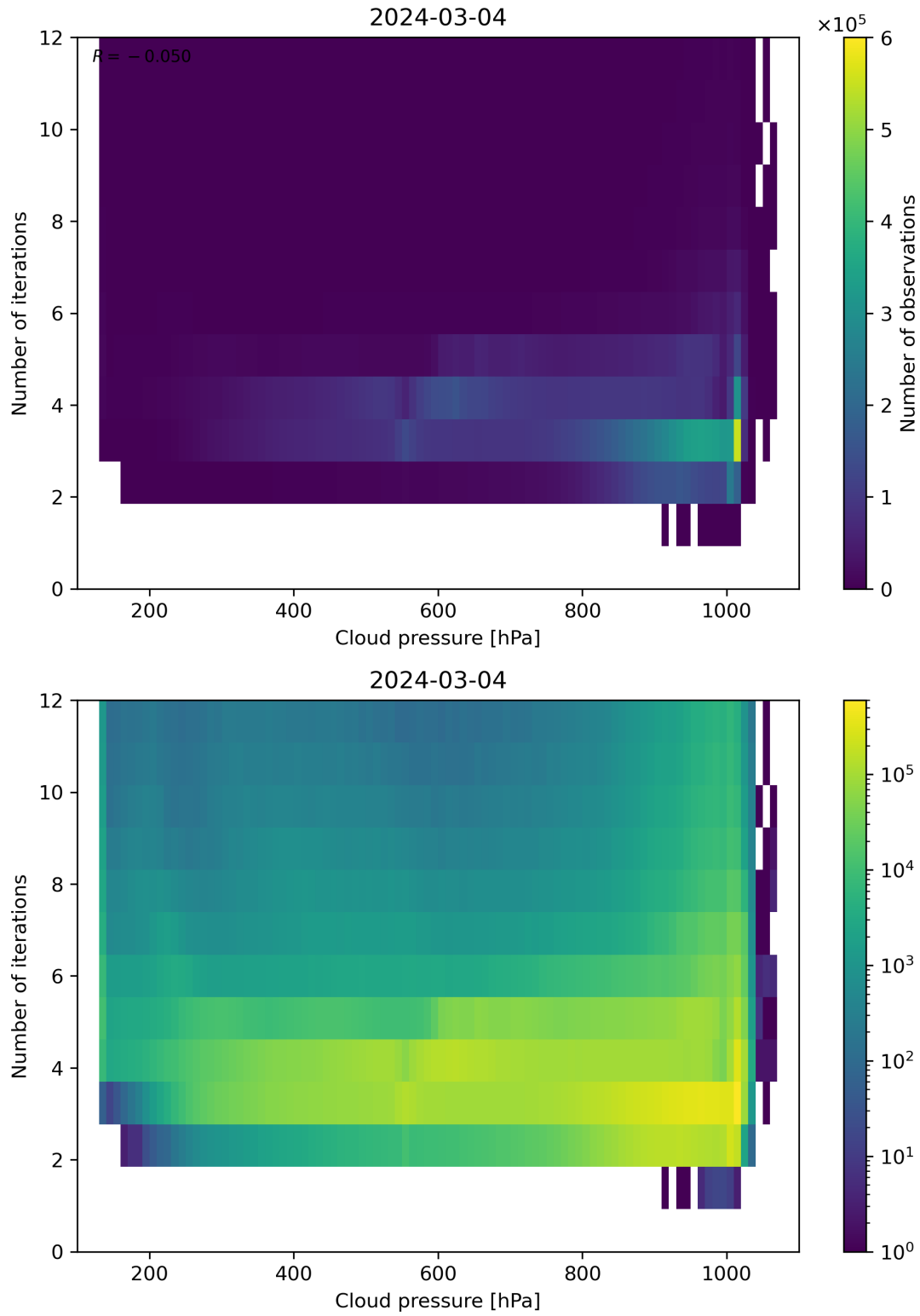
Figure 81: Scatter density plot of “Cloud pressure” against “Number of iterations” for 2024-03-04 to 2024-03-05.
