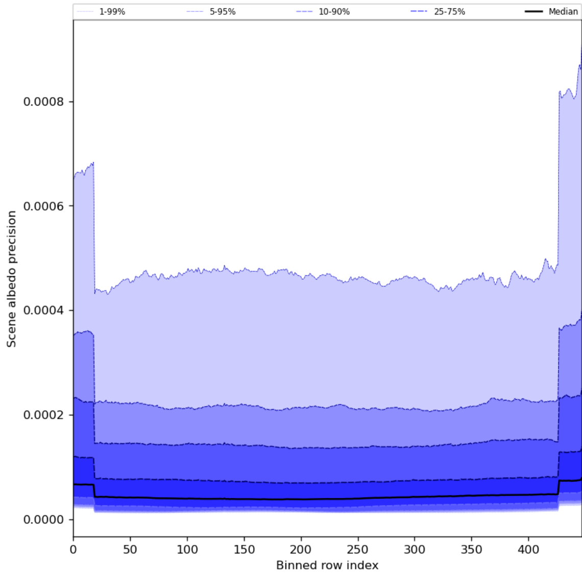
Figure 52: Along track statistics of “Scene albedo precision” for 2024-03-04 to 2024-03-05
