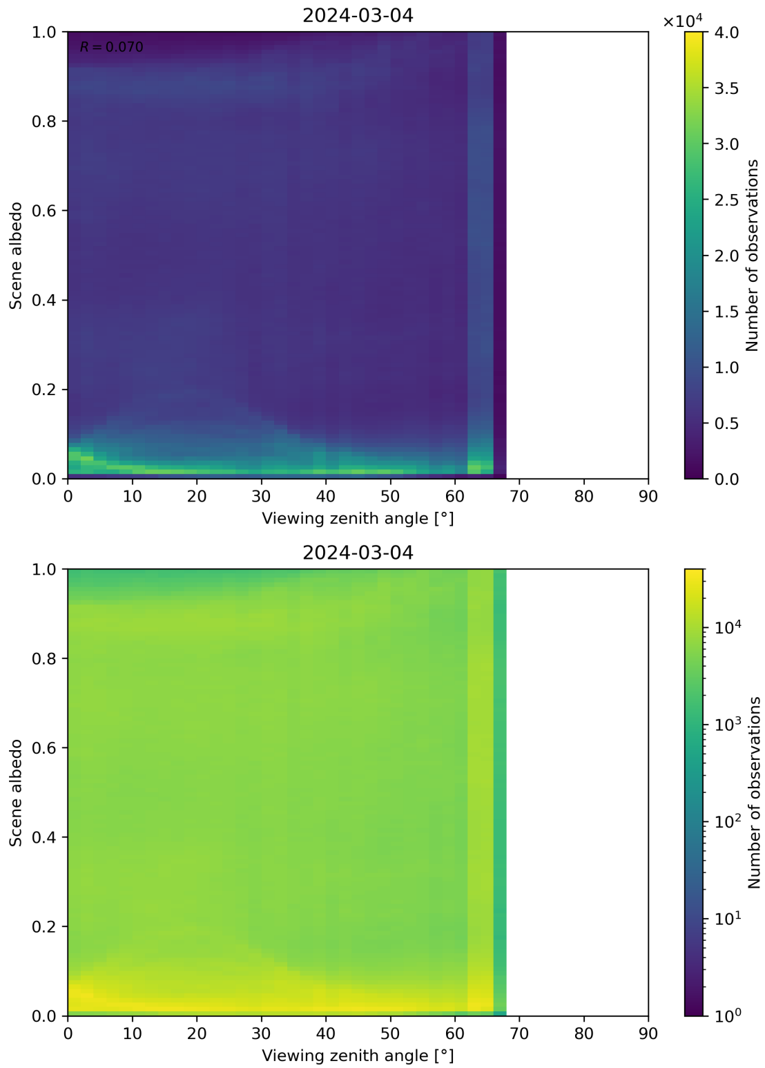
Figure 126: Scatter density plot of “Viewing zenith angle” against “Scene albedo” for 2024-03-04 to 2024-03-05.
