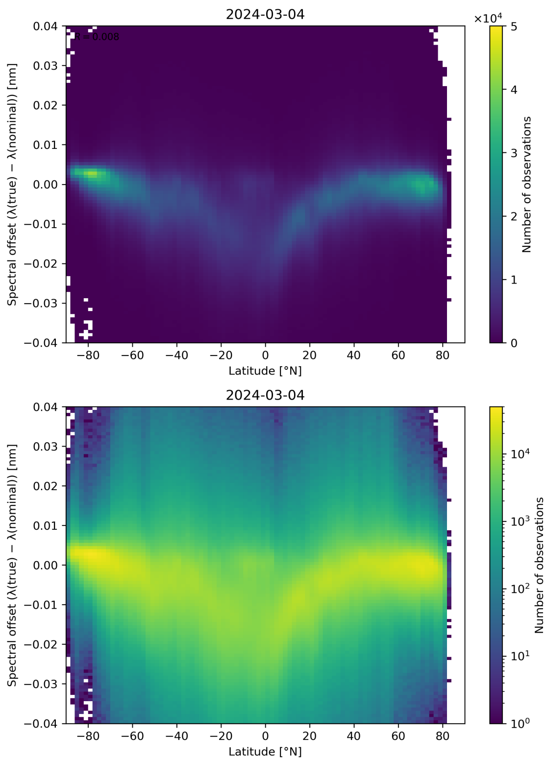
Figure 96: Scatter density plot of “Latitude” against “Spectral offset ( \lambda(\text{true}) - \lambda(\text{nominal}) )” for 2024-03-04 to 2024-03-05.
