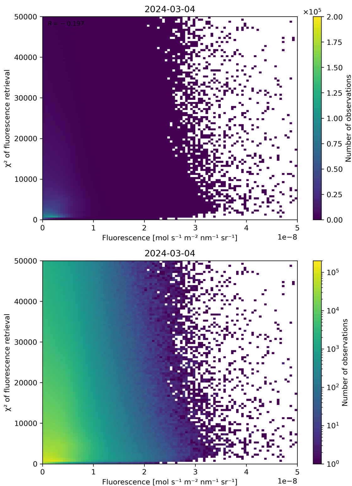
Figure 85: Scatter density plot of “Fluorescence” against “ \chi^2 of fluorescence retrieval” for 2024-03-04 to 2024-03-05.
