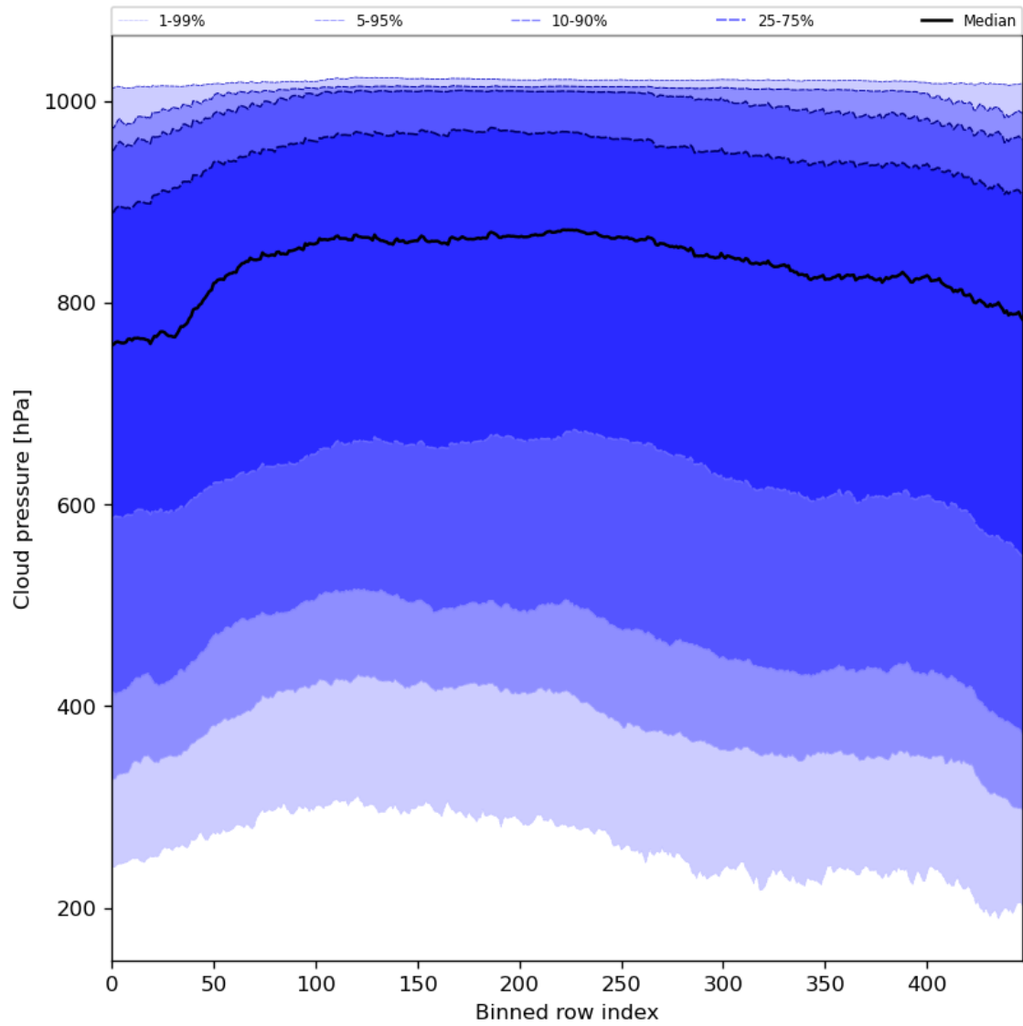
Figure 47: Along track statistics of “Cloud pressure” for 2024-03-04 to 2024-03-05
