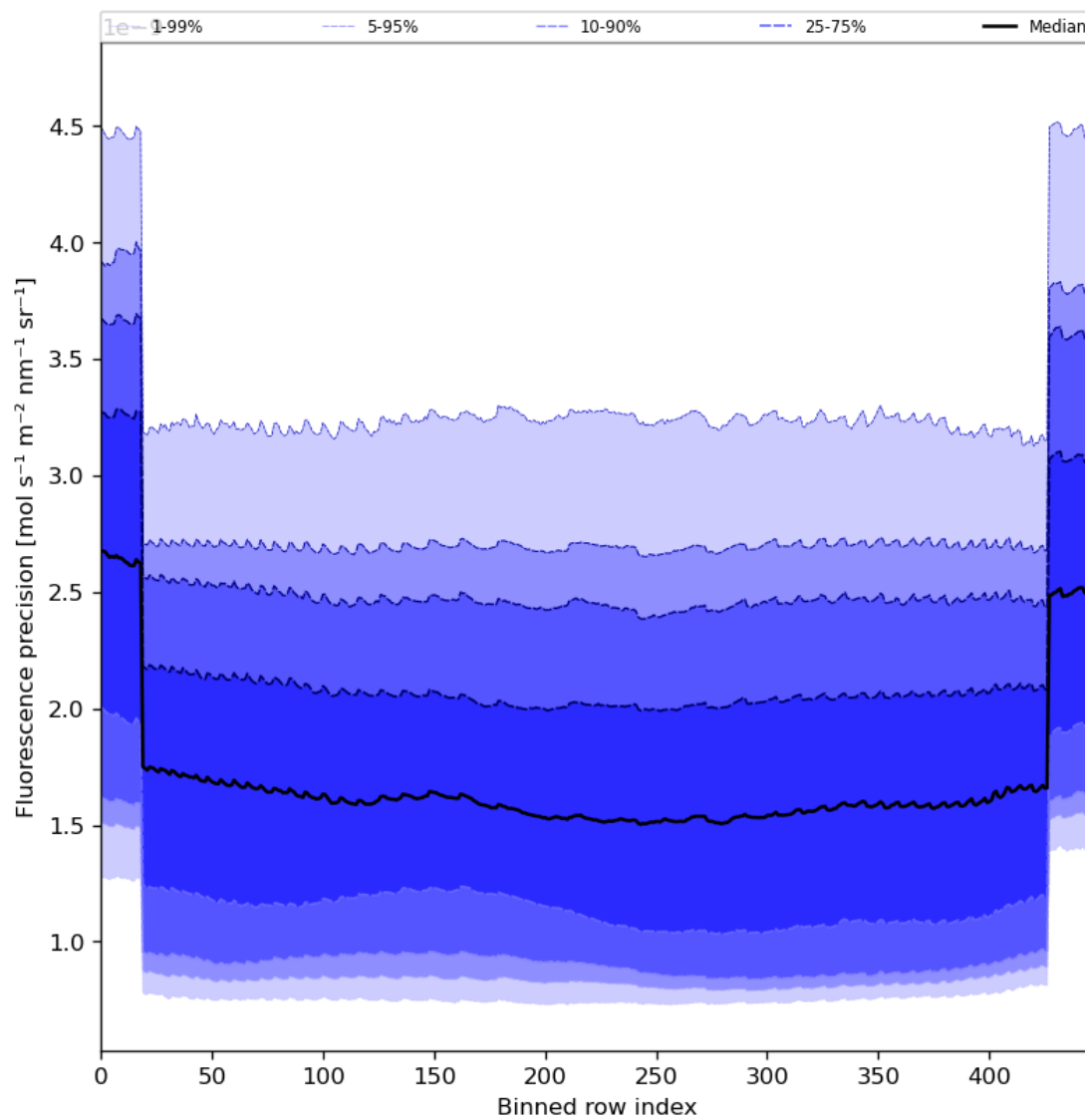
Figure 58: Along track statistics of “Fluorescence precision” for 2024-03-04 to 2024-03-05
