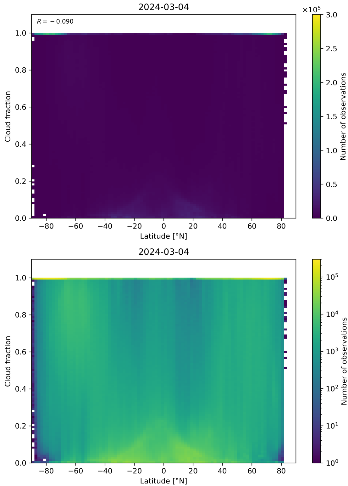
Figure 90: Scatter density plot of “Latitude” against “Cloud fraction” for 2024-03-04 to 2024-03-05.
