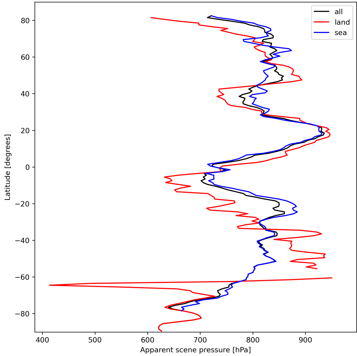
Figure 19: Zonal average of “Apparent scene pressure” for 2024-03-04 to 2024-03-05.
