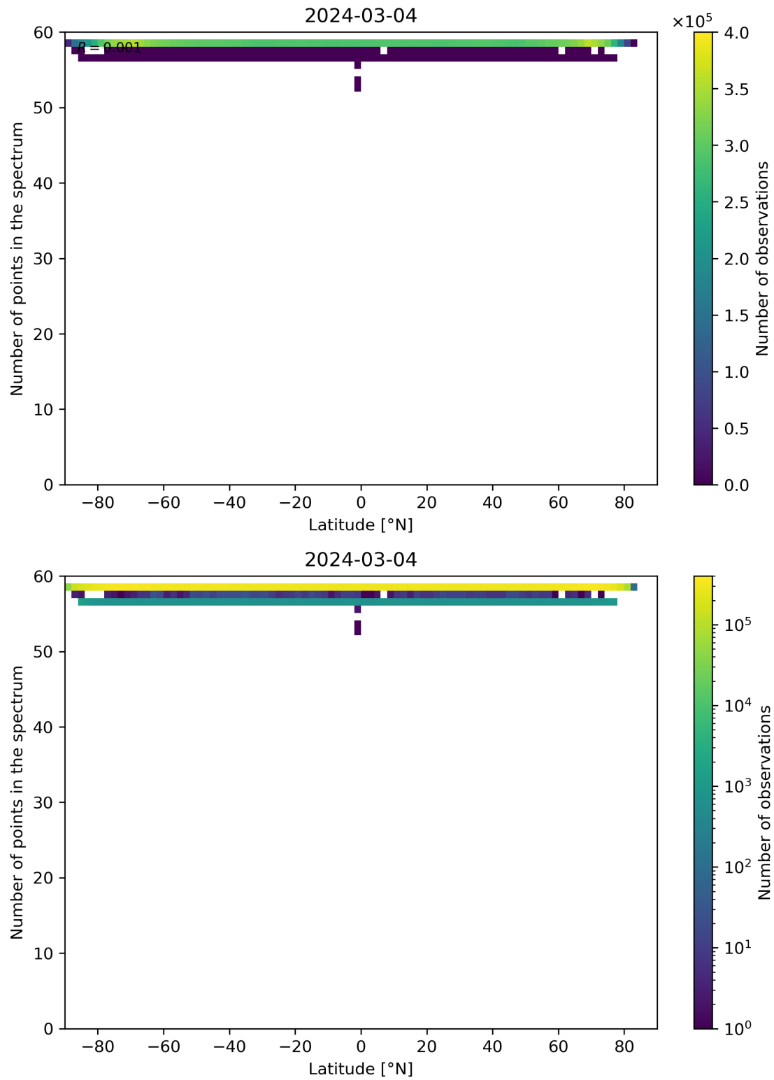
Figure 94: Scatter density plot of “Latitude” against “Number of points in the spectrum” for 2024-03-04 to 2024-03-05.
