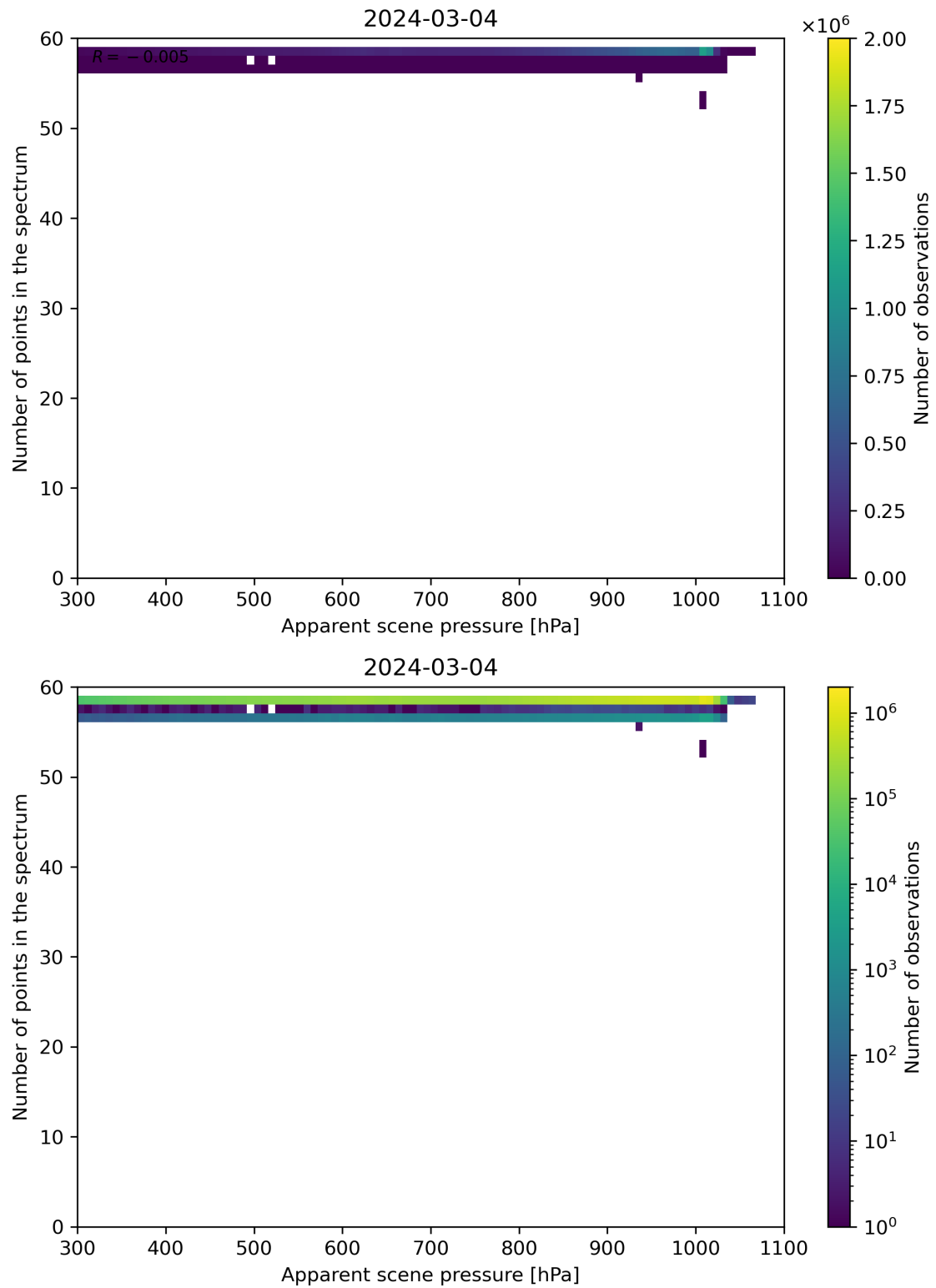
Figure 66: Scatter density plot of “Apparent scene pressure” against “Number of points in the spectrum” for 2024-03-04 to 2024-03-05.
