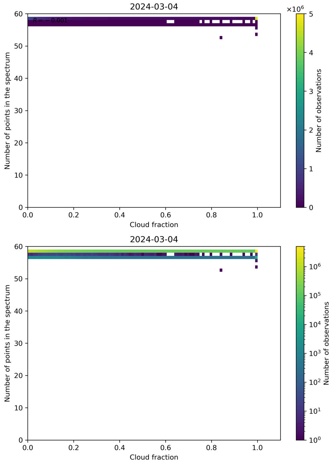
Figure 74: Scatter density plot of “Cloud fraction” against “Number of points in the spectrum” for 2024-03-04 to 2024-03-05.
