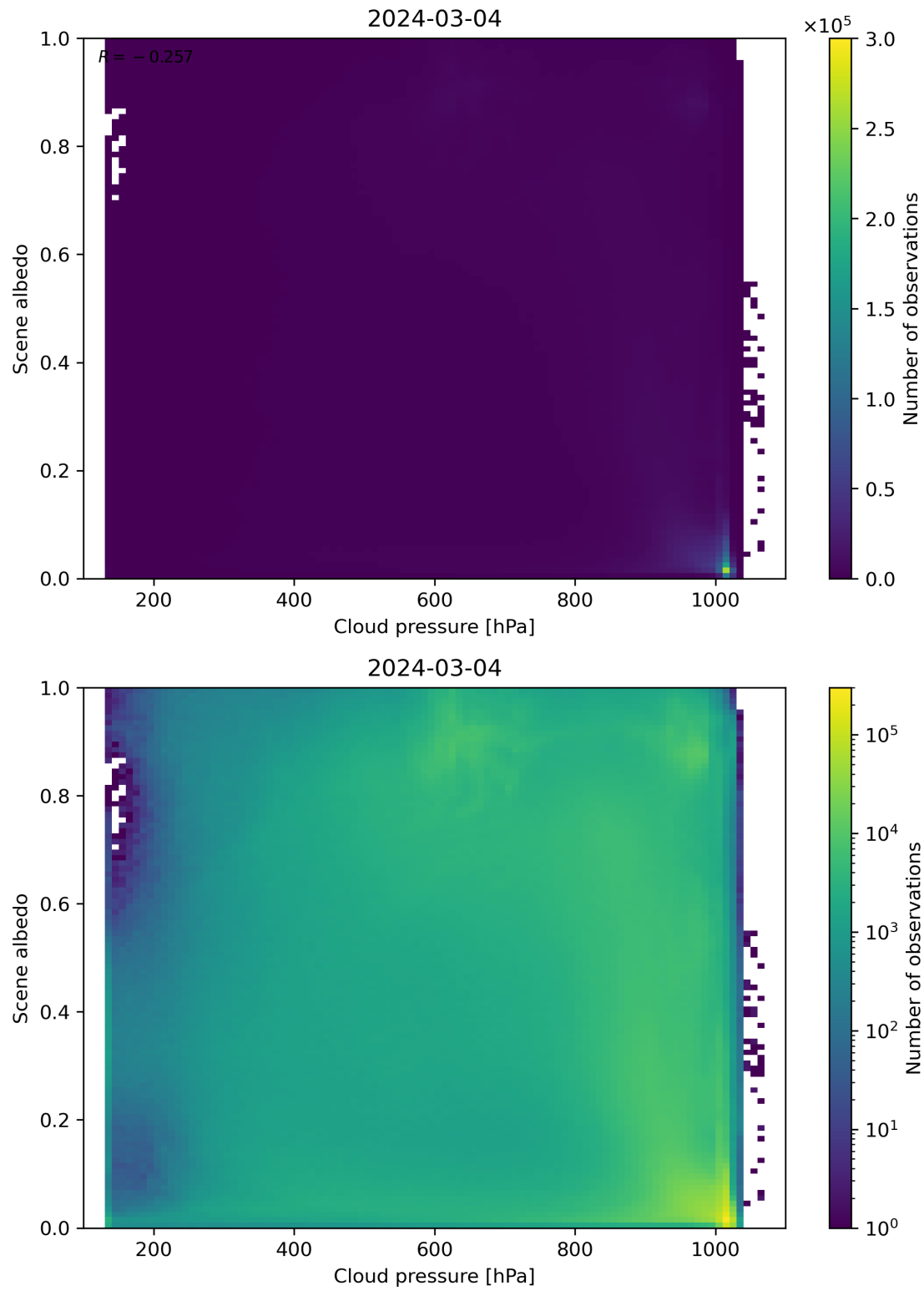
Figure 83: Scatter density plot of “Cloud pressure” against “Scene albedo” for 2024-03-04 to 2024-03-05.
