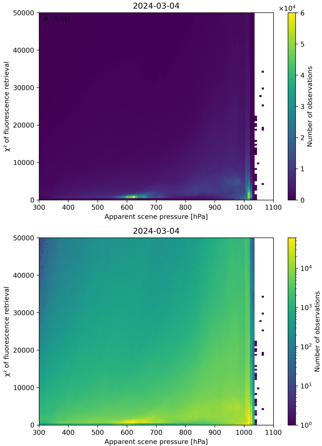
Figure 63: Scatter density plot of “Apparent scene pressure” against “ \chi^2 of fluorescence retrieval” for 2024-03-04 to 2024-03-05.
