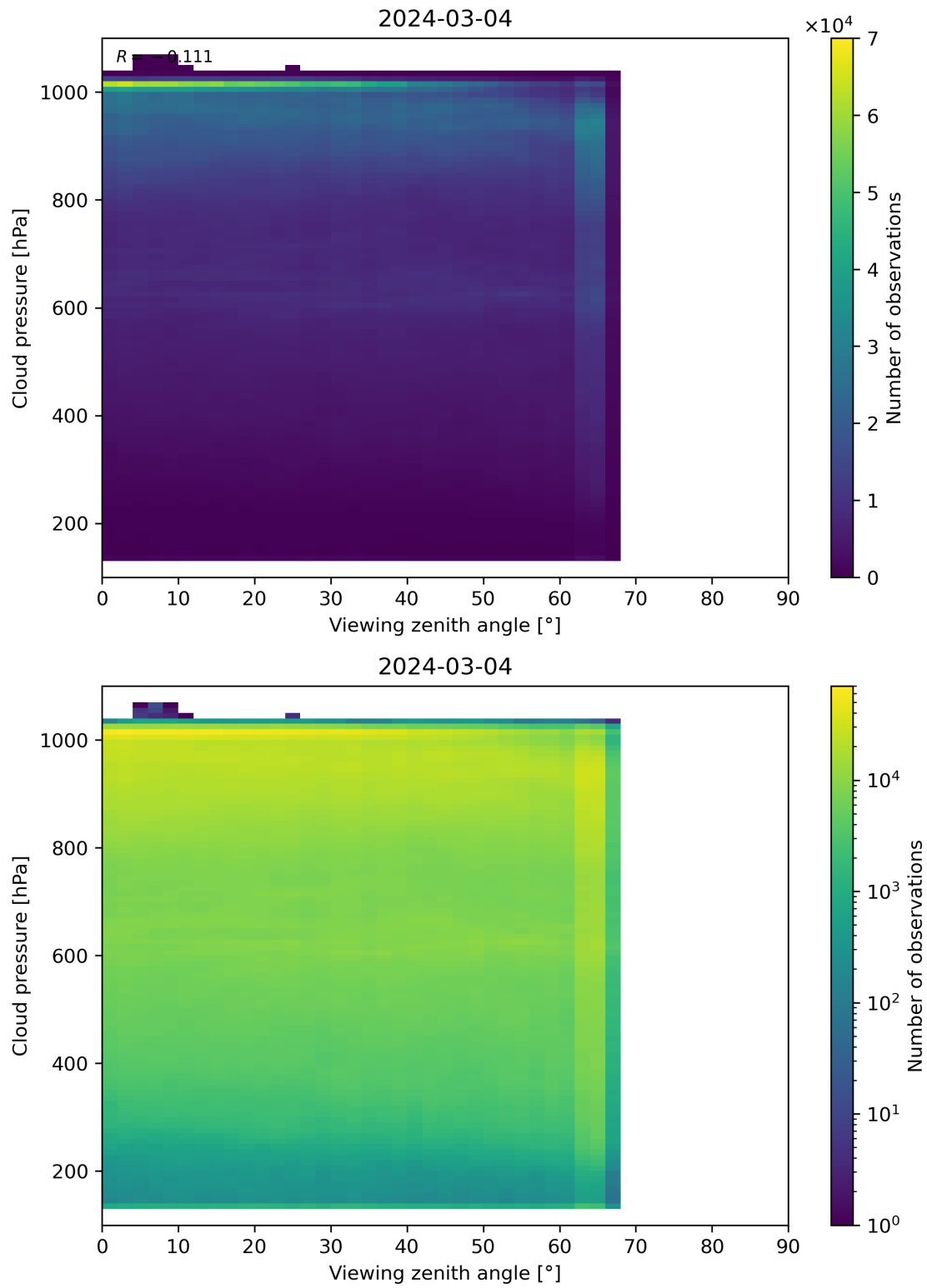
Figure 121: Scatter density plot of “Viewing zenith angle” against “Cloud pressure” for 2024-03-04 to 2024-03-05.
