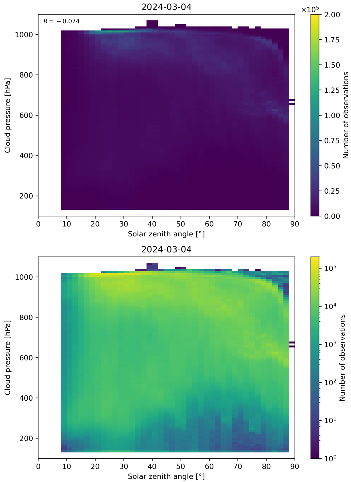
Figure 111: Scatter density plot of “Solar zenith angle” against “Cloud pressure” for 2024-03-04 to 2024-03-05.
