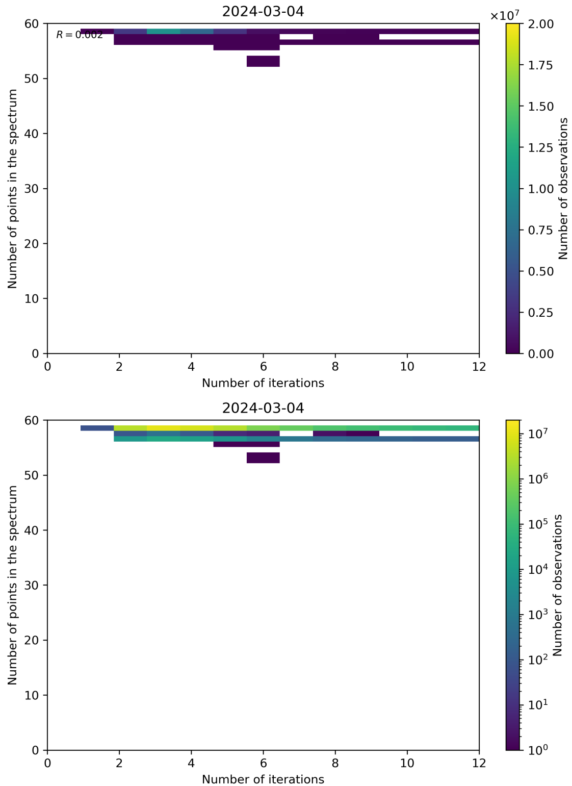
Figure 99: Scatter density plot of “Number of iterations” against “Number of points in the spectrum” for 2024-03-04 to 2024-03-05.
