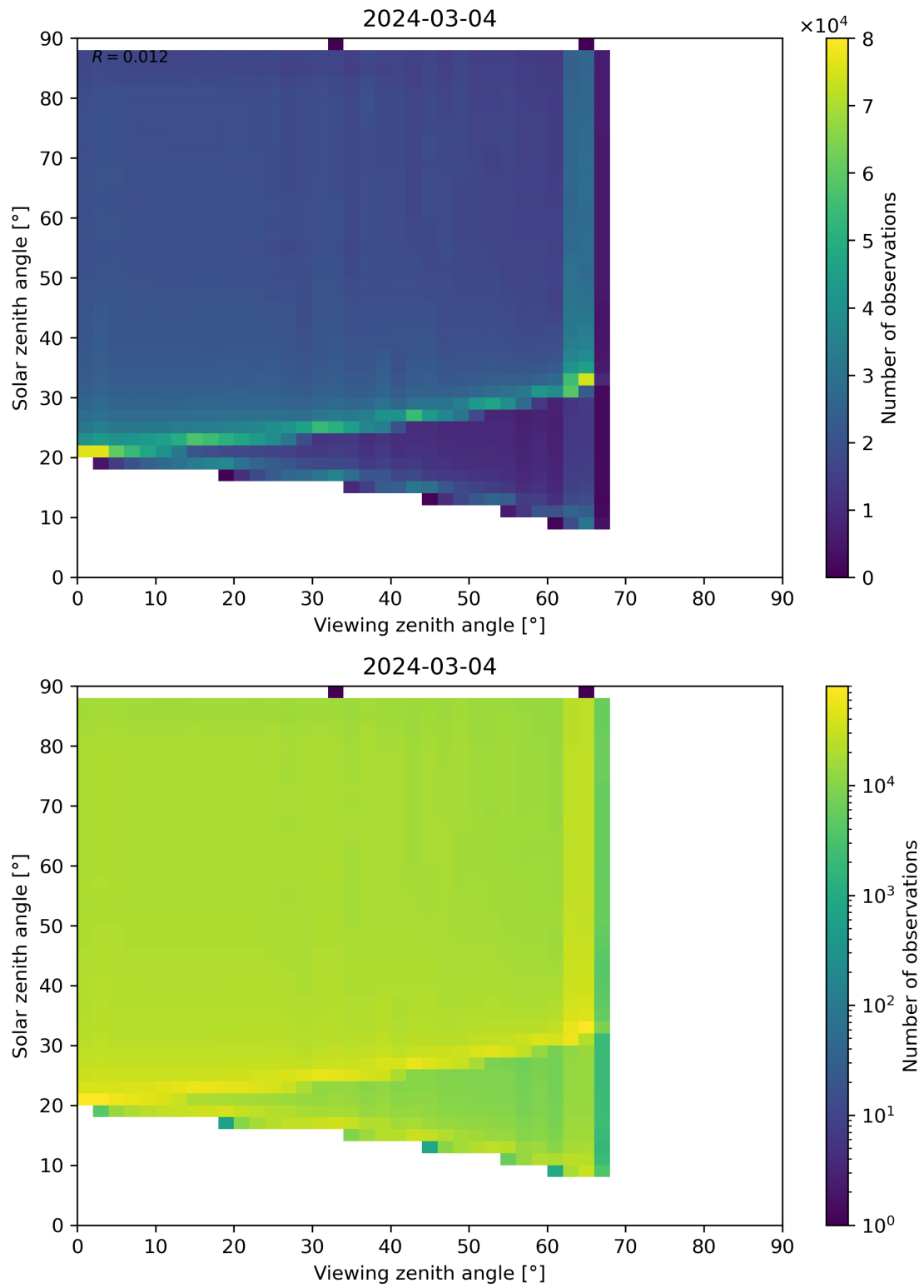
Figure 127: Scatter density plot of “Viewing zenith angle” against “Solar zenith angle” for 2024-03-04 to 2024-03-05.
