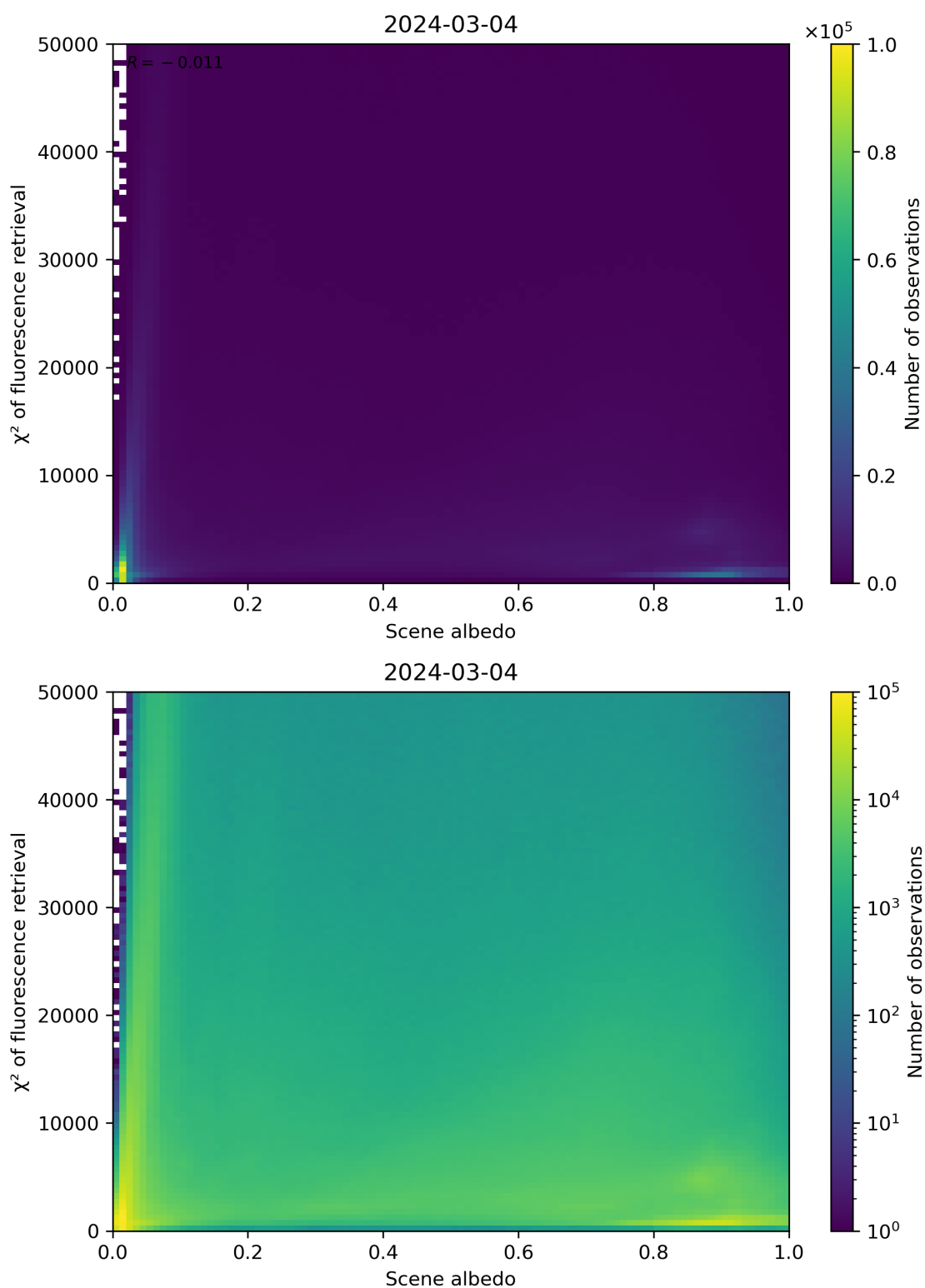
Figure 103: Scatter density plot of “Scene albedo” against “ \chi^2 of fluorescence retrieval” for 2024-03-04 to 2024-03-05.
