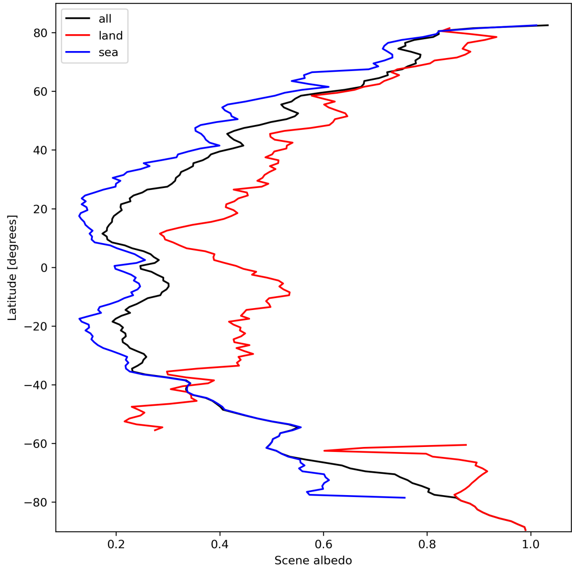
Figure 17: Zonal average of “Scene albedo” for 2024-03-04 to 2024-03-05.
