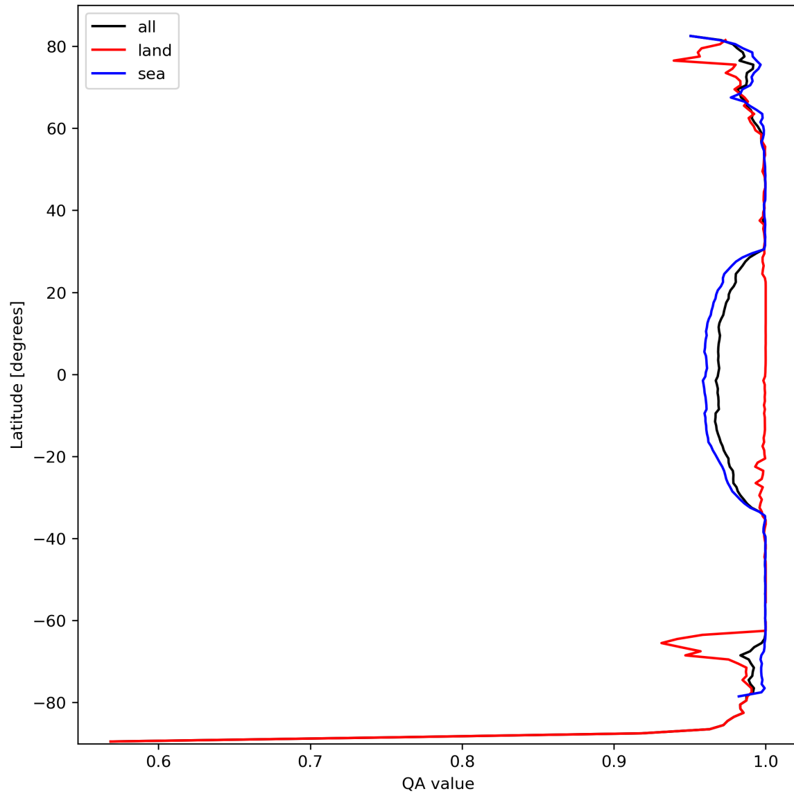
Figure 12: Zonal average of “QA value” for 2024-03-04 to 2024-03-05.
