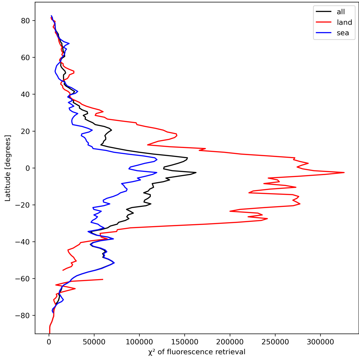
Figure 25: Zonal average of “ \chi^2 of fluorescence retrieval” for 2024-03-04 to 2024-03-05.
