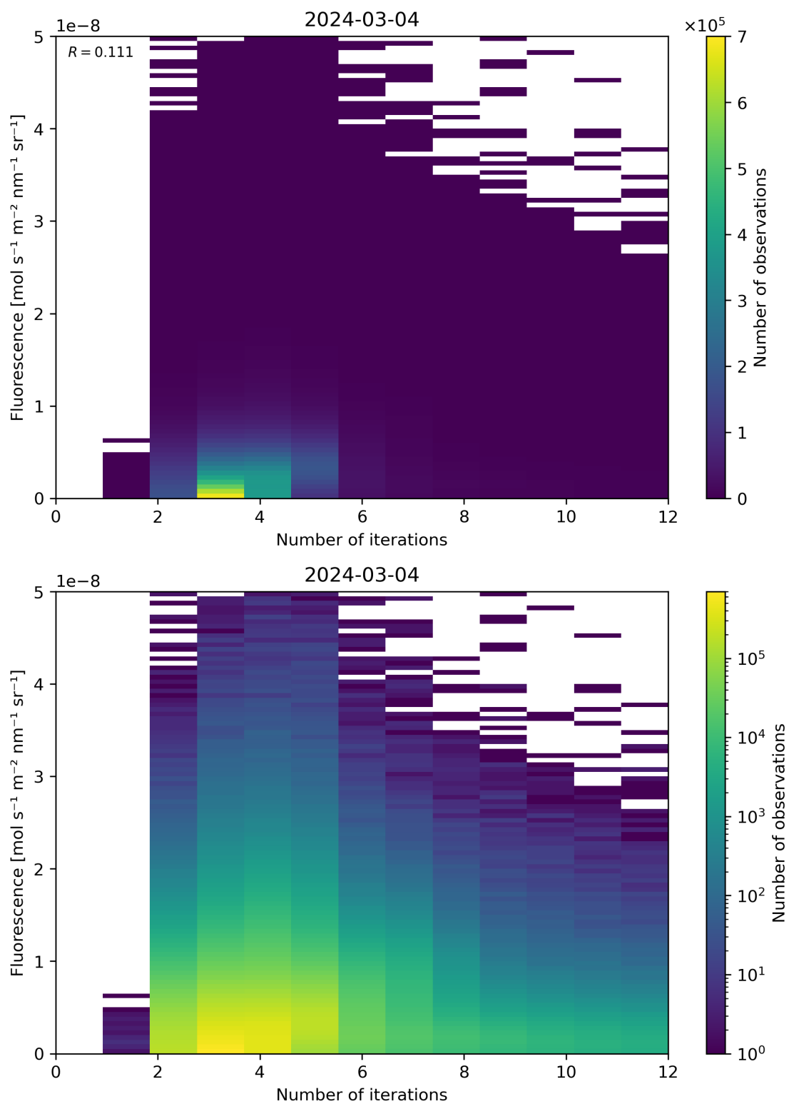
Figure 98: Scatter density plot of “Number of iterations” against “Fluorescence” for 2024-03-04 to 2024-03-05.
