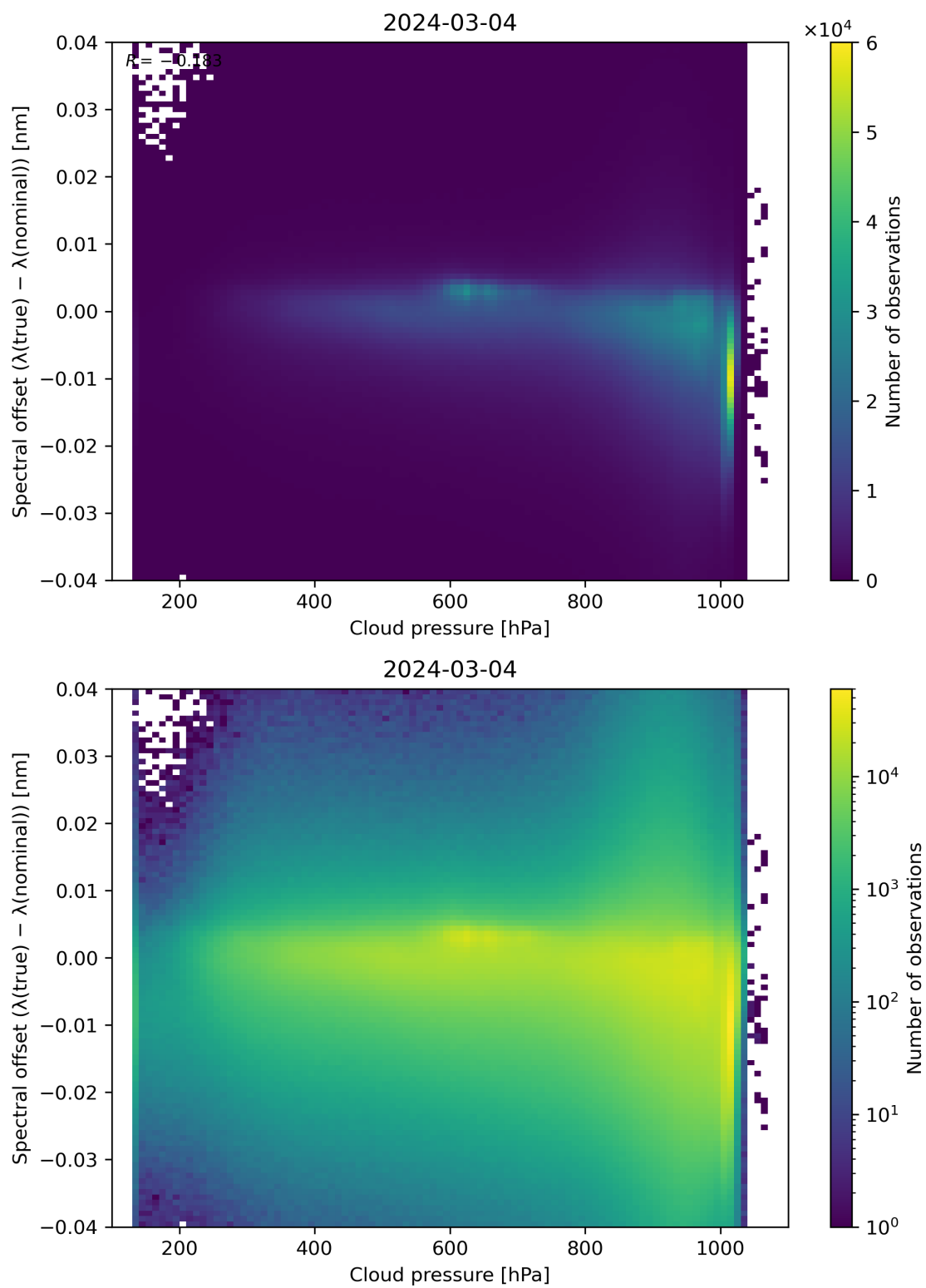
Figure 84: Scatter density plot of “Cloud pressure” against “Spectral offset ( \lambda(\text{true}) - \lambda(\text{nominal}) )” for 2024-03-04 to 2024-03-05.
