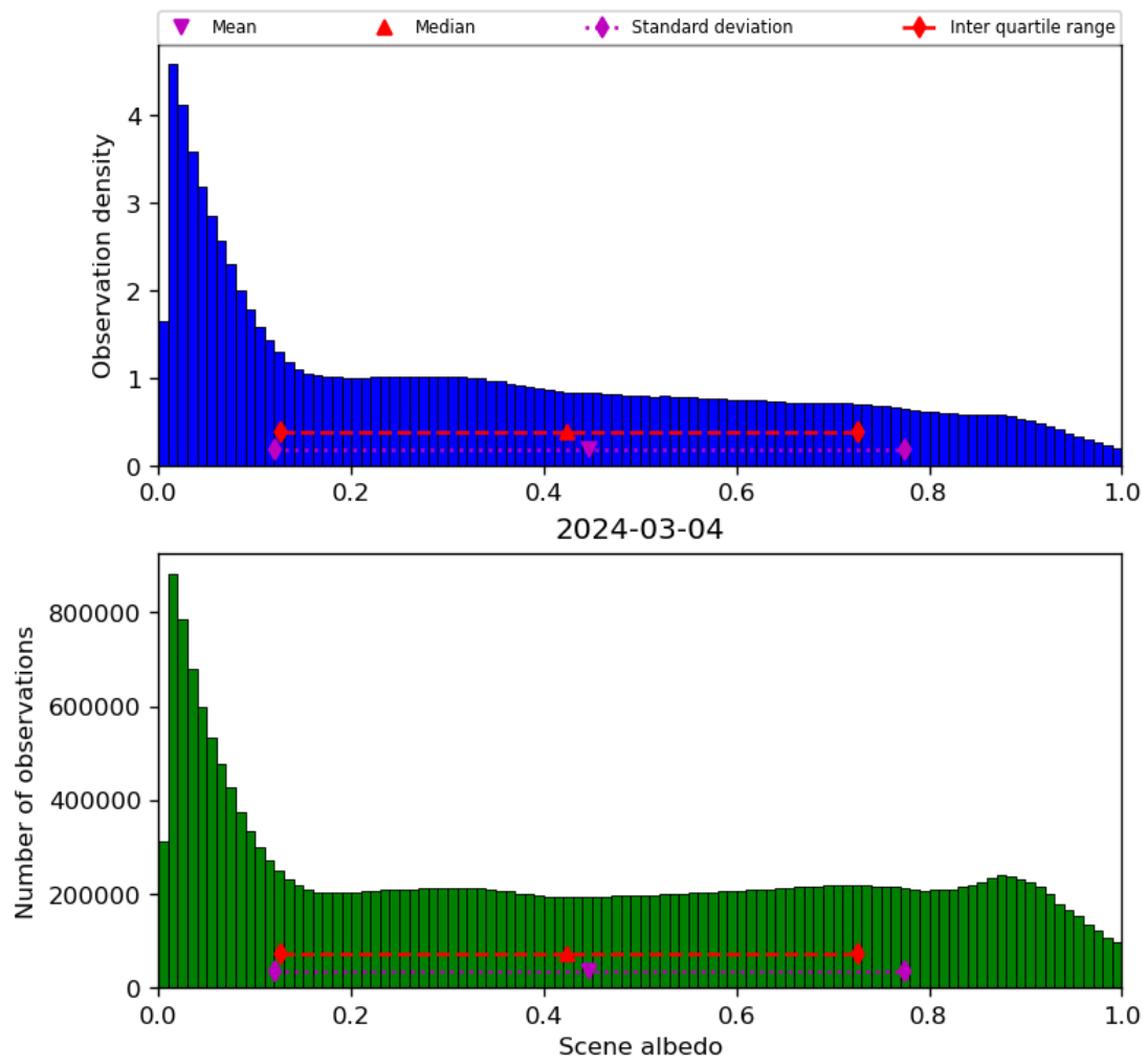
Figure 34: Histogram of “Scene albedo” for 2024-03-04 to 2024-03-05
