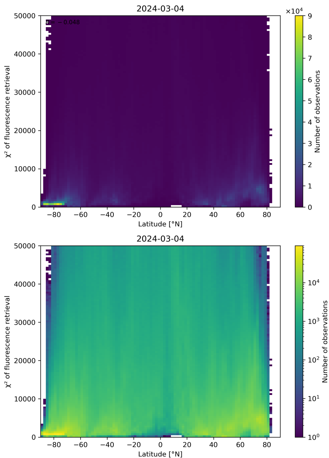
Figure 89: Scatter density plot of “Latitude” against “ \chi^2 of fluorescence retrieval” for 2024-03-04 to 2024-03-05.
