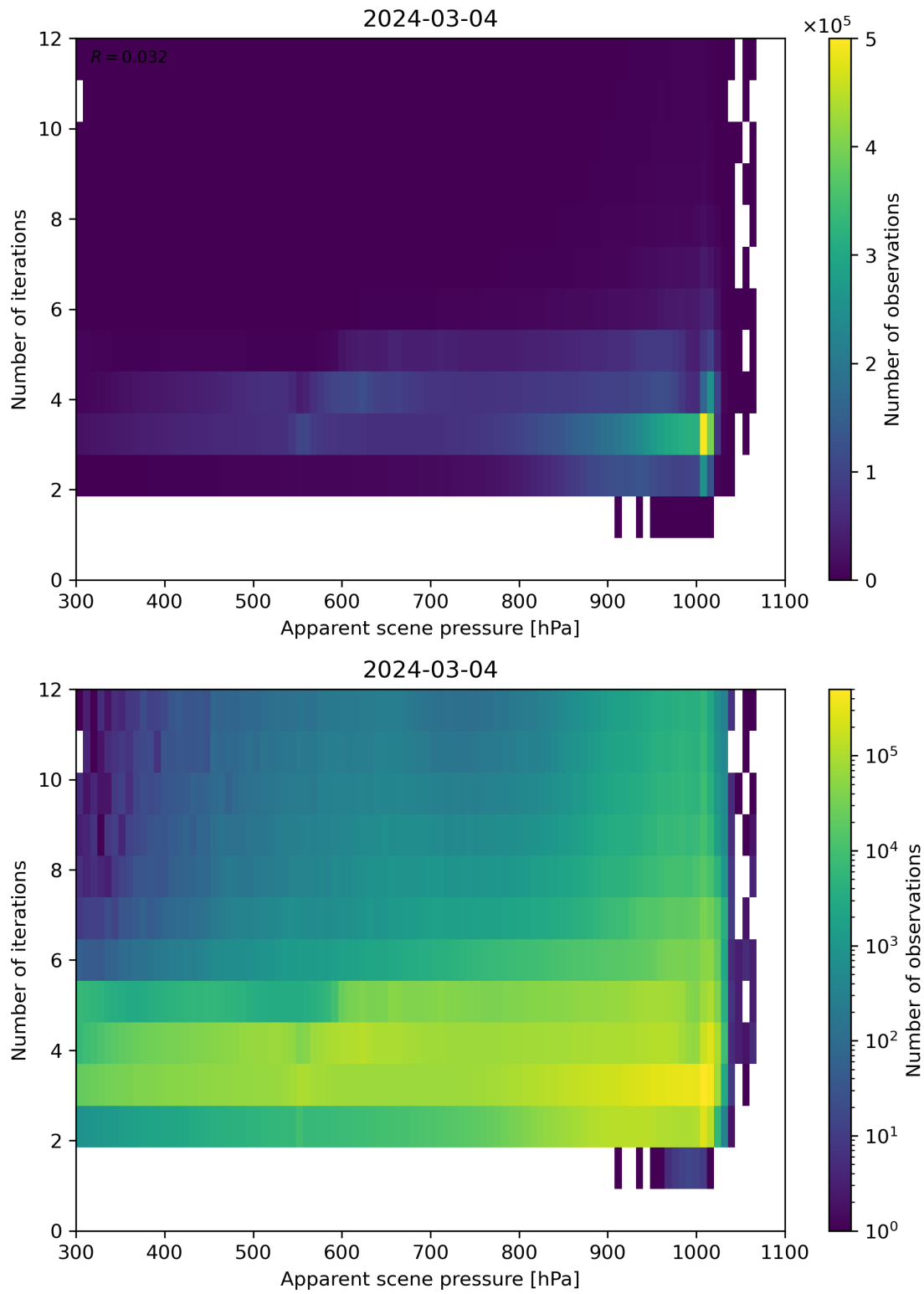
Figure 65: Scatter density plot of “Apparent scene pressure” against “Number of iterations” for 2024-03-04 to 2024-03-05.
