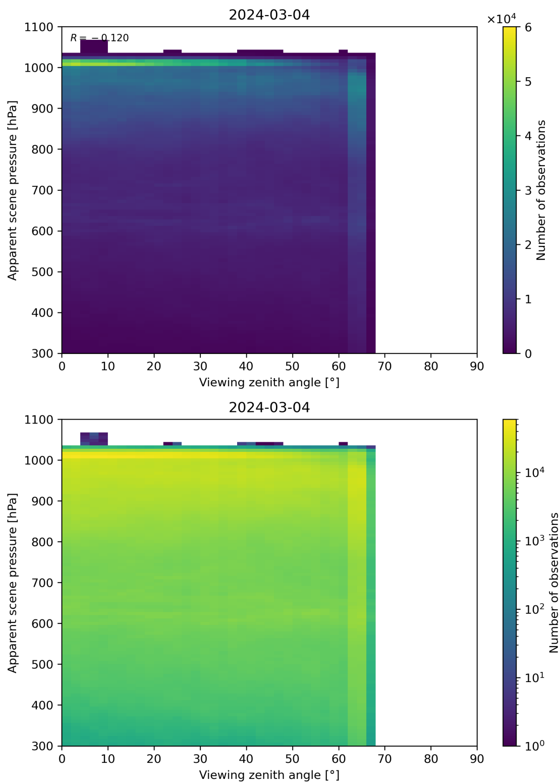
Figure 118: Scatter density plot of “Viewing zenith angle” against “Apparent scene pressure” for 2024-03-04 to 2024-03-05.
