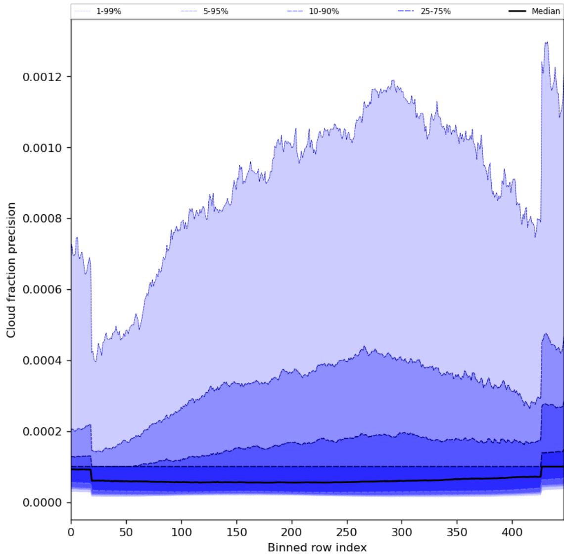
Figure 50: Along track statistics of “Cloud fraction precision” for 2024-03-04 to 2024-03-05
