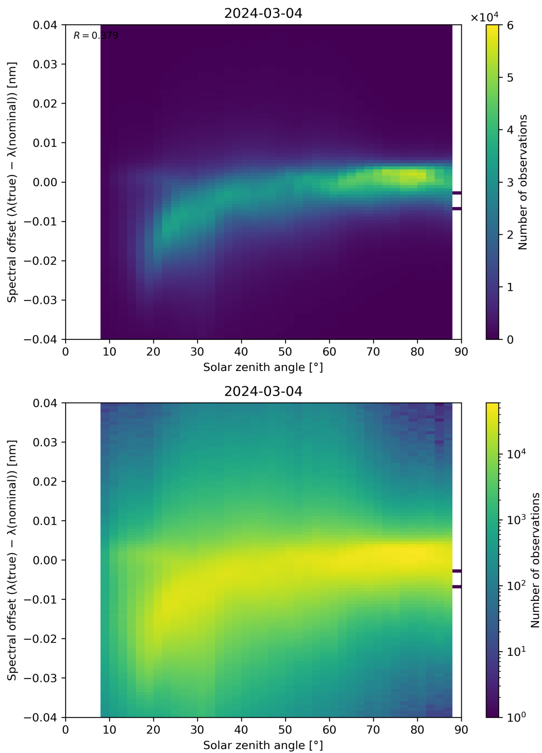
Figure 117: Scatter density plot of “Solar zenith angle” against “Spectral offset ( \lambda(\text{true}) - \lambda(\text{nominal}) )” for 2024-03-04 to 2024-03-05.
