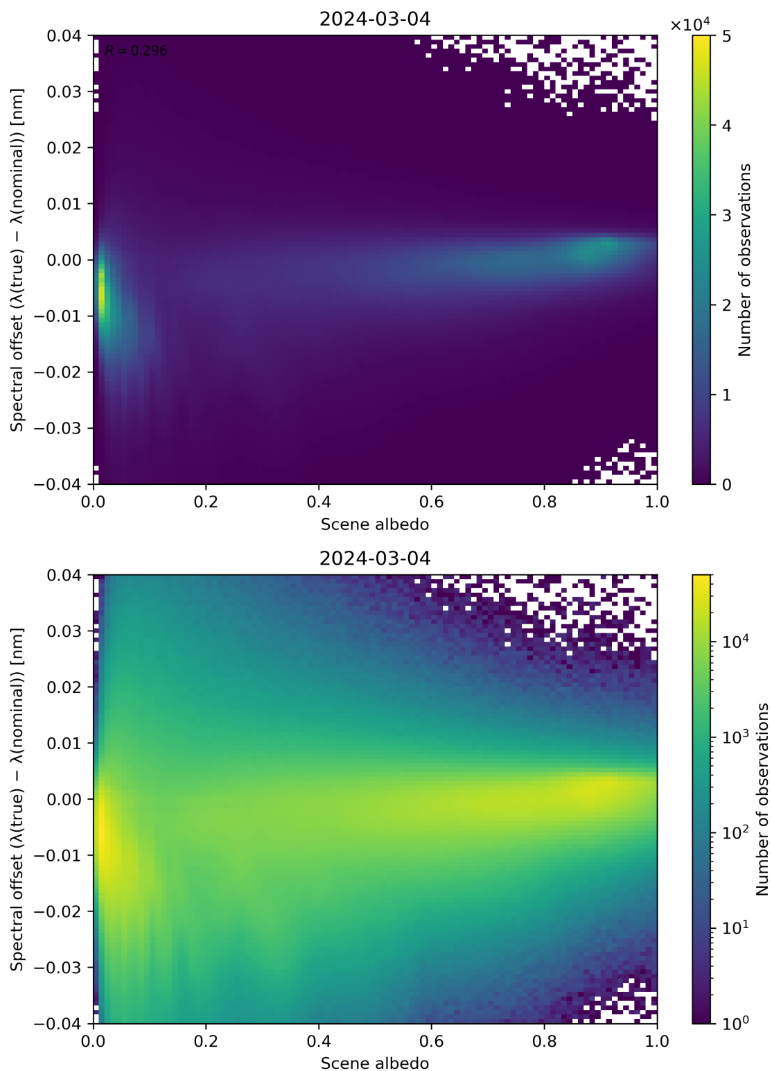
Figure 107: Scatter density plot of “Scene albedo” against “Spectral offset ( \lambda(\text{true}) - \lambda(\text{nominal}) )” for 2024-03-04 to 2024-03-05.
