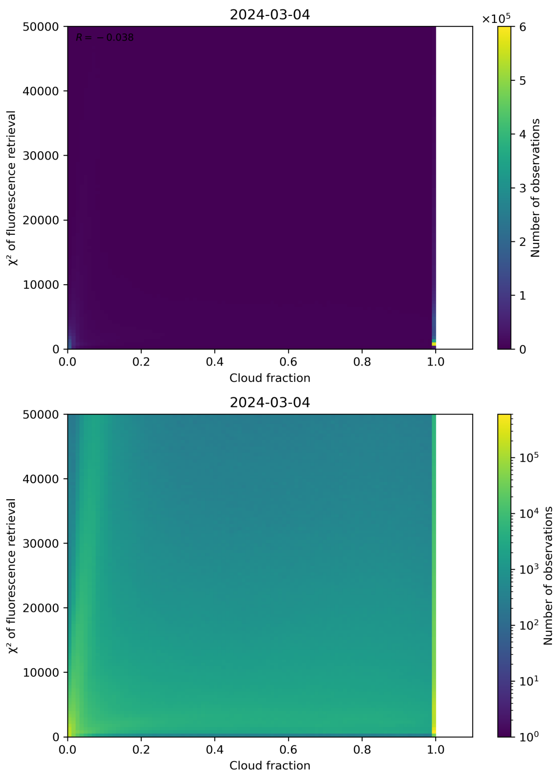
Figure 71: Scatter density plot of “Cloud fraction” against “ \chi^2 of fluorescence retrieval” for 2024-03-04 to 2024-03-05.
