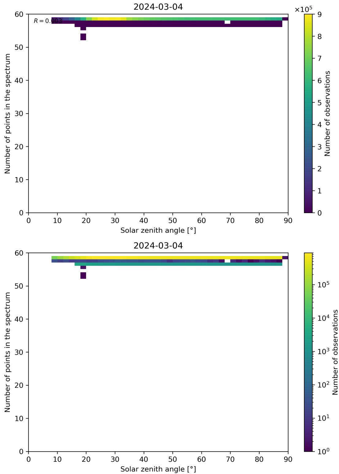
Figure 115: Scatter density plot of “Solar zenith angle” against “Number of points in the spectrum” for 2024-03-04 to 2024-03-05.
