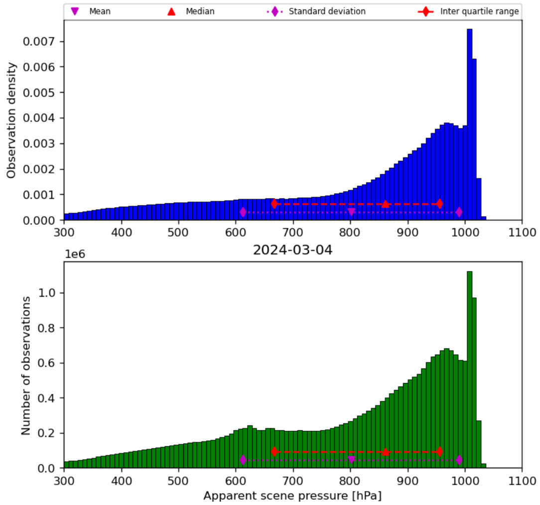
Figure 36: Histogram of “Apparent scene pressure” for 2024-03-04 to 2024-03-05
