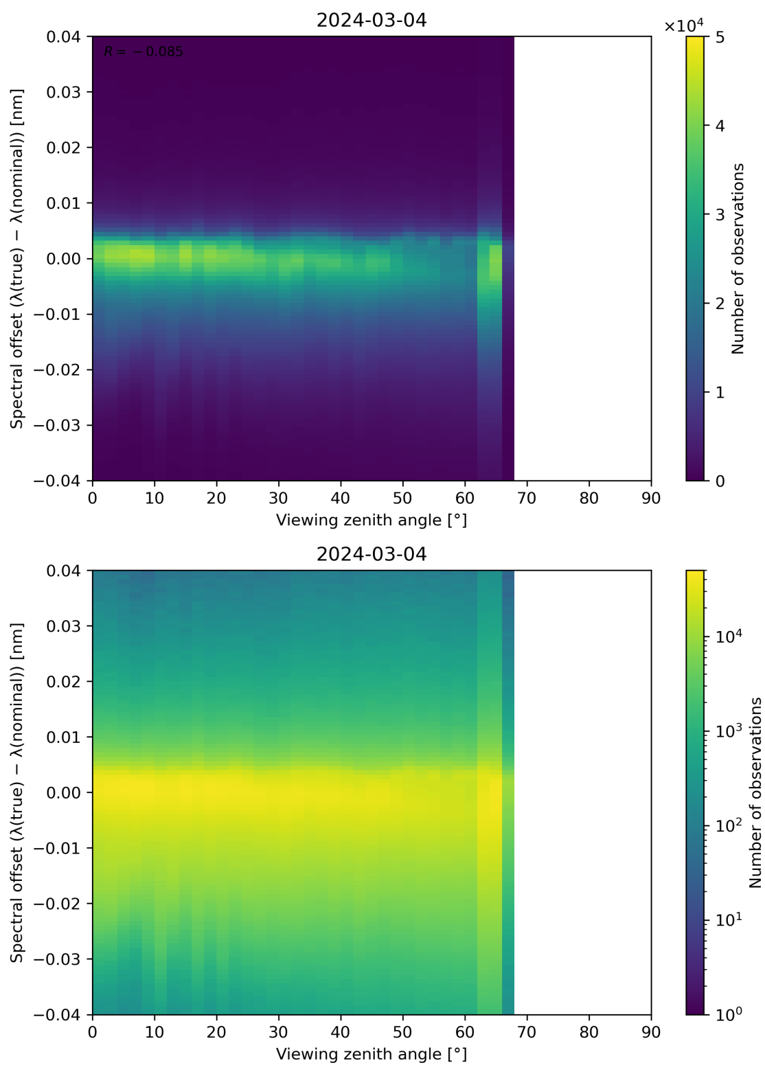
Figure 128: Scatter density plot of “Viewing zenith angle” against “Spectral offset ( \lambda(\text{true}) - \lambda(\text{nominal}) )” for 2024-03-04 to 2024-03-05.
