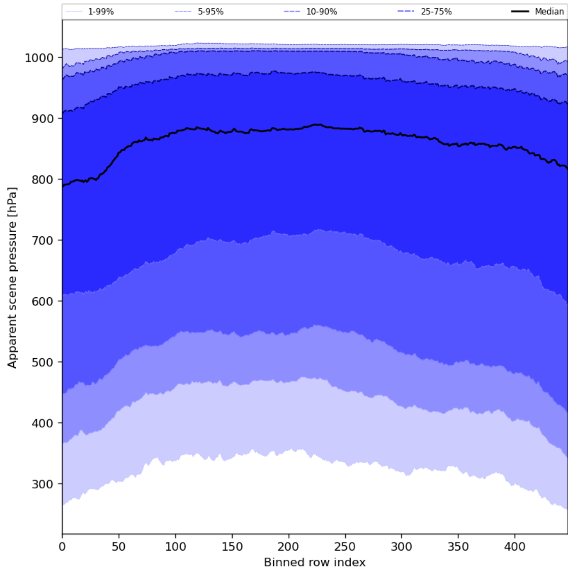
Figure 53: Along track statistics of “Apparent scene pressure” for 2024-03-04 to 2024-03-05
