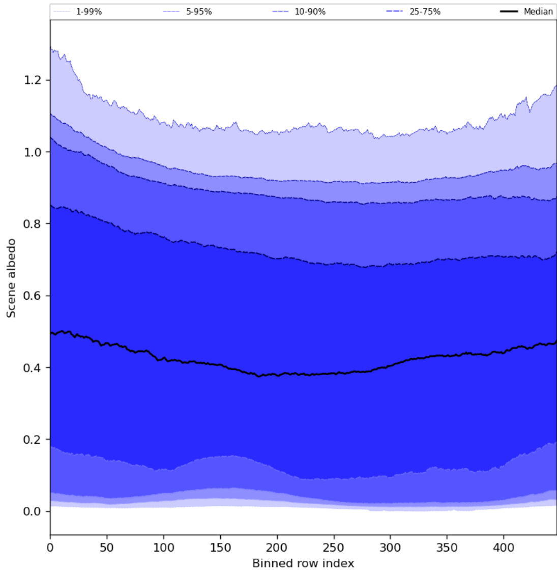
Figure 51: Along track statistics of “Scene albedo” for 2024-03-04 to 2024-03-05
