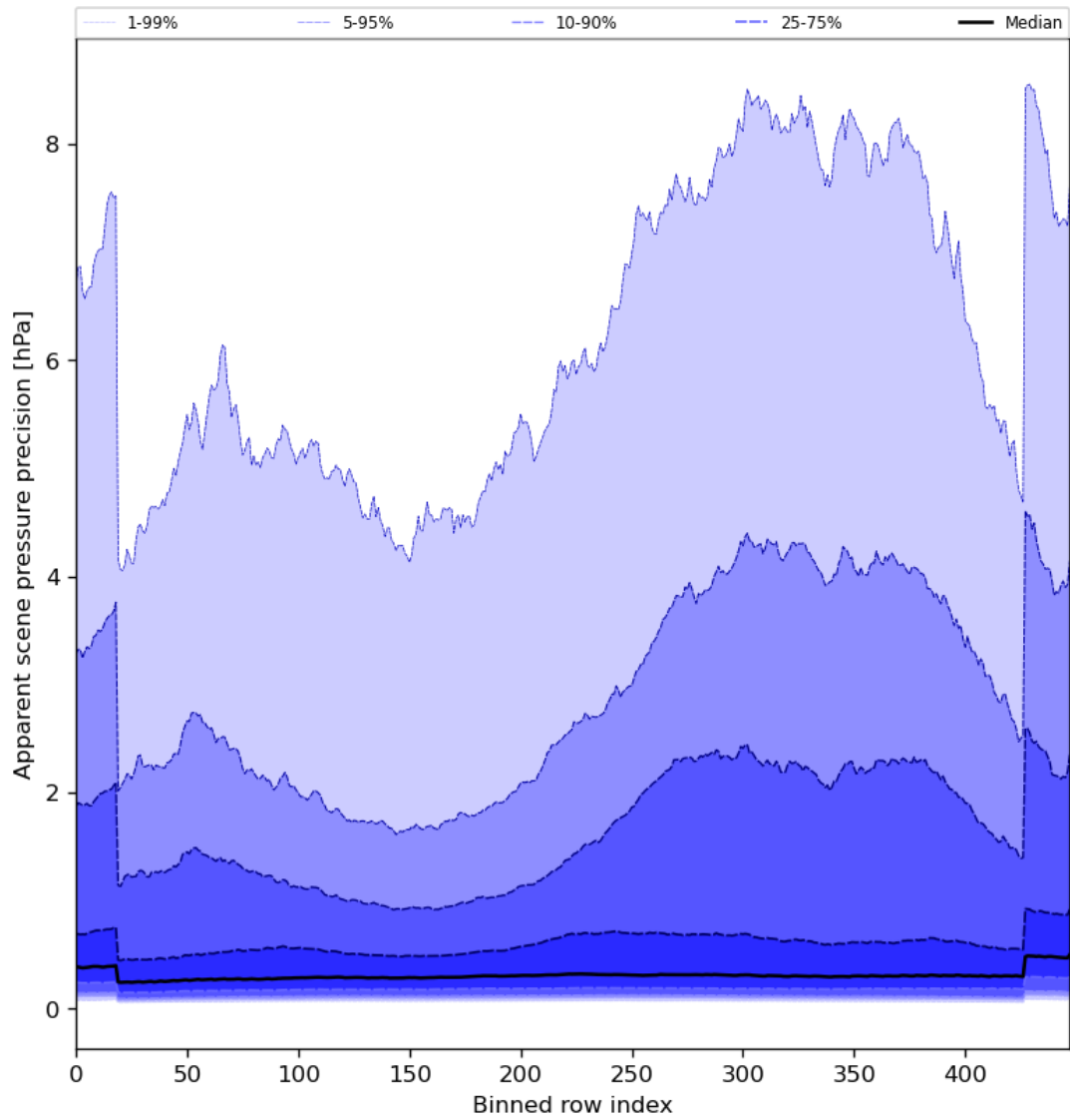
Figure 54: Along track statistics of “Apparent scene pressure precision” for 2024-03-04 to 2024-03-05
