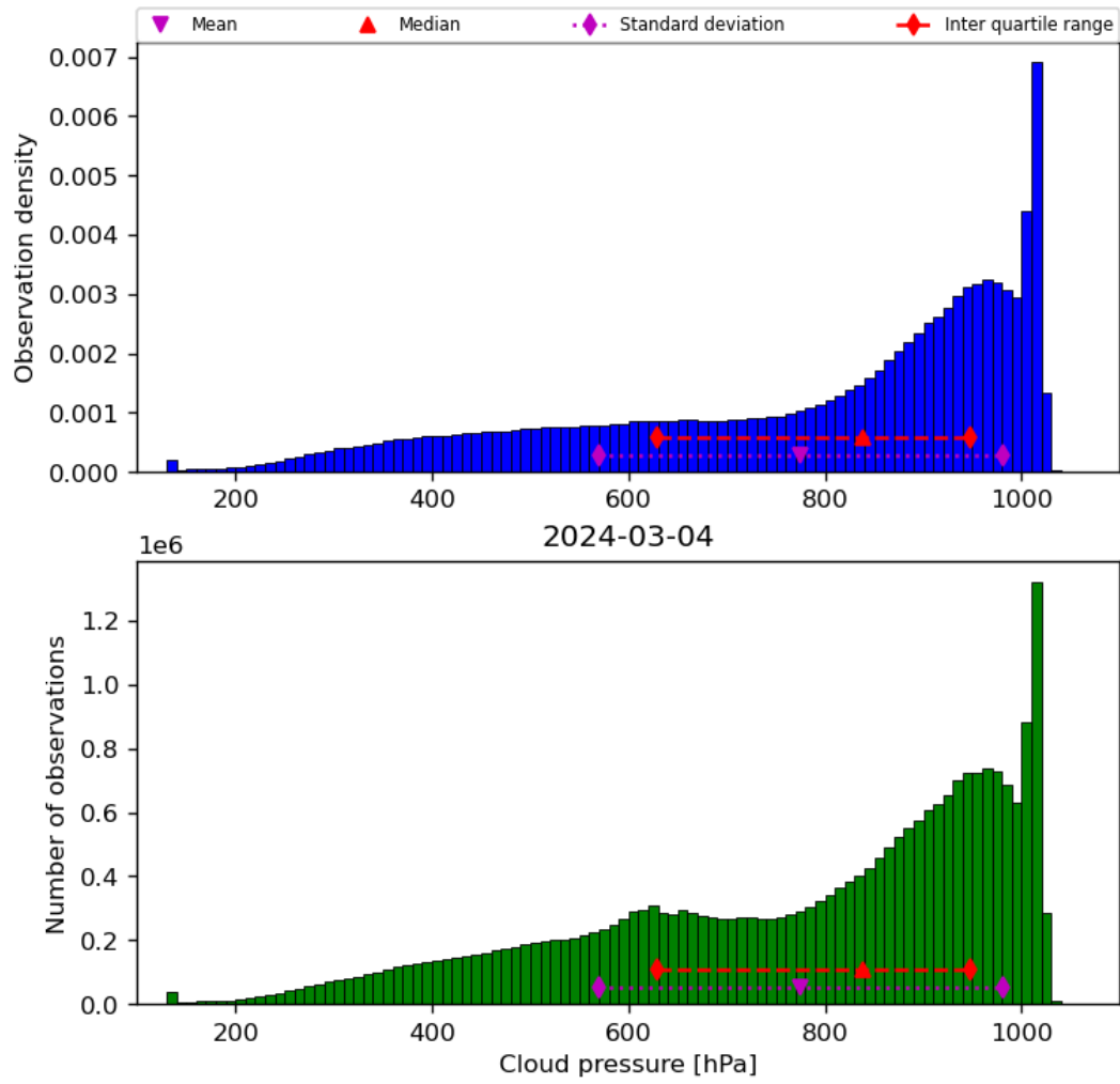
Figure 30: Histogram of “Cloud pressure” for 2024-03-04 to 2024-03-05
