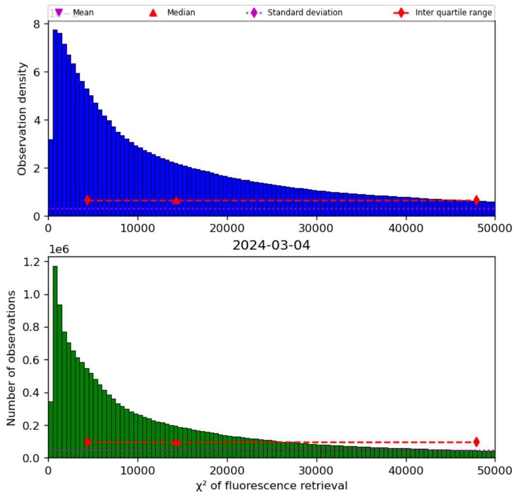
Figure 42: Histogram of “ \chi^2 of fluorescence retrieval” for 2024-03-04 to 2024-03-05
