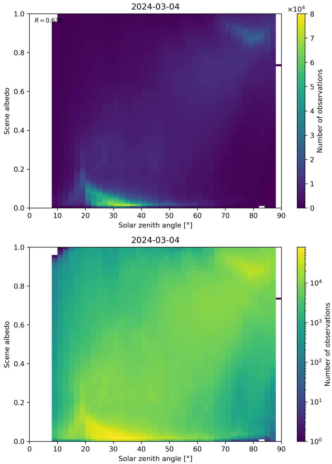
Figure 116: Scatter density plot of “Solar zenith angle” against “Scene albedo” for 2024-03-04 to 2024-03-05.
