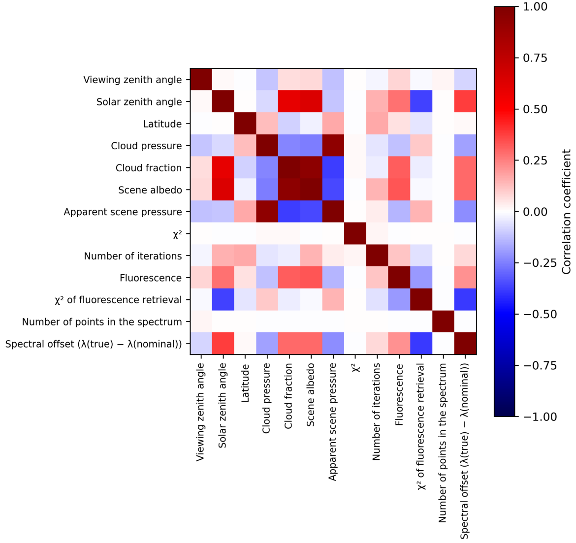
Figure 2: Map of correlation matrix for 2024-03-04 to 2024-03-05.
