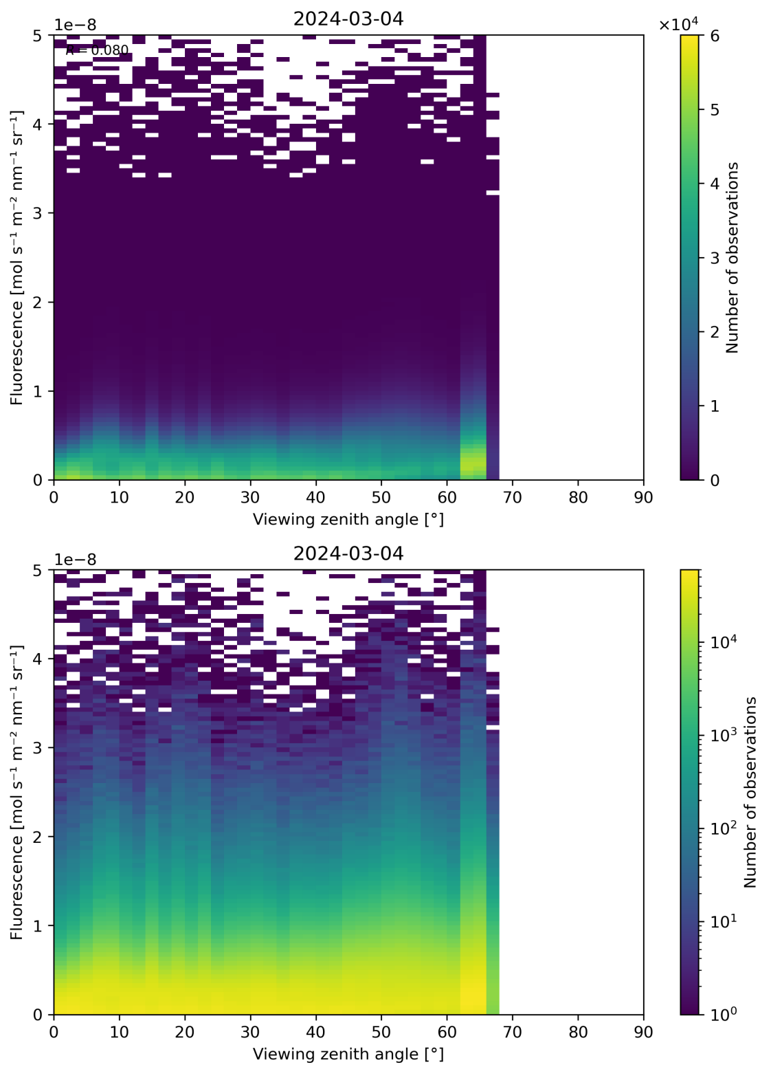
Figure 122: Scatter density plot of “Viewing zenith angle” against “Fluorescence” for 2024-03-04 to 2024-03-05.
