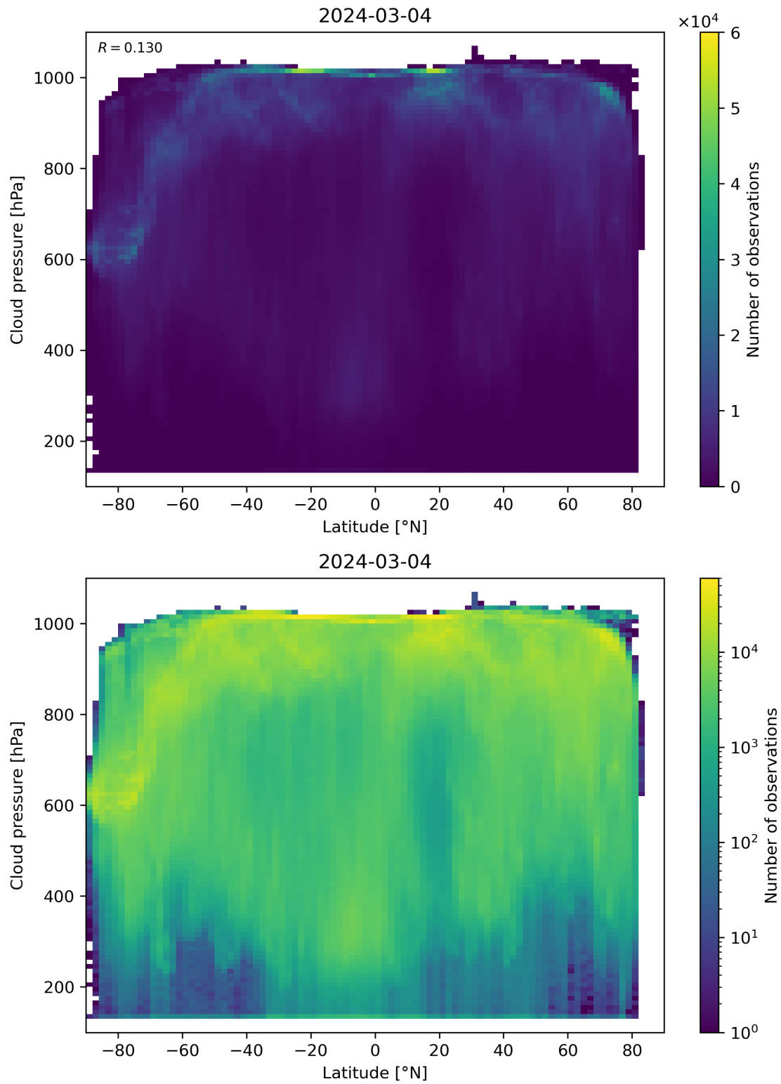
Figure 91: Scatter density plot of “Latitude” against “Cloud pressure” for 2024-03-04 to 2024-03-05.
