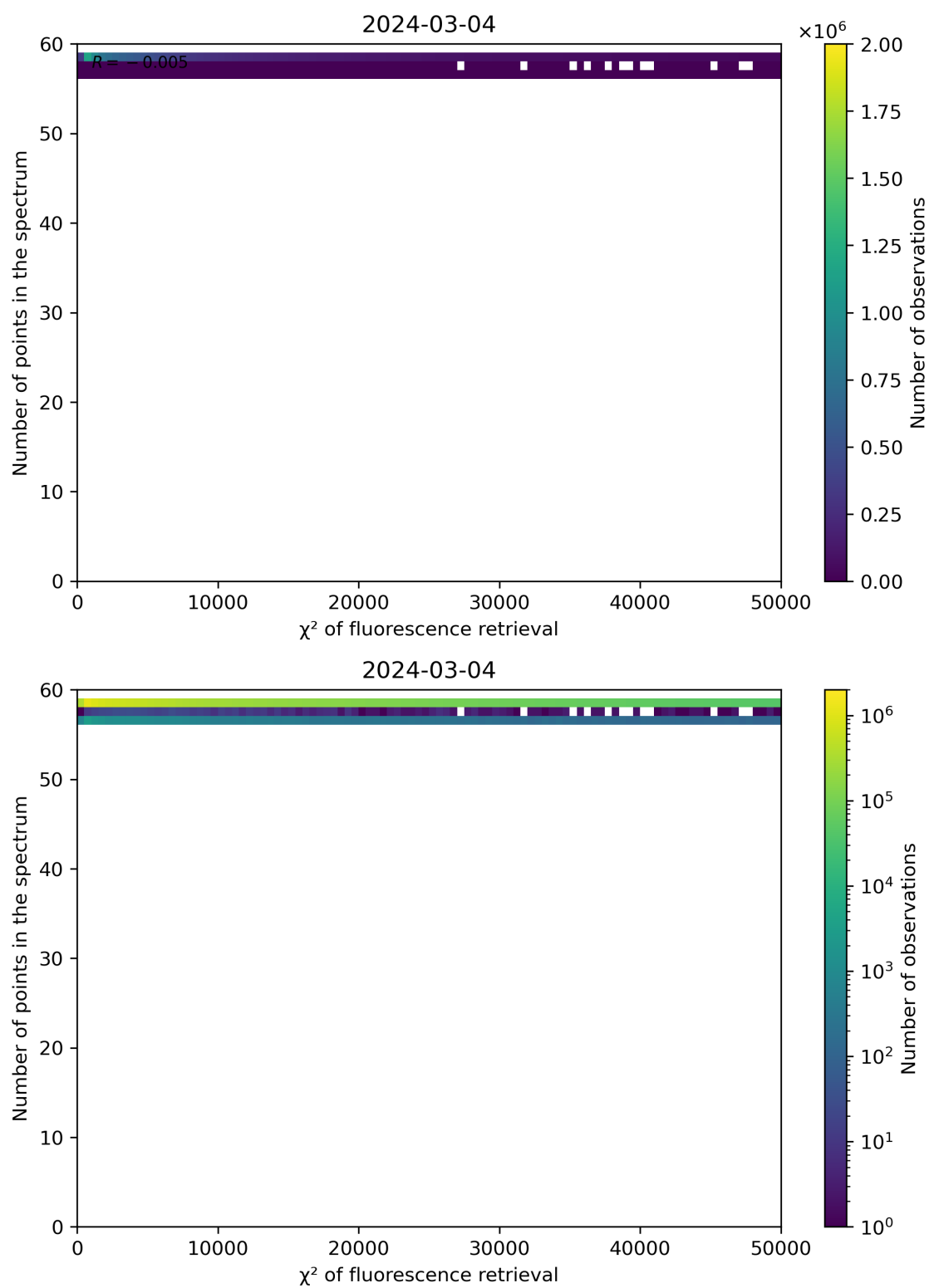
Figure 68: Scatter density plot of " \chi^2 of fluorescence retrieval" against "Number of points in the spectrum" for 2024-03-04 to 2024-03-05.
