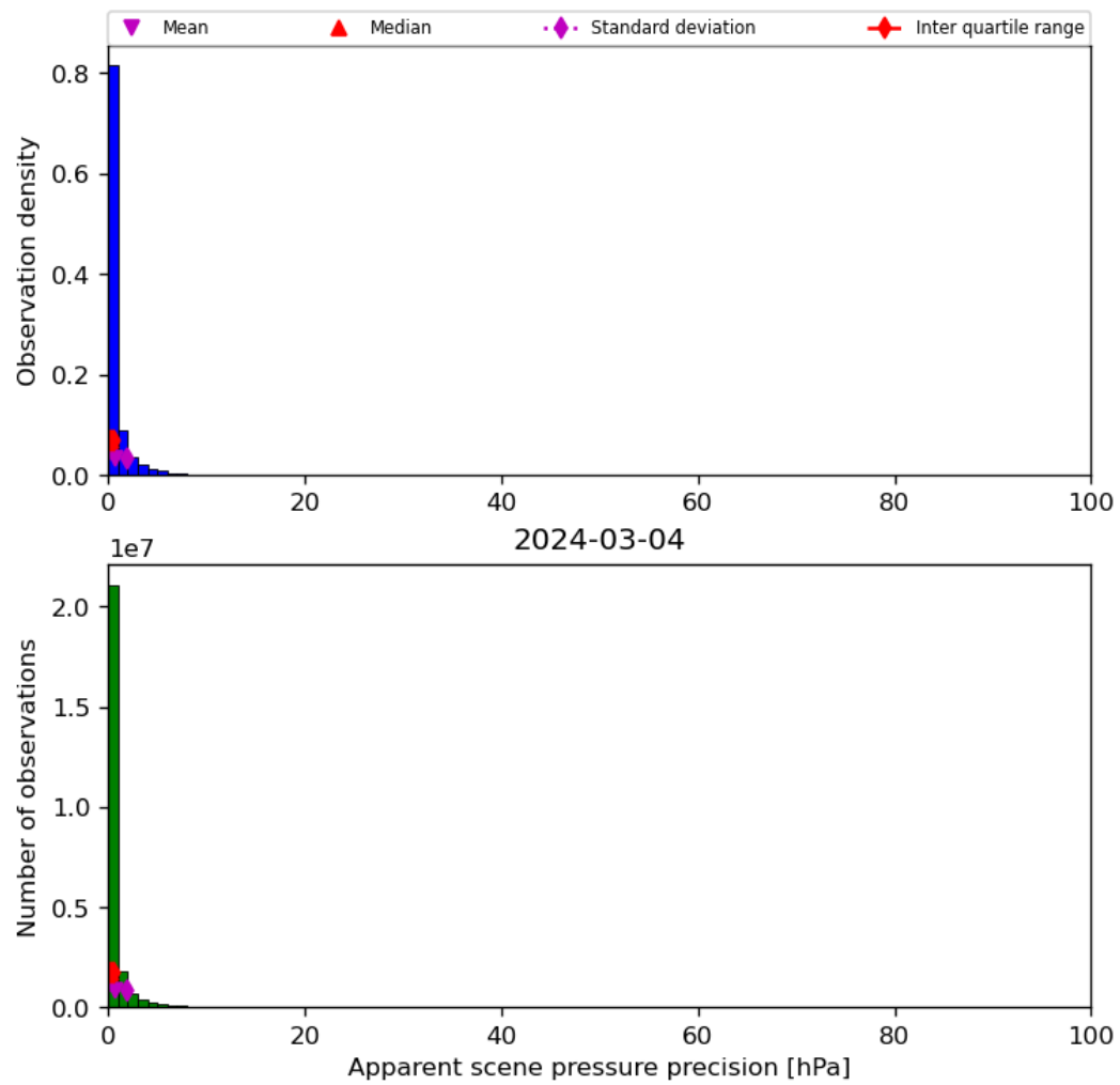
Figure 37: Histogram of “Apparent scene pressure precision” for 2024-03-04 to 2024-03-05
