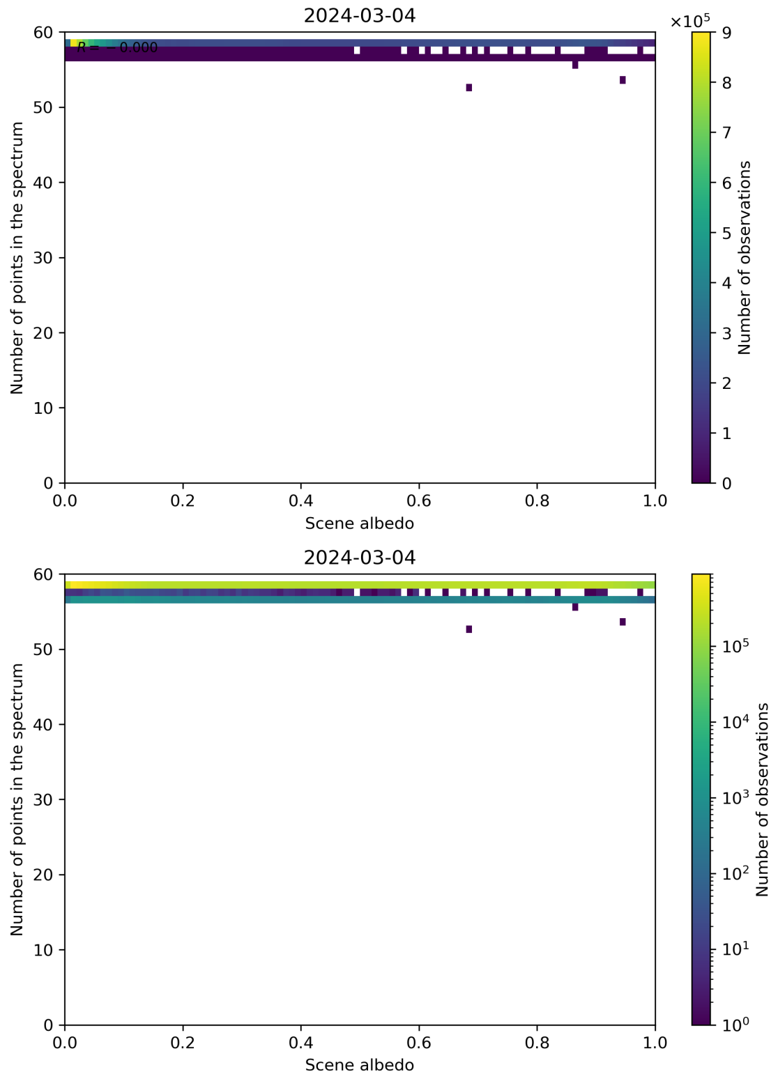
Figure 106: Scatter density plot of “Scene albedo” against “Number of points in the spectrum” for 2024-03-04 to 2024-03-05.
