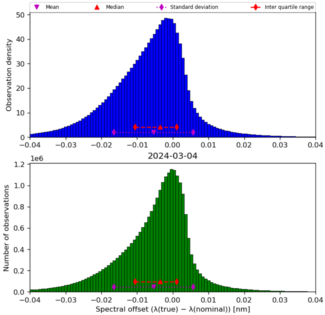
Figure 45: Histogram of “Spectral offset ( \lambda(\text{true}) - \lambda(\text{nominal}) )” for 2024-03-04 to 2024-03-05
