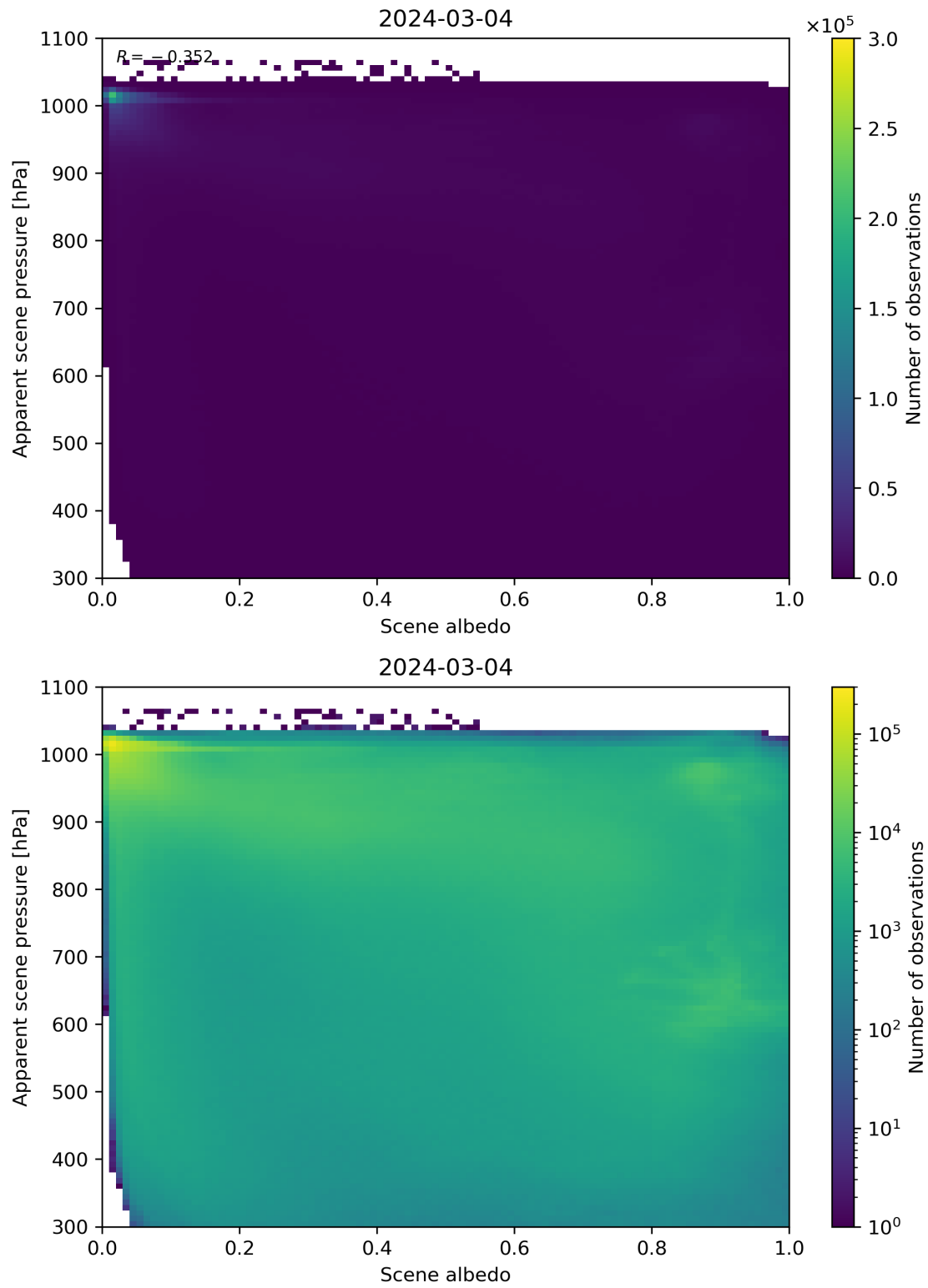
Figure 102: Scatter density plot of “Scene albedo” against “Apparent scene pressure” for 2024-03-04 to 2024-03-05.
