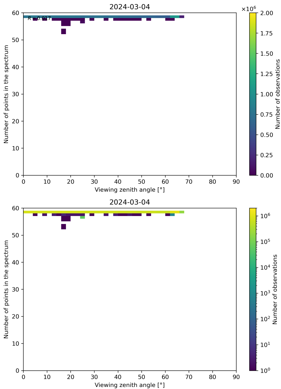
Figure 125: Scatter density plot of “Viewing zenith angle” against “Number of points in the spectrum” for 2024-03-04 to 2024-03-05.
