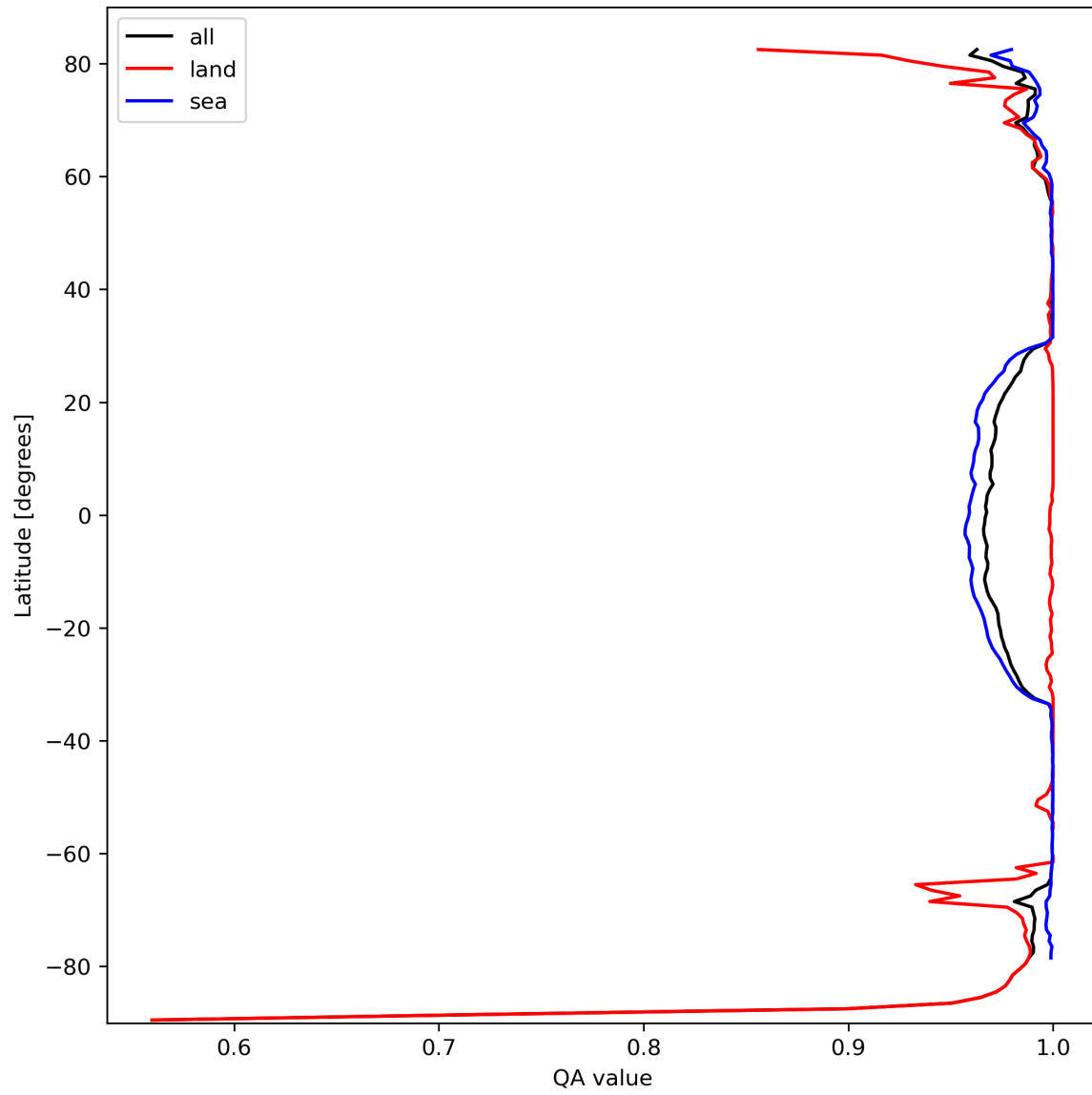
Figure 12: Zonal average of “QA value” for 2024-03-04 to 2024-03-06.
