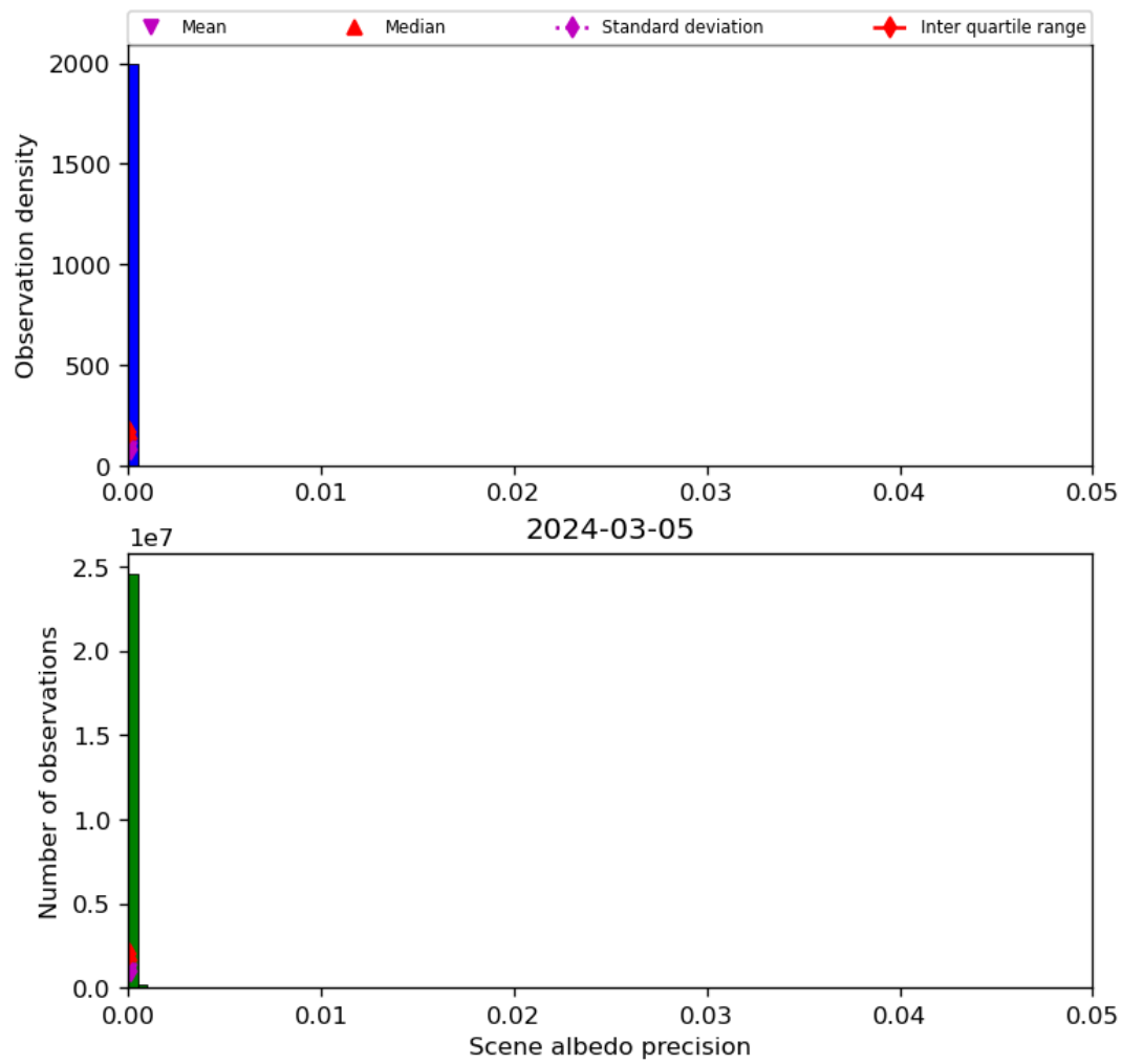
Figure 35: Histogram of “Scene albedo precision” for 2024-03-04 to 2024-03-06
