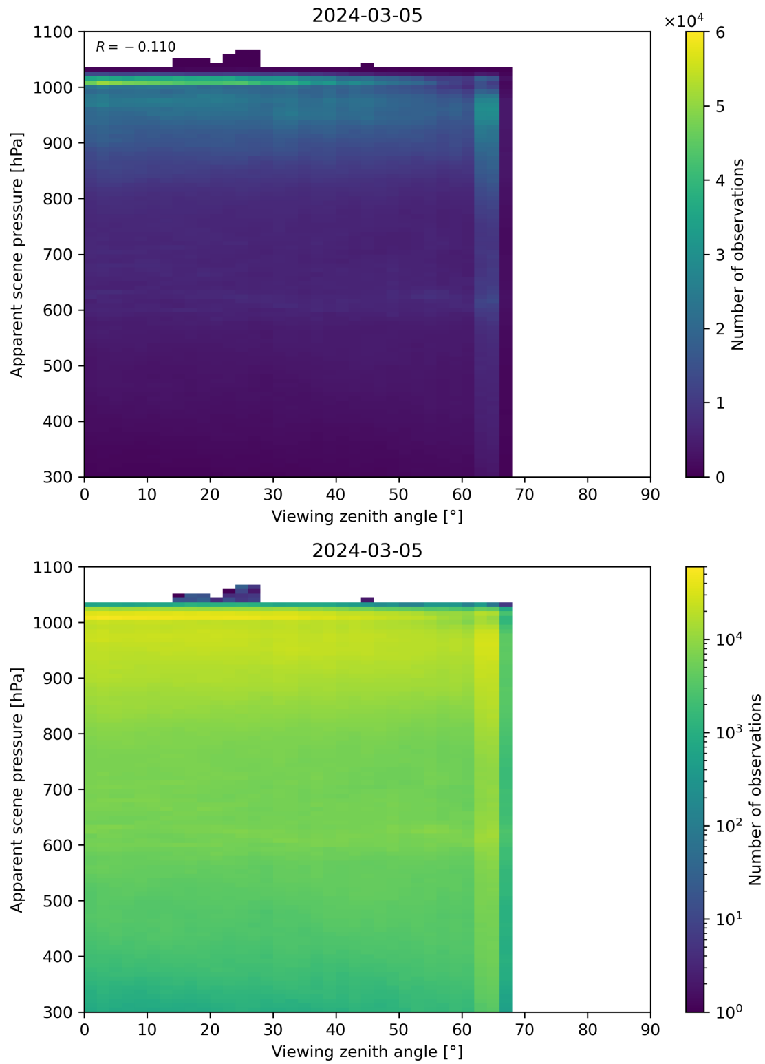
Figure 118: Scatter density plot of “Viewing zenith angle” against “Apparent scene pressure” for 2024-03-04 to 2024-03-06.
