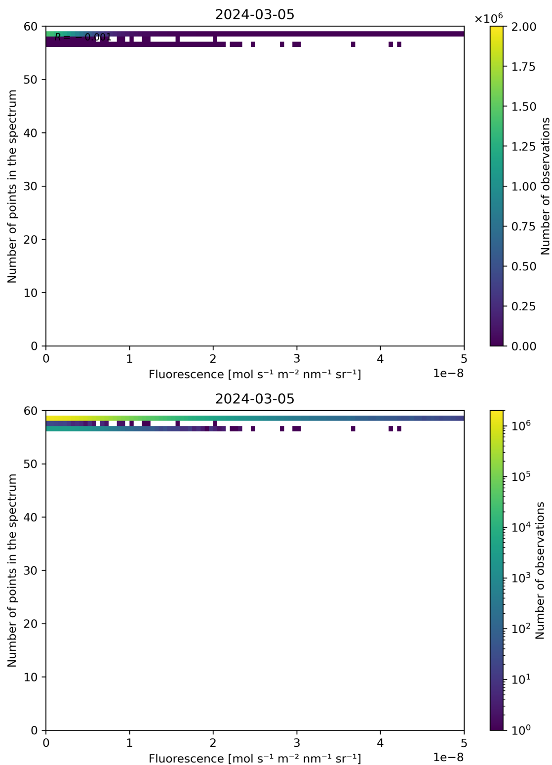
Figure 86: Scatter density plot of “Fluorescence” against “Number of points in the spectrum” for 2024-03-04 to 2024-03-06.
