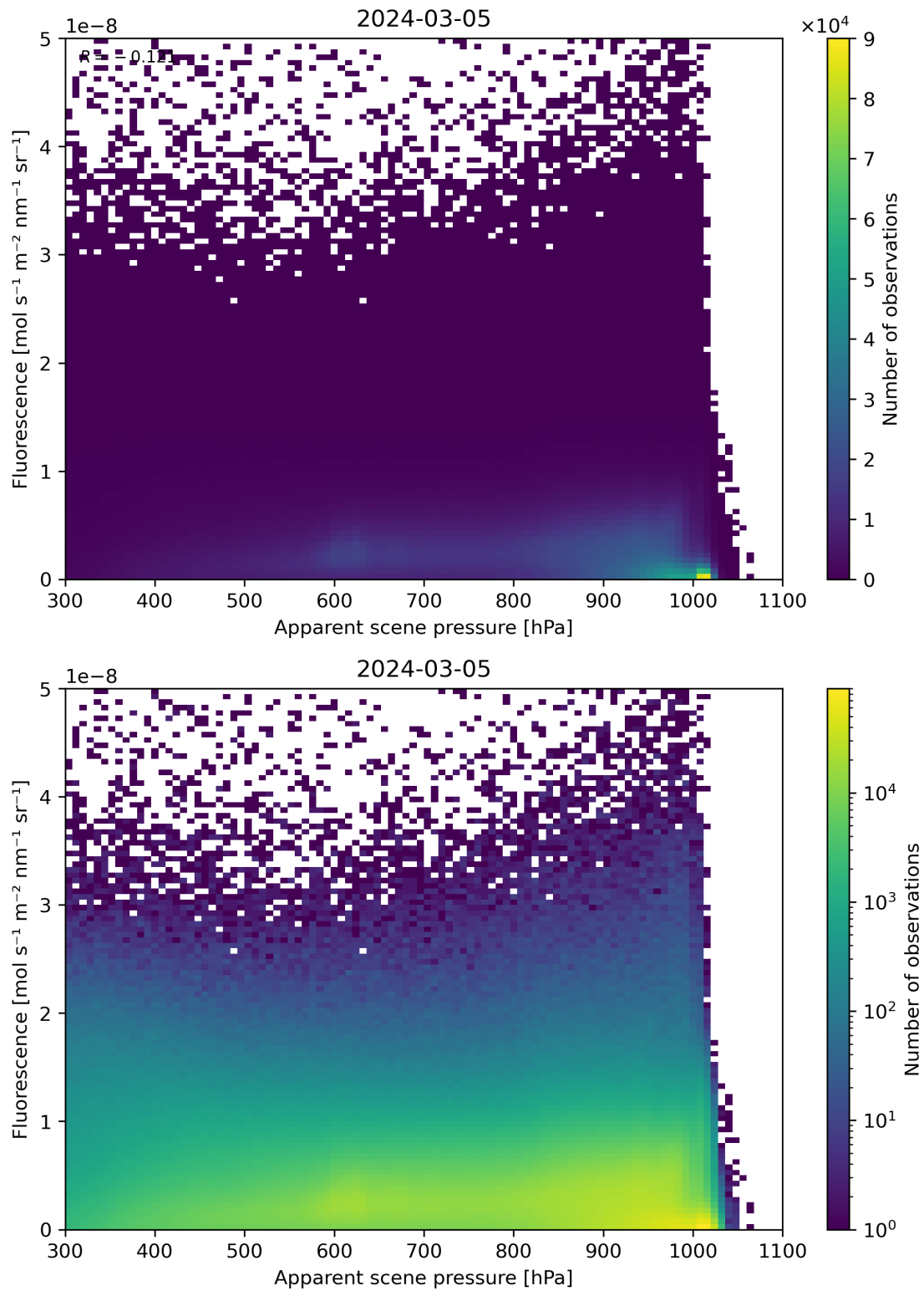
Figure 64: Scatter density plot of “Apparent scene pressure” against “Fluorescence” for 2024-03-04 to 2024-03-06.
