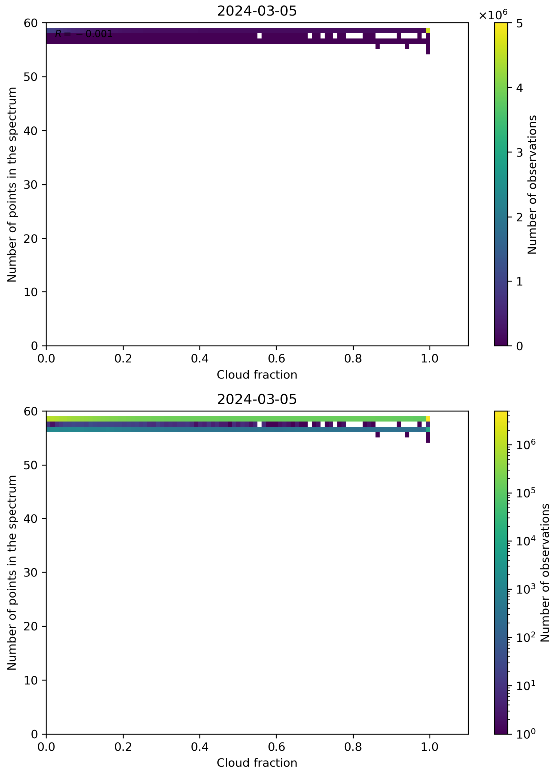
Figure 74: Scatter density plot of “Cloud fraction” against “Number of points in the spectrum” for 2024-03-04 to 2024-03-06.
