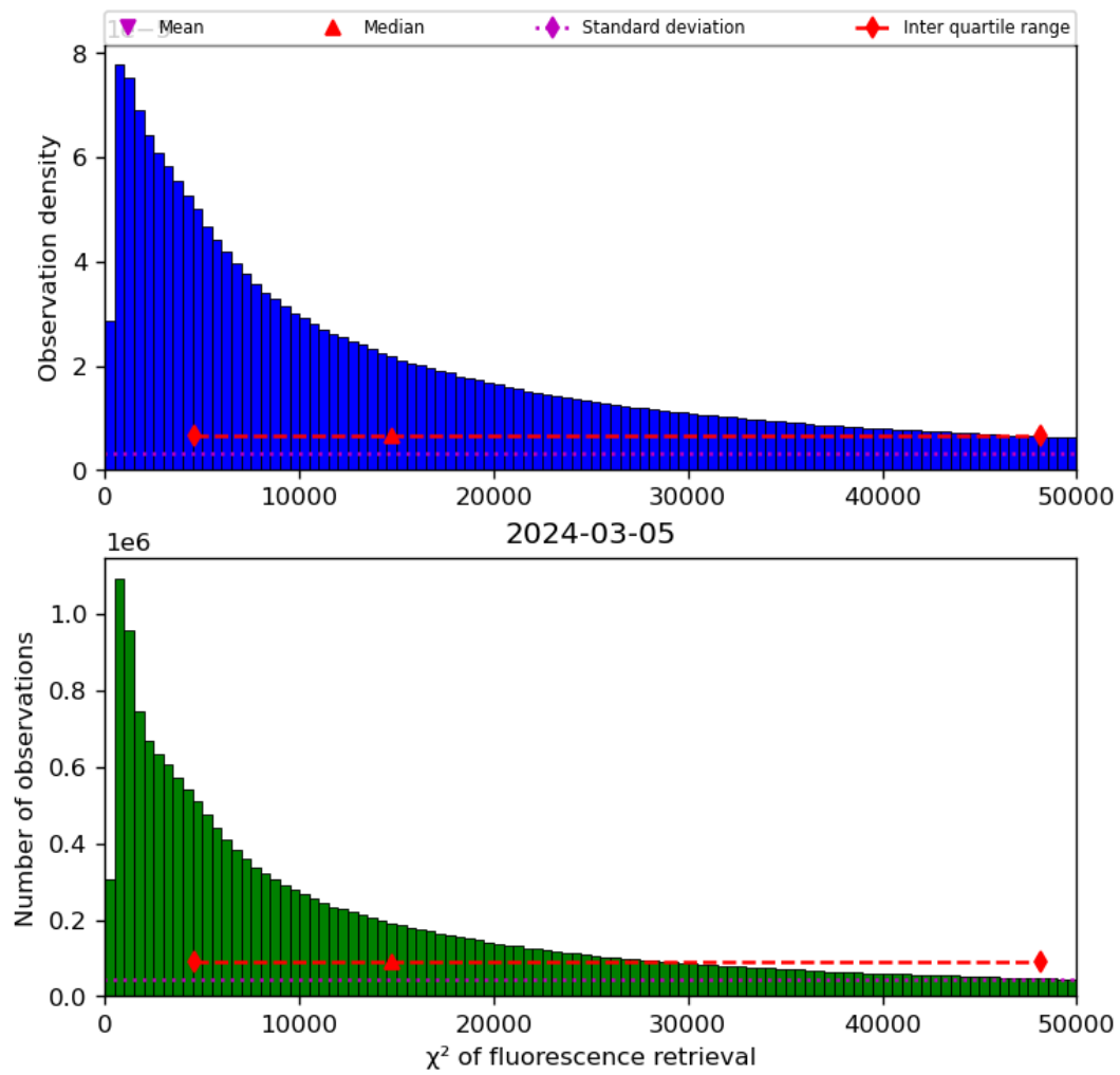
Figure 42: Histogram of “ \chi^2 of fluorescence retrieval” for 2024-03-04 to 2024-03-06
