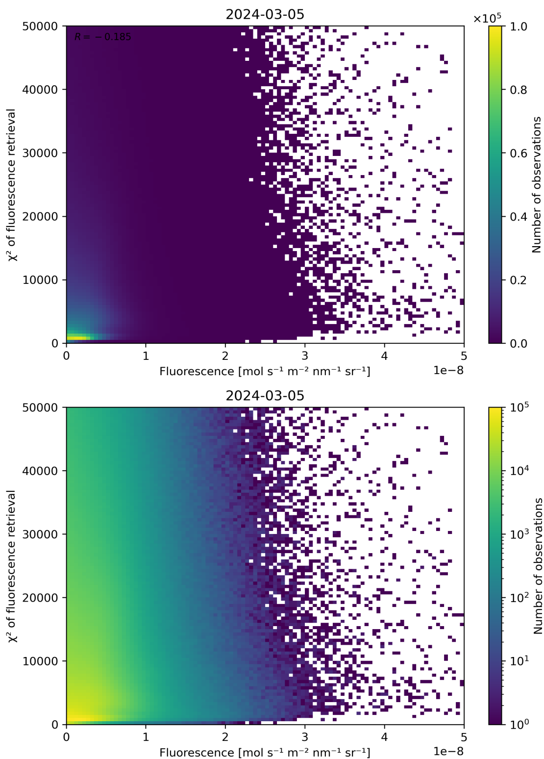
Figure 85: Scatter density plot of “Fluorescence” against “ \chi^2 of fluorescence retrieval” for 2024-03-04 to 2024-03-06.
