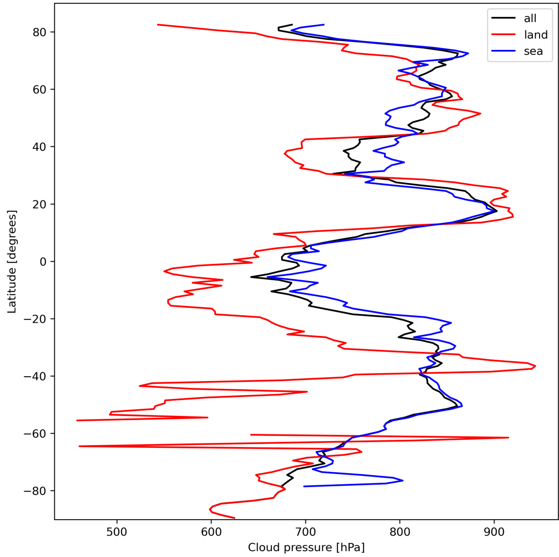
Figure 13: Zonal average of “Cloud pressure” for 2024-03-04 to 2024-03-06.
