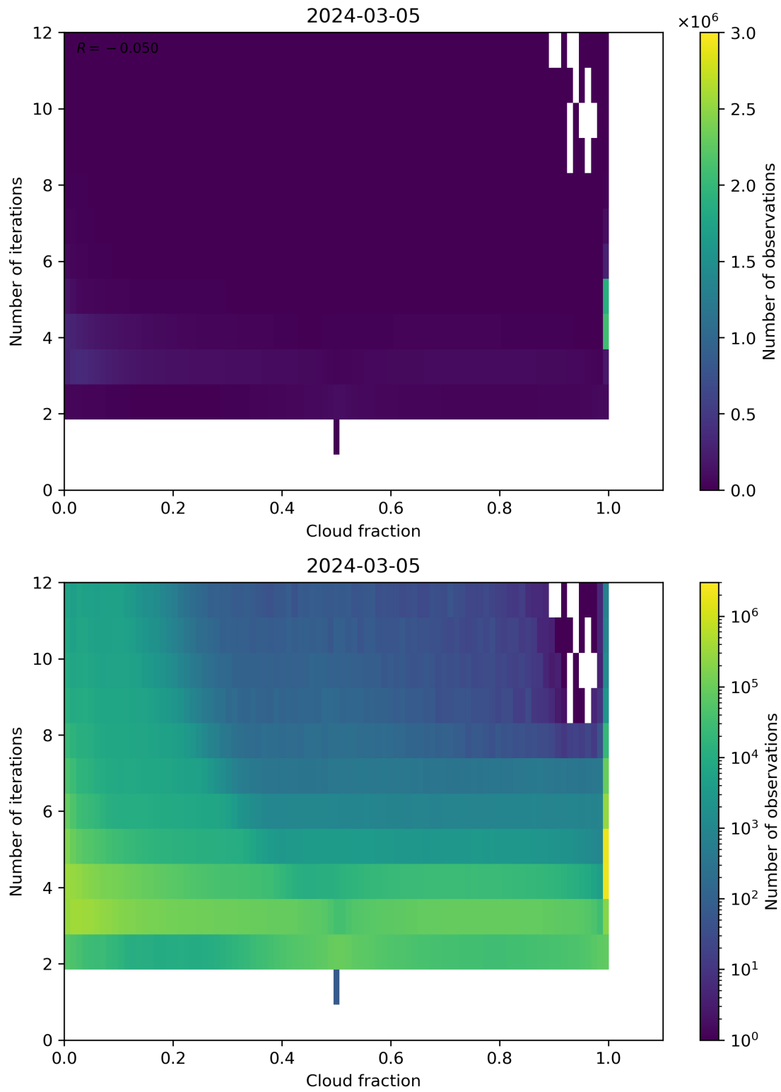
Figure 73: Scatter density plot of “Cloud fraction” against “Number of iterations” for 2024-03-04 to 2024-03-06.
