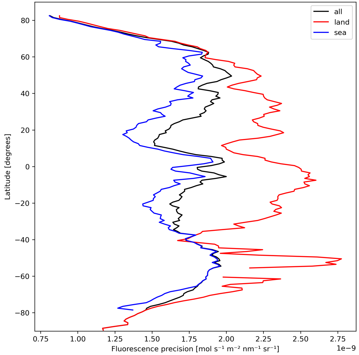
Figure 24: Zonal average of “Fluorescence precision” for 2024-03-04 to 2024-03-06.
