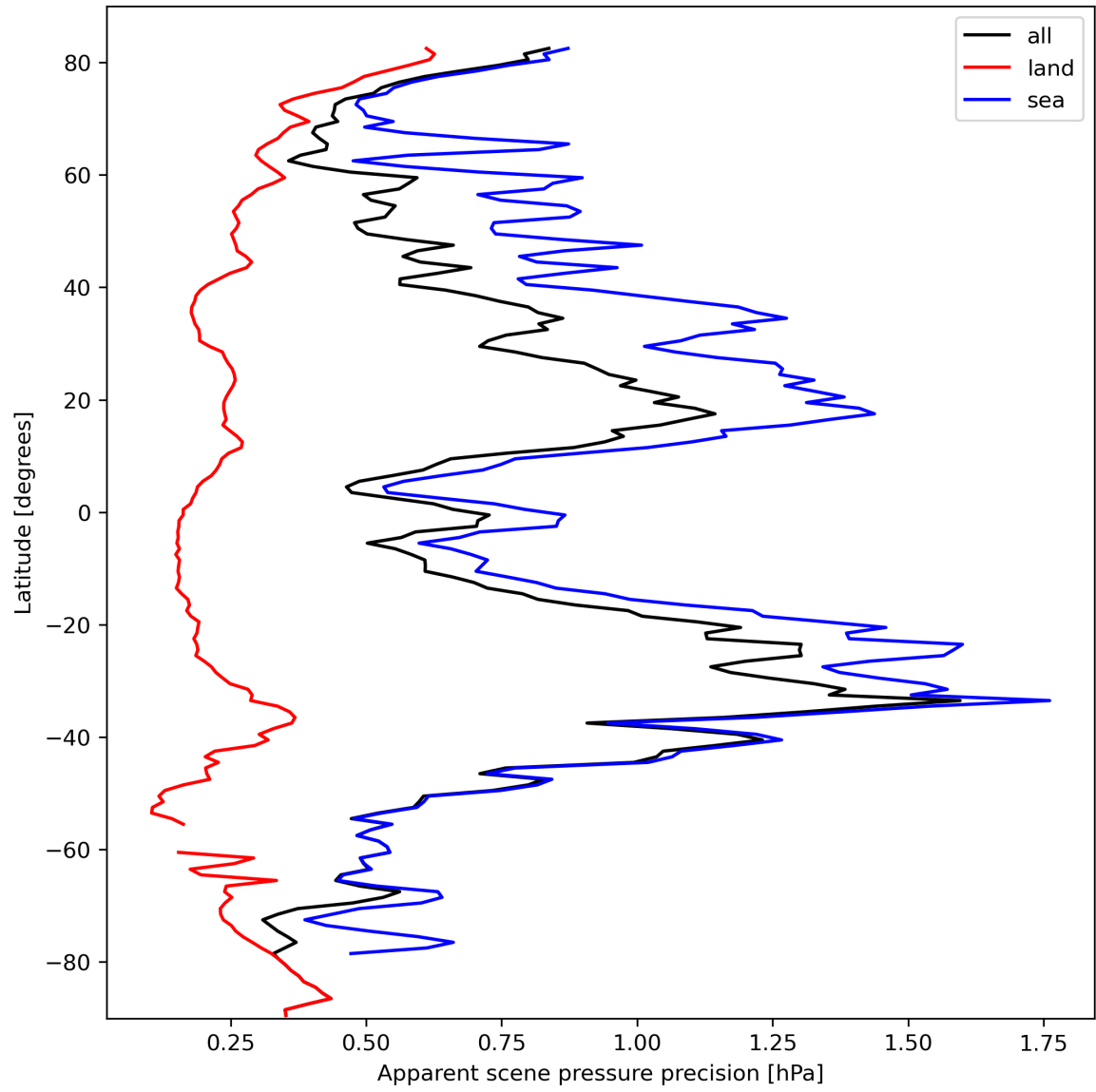
Figure 20: Zonal average of “Apparent scene pressure precision” for 2024-03-04 to 2024-03-06.
