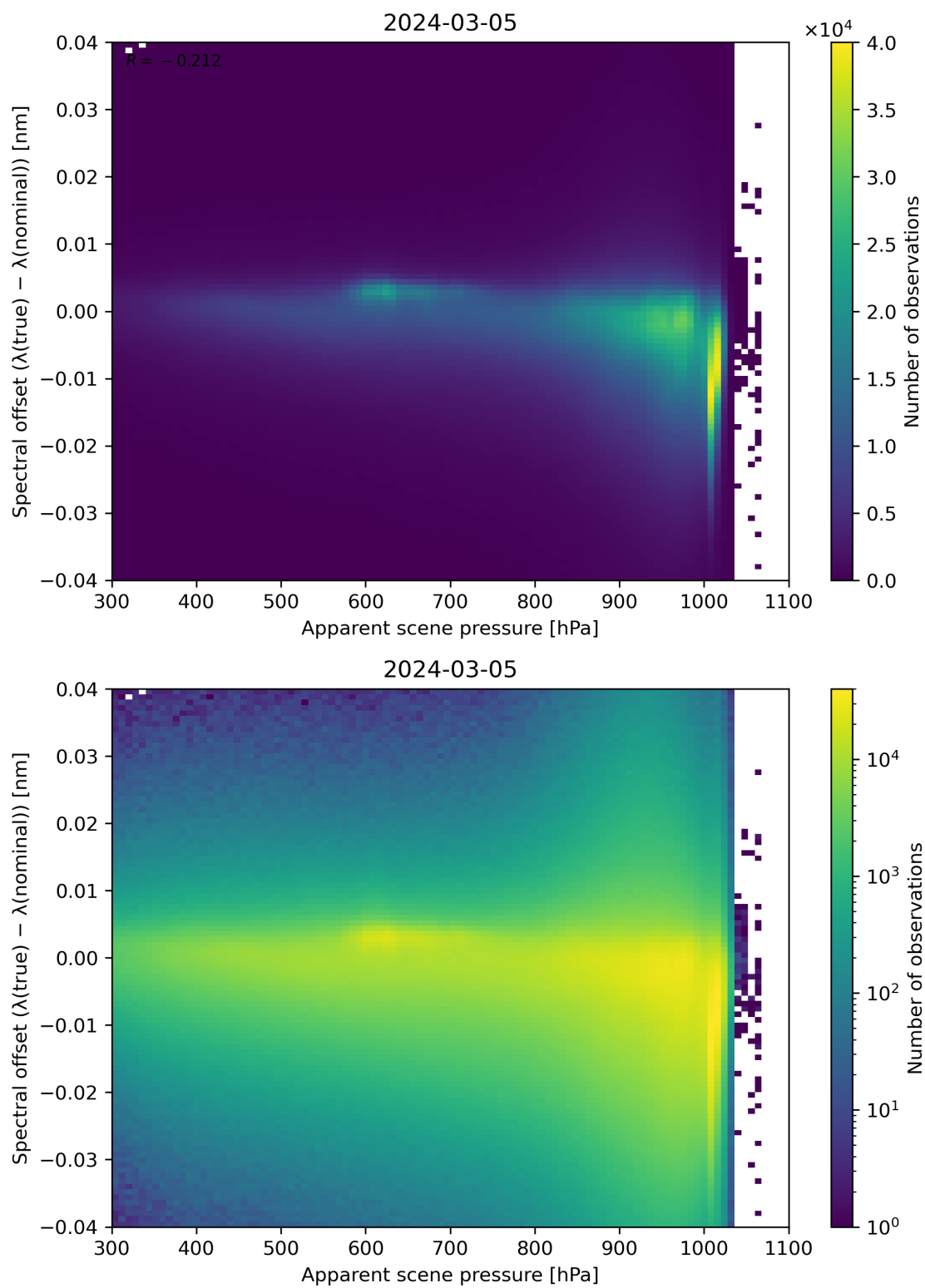
Figure 67: Scatter density plot of “Apparent scene pressure” against “Spectral offset ( \lambda(\text{true}) - \lambda(\text{nominal}) )” for 2024-03-04 to 2024-03-06.
