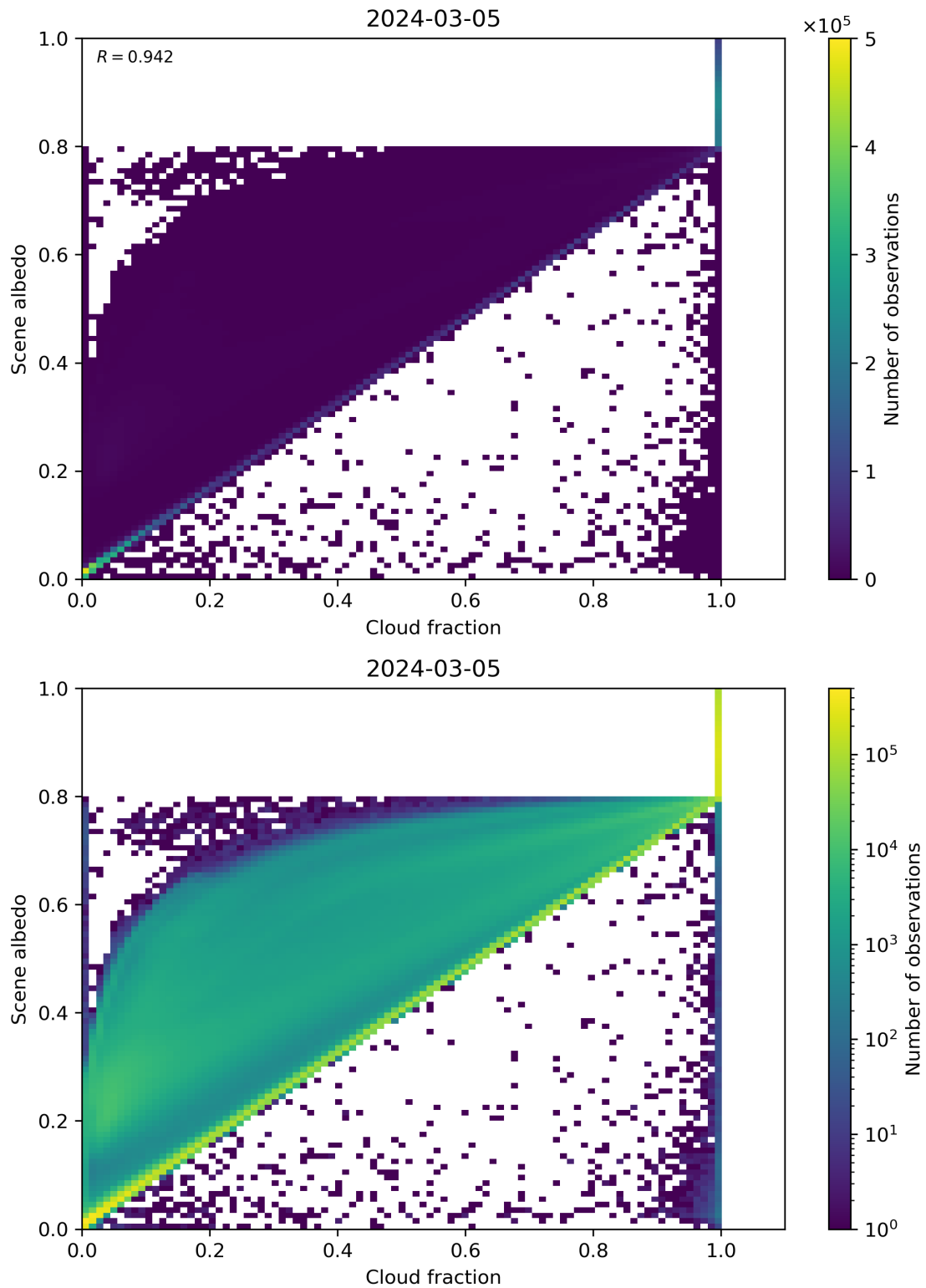
Figure 75: Scatter density plot of “Cloud fraction” against “Scene albedo” for 2024-03-04 to 2024-03-06.
