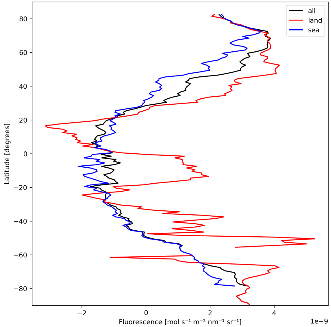
Figure 23: Zonal average of “Fluorescence” for 2024-03-04 to 2024-03-06.
