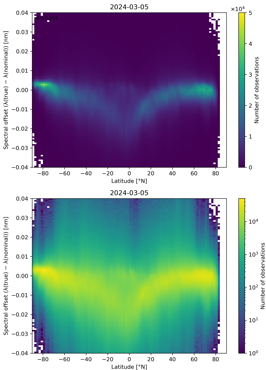
Figure 96: Scatter density plot of “Latitude” against “Spectral offset ( \lambda(\text{true}) - \lambda(\text{nominal}) )” for 2024-03-04 to 2024-03-06.
