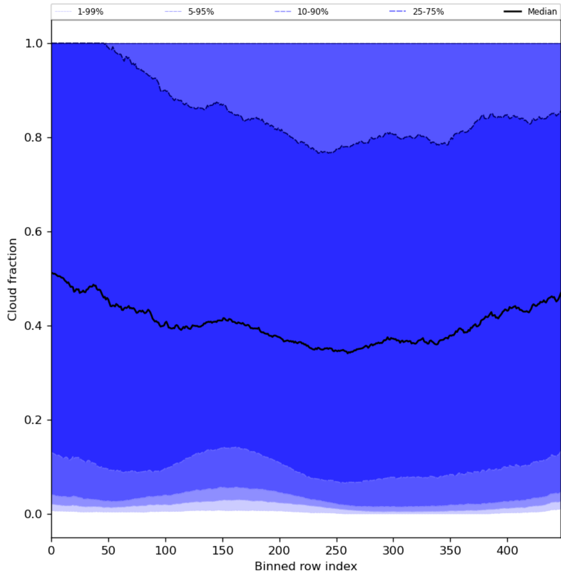
Figure 49: Along track statistics of “Cloud fraction” for 2024-03-04 to 2024-03-06
