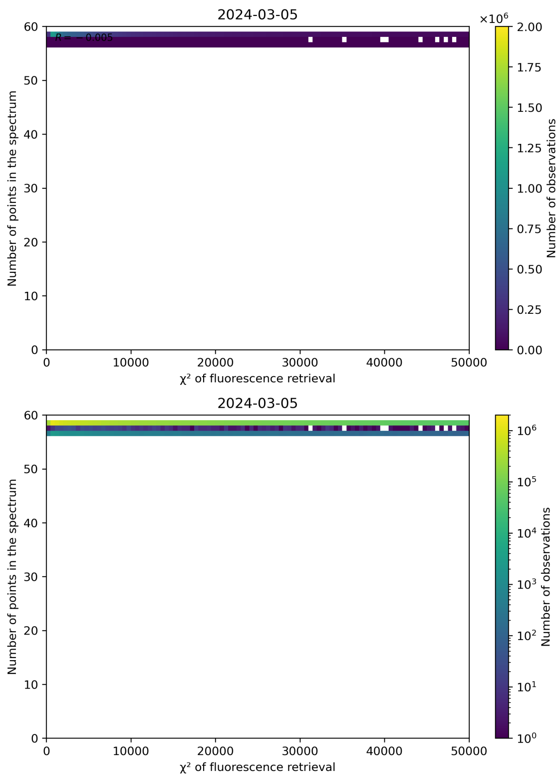
Figure 68: Scatter density plot of " \chi^2 of fluorescence retrieval" against "Number of points in the spectrum" for 2024-03-04 to 2024-03-06.
