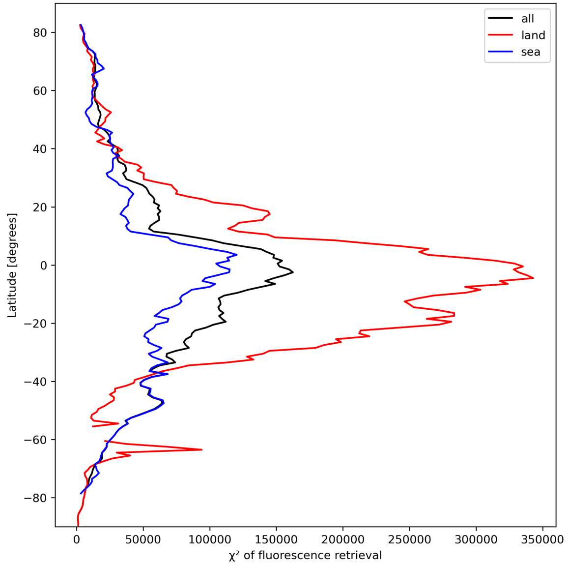
Figure 25: Zonal average of “ \chi^2 of fluorescence retrieval” for 2024-03-04 to 2024-03-06.
