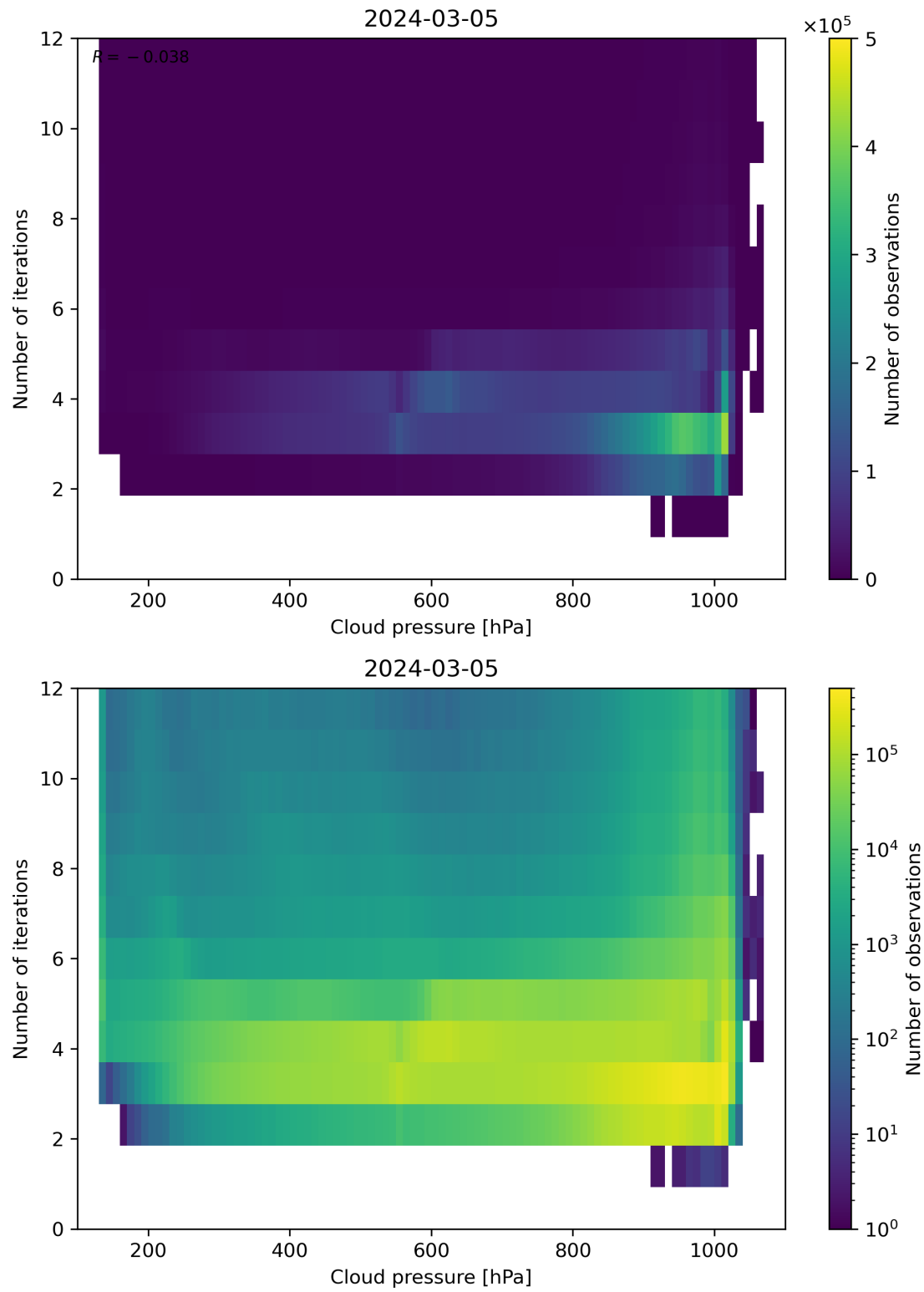
Figure 81: Scatter density plot of “Cloud pressure” against “Number of iterations” for 2024-03-04 to 2024-03-06.
