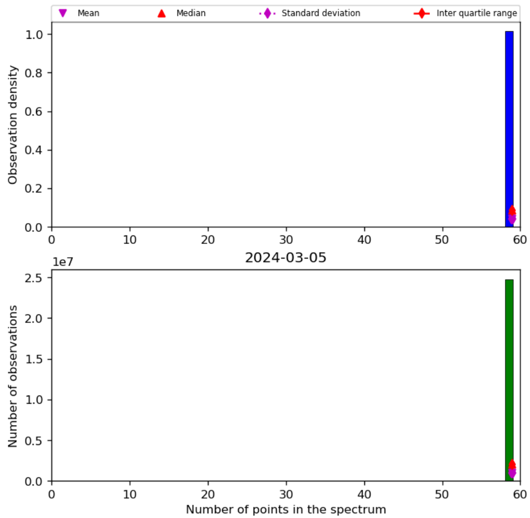
Figure 44: Histogram of “Number of points in the spectrum” for 2024-03-04 to 2024-03-06
