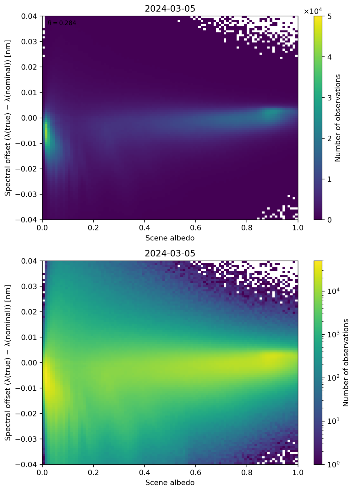
Figure 107: Scatter density plot of “Scene albedo” against “Spectral offset ( \lambda(\text{true}) - \lambda(\text{nominal}) )” for 2024-03-04 to 2024-03-06.
