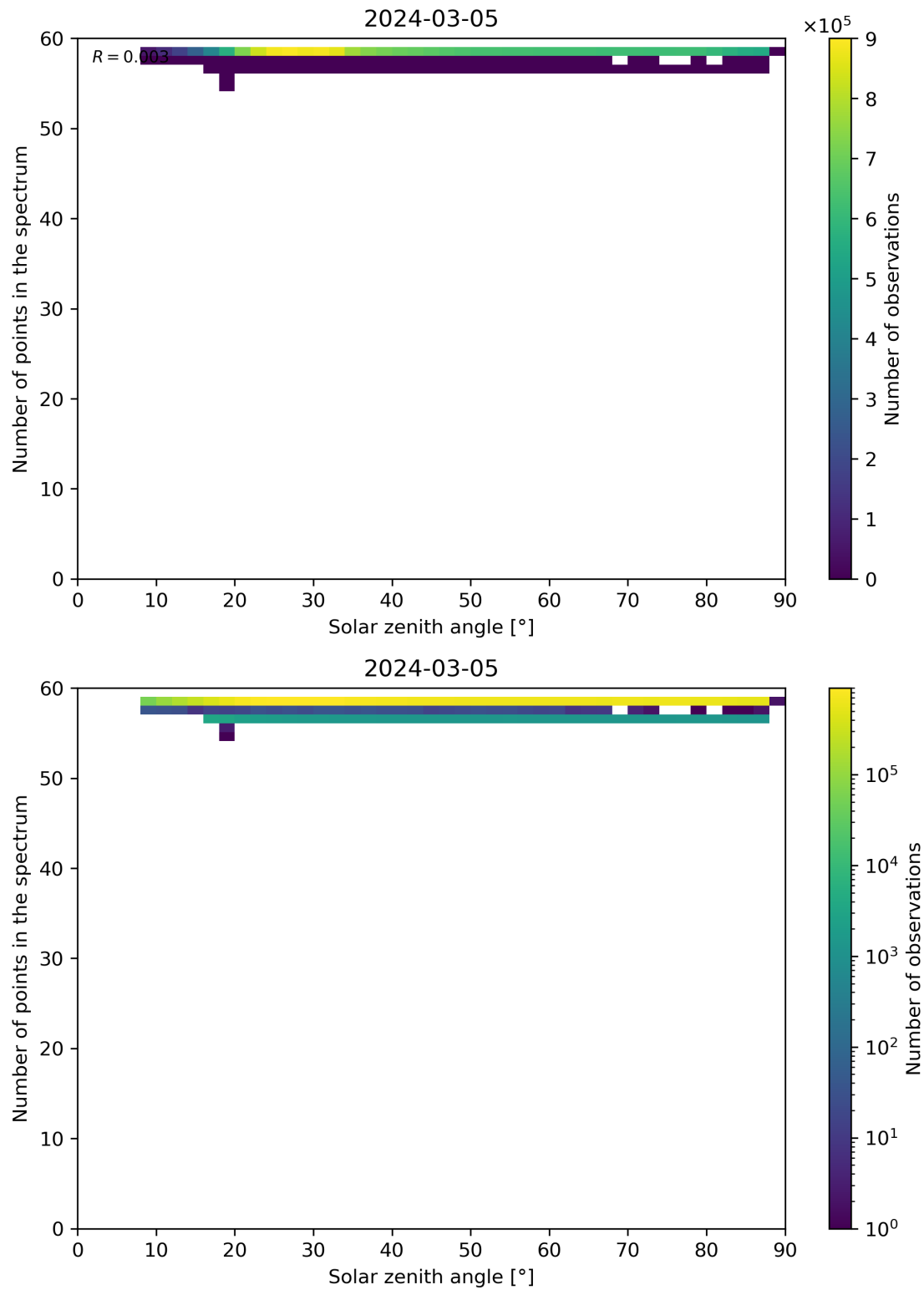
Figure 115: Scatter density plot of “Solar zenith angle” against “Number of points in the spectrum” for 2024-03-04 to 2024-03-06.
