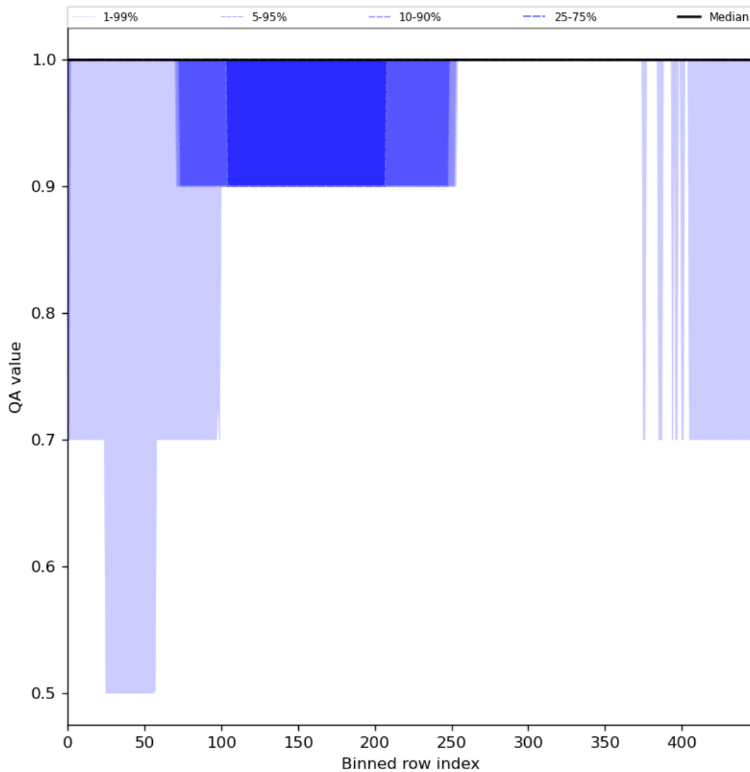
Figure 46: Along track statistics of “QA value” for 2024-03-04 to 2024-03-06
