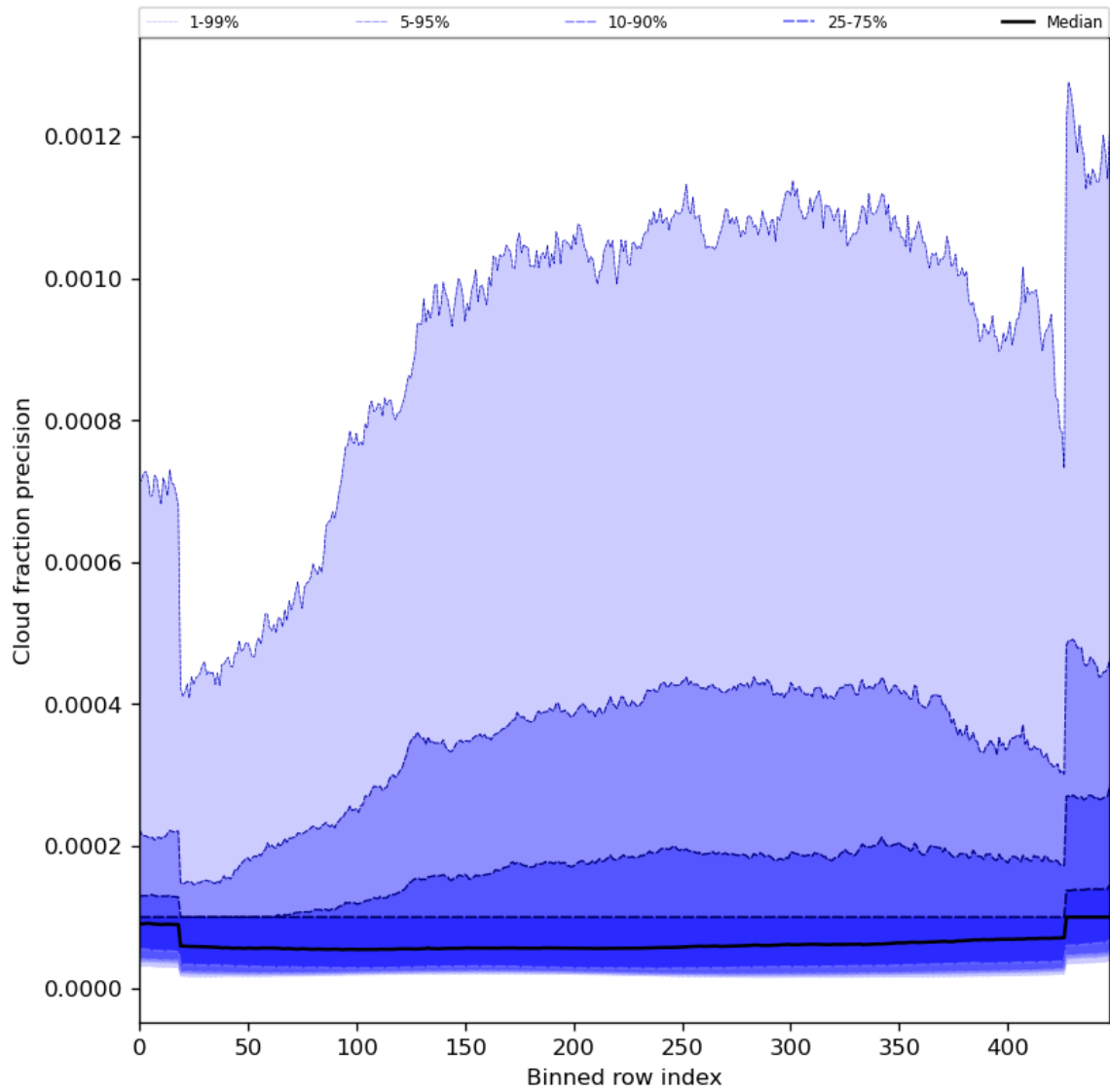
Figure 50: Along track statistics of “Cloud fraction precision” for 2024-03-04 to 2024-03-06
