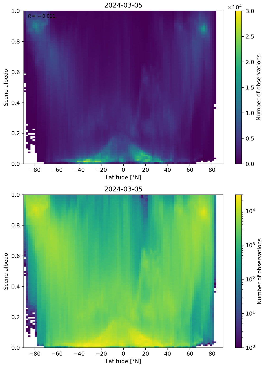
Figure 95: Scatter density plot of “Latitude” against “Scene albedo” for 2024-03-04 to 2024-03-06.
