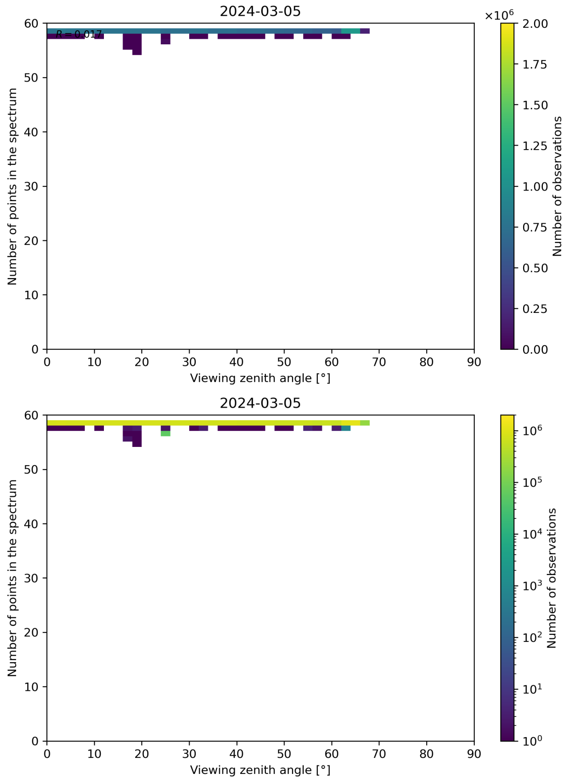
Figure 125: Scatter density plot of “Viewing zenith angle” against “Number of points in the spectrum” for 2024-03-04 to 2024-03-06.
