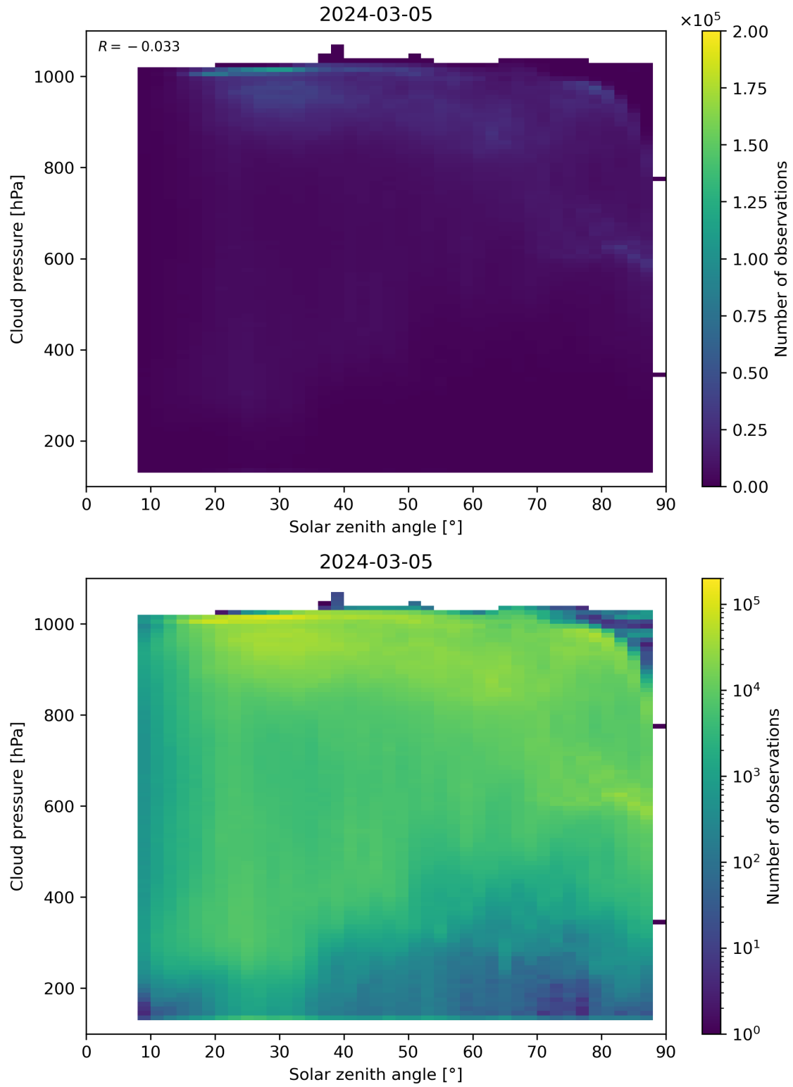
Figure 111: Scatter density plot of “Solar zenith angle” against “Cloud pressure” for 2024-03-04 to 2024-03-06.
