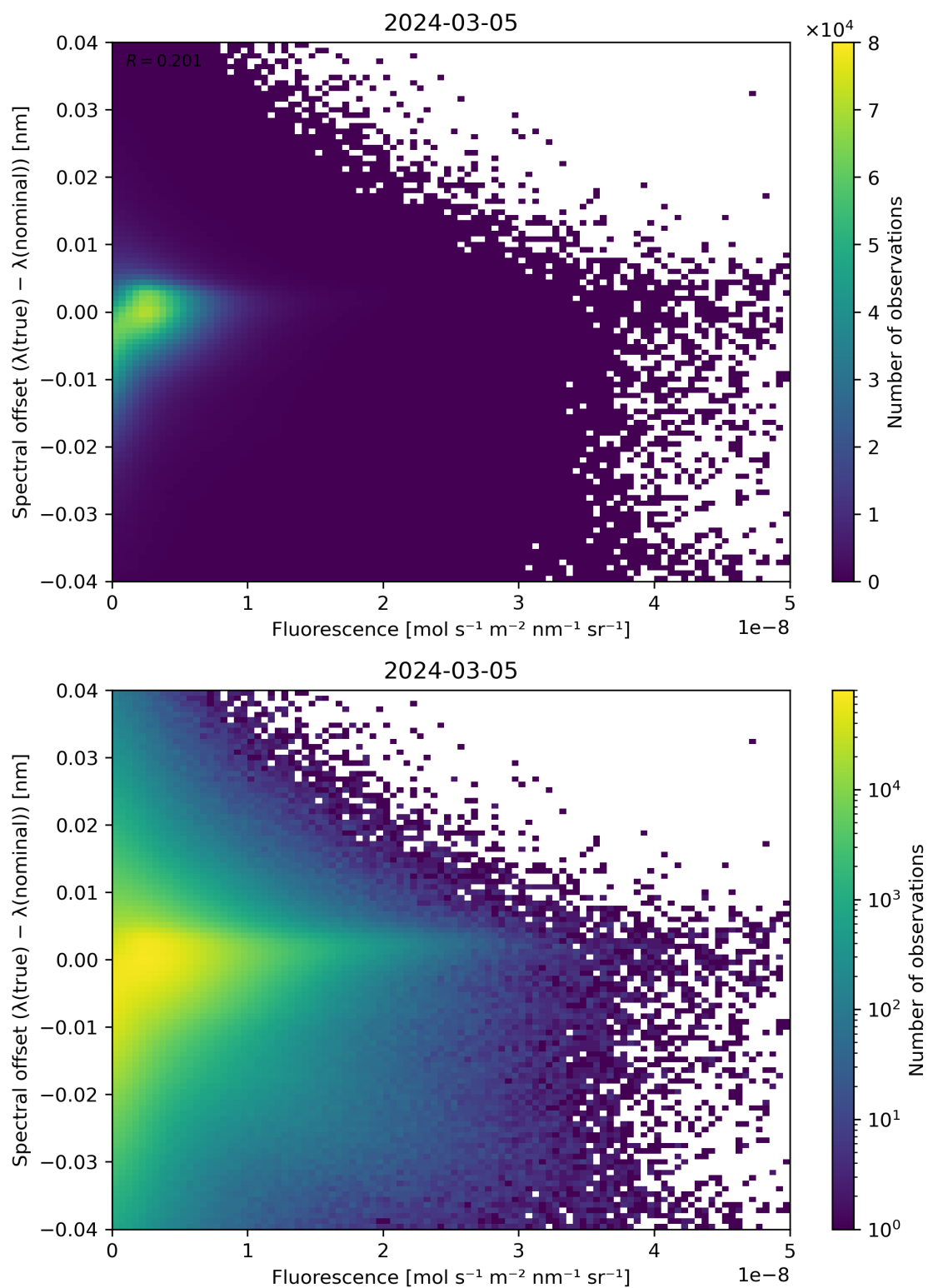
Figure 87: Scatter density plot of “Fluorescence” against “Spectral offset ( \lambda(\text{true}) - \lambda(\text{nominal}) )” for 2024-03-04 to 2024-03-06.
