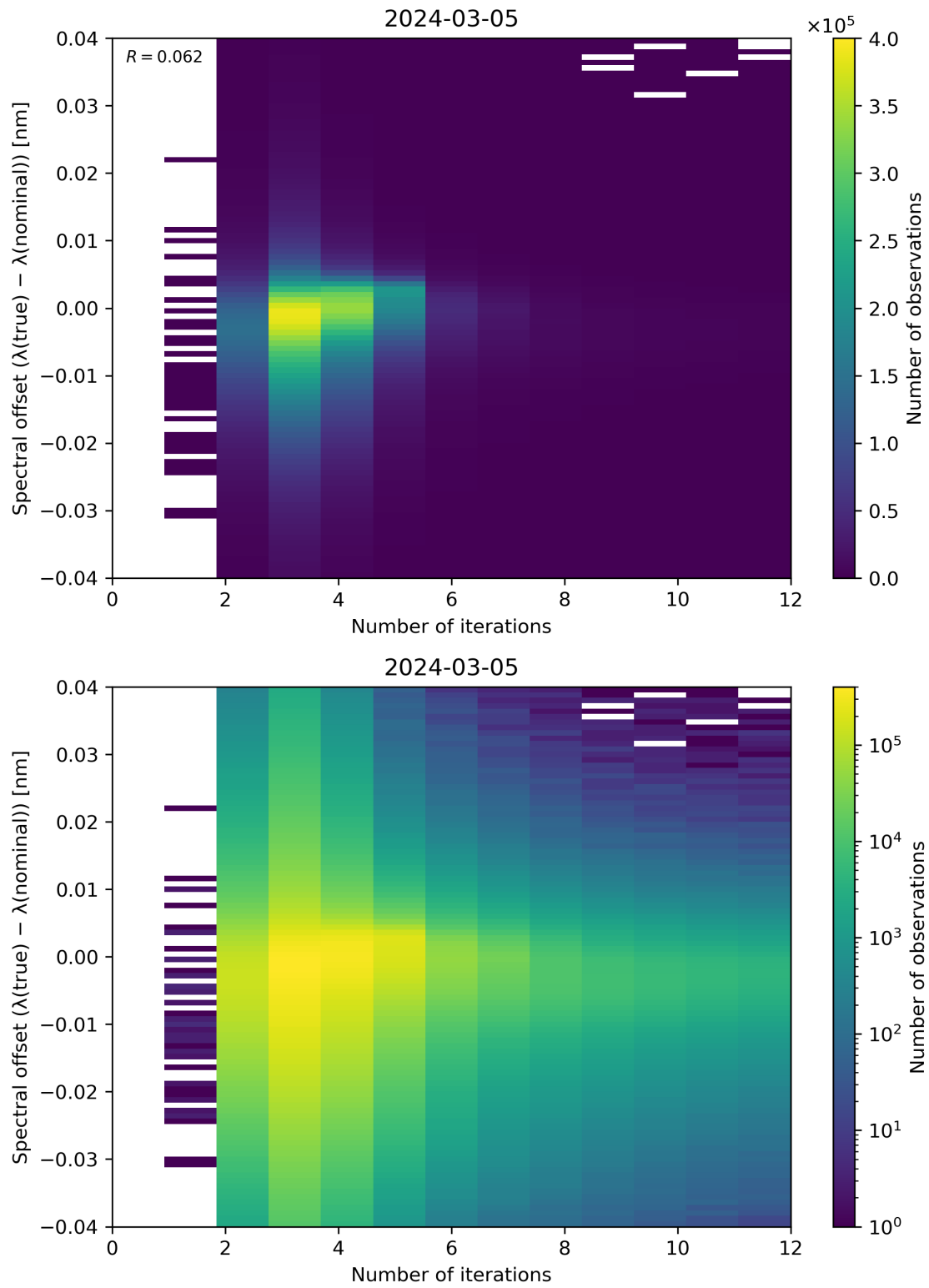
Figure 100: Scatter density plot of “Number of iterations” against “Spectral offset ( \lambda(\text{true}) - \lambda(\text{nominal}) )” for 2024-03-04 to 2024-03-06.
