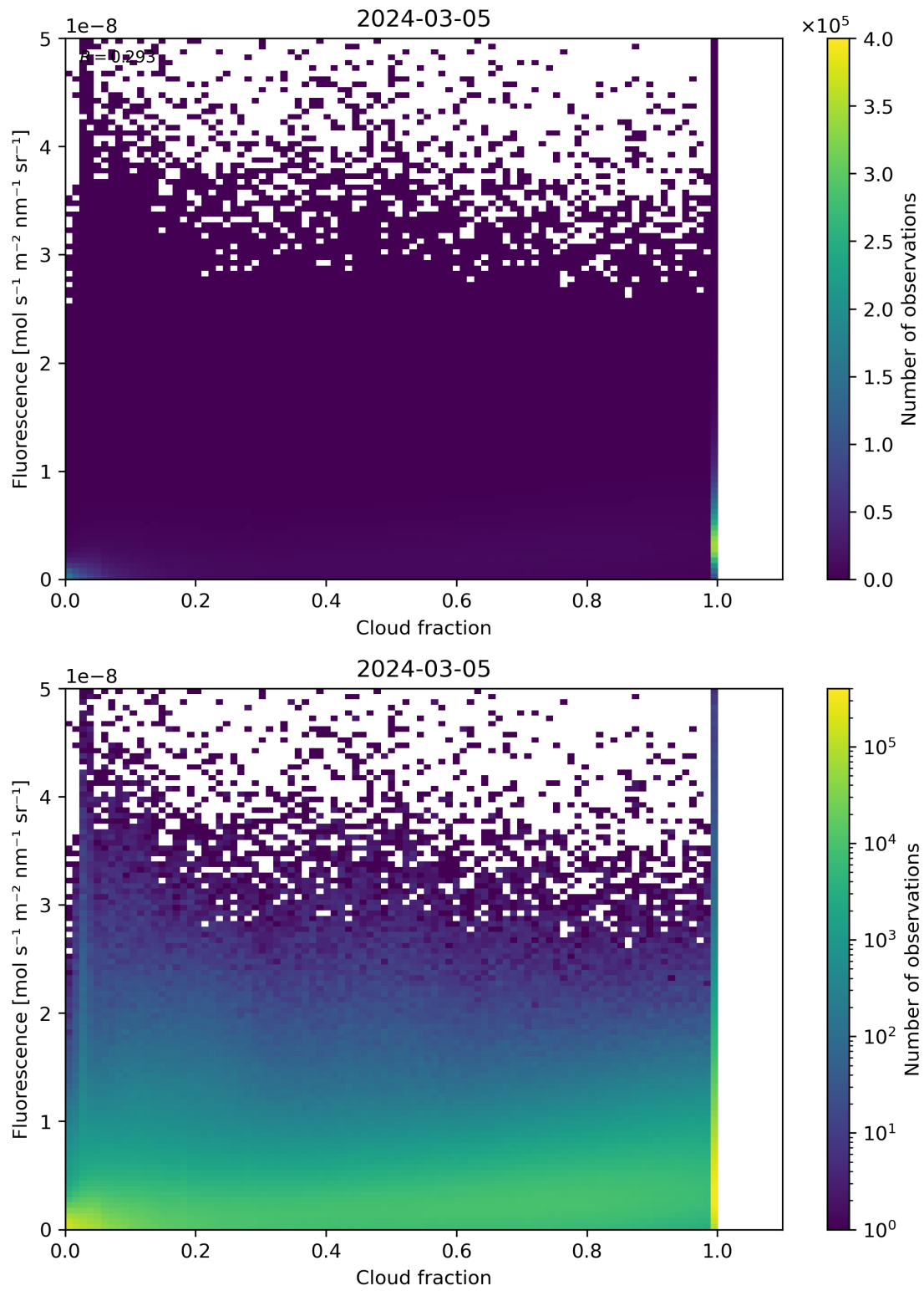
Figure 72: Scatter density plot of “Cloud fraction” against “Fluorescence” for 2024-03-04 to 2024-03-06.
