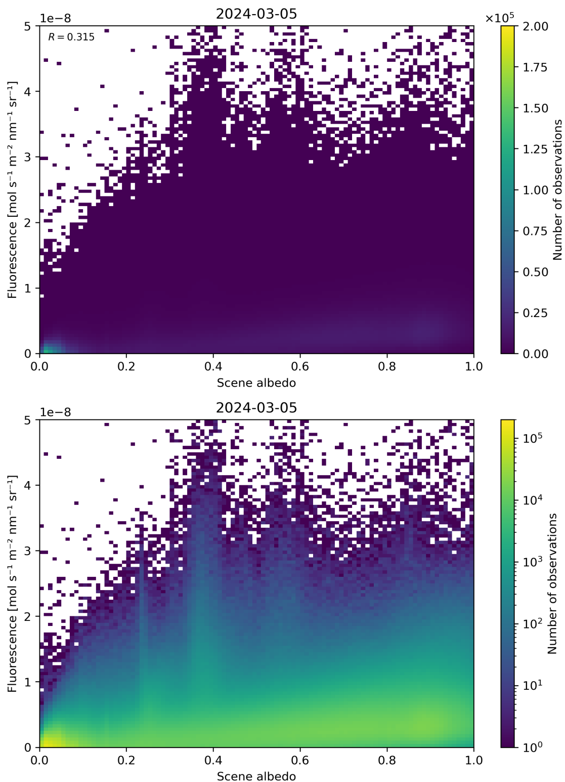
Figure 104: Scatter density plot of “Scene albedo” against “Fluorescence” for 2024-03-04 to 2024-03-06.
