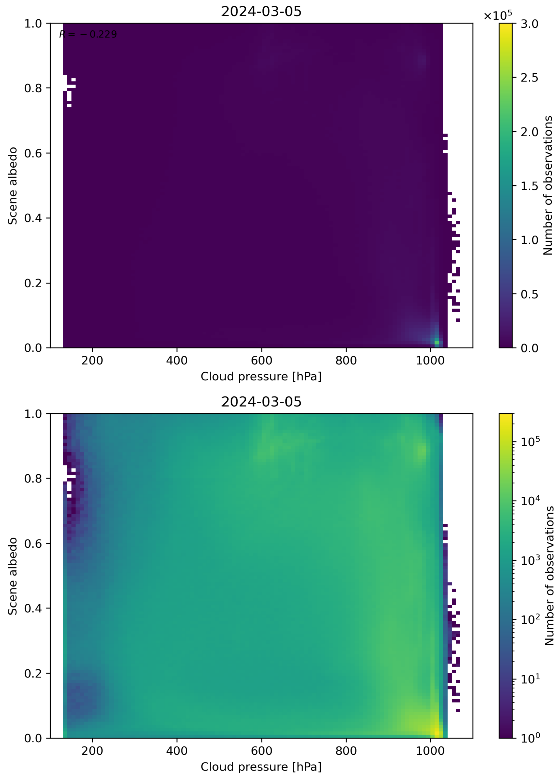
Figure 83: Scatter density plot of “Cloud pressure” against “Scene albedo” for 2024-03-04 to 2024-03-06.
