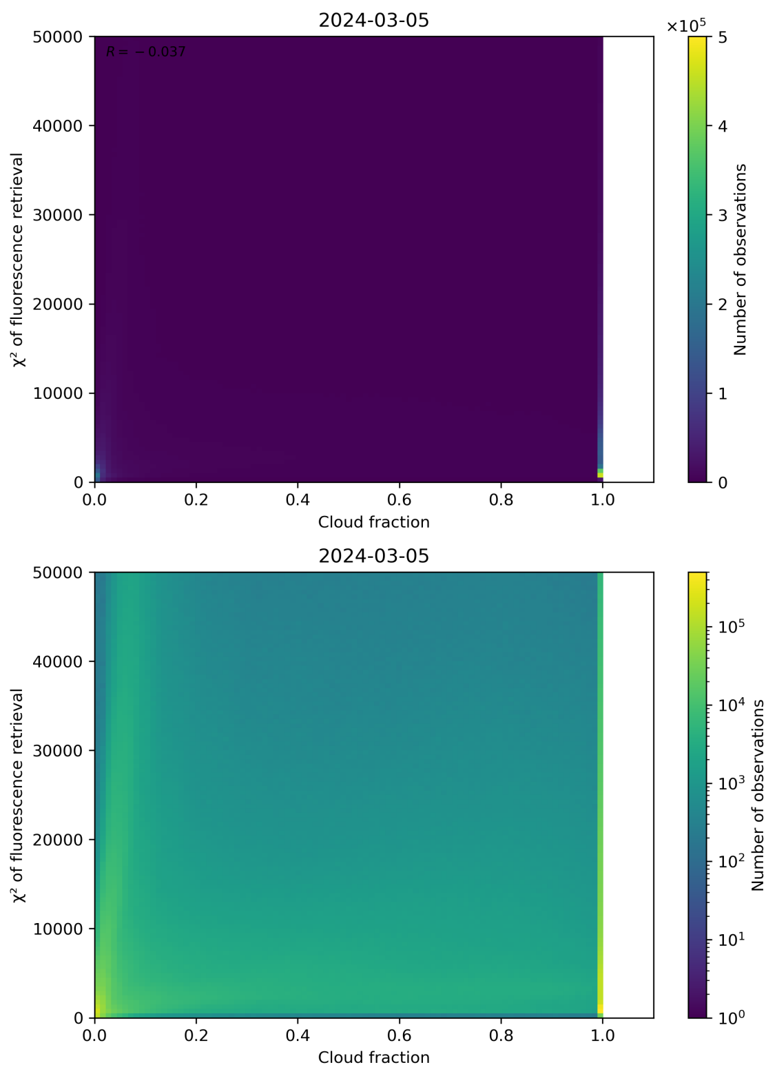
Figure 71: Scatter density plot of “Cloud fraction” against “ \chi^2 of fluorescence retrieval” for 2024-03-04 to 2024-03-06.
