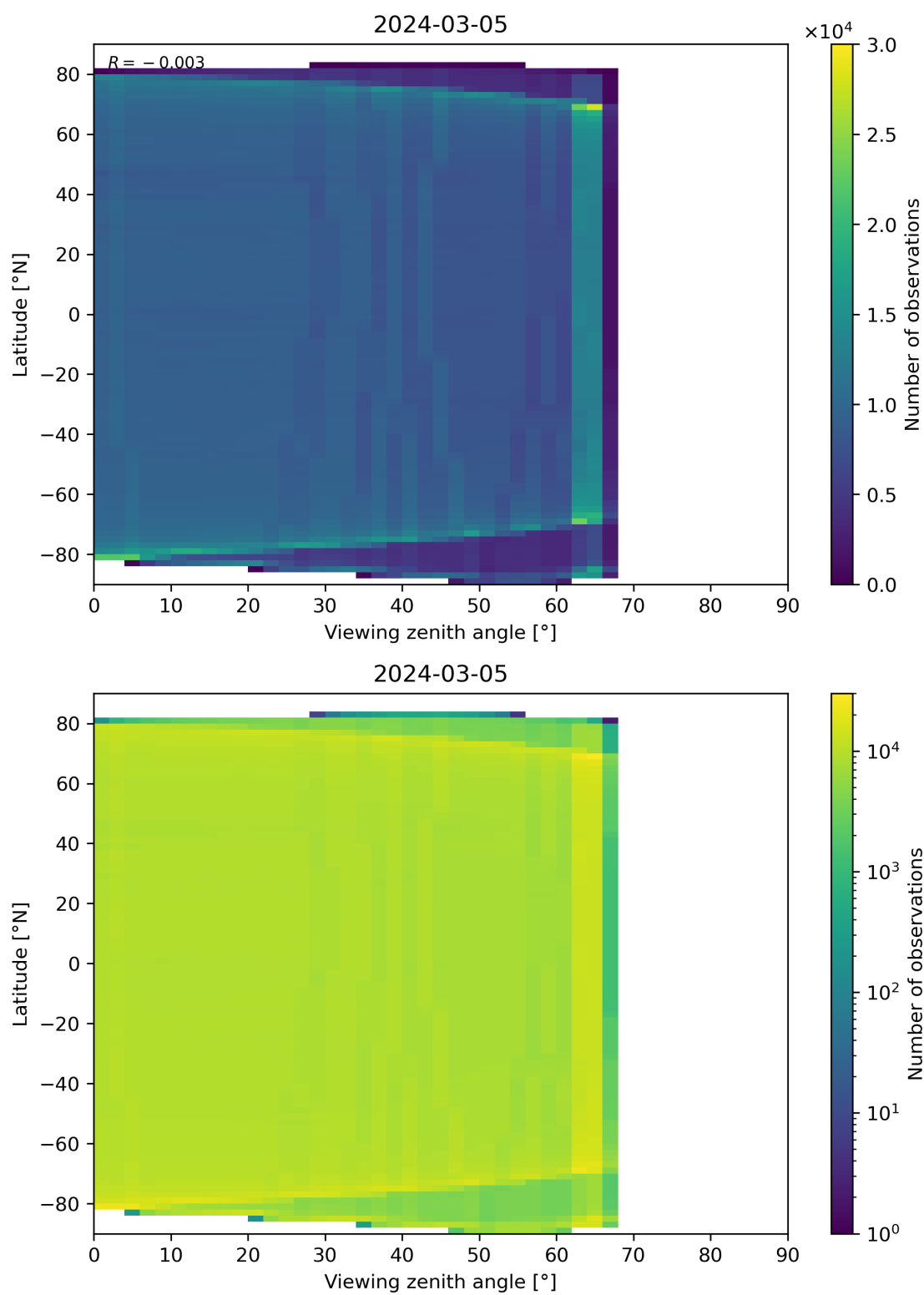
Figure 123: Scatter density plot of “Viewing zenith angle” against “Latitude” for 2024-03-04 to 2024-03-06.
