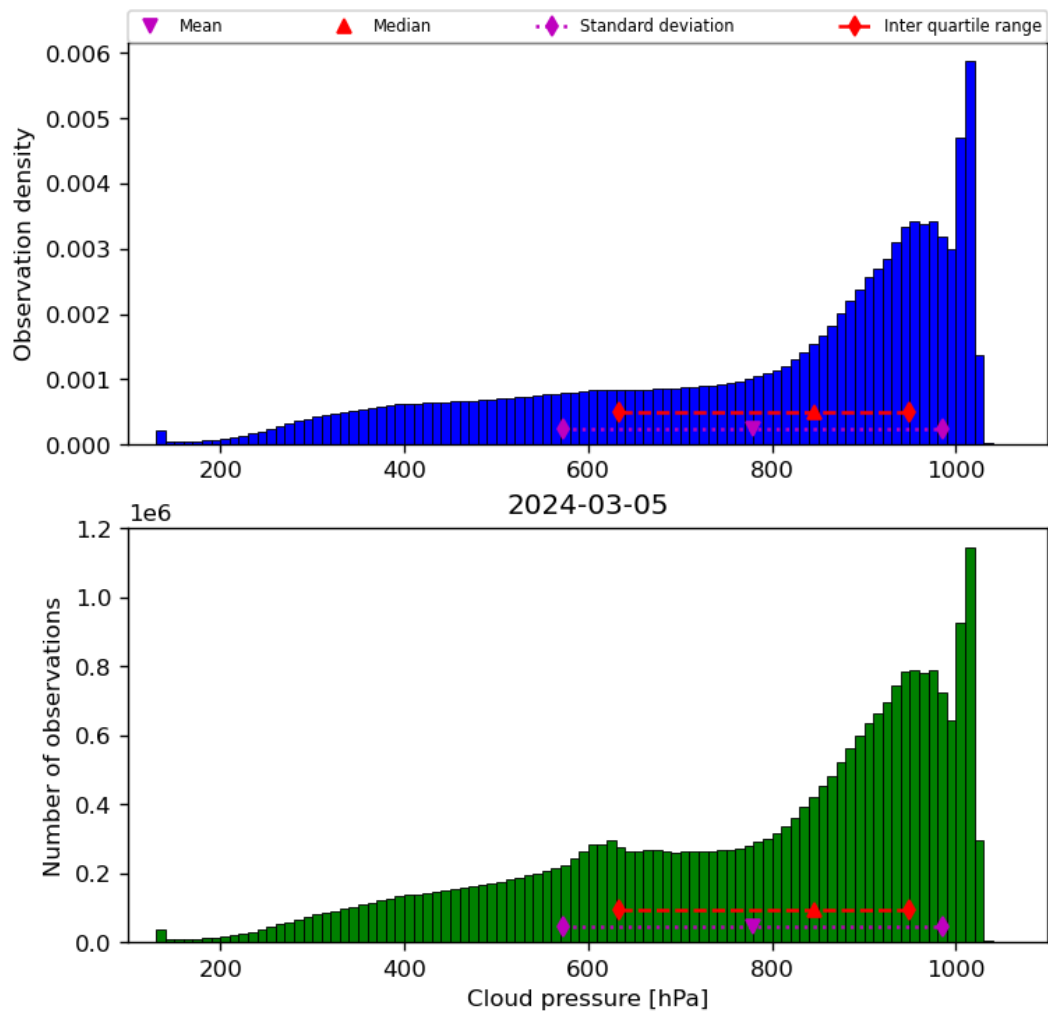
Figure 30: Histogram of “Cloud pressure” for 2024-03-04 to 2024-03-06
