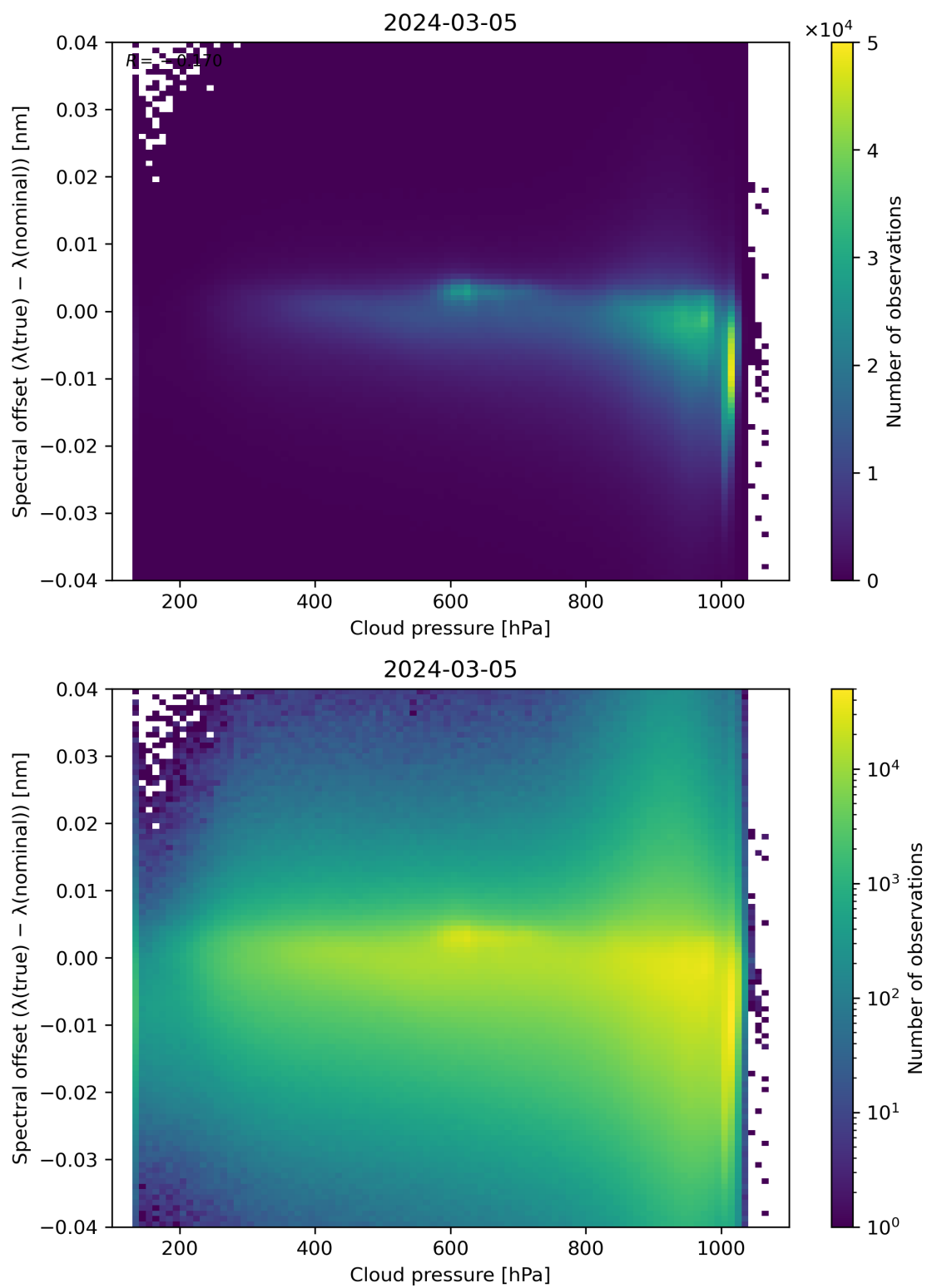
Figure 84: Scatter density plot of “Cloud pressure” against “Spectral offset ( \lambda(\text{true}) - \lambda(\text{nominal}) )” for 2024-03-04 to 2024-03-06.
