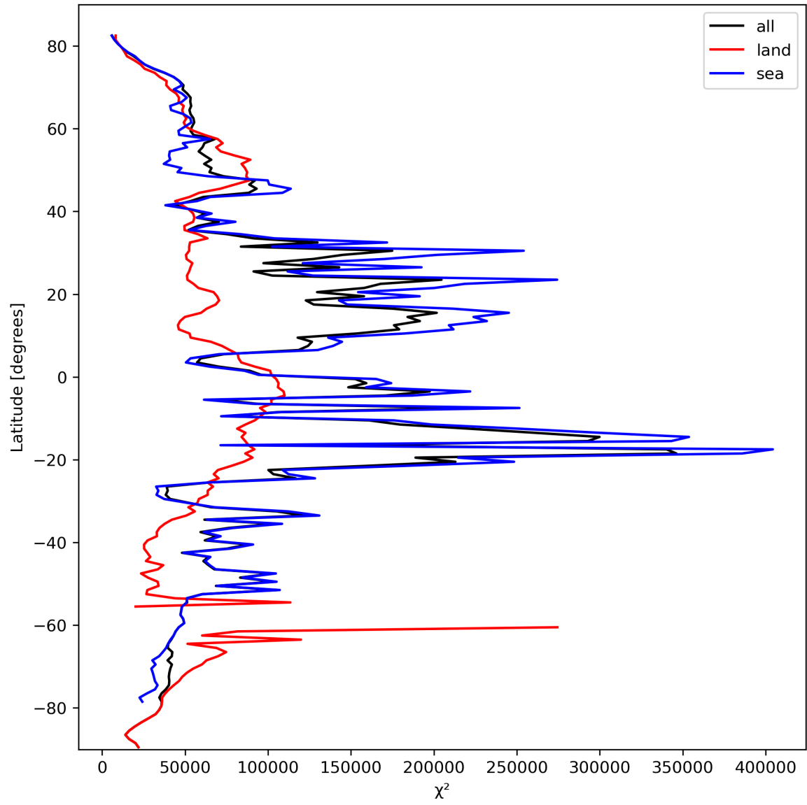
Figure 21: Zonal average of “ \chi^2 ” for 2024-03-04 to 2024-03-06.
