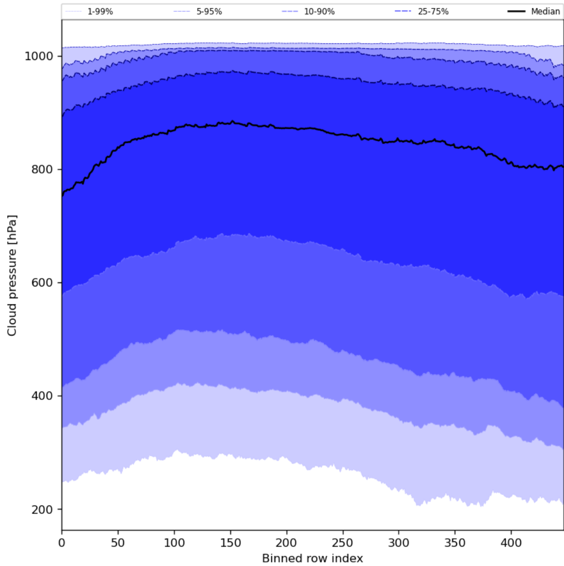
Figure 47: Along track statistics of “Cloud pressure” for 2024-03-04 to 2024-03-06
