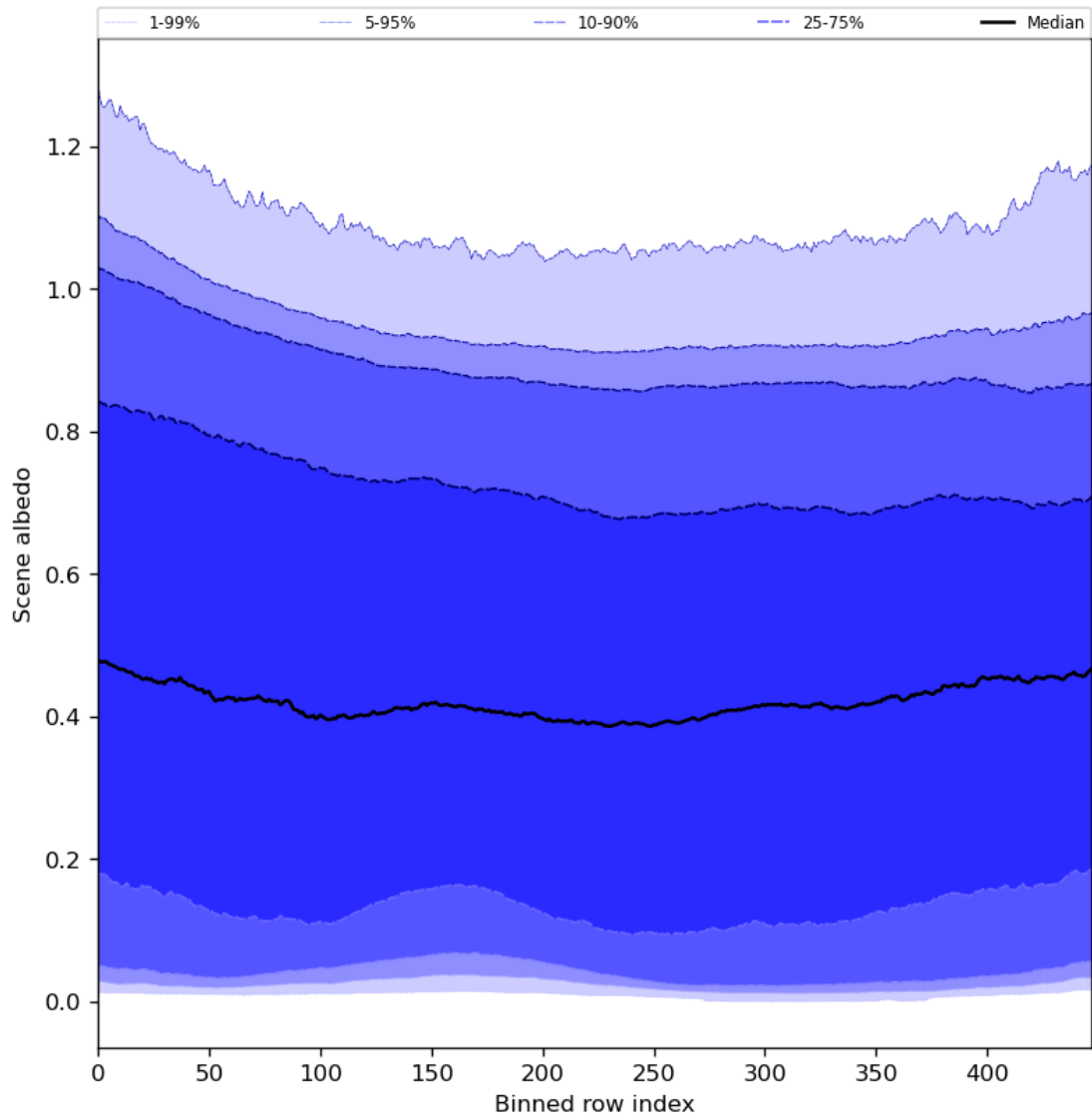
Figure 51: Along track statistics of “Scene albedo” for 2024-03-04 to 2024-03-06
