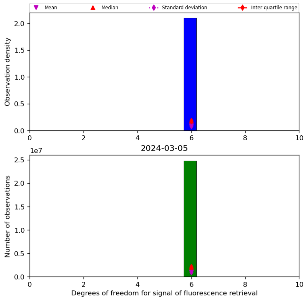
Figure 43: Histogram of “Degrees of freedom for signal of fluorescence retrieval” for 2024-03-04 to 2024-03-06
