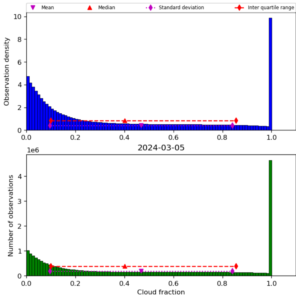
Figure 32: Histogram of “Cloud fraction” for 2024-03-04 to 2024-03-06
