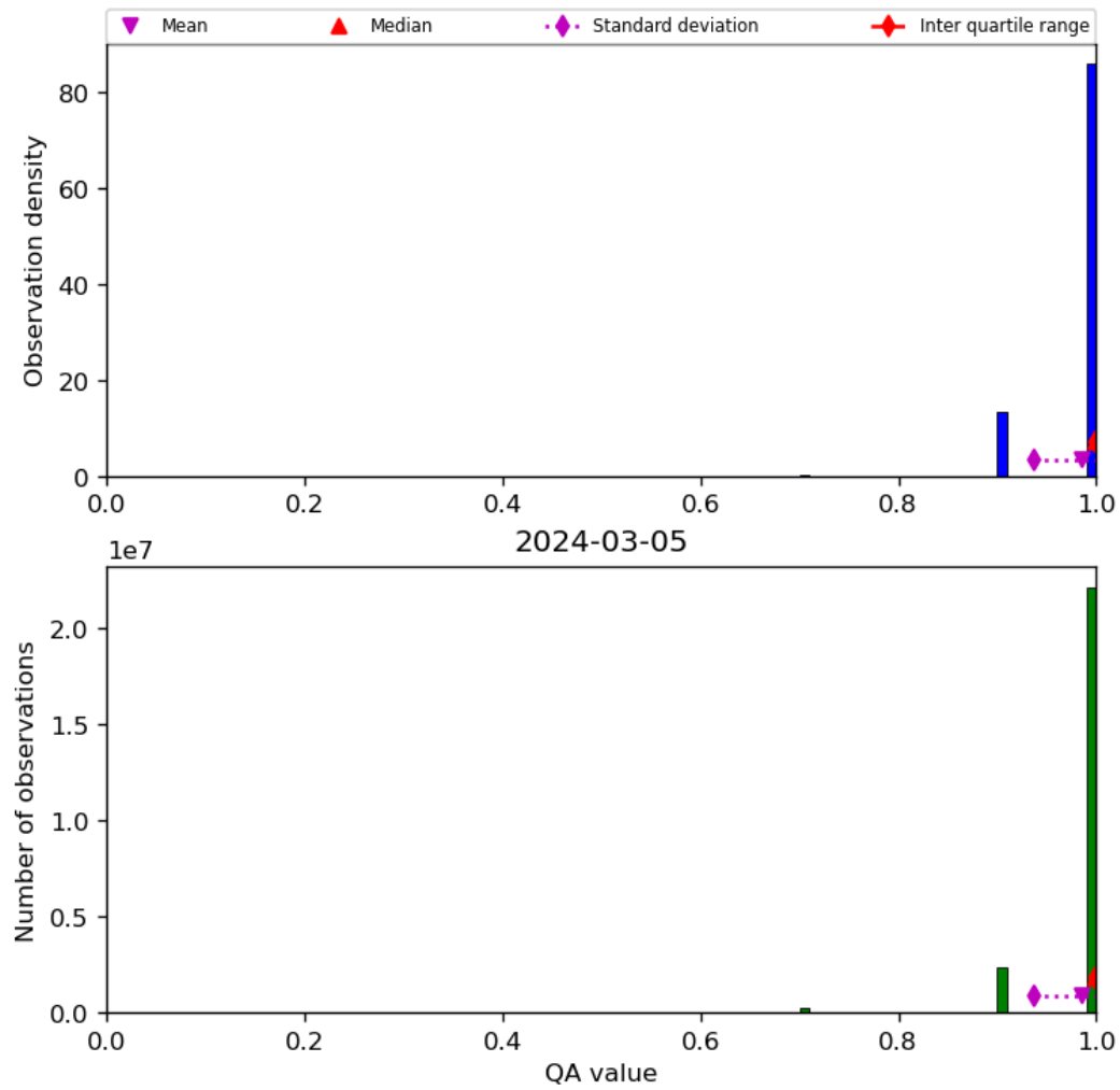
Figure 29: Histogram of “QA value” for 2024-03-04 to 2024-03-06
