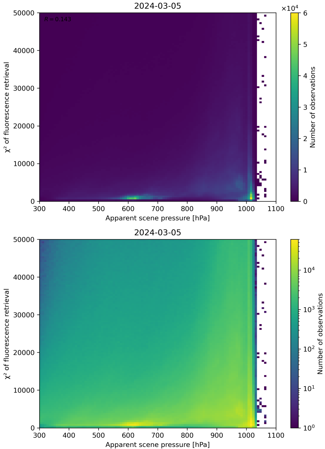
Figure 63: Scatter density plot of “Apparent scene pressure” against “ \chi^2 of fluorescence retrieval” for 2024-03-04 to 2024-03-06.
