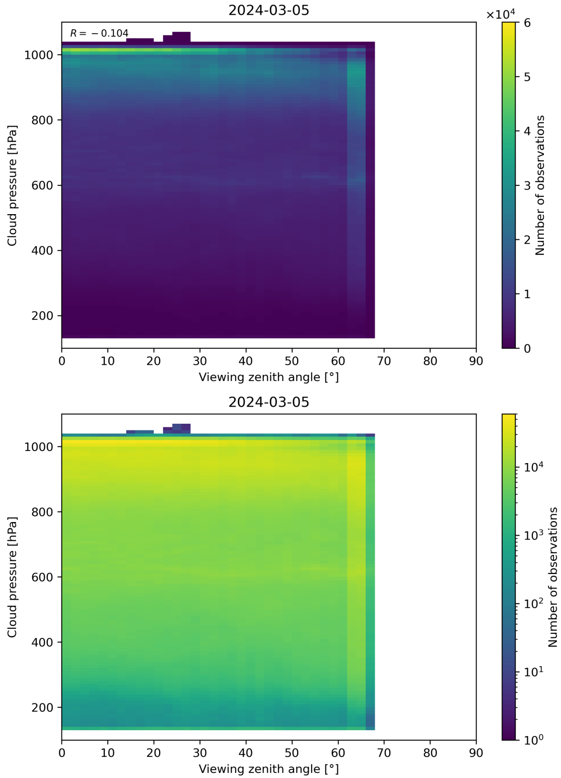
Figure 121: Scatter density plot of “Viewing zenith angle” against “Cloud pressure” for 2024-03-04 to 2024-03-06.
