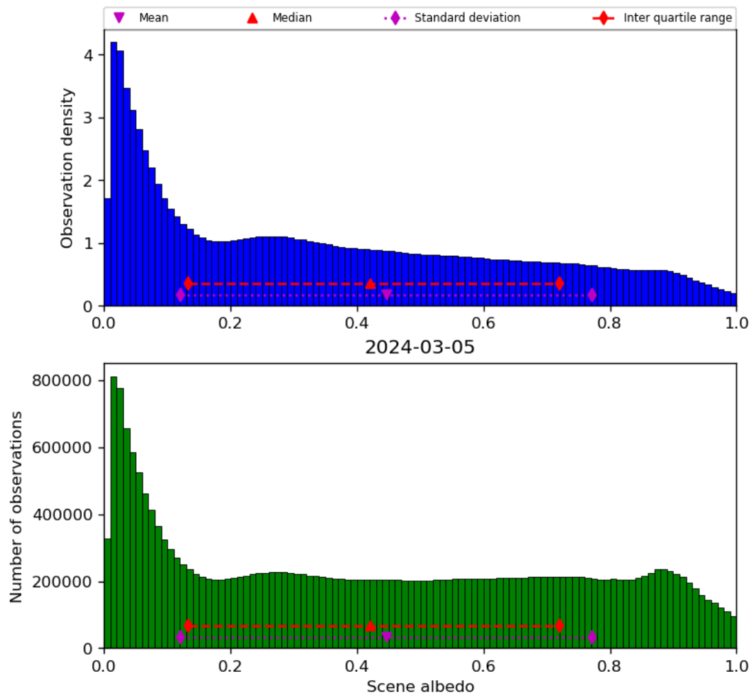
Figure 34: Histogram of “Scene albedo” for 2024-03-04 to 2024-03-06
