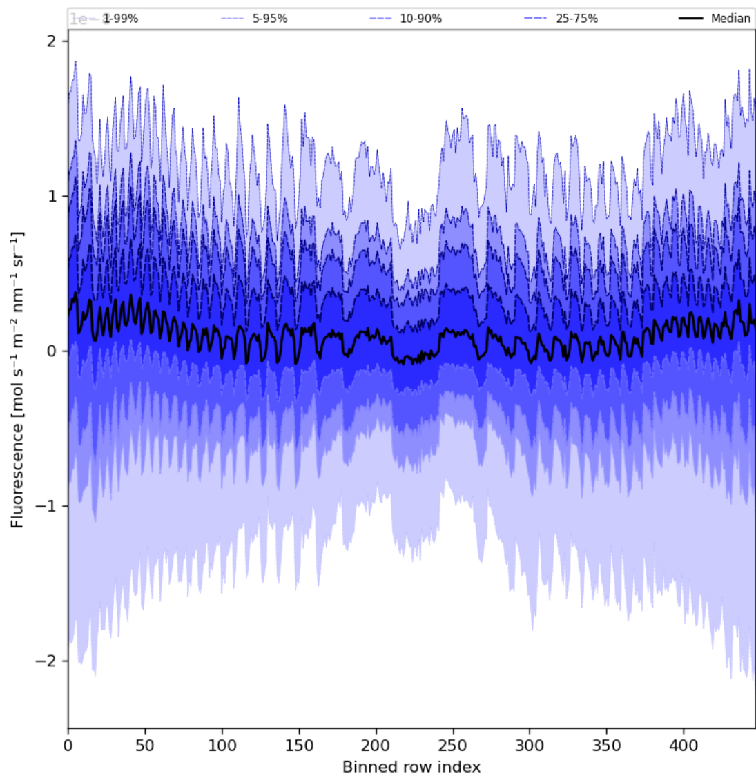
Figure 57: Along track statistics of “Fluorescence” for 2024-03-04 to 2024-03-06
