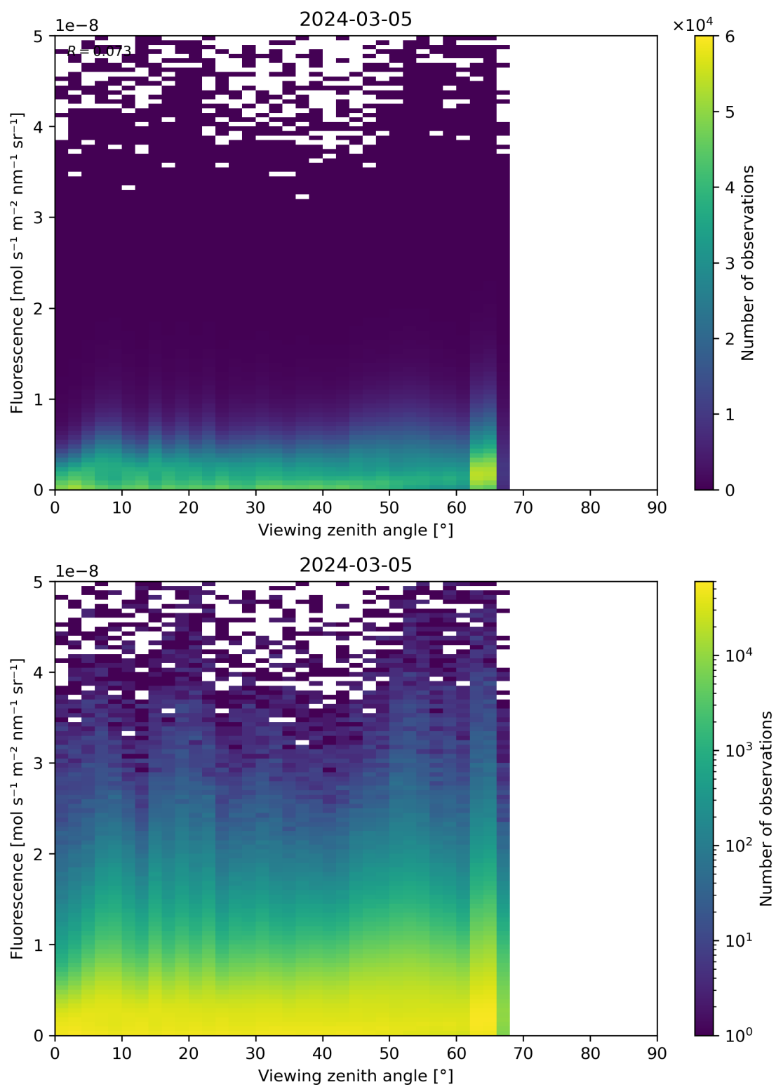
Figure 122: Scatter density plot of “Viewing zenith angle” against “Fluorescence” for 2024-03-04 to 2024-03-06.
