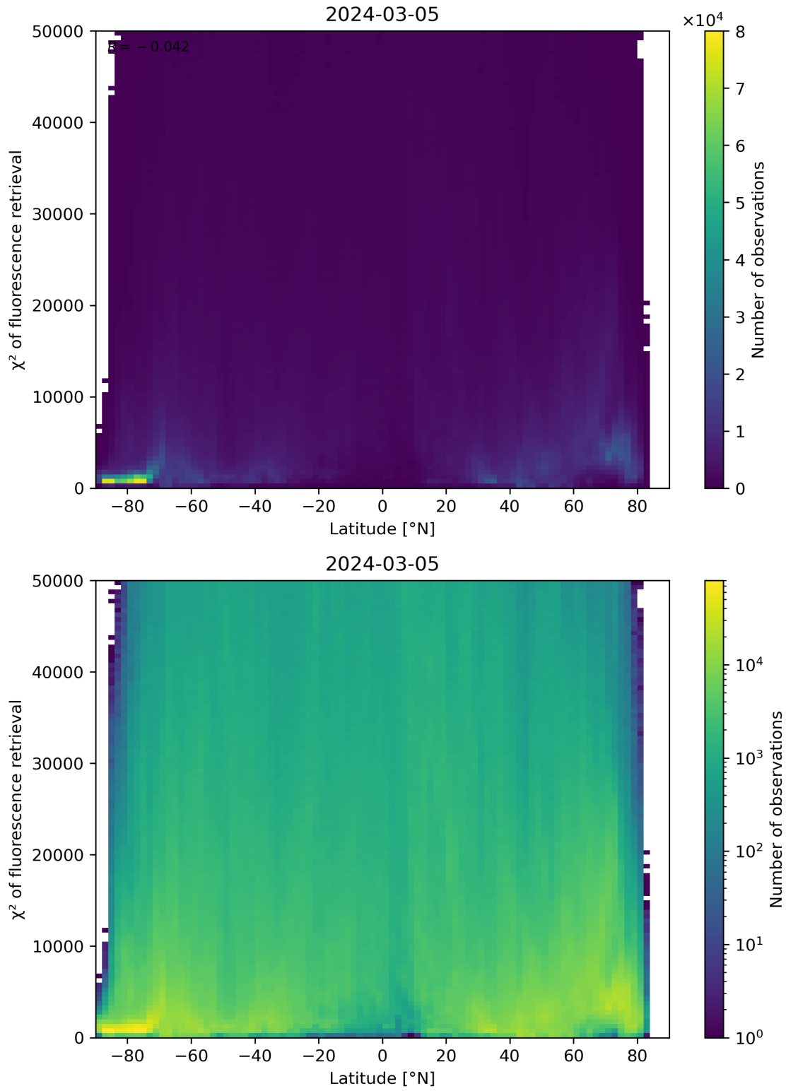
Figure 89: Scatter density plot of “Latitude” against “ \chi^2 of fluorescence retrieval” for 2024-03-04 to 2024-03-06.
