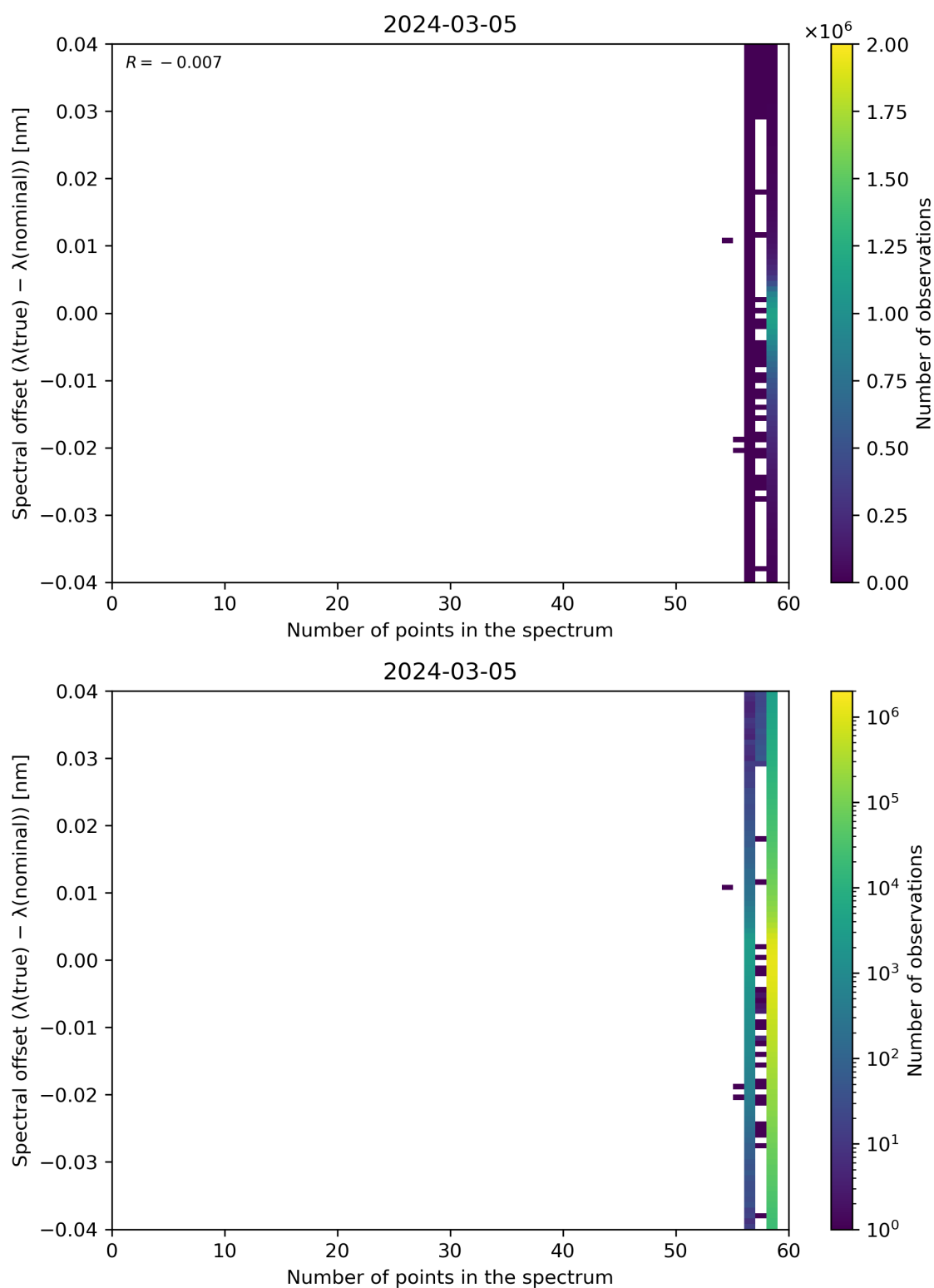
Figure 101: Scatter density plot of “Number of points in the spectrum” against “Spectral offset ( \lambda(\text{true}) - \lambda(\text{nominal}) )” for 2024-03-04 to 2024-03-06.
