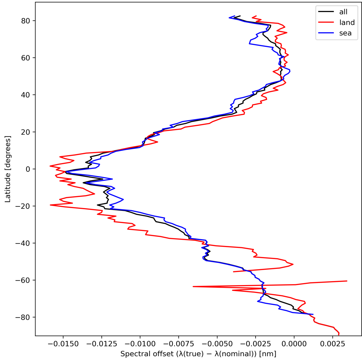
Figure 28: Zonal average of “Spectral offset ( \lambda(\text{true}) - \lambda(\text{nominal}) )” for 2024-03-04 to 2024-03-06.
