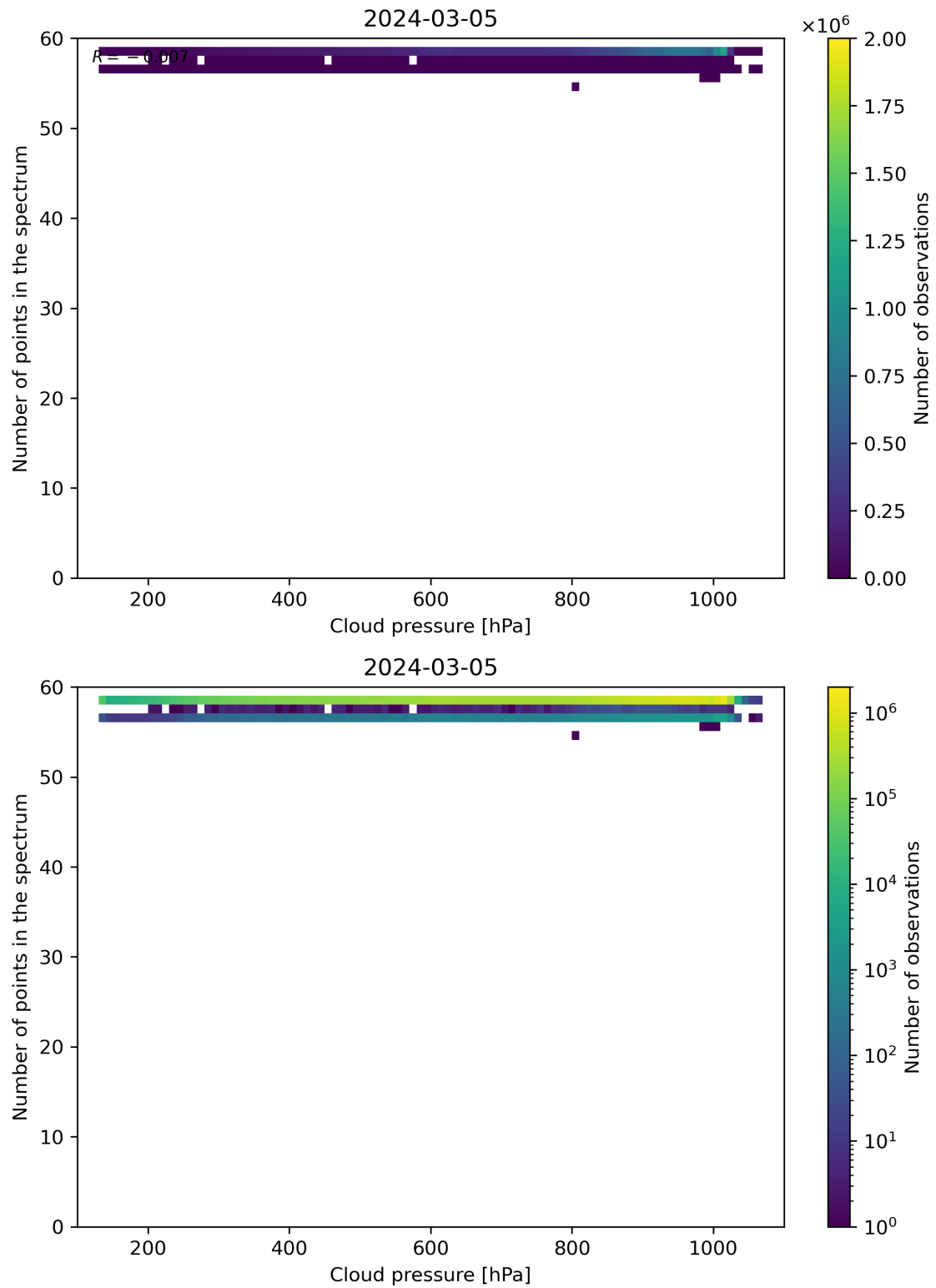
Figure 82: Scatter density plot of “Cloud pressure” against “Number of points in the spectrum” for 2024-03-04 to 2024-03-06.
