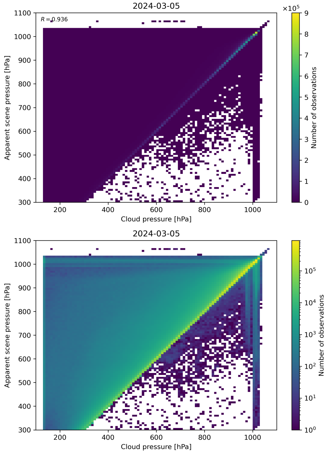
Figure 77: Scatter density plot of “Cloud pressure” against “Apparent scene pressure” for 2024-03-04 to 2024-03-06.
