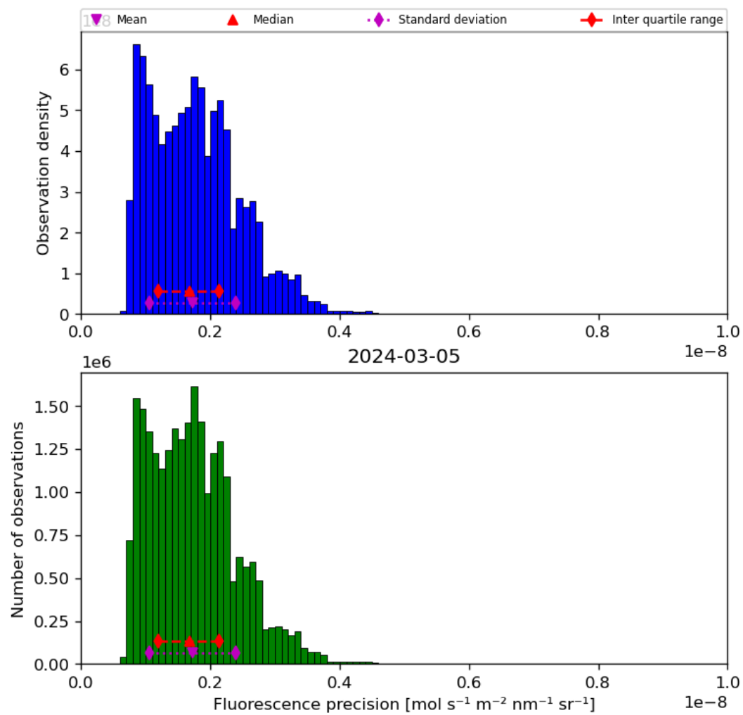
Figure 41: Histogram of “Fluorescence precision” for 2024-03-04 to 2024-03-06
