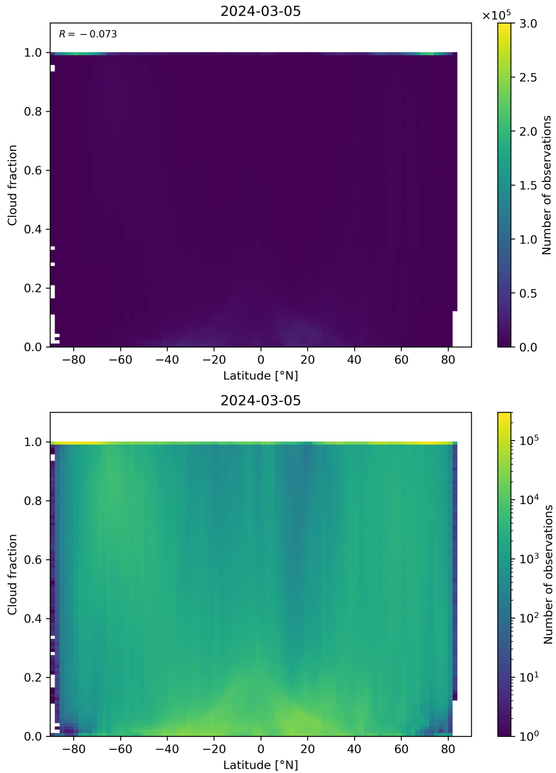
Figure 90: Scatter density plot of “Latitude” against “Cloud fraction” for 2024-03-04 to 2024-03-06.
