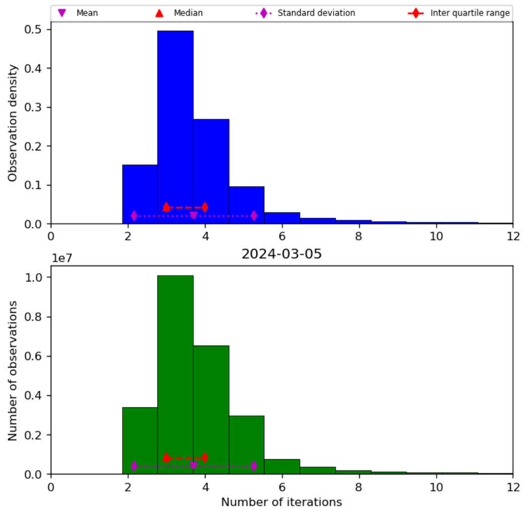
Figure 39: Histogram of “Number of iterations” for 2024-03-04 to 2024-03-06
