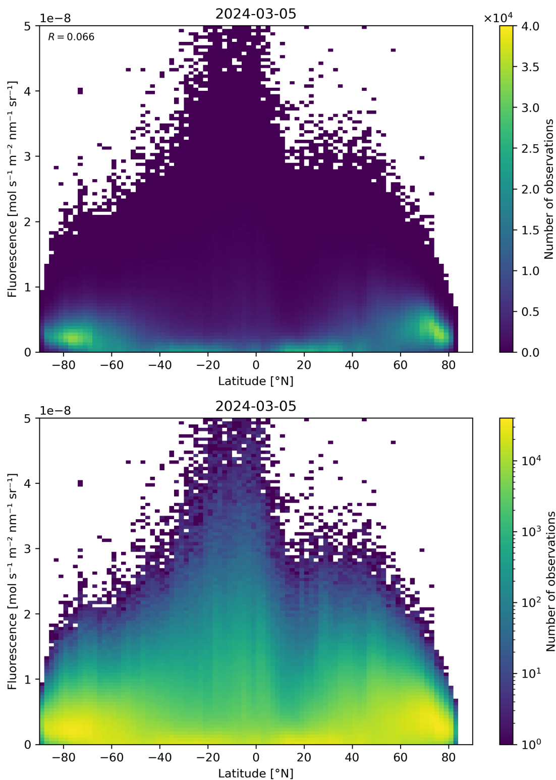
Figure 92: Scatter density plot of “Latitude” against “Fluorescence” for 2024-03-04 to 2024-03-06.
