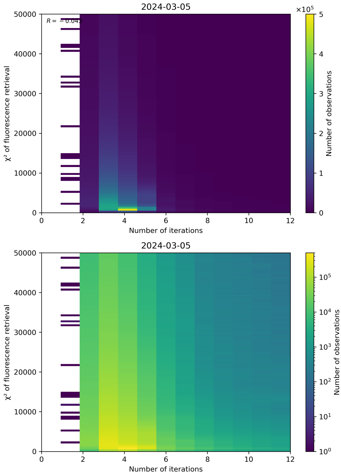
Figure 97: Scatter density plot of “Number of iterations” against “ \chi^2 of fluorescence retrieval” for 2024-03-04 to 2024-03-06.
