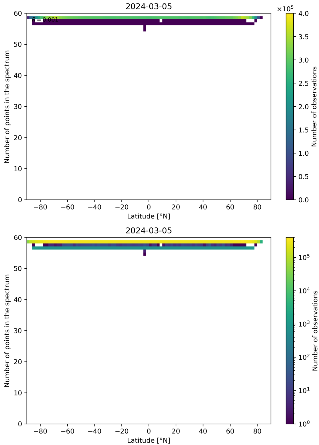
Figure 94: Scatter density plot of “Latitude” against “Number of points in the spectrum” for 2024-03-04 to 2024-03-06.
