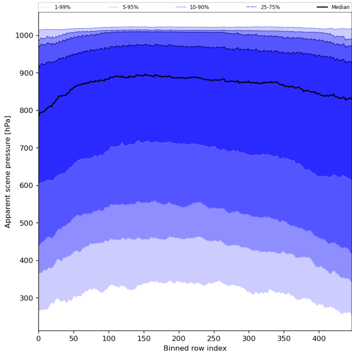
Figure 53: Along track statistics of “Apparent scene pressure” for 2024-03-04 to 2024-03-06
