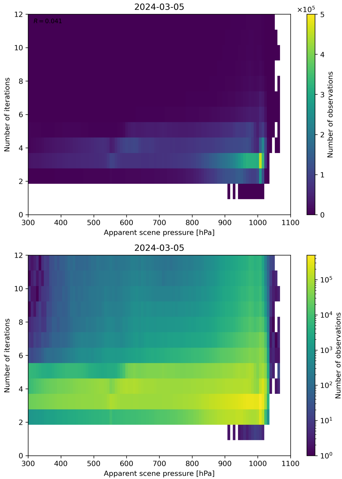
Figure 65: Scatter density plot of “Apparent scene pressure” against “Number of iterations” for 2024-03-04 to 2024-03-06.
