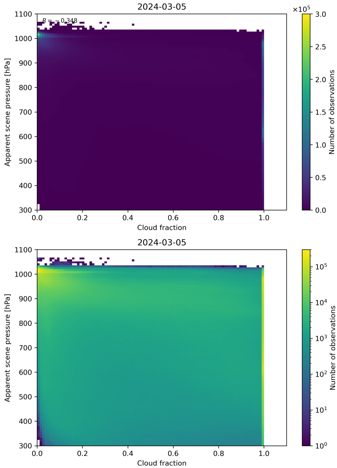
Figure 70: Scatter density plot of “Cloud fraction” against “Apparent scene pressure” for 2024-03-04 to 2024-03-06.
