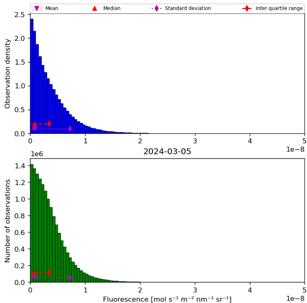
Figure 40: Histogram of “Fluorescence” for 2024-03-04 to 2024-03-06
