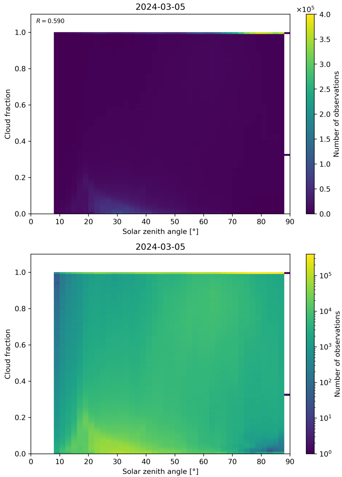
Figure 110: Scatter density plot of “Solar zenith angle” against “Cloud fraction” for 2024-03-04 to 2024-03-06.
