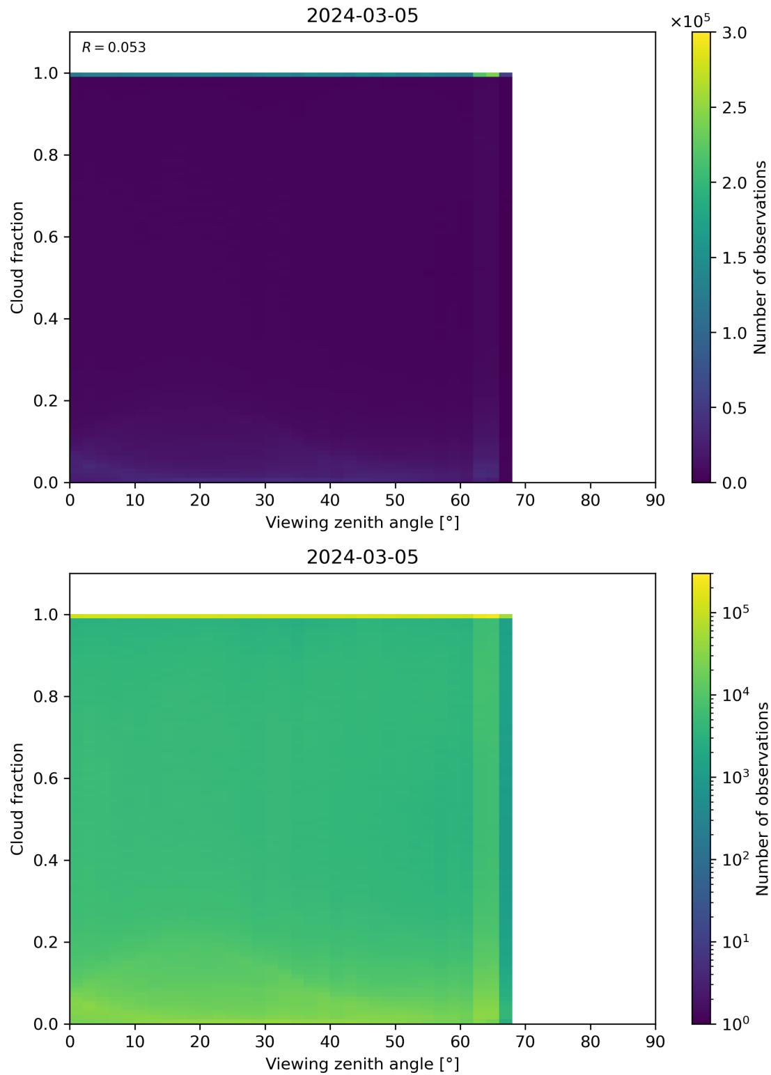
Figure 120: Scatter density plot of “Viewing zenith angle” against “Cloud fraction” for 2024-03-04 to 2024-03-06.
