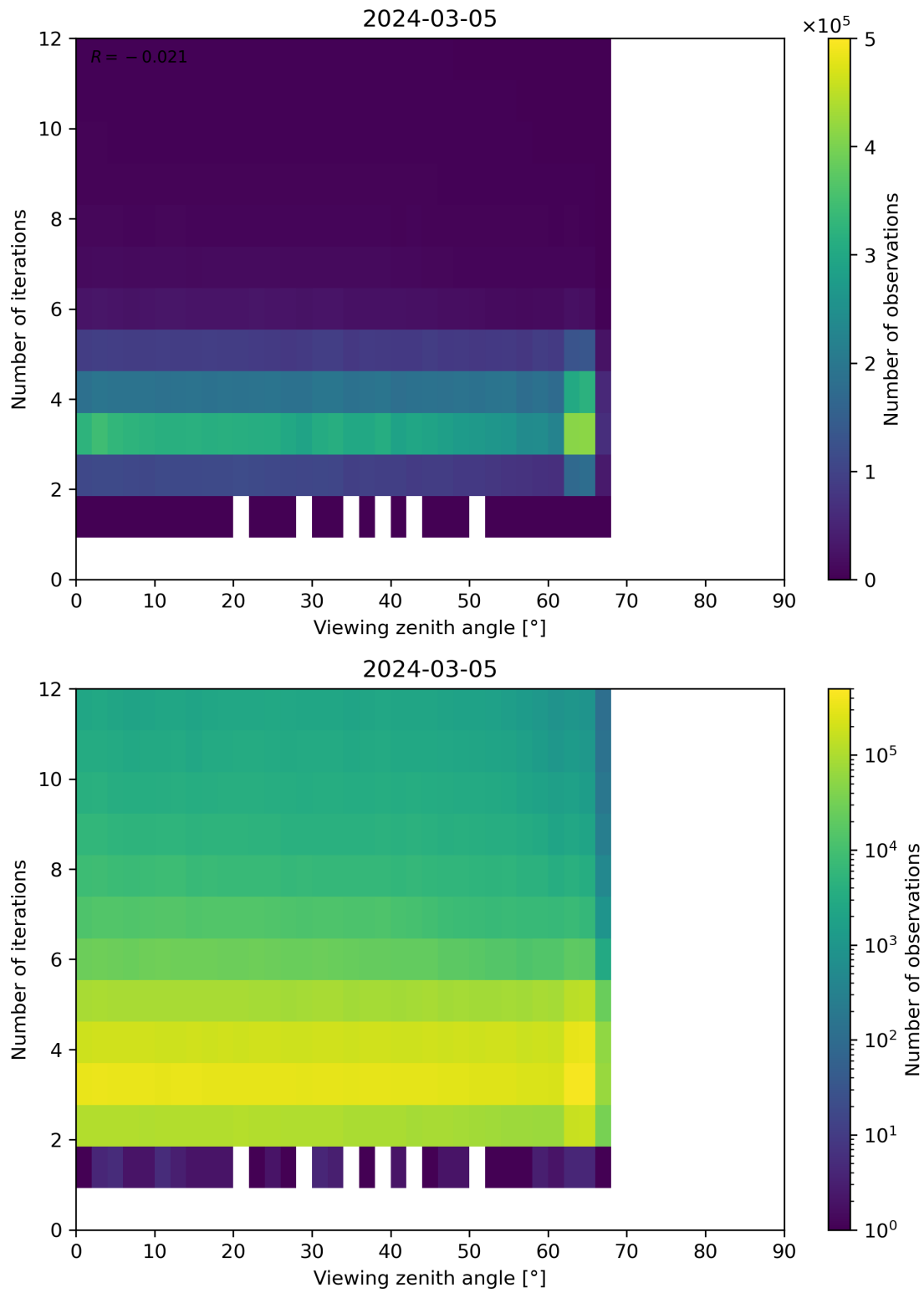
Figure 124: Scatter density plot of “Viewing zenith angle” against “Number of iterations” for 2024-03-04 to 2024-03-06.
