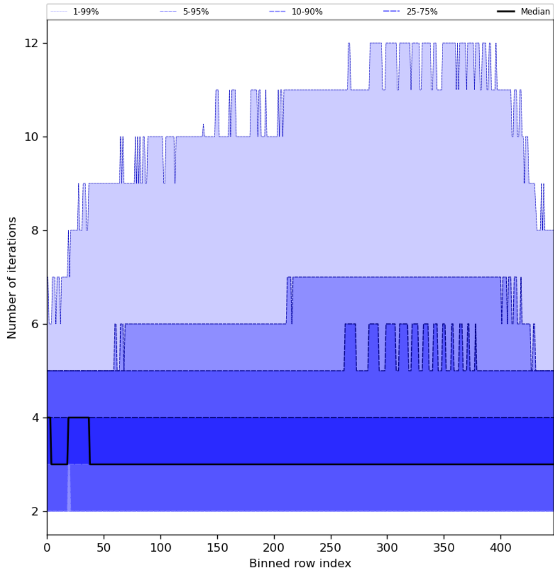
Figure 56: Along track statistics of “Number of iterations” for 2024-03-04 to 2024-03-06
