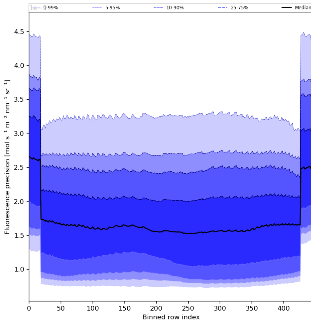
Figure 58: Along track statistics of "Fluorescence precision" for 2024-03-04 to 2024-03-06
