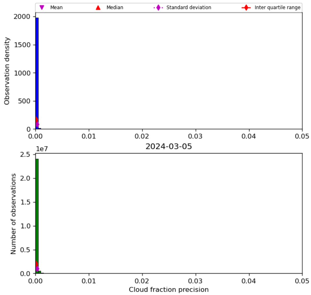
Figure 33: Histogram of “Cloud fraction precision” for 2024-03-04 to 2024-03-06
