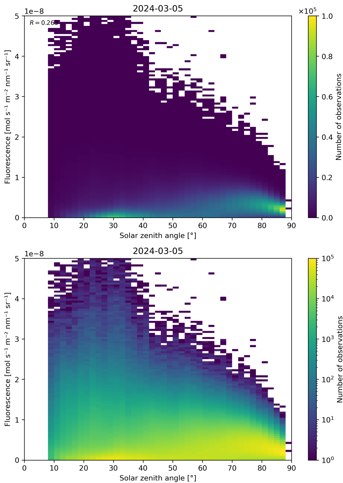
Figure 112: Scatter density plot of “Solar zenith angle” against “Fluorescence” for 2024-03-04 to 2024-03-06.
