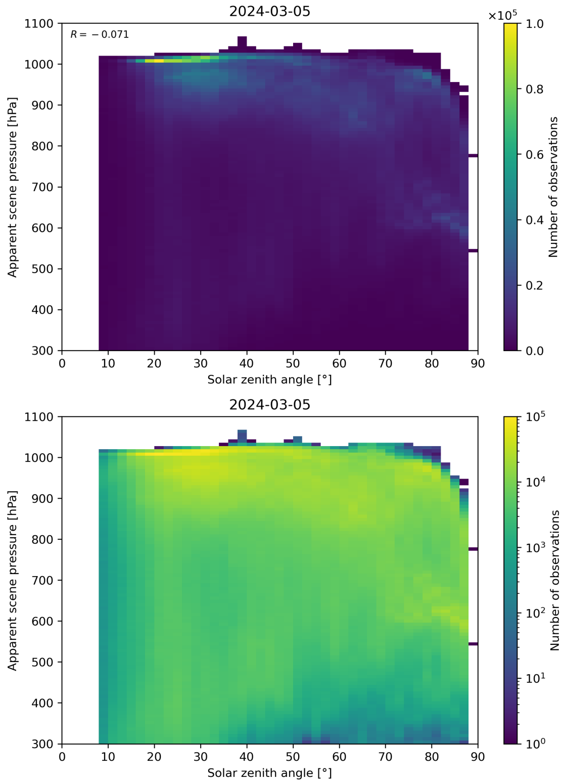
Figure 108: Scatter density plot of “Solar zenith angle” against “Apparent scene pressure” for 2024-03-04 to 2024-03-06.
