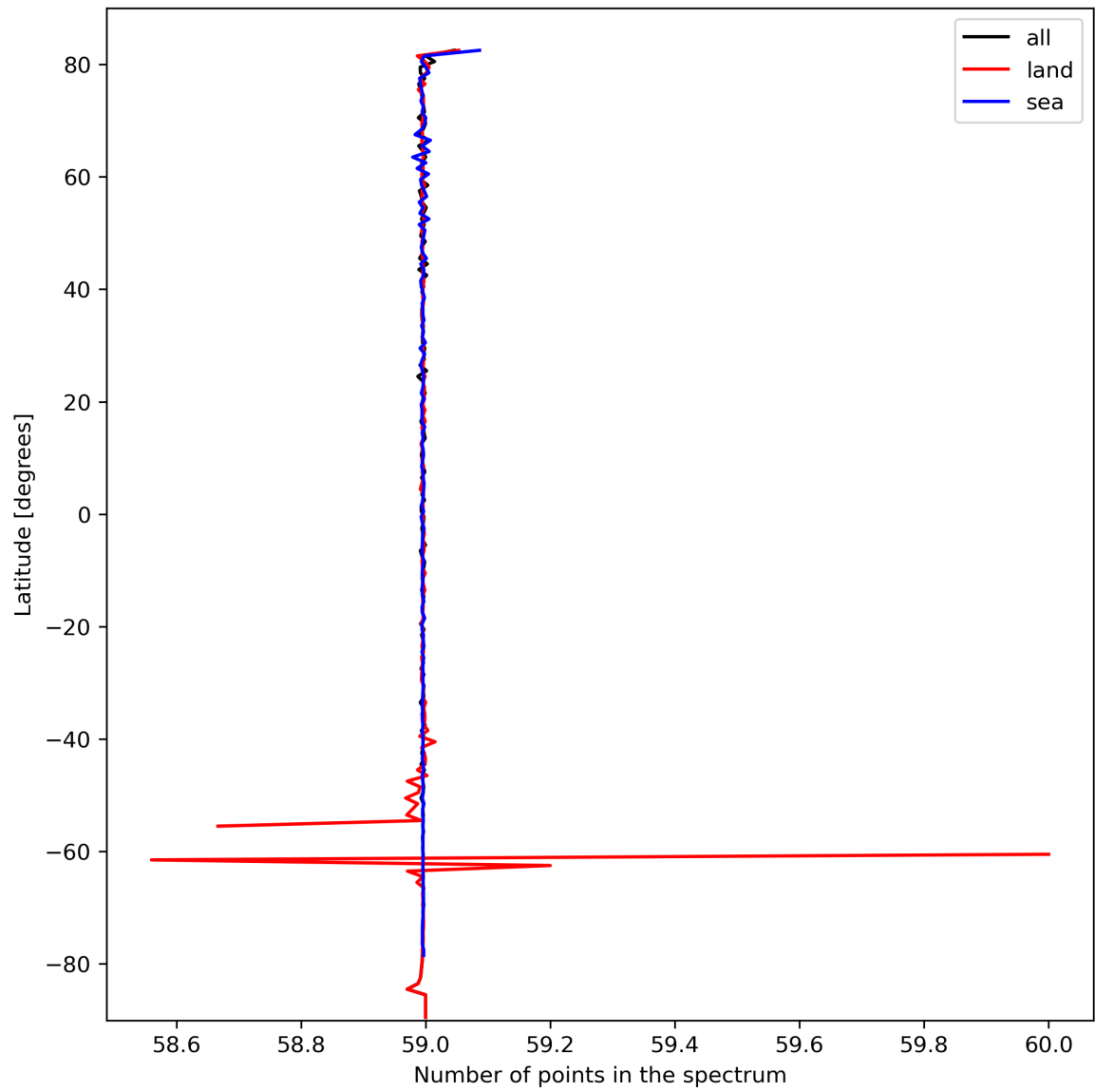
Figure 27: Zonal average of “Number of points in the spectrum” for 2024-03-04 to 2024-03-06.
