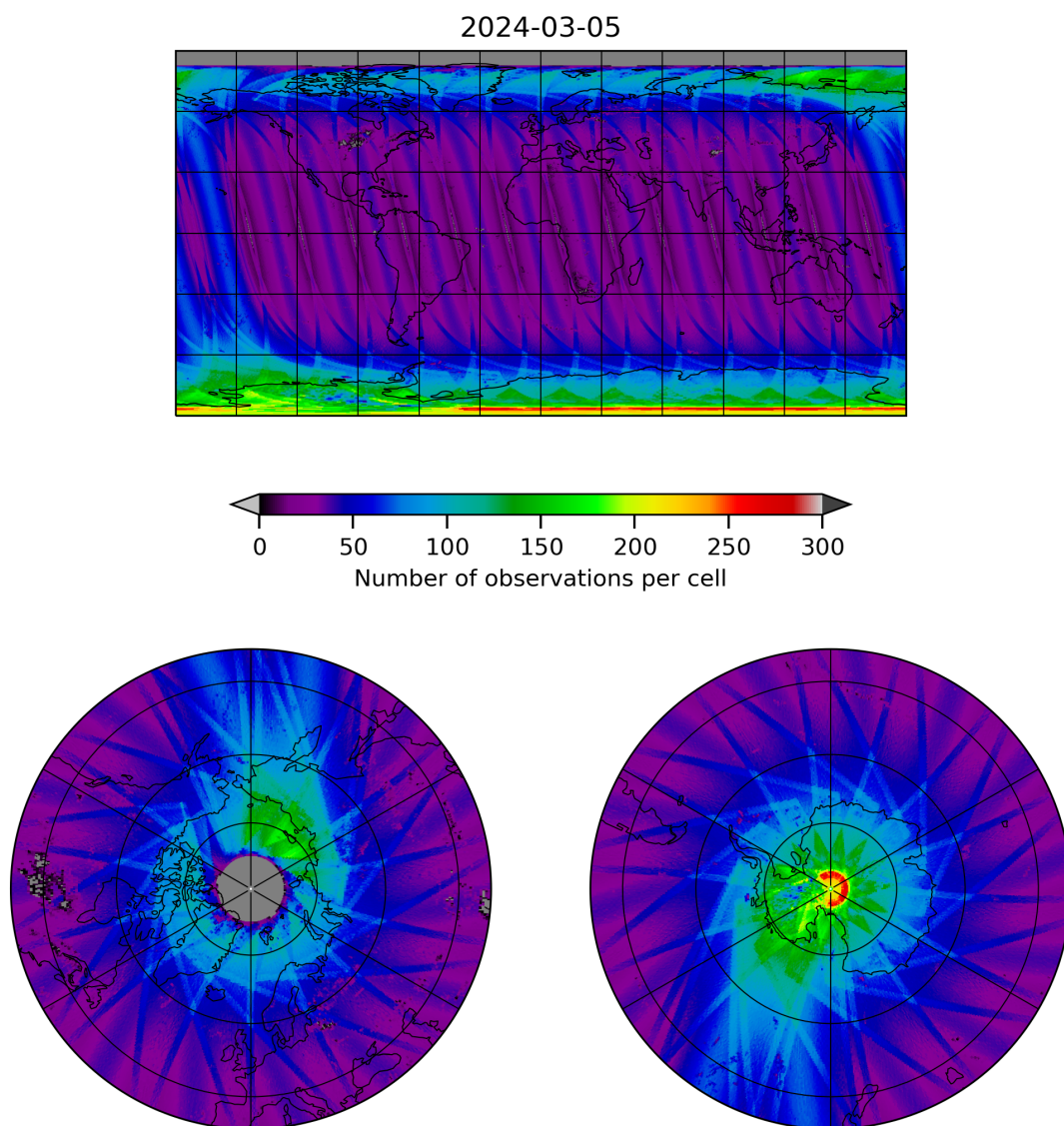
Figure 11: Map of the number of observations for 2024-03-04 to 2024-03-06
