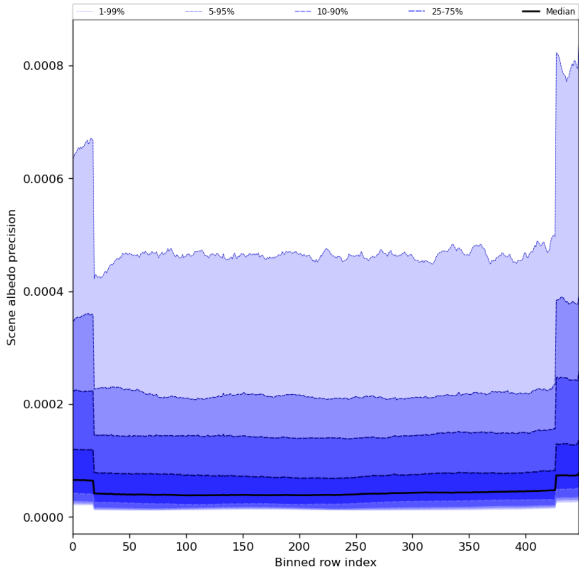
Figure 52: Along track statistics of “Scene albedo precision” for 2024-03-04 to 2024-03-06
