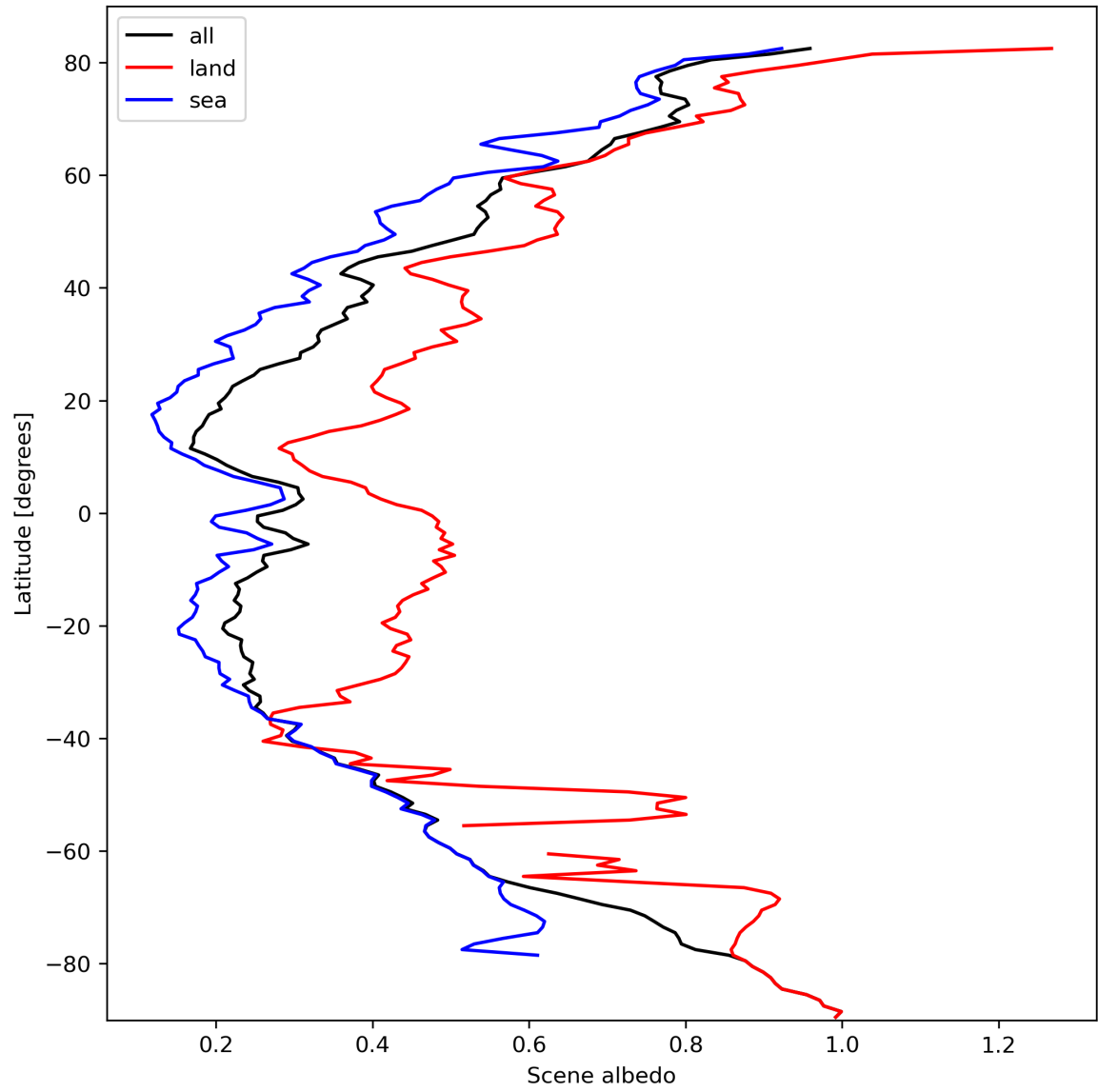
Figure 17: Zonal average of “Scene albedo” for 2024-03-04 to 2024-03-06.
