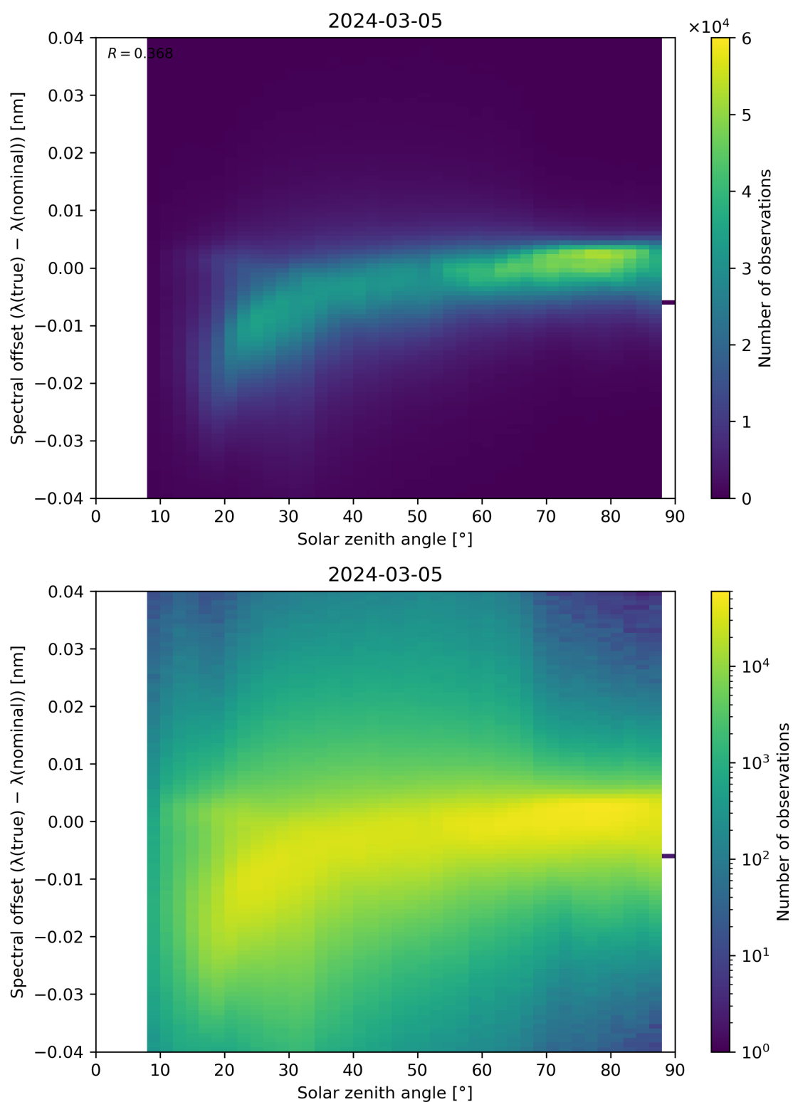
Figure 117: Scatter density plot of “Solar zenith angle” against “Spectral offset ( \lambda(\text{true}) - \lambda(\text{nominal}) )” for 2024-03-04 to 2024-03-06.
