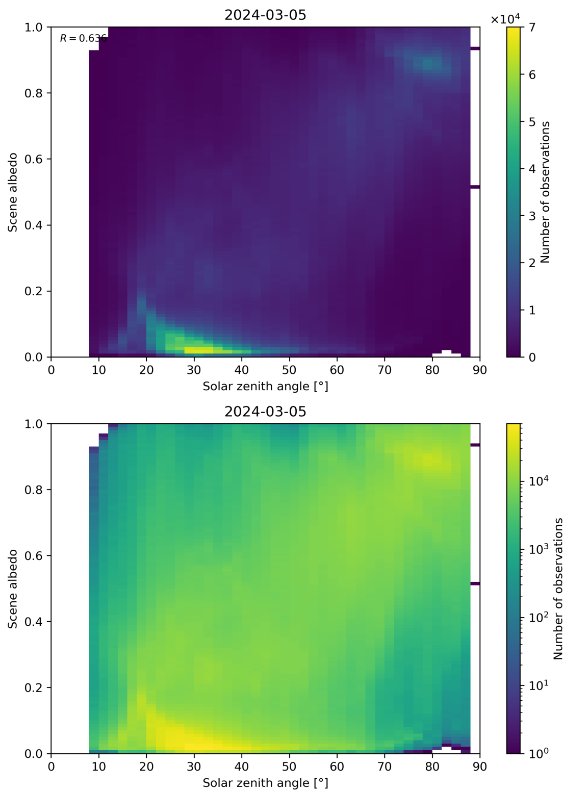
Figure 116: Scatter density plot of “Solar zenith angle” against “Scene albedo” for 2024-03-04 to 2024-03-06.
