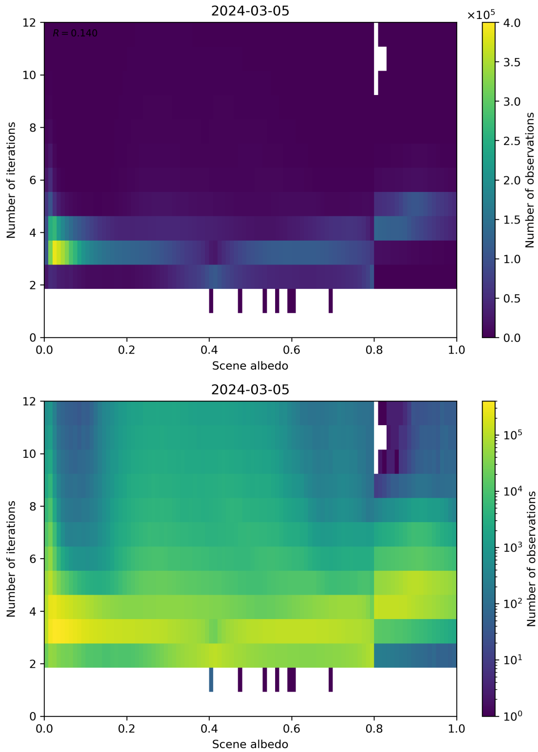
Figure 105: Scatter density plot of “Scene albedo” against “Number of iterations” for 2024-03-04 to 2024-03-06.
