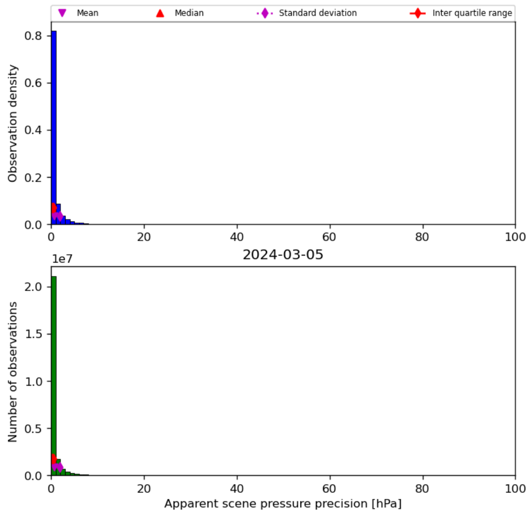
Figure 37: Histogram of “Apparent scene pressure precision” for 2024-03-04 to 2024-03-06
