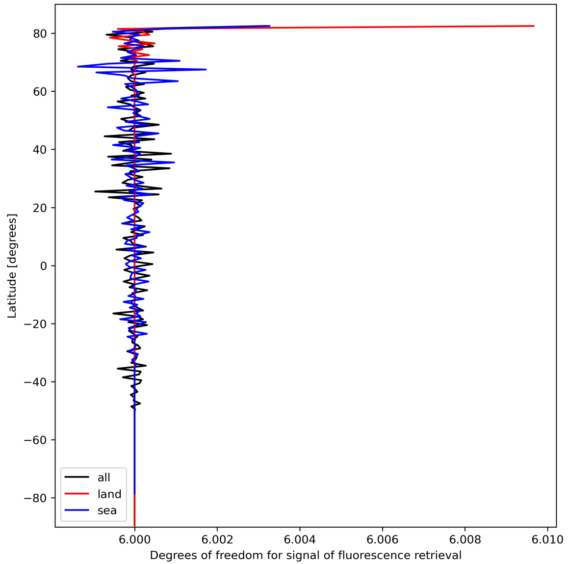
Figure 26: Zonal average of “Degrees of freedom for signal of fluorescence retrieval” for 2024-03-04 to 2024-03-06.
