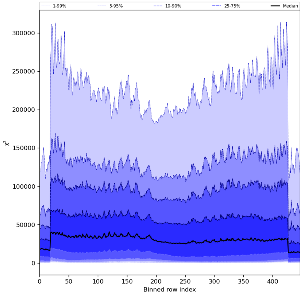
Figure 55: Along track statistics of “ \chi^2 ” for 2024-03-04 to 2024-03-06
