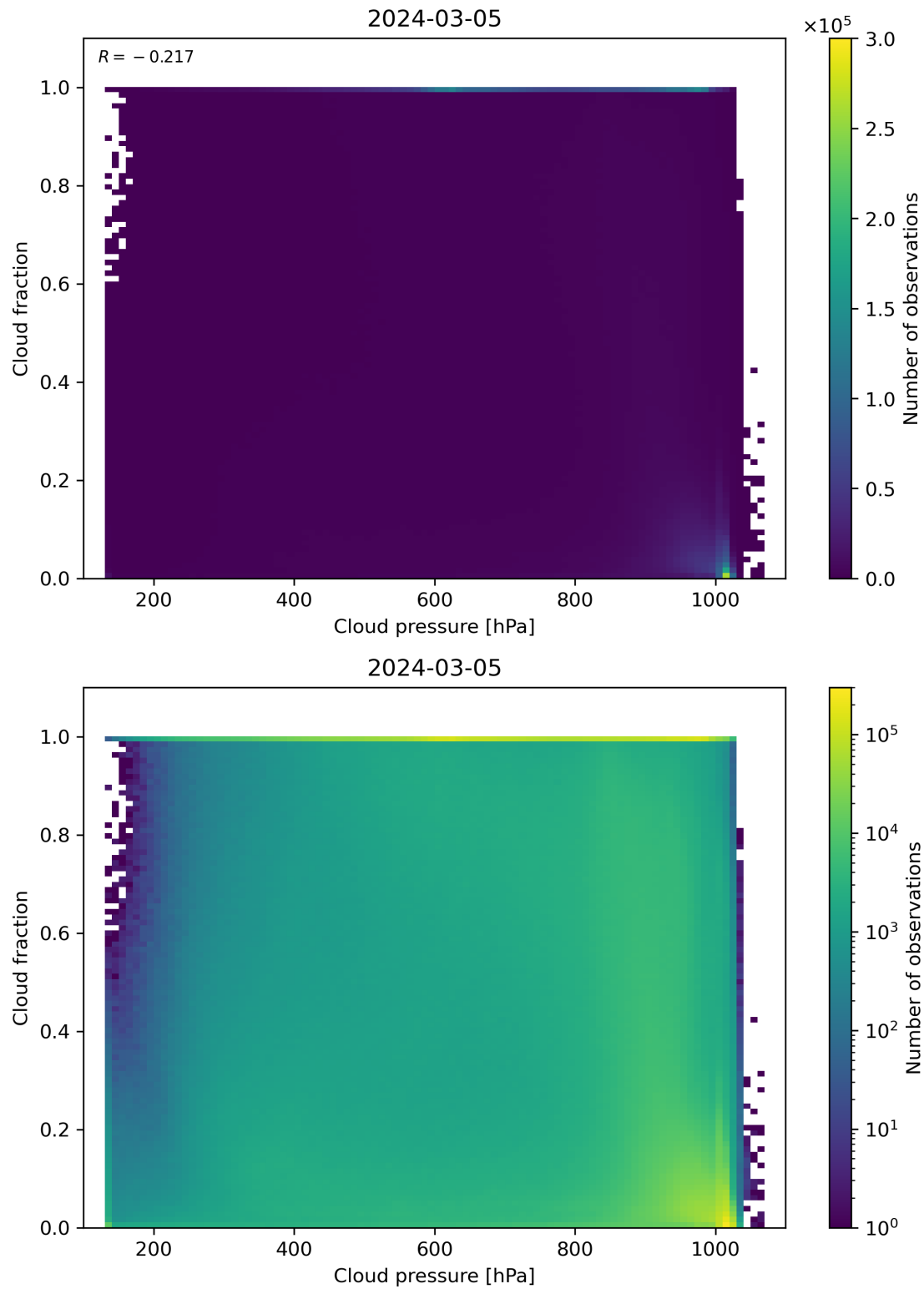
Figure 79: Scatter density plot of “Cloud pressure” against “Cloud fraction” for 2024-03-04 to 2024-03-06.
