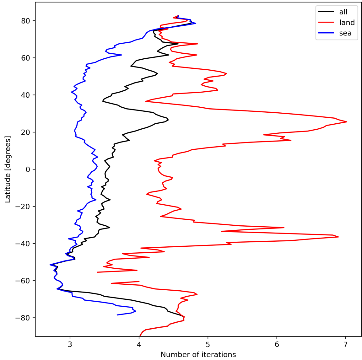
Figure 22: Zonal average of “Number of iterations” for 2024-03-04 to 2024-03-06.
