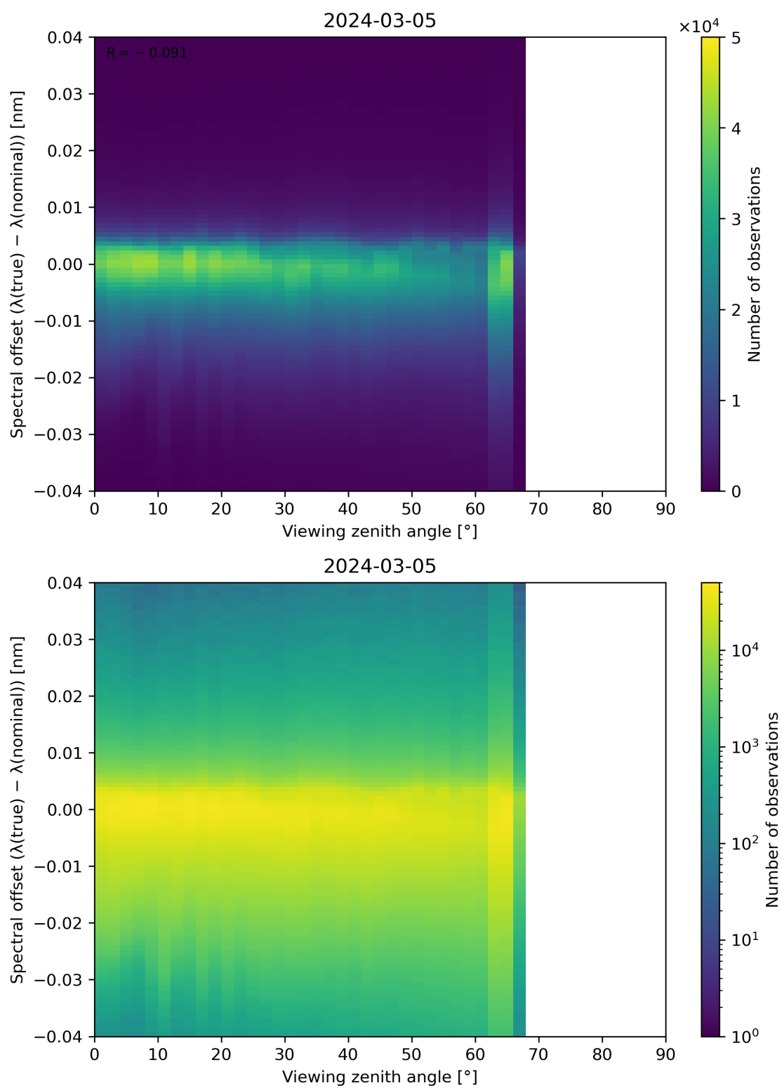
Figure 128: Scatter density plot of “Viewing zenith angle” against “Spectral offset ( \lambda(\text{true}) - \lambda(\text{nominal}) )” for 2024-03-04 to 2024-03-06.
