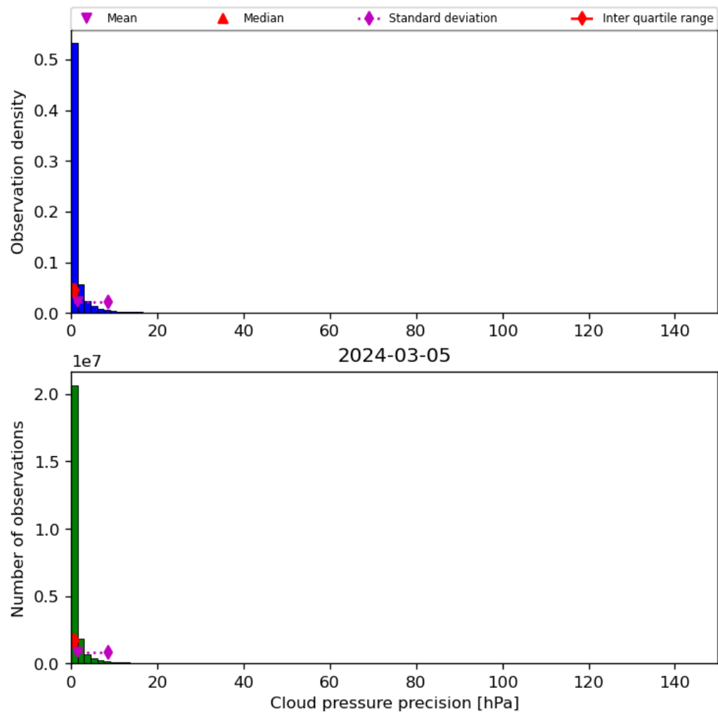
Figure 31: Histogram of “Cloud pressure precision” for 2024-03-04 to 2024-03-06
