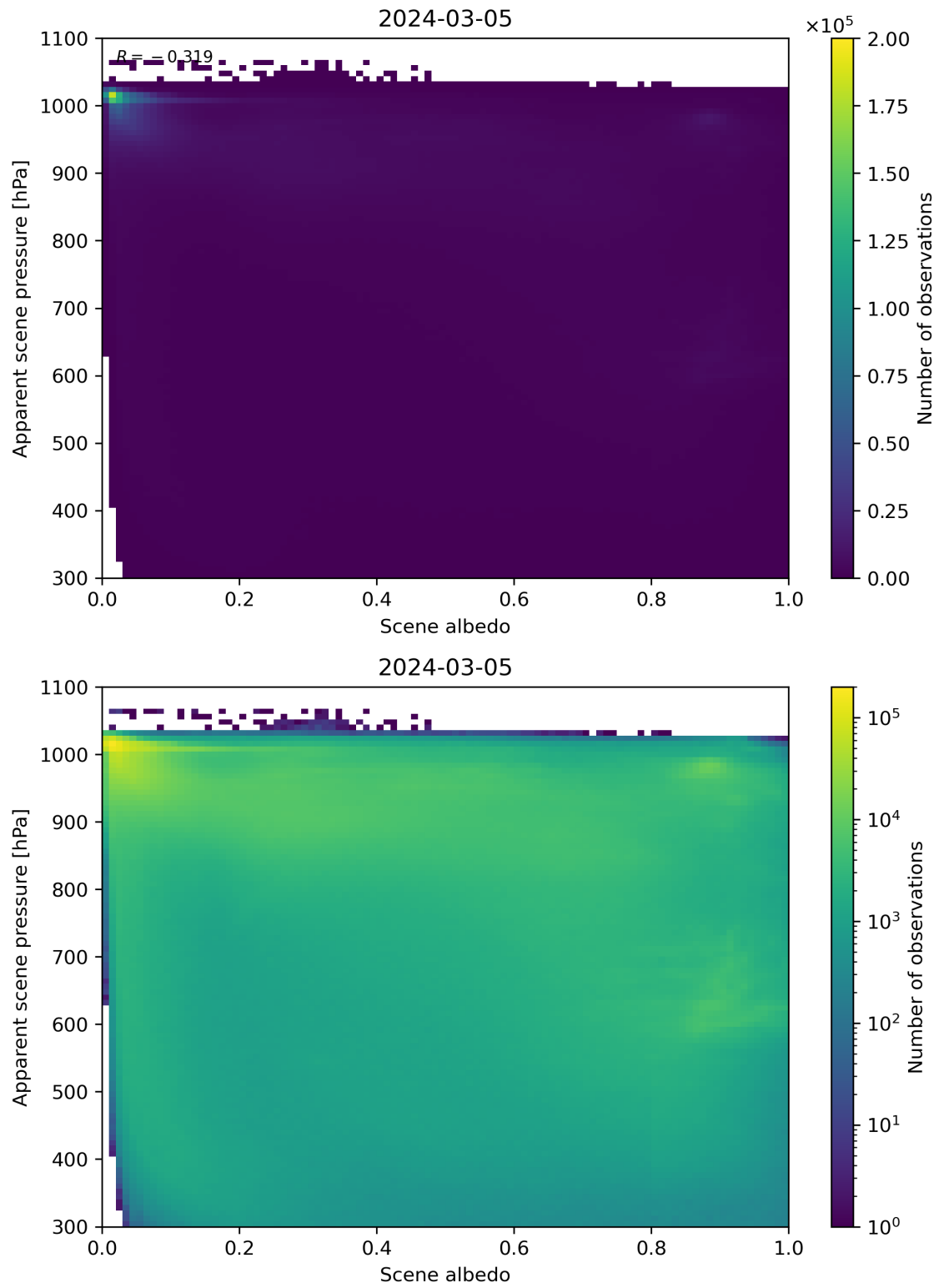
Figure 102: Scatter density plot of “Scene albedo” against “Apparent scene pressure” for 2024-03-04 to 2024-03-06.
