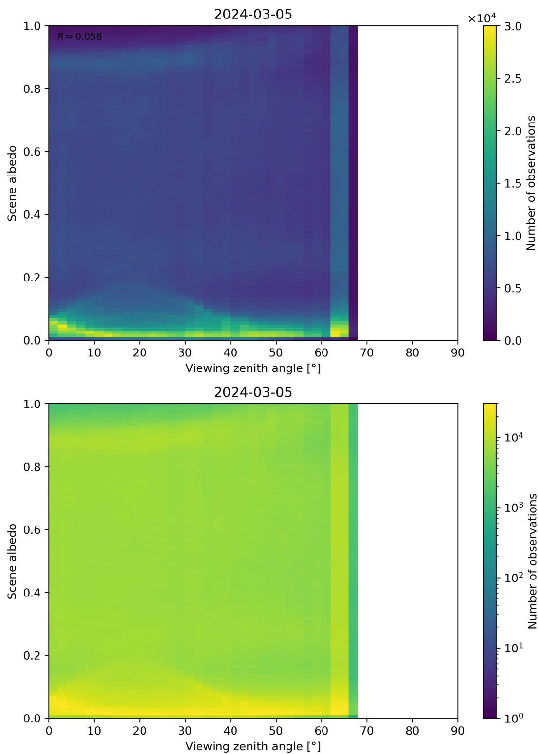
Figure 126: Scatter density plot of “Viewing zenith angle” against “Scene albedo” for 2024-03-04 to 2024-03-06.
