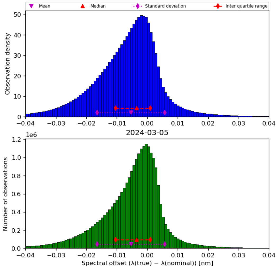
Figure 45: Histogram of “Spectral offset ( \lambda(\text{true}) - \lambda(\text{nominal}) )” for 2024-03-04 to 2024-03-06
