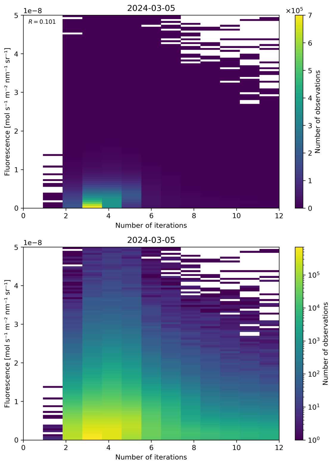
Figure 98: Scatter density plot of “Number of iterations” against “Fluorescence” for 2024-03-04 to 2024-03-06.
