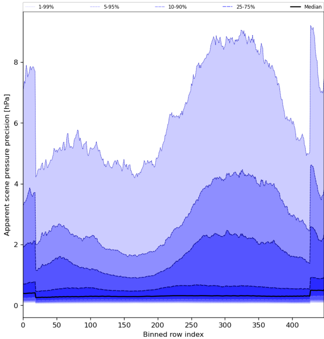
Figure 54: Along track statistics of “Apparent scene pressure precision” for 2024-03-04 to 2024-03-06
