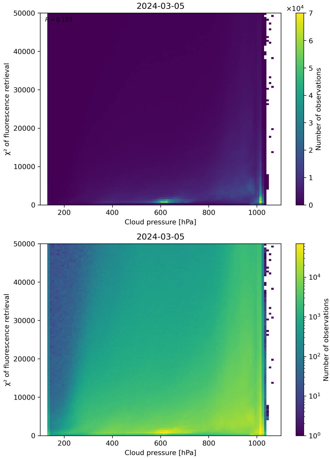
Figure 78: Scatter density plot of “Cloud pressure” against “ \chi^2 of fluorescence retrieval” for 2024-03-04 to 2024-03-06.
