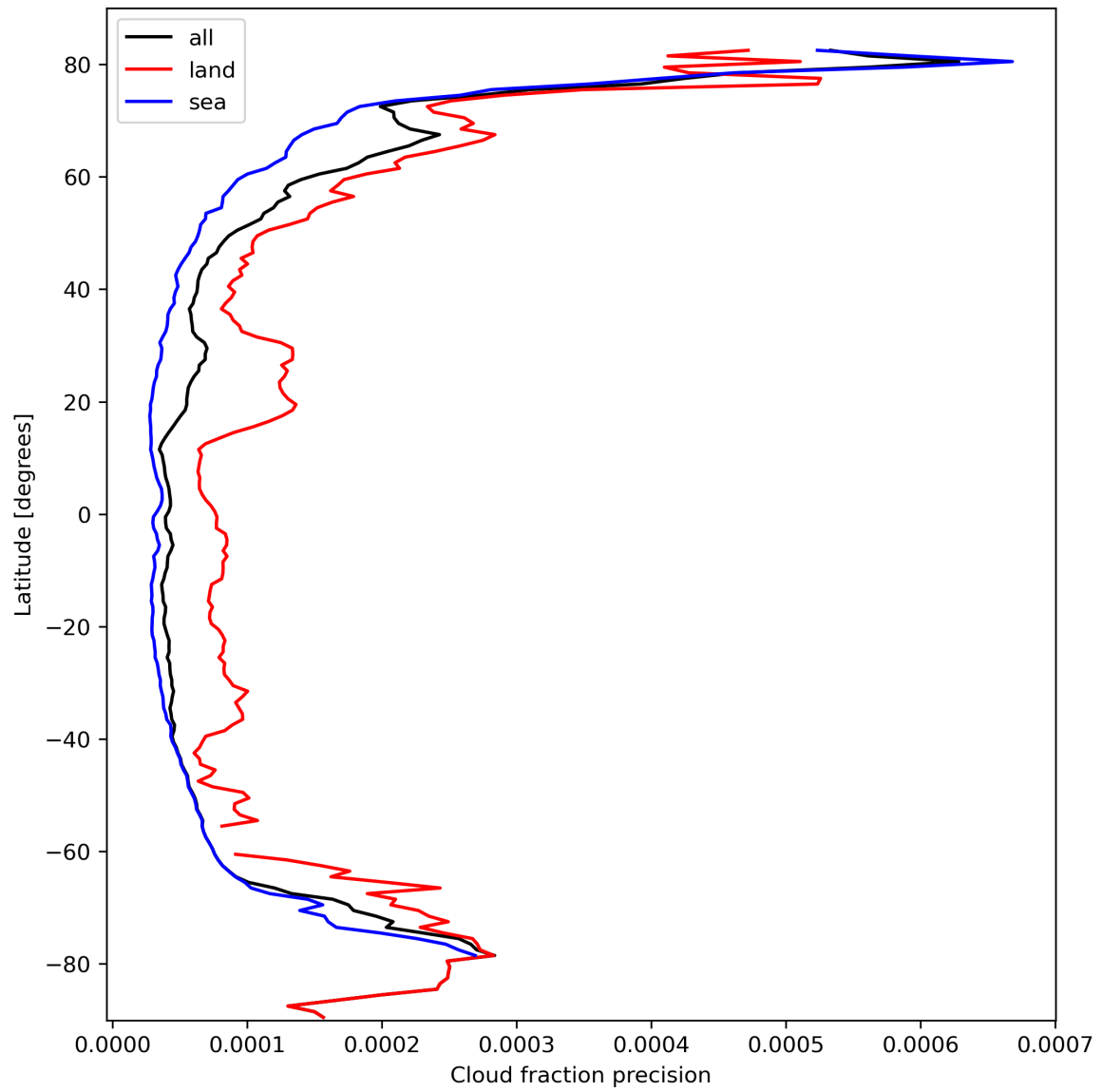
Figure 16: Zonal average of “Cloud fraction precision” for 2024-03-04 to 2024-03-06.
