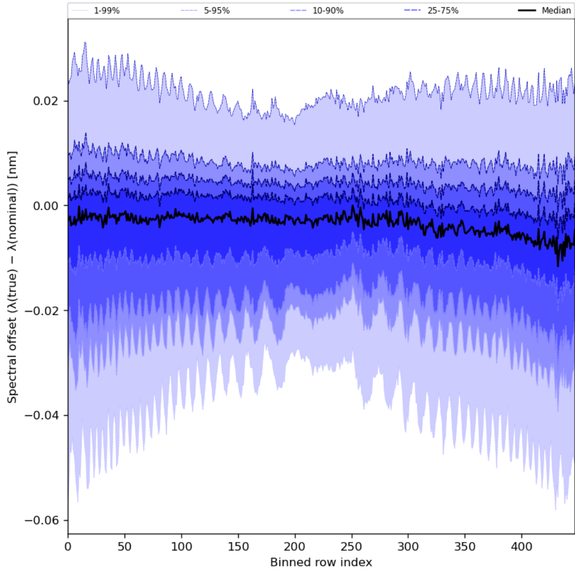
Figure 62: Along track statistics of “Spectral offset ( \lambda(\text{true}) - \lambda(\text{nominal}) )” for 2024-03-04 to 2024-03-06
