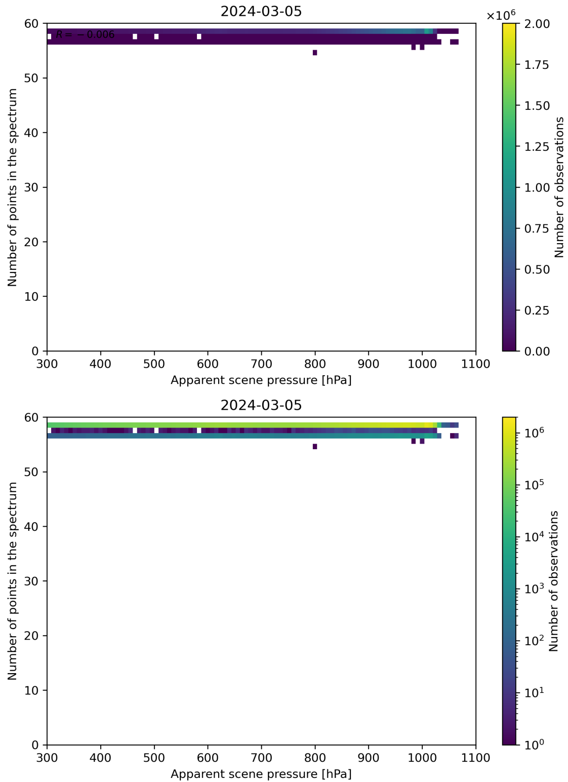
Figure 66: Scatter density plot of “Apparent scene pressure” against “Number of points in the spectrum” for 2024-03-04 to 2024-03-06.
