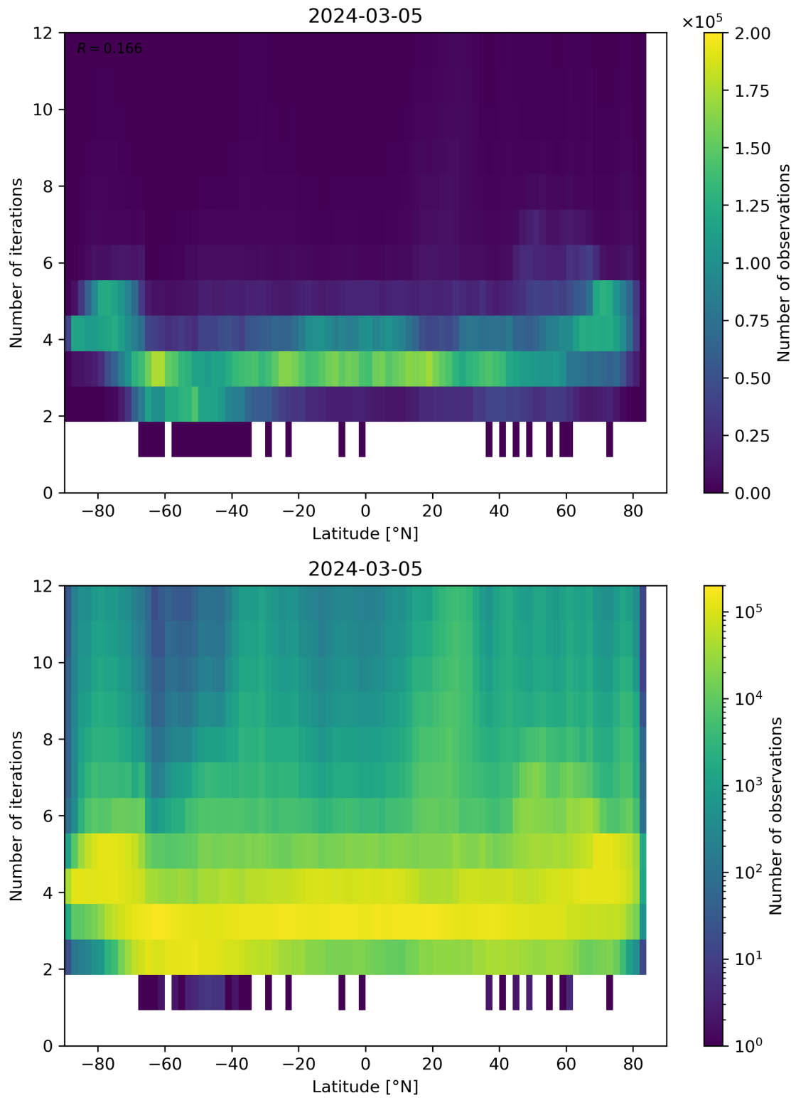
Figure 93: Scatter density plot of “Latitude” against “Number of iterations” for 2024-03-04 to 2024-03-06.
