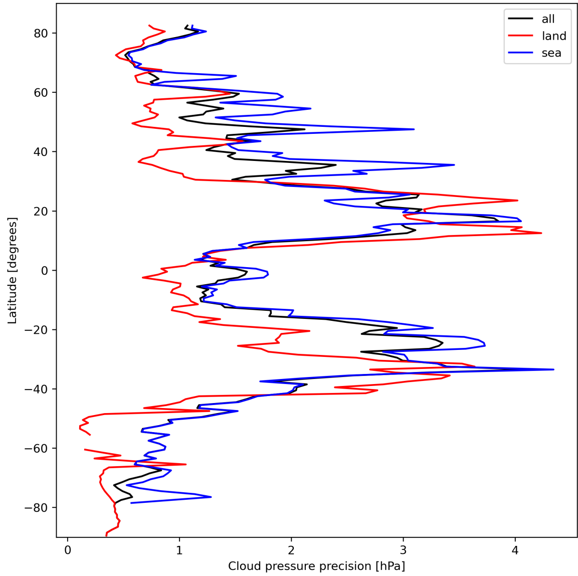
Figure 14: Zonal average of “Cloud pressure precision” for 2024-03-04 to 2024-03-06.
