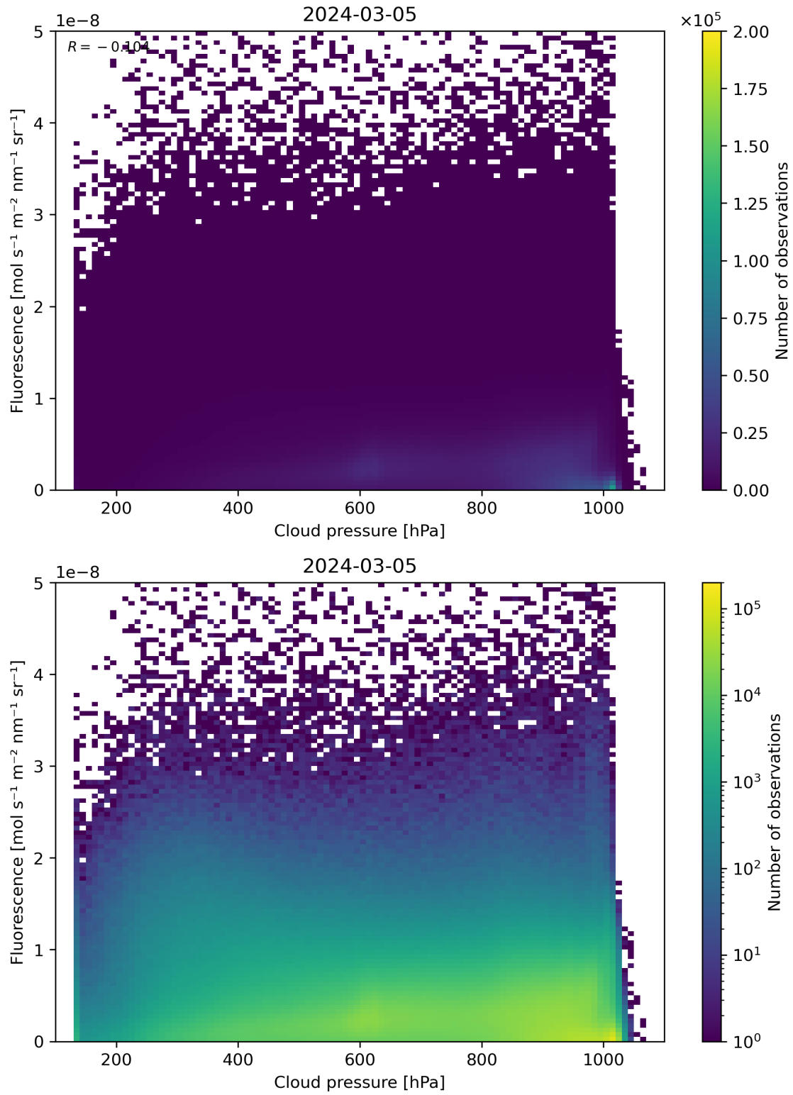
Figure 80: Scatter density plot of “Cloud pressure” against “Fluorescence” for 2024-03-04 to 2024-03-06.
