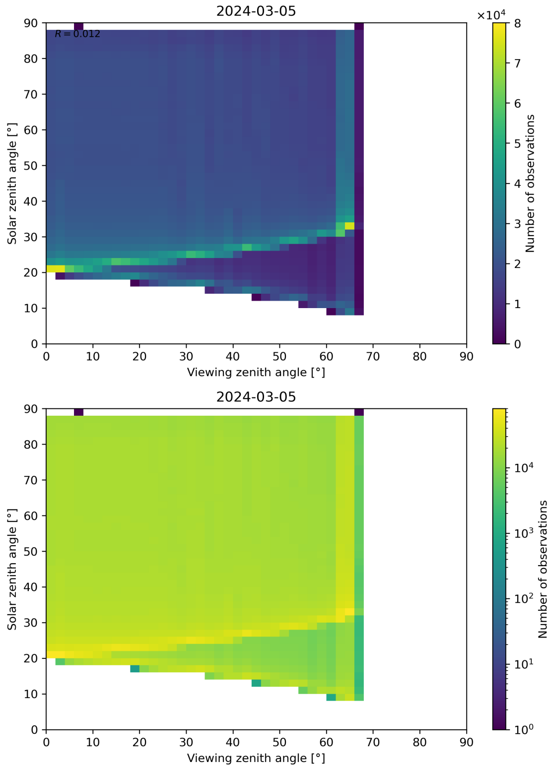
Figure 127: Scatter density plot of “Viewing zenith angle” against “Solar zenith angle” for 2024-03-04 to 2024-03-06.
