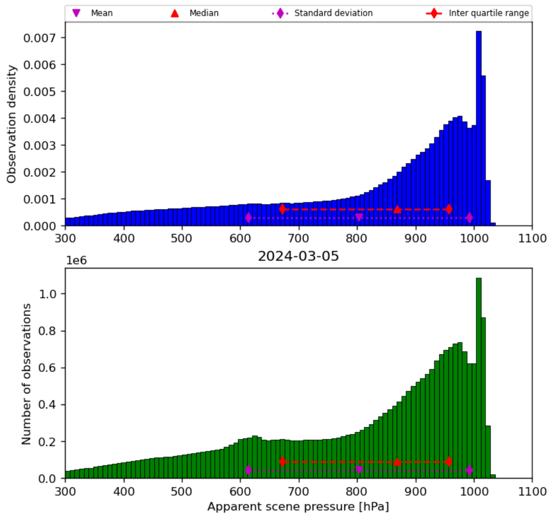
Figure 36: Histogram of “Apparent scene pressure” for 2024-03-04 to 2024-03-06
