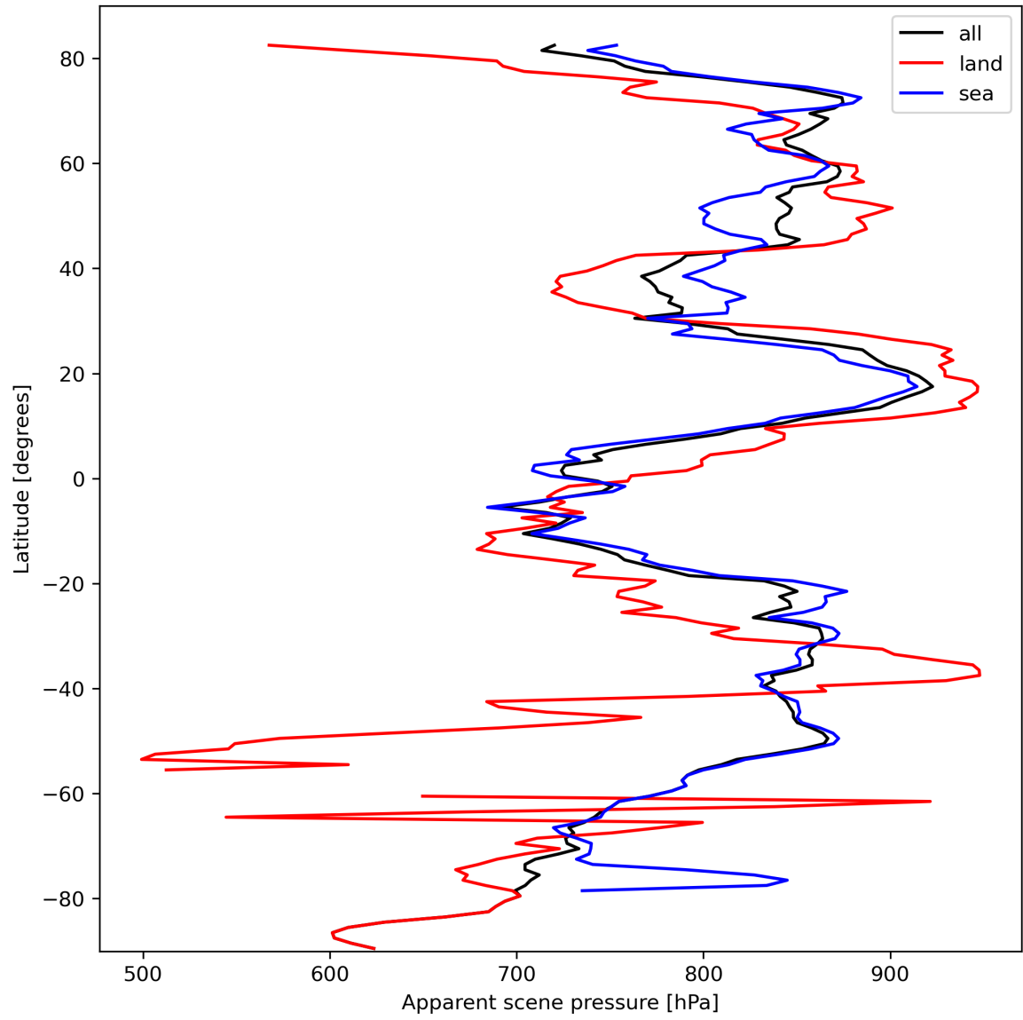
Figure 19: Zonal average of “Apparent scene pressure” for 2024-03-04 to 2024-03-06.
