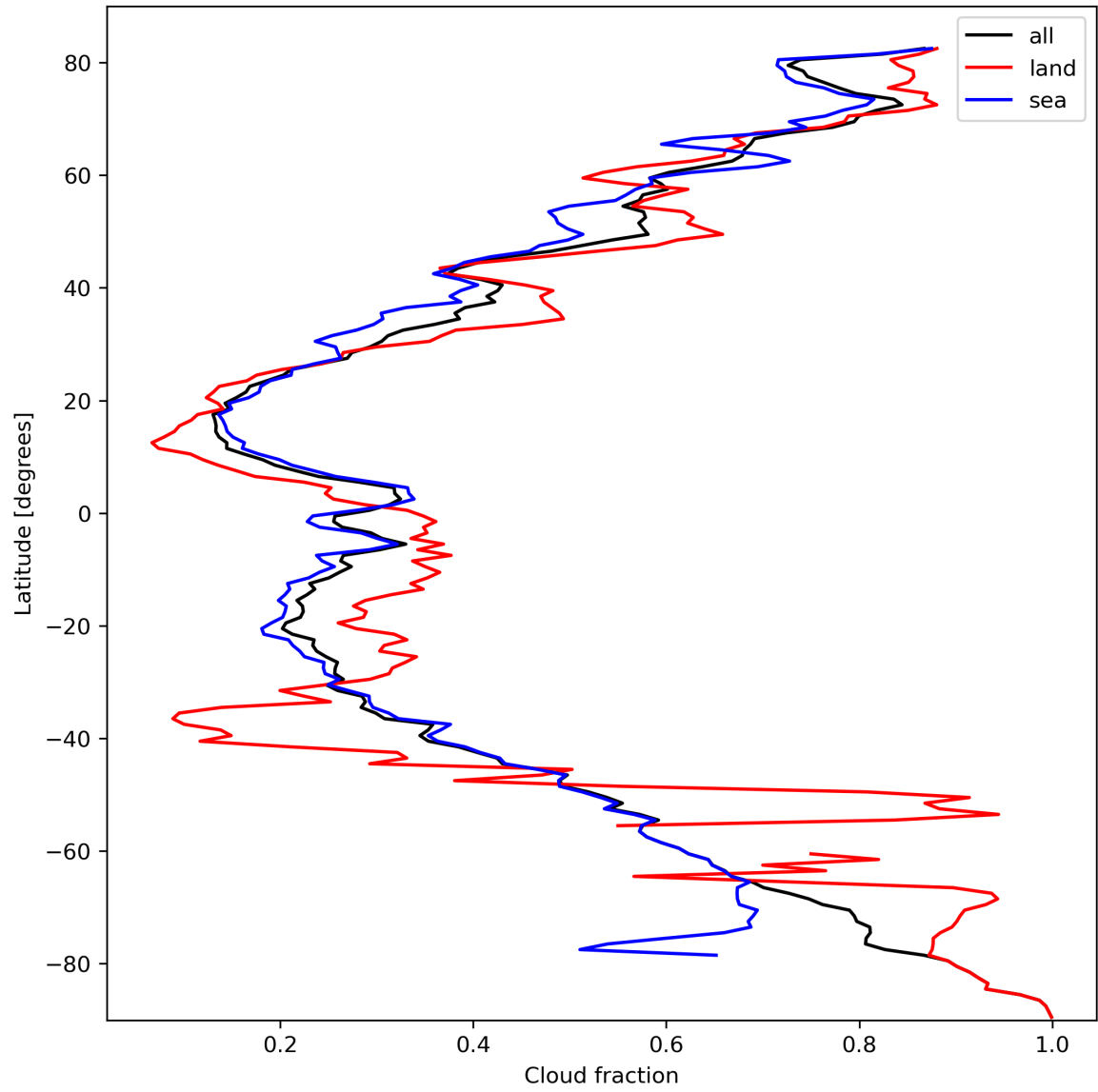
Figure 15: Zonal average of “Cloud fraction” for 2024-03-04 to 2024-03-06.
