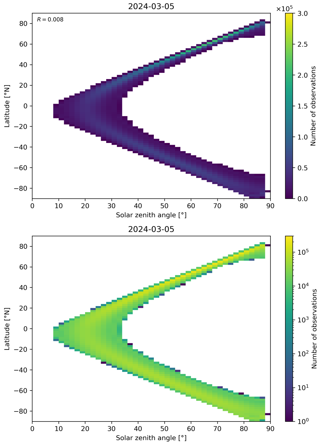
Figure 113: Scatter density plot of “Solar zenith angle” against “Latitude” for 2024-03-04 to 2024-03-06.
