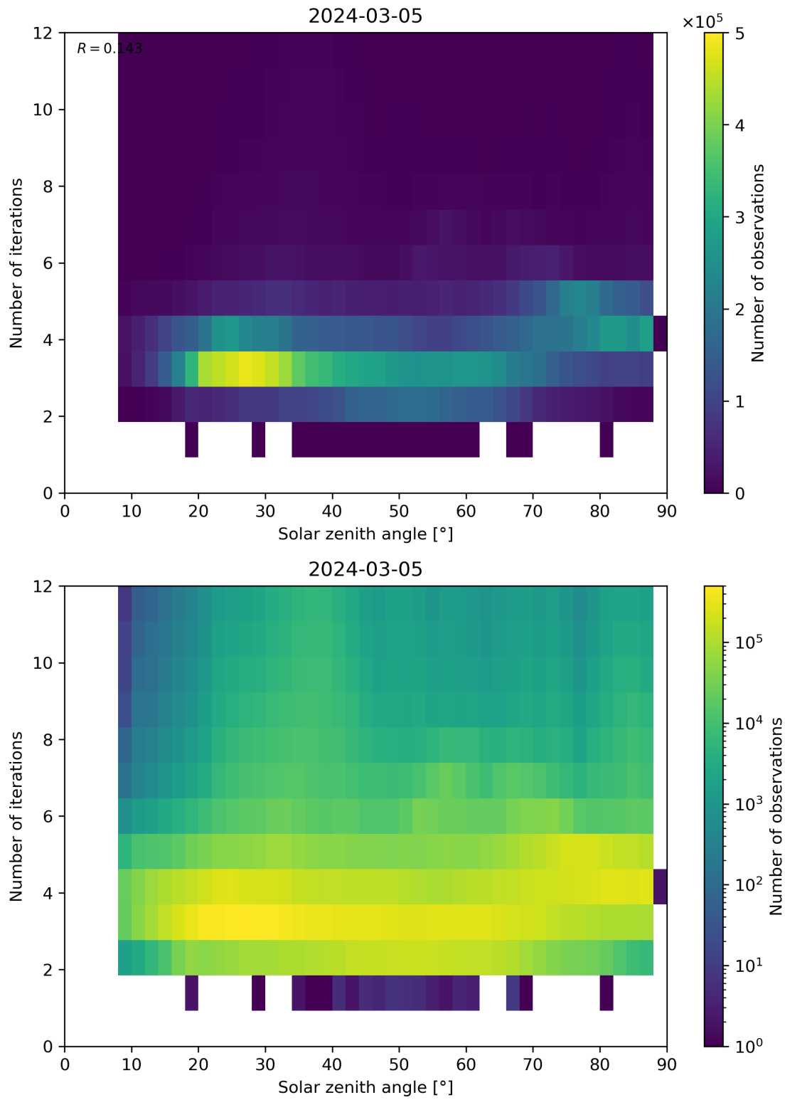
Figure 114: Scatter density plot of “Solar zenith angle” against “Number of iterations” for 2024-03-04 to 2024-03-06.
