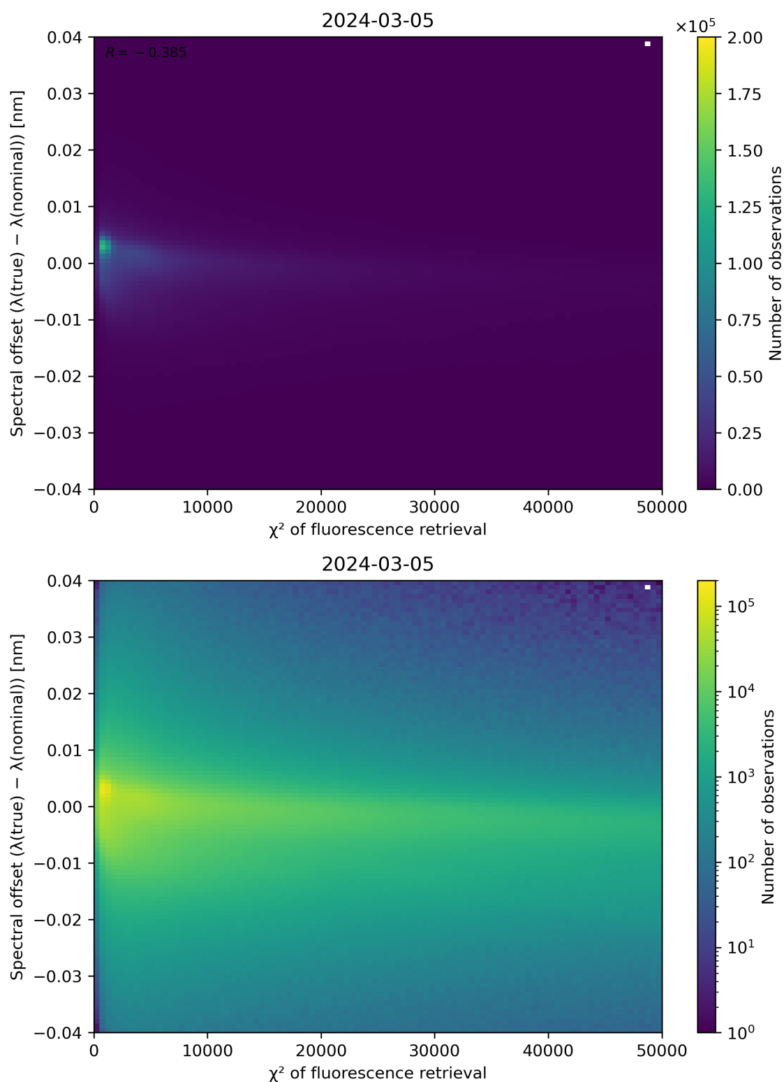
Figure 69: Scatter density plot of “ \chi^2 of fluorescence retrieval” against “Spectral offset ( \lambda(\text{true}) - \lambda(\text{nominal}) )” for 2024-03-04 to 2024-03-06.
