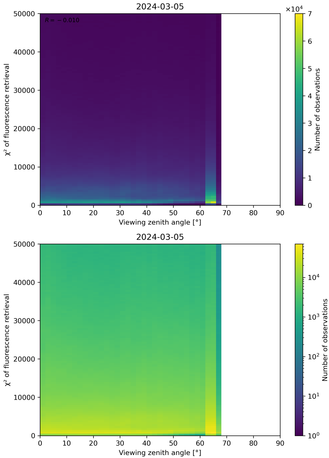
Figure 119: Scatter density plot of “Viewing zenith angle” against “ \chi^2 of fluorescence retrieval” for 2024-03-04 to 2024-03-06.
