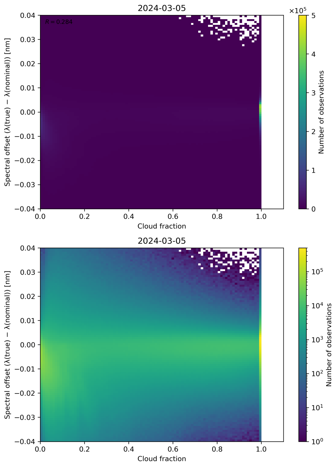
Figure 76: Scatter density plot of “Cloud fraction” against “Spectral offset ( \lambda(\text{true}) - \lambda(\text{nominal}) )” for 2024-03-04 to 2024-03-06.
