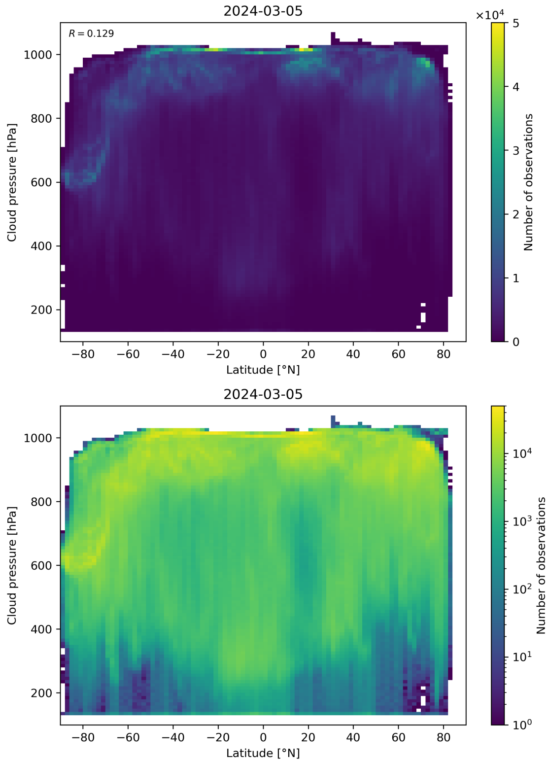
Figure 91: Scatter density plot of “Latitude” against “Cloud pressure” for 2024-03-04 to 2024-03-06.
