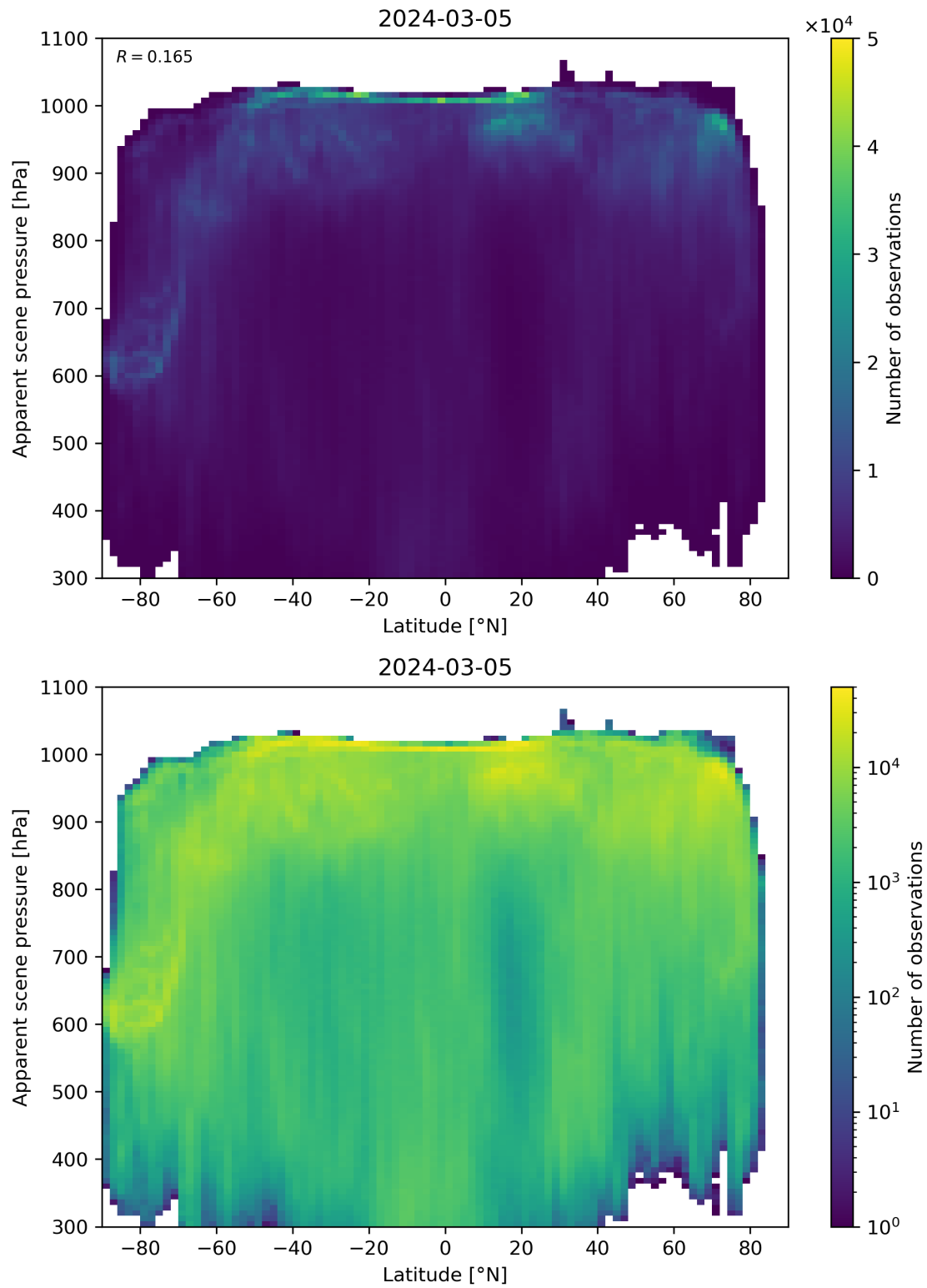
Figure 88: Scatter density plot of “Latitude” against “Apparent scene pressure” for 2024-03-04 to 2024-03-06.
