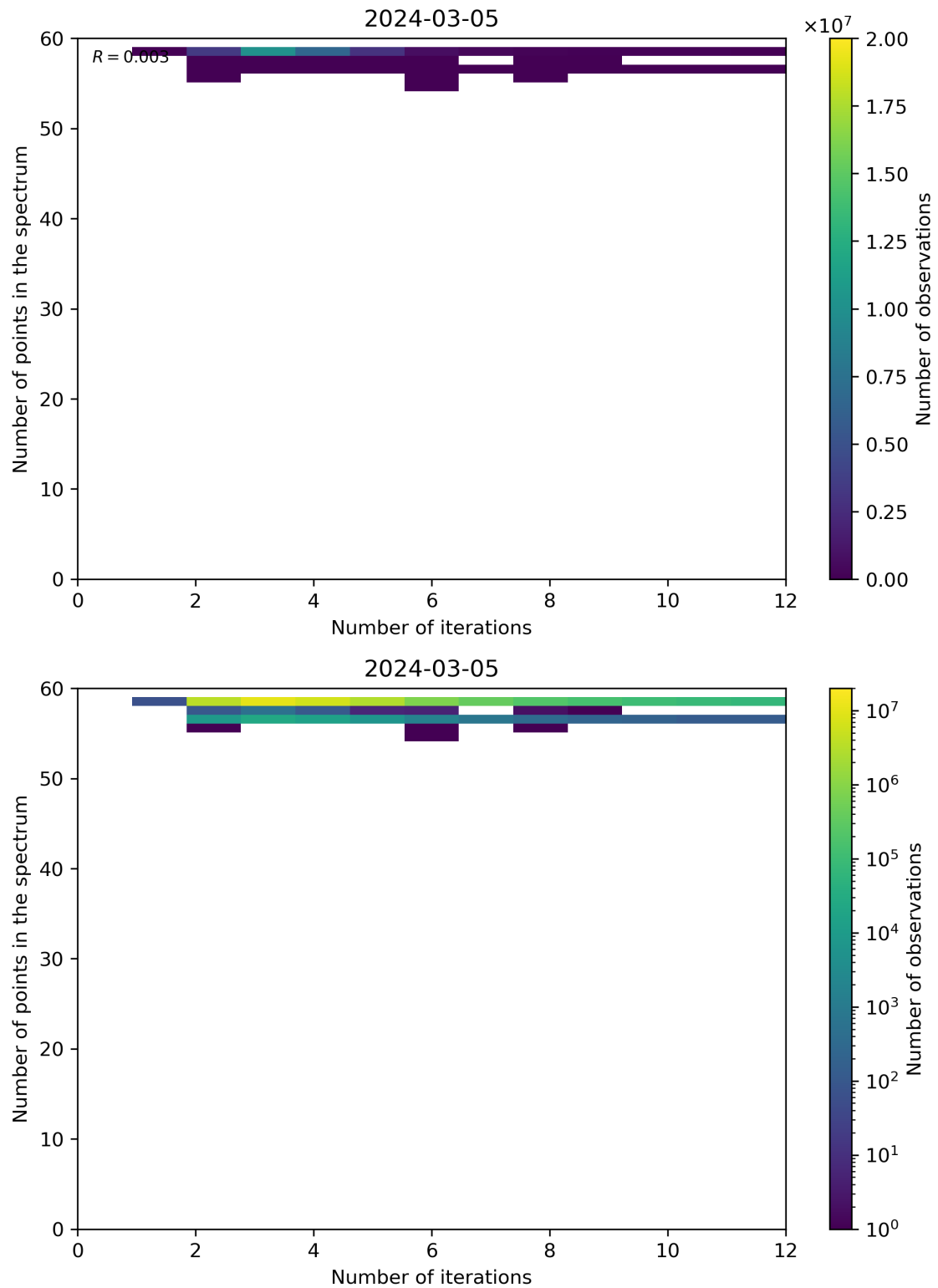
Figure 99: Scatter density plot of “Number of iterations” against “Number of points in the spectrum” for 2024-03-04 to 2024-03-06.
