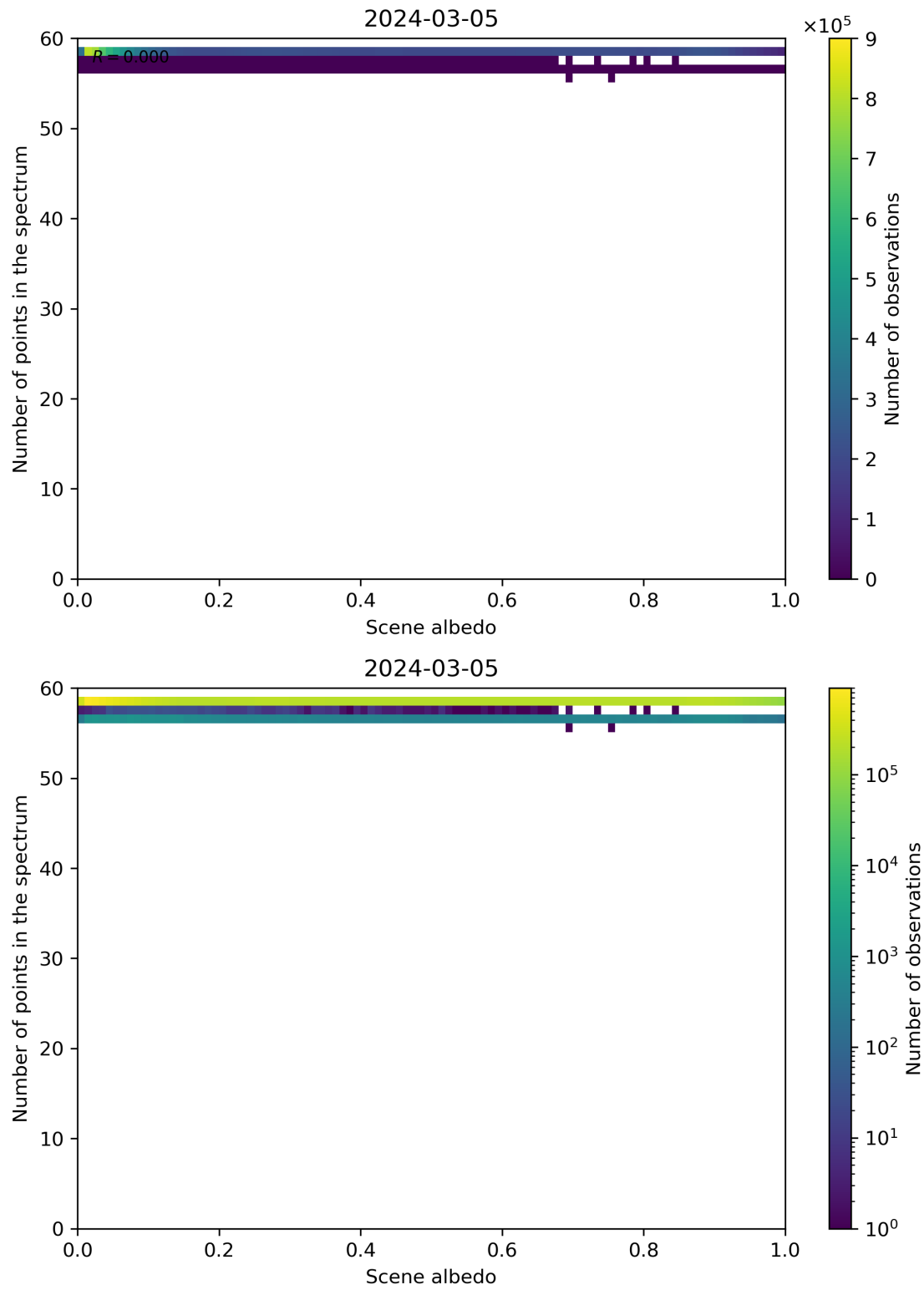
Figure 106: Scatter density plot of “Scene albedo” against “Number of points in the spectrum” for 2024-03-04 to 2024-03-06.
