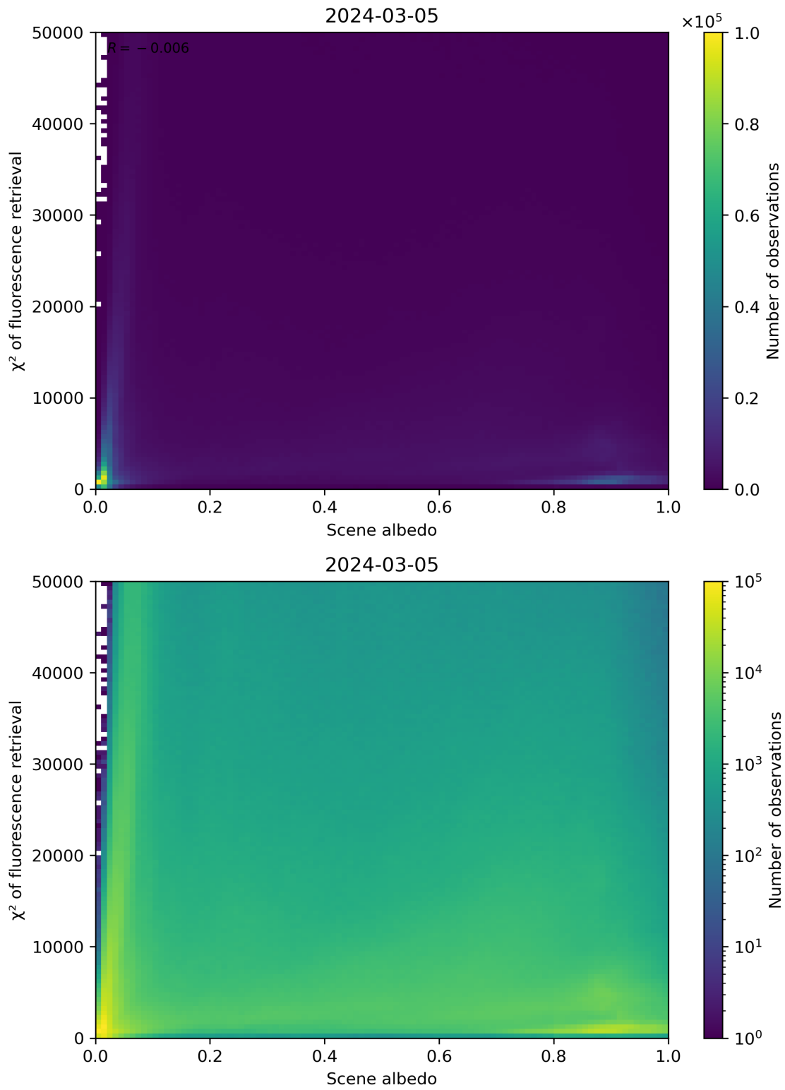
Figure 103: Scatter density plot of “Scene albedo” against “ \chi^2 of fluorescence retrieval” for 2024-03-04 to 2024-03-06.
