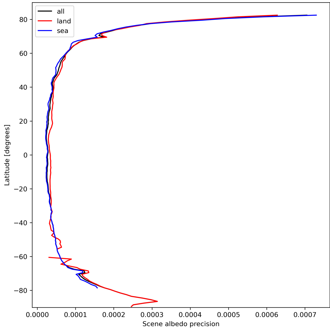
Figure 18: Zonal average of “Scene albedo precision” for 2024-03-04 to 2024-03-06.
