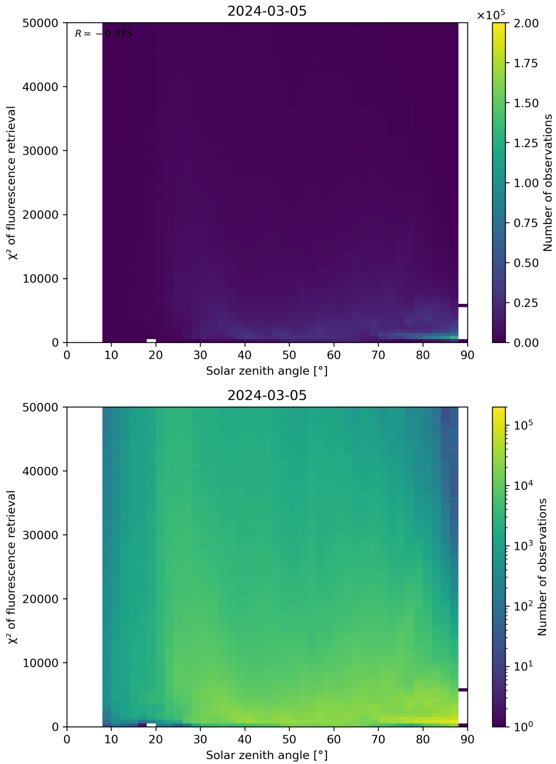
Figure 109: Scatter density plot of “Solar zenith angle” against “ \chi^2 of fluorescence retrieval” for 2024-03-04 to 2024-03-06.
