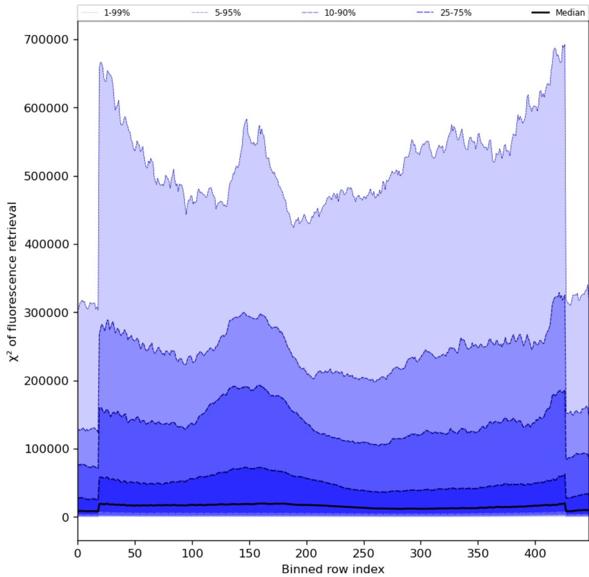
Figure 59: Along track statistics of “ \chi^2 of fluorescence retrieval” for 2024-03-04 to 2024-03-06
