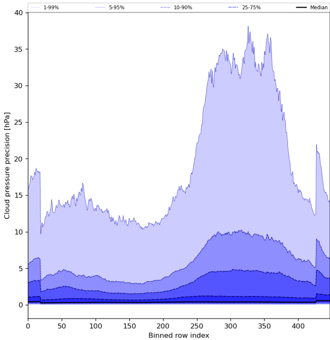
Figure 48: Along track statistics of “Cloud pressure precision” for 2024-03-04 to 2024-03-06
