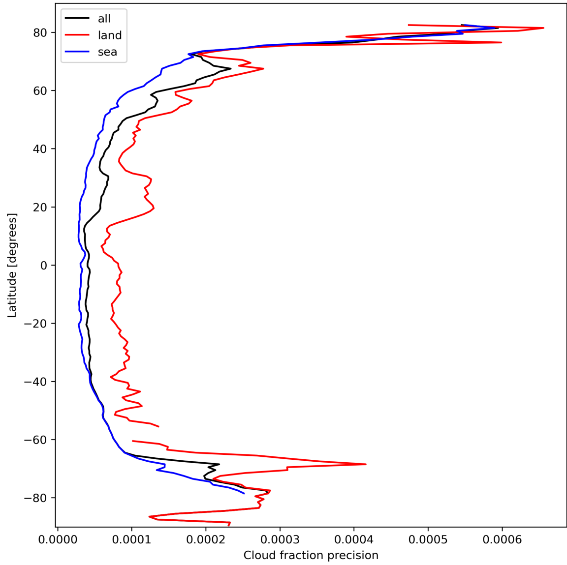
Figure 16: Zonal average of “Cloud fraction precision” for 2024-03-05 to 2024-03-07.
