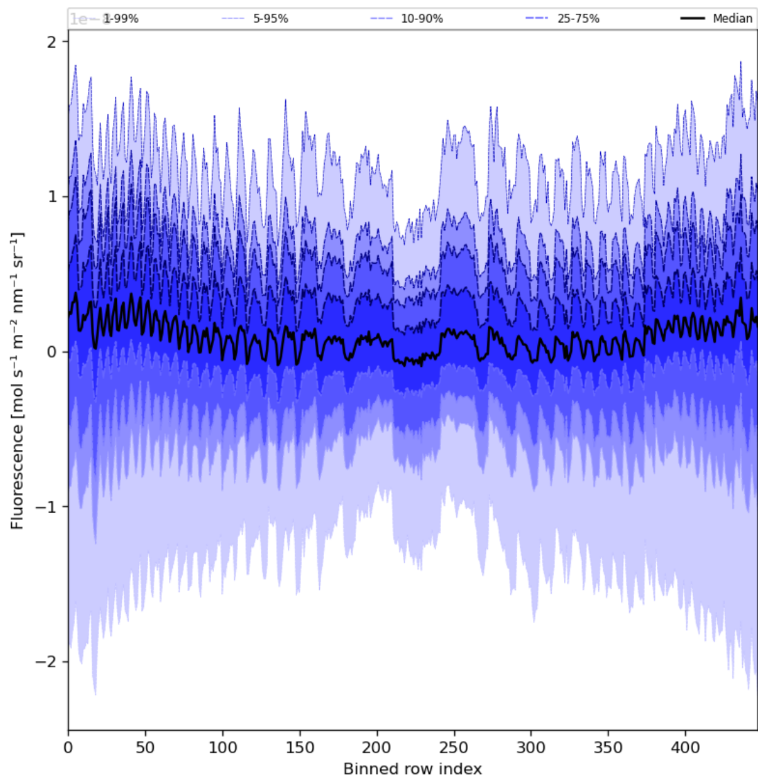
Figure 57: Along track statistics of “Fluorescence” for 2024-03-05 to 2024-03-07
