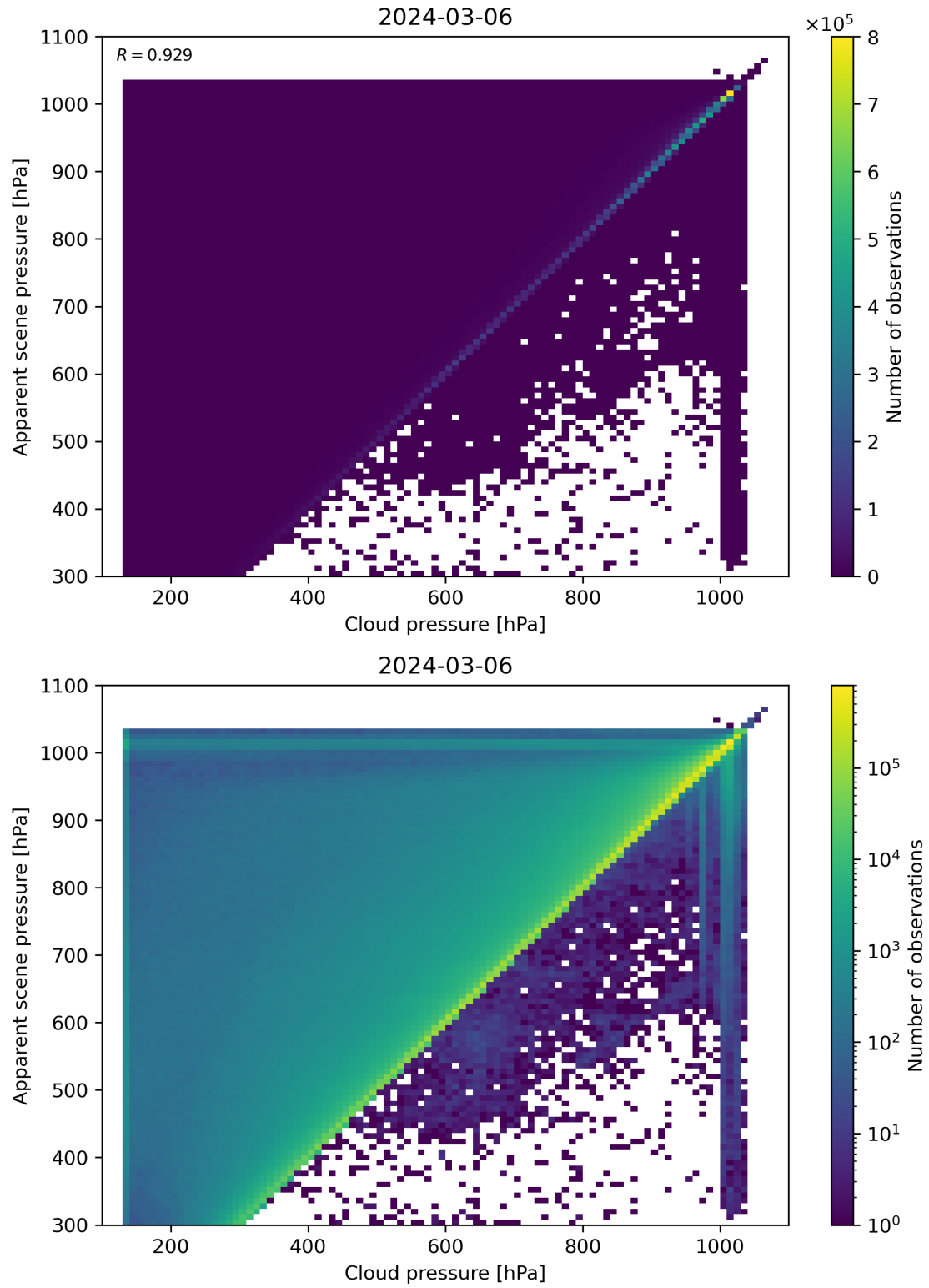
Figure 77: Scatter density plot of “Cloud pressure” against “Apparent scene pressure” for 2024-03-05 to 2024-03-07.
