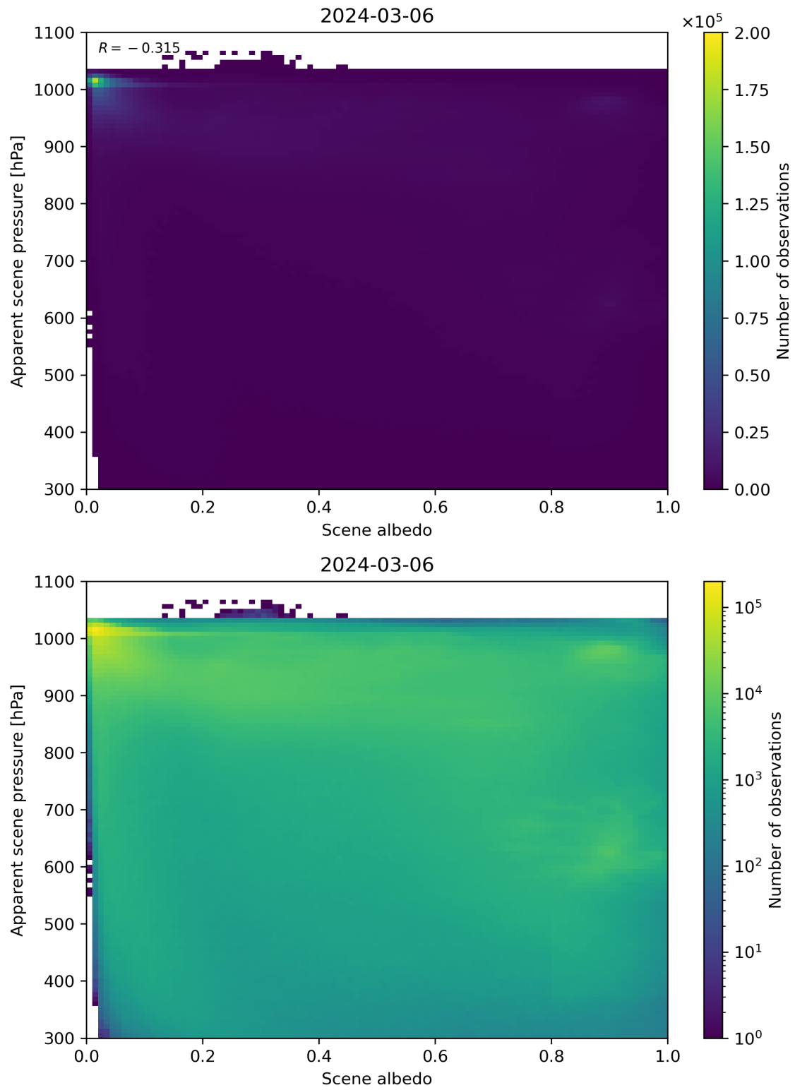
Figure 102: Scatter density plot of “Scene albedo” against “Apparent scene pressure” for 2024-03-05 to 2024-03-07.
