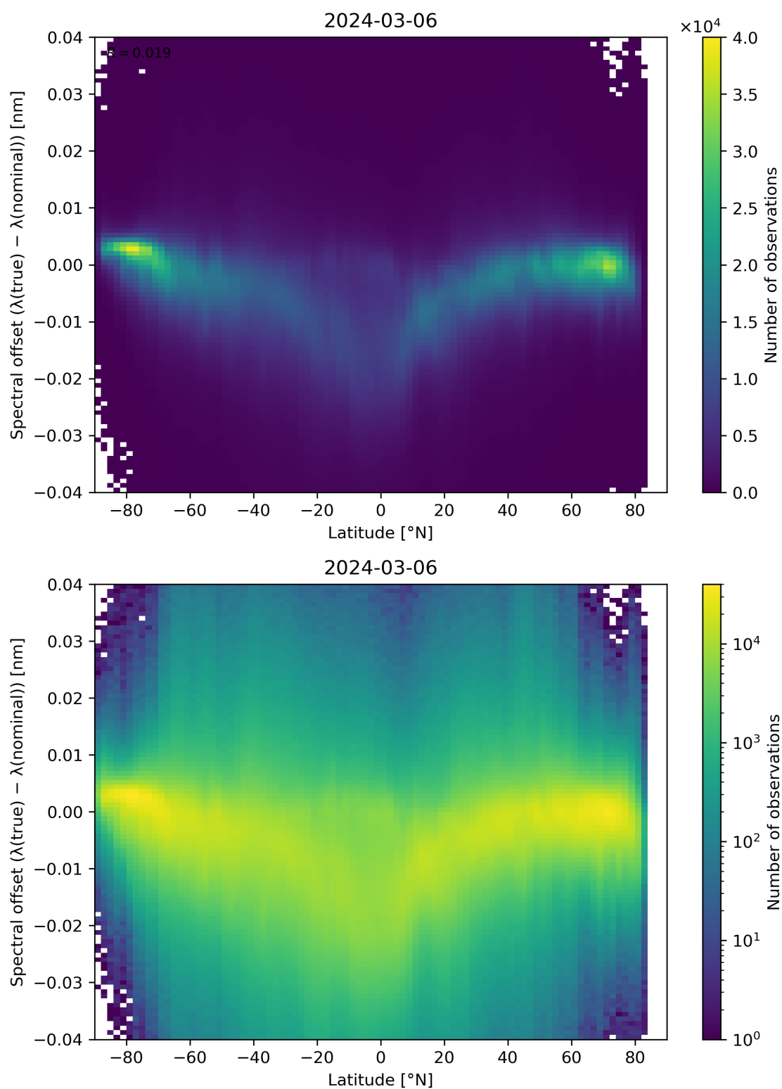
Figure 96: Scatter density plot of “Latitude” against “Spectral offset ( \lambda(\text{true}) - \lambda(\text{nominal}) )” for 2024-03-05 to 2024-03-07.
