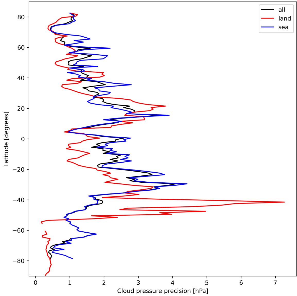
Figure 14: Zonal average of “Cloud pressure precision” for 2024-03-05 to 2024-03-07.
