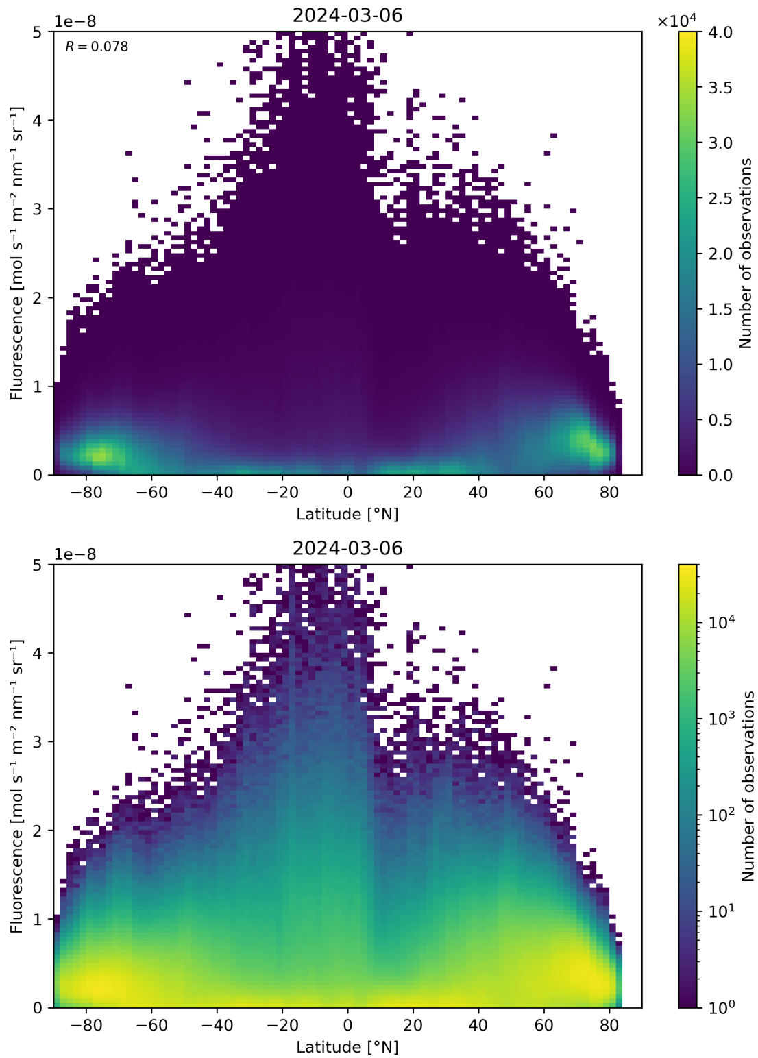
Figure 92: Scatter density plot of “Latitude” against “Fluorescence” for 2024-03-05 to 2024-03-07.
