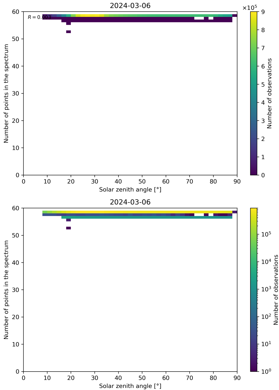
Figure 115: Scatter density plot of “Solar zenith angle” against “Number of points in the spectrum” for 2024-03-05 to 2024-03-07.
