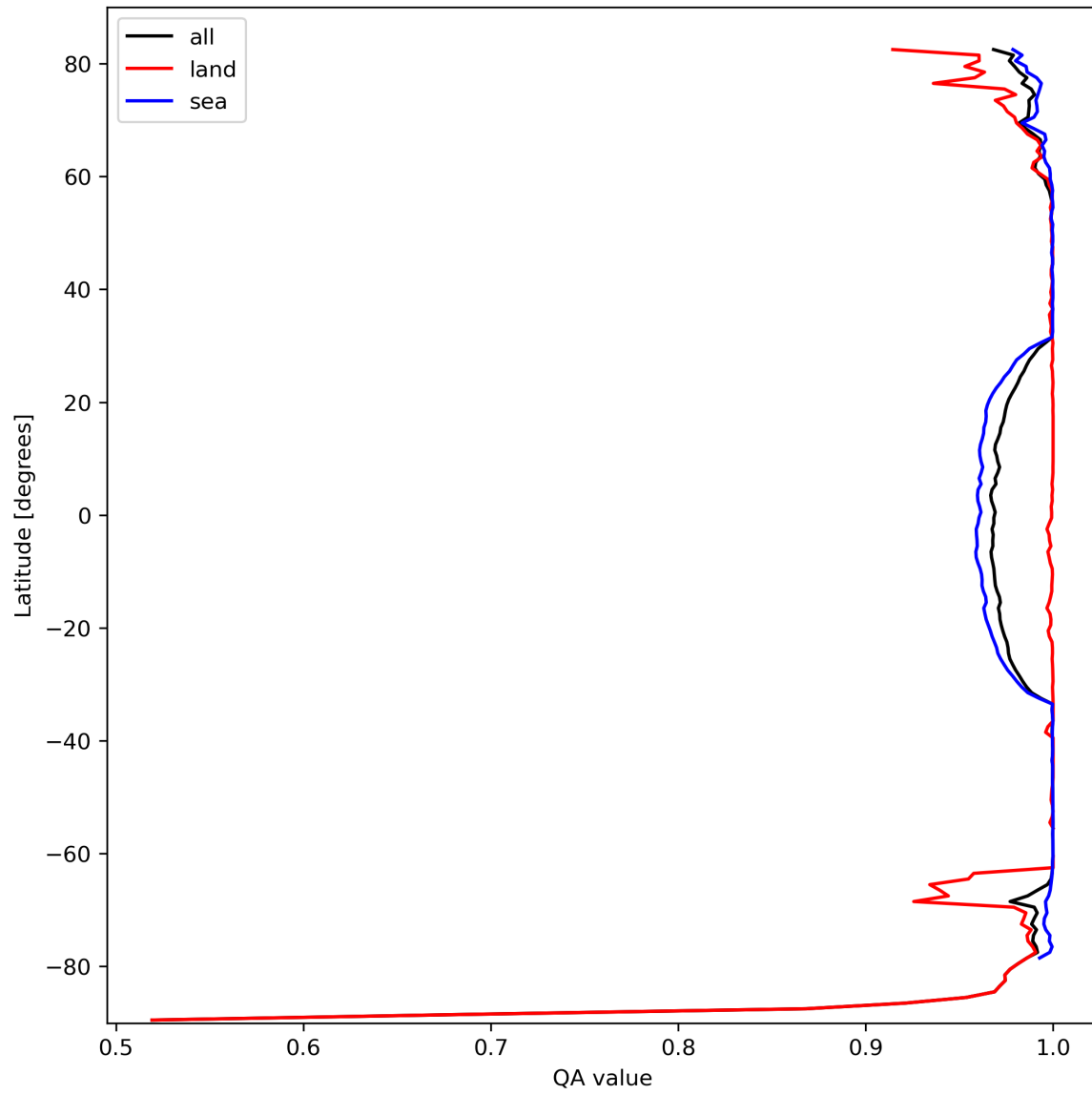
Figure 12: Zonal average of “QA value” for 2024-03-05 to 2024-03-07.
