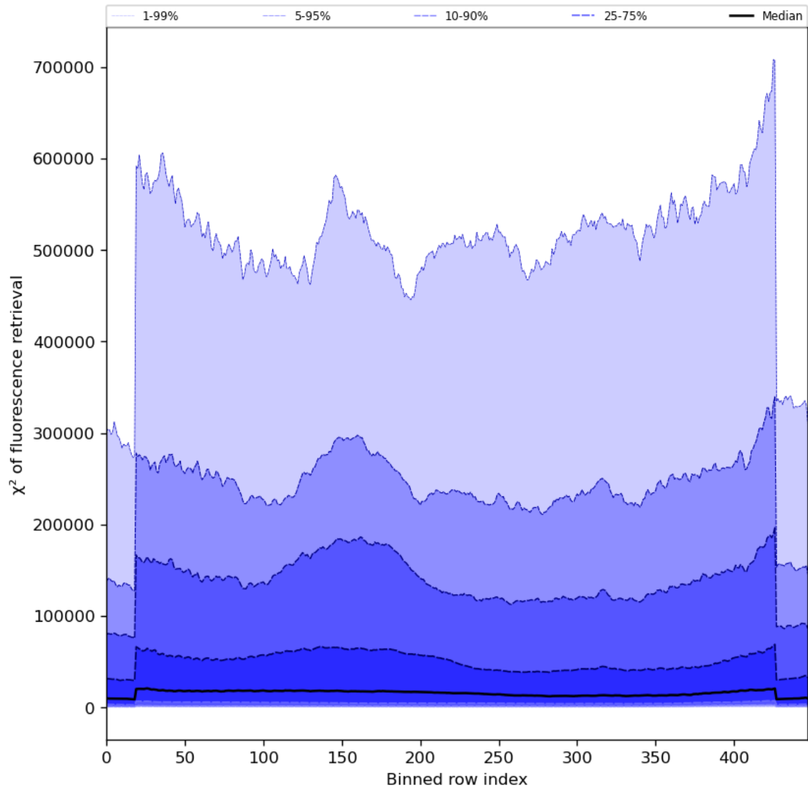
Figure 59: Along track statistics of “ \chi^2 of fluorescence retrieval” for 2024-03-05 to 2024-03-07
