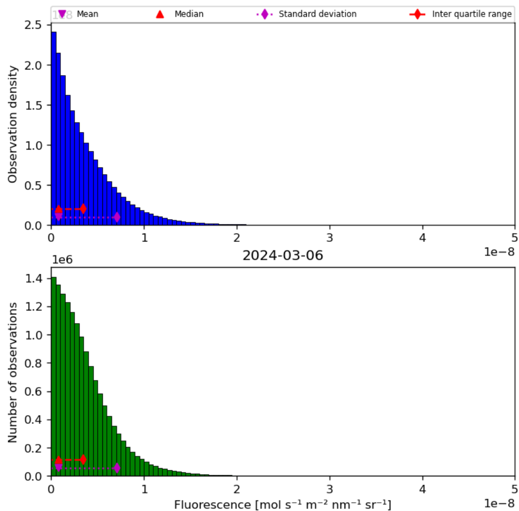
Figure 40: Histogram of “Fluorescence” for 2024-03-05 to 2024-03-07
