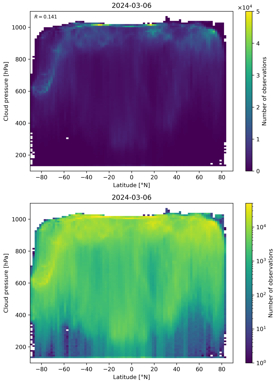
Figure 91: Scatter density plot of “Latitude” against “Cloud pressure” for 2024-03-05 to 2024-03-07.
