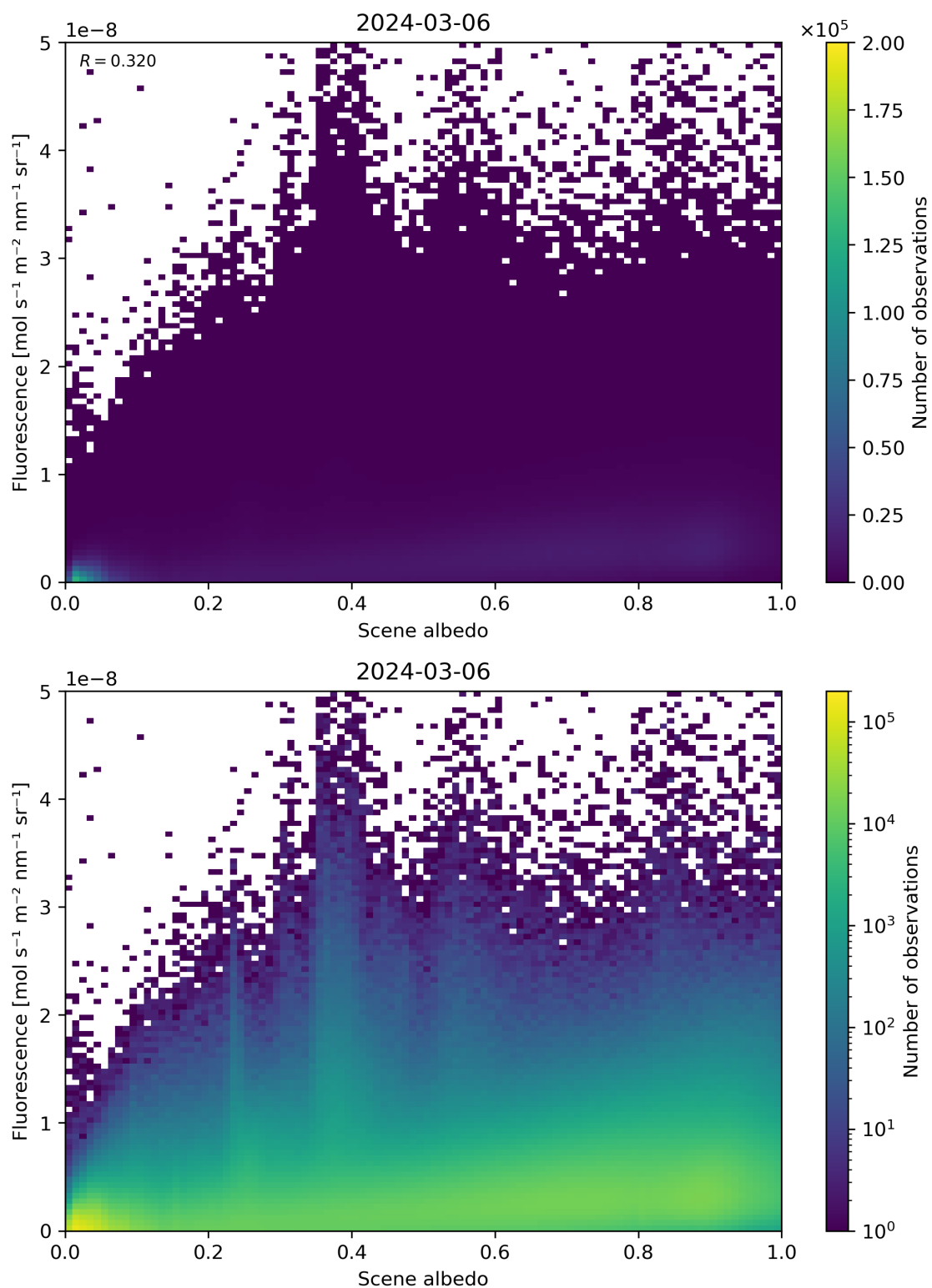
Figure 104: Scatter density plot of “Scene albedo” against “Fluorescence” for 2024-03-05 to 2024-03-07.
