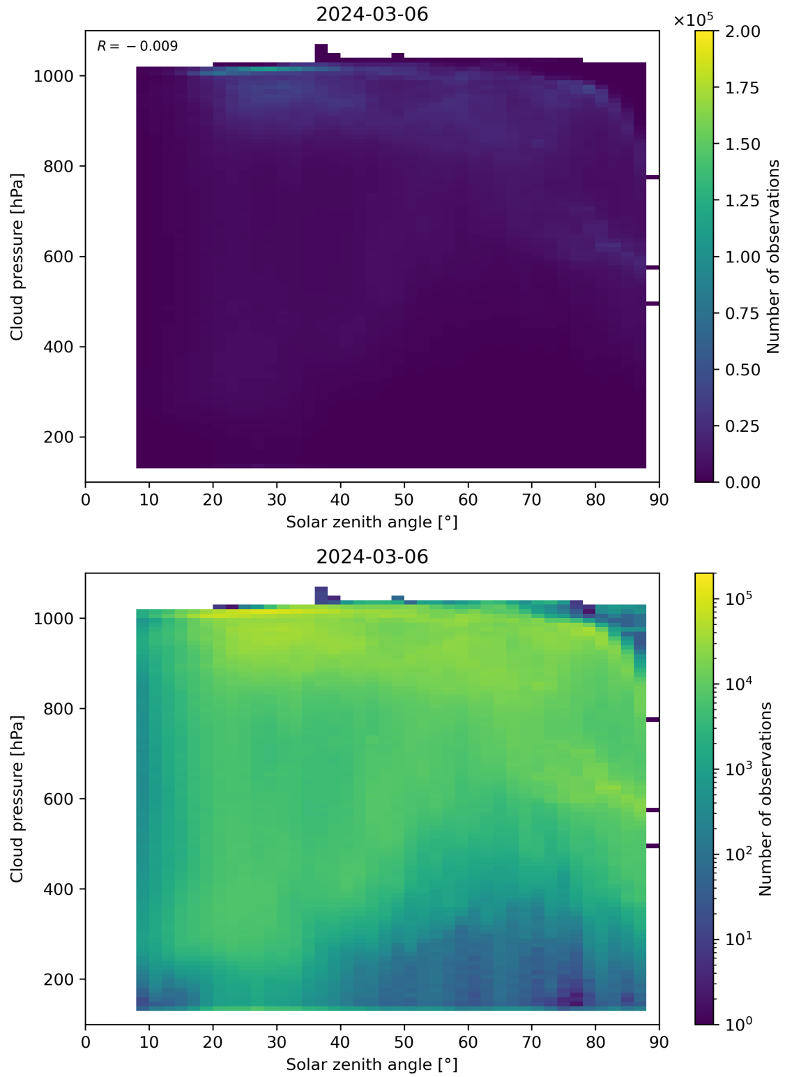
Figure 111: Scatter density plot of “Solar zenith angle” against “Cloud pressure” for 2024-03-05 to 2024-03-07.
