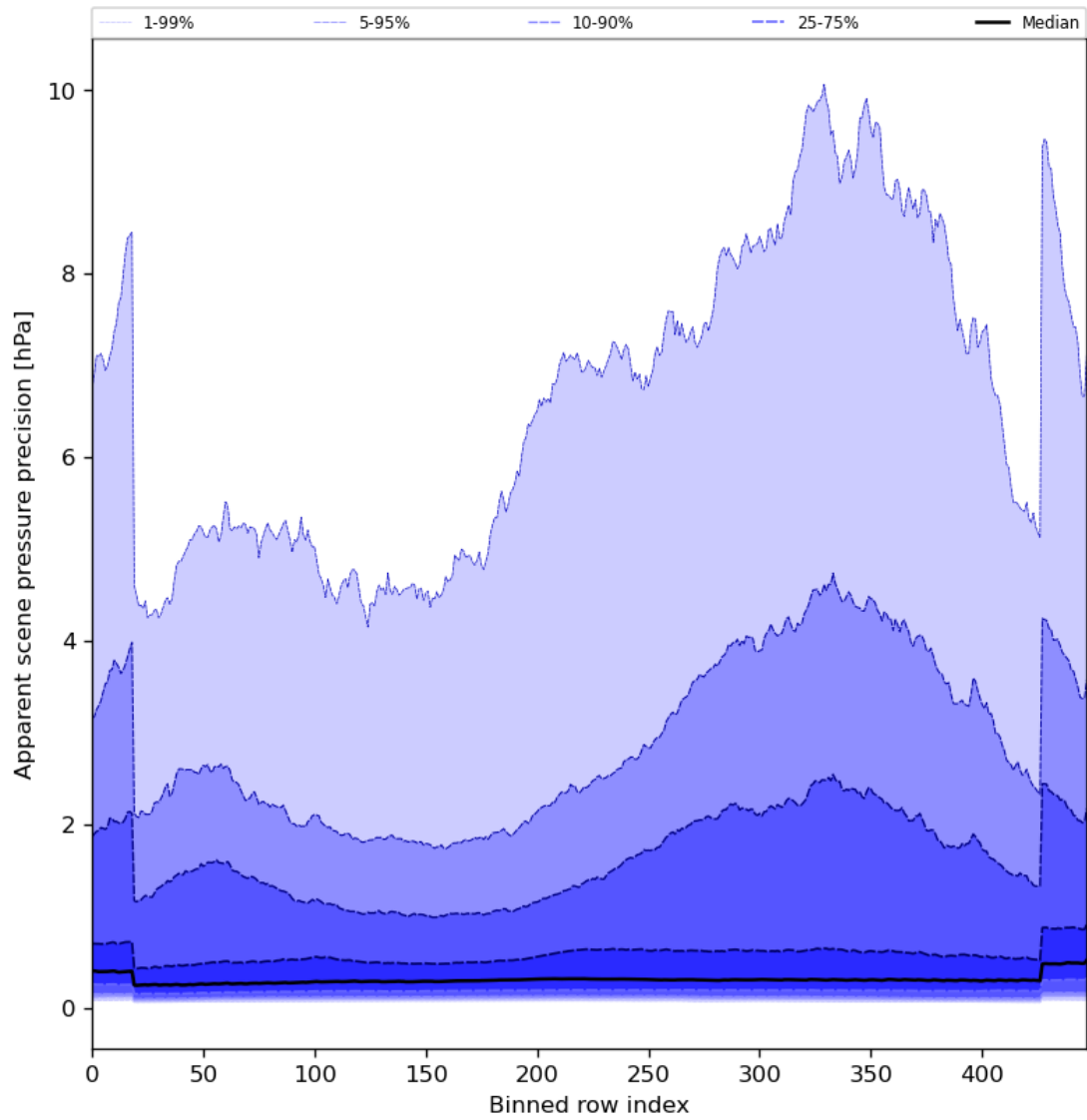
Figure 54: Along track statistics of “Apparent scene pressure precision” for 2024-03-05 to 2024-03-07
