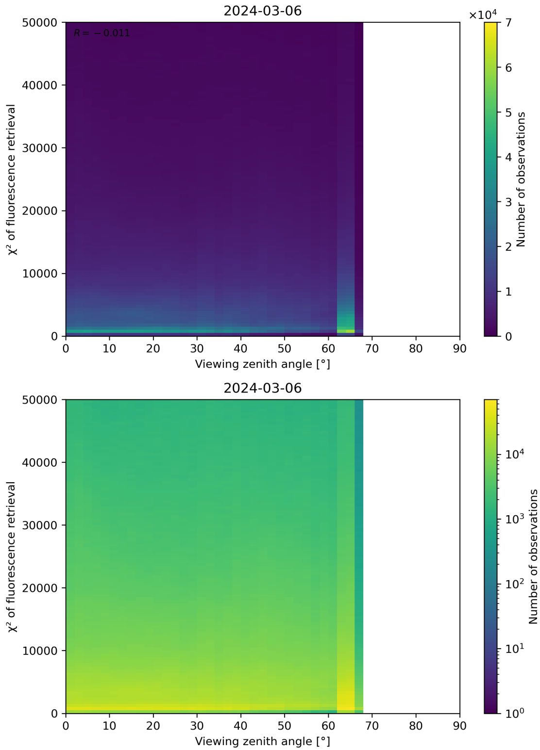
Figure 119: Scatter density plot of “Viewing zenith angle” against “ \chi^2 of fluorescence retrieval” for 2024-03-05 to 2024-03-07.
