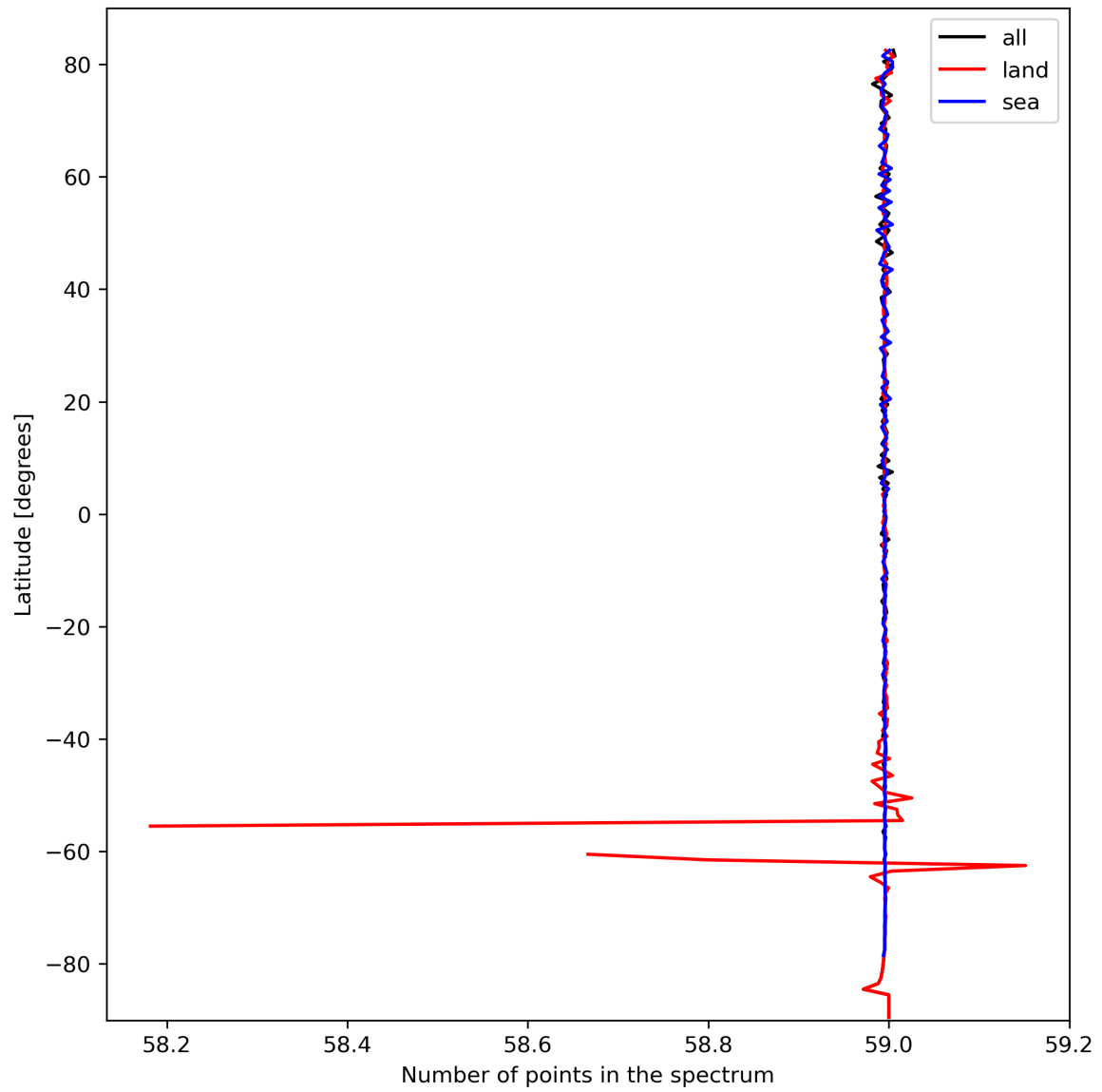
Figure 27: Zonal average of “Number of points in the spectrum” for 2024-03-05 to 2024-03-07.
