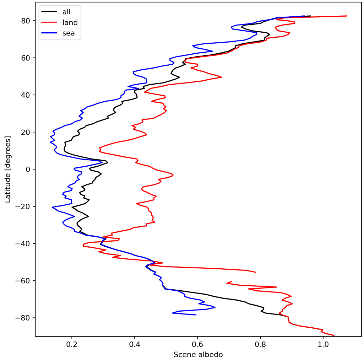
Figure 17: Zonal average of “Scene albedo” for 2024-03-05 to 2024-03-07.
