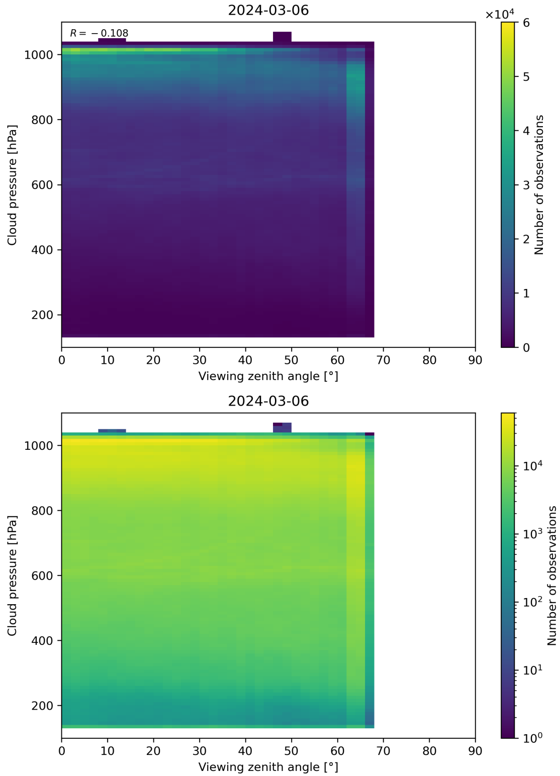
Figure 121: Scatter density plot of “Viewing zenith angle” against “Cloud pressure” for 2024-03-05 to 2024-03-07.
