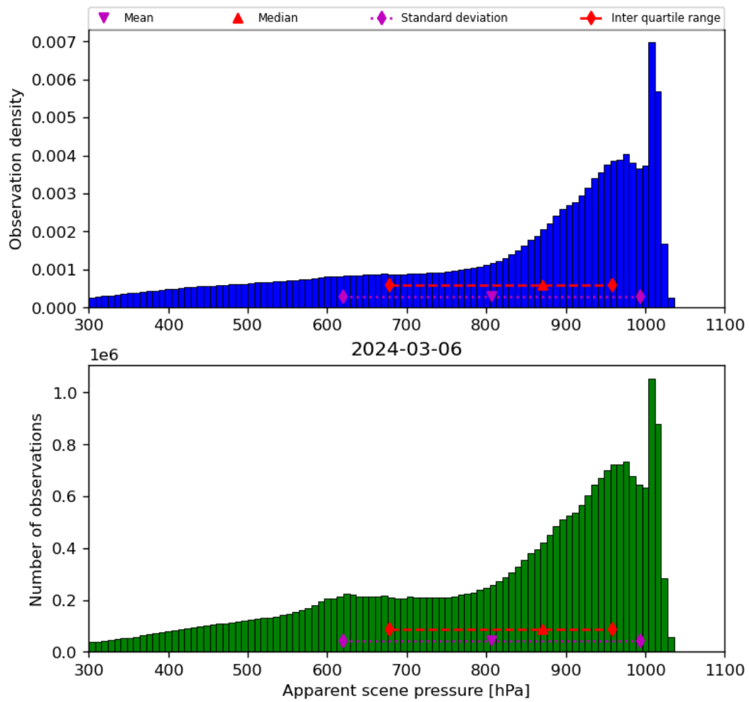
Figure 36: Histogram of “Apparent scene pressure” for 2024-03-05 to 2024-03-07
