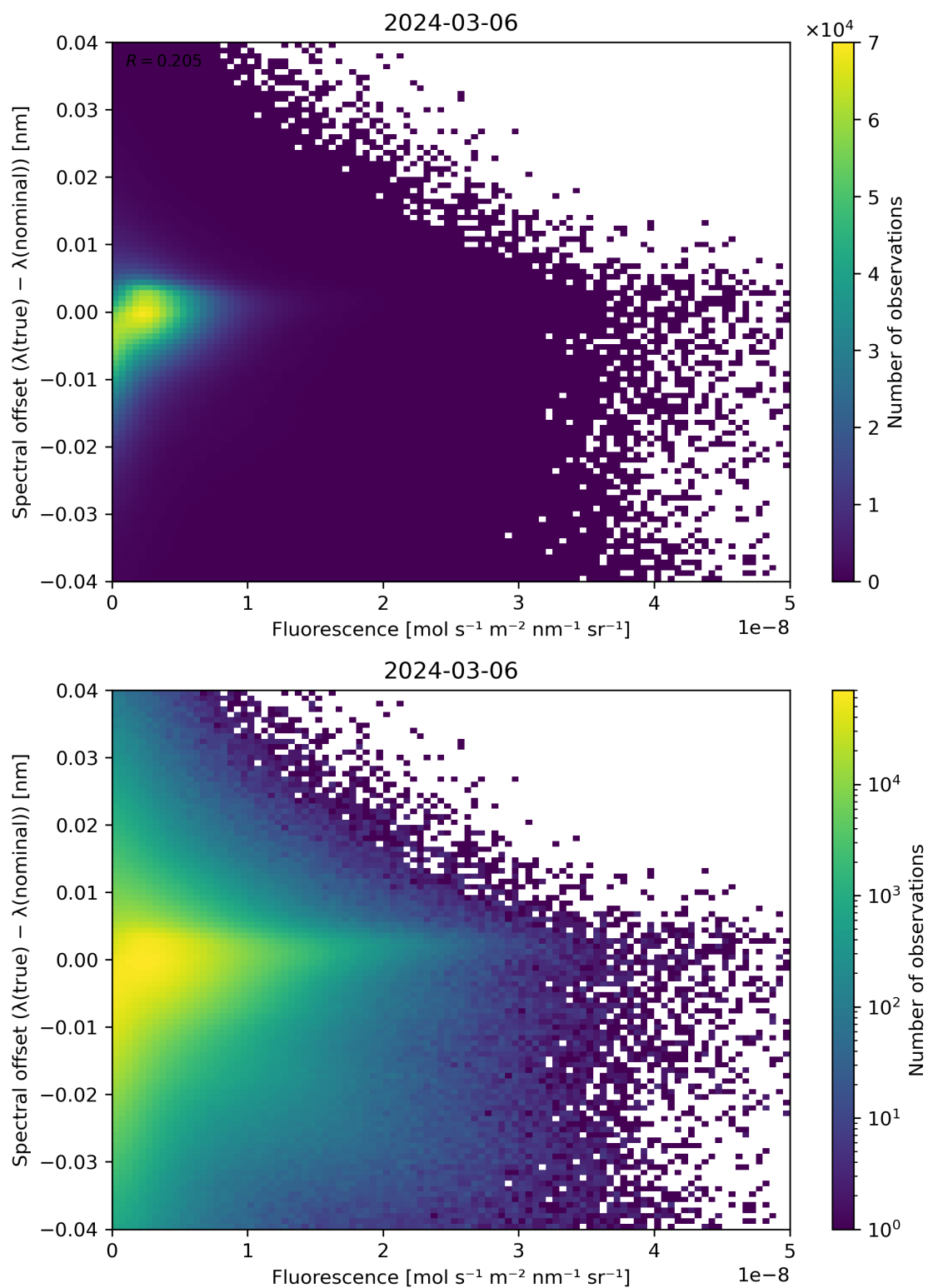
Figure 87: Scatter density plot of “Fluorescence” against “Spectral offset ( \lambda(\text{true}) - \lambda(\text{nominal}) )” for 2024-03-05 to 2024-03-07.
