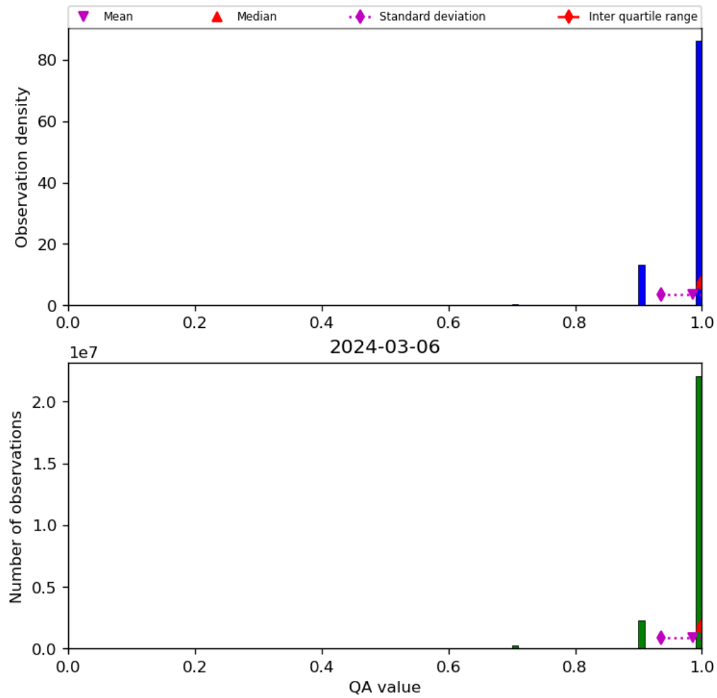
Figure 29: Histogram of “QA value” for 2024-03-05 to 2024-03-07
