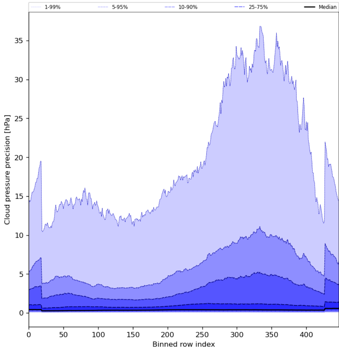
Figure 48: Along track statistics of “Cloud pressure precision” for 2024-03-05 to 2024-03-07
