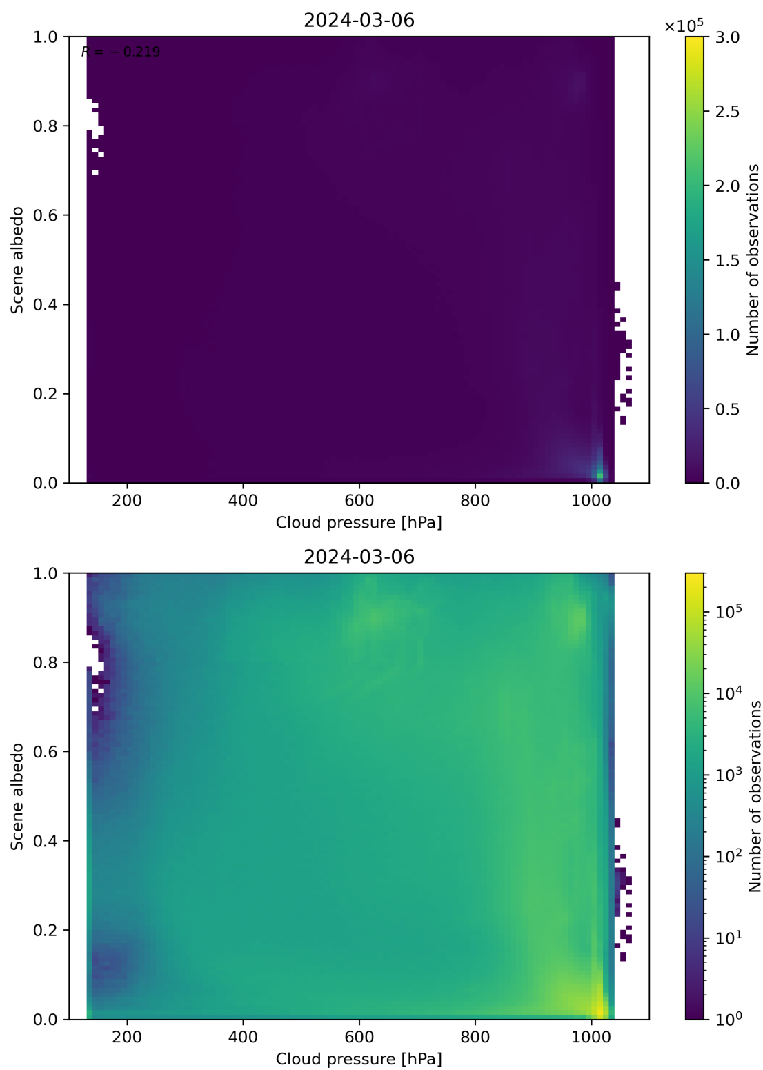
Figure 83: Scatter density plot of “Cloud pressure” against “Scene albedo” for 2024-03-05 to 2024-03-07.
