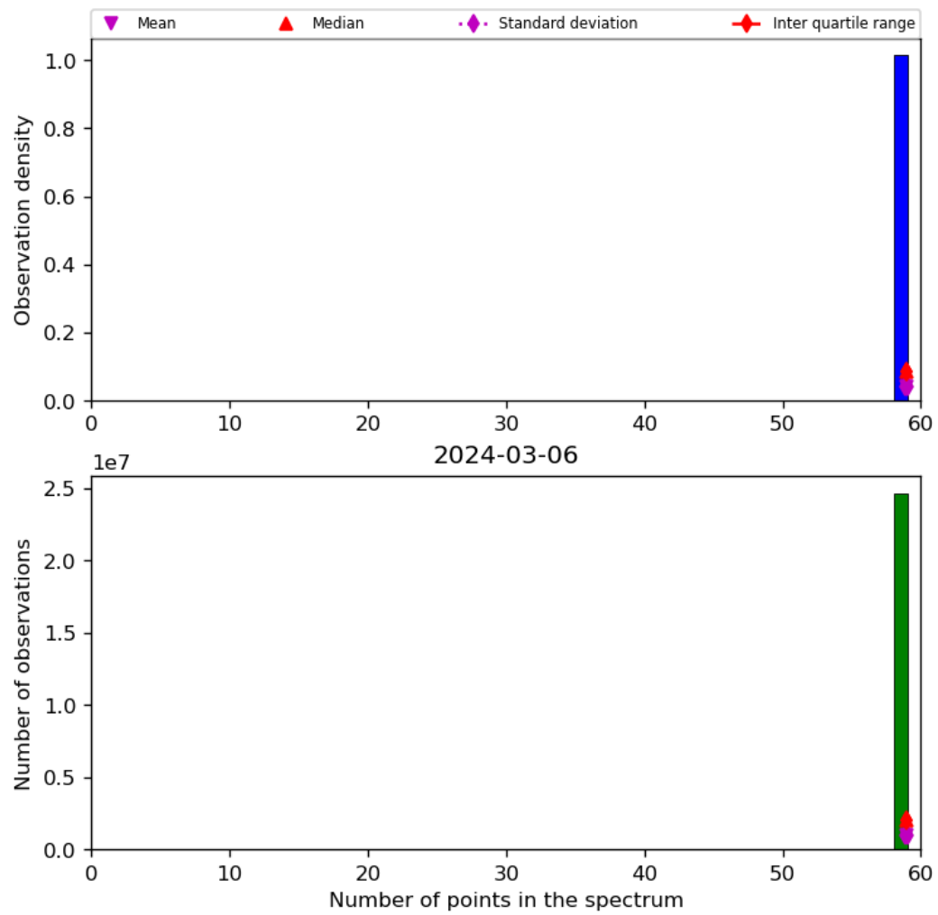
Figure 44: Histogram of “Number of points in the spectrum” for 2024-03-05 to 2024-03-07
