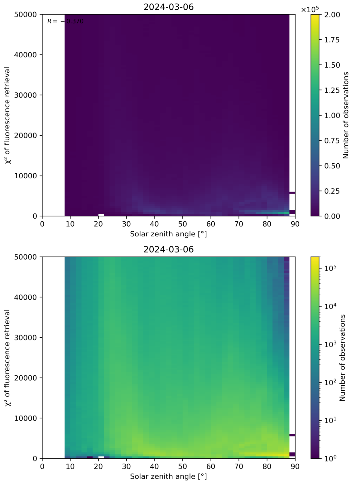
Figure 109: Scatter density plot of “Solar zenith angle” against “ \chi^2 of fluorescence retrieval” for 2024-03-05 to 2024-03-07.
