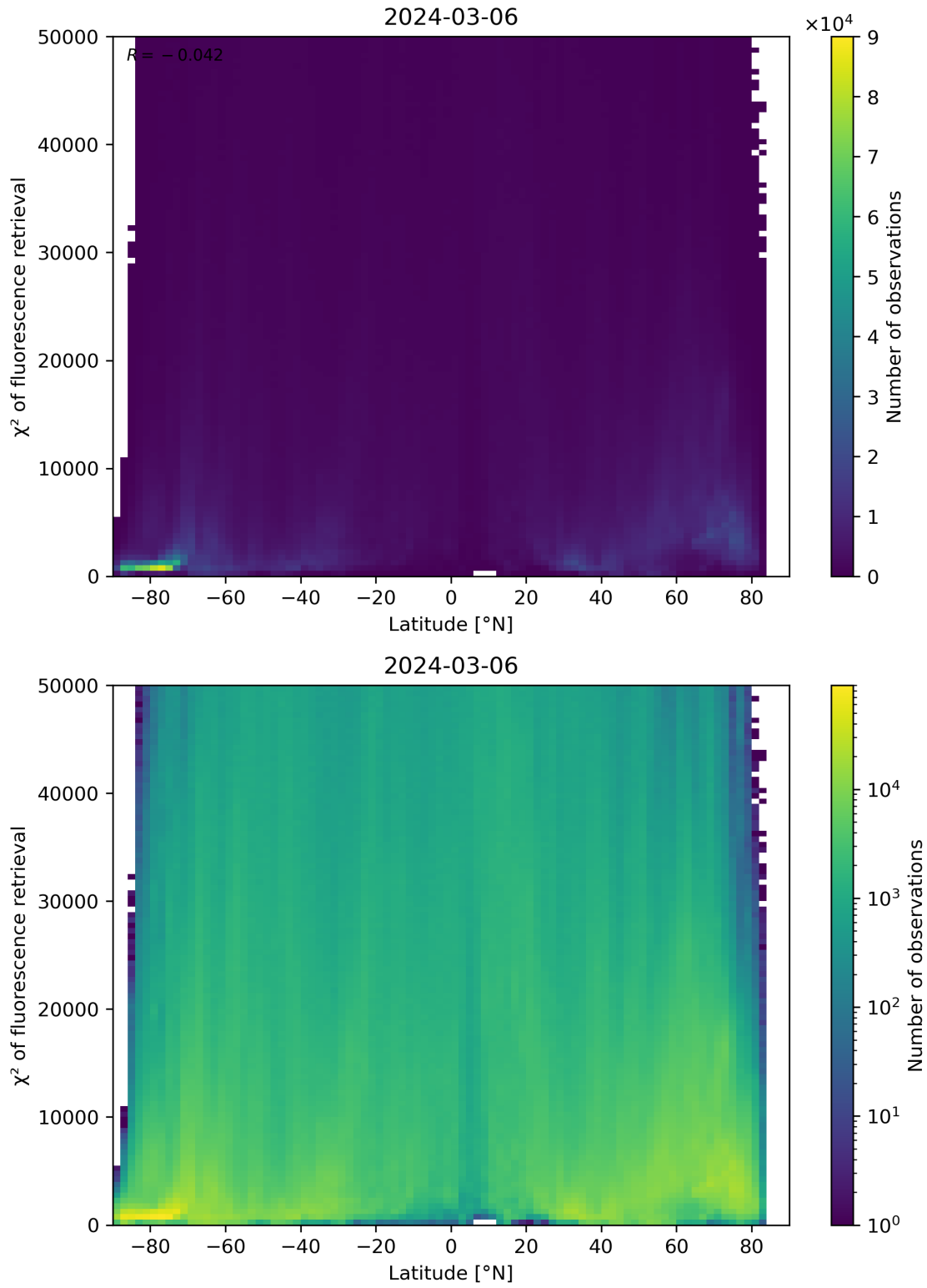
Figure 89: Scatter density plot of “Latitude” against “ \chi^2 of fluorescence retrieval” for 2024-03-05 to 2024-03-07.
