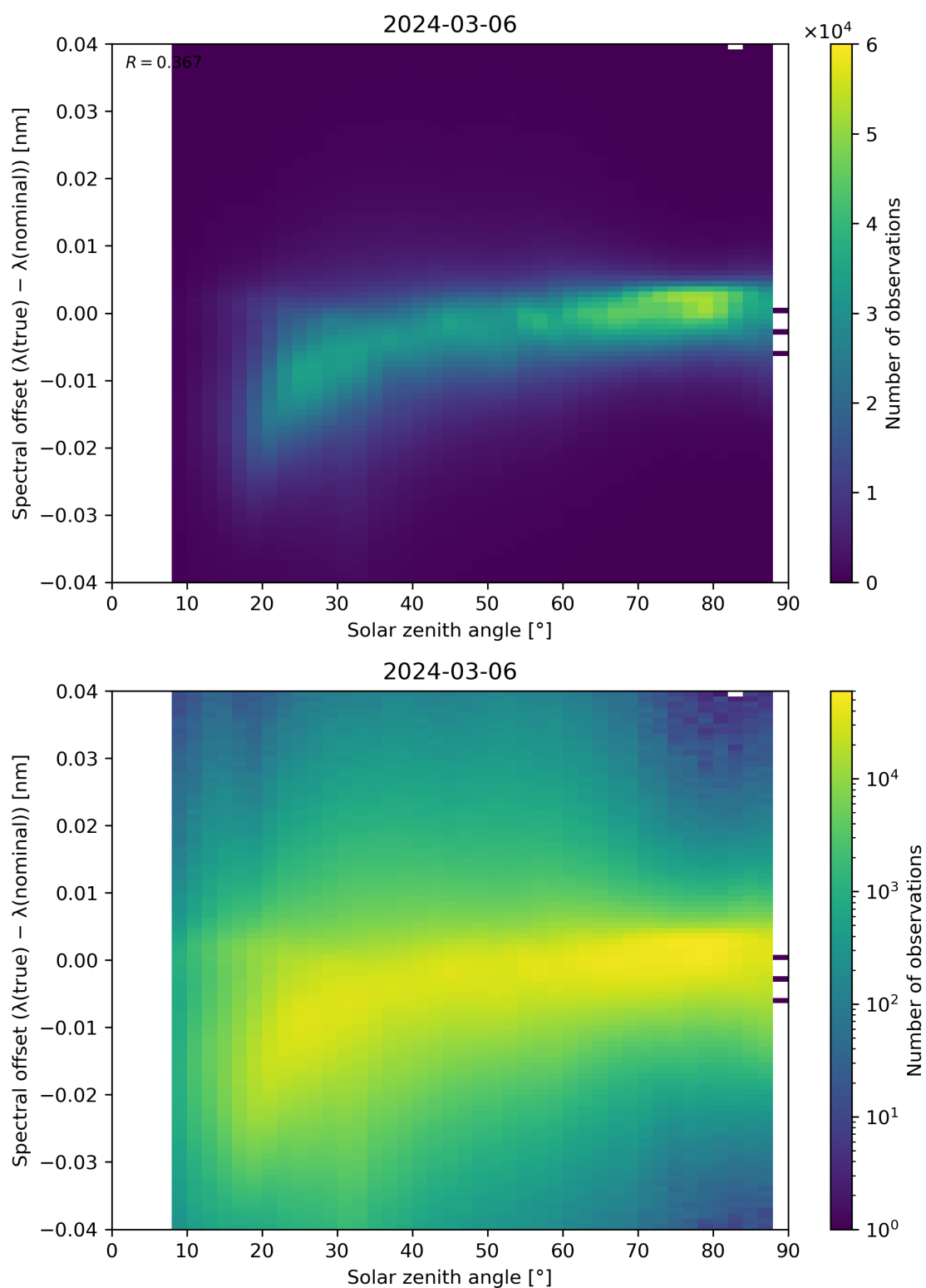
Figure 117: Scatter density plot of “Solar zenith angle” against “Spectral offset ( \lambda(\text{true}) - \lambda(\text{nominal}) )” for 2024-03-05 to 2024-03-07.
