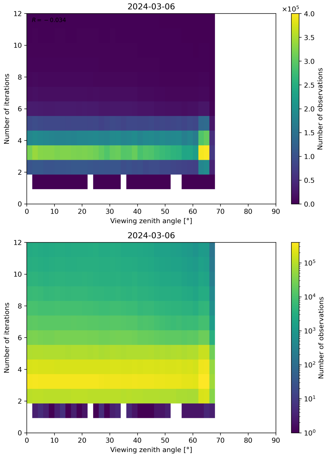
Figure 124: Scatter density plot of “Viewing zenith angle” against “Number of iterations” for 2024-03-05 to 2024-03-07.
