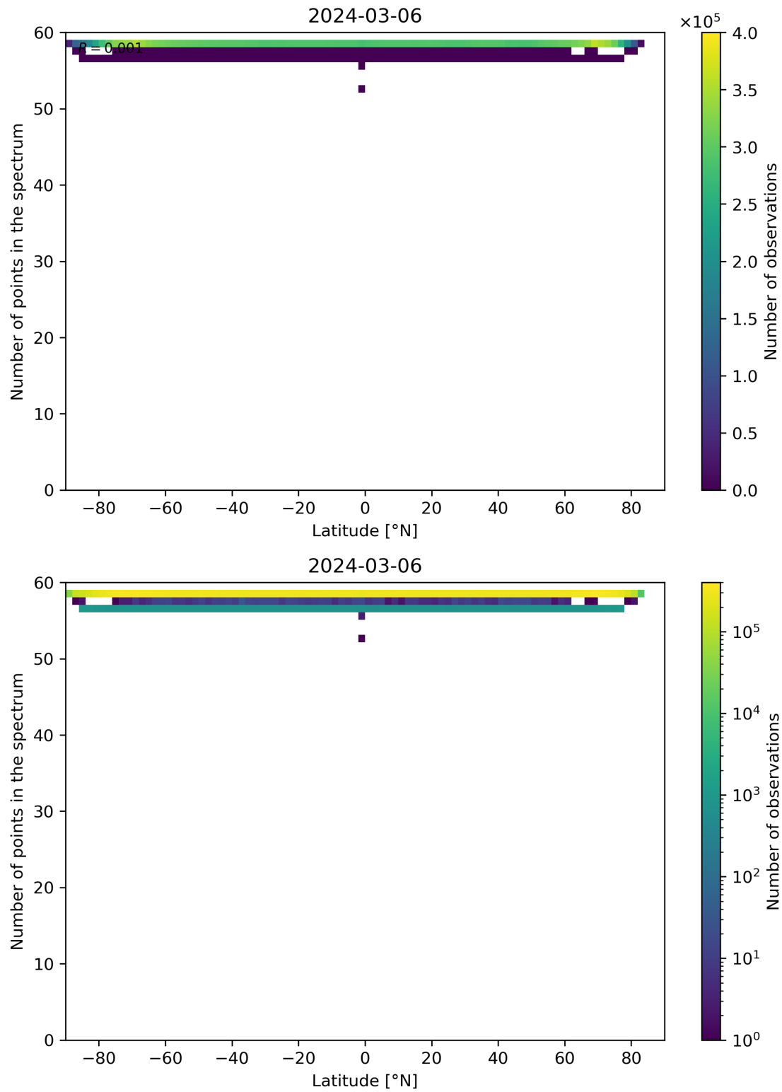
Figure 94: Scatter density plot of “Latitude” against “Number of points in the spectrum” for 2024-03-05 to 2024-03-07.
