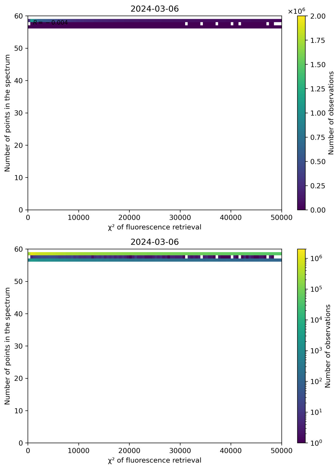
Figure 68: Scatter density plot of " \chi^2 of fluorescence retrieval" against "Number of points in the spectrum" for 2024-03-05 to 2024-03-07.
