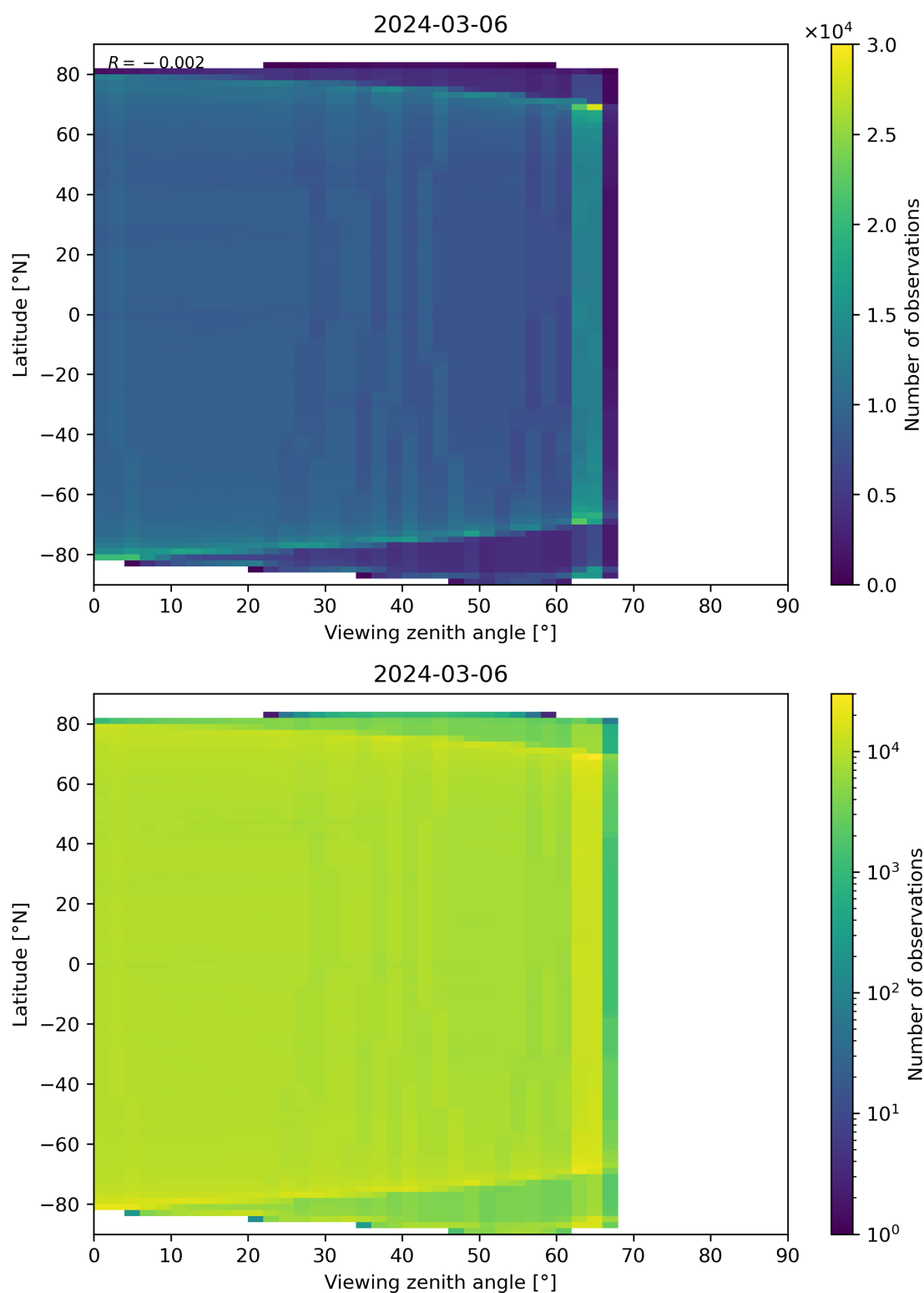
Figure 123: Scatter density plot of “Viewing zenith angle” against “Latitude” for 2024-03-05 to 2024-03-07.
