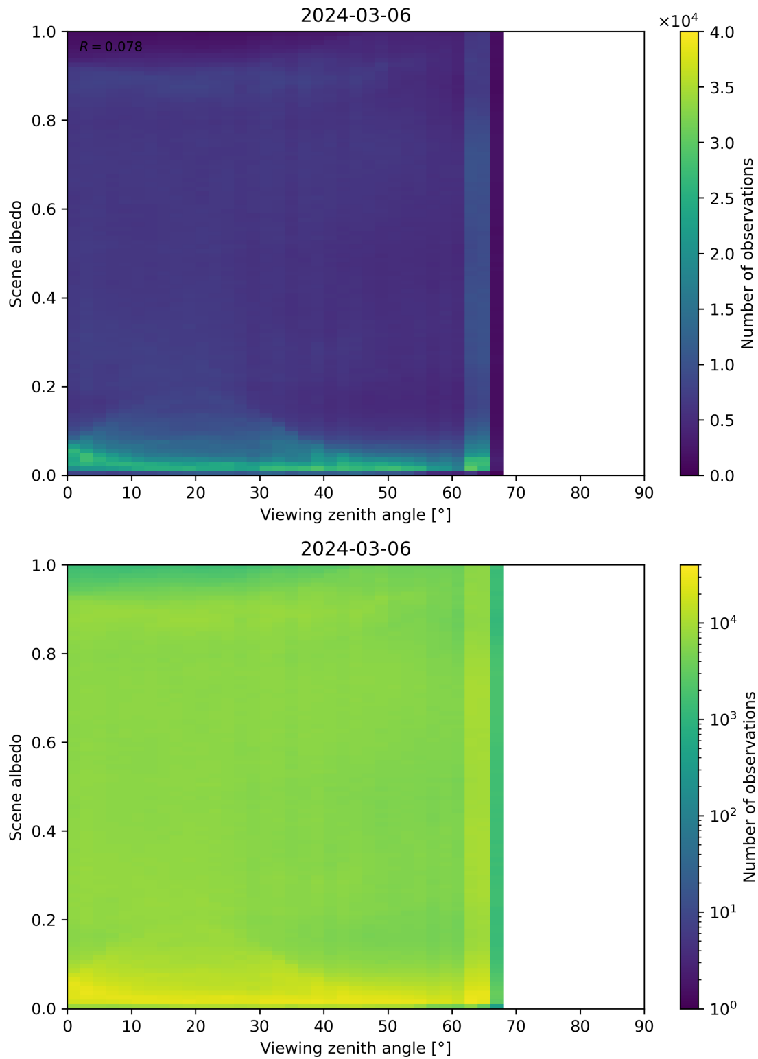
Figure 126: Scatter density plot of “Viewing zenith angle” against “Scene albedo” for 2024-03-05 to 2024-03-07.
