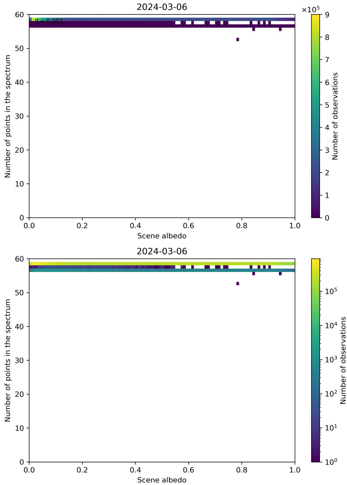
Figure 106: Scatter density plot of “Scene albedo” against “Number of points in the spectrum” for 2024-03-05 to 2024-03-07.
