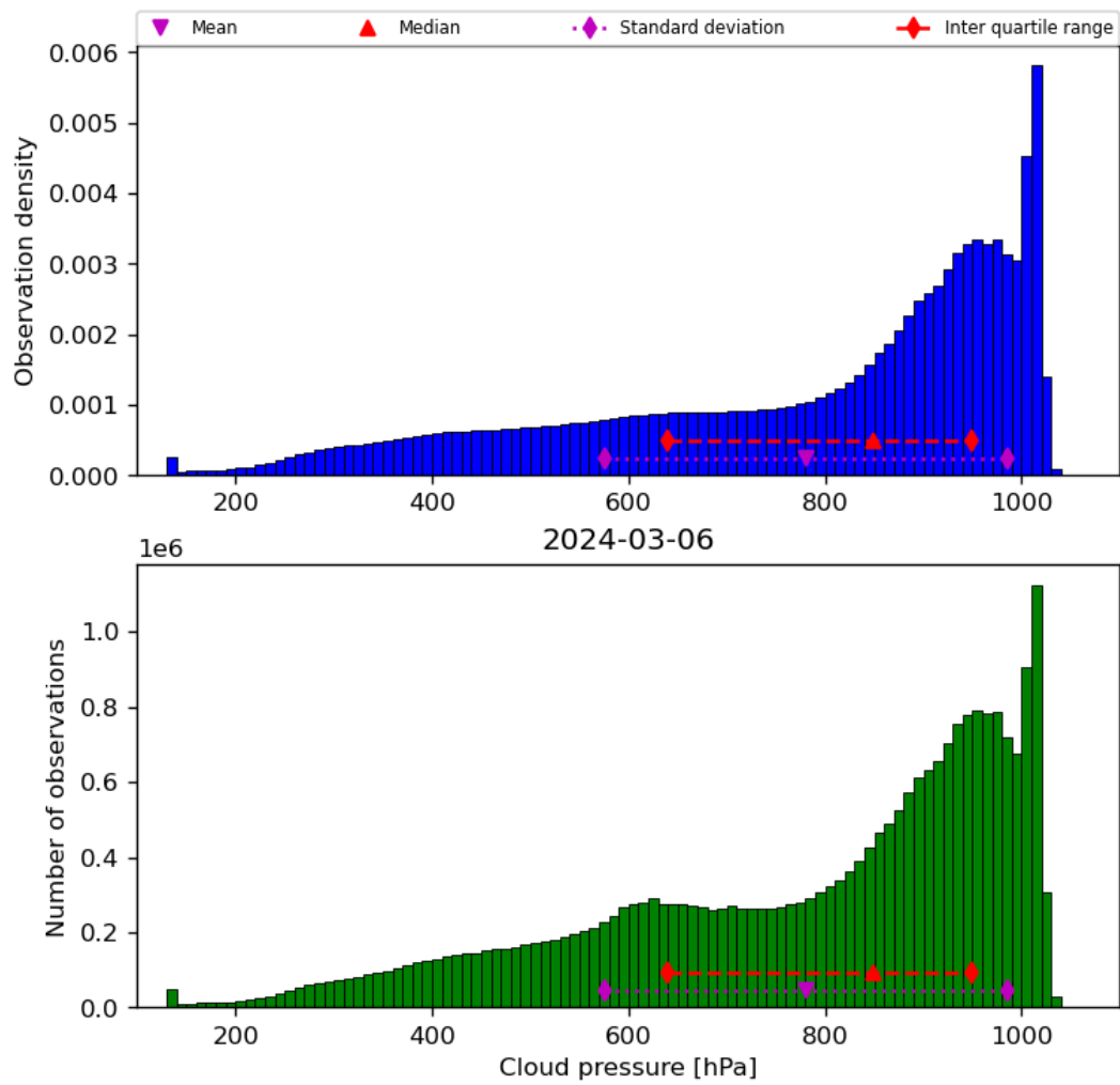
Figure 30: Histogram of “Cloud pressure” for 2024-03-05 to 2024-03-07
