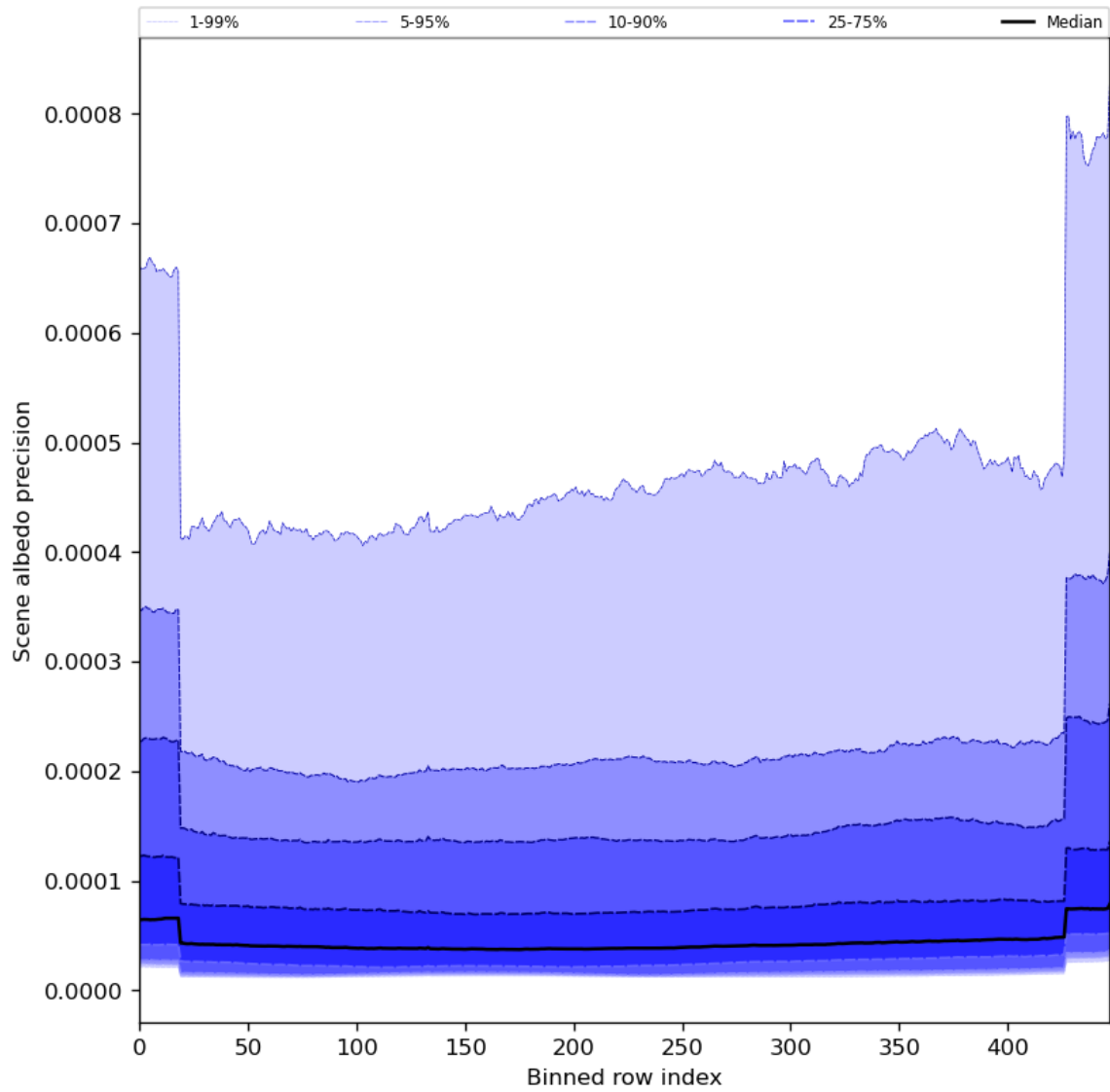
Figure 52: Along track statistics of “Scene albedo precision” for 2024-03-05 to 2024-03-07
