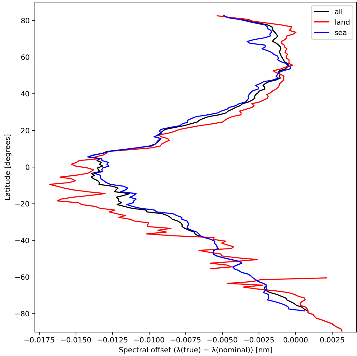
Figure 28: Zonal average of “Spectral offset ( \lambda(\text{true}) - \lambda(\text{nominal}) )” for 2024-03-05 to 2024-03-07.
