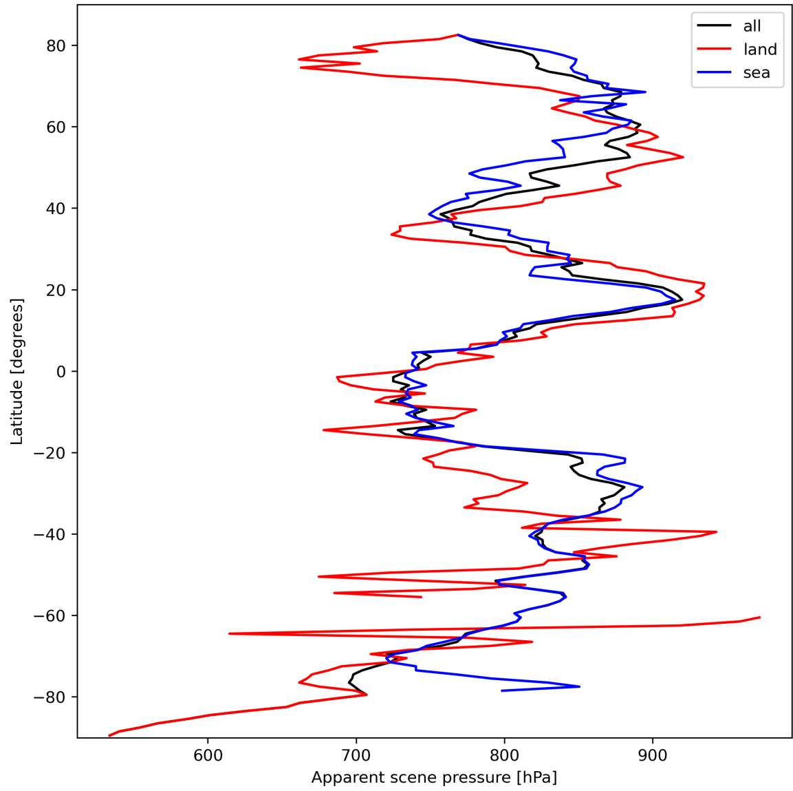
Figure 19: Zonal average of “Apparent scene pressure” for 2024-03-05 to 2024-03-07.
