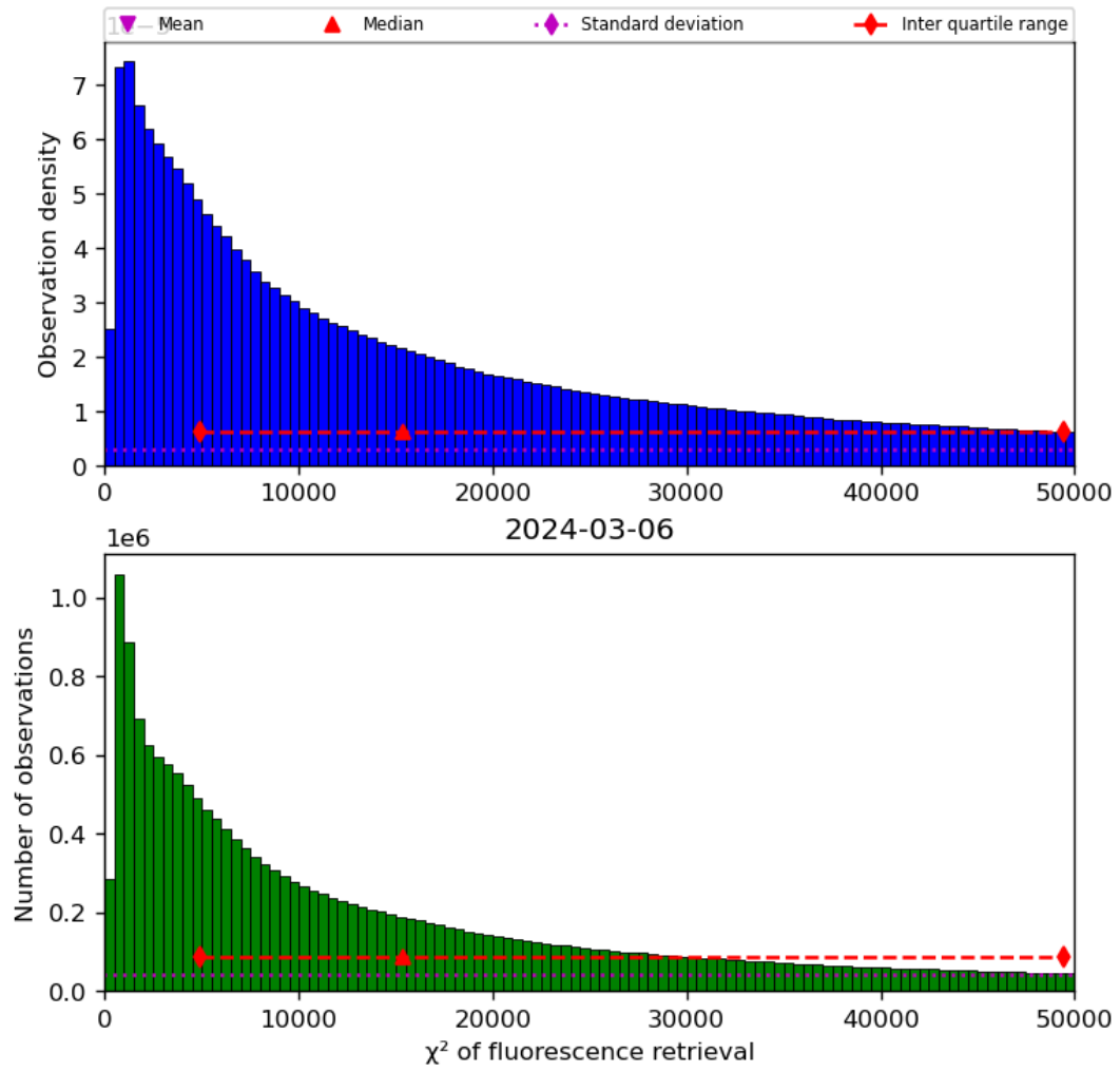
Figure 42: Histogram of “ \chi^2 of fluorescence retrieval” for 2024-03-05 to 2024-03-07
