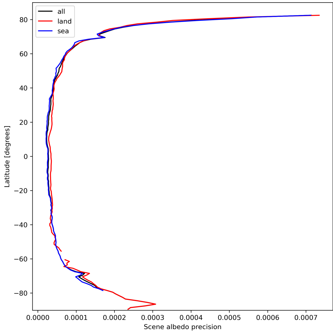
Figure 18: Zonal average of “Scene albedo precision” for 2024-03-05 to 2024-03-07.
