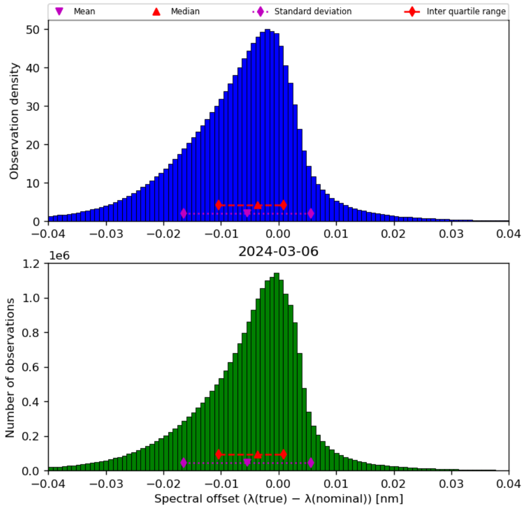
Figure 45: Histogram of “Spectral offset ( \lambda(\text{true}) - \lambda(\text{nominal}) )” for 2024-03-05 to 2024-03-07
