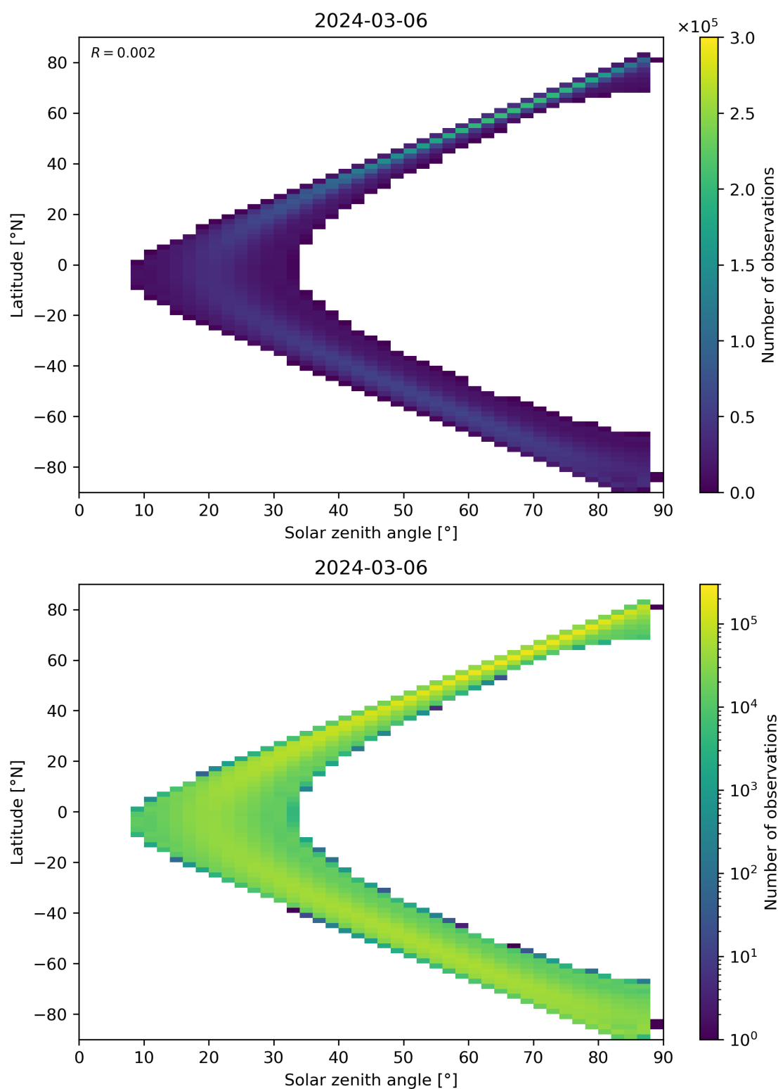
Figure 113: Scatter density plot of “Solar zenith angle” against “Latitude” for 2024-03-05 to 2024-03-07.
