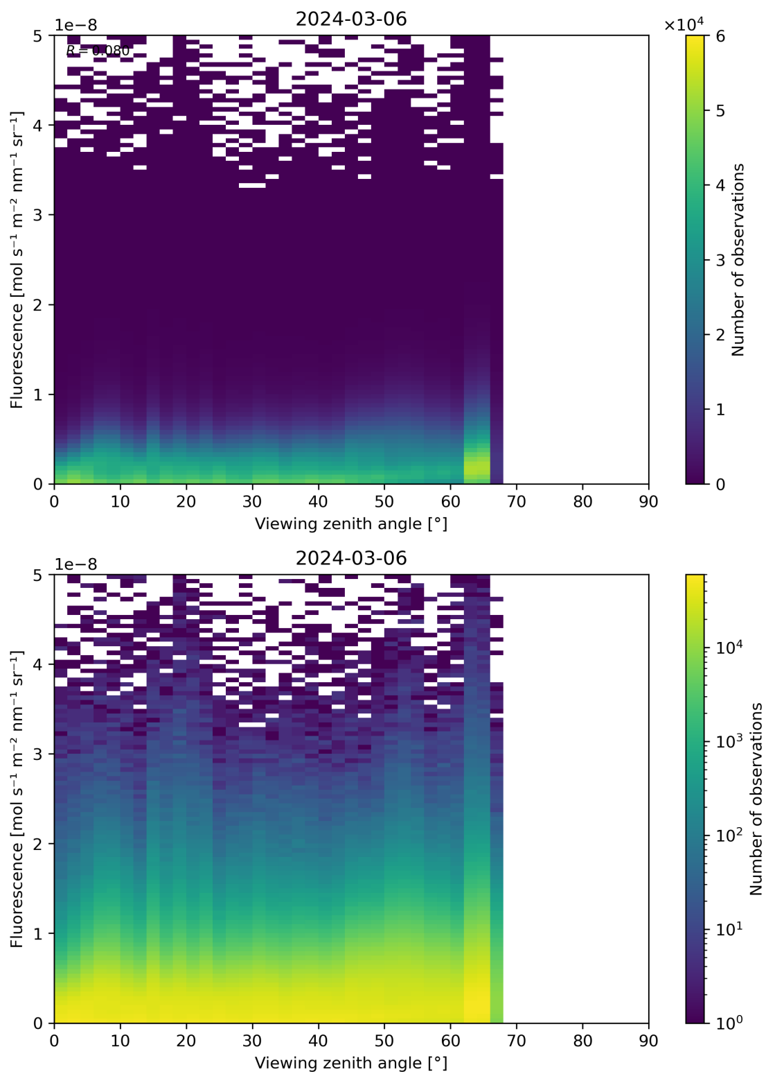
Figure 122: Scatter density plot of “Viewing zenith angle” against “Fluorescence” for 2024-03-05 to 2024-03-07.
