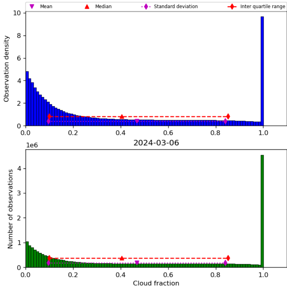
Figure 32: Histogram of “Cloud fraction” for 2024-03-05 to 2024-03-07
