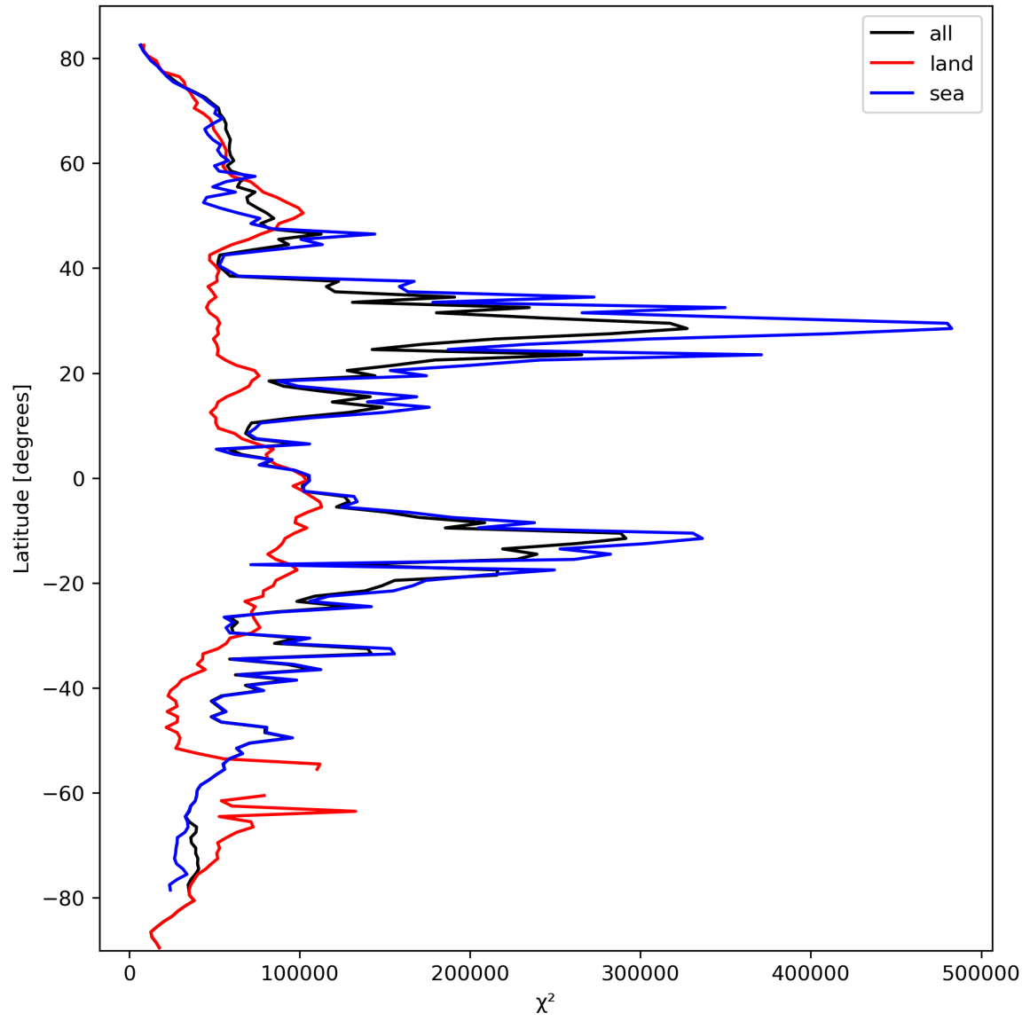
Figure 21: Zonal average of “ \chi^2 ” for 2024-03-05 to 2024-03-07.
