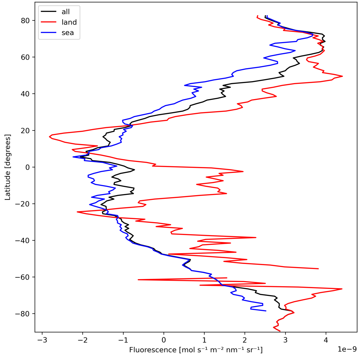
Figure 23: Zonal average of “Fluorescence” for 2024-03-05 to 2024-03-07.
