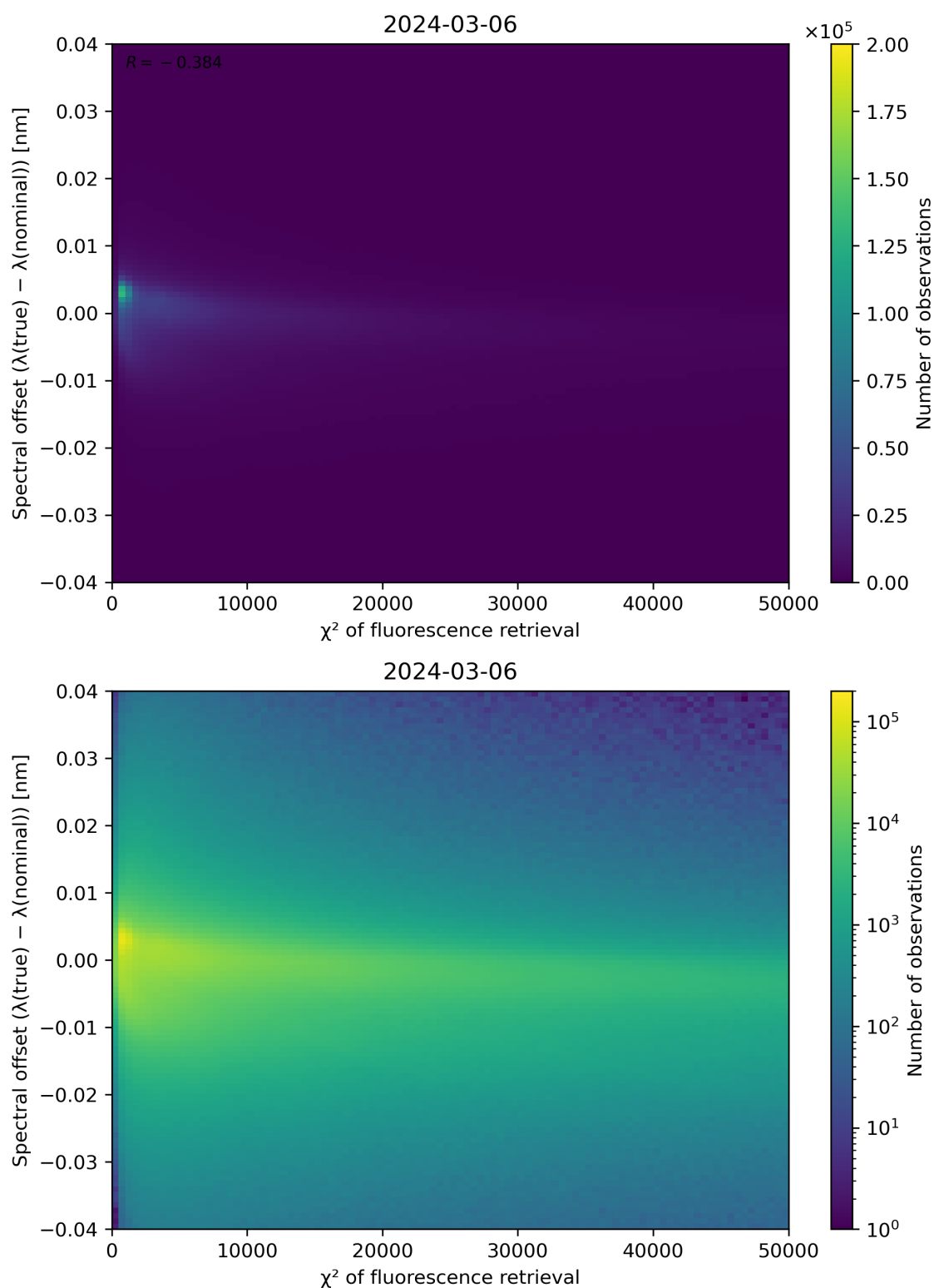
Figure 69: Scatter density plot of " \chi^2 of fluorescence retrieval" against "Spectral offset ( \lambda(\text{true}) - \lambda(\text{nominal}) )" for 2024-03-05 to 2024-03-07.
