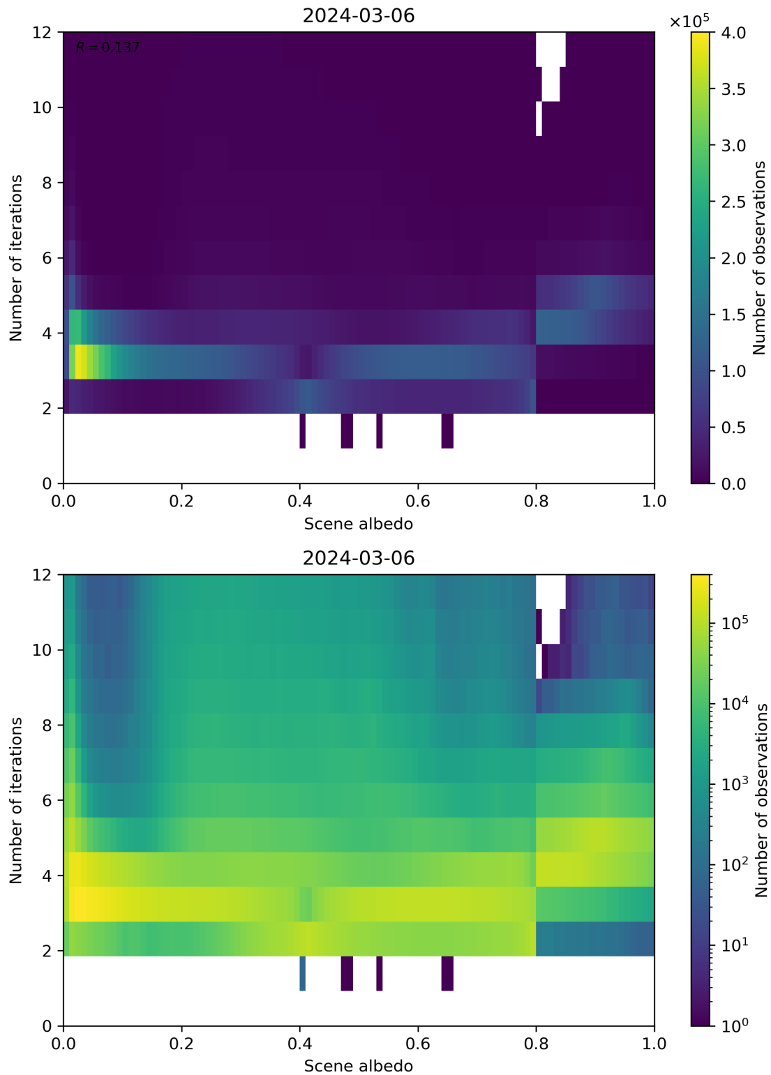
Figure 105: Scatter density plot of “Scene albedo” against “Number of iterations” for 2024-03-05 to 2024-03-07.
