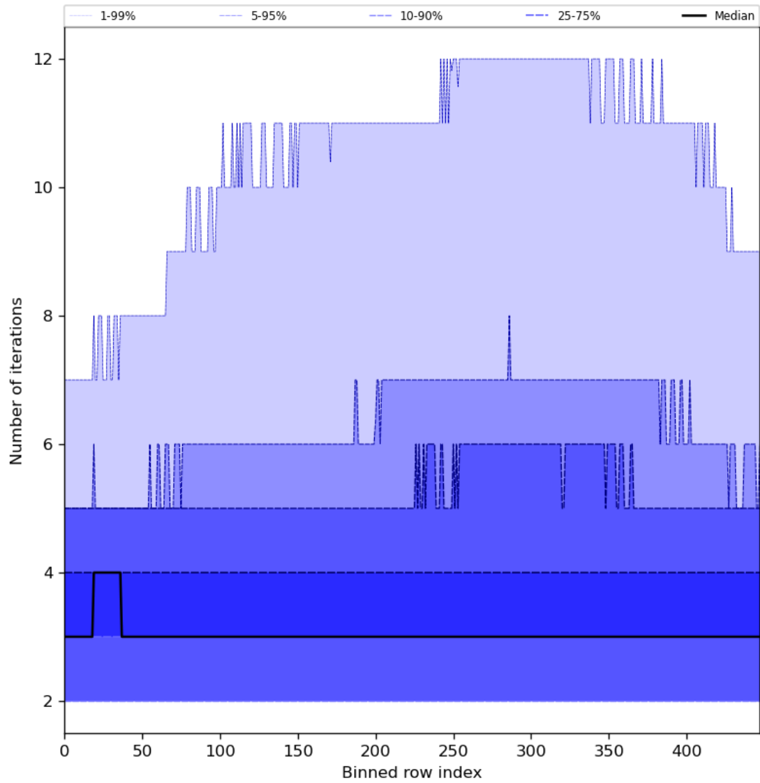
Figure 56: Along track statistics of “Number of iterations” for 2024-03-05 to 2024-03-07
