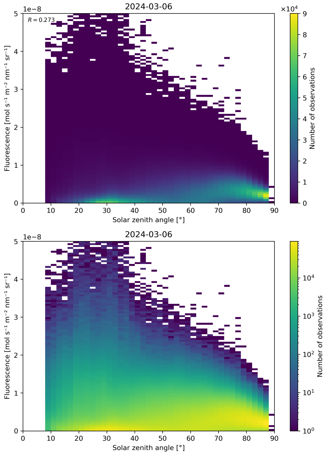
Figure 112: Scatter density plot of “Solar zenith angle” against “Fluorescence” for 2024-03-05 to 2024-03-07.
