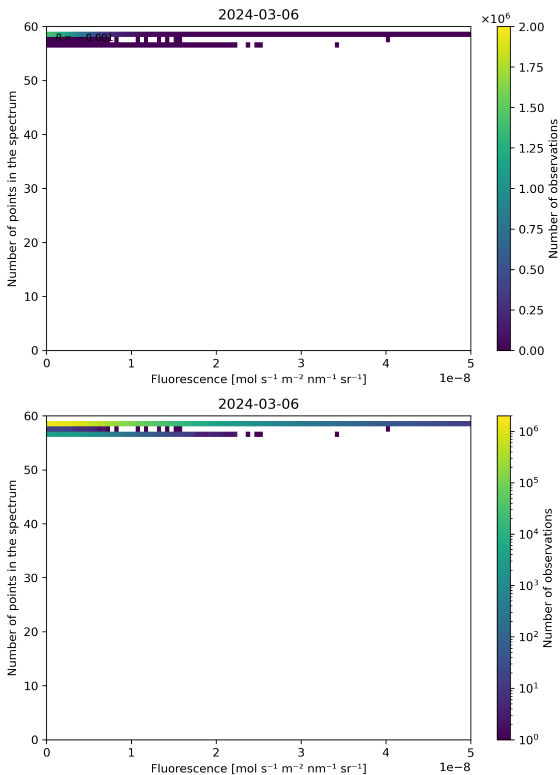
Figure 86: Scatter density plot of “Fluorescence” against “Number of points in the spectrum” for 2024-03-05 to 2024-03-07.
