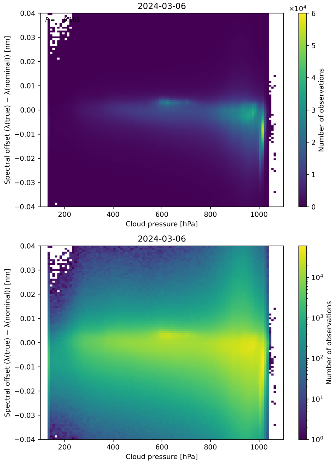
Figure 84: Scatter density plot of “Cloud pressure” against “Spectral offset ( \lambda(\text{true}) - \lambda(\text{nominal}) )” for 2024-03-05 to 2024-03-07.
