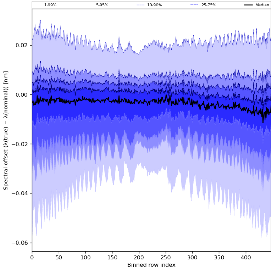
Figure 62: Along track statistics of “Spectral offset ( \lambda(\text{true}) - \lambda(\text{nominal}) )” for 2024-03-05 to 2024-03-07
