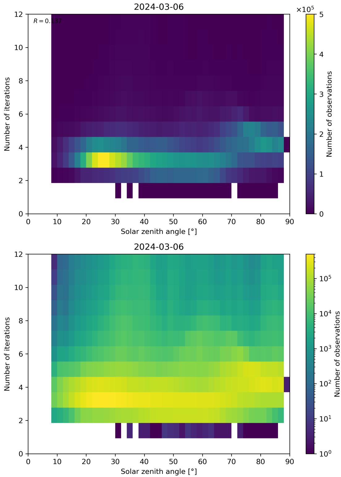
Figure 114: Scatter density plot of “Solar zenith angle” against “Number of iterations” for 2024-03-05 to 2024-03-07.
