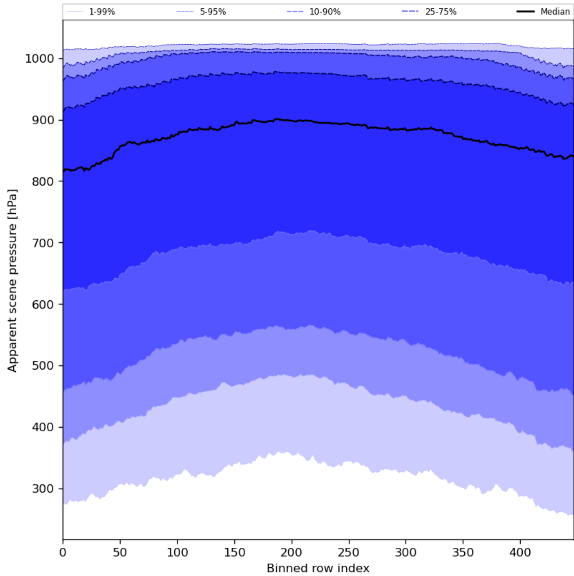
Figure 53: Along track statistics of “Apparent scene pressure” for 2024-03-05 to 2024-03-07
