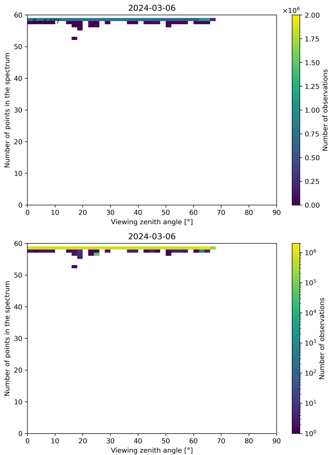
Figure 125: Scatter density plot of “Viewing zenith angle” against “Number of points in the spectrum” for 2024-03-05 to 2024-03-07.
