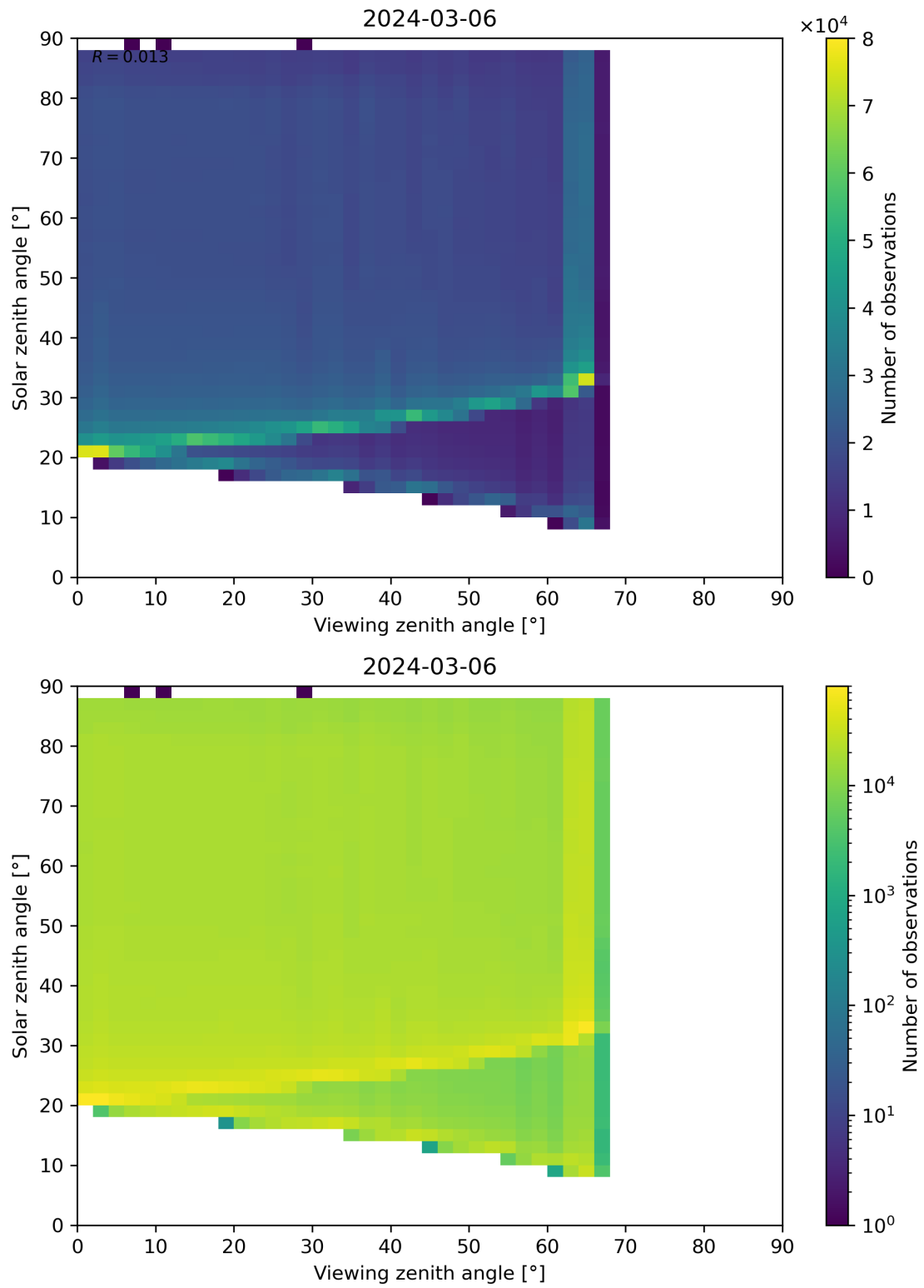
Figure 127: Scatter density plot of “Viewing zenith angle” against “Solar zenith angle” for 2024-03-05 to 2024-03-07.
