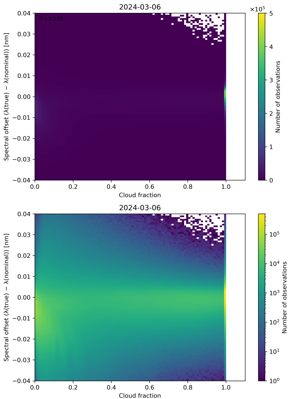
Figure 76: Scatter density plot of “Cloud fraction” against “Spectral offset ( \lambda(\text{true}) - \lambda(\text{nominal}) )” for 2024-03-05 to 2024-03-07.
