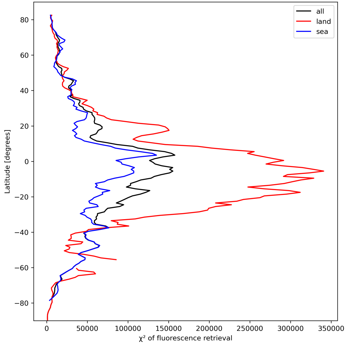
Figure 25: Zonal average of “ \chi^2 of fluorescence retrieval” for 2024-03-05 to 2024-03-07.
