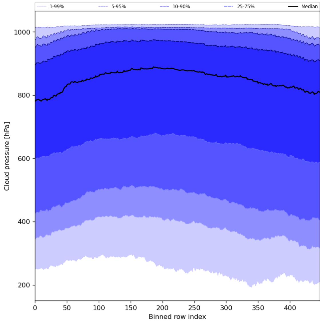
Figure 47: Along track statistics of “Cloud pressure” for 2024-03-05 to 2024-03-07
