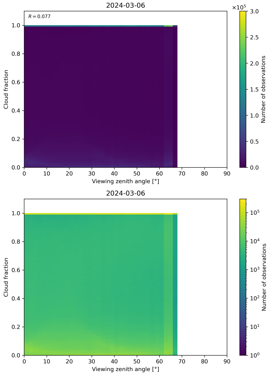
Figure 120: Scatter density plot of “Viewing zenith angle” against “Cloud fraction” for 2024-03-05 to 2024-03-07.
