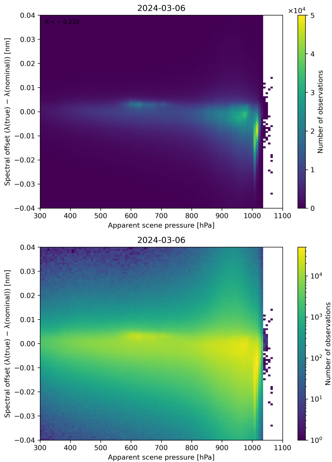
Figure 67: Scatter density plot of “Apparent scene pressure” against “Spectral offset ( \lambda(\text{true}) - \lambda(\text{nominal}) )” for 2024-03-05 to 2024-03-07.
