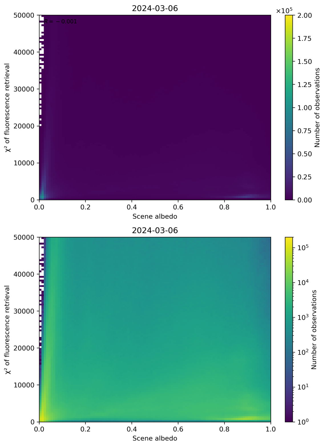
Figure 103: Scatter density plot of “Scene albedo” against “ \chi^2 of fluorescence retrieval” for 2024-03-05 to 2024-03-07.
