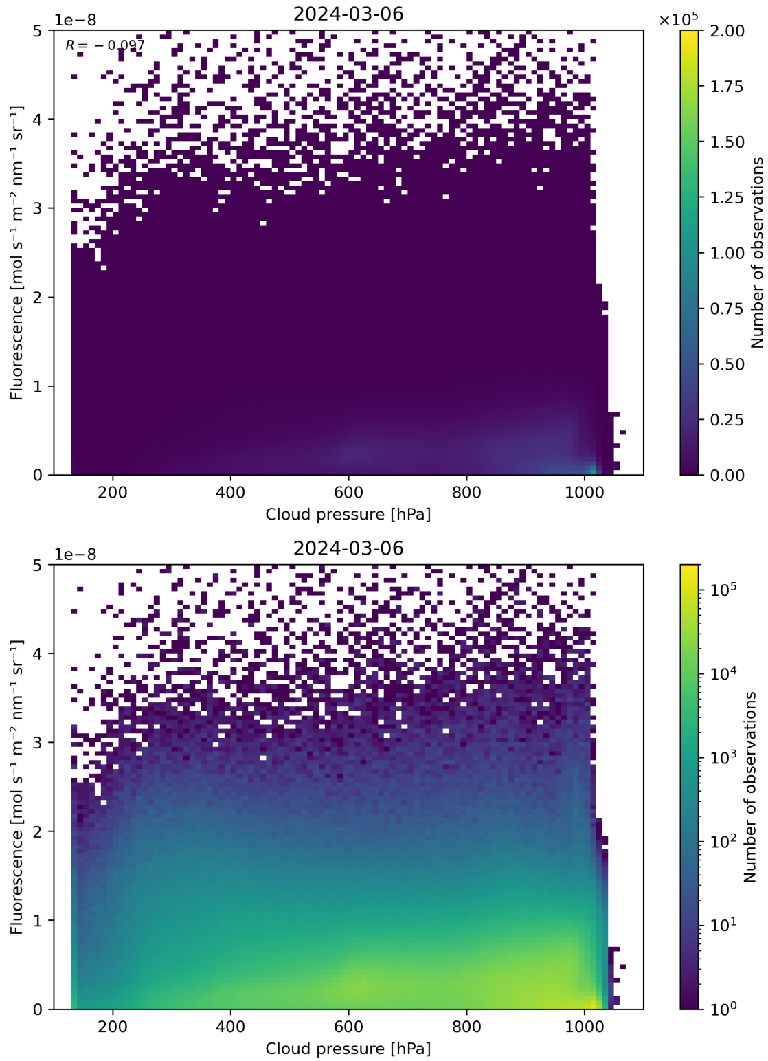
Figure 80: Scatter density plot of “Cloud pressure” against “Fluorescence” for 2024-03-05 to 2024-03-07.
