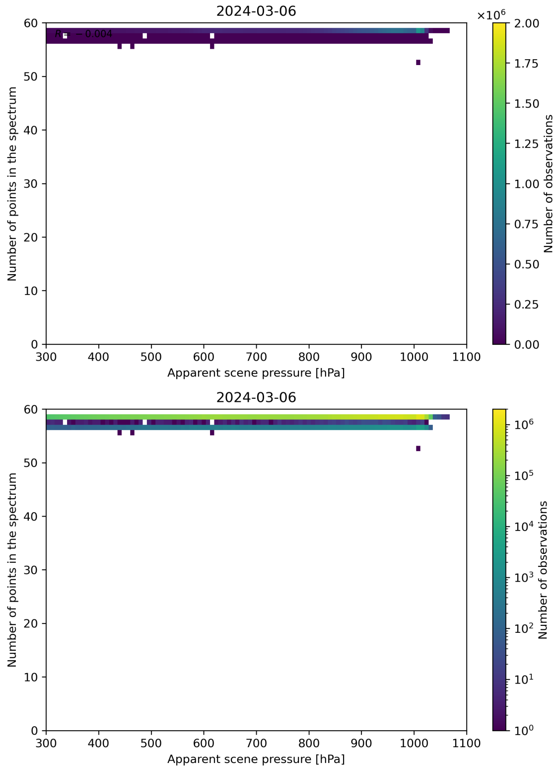
Figure 66: Scatter density plot of “Apparent scene pressure” against “Number of points in the spectrum” for 2024-03-05 to 2024-03-07.
