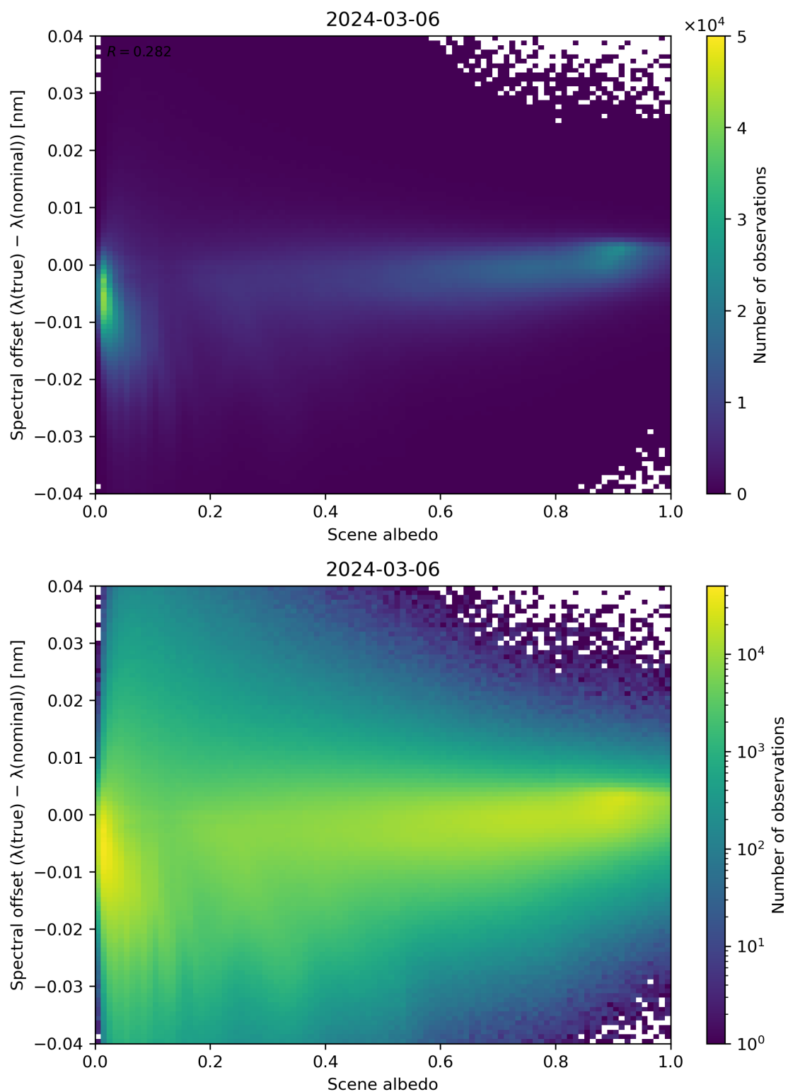
Figure 107: Scatter density plot of “Scene albedo” against “Spectral offset ( \lambda(\text{true}) - \lambda(\text{nominal}) )” for 2024-03-05 to 2024-03-07.
