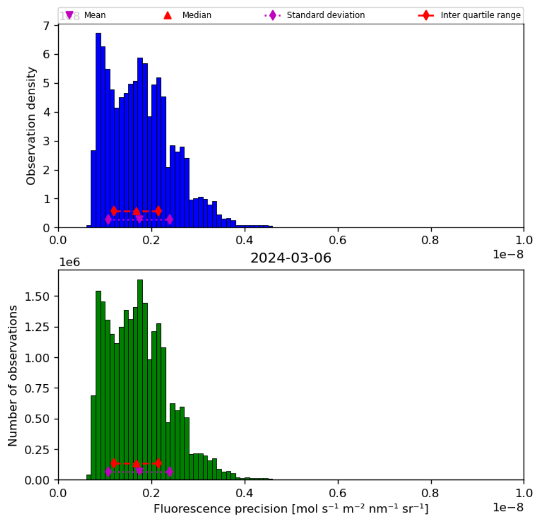
Figure 41: Histogram of “Fluorescence precision” for 2024-03-05 to 2024-03-07
