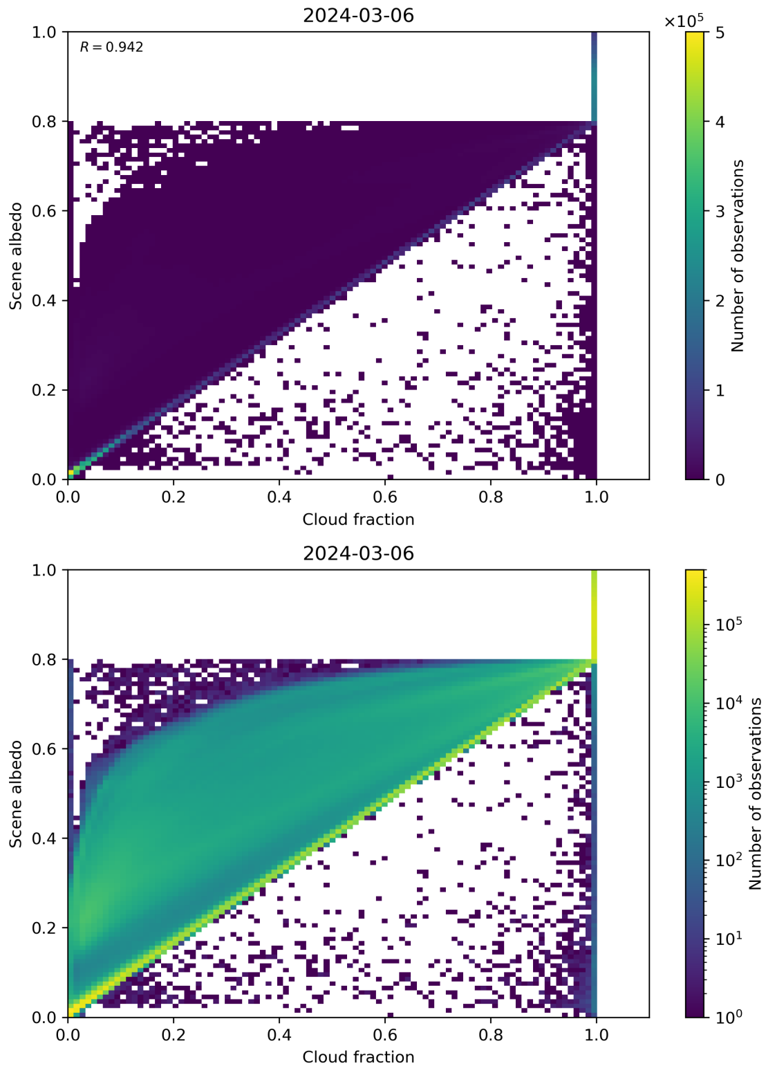
Figure 75: Scatter density plot of “Cloud fraction” against “Scene albedo” for 2024-03-05 to 2024-03-07.
