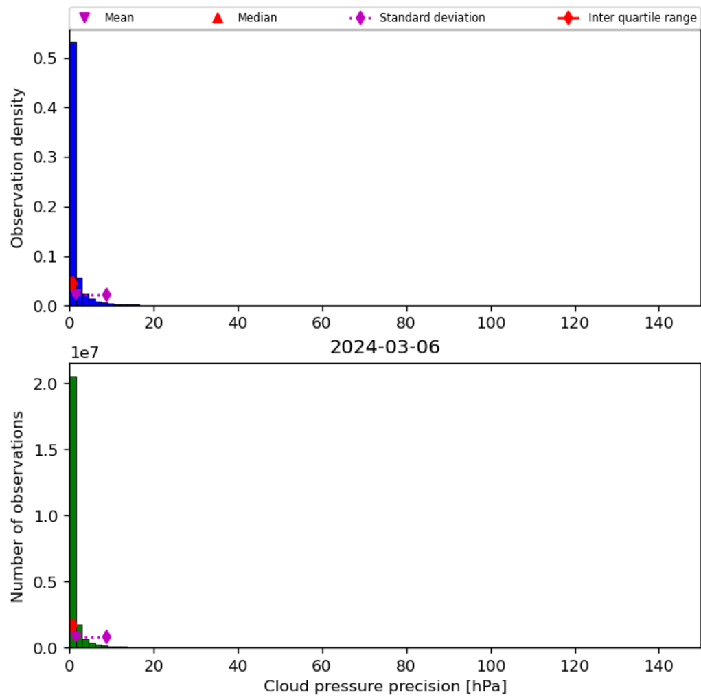
Figure 31: Histogram of “Cloud pressure precision” for 2024-03-05 to 2024-03-07
