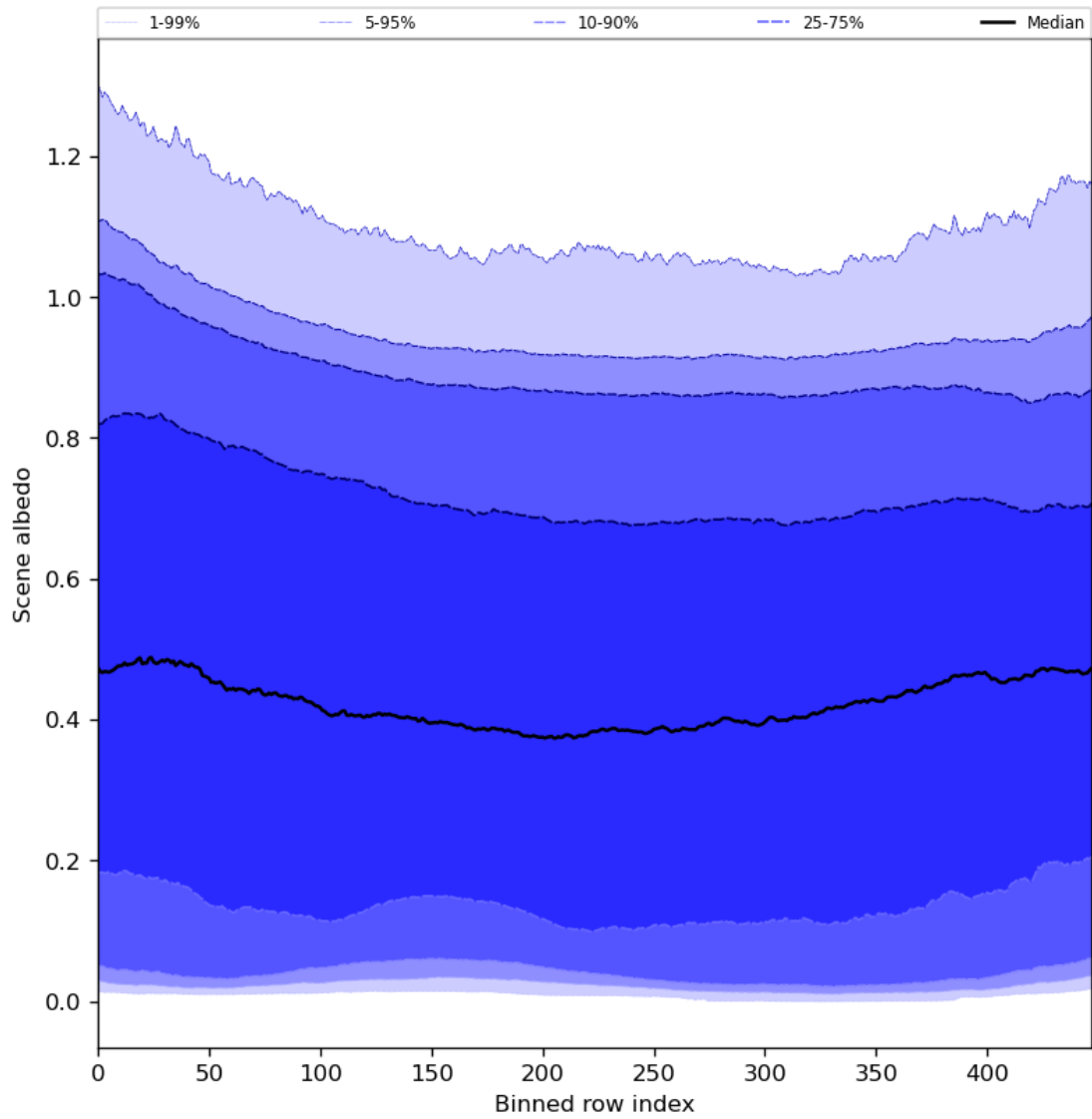
Figure 51: Along track statistics of “Scene albedo” for 2024-03-05 to 2024-03-07
