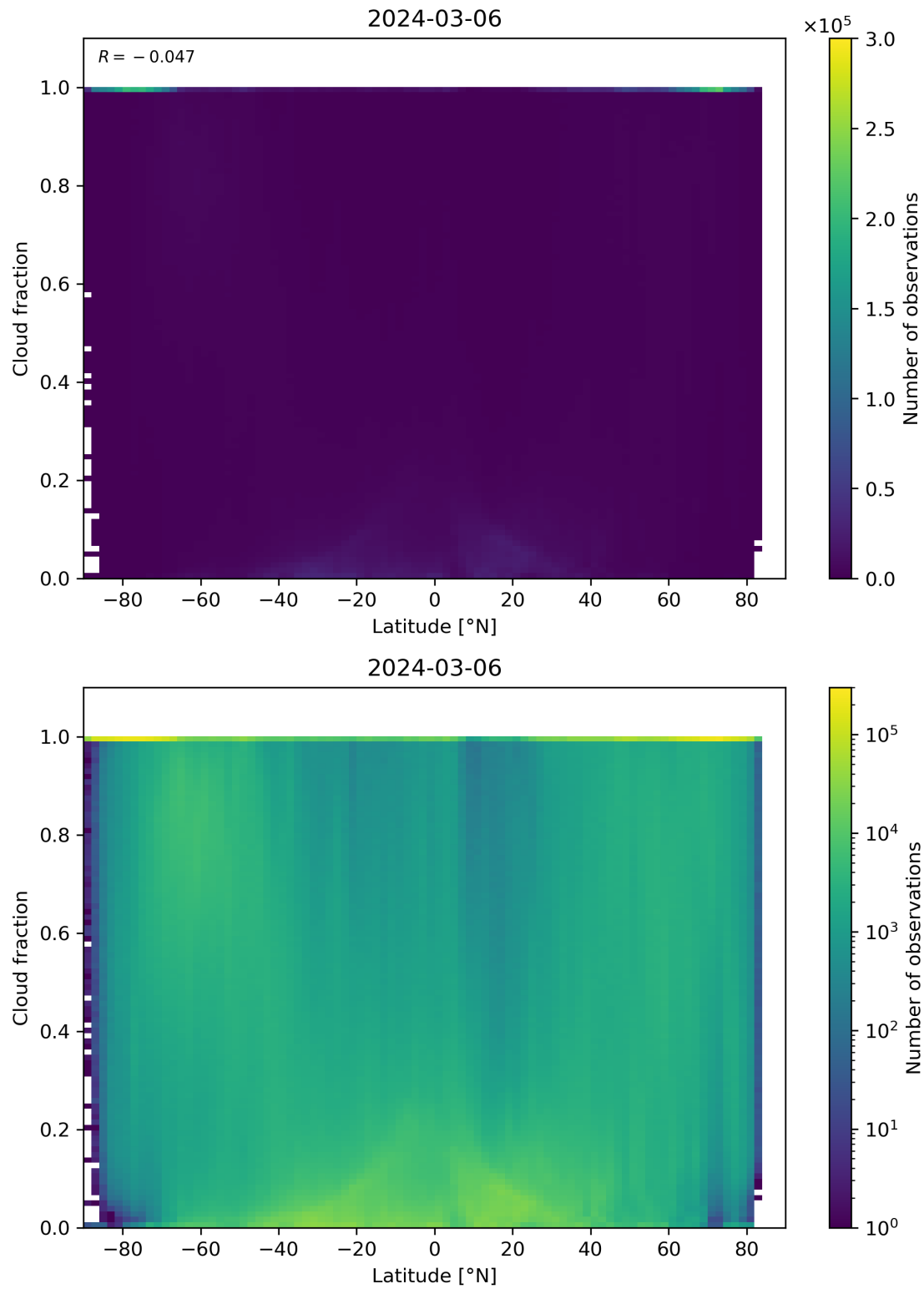
Figure 90: Scatter density plot of “Latitude” against “Cloud fraction” for 2024-03-05 to 2024-03-07.
