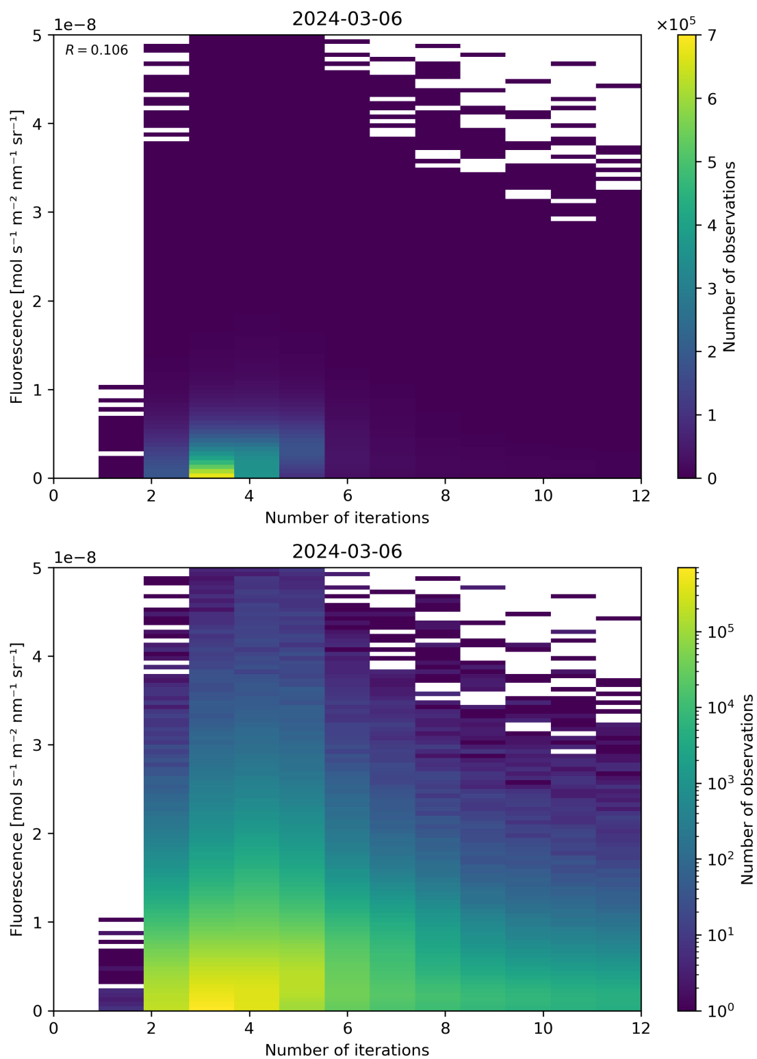
Figure 98: Scatter density plot of “Number of iterations” against “Fluorescence” for 2024-03-05 to 2024-03-07.
