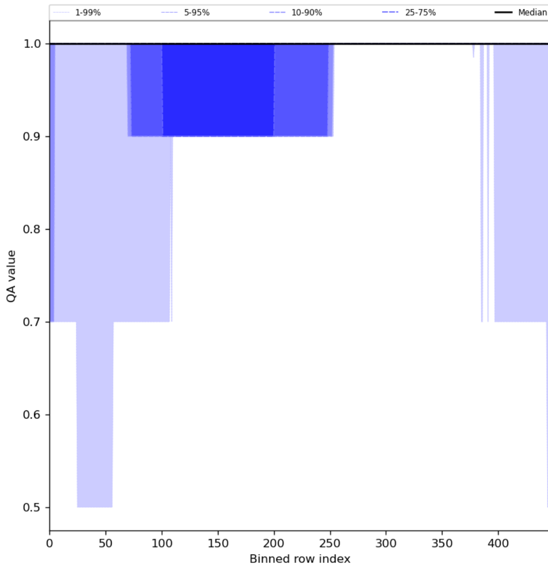
Figure 46: Along track statistics of “QA value” for 2024-03-05 to 2024-03-07
