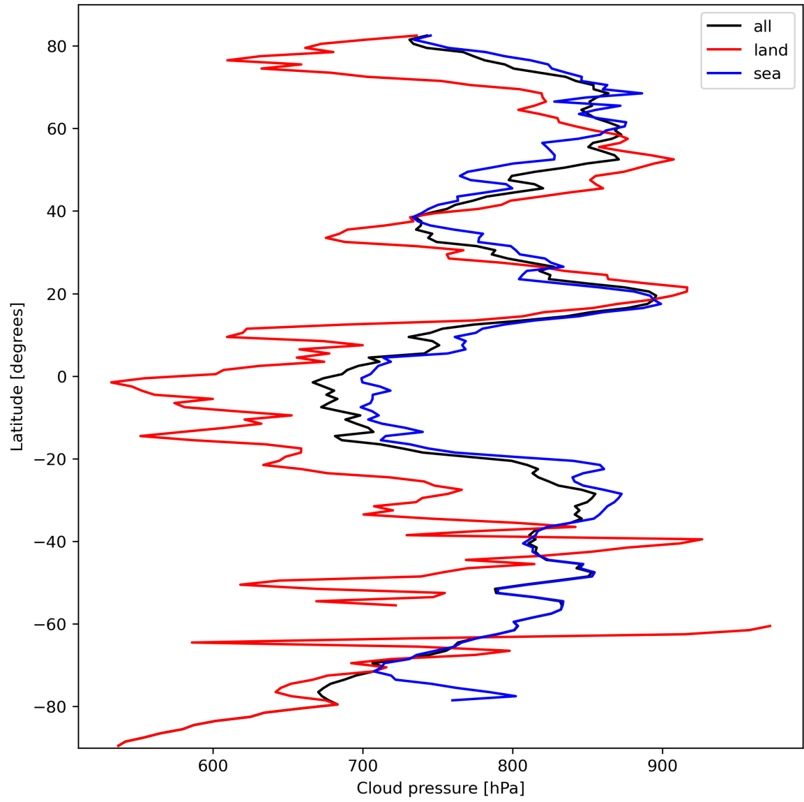
Figure 13: Zonal average of “Cloud pressure” for 2024-03-05 to 2024-03-07.
