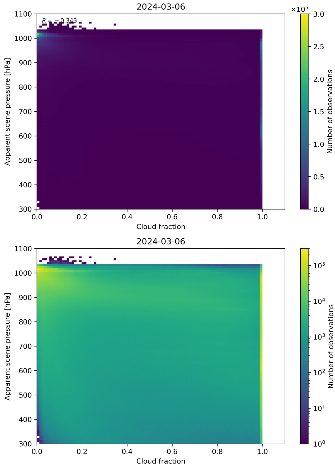
Figure 70: Scatter density plot of “Cloud fraction” against “Apparent scene pressure” for 2024-03-05 to 2024-03-07.
