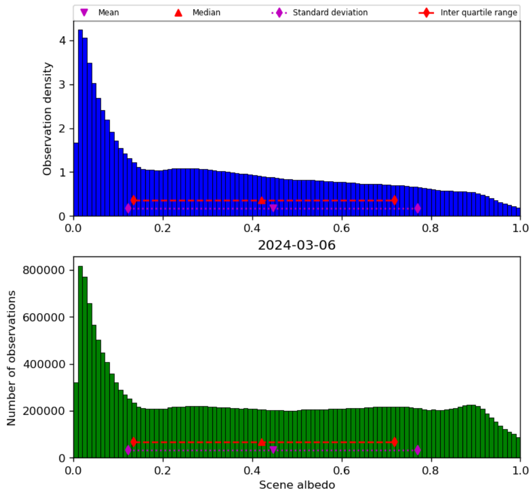
Figure 34: Histogram of “Scene albedo” for 2024-03-05 to 2024-03-07
