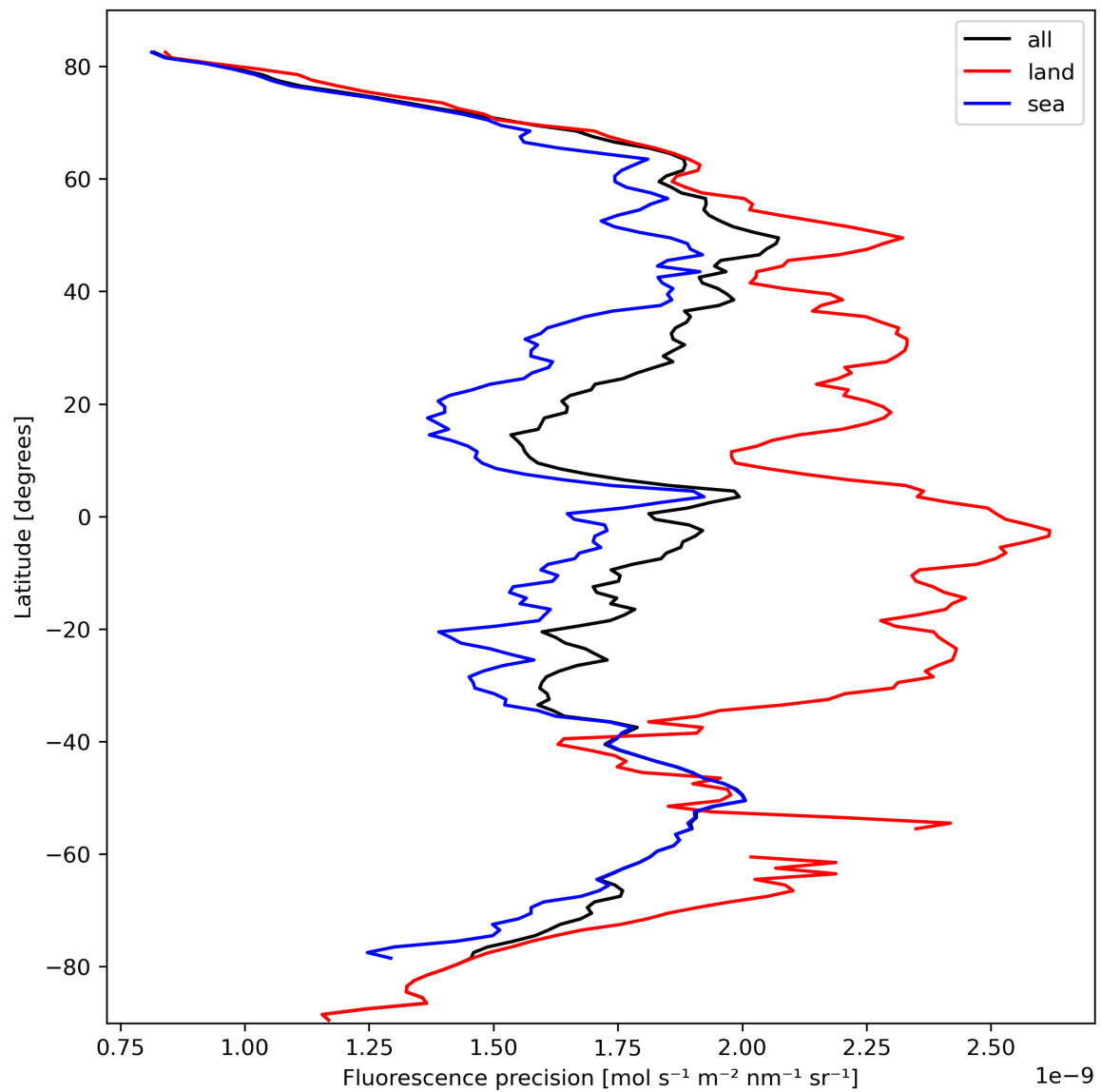
Figure 24: Zonal average of “Fluorescence precision” for 2024-03-05 to 2024-03-07.
