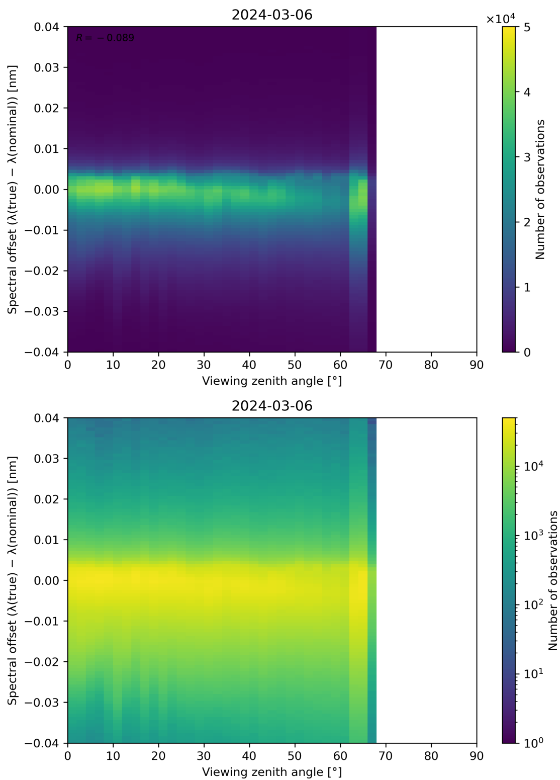
Figure 128: Scatter density plot of “Viewing zenith angle” against “Spectral offset ( \lambda(\text{true}) - \lambda(\text{nominal}) )” for 2024-03-05 to 2024-03-07.
