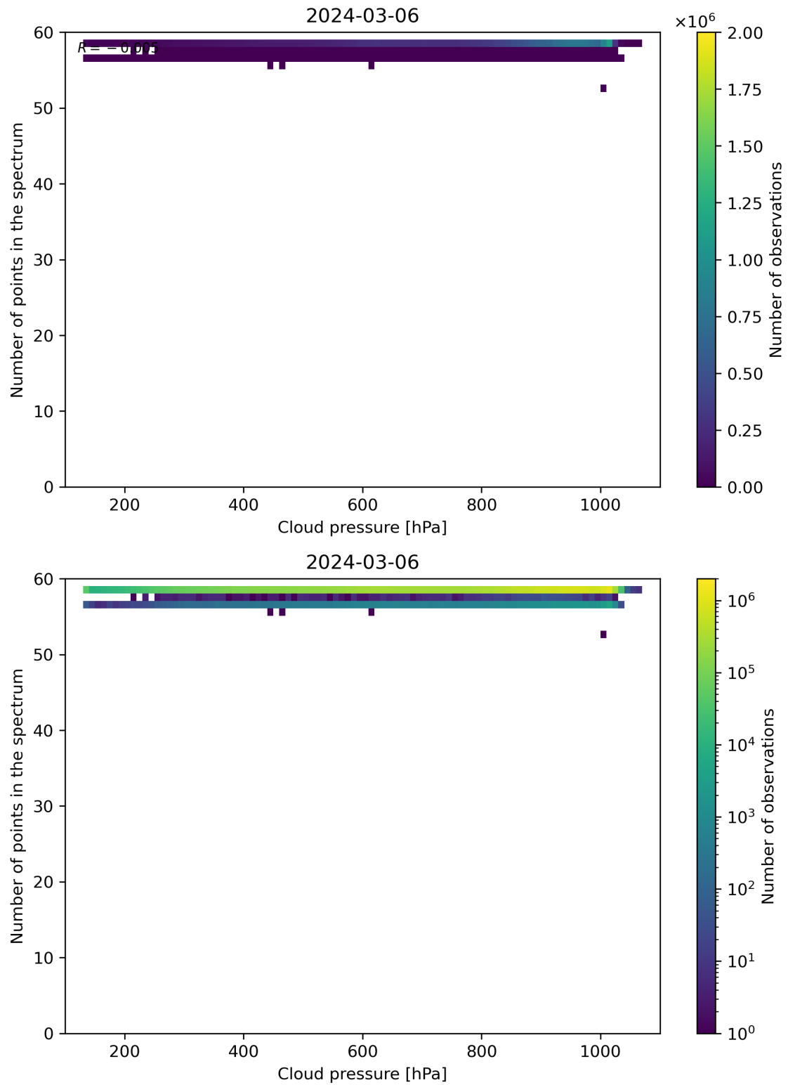
Figure 82: Scatter density plot of “Cloud pressure” against “Number of points in the spectrum” for 2024-03-05 to 2024-03-07.
