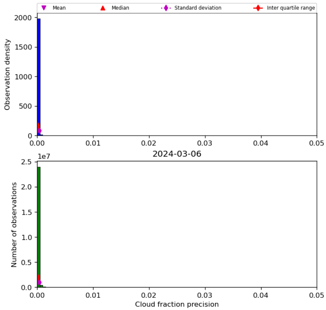
Figure 33: Histogram of “Cloud fraction precision” for 2024-03-05 to 2024-03-07
