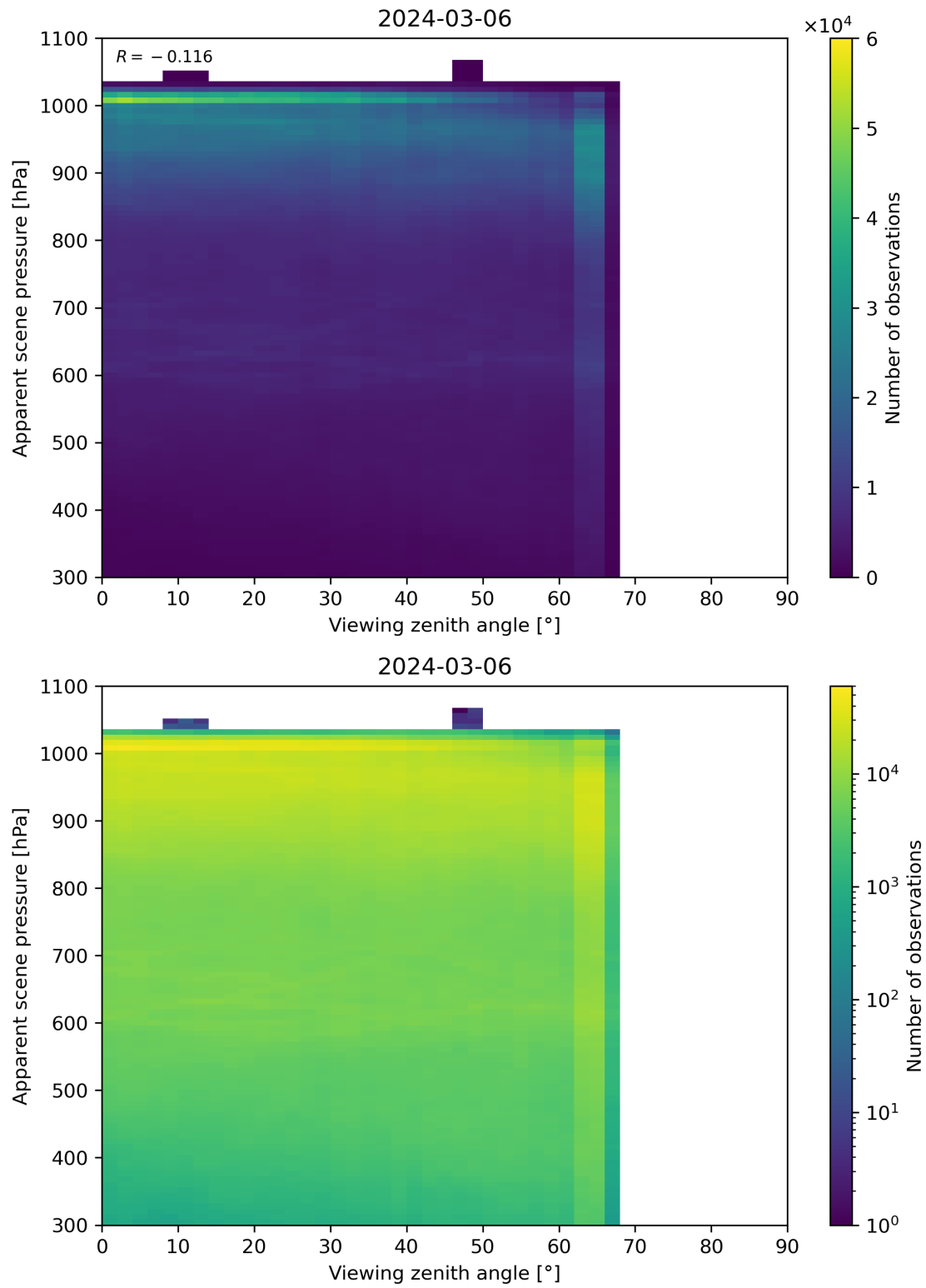
Figure 118: Scatter density plot of “Viewing zenith angle” against “Apparent scene pressure” for 2024-03-05 to 2024-03-07.
