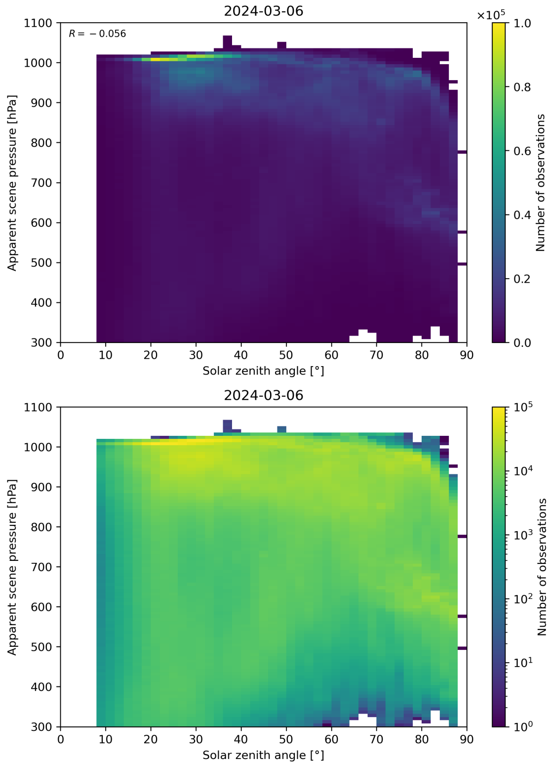
Figure 108: Scatter density plot of “Solar zenith angle” against “Apparent scene pressure” for 2024-03-05 to 2024-03-07.
