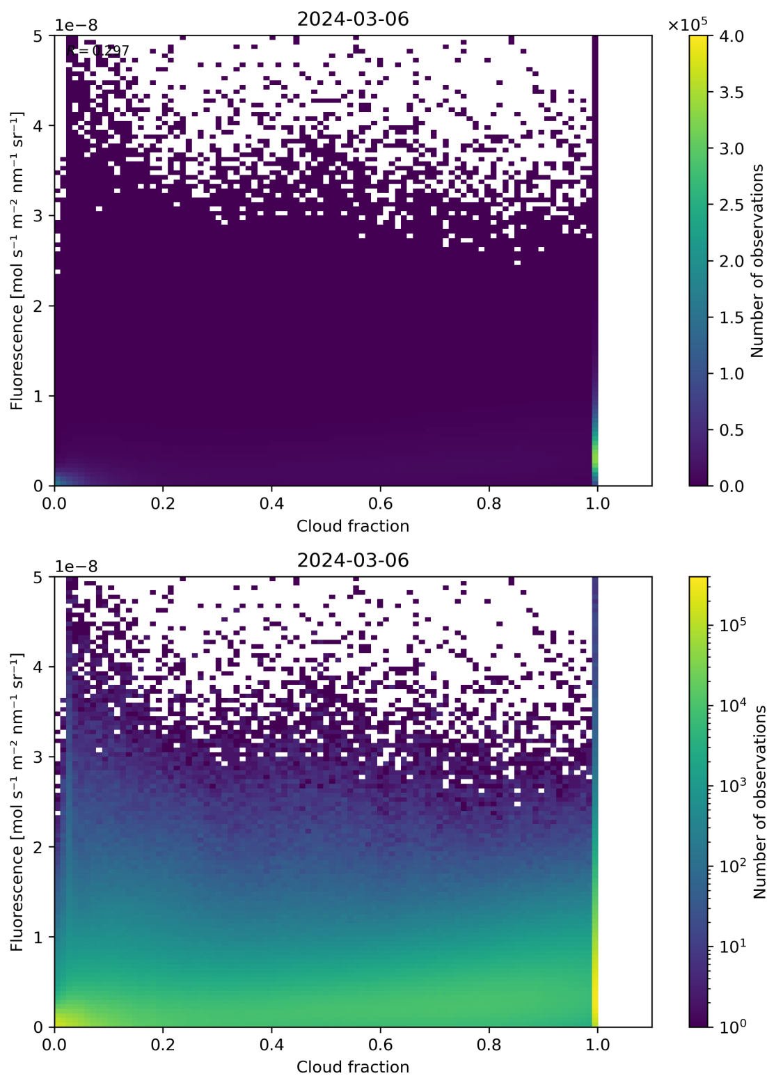
Figure 72: Scatter density plot of “Cloud fraction” against “Fluorescence” for 2024-03-05 to 2024-03-07.
