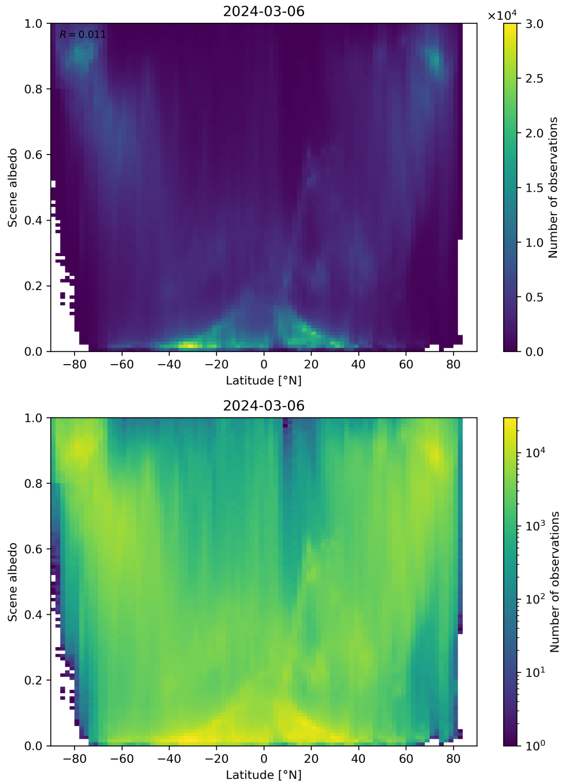
Figure 95: Scatter density plot of “Latitude” against “Scene albedo” for 2024-03-05 to 2024-03-07.
