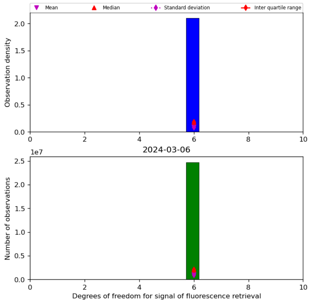
Figure 43: Histogram of “Degrees of freedom for signal of fluorescence retrieval” for 2024-03-05 to 2024-03-07
