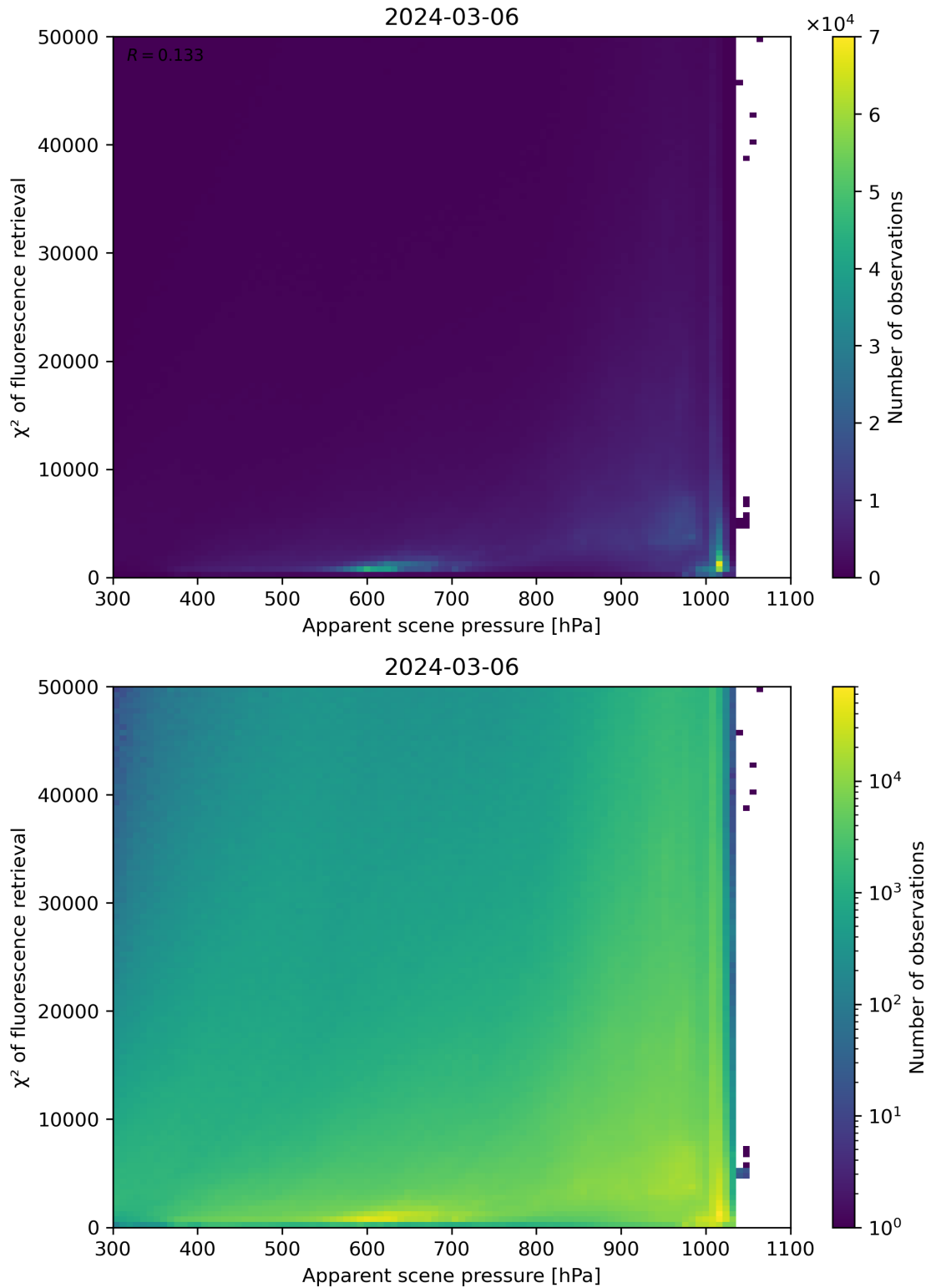
Figure 63: Scatter density plot of “Apparent scene pressure” against “ \chi^2 of fluorescence retrieval” for 2024-03-05 to 2024-03-07.
