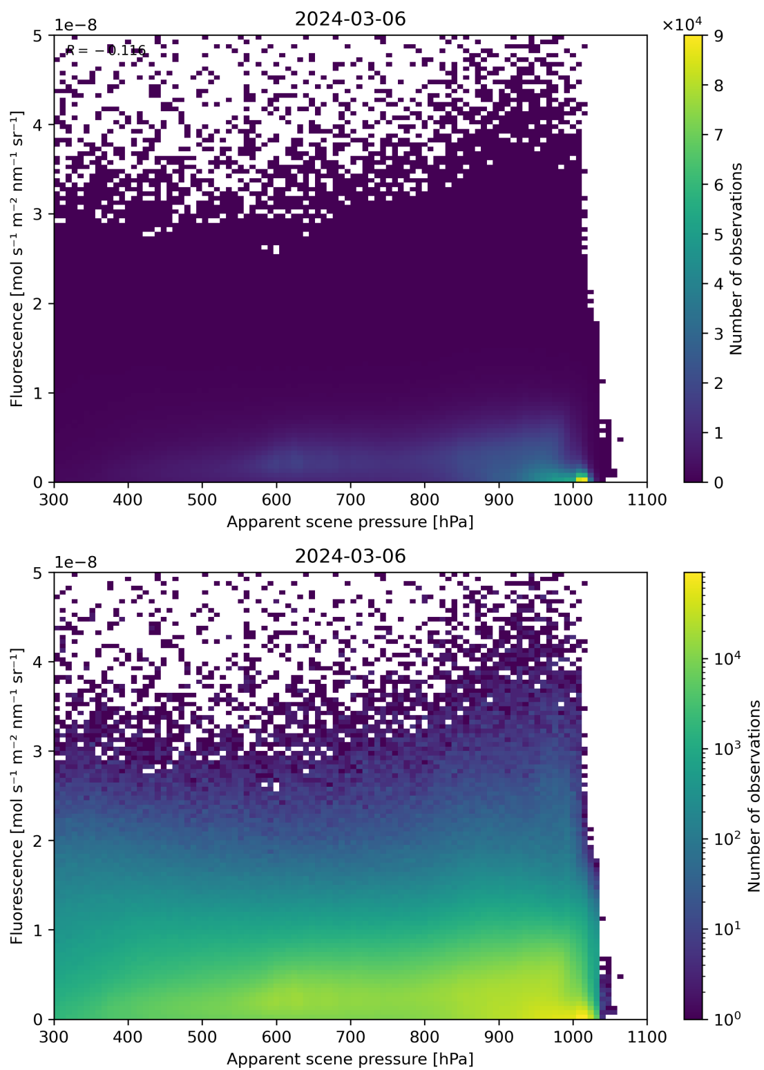
Figure 64: Scatter density plot of “Apparent scene pressure” against “Fluorescence” for 2024-03-05 to 2024-03-07.
