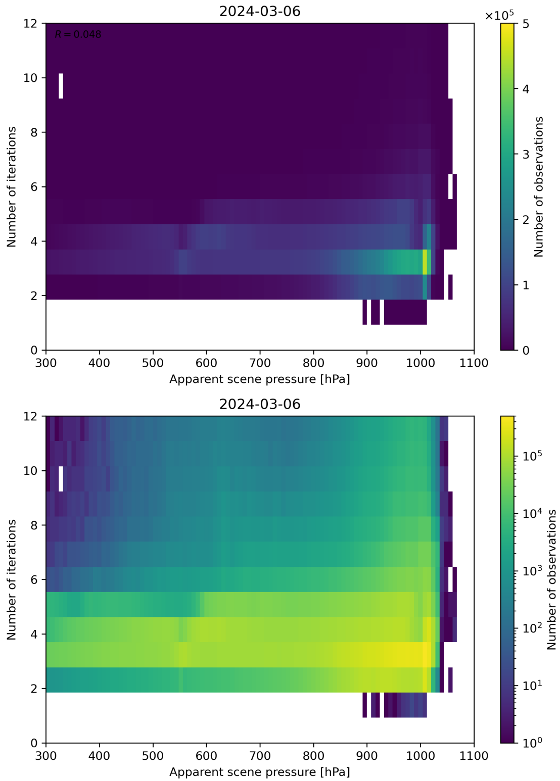
Figure 65: Scatter density plot of “Apparent scene pressure” against “Number of iterations” for 2024-03-05 to 2024-03-07.
