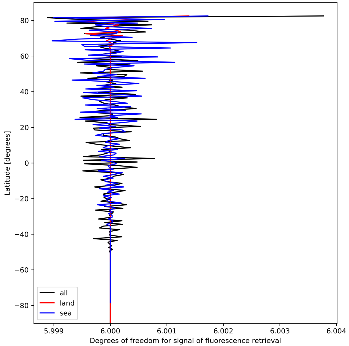
Figure 26: Zonal average of “Degrees of freedom for signal of fluorescence retrieval” for 2024-03-05 to 2024-03-07.
