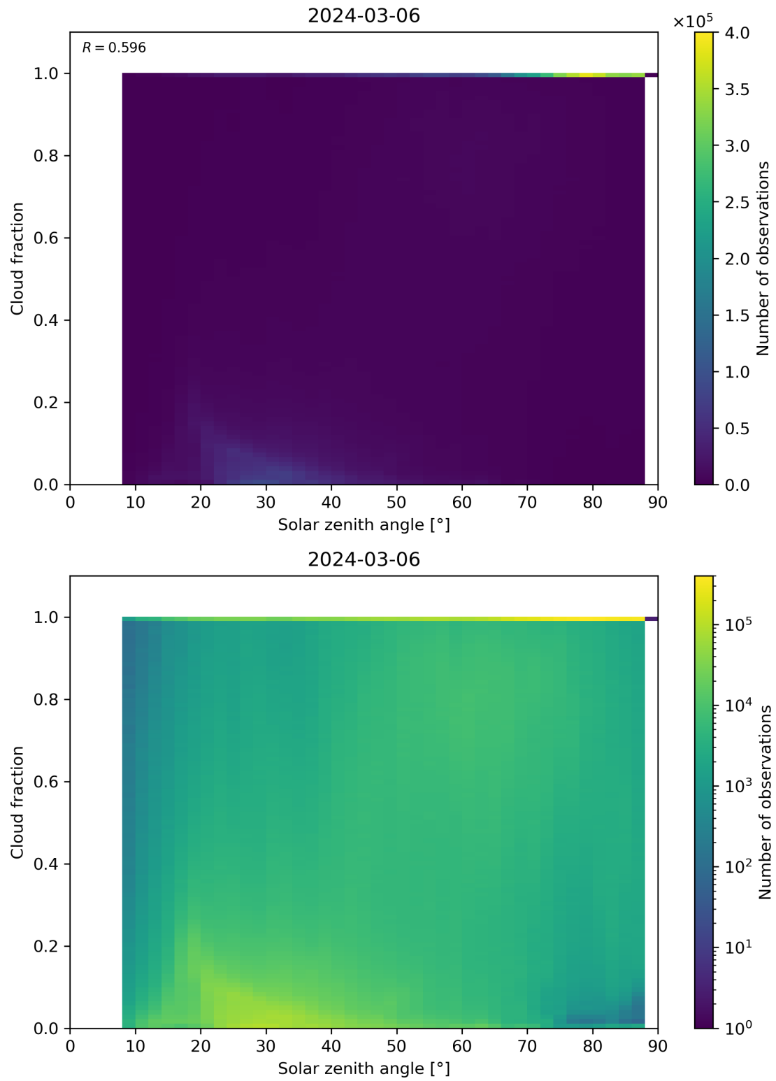
Figure 110: Scatter density plot of “Solar zenith angle” against “Cloud fraction” for 2024-03-05 to 2024-03-07.
