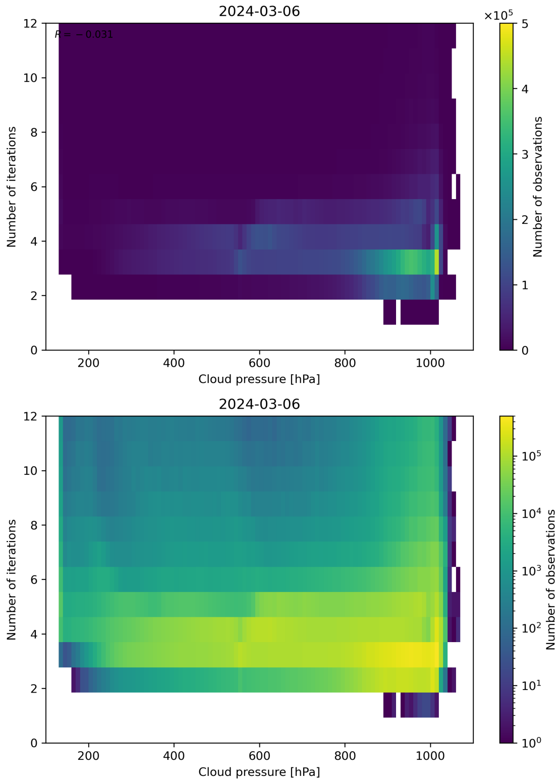
Figure 81: Scatter density plot of “Cloud pressure” against “Number of iterations” for 2024-03-05 to 2024-03-07.
