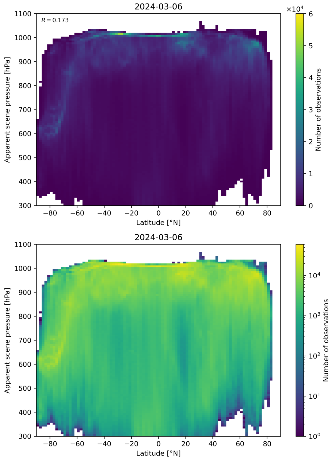
Figure 88: Scatter density plot of “Latitude” against “Apparent scene pressure” for 2024-03-05 to 2024-03-07.
