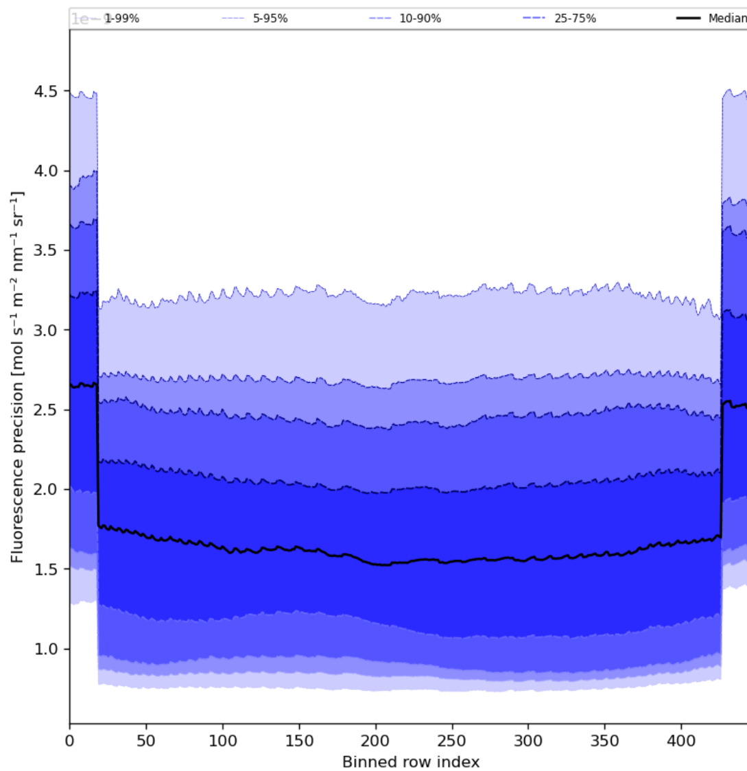
Figure 58: Along track statistics of “Fluorescence precision” for 2024-03-05 to 2024-03-07
