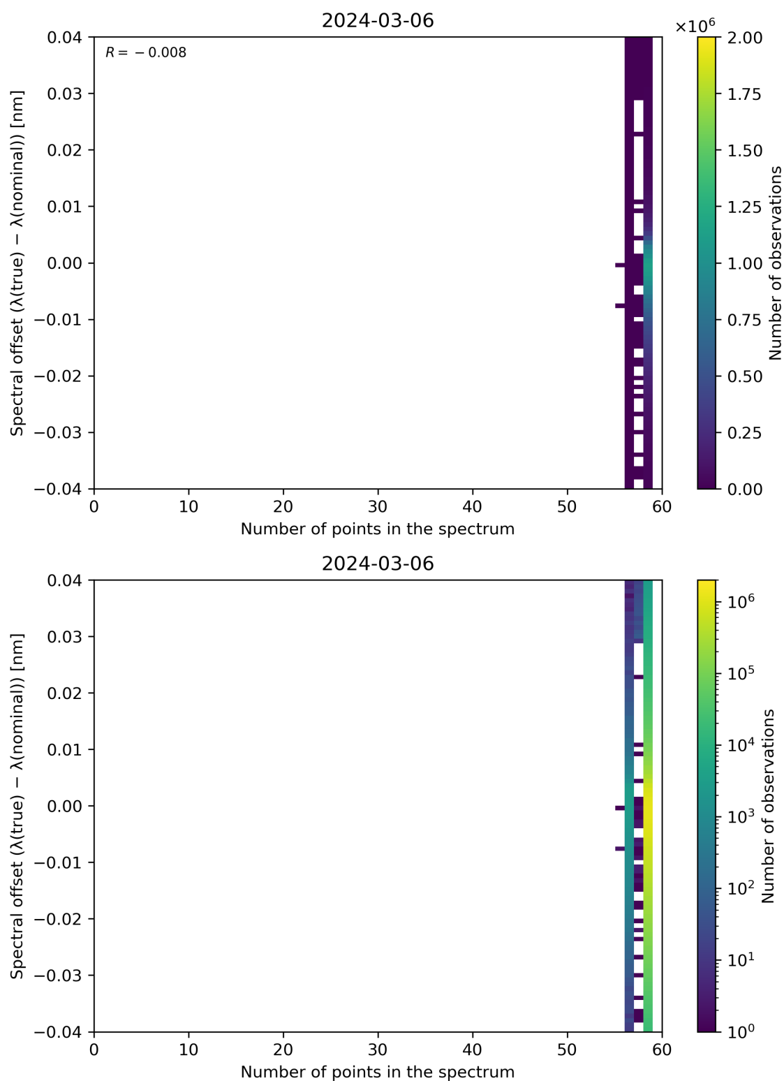
Figure 101: Scatter density plot of “Number of points in the spectrum” against “Spectral offset ( \lambda(\text{true}) - \lambda(\text{nominal}) )” for 2024-03-05 to 2024-03-07.
