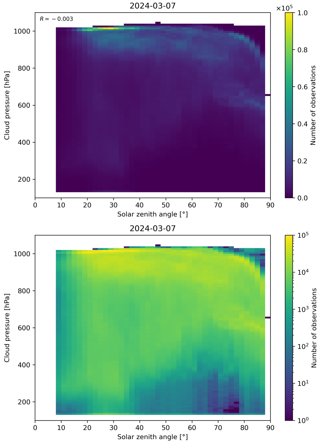
Figure 111: Scatter density plot of “Solar zenith angle” against “Cloud pressure” for 2024-03-06 to 2024-03-08.
