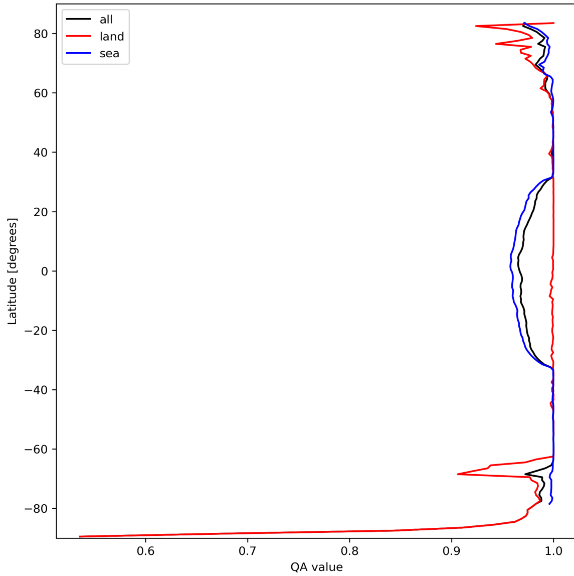
Figure 12: Zonal average of “QA value” for 2024-03-06 to 2024-03-08.
