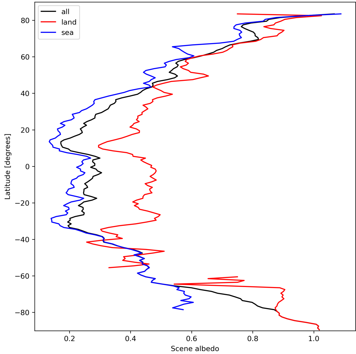
Figure 17: Zonal average of “Scene albedo” for 2024-03-06 to 2024-03-08.
