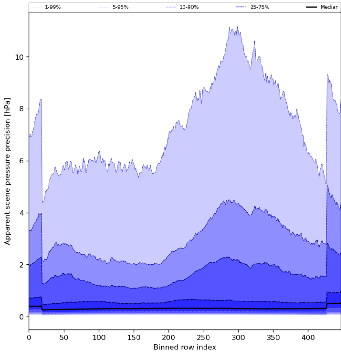
Figure 54: Along track statistics of “Apparent scene pressure precision” for 2024-03-06 to 2024-03-08
