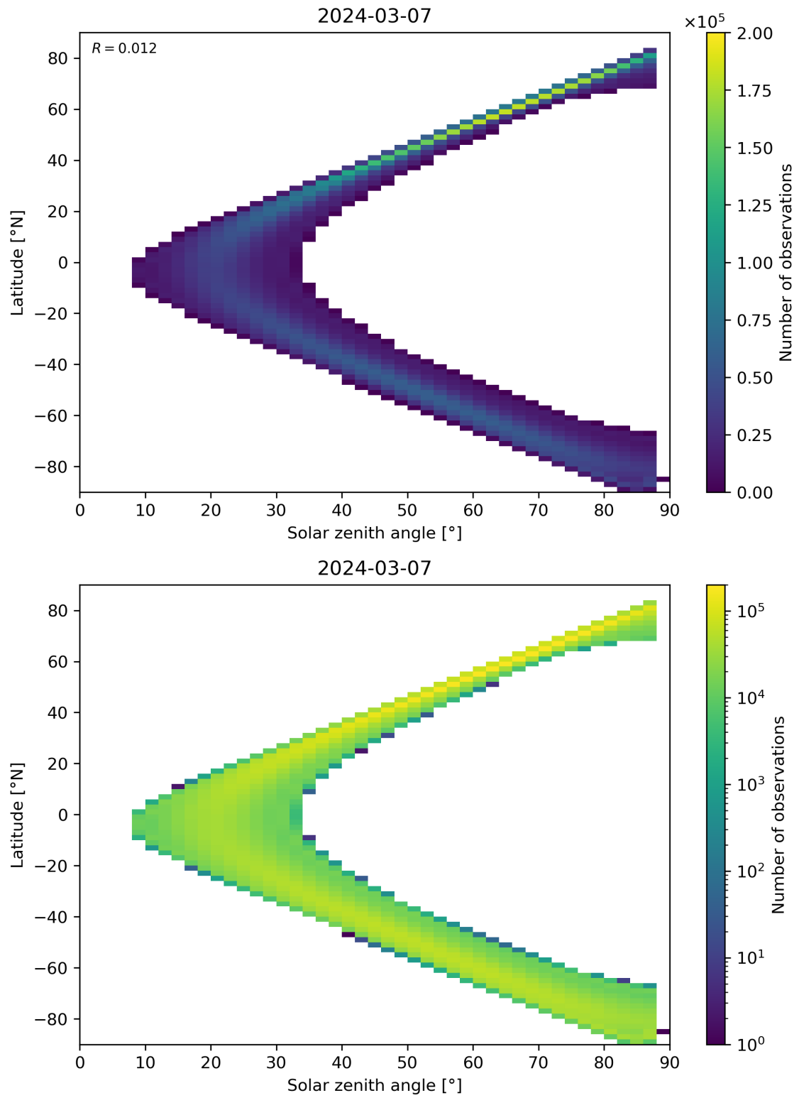
Figure 113: Scatter density plot of “Solar zenith angle” against “Latitude” for 2024-03-06 to 2024-03-08.
