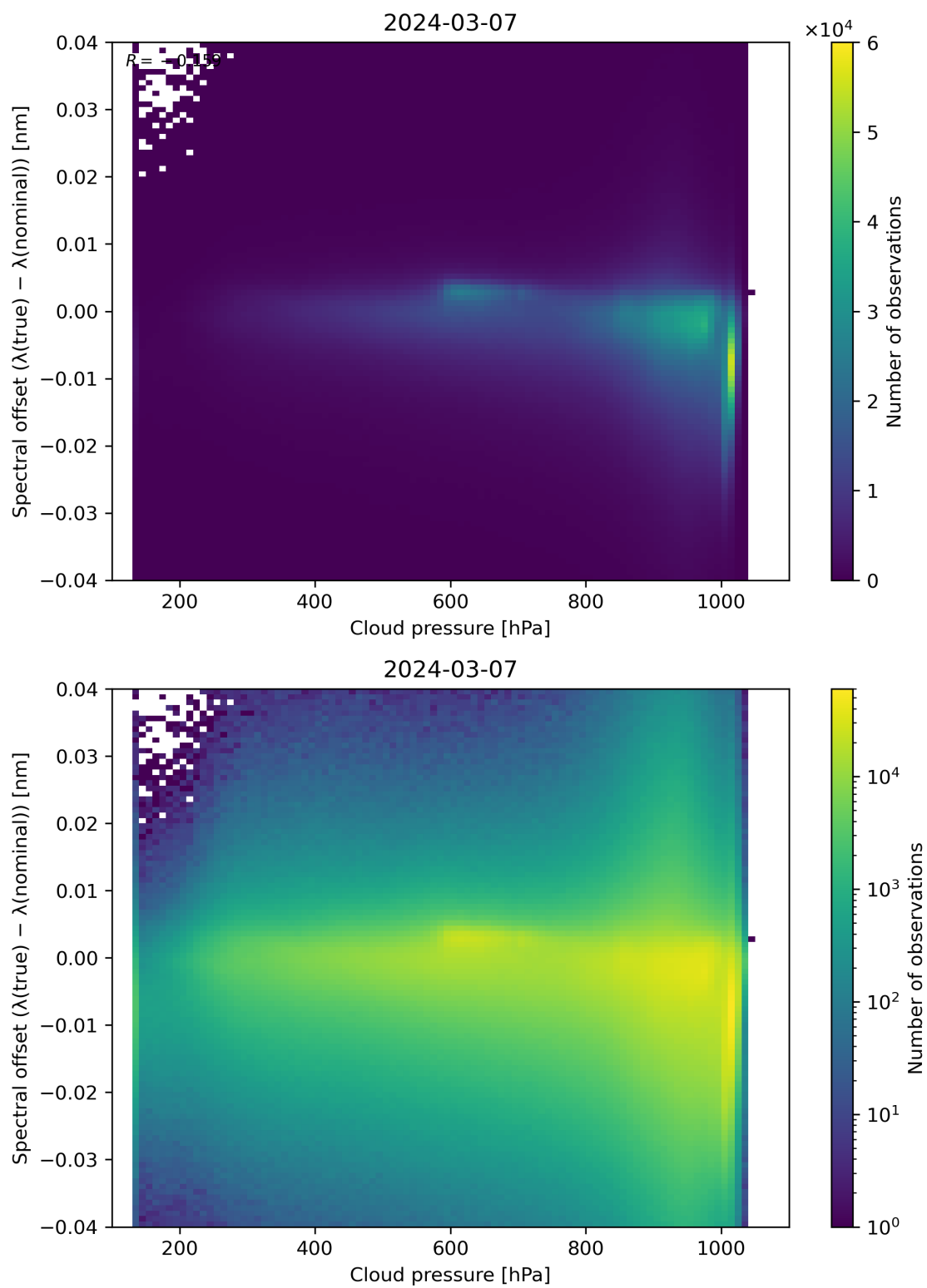
Figure 84: Scatter density plot of “Cloud pressure” against “Spectral offset ( \lambda(\text{true}) - \lambda(\text{nominal}) )” for 2024-03-06 to 2024-03-08.
