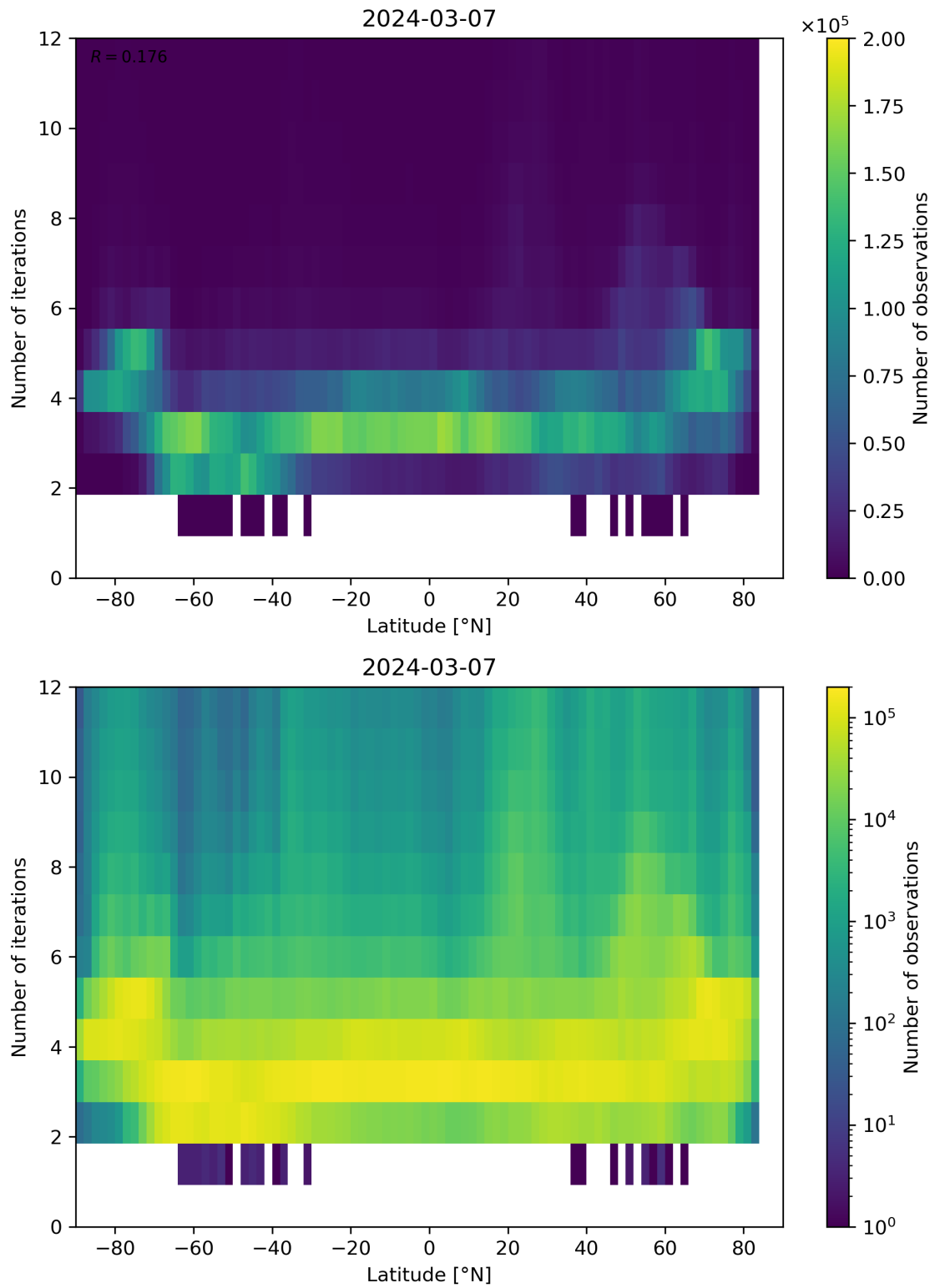
Figure 93: Scatter density plot of “Latitude” against “Number of iterations” for 2024-03-06 to 2024-03-08.
