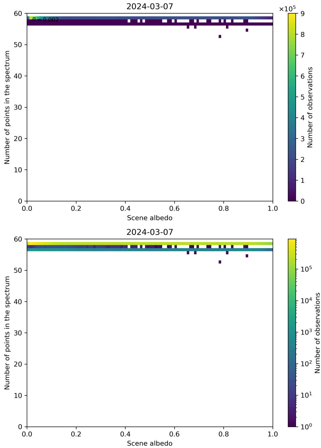
Figure 106: Scatter density plot of “Scene albedo” against “Number of points in the spectrum” for 2024-03-06 to 2024-03-08.
