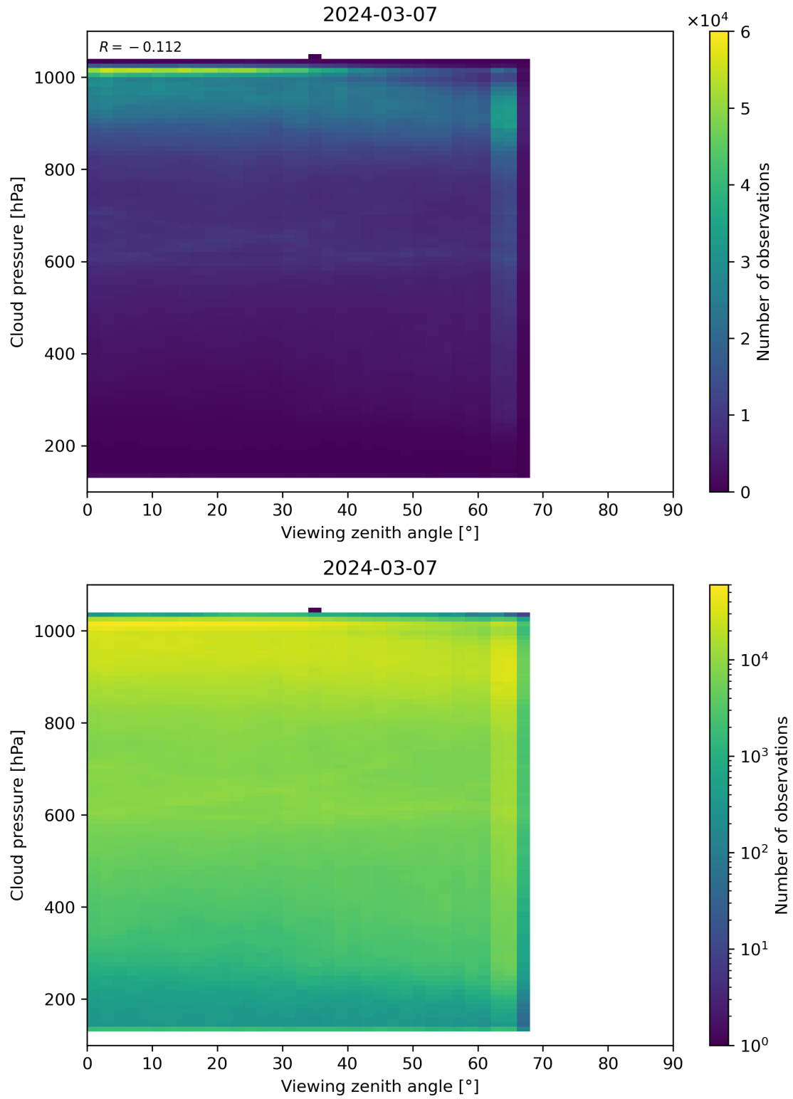
Figure 121: Scatter density plot of “Viewing zenith angle” against “Cloud pressure” for 2024-03-06 to 2024-03-08.
