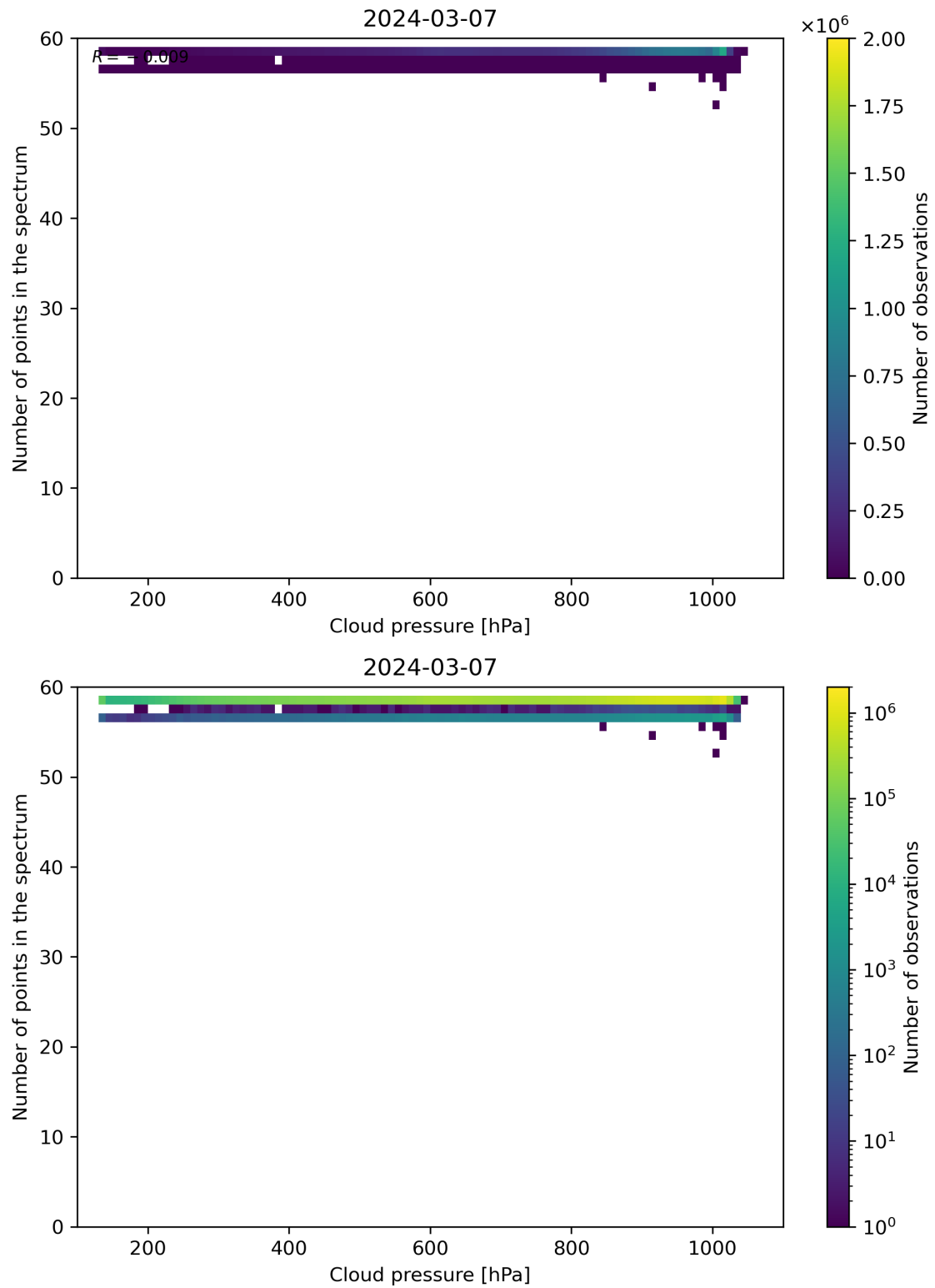
Figure 82: Scatter density plot of “Cloud pressure” against “Number of points in the spectrum” for 2024-03-06 to 2024-03-08.
