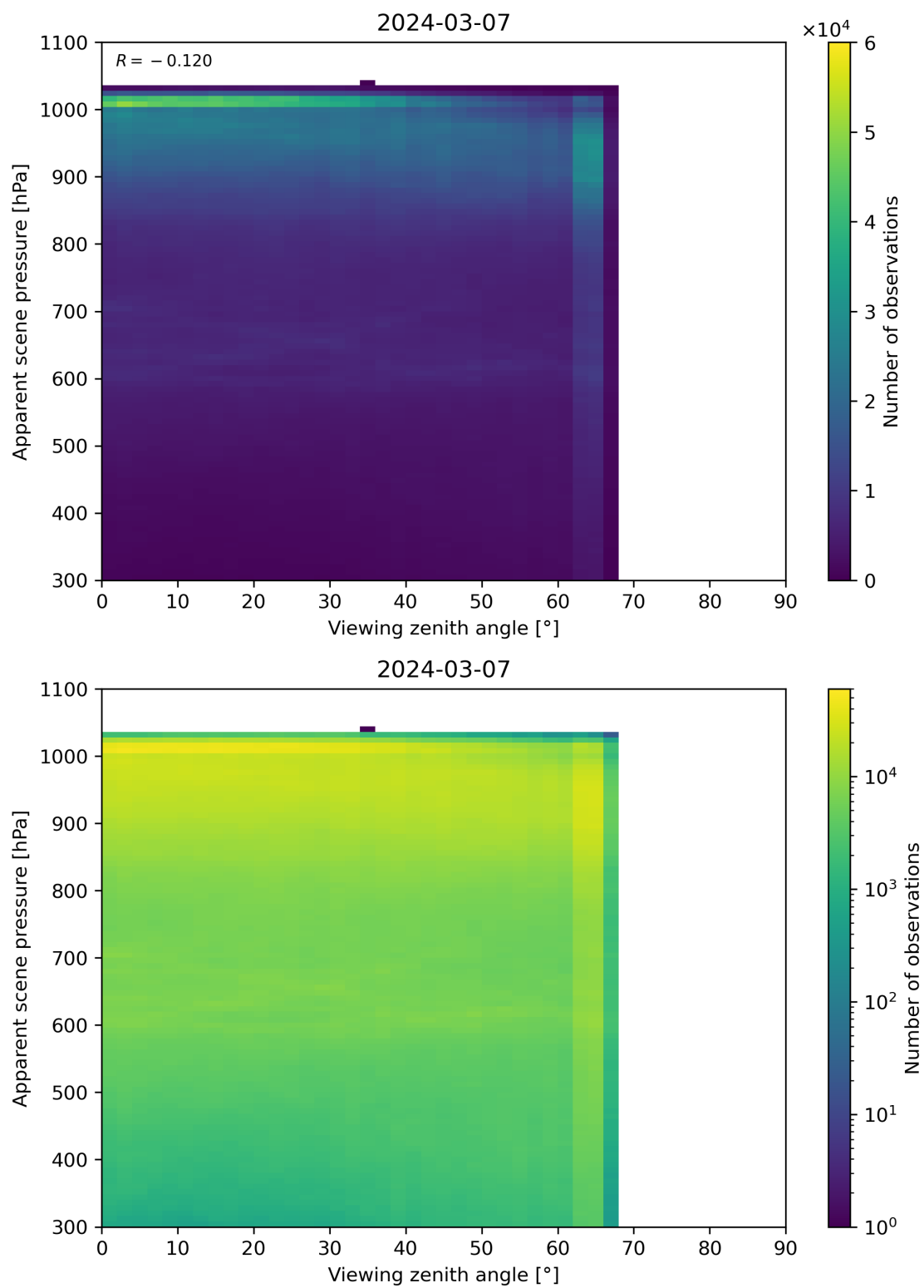
Figure 118: Scatter density plot of “Viewing zenith angle” against “Apparent scene pressure” for 2024-03-06 to 2024-03-08.
