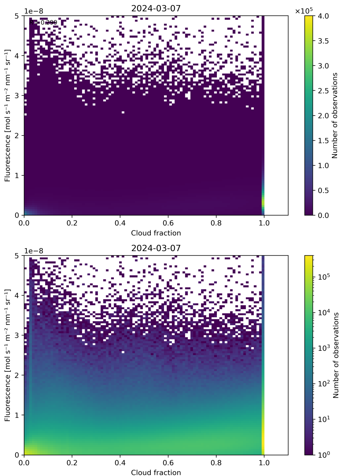
Figure 72: Scatter density plot of “Cloud fraction” against “Fluorescence” for 2024-03-06 to 2024-03-08.
