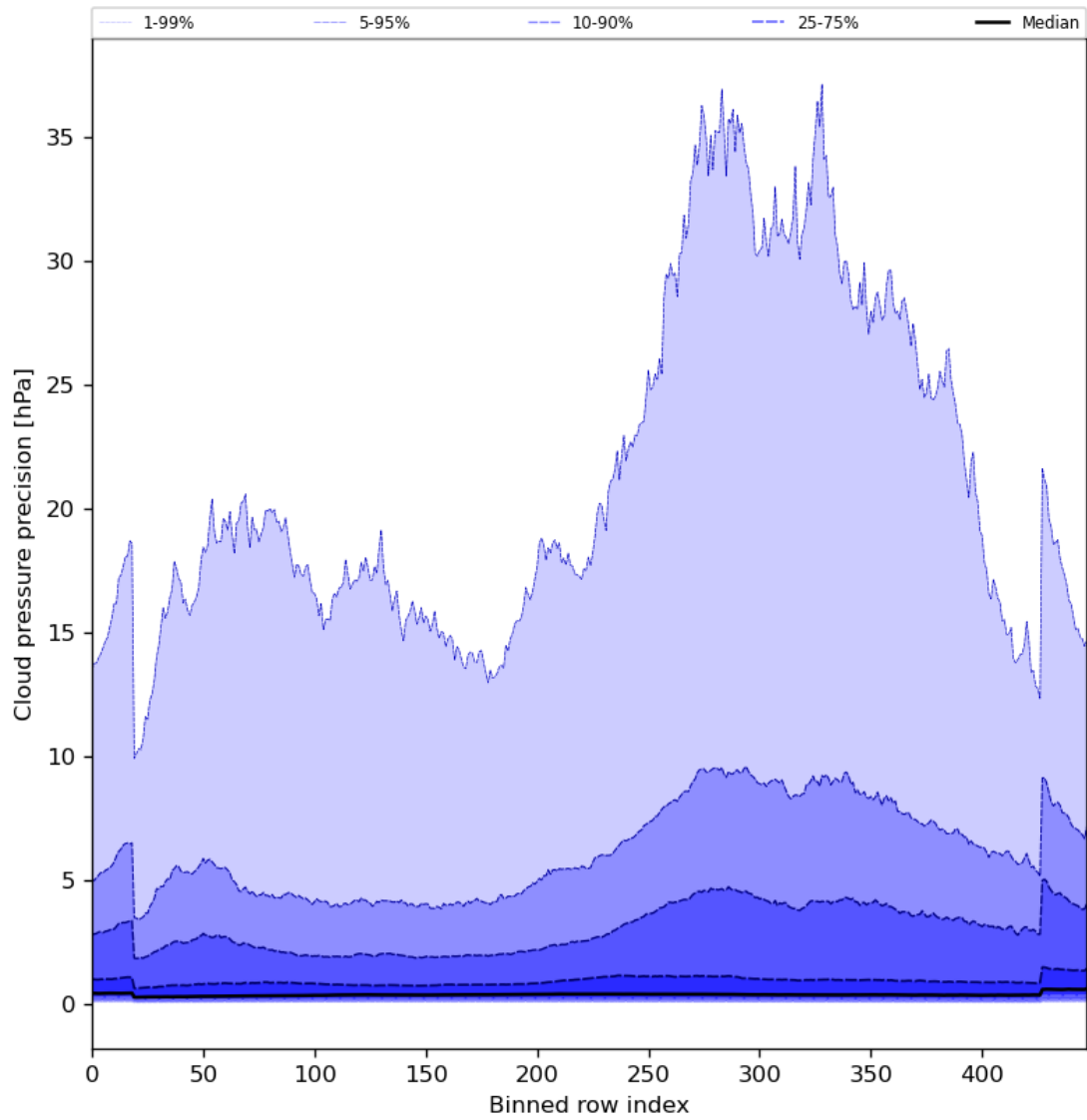
Figure 48: Along track statistics of “Cloud pressure precision” for 2024-03-06 to 2024-03-08
