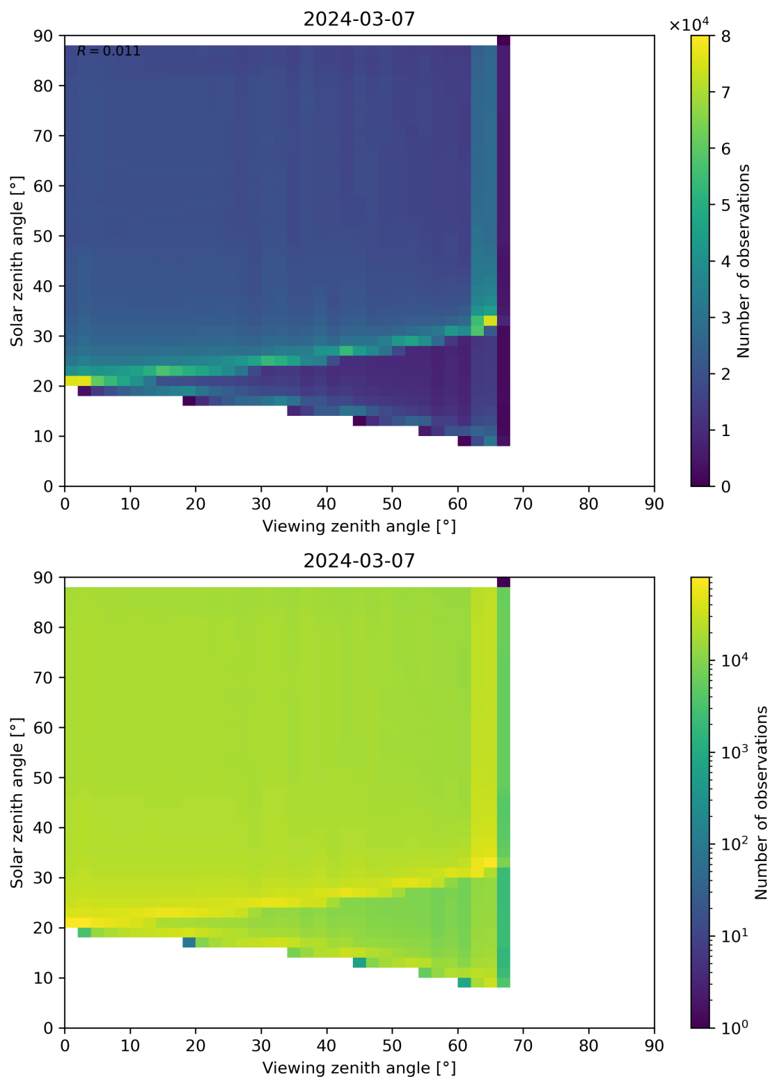
Figure 127: Scatter density plot of “Viewing zenith angle” against “Solar zenith angle” for 2024-03-06 to 2024-03-08.
