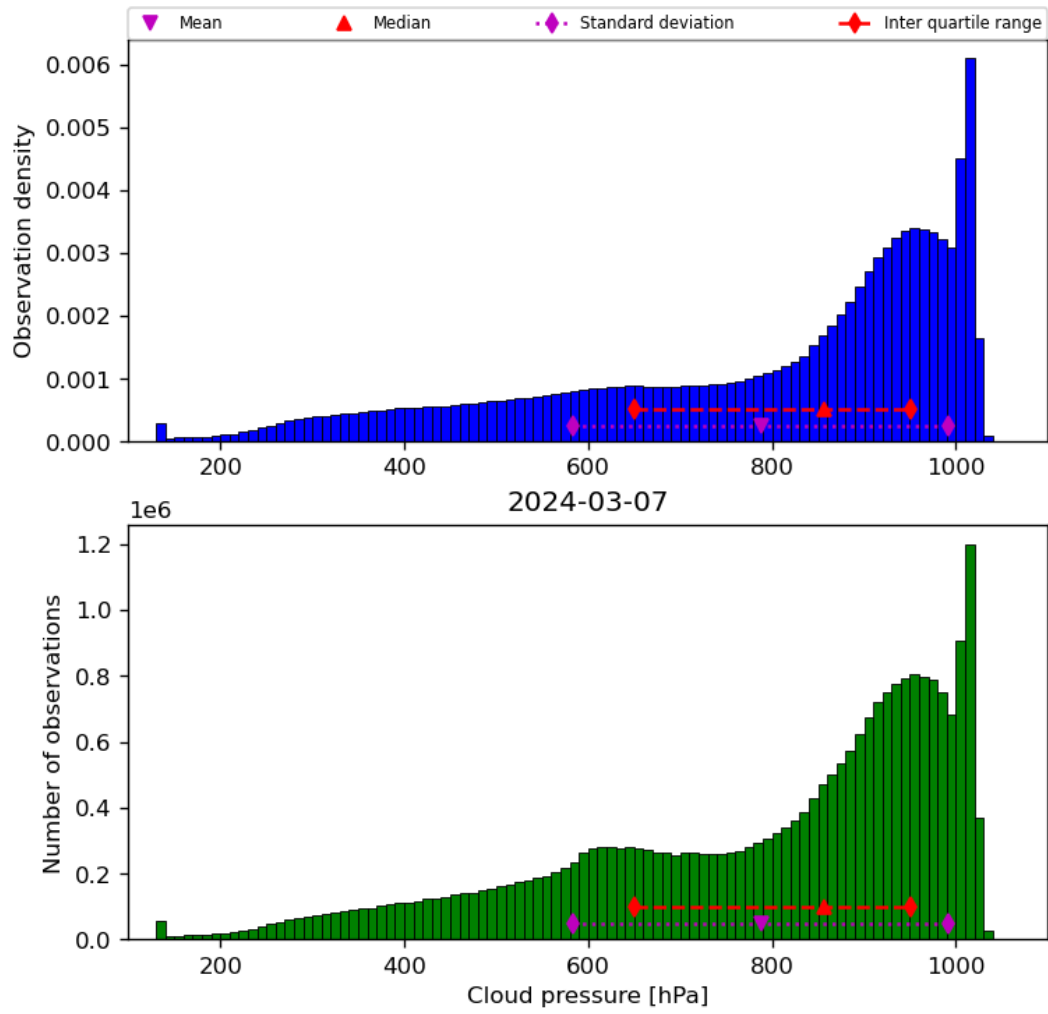
Figure 30: Histogram of “Cloud pressure” for 2024-03-06 to 2024-03-08
