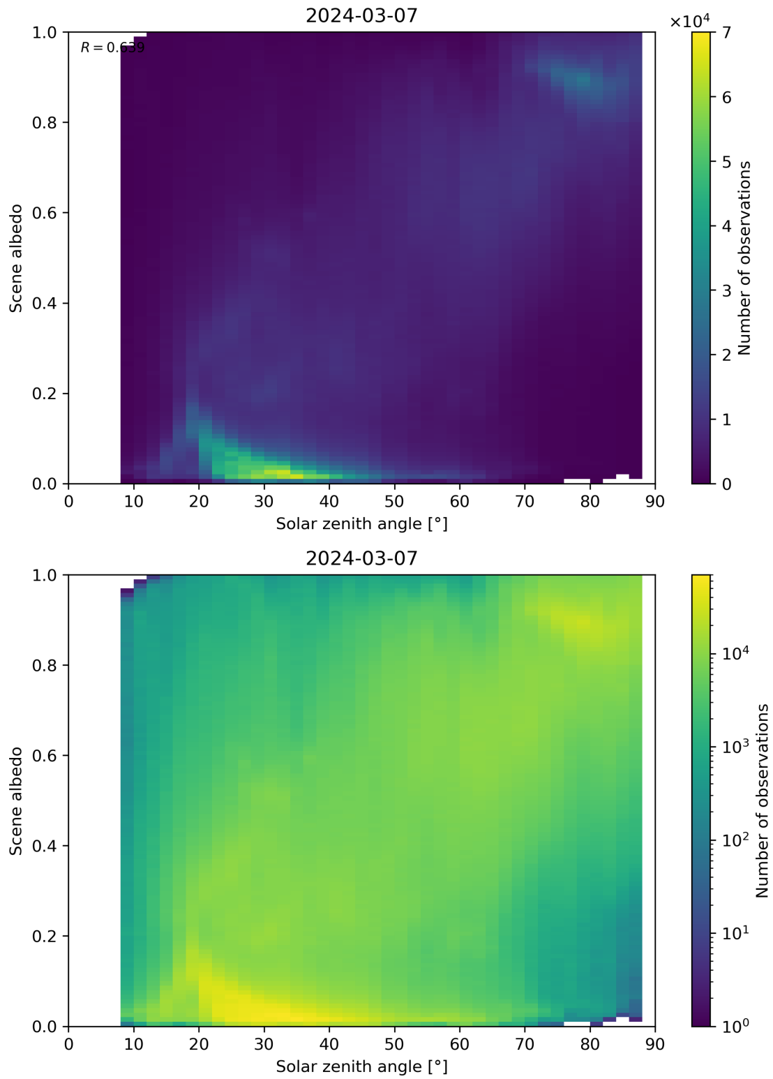
Figure 116: Scatter density plot of “Solar zenith angle” against “Scene albedo” for 2024-03-06 to 2024-03-08.
