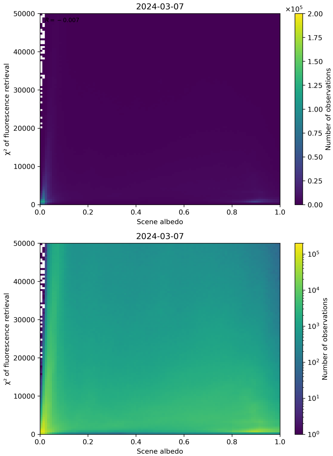
Figure 103: Scatter density plot of “Scene albedo” against “ \chi^2 of fluorescence retrieval” for 2024-03-06 to 2024-03-08.
