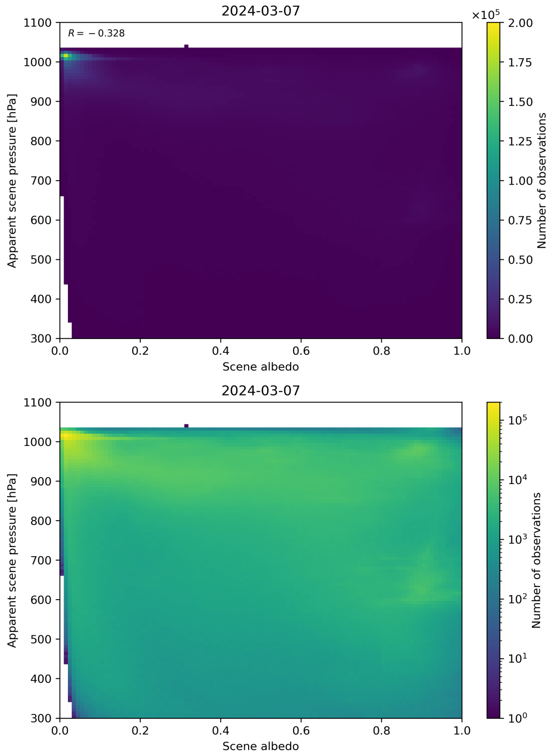
Figure 102: Scatter density plot of “Scene albedo” against “Apparent scene pressure” for 2024-03-06 to 2024-03-08.
