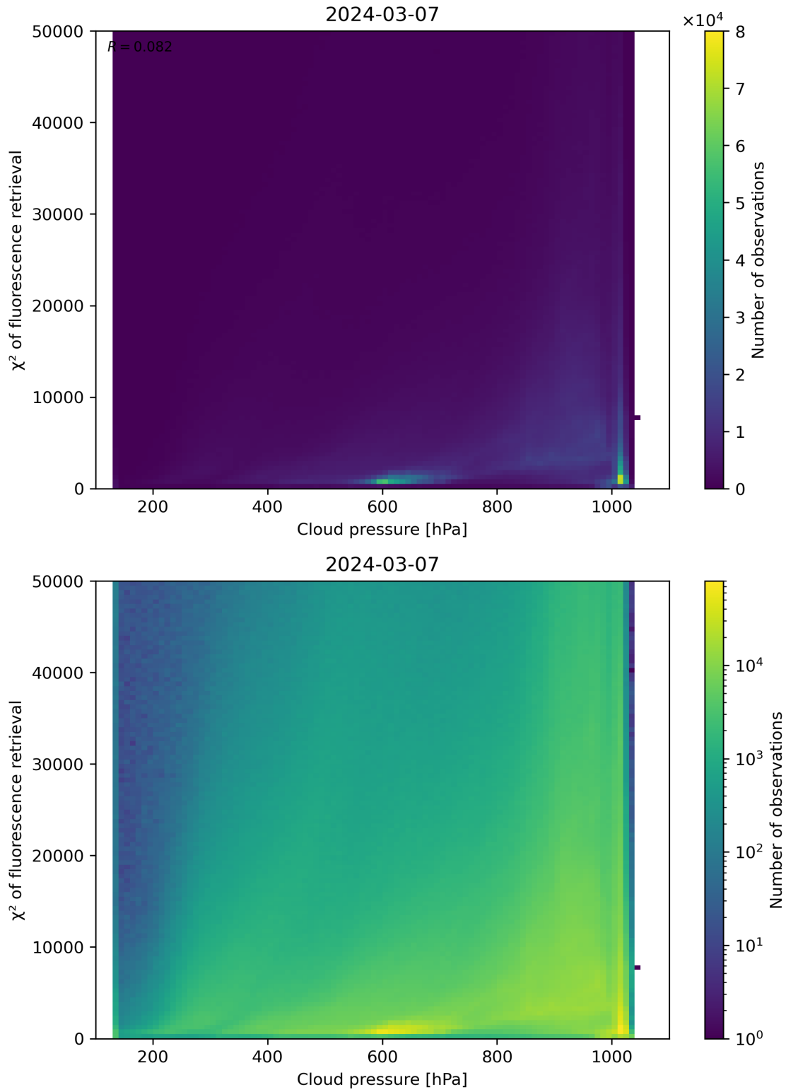
Figure 78: Scatter density plot of “Cloud pressure” against “ \chi^2 of fluorescence retrieval” for 2024-03-06 to 2024-03-08.
