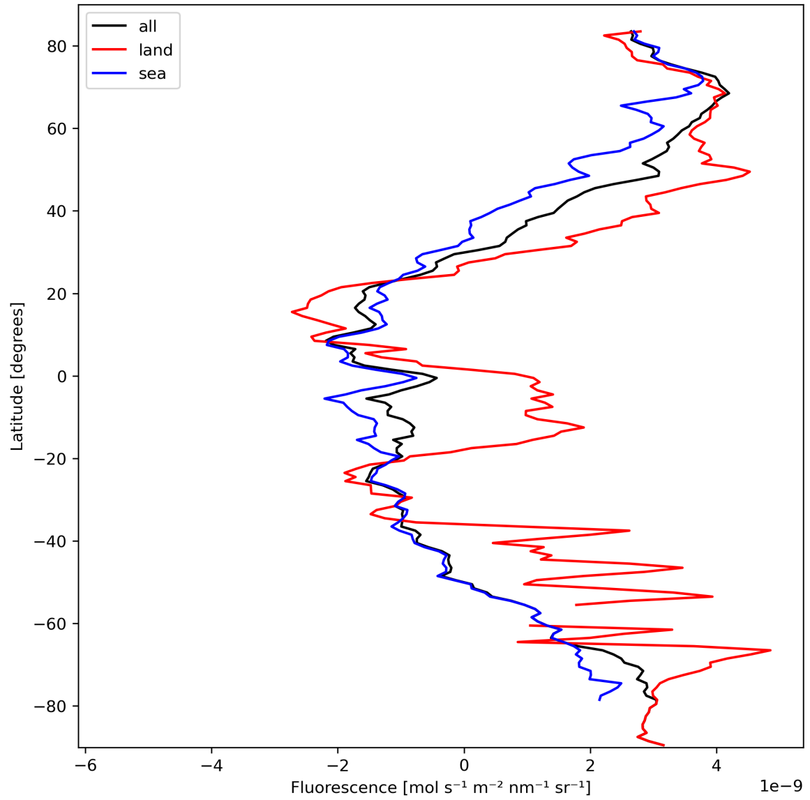
Figure 23: Zonal average of “Fluorescence” for 2024-03-06 to 2024-03-08.
