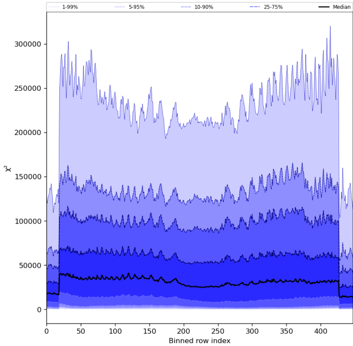
Figure 55: Along track statistics of “ \chi^2 ” for 2024-03-06 to 2024-03-08
