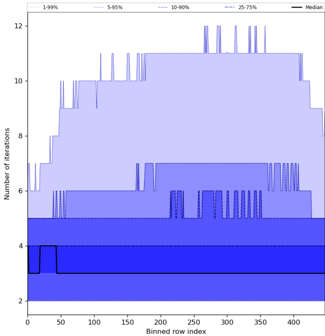
Figure 56: Along track statistics of “Number of iterations” for 2024-03-06 to 2024-03-08
