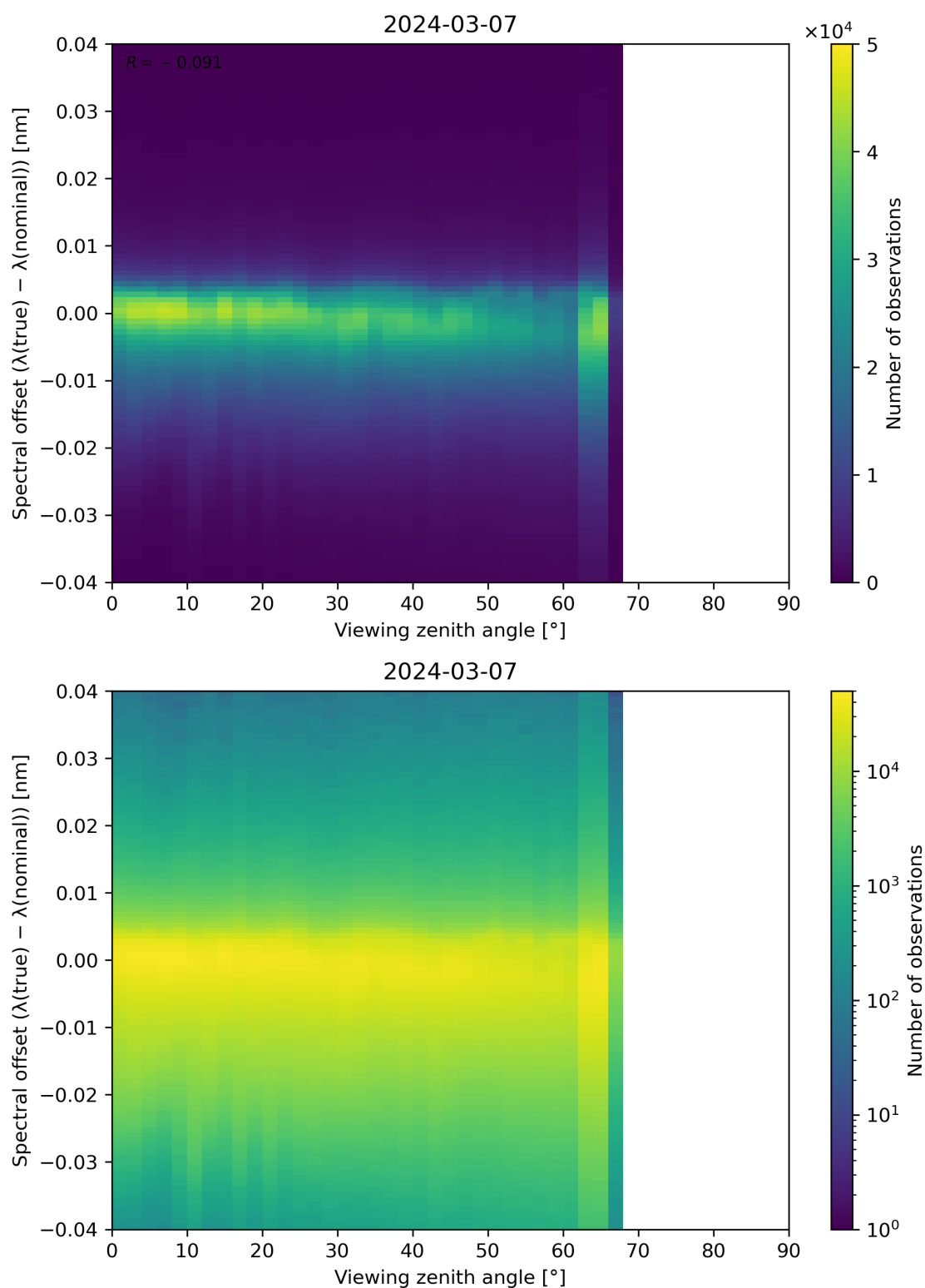
Figure 128: Scatter density plot of “Viewing zenith angle” against “Spectral offset ( \lambda(\text{true}) - \lambda(\text{nominal}) )” for 2024-03-06 to 2024-03-08.
