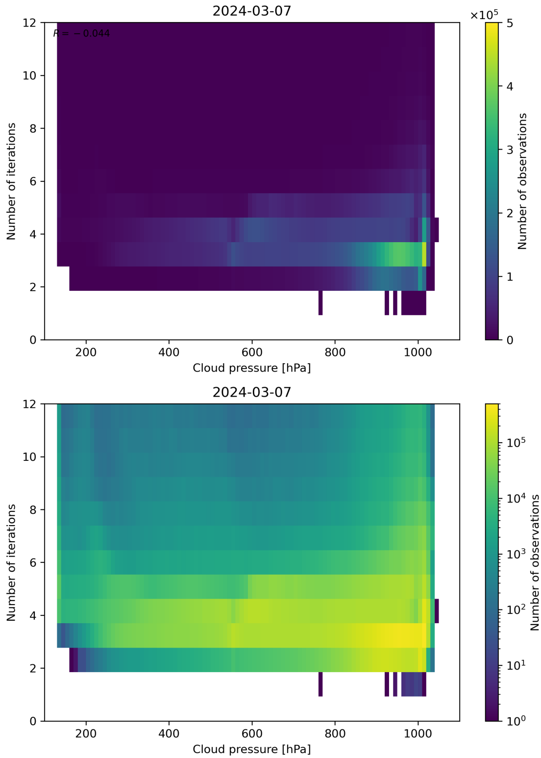
Figure 81: Scatter density plot of “Cloud pressure” against “Number of iterations” for 2024-03-06 to 2024-03-08.
