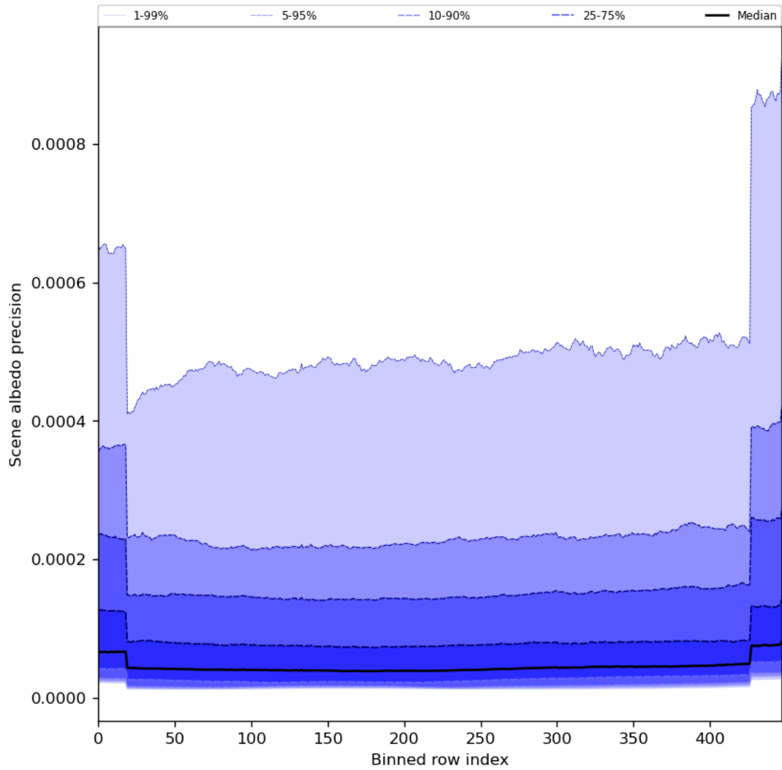
Figure 52: Along track statistics of “Scene albedo precision” for 2024-03-06 to 2024-03-08
