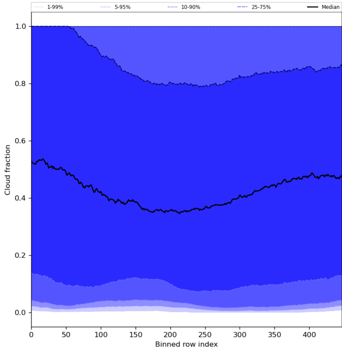
Figure 49: Along track statistics of “Cloud fraction” for 2024-03-06 to 2024-03-08
