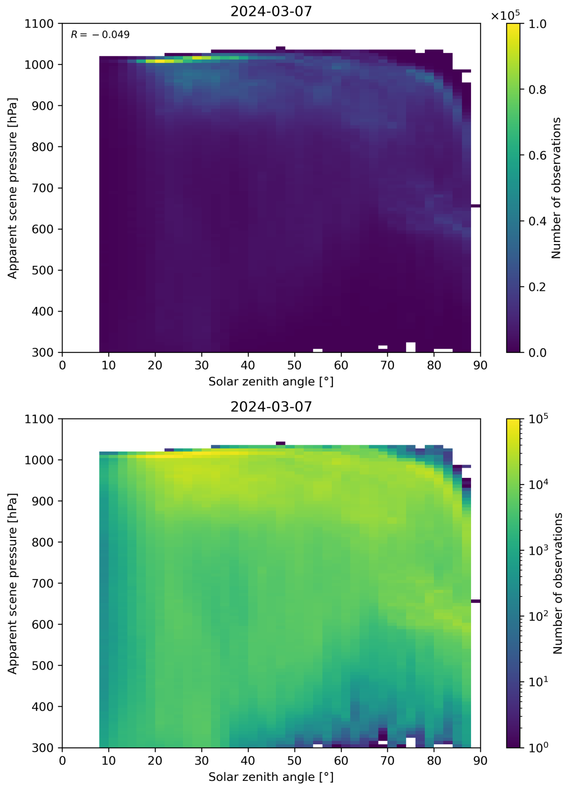
Figure 108: Scatter density plot of “Solar zenith angle” against “Apparent scene pressure” for 2024-03-06 to 2024-03-08.
