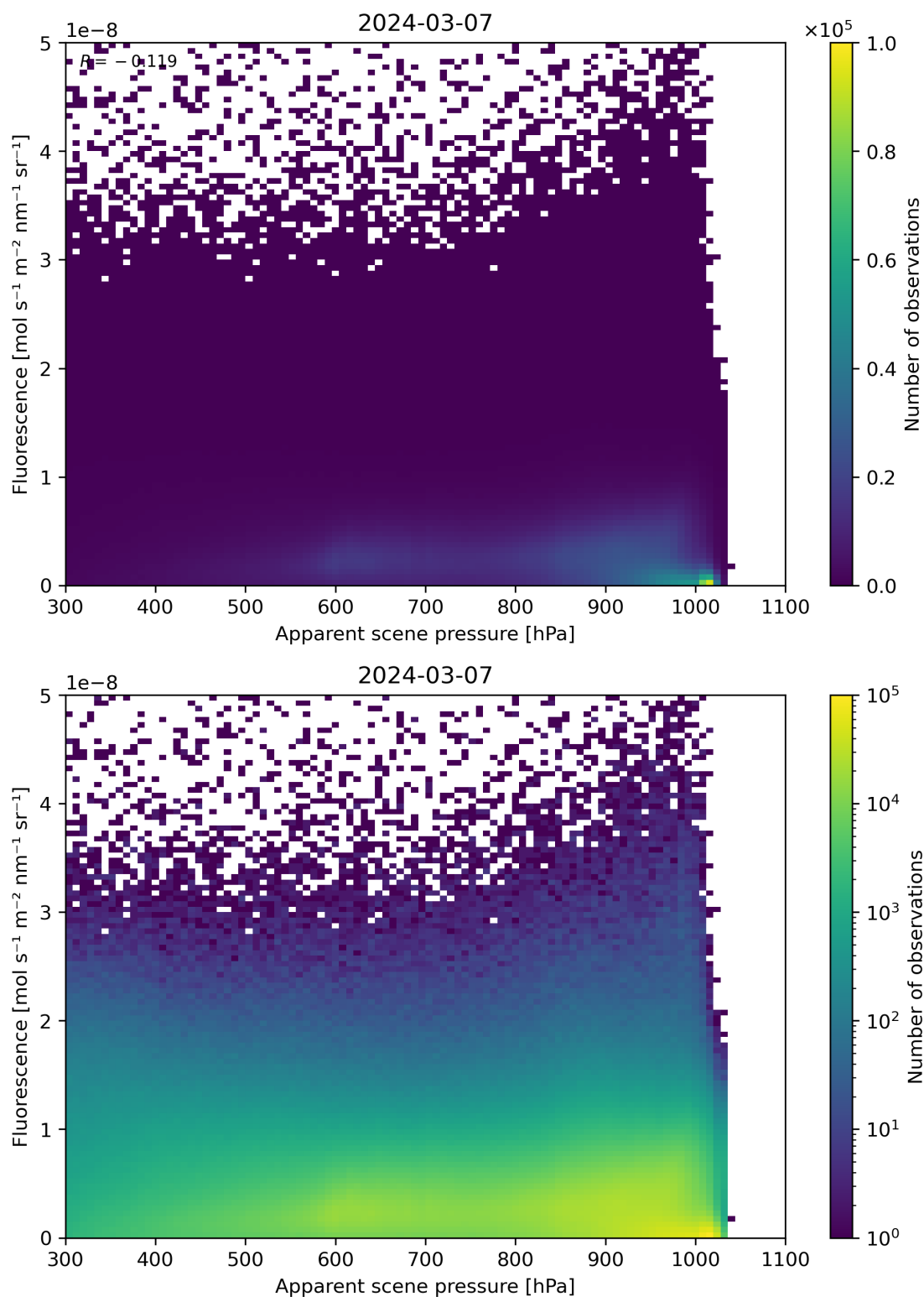
Figure 64: Scatter density plot of “Apparent scene pressure” against “Fluorescence” for 2024-03-06 to 2024-03-08.
