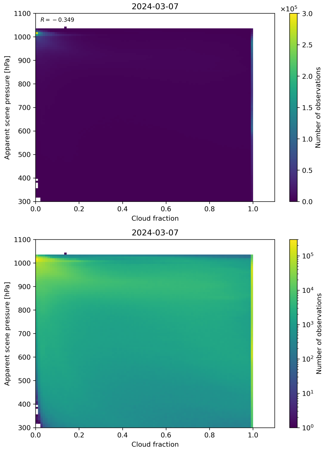
Figure 70: Scatter density plot of “Cloud fraction” against “Apparent scene pressure” for 2024-03-06 to 2024-03-08.
