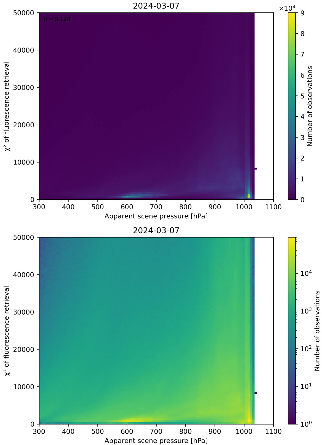
Figure 63: Scatter density plot of “Apparent scene pressure” against “ \chi^2 of fluorescence retrieval” for 2024-03-06 to 2024-03-08.
