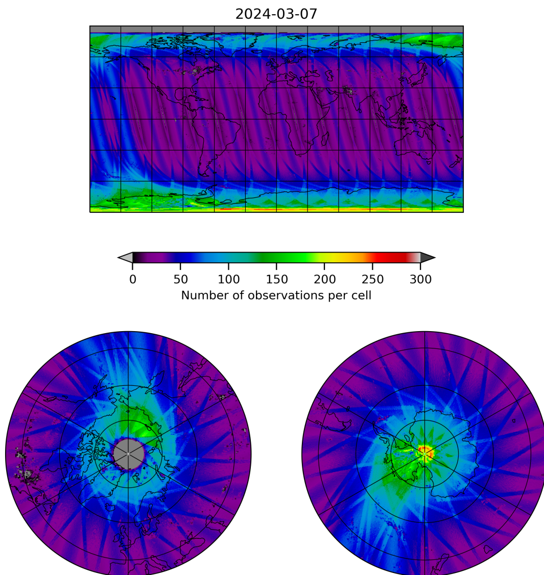
Figure 11: Map of the number of observations for 2024-03-06 to 2024-03-08
