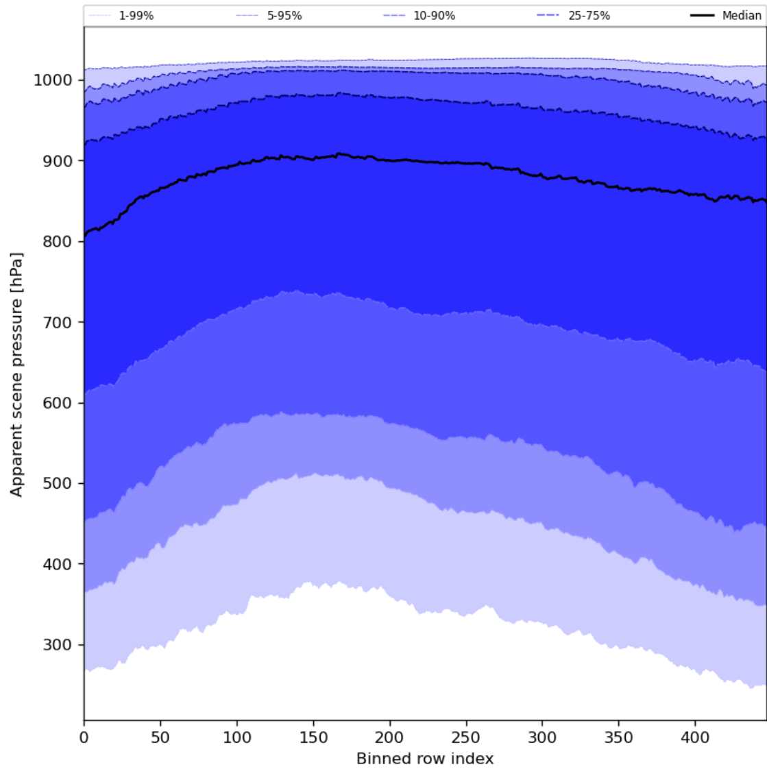
Figure 53: Along track statistics of “Apparent scene pressure” for 2024-03-06 to 2024-03-08
