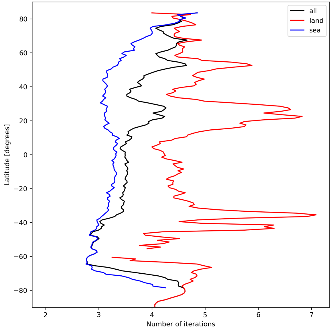
Figure 22: Zonal average of “Number of iterations” for 2024-03-06 to 2024-03-08.
