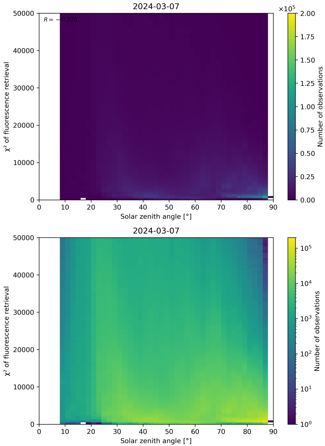
Figure 109: Scatter density plot of “Solar zenith angle” against “ \chi^2 of fluorescence retrieval” for 2024-03-06 to 2024-03-08.
