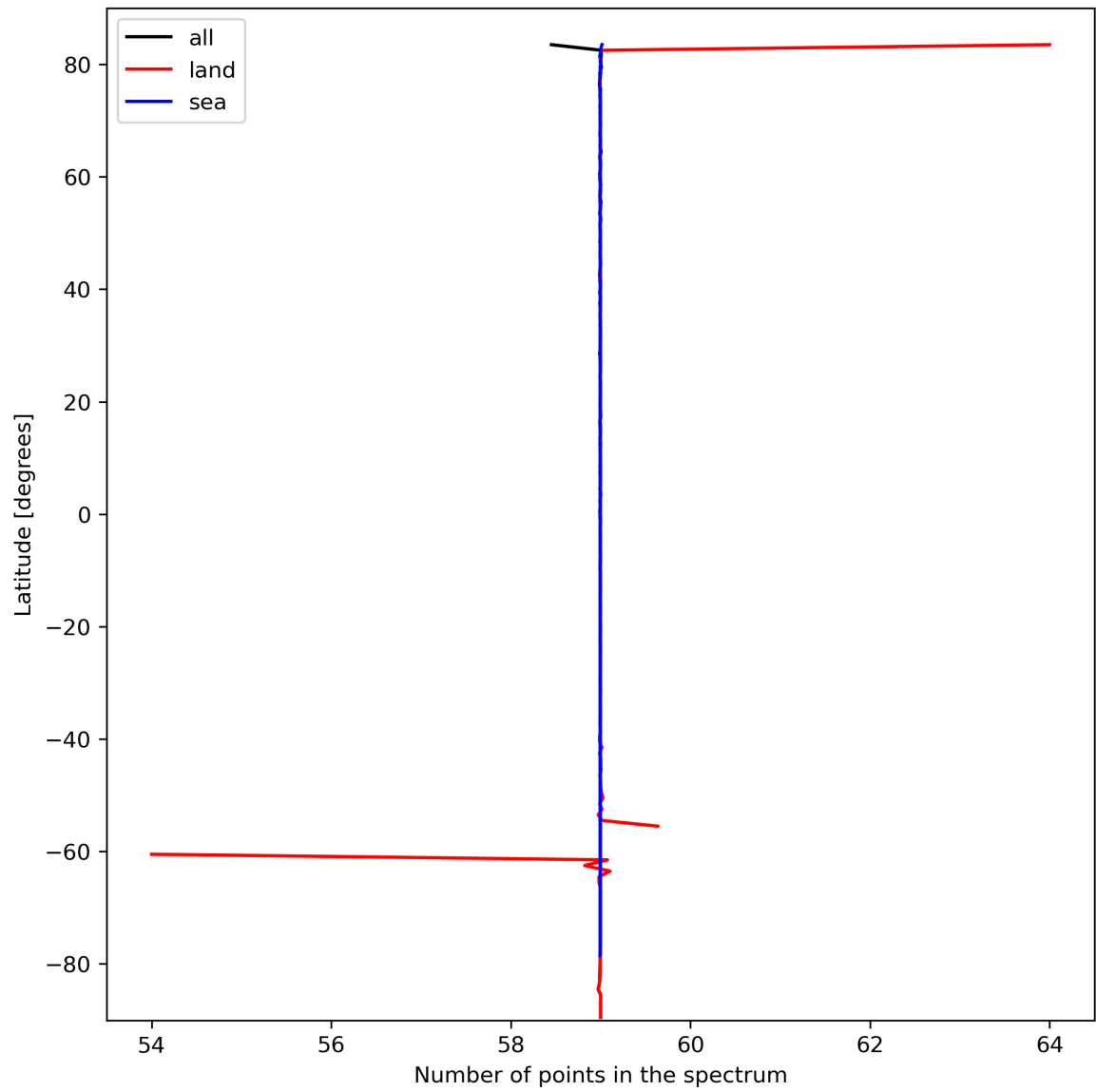
Figure 27: Zonal average of “Number of points in the spectrum” for 2024-03-06 to 2024-03-08.
