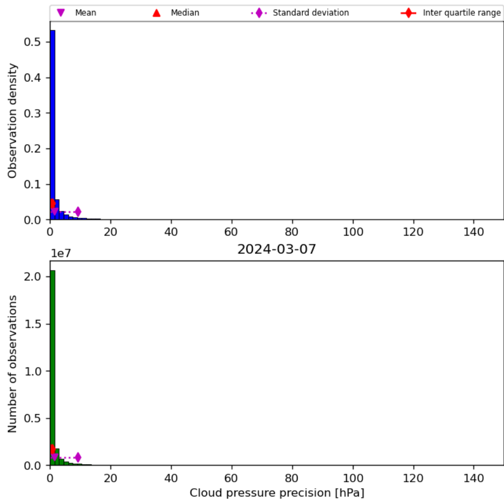
Figure 31: Histogram of “Cloud pressure precision” for 2024-03-06 to 2024-03-08
