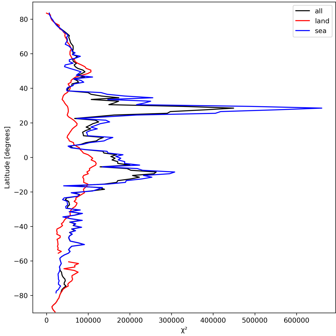
Figure 21: Zonal average of “ \chi^2 ” for 2024-03-06 to 2024-03-08.
