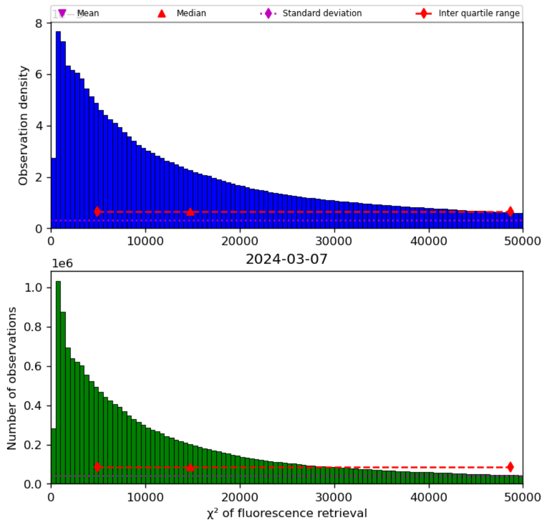
Figure 42: Histogram of “ \chi^2 of fluorescence retrieval” for 2024-03-06 to 2024-03-08
