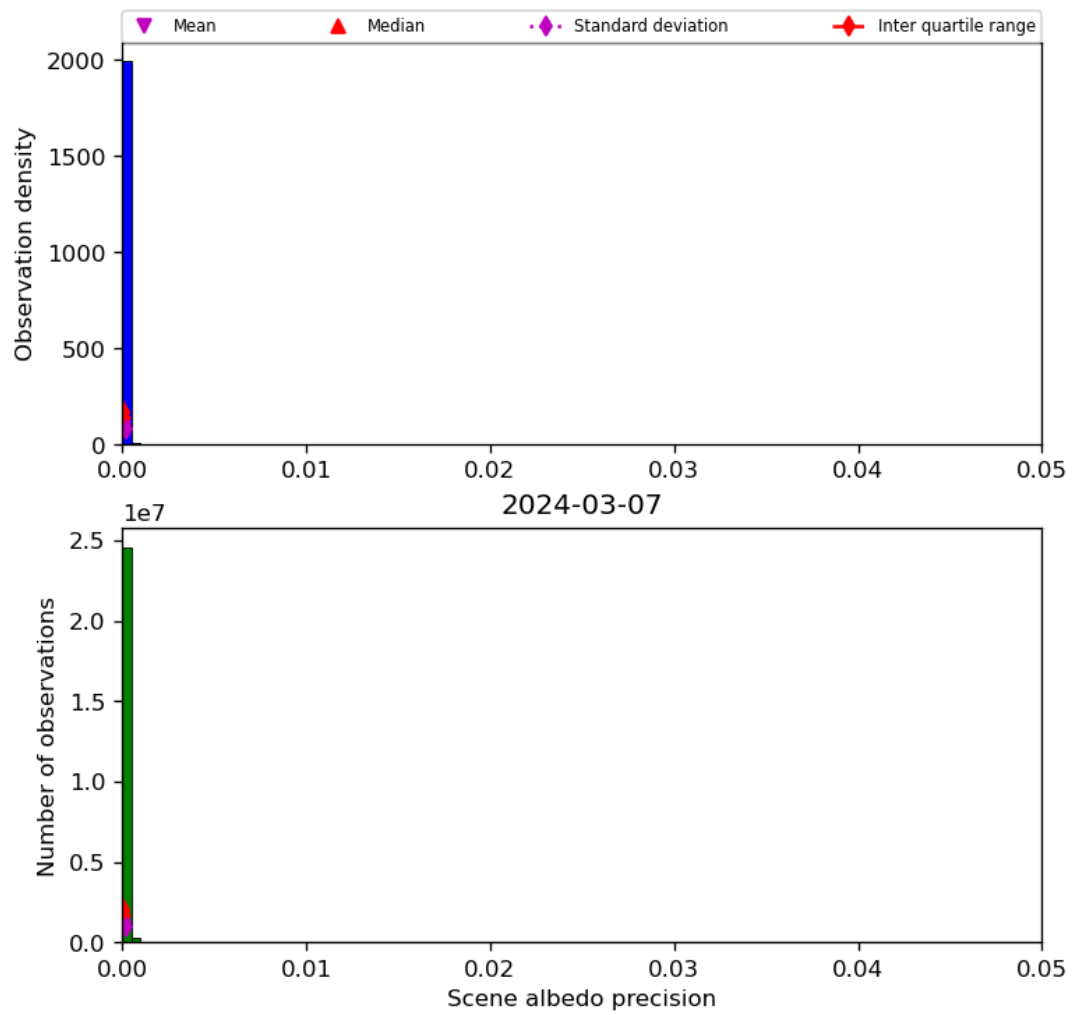
Figure 35: Histogram of “Scene albedo precision” for 2024-03-06 to 2024-03-08
