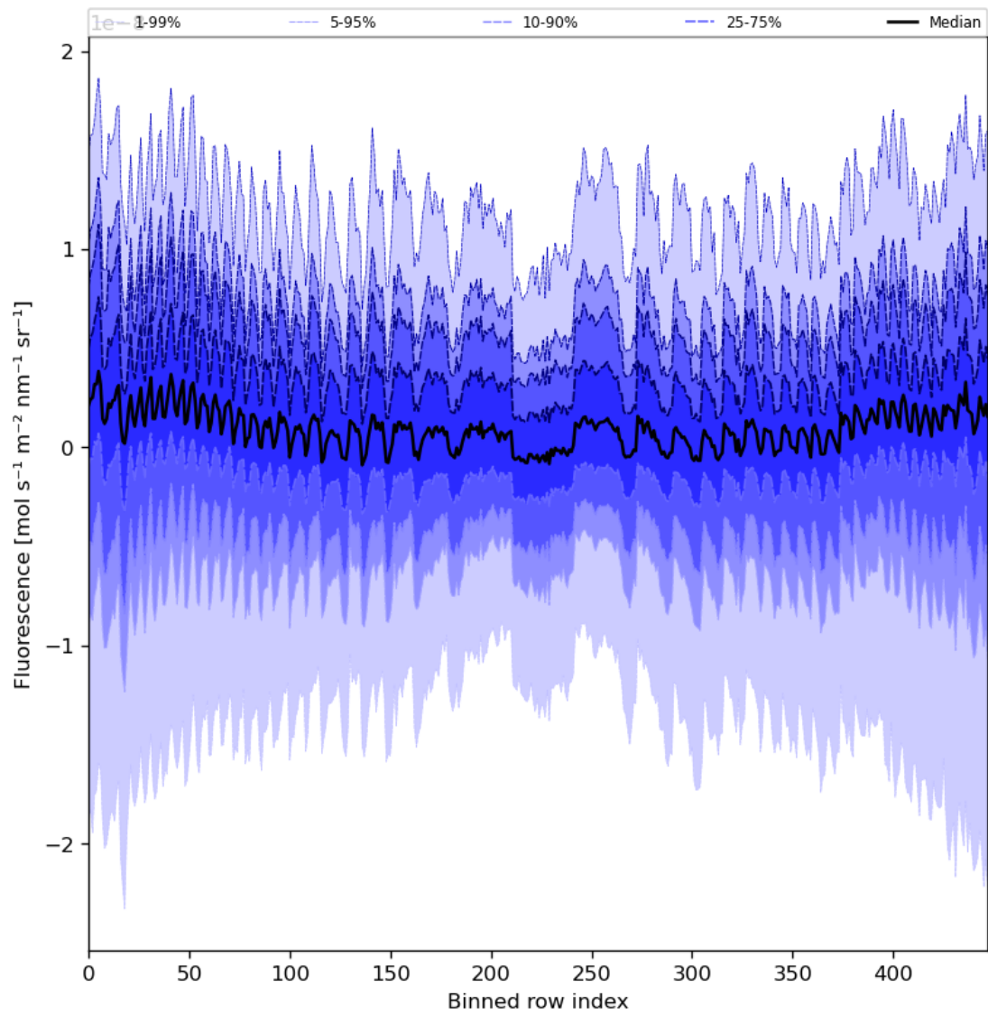
Figure 57: Along track statistics of “Fluorescence” for 2024-03-06 to 2024-03-08
