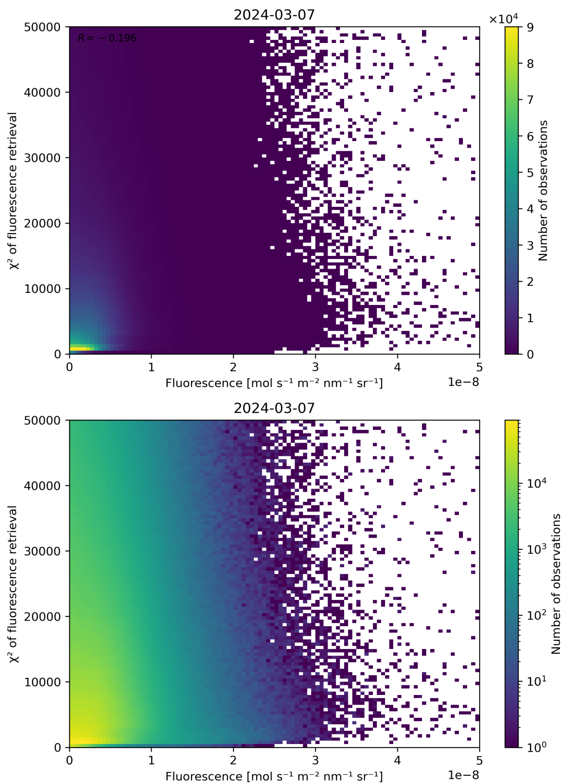
Figure 85: Scatter density plot of “Fluorescence” against “ \chi^2 of fluorescence retrieval” for 2024-03-06 to 2024-03-08.
