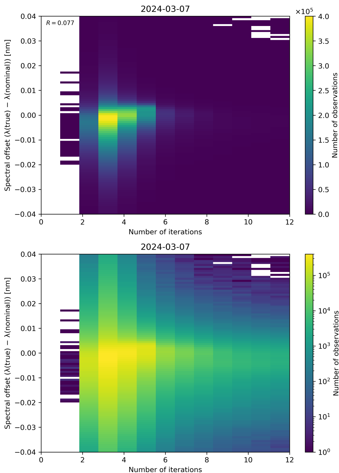
Figure 100: Scatter density plot of “Number of iterations” against “Spectral offset ( \lambda(\text{true}) - \lambda(\text{nominal}) )” for 2024-03-06 to 2024-03-08.
