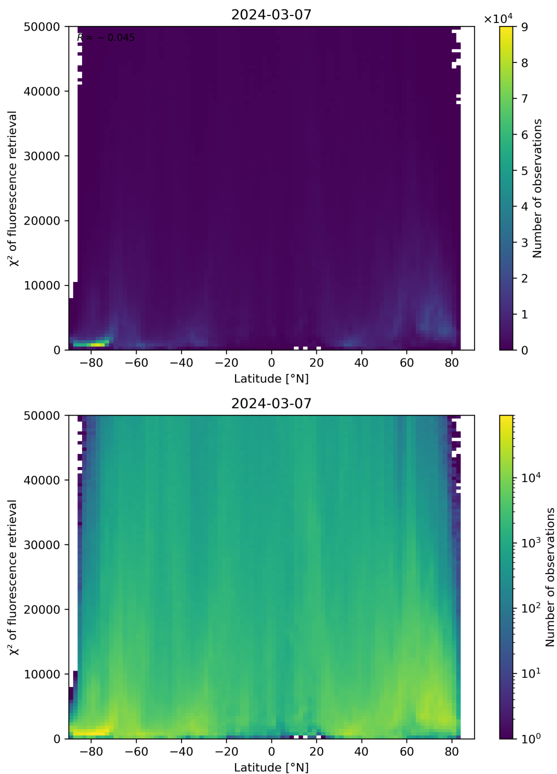
Figure 89: Scatter density plot of “Latitude” against “ \chi^2 of fluorescence retrieval” for 2024-03-06 to 2024-03-08.
