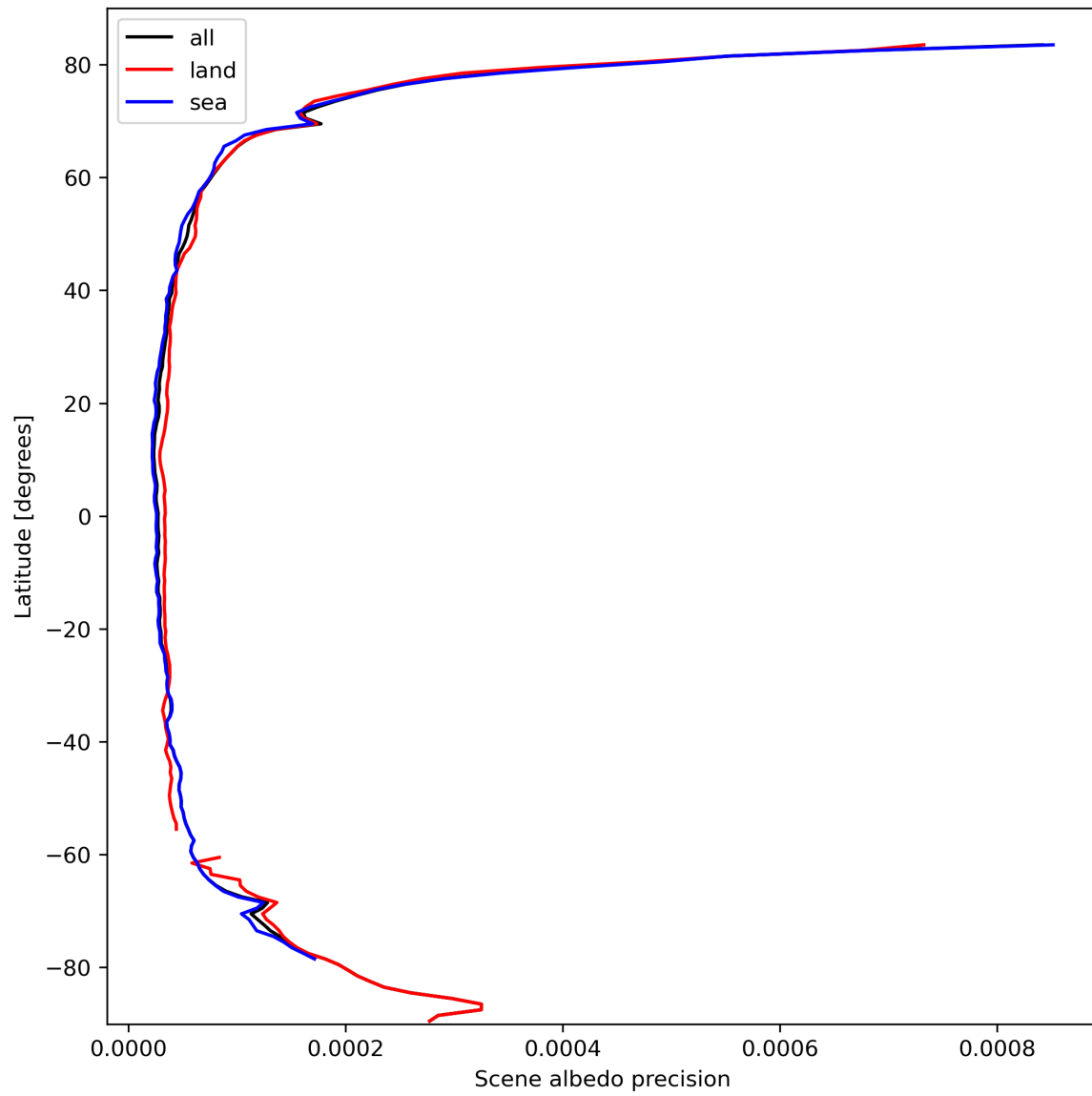
Figure 18: Zonal average of “Scene albedo precision” for 2024-03-06 to 2024-03-08.
