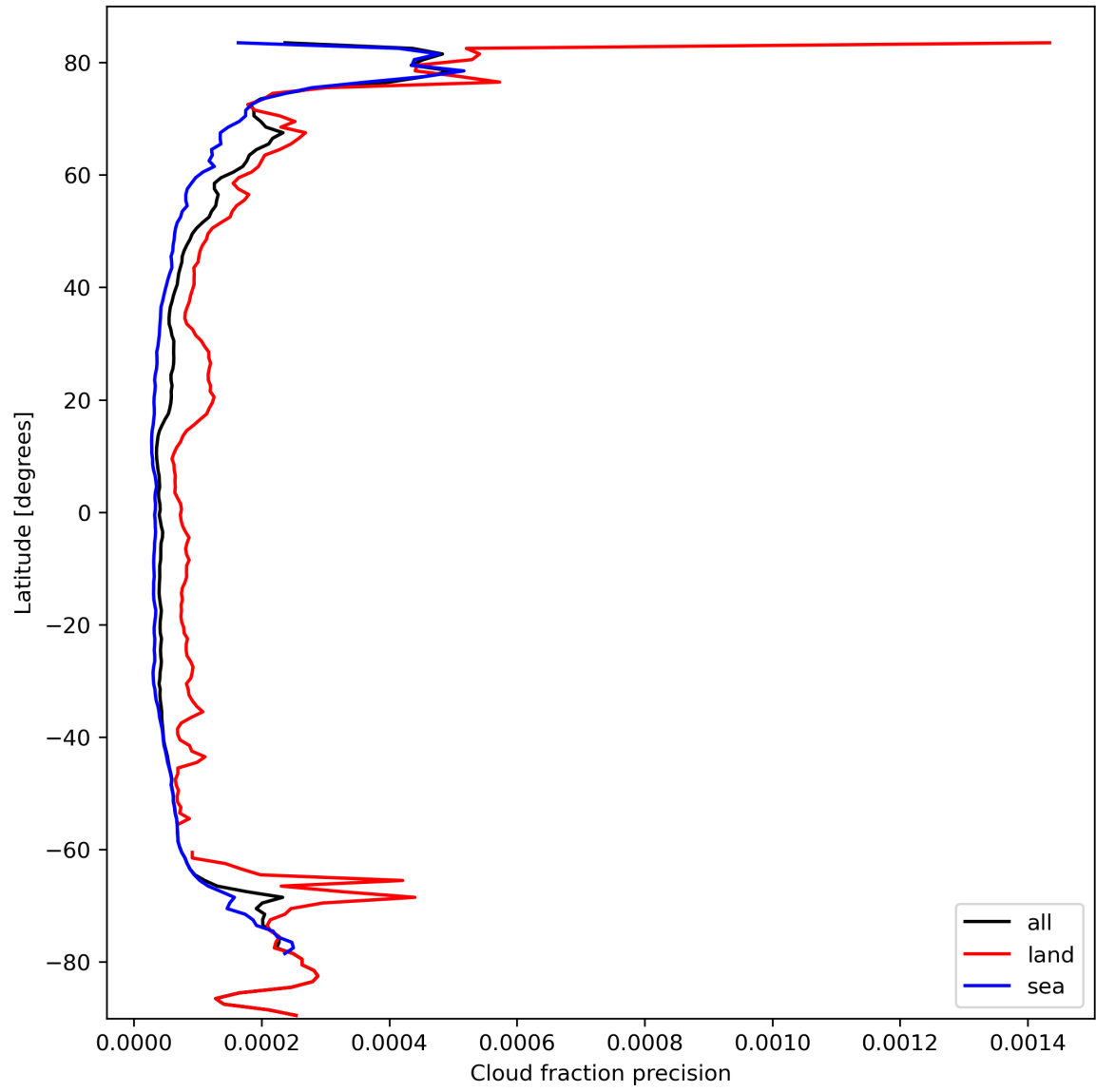
Figure 16: Zonal average of “Cloud fraction precision” for 2024-03-06 to 2024-03-08.
