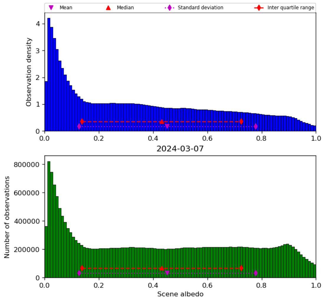
Figure 34: Histogram of “Scene albedo” for 2024-03-06 to 2024-03-08
