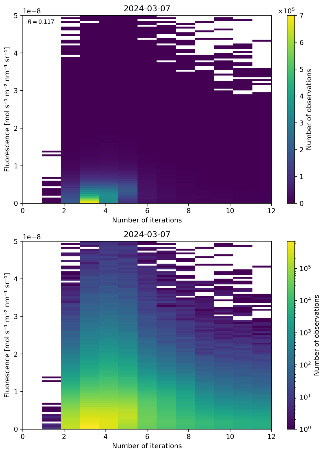
Figure 98: Scatter density plot of “Number of iterations” against “Fluorescence” for 2024-03-06 to 2024-03-08.
