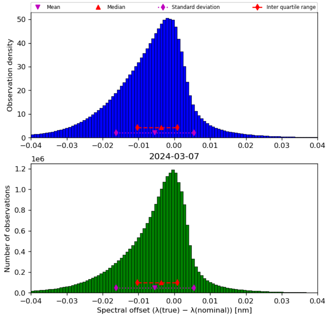
Figure 45: Histogram of “Spectral offset ( \lambda(\text{true}) - \lambda(\text{nominal}) )” for 2024-03-06 to 2024-03-08
