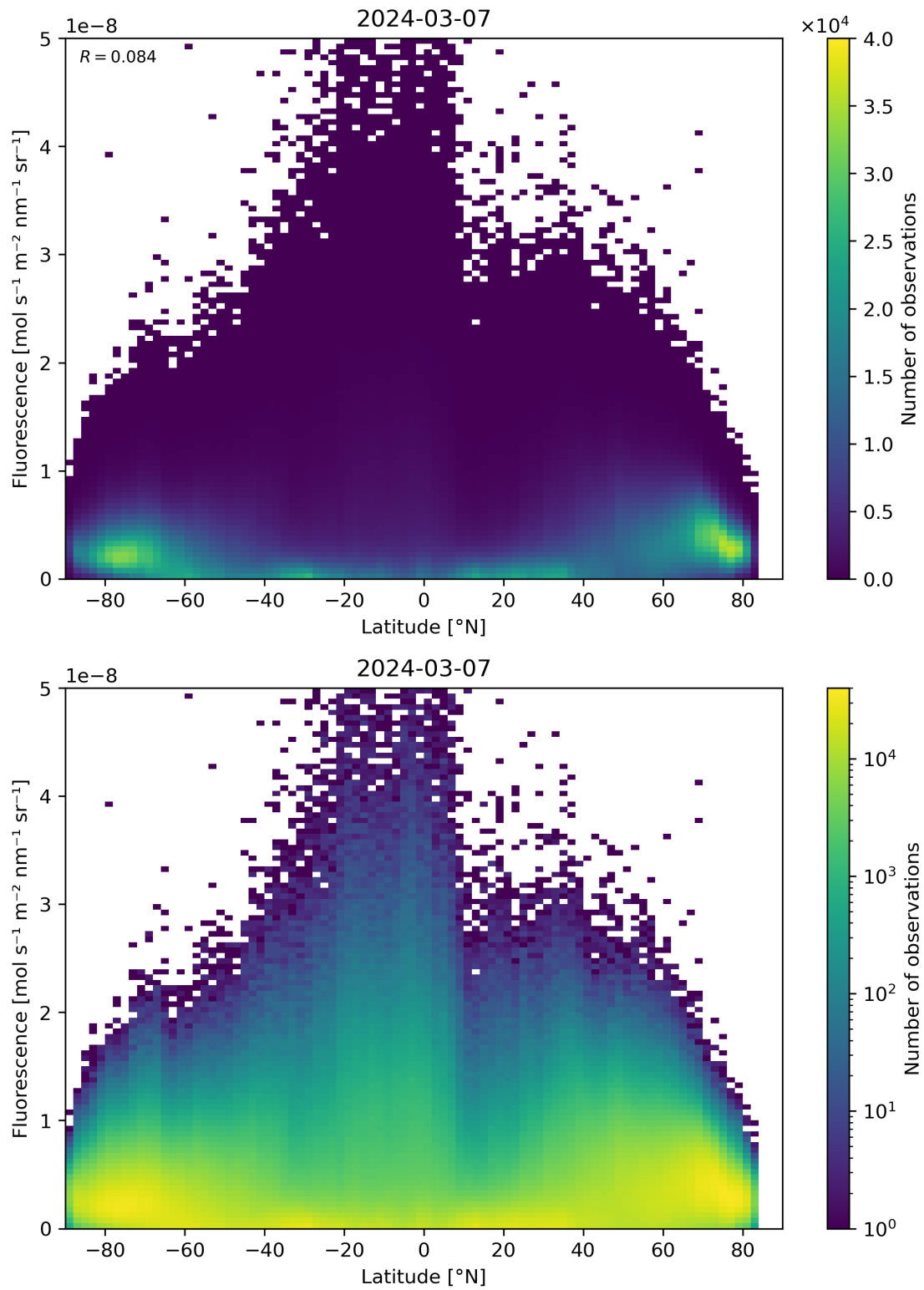
Figure 92: Scatter density plot of “Latitude” against “Fluorescence” for 2024-03-06 to 2024-03-08.
