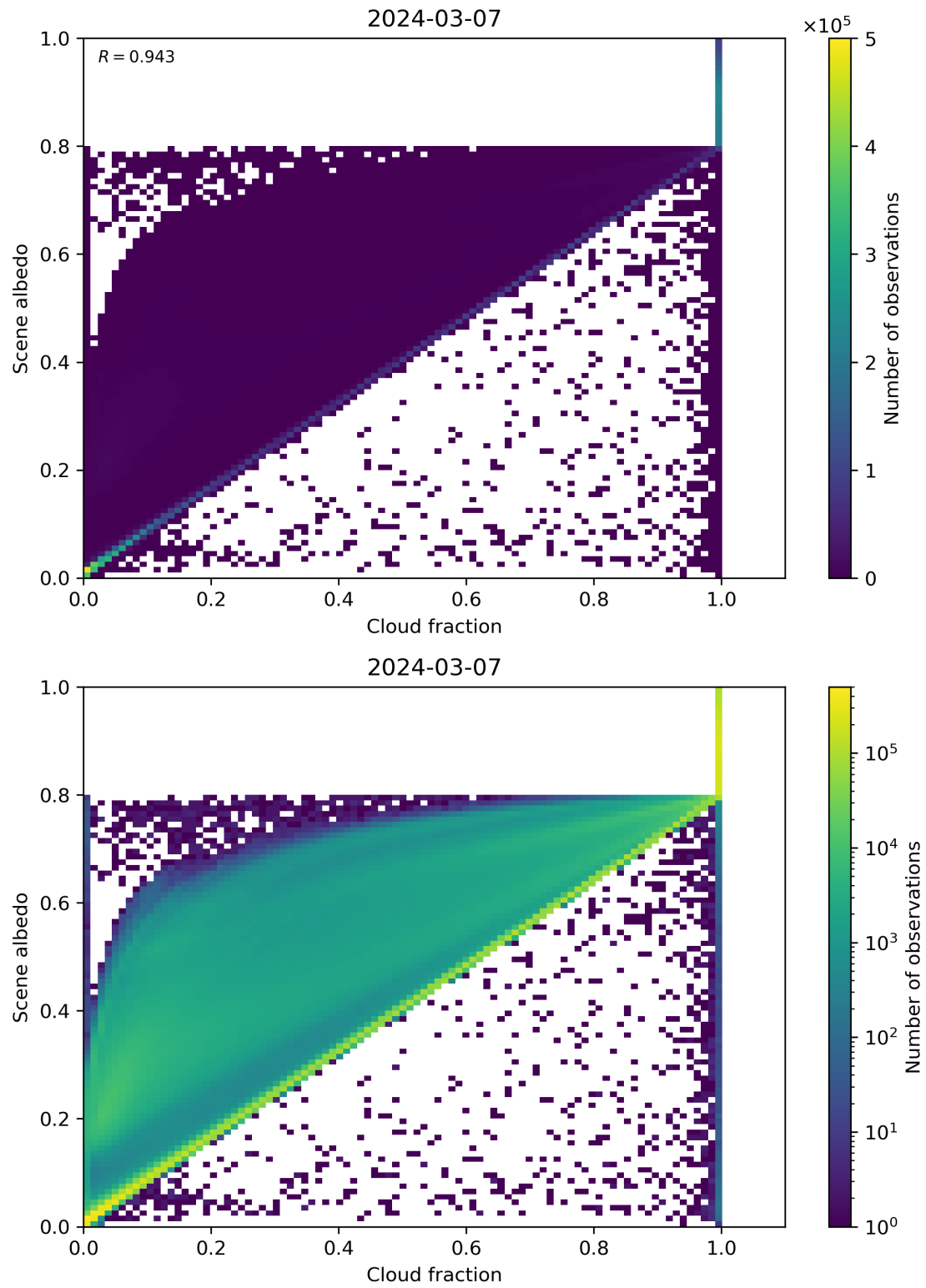
Figure 75: Scatter density plot of “Cloud fraction” against “Scene albedo” for 2024-03-06 to 2024-03-08.
