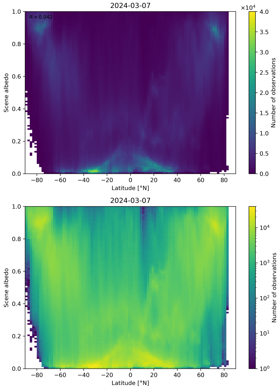
Figure 95: Scatter density plot of “Latitude” against “Scene albedo” for 2024-03-06 to 2024-03-08.
