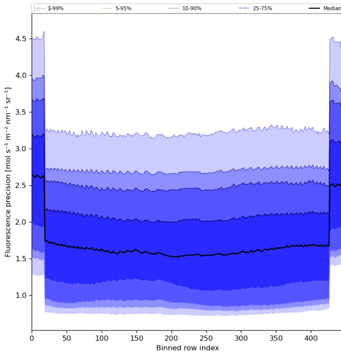
Figure 58: Along track statistics of “Fluorescence precision” for 2024-03-06 to 2024-03-08
