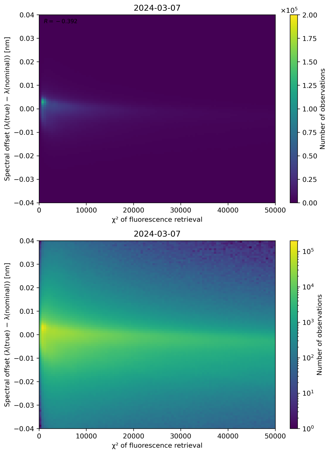
Figure 69: Scatter density plot of “ \chi^2 of fluorescence retrieval” against “Spectral offset ( \lambda(\text{true}) - \lambda(\text{nominal}) )” for 2024-03-06 to 2024-03-08.
