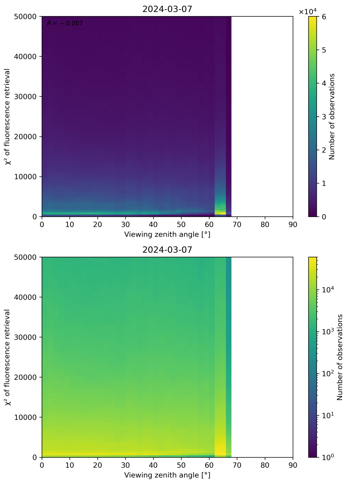
Figure 119: Scatter density plot of “Viewing zenith angle” against “ \chi^2 of fluorescence retrieval” for 2024-03-06 to 2024-03-08.
