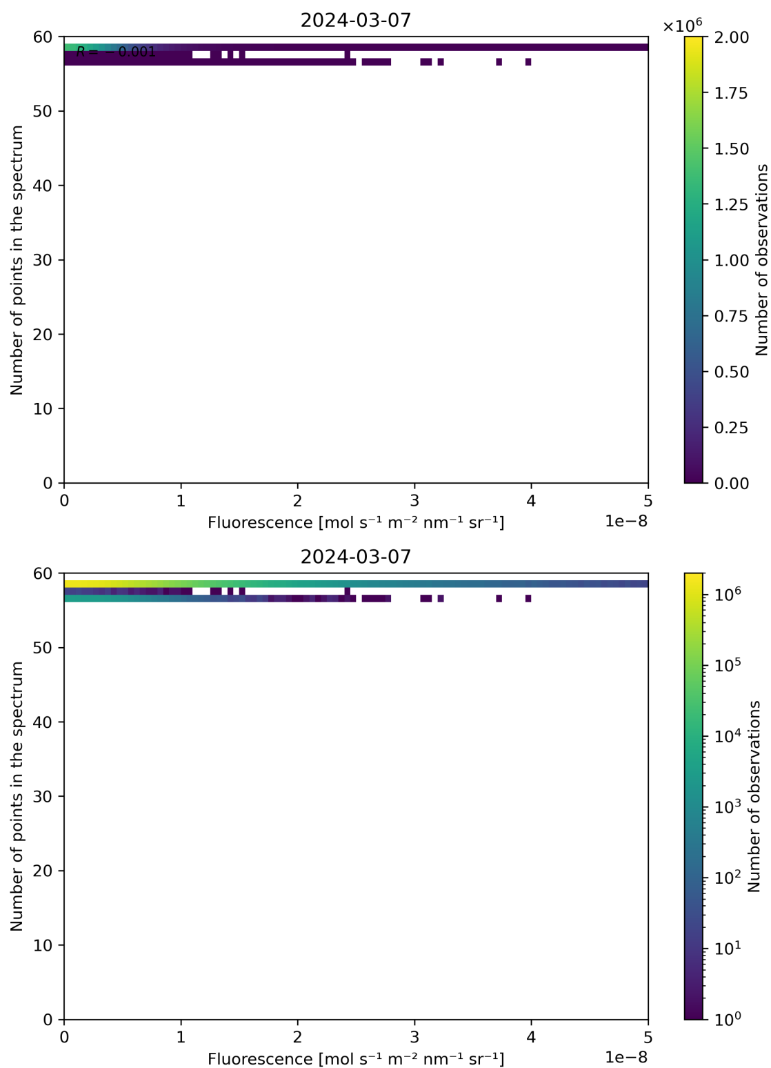
Figure 86: Scatter density plot of “Fluorescence” against “Number of points in the spectrum” for 2024-03-06 to 2024-03-08.
