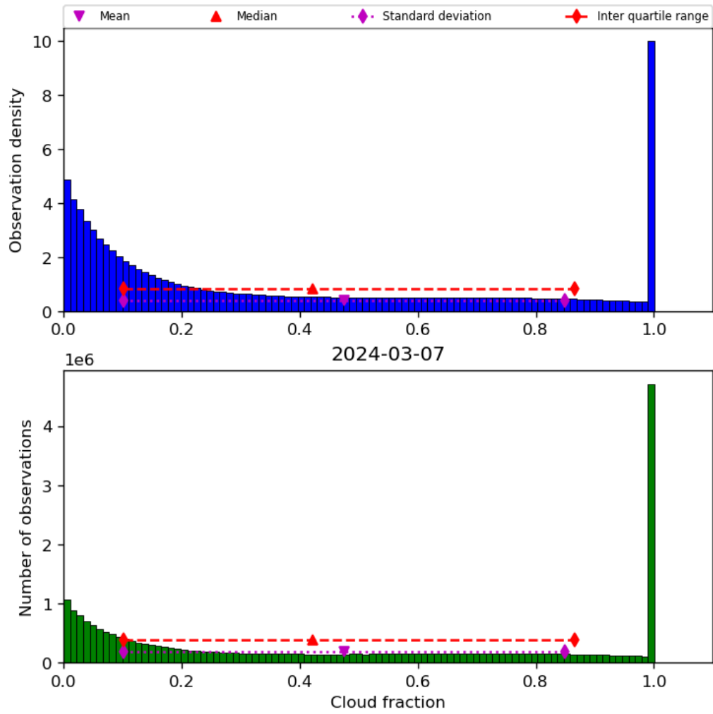
Figure 32: Histogram of “Cloud fraction” for 2024-03-06 to 2024-03-08
