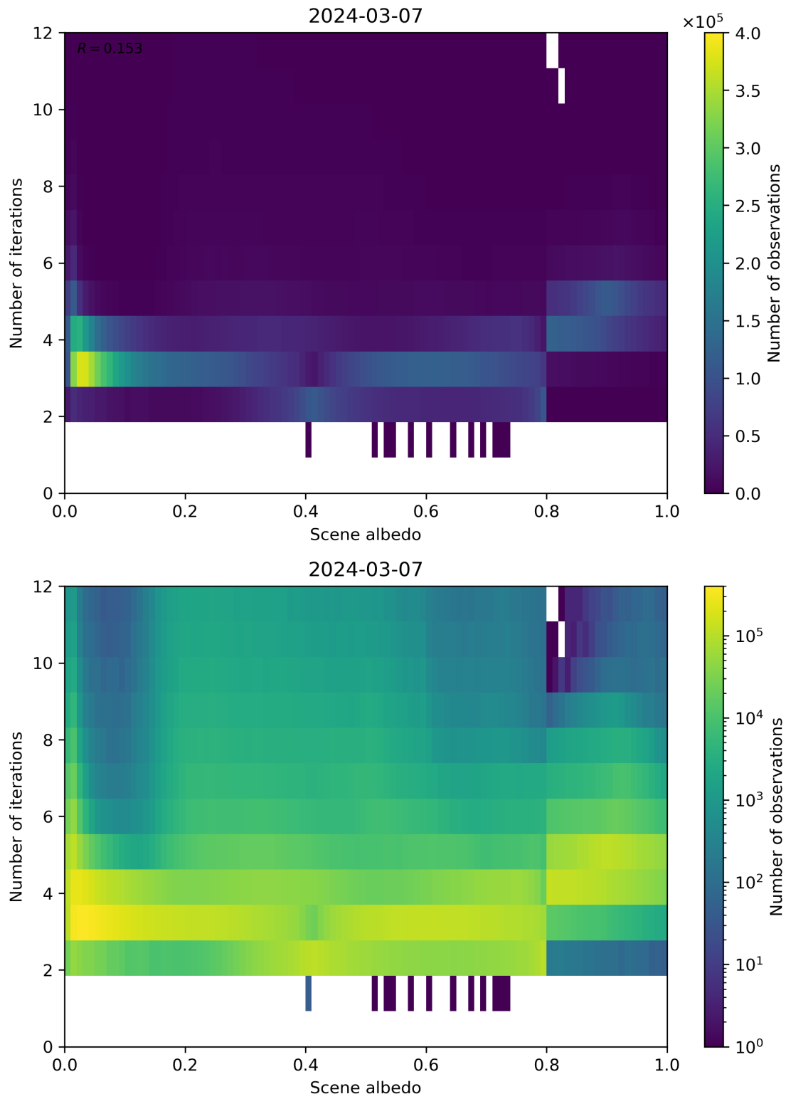
Figure 105: Scatter density plot of “Scene albedo” against “Number of iterations” for 2024-03-06 to 2024-03-08.
