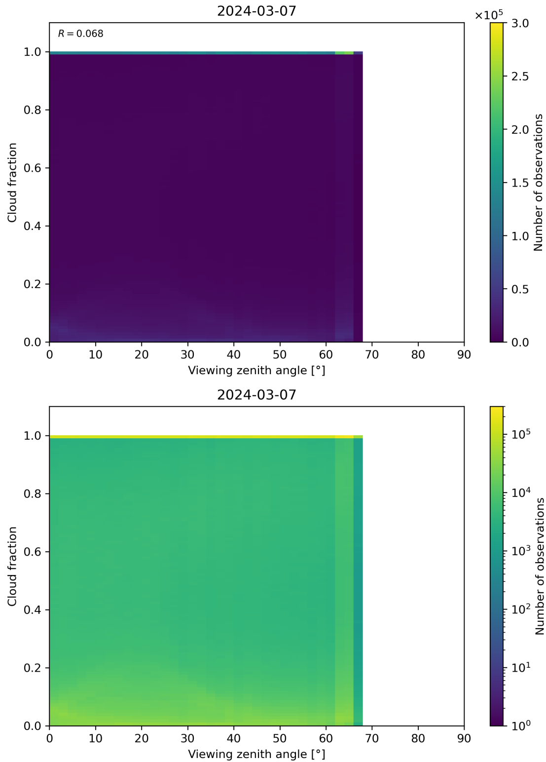
Figure 120: Scatter density plot of “Viewing zenith angle” against “Cloud fraction” for 2024-03-06 to 2024-03-08.
