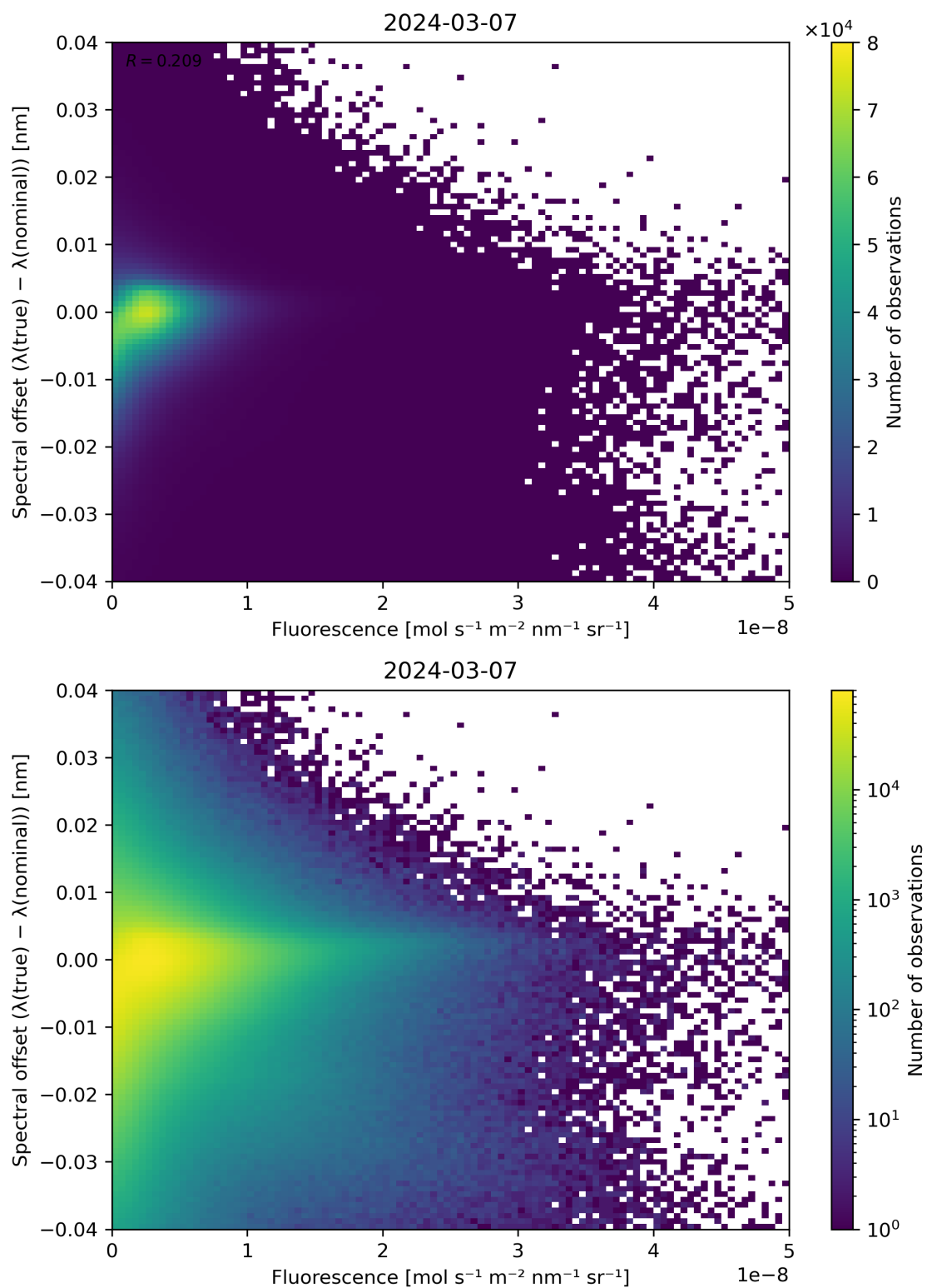
Figure 87: Scatter density plot of “Fluorescence” against “Spectral offset ( \lambda(\text{true}) - \lambda(\text{nominal}) )” for 2024-03-06 to 2024-03-08.
