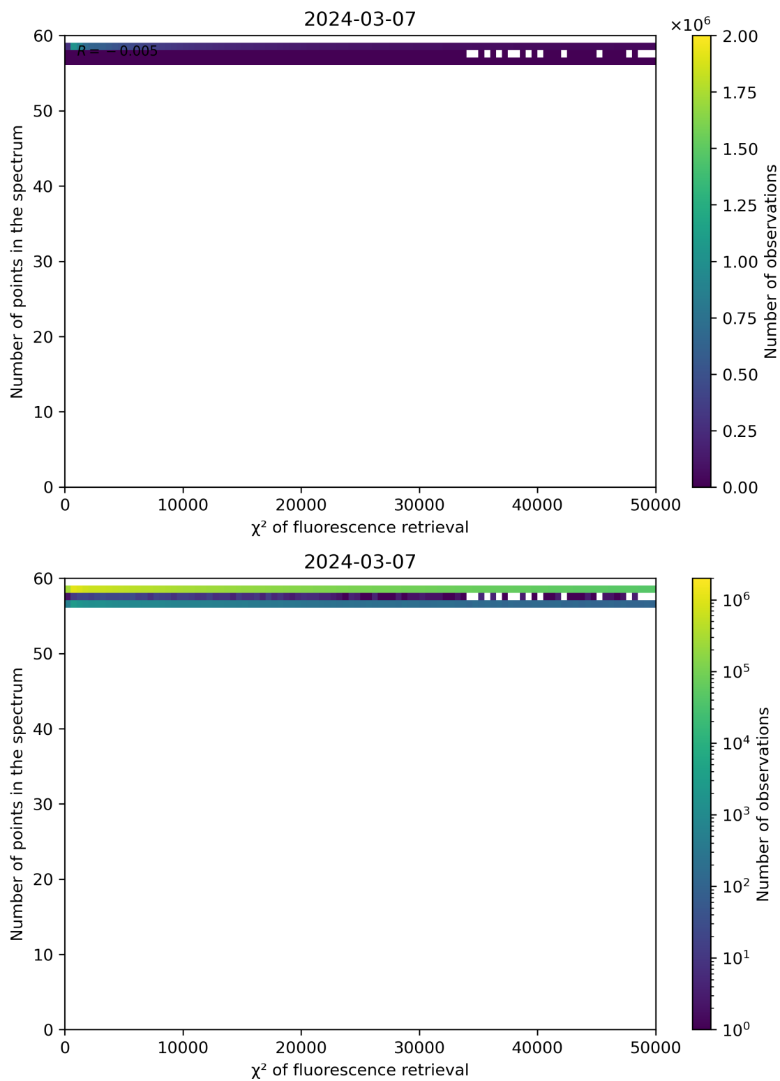
Figure 68: Scatter density plot of “ \chi^2 of fluorescence retrieval” against “Number of points in the spectrum” for 2024-03-06 to 2024-03-08.
