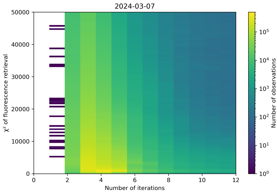
Figure 97: Scatter density plot of “Number of iterations” against “ \chi^2 of fluorescence retrieval” for 2024-03-06 to 2024-03-08.
