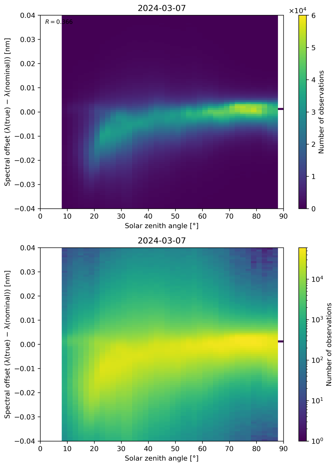
Figure 117: Scatter density plot of “Solar zenith angle” against “Spectral offset ( \lambda(\text{true}) - \lambda(\text{nominal}) )” for 2024-03-06 to 2024-03-08.
