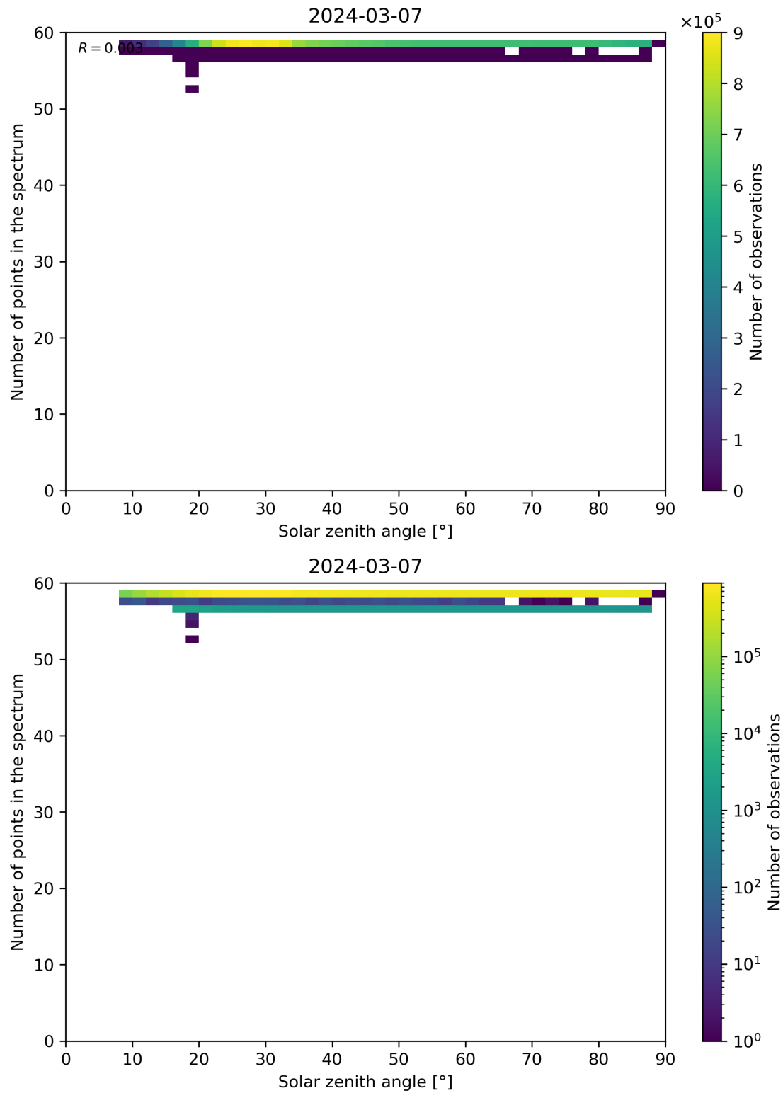
Figure 115: Scatter density plot of “Solar zenith angle” against “Number of points in the spectrum” for 2024-03-06 to 2024-03-08.
