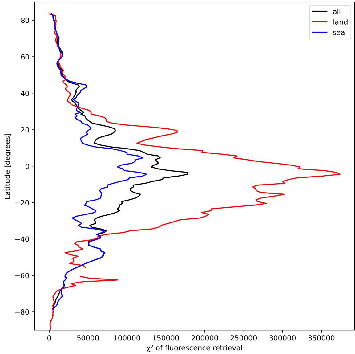
Figure 25: Zonal average of “ \chi^2 of fluorescence retrieval” for 2024-03-06 to 2024-03-08.
