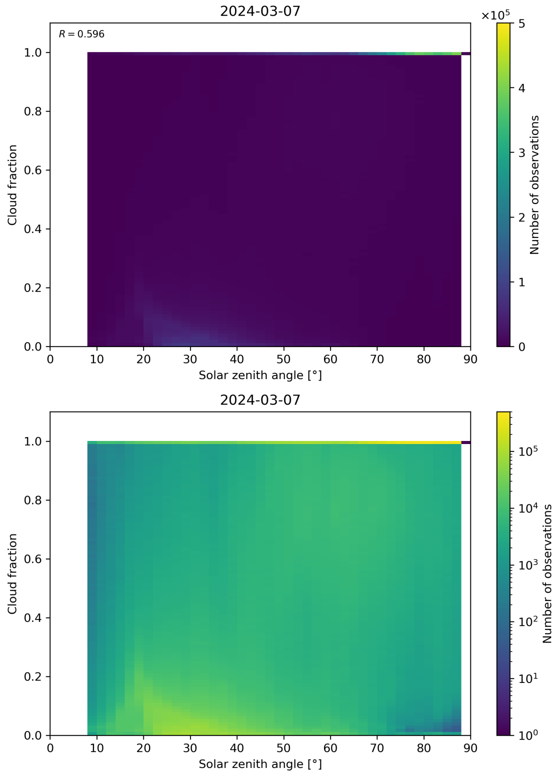
Figure 110: Scatter density plot of “Solar zenith angle” against “Cloud fraction” for 2024-03-06 to 2024-03-08.
