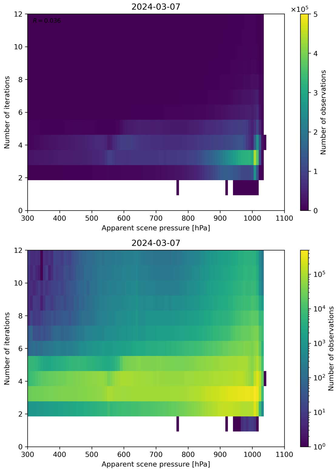
Figure 65: Scatter density plot of “Apparent scene pressure” against “Number of iterations” for 2024-03-06 to 2024-03-08.
