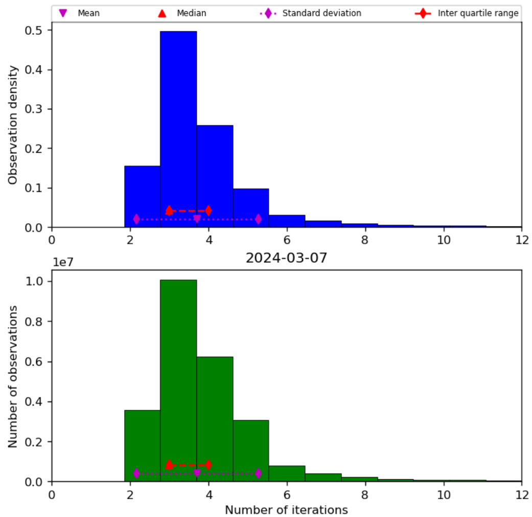
Figure 39: Histogram of “Number of iterations” for 2024-03-06 to 2024-03-08
