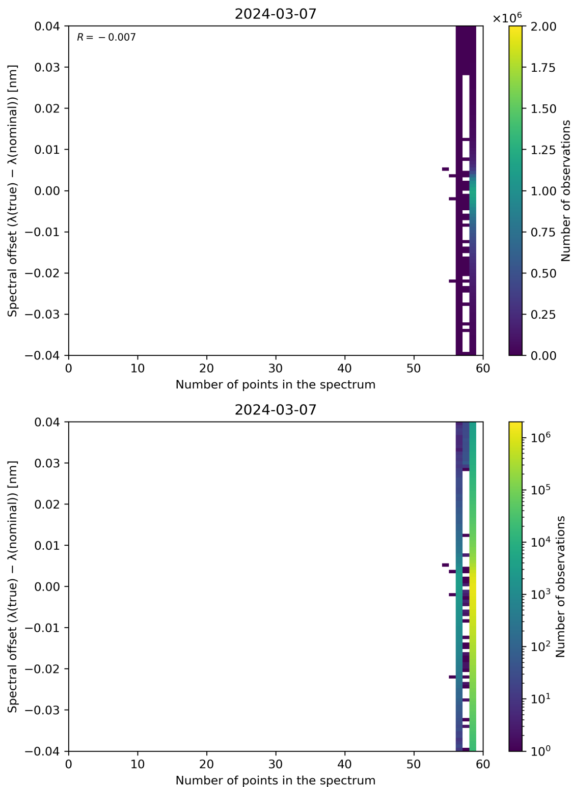
Figure 101: Scatter density plot of “Number of points in the spectrum” against “Spectral offset ( \lambda(\text{true}) - \lambda(\text{nominal}) )” for 2024-03-06 to 2024-03-08.
