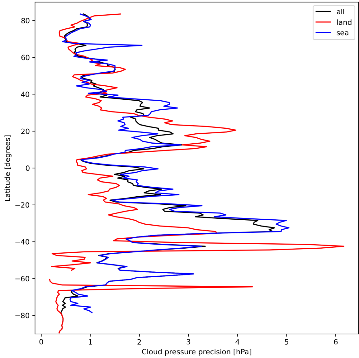
Figure 14: Zonal average of “Cloud pressure precision” for 2024-03-06 to 2024-03-08.
