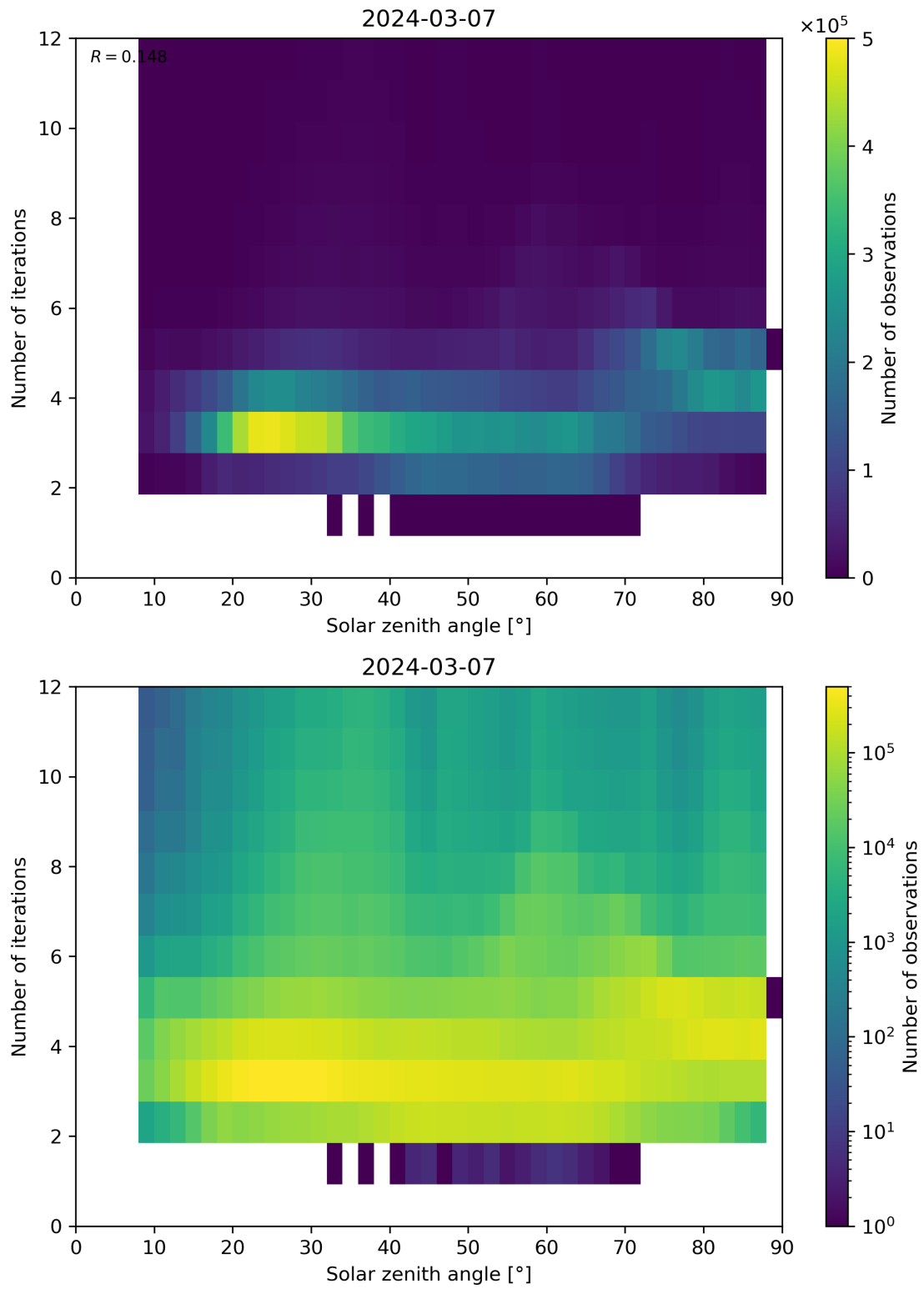
Figure 114: Scatter density plot of “Solar zenith angle” against “Number of iterations” for 2024-03-06 to 2024-03-08.
