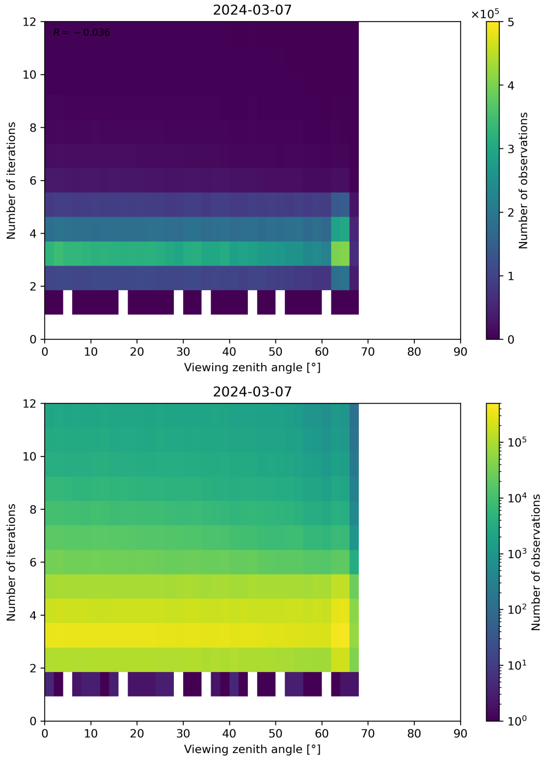
Figure 124: Scatter density plot of “Viewing zenith angle” against “Number of iterations” for 2024-03-06 to 2024-03-08.
