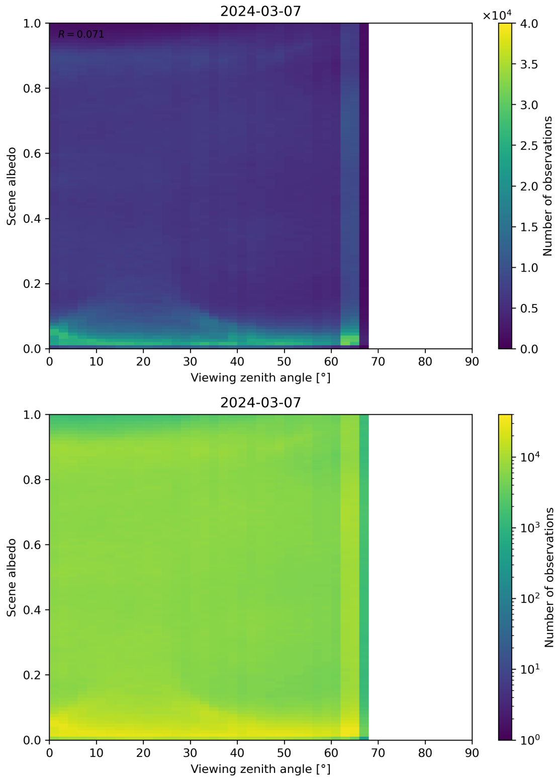
Figure 126: Scatter density plot of “Viewing zenith angle” against “Scene albedo” for 2024-03-06 to 2024-03-08.
