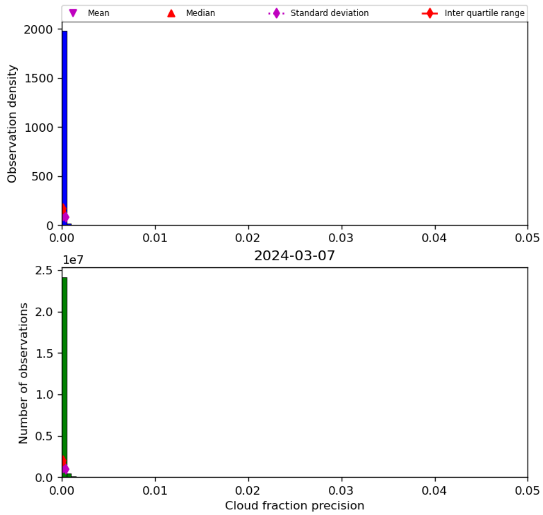
Figure 33: Histogram of “Cloud fraction precision” for 2024-03-06 to 2024-03-08
