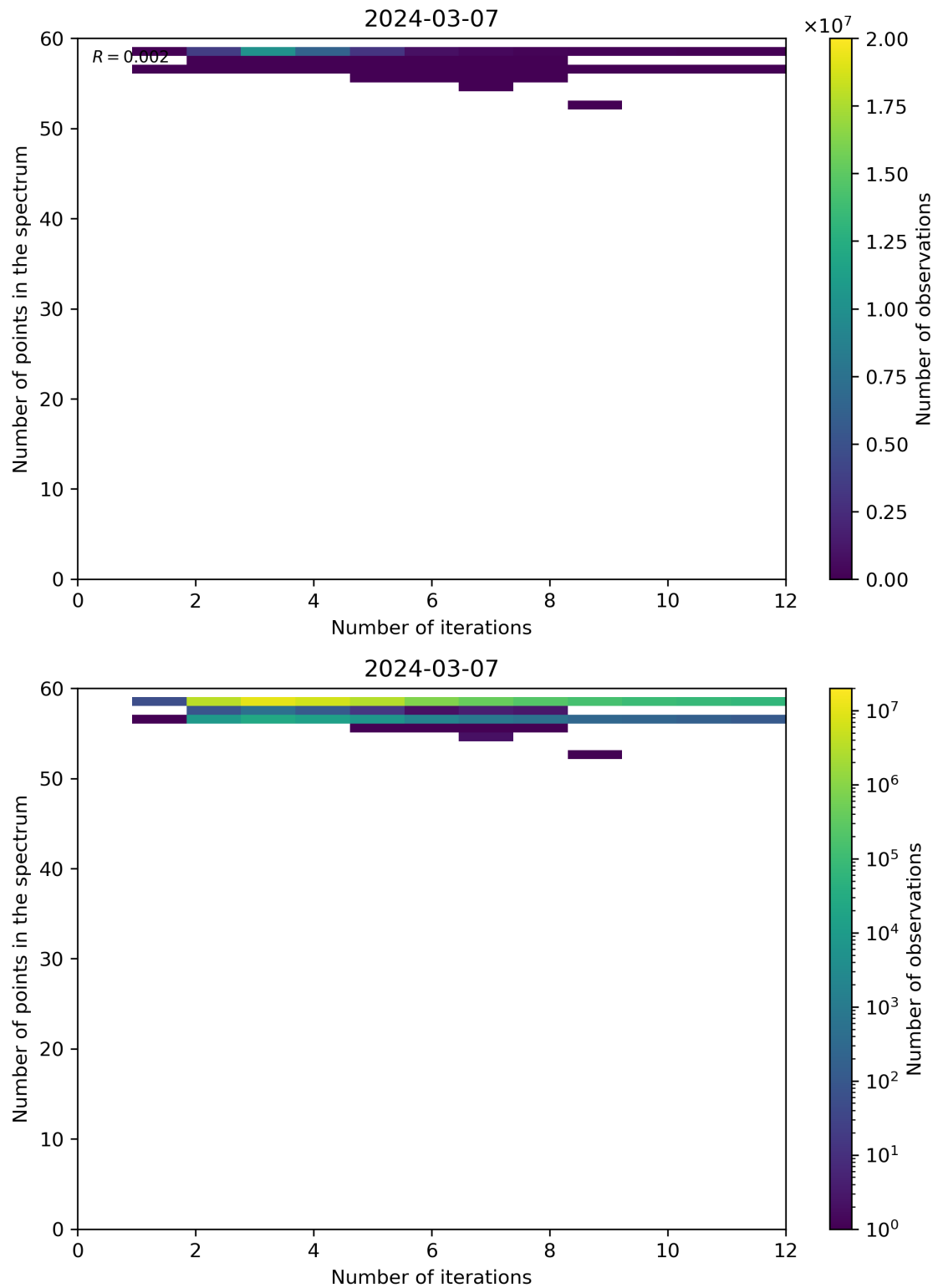
Figure 99: Scatter density plot of “Number of iterations” against “Number of points in the spectrum” for 2024-03-06 to 2024-03-08.
