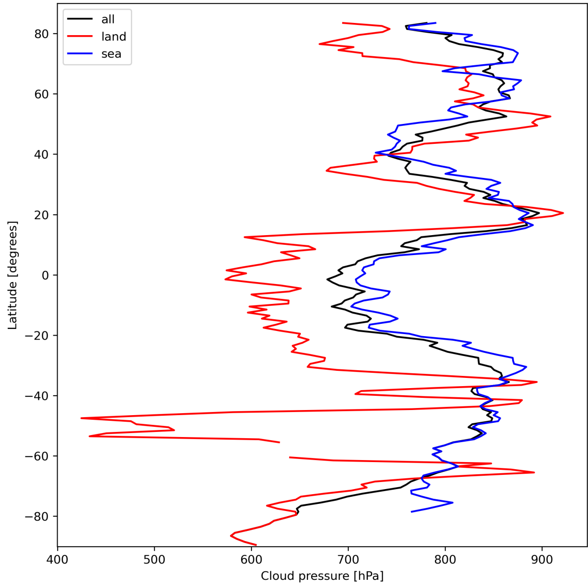
Figure 13: Zonal average of “Cloud pressure” for 2024-03-06 to 2024-03-08.
