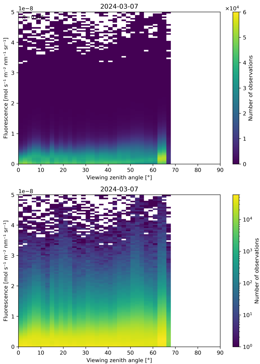
Figure 122: Scatter density plot of “Viewing zenith angle” against “Fluorescence” for 2024-03-06 to 2024-03-08.
