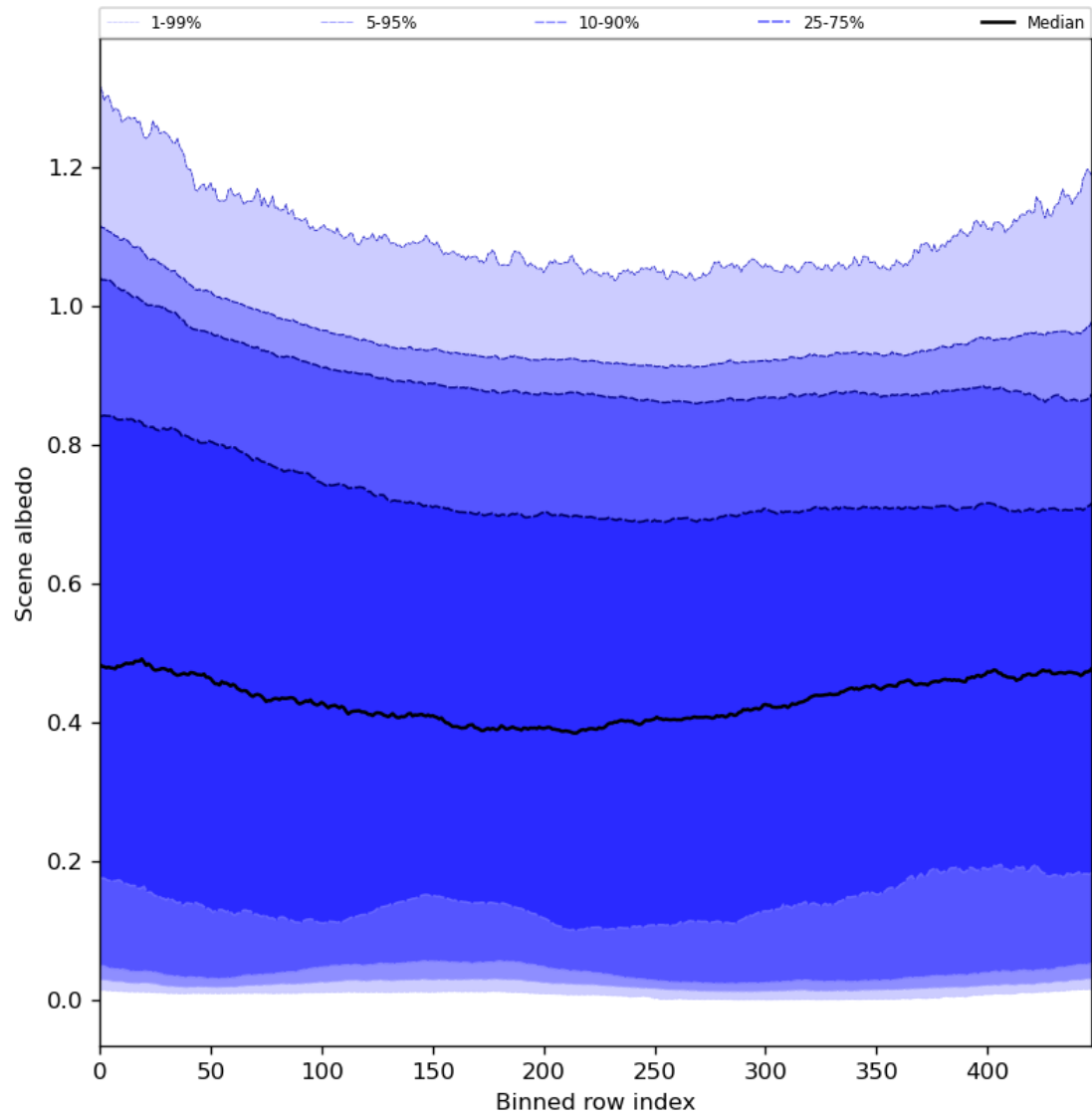
Figure 51: Along track statistics of “Scene albedo” for 2024-03-06 to 2024-03-08
