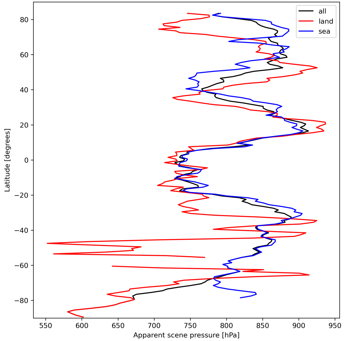
Figure 19: Zonal average of “Apparent scene pressure” for 2024-03-06 to 2024-03-08.
