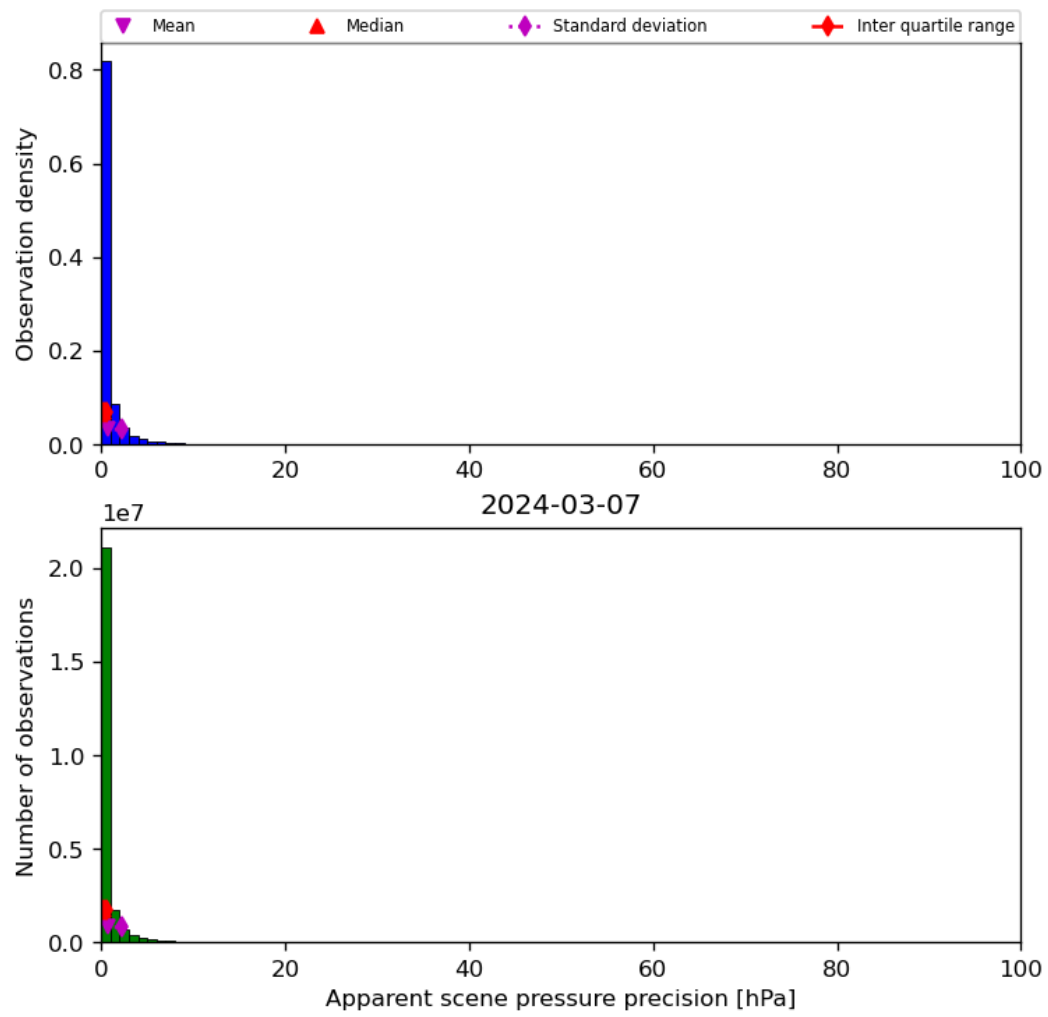
Figure 37: Histogram of “Apparent scene pressure precision” for 2024-03-06 to 2024-03-08
