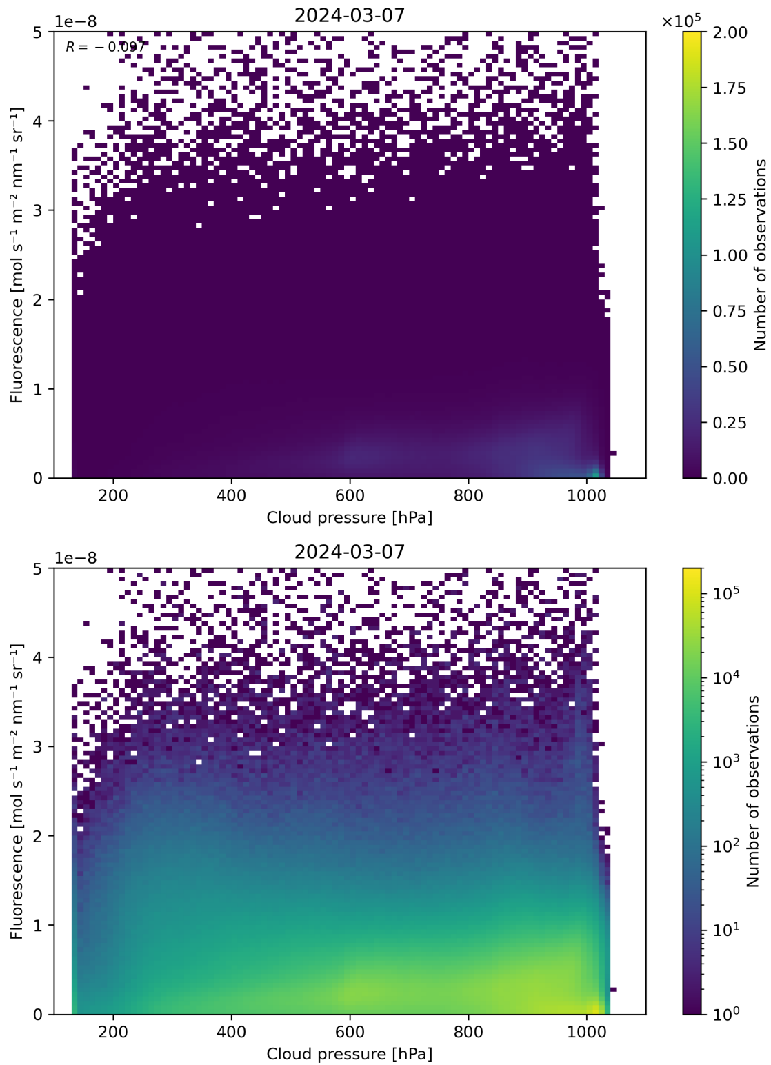
Figure 80: Scatter density plot of “Cloud pressure” against “Fluorescence” for 2024-03-06 to 2024-03-08.
