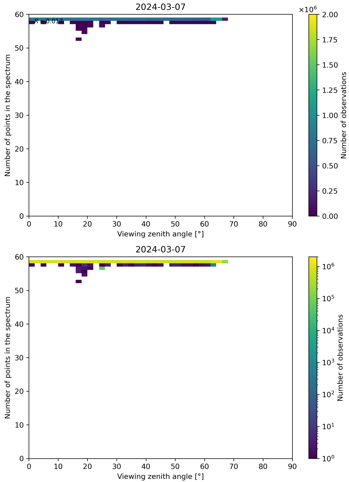
Figure 125: Scatter density plot of “Viewing zenith angle” against “Number of points in the spectrum” for 2024-03-06 to 2024-03-08.
