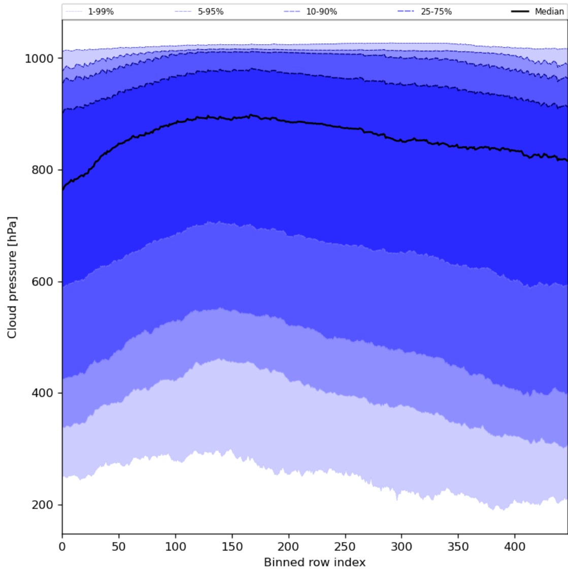
Figure 47: Along track statistics of “Cloud pressure” for 2024-03-06 to 2024-03-08
