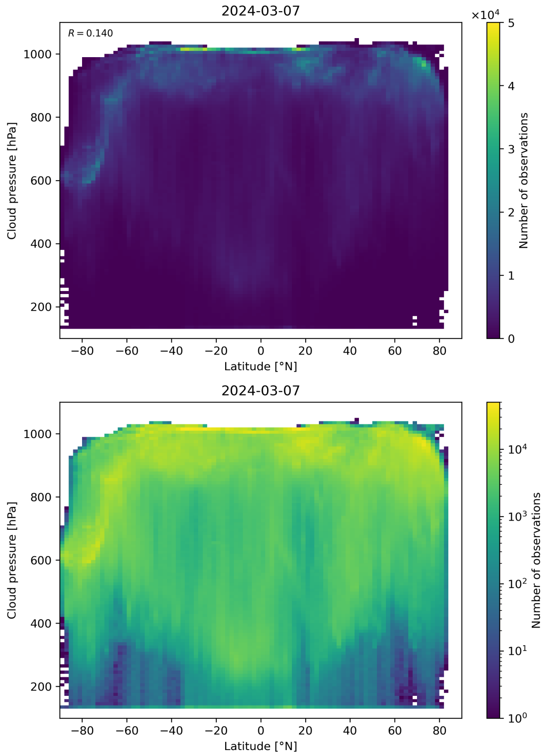
Figure 91: Scatter density plot of “Latitude” against “Cloud pressure” for 2024-03-06 to 2024-03-08.
