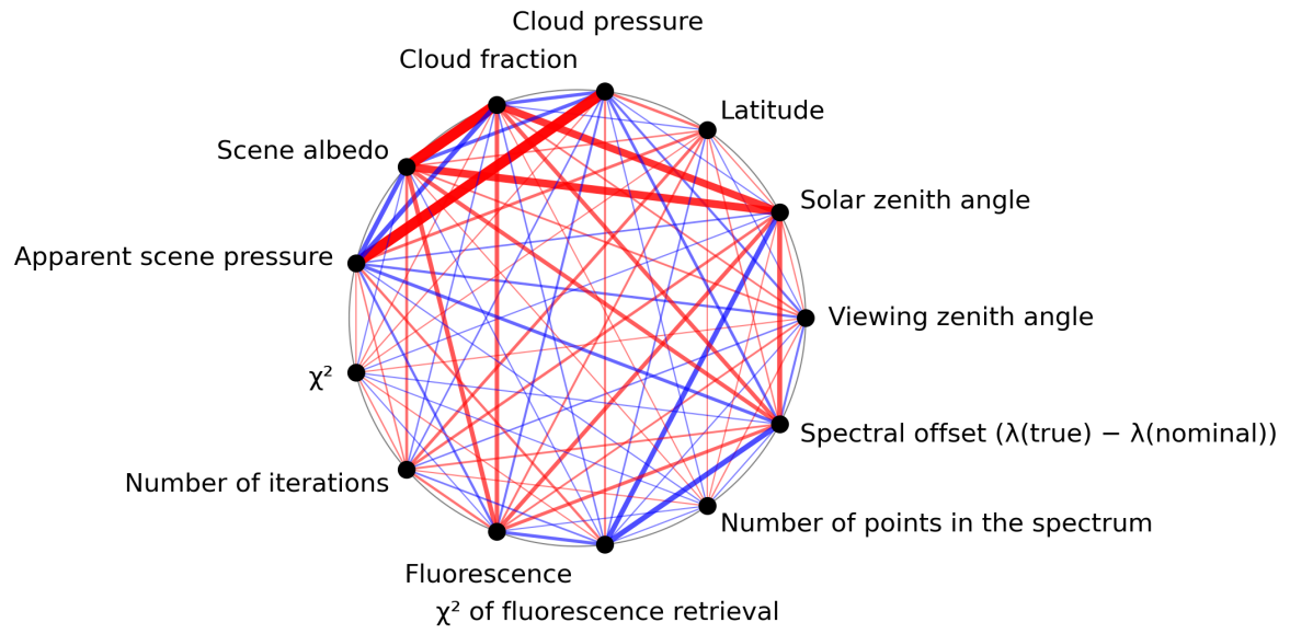
Figure 1: Map of correlation graph for 2024-03-06 to 2024-03-08.
