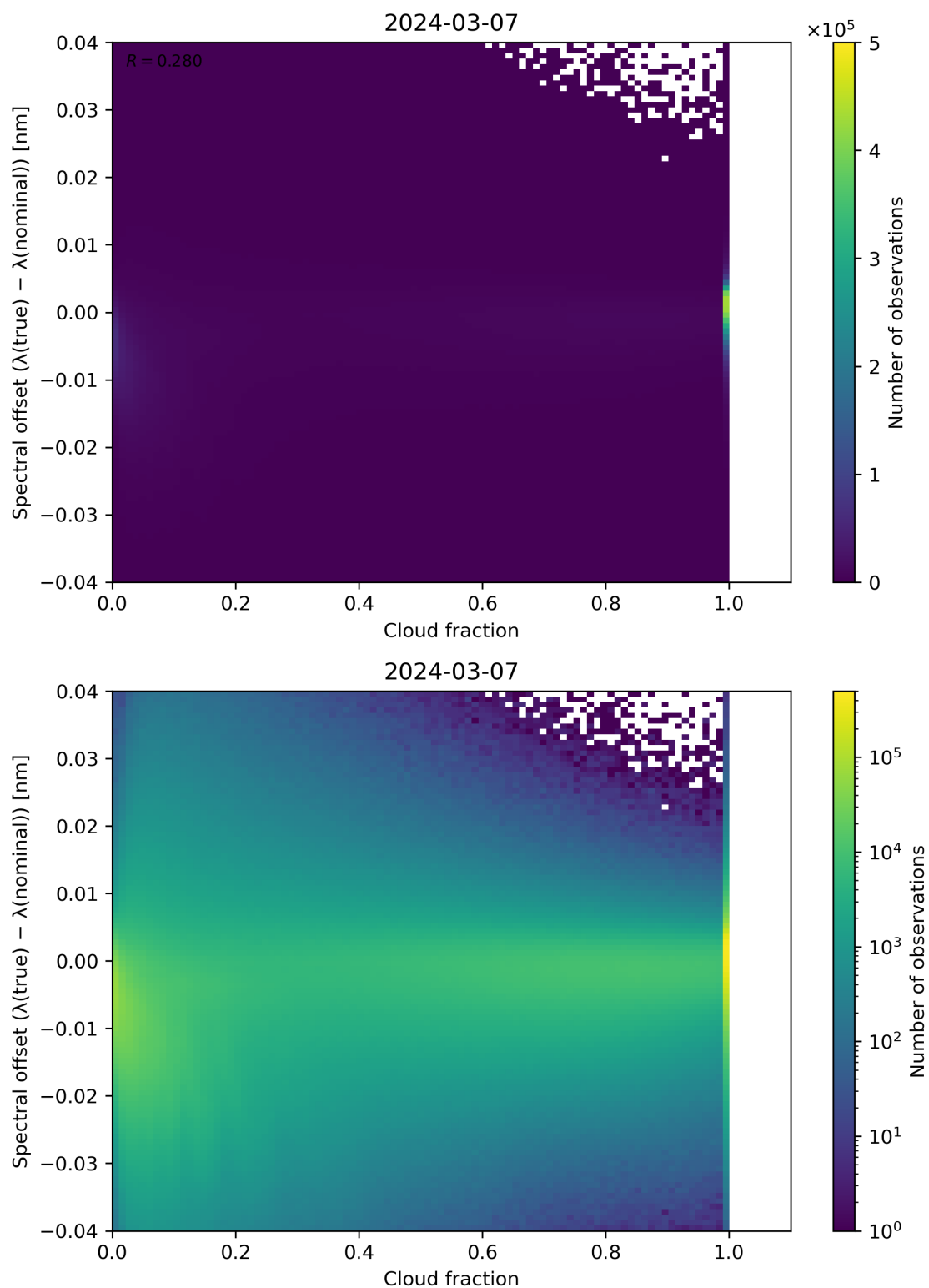
Figure 76: Scatter density plot of “Cloud fraction” against “Spectral offset ( \lambda(\text{true}) - \lambda(\text{nominal}) )” for 2024-03-06 to 2024-03-08.
