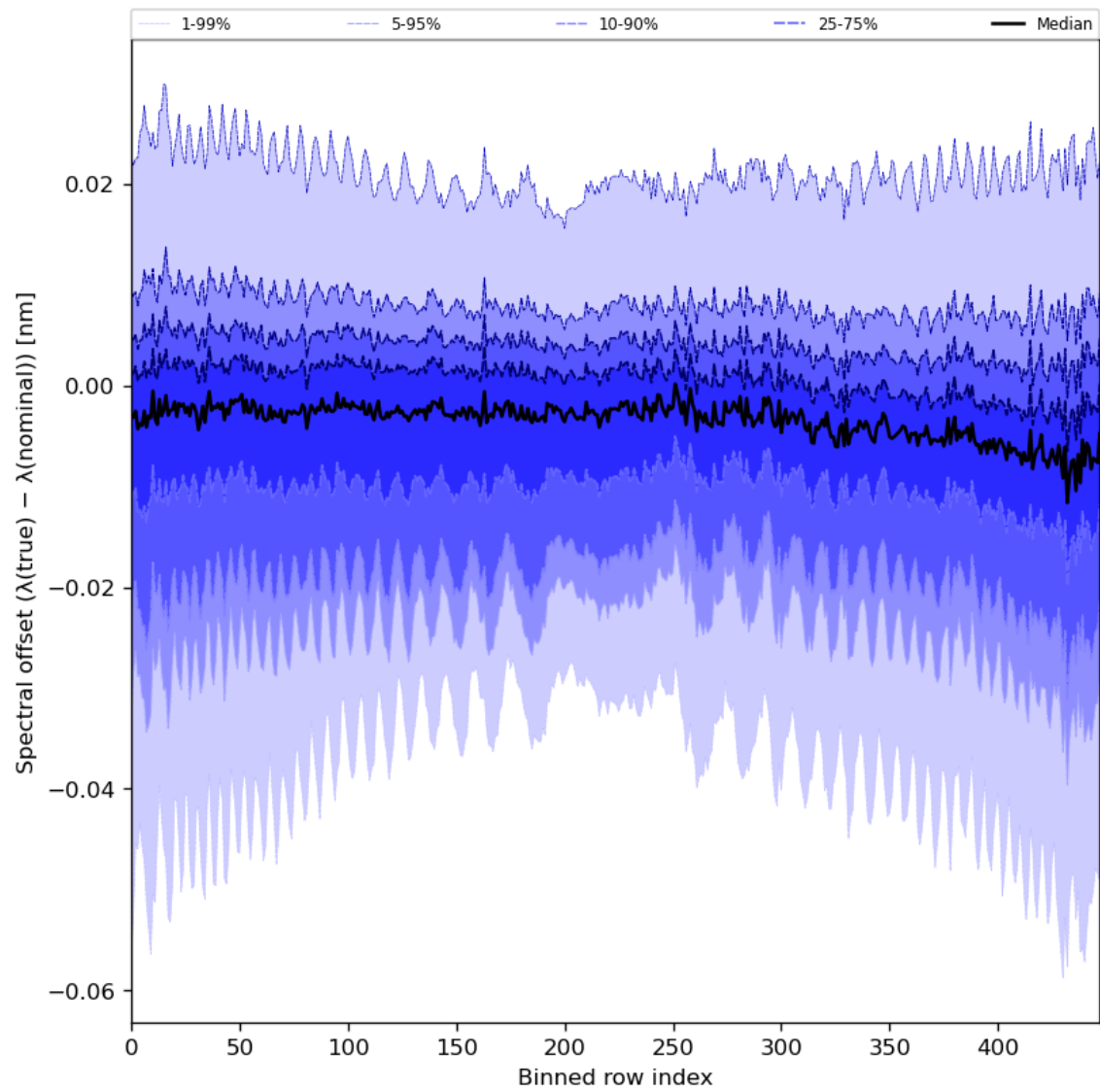
Figure 62: Along track statistics of “Spectral offset ( \lambda(\text{true}) - \lambda(\text{nominal}) )” for 2024-03-06 to 2024-03-08
