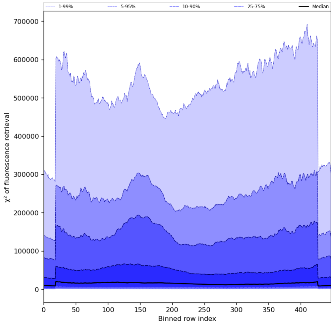
Figure 59: Along track statistics of “ \chi^2 of fluorescence retrieval” for 2024-03-06 to 2024-03-08
