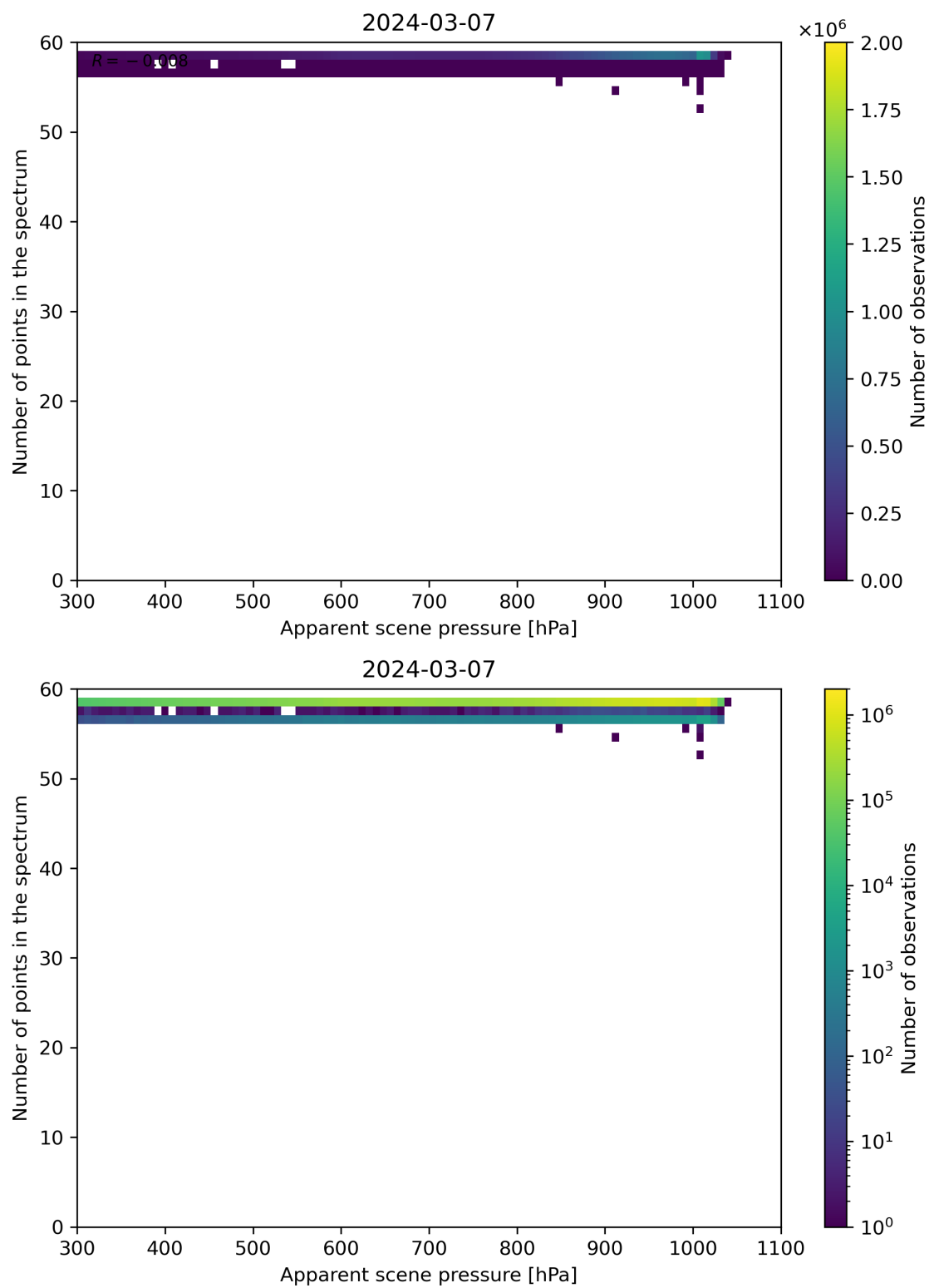
Figure 66: Scatter density plot of “Apparent scene pressure” against “Number of points in the spectrum” for 2024-03-06 to 2024-03-08.
