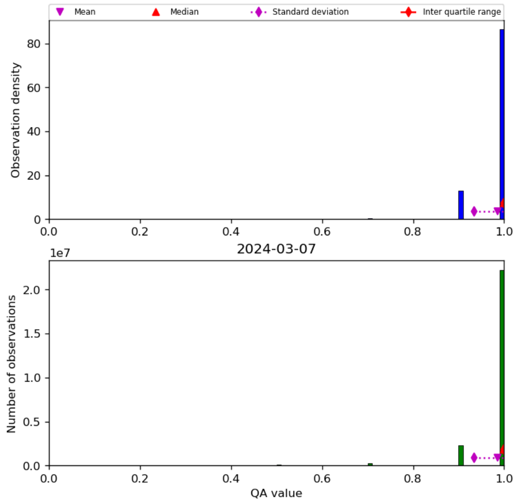
Figure 29: Histogram of “QA value” for 2024-03-06 to 2024-03-08
