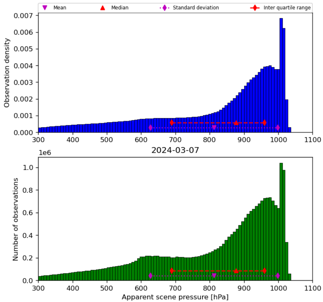
Figure 36: Histogram of “Apparent scene pressure” for 2024-03-06 to 2024-03-08
