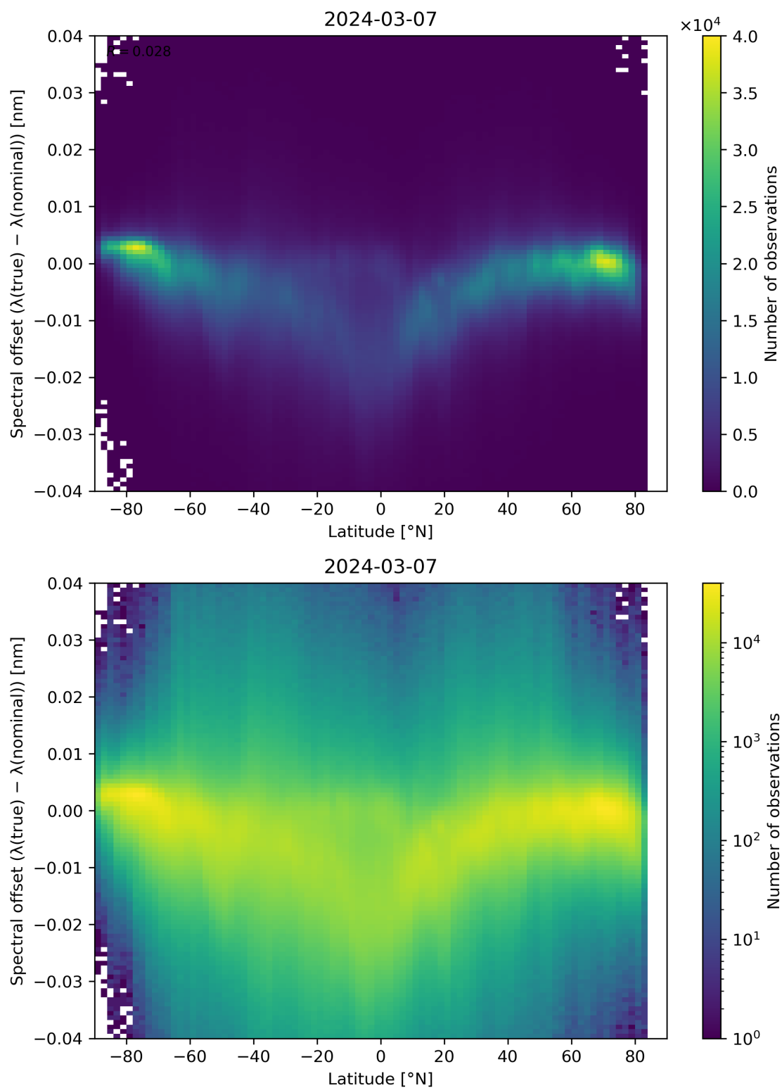
Figure 96: Scatter density plot of “Latitude” against “Spectral offset ( \lambda(\text{true}) - \lambda(\text{nominal}) )” for 2024-03-06 to 2024-03-08.
