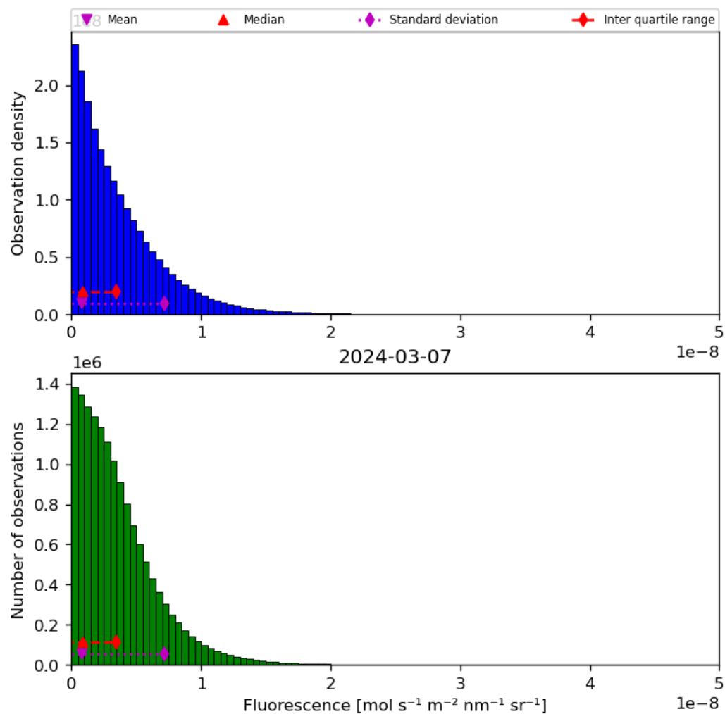
Figure 40: Histogram of “Fluorescence” for 2024-03-06 to 2024-03-08
