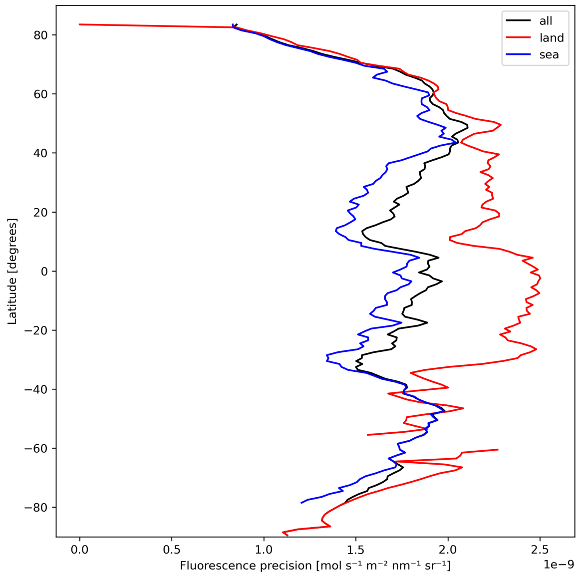
Figure 24: Zonal average of “Fluorescence precision” for 2024-03-06 to 2024-03-08.
