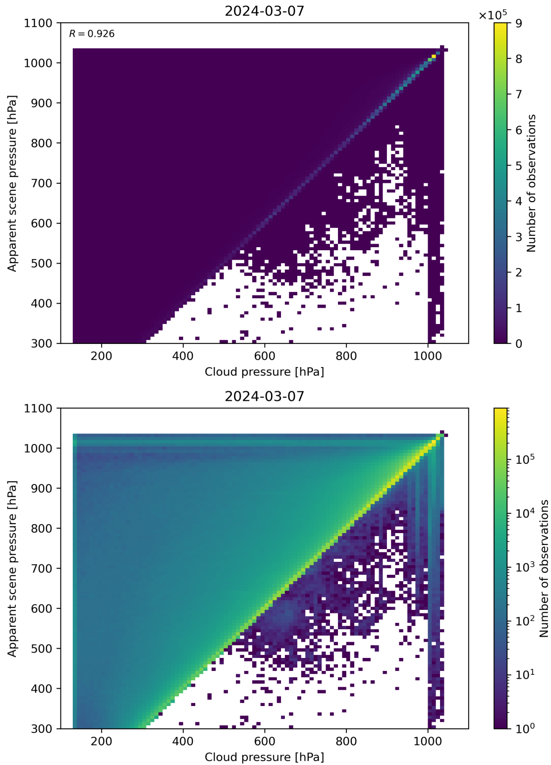
Figure 77: Scatter density plot of “Cloud pressure” against “Apparent scene pressure” for 2024-03-06 to 2024-03-08.
