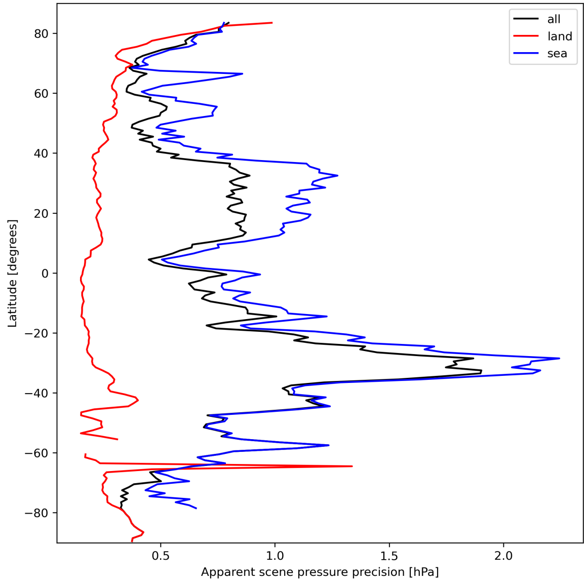
Figure 20: Zonal average of “Apparent scene pressure precision” for 2024-03-06 to 2024-03-08.
