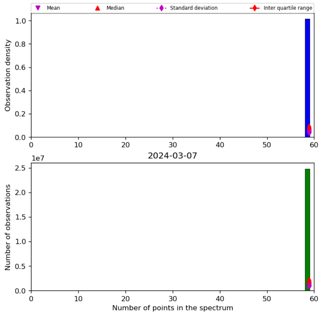
Figure 44: Histogram of “Number of points in the spectrum” for 2024-03-06 to 2024-03-08
