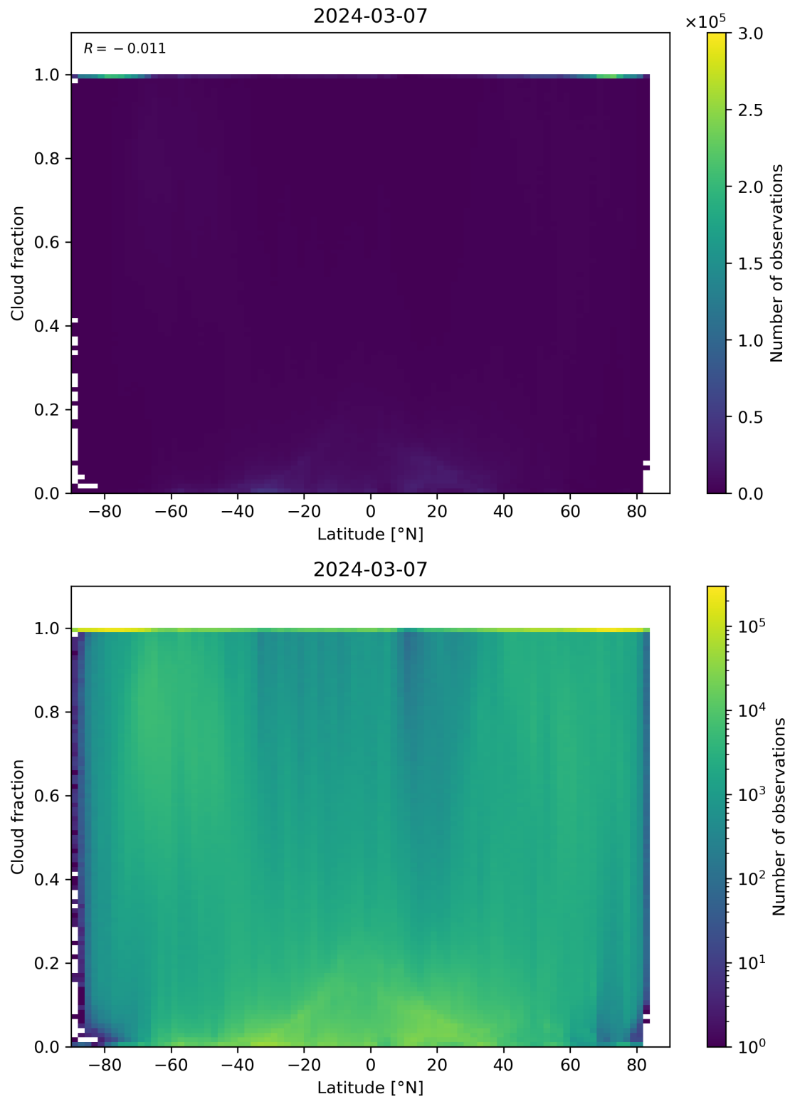
Figure 90: Scatter density plot of “Latitude” against “Cloud fraction” for 2024-03-06 to 2024-03-08.
