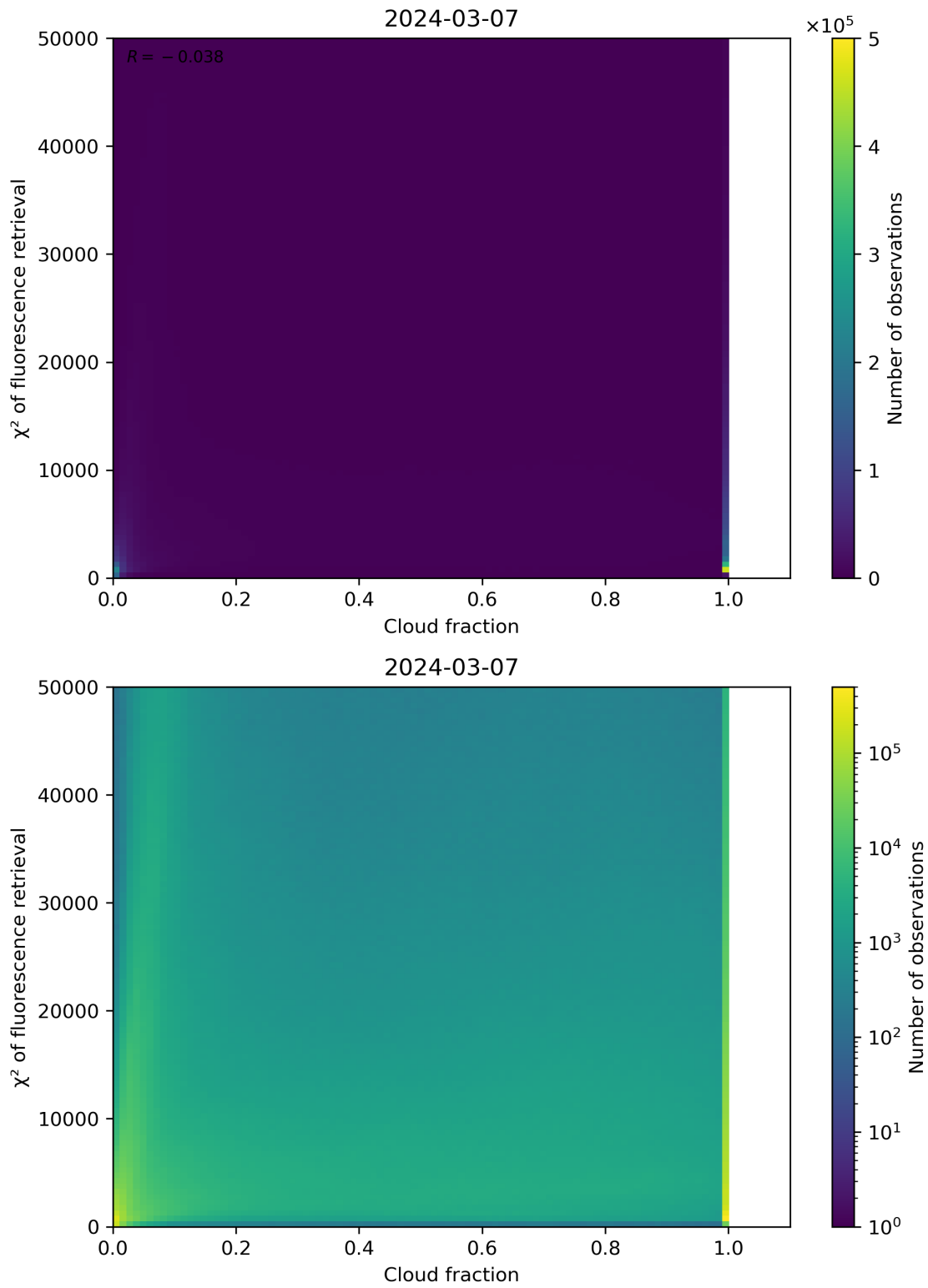
Figure 71: Scatter density plot of “Cloud fraction” against “ \chi^2 of fluorescence retrieval” for 2024-03-06 to 2024-03-08.
