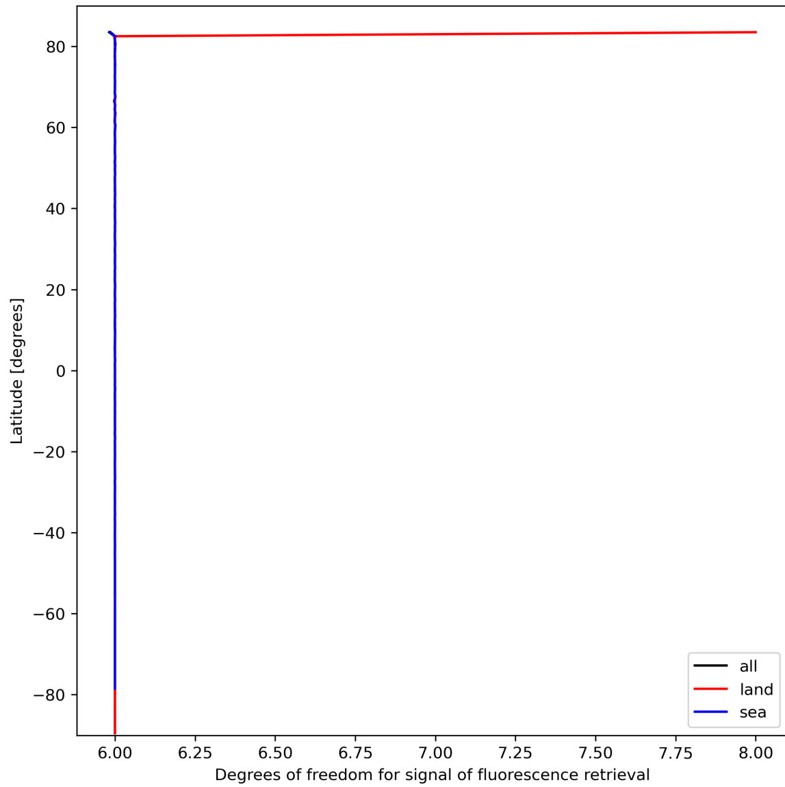
Figure 26: Zonal average of “Degrees of freedom for signal of fluorescence retrieval” for 2024-03-06 to 2024-03-08.
