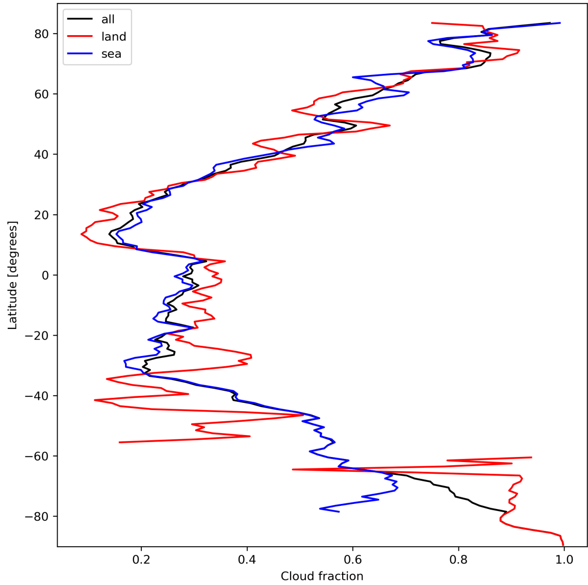
Figure 15: Zonal average of “Cloud fraction” for 2024-03-06 to 2024-03-08.
