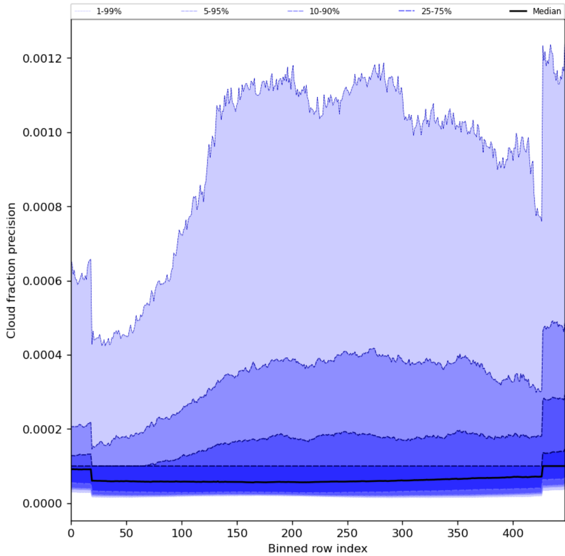
Figure 50: Along track statistics of “Cloud fraction precision” for 2024-03-06 to 2024-03-08
