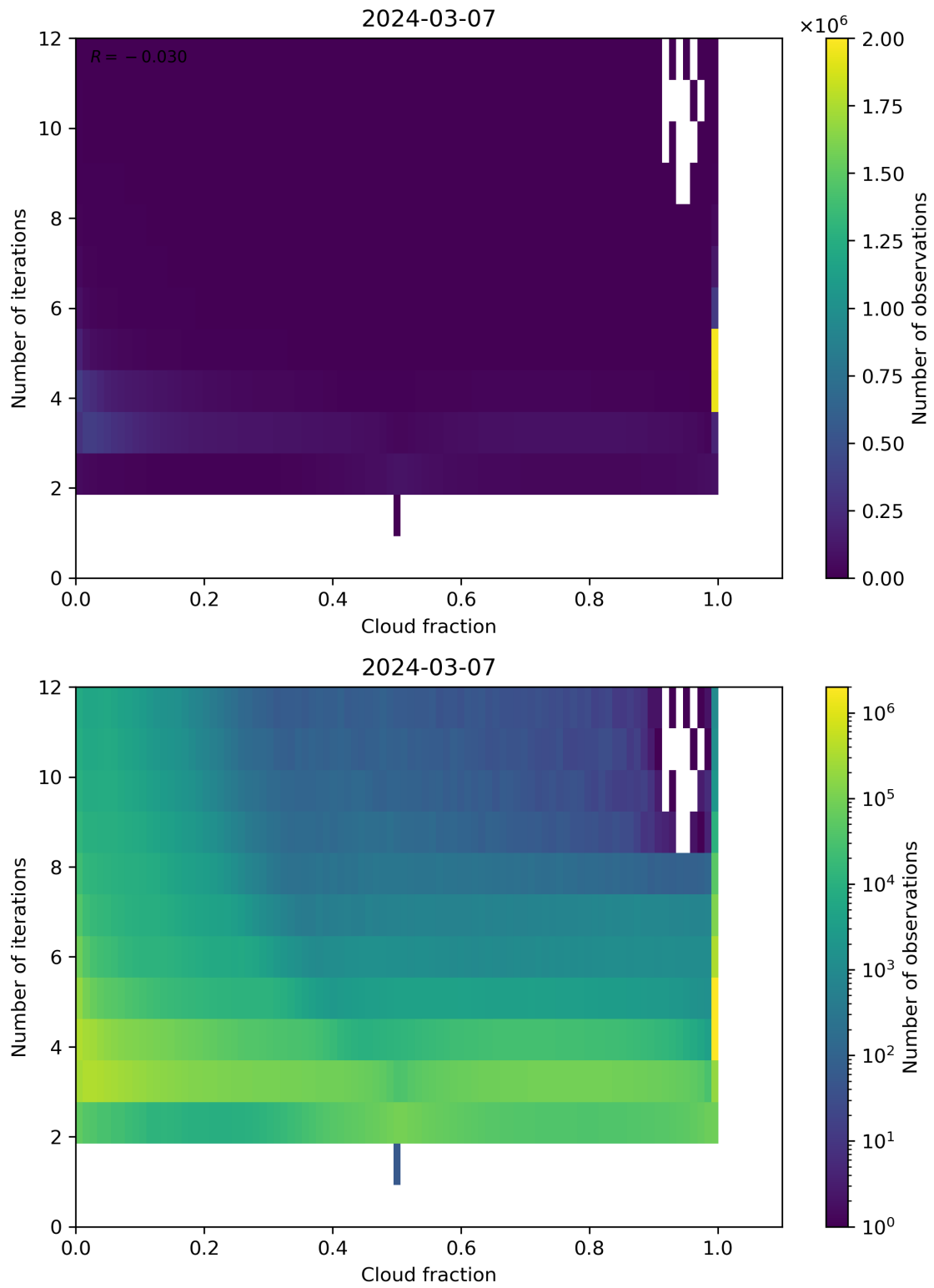
Figure 73: Scatter density plot of “Cloud fraction” against “Number of iterations” for 2024-03-06 to 2024-03-08.
