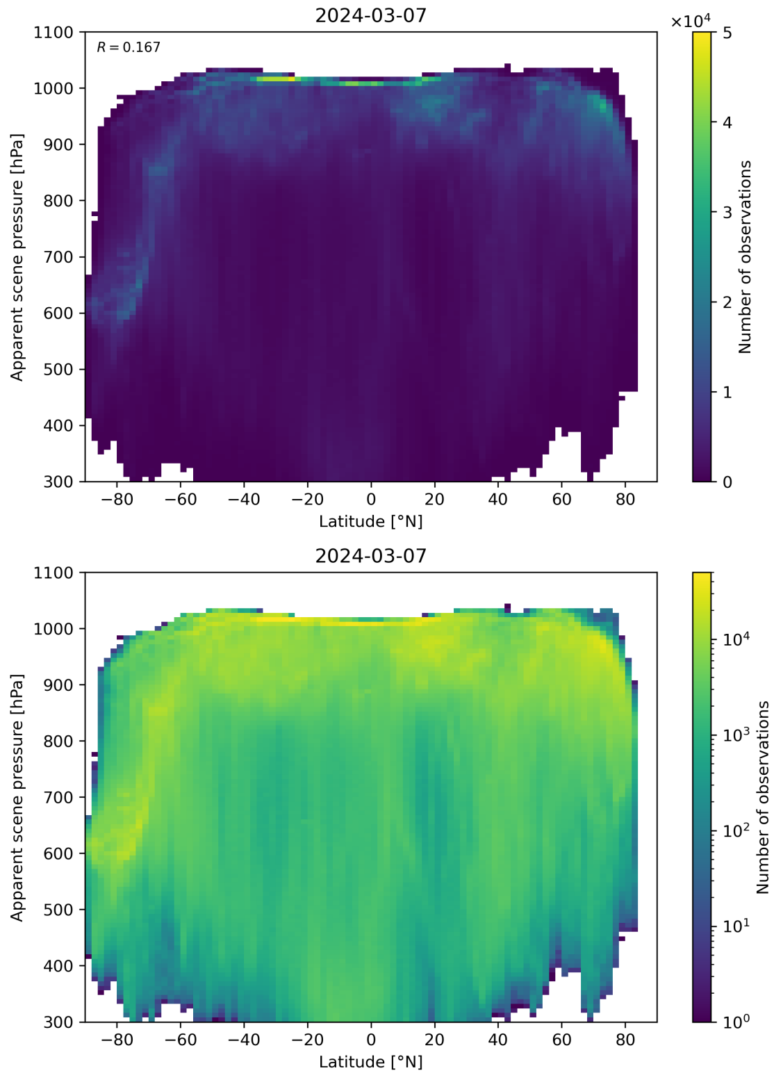
Figure 88: Scatter density plot of “Latitude” against “Apparent scene pressure” for 2024-03-06 to 2024-03-08.
