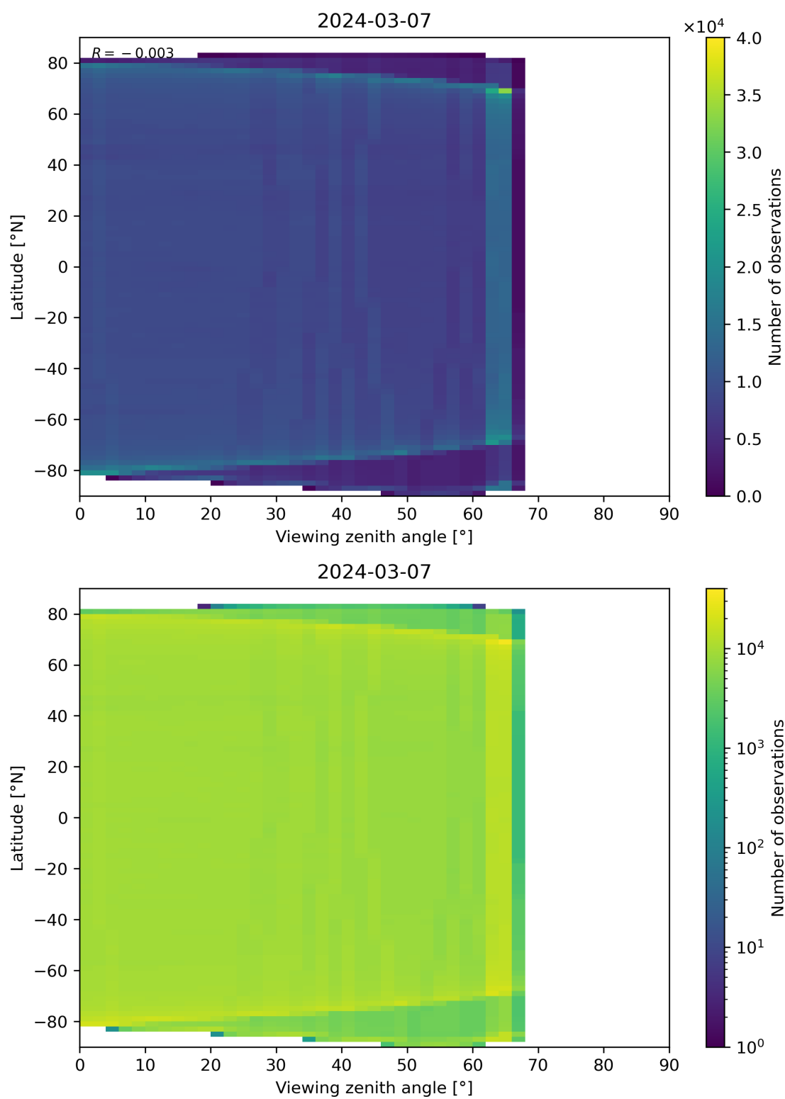
Figure 123: Scatter density plot of “Viewing zenith angle” against “Latitude” for 2024-03-06 to 2024-03-08.
