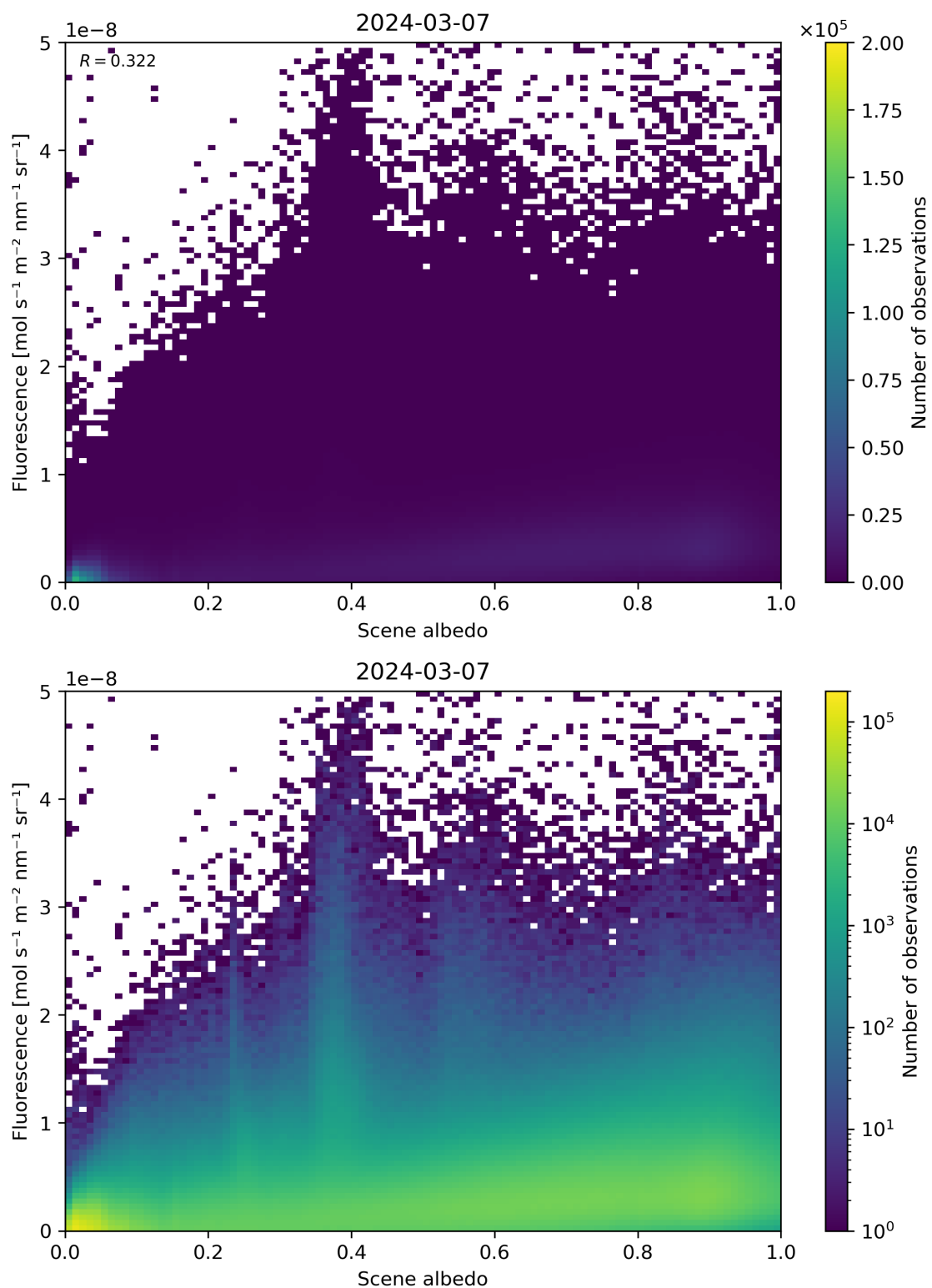
Figure 104: Scatter density plot of “Scene albedo” against “Fluorescence” for 2024-03-06 to 2024-03-08.
