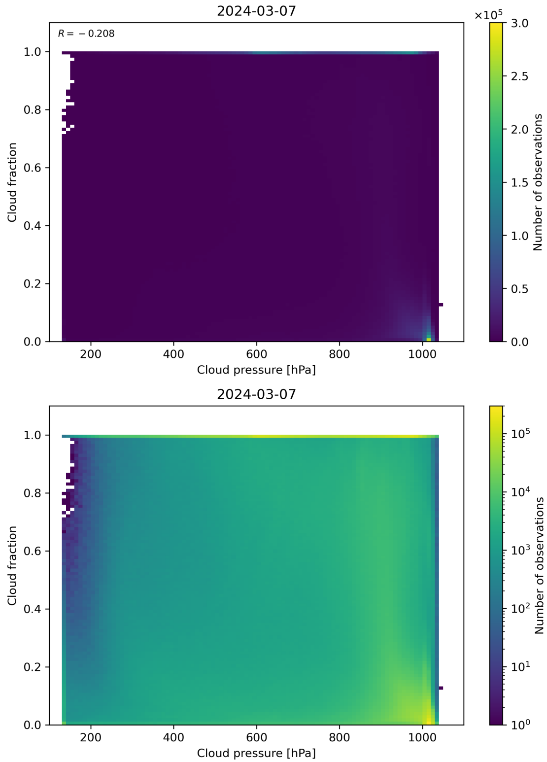
Figure 79: Scatter density plot of “Cloud pressure” against “Cloud fraction” for 2024-03-06 to 2024-03-08.
