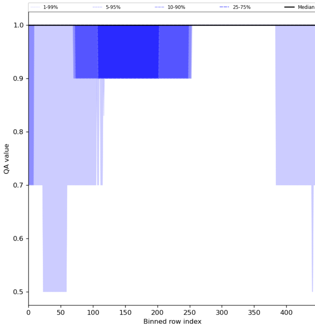
Figure 46: Along track statistics of “QA value” for 2024-03-06 to 2024-03-08
