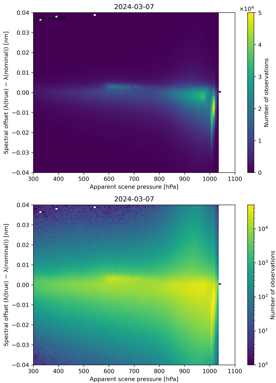
Figure 67: Scatter density plot of “Apparent scene pressure” against “Spectral offset ( \lambda(\text{true}) - \lambda(\text{nominal}) )” for 2024-03-06 to 2024-03-08.
