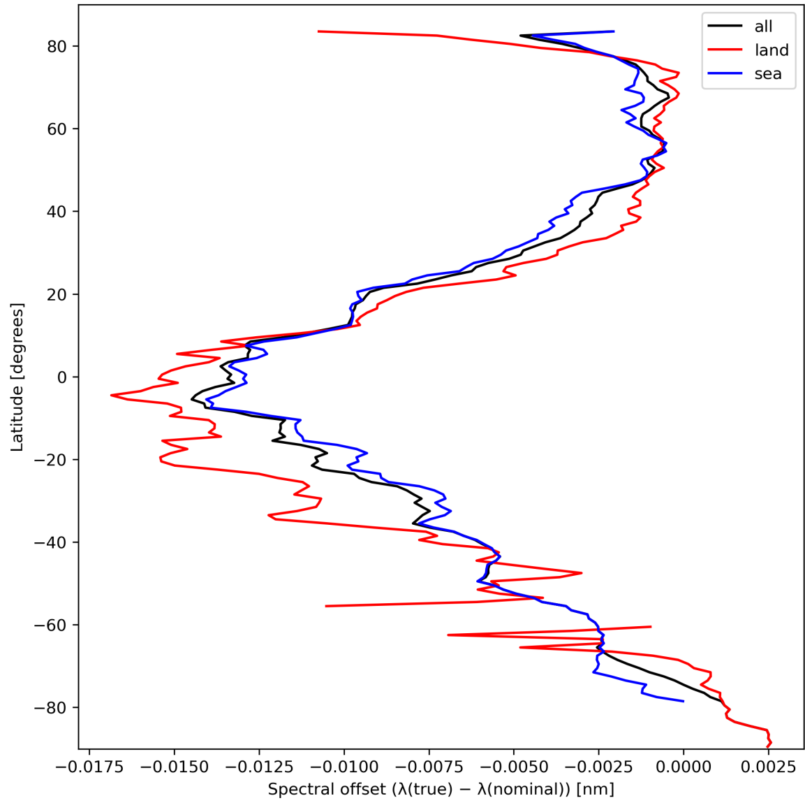
Figure 28: Zonal average of “Spectral offset ( \lambda(\text{true}) - \lambda(\text{nominal}) )” for 2024-03-06 to 2024-03-08.
