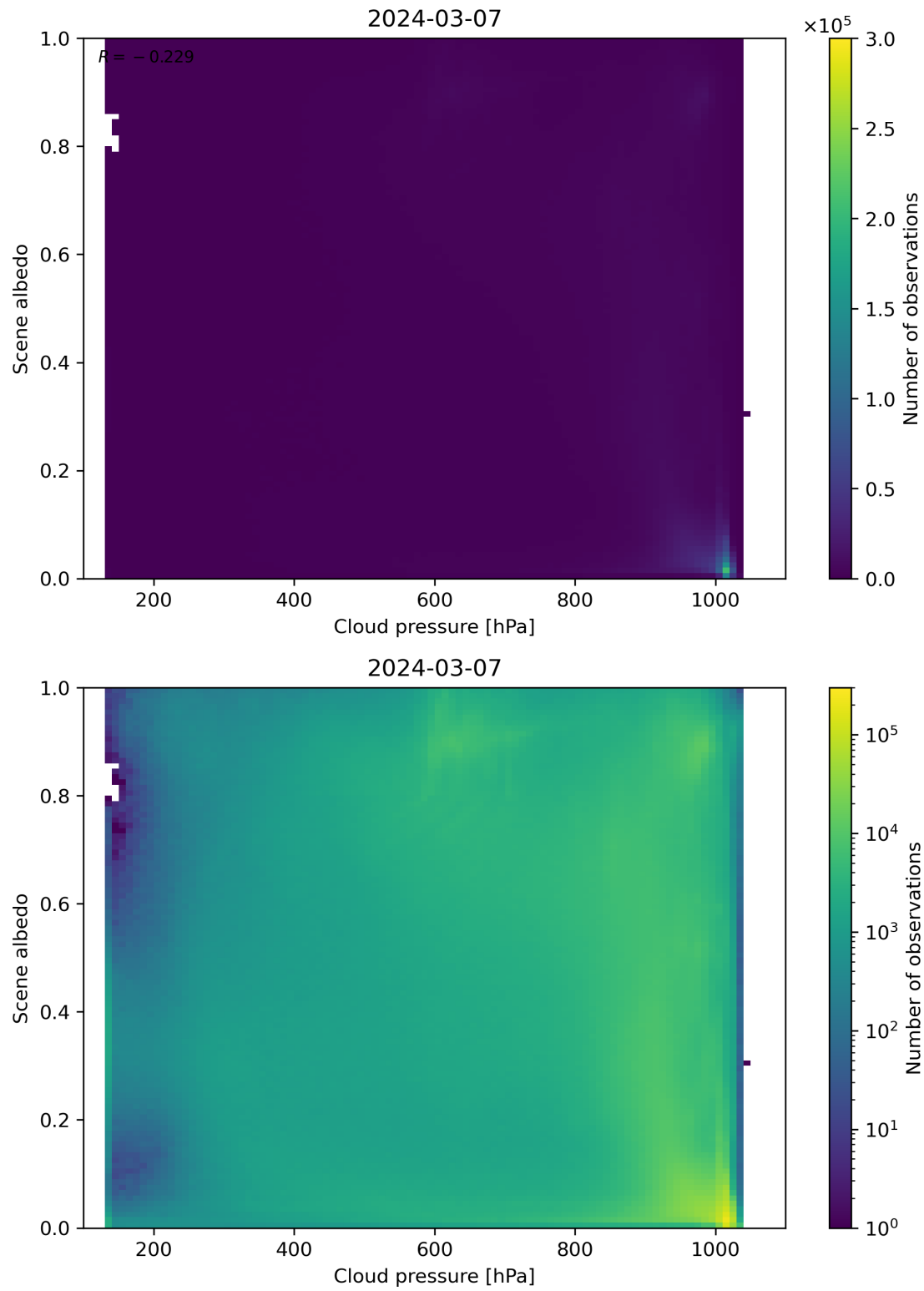
Figure 83: Scatter density plot of “Cloud pressure” against “Scene albedo” for 2024-03-06 to 2024-03-08.
