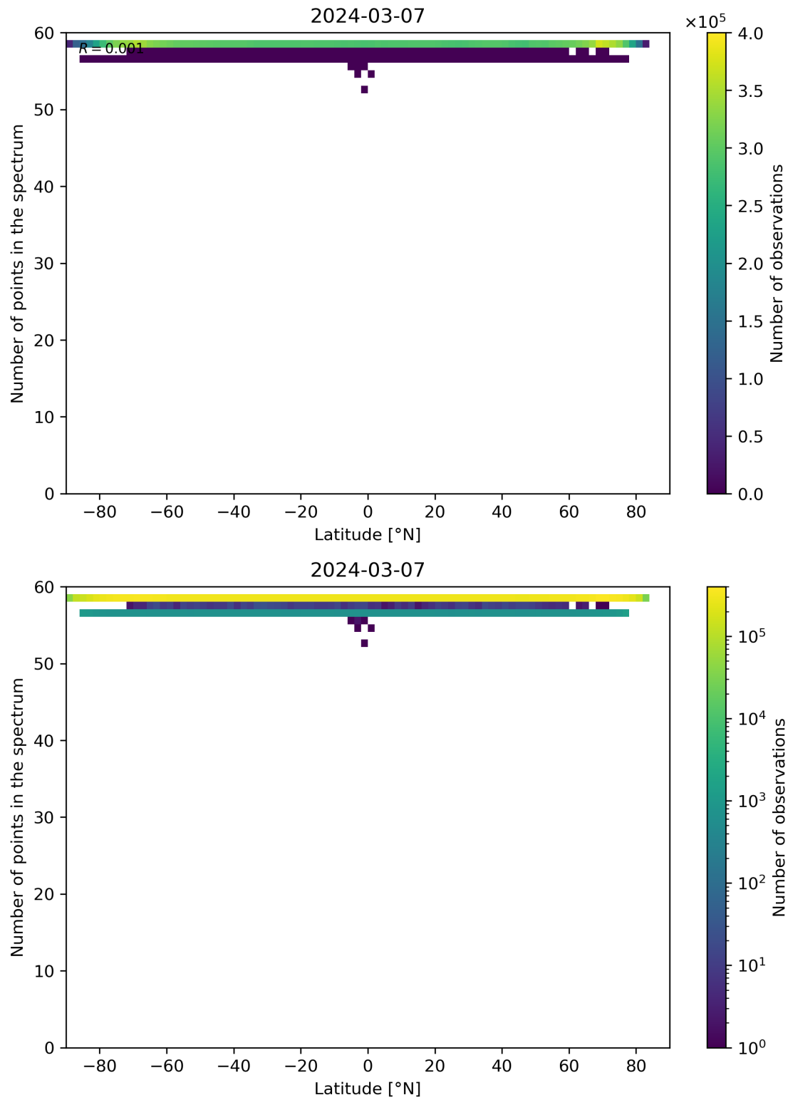
Figure 94: Scatter density plot of “Latitude” against “Number of points in the spectrum” for 2024-03-06 to 2024-03-08.
