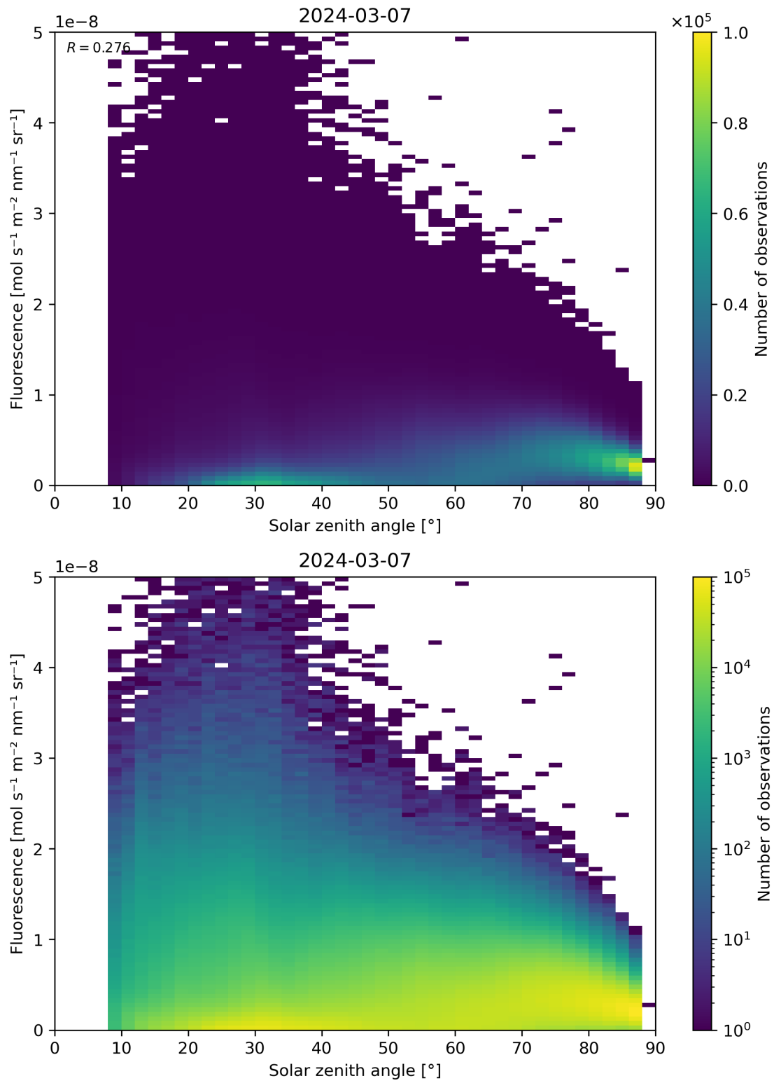
Figure 112: Scatter density plot of “Solar zenith angle” against “Fluorescence” for 2024-03-06 to 2024-03-08.
