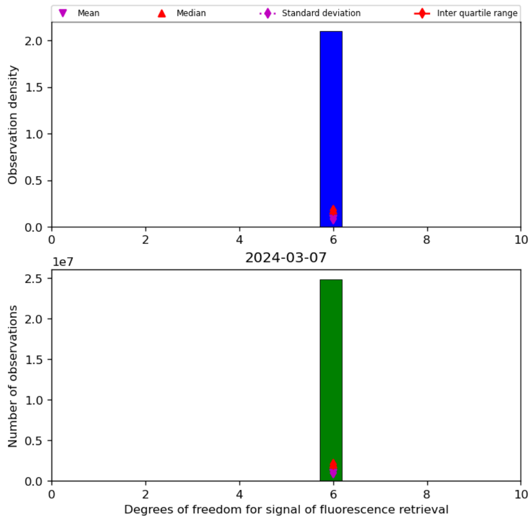
Figure 43: Histogram of “Degrees of freedom for signal of fluorescence retrieval” for 2024-03-06 to 2024-03-08
