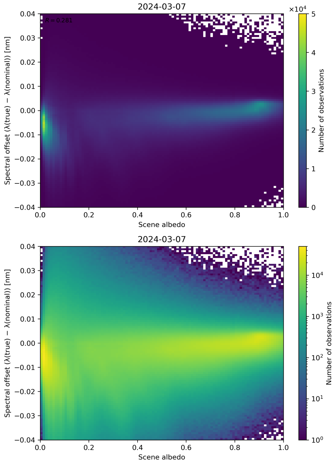
Figure 107: Scatter density plot of “Scene albedo” against “Spectral offset ( \lambda(\text{true}) - \lambda(\text{nominal}) )” for 2024-03-06 to 2024-03-08.
