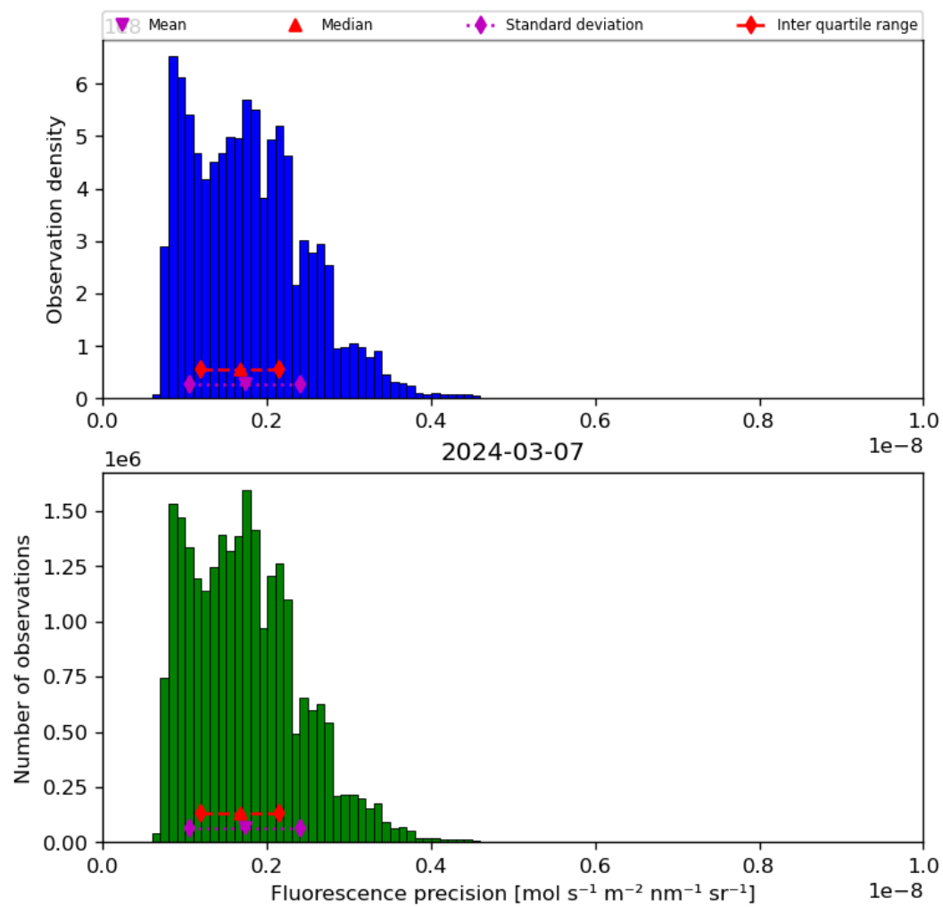
Figure 41: Histogram of “Fluorescence precision” for 2024-03-06 to 2024-03-08
