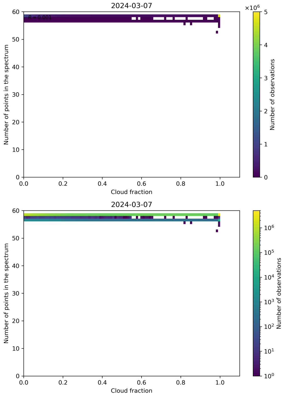
Figure 74: Scatter density plot of “Cloud fraction” against “Number of points in the spectrum” for 2024-03-06 to 2024-03-08.
