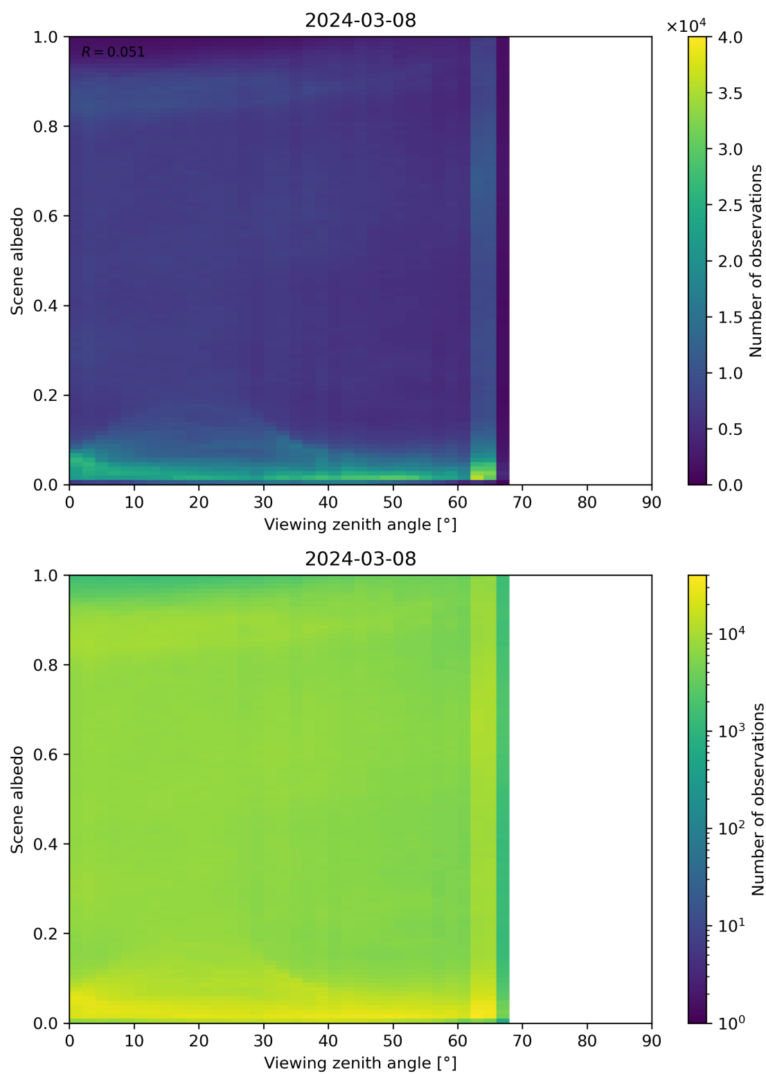
Figure 126: Scatter density plot of “Viewing zenith angle” against “Scene albedo” for 2024-03-07 to 2024-03-09.
