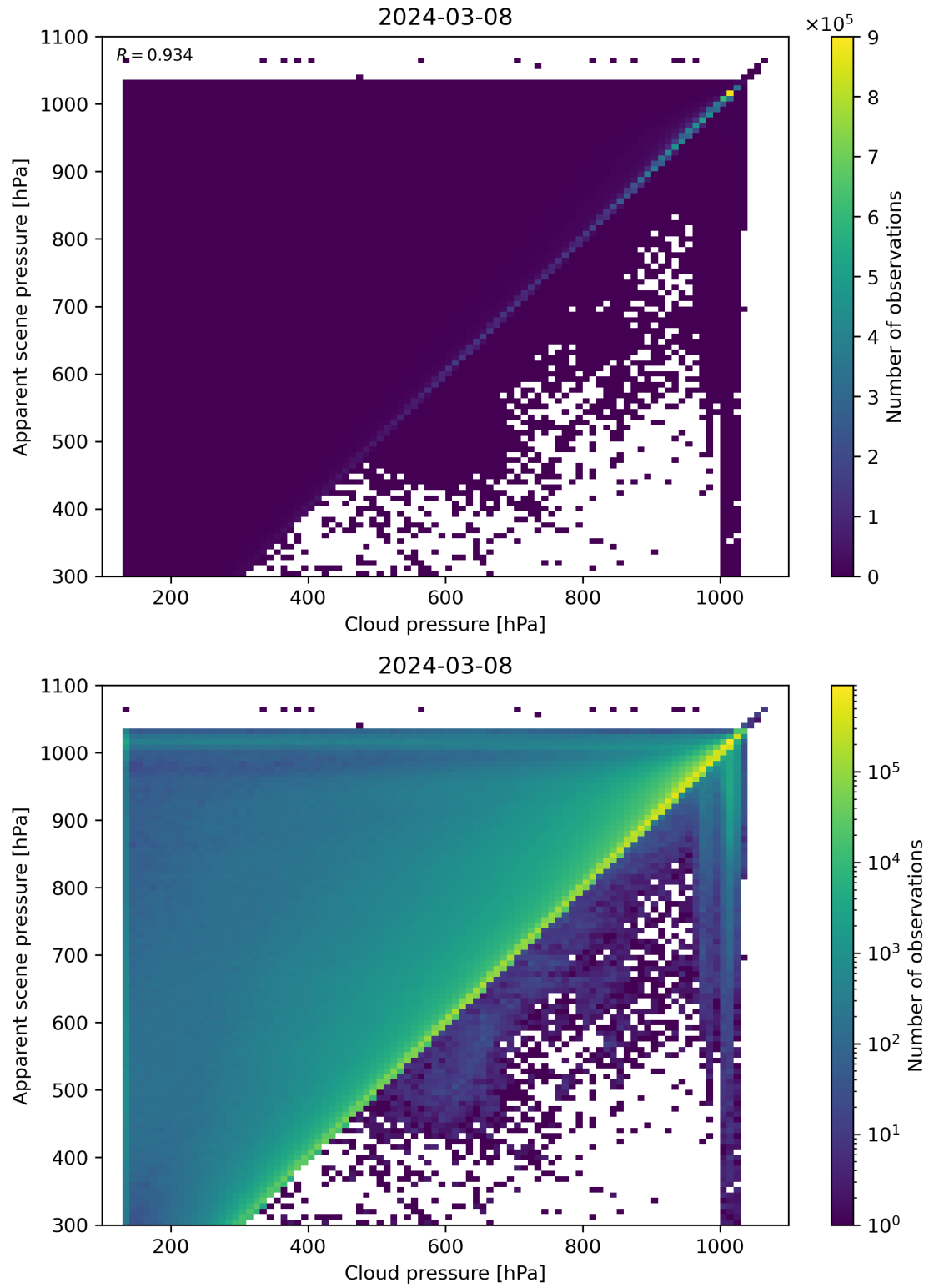
Figure 77: Scatter density plot of “Cloud pressure” against “Apparent scene pressure” for 2024-03-07 to 2024-03-09.
