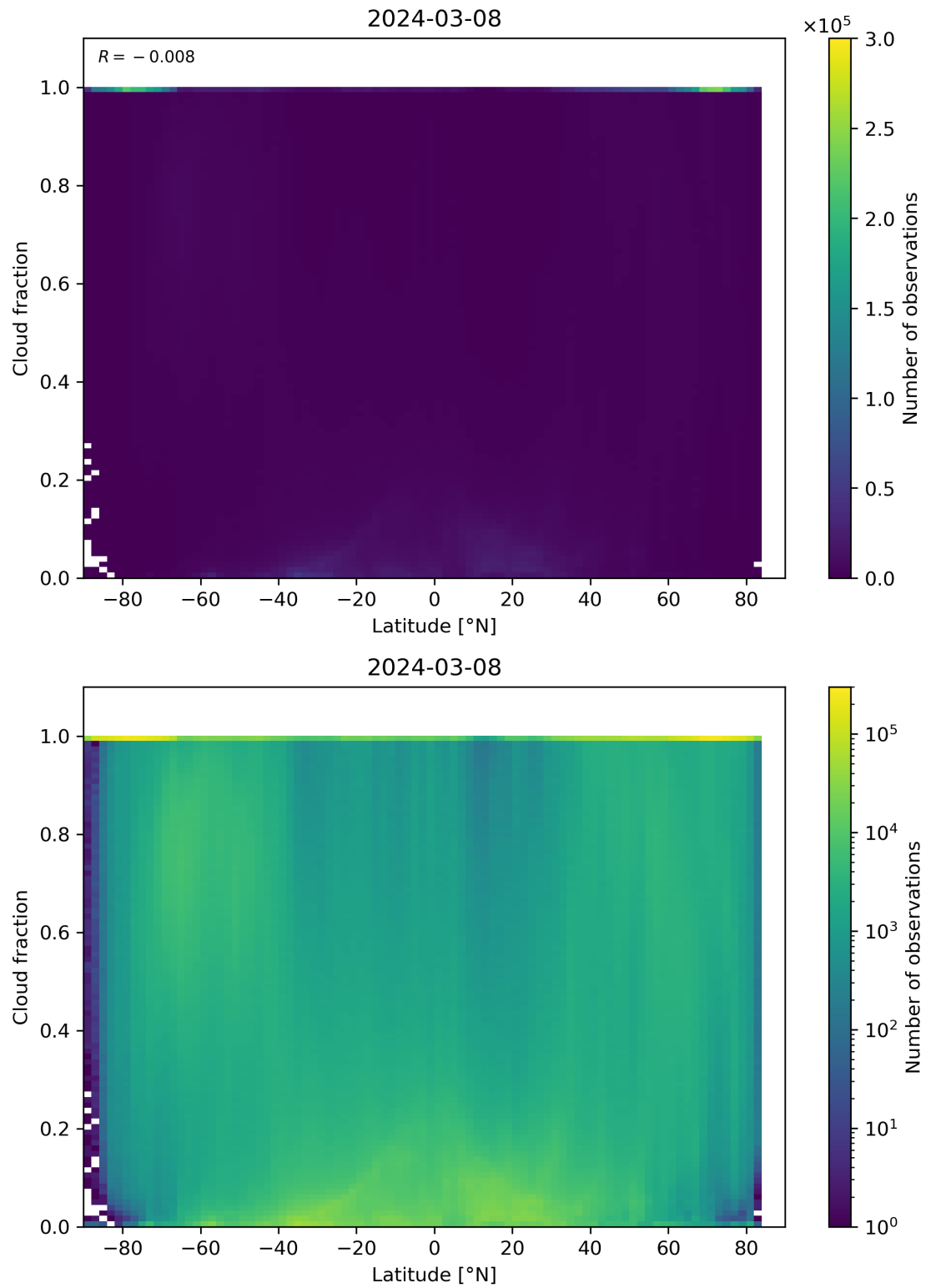
Figure 90: Scatter density plot of “Latitude” against “Cloud fraction” for 2024-03-07 to 2024-03-09.
