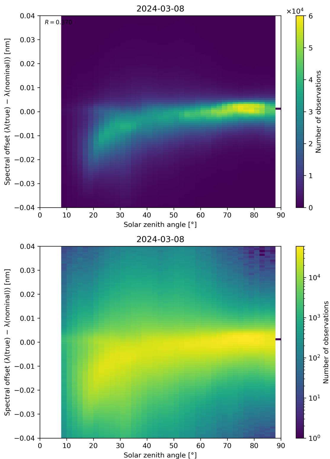
Figure 117: Scatter density plot of “Solar zenith angle” against “Spectral offset ( \lambda(\text{true}) - \lambda(\text{nominal}) )” for 2024-03-07 to 2024-03-09.
