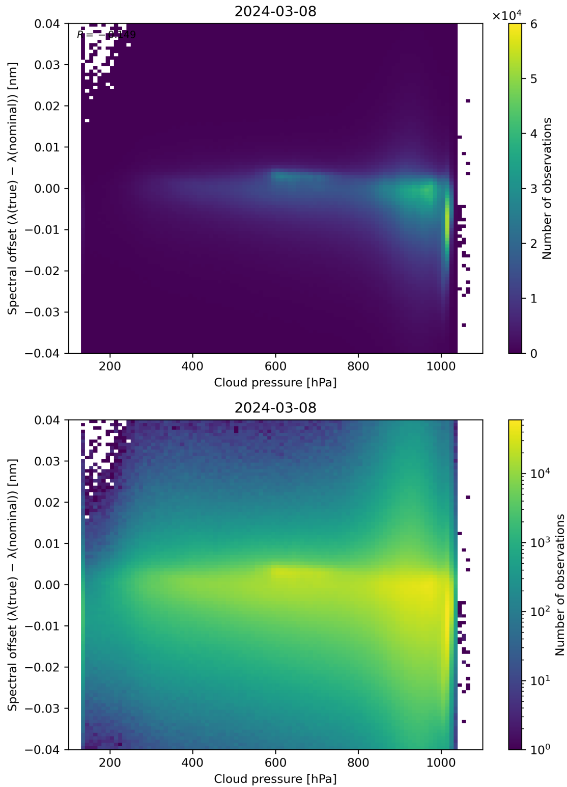
Figure 84: Scatter density plot of “Cloud pressure” against “Spectral offset ( \lambda(\text{true}) - \lambda(\text{nominal}) )” for 2024-03-07 to 2024-03-09.
