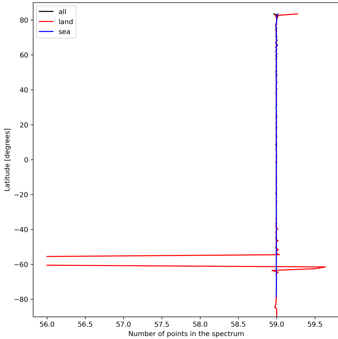
Figure 27: Zonal average of “Number of points in the spectrum” for 2024-03-07 to 2024-03-09.
