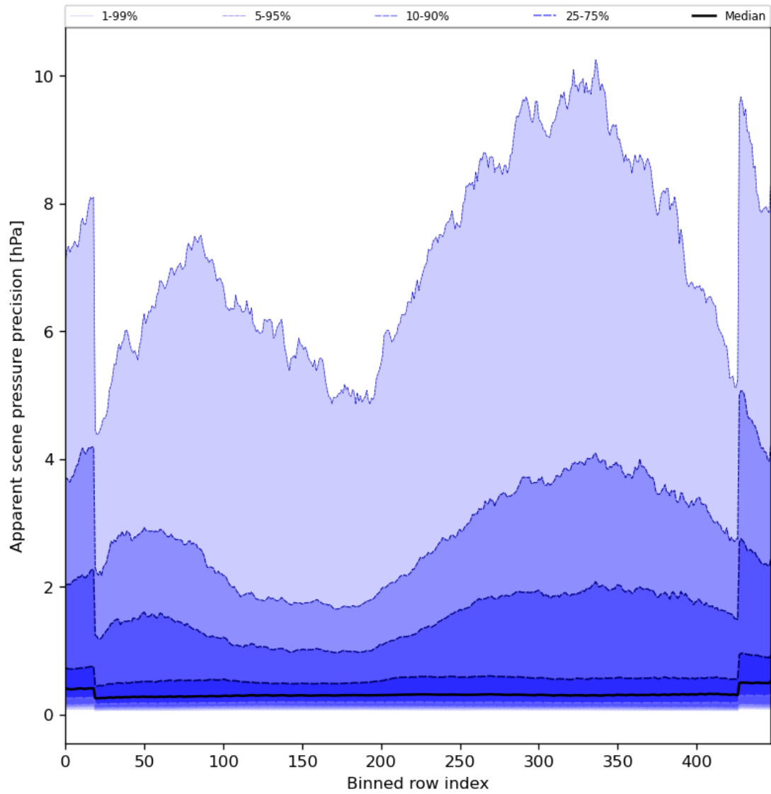
Figure 54: Along track statistics of “Apparent scene pressure precision” for 2024-03-07 to 2024-03-09
