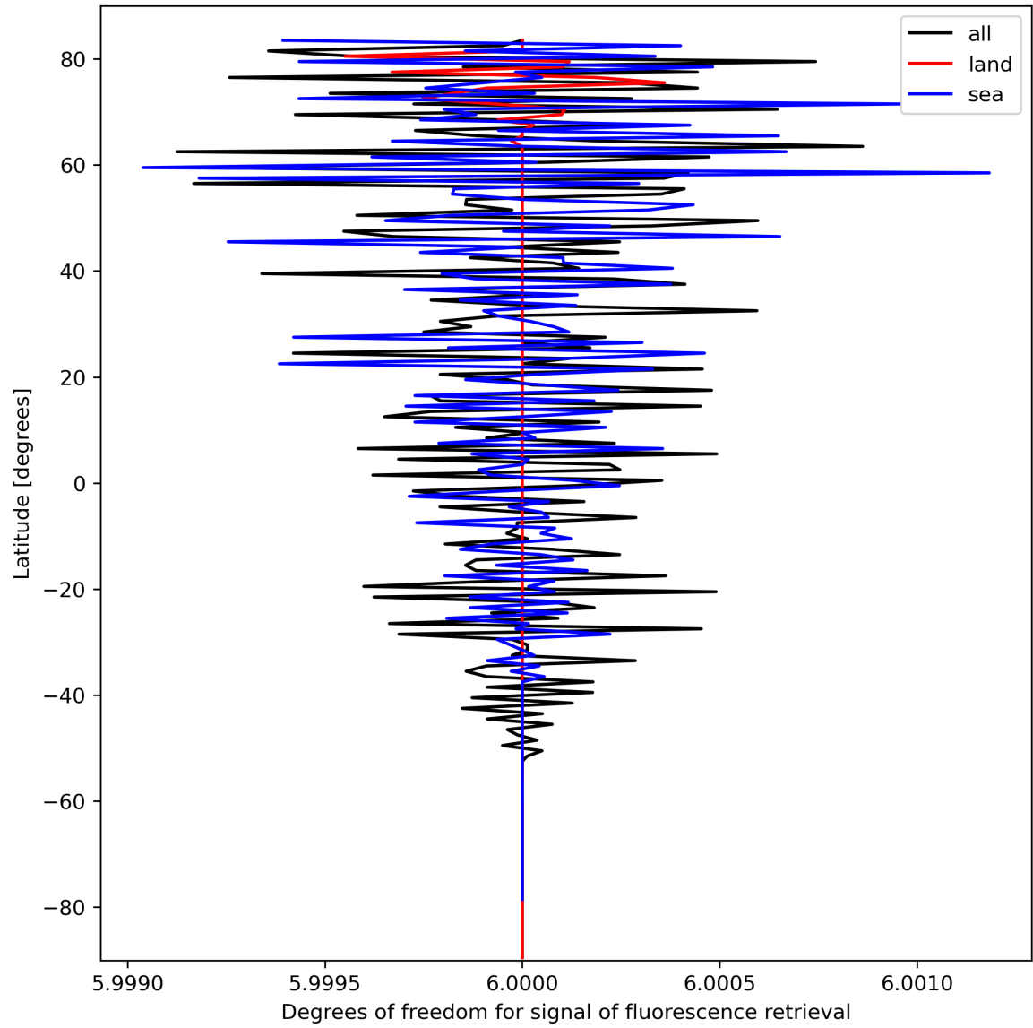
Figure 26: Zonal average of “Degrees of freedom for signal of fluorescence retrieval” for 2024-03-07 to 2024-03-09.
