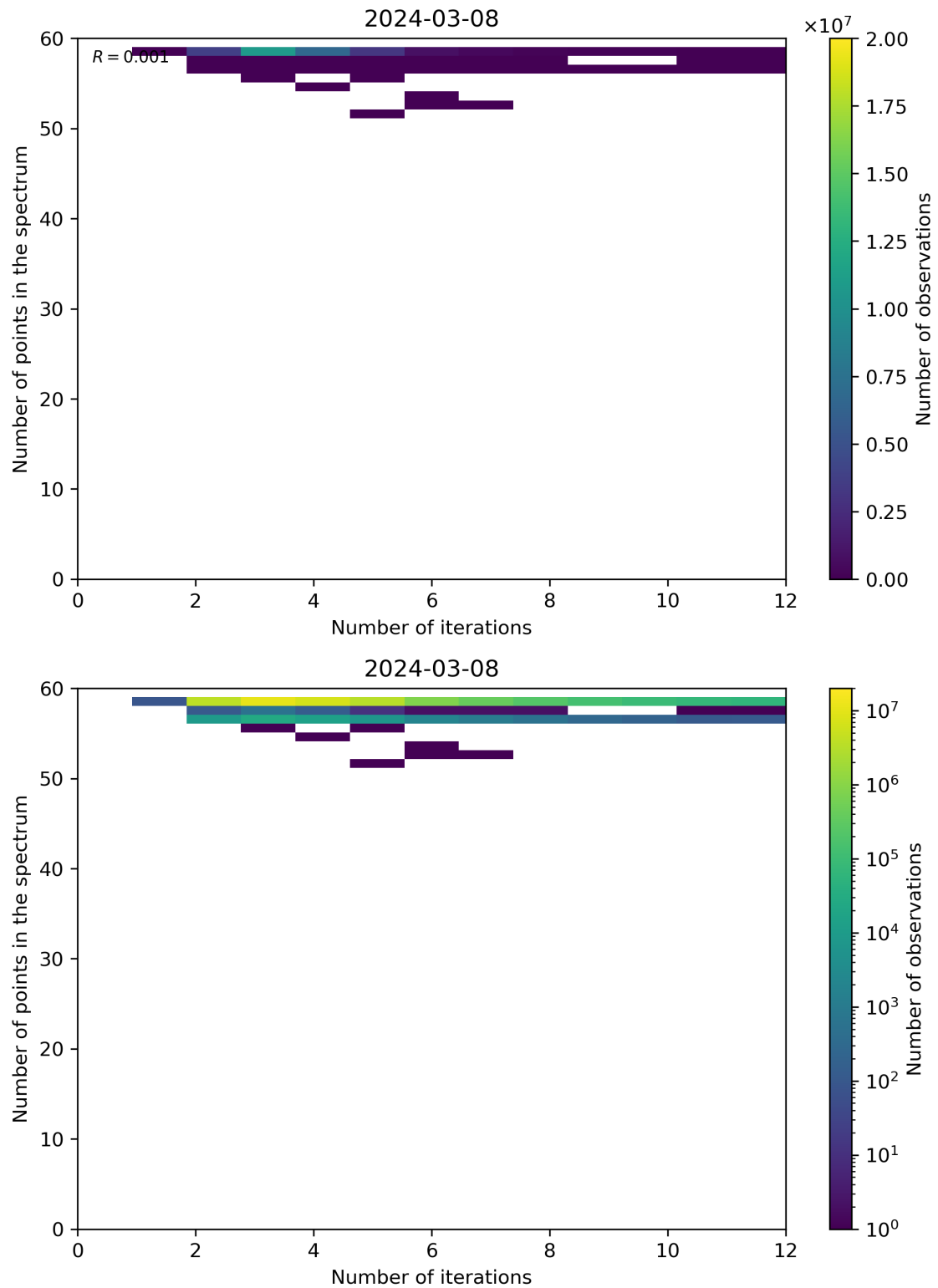
Figure 99: Scatter density plot of “Number of iterations” against “Number of points in the spectrum” for 2024-03-07 to 2024-03-09.
