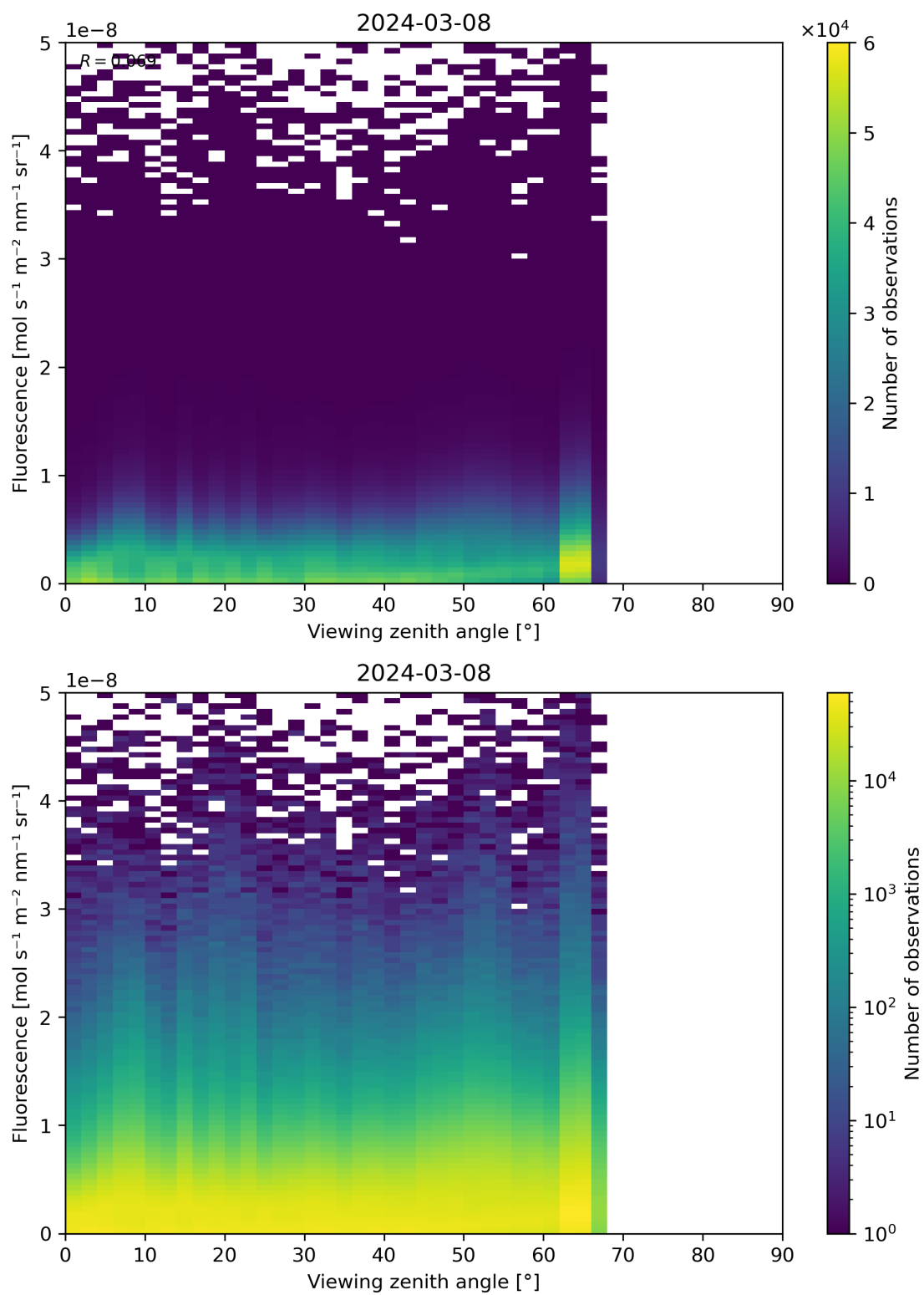
Figure 122: Scatter density plot of “Viewing zenith angle” against “Fluorescence” for 2024-03-07 to 2024-03-09.
