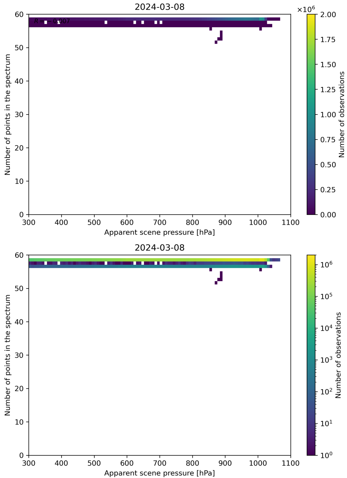
Figure 66: Scatter density plot of “Apparent scene pressure” against “Number of points in the spectrum” for 2024-03-07 to 2024-03-09.
