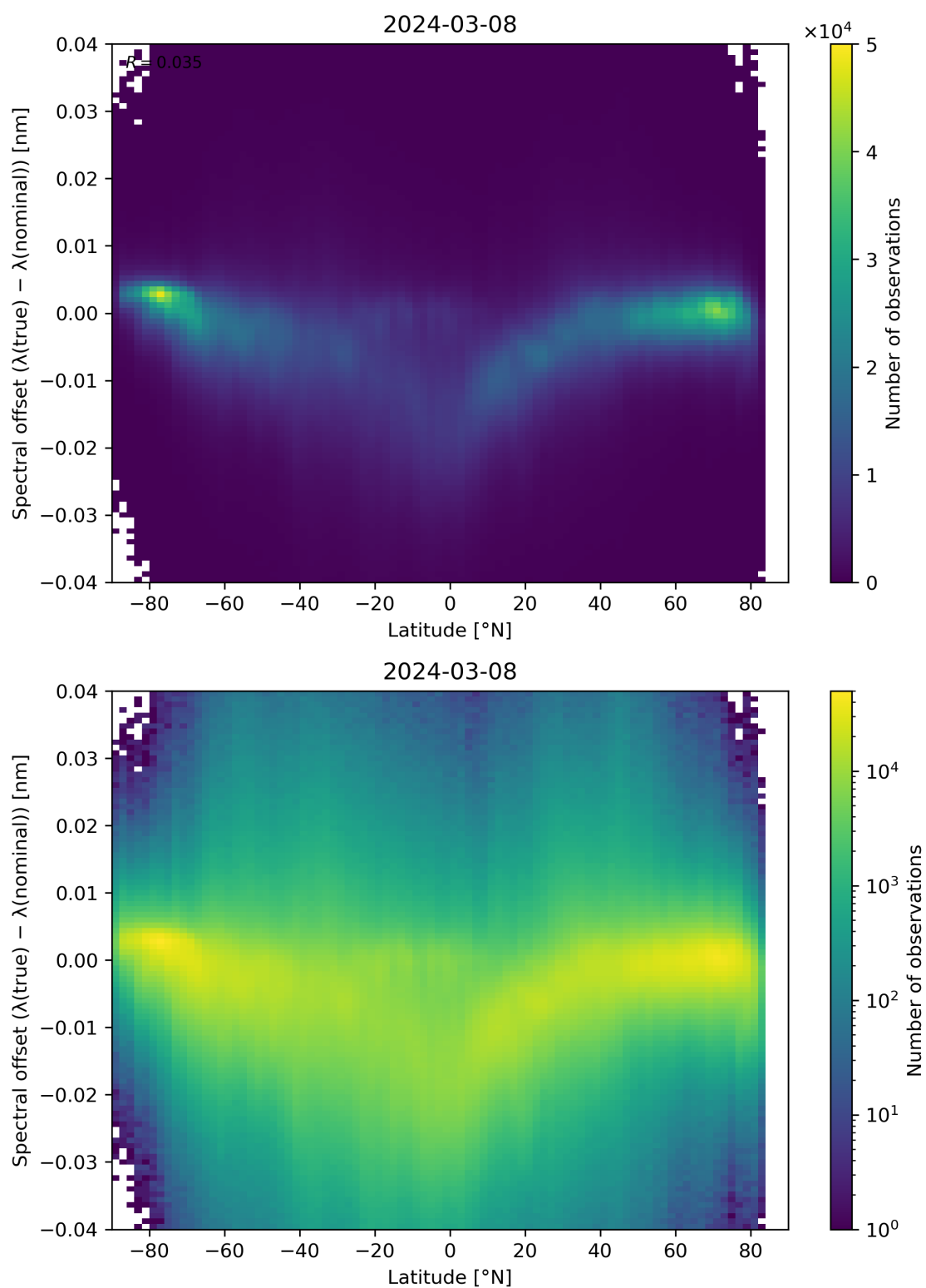
Figure 96: Scatter density plot of “Latitude” against “Spectral offset ( \lambda(\text{true}) - \lambda(\text{nominal}) )” for 2024-03-07 to 2024-03-09.
