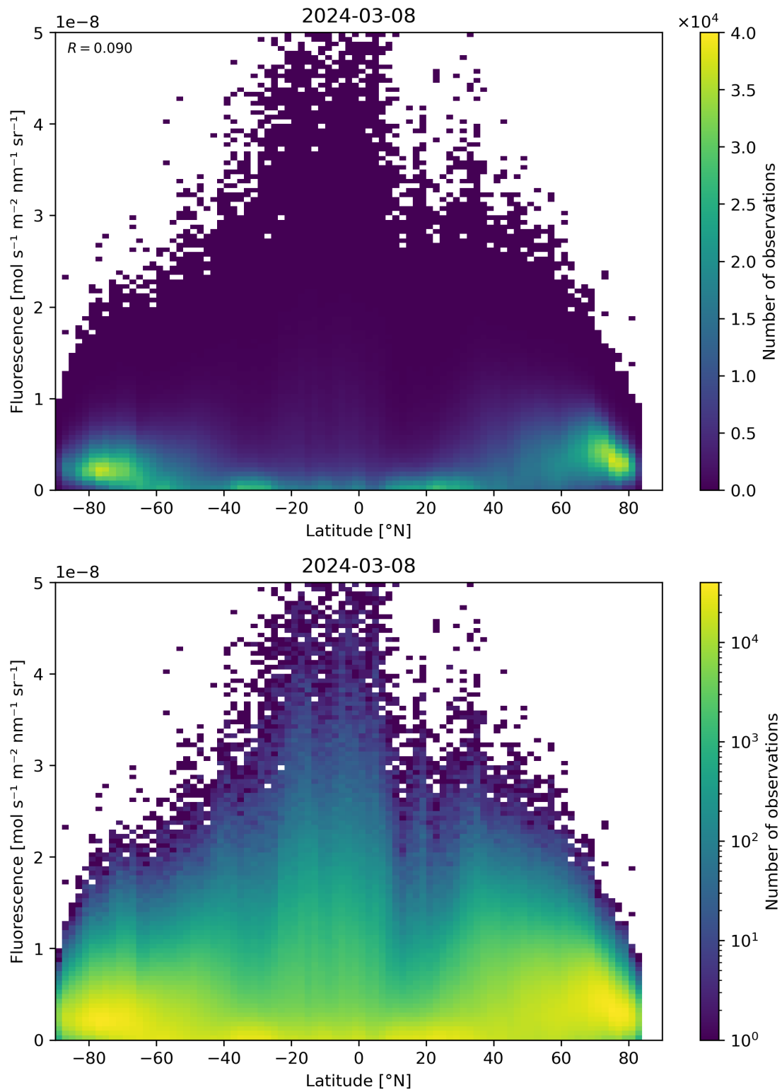
Figure 92: Scatter density plot of “Latitude” against “Fluorescence” for 2024-03-07 to 2024-03-09.
