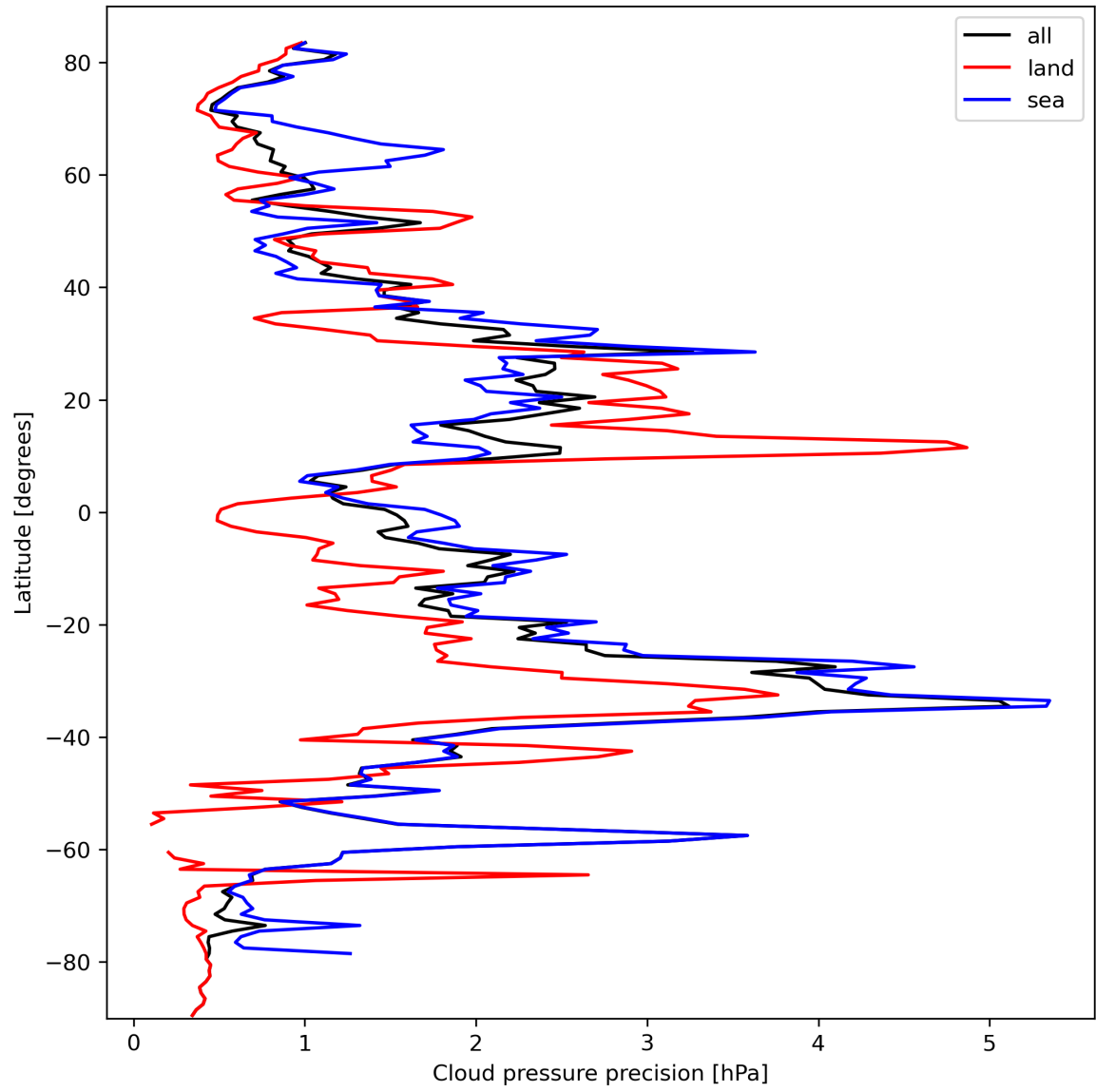
Figure 14: Zonal average of “Cloud pressure precision” for 2024-03-07 to 2024-03-09.
