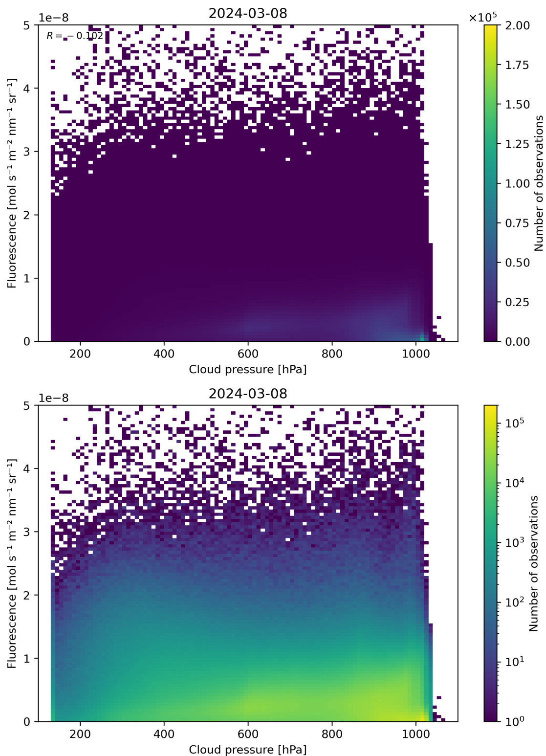
Figure 80: Scatter density plot of “Cloud pressure” against “Fluorescence” for 2024-03-07 to 2024-03-09.
