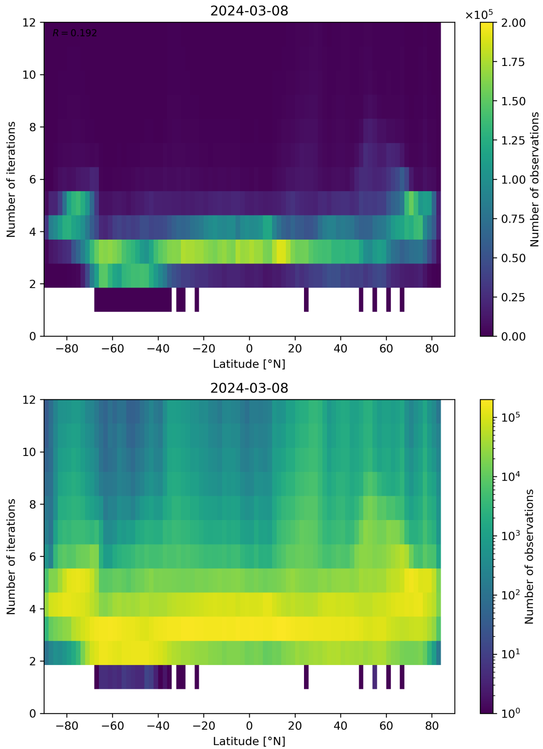
Figure 93: Scatter density plot of “Latitude” against “Number of iterations” for 2024-03-07 to 2024-03-09.
