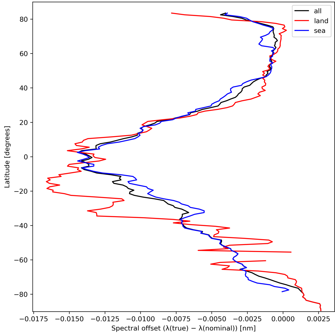
Figure 28: Zonal average of “Spectral offset ( \lambda(\text{true}) - \lambda(\text{nominal}) )” for 2024-03-07 to 2024-03-09.
