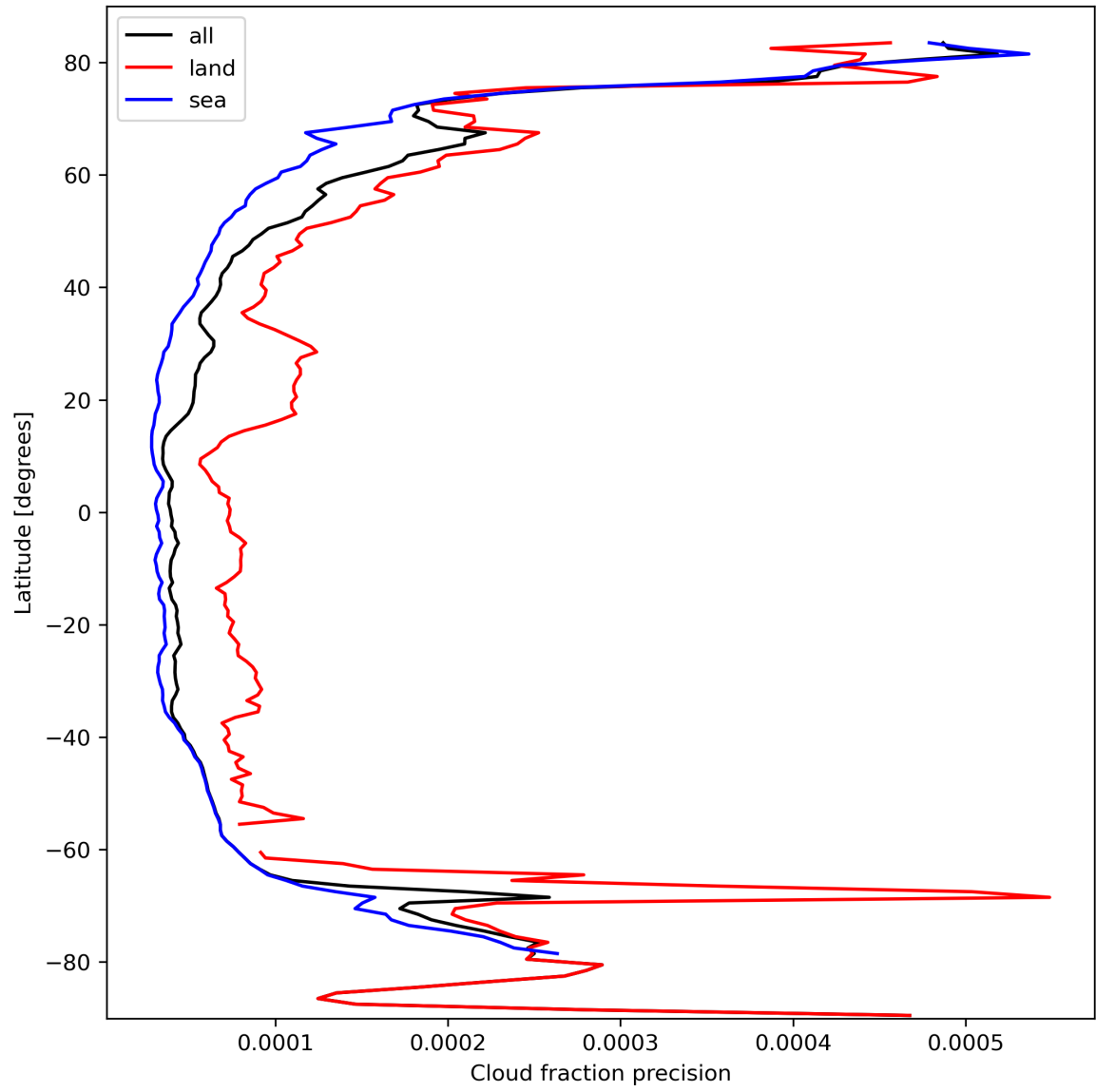
Figure 16: Zonal average of “Cloud fraction precision” for 2024-03-07 to 2024-03-09.
