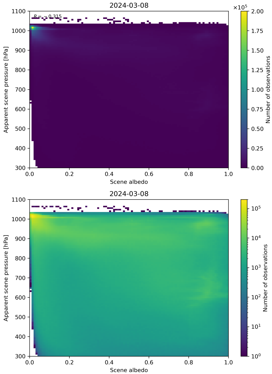
Figure 102: Scatter density plot of “Scene albedo” against “Apparent scene pressure” for 2024-03-07 to 2024-03-09.
