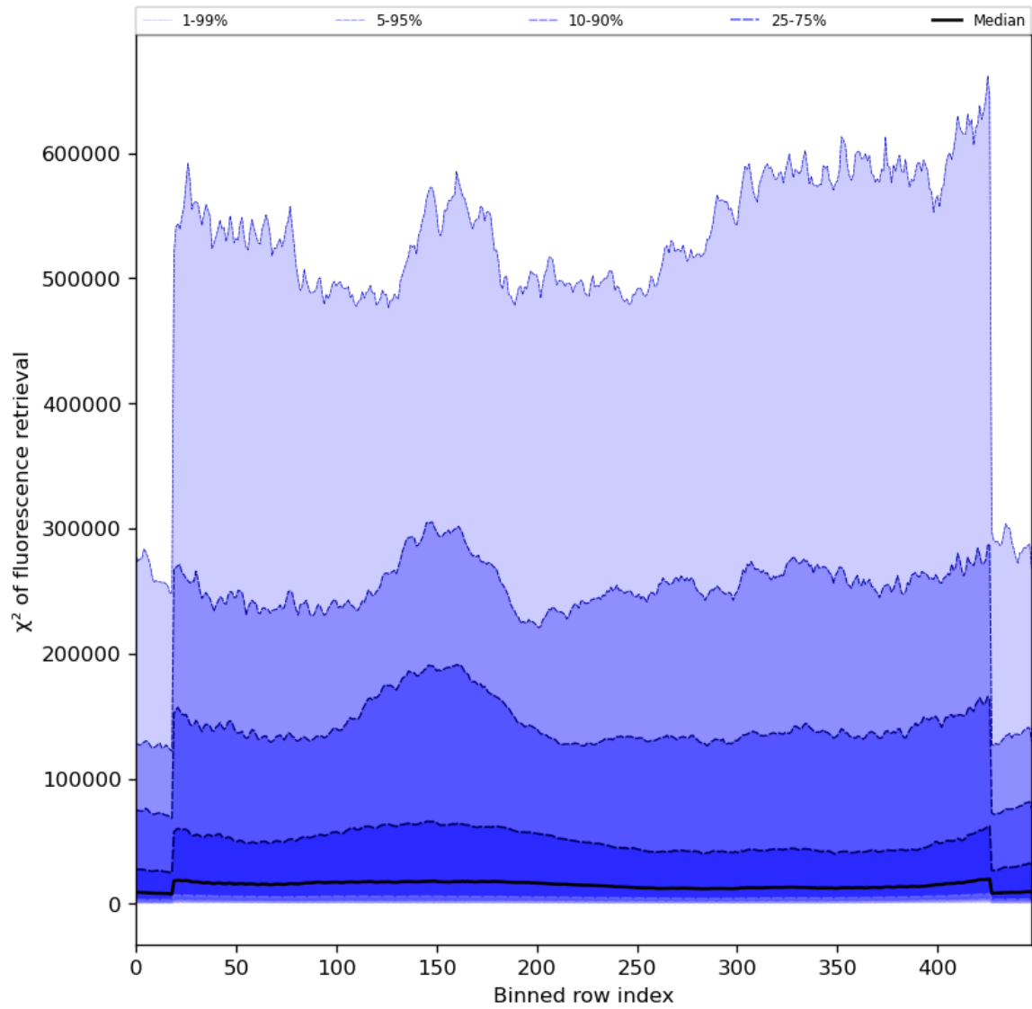
Figure 59: Along track statistics of “ \chi^2 of fluorescence retrieval” for 2024-03-07 to 2024-03-09
