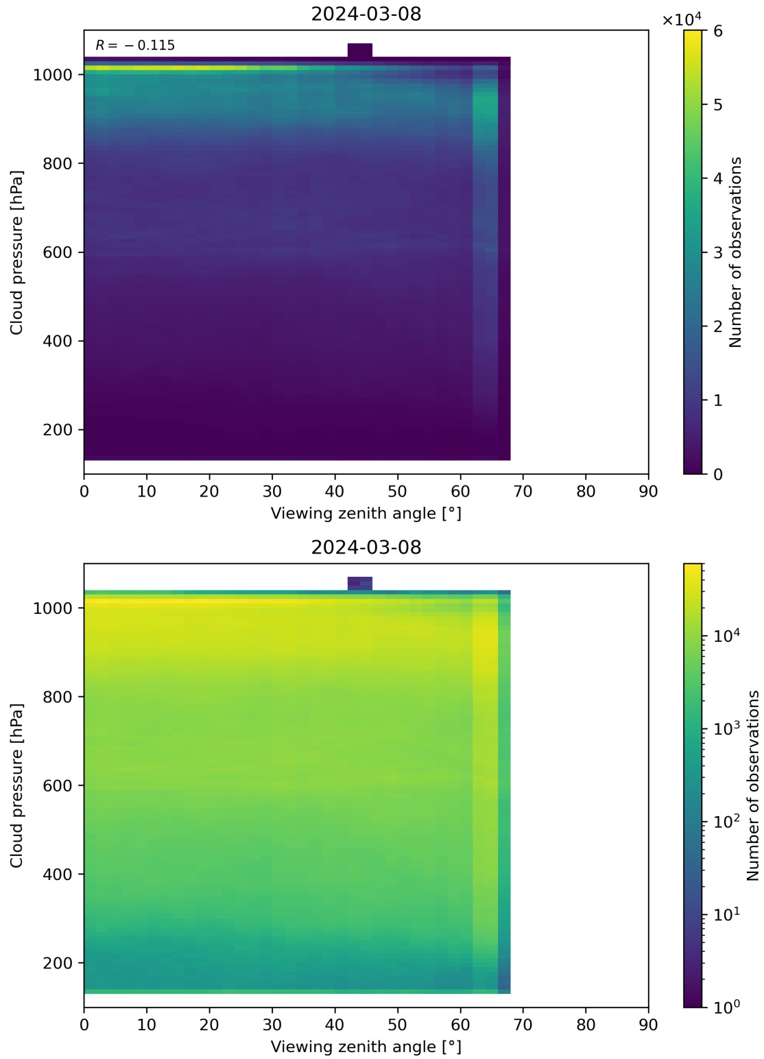
Figure 121: Scatter density plot of “Viewing zenith angle” against “Cloud pressure” for 2024-03-07 to 2024-03-09.
