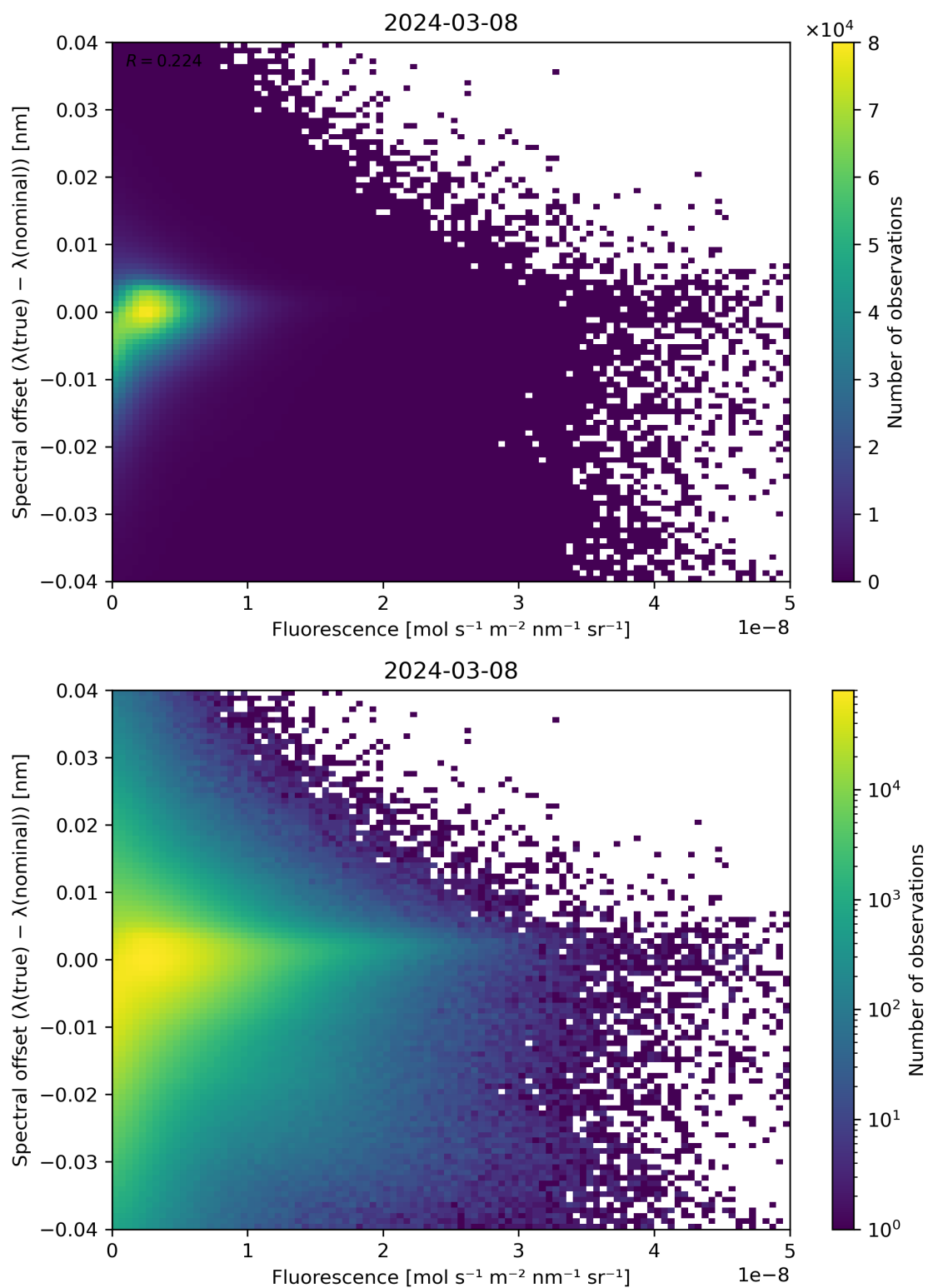
Figure 87: Scatter density plot of “Fluorescence” against “Spectral offset ( \lambda(\text{true}) - \lambda(\text{nominal}) )” for 2024-03-07 to 2024-03-09.
