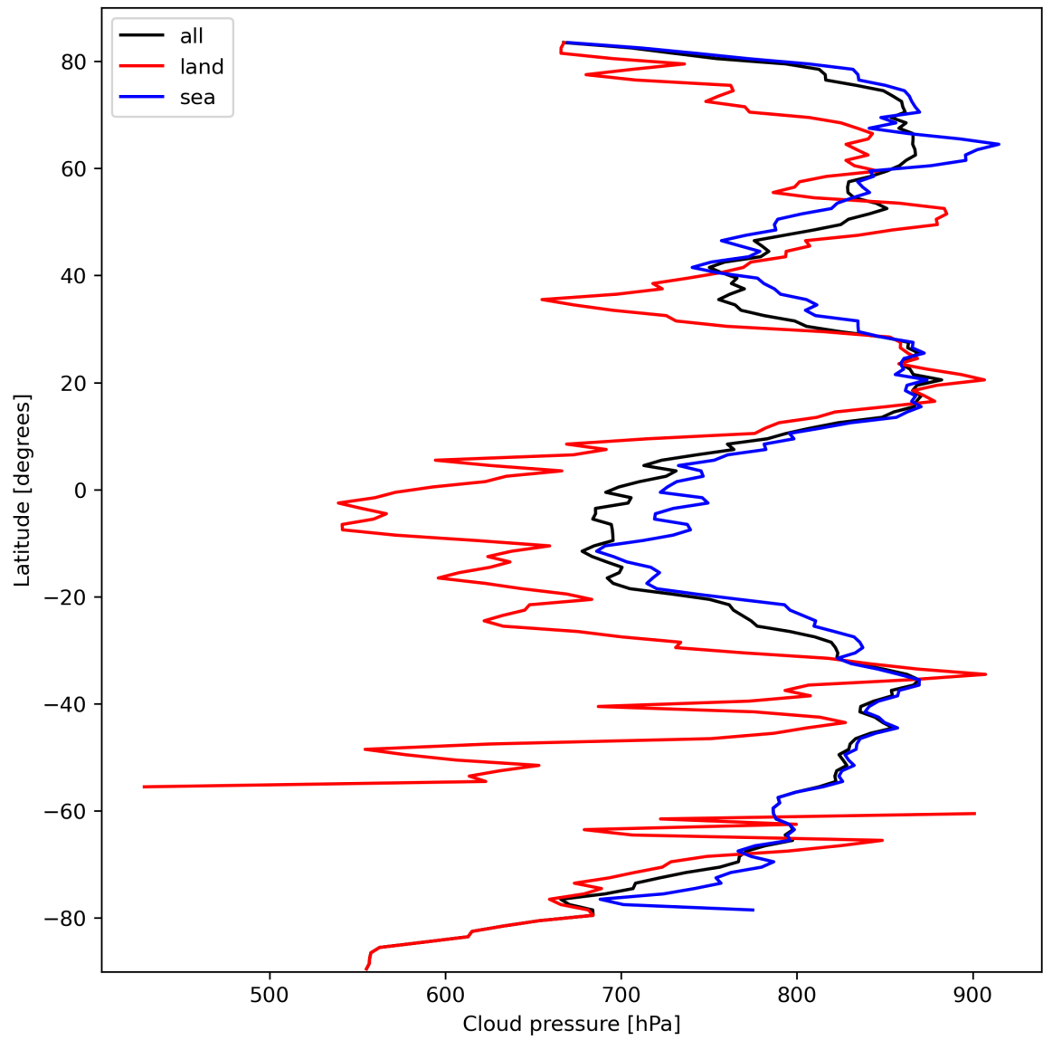
Figure 13: Zonal average of “Cloud pressure” for 2024-03-07 to 2024-03-09.
