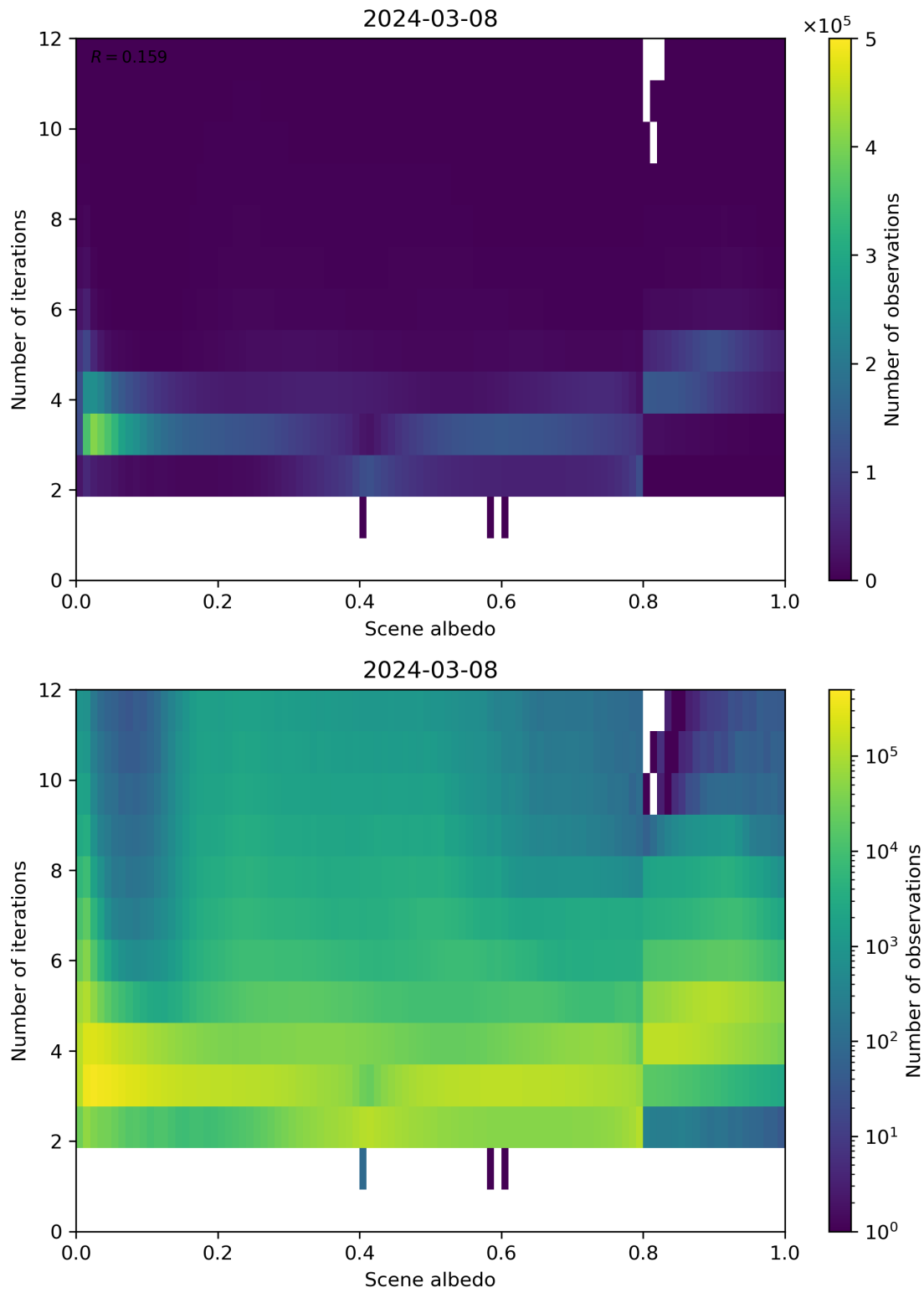
Figure 105: Scatter density plot of “Scene albedo” against “Number of iterations” for 2024-03-07 to 2024-03-09.
