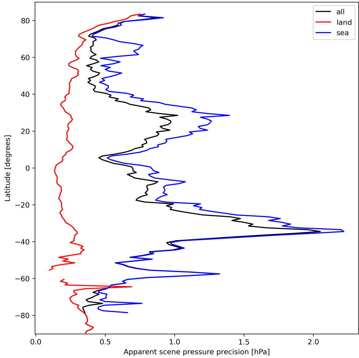
Figure 20: Zonal average of “Apparent scene pressure precision” for 2024-03-07 to 2024-03-09.
