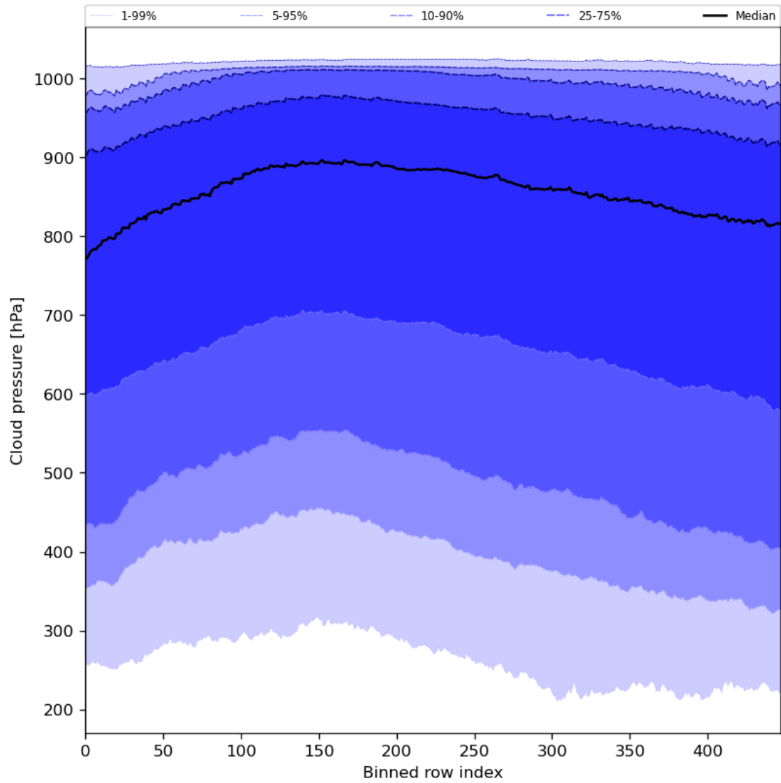
Figure 47: Along track statistics of “Cloud pressure” for 2024-03-07 to 2024-03-09
