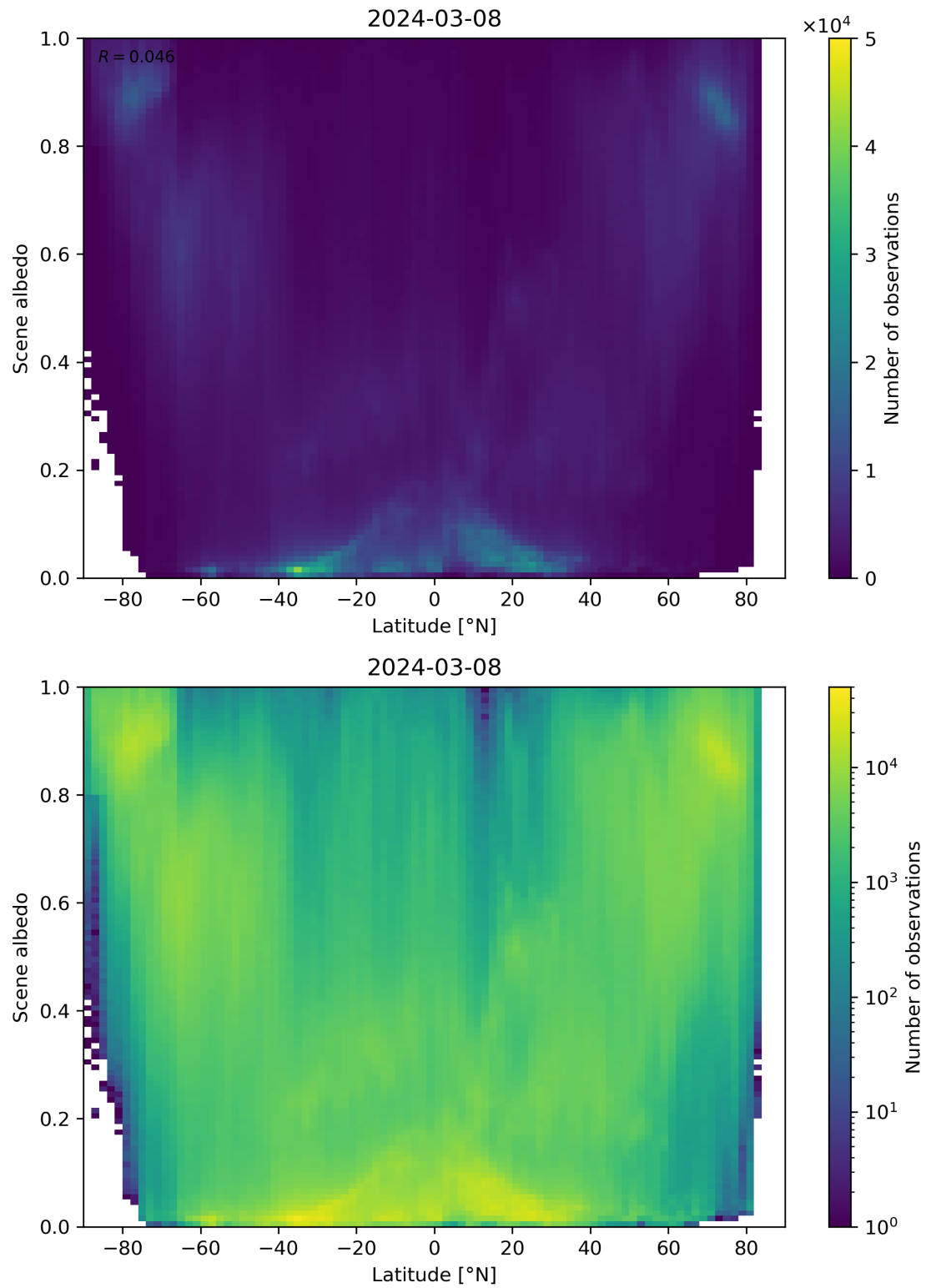
Figure 95: Scatter density plot of “Latitude” against “Scene albedo” for 2024-03-07 to 2024-03-09.
