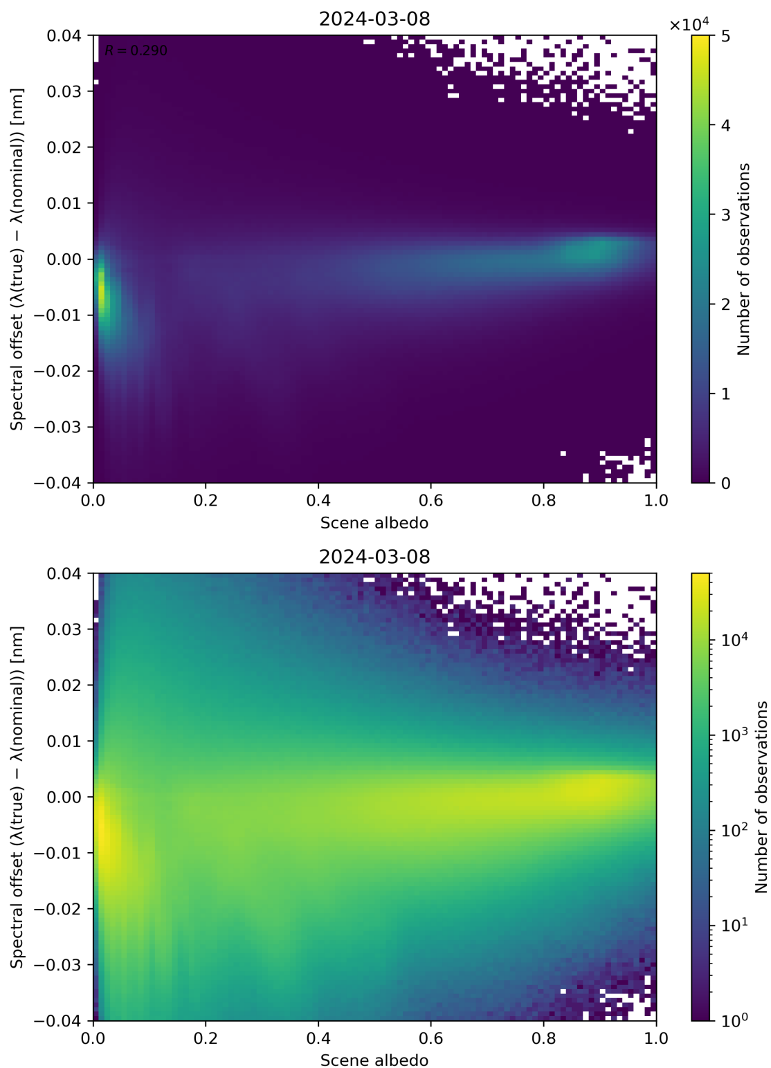
Figure 107: Scatter density plot of “Scene albedo” against “Spectral offset ( \lambda(\text{true}) - \lambda(\text{nominal}) )” for 2024-03-07 to 2024-03-09.
