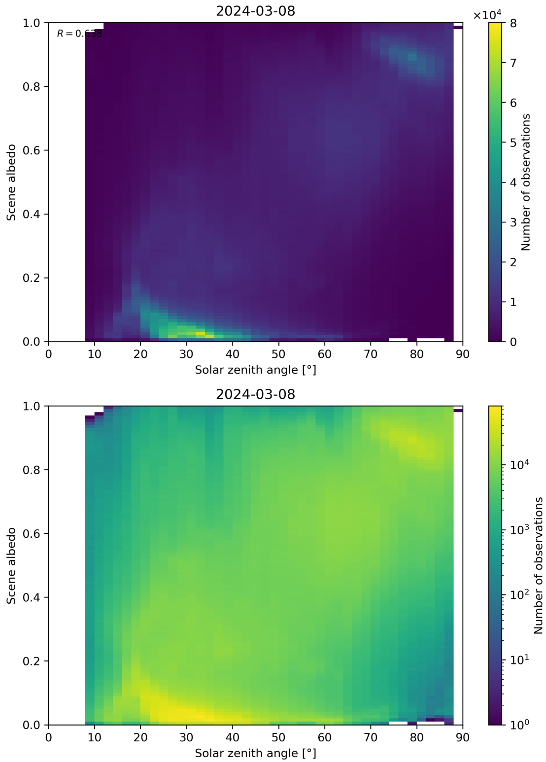
Figure 116: Scatter density plot of “Solar zenith angle” against “Scene albedo” for 2024-03-07 to 2024-03-09.
