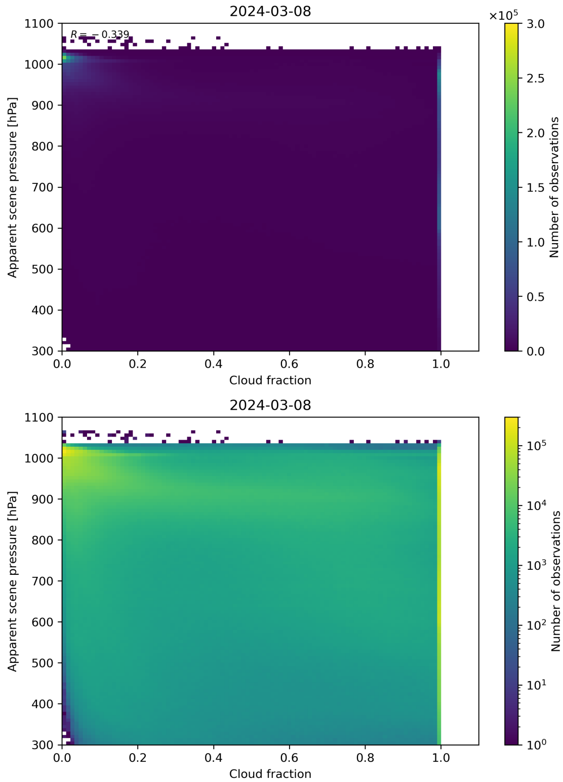
Figure 70: Scatter density plot of “Cloud fraction” against “Apparent scene pressure” for 2024-03-07 to 2024-03-09.
