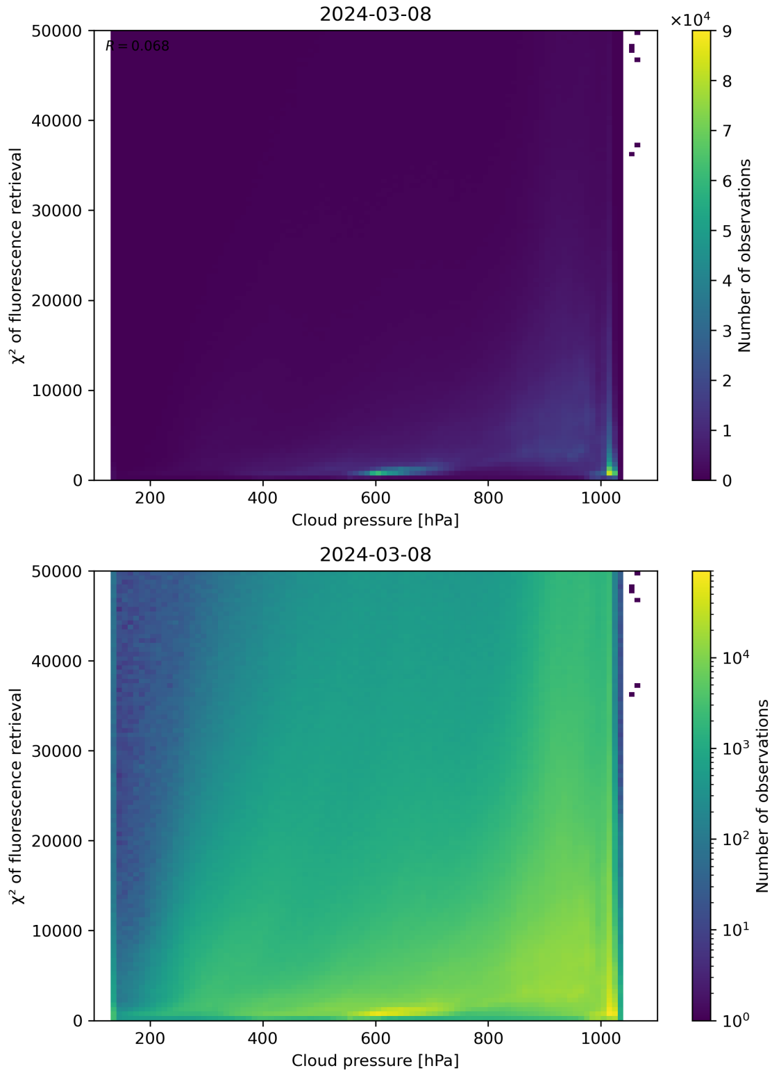
Figure 78: Scatter density plot of “Cloud pressure” against “ \chi^2 of fluorescence retrieval” for 2024-03-07 to 2024-03-09.
