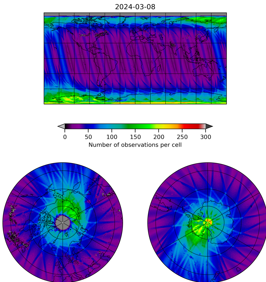
Figure 11: Map of the number of observations for 2024-03-07 to 2024-03-09
