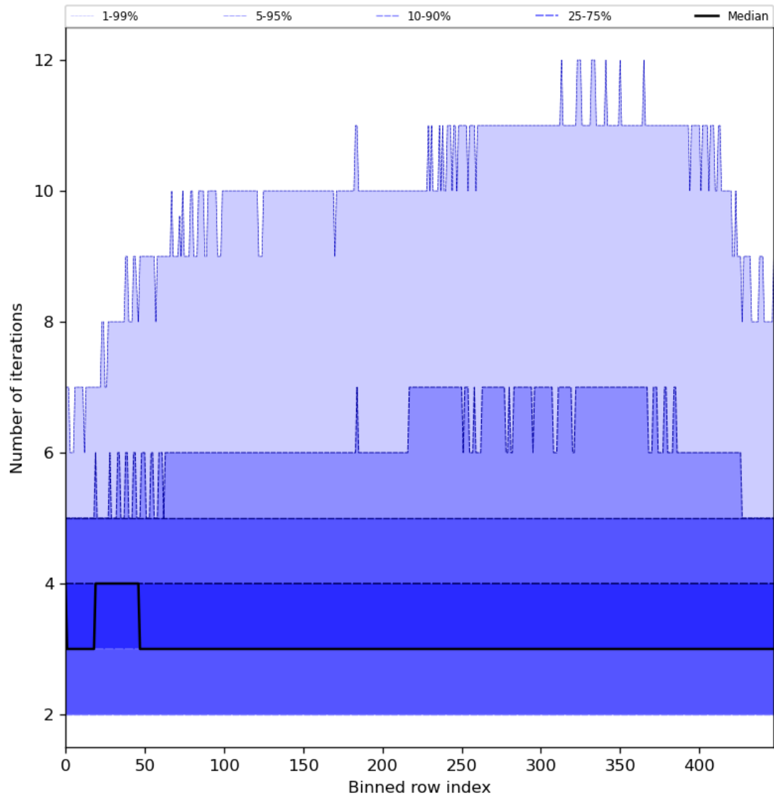
Figure 56: Along track statistics of “Number of iterations” for 2024-03-07 to 2024-03-09
