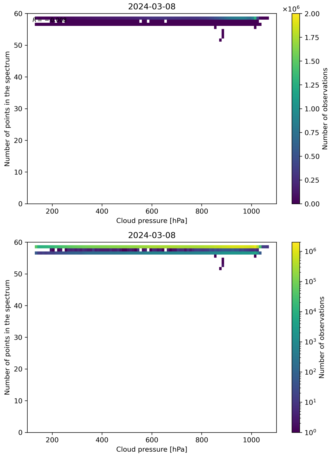
Figure 82: Scatter density plot of “Cloud pressure” against “Number of points in the spectrum” for 2024-03-07 to 2024-03-09.
