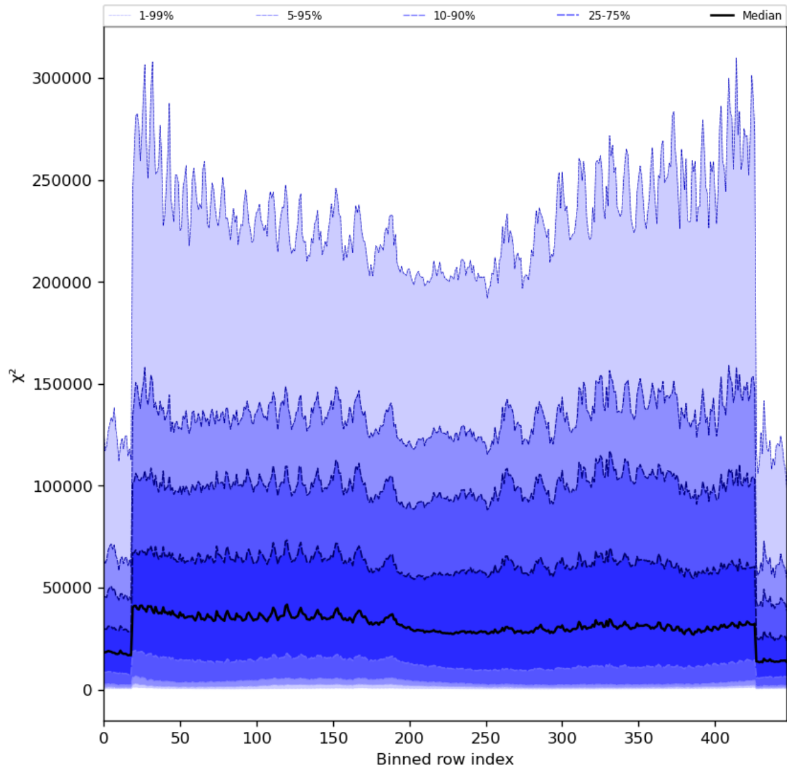
Figure 55: Along track statistics of “ \chi^2 ” for 2024-03-07 to 2024-03-09
