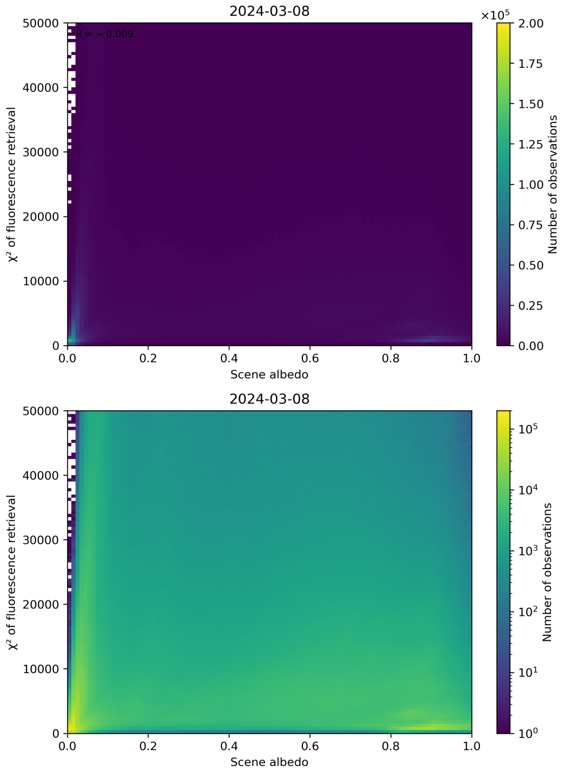
Figure 103: Scatter density plot of “Scene albedo” against “ \chi^2 of fluorescence retrieval” for 2024-03-07 to 2024-03-09.
