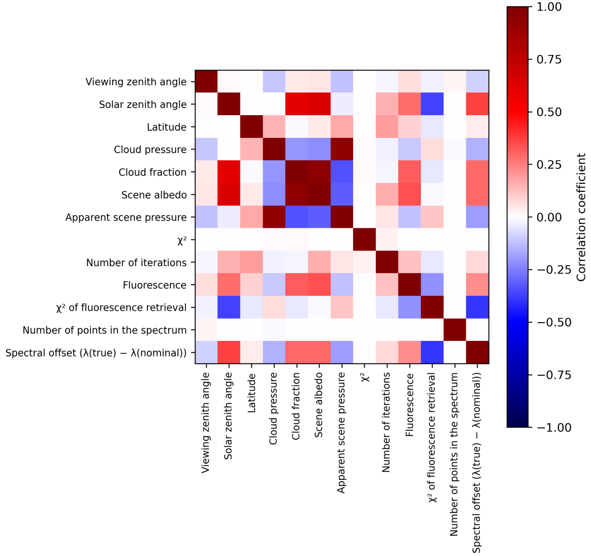
Figure 2: Map of correlation matrix for 2024-03-07 to 2024-03-09.
