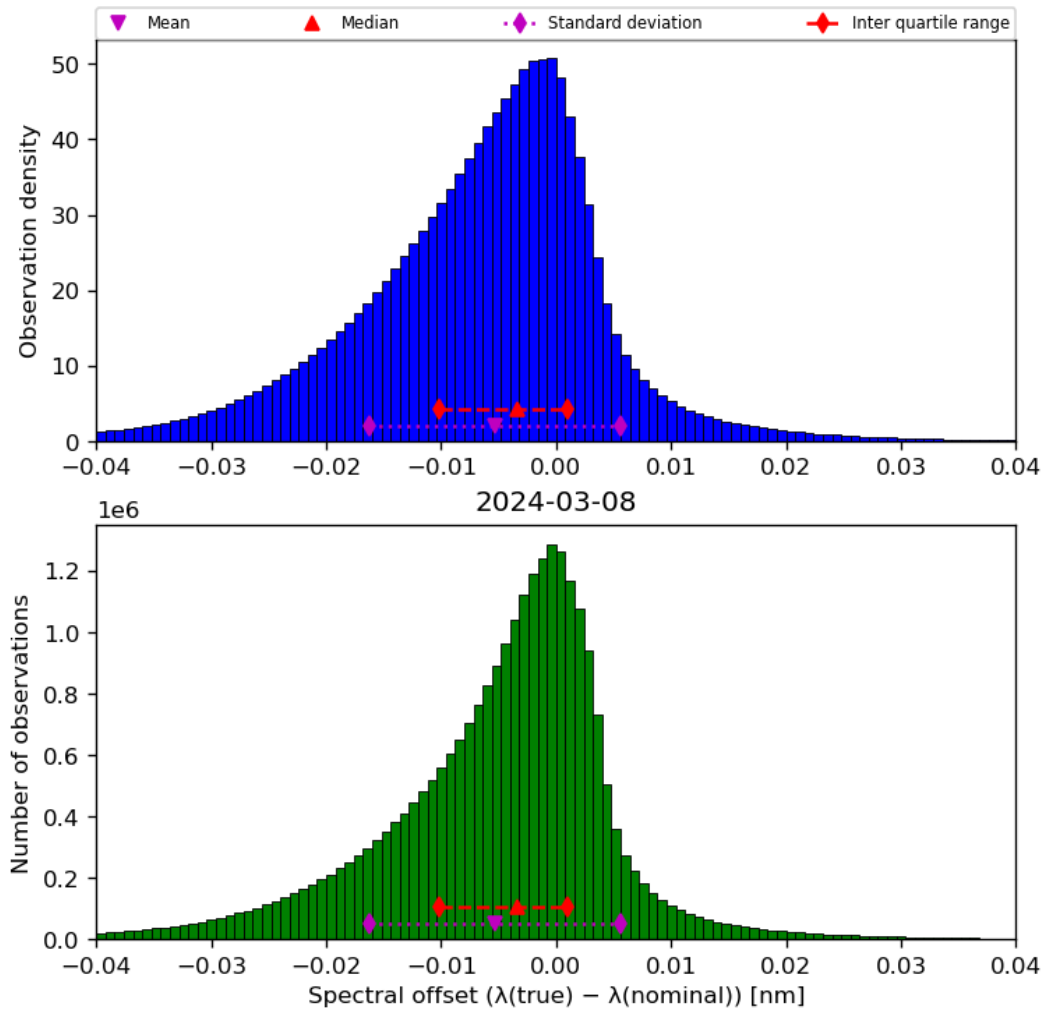
Figure 45: Histogram of “Spectral offset ( \lambda(\text{true}) - \lambda(\text{nominal}) )” for 2024-03-07 to 2024-03-09
