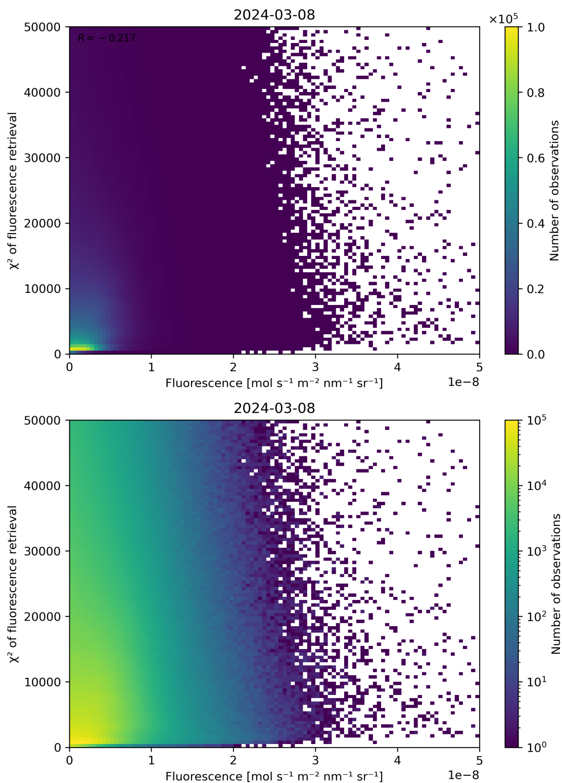
Figure 85: Scatter density plot of “Fluorescence” against “ \chi^2 of fluorescence retrieval” for 2024-03-07 to 2024-03-09.
