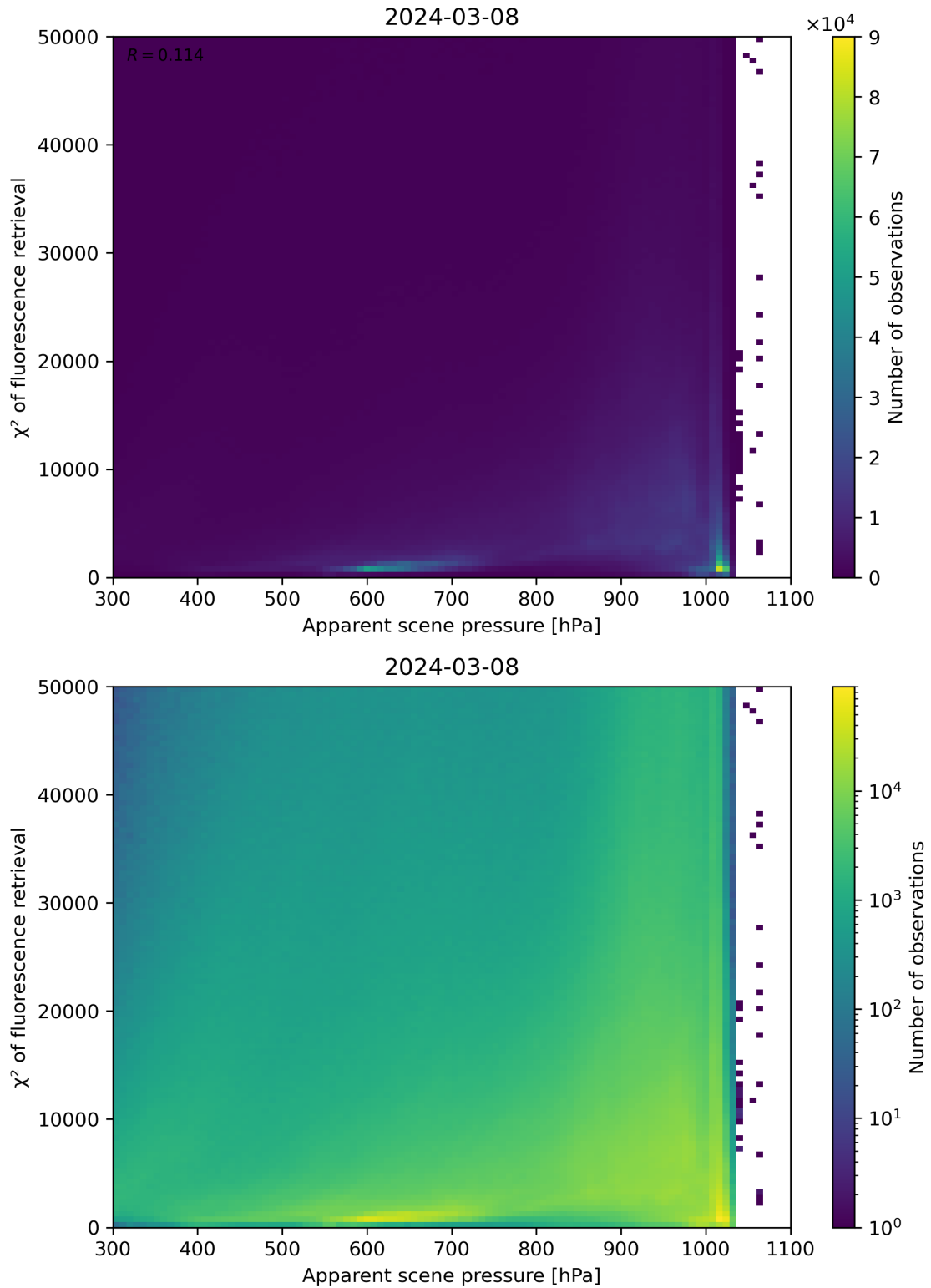
Figure 63: Scatter density plot of “Apparent scene pressure” against “ \chi^2 of fluorescence retrieval” for 2024-03-07 to 2024-03-09.
