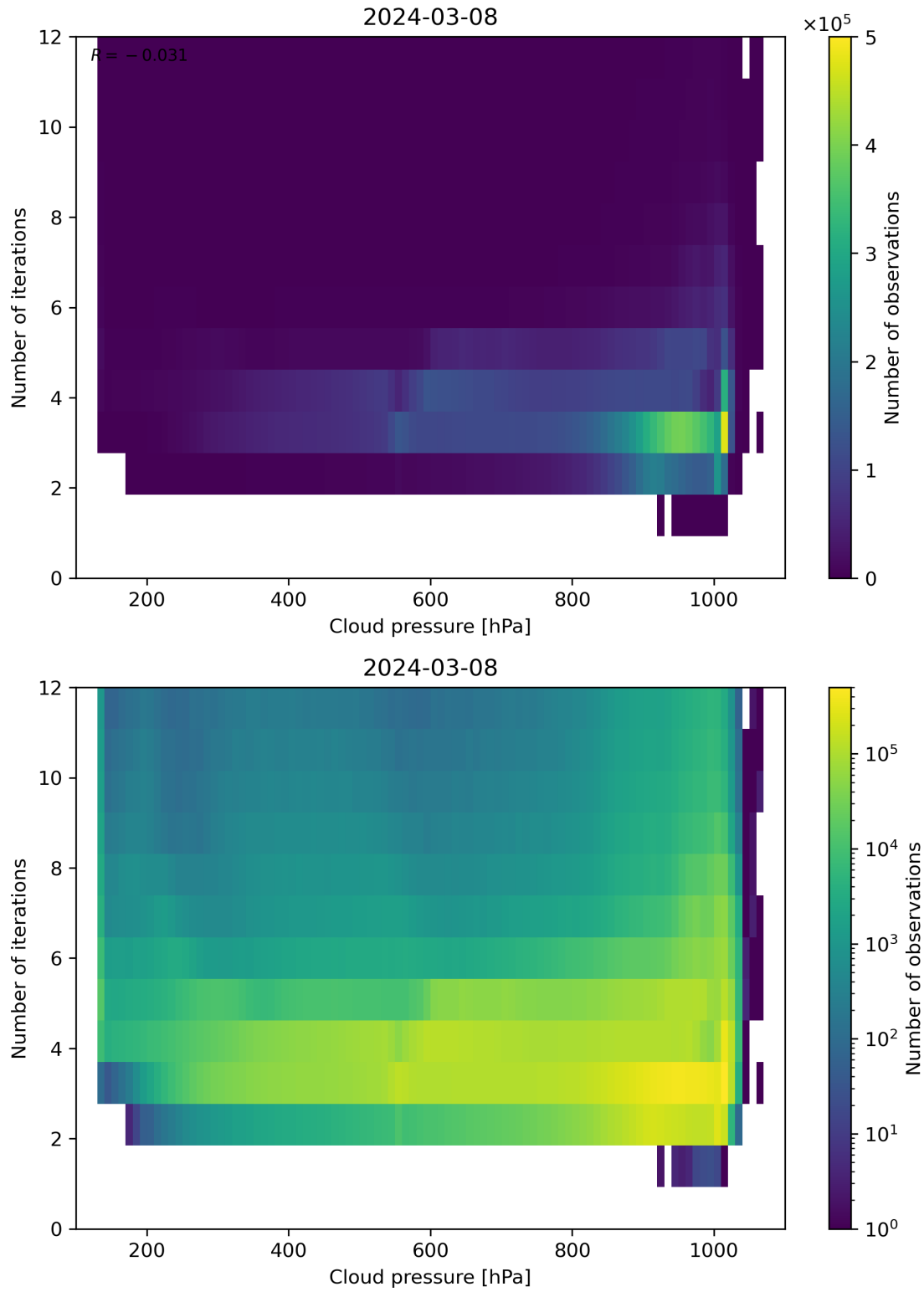
Figure 81: Scatter density plot of “Cloud pressure” against “Number of iterations” for 2024-03-07 to 2024-03-09.
