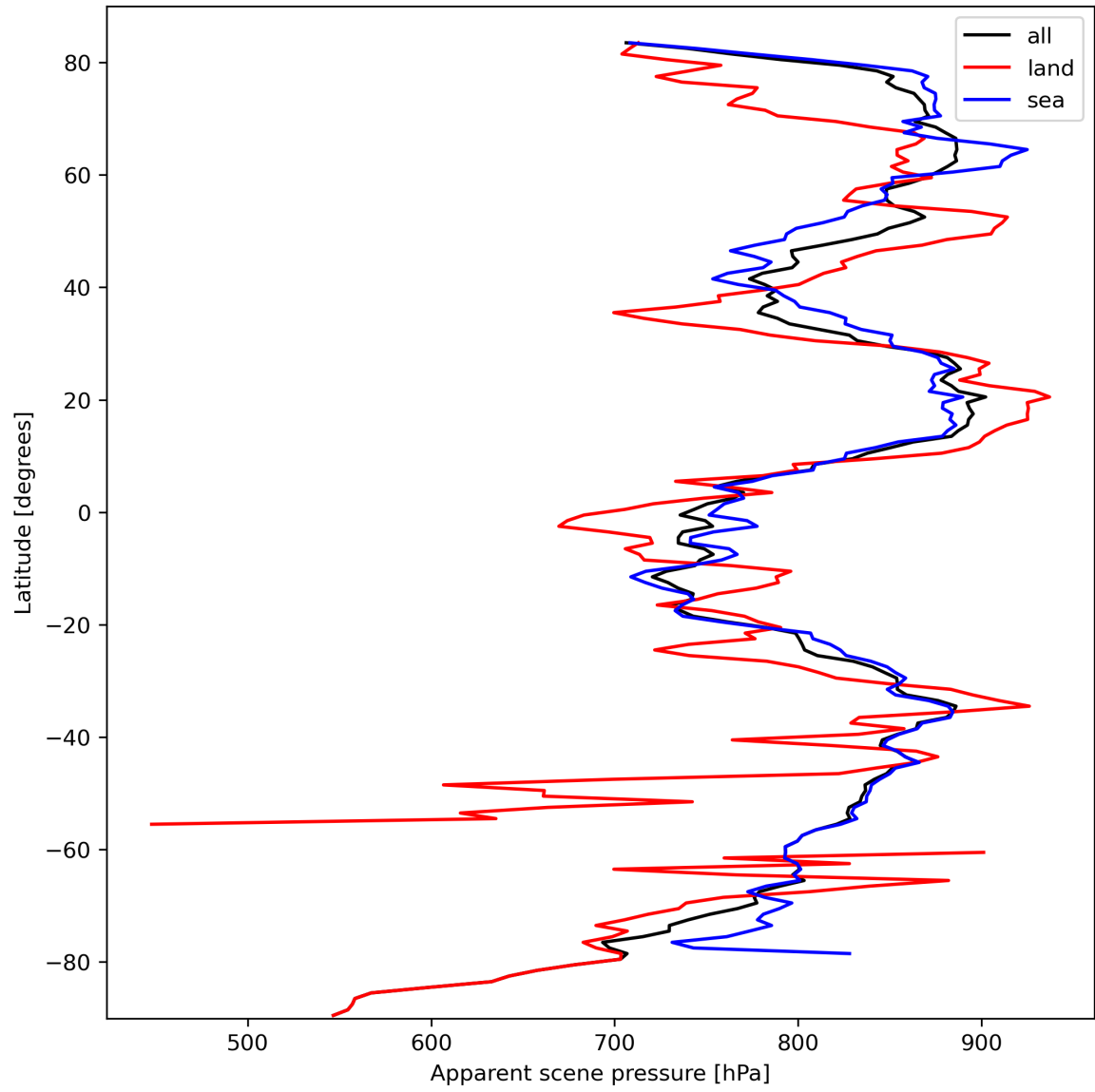
Figure 19: Zonal average of “Apparent scene pressure” for 2024-03-07 to 2024-03-09.
