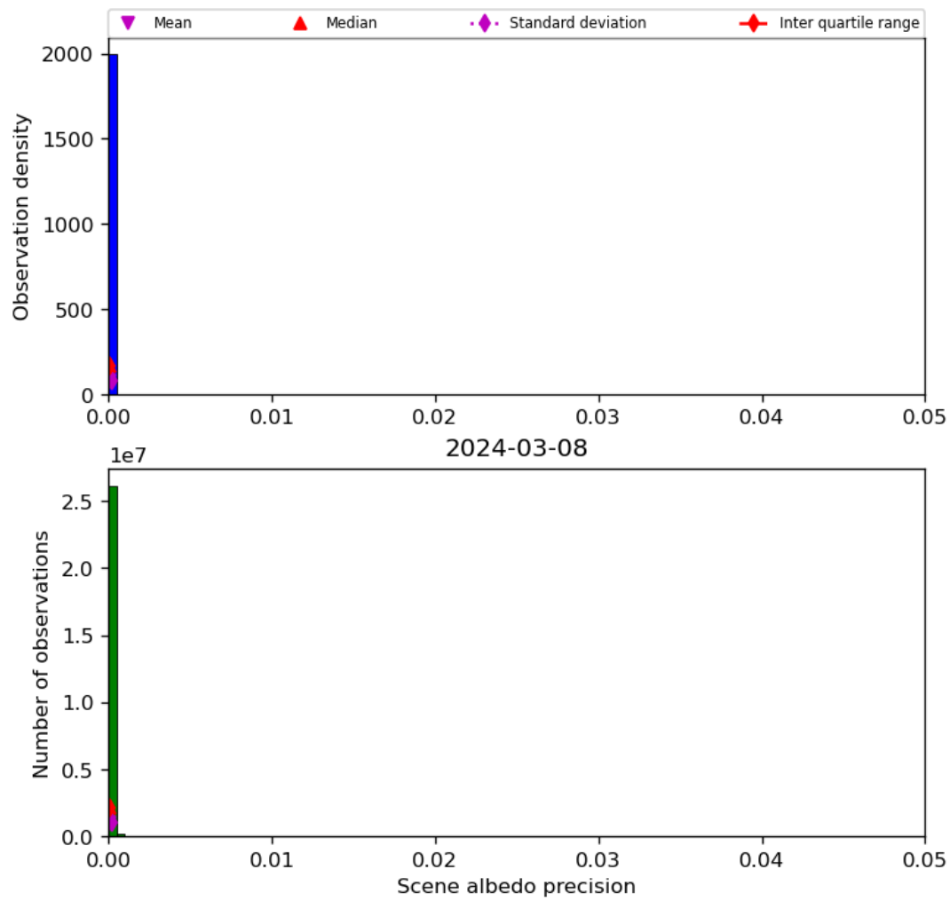
Figure 35: Histogram of “Scene albedo precision” for 2024-03-07 to 2024-03-09
