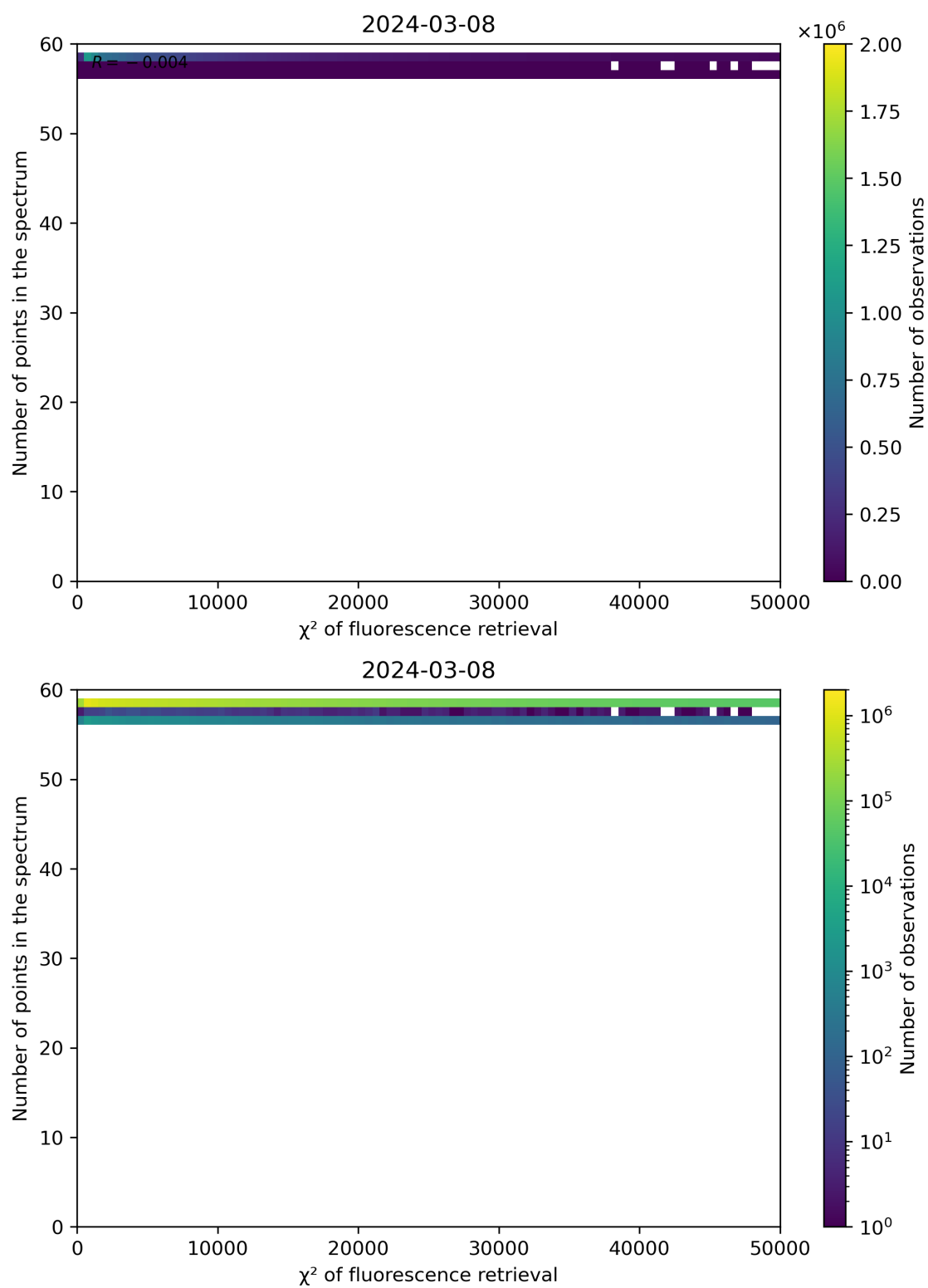
Figure 68: Scatter density plot of " \chi^2 of fluorescence retrieval" against "Number of points in the spectrum" for 2024-03-07 to 2024-03-09.
