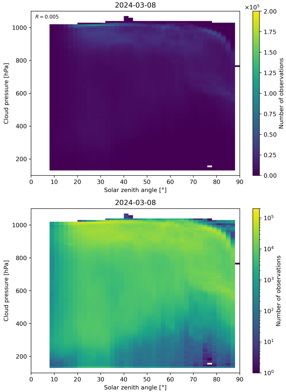
Figure 111: Scatter density plot of “Solar zenith angle” against “Cloud pressure” for 2024-03-07 to 2024-03-09.
