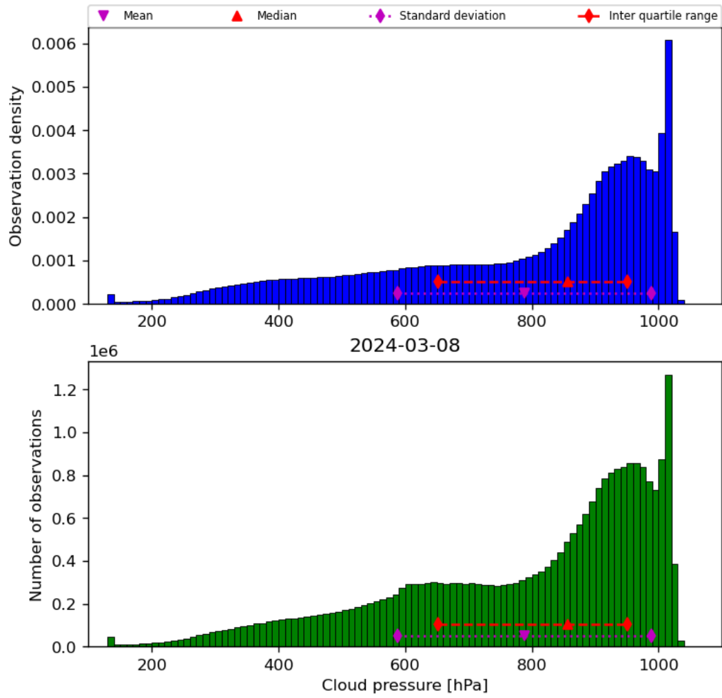
Figure 30: Histogram of “Cloud pressure” for 2024-03-07 to 2024-03-09
