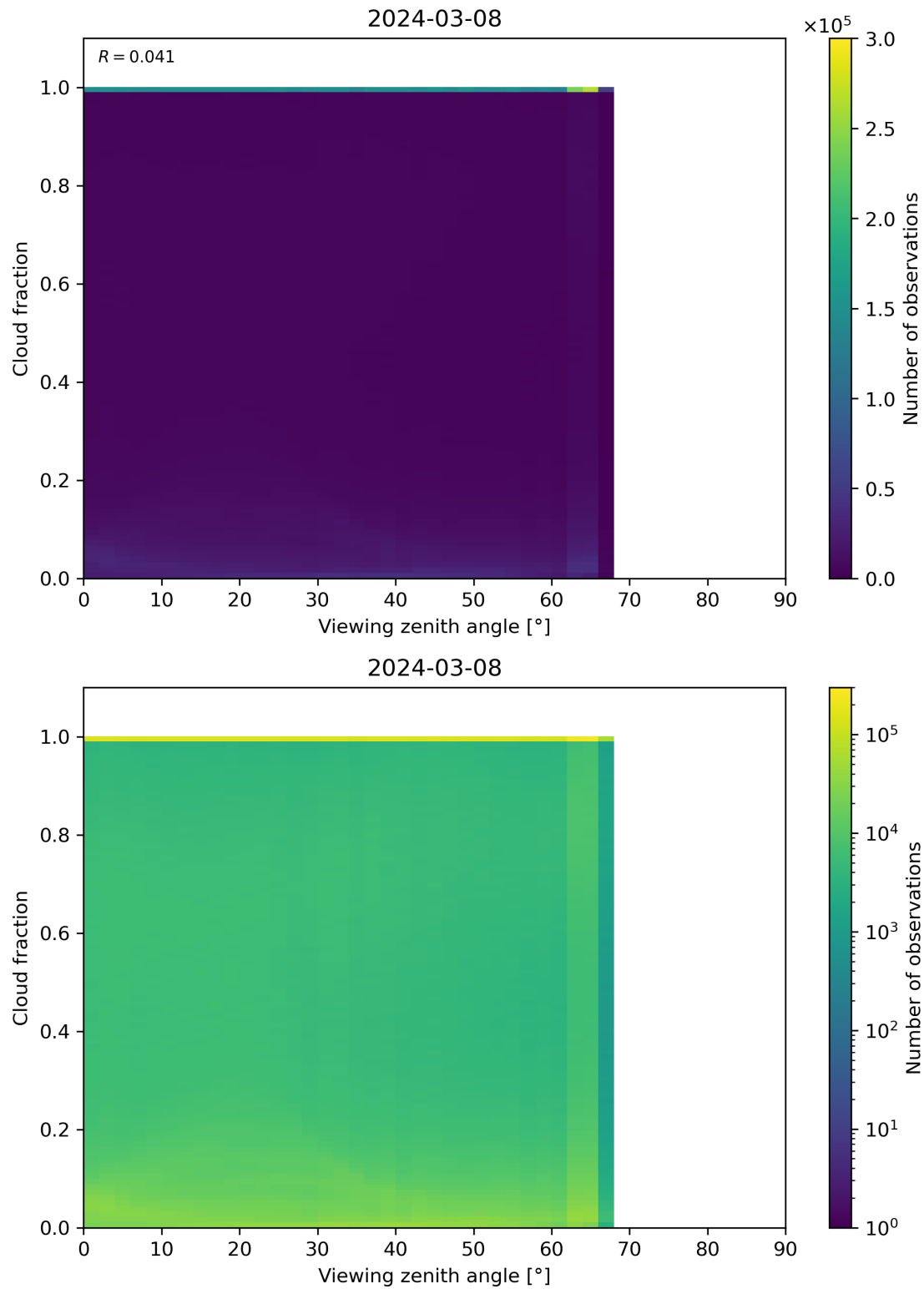
Figure 120: Scatter density plot of “Viewing zenith angle” against “Cloud fraction” for 2024-03-07 to 2024-03-09.
