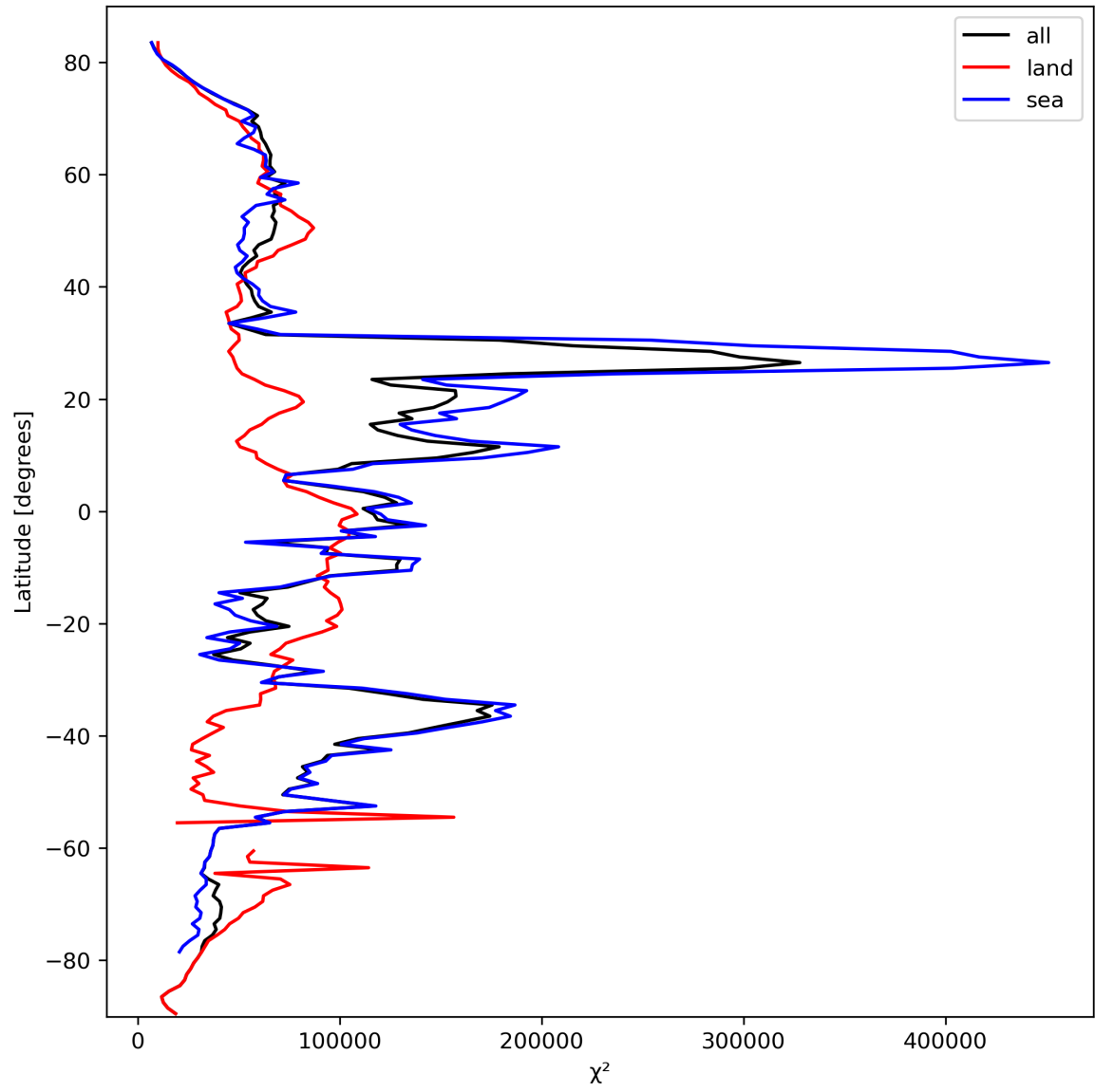
Figure 21: Zonal average of “ \chi^2 ” for 2024-03-07 to 2024-03-09.
