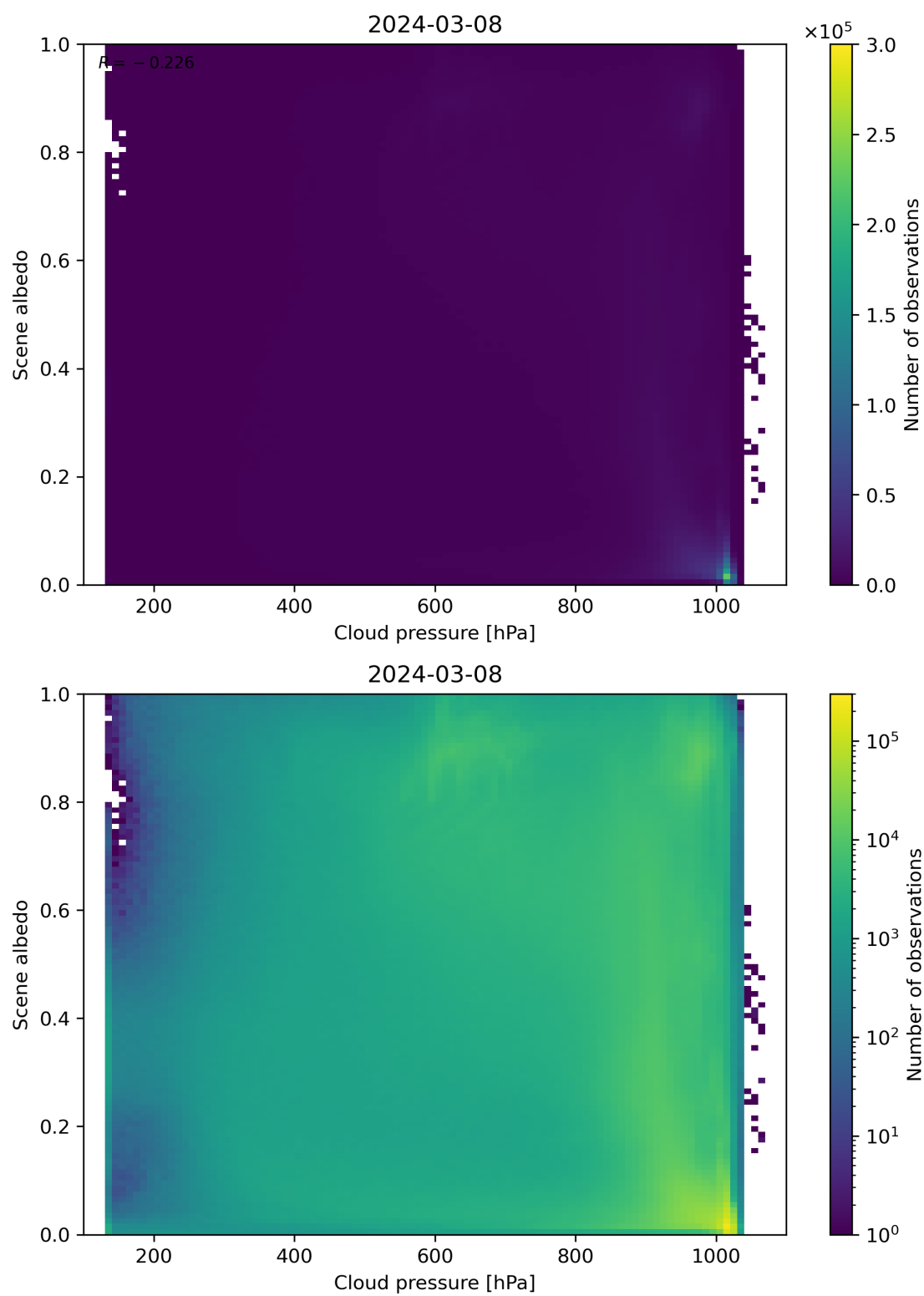
Figure 83: Scatter density plot of “Cloud pressure” against “Scene albedo” for 2024-03-07 to 2024-03-09.
