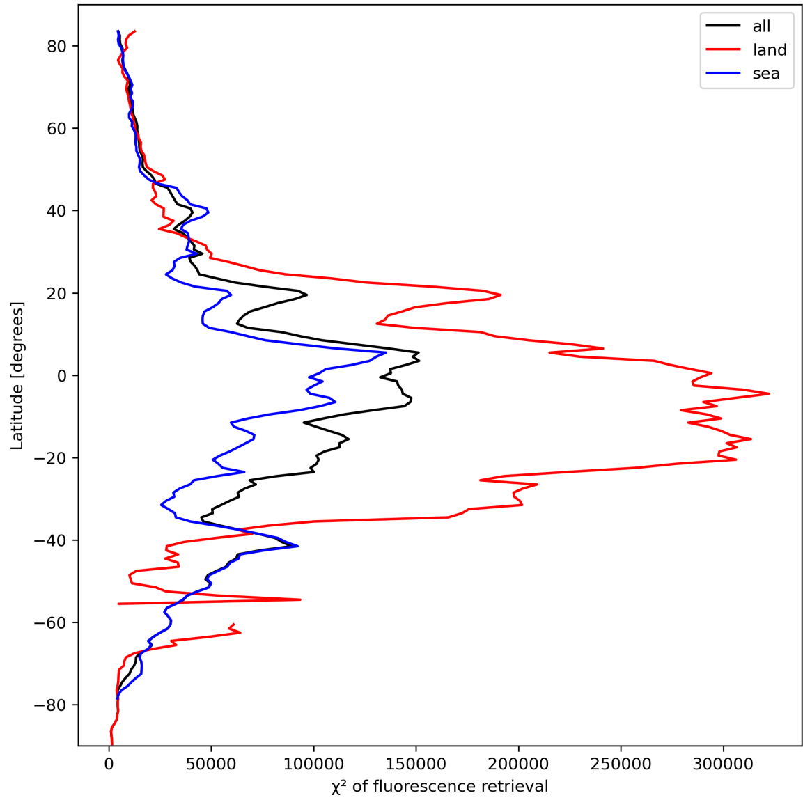
Figure 25: Zonal average of “ \chi^2 of fluorescence retrieval” for 2024-03-07 to 2024-03-09.
