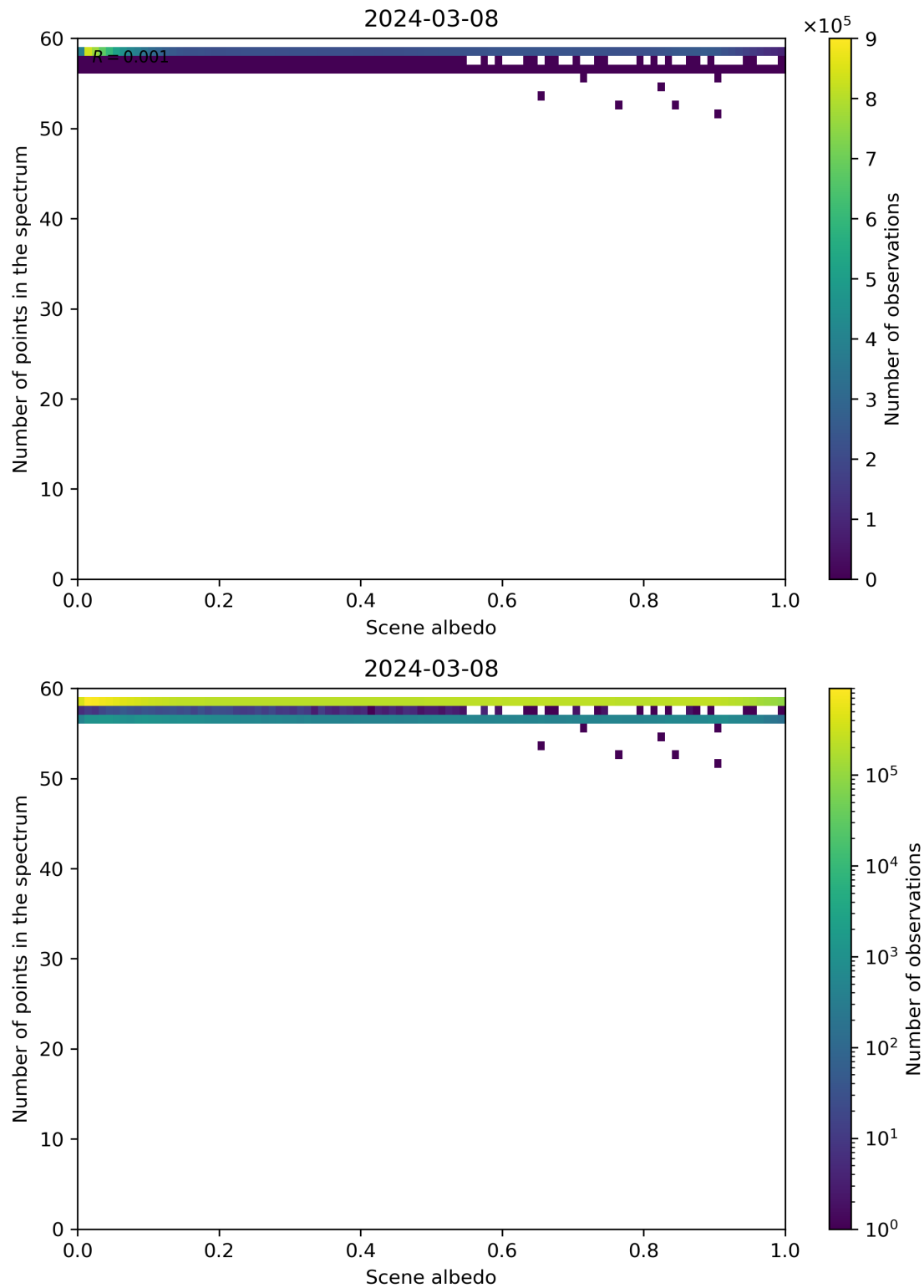
Figure 106: Scatter density plot of “Scene albedo” against “Number of points in the spectrum” for 2024-03-07 to 2024-03-09.
