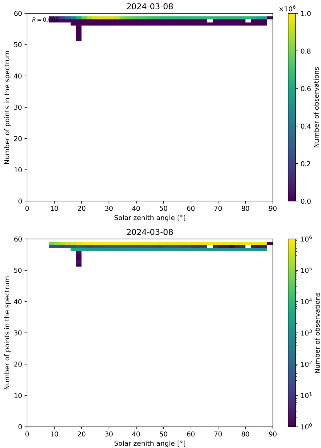
Figure 115: Scatter density plot of “Solar zenith angle” against “Number of points in the spectrum” for 2024-03-07 to 2024-03-09.
