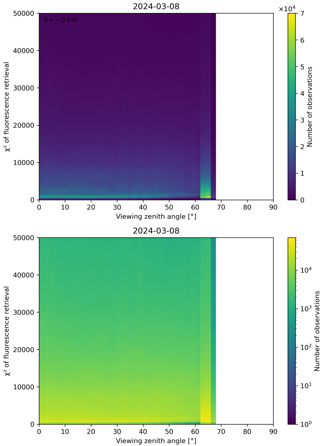
Figure 119: Scatter density plot of “Viewing zenith angle” against “ \chi^2 of fluorescence retrieval” for 2024-03-07 to 2024-03-09.
