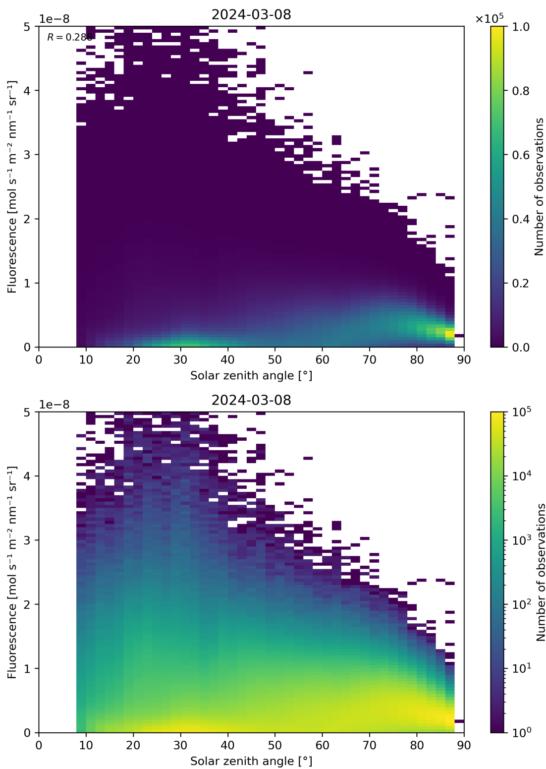
Figure 112: Scatter density plot of “Solar zenith angle” against “Fluorescence” for 2024-03-07 to 2024-03-09.
