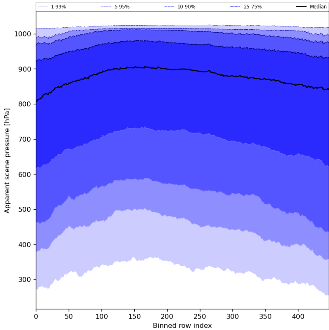
Figure 53: Along track statistics of “Apparent scene pressure” for 2024-03-07 to 2024-03-09
