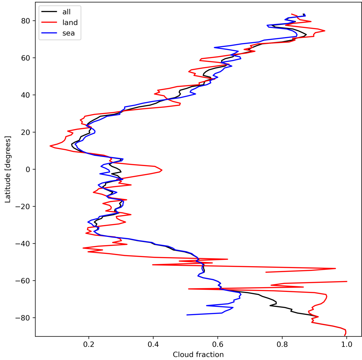
Figure 15: Zonal average of “Cloud fraction” for 2024-03-07 to 2024-03-09.
