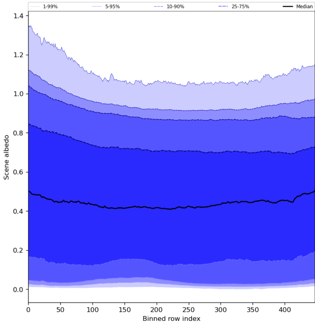
Figure 51: Along track statistics of “Scene albedo” for 2024-03-07 to 2024-03-09
