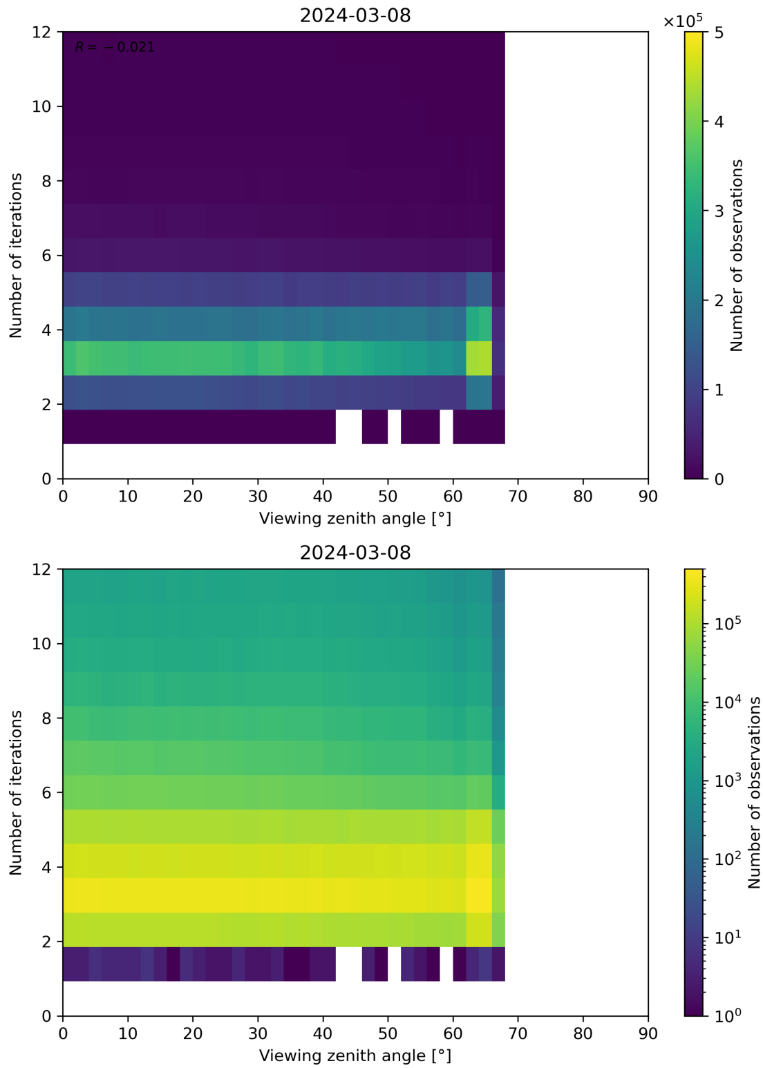
Figure 124: Scatter density plot of “Viewing zenith angle” against “Number of iterations” for 2024-03-07 to 2024-03-09.
