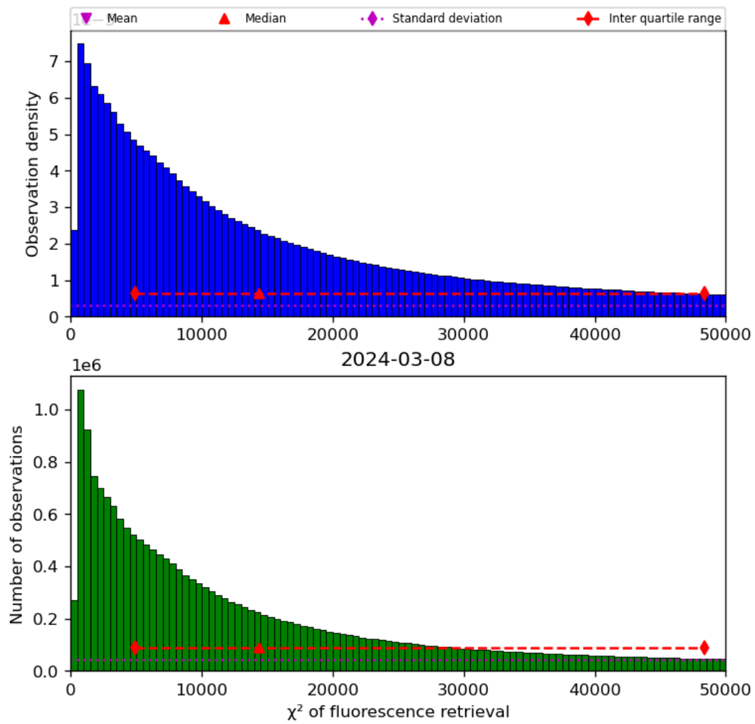
Figure 42: Histogram of “ \chi^2 of fluorescence retrieval” for 2024-03-07 to 2024-03-09
