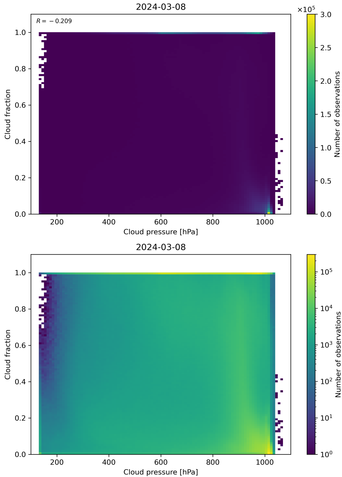
Figure 79: Scatter density plot of “Cloud pressure” against “Cloud fraction” for 2024-03-07 to 2024-03-09.
