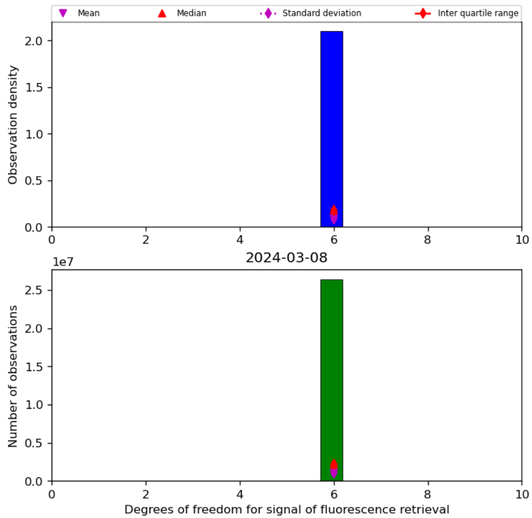
Figure 43: Histogram of “Degrees of freedom for signal of fluorescence retrieval” for 2024-03-07 to 2024-03-09
