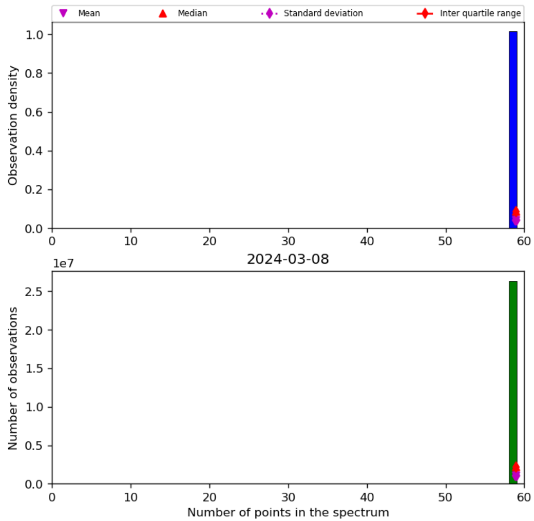
Figure 44: Histogram of "Number of points in the spectrum" for 2024-03-07 to 2024-03-09
