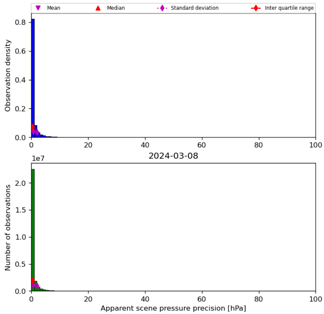
Figure 37: Histogram of “Apparent scene pressure precision” for 2024-03-07 to 2024-03-09
