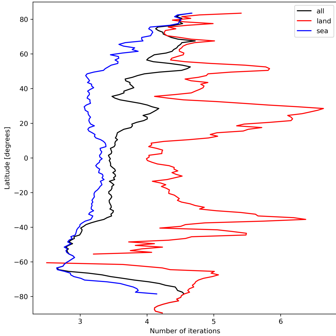
Figure 22: Zonal average of “Number of iterations” for 2024-03-07 to 2024-03-09.
