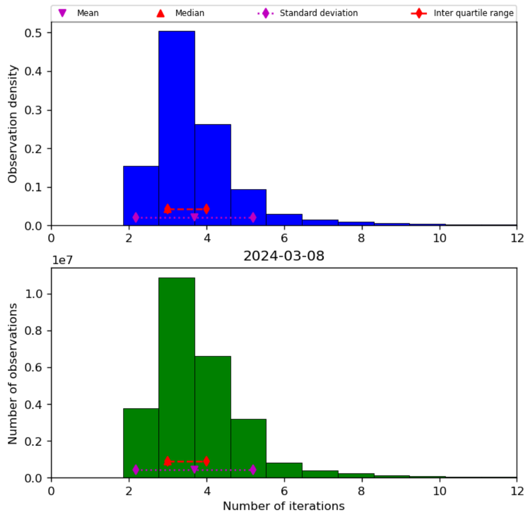
Figure 39: Histogram of “Number of iterations” for 2024-03-07 to 2024-03-09
