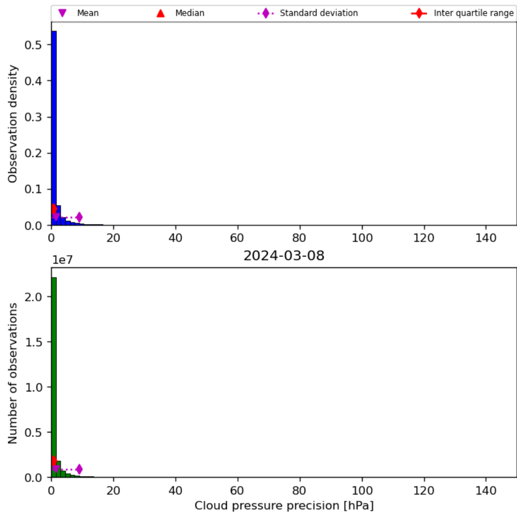
Figure 31: Histogram of “Cloud pressure precision” for 2024-03-07 to 2024-03-09
