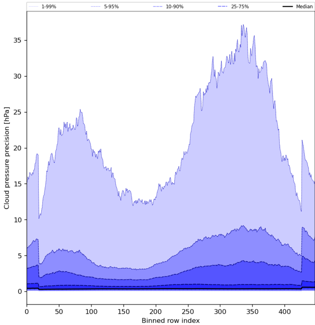
Figure 48: Along track statistics of “Cloud pressure precision” for 2024-03-07 to 2024-03-09
