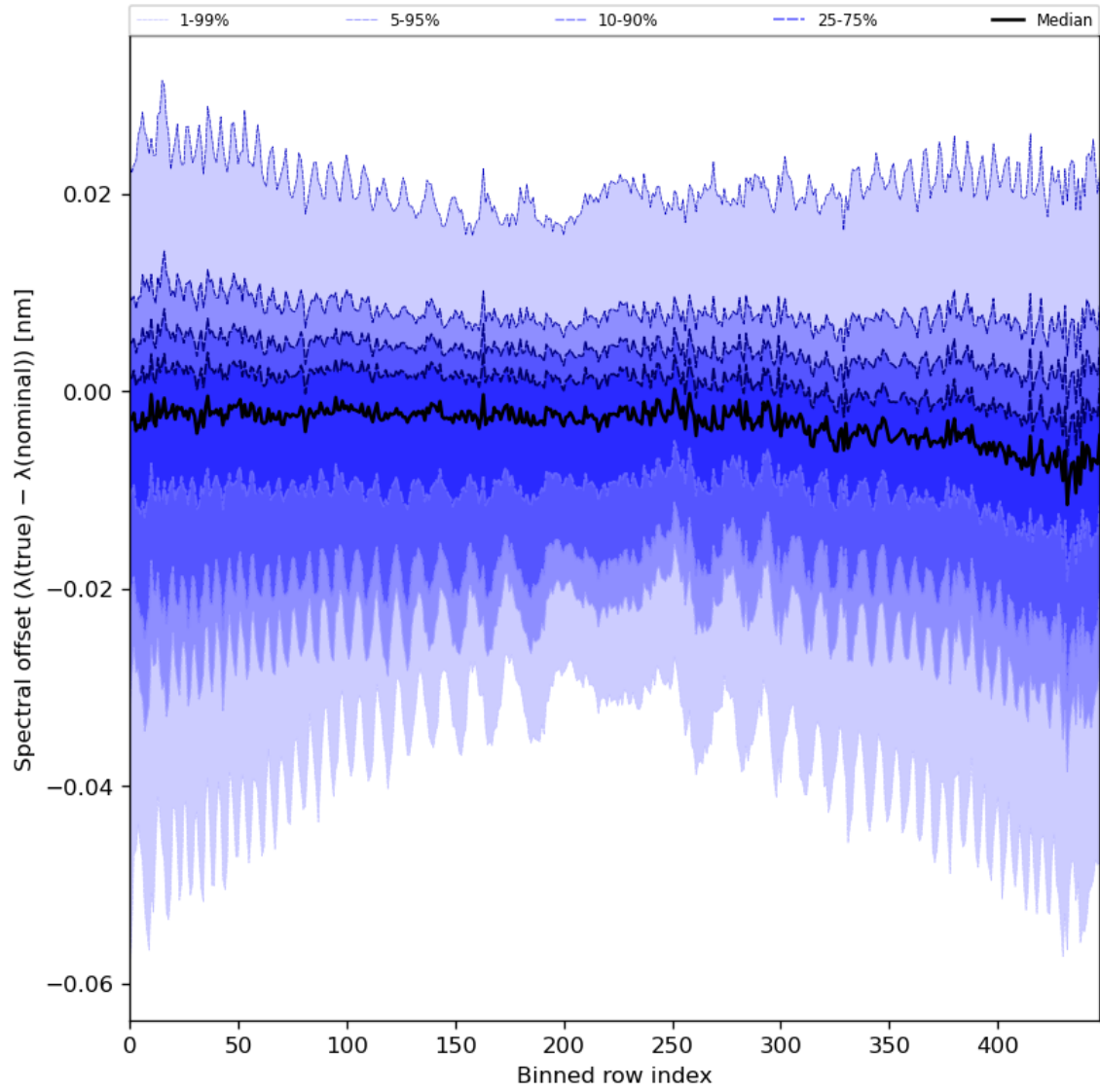
Figure 62: Along track statistics of “Spectral offset ( \lambda(\text{true}) - \lambda(\text{nominal}) )” for 2024-03-07 to 2024-03-09
