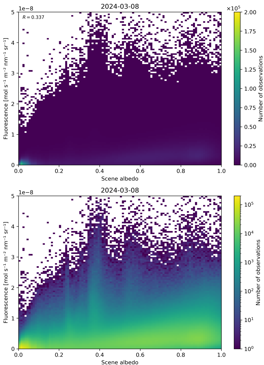
Figure 104: Scatter density plot of “Scene albedo” against “Fluorescence” for 2024-03-07 to 2024-03-09.
