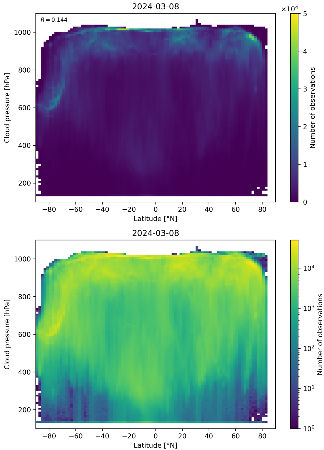
Figure 91: Scatter density plot of “Latitude” against “Cloud pressure” for 2024-03-07 to 2024-03-09.
