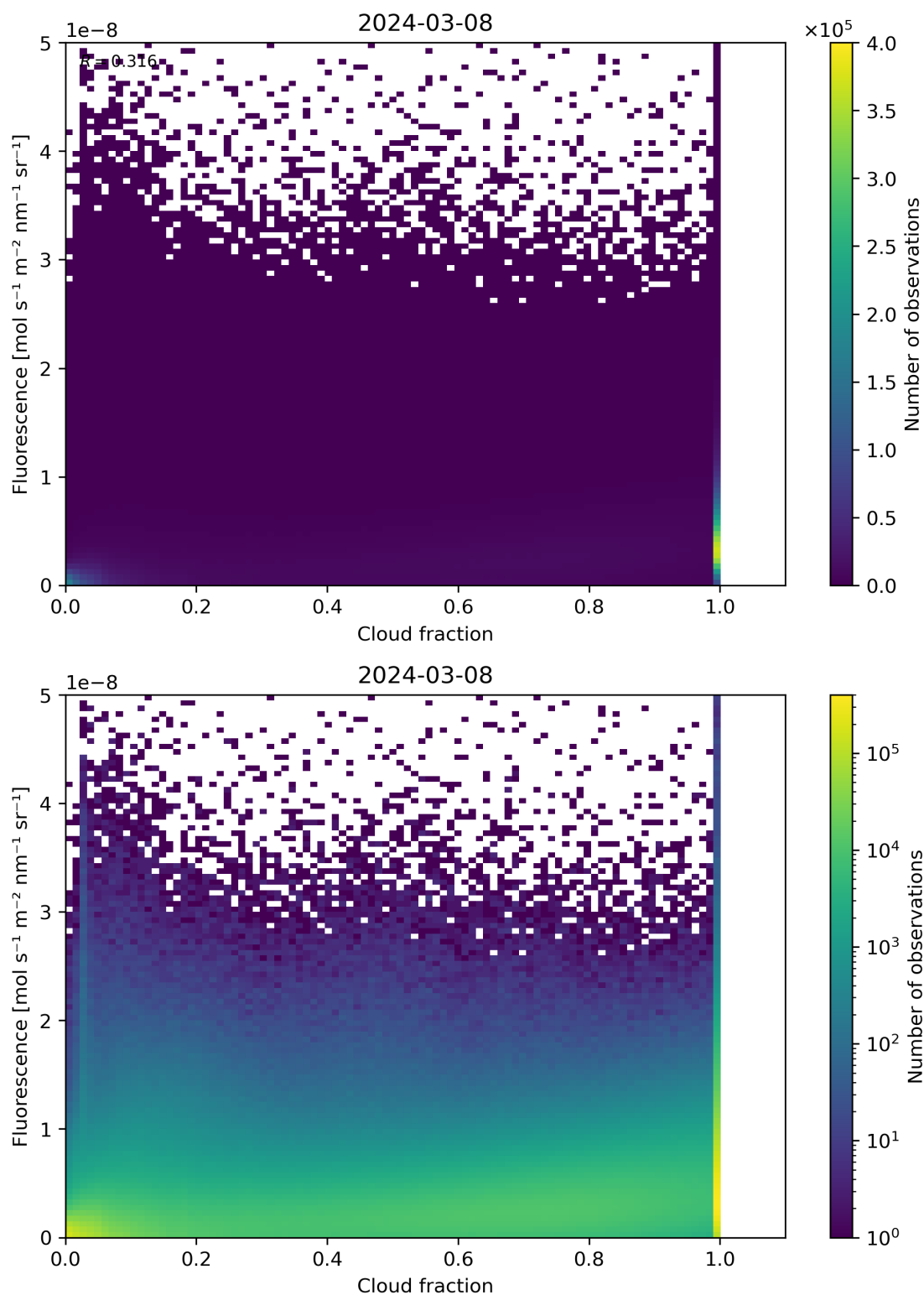
Figure 72: Scatter density plot of “Cloud fraction” against “Fluorescence” for 2024-03-07 to 2024-03-09.
