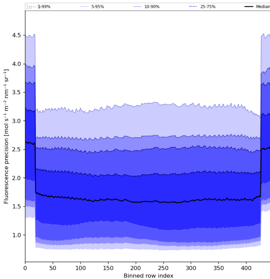
Figure 58: Along track statistics of “Fluorescence precision” for 2024-03-07 to 2024-03-09
