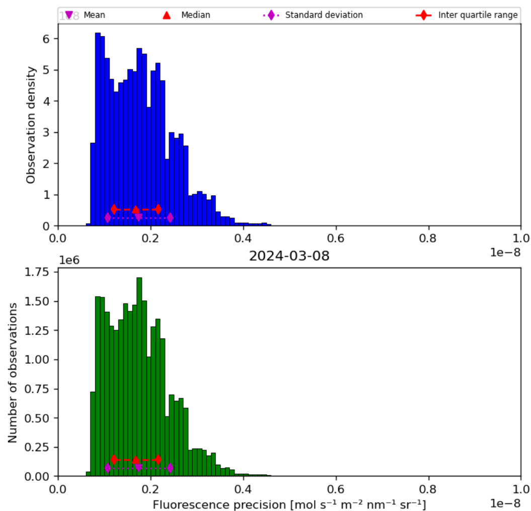
Figure 41: Histogram of “Fluorescence precision” for 2024-03-07 to 2024-03-09
