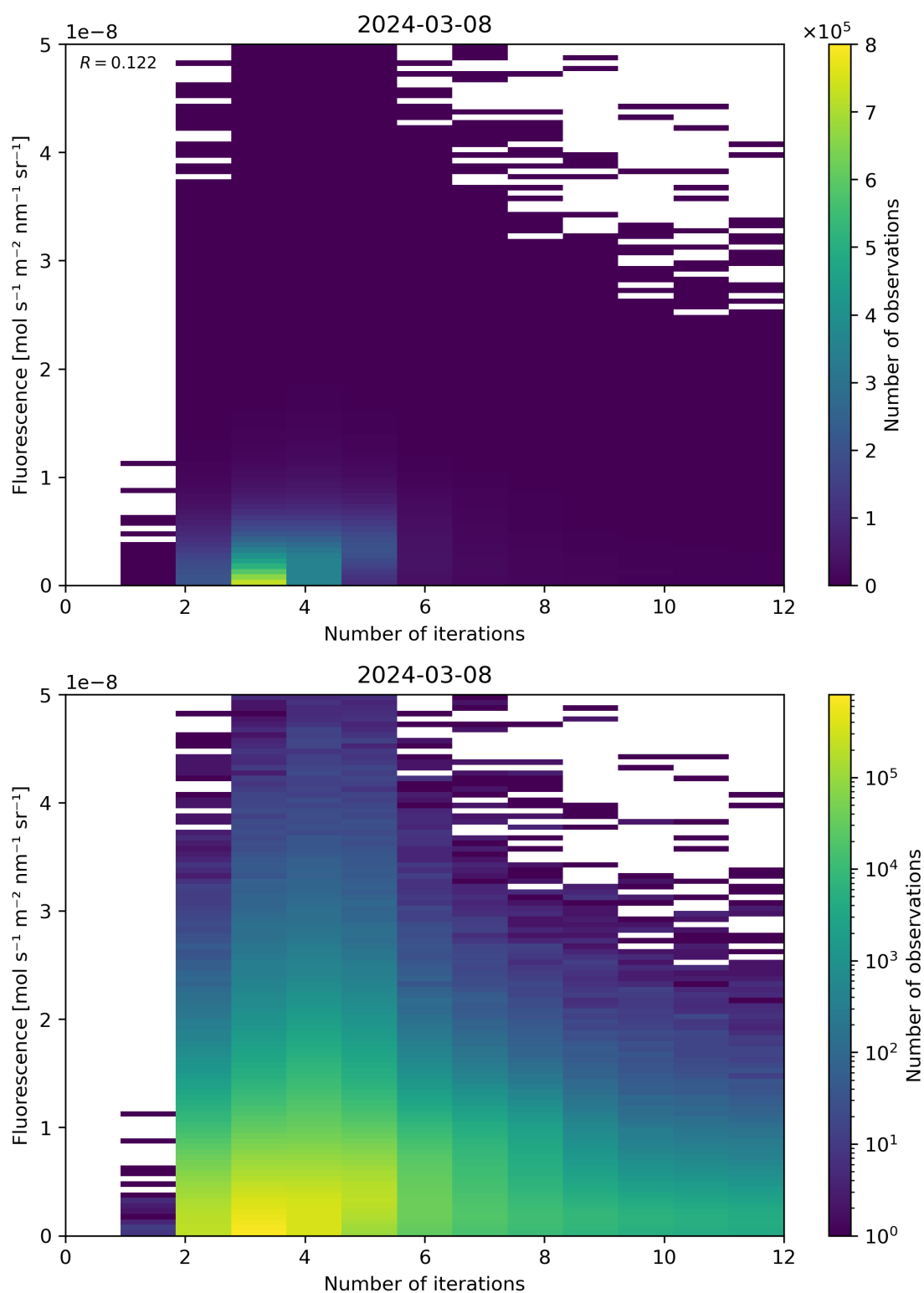
Figure 98: Scatter density plot of “Number of iterations” against “Fluorescence” for 2024-03-07 to 2024-03-09.
