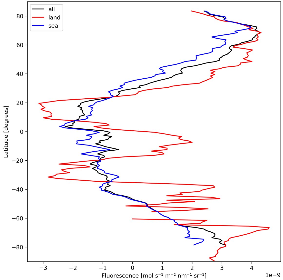
Figure 23: Zonal average of “Fluorescence” for 2024-03-07 to 2024-03-09.
