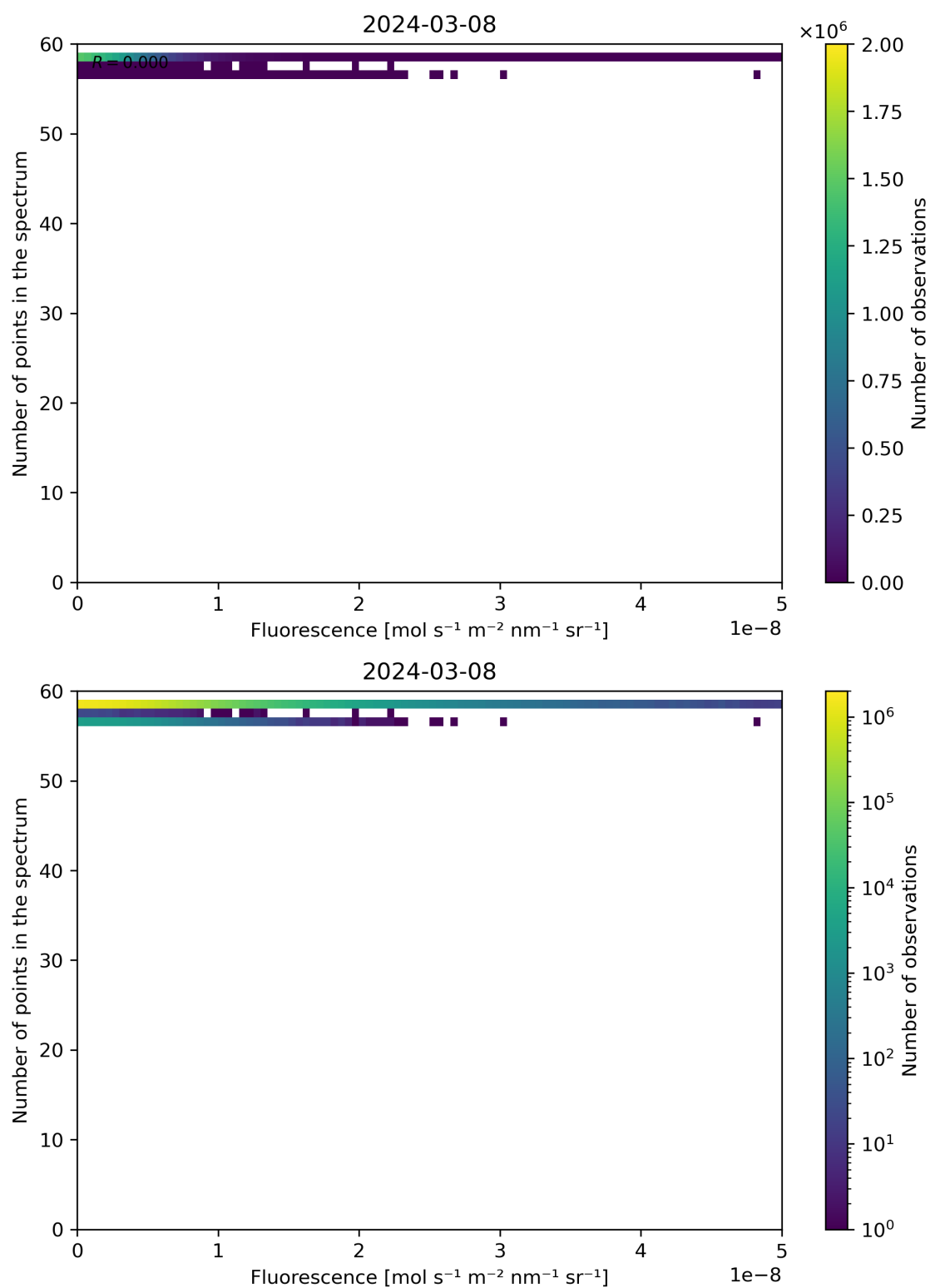
Figure 86: Scatter density plot of “Fluorescence” against “Number of points in the spectrum” for 2024-03-07 to 2024-03-09.
