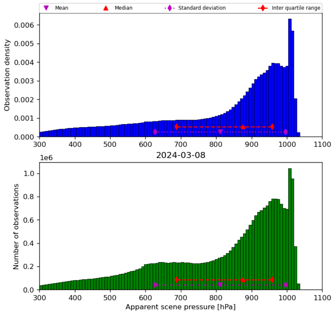
Figure 36: Histogram of “Apparent scene pressure” for 2024-03-07 to 2024-03-09
