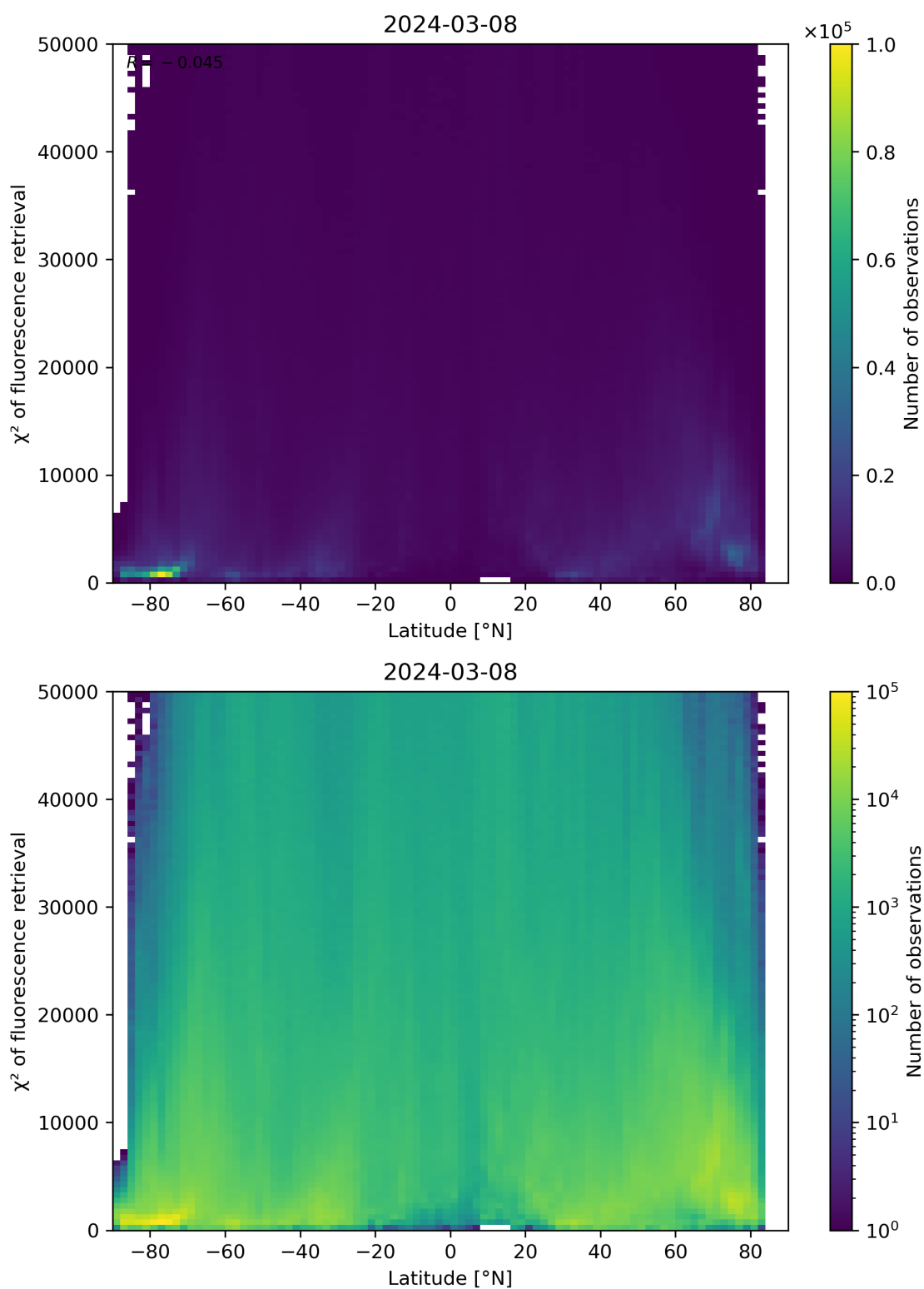
Figure 89: Scatter density plot of “Latitude” against “ \chi^2 of fluorescence retrieval” for 2024-03-07 to 2024-03-09.
