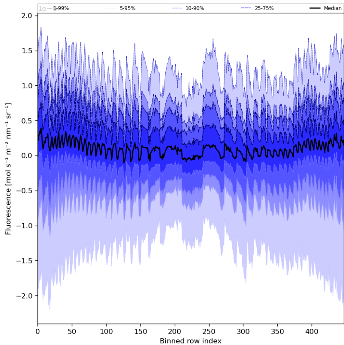
Figure 57: Along track statistics of “Fluorescence” for 2024-03-07 to 2024-03-09
