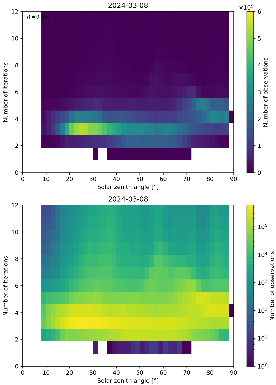
Figure 114: Scatter density plot of “Solar zenith angle” against “Number of iterations” for 2024-03-07 to 2024-03-09.
