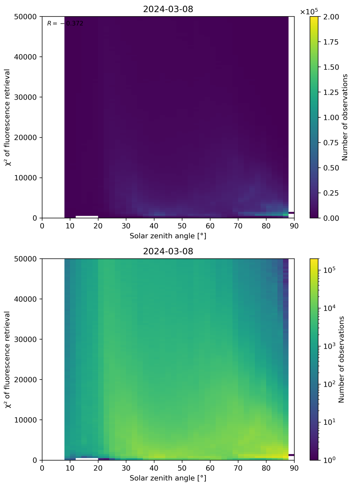
Figure 109: Scatter density plot of “Solar zenith angle” against “ \chi^2 of fluorescence retrieval” for 2024-03-07 to 2024-03-09.
