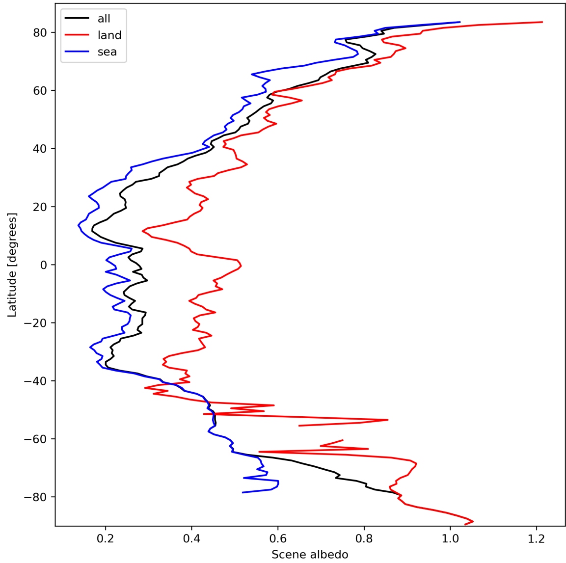
Figure 17: Zonal average of “Scene albedo” for 2024-03-07 to 2024-03-09.
