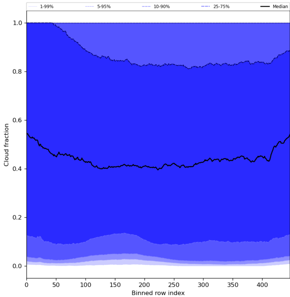
Figure 49: Along track statistics of “Cloud fraction” for 2024-03-07 to 2024-03-09
