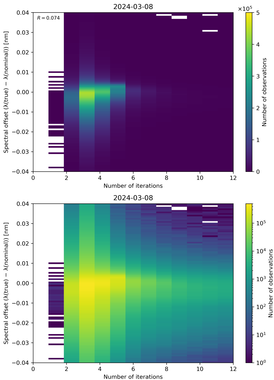
Figure 100: Scatter density plot of “Number of iterations” against “Spectral offset ( \lambda(\text{true}) - \lambda(\text{nominal}) )” for 2024-03-07 to 2024-03-09.
