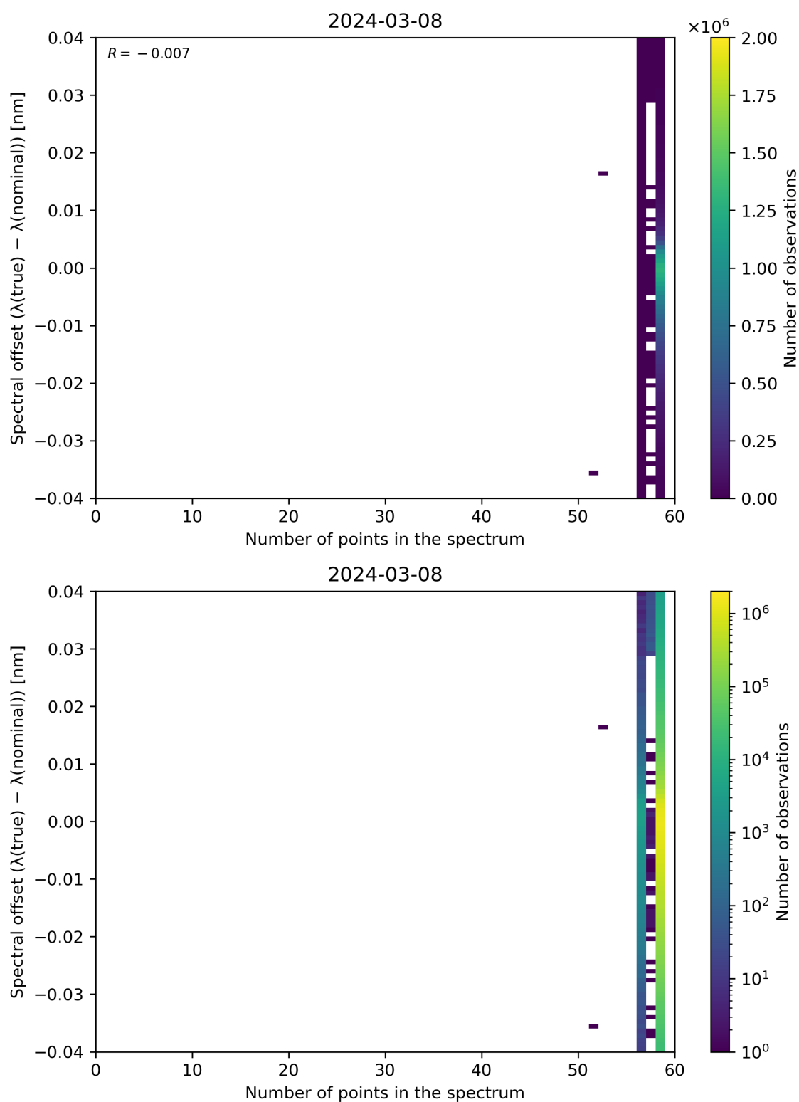
Figure 101: Scatter density plot of “Number of points in the spectrum” against “Spectral offset ( \lambda(\text{true}) - \lambda(\text{nominal}) )” for 2024-03-07 to 2024-03-09.
