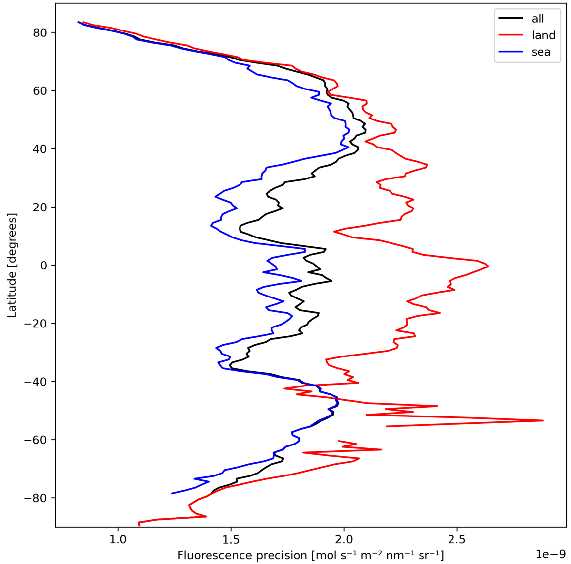
Figure 24: Zonal average of “Fluorescence precision” for 2024-03-07 to 2024-03-09.
