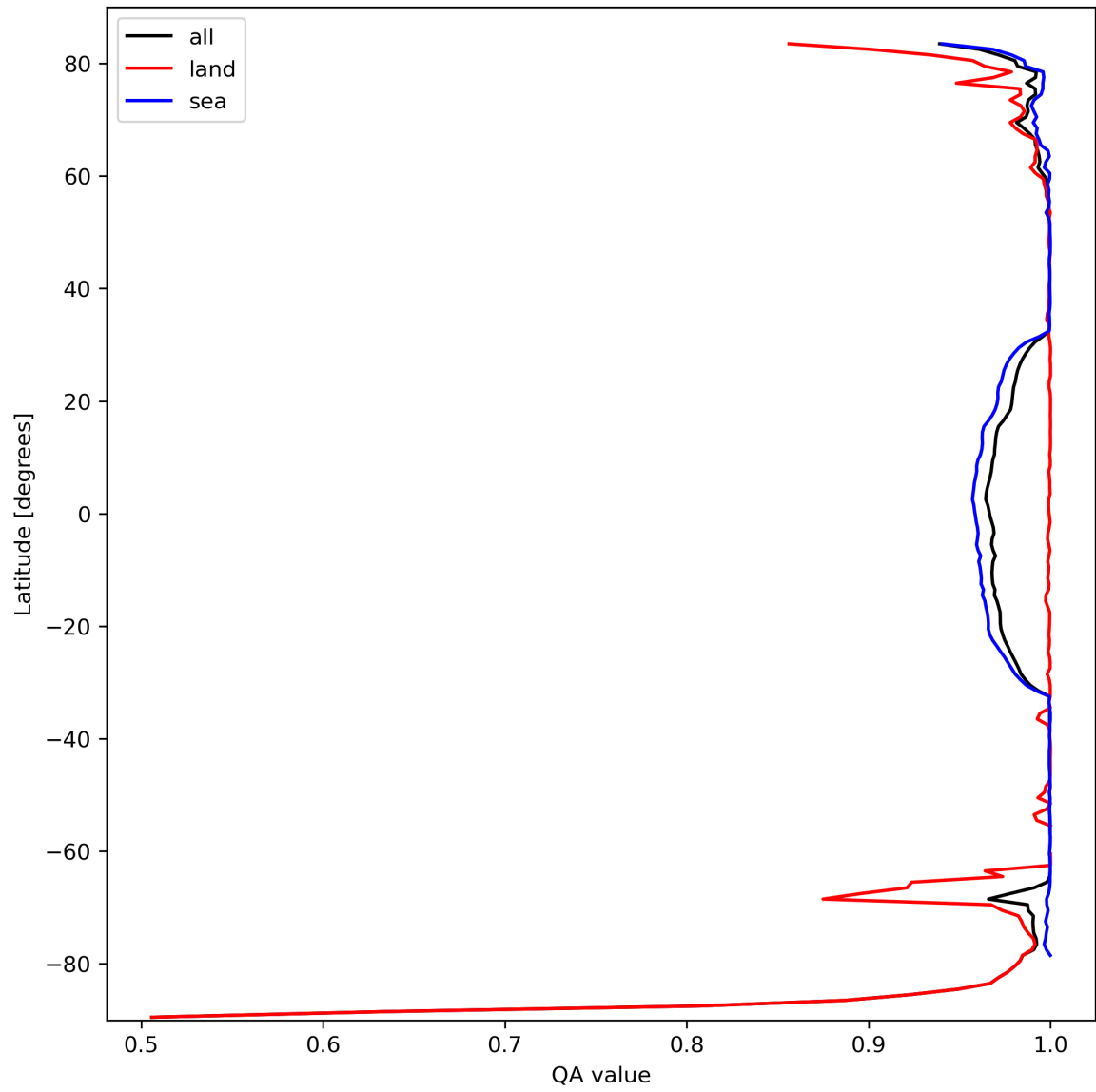
Figure 12: Zonal average of “QA value” for 2024-03-07 to 2024-03-09.
