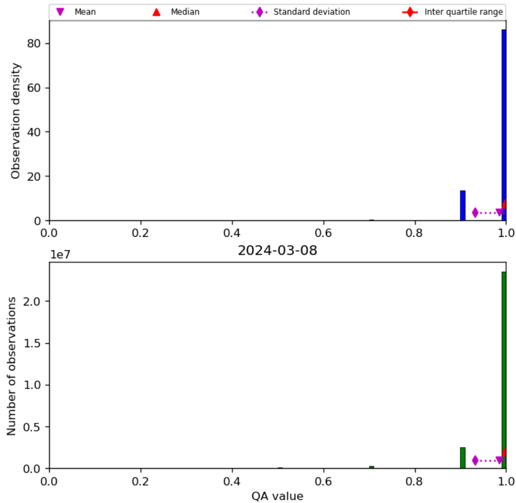
Figure 29: Histogram of “QA value” for 2024-03-07 to 2024-03-09
