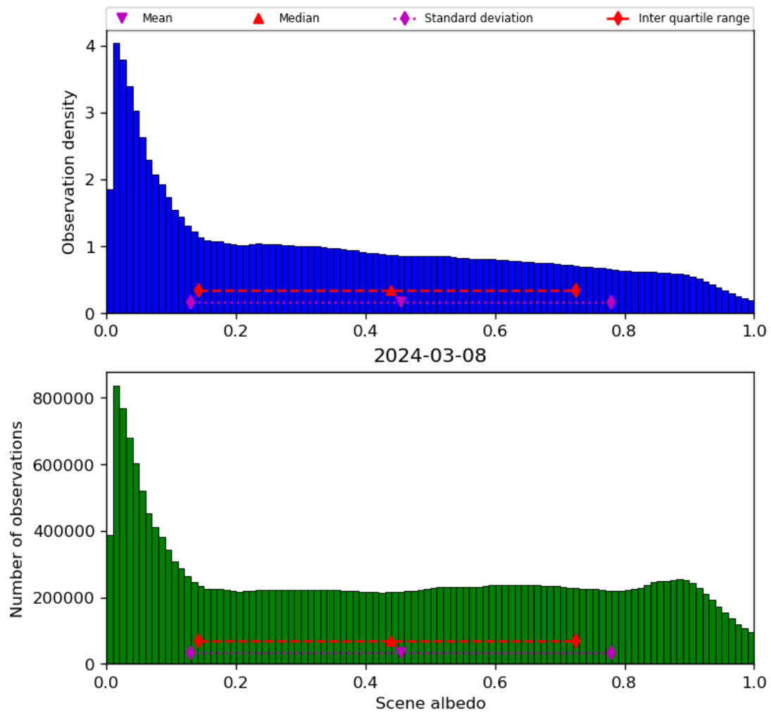
Figure 34: Histogram of “Scene albedo” for 2024-03-07 to 2024-03-09
