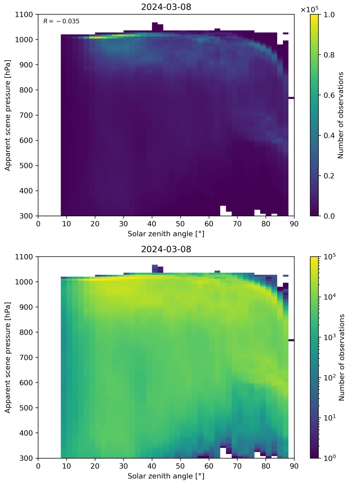
Figure 108: Scatter density plot of “Solar zenith angle” against “Apparent scene pressure” for 2024-03-07 to 2024-03-09.
