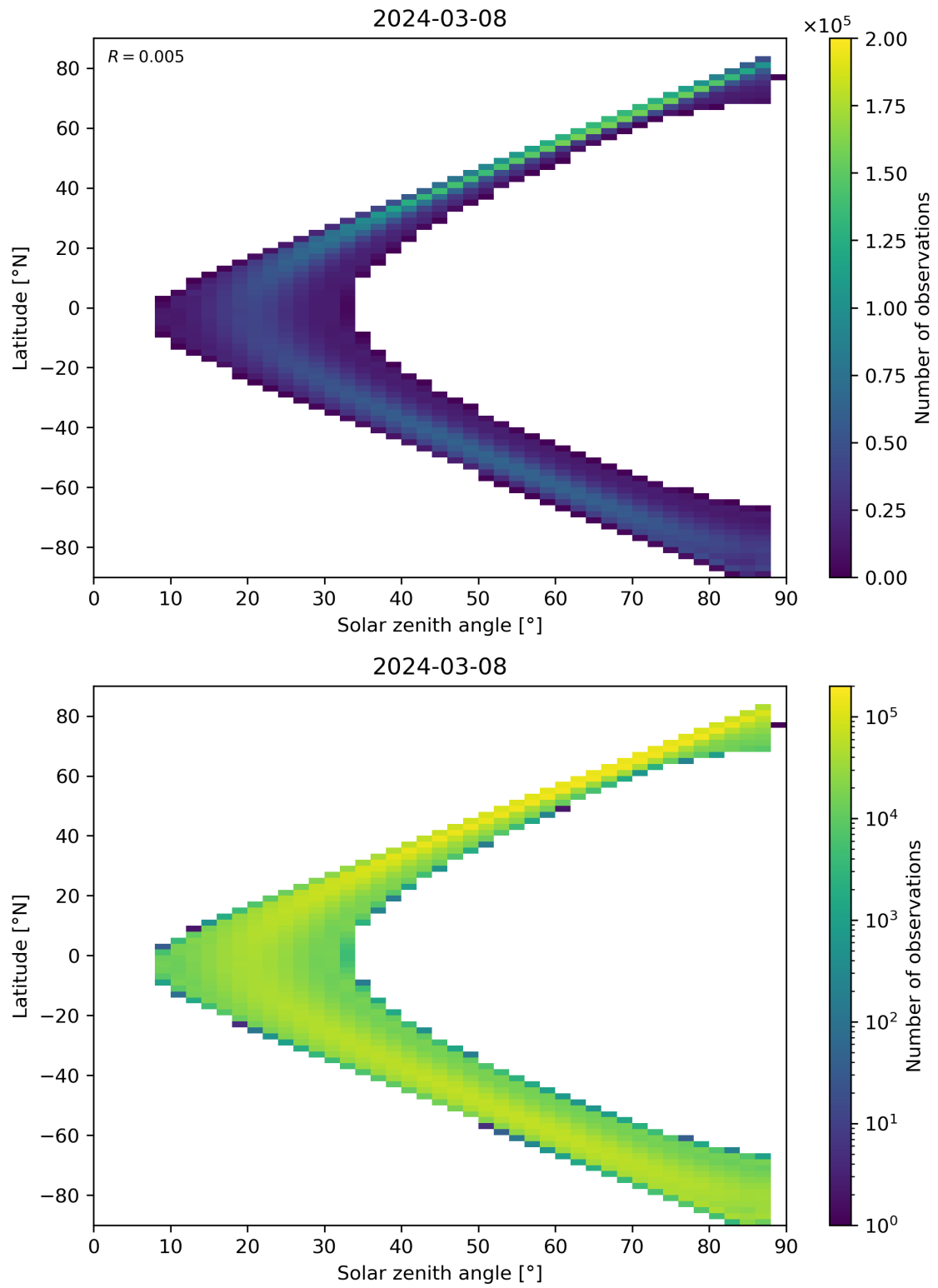
Figure 113: Scatter density plot of “Solar zenith angle” against “Latitude” for 2024-03-07 to 2024-03-09.
