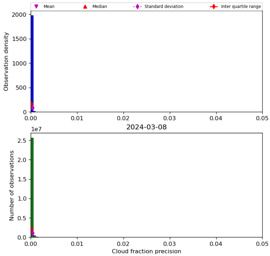
Figure 33: Histogram of “Cloud fraction precision” for 2024-03-07 to 2024-03-09
