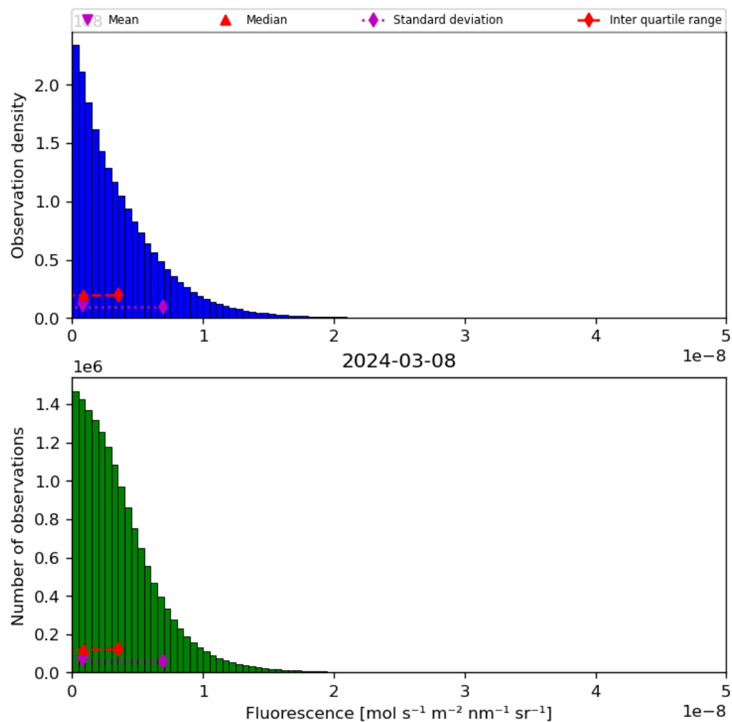
Figure 40: Histogram of “Fluorescence” for 2024-03-07 to 2024-03-09
