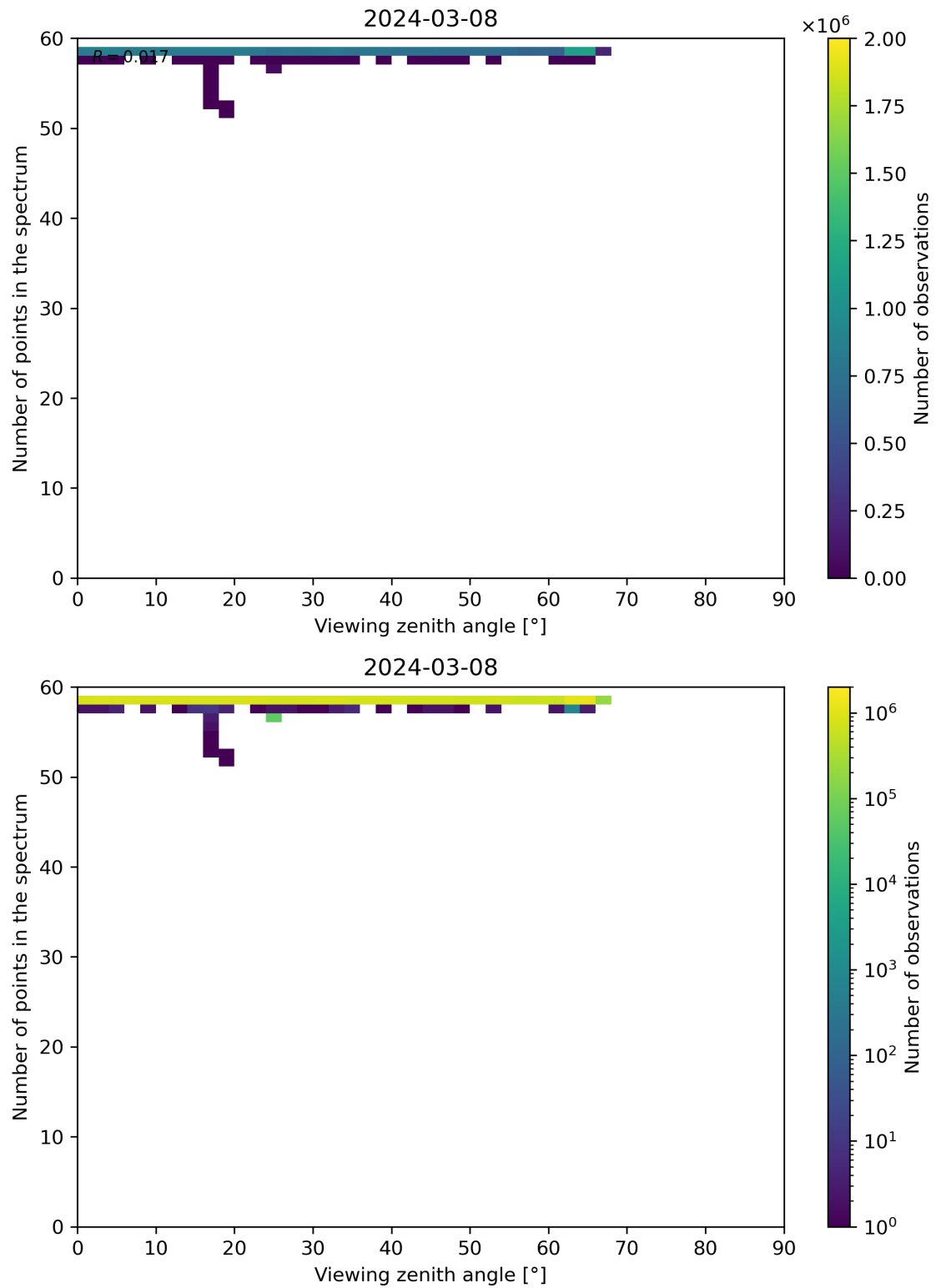
Figure 125: Scatter density plot of “Viewing zenith angle” against “Number of points in the spectrum” for 2024-03-07 to 2024-03-09.
