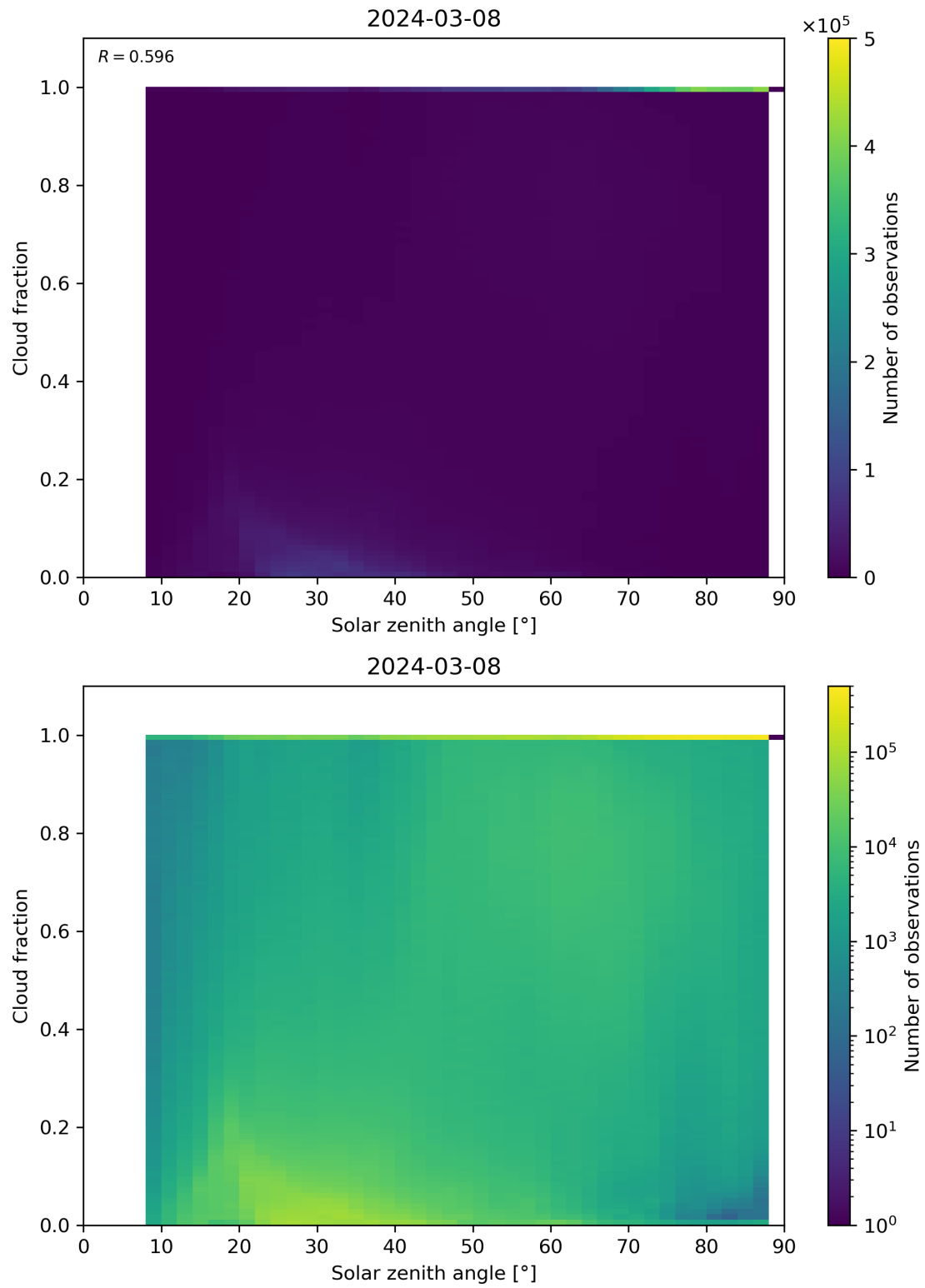
Figure 110: Scatter density plot of “Solar zenith angle” against “Cloud fraction” for 2024-03-07 to 2024-03-09.
