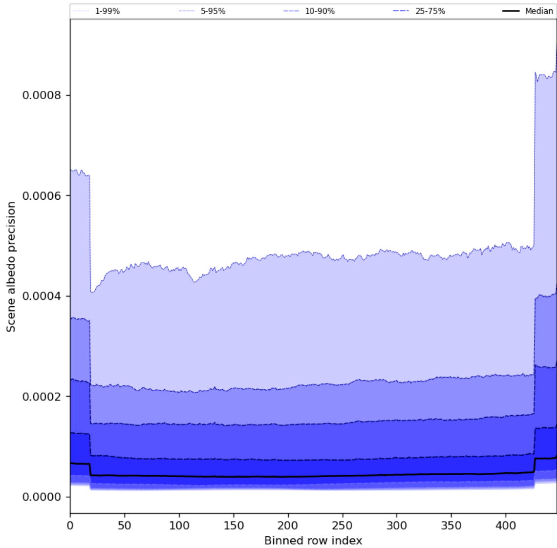
Figure 52: Along track statistics of “Scene albedo precision” for 2024-03-07 to 2024-03-09
