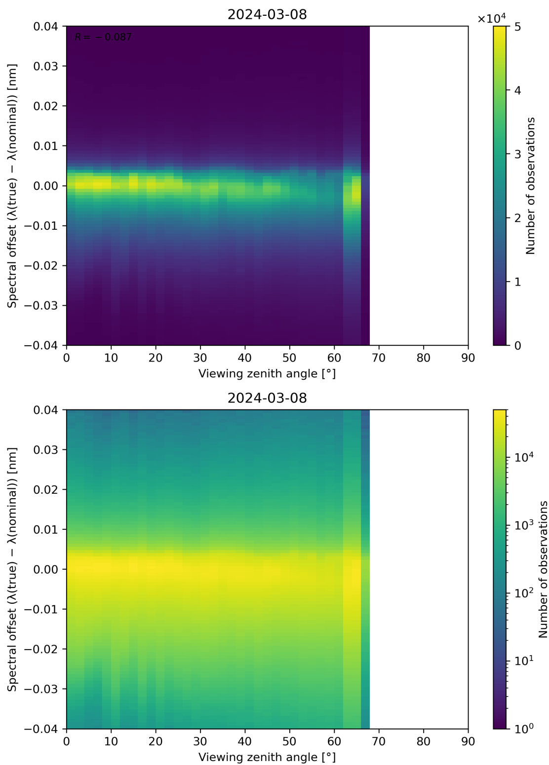
Figure 128: Scatter density plot of “Viewing zenith angle” against “Spectral offset ( \lambda(\text{true}) - \lambda(\text{nominal}) )” for 2024-03-07 to 2024-03-09.
