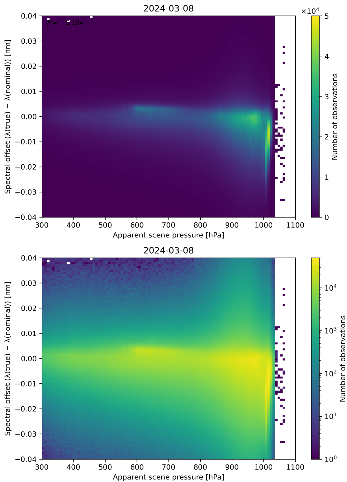
Figure 67: Scatter density plot of “Apparent scene pressure” against “Spectral offset ( \lambda(\text{true}) - \lambda(\text{nominal}) )” for 2024-03-07 to 2024-03-09.
