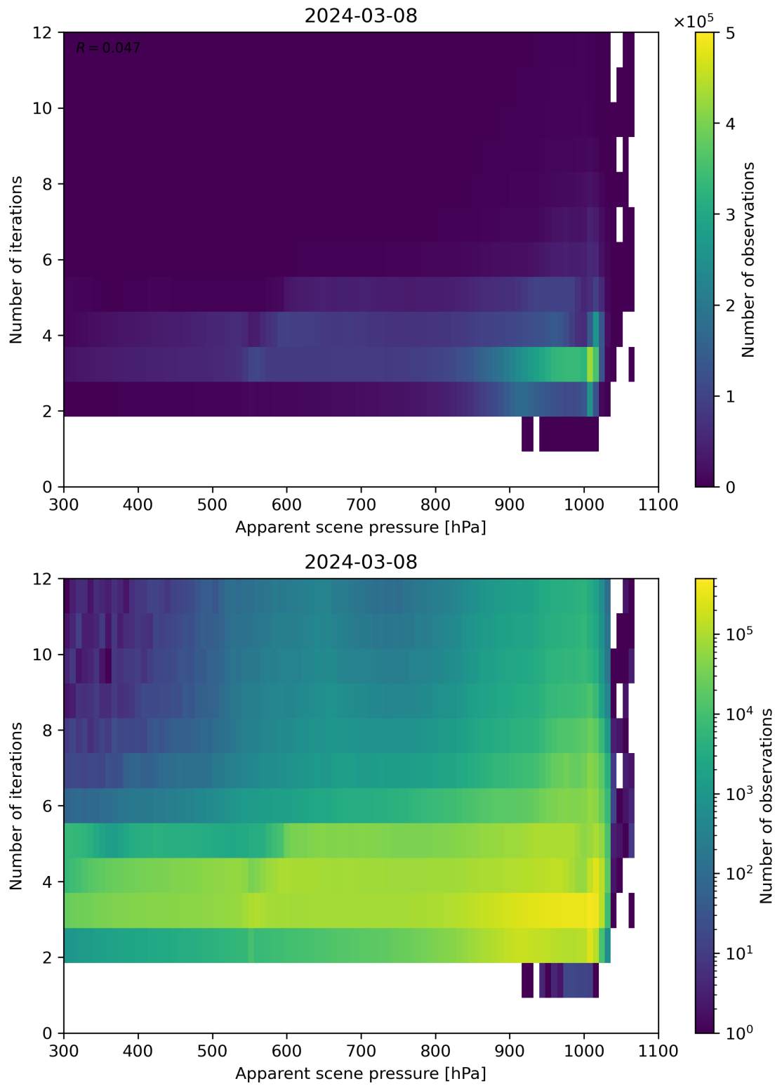
Figure 65: Scatter density plot of “Apparent scene pressure” against “Number of iterations” for 2024-03-07 to 2024-03-09.
