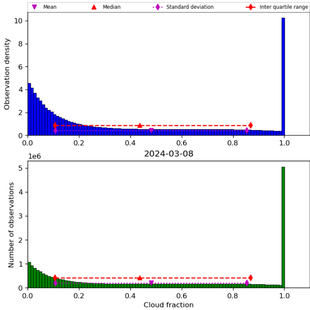
Figure 32: Histogram of “Cloud fraction” for 2024-03-07 to 2024-03-09
