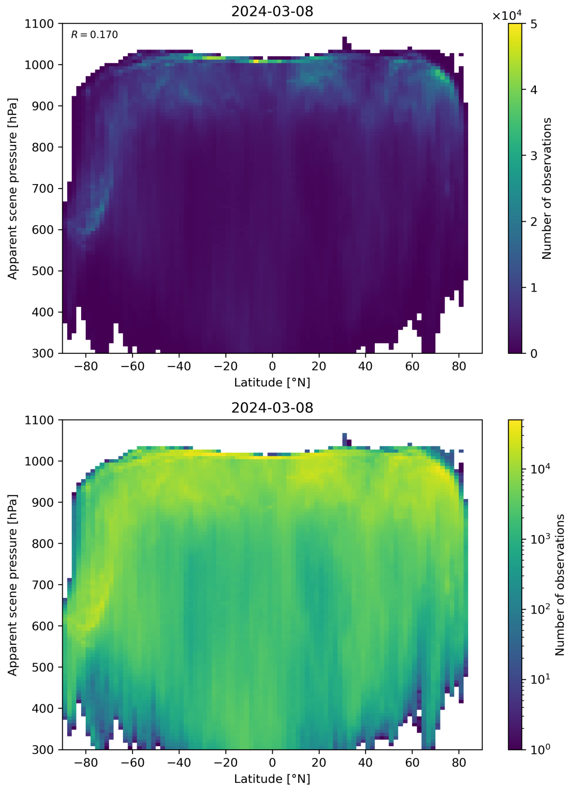
Figure 88: Scatter density plot of “Latitude” against “Apparent scene pressure” for 2024-03-07 to 2024-03-09.
