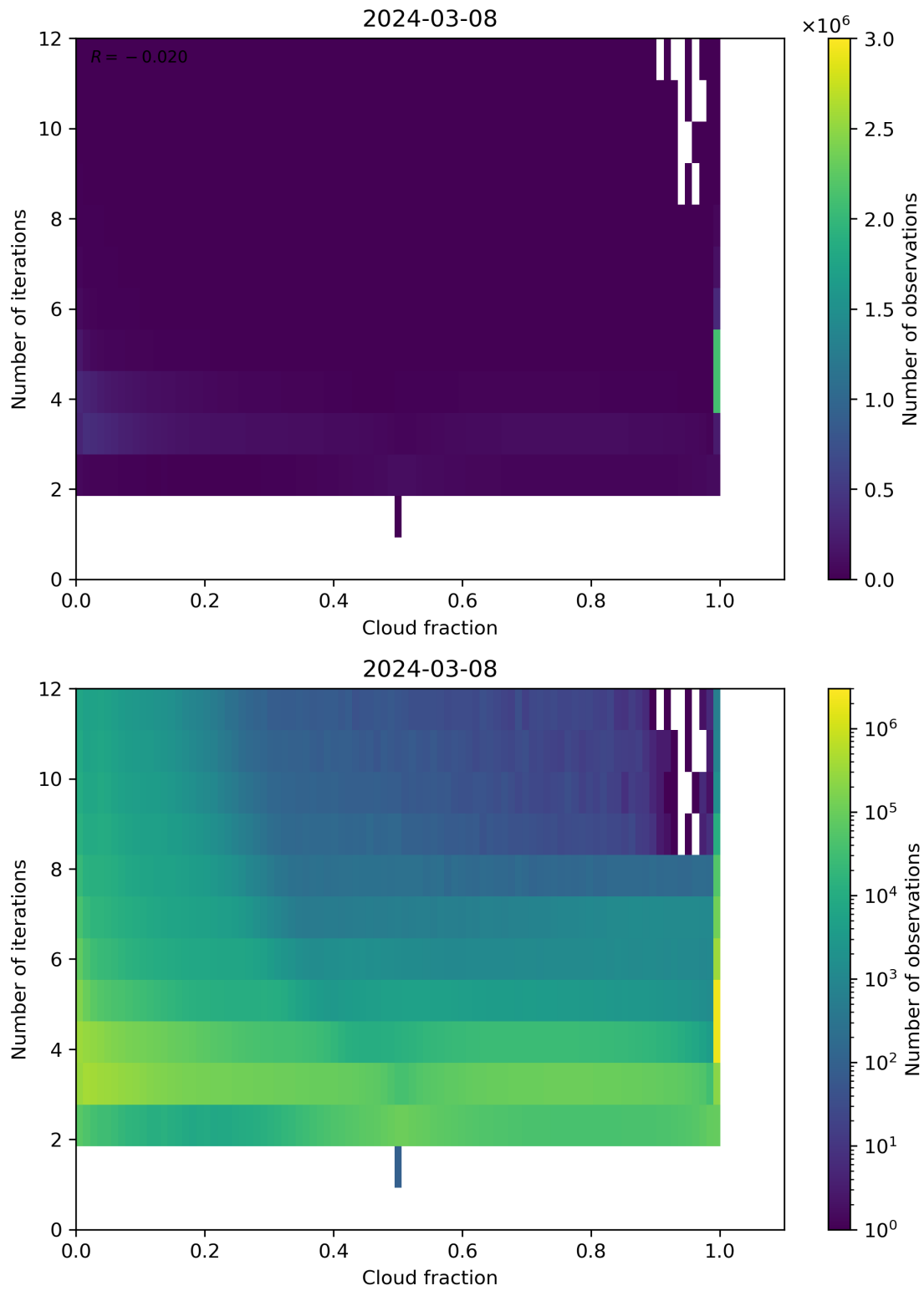
Figure 73: Scatter density plot of “Cloud fraction” against “Number of iterations” for 2024-03-07 to 2024-03-09.
