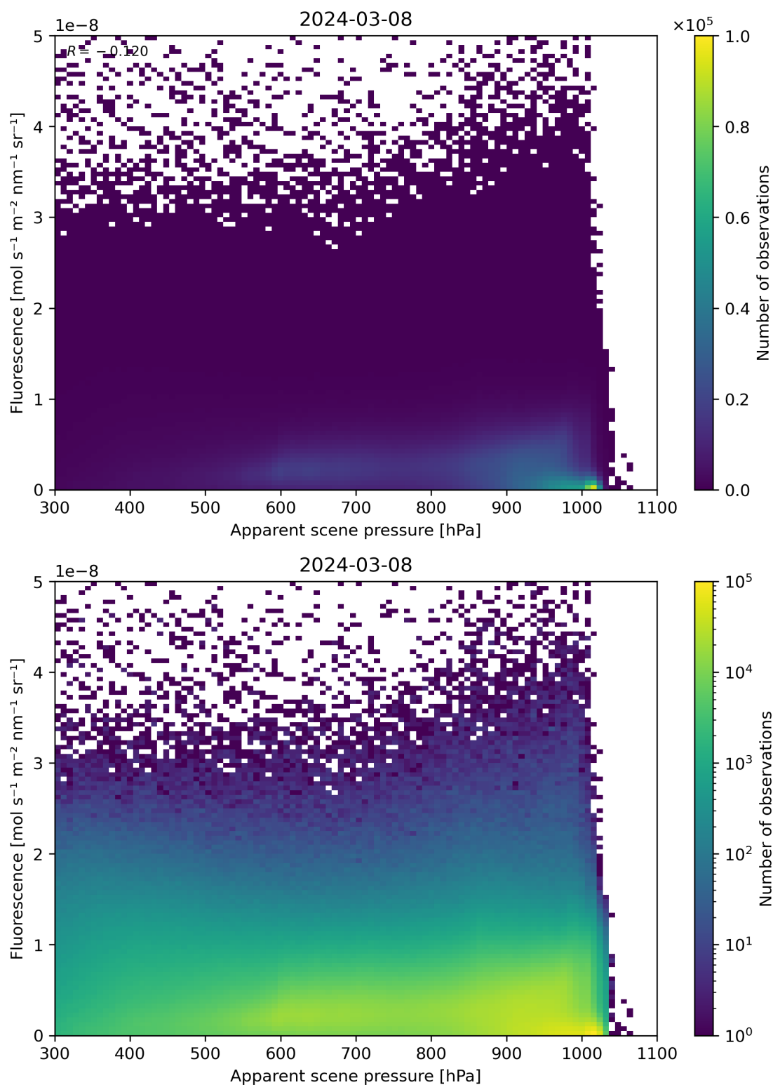
Figure 64: Scatter density plot of “Apparent scene pressure” against “Fluorescence” for 2024-03-07 to 2024-03-09.
