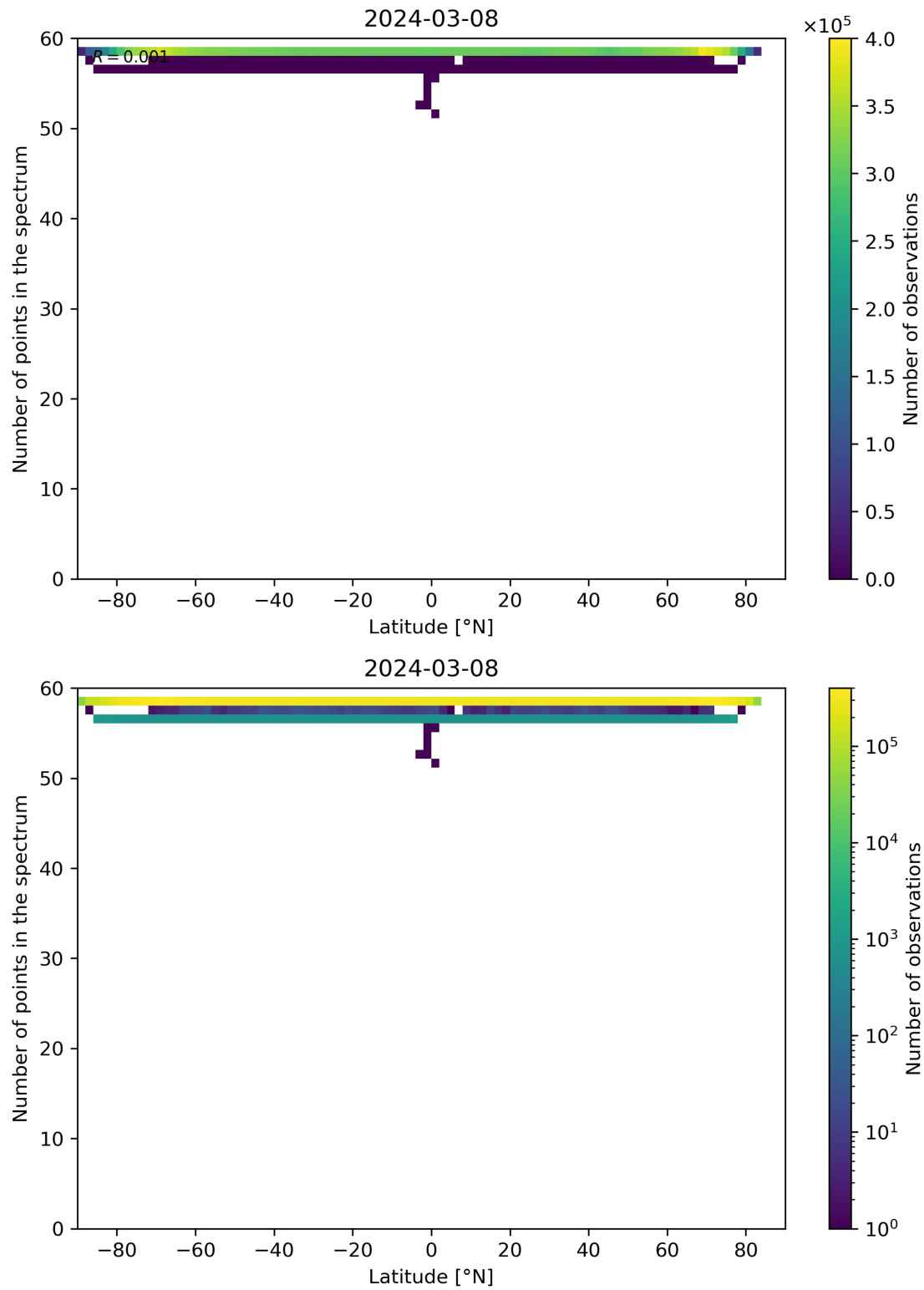
Figure 94: Scatter density plot of “Latitude” against “Number of points in the spectrum” for 2024-03-07 to 2024-03-09.
