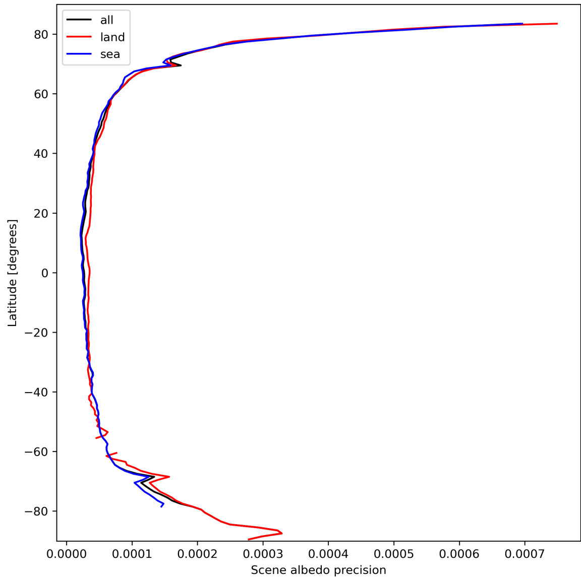
Figure 18: Zonal average of “Scene albedo precision” for 2024-03-07 to 2024-03-09.
