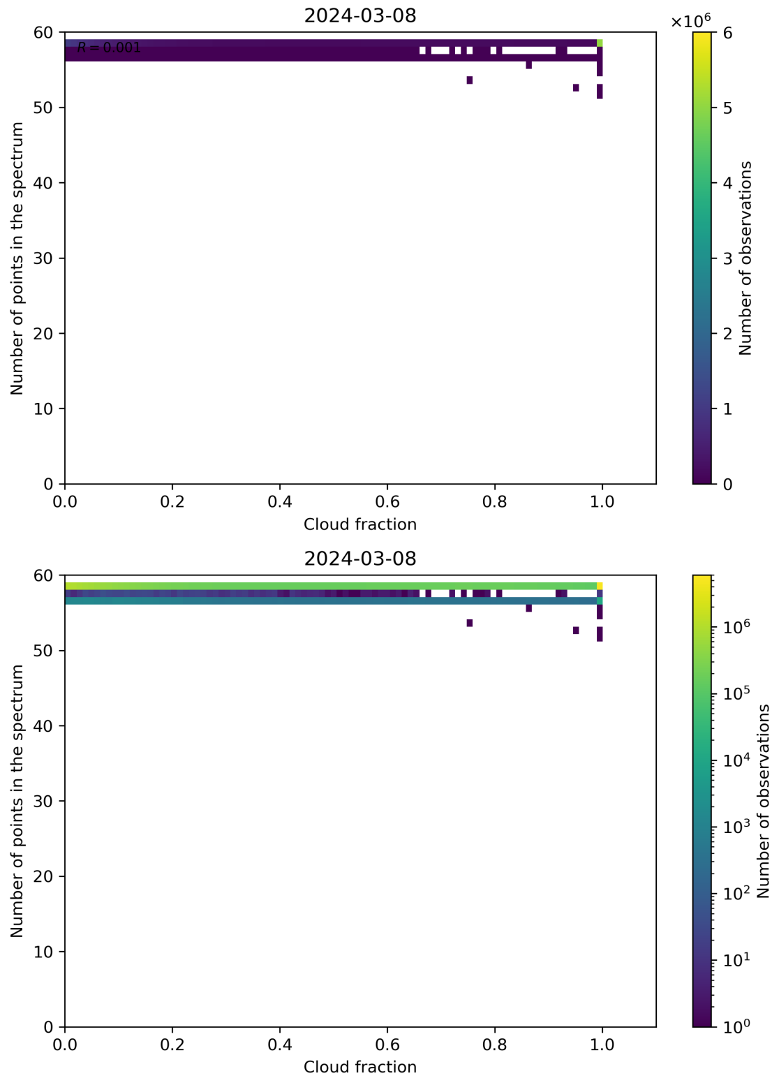
Figure 74: Scatter density plot of “Cloud fraction” against “Number of points in the spectrum” for 2024-03-07 to 2024-03-09.
