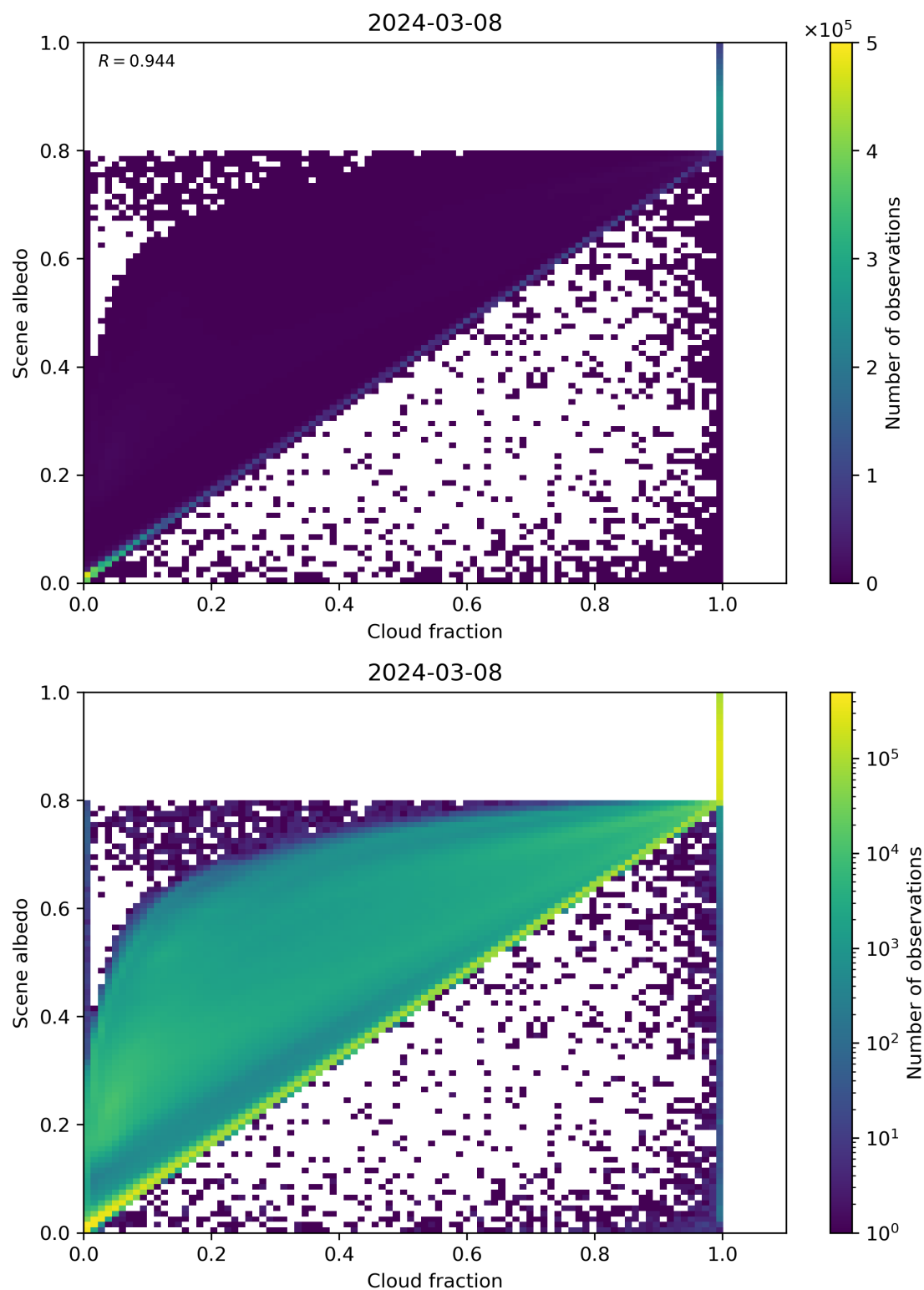
Figure 75: Scatter density plot of “Cloud fraction” against “Scene albedo” for 2024-03-07 to 2024-03-09.
