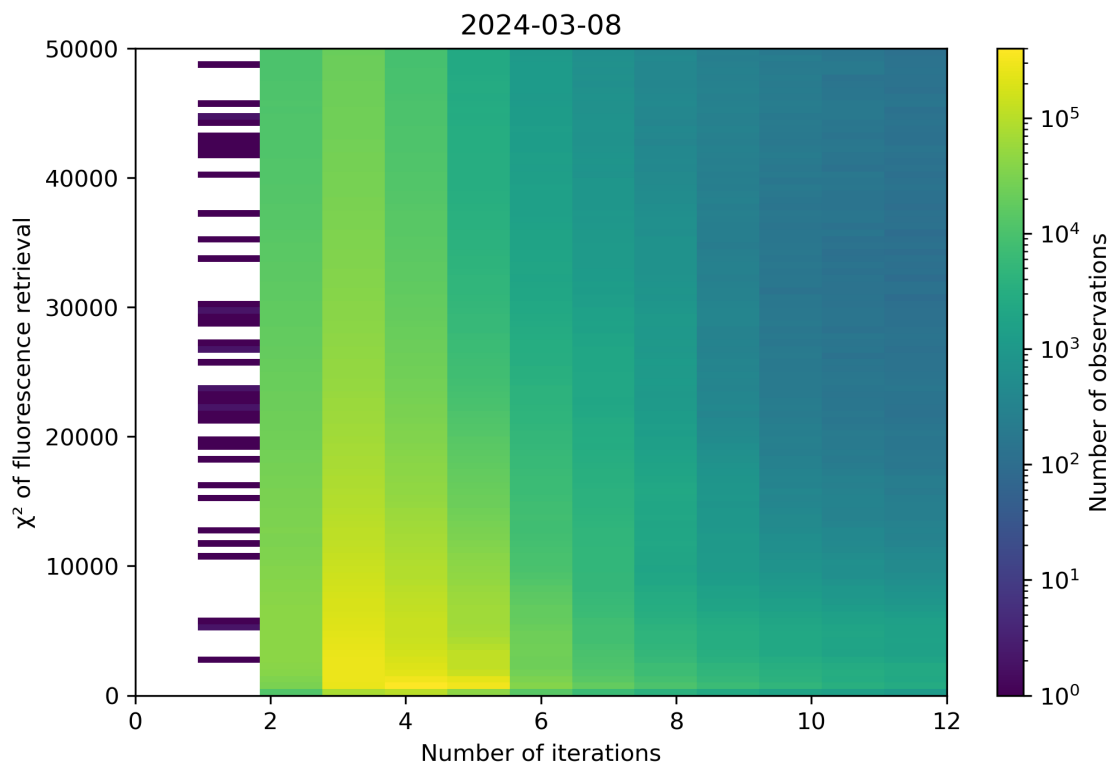
Figure 97: Scatter density plot of “Number of iterations” against “ \chi^2 of fluorescence retrieval” for 2024-03-07 to 2024-03-09.
