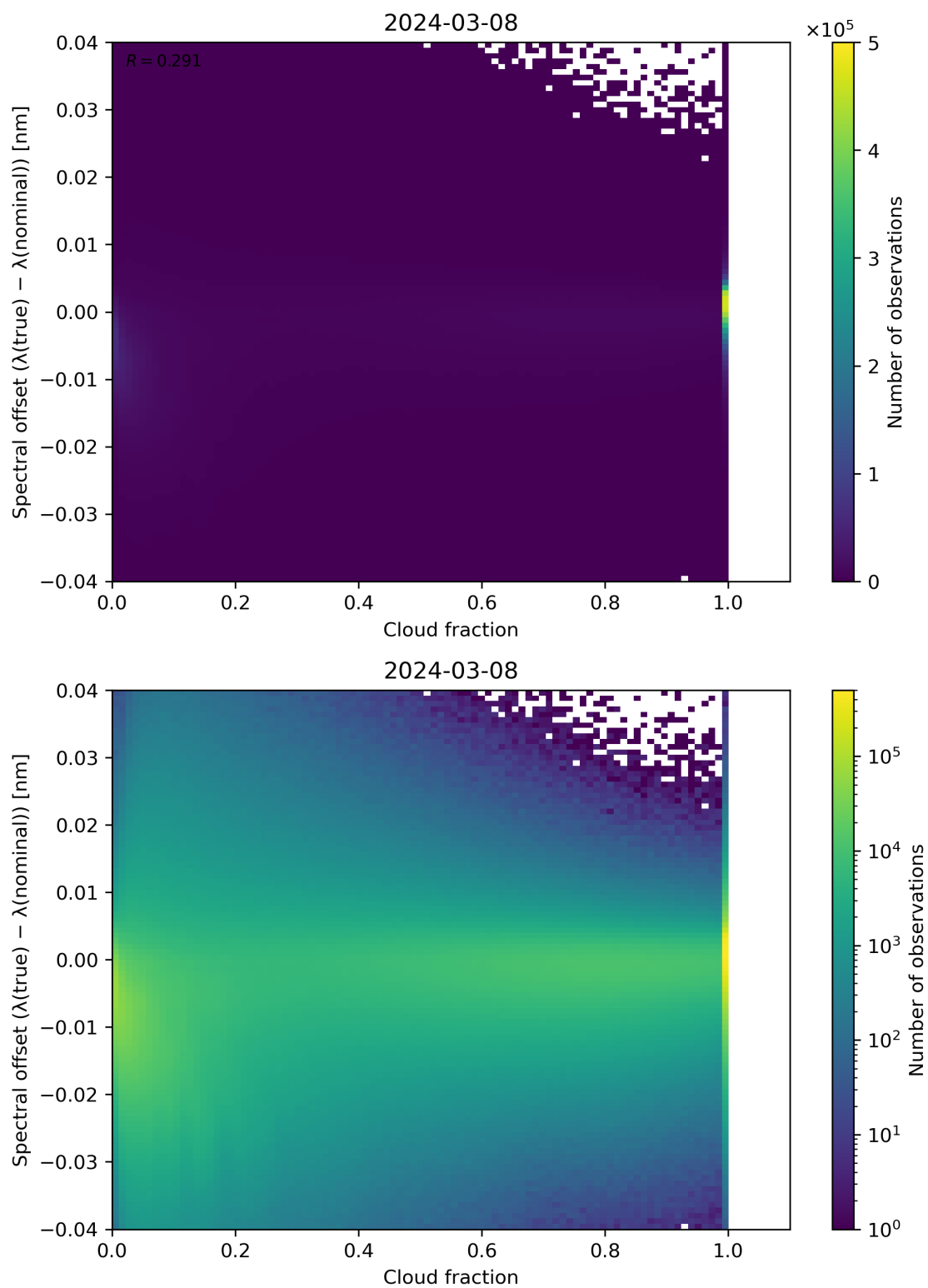
Figure 76: Scatter density plot of “Cloud fraction” against “Spectral offset ( \lambda(\text{true}) - \lambda(\text{nominal}) )” for 2024-03-07 to 2024-03-09.
