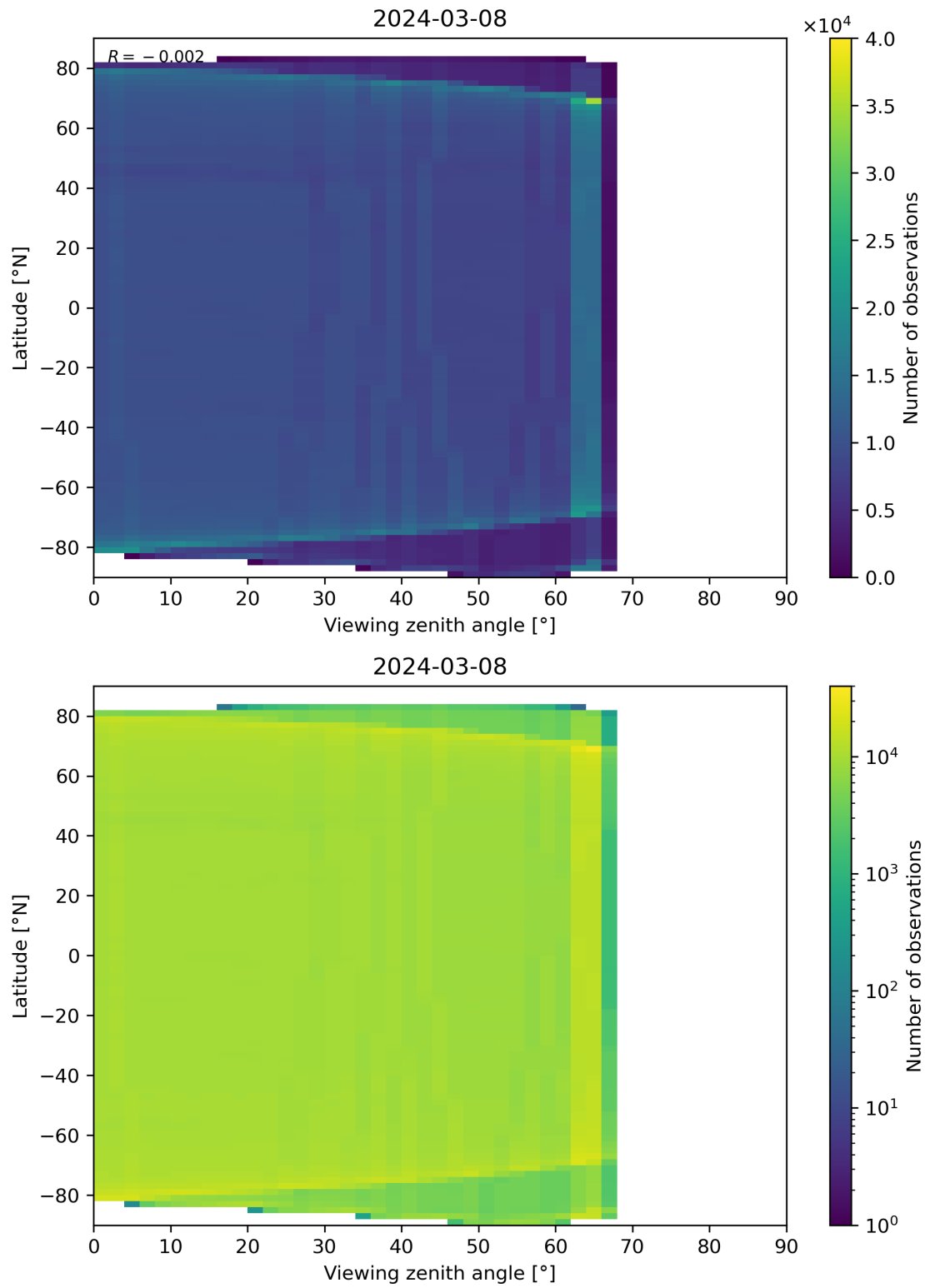
Figure 123: Scatter density plot of “Viewing zenith angle” against “Latitude” for 2024-03-07 to 2024-03-09.
