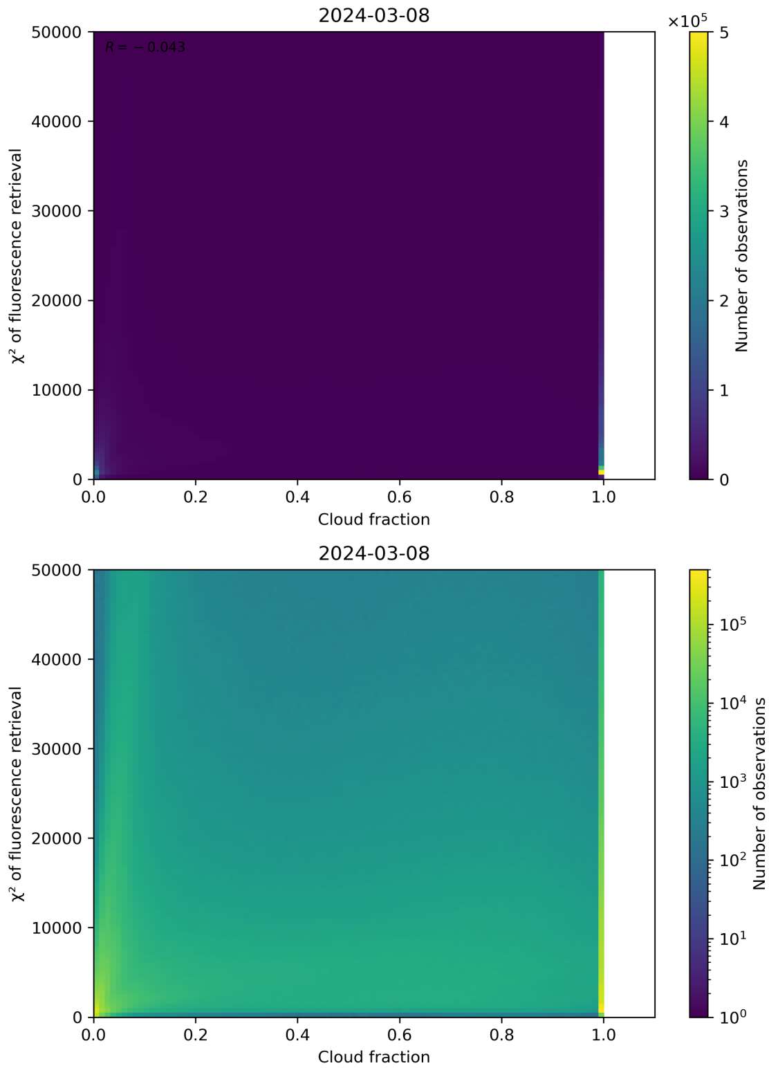
Figure 71: Scatter density plot of “Cloud fraction” against “ \chi^2 of fluorescence retrieval” for 2024-03-07 to 2024-03-09.
