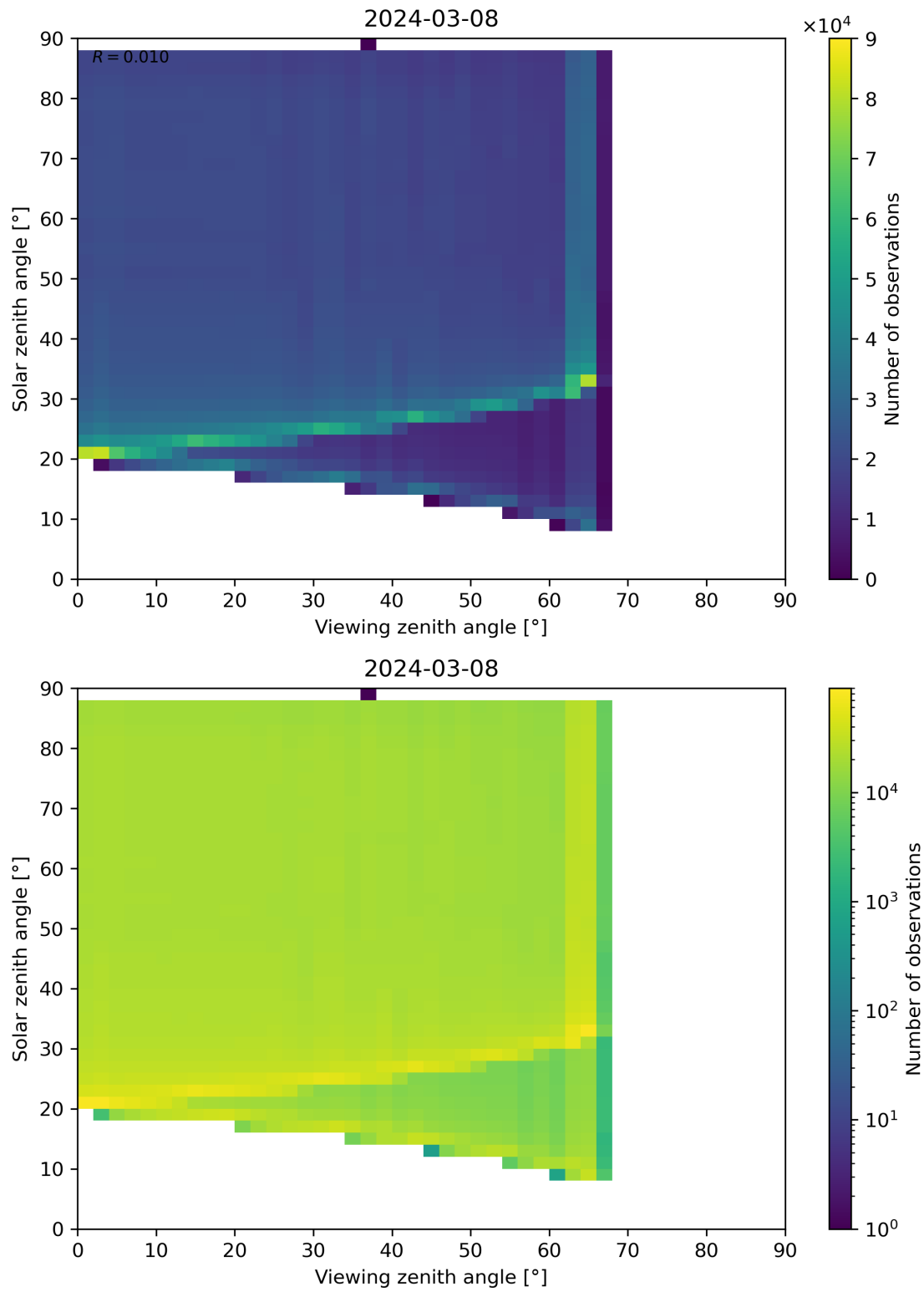
Figure 127: Scatter density plot of “Viewing zenith angle” against “Solar zenith angle” for 2024-03-07 to 2024-03-09.
