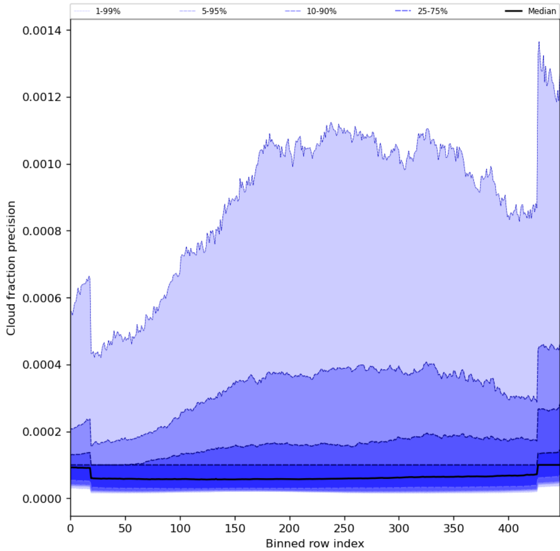
Figure 50: Along track statistics of “Cloud fraction precision” for 2024-03-07 to 2024-03-09
