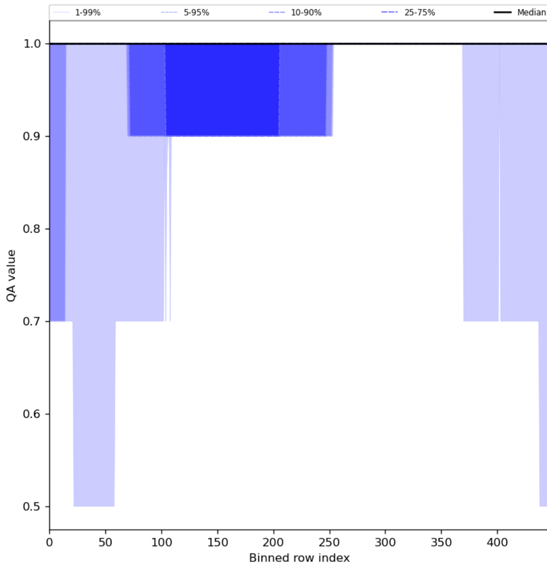
Figure 46: Along track statistics of “QA value” for 2024-03-07 to 2024-03-09
