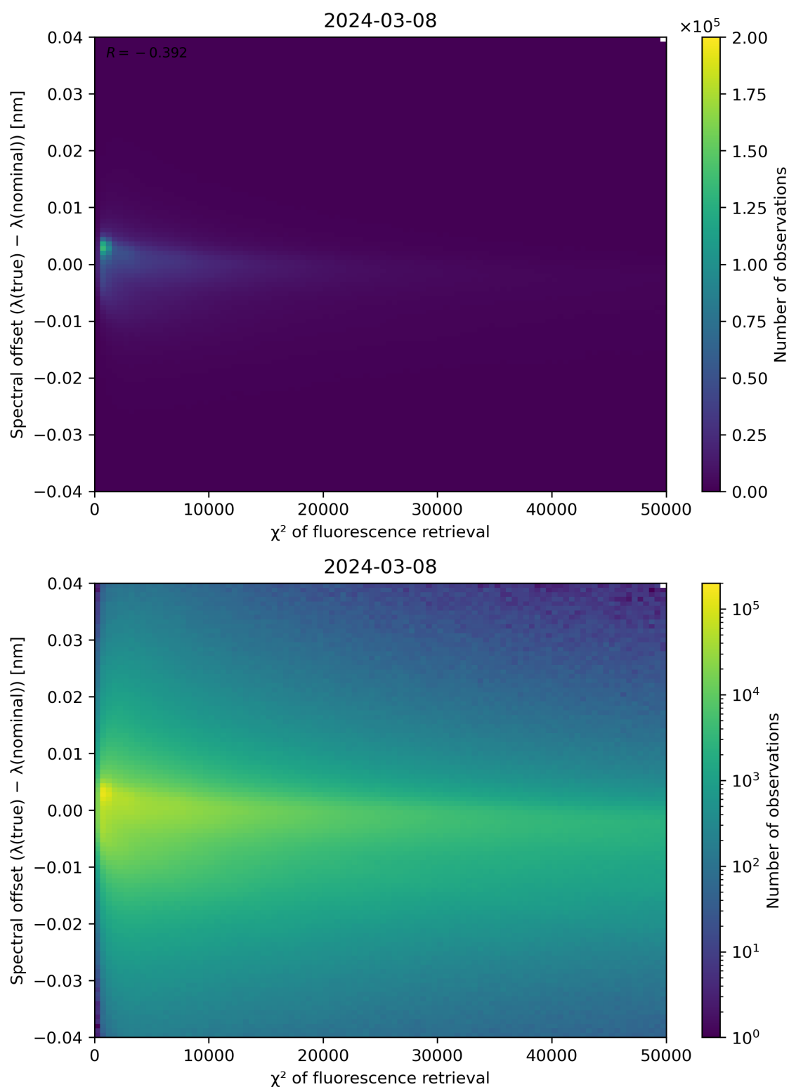
Figure 69: Scatter density plot of " \chi^2 of fluorescence retrieval" against "Spectral offset ( \lambda(\text{true}) - \lambda(\text{nominal}) )" for 2024-03-07 to 2024-03-09.
