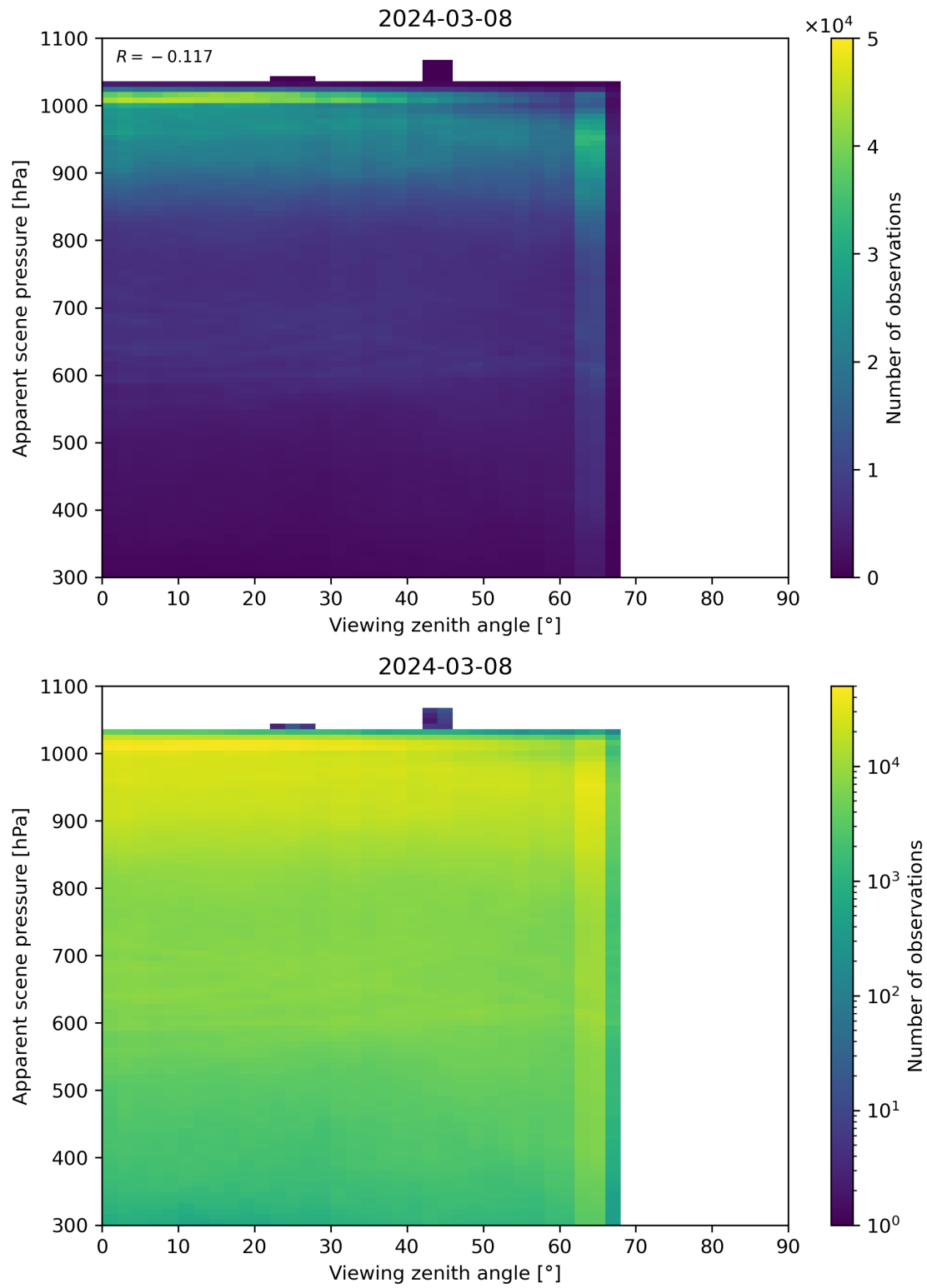
Figure 118: Scatter density plot of “Viewing zenith angle” against “Apparent scene pressure” for 2024-03-07 to 2024-03-09.
