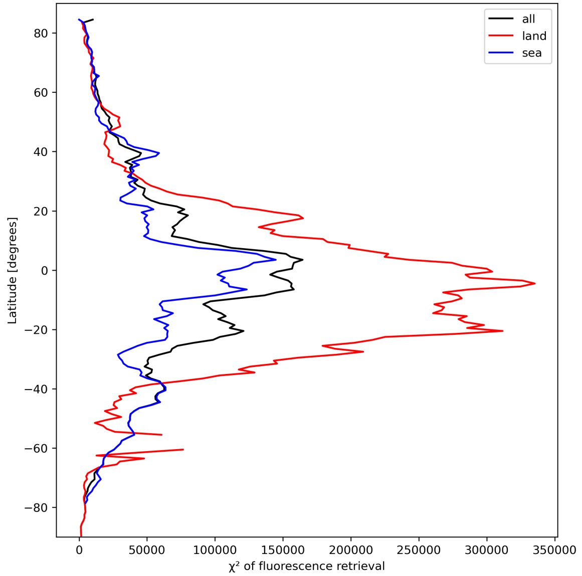
Figure 25: Zonal average of “ \chi^2 of fluorescence retrieval” for 2024-03-09 to 2024-03-10.
