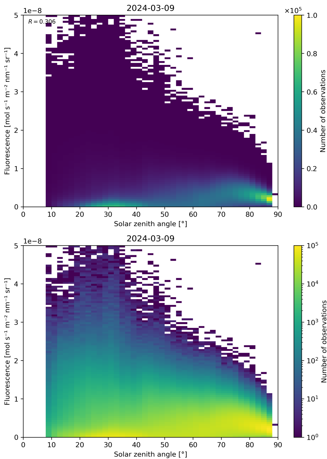
Figure 112: Scatter density plot of “Solar zenith angle” against “Fluorescence” for 2024-03-09 to 2024-03-10.
