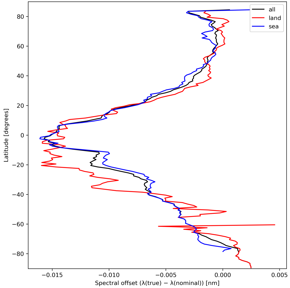
Figure 28: Zonal average of “Spectral offset ( \lambda(\text{true}) - \lambda(\text{nominal}) )” for 2024-03-09 to 2024-03-10.
