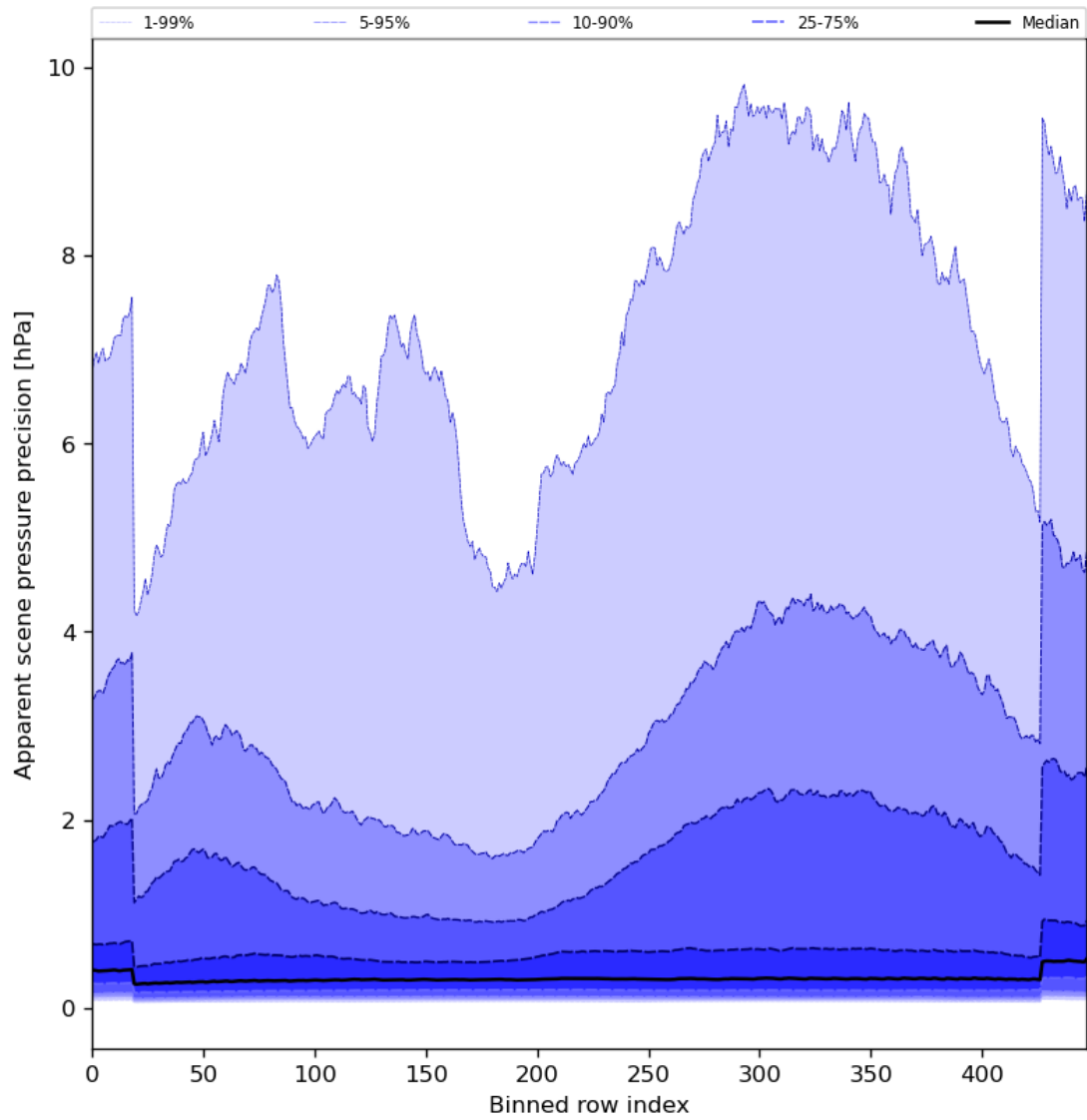
Figure 54: Along track statistics of “Apparent scene pressure precision” for 2024-03-09 to 2024-03-10
