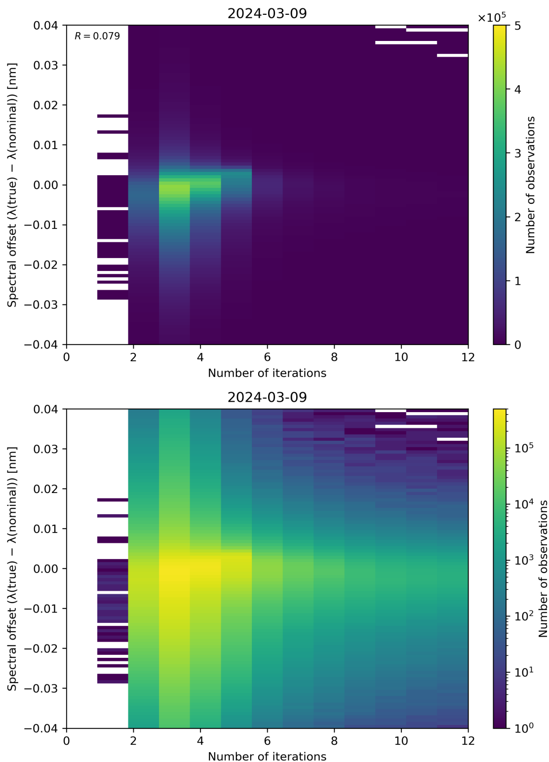
Figure 100: Scatter density plot of “Number of iterations” against “Spectral offset ( \lambda(\text{true}) - \lambda(\text{nominal}) )” for 2024-03-09 to 2024-03-10.
