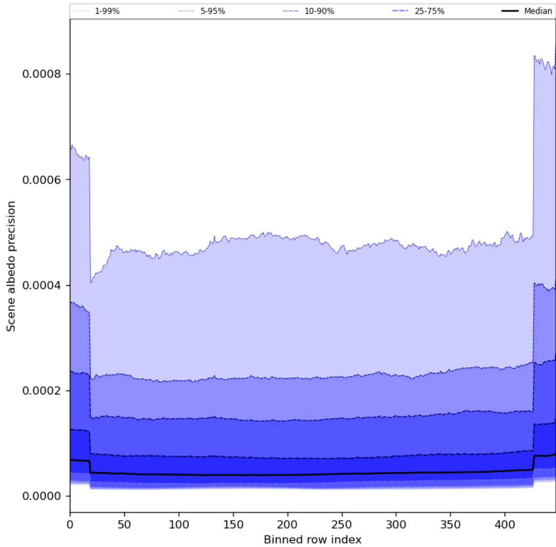
Figure 52: Along track statistics of “Scene albedo precision” for 2024-03-09 to 2024-03-10
