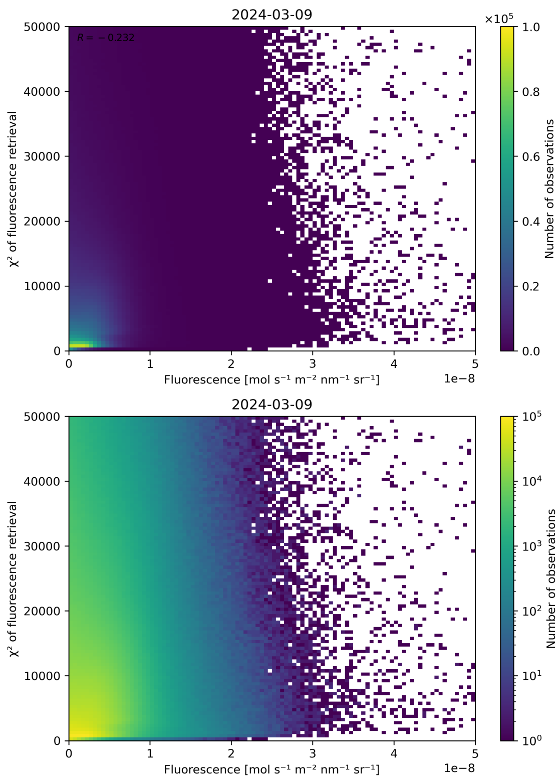
Figure 85: Scatter density plot of “Fluorescence” against “ \chi^2 of fluorescence retrieval” for 2024-03-09 to 2024-03-10.
