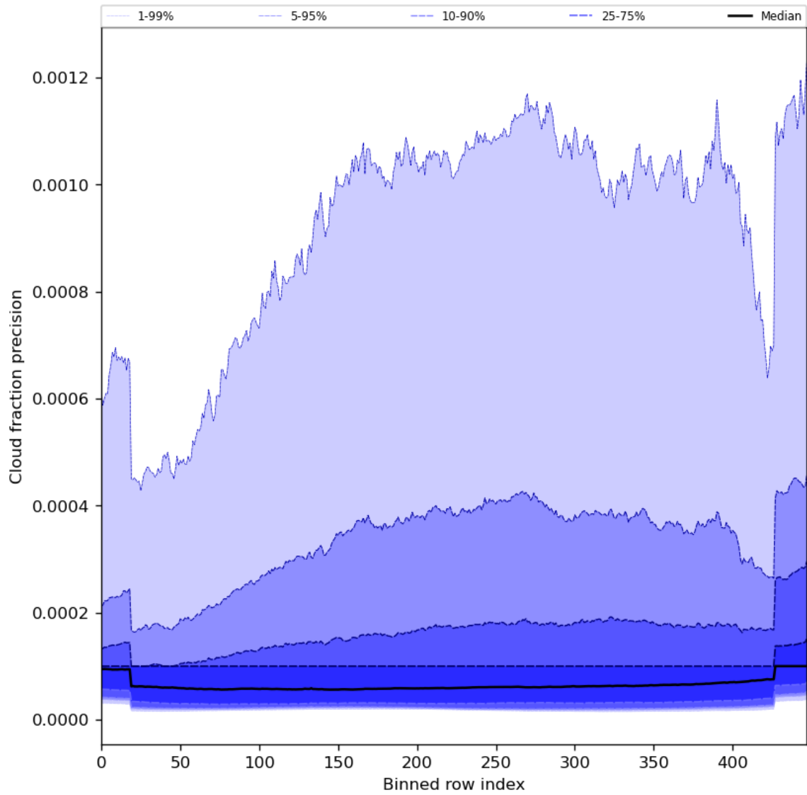
Figure 50: Along track statistics of “Cloud fraction precision” for 2024-03-09 to 2024-03-10
