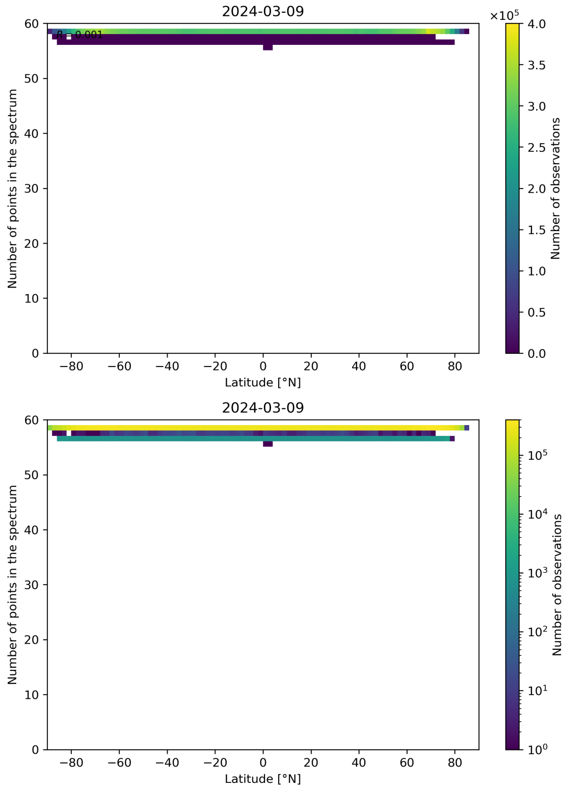
Figure 94: Scatter density plot of “Latitude” against “Number of points in the spectrum” for 2024-03-09 to 2024-03-10.
