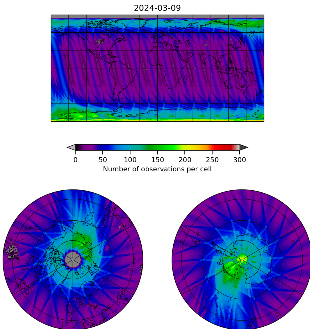
Figure 11: Map of the number of observations for 2024-03-09 to 2024-03-10
