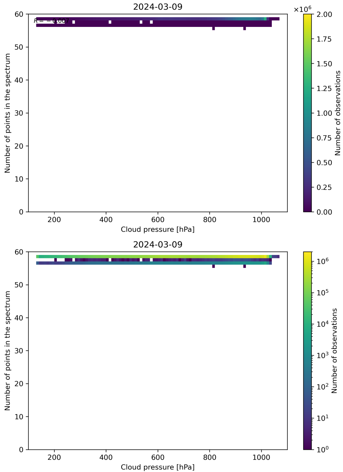
Figure 82: Scatter density plot of “Cloud pressure” against “Number of points in the spectrum” for 2024-03-09 to 2024-03-10.
