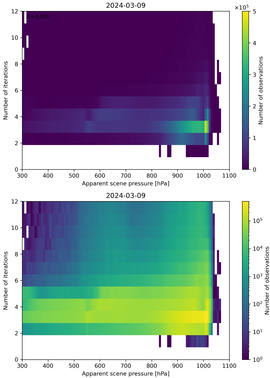
Figure 65: Scatter density plot of “Apparent scene pressure” against “Number of iterations” for 2024-03-09 to 2024-03-10.
