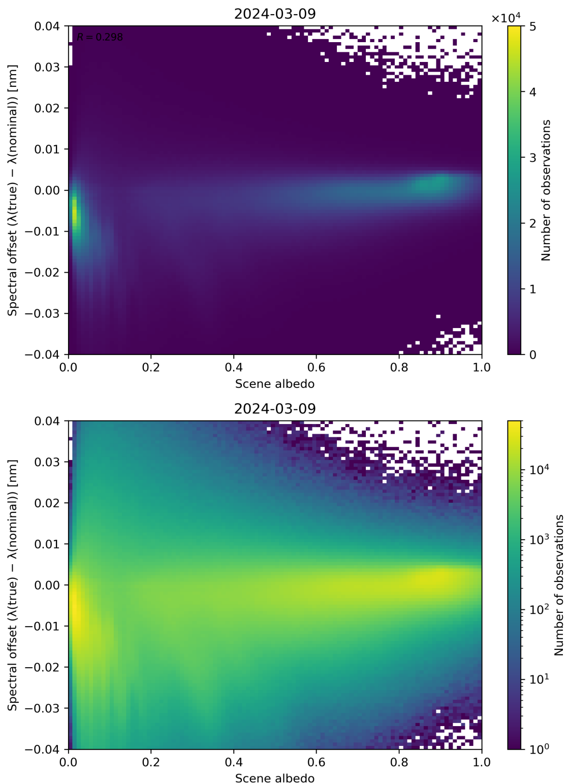
Figure 107: Scatter density plot of “Scene albedo” against “Spectral offset ( \lambda(\text{true}) - \lambda(\text{nominal}) )” for 2024-03-09 to 2024-03-10.
