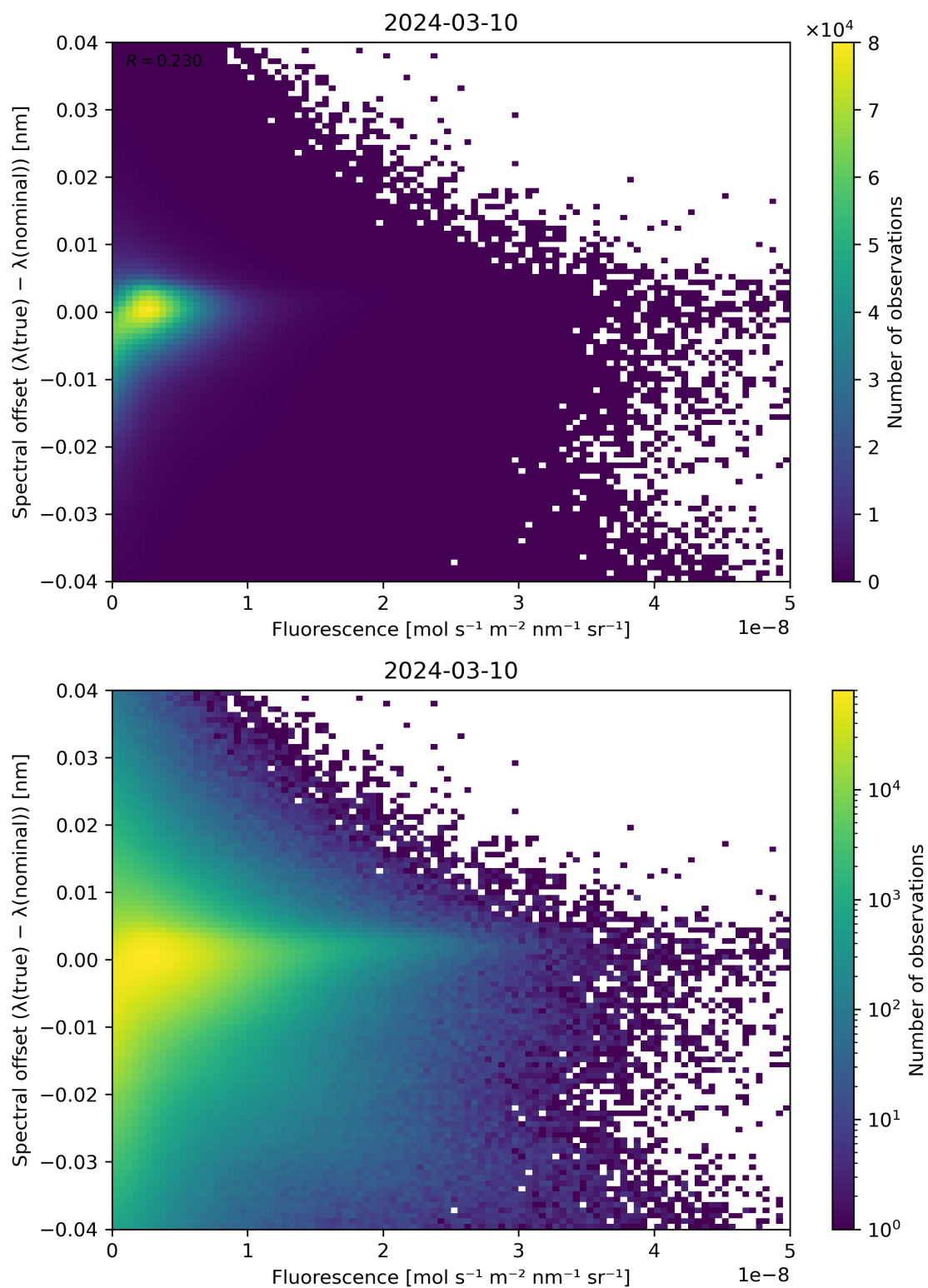
Figure 87: Scatter density plot of “Fluorescence” against “Spectral offset ( \lambda(\text{true}) - \lambda(\text{nominal}) )” for 2024-03-09 to 2024-03-11.
