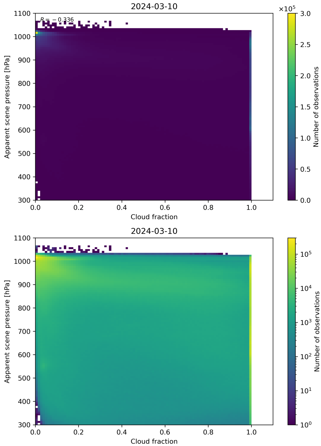
Figure 70: Scatter density plot of “Cloud fraction” against “Apparent scene pressure” for 2024-03-09 to 2024-03-11.
