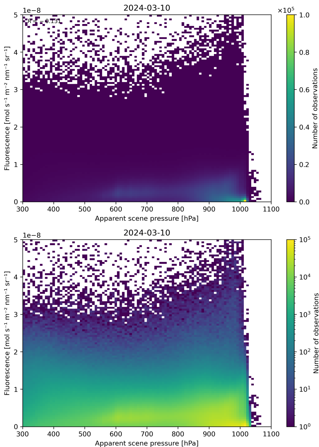
Figure 64: Scatter density plot of “Apparent scene pressure” against “Fluorescence” for 2024-03-09 to 2024-03-11.
