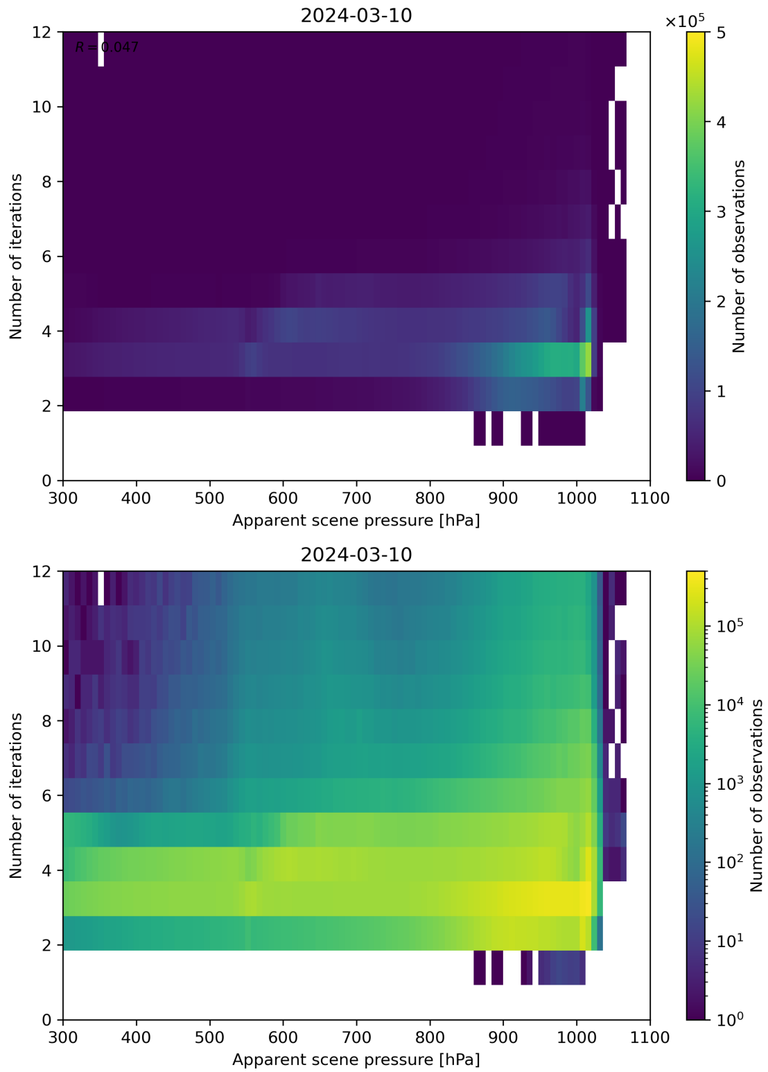
Figure 65: Scatter density plot of “Apparent scene pressure” against “Number of iterations” for 2024-03-09 to 2024-03-11.
