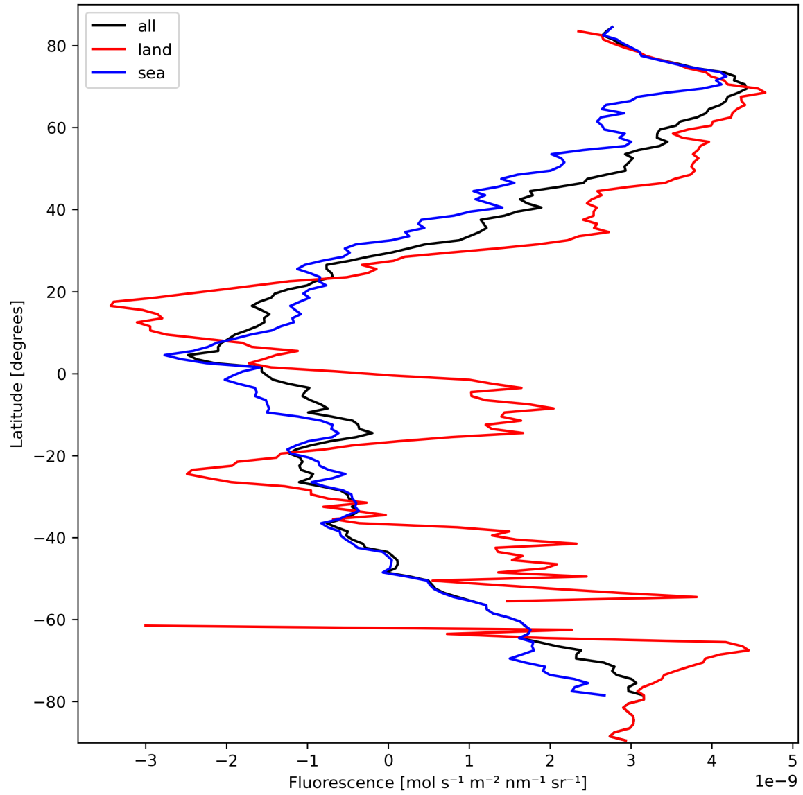
Figure 23: Zonal average of “Fluorescence” for 2024-03-09 to 2024-03-11.
