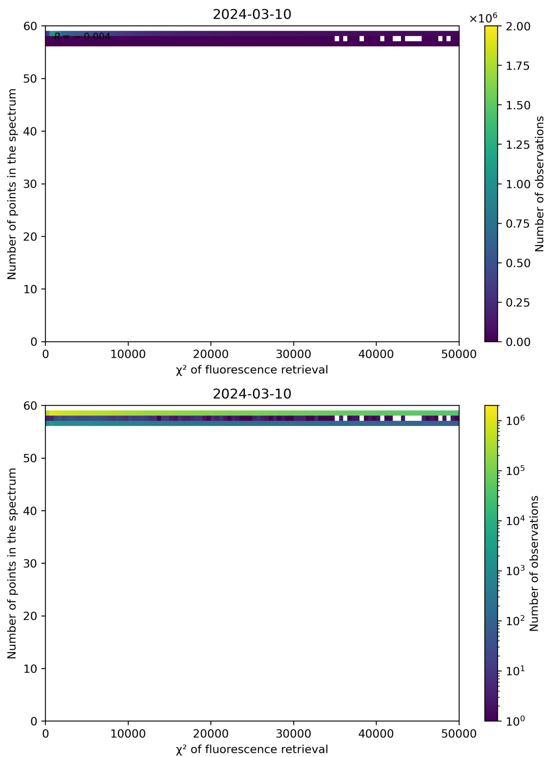
Figure 68: Scatter density plot of " \chi^2 of fluorescence retrieval" against "Number of points in the spectrum" for 2024-03-09 to 2024-03-11.
