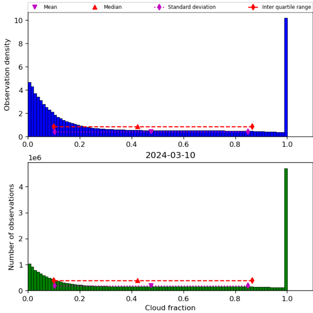
Figure 32: Histogram of “Cloud fraction” for 2024-03-09 to 2024-03-11
