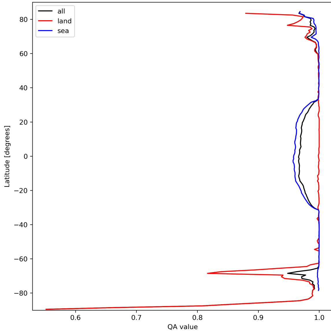
Figure 12: Zonal average of “QA value” for 2024-03-09 to 2024-03-11.
