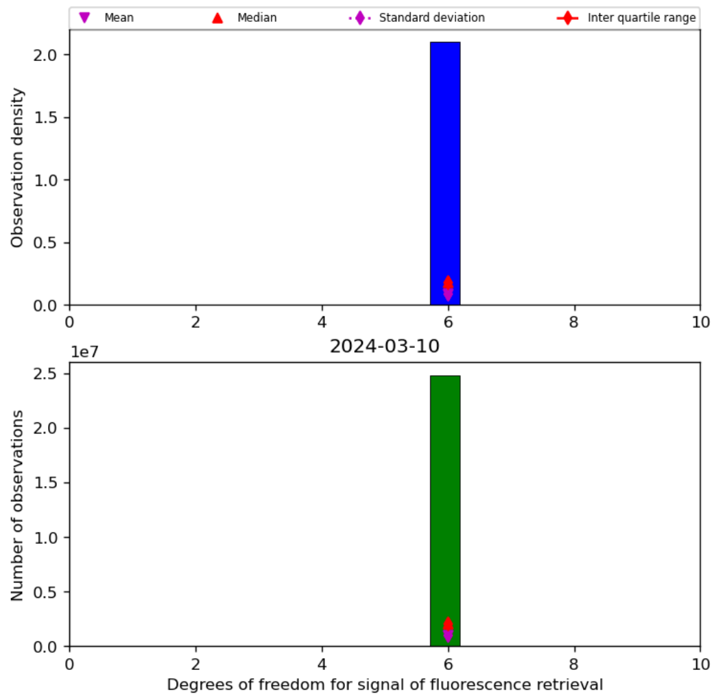
Figure 43: Histogram of “Degrees of freedom for signal of fluorescence retrieval” for 2024-03-09 to 2024-03-11
