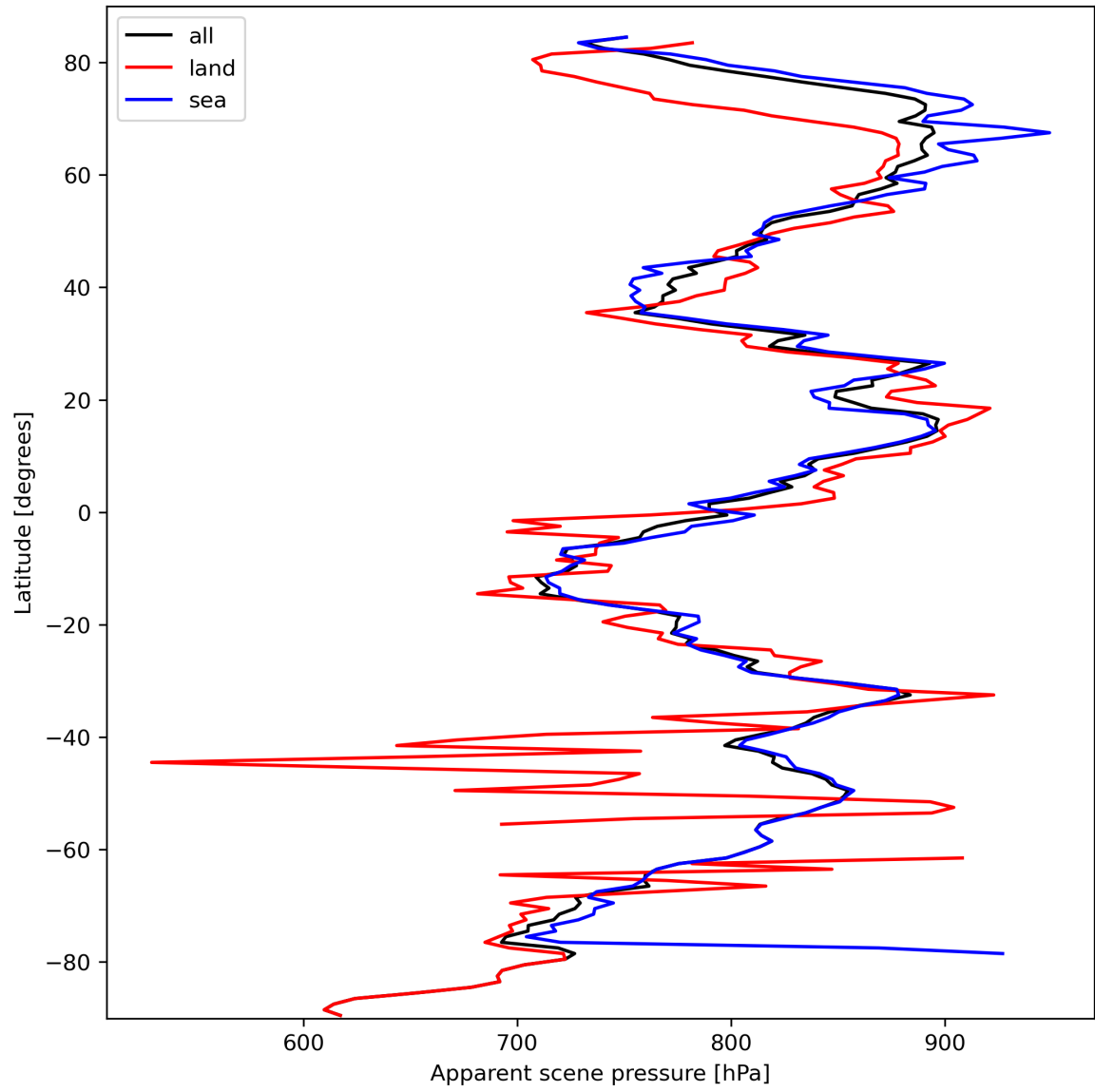
Figure 19: Zonal average of “Apparent scene pressure” for 2024-03-09 to 2024-03-11.
