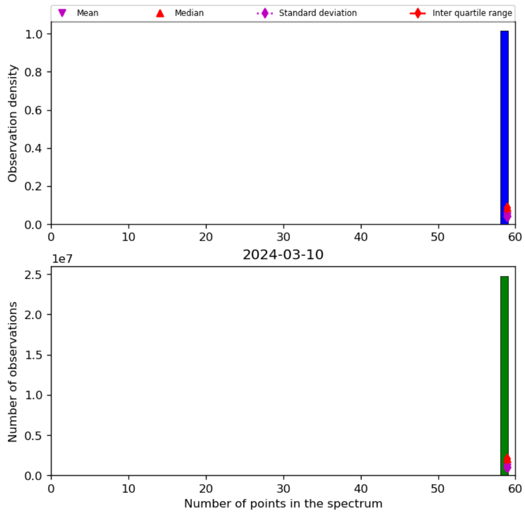
Figure 44: Histogram of "Number of points in the spectrum" for 2024-03-09 to 2024-03-11
