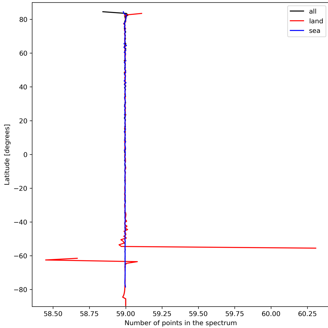
Figure 27: Zonal average of “Number of points in the spectrum” for 2024-03-09 to 2024-03-11.
