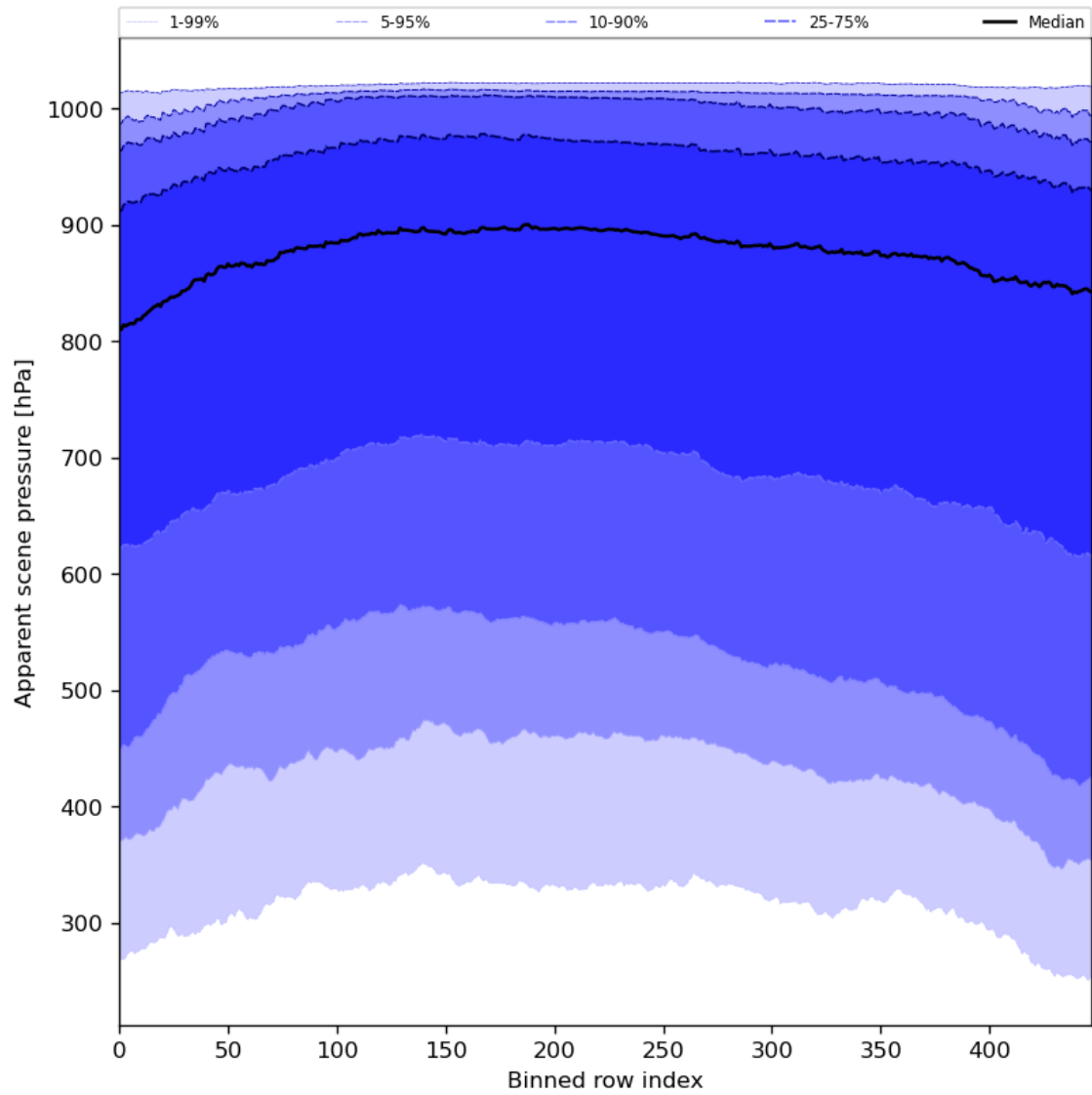
Figure 53: Along track statistics of “Apparent scene pressure” for 2024-03-09 to 2024-03-11
