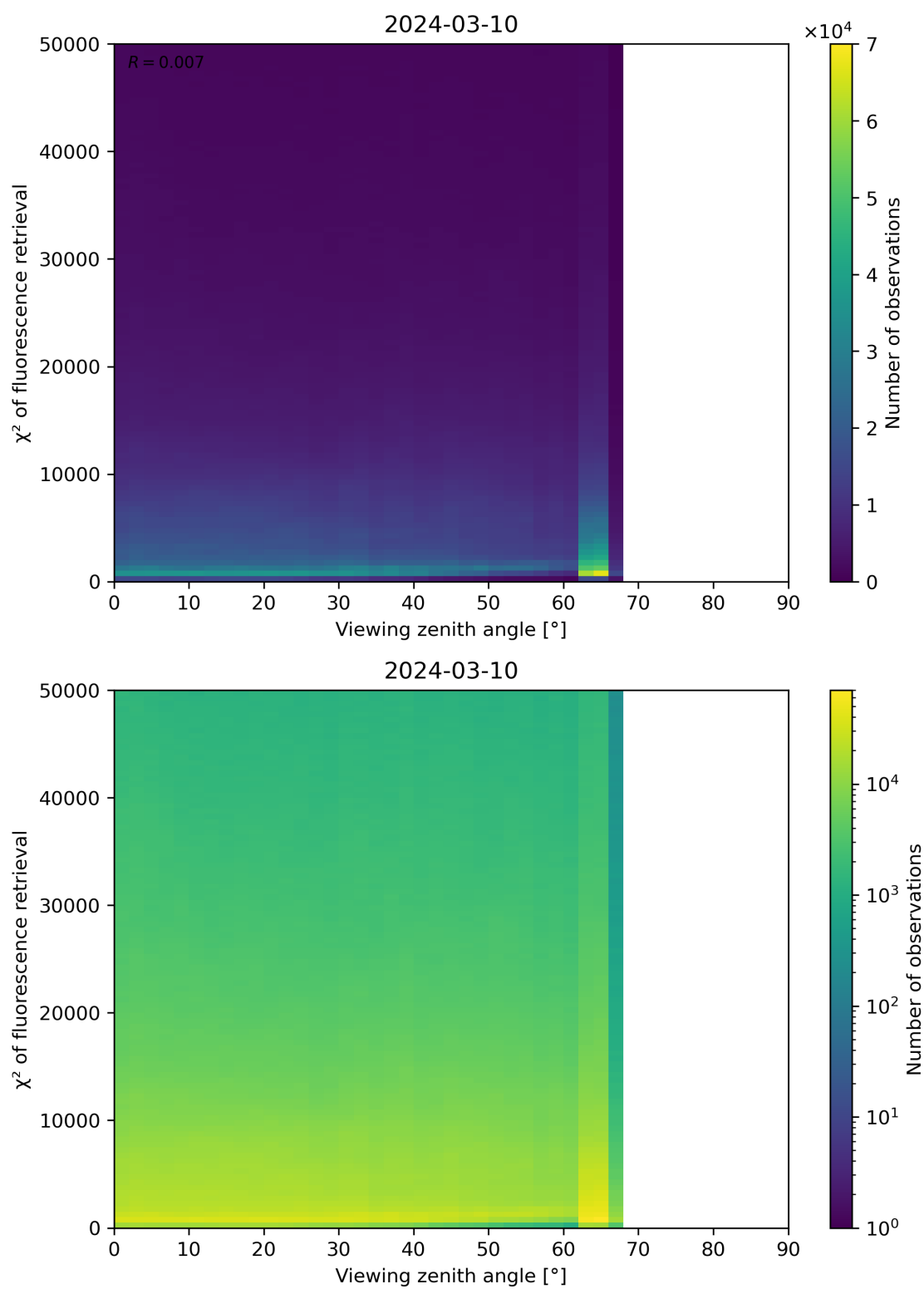
Figure 119: Scatter density plot of “Viewing zenith angle” against “ \chi^2 of fluorescence retrieval” for 2024-03-09 to 2024-03-11.
