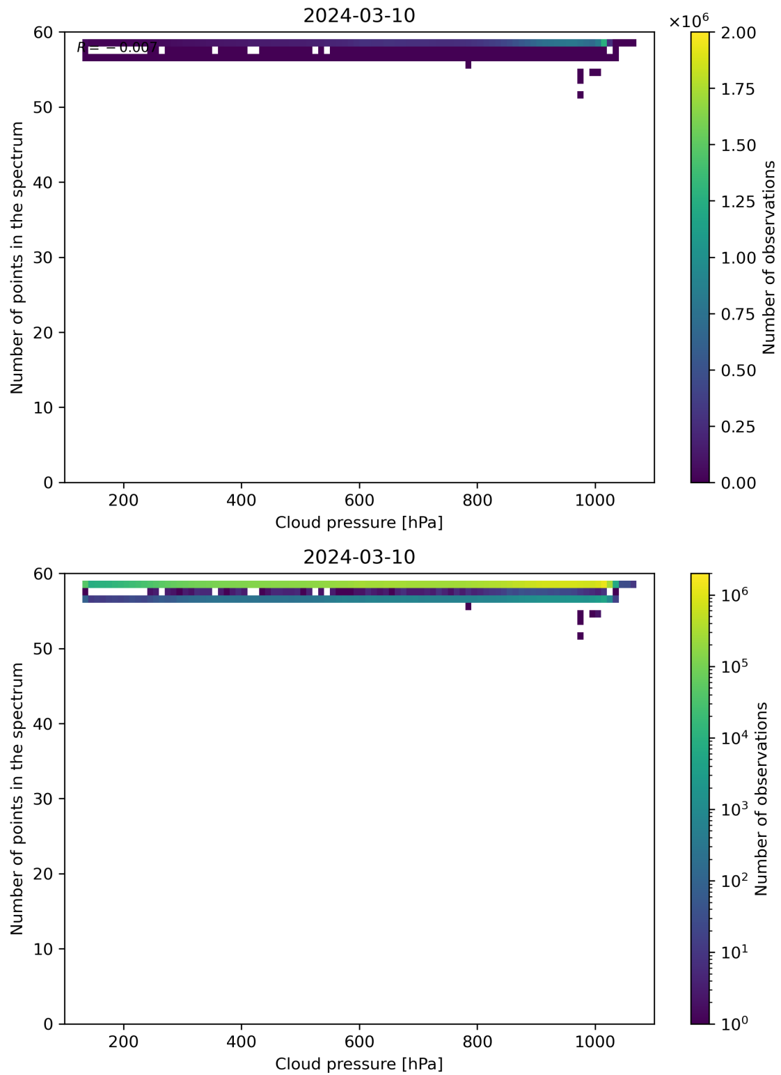
Figure 82: Scatter density plot of “Cloud pressure” against “Number of points in the spectrum” for 2024-03-09 to 2024-03-11.
