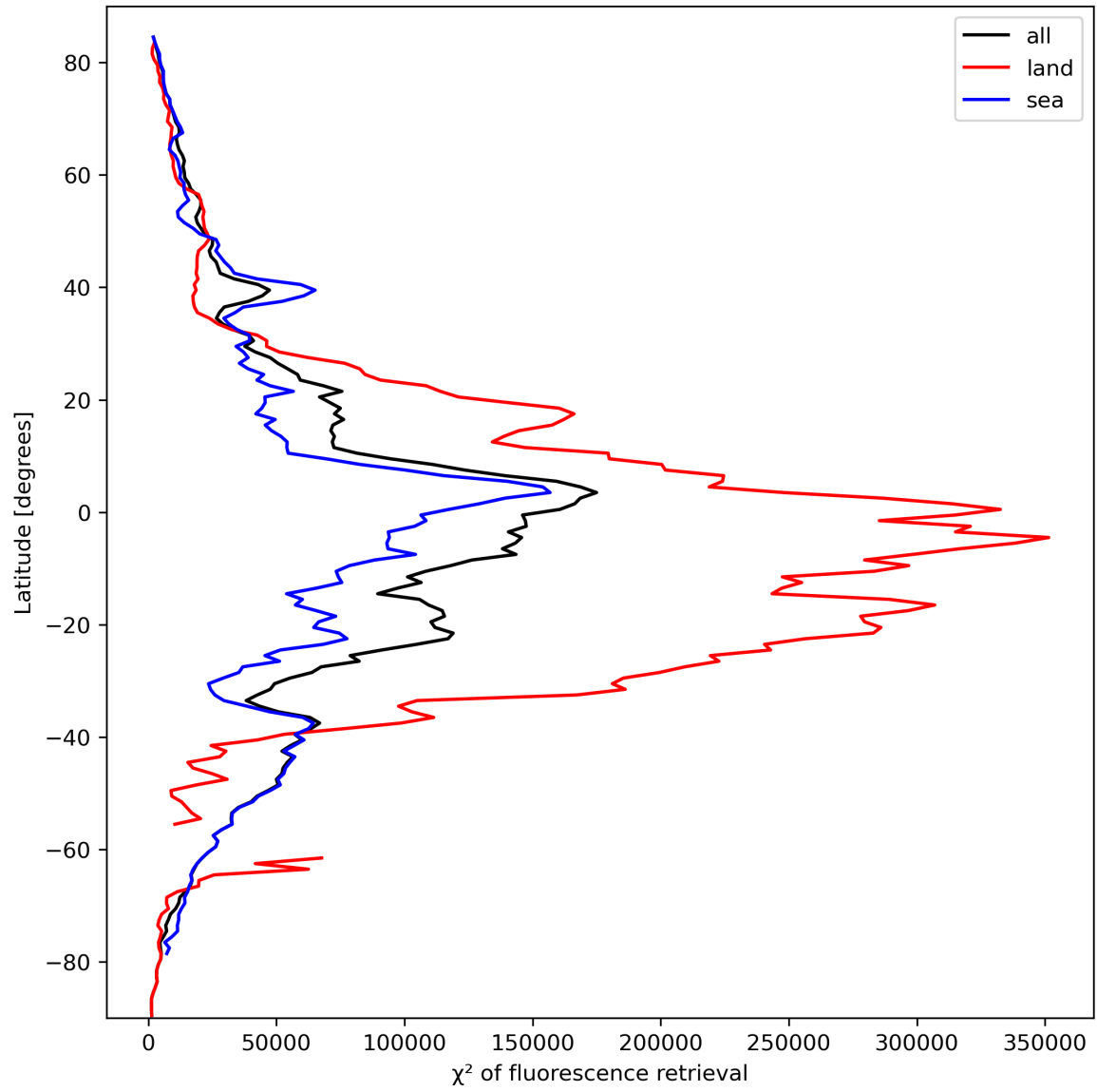
Figure 25: Zonal average of “ \chi^2 of fluorescence retrieval” for 2024-03-09 to 2024-03-11.
