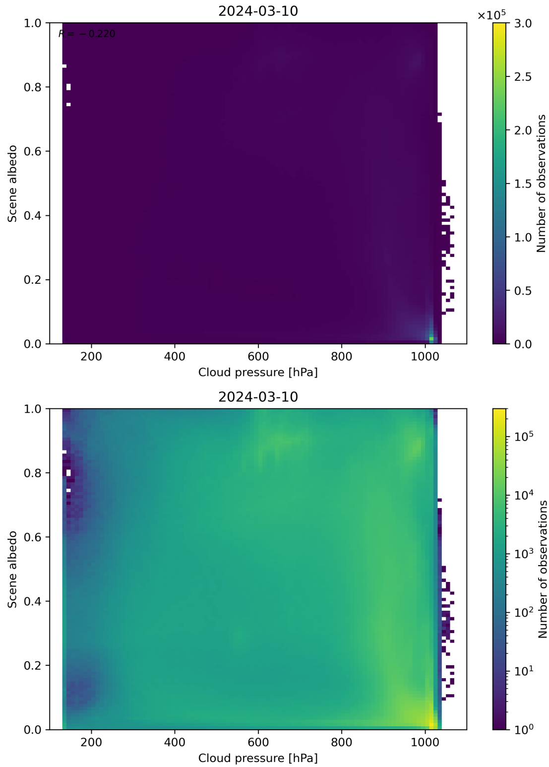
Figure 83: Scatter density plot of “Cloud pressure” against “Scene albedo” for 2024-03-09 to 2024-03-11.
