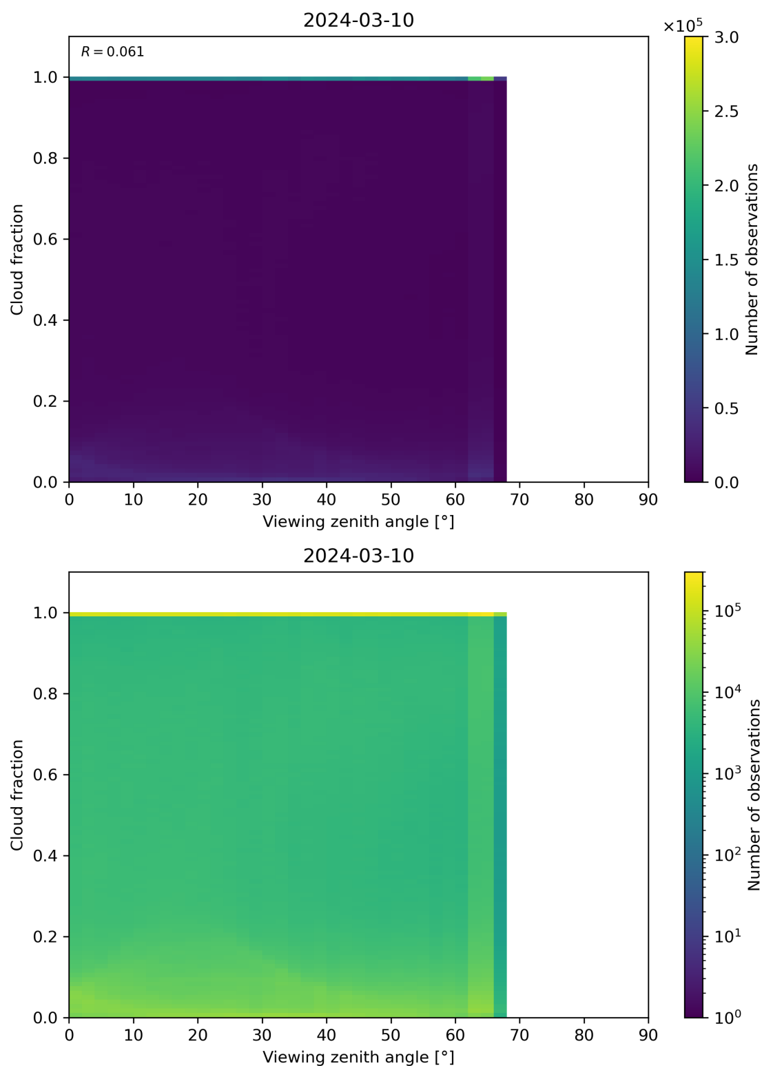
Figure 120: Scatter density plot of “Viewing zenith angle” against “Cloud fraction” for 2024-03-09 to 2024-03-11.
