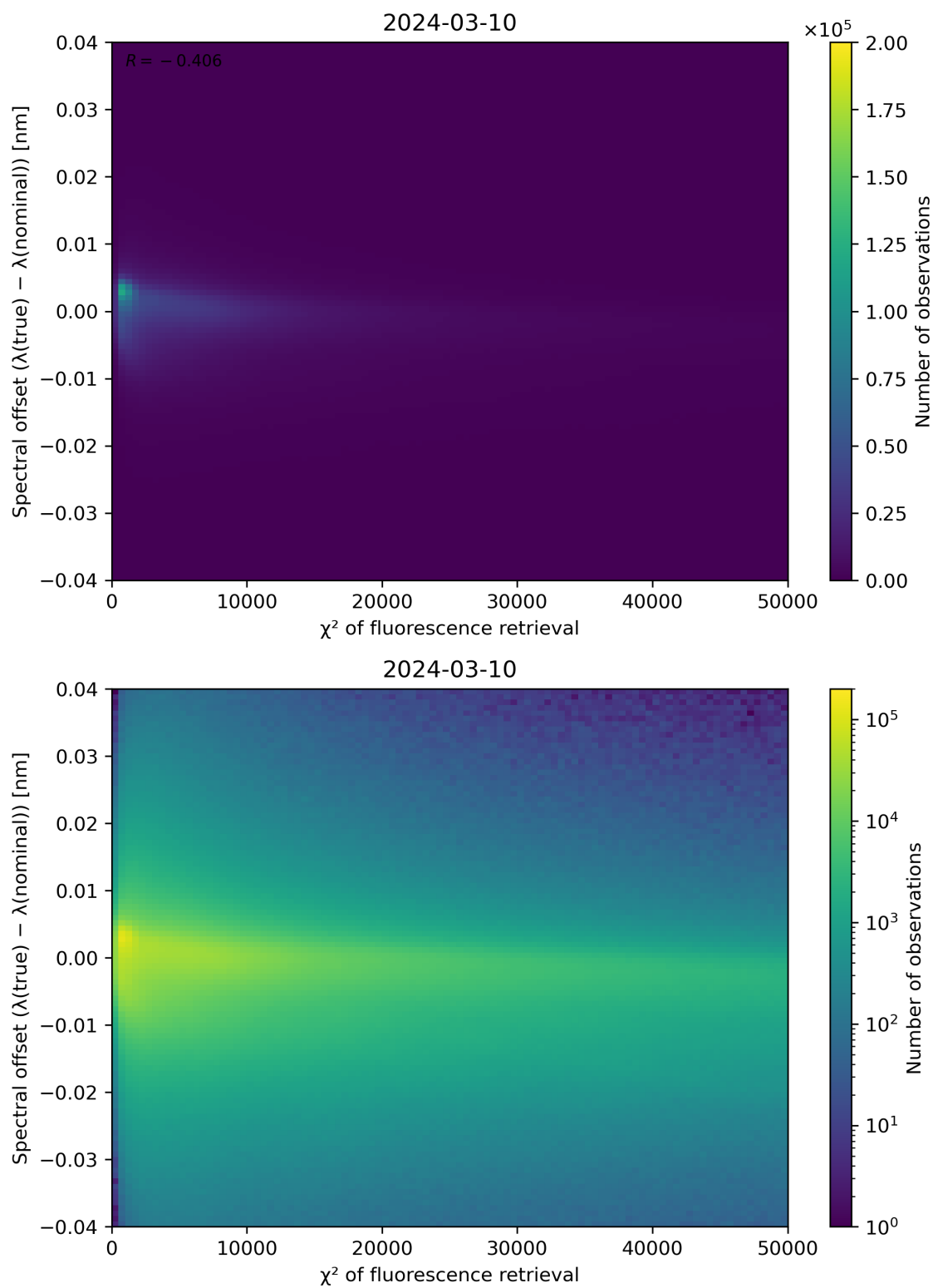
Figure 69: Scatter density plot of " \chi^2 of fluorescence retrieval" against "Spectral offset ( \lambda(\text{true}) - \lambda(\text{nominal}) )" for 2024-03-09 to 2024-03-11.
