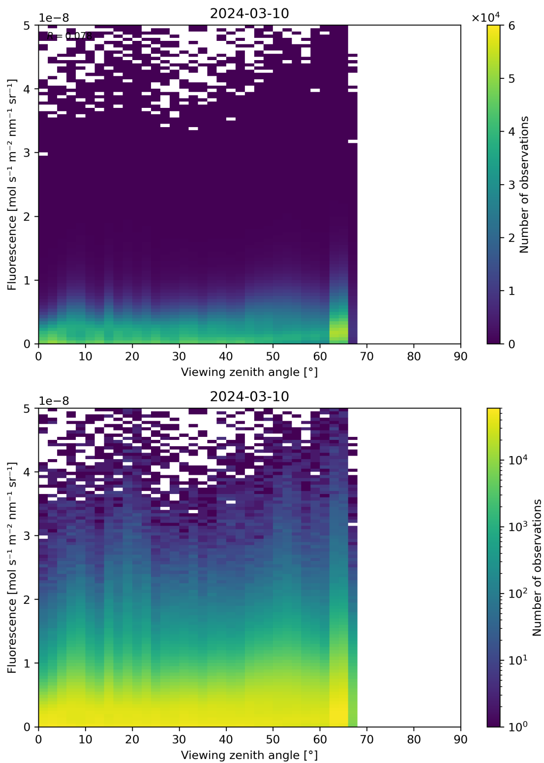
Figure 122: Scatter density plot of “Viewing zenith angle” against “Fluorescence” for 2024-03-09 to 2024-03-11.
