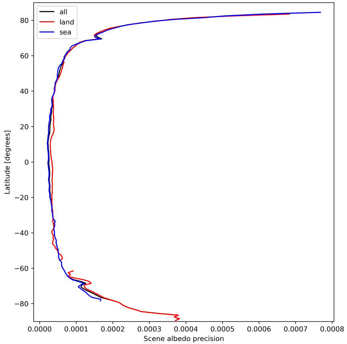
Figure 18: Zonal average of “Scene albedo precision” for 2024-03-09 to 2024-03-11.
