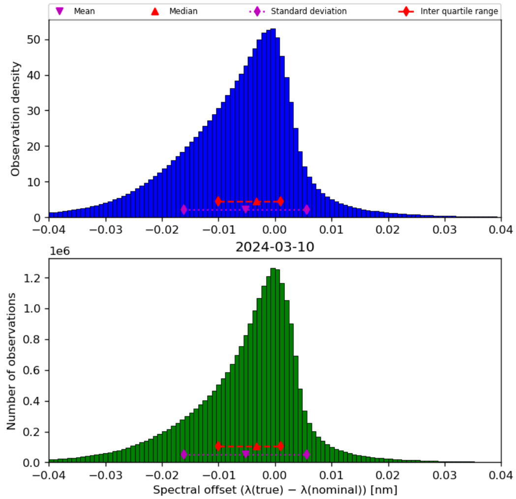
Figure 45: Histogram of “Spectral offset ( \lambda(\text{true}) - \lambda(\text{nominal}) )” for 2024-03-09 to 2024-03-11
