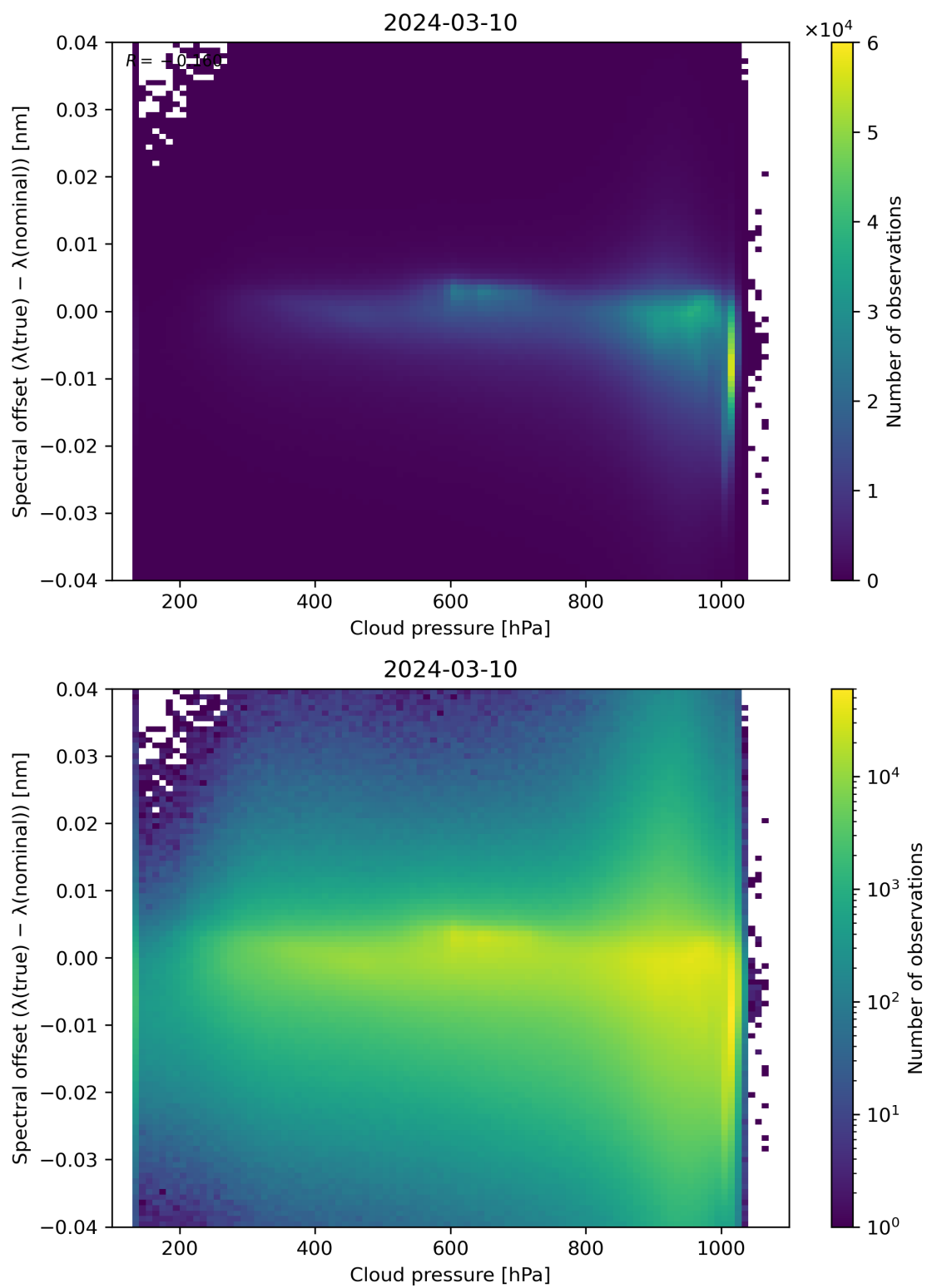
Figure 84: Scatter density plot of “Cloud pressure” against “Spectral offset ( \lambda(\text{true}) - \lambda(\text{nominal}) )” for 2024-03-09 to 2024-03-11.
