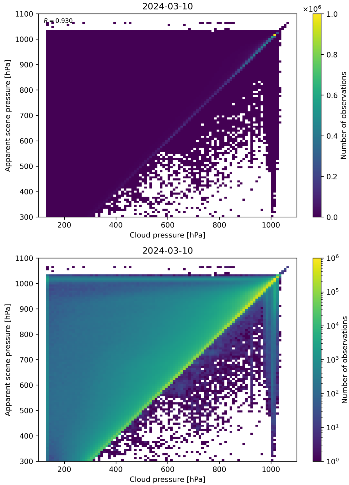
Figure 77: Scatter density plot of “Cloud pressure” against “Apparent scene pressure” for 2024-03-09 to 2024-03-11.
