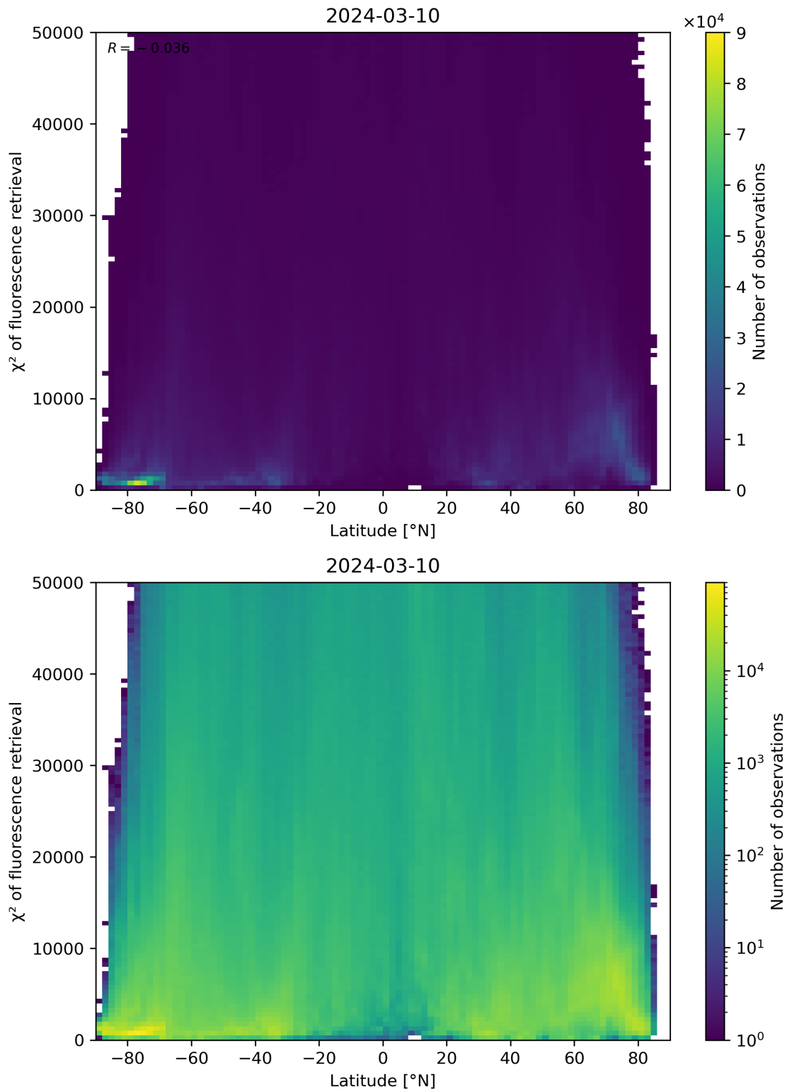
Figure 89: Scatter density plot of “Latitude” against “ \chi^2 of fluorescence retrieval” for 2024-03-09 to 2024-03-11.
