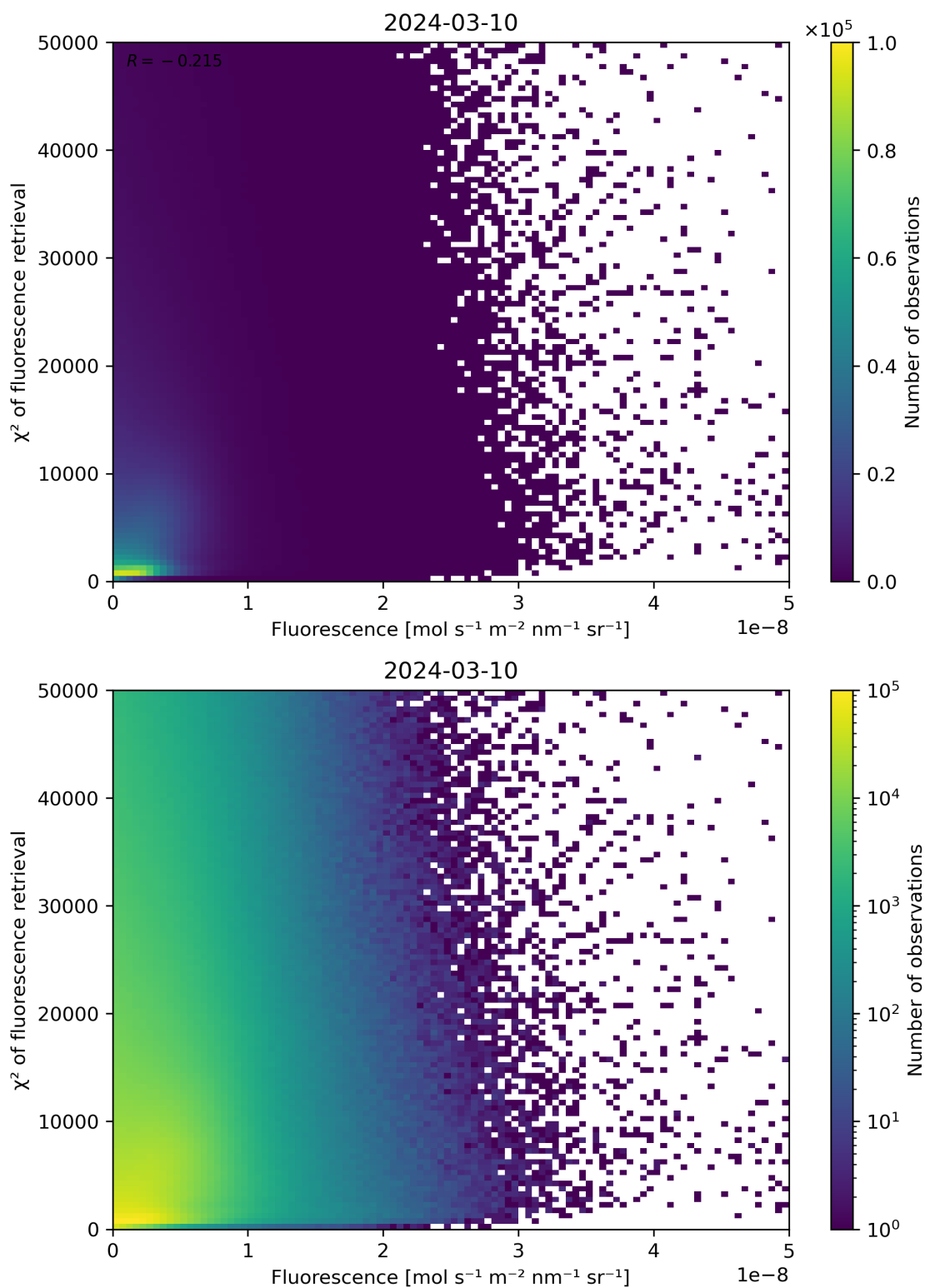
Figure 85: Scatter density plot of “Fluorescence” against “ \chi^2 of fluorescence retrieval” for 2024-03-09 to 2024-03-11.
