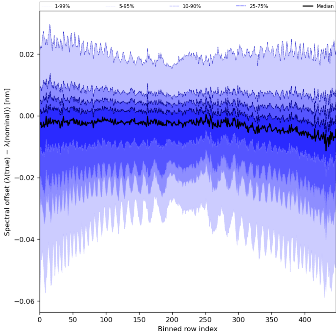
Figure 62: Along track statistics of “Spectral offset ( \lambda(\text{true}) - \lambda(\text{nominal}) )” for 2024-03-09 to 2024-03-11
