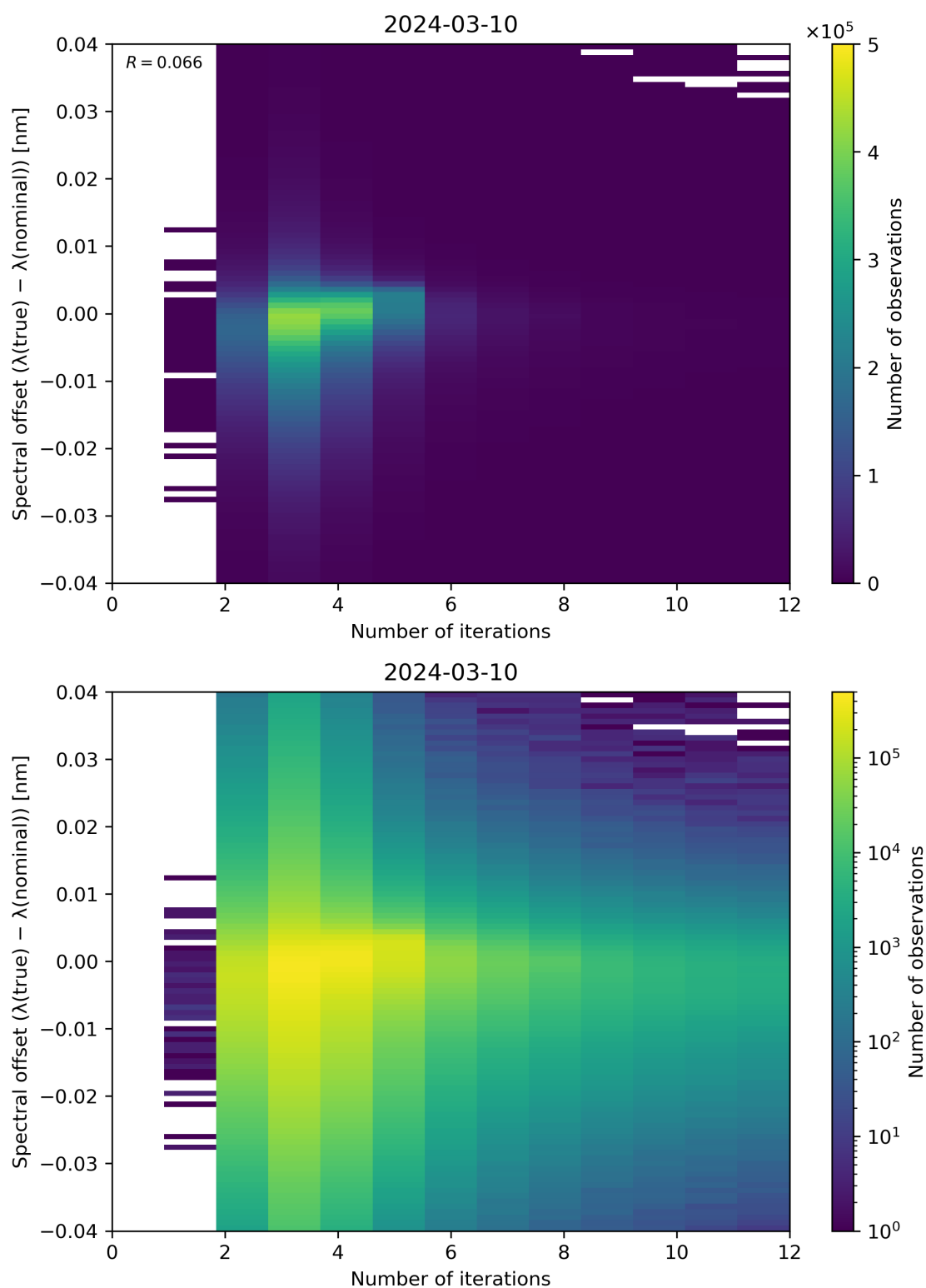
Figure 100: Scatter density plot of “Number of iterations” against “Spectral offset ( \lambda(\text{true}) - \lambda(\text{nominal}) )” for 2024-03-09 to 2024-03-11.
