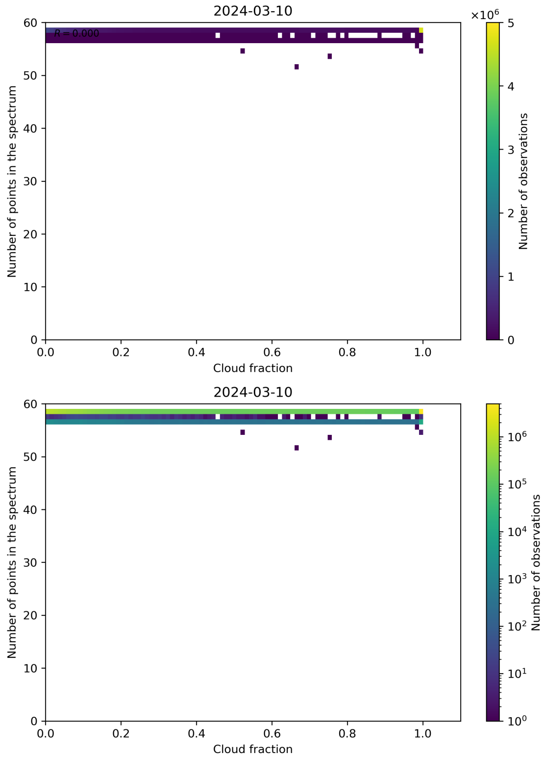
Figure 74: Scatter density plot of “Cloud fraction” against “Number of points in the spectrum” for 2024-03-09 to 2024-03-11.
