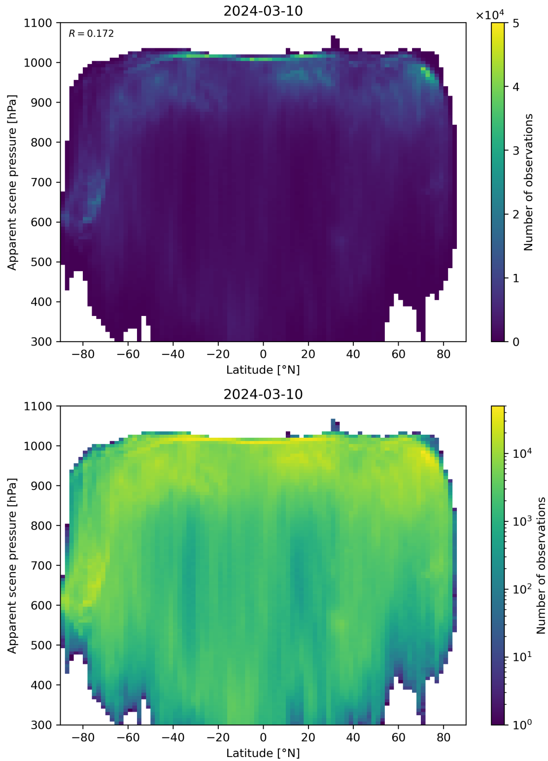
Figure 88: Scatter density plot of “Latitude” against “Apparent scene pressure” for 2024-03-09 to 2024-03-11.
