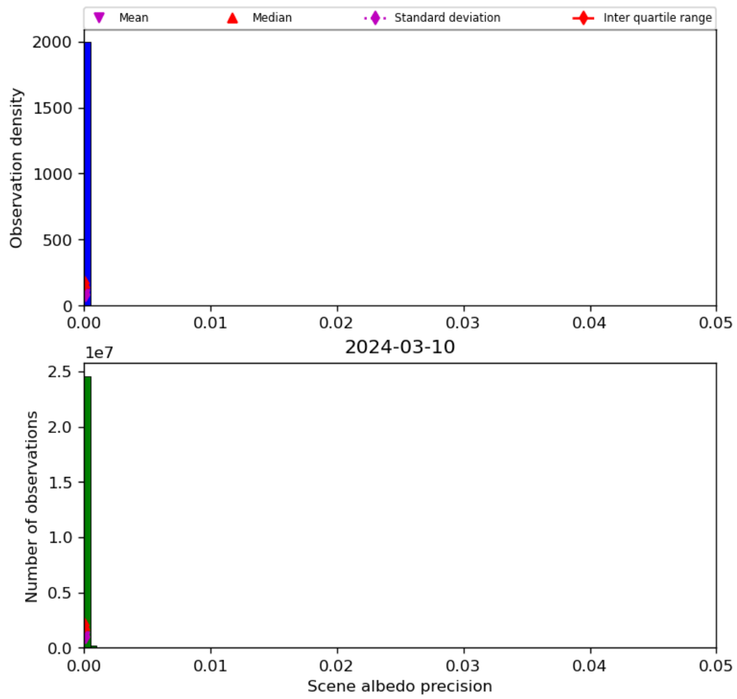
Figure 35: Histogram of “Scene albedo precision” for 2024-03-09 to 2024-03-11
