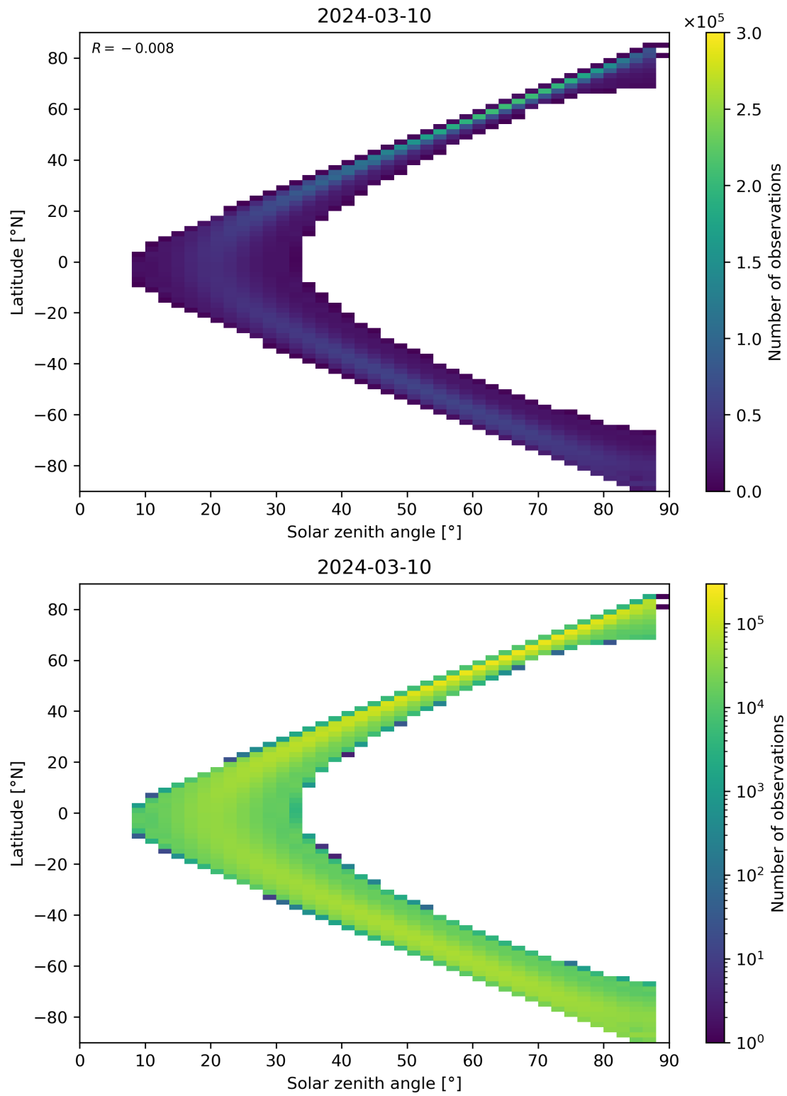
Figure 113: Scatter density plot of “Solar zenith angle” against “Latitude” for 2024-03-09 to 2024-03-11.
