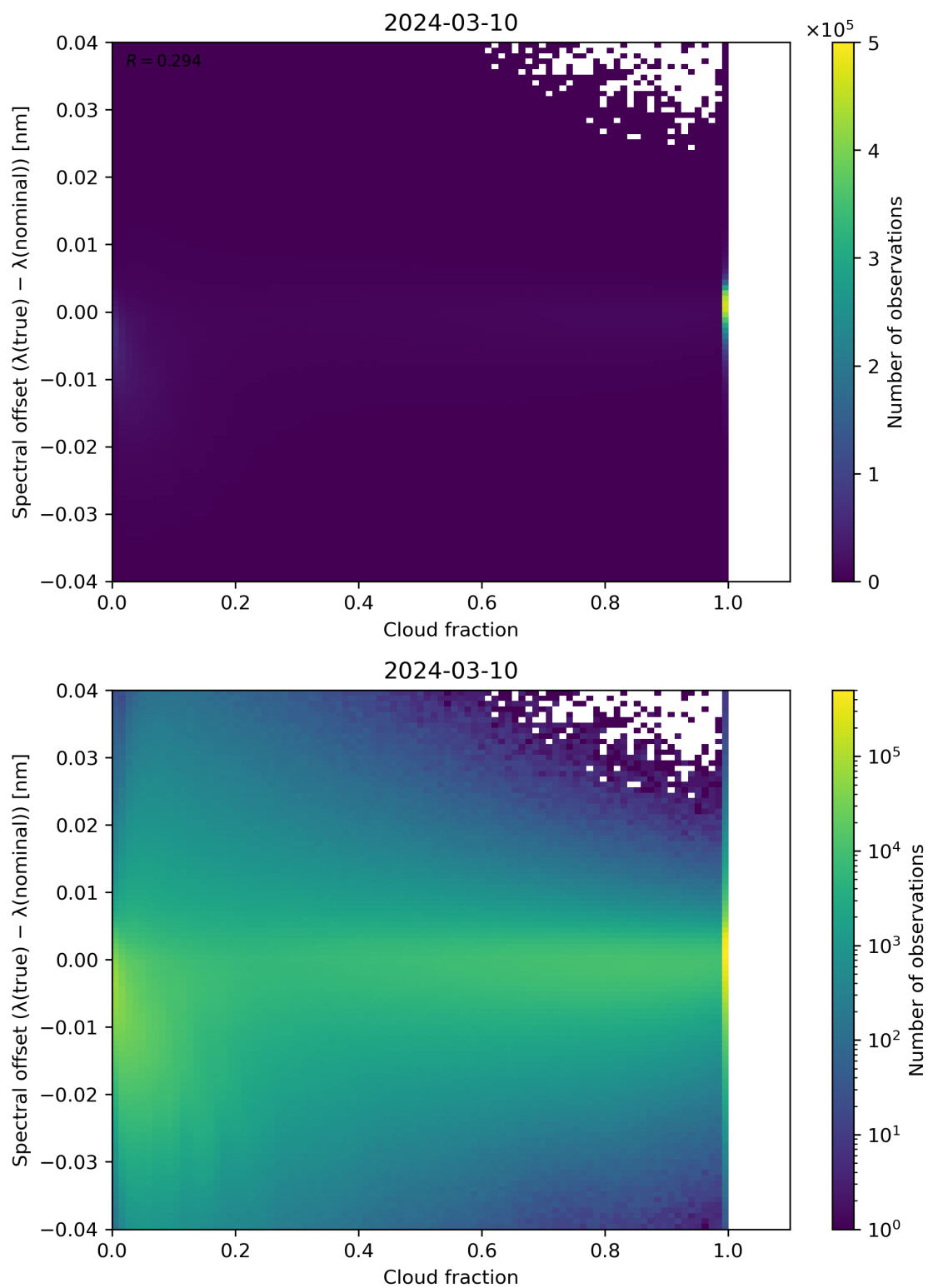
Figure 76: Scatter density plot of “Cloud fraction” against “Spectral offset ( \lambda(\text{true}) - \lambda(\text{nominal}) )” for 2024-03-09 to 2024-03-11.
