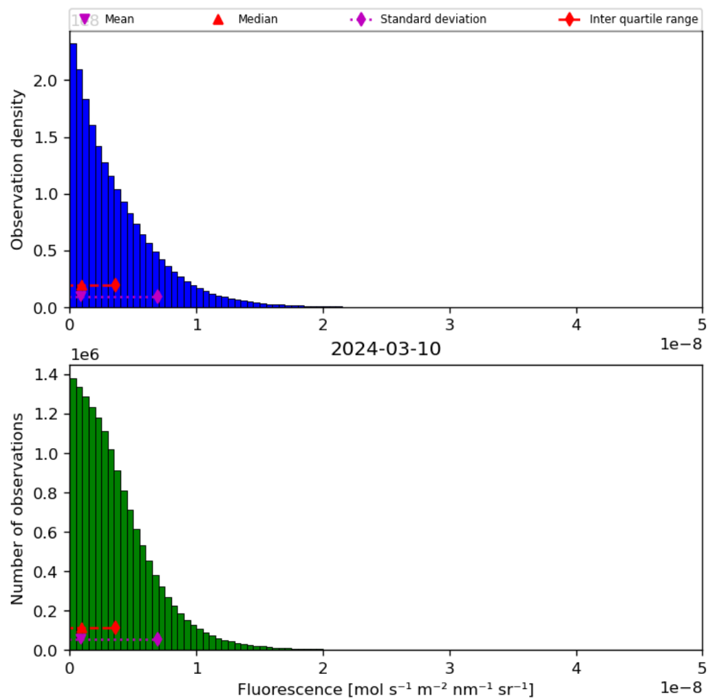
Figure 40: Histogram of “Fluorescence” for 2024-03-09 to 2024-03-11
