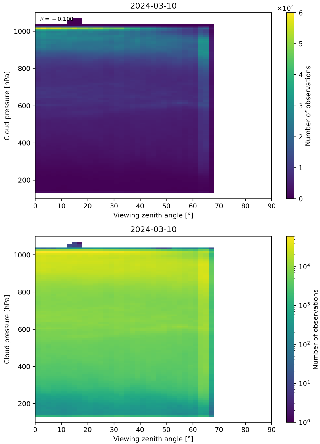
Figure 121: Scatter density plot of “Viewing zenith angle” against “Cloud pressure” for 2024-03-09 to 2024-03-11.
