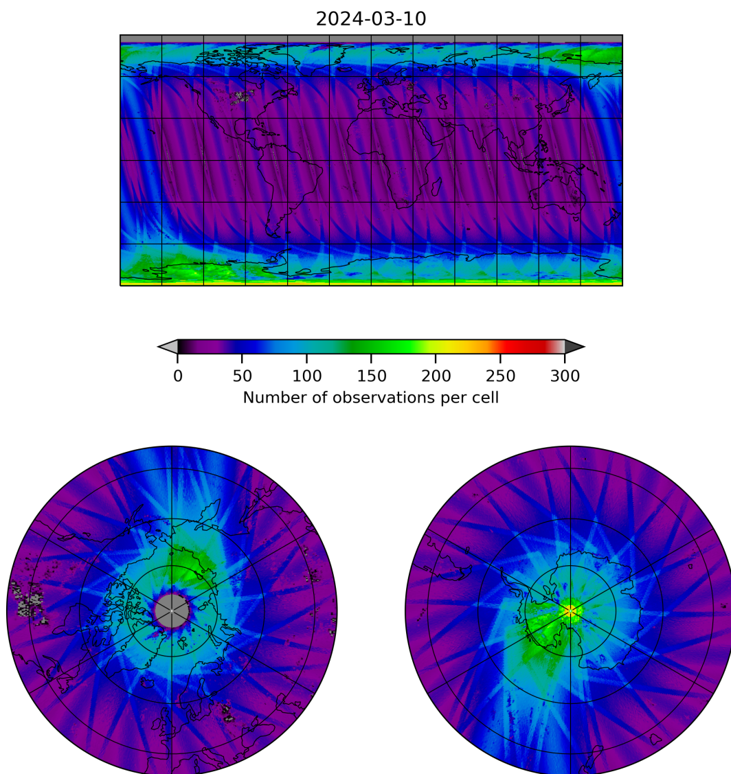
Figure 11: Map of the number of observations for 2024-03-09 to 2024-03-11
