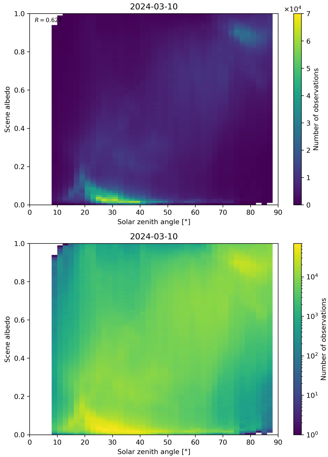
Figure 116: Scatter density plot of “Solar zenith angle” against “Scene albedo” for 2024-03-09 to 2024-03-11.
