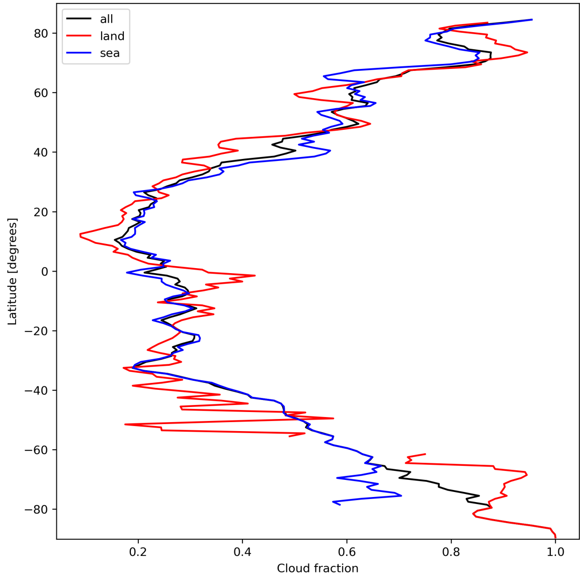
Figure 15: Zonal average of “Cloud fraction” for 2024-03-09 to 2024-03-11.
