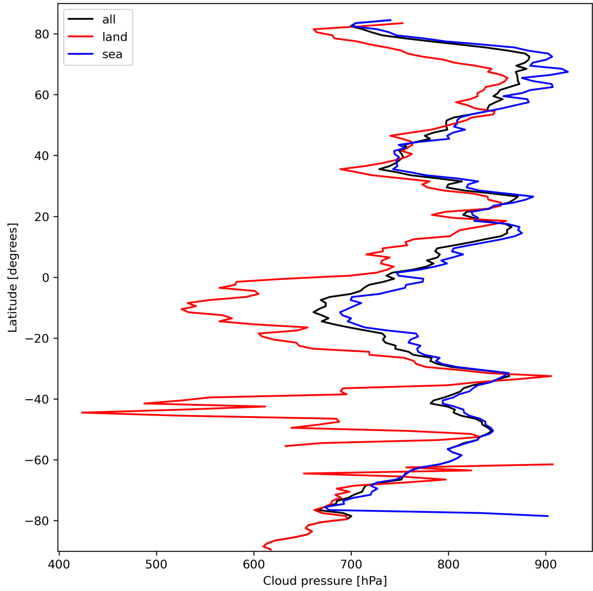
Figure 13: Zonal average of “Cloud pressure” for 2024-03-09 to 2024-03-11.
