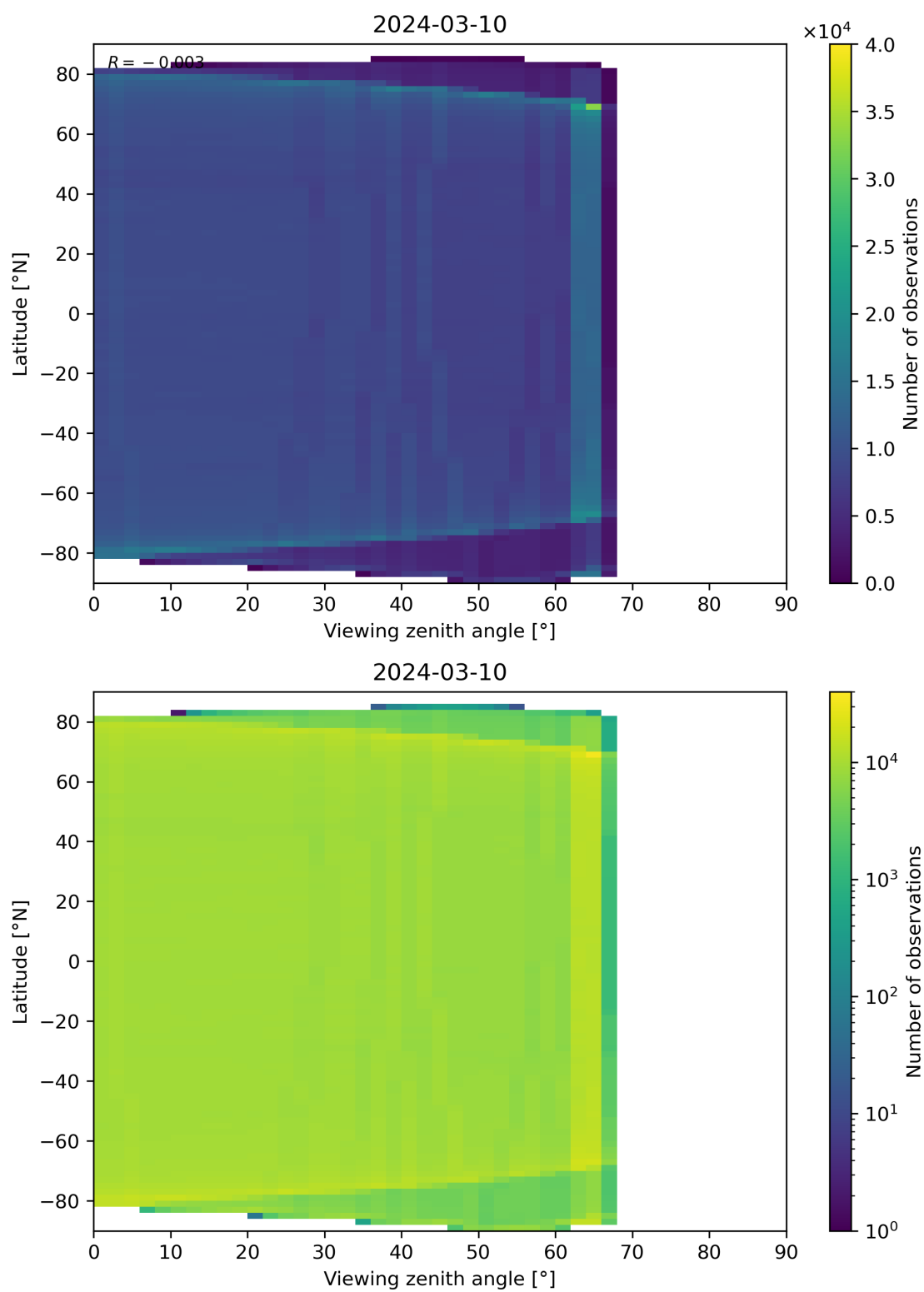
Figure 123: Scatter density plot of “Viewing zenith angle” against “Latitude” for 2024-03-09 to 2024-03-11.
