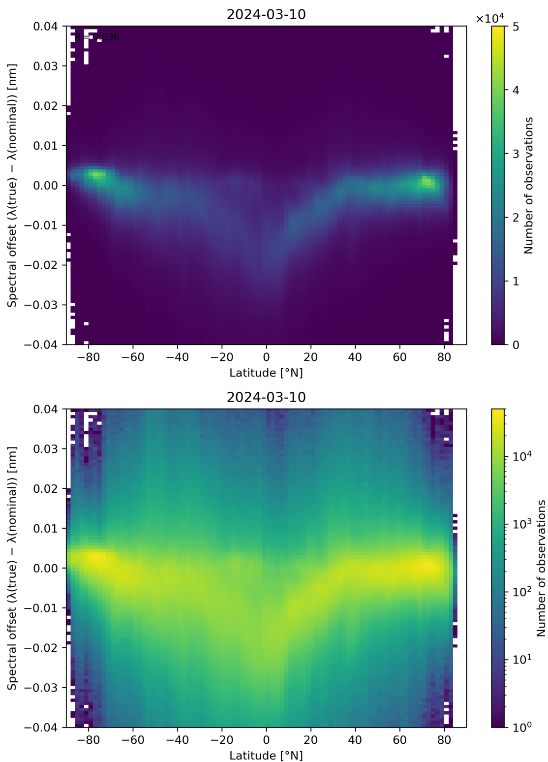
Figure 96: Scatter density plot of “Latitude” against “Spectral offset ( \lambda(\text{true}) - \lambda(\text{nominal}) )” for 2024-03-09 to 2024-03-11.
