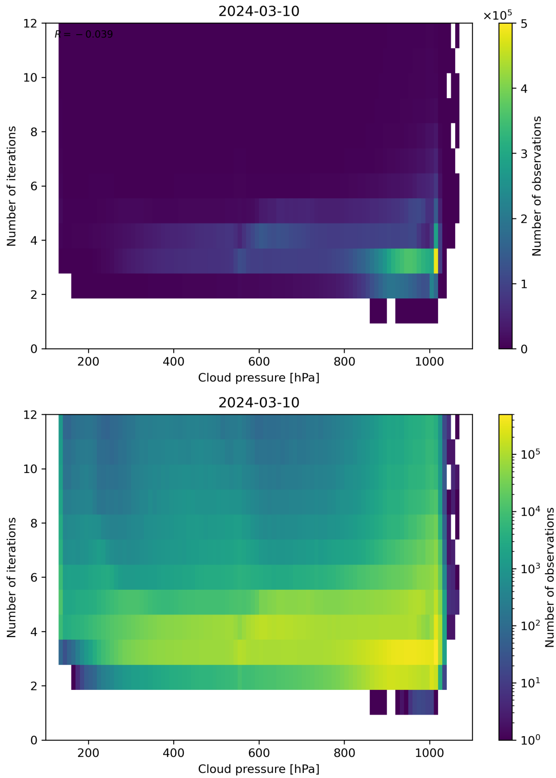
Figure 81: Scatter density plot of “Cloud pressure” against “Number of iterations” for 2024-03-09 to 2024-03-11.
