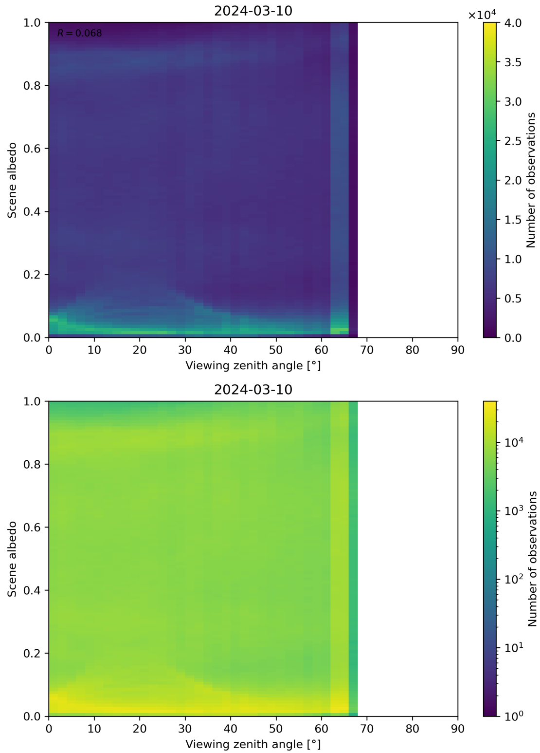
Figure 126: Scatter density plot of “Viewing zenith angle” against “Scene albedo” for 2024-03-09 to 2024-03-11.
