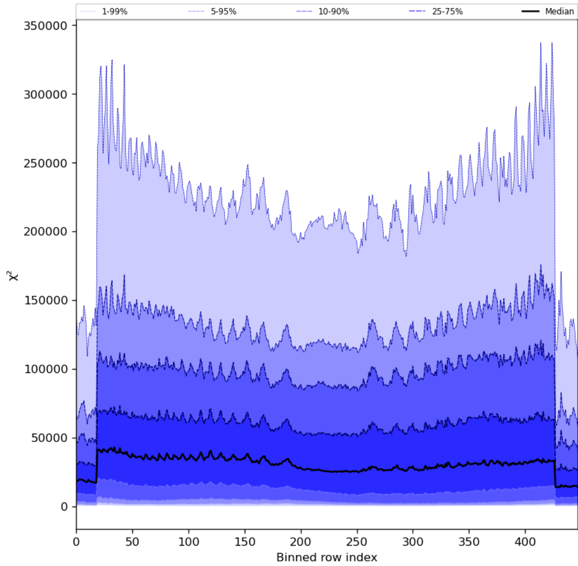
Figure 55: Along track statistics of “ \chi^2 ” for 2024-03-09 to 2024-03-11
