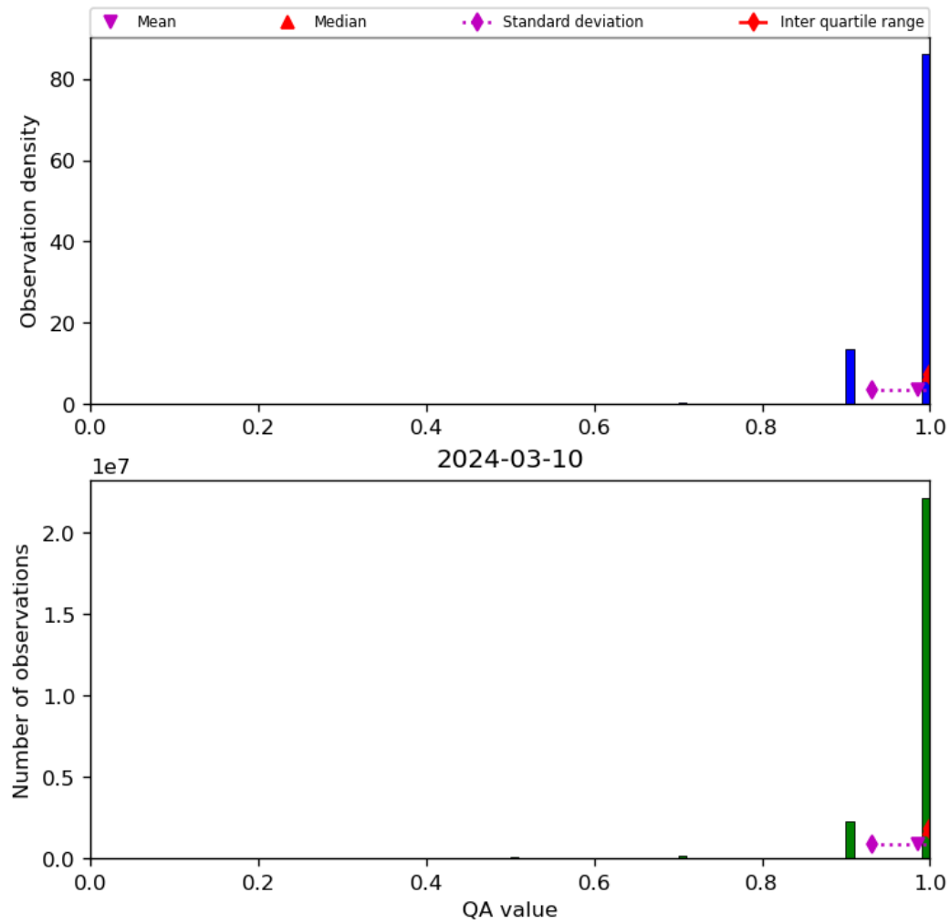
Figure 29: Histogram of “QA value” for 2024-03-09 to 2024-03-11
