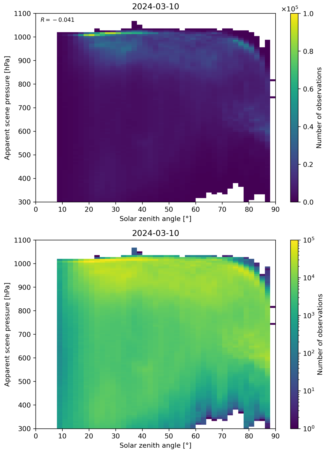
Figure 108: Scatter density plot of “Solar zenith angle” against “Apparent scene pressure” for 2024-03-09 to 2024-03-11.
