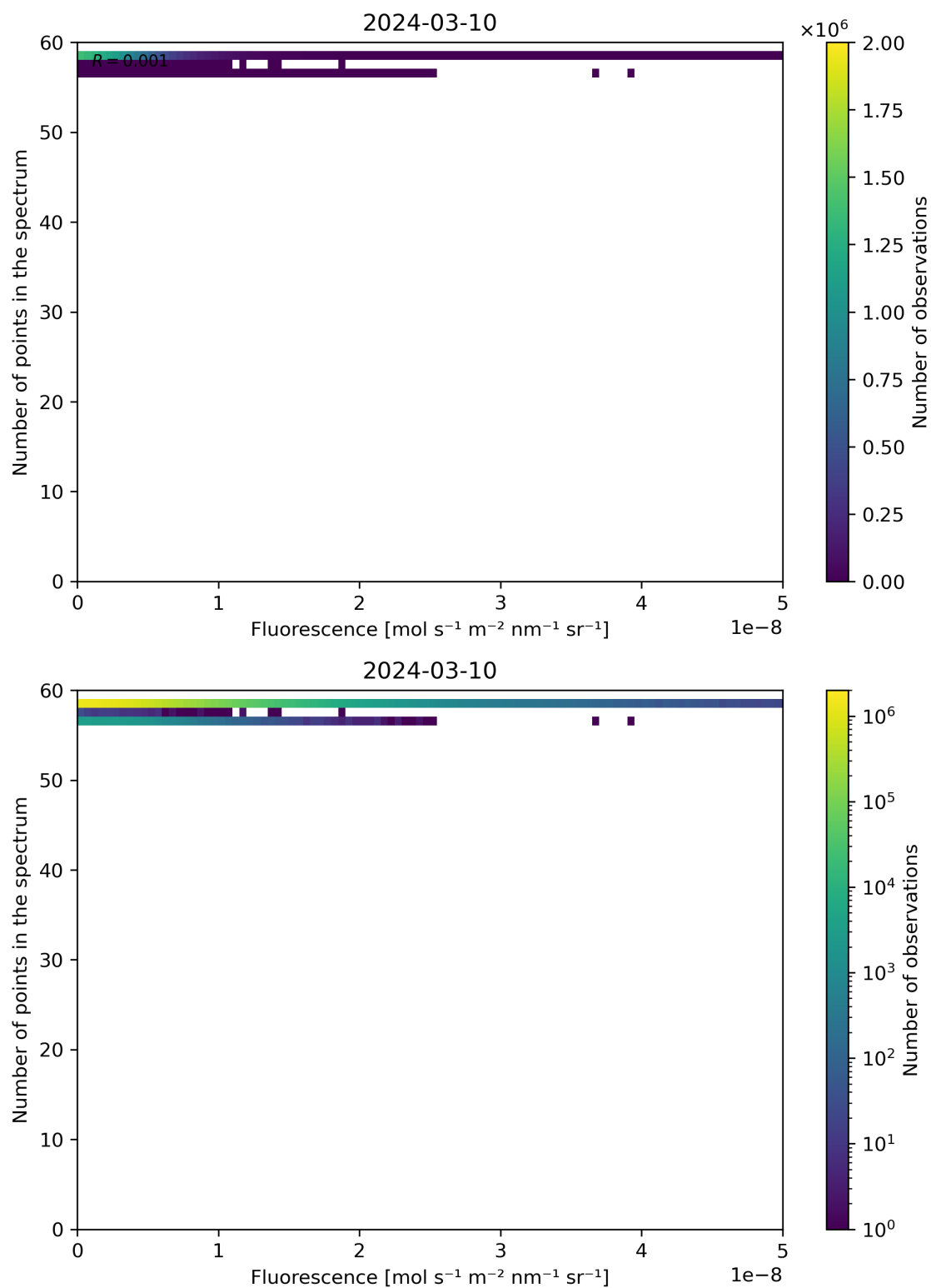
Figure 86: Scatter density plot of “Fluorescence” against “Number of points in the spectrum” for 2024-03-09 to 2024-03-11.
