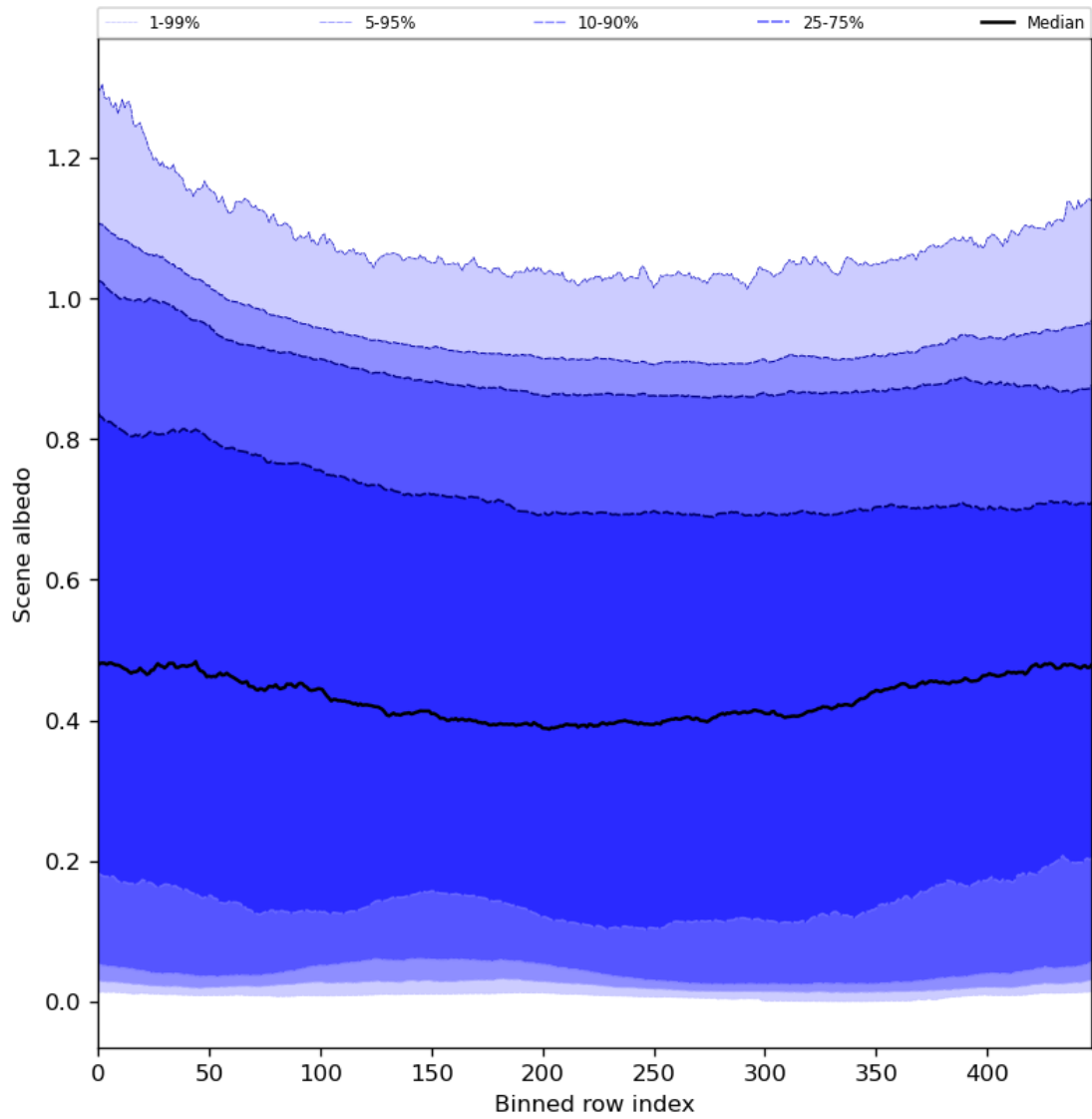
Figure 51: Along track statistics of “Scene albedo” for 2024-03-09 to 2024-03-11
