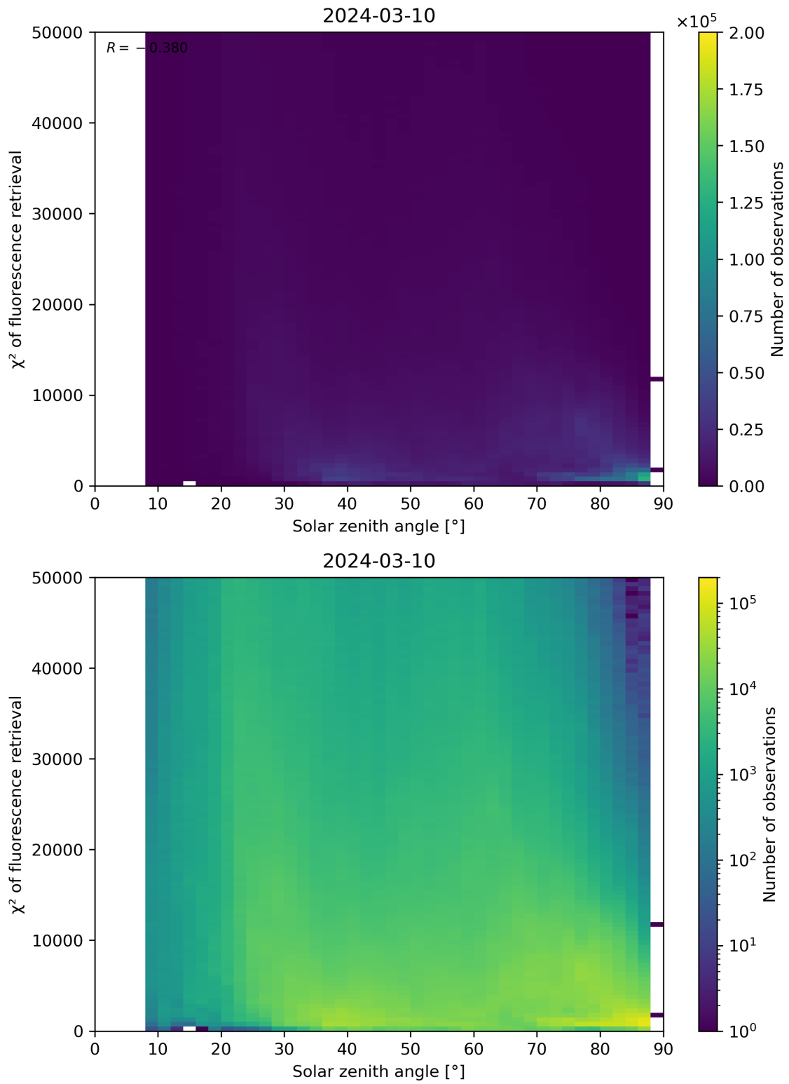
Figure 109: Scatter density plot of “Solar zenith angle” against “ \chi^2 of fluorescence retrieval” for 2024-03-09 to 2024-03-11.
