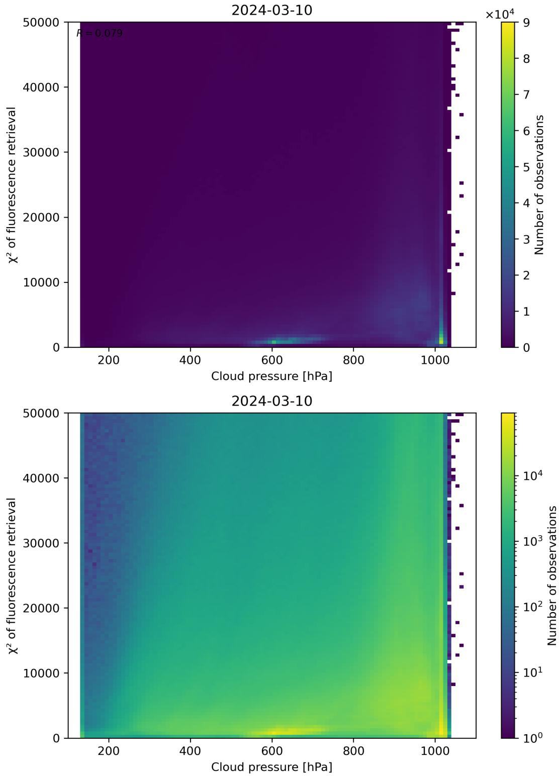
Figure 78: Scatter density plot of “Cloud pressure” against “ \chi^2 of fluorescence retrieval” for 2024-03-09 to 2024-03-11.
