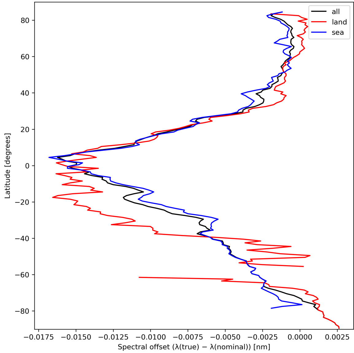
Figure 28: Zonal average of “Spectral offset ( \lambda(\text{true}) - \lambda(\text{nominal}) )” for 2024-03-09 to 2024-03-11.
