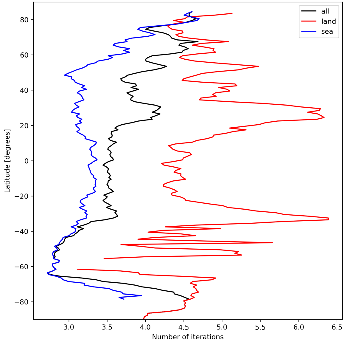
Figure 22: Zonal average of “Number of iterations” for 2024-03-09 to 2024-03-11.
