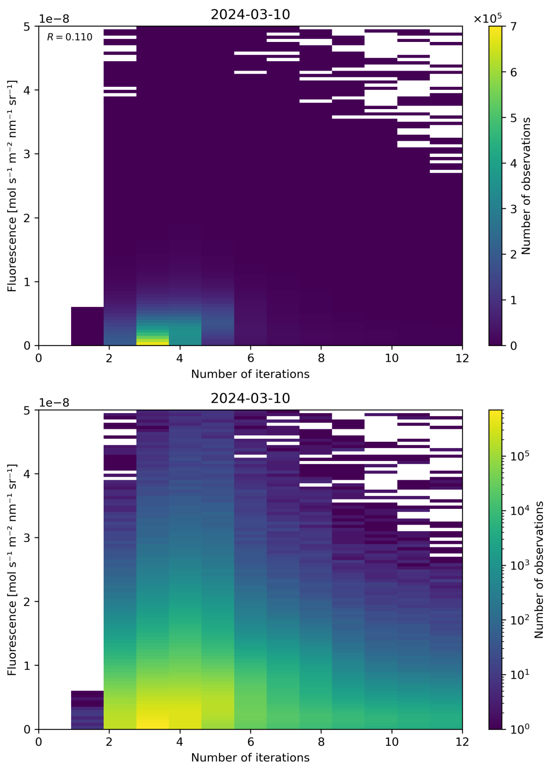
Figure 98: Scatter density plot of “Number of iterations” against “Fluorescence” for 2024-03-09 to 2024-03-11.
