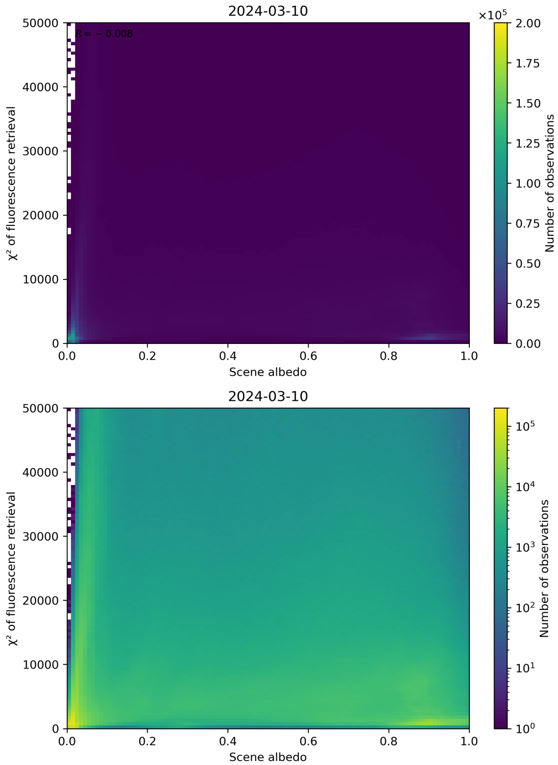
Figure 103: Scatter density plot of “Scene albedo” against “ \chi^2 of fluorescence retrieval” for 2024-03-09 to 2024-03-11.
