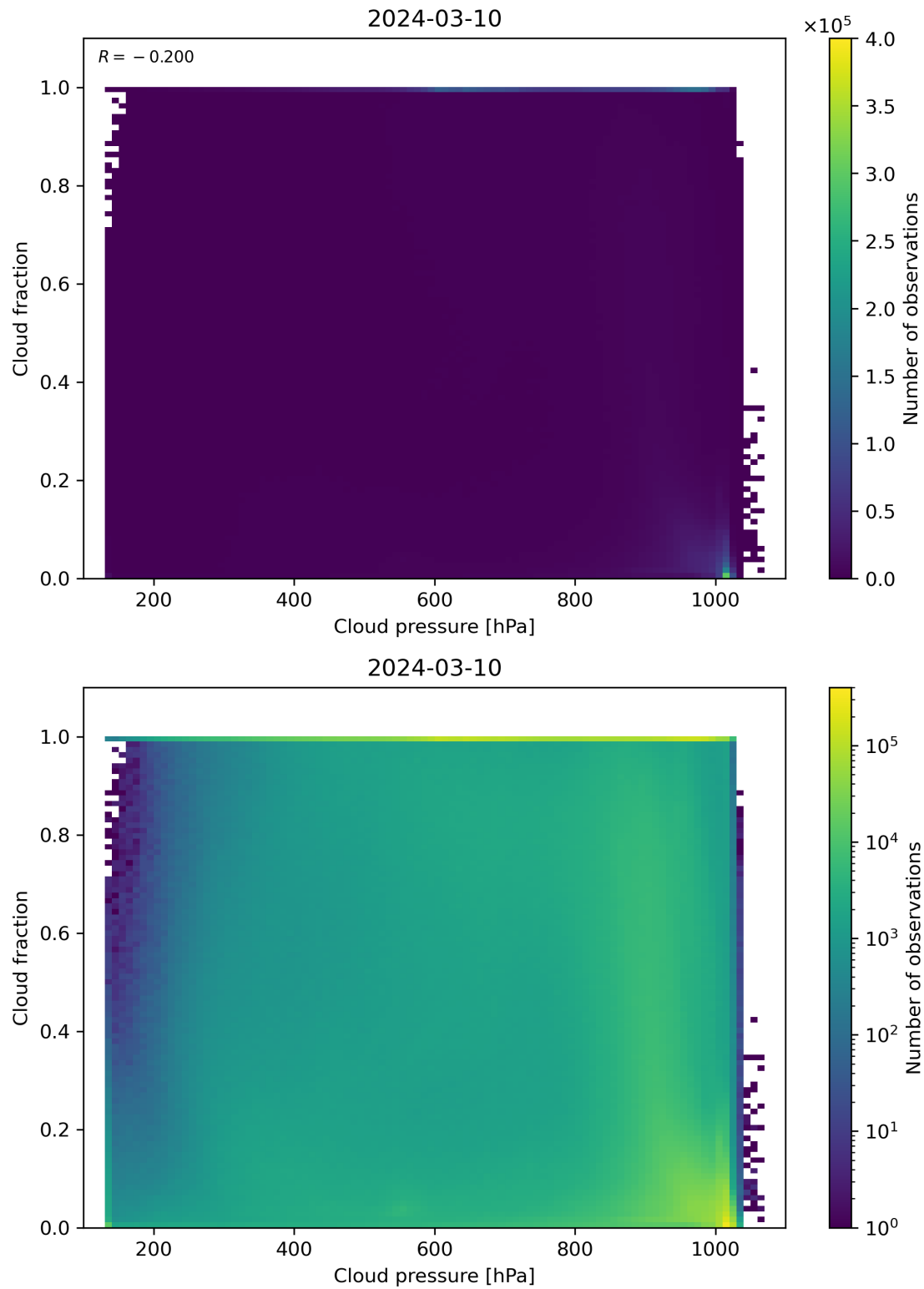
Figure 79: Scatter density plot of “Cloud pressure” against “Cloud fraction” for 2024-03-09 to 2024-03-11.
