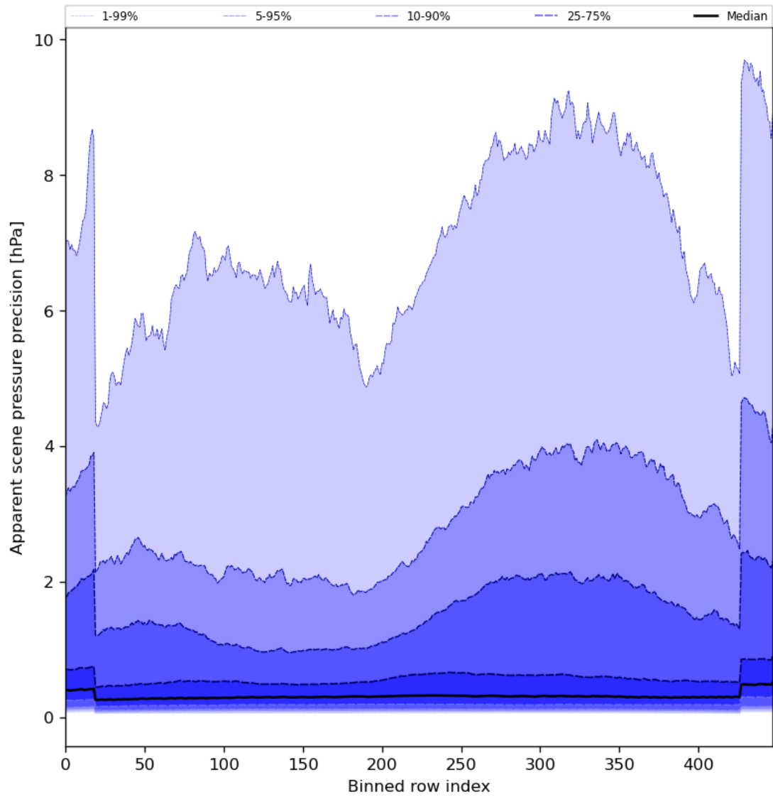
Figure 54: Along track statistics of “Apparent scene pressure precision” for 2024-03-09 to 2024-03-11
