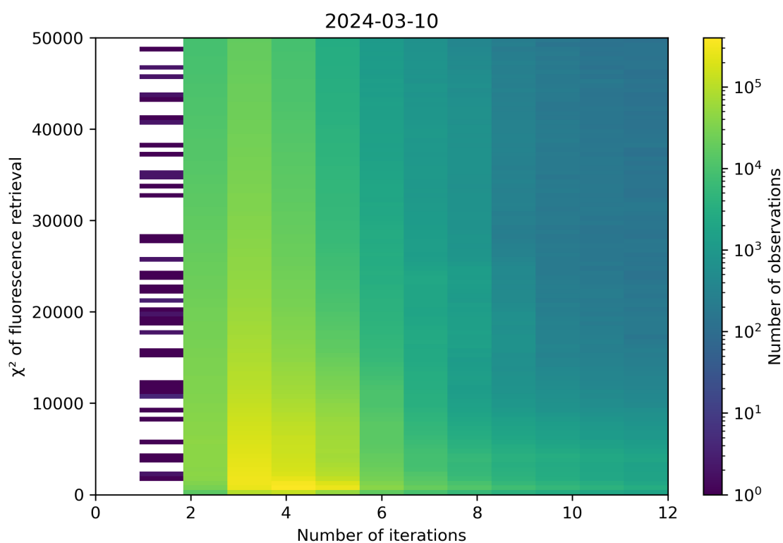
Figure 97: Scatter density plot of “Number of iterations” against “ \chi^2 of fluorescence retrieval” for 2024-03-09 to 2024-03-11.
