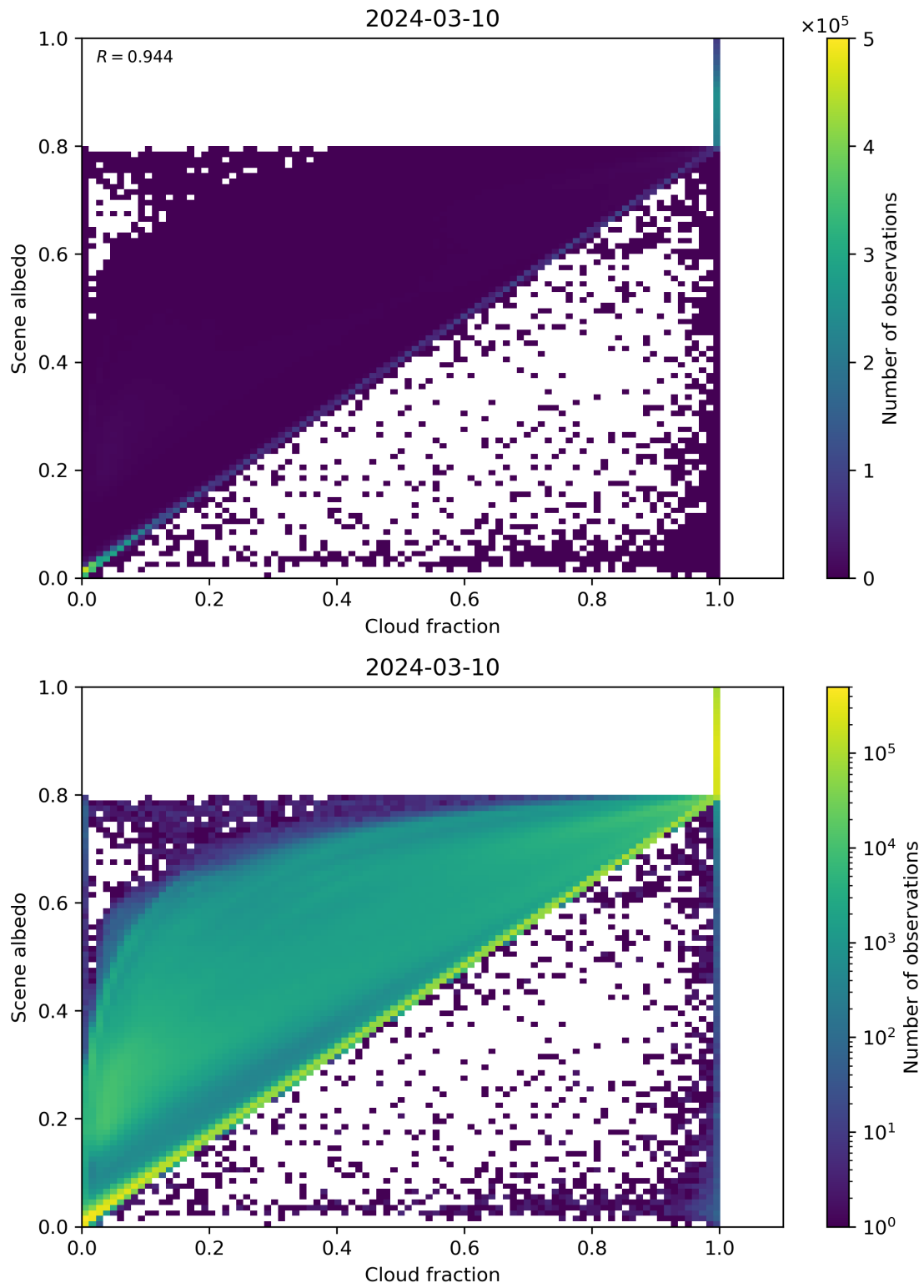
Figure 75: Scatter density plot of “Cloud fraction” against “Scene albedo” for 2024-03-09 to 2024-03-11.
