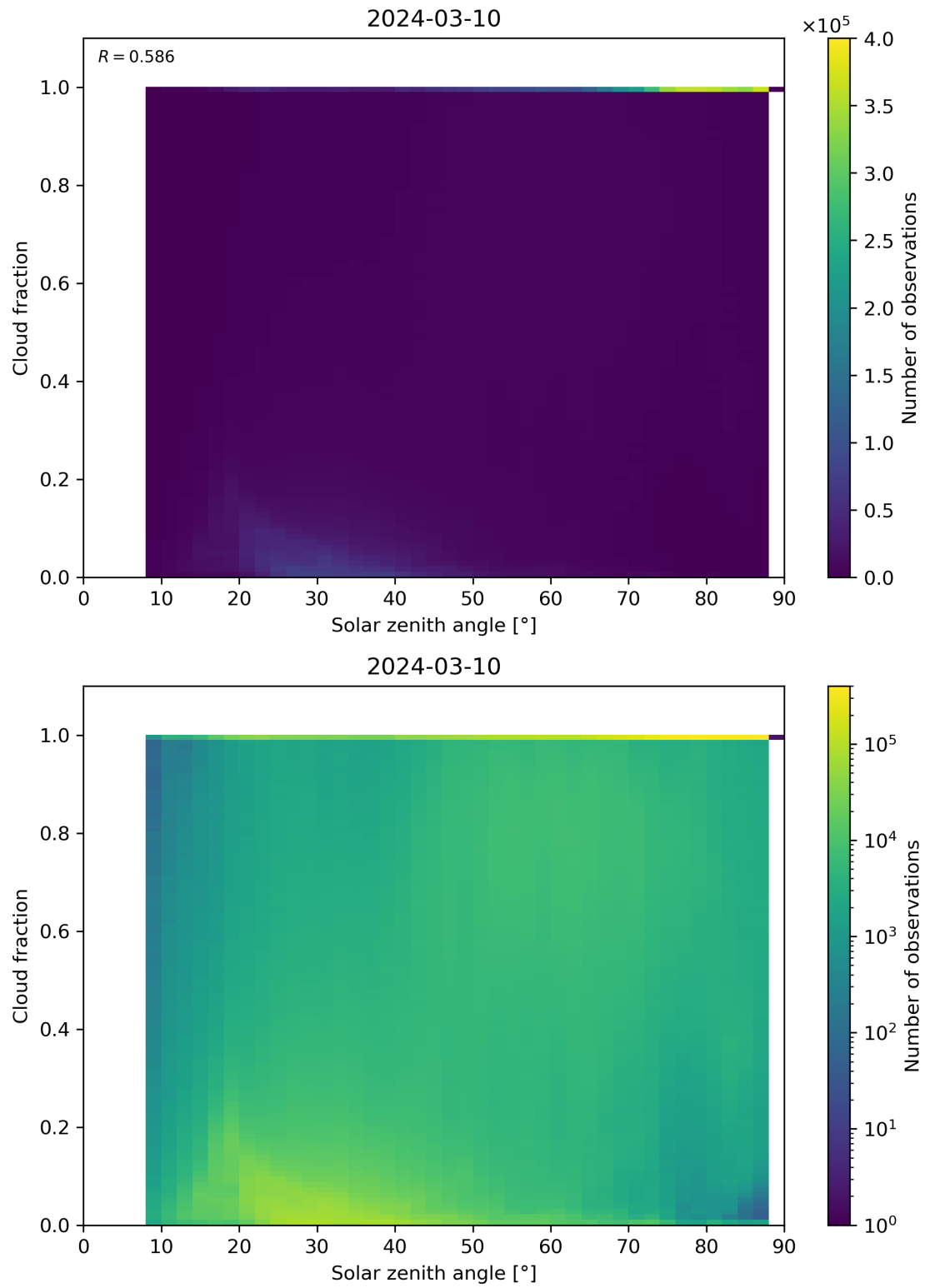
Figure 110: Scatter density plot of “Solar zenith angle” against “Cloud fraction” for 2024-03-09 to 2024-03-11.
