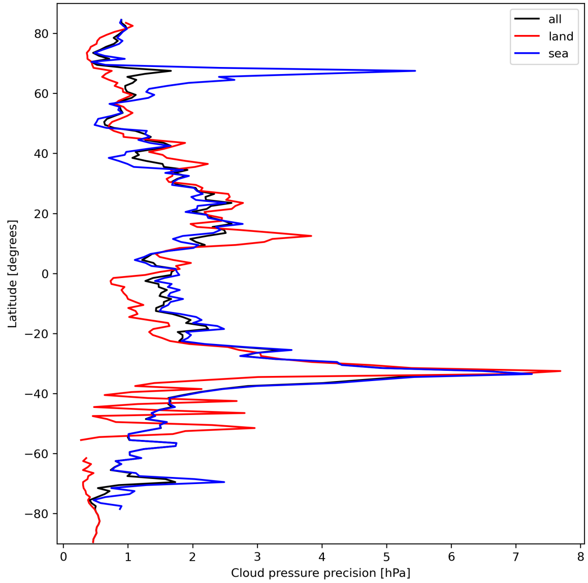
Figure 14: Zonal average of “Cloud pressure precision” for 2024-03-09 to 2024-03-11.
