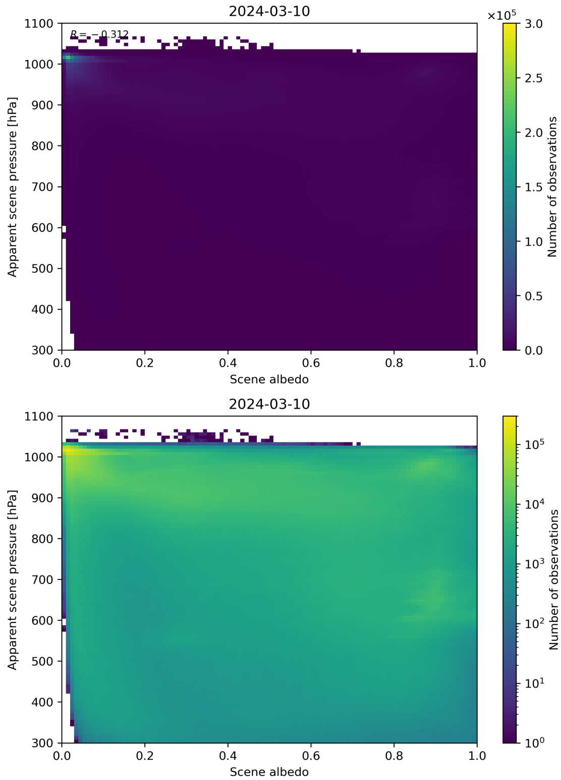
Figure 102: Scatter density plot of “Scene albedo” against “Apparent scene pressure” for 2024-03-09 to 2024-03-11.
