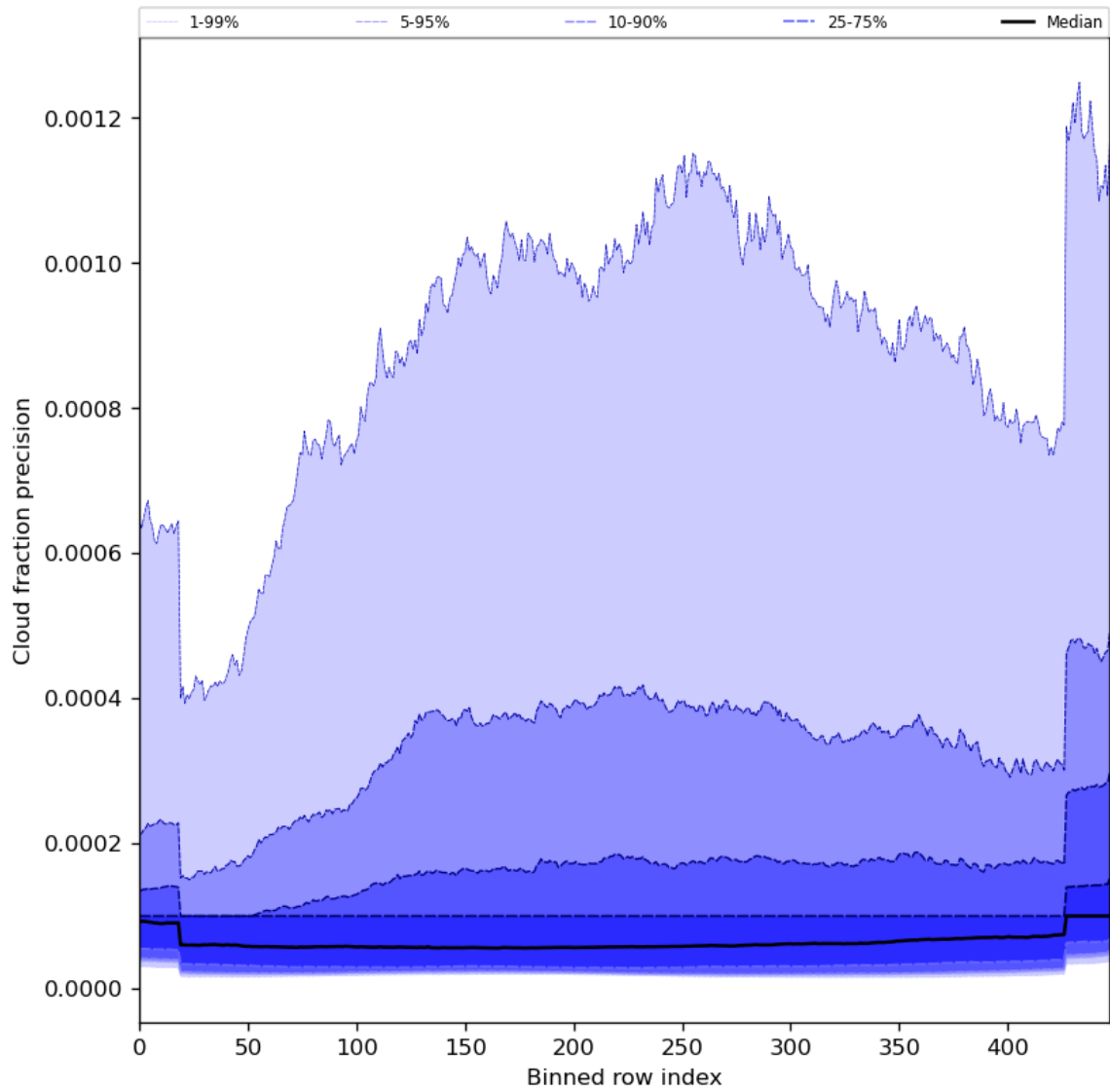
Figure 50: Along track statistics of “Cloud fraction precision” for 2024-03-09 to 2024-03-11
