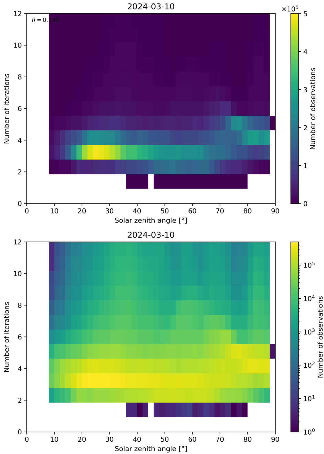
Figure 114: Scatter density plot of “Solar zenith angle” against “Number of iterations” for 2024-03-09 to 2024-03-11.
