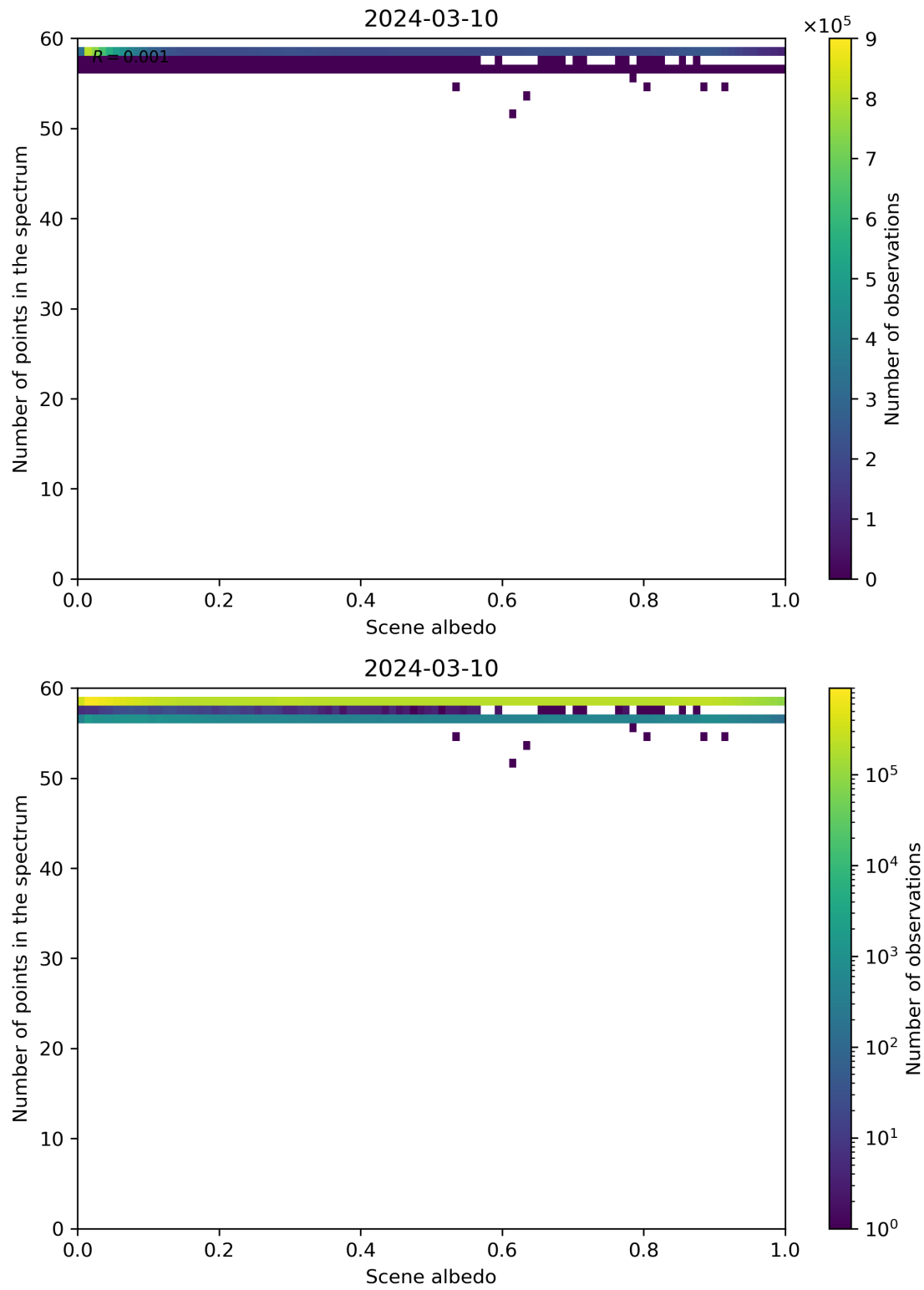
Figure 106: Scatter density plot of “Scene albedo” against “Number of points in the spectrum” for 2024-03-09 to 2024-03-11.
