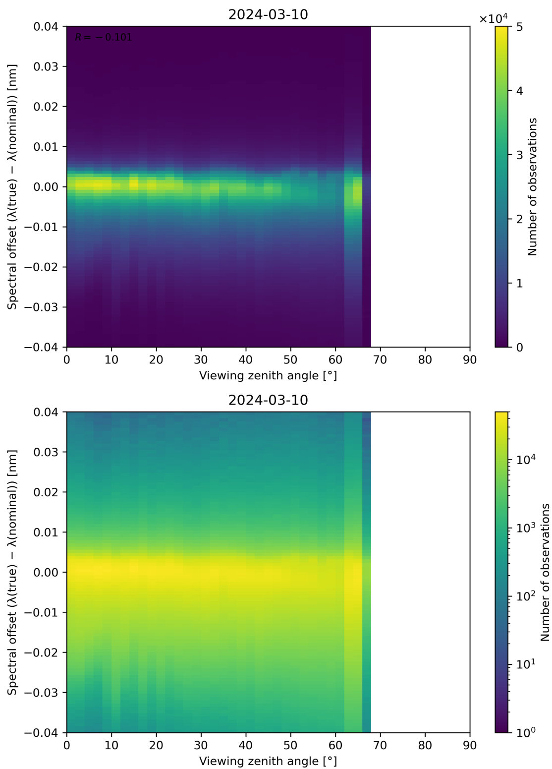
Figure 128: Scatter density plot of “Viewing zenith angle” against “Spectral offset ( \lambda(\text{true}) - \lambda(\text{nominal}) )” for 2024-03-09 to 2024-03-11.
