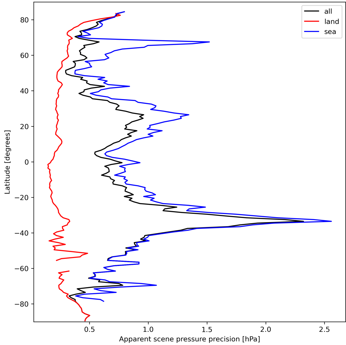
Figure 20: Zonal average of “Apparent scene pressure precision” for 2024-03-09 to 2024-03-11.
