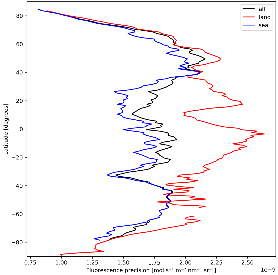
Figure 24: Zonal average of “Fluorescence precision” for 2024-03-09 to 2024-03-11.
