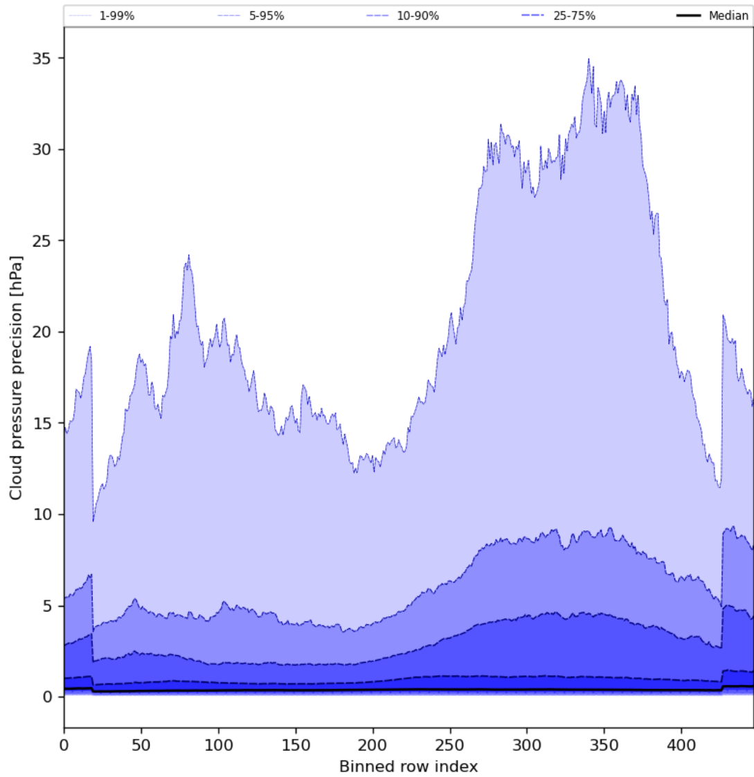
Figure 48: Along track statistics of “Cloud pressure precision” for 2024-03-09 to 2024-03-11
