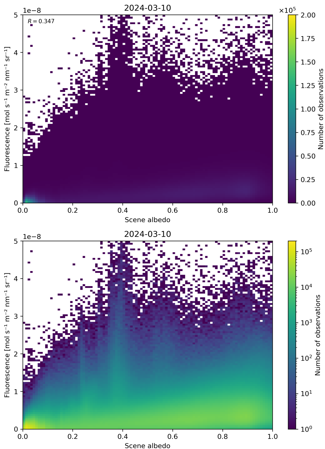
Figure 104: Scatter density plot of “Scene albedo” against “Fluorescence” for 2024-03-09 to 2024-03-11.
