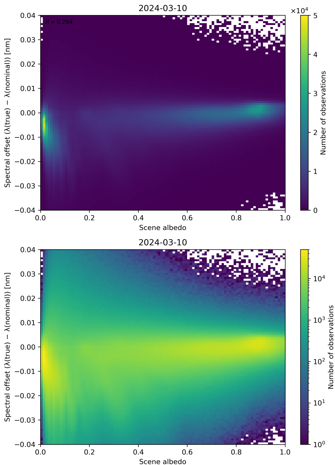
Figure 107: Scatter density plot of “Scene albedo” against “Spectral offset ( \lambda(\text{true}) - \lambda(\text{nominal}) )” for 2024-03-09 to 2024-03-11.
