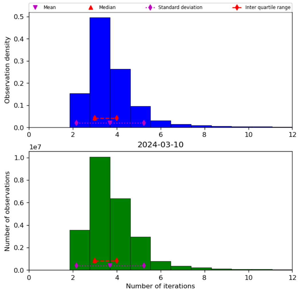
Figure 39: Histogram of “Number of iterations” for 2024-03-09 to 2024-03-11
