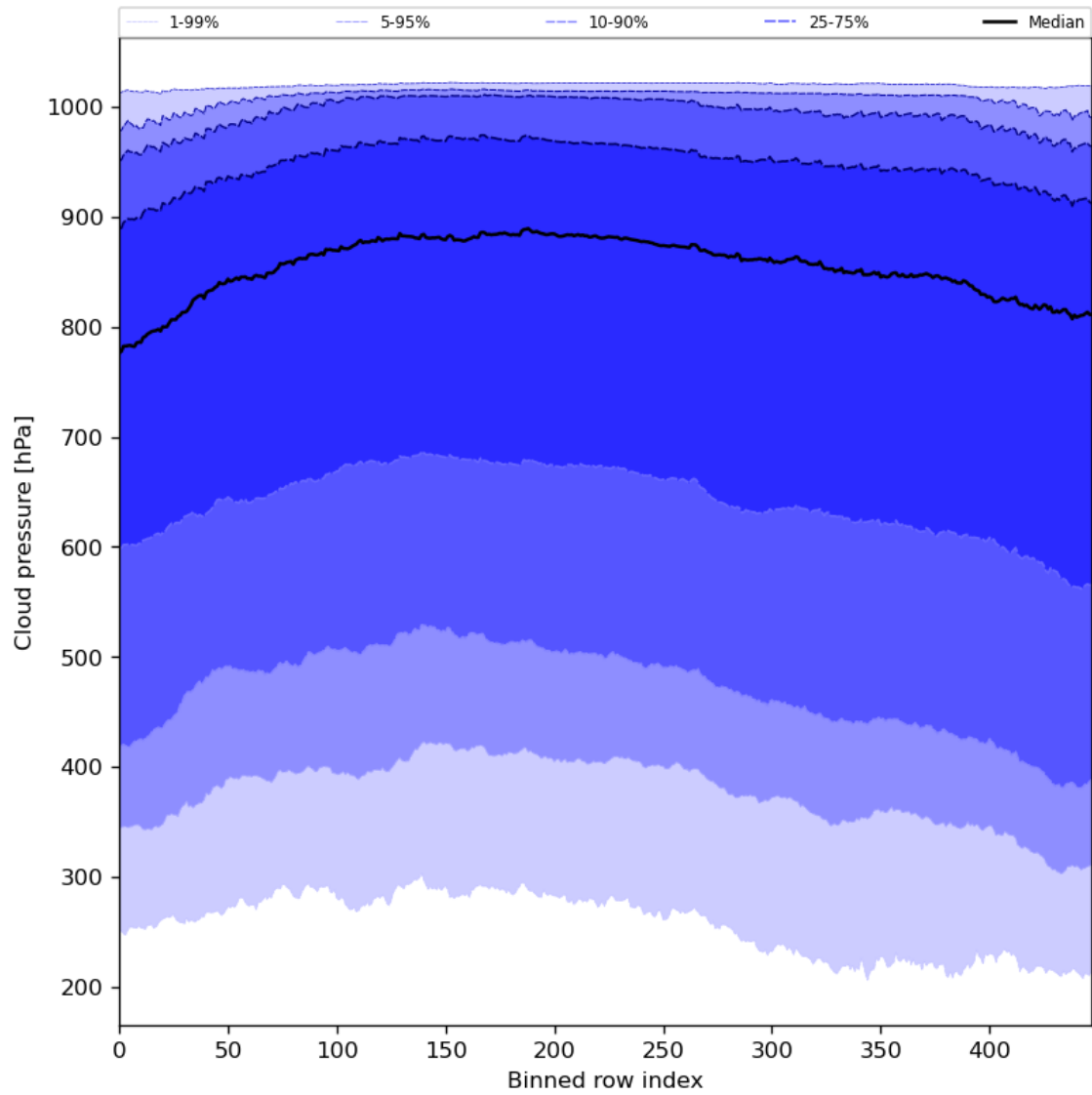
Figure 47: Along track statistics of “Cloud pressure” for 2024-03-09 to 2024-03-11
