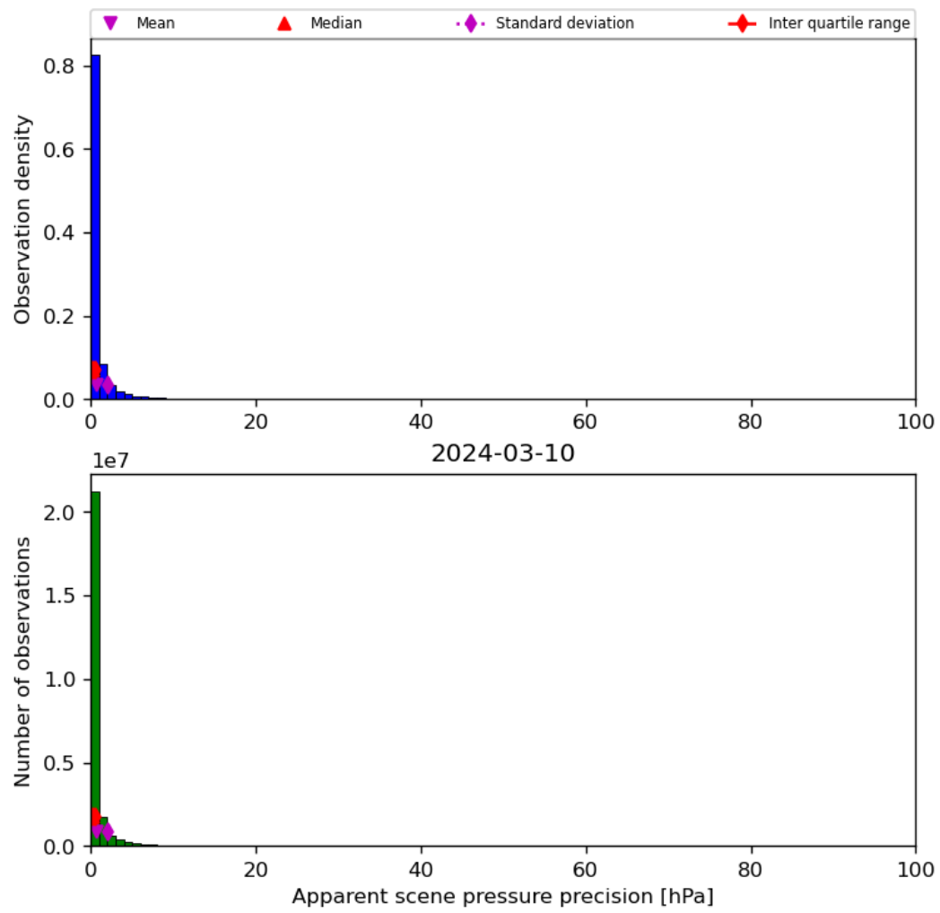
Figure 37: Histogram of “Apparent scene pressure precision” for 2024-03-09 to 2024-03-11
