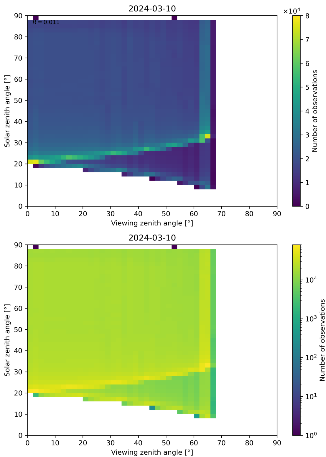
Figure 127: Scatter density plot of “Viewing zenith angle” against “Solar zenith angle” for 2024-03-09 to 2024-03-11.
