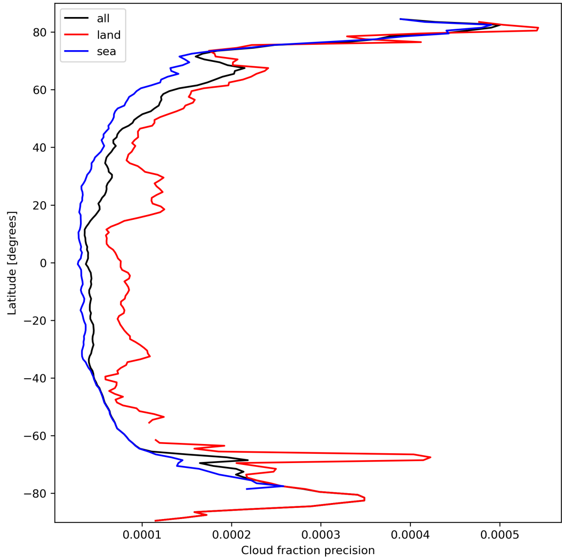
Figure 16: Zonal average of “Cloud fraction precision” for 2024-03-09 to 2024-03-11.
