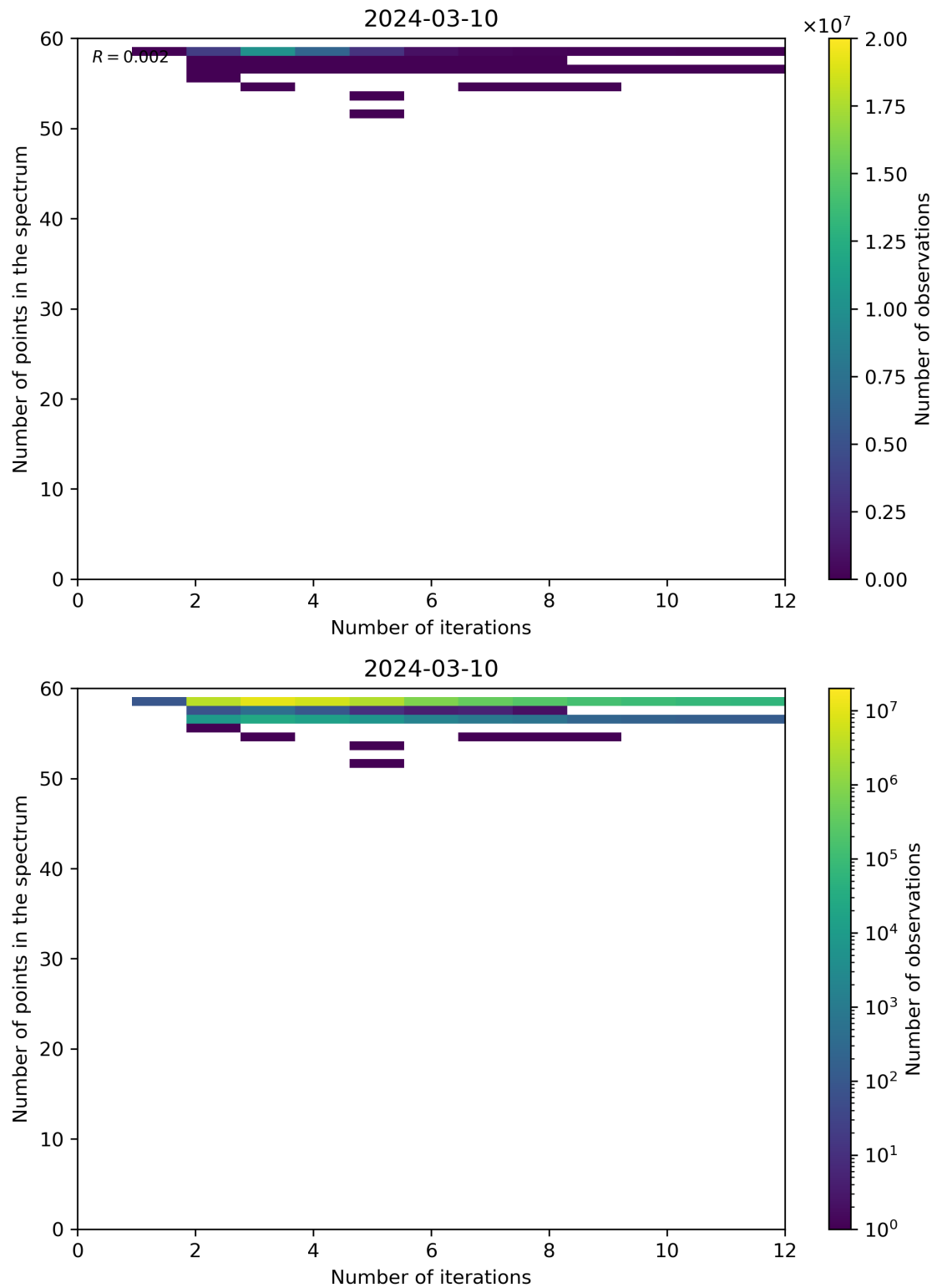
Figure 99: Scatter density plot of “Number of iterations” against “Number of points in the spectrum” for 2024-03-09 to 2024-03-11.
