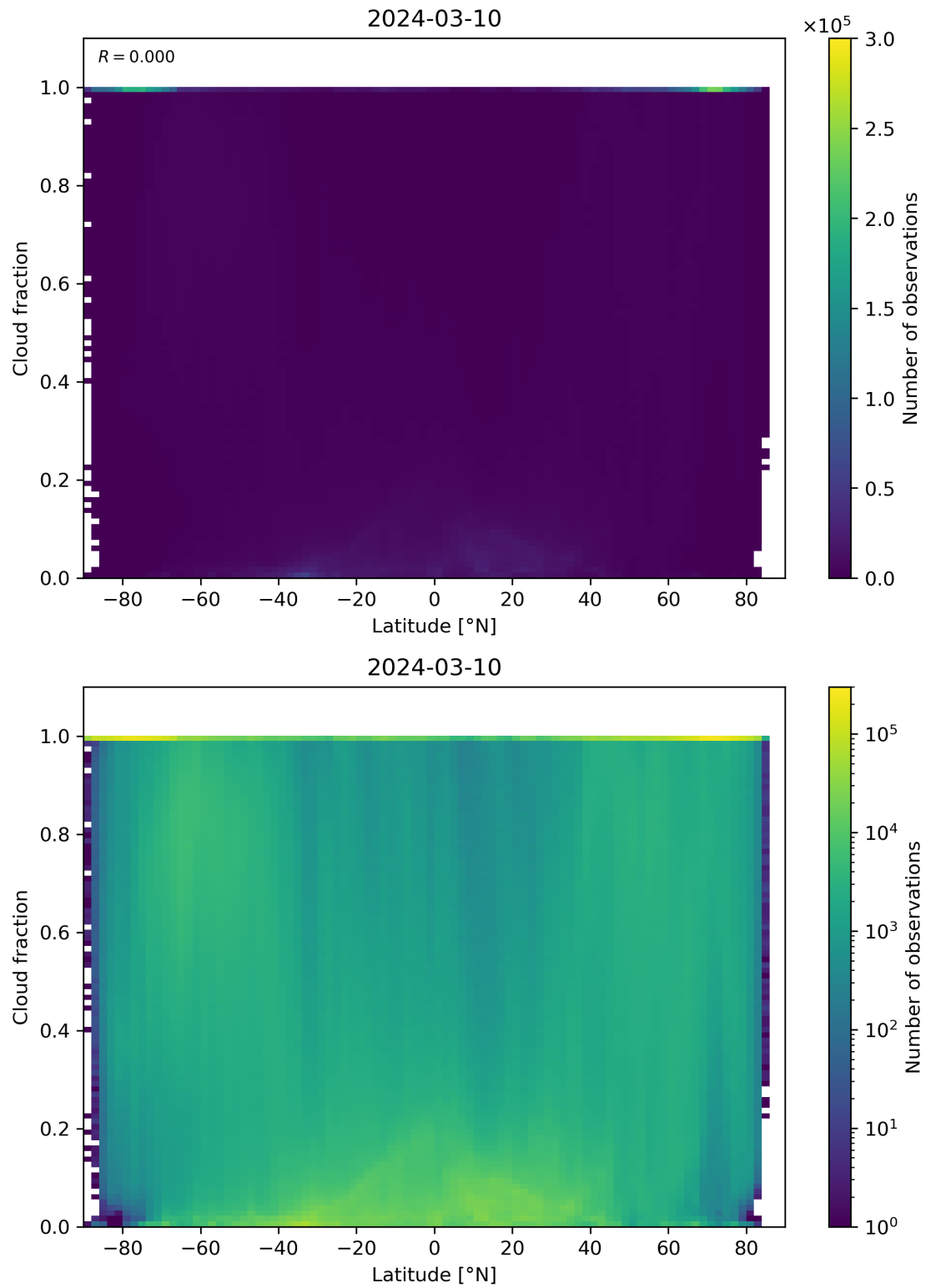
Figure 90: Scatter density plot of “Latitude” against “Cloud fraction” for 2024-03-09 to 2024-03-11.
