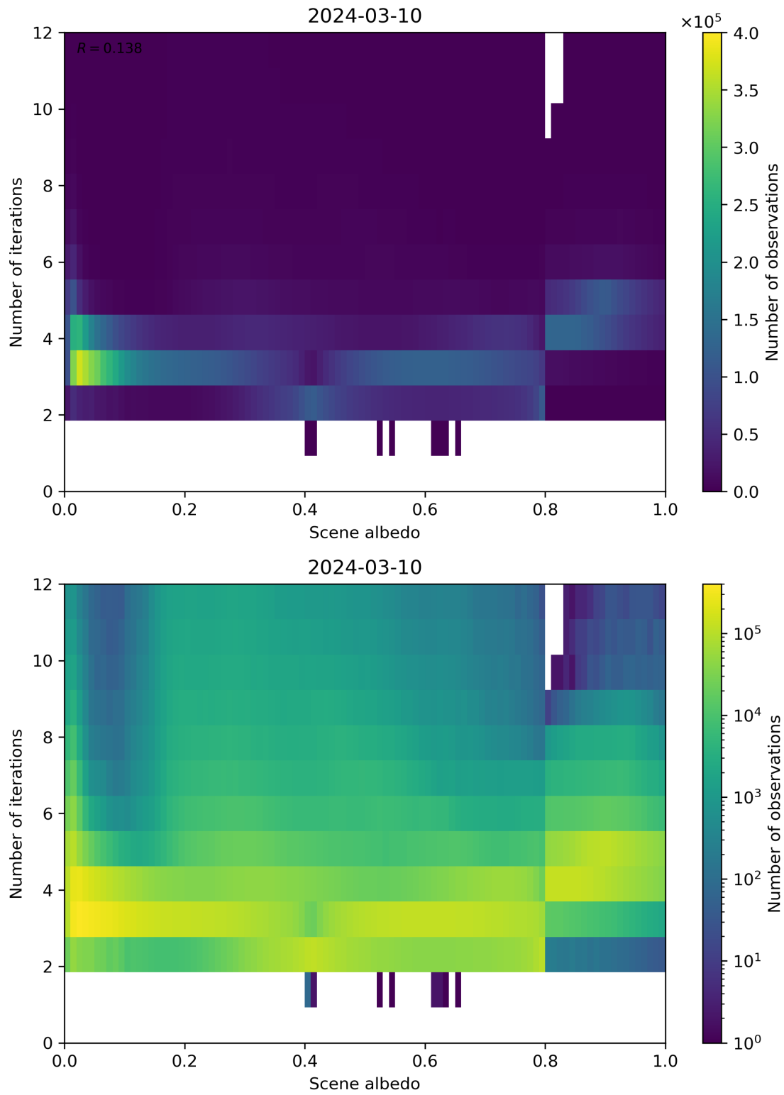
Figure 105: Scatter density plot of “Scene albedo” against “Number of iterations” for 2024-03-09 to 2024-03-11.
