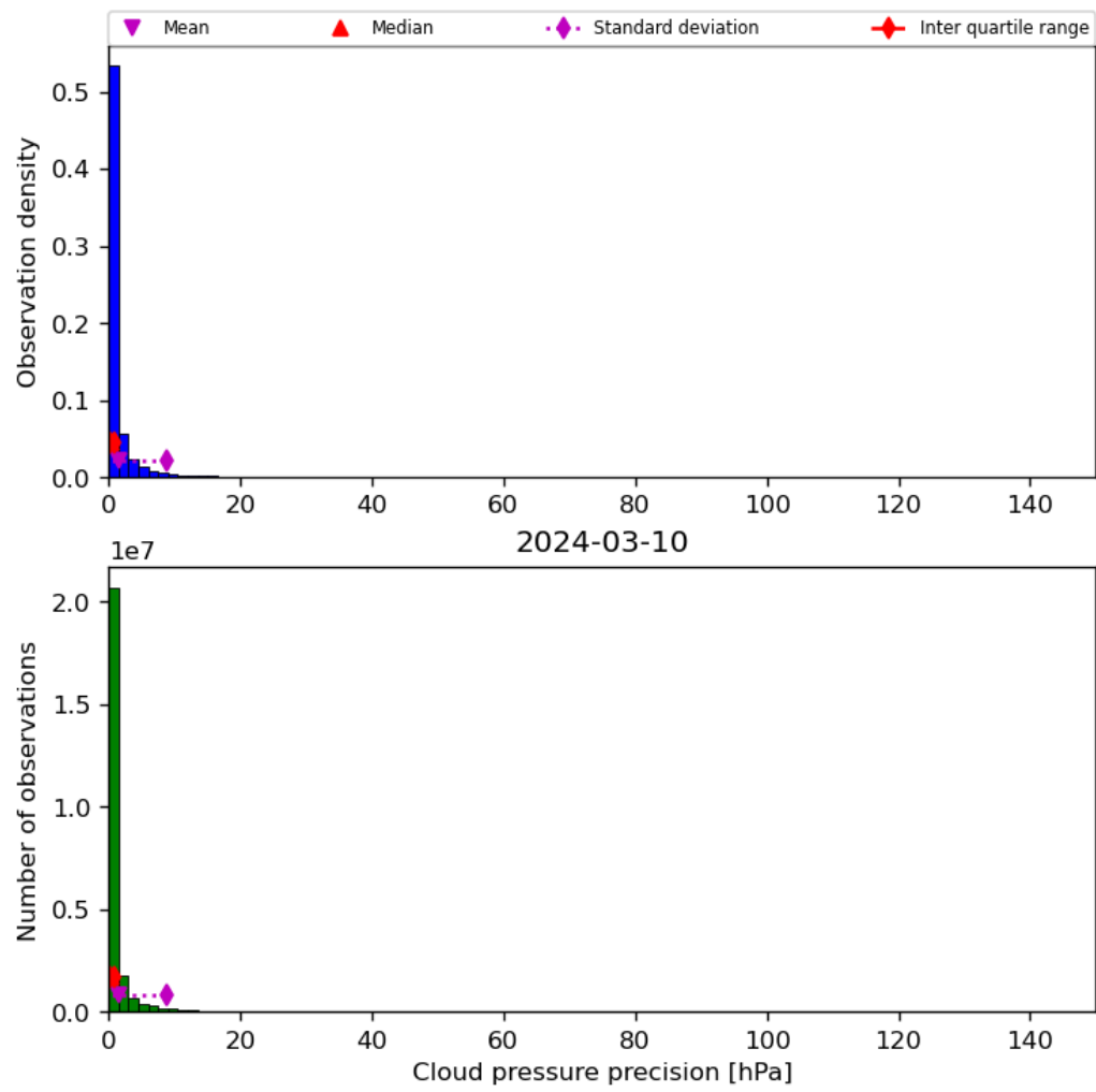
Figure 31: Histogram of “Cloud pressure precision” for 2024-03-09 to 2024-03-11
