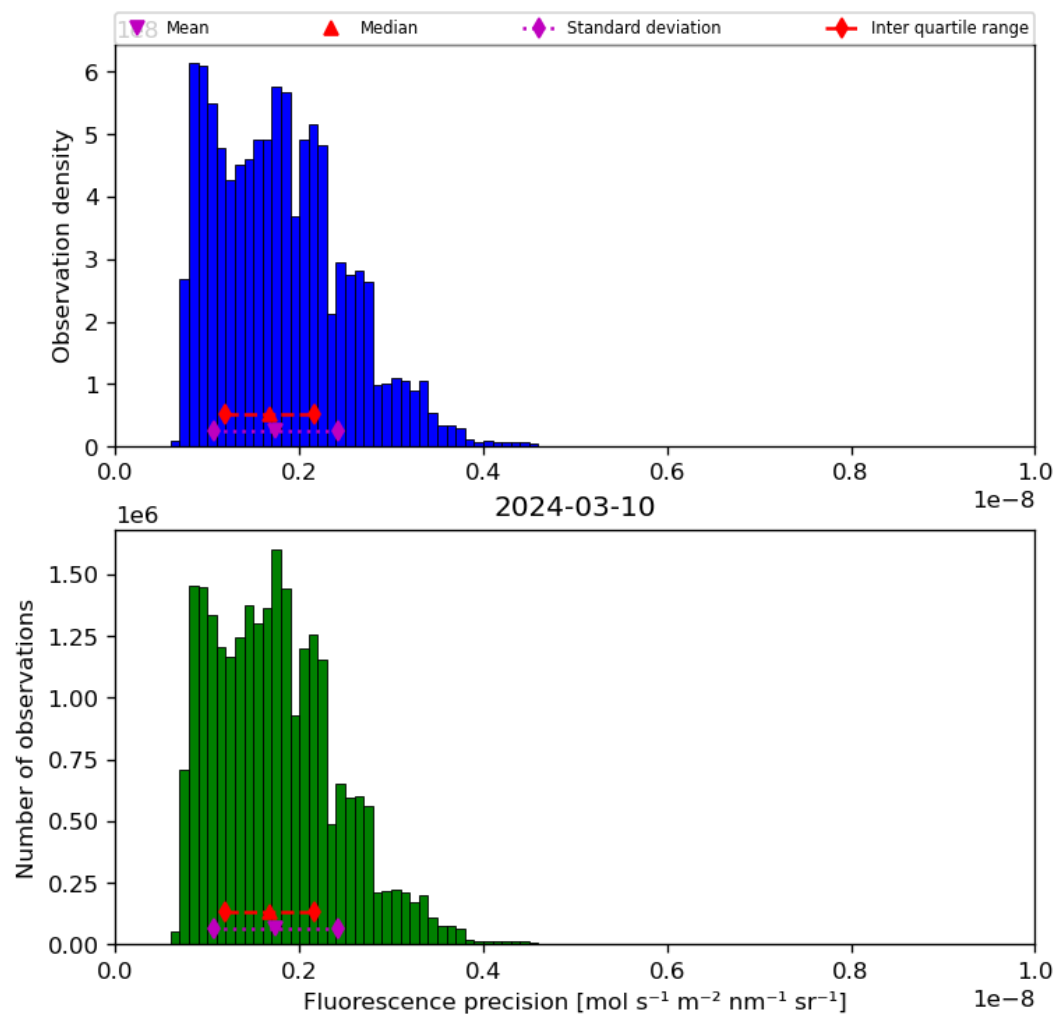
Figure 41: Histogram of “Fluorescence precision” for 2024-03-09 to 2024-03-11
