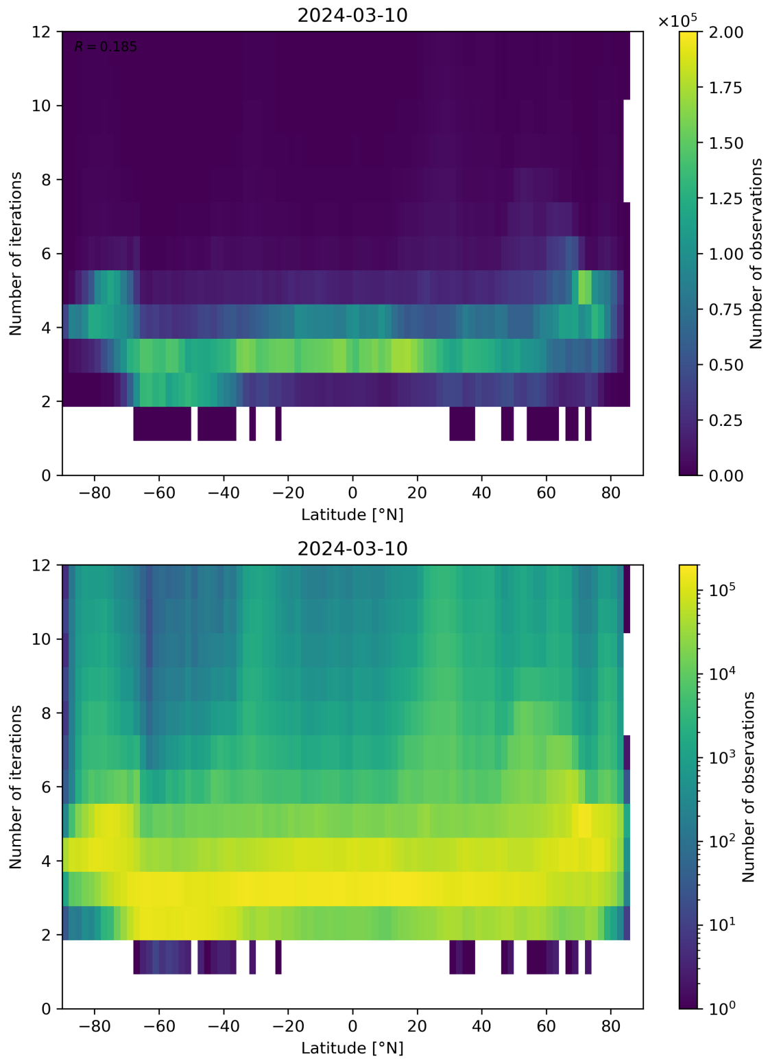
Figure 93: Scatter density plot of “Latitude” against “Number of iterations” for 2024-03-09 to 2024-03-11.
