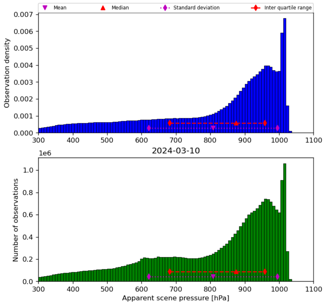
Figure 36: Histogram of “Apparent scene pressure” for 2024-03-09 to 2024-03-11
