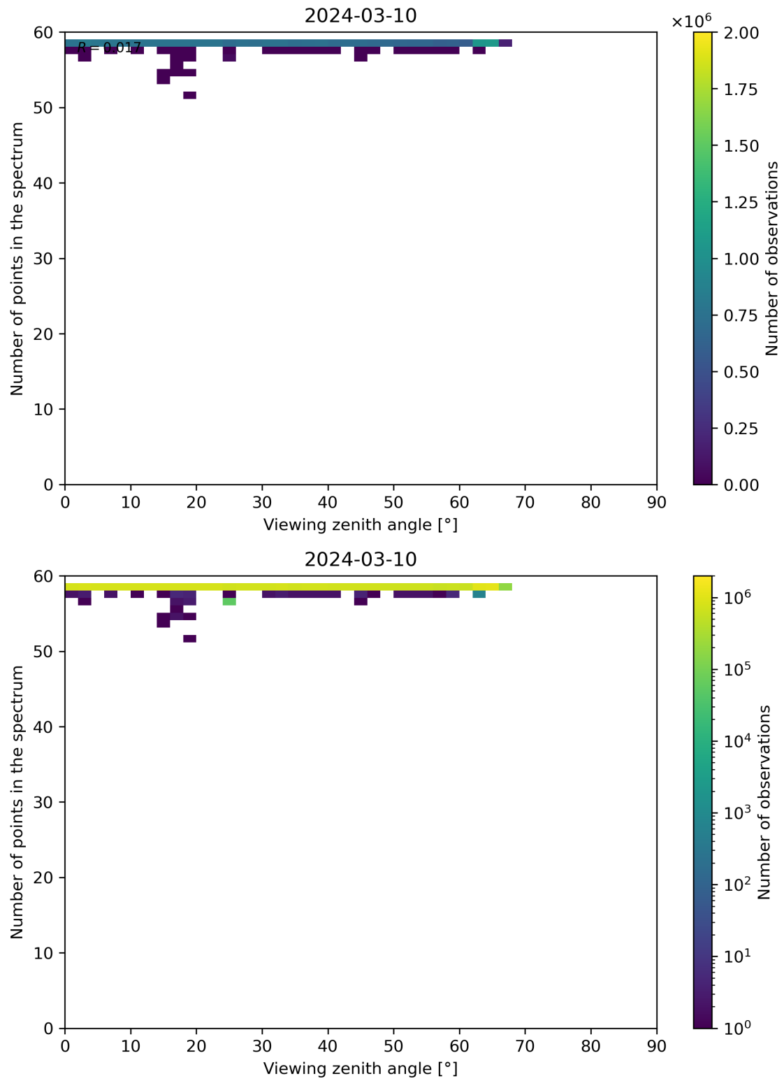
Figure 125: Scatter density plot of “Viewing zenith angle” against “Number of points in the spectrum” for 2024-03-09 to 2024-03-11.
