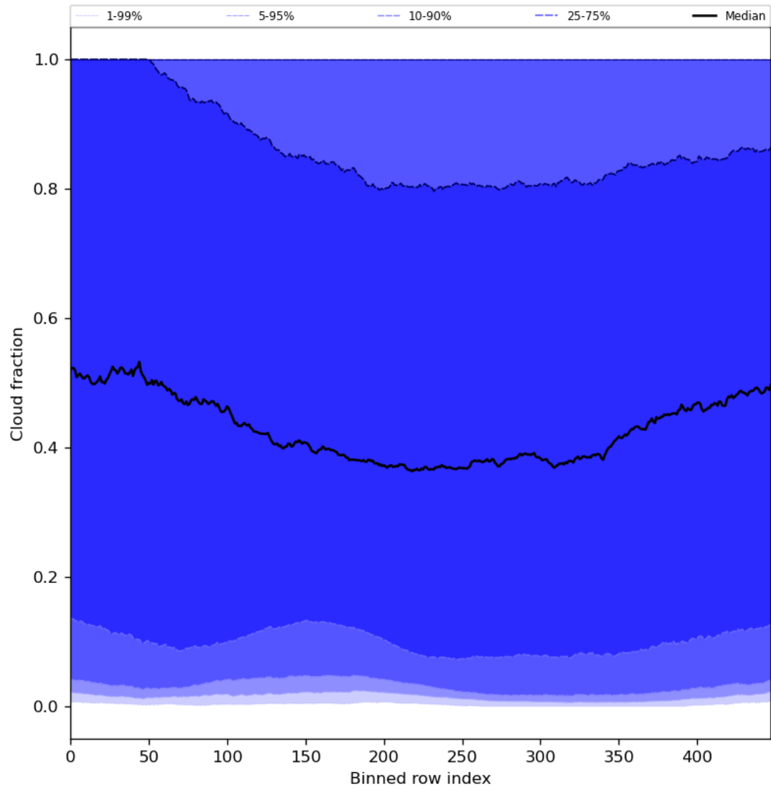
Figure 49: Along track statistics of “Cloud fraction” for 2024-03-09 to 2024-03-11
