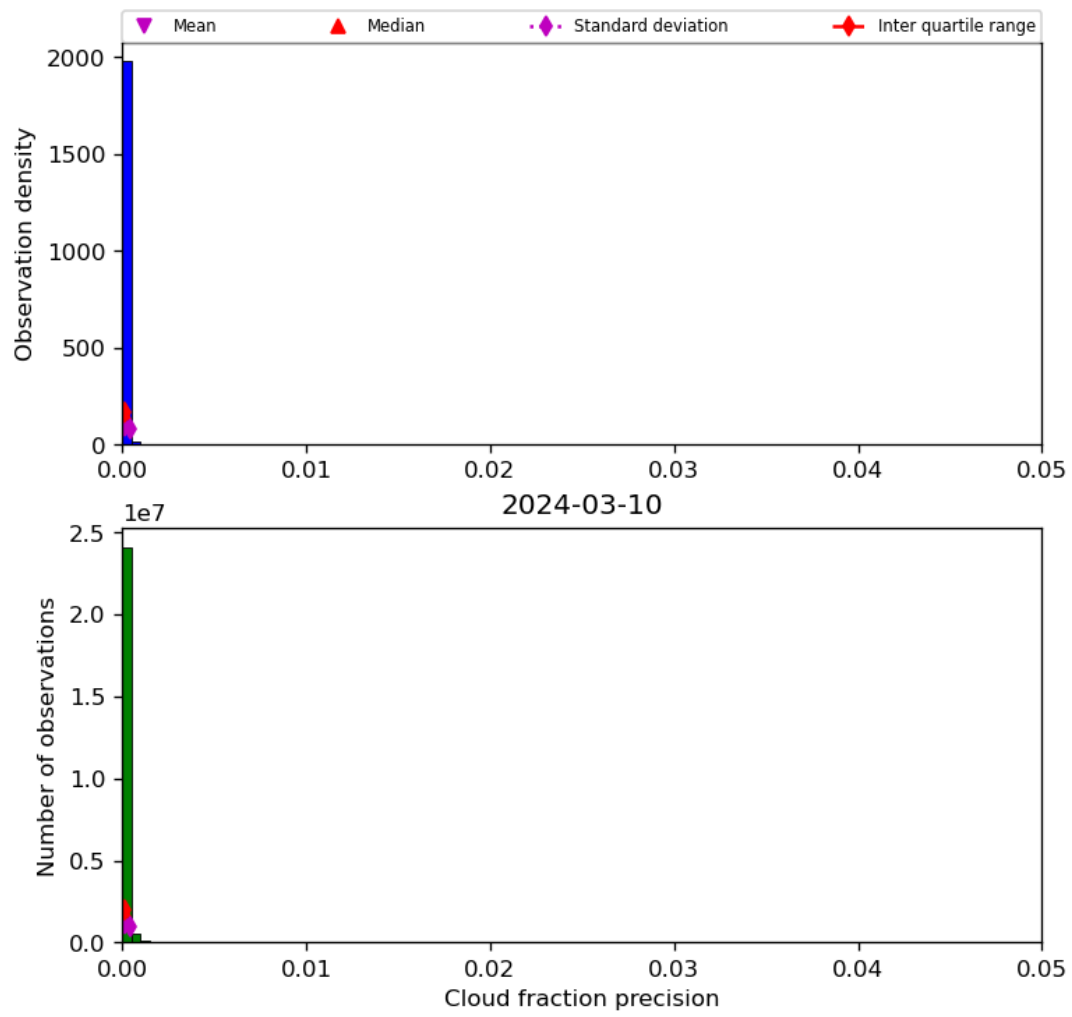
Figure 33: Histogram of “Cloud fraction precision” for 2024-03-09 to 2024-03-11
