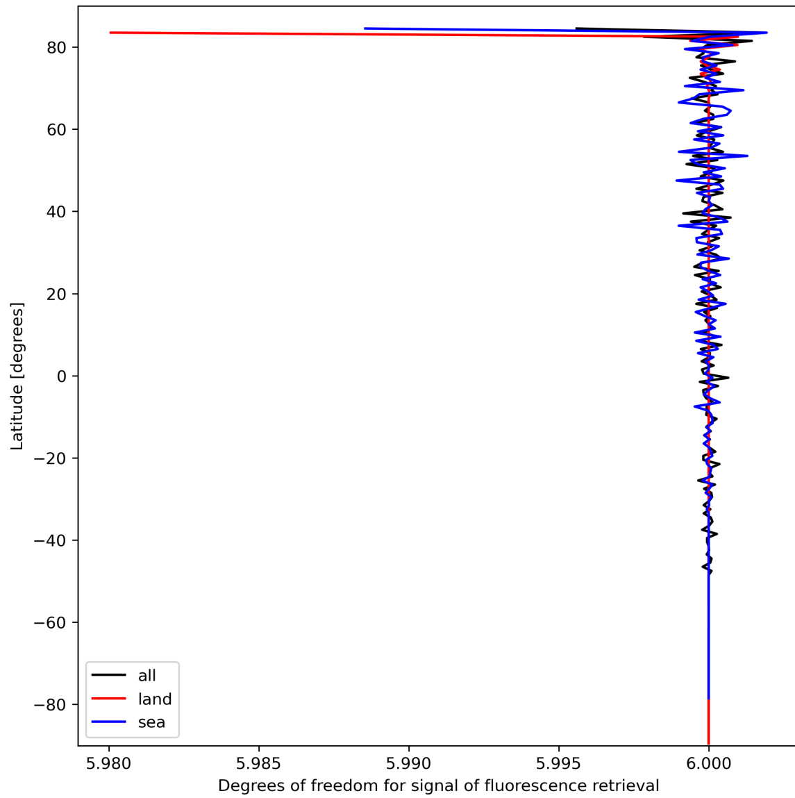
Figure 26: Zonal average of “Degrees of freedom for signal of fluorescence retrieval” for 2024-03-09 to 2024-03-11.
