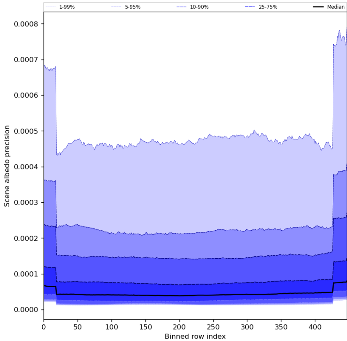
Figure 52: Along track statistics of “Scene albedo precision” for 2024-03-09 to 2024-03-11
