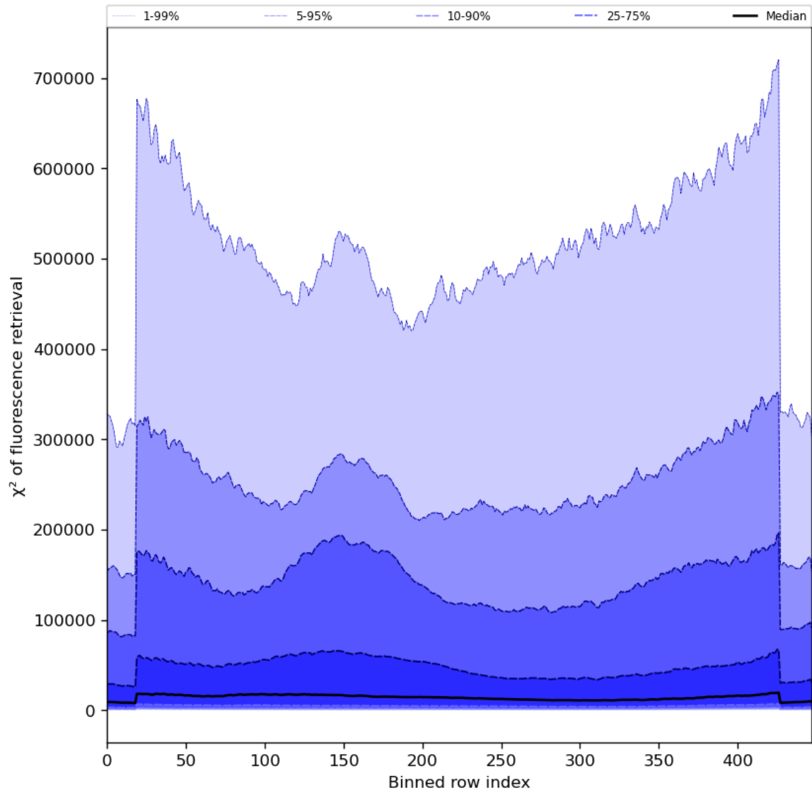
Figure 59: Along track statistics of “ \chi^2 of fluorescence retrieval” for 2024-03-09 to 2024-03-11
