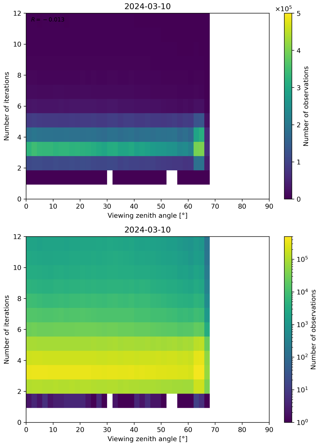
Figure 124: Scatter density plot of “Viewing zenith angle” against “Number of iterations” for 2024-03-09 to 2024-03-11.
