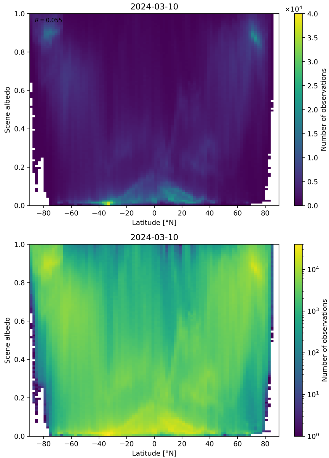
Figure 95: Scatter density plot of “Latitude” against “Scene albedo” for 2024-03-09 to 2024-03-11.
