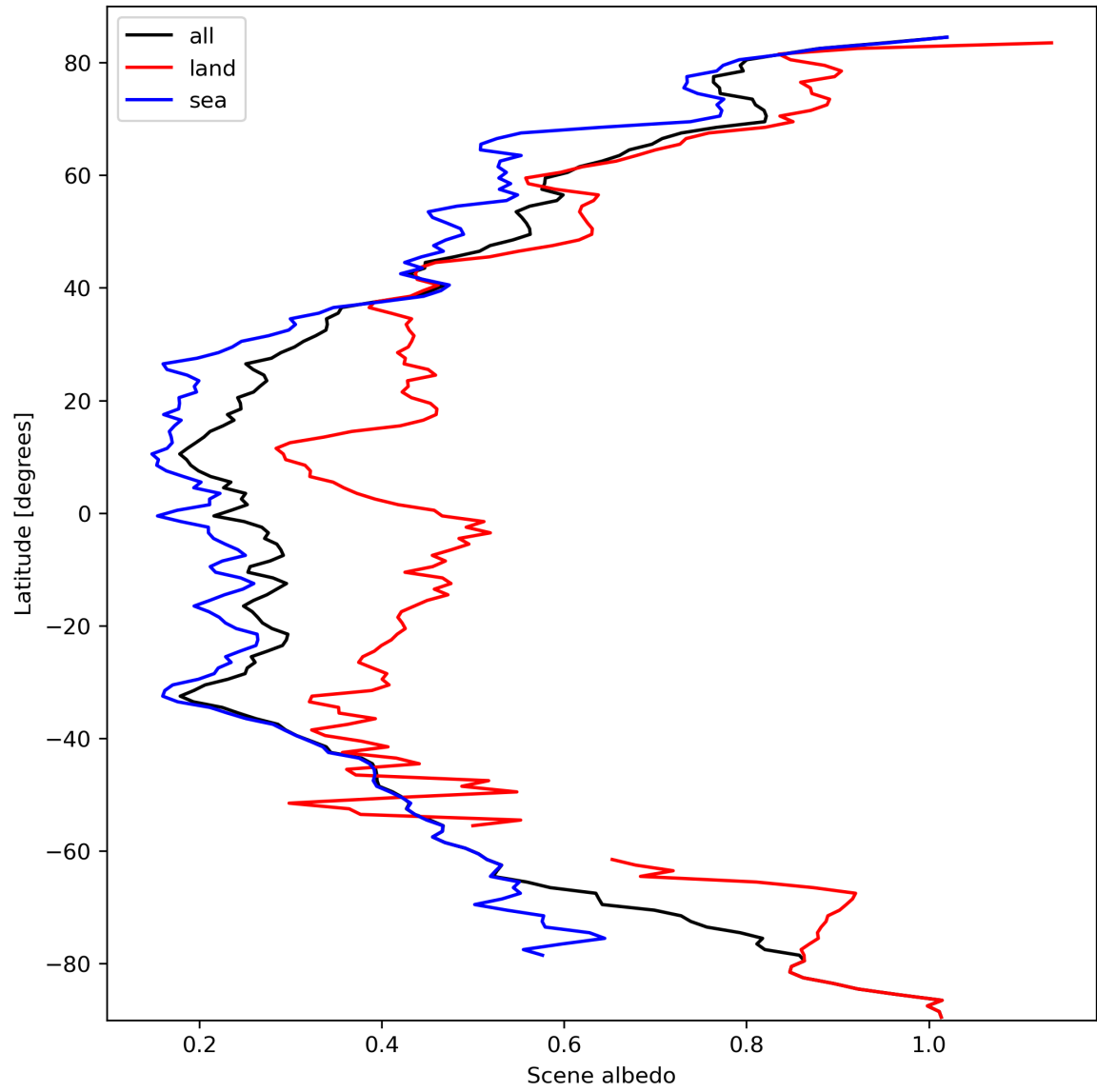
Figure 17: Zonal average of “Scene albedo” for 2024-03-09 to 2024-03-11.
