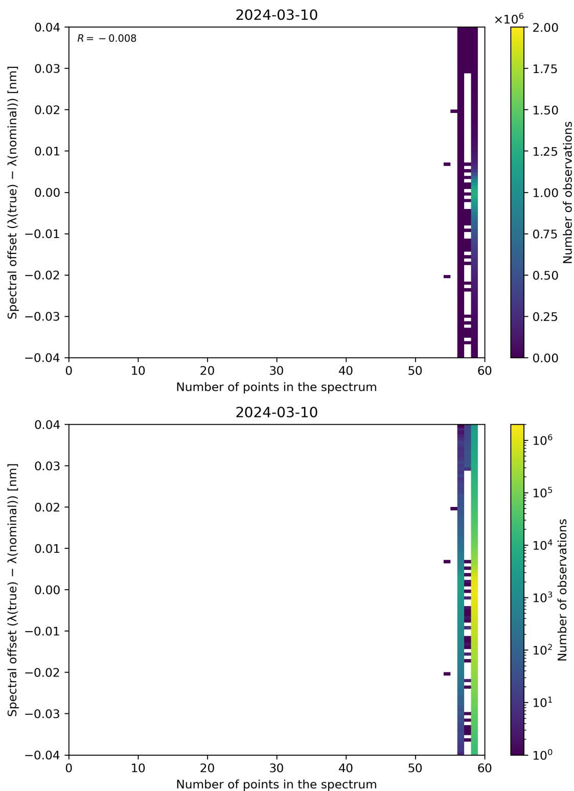
Figure 101: Scatter density plot of “Number of points in the spectrum” against “Spectral offset ( \lambda(\text{true}) - \lambda(\text{nominal}) )” for 2024-03-09 to 2024-03-11.
