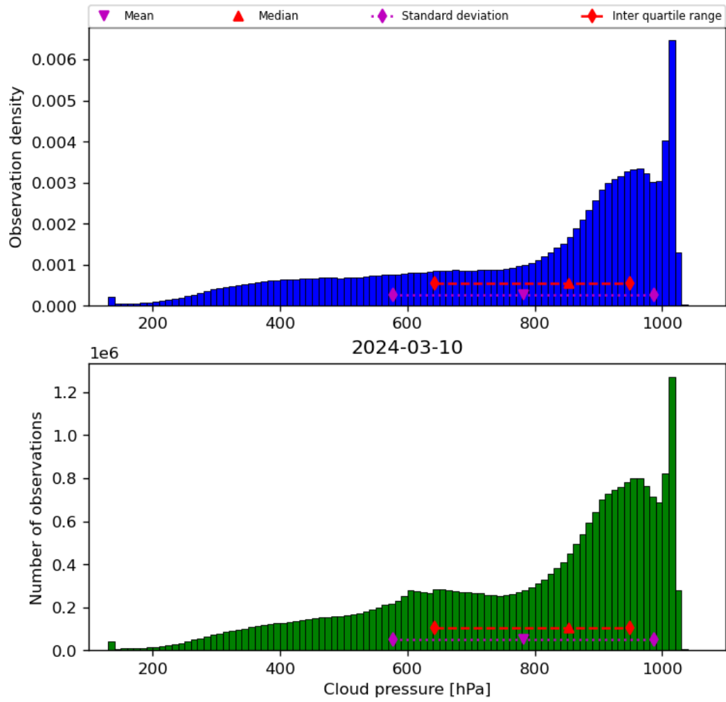
Figure 30: Histogram of “Cloud pressure” for 2024-03-09 to 2024-03-11
