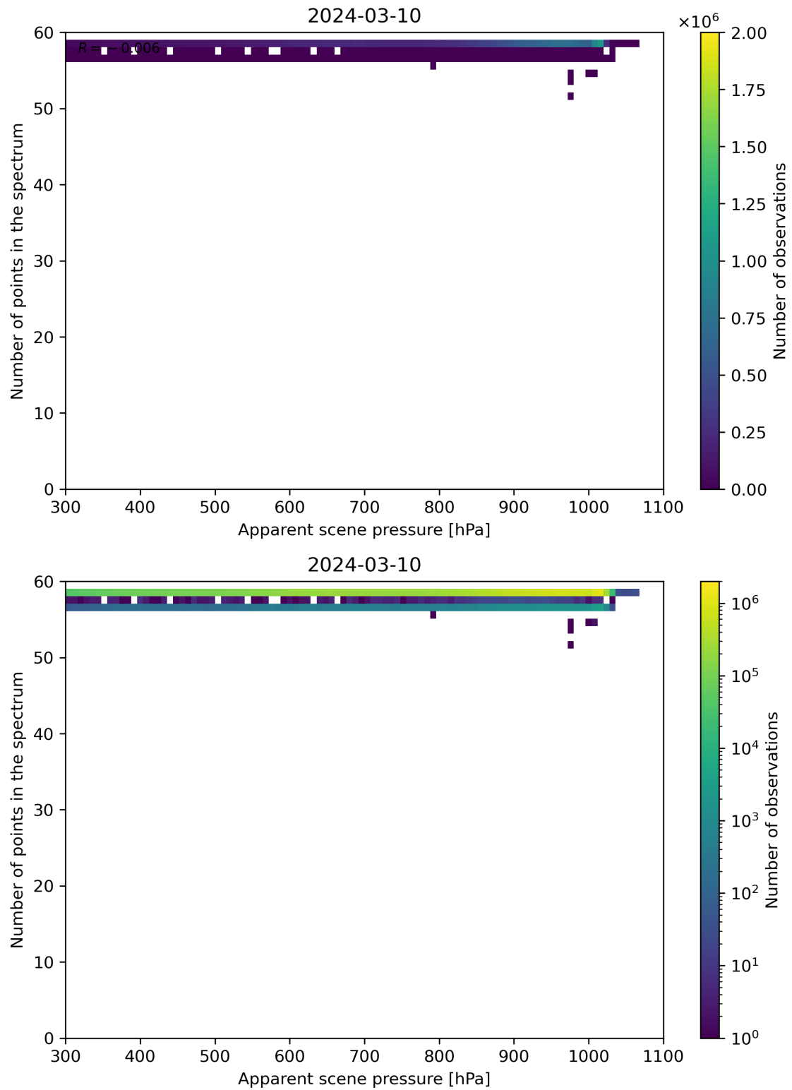
Figure 66: Scatter density plot of “Apparent scene pressure” against “Number of points in the spectrum” for 2024-03-09 to 2024-03-11.
