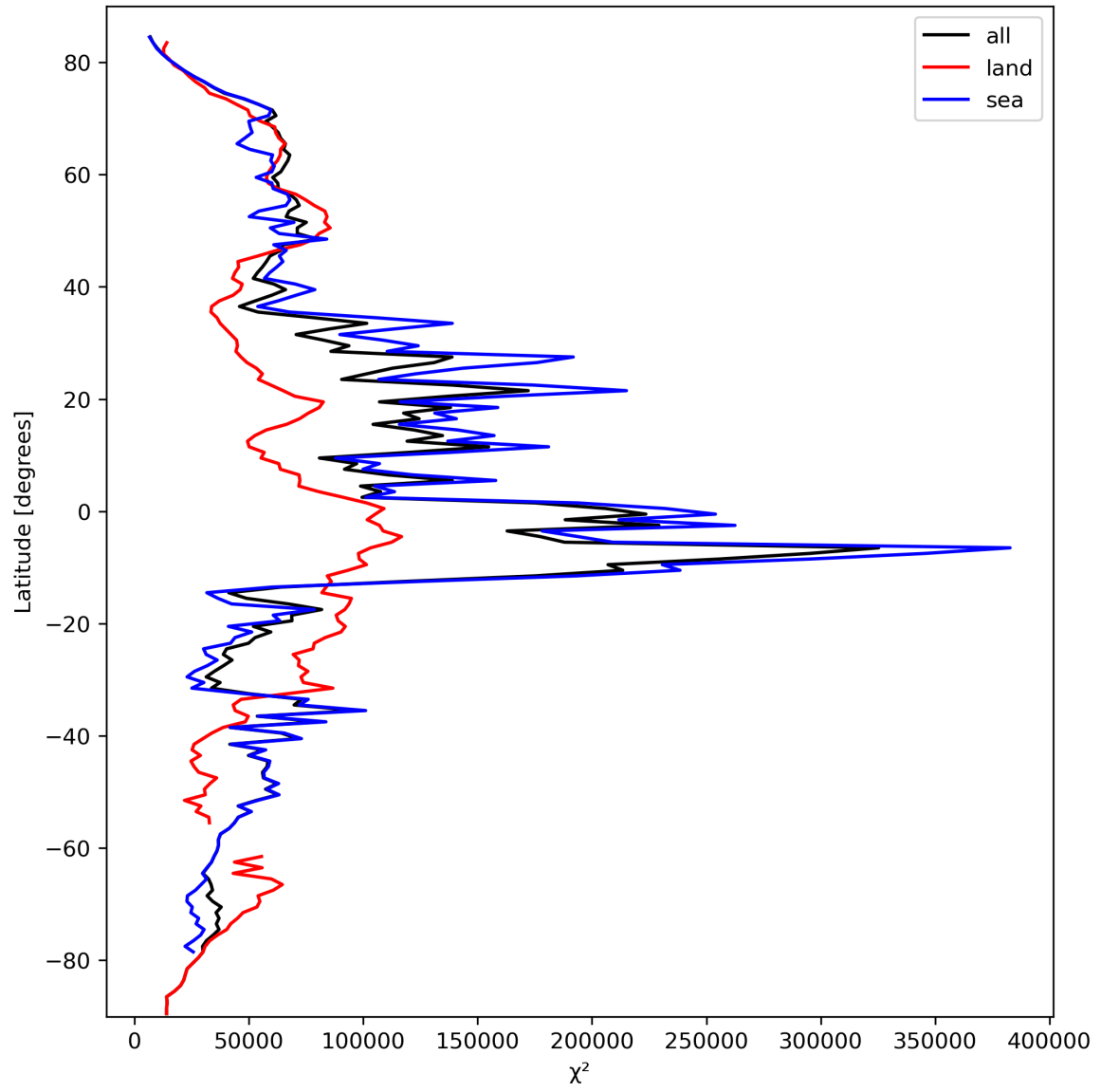
Figure 21: Zonal average of “ \chi^2 ” for 2024-03-09 to 2024-03-11.
