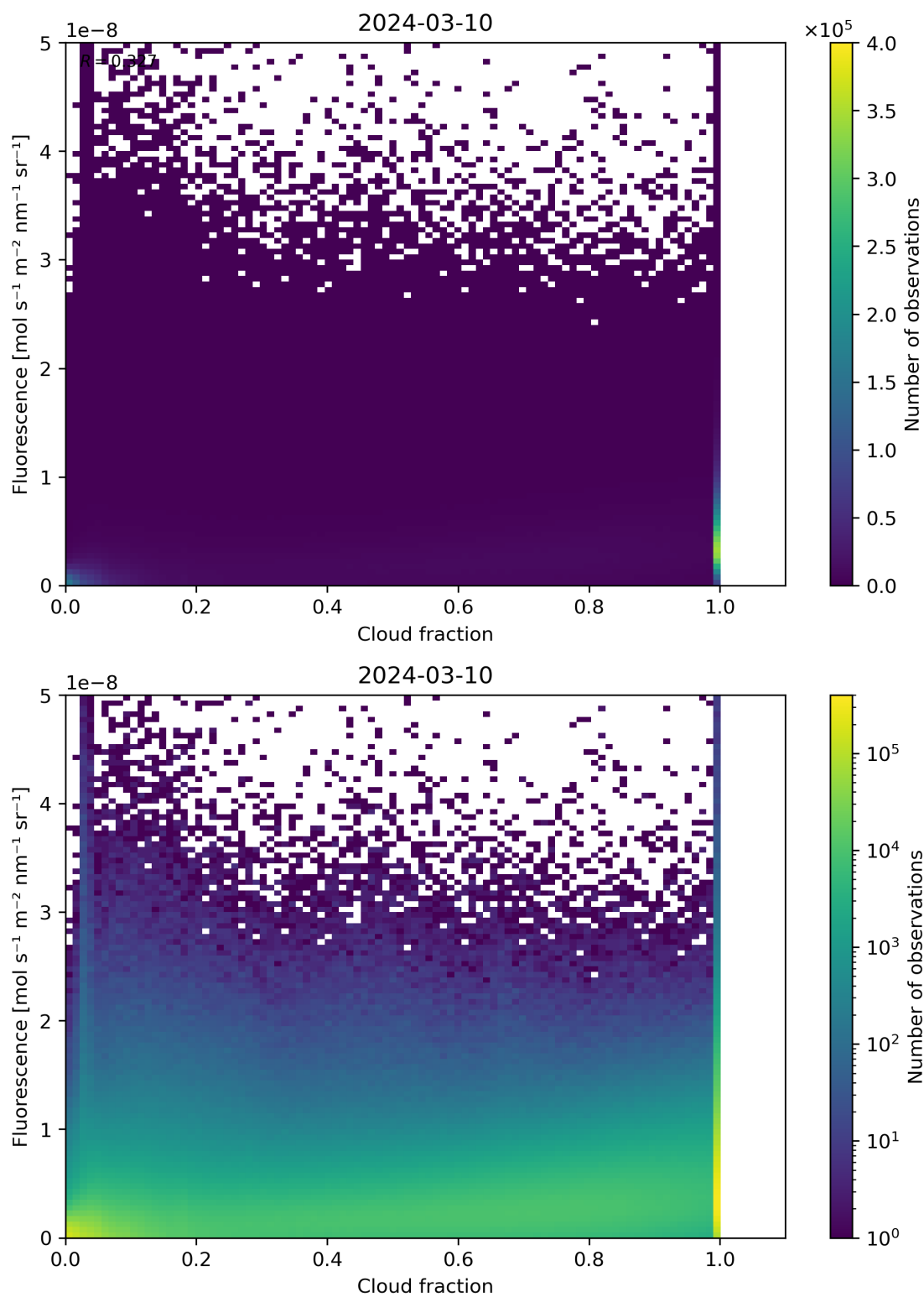
Figure 72: Scatter density plot of “Cloud fraction” against “Fluorescence” for 2024-03-09 to 2024-03-11.
