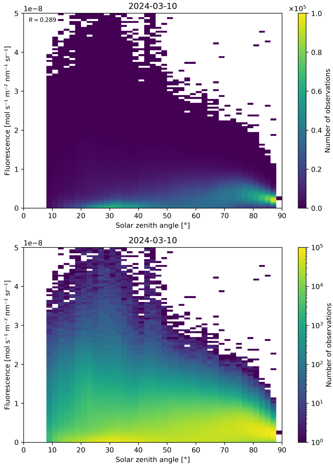
Figure 112: Scatter density plot of “Solar zenith angle” against “Fluorescence” for 2024-03-09 to 2024-03-11.
