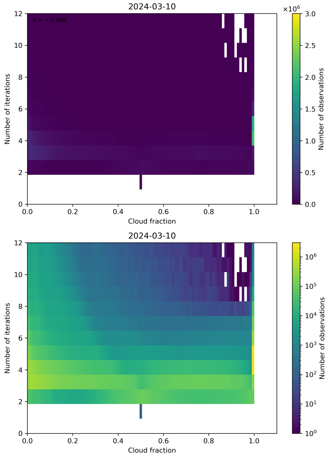
Figure 73: Scatter density plot of “Cloud fraction” against “Number of iterations” for 2024-03-09 to 2024-03-11.
