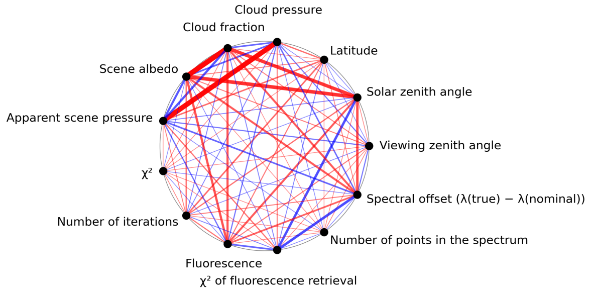
Figure 1: Map of correlation graph for 2024-03-09 to 2024-03-11.
