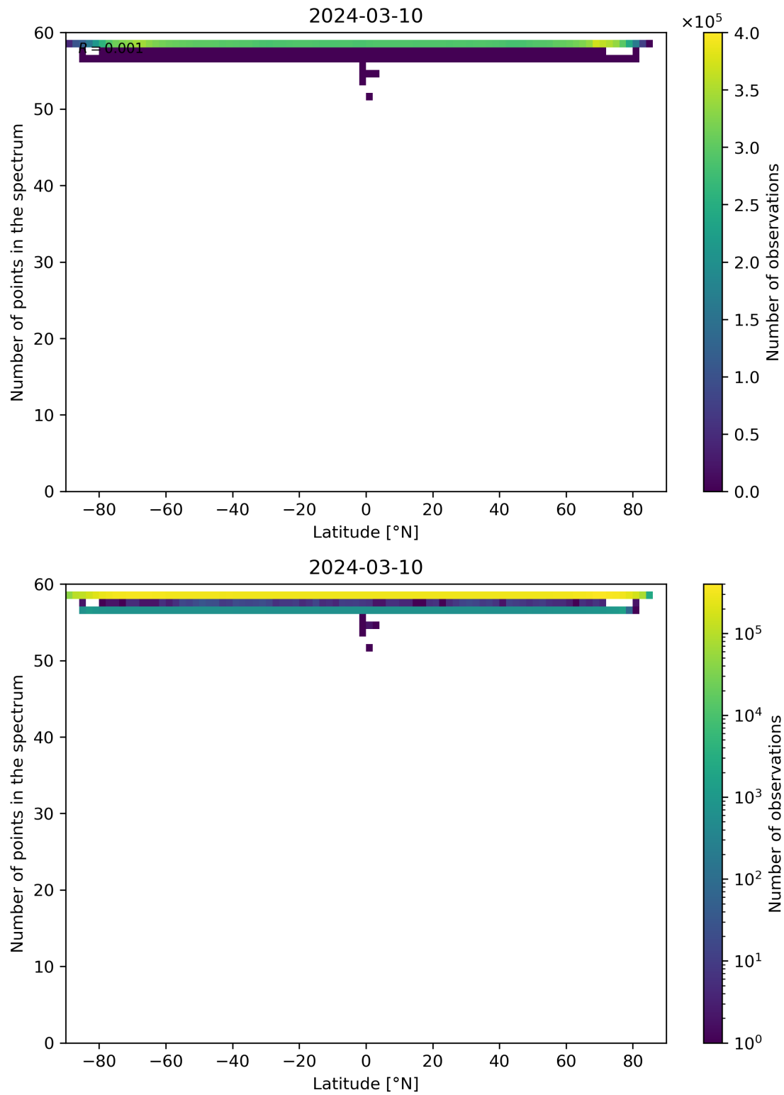
Figure 94: Scatter density plot of “Latitude” against “Number of points in the spectrum” for 2024-03-09 to 2024-03-11.
