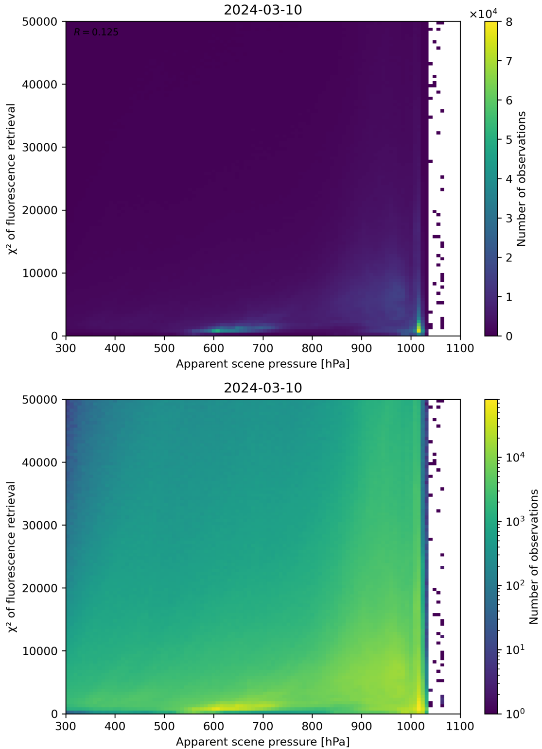
Figure 63: Scatter density plot of “Apparent scene pressure” against “ \chi^2 of fluorescence retrieval” for 2024-03-09 to 2024-03-11.
