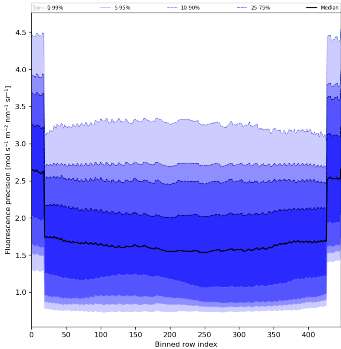
Figure 58: Along track statistics of “Fluorescence precision” for 2024-03-09 to 2024-03-11
