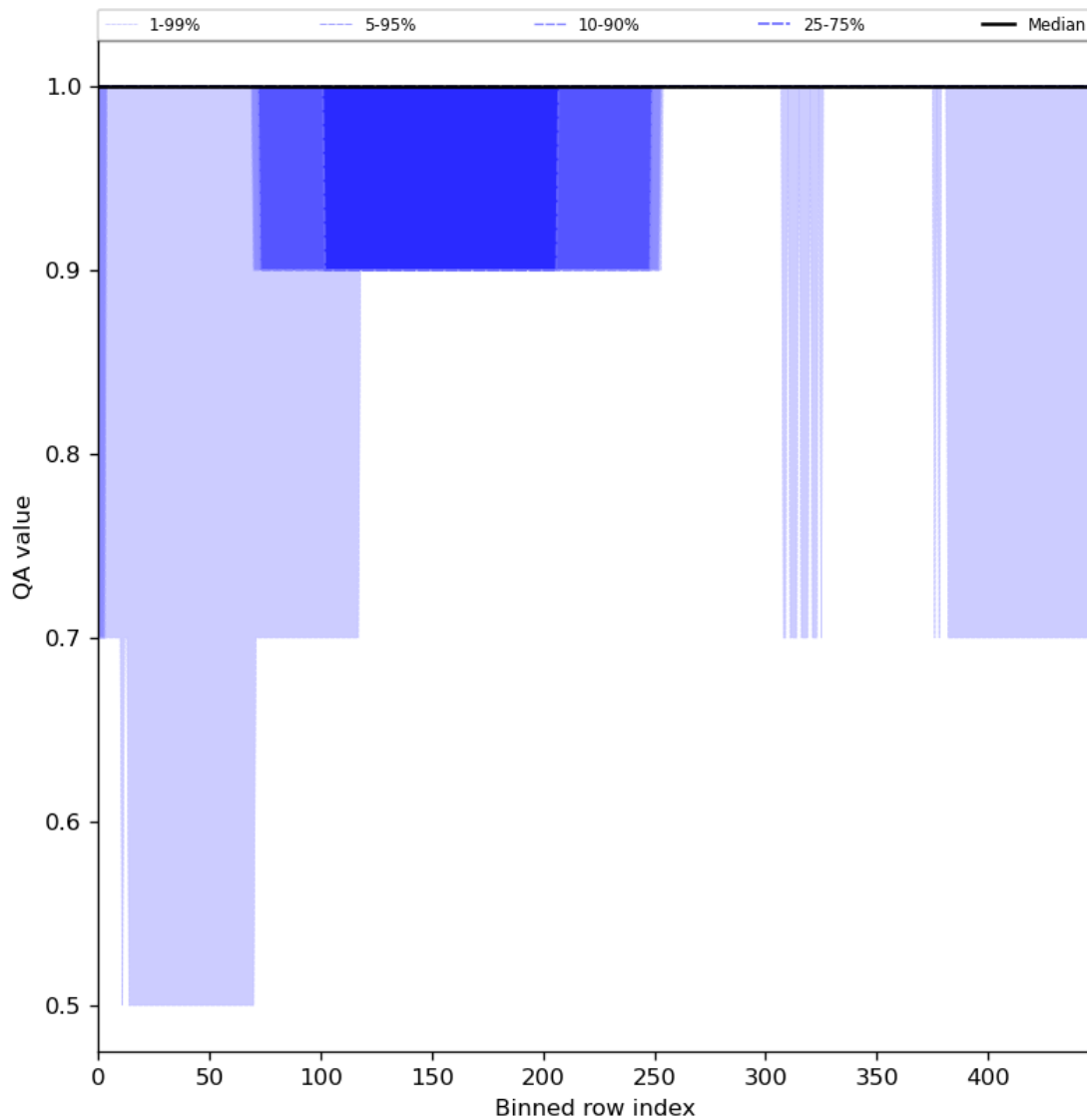
Figure 46: Along track statistics of “QA value” for 2024-03-09 to 2024-03-11
