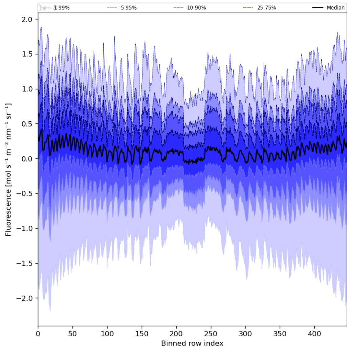
Figure 57: Along track statistics of “Fluorescence” for 2024-03-09 to 2024-03-11
