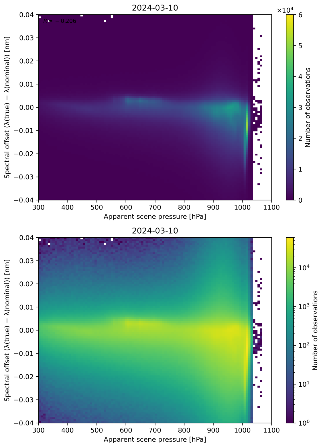
Figure 67: Scatter density plot of “Apparent scene pressure” against “Spectral offset ( \lambda(\text{true}) - \lambda(\text{nominal}) )” for 2024-03-09 to 2024-03-11.
