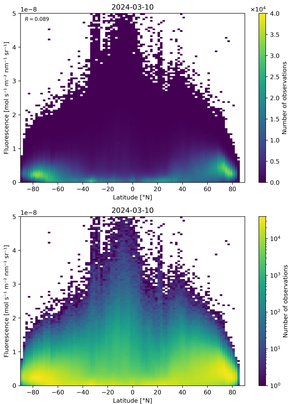
Figure 92: Scatter density plot of “Latitude” against “Fluorescence” for 2024-03-09 to 2024-03-11.
