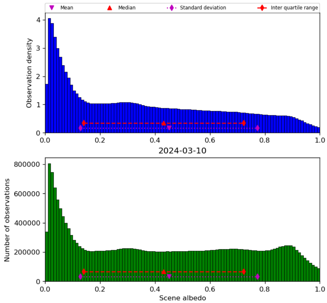
Figure 34: Histogram of “Scene albedo” for 2024-03-09 to 2024-03-11
