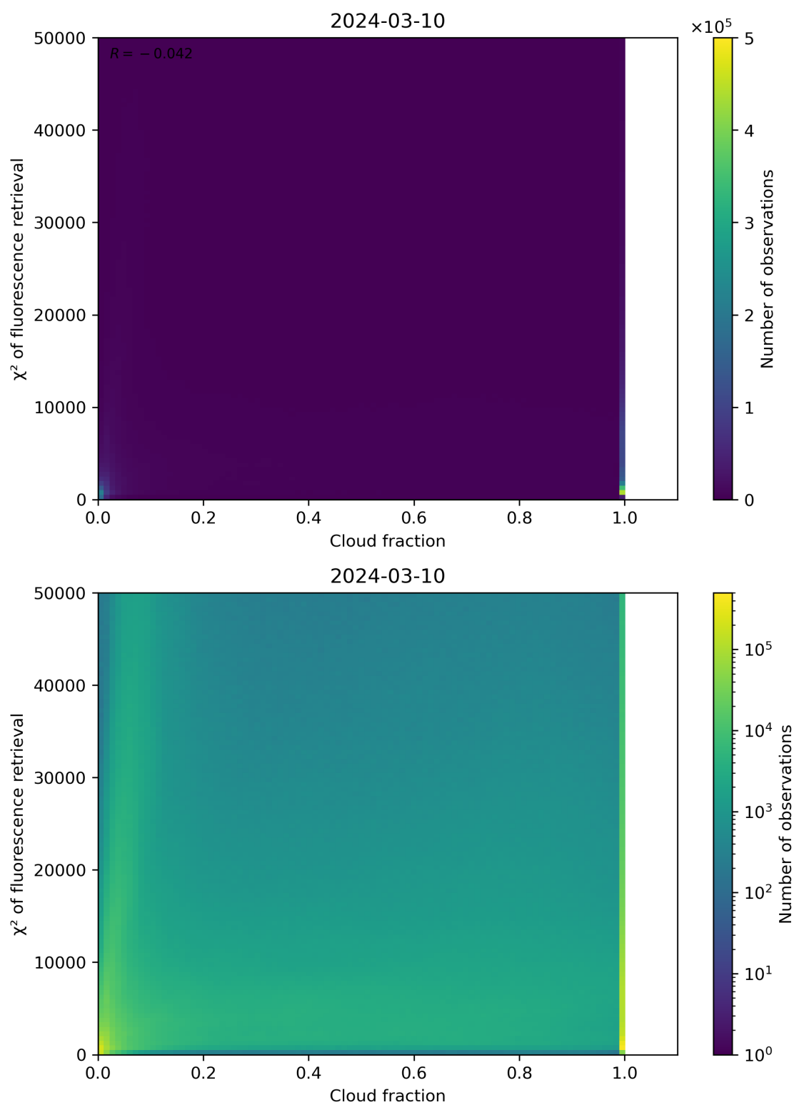
Figure 71: Scatter density plot of “Cloud fraction” against “ \chi^2 of fluorescence retrieval” for 2024-03-09 to 2024-03-11.
