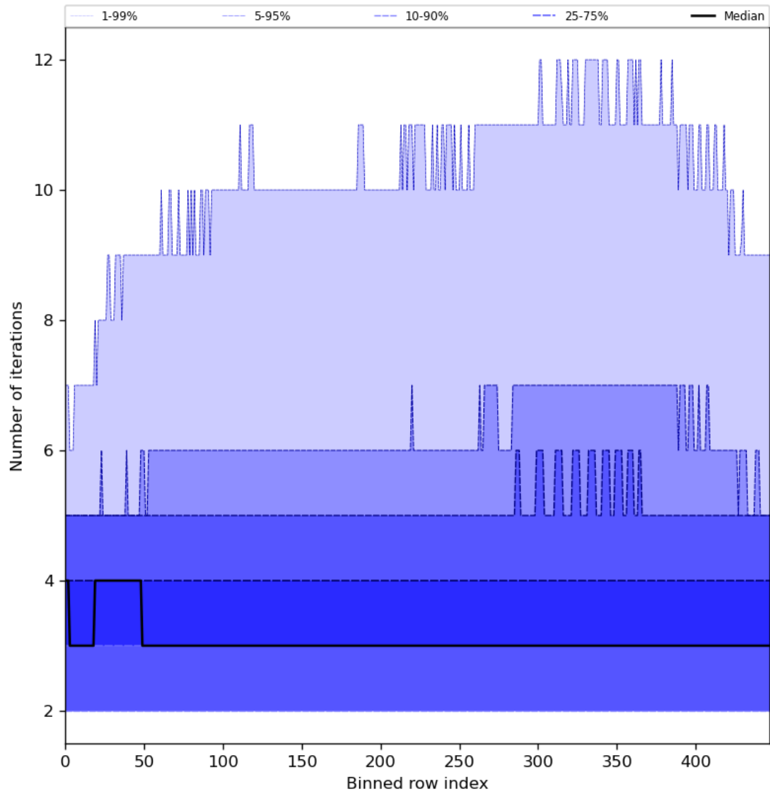
Figure 56: Along track statistics of “Number of iterations” for 2024-03-09 to 2024-03-11
