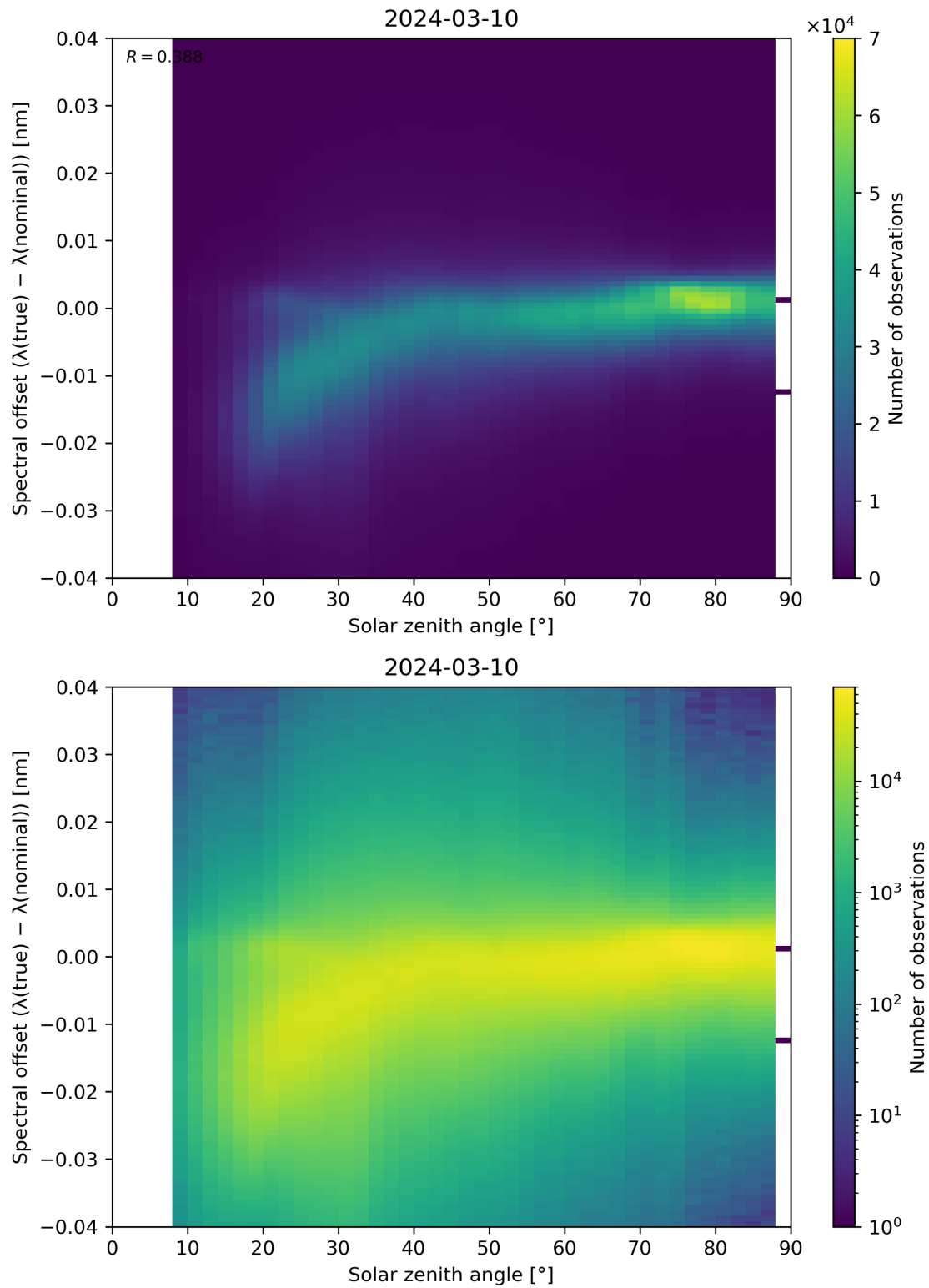
Figure 117: Scatter density plot of “Solar zenith angle” against “Spectral offset ( \lambda(\text{true}) - \lambda(\text{nominal}) )” for 2024-03-09 to 2024-03-11.
