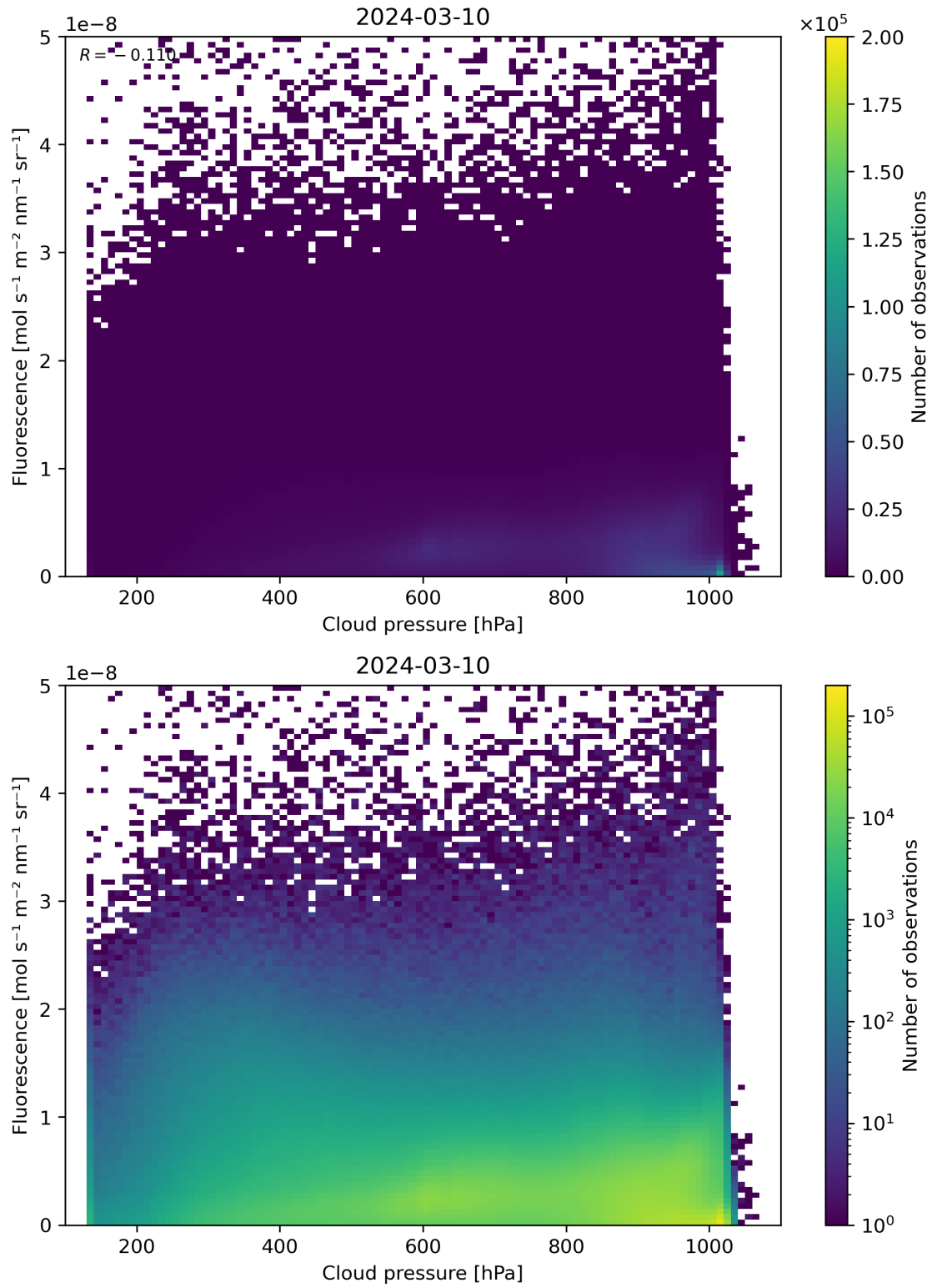
Figure 80: Scatter density plot of “Cloud pressure” against “Fluorescence” for 2024-03-09 to 2024-03-11.
