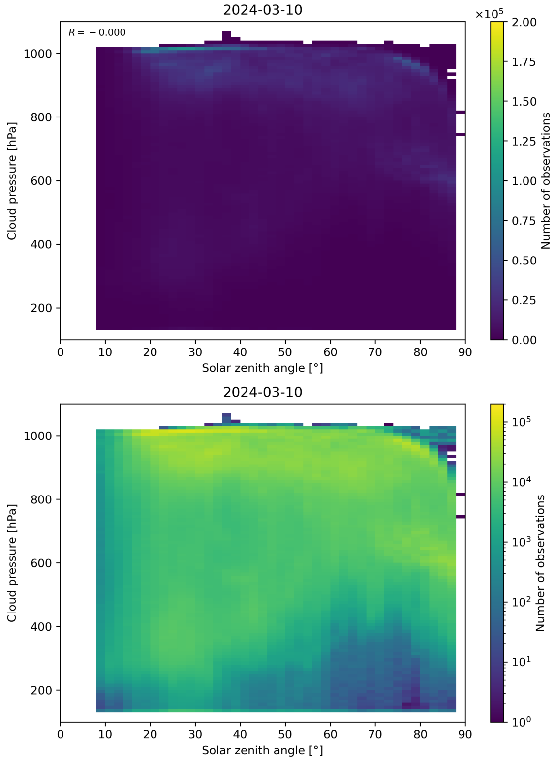
Figure 111: Scatter density plot of “Solar zenith angle” against “Cloud pressure” for 2024-03-09 to 2024-03-11.
