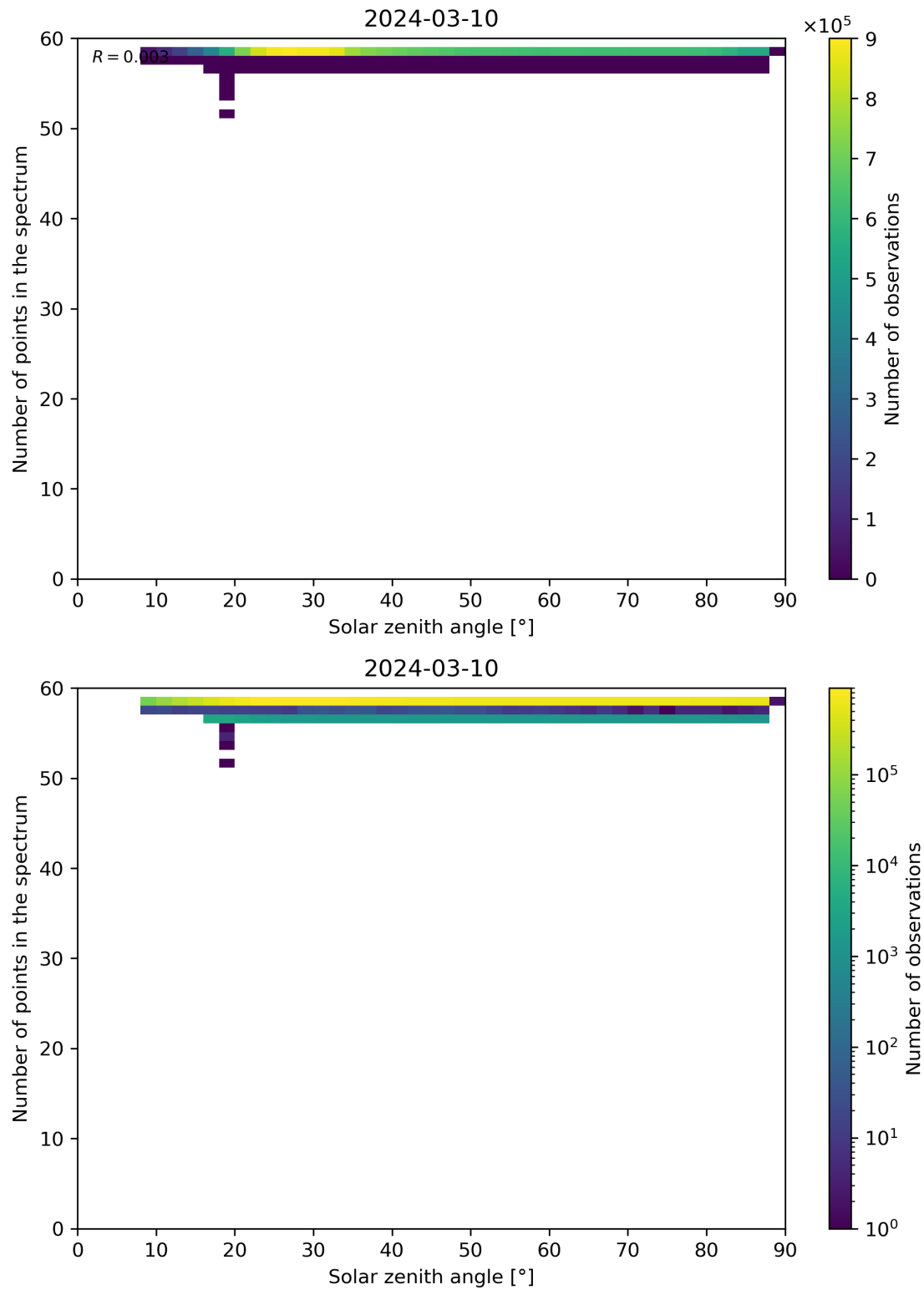
Figure 115: Scatter density plot of “Solar zenith angle” against “Number of points in the spectrum” for 2024-03-09 to 2024-03-11.
