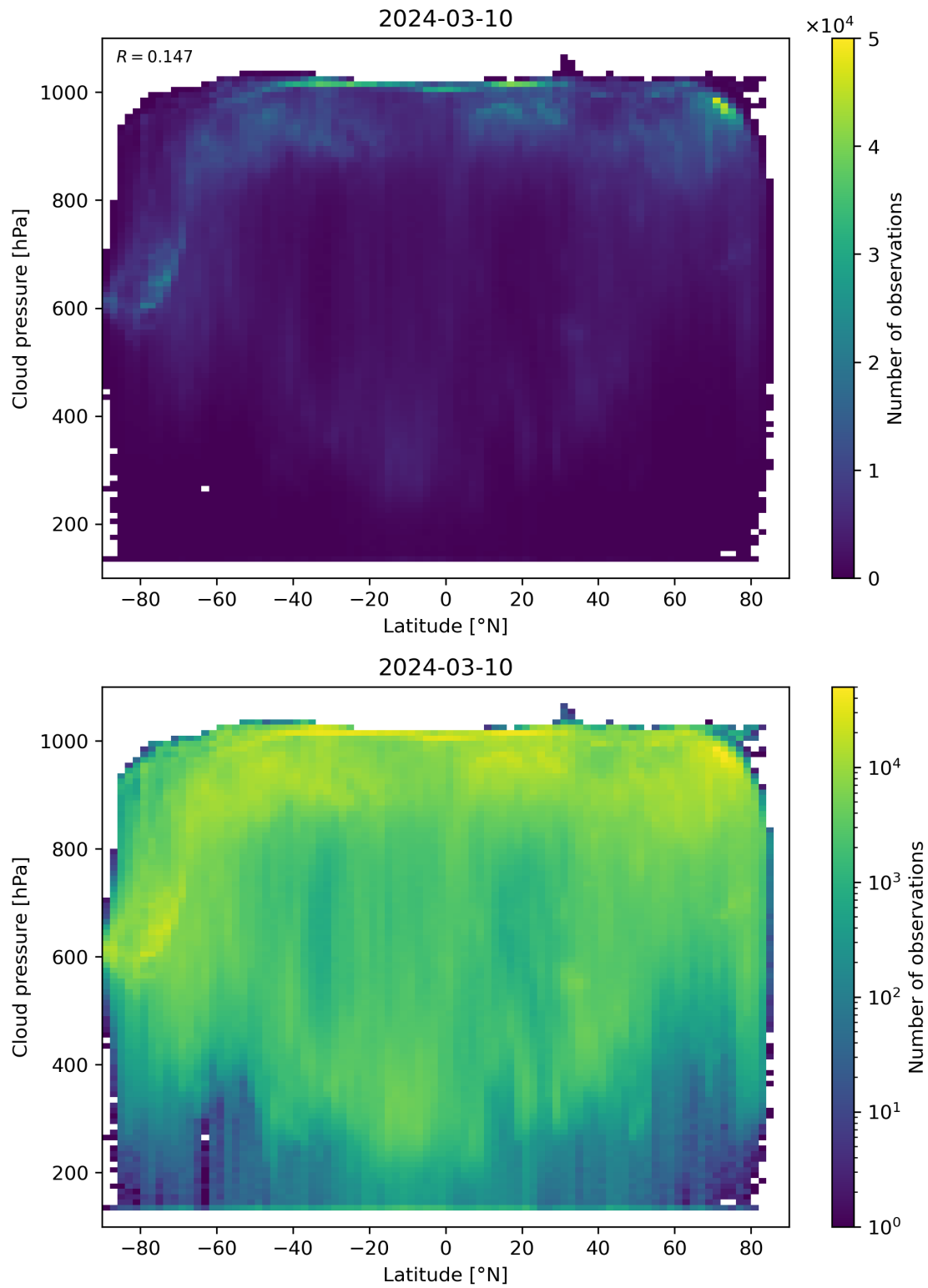
Figure 91: Scatter density plot of “Latitude” against “Cloud pressure” for 2024-03-09 to 2024-03-11.
