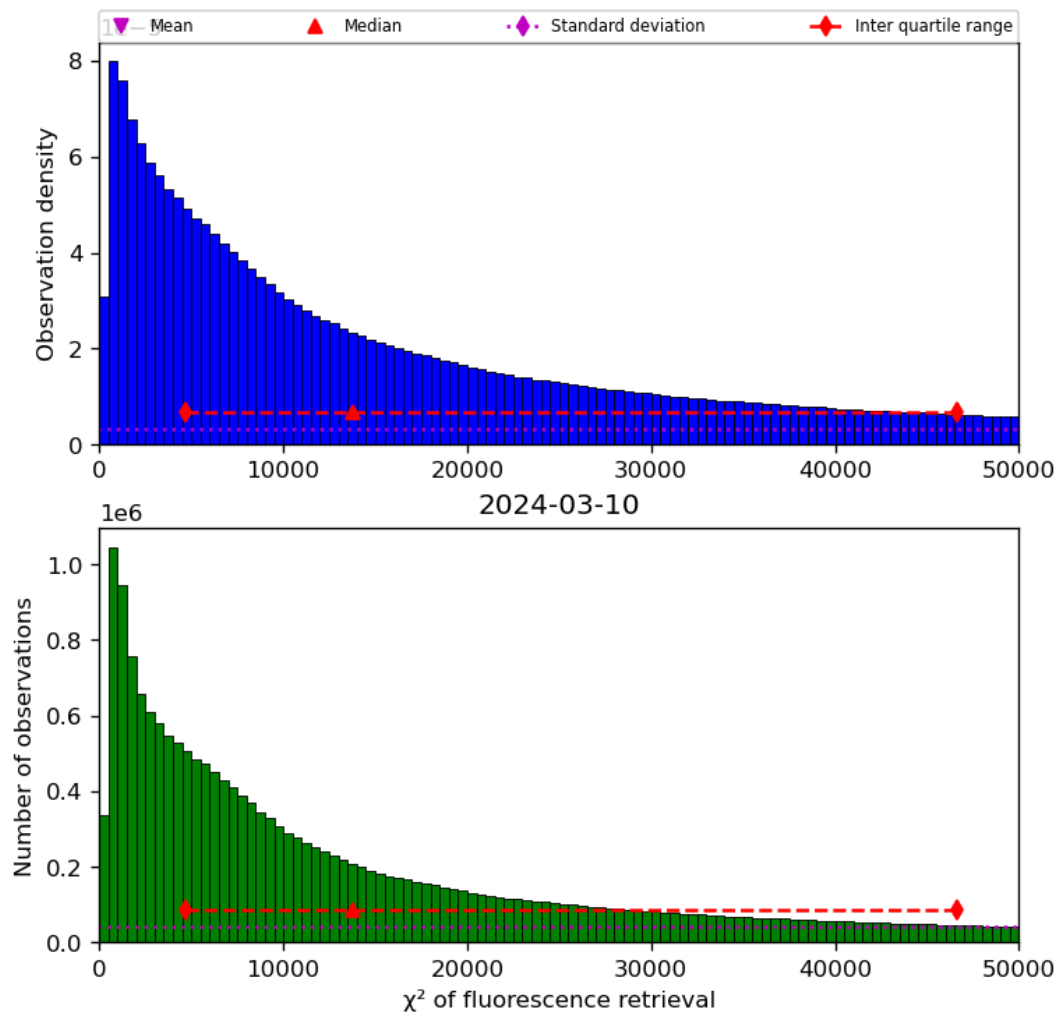
Figure 42: Histogram of “ \chi^2 of fluorescence retrieval” for 2024-03-09 to 2024-03-11
