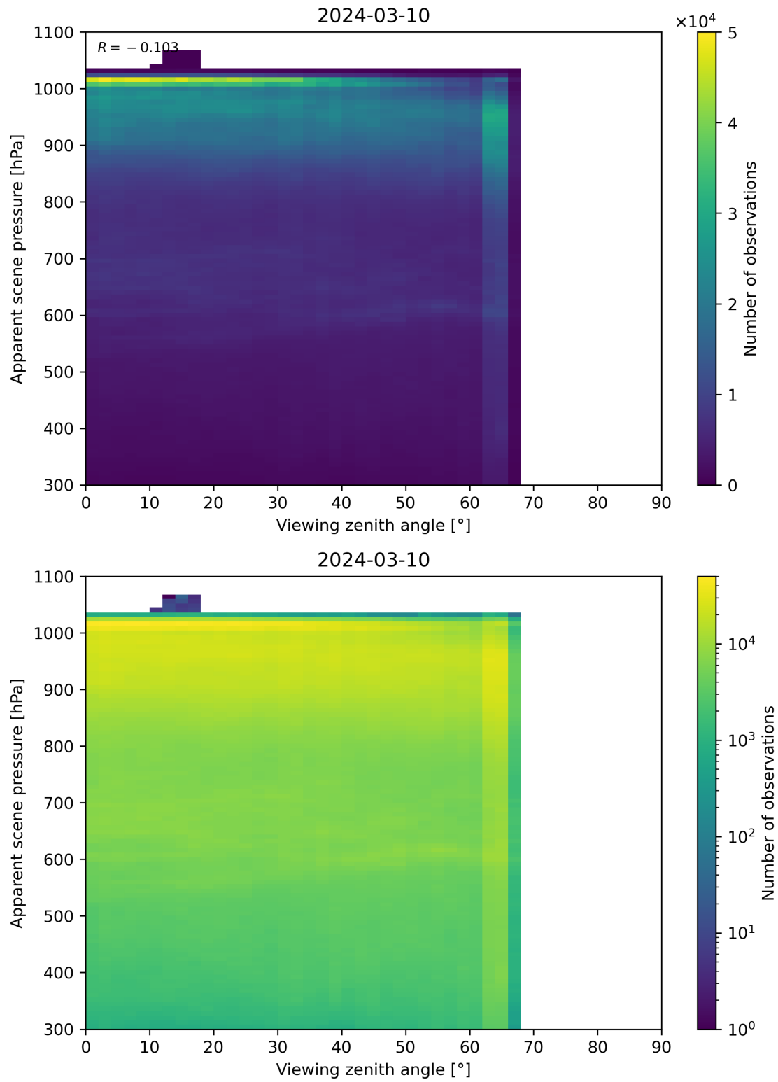
Figure 118: Scatter density plot of “Viewing zenith angle” against “Apparent scene pressure” for 2024-03-09 to 2024-03-11.
