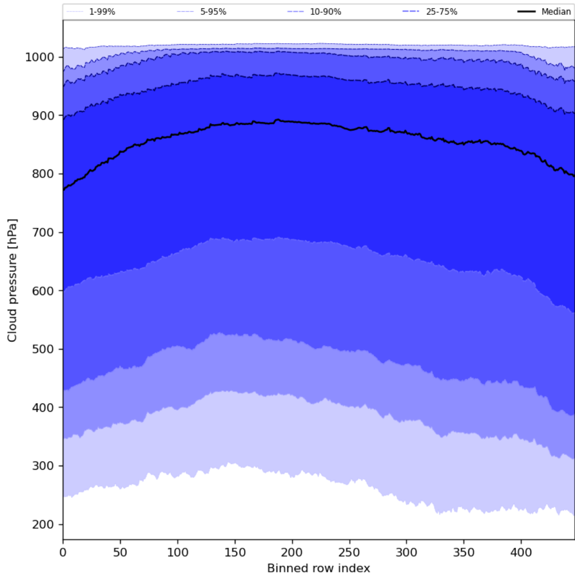
Figure 47: Along track statistics of “Cloud pressure” for 2024-03-10 to 2024-03-12
