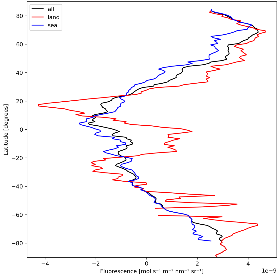
Figure 23: Zonal average of “Fluorescence” for 2024-03-10 to 2024-03-12.
