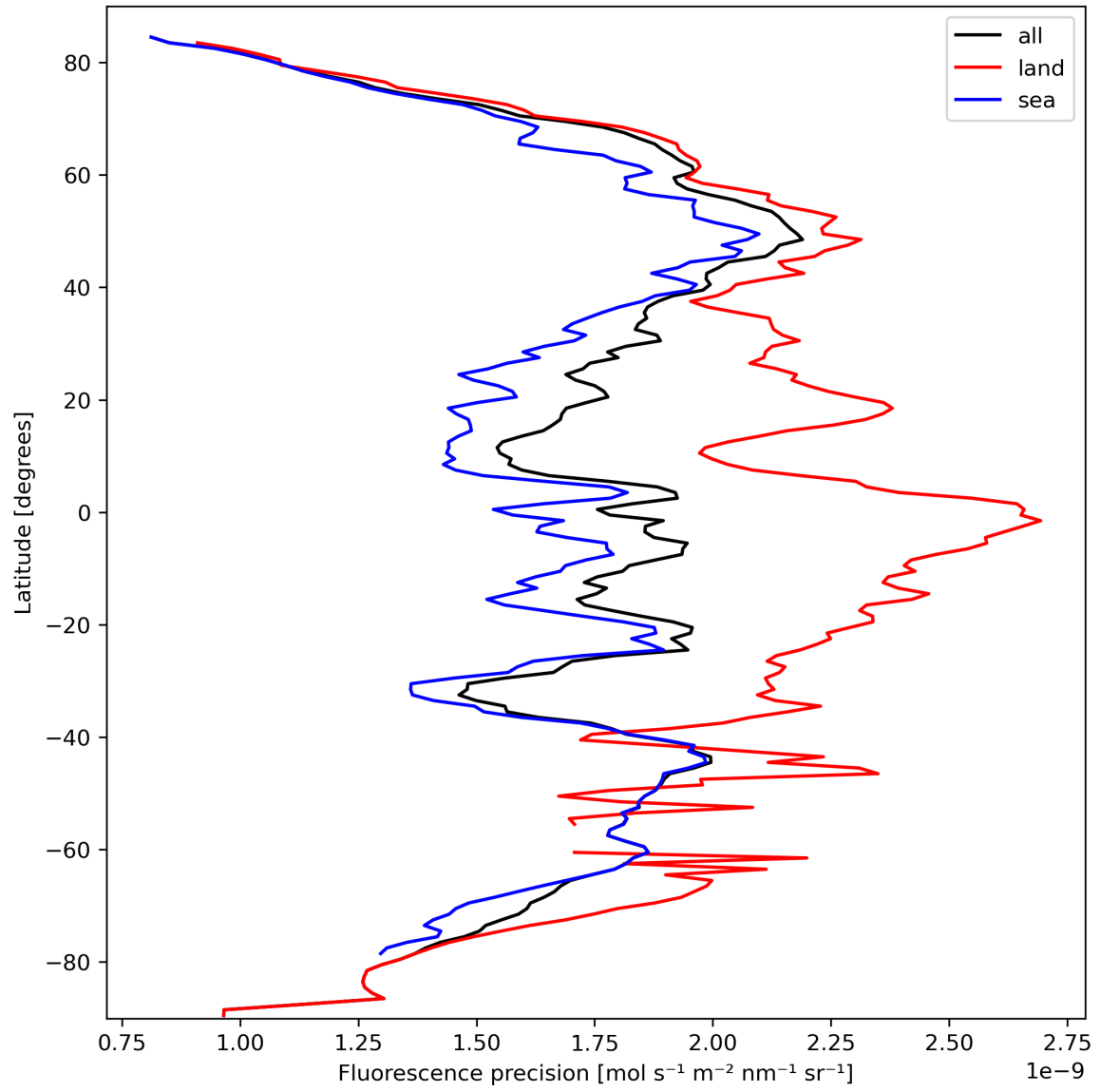
Figure 24: Zonal average of “Fluorescence precision” for 2024-03-10 to 2024-03-12.
