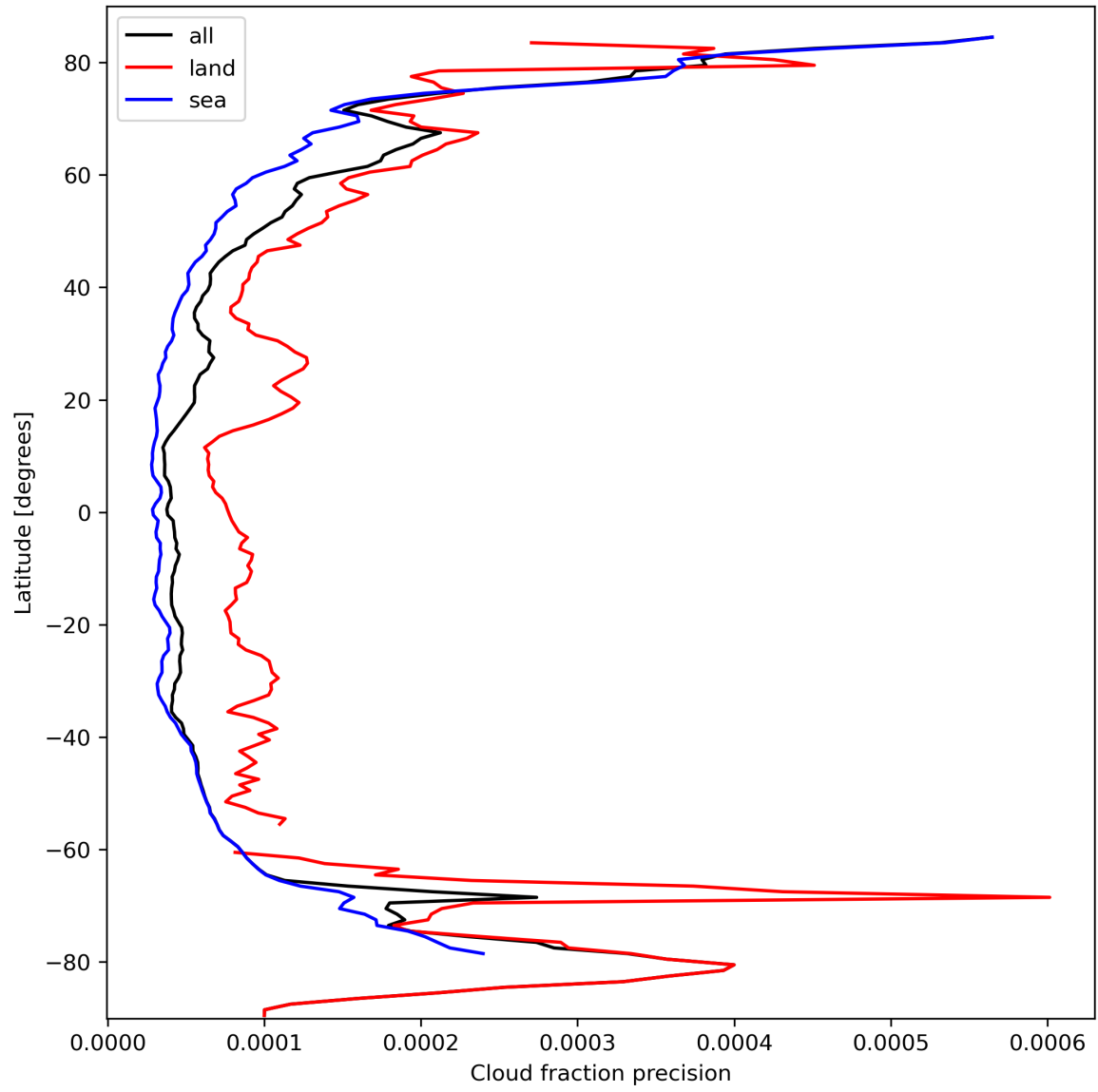
Figure 16: Zonal average of “Cloud fraction precision” for 2024-03-10 to 2024-03-12.
