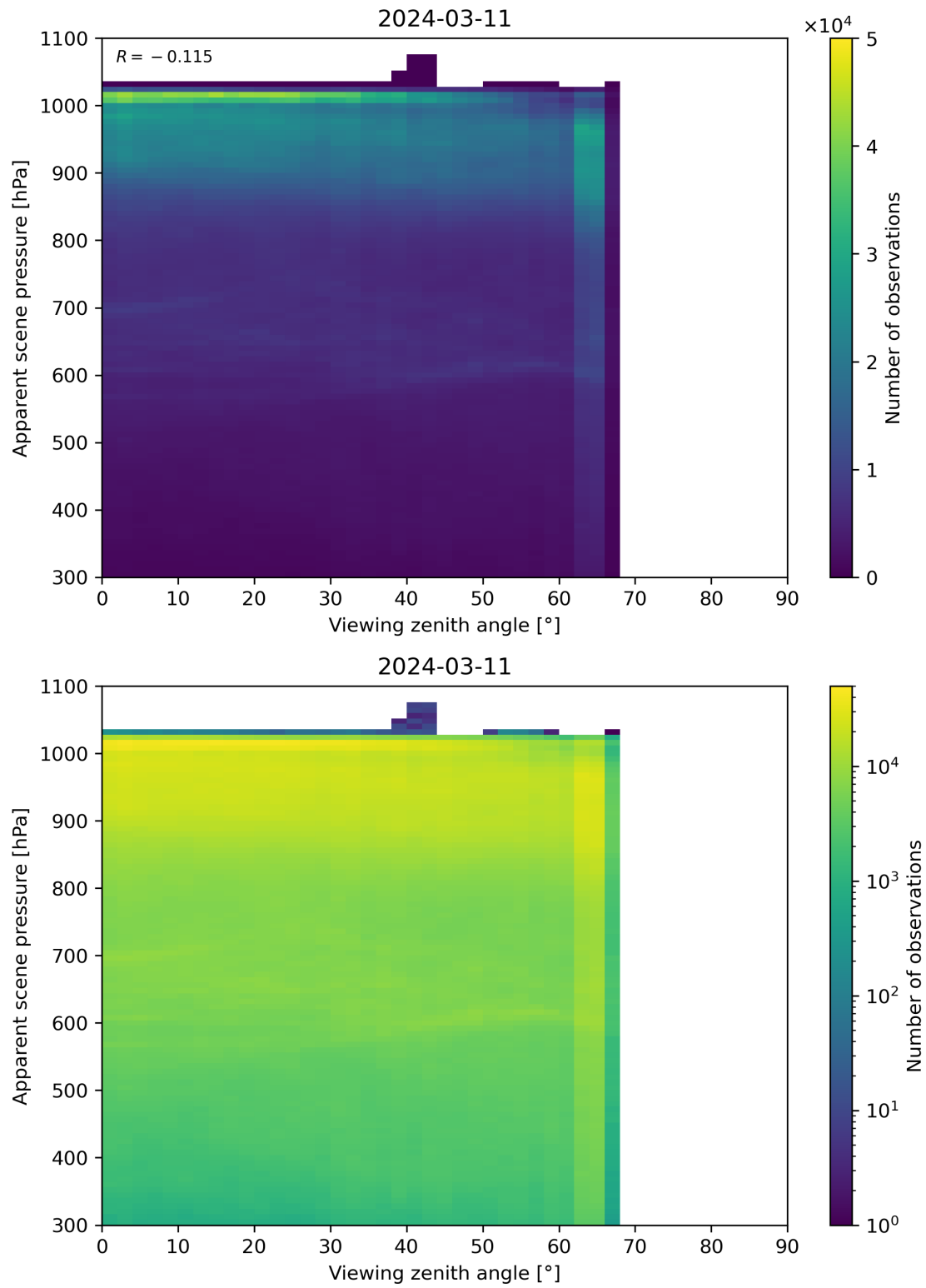
Figure 118: Scatter density plot of “Viewing zenith angle” against “Apparent scene pressure” for 2024-03-10 to 2024-03-12.
