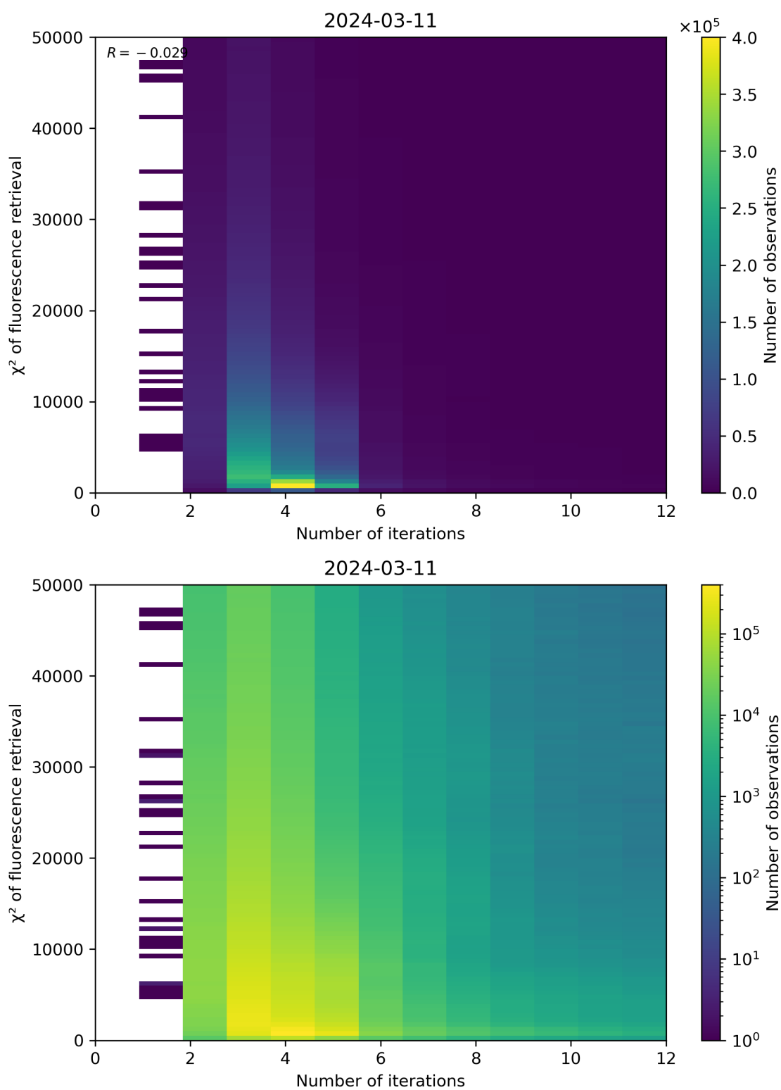
Figure 97: Scatter density plot of “Number of iterations” against “ \chi^2 of fluorescence retrieval” for 2024-03-10 to 2024-03-12.
