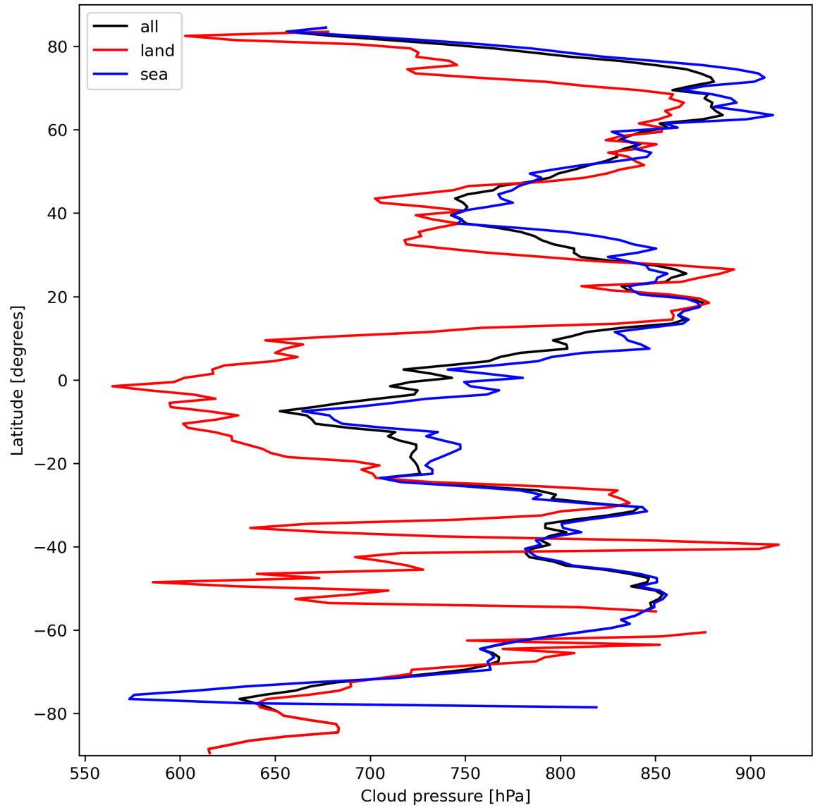
Figure 13: Zonal average of “Cloud pressure” for 2024-03-10 to 2024-03-12.
