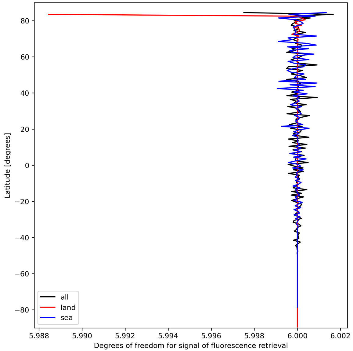
Figure 26: Zonal average of “Degrees of freedom for signal of fluorescence retrieval” for 2024-03-10 to 2024-03-12.
