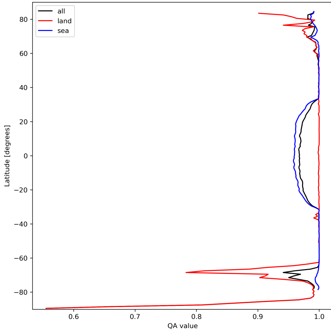
Figure 12: Zonal average of “QA value” for 2024-03-10 to 2024-03-12.
