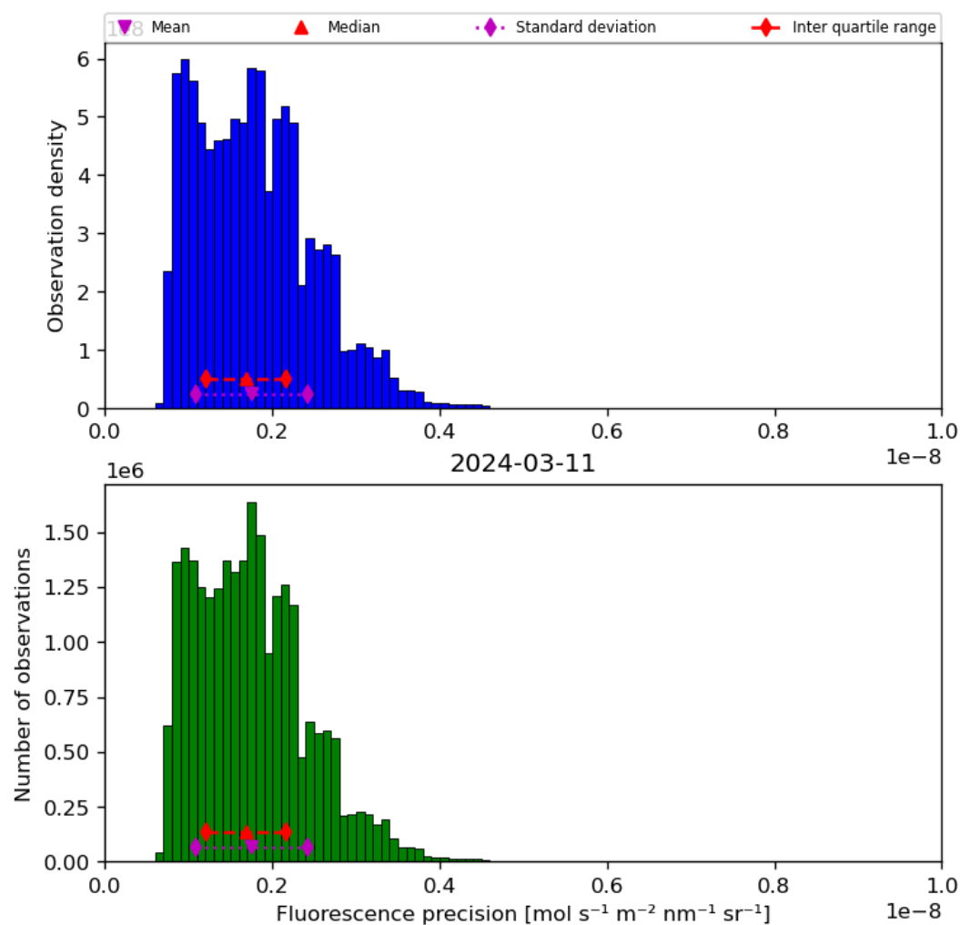
Figure 41: Histogram of “Fluorescence precision” for 2024-03-10 to 2024-03-12
