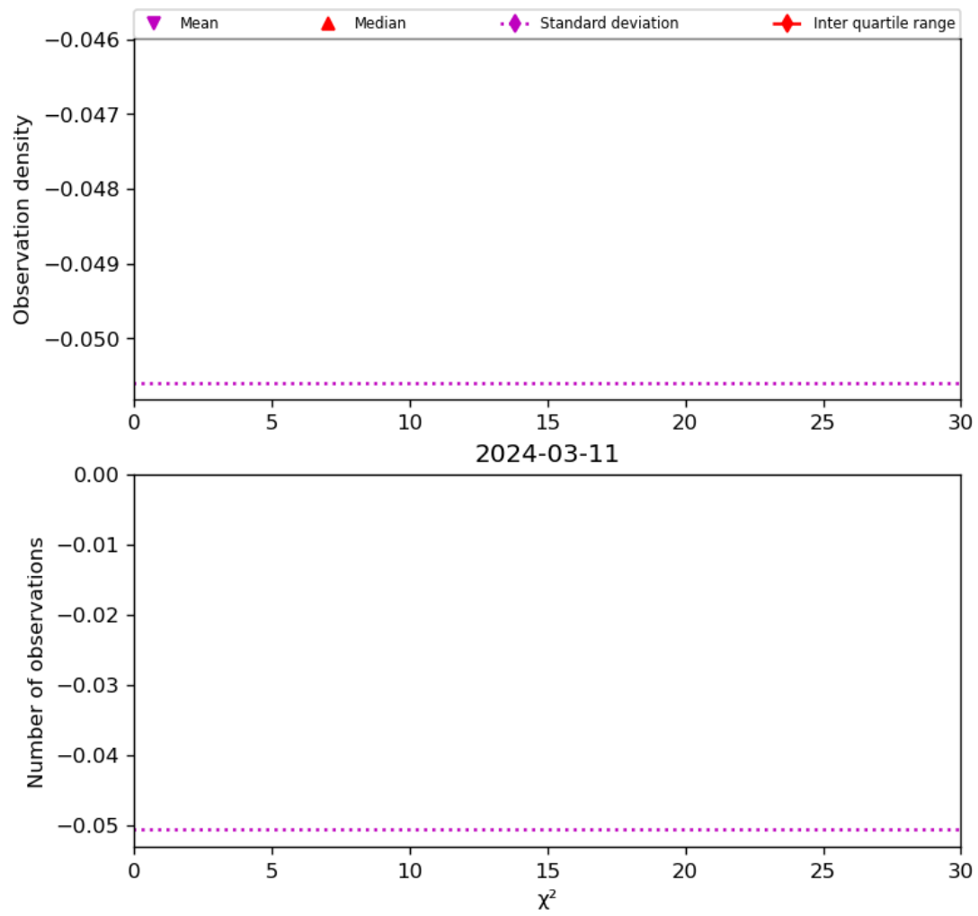
Figure 38: Histogram of " \chi^2 " for 2024-03-10 to 2024-03-12
