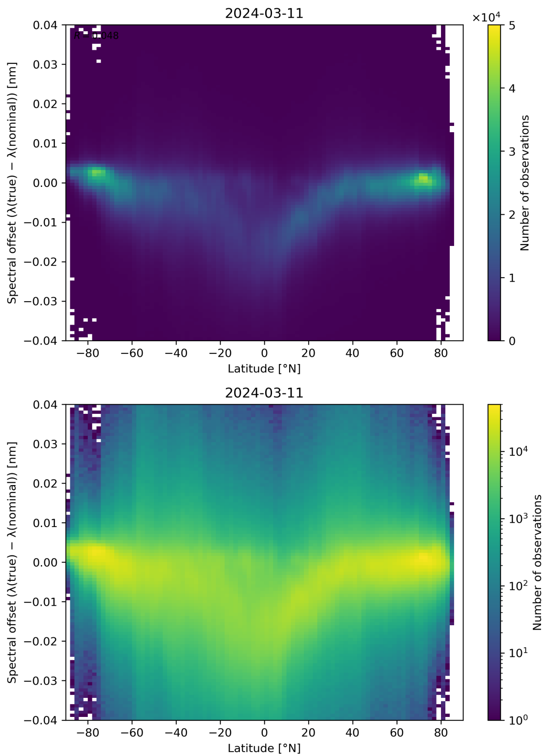
Figure 96: Scatter density plot of “Latitude” against “Spectral offset ( \lambda(\text{true}) - \lambda(\text{nominal}) )” for 2024-03-10 to 2024-03-12.
