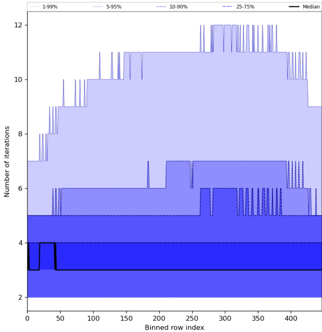
Figure 56: Along track statistics of “Number of iterations” for 2024-03-10 to 2024-03-12
