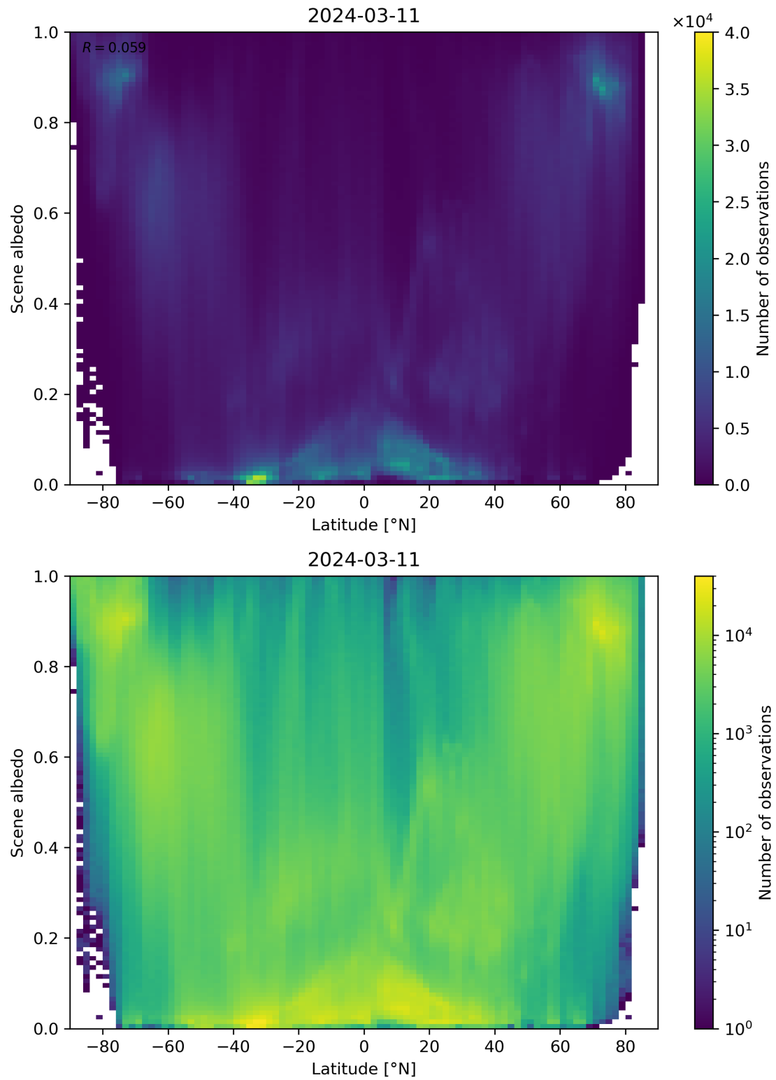
Figure 95: Scatter density plot of “Latitude” against “Scene albedo” for 2024-03-10 to 2024-03-12.
