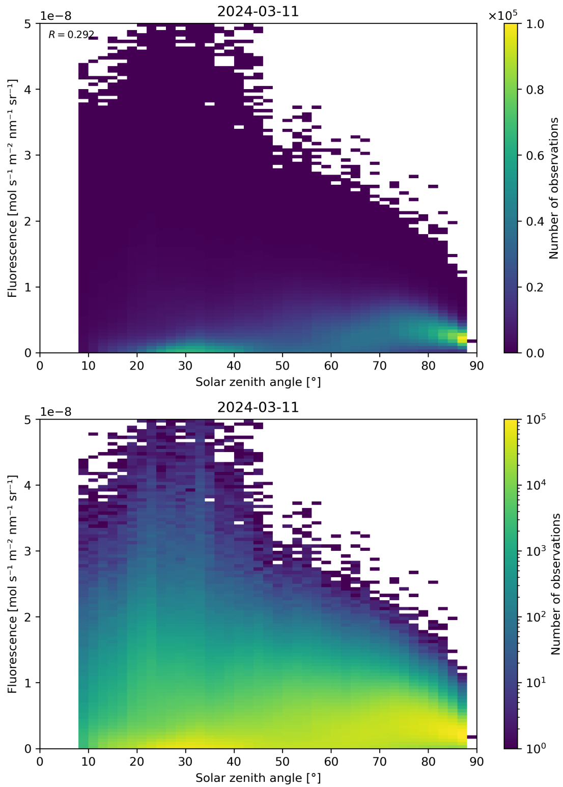
Figure 112: Scatter density plot of “Solar zenith angle” against “Fluorescence” for 2024-03-10 to 2024-03-12.
