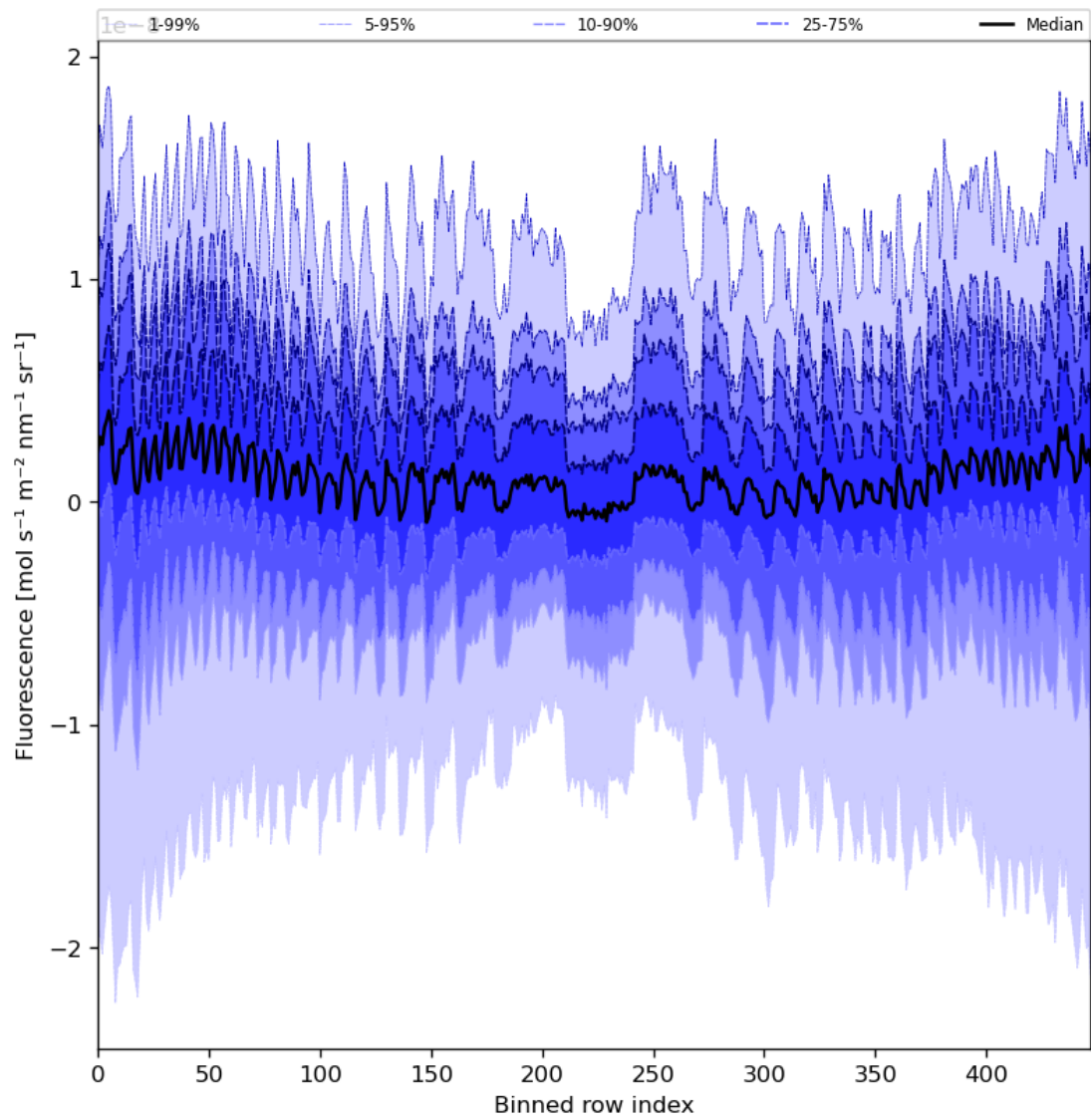
Figure 57: Along track statistics of “Fluorescence” for 2024-03-10 to 2024-03-12
