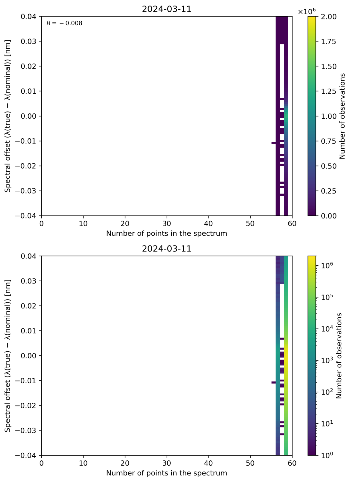
Figure 101: Scatter density plot of “Number of points in the spectrum” against “Spectral offset ( \lambda(\text{true}) - \lambda(\text{nominal}) )” for 2024-03-10 to 2024-03-12.
