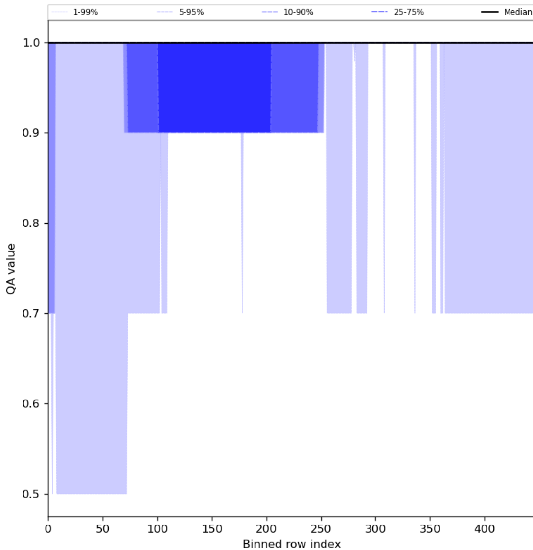
Figure 46: Along track statistics of “QA value” for 2024-03-10 to 2024-03-12
