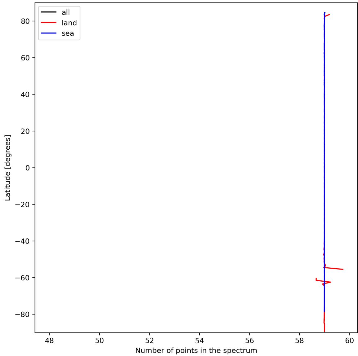
Figure 27: Zonal average of “Number of points in the spectrum” for 2024-03-10 to 2024-03-12.
