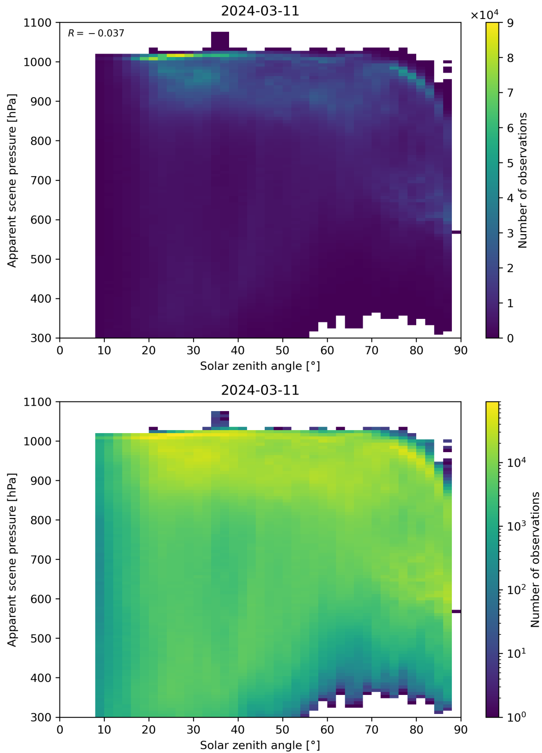
Figure 108: Scatter density plot of “Solar zenith angle” against “Apparent scene pressure” for 2024-03-10 to 2024-03-12.
