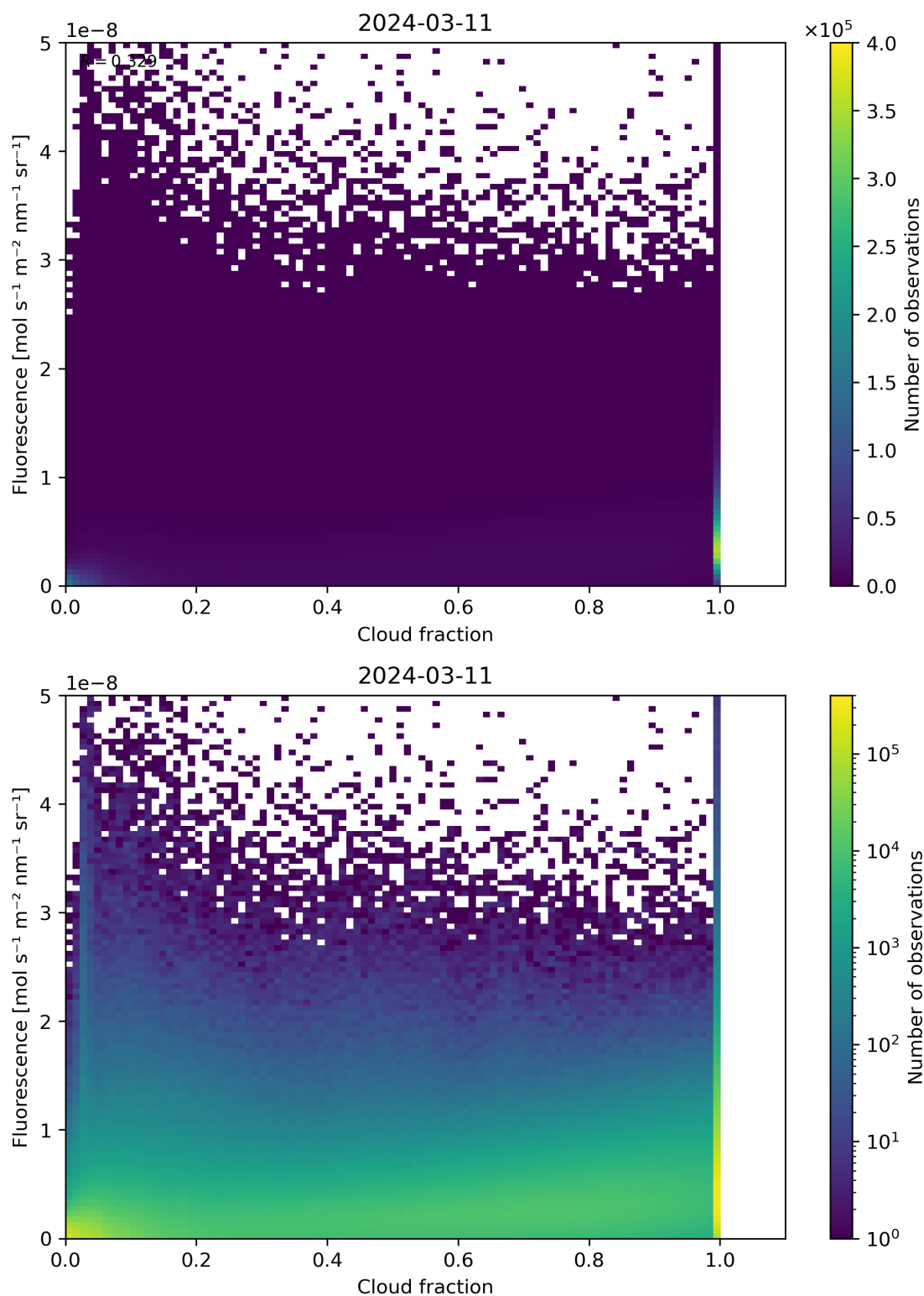
Figure 72: Scatter density plot of “Cloud fraction” against “Fluorescence” for 2024-03-10 to 2024-03-12.
