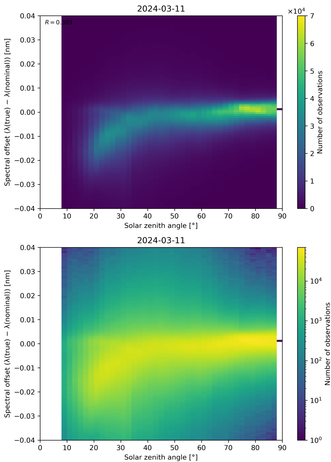
Figure 117: Scatter density plot of “Solar zenith angle” against “Spectral offset ( \lambda(\text{true}) - \lambda(\text{nominal}) )” for 2024-03-10 to 2024-03-12.
