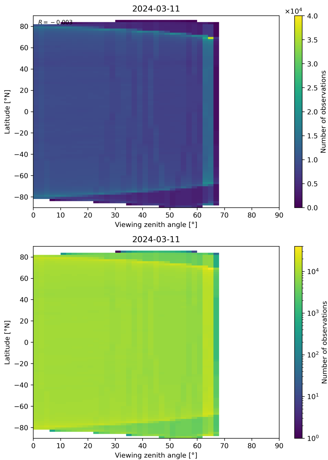
Figure 123: Scatter density plot of “Viewing zenith angle” against “Latitude” for 2024-03-10 to 2024-03-12.
