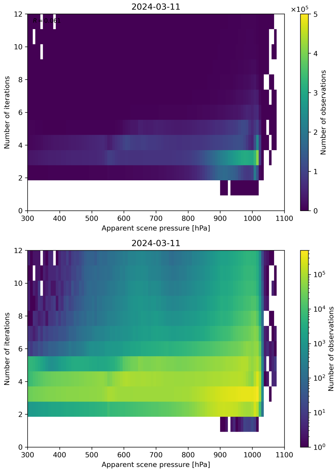
Figure 65: Scatter density plot of “Apparent scene pressure” against “Number of iterations” for 2024-03-10 to 2024-03-12.
