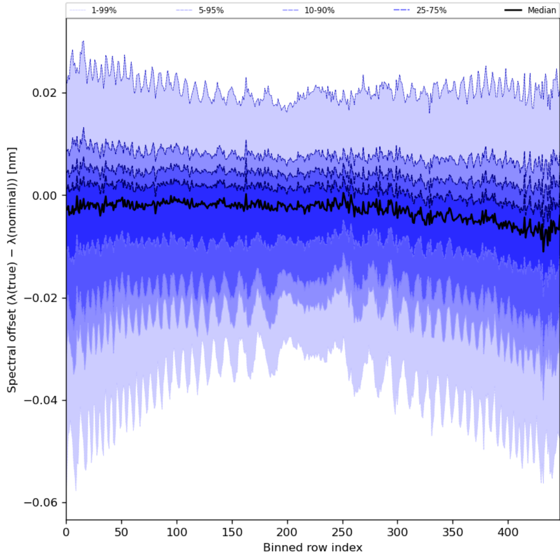
Figure 62: Along track statistics of “Spectral offset ( \lambda(\text{true}) - \lambda(\text{nominal}) )” for 2024-03-10 to 2024-03-12
