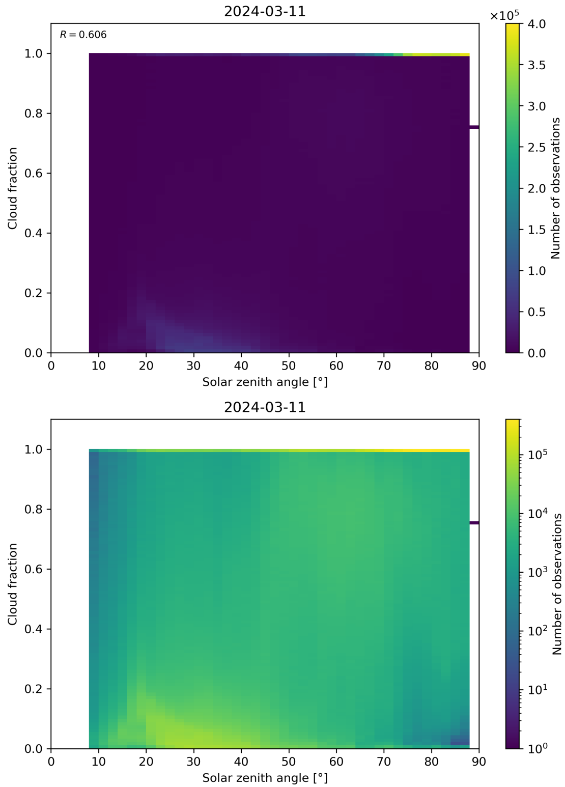
Figure 110: Scatter density plot of “Solar zenith angle” against “Cloud fraction” for 2024-03-10 to 2024-03-12.
