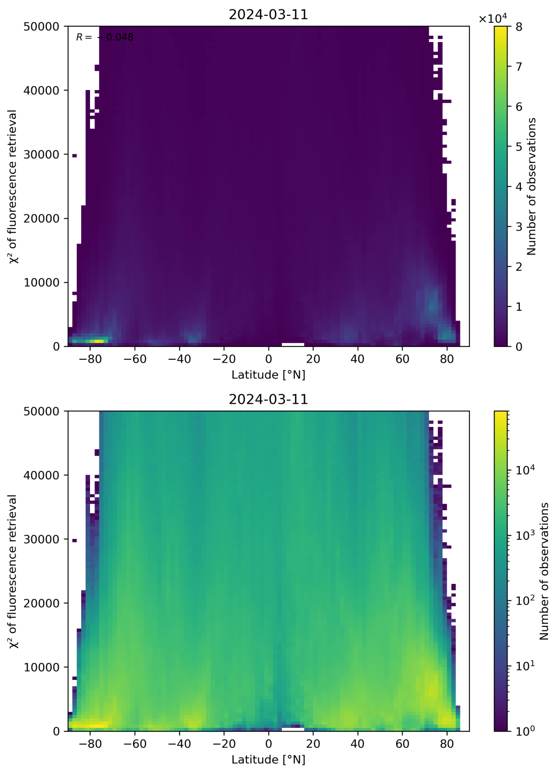
Figure 89: Scatter density plot of “Latitude” against “ \chi^2 of fluorescence retrieval” for 2024-03-10 to 2024-03-12.
