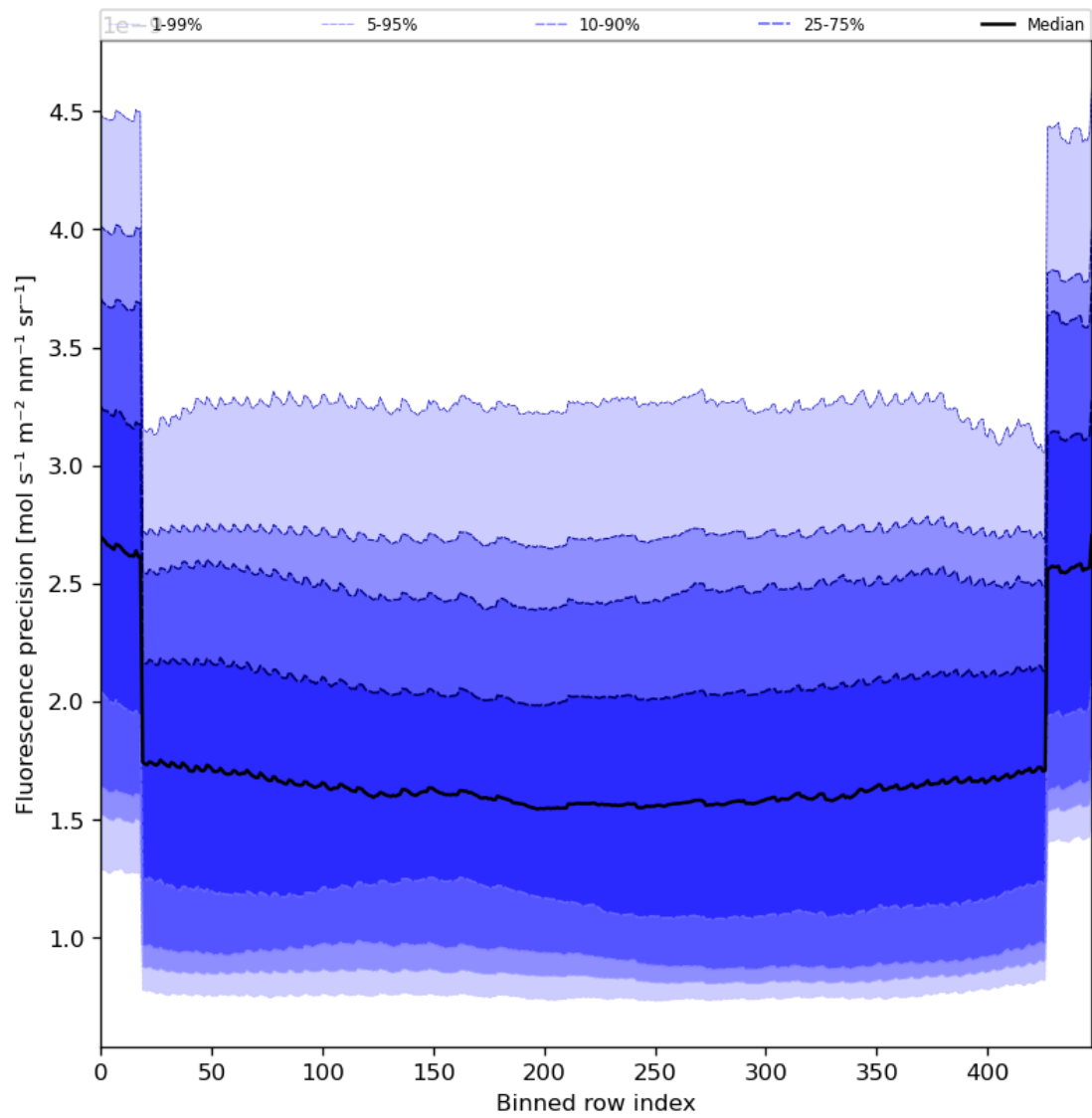
Figure 58: Along track statistics of “Fluorescence precision” for 2024-03-10 to 2024-03-12
