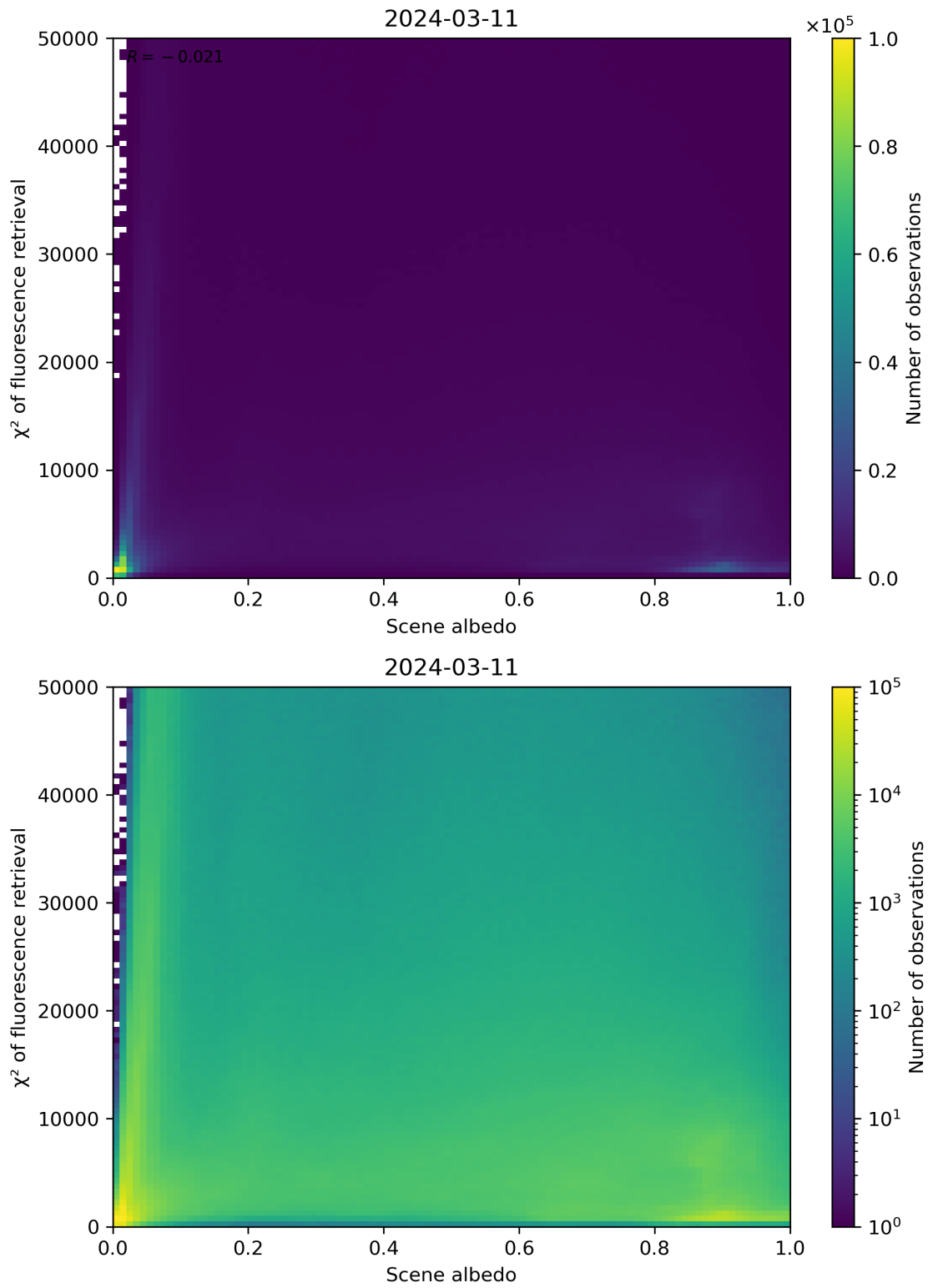
Figure 103: Scatter density plot of “Scene albedo” against “ \chi^2 of fluorescence retrieval” for 2024-03-10 to 2024-03-12.
