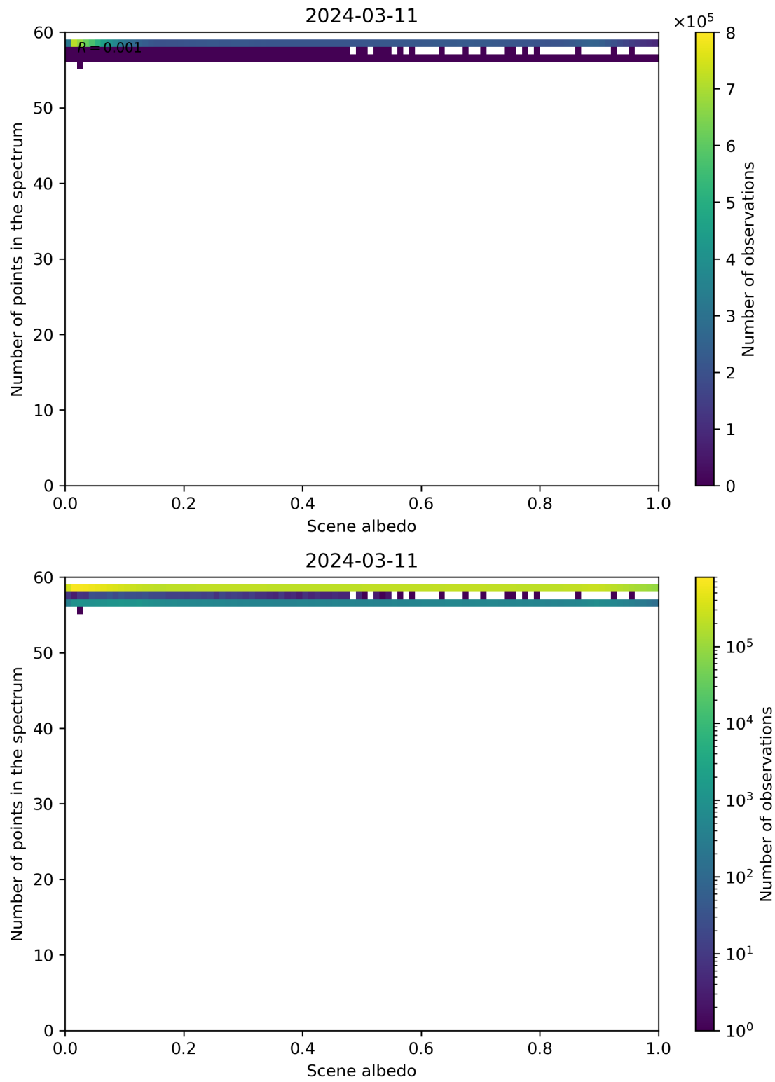
Figure 106: Scatter density plot of “Scene albedo” against “Number of points in the spectrum” for 2024-03-10 to 2024-03-12.
