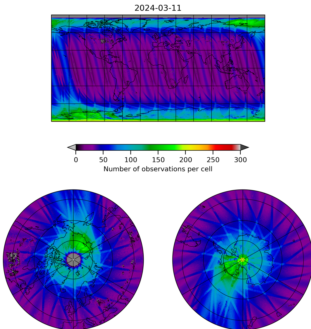
Figure 11: Map of the number of observations for 2024-03-10 to 2024-03-12
