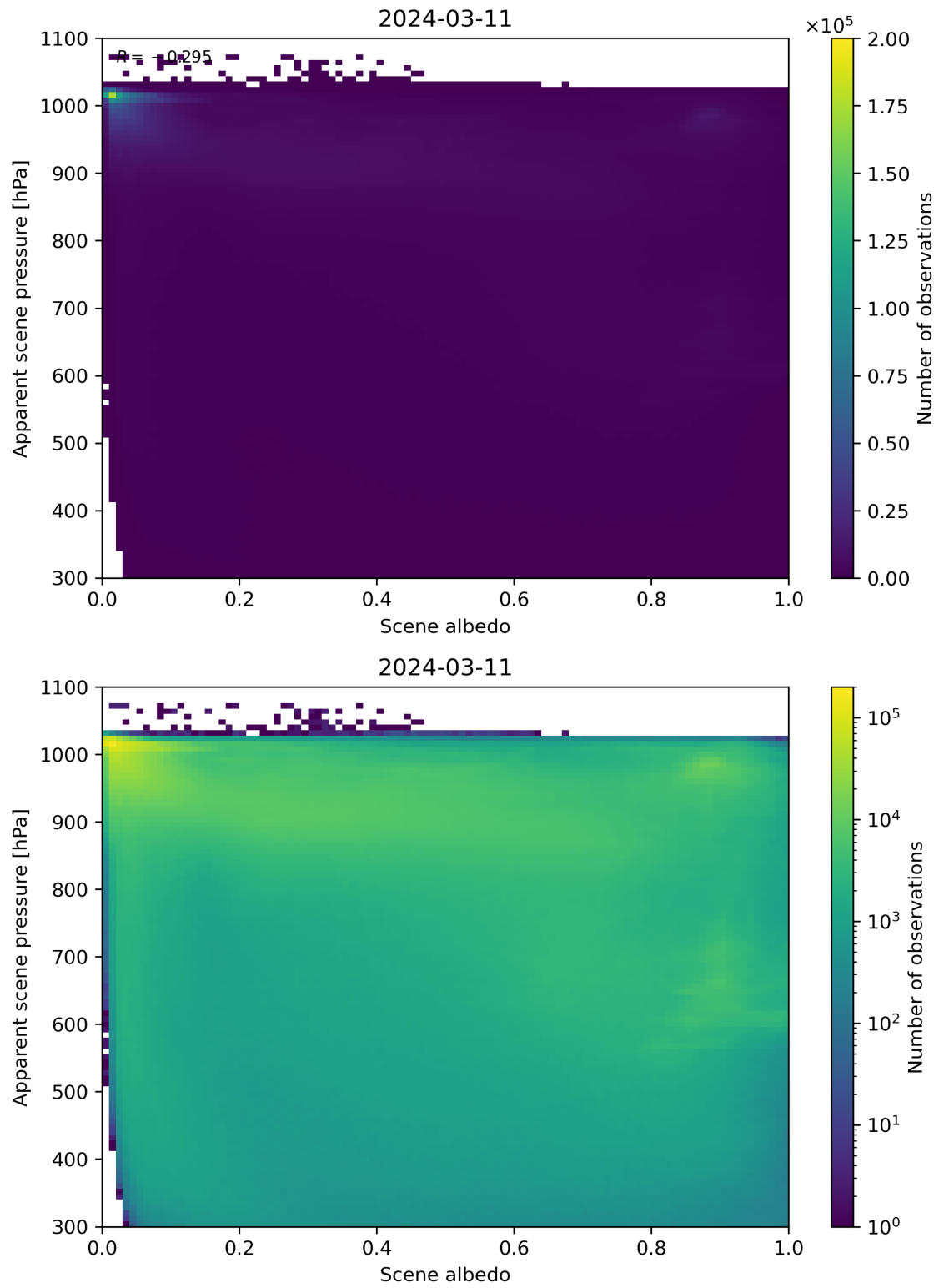
Figure 102: Scatter density plot of “Scene albedo” against “Apparent scene pressure” for 2024-03-10 to 2024-03-12.
