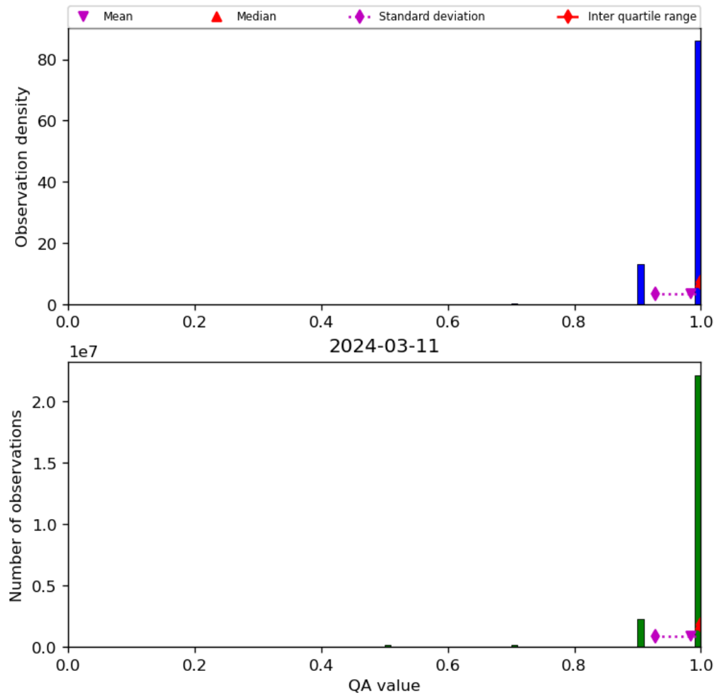
Figure 29: Histogram of “QA value” for 2024-03-10 to 2024-03-12
