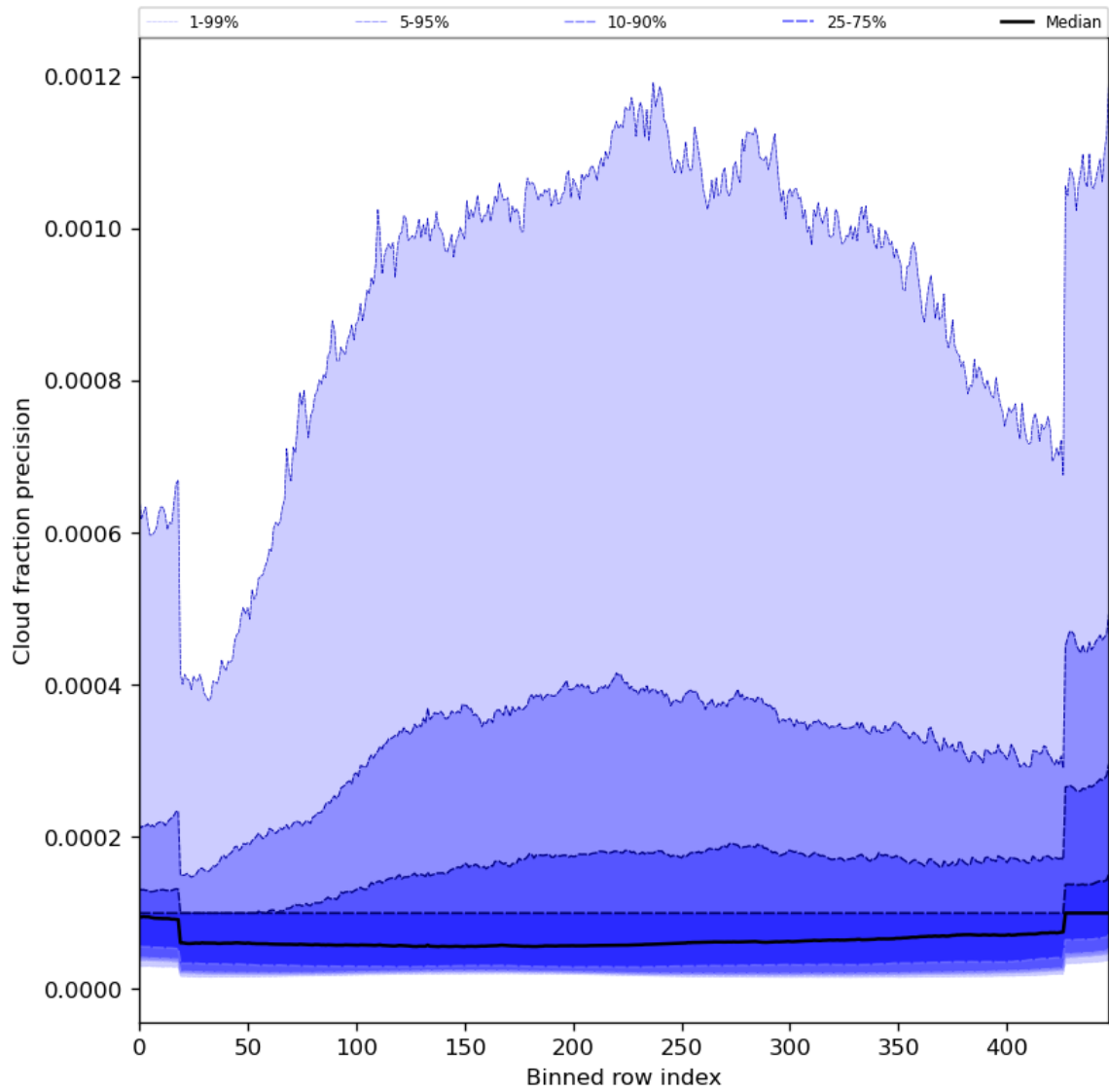
Figure 50: Along track statistics of “Cloud fraction precision” for 2024-03-10 to 2024-03-12
