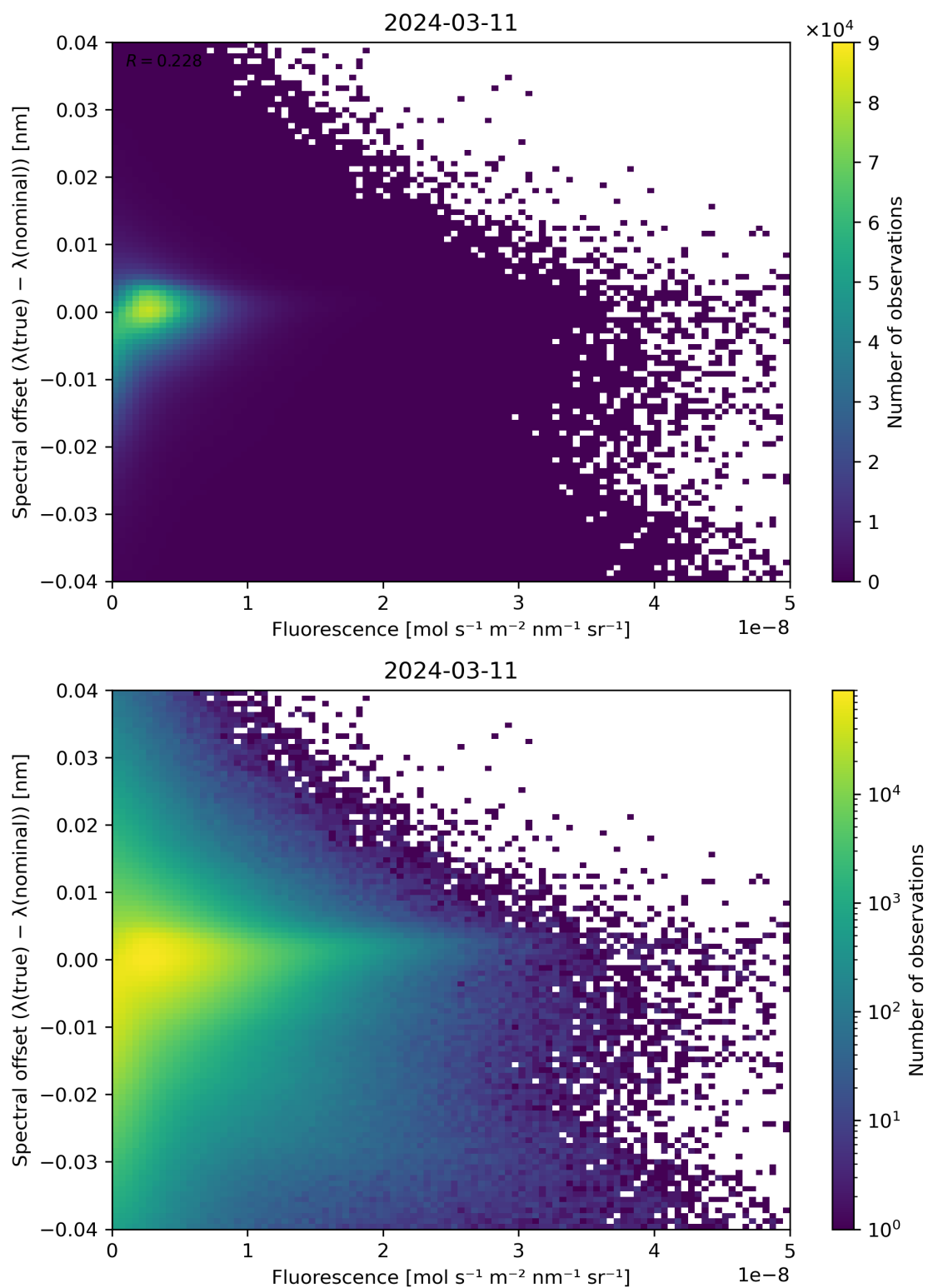
Figure 87: Scatter density plot of “Fluorescence” against “Spectral offset ( \lambda(\text{true}) - \lambda(\text{nominal}) )” for 2024-03-10 to 2024-03-12.
