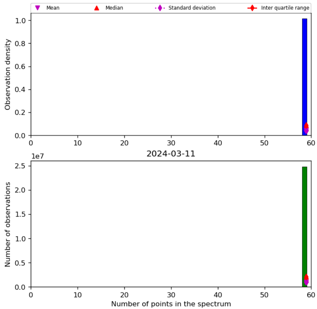
Figure 44: Histogram of “Number of points in the spectrum” for 2024-03-10 to 2024-03-12
