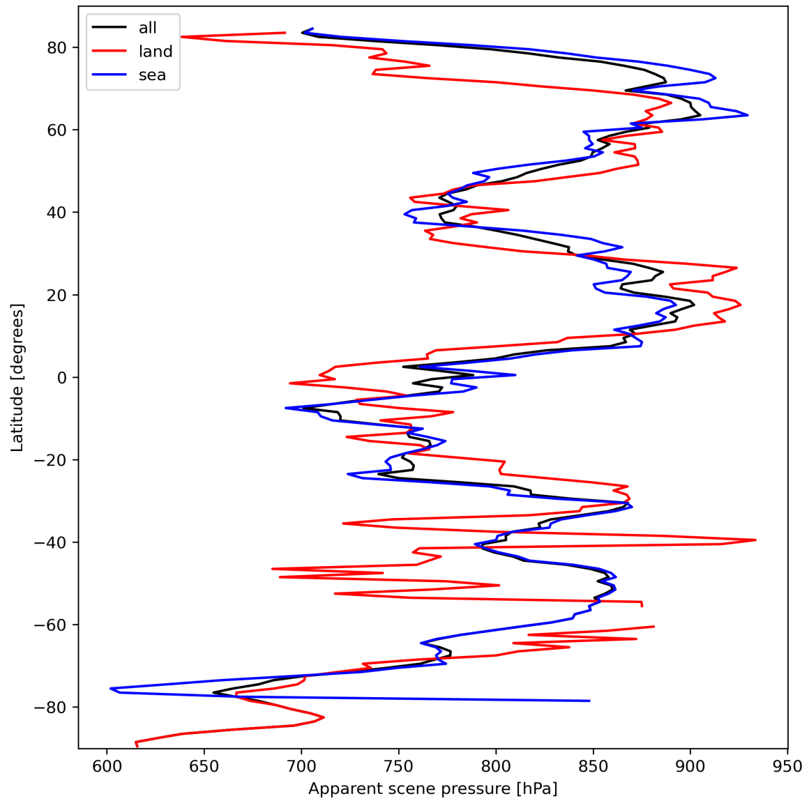
Figure 19: Zonal average of “Apparent scene pressure” for 2024-03-10 to 2024-03-12.
