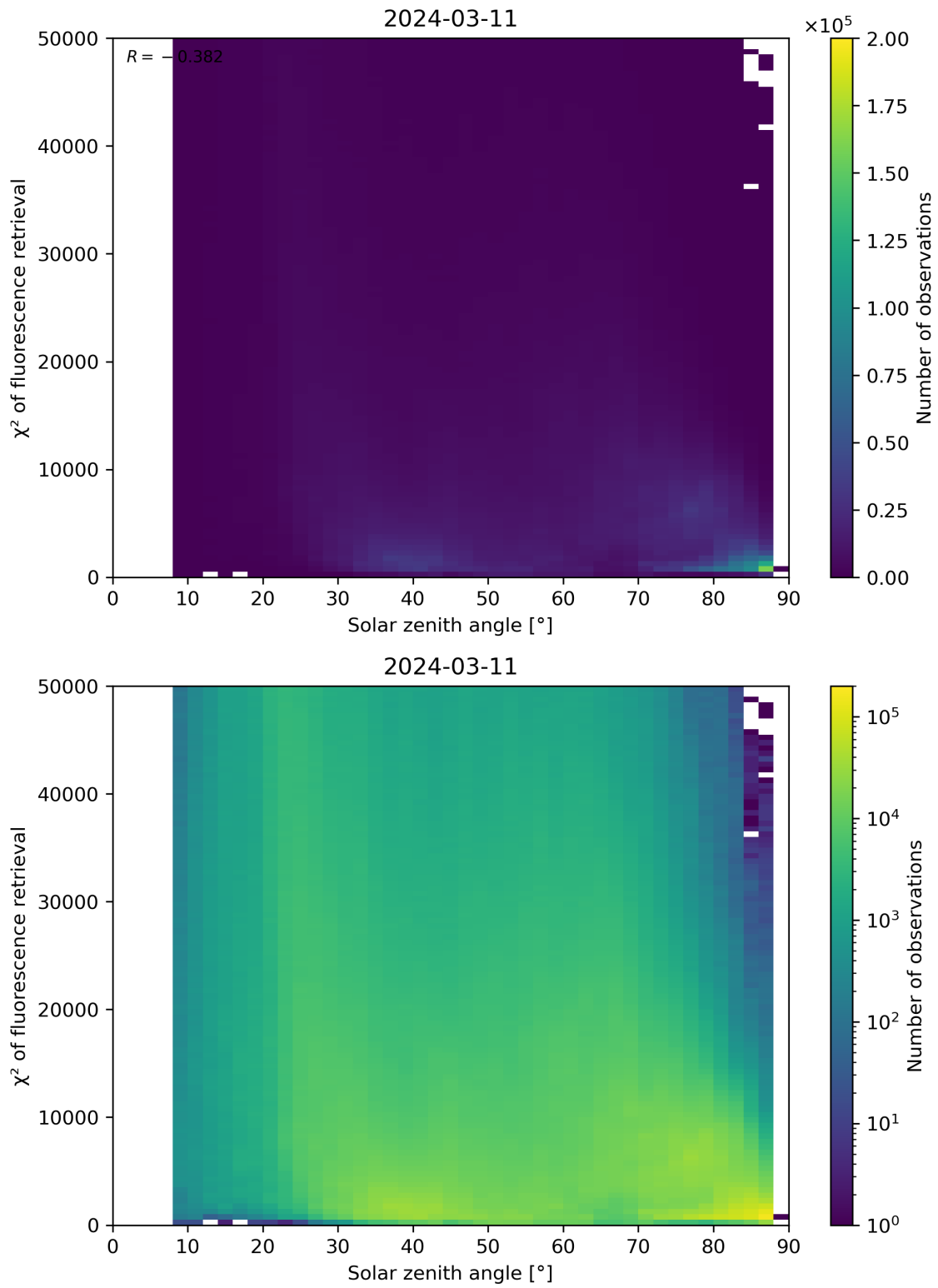
Figure 109: Scatter density plot of “Solar zenith angle” against “ \chi^2 of fluorescence retrieval” for 2024-03-10 to 2024-03-12.
