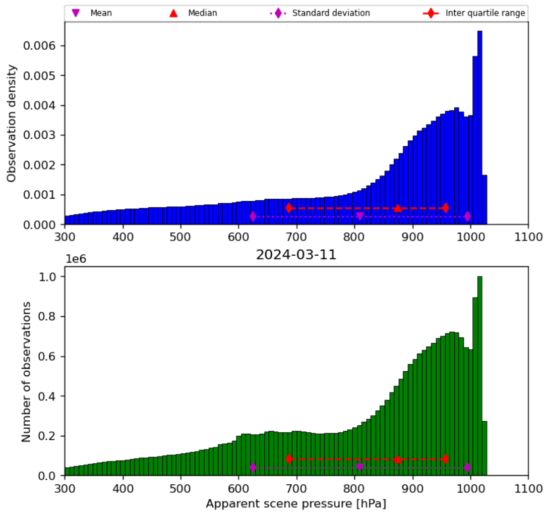
Figure 36: Histogram of “Apparent scene pressure” for 2024-03-10 to 2024-03-12
