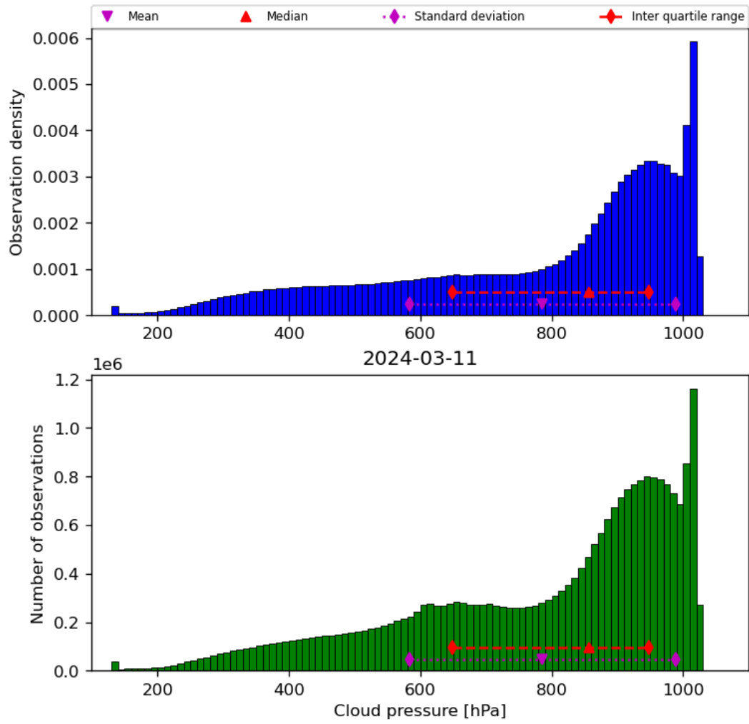
Figure 30: Histogram of “Cloud pressure” for 2024-03-10 to 2024-03-12
