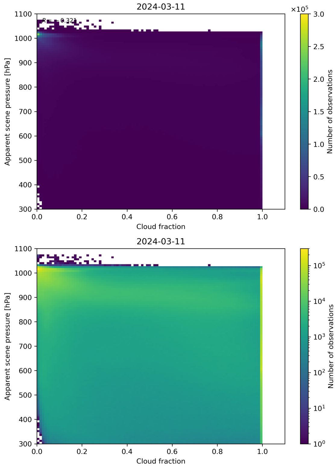
Figure 70: Scatter density plot of “Cloud fraction” against “Apparent scene pressure” for 2024-03-10 to 2024-03-12.
