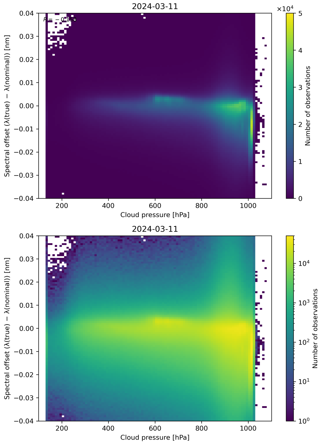
Figure 84: Scatter density plot of “Cloud pressure” against “Spectral offset ( \lambda(\text{true}) - \lambda(\text{nominal}) )” for 2024-03-10 to 2024-03-12.
