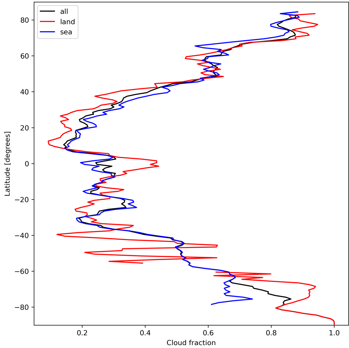
Figure 15: Zonal average of “Cloud fraction” for 2024-03-10 to 2024-03-12.
