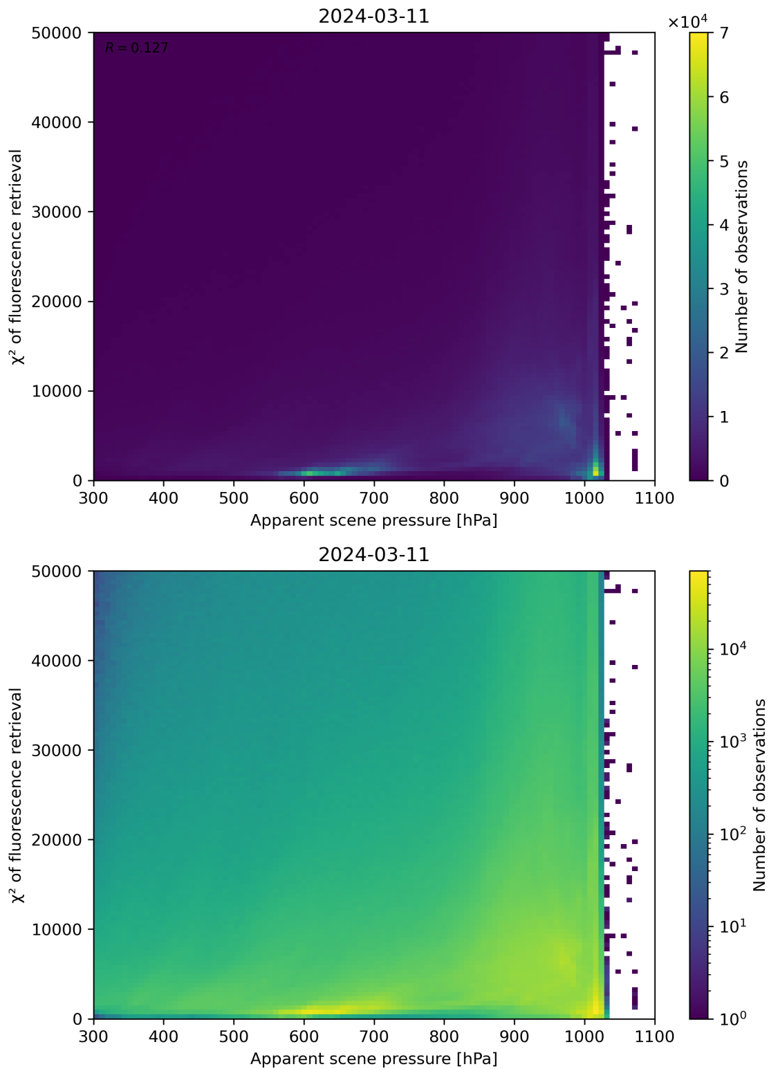
Figure 63: Scatter density plot of “Apparent scene pressure” against “ \chi^2 of fluorescence retrieval” for 2024-03-10 to 2024-03-12.
