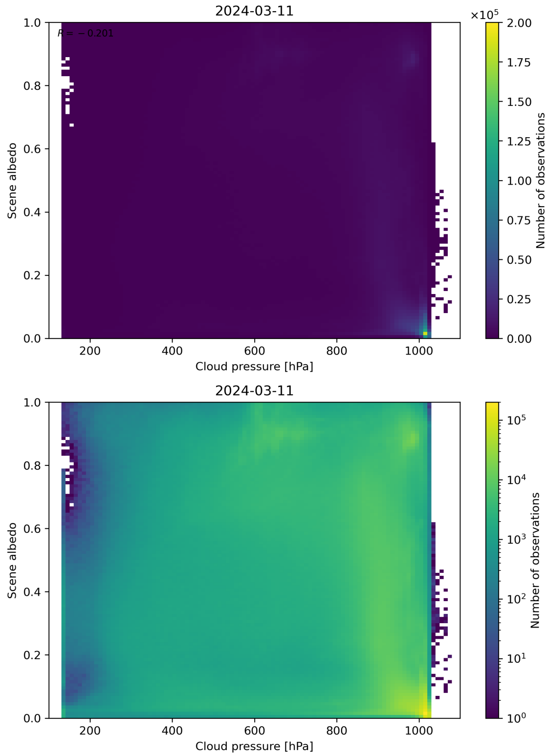
Figure 83: Scatter density plot of “Cloud pressure” against “Scene albedo” for 2024-03-10 to 2024-03-12.
