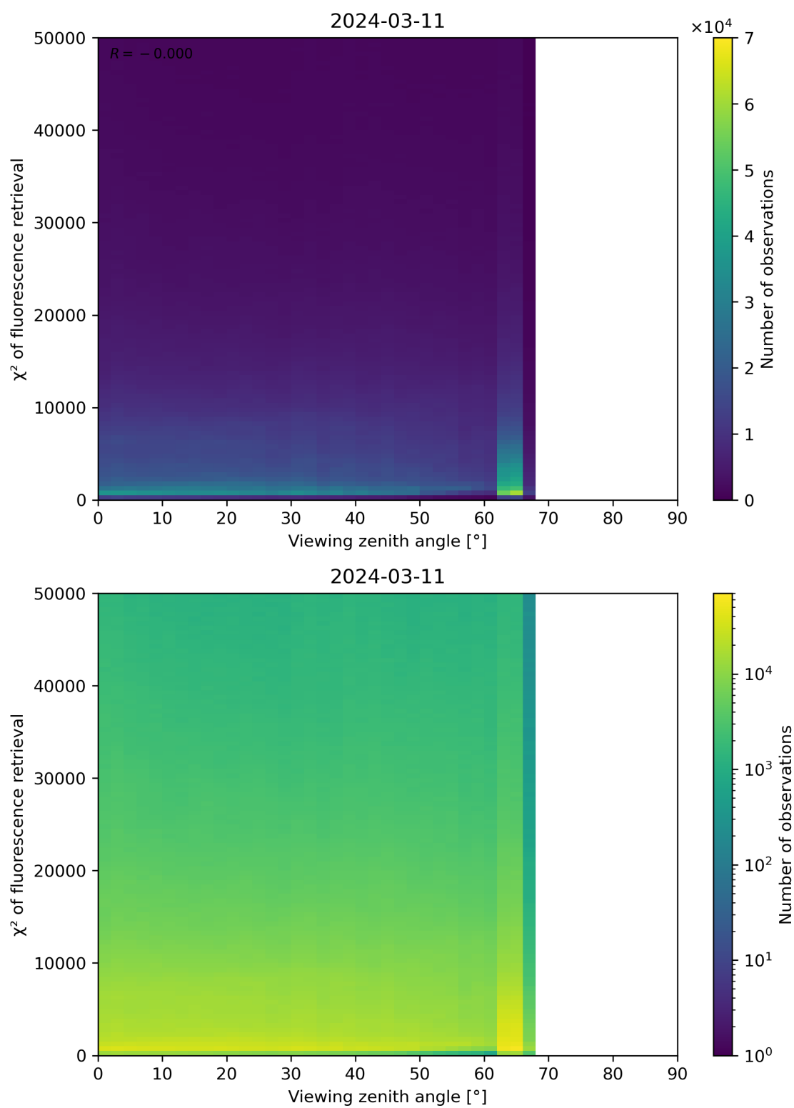
Figure 119: Scatter density plot of “Viewing zenith angle” against “ \chi^2 of fluorescence retrieval” for 2024-03-10 to 2024-03-12.
