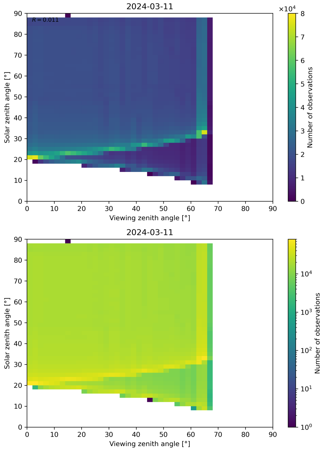
Figure 127: Scatter density plot of “Viewing zenith angle” against “Solar zenith angle” for 2024-03-10 to 2024-03-12.
