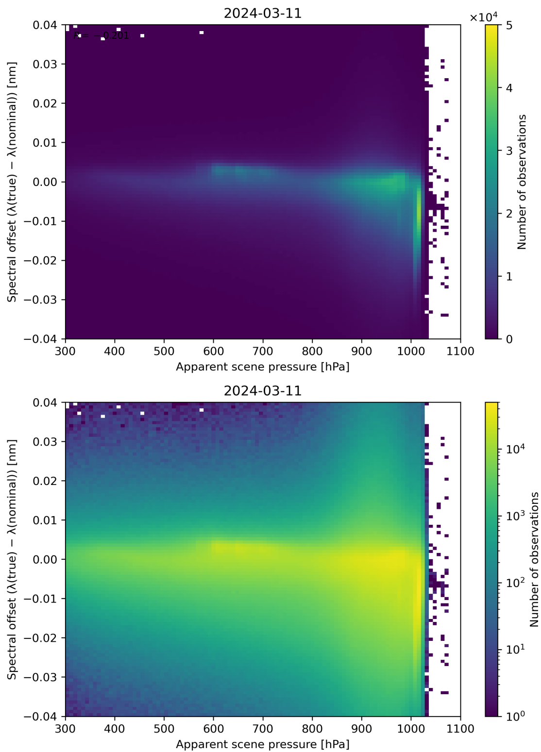
Figure 67: Scatter density plot of “Apparent scene pressure” against “Spectral offset ( \lambda(\text{true}) - \lambda(\text{nominal}) )” for 2024-03-10 to 2024-03-12.
