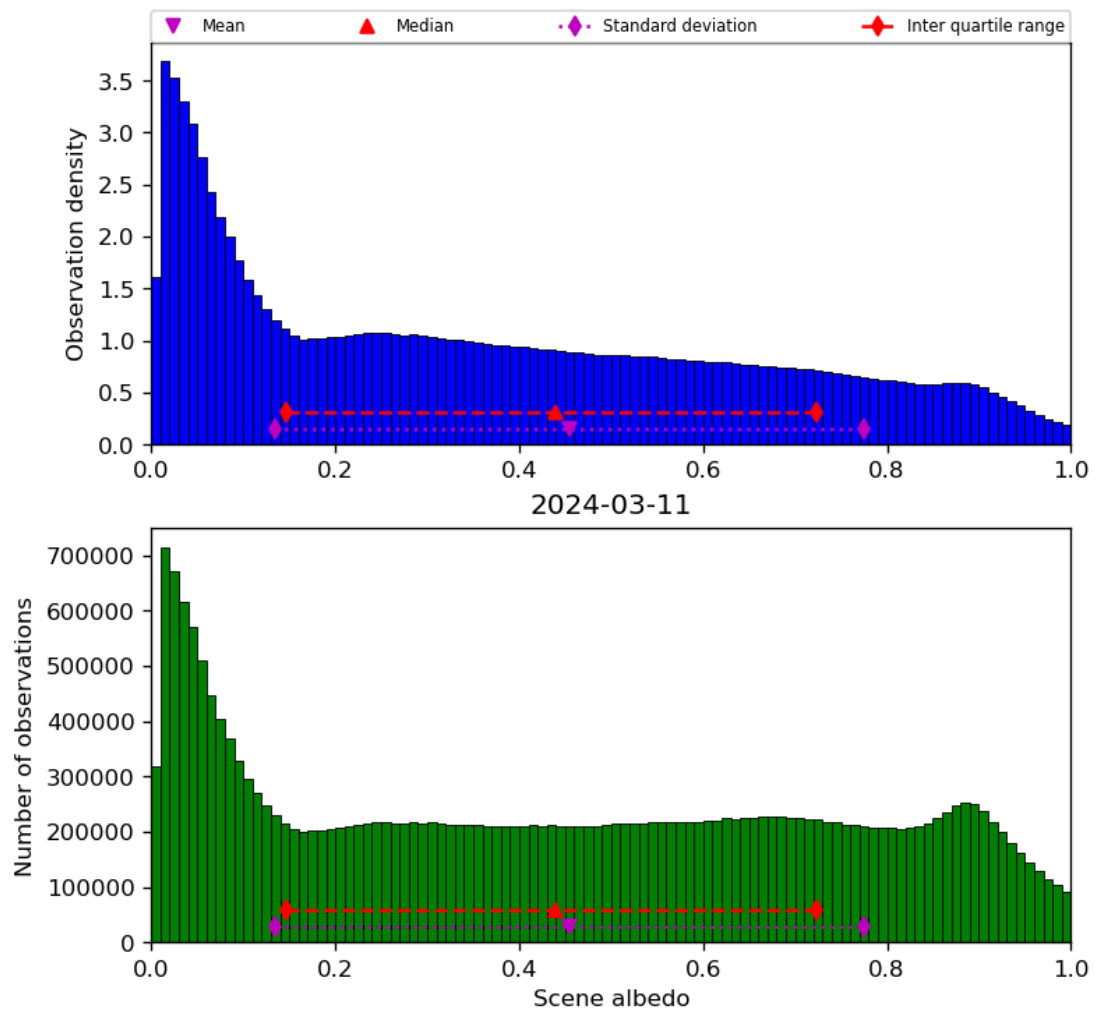
Figure 34: Histogram of “Scene albedo” for 2024-03-10 to 2024-03-12
