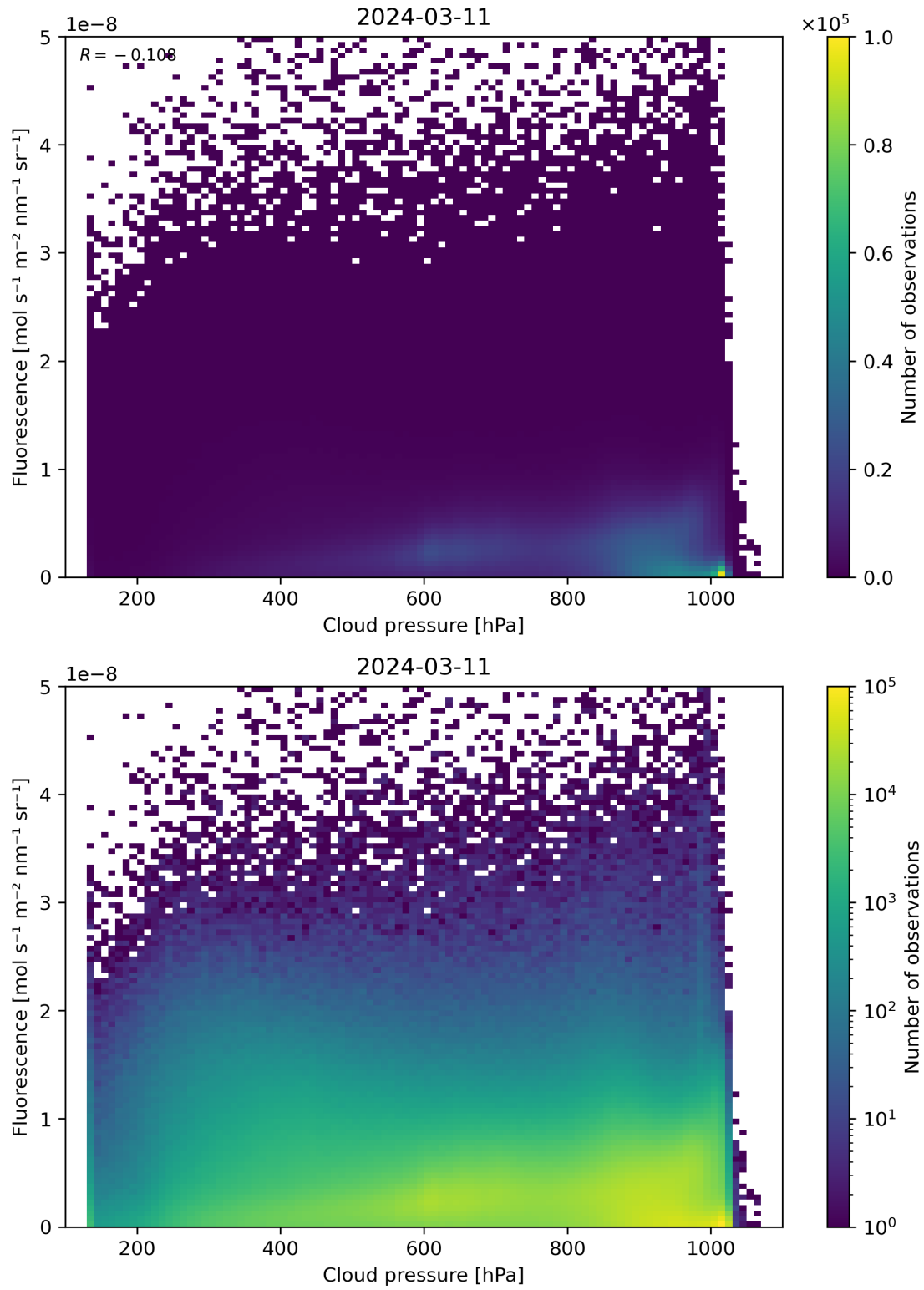
Figure 80: Scatter density plot of “Cloud pressure” against “Fluorescence” for 2024-03-10 to 2024-03-12.
