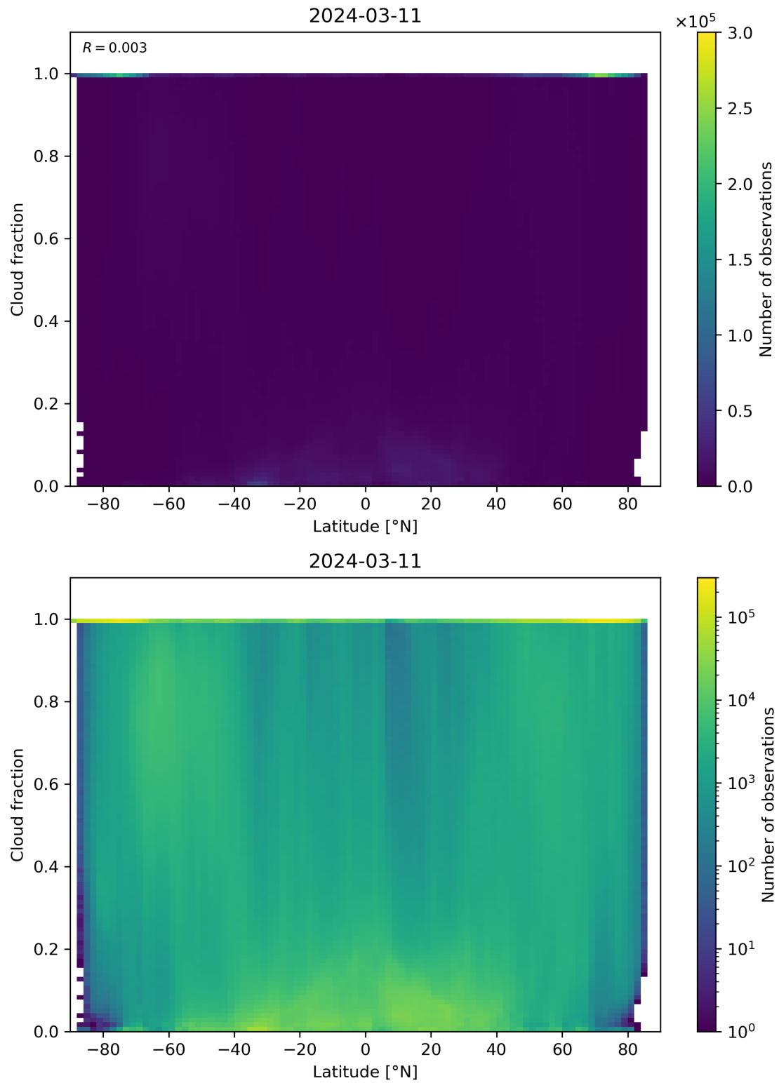
Figure 90: Scatter density plot of “Latitude” against “Cloud fraction” for 2024-03-10 to 2024-03-12.
