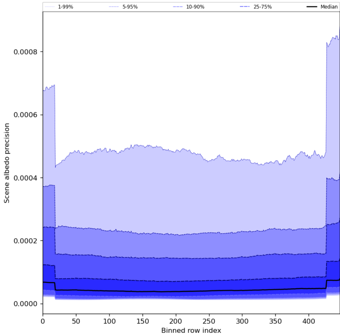
Figure 52: Along track statistics of “Scene albedo precision” for 2024-03-10 to 2024-03-12
