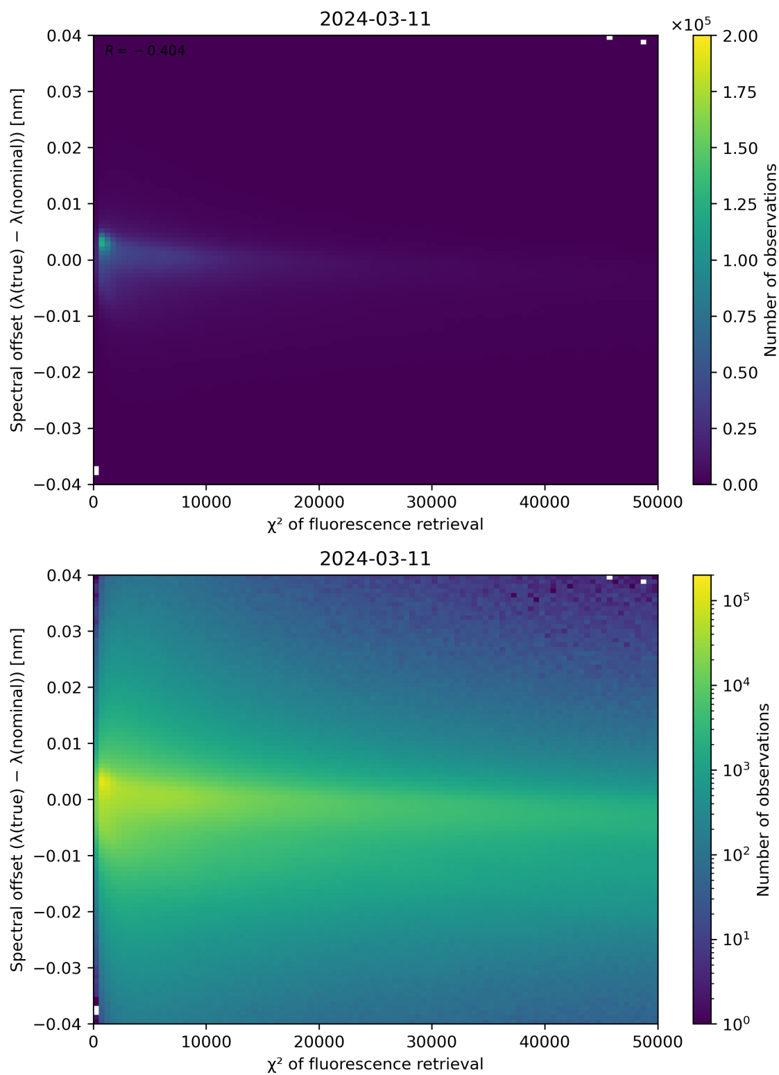
Figure 69: Scatter density plot of " \chi^2 of fluorescence retrieval" against "Spectral offset ( \lambda(\text{true}) - \lambda(\text{nominal}) )" for 2024-03-10 to 2024-03-12.
