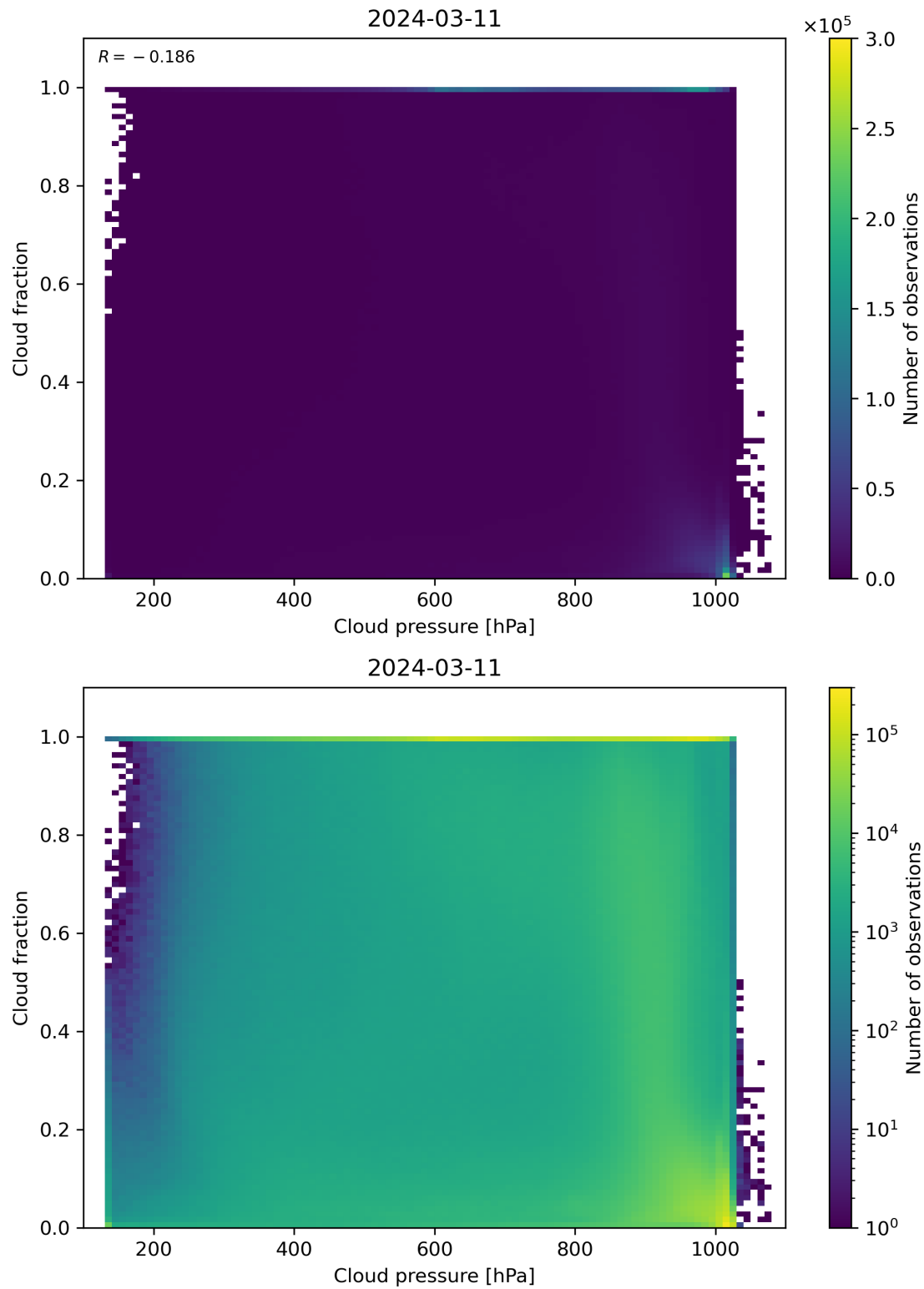
Figure 79: Scatter density plot of “Cloud pressure” against “Cloud fraction” for 2024-03-10 to 2024-03-12.
