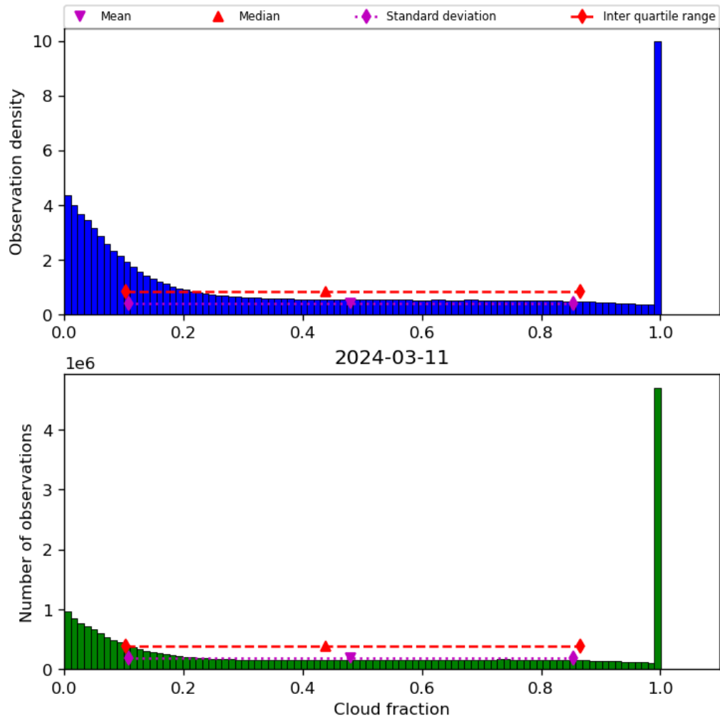
Figure 32: Histogram of “Cloud fraction” for 2024-03-10 to 2024-03-12
