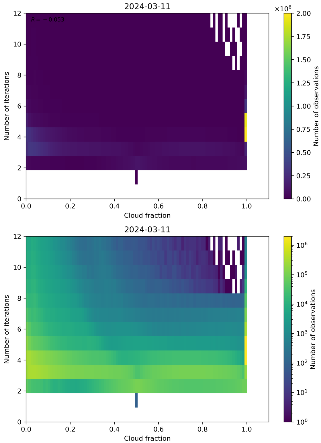
Figure 73: Scatter density plot of “Cloud fraction” against “Number of iterations” for 2024-03-10 to 2024-03-12.
