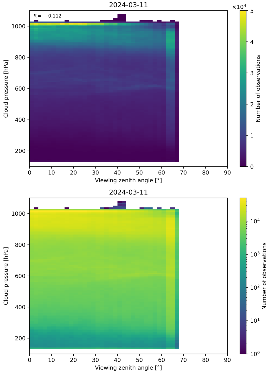
Figure 121: Scatter density plot of “Viewing zenith angle” against “Cloud pressure” for 2024-03-10 to 2024-03-12.
