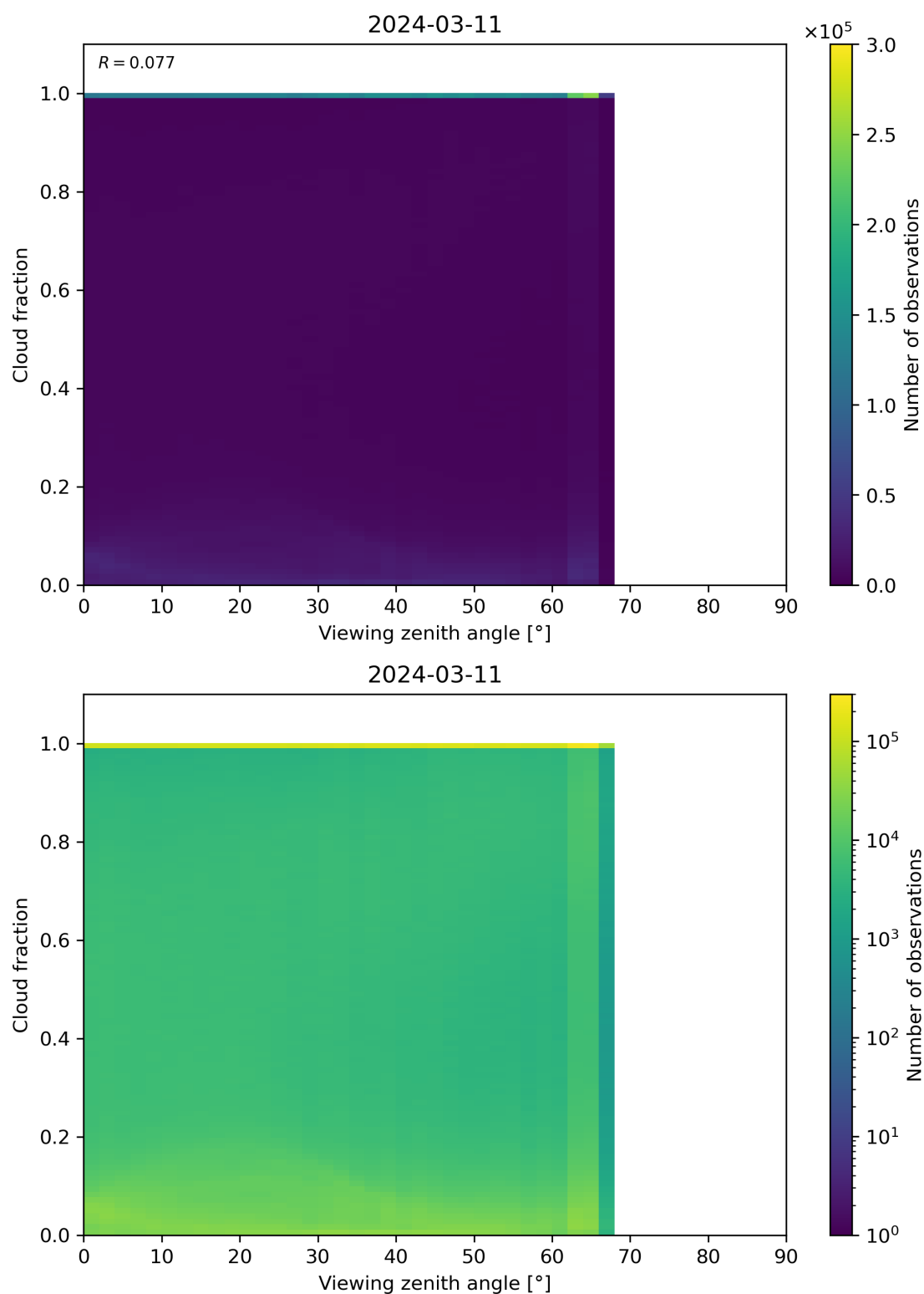
Figure 120: Scatter density plot of “Viewing zenith angle” against “Cloud fraction” for 2024-03-10 to 2024-03-12.
