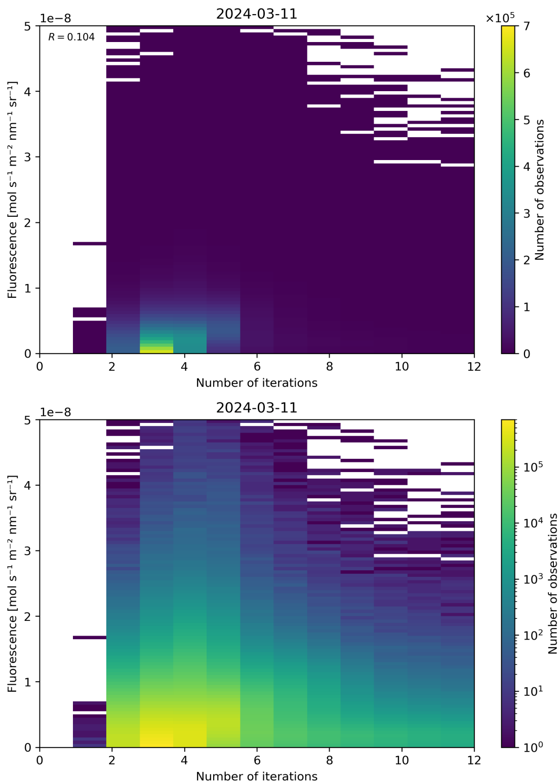
Figure 98: Scatter density plot of “Number of iterations” against “Fluorescence” for 2024-03-10 to 2024-03-12.
