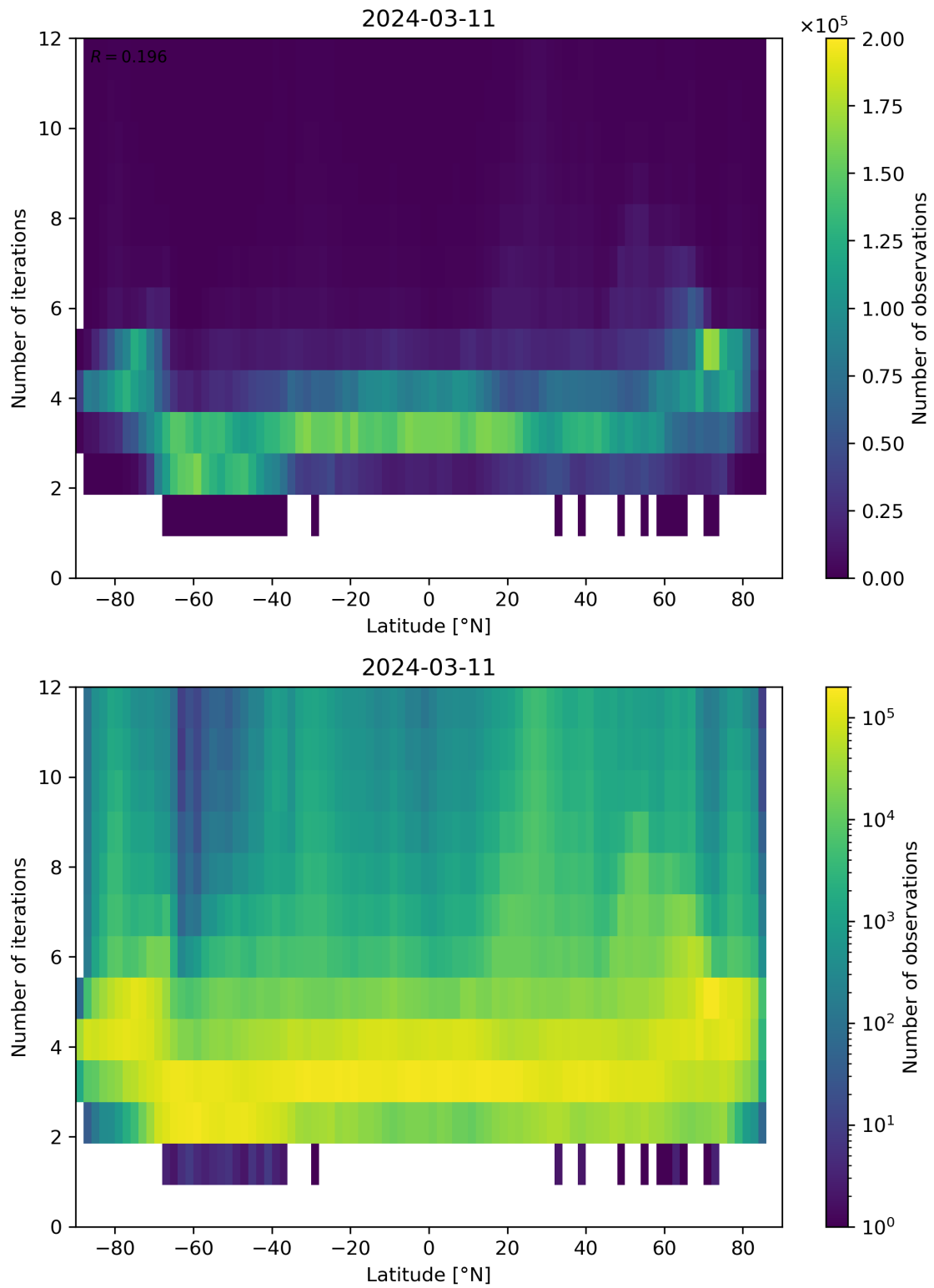
Figure 93: Scatter density plot of “Latitude” against “Number of iterations” for 2024-03-10 to 2024-03-12.
