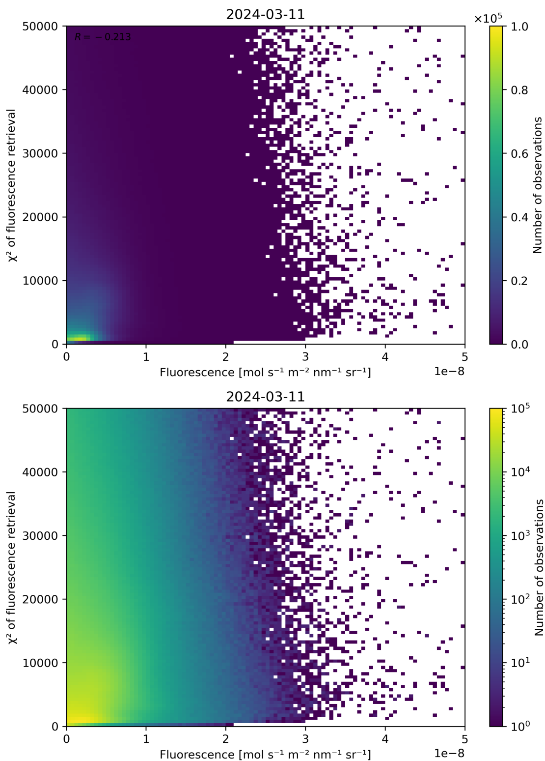
Figure 85: Scatter density plot of “Fluorescence” against “ \chi^2 of fluorescence retrieval” for 2024-03-10 to 2024-03-12.
