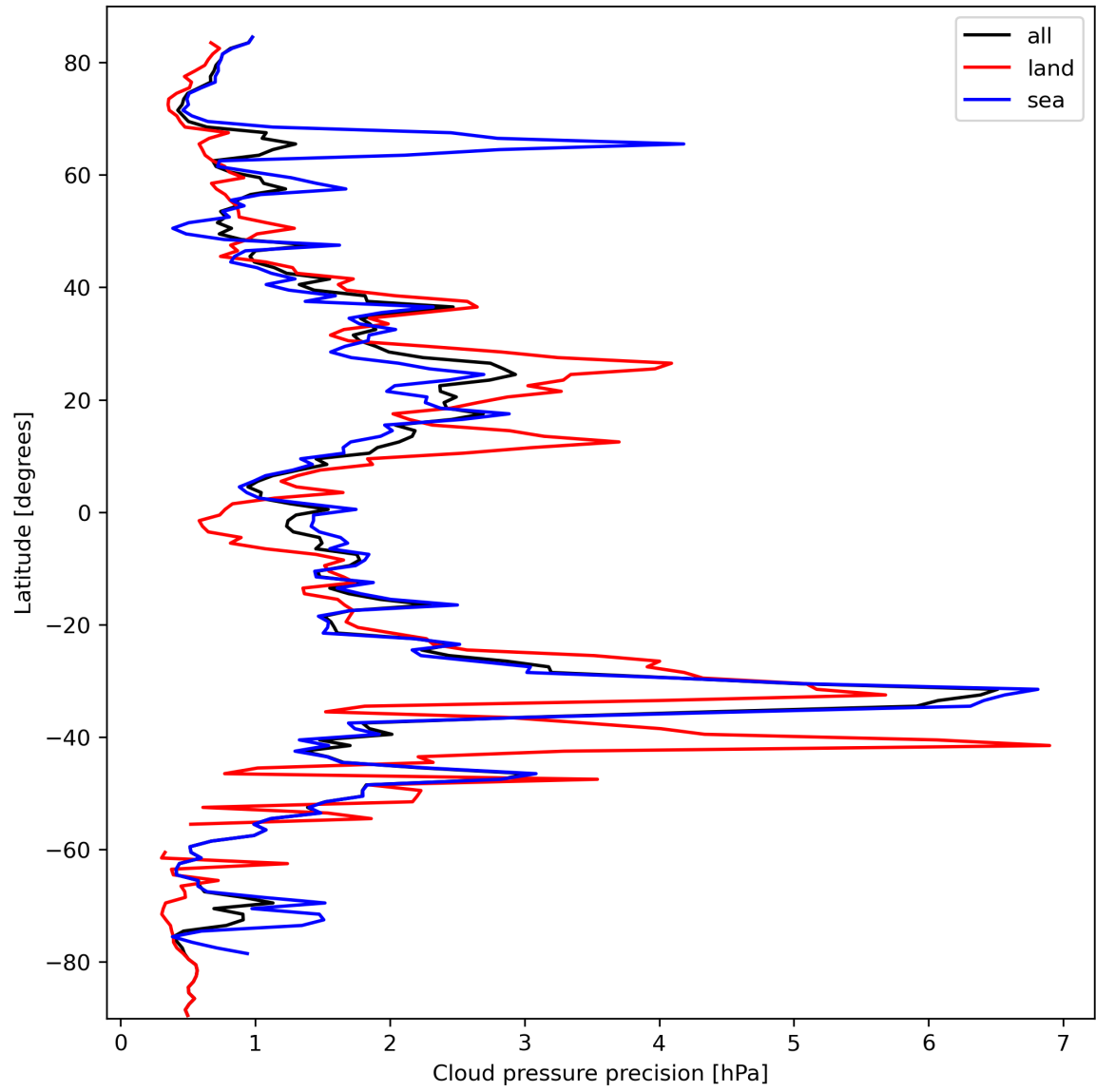
Figure 14: Zonal average of “Cloud pressure precision” for 2024-03-10 to 2024-03-12.
