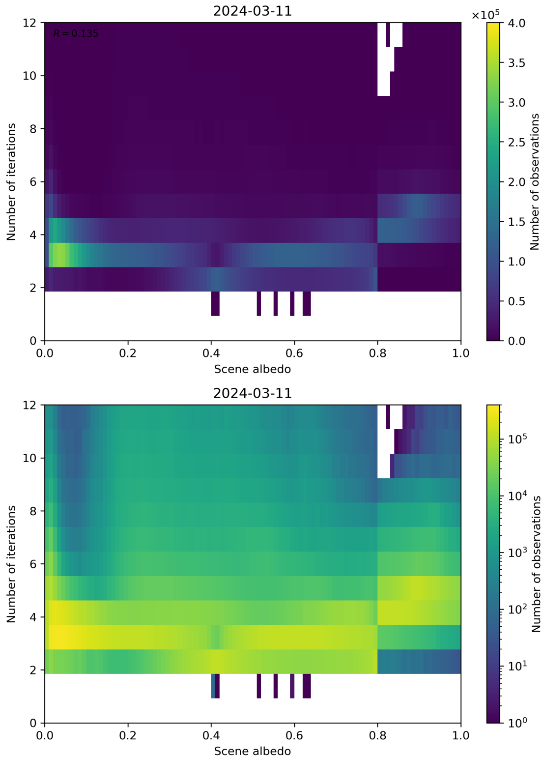
Figure 105: Scatter density plot of “Scene albedo” against “Number of iterations” for 2024-03-10 to 2024-03-12.
