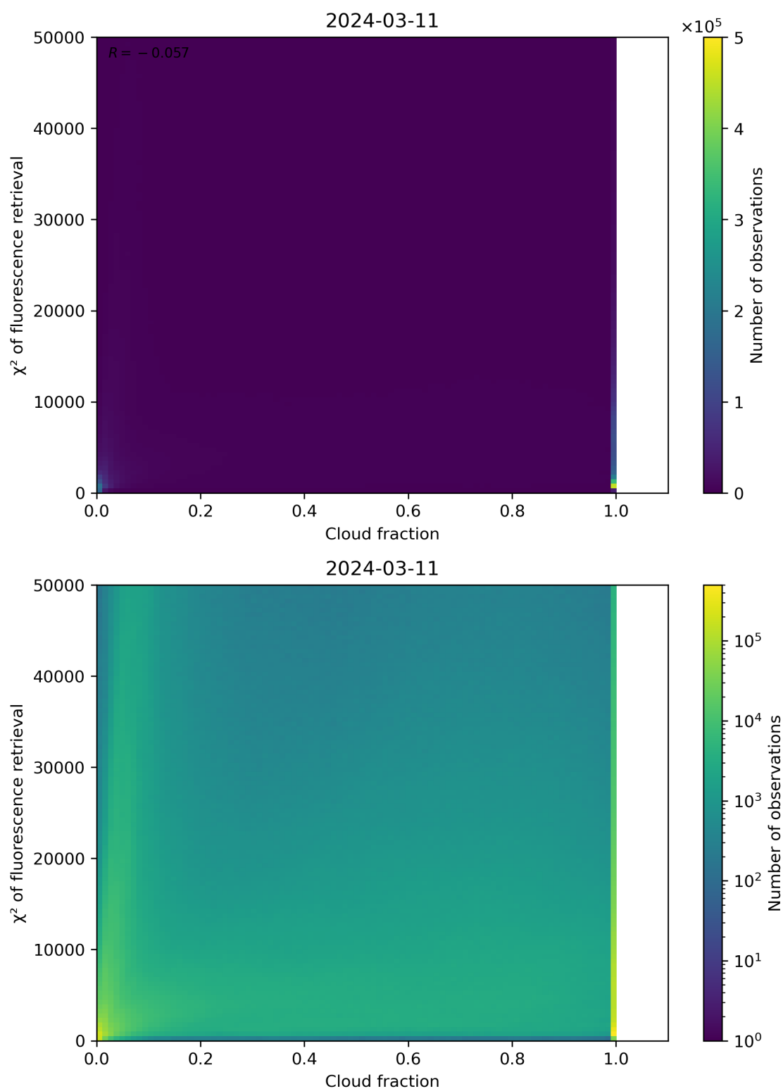
Figure 71: Scatter density plot of “Cloud fraction” against “ \chi^2 of fluorescence retrieval” for 2024-03-10 to 2024-03-12.
