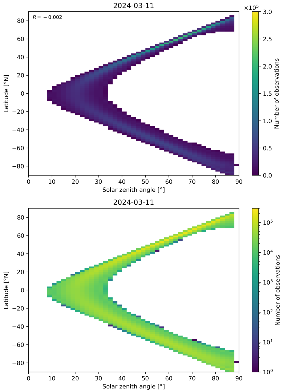
Figure 113: Scatter density plot of “Solar zenith angle” against “Latitude” for 2024-03-10 to 2024-03-12.
