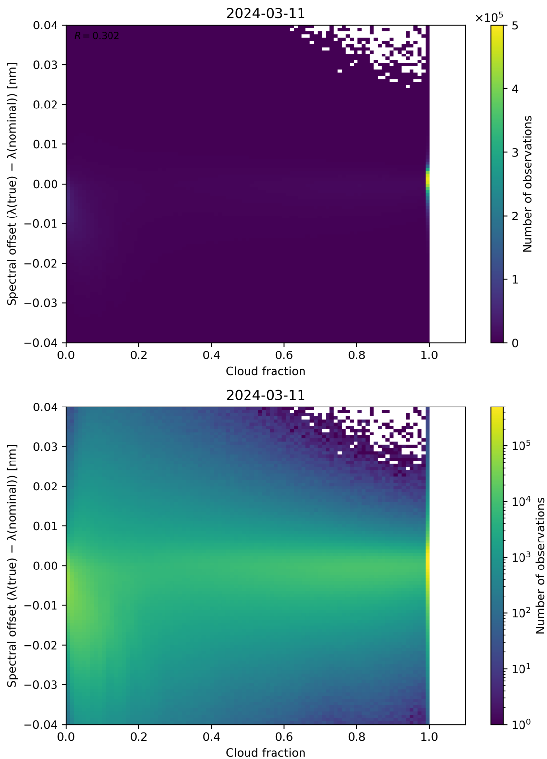
Figure 76: Scatter density plot of “Cloud fraction” against “Spectral offset ( \lambda(\text{true}) - \lambda(\text{nominal}) )” for 2024-03-10 to 2024-03-12.
