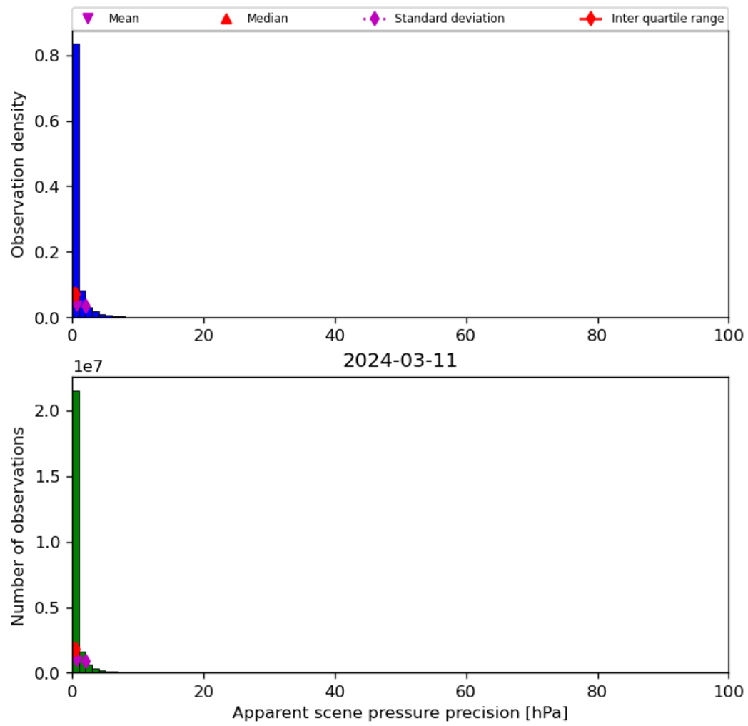
Figure 37: Histogram of “Apparent scene pressure precision” for 2024-03-10 to 2024-03-12
