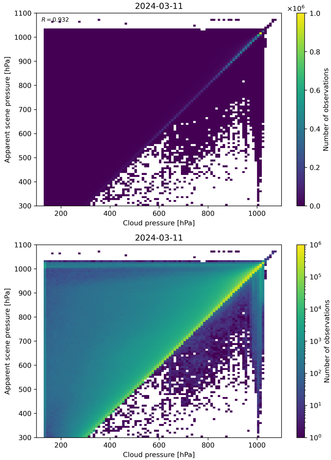
Figure 77: Scatter density plot of “Cloud pressure” against “Apparent scene pressure” for 2024-03-10 to 2024-03-12.
