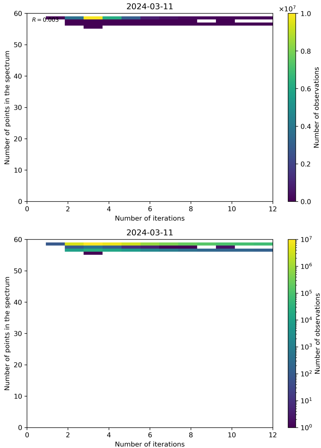
Figure 99: Scatter density plot of “Number of iterations” against “Number of points in the spectrum” for 2024-03-10 to 2024-03-12.
