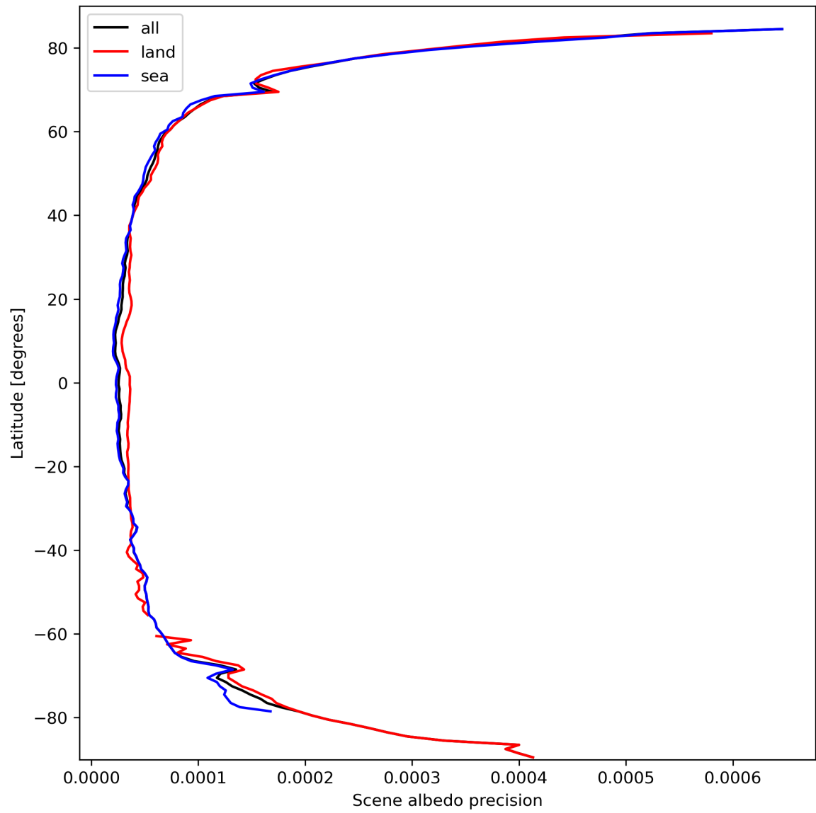
Figure 18: Zonal average of “Scene albedo precision” for 2024-03-10 to 2024-03-12.
