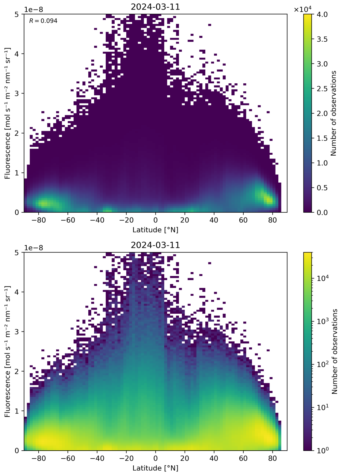
Figure 92: Scatter density plot of “Latitude” against “Fluorescence” for 2024-03-10 to 2024-03-12.
