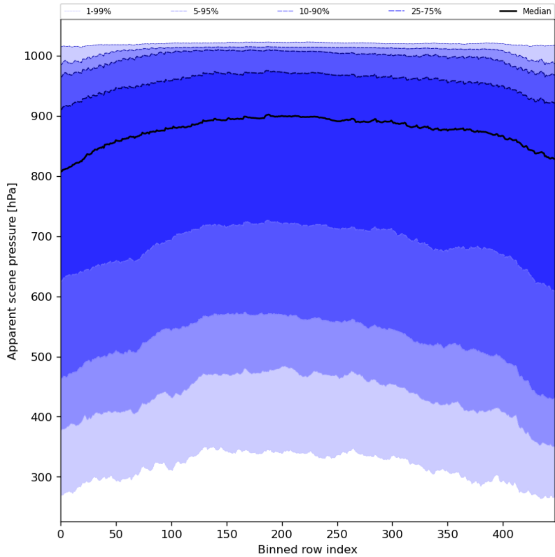
Figure 53: Along track statistics of “Apparent scene pressure” for 2024-03-10 to 2024-03-12
