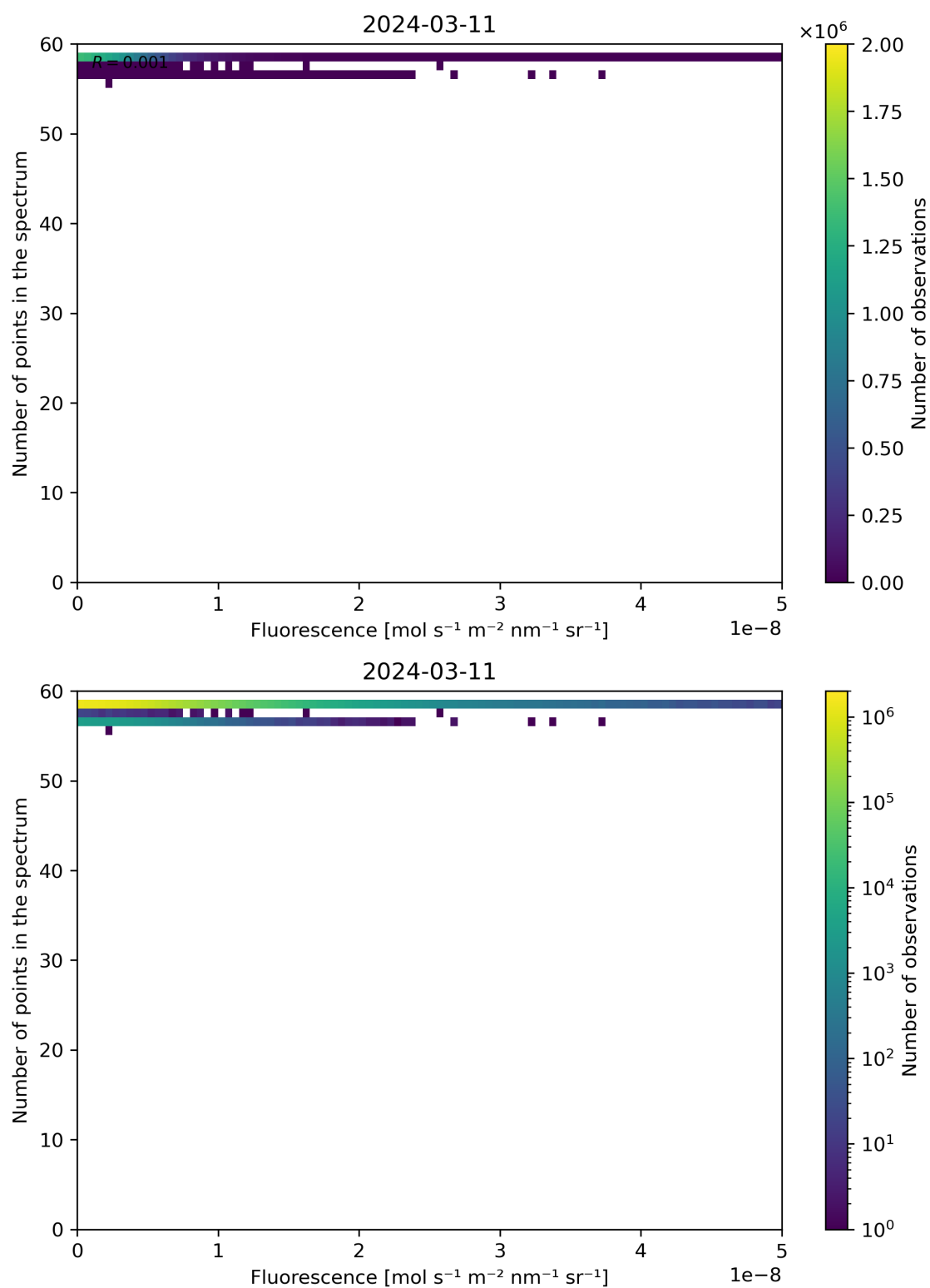
Figure 86: Scatter density plot of “Fluorescence” against “Number of points in the spectrum” for 2024-03-10 to 2024-03-12.
