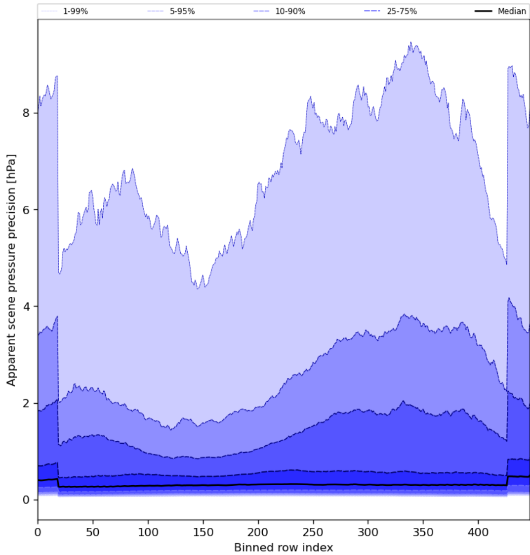
Figure 54: Along track statistics of “Apparent scene pressure precision” for 2024-03-10 to 2024-03-12
