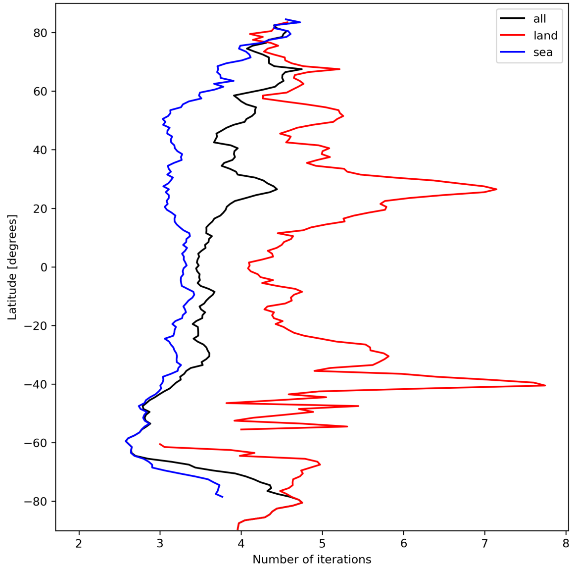
Figure 22: Zonal average of “Number of iterations” for 2024-03-10 to 2024-03-12.
