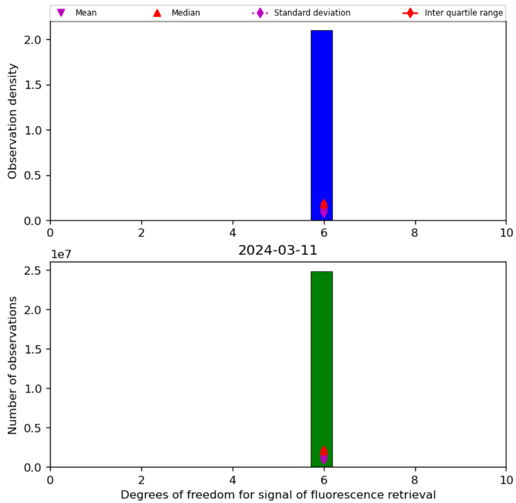
Figure 43: Histogram of “Degrees of freedom for signal of fluorescence retrieval” for 2024-03-10 to 2024-03-12
