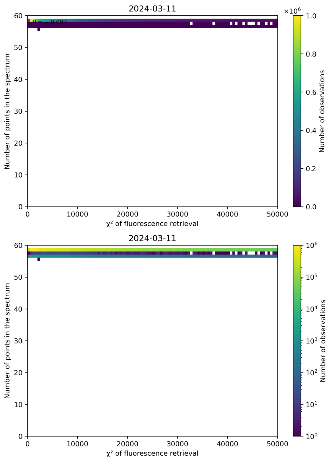
Figure 68: Scatter density plot of " \chi^2 of fluorescence retrieval" against "Number of points in the spectrum" for 2024-03-10 to 2024-03-12.
