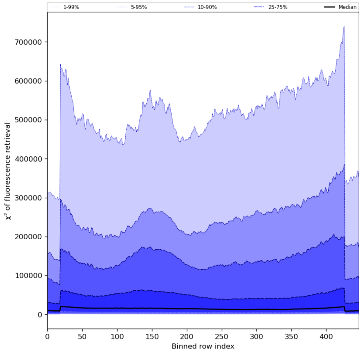
Figure 59: Along track statistics of “ \chi^2 of fluorescence retrieval” for 2024-03-10 to 2024-03-12
