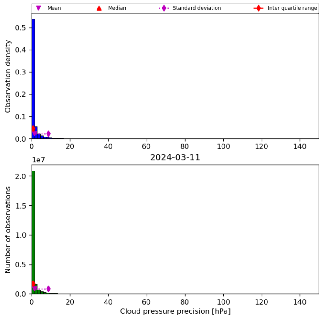
Figure 31: Histogram of “Cloud pressure precision” for 2024-03-10 to 2024-03-12
