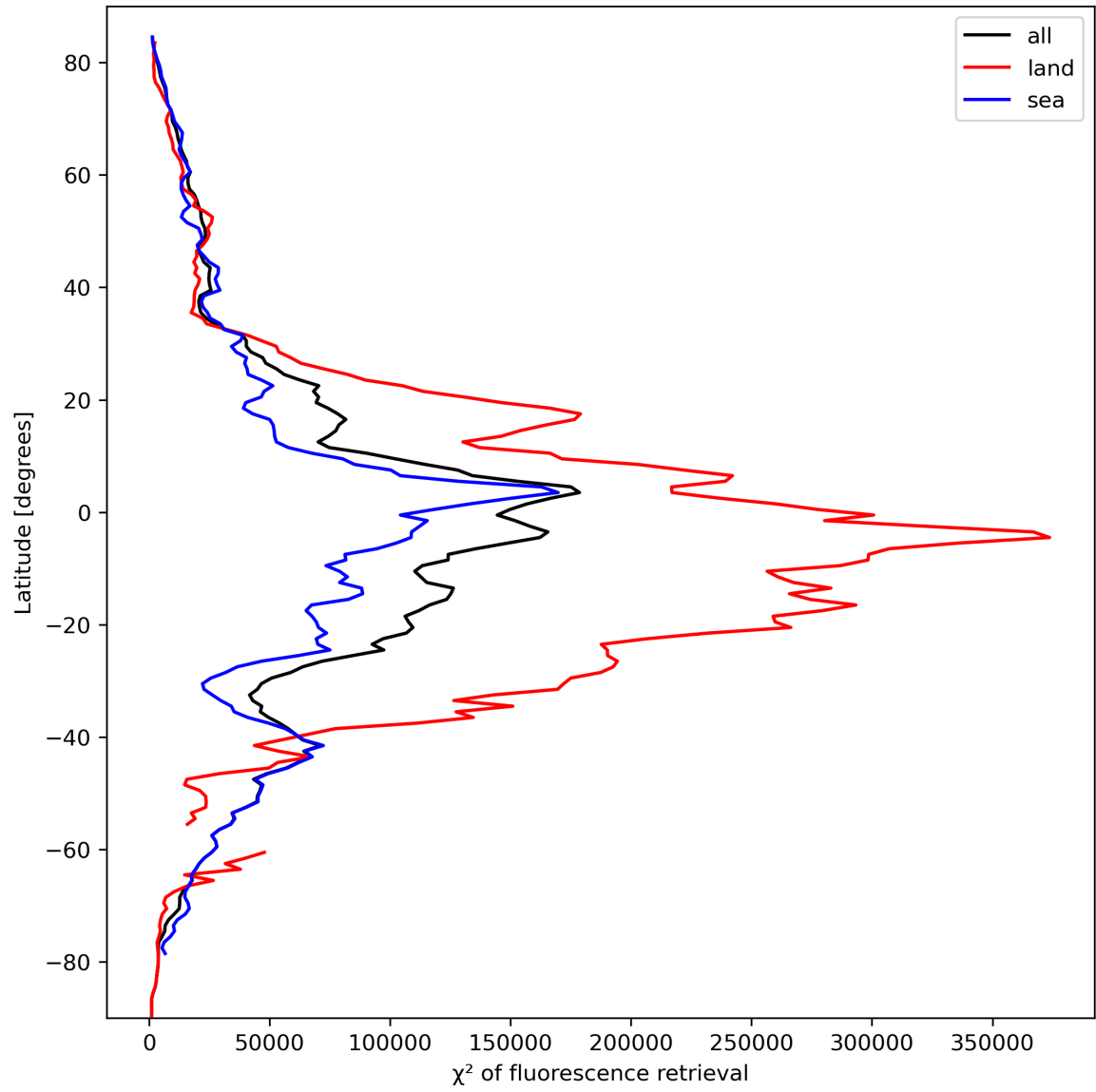
Figure 25: Zonal average of “ \chi^2 of fluorescence retrieval” for 2024-03-10 to 2024-03-12.
