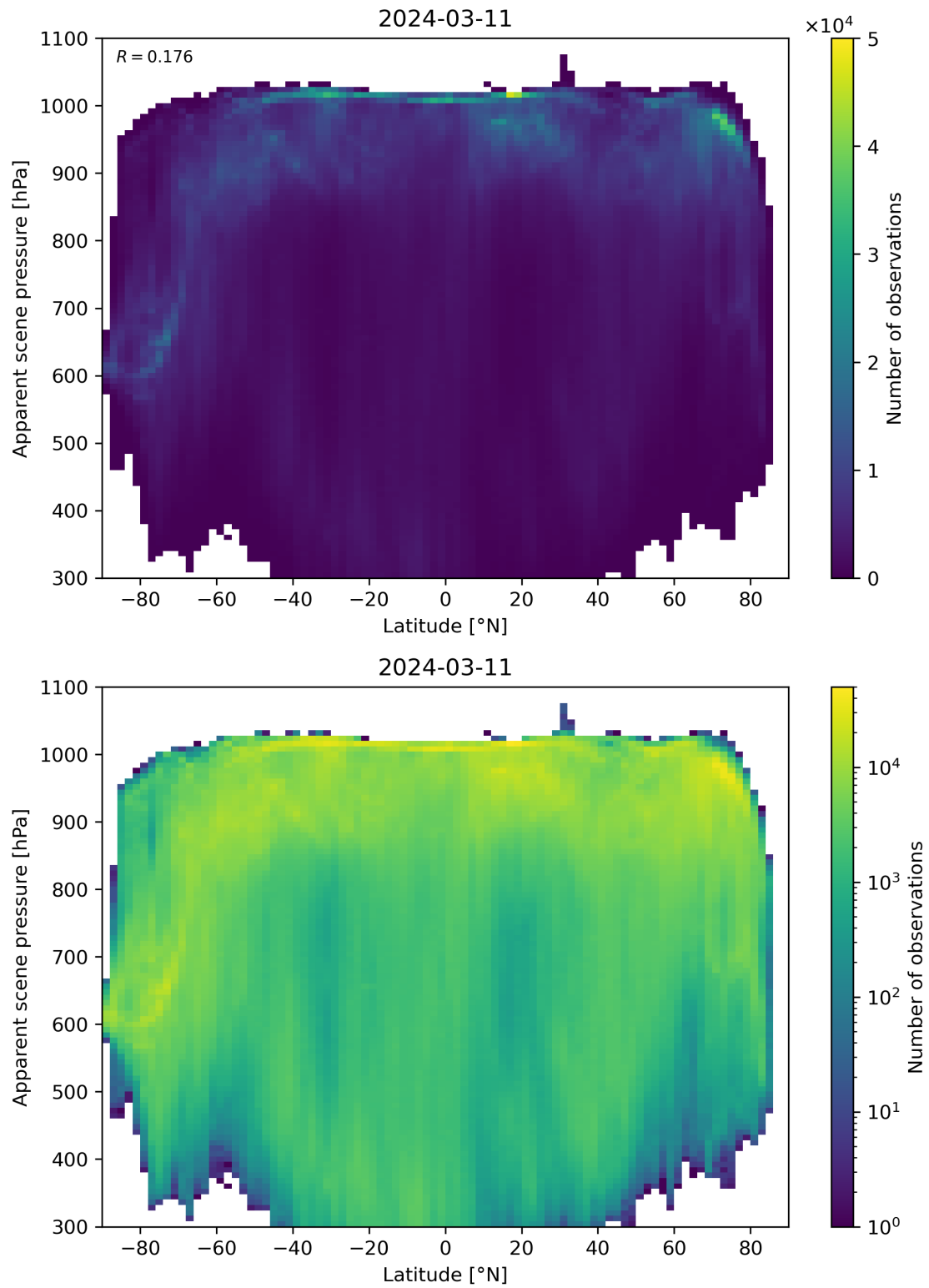
Figure 88: Scatter density plot of “Latitude” against “Apparent scene pressure” for 2024-03-10 to 2024-03-12.
