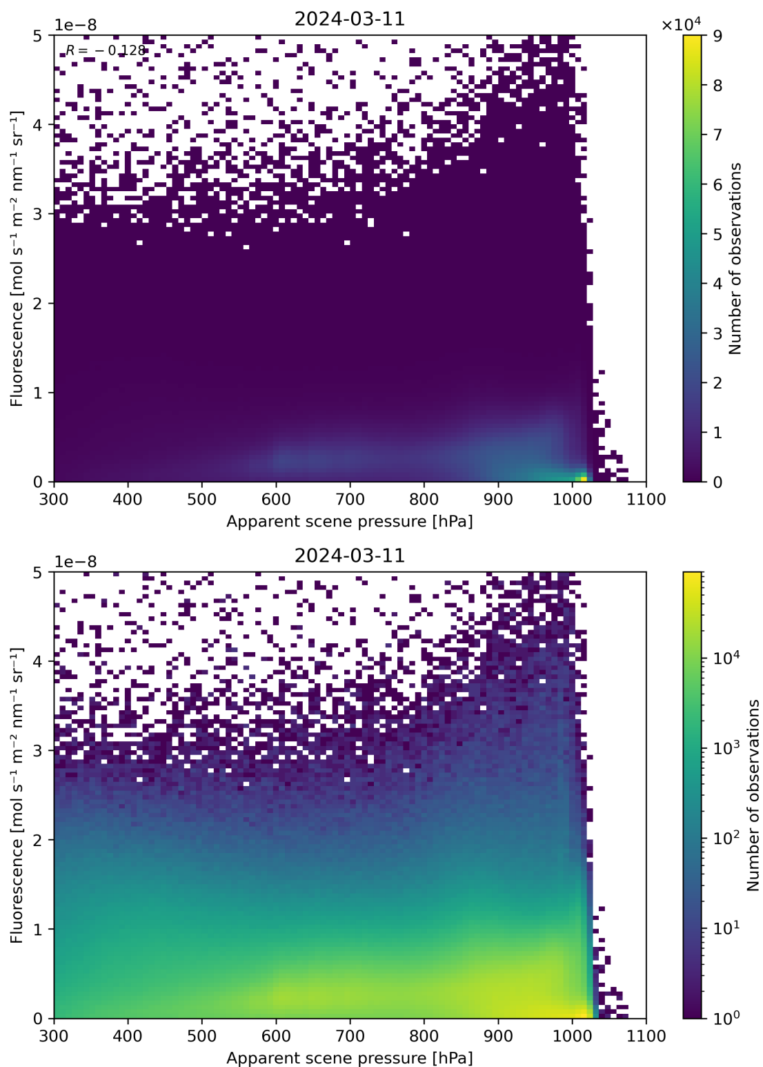
Figure 64: Scatter density plot of “Apparent scene pressure” against “Fluorescence” for 2024-03-10 to 2024-03-12.
