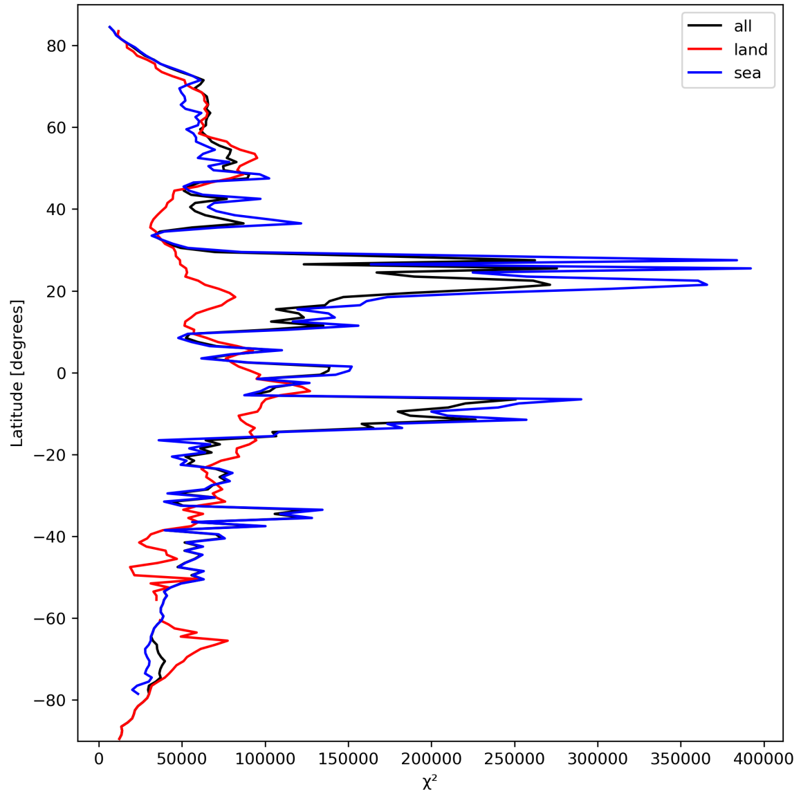
Figure 21: Zonal average of “ \chi^2 ” for 2024-03-10 to 2024-03-12.
