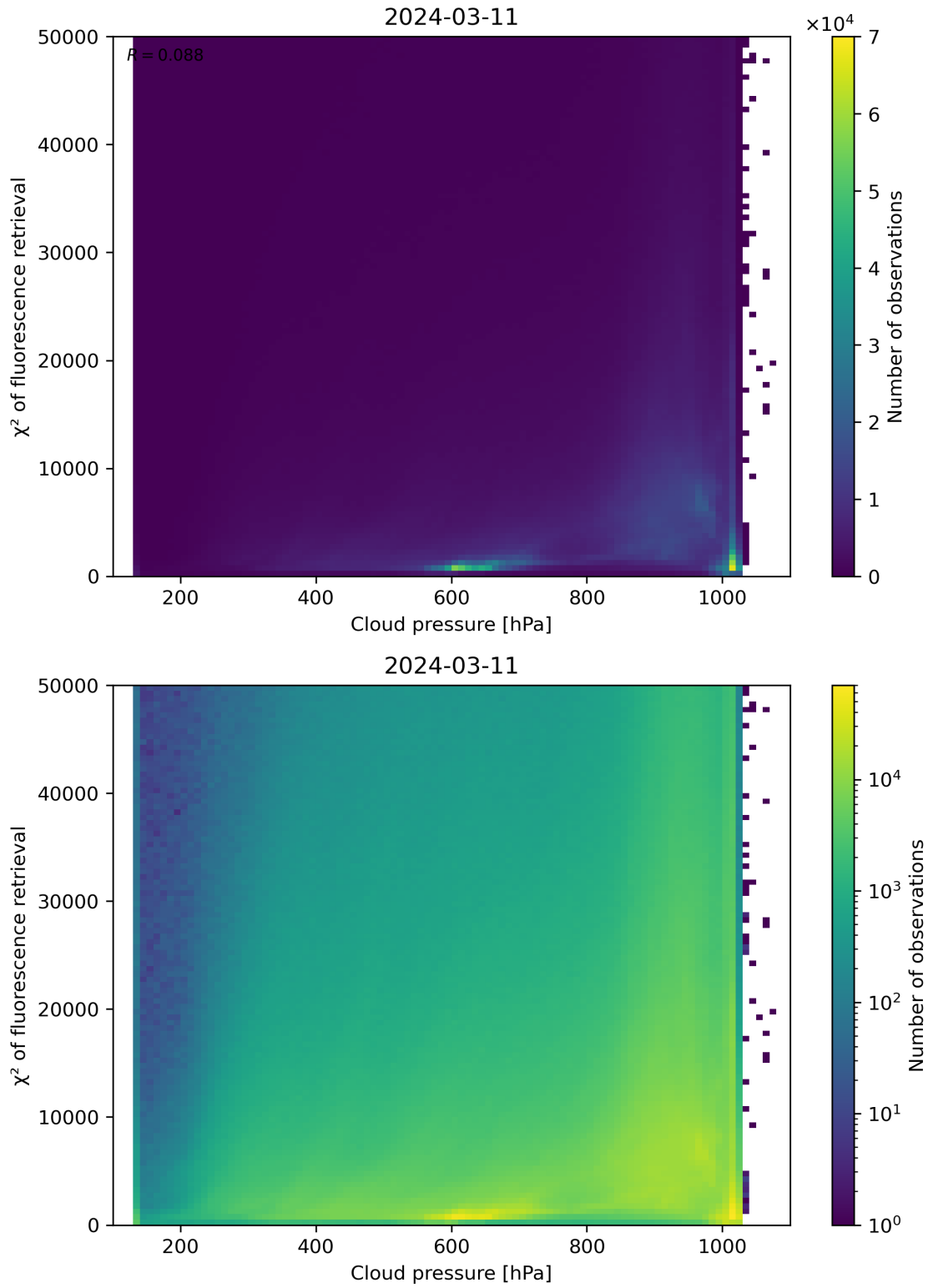
Figure 78: Scatter density plot of “Cloud pressure” against “ \chi^2 of fluorescence retrieval” for 2024-03-10 to 2024-03-12.
