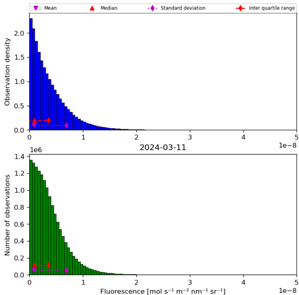
Figure 40: Histogram of “Fluorescence” for 2024-03-10 to 2024-03-12
