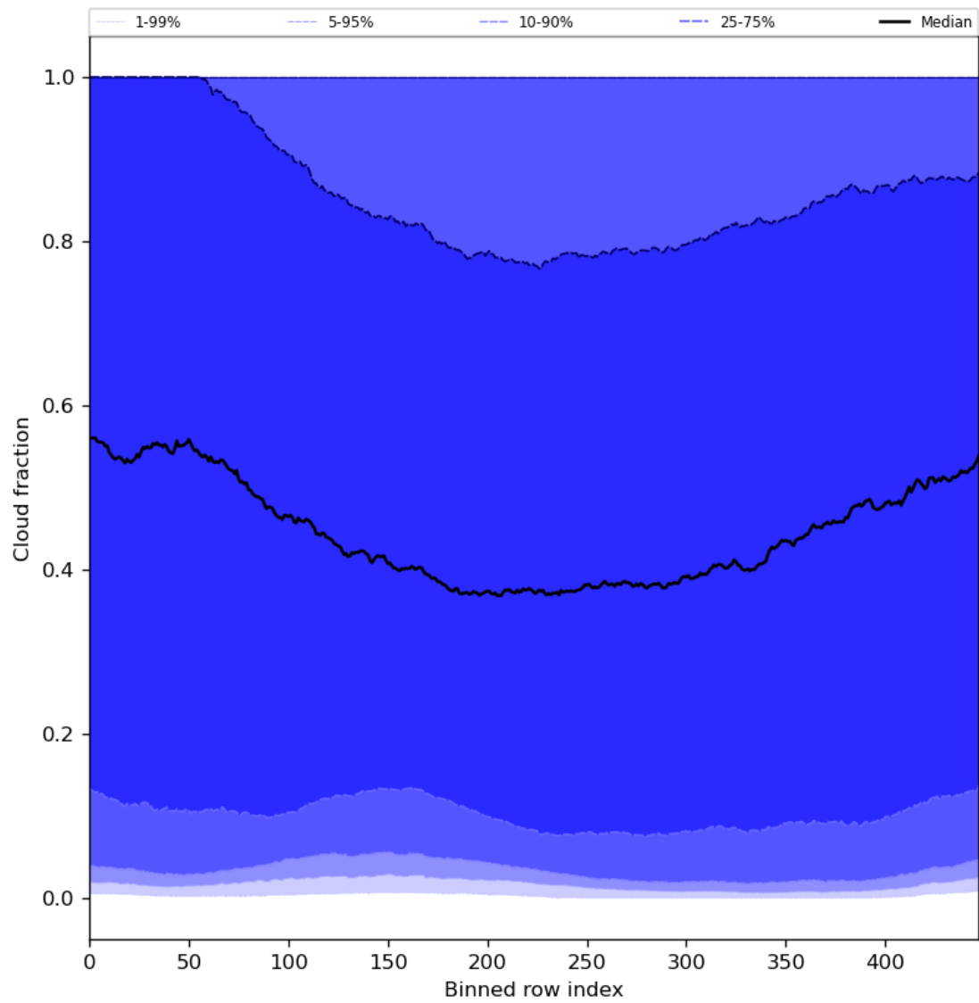
Figure 49: Along track statistics of “Cloud fraction” for 2024-03-10 to 2024-03-12
