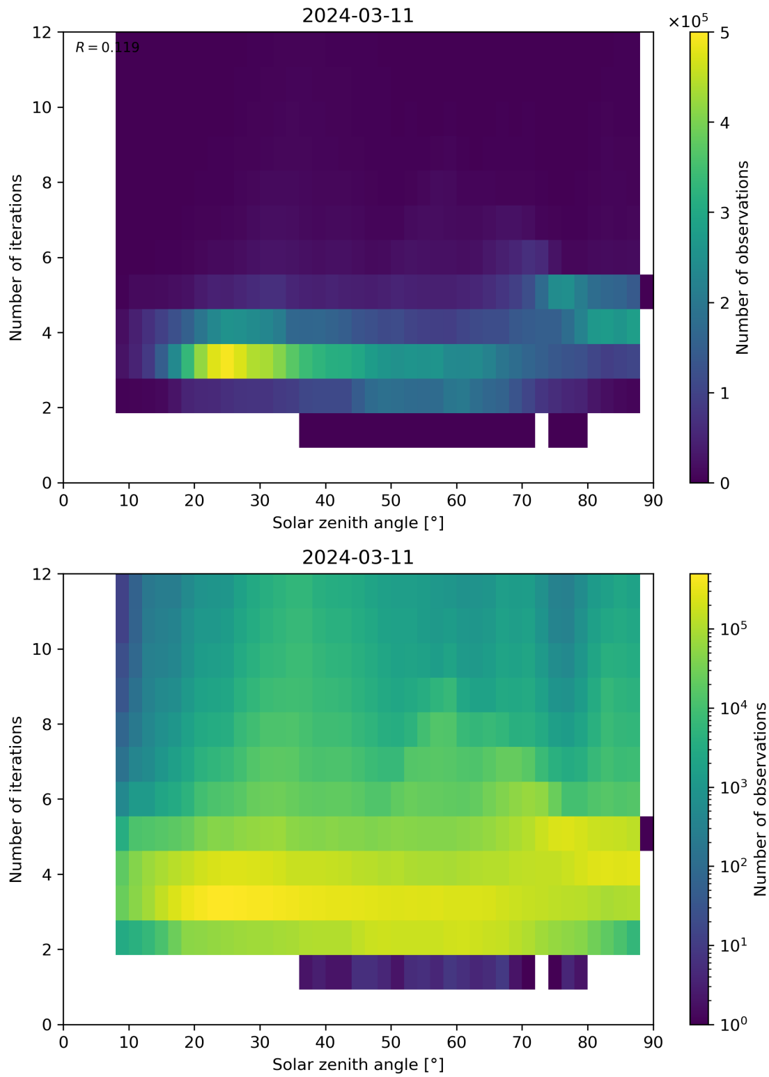
Figure 114: Scatter density plot of “Solar zenith angle” against “Number of iterations” for 2024-03-10 to 2024-03-12.
