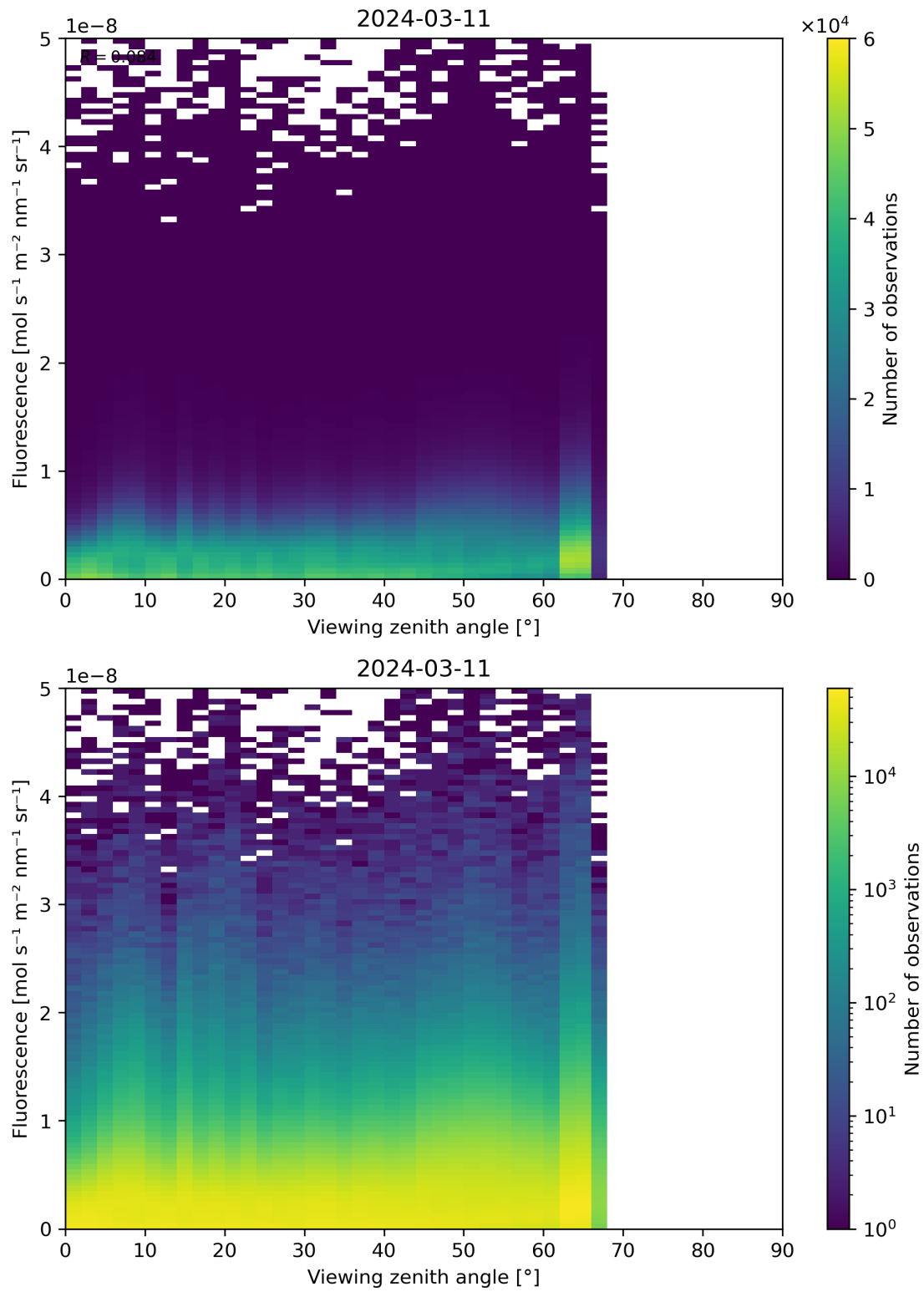
Figure 122: Scatter density plot of “Viewing zenith angle” against “Fluorescence” for 2024-03-10 to 2024-03-12.
