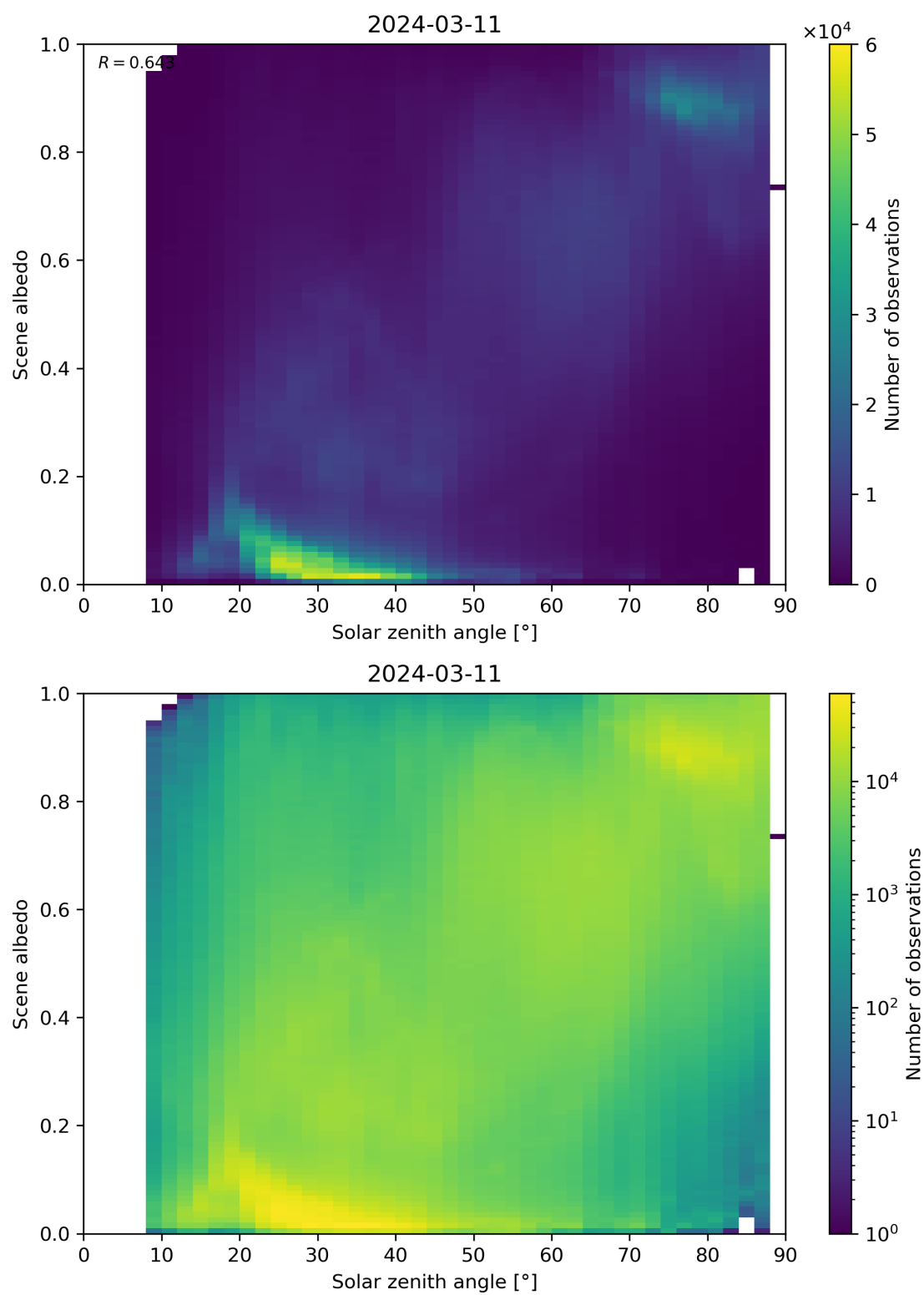
Figure 116: Scatter density plot of “Solar zenith angle” against “Scene albedo” for 2024-03-10 to 2024-03-12.
