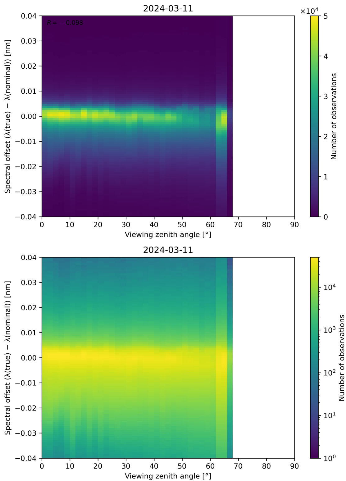
Figure 128: Scatter density plot of “Viewing zenith angle” against “Spectral offset ( \lambda(\text{true}) - \lambda(\text{nominal}) )” for 2024-03-10 to 2024-03-12.
