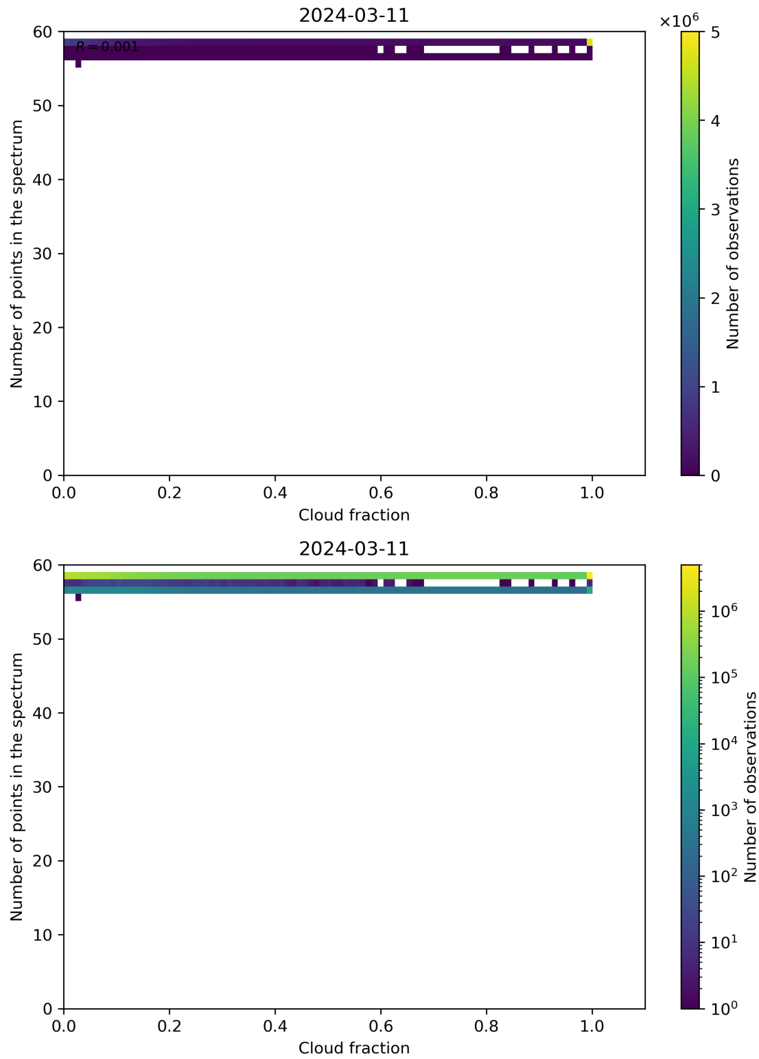
Figure 74: Scatter density plot of “Cloud fraction” against “Number of points in the spectrum” for 2024-03-10 to 2024-03-12.
