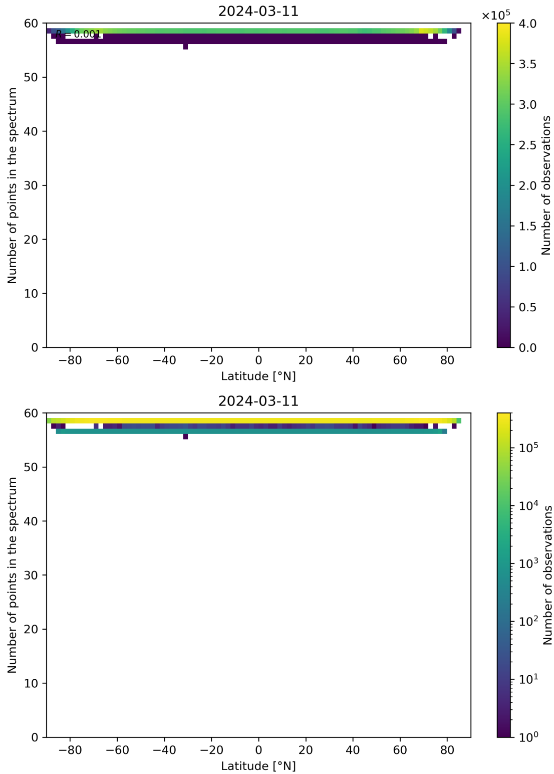
Figure 94: Scatter density plot of “Latitude” against “Number of points in the spectrum” for 2024-03-10 to 2024-03-12.
