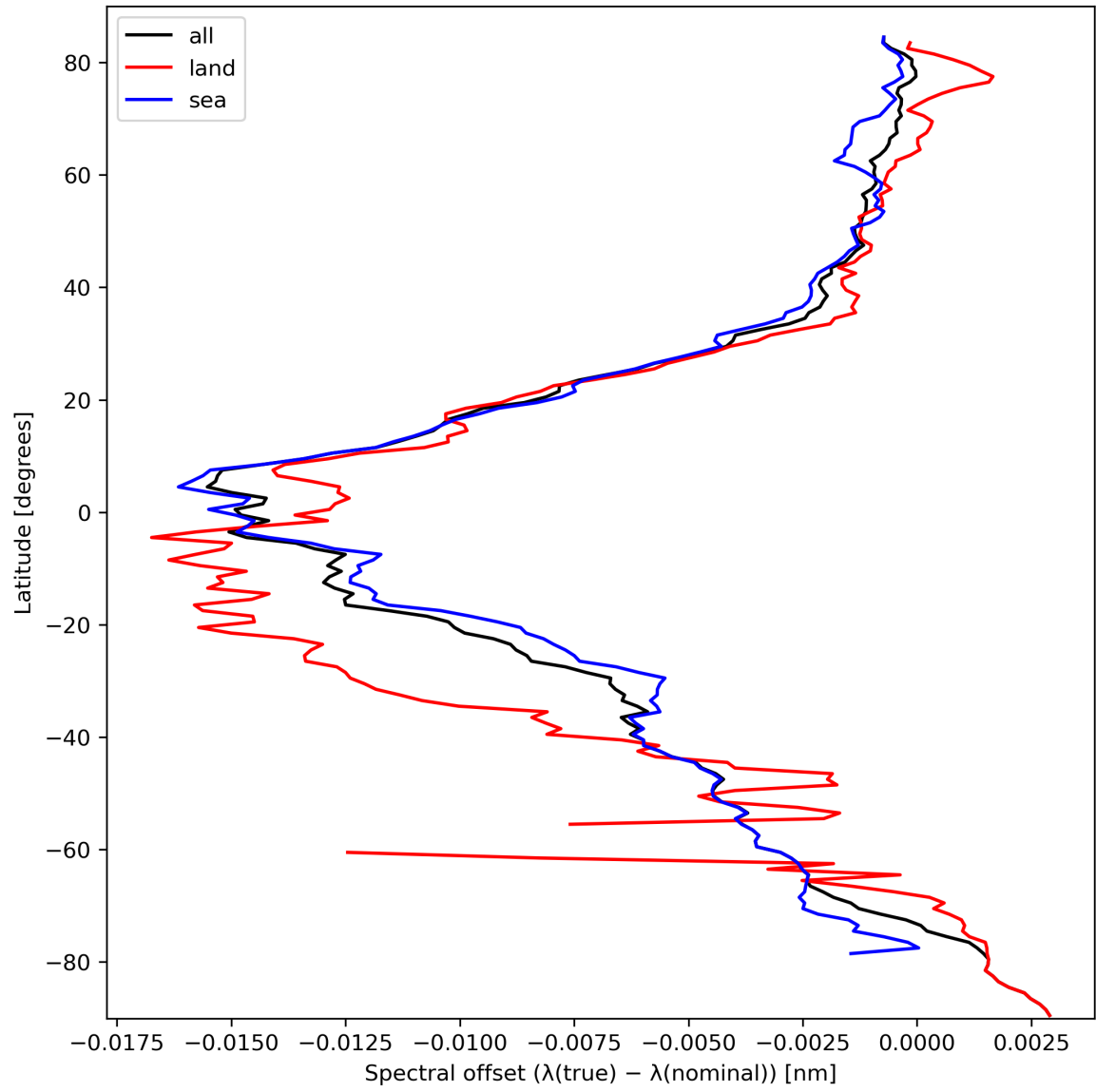
Figure 28: Zonal average of “Spectral offset ( \lambda(\text{true}) - \lambda(\text{nominal}) )” for 2024-03-10 to 2024-03-12.
