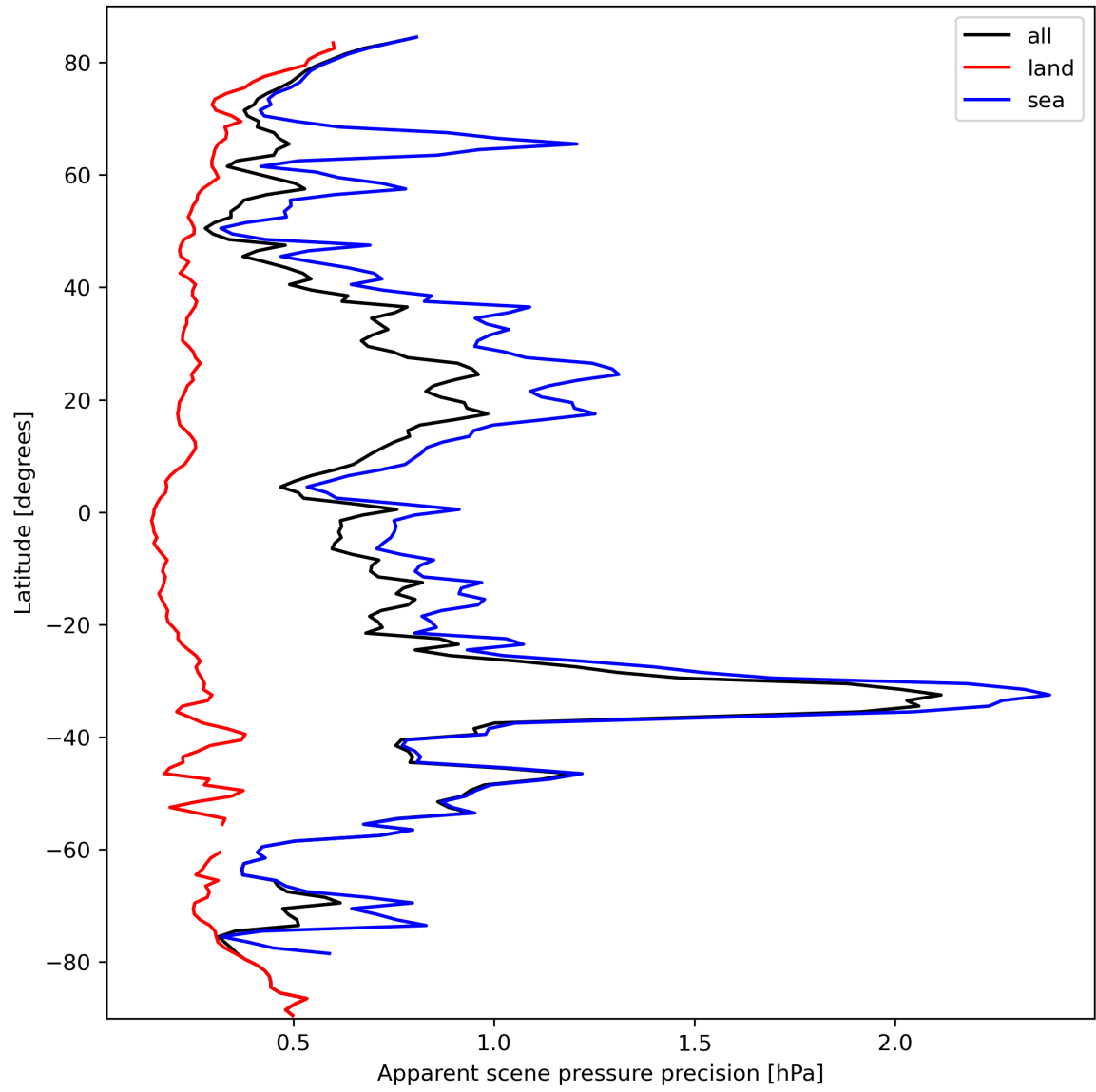
Figure 20: Zonal average of “Apparent scene pressure precision” for 2024-03-10 to 2024-03-12.
