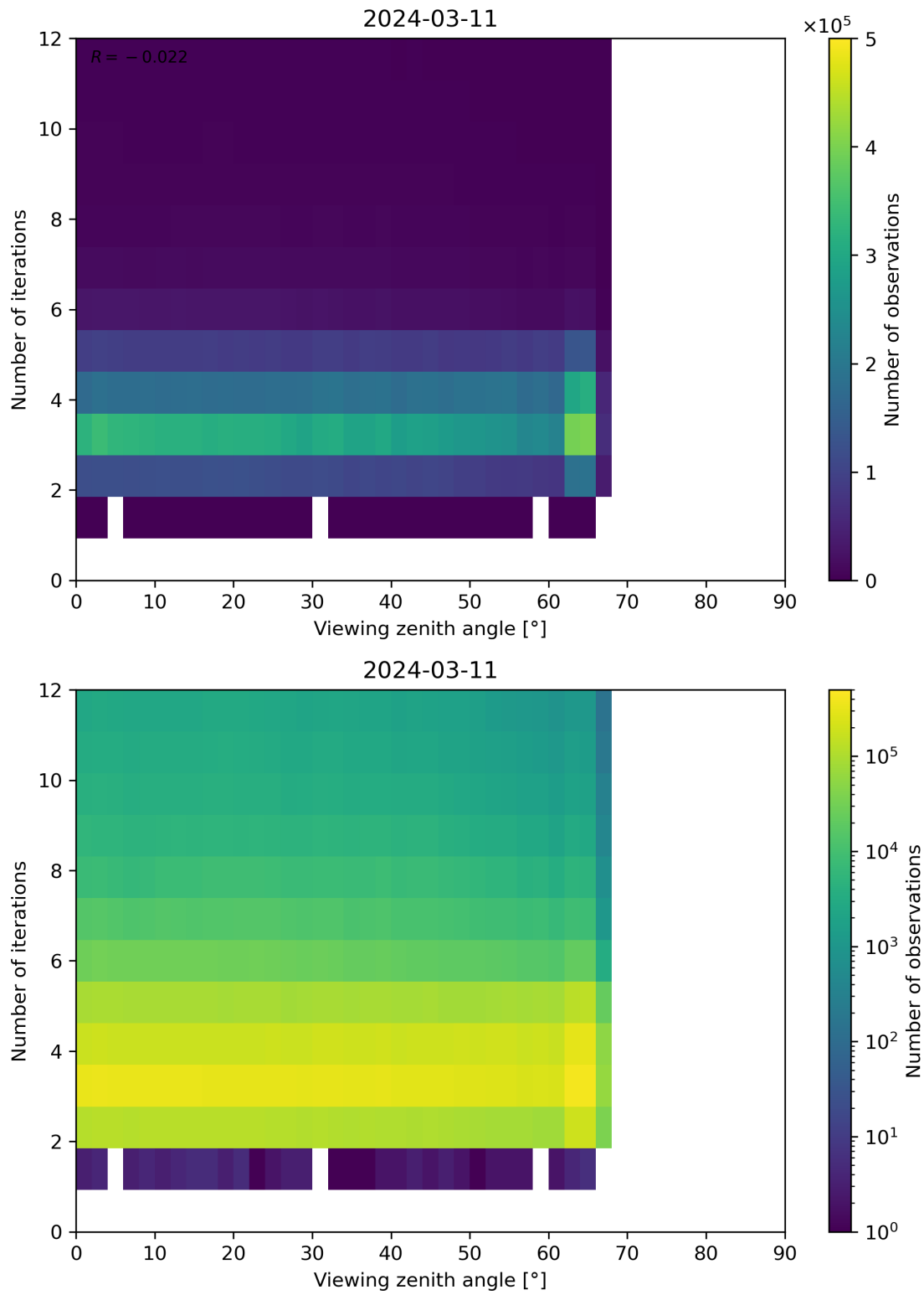
Figure 124: Scatter density plot of “Viewing zenith angle” against “Number of iterations” for 2024-03-10 to 2024-03-12.
