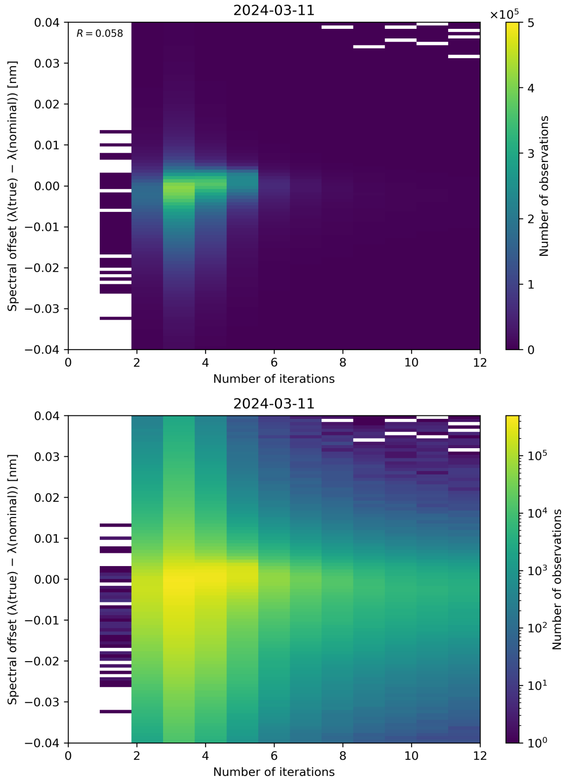
Figure 100: Scatter density plot of “Number of iterations” against “Spectral offset ( \lambda(\text{true}) - \lambda(\text{nominal}) )” for 2024-03-10 to 2024-03-12.
