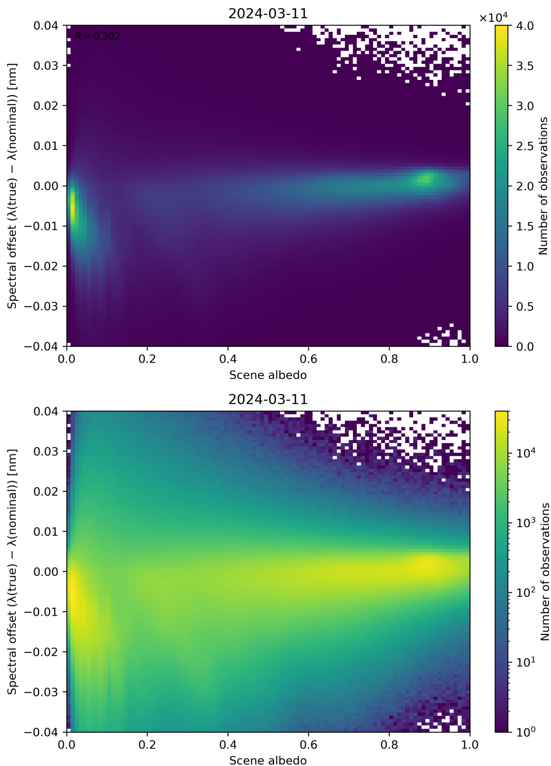
Figure 107: Scatter density plot of “Scene albedo” against “Spectral offset ( \lambda(\text{true}) - \lambda(\text{nominal}) )” for 2024-03-10 to 2024-03-12.
