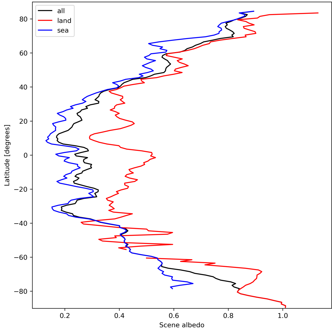
Figure 17: Zonal average of “Scene albedo” for 2024-03-10 to 2024-03-12.
