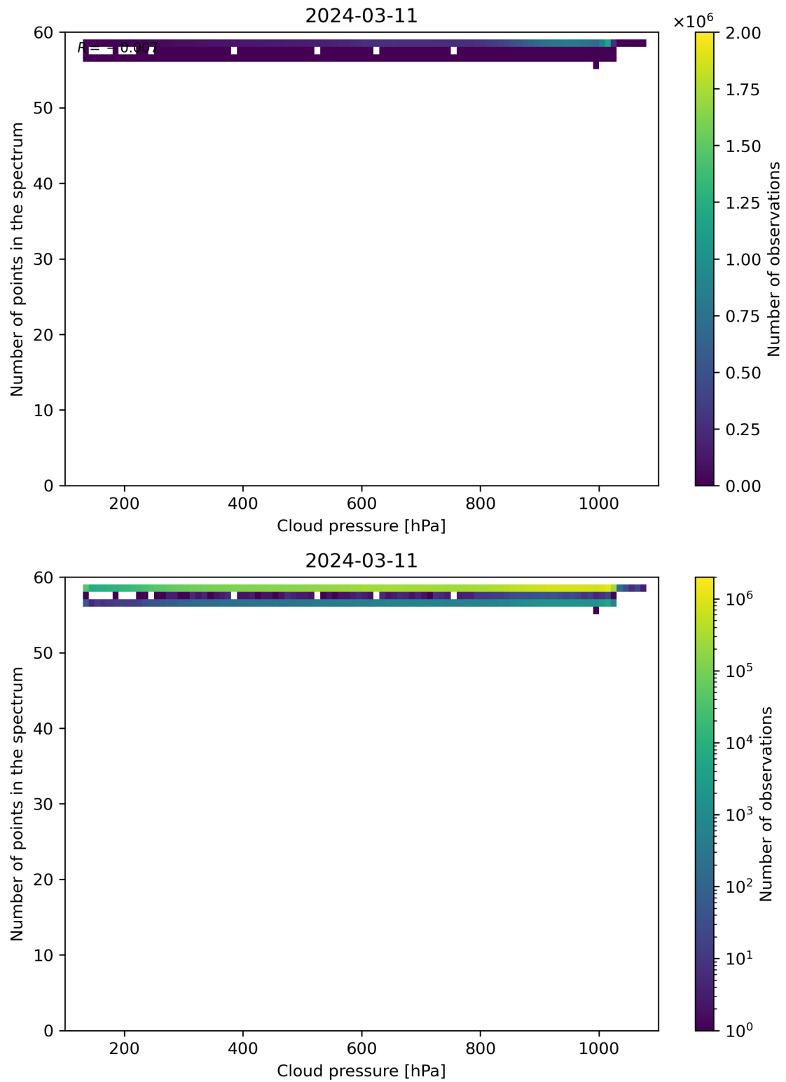
Figure 82: Scatter density plot of “Cloud pressure” against “Number of points in the spectrum” for 2024-03-10 to 2024-03-12.
