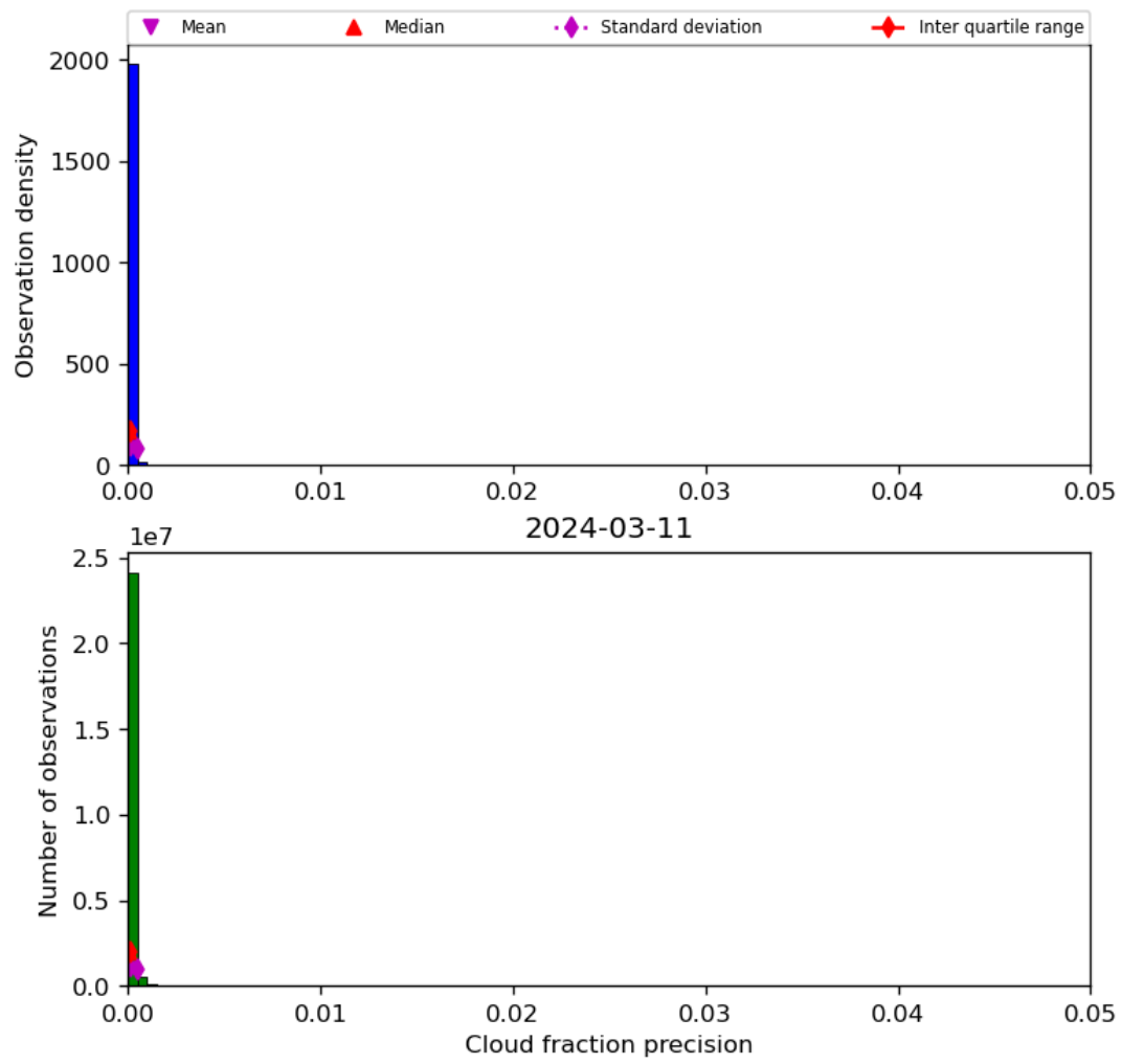
Figure 33: Histogram of “Cloud fraction precision” for 2024-03-10 to 2024-03-12
