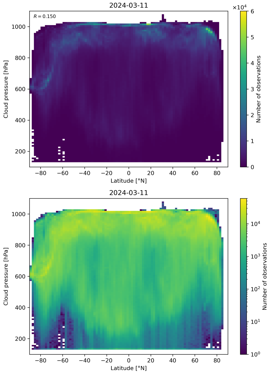
Figure 91: Scatter density plot of “Latitude” against “Cloud pressure” for 2024-03-10 to 2024-03-12.
