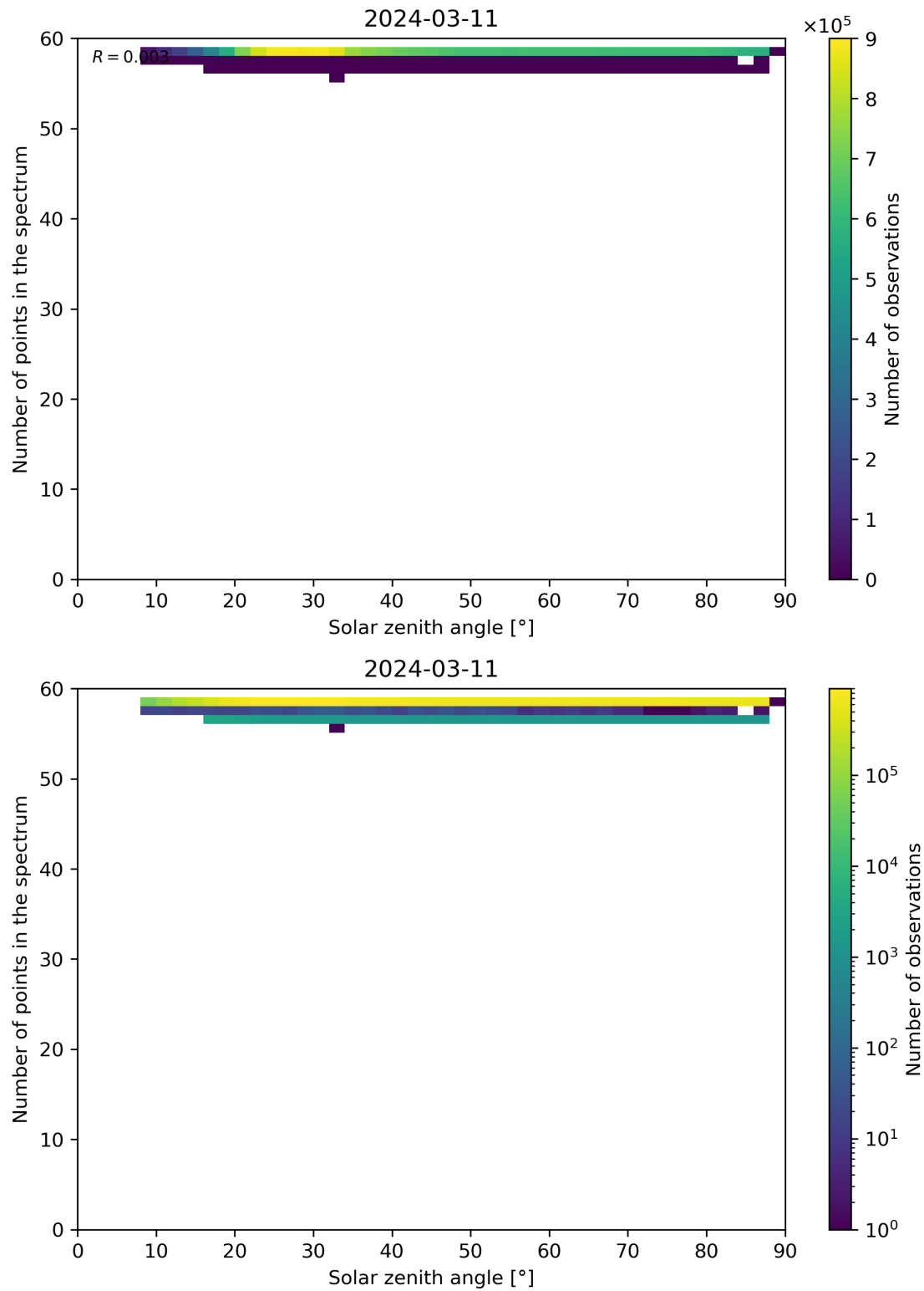
Figure 115: Scatter density plot of “Solar zenith angle” against “Number of points in the spectrum” for 2024-03-10 to 2024-03-12.
