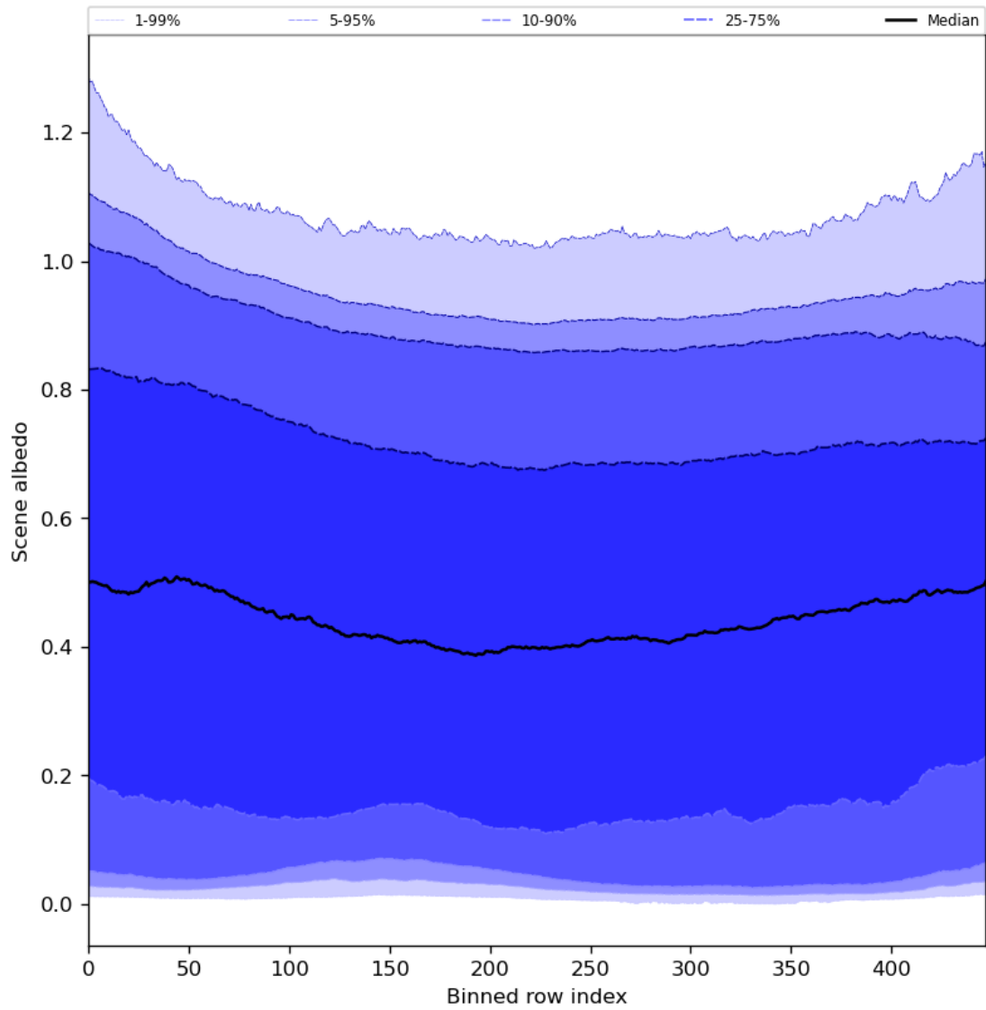
Figure 51: Along track statistics of “Scene albedo” for 2024-03-10 to 2024-03-12
