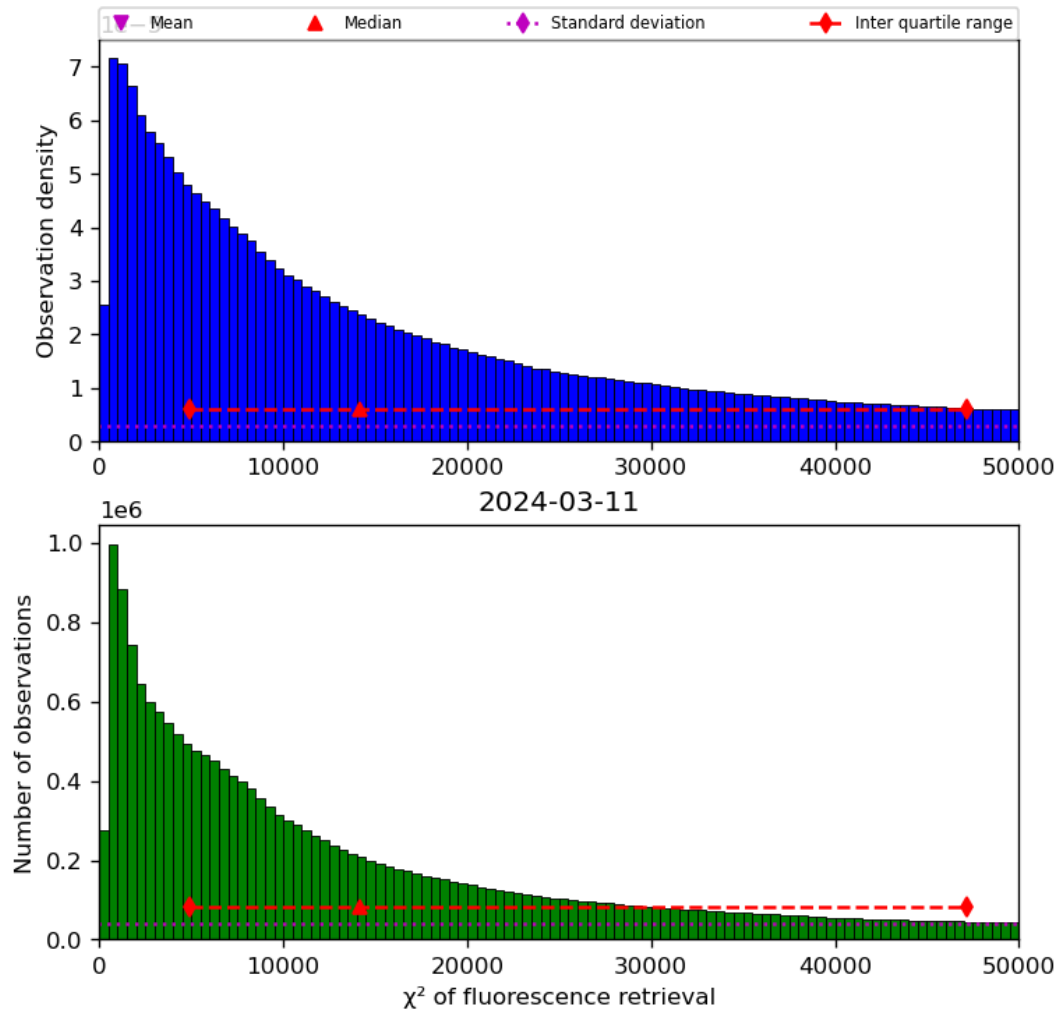
Figure 42: Histogram of “ \chi^2 of fluorescence retrieval” for 2024-03-10 to 2024-03-12
