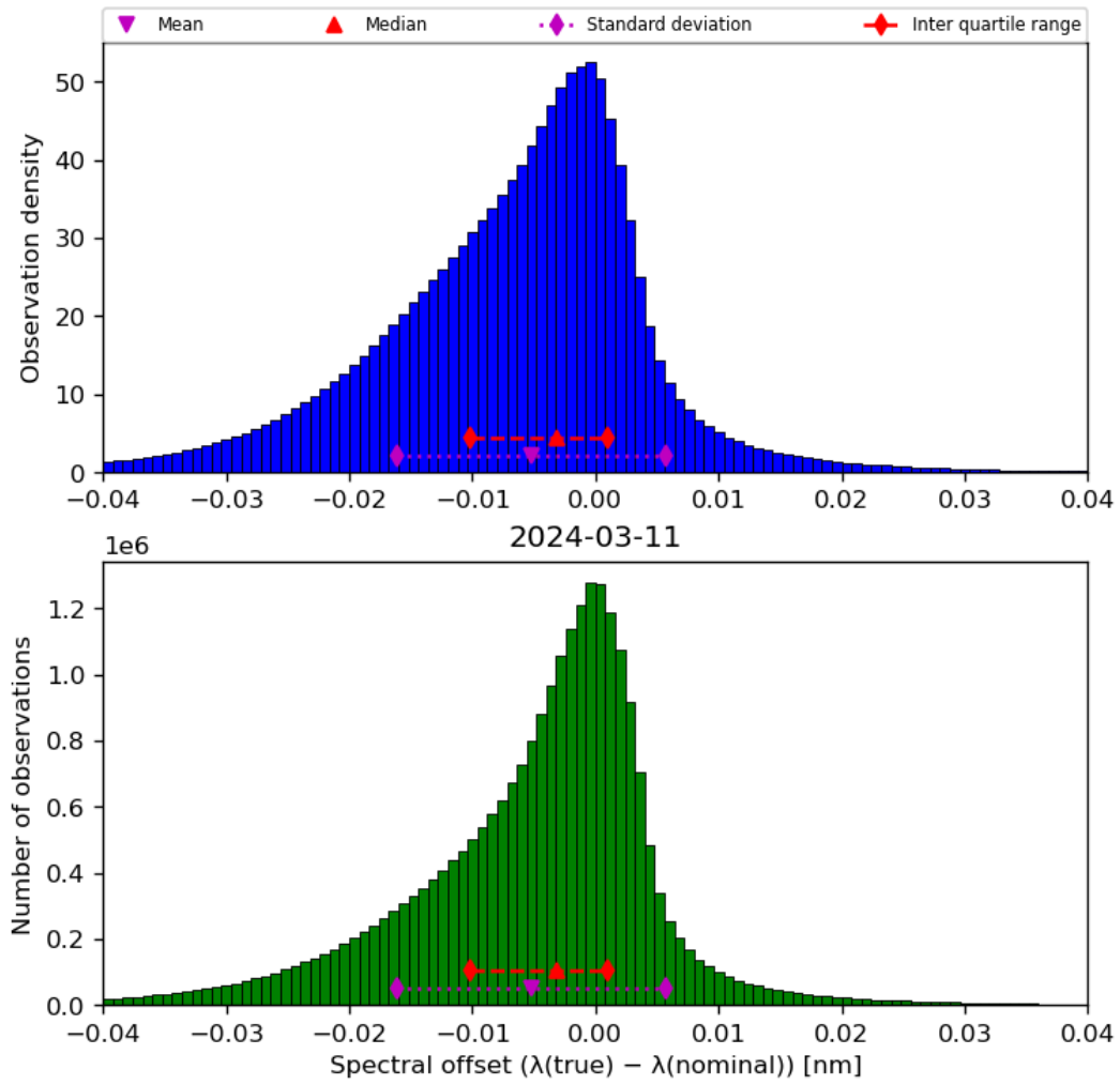
Figure 45: Histogram of “Spectral offset ( \lambda(\text{true}) - \lambda(\text{nominal}) )” for 2024-03-10 to 2024-03-12
