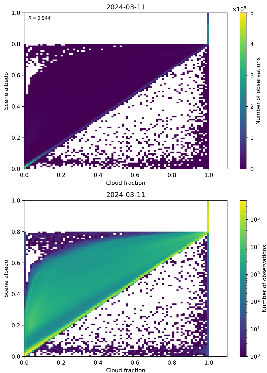
Figure 75: Scatter density plot of “Cloud fraction” against “Scene albedo” for 2024-03-10 to 2024-03-12.
