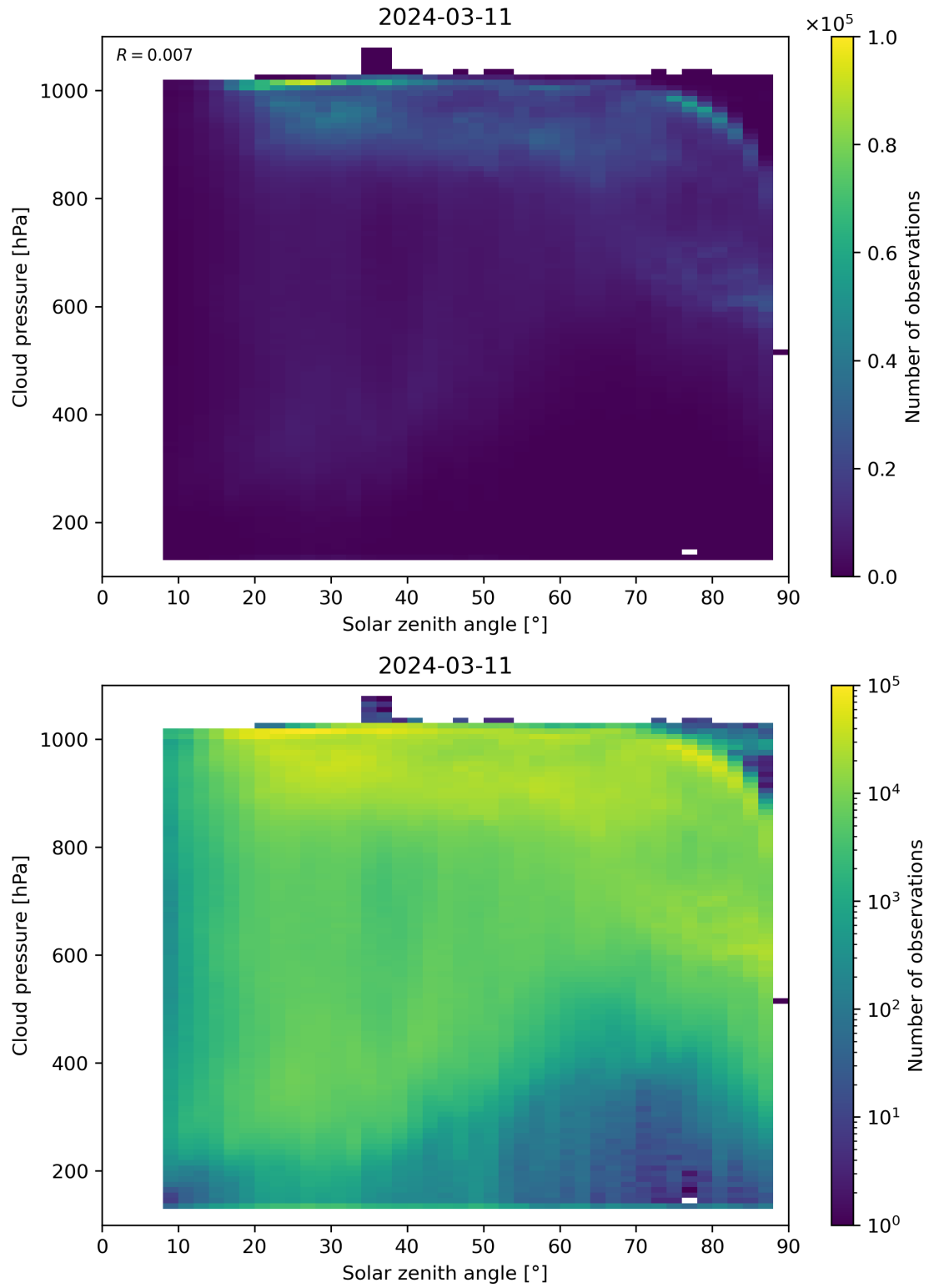
Figure 111: Scatter density plot of “Solar zenith angle” against “Cloud pressure” for 2024-03-10 to 2024-03-12.
