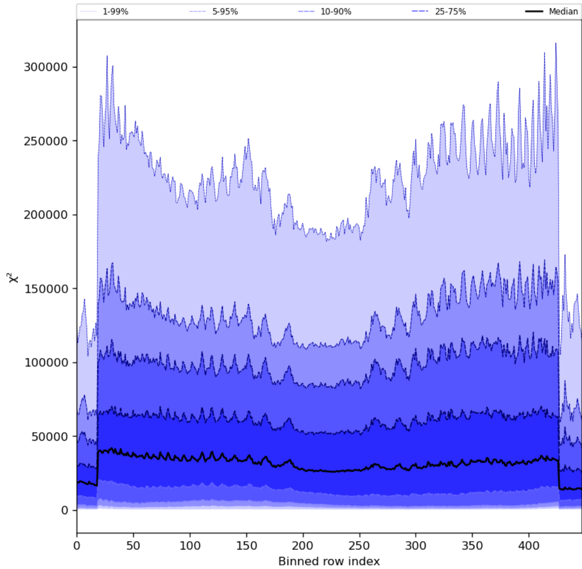
Figure 55: Along track statistics of “ \chi^2 ” for 2024-03-10 to 2024-03-12
