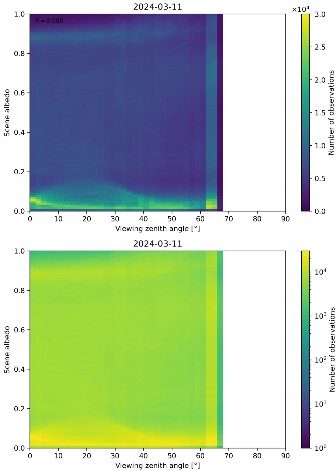
Figure 126: Scatter density plot of “Viewing zenith angle” against “Scene albedo” for 2024-03-10 to 2024-03-12.
