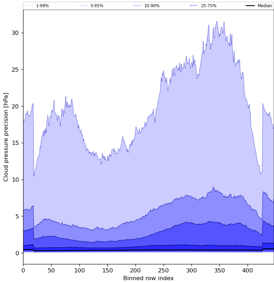
Figure 48: Along track statistics of “Cloud pressure precision” for 2024-03-10 to 2024-03-12
