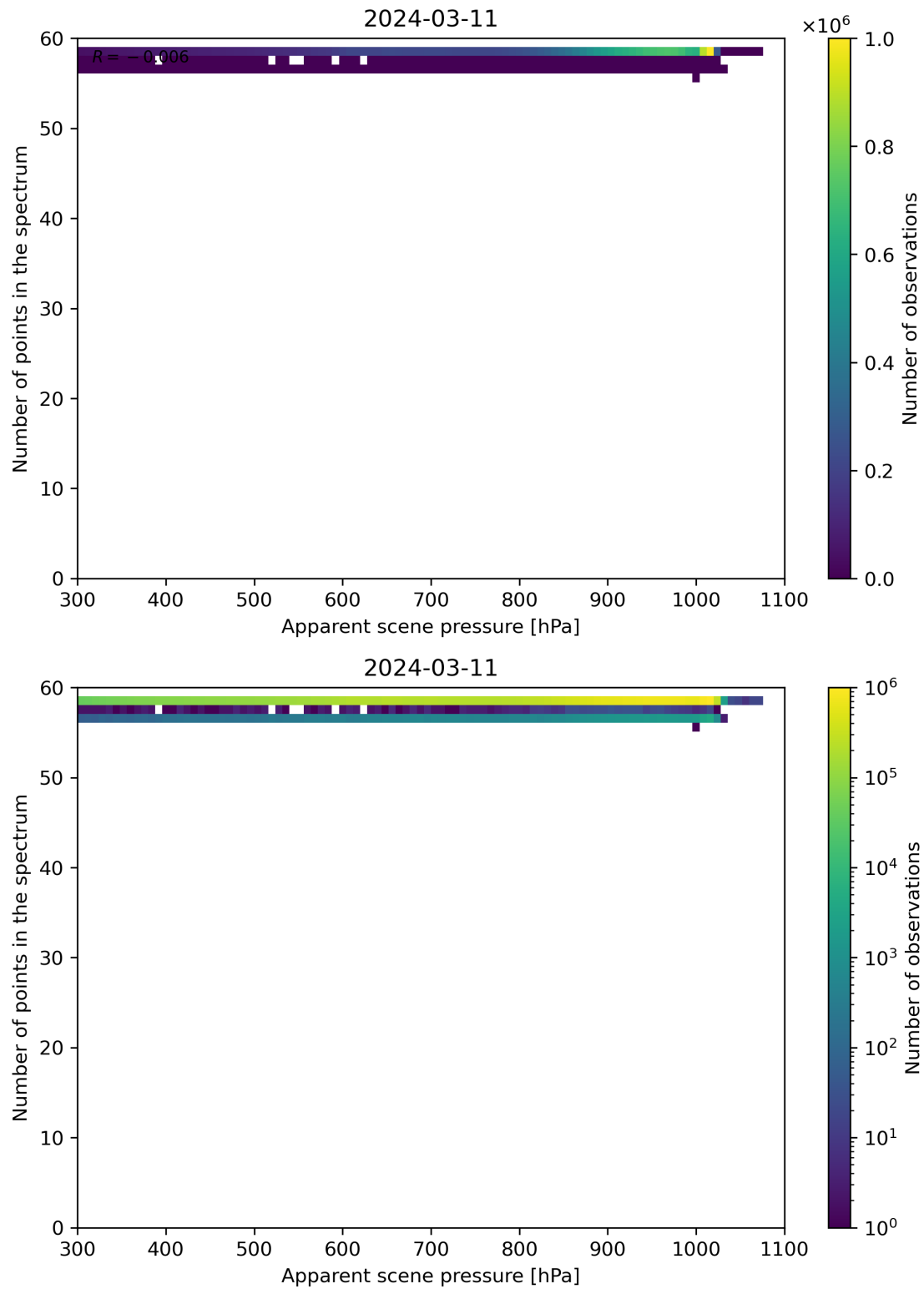
Figure 66: Scatter density plot of “Apparent scene pressure” against “Number of points in the spectrum” for 2024-03-10 to 2024-03-12.
