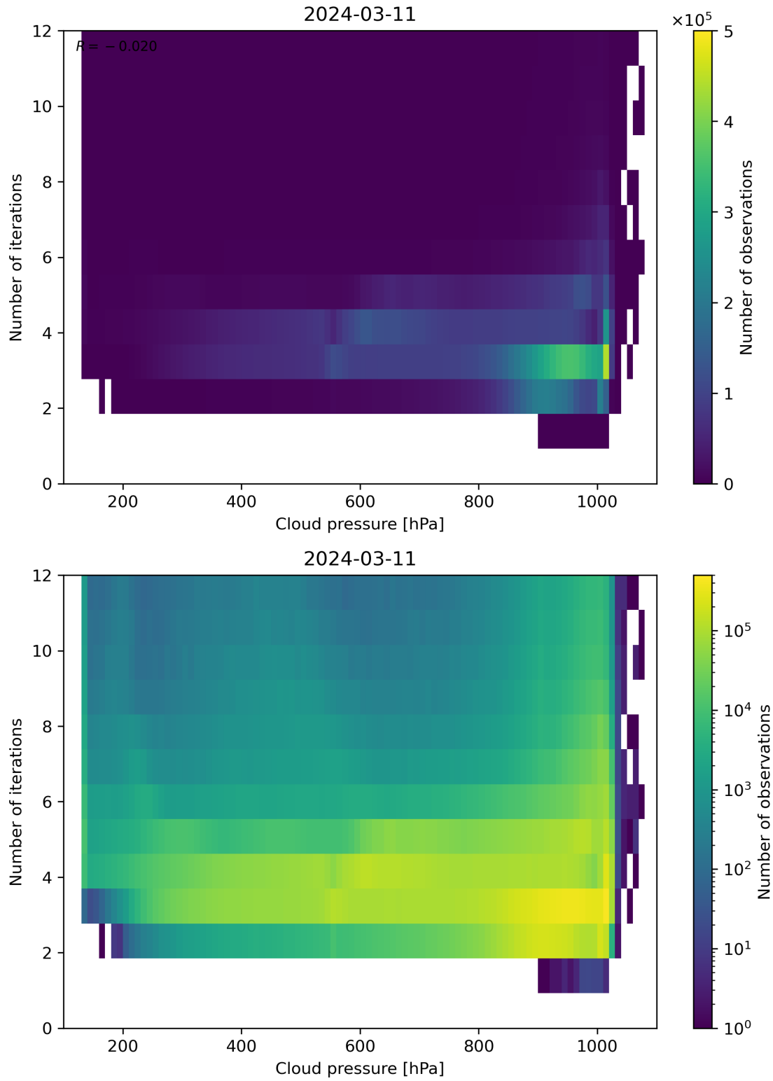
Figure 81: Scatter density plot of “Cloud pressure” against “Number of iterations” for 2024-03-10 to 2024-03-12.
