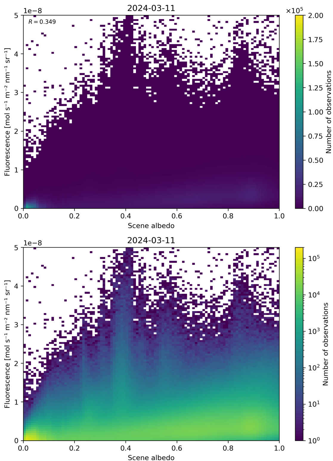
Figure 104: Scatter density plot of “Scene albedo” against “Fluorescence” for 2024-03-10 to 2024-03-12.
