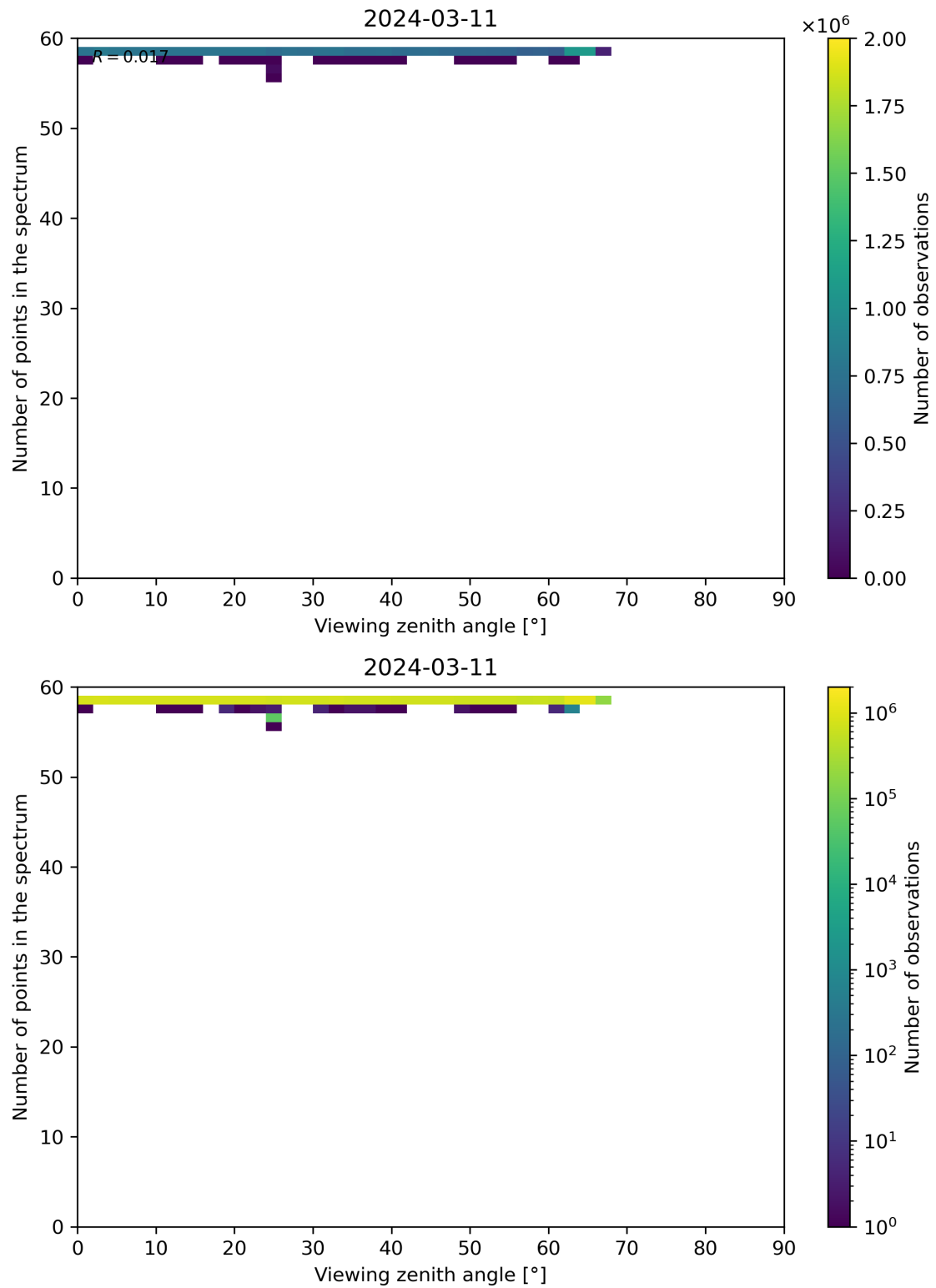
Figure 125: Scatter density plot of “Viewing zenith angle” against “Number of points in the spectrum” for 2024-03-10 to 2024-03-12.
