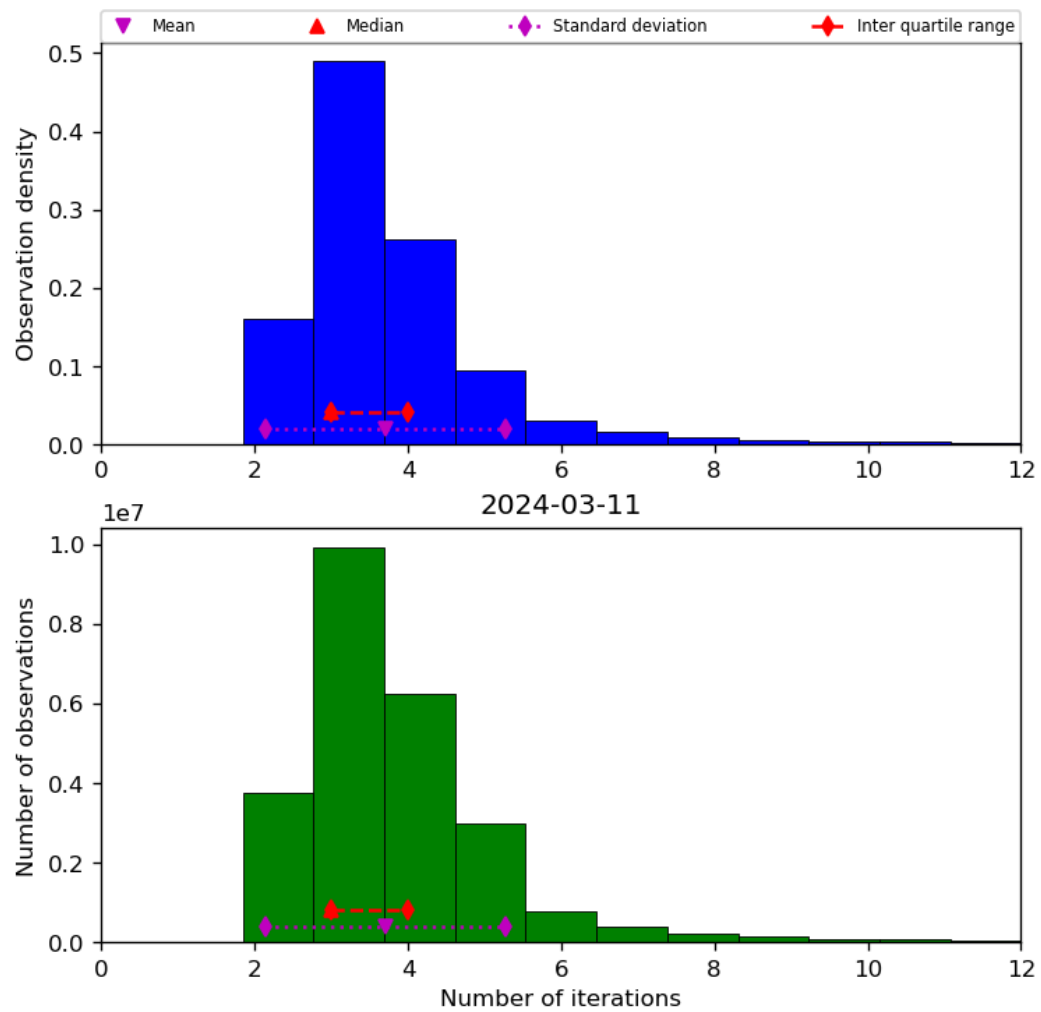
Figure 39: Histogram of “Number of iterations” for 2024-03-10 to 2024-03-12
