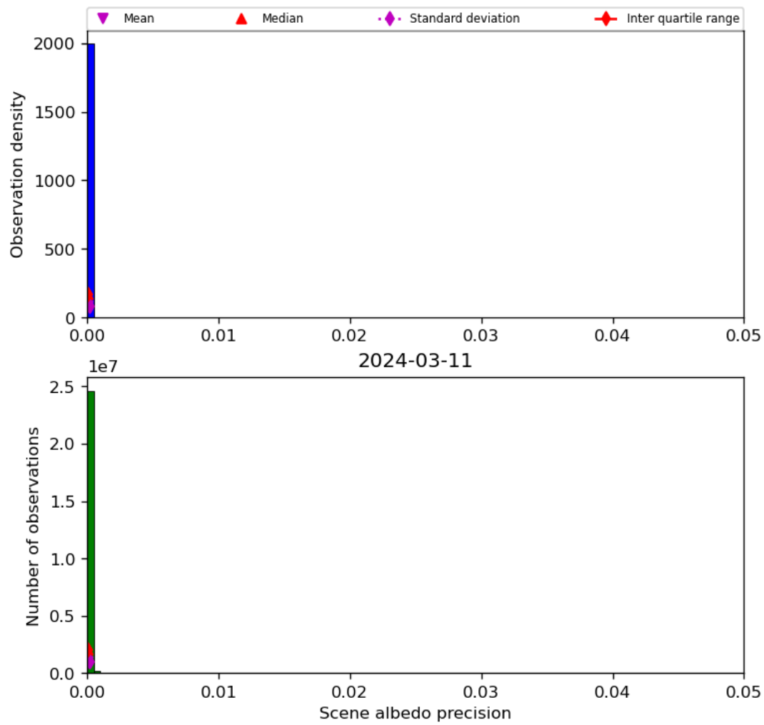
Figure 35: Histogram of “Scene albedo precision” for 2024-03-10 to 2024-03-12
