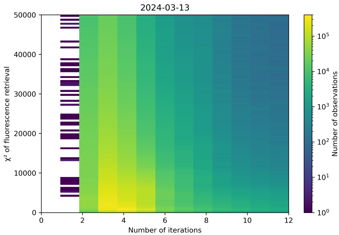
Figure 97: Scatter density plot of “Number of iterations” against “ \chi^2 of fluorescence retrieval” for 2024-03-12 to 2024-03-14.
