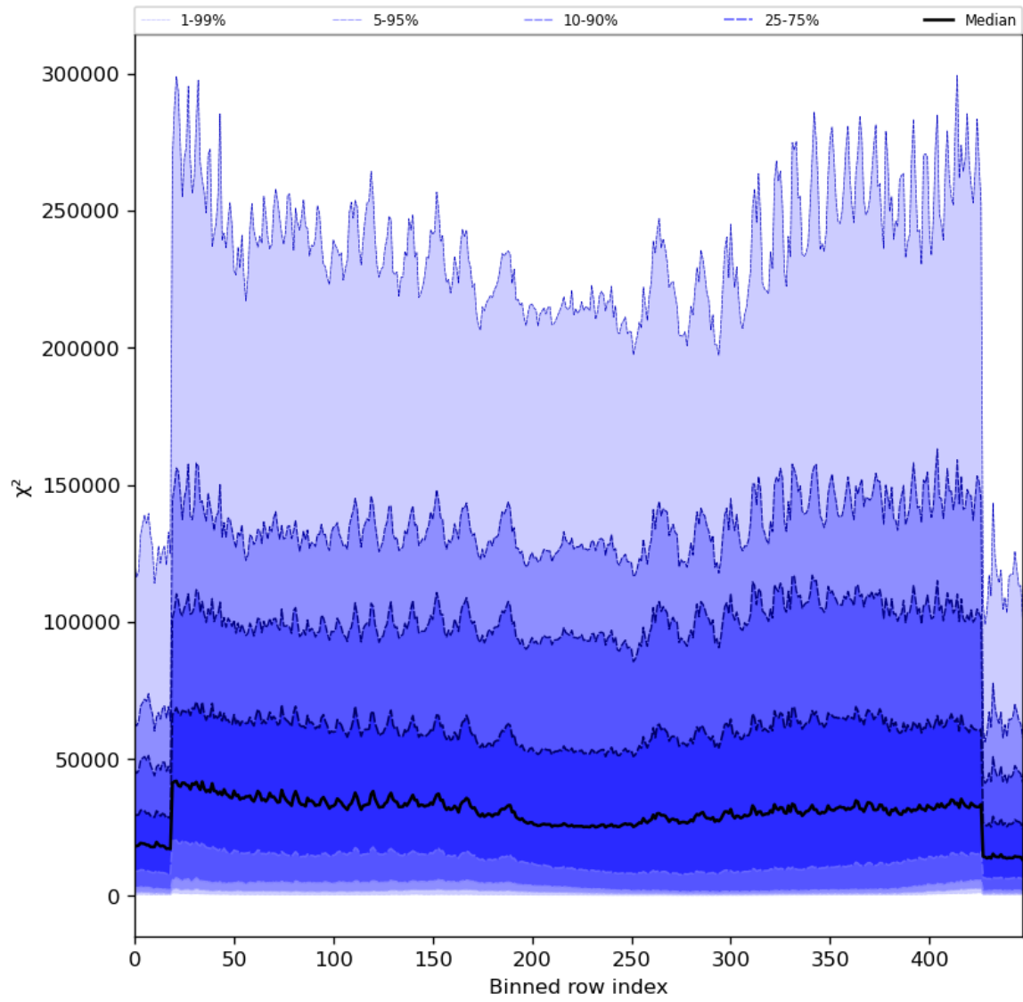
Figure 55: Along track statistics of “ \chi^2 ” for 2024-03-12 to 2024-03-14
