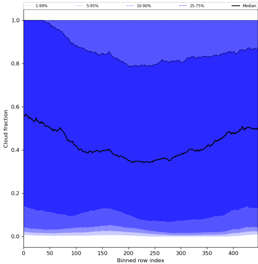
Figure 49: Along track statistics of “Cloud fraction” for 2024-03-12 to 2024-03-14
