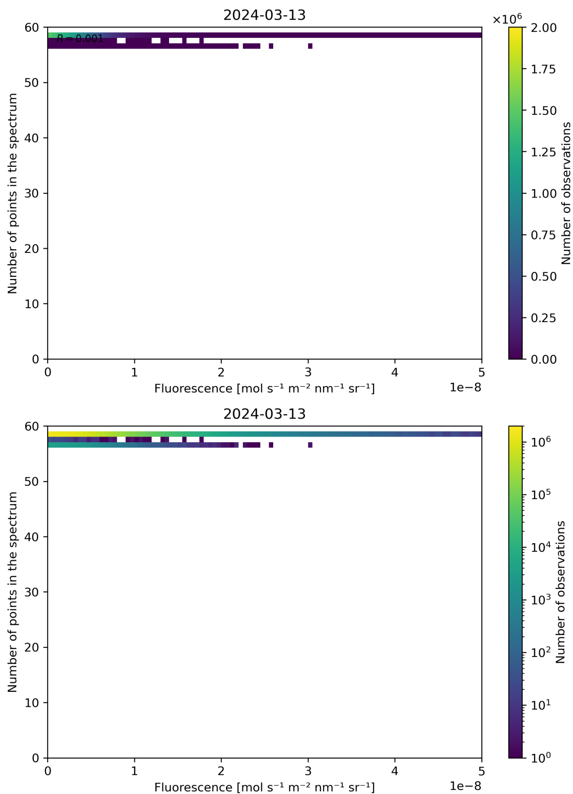
Figure 86: Scatter density plot of “Fluorescence” against “Number of points in the spectrum” for 2024-03-12 to 2024-03-14.
