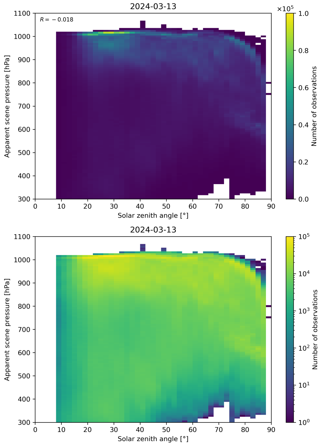
Figure 108: Scatter density plot of “Solar zenith angle” against “Apparent scene pressure” for 2024-03-12 to 2024-03-14.
