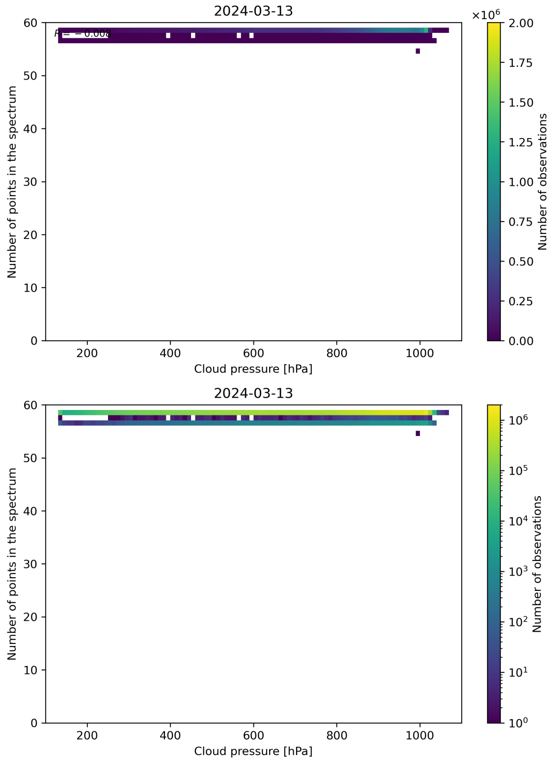
Figure 82: Scatter density plot of “Cloud pressure” against “Number of points in the spectrum” for 2024-03-12 to 2024-03-14.
