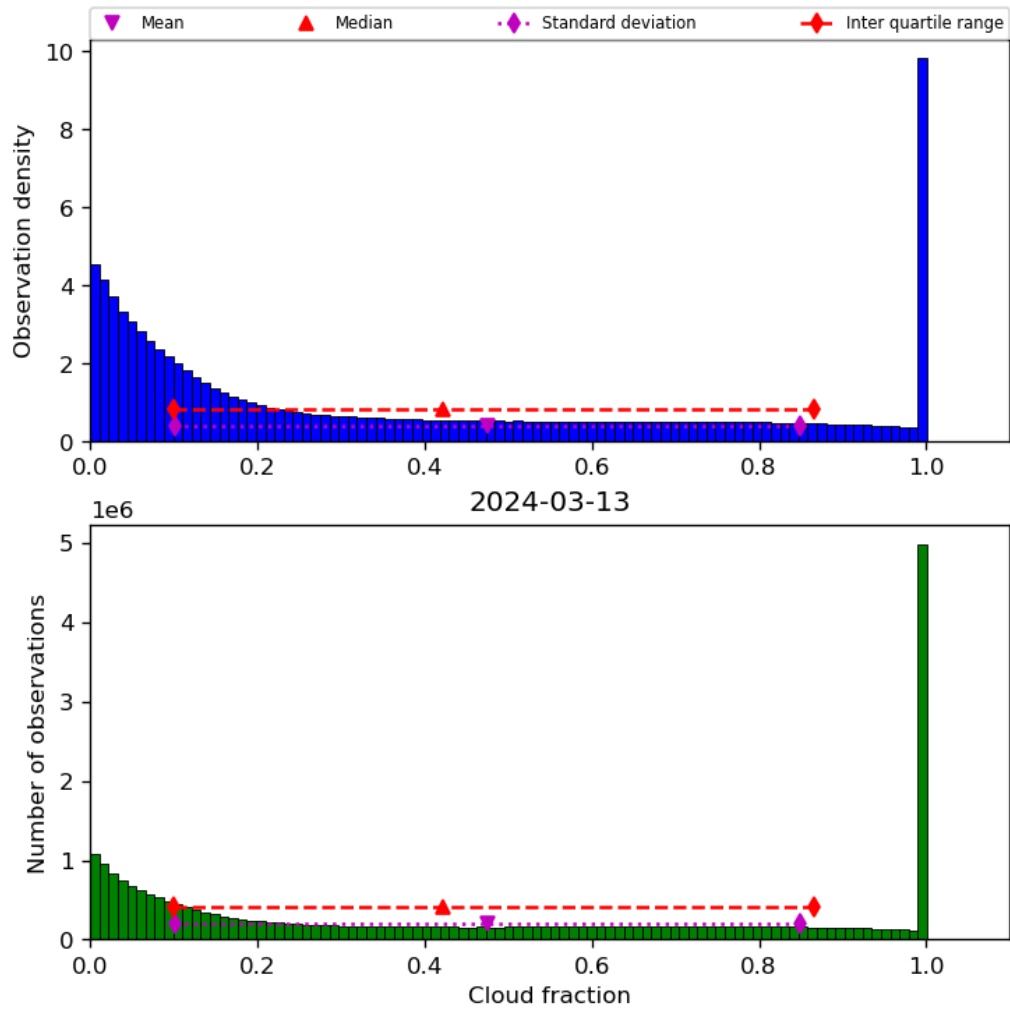
Figure 32: Histogram of “Cloud fraction” for 2024-03-12 to 2024-03-14
