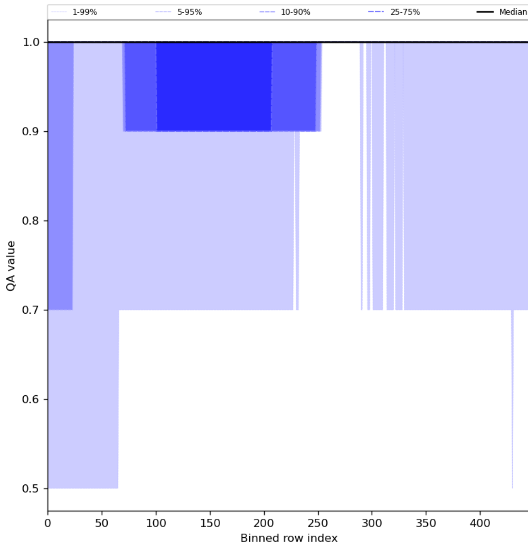
Figure 46: Along track statistics of “QA value” for 2024-03-12 to 2024-03-14
