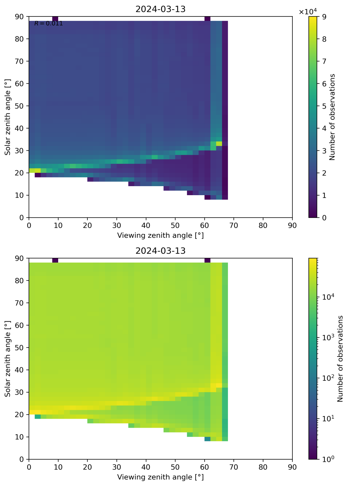
Figure 127: Scatter density plot of “Viewing zenith angle” against “Solar zenith angle” for 2024-03-12 to 2024-03-14.
