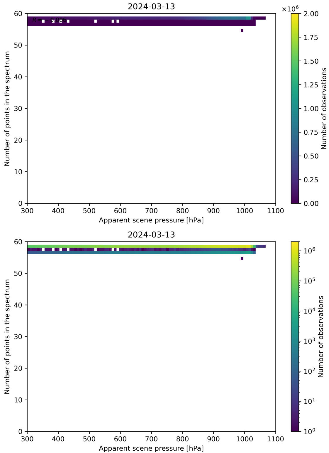
Figure 66: Scatter density plot of “Apparent scene pressure” against “Number of points in the spectrum” for 2024-03-12 to 2024-03-14.
