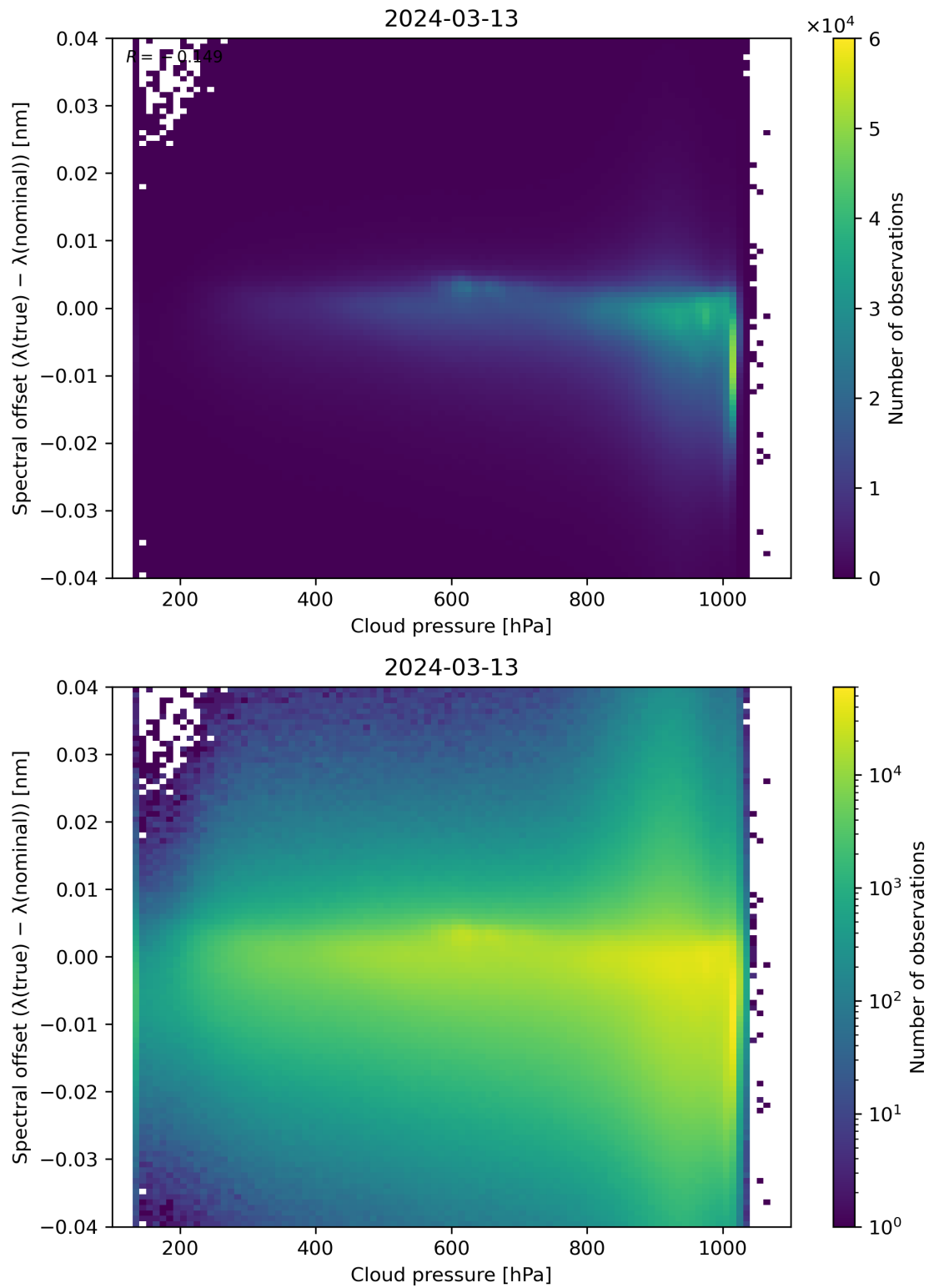
Figure 84: Scatter density plot of “Cloud pressure” against “Spectral offset ( \lambda(\text{true}) - \lambda(\text{nominal}) )” for 2024-03-12 to 2024-03-14.
