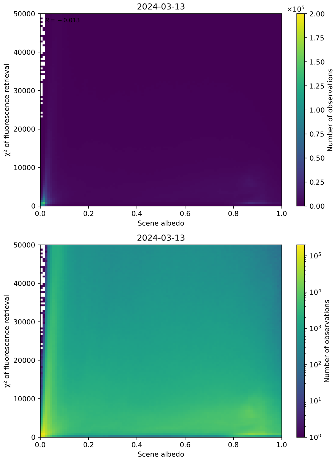
Figure 103: Scatter density plot of “Scene albedo” against “ \chi^2 of fluorescence retrieval” for 2024-03-12 to 2024-03-14.
