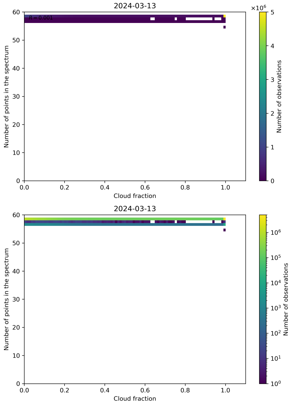
Figure 74: Scatter density plot of “Cloud fraction” against “Number of points in the spectrum” for 2024-03-12 to 2024-03-14.
