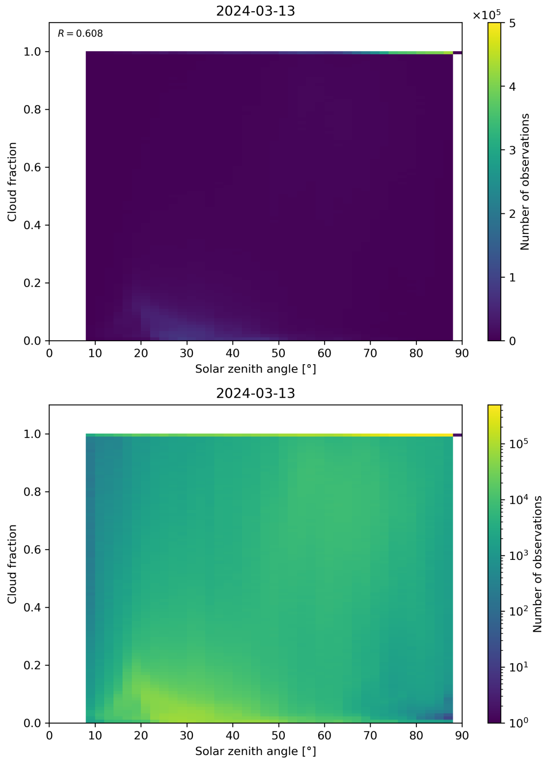
Figure 110: Scatter density plot of “Solar zenith angle” against “Cloud fraction” for 2024-03-12 to 2024-03-14.
