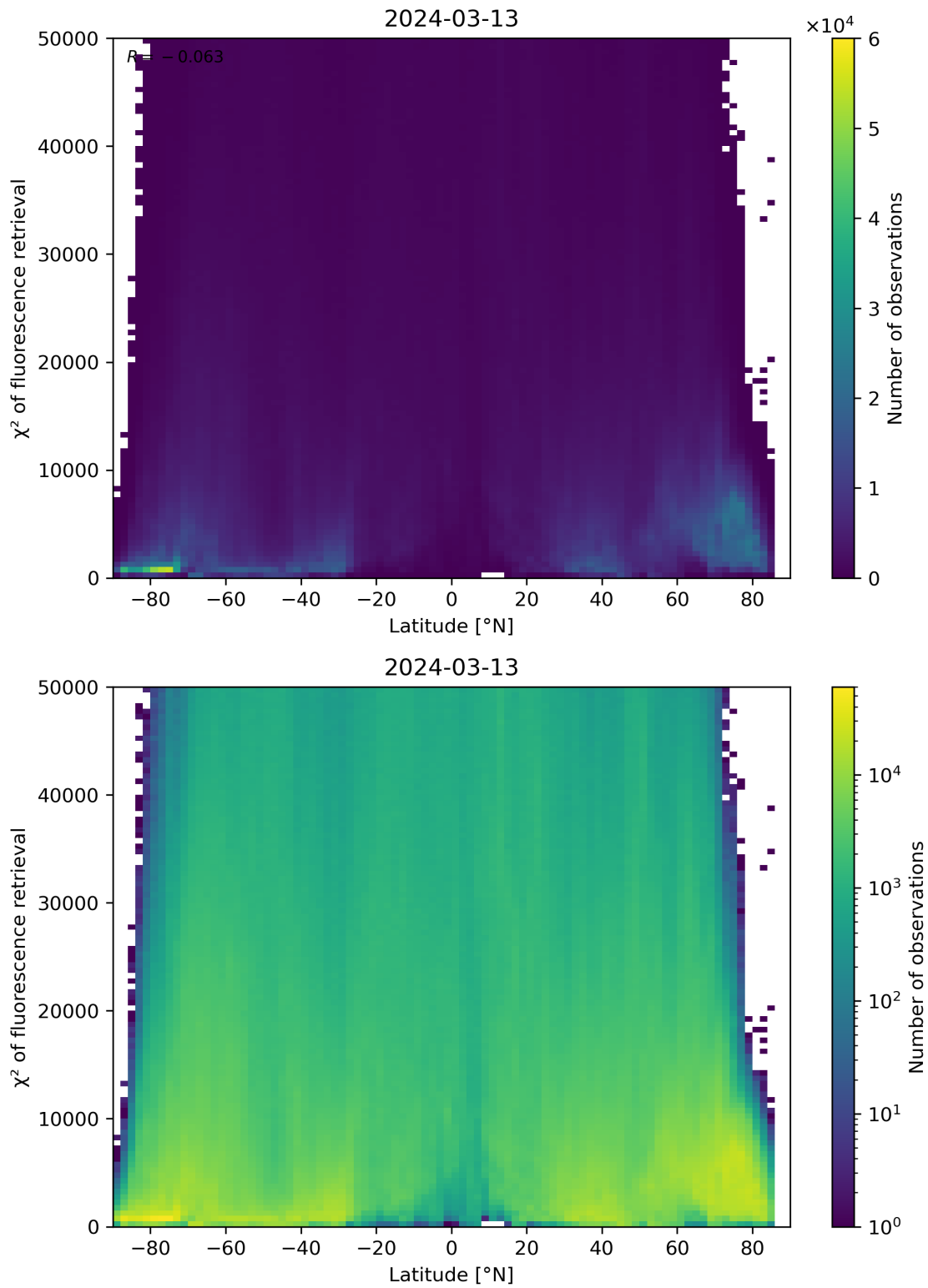
Figure 89: Scatter density plot of “Latitude” against “ \chi^2 of fluorescence retrieval” for 2024-03-12 to 2024-03-14.
