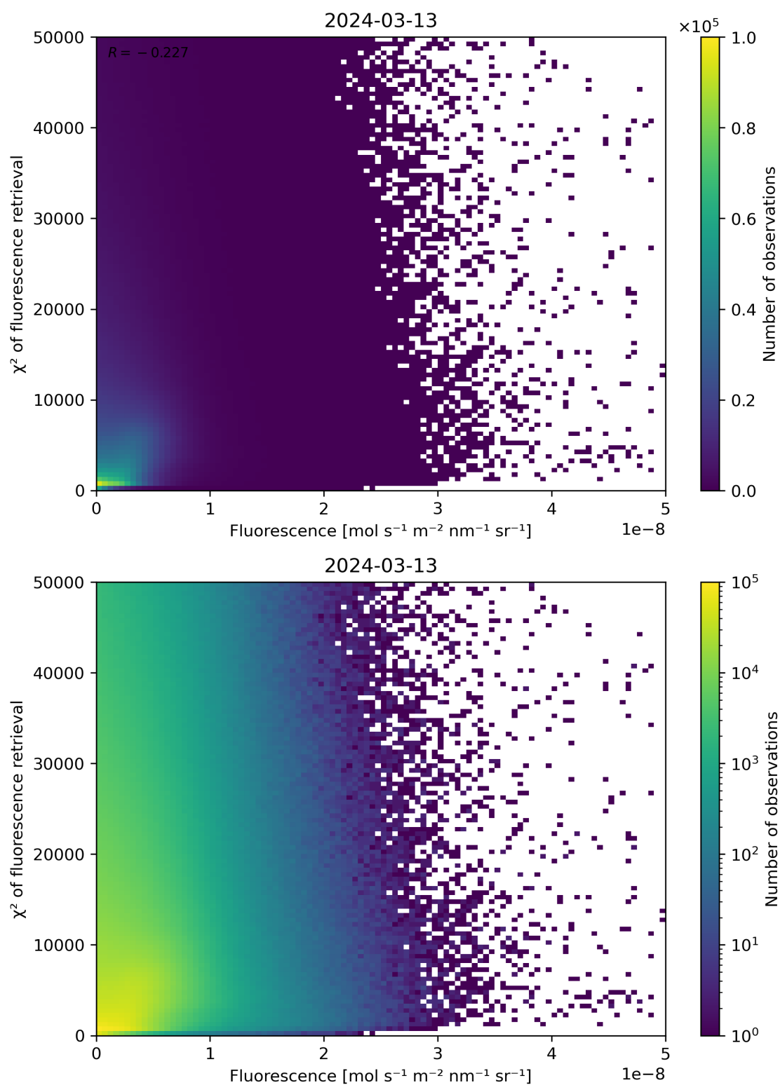
Figure 85: Scatter density plot of “Fluorescence” against “ \chi^2 of fluorescence retrieval” for 2024-03-12 to 2024-03-14.
