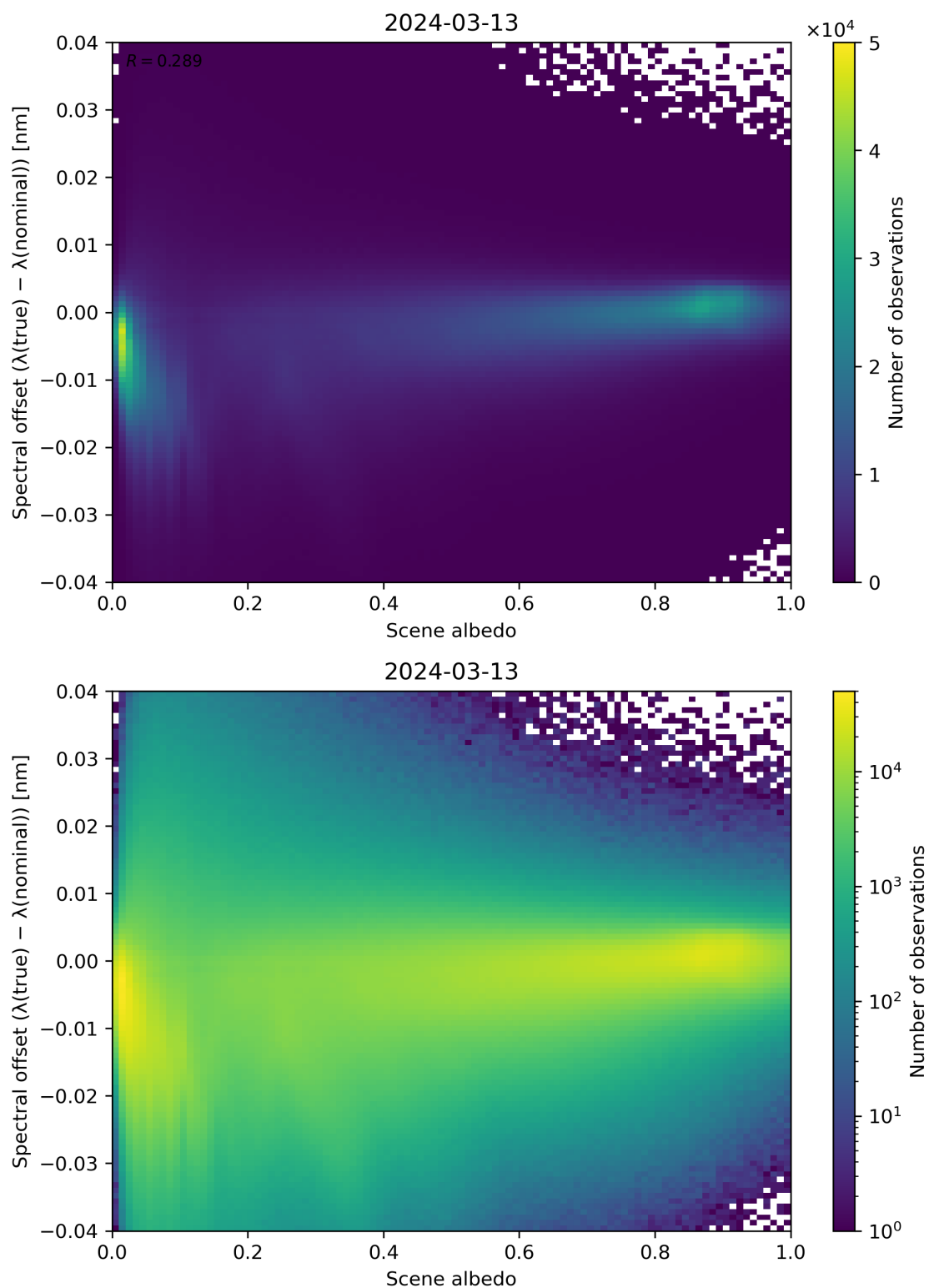
Figure 107: Scatter density plot of “Scene albedo” against “Spectral offset ( \lambda(\text{true}) - \lambda(\text{nominal}) )” for 2024-03-12 to 2024-03-14.
