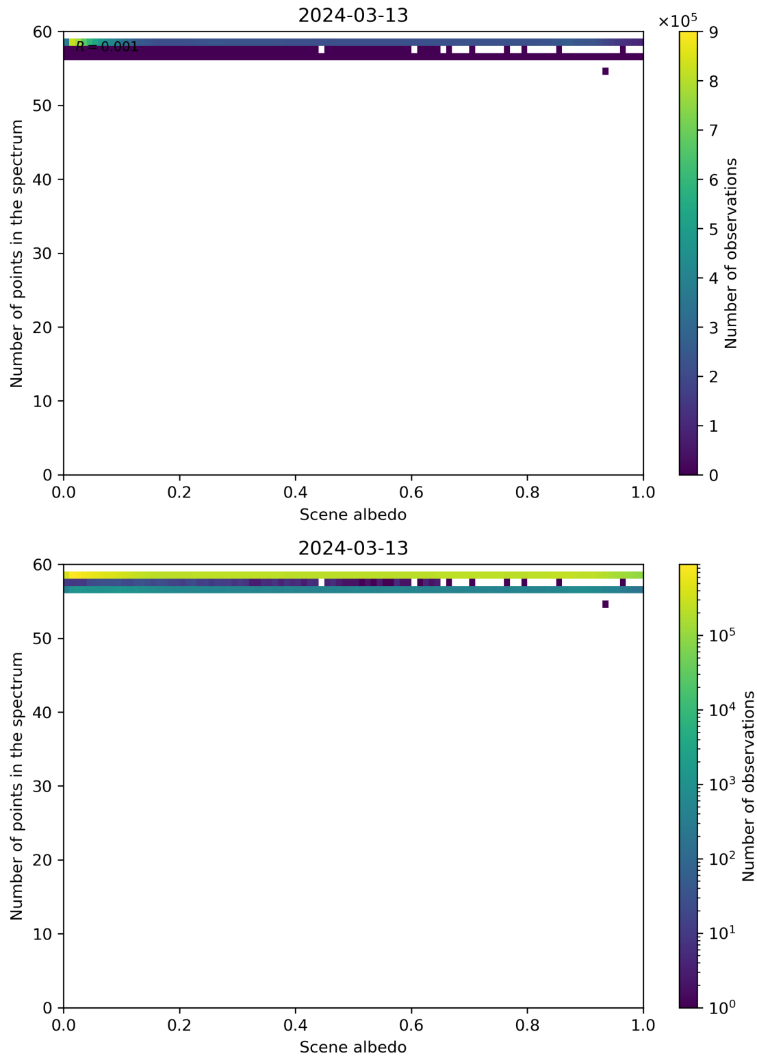
Figure 106: Scatter density plot of “Scene albedo” against “Number of points in the spectrum” for 2024-03-12 to 2024-03-14.
