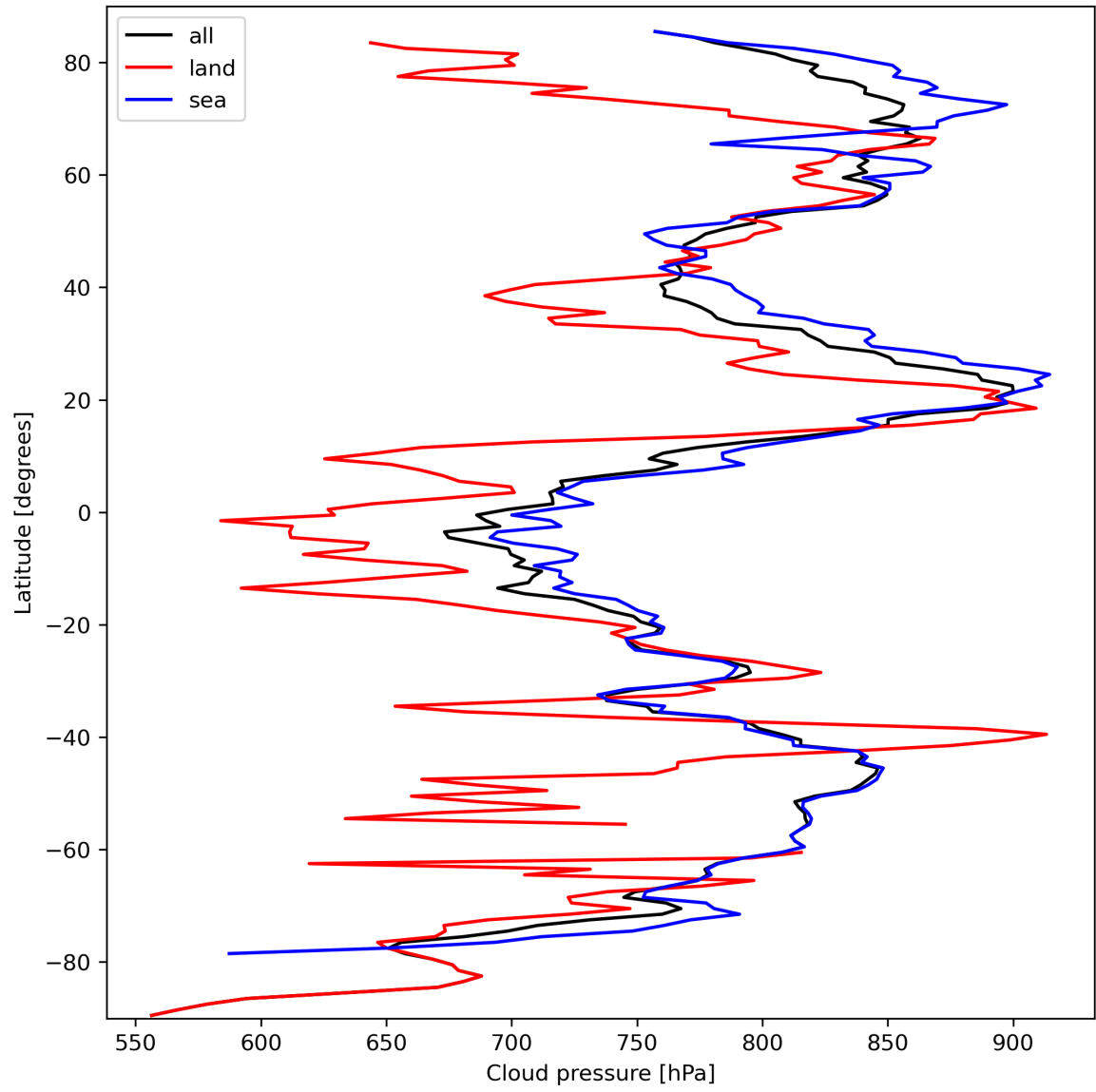
Figure 13: Zonal average of “Cloud pressure” for 2024-03-12 to 2024-03-14.
