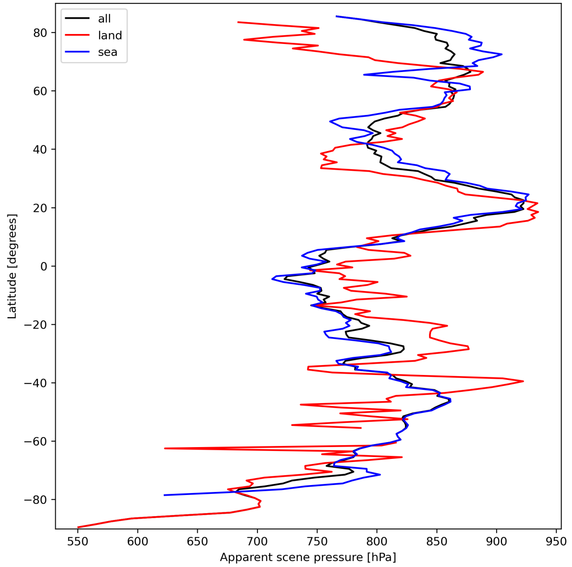
Figure 19: Zonal average of “Apparent scene pressure” for 2024-03-12 to 2024-03-14.
