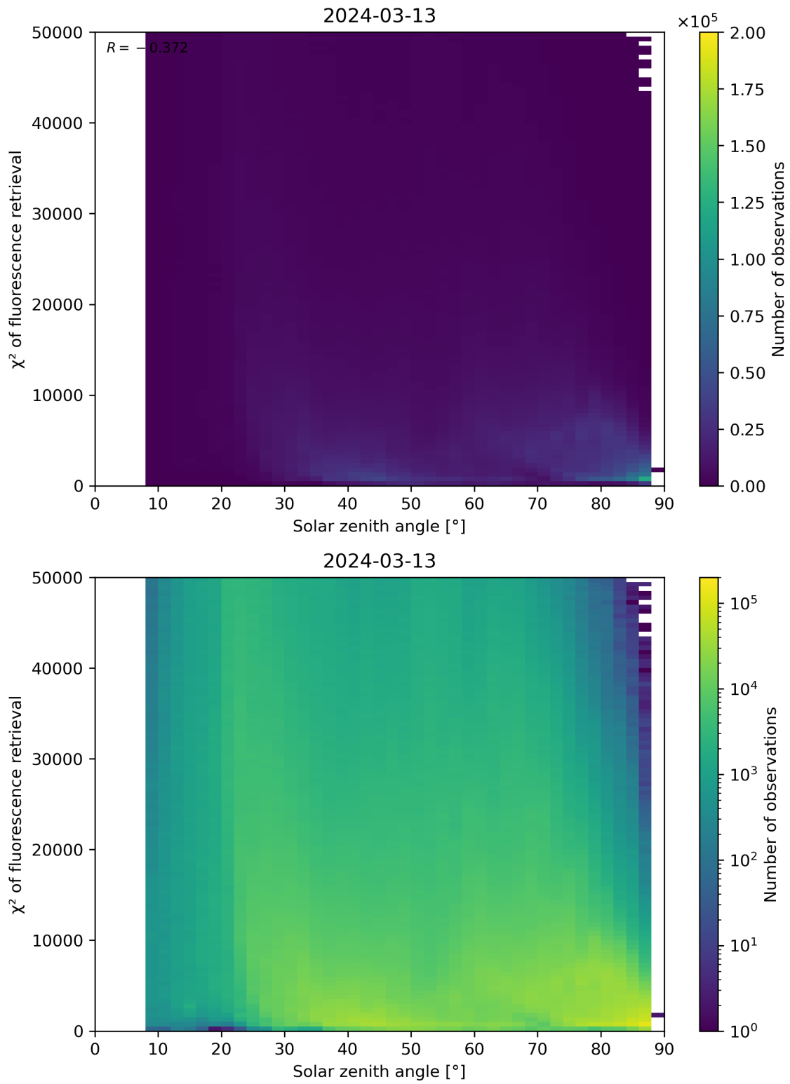
Figure 109: Scatter density plot of “Solar zenith angle” against “ \chi^2 of fluorescence retrieval” for 2024-03-12 to 2024-03-14.
