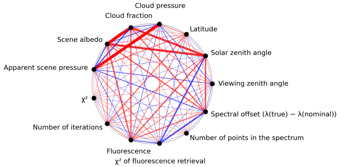
Figure 1: Map of correlation graph for 2024-03-12 to 2024-03-14.
