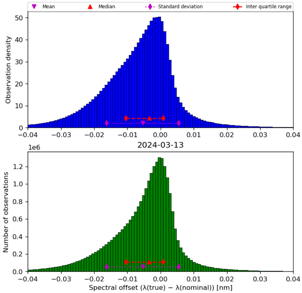
Figure 45: Histogram of “Spectral offset ( \lambda(\text{true}) - \lambda(\text{nominal}) )” for 2024-03-12 to 2024-03-14
