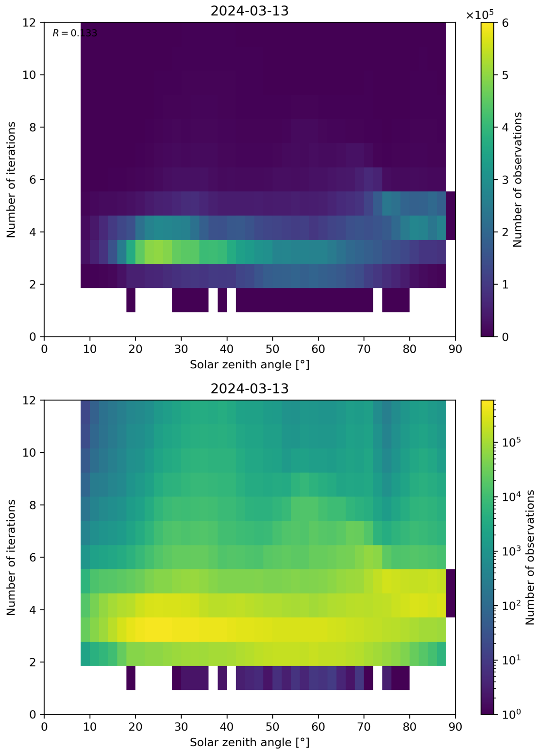
Figure 114: Scatter density plot of “Solar zenith angle” against “Number of iterations” for 2024-03-12 to 2024-03-14.
