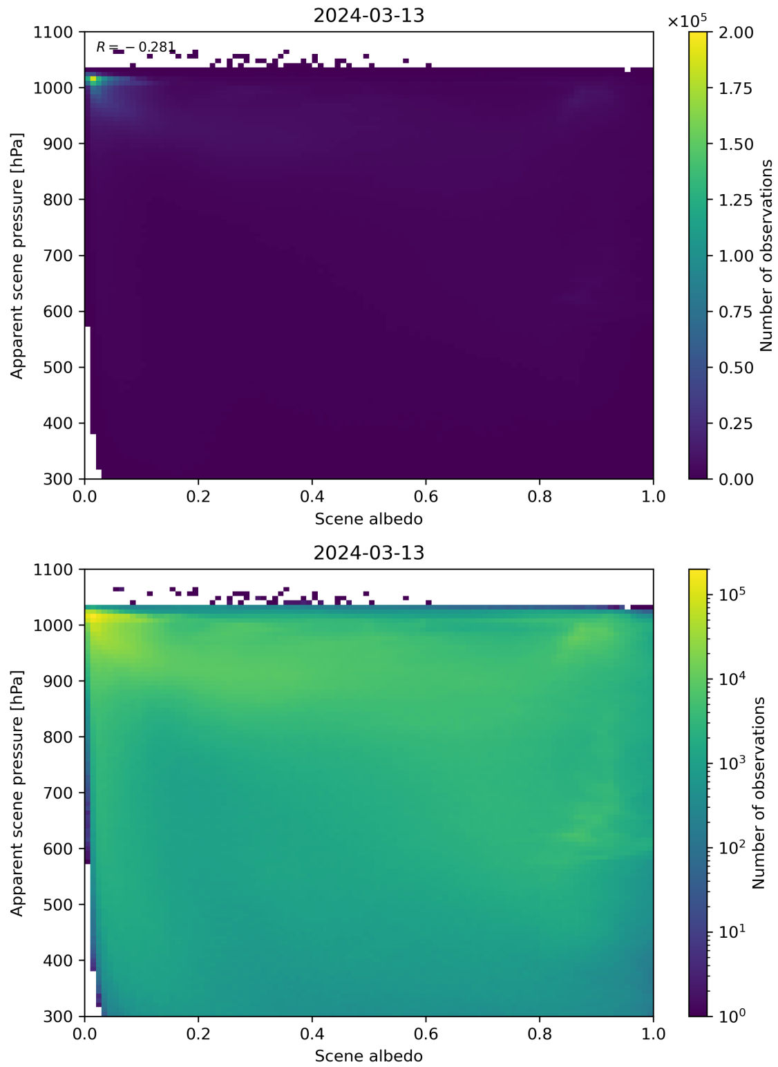
Figure 102: Scatter density plot of “Scene albedo” against “Apparent scene pressure” for 2024-03-12 to 2024-03-14.
