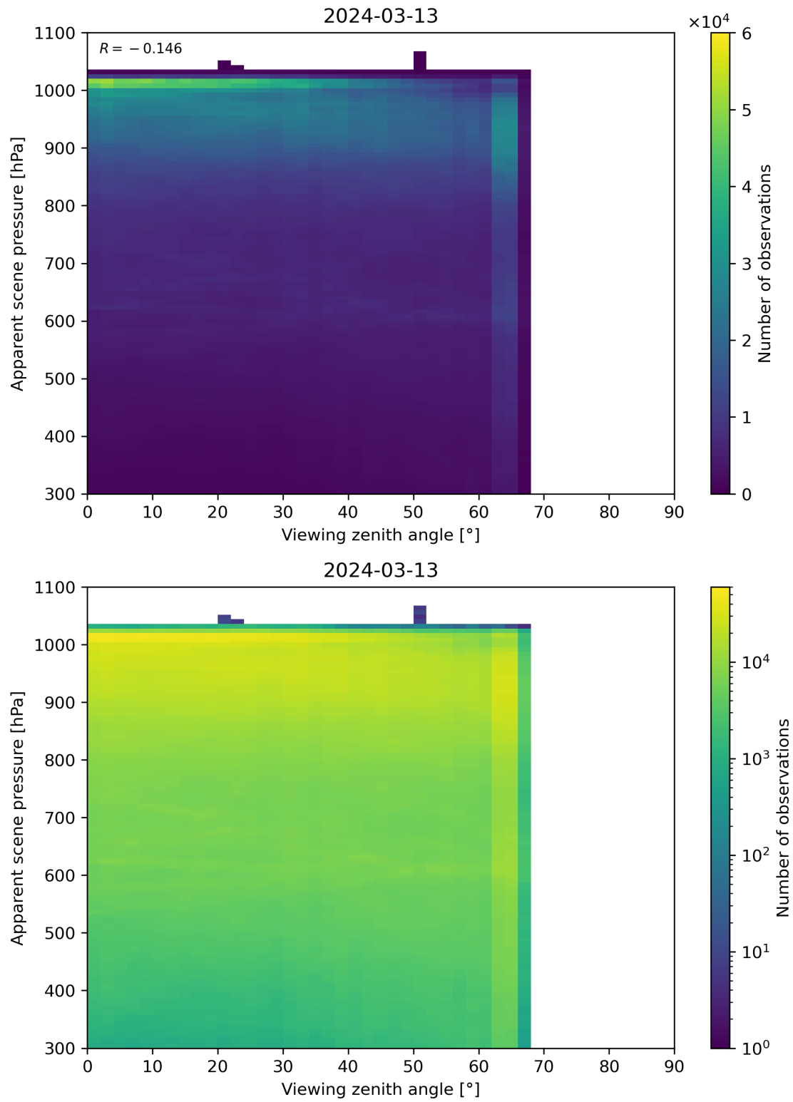
Figure 118: Scatter density plot of “Viewing zenith angle” against “Apparent scene pressure” for 2024-03-12 to 2024-03-14.
