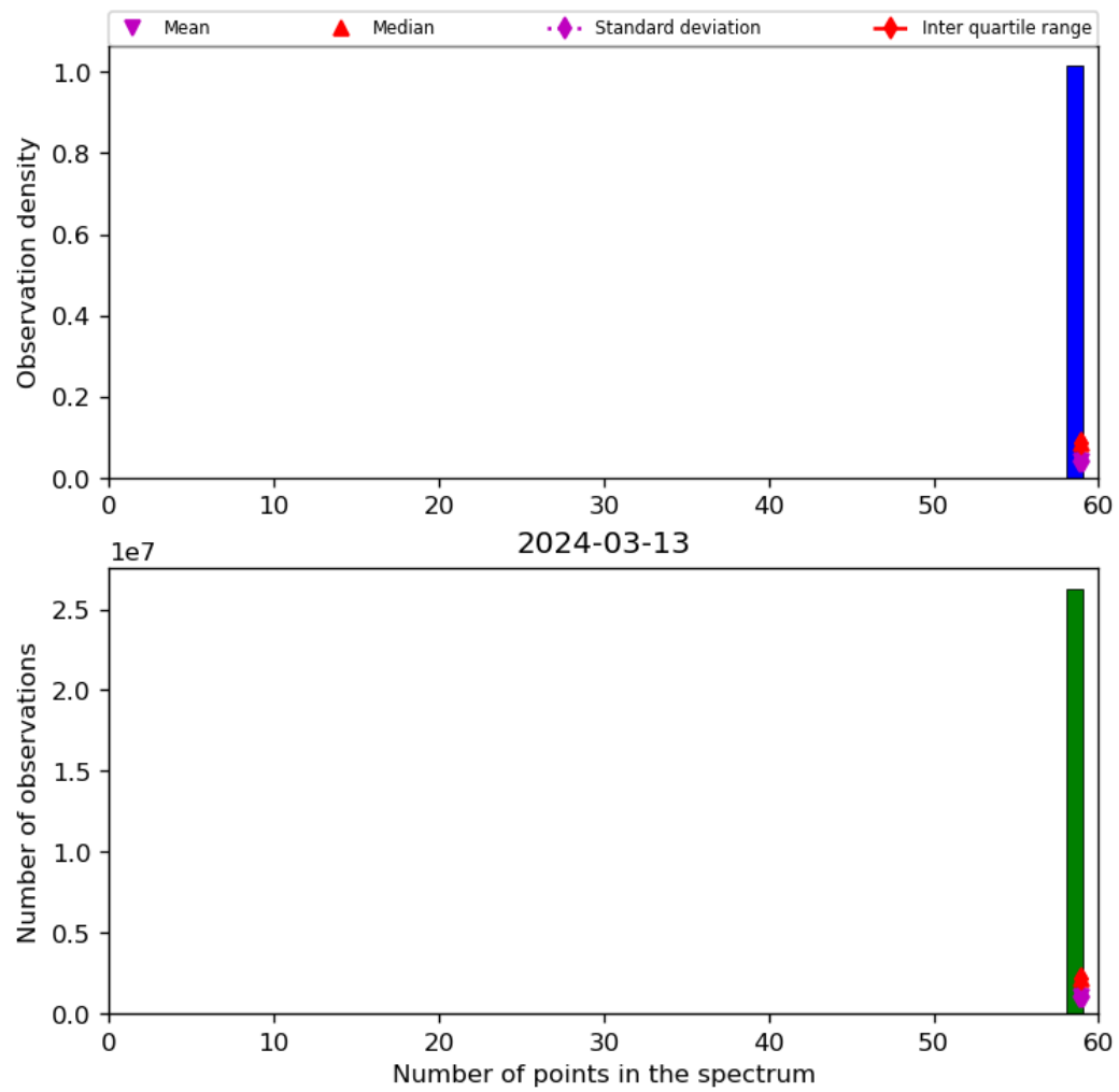
Figure 44: Histogram of “Number of points in the spectrum” for 2024-03-12 to 2024-03-14
