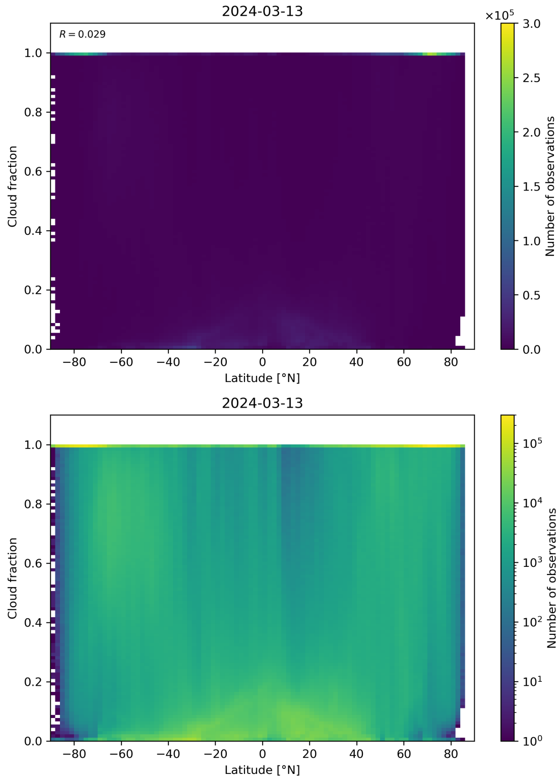
Figure 90: Scatter density plot of “Latitude” against “Cloud fraction” for 2024-03-12 to 2024-03-14.
