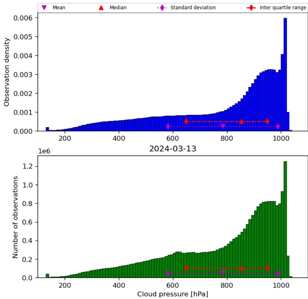
Figure 30: Histogram of “Cloud pressure” for 2024-03-12 to 2024-03-14
