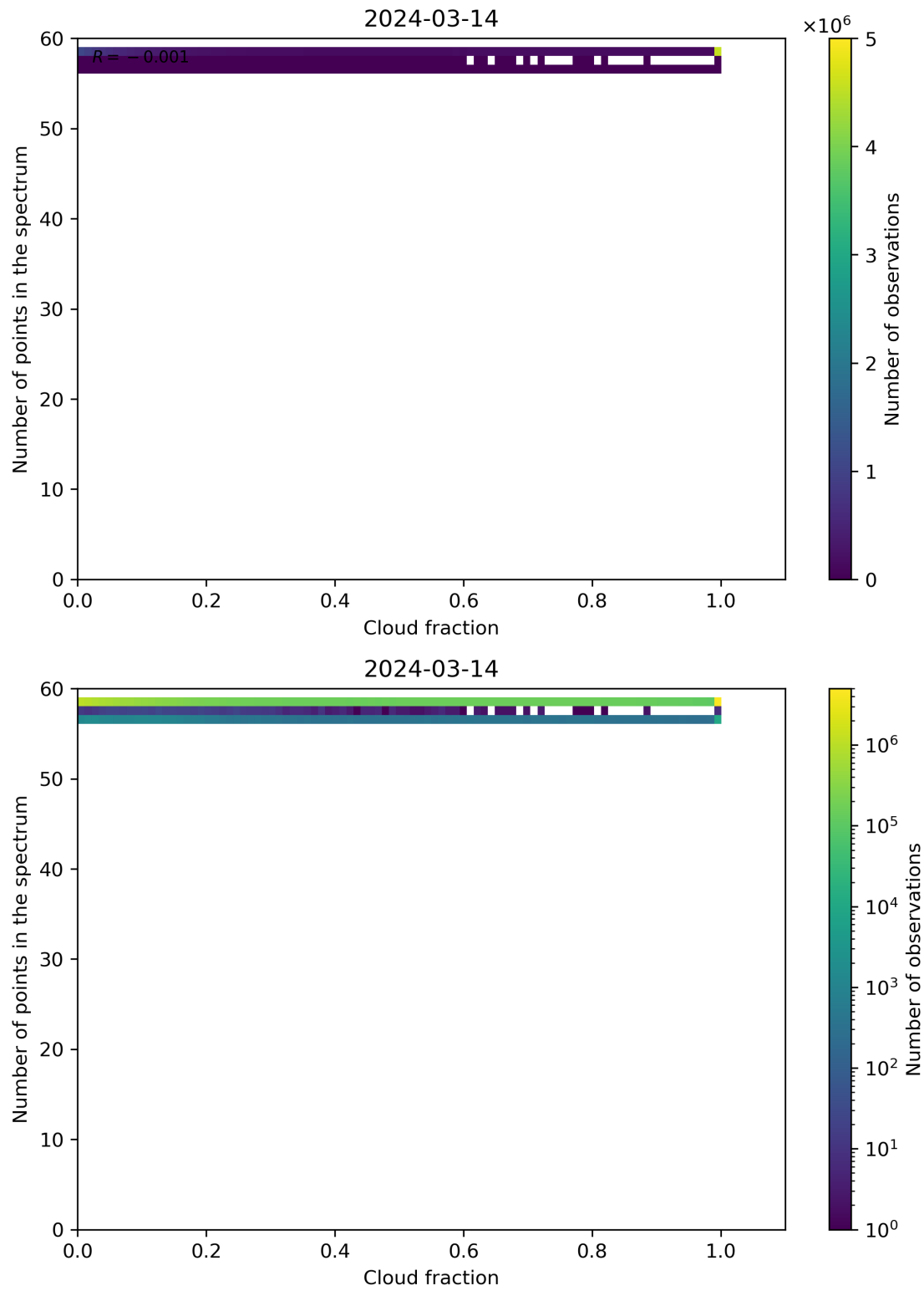
Figure 74: Scatter density plot of “Cloud fraction” against “Number of points in the spectrum” for 2024-03-14 to 2024-03-15.
