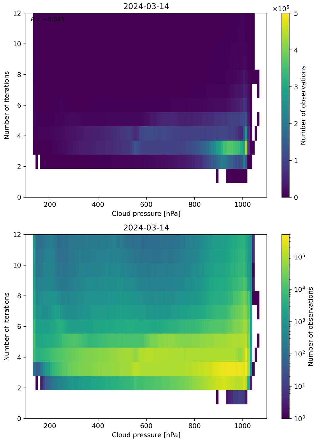
Figure 81: Scatter density plot of “Cloud pressure” against “Number of iterations” for 2024-03-14 to 2024-03-15.
