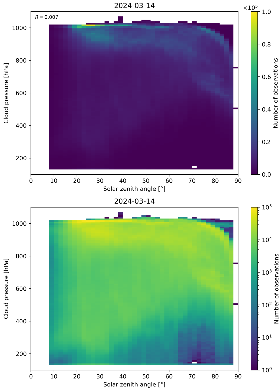
Figure 111: Scatter density plot of “Solar zenith angle” against “Cloud pressure” for 2024-03-14 to 2024-03-15.
