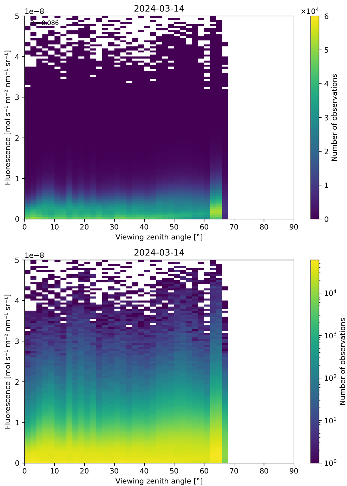
Figure 122: Scatter density plot of “Viewing zenith angle” against “Fluorescence” for 2024-03-14 to 2024-03-15.
