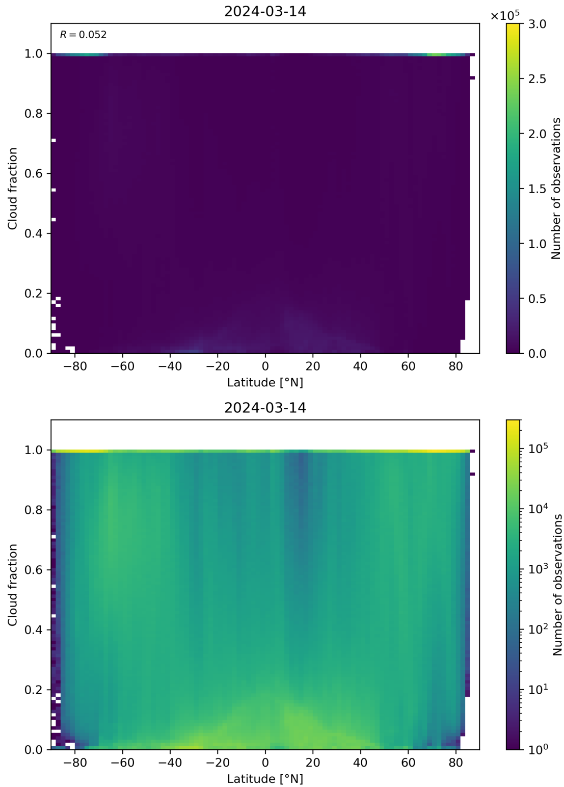
Figure 90: Scatter density plot of “Latitude” against “Cloud fraction” for 2024-03-14 to 2024-03-15.
