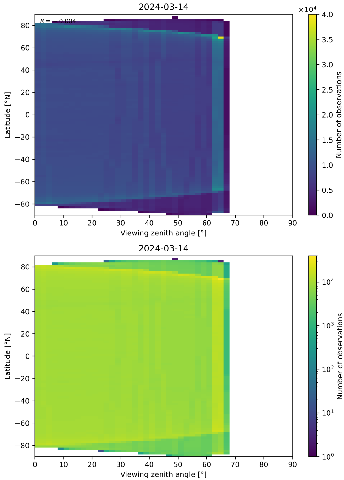
Figure 123: Scatter density plot of “Viewing zenith angle” against “Latitude” for 2024-03-14 to 2024-03-15.
