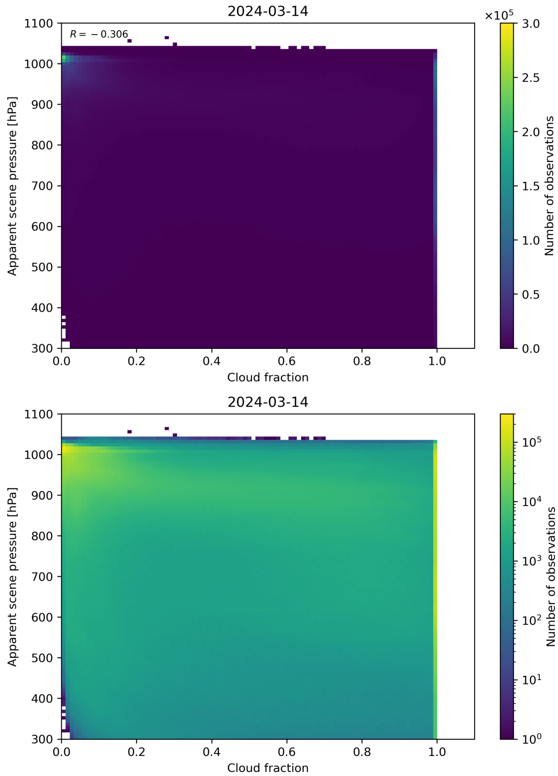
Figure 70: Scatter density plot of “Cloud fraction” against “Apparent scene pressure” for 2024-03-14 to 2024-03-15.
