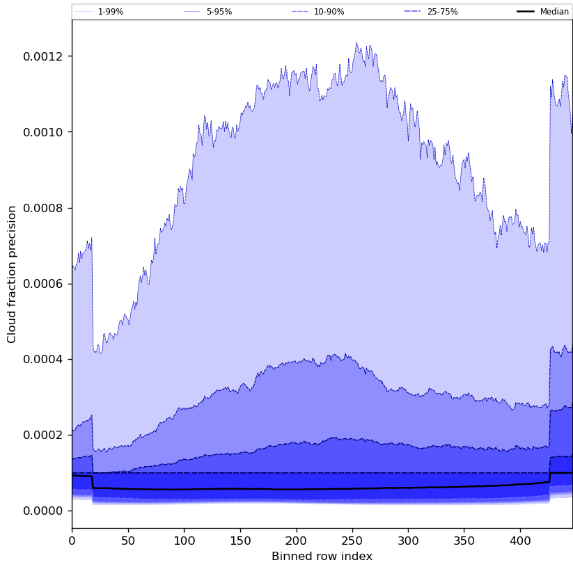
Figure 50: Along track statistics of “Cloud fraction precision” for 2024-03-14 to 2024-03-15
