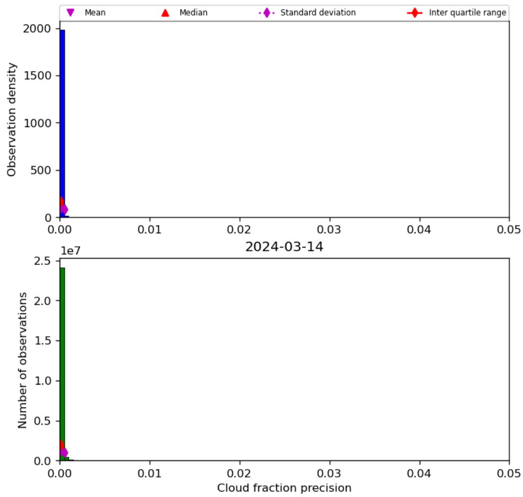
Figure 33: Histogram of “Cloud fraction precision” for 2024-03-14 to 2024-03-15
