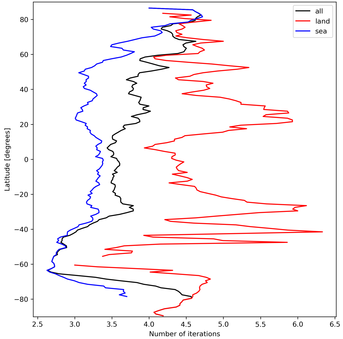
Figure 22: Zonal average of “Number of iterations” for 2024-03-14 to 2024-03-15.
