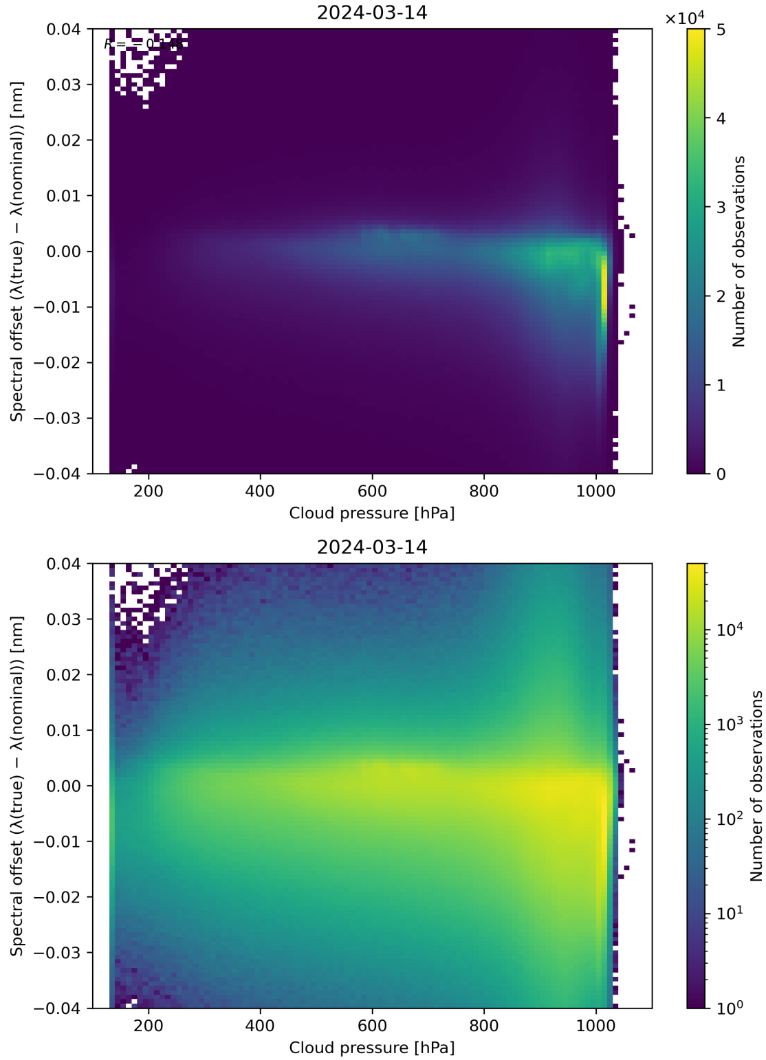
Figure 84: Scatter density plot of “Cloud pressure” against “Spectral offset ( \lambda(\text{true}) - \lambda(\text{nominal}) )” for 2024-03-14 to 2024-03-15.
