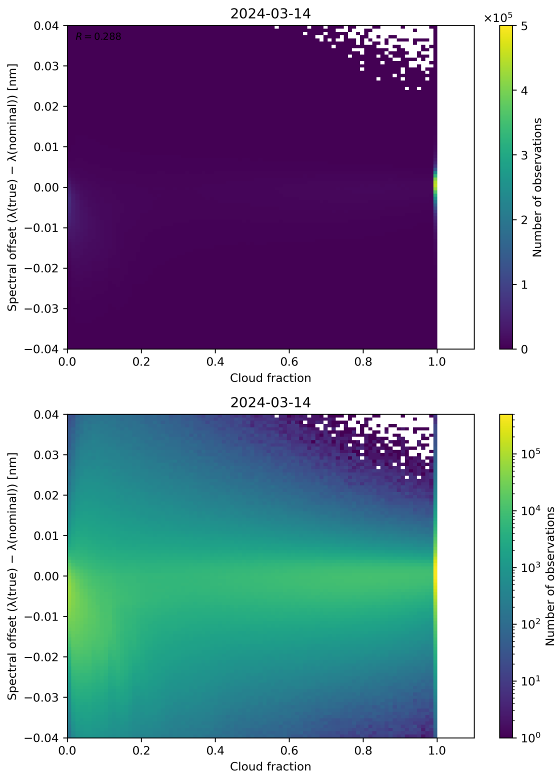
Figure 76: Scatter density plot of “Cloud fraction” against “Spectral offset ( \lambda(\text{true}) - \lambda(\text{nominal}) )” for 2024-03-14 to 2024-03-15.
