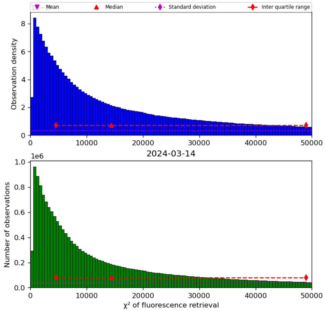
Figure 42: Histogram of “ \chi^2 of fluorescence retrieval” for 2024-03-14 to 2024-03-15
