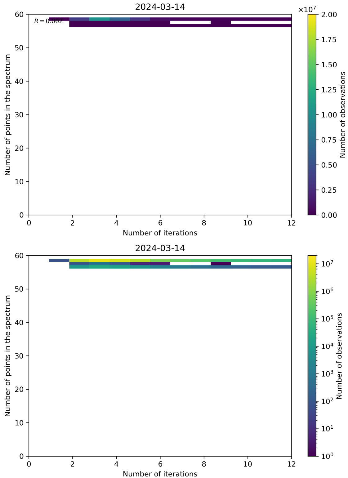
Figure 99: Scatter density plot of “Number of iterations” against “Number of points in the spectrum” for 2024-03-14 to 2024-03-15.
