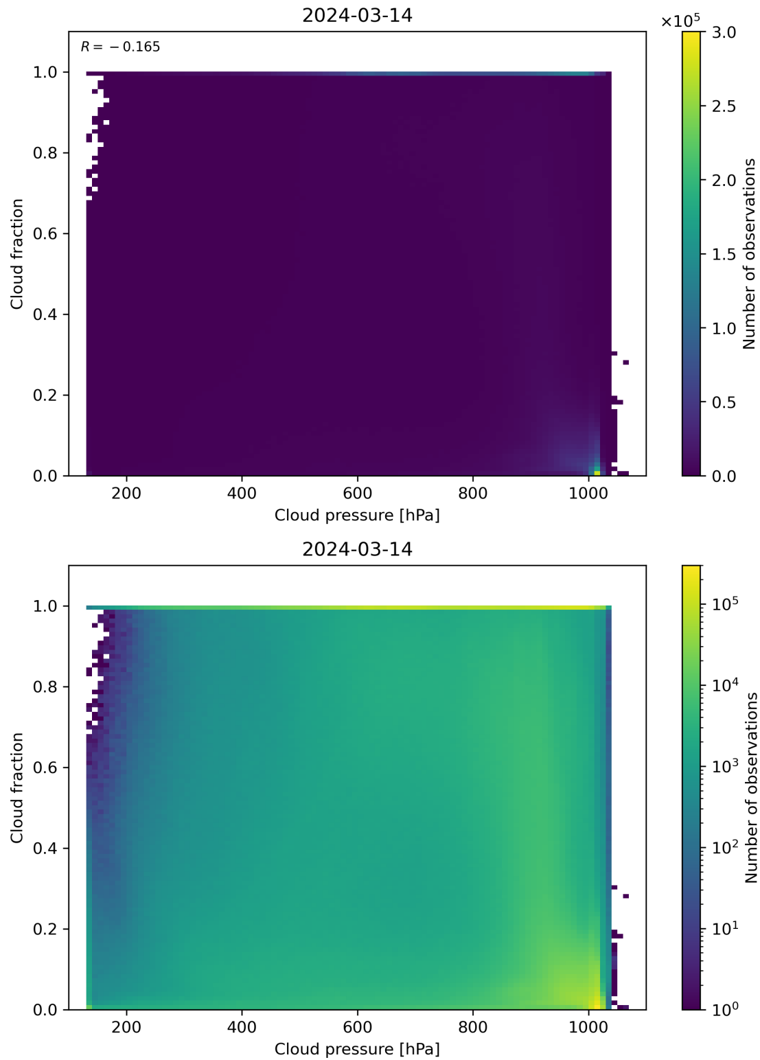
Figure 79: Scatter density plot of “Cloud pressure” against “Cloud fraction” for 2024-03-14 to 2024-03-15.
