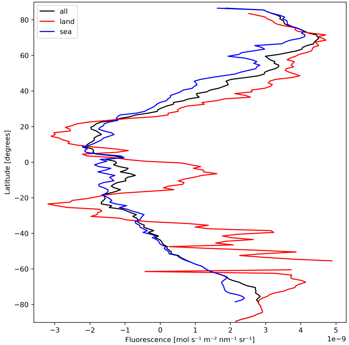
Figure 23: Zonal average of “Fluorescence” for 2024-03-14 to 2024-03-15.
