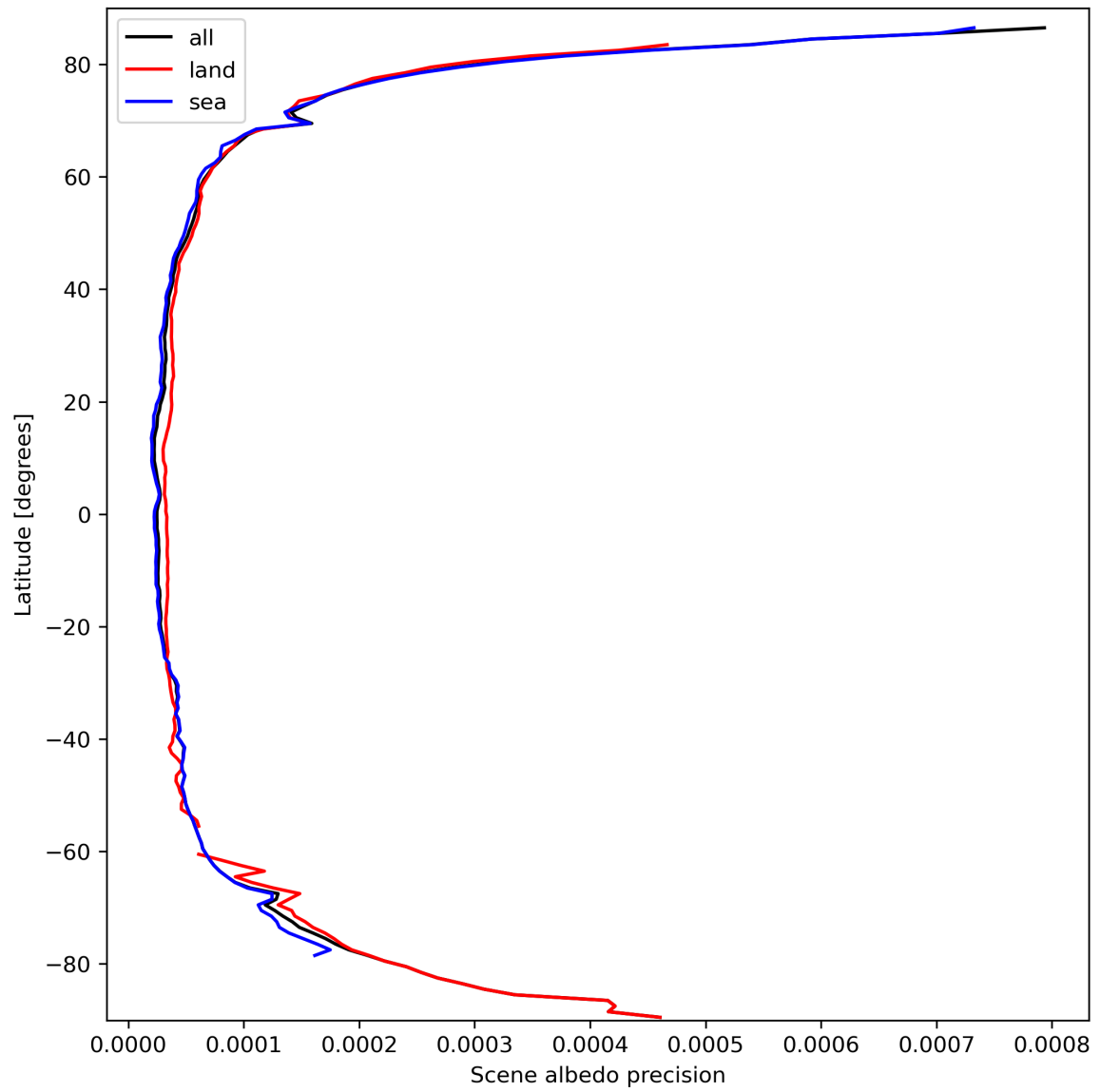
Figure 18: Zonal average of “Scene albedo precision” for 2024-03-14 to 2024-03-15.
