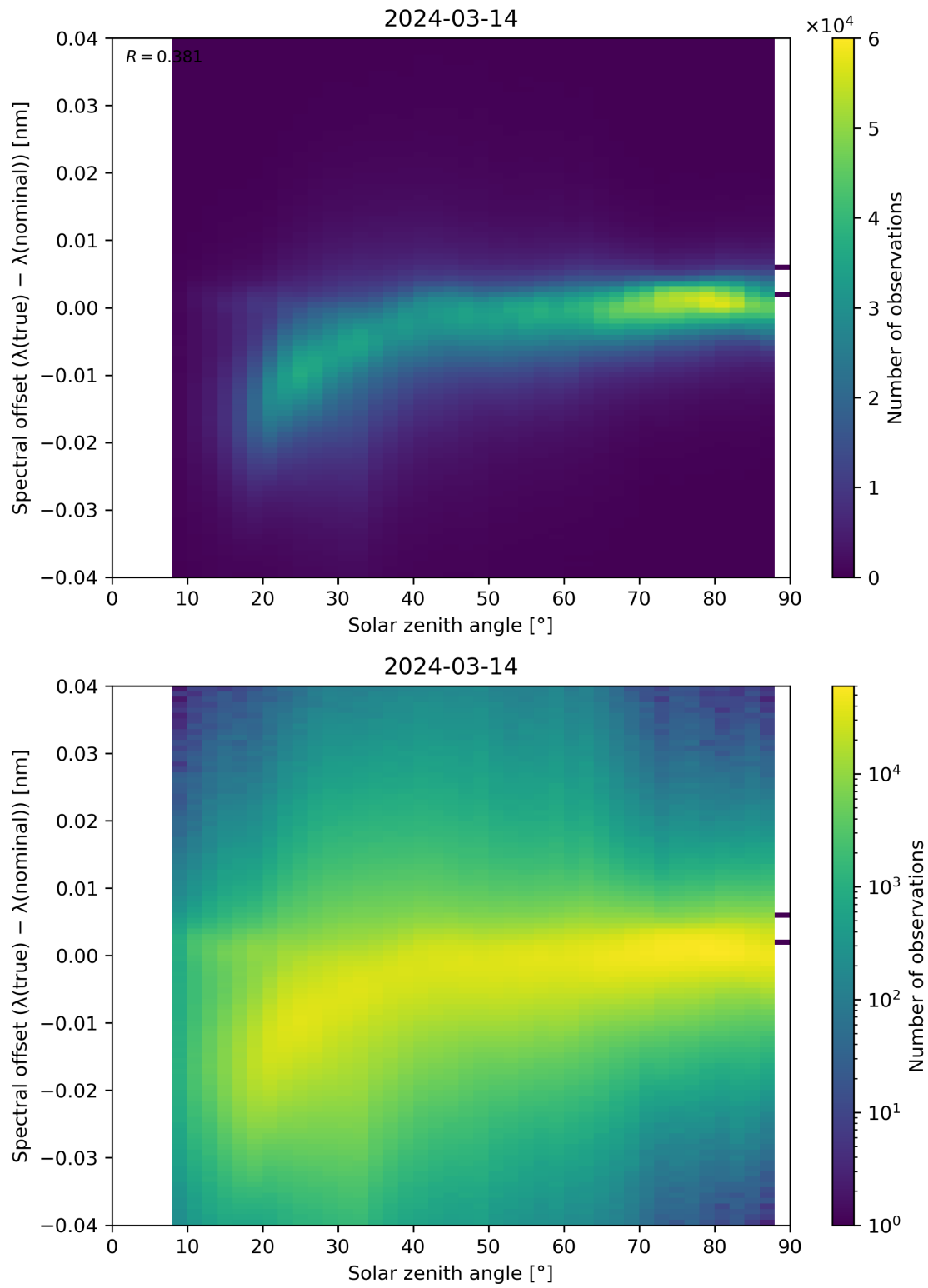
Figure 117: Scatter density plot of “Solar zenith angle” against “Spectral offset ( \lambda(\text{true}) - \lambda(\text{nominal}) )” for 2024-03-14 to 2024-03-15.
