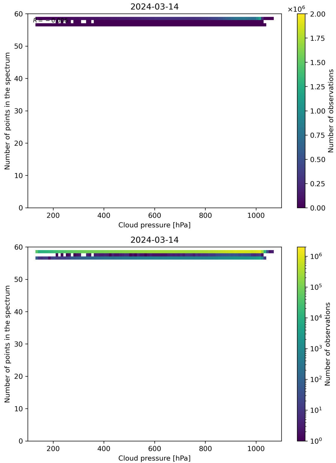
Figure 82: Scatter density plot of “Cloud pressure” against “Number of points in the spectrum” for 2024-03-14 to 2024-03-15.
