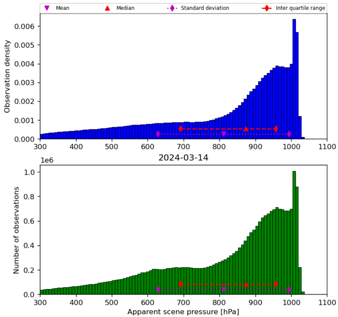
Figure 36: Histogram of “Apparent scene pressure” for 2024-03-14 to 2024-03-15
