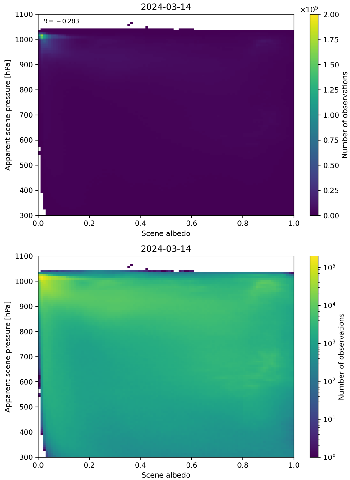
Figure 102: Scatter density plot of “Scene albedo” against “Apparent scene pressure” for 2024-03-14 to 2024-03-15.
