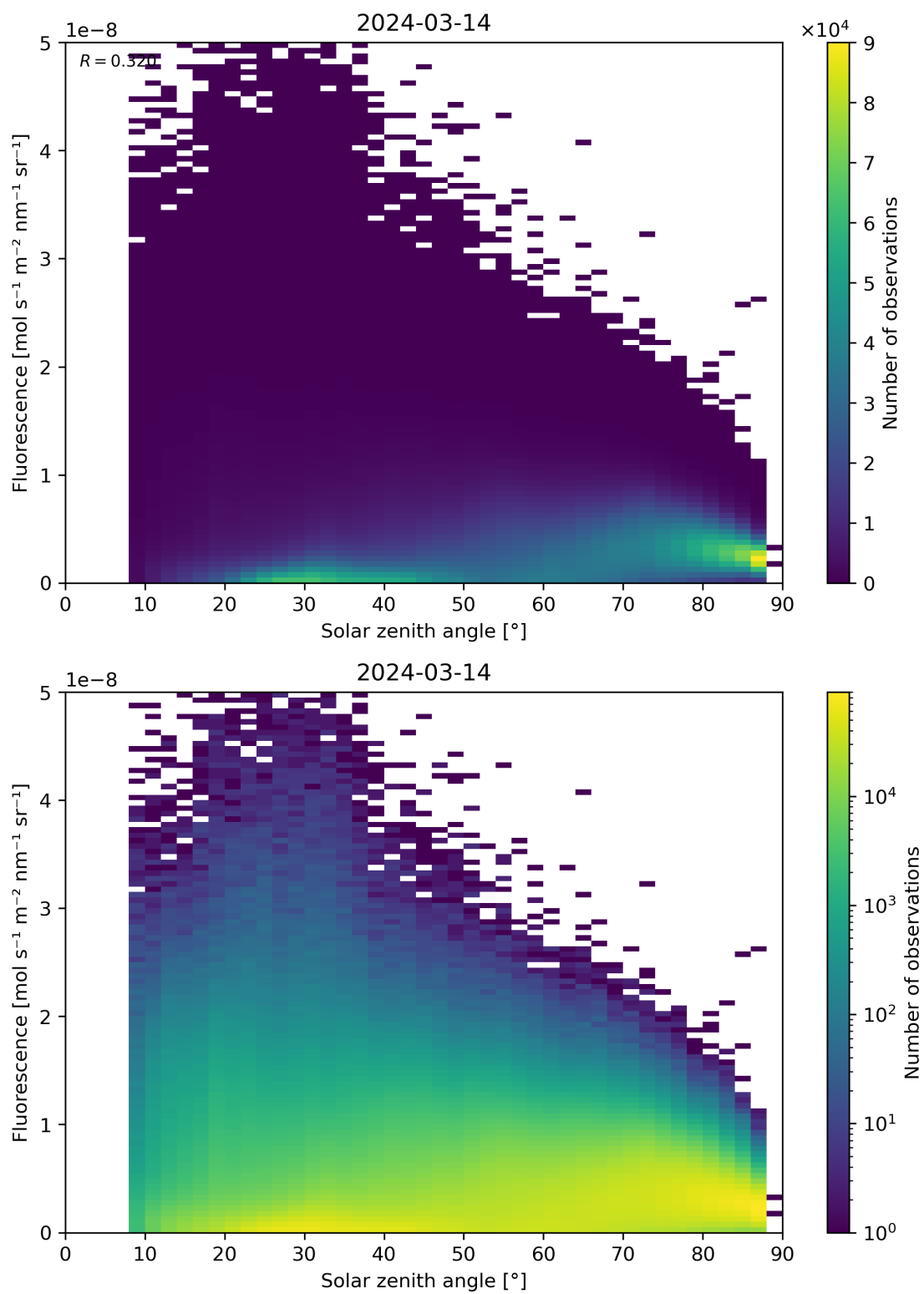
Figure 112: Scatter density plot of “Solar zenith angle” against “Fluorescence” for 2024-03-14 to 2024-03-15.
