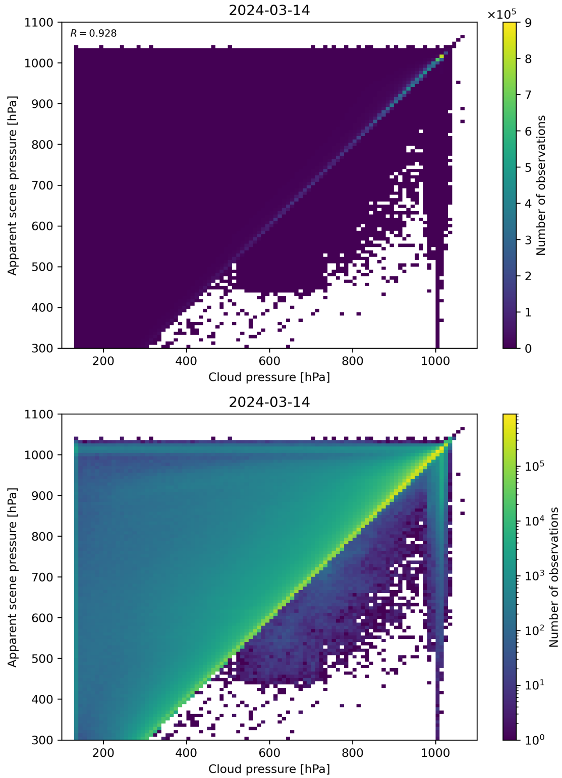
Figure 77: Scatter density plot of “Cloud pressure” against “Apparent scene pressure” for 2024-03-14 to 2024-03-15.
