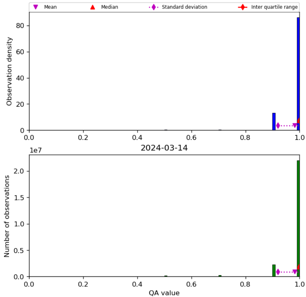
Figure 29: Histogram of “QA value” for 2024-03-14 to 2024-03-15
