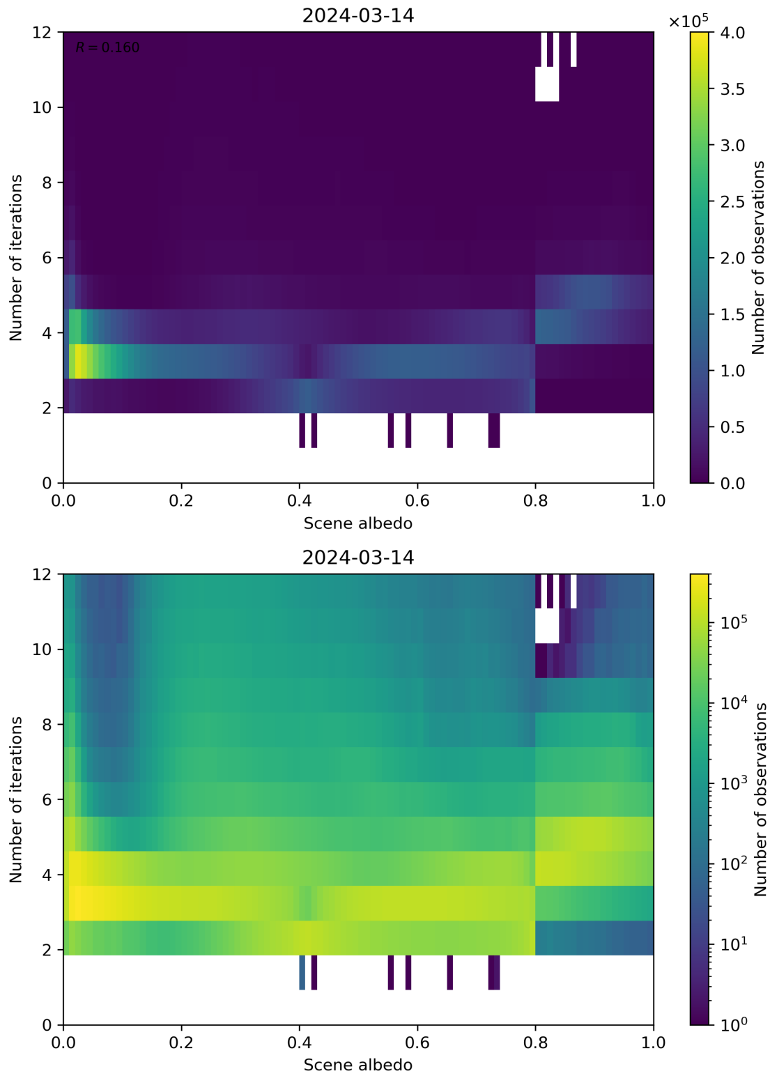
Figure 105: Scatter density plot of “Scene albedo” against “Number of iterations” for 2024-03-14 to 2024-03-15.
