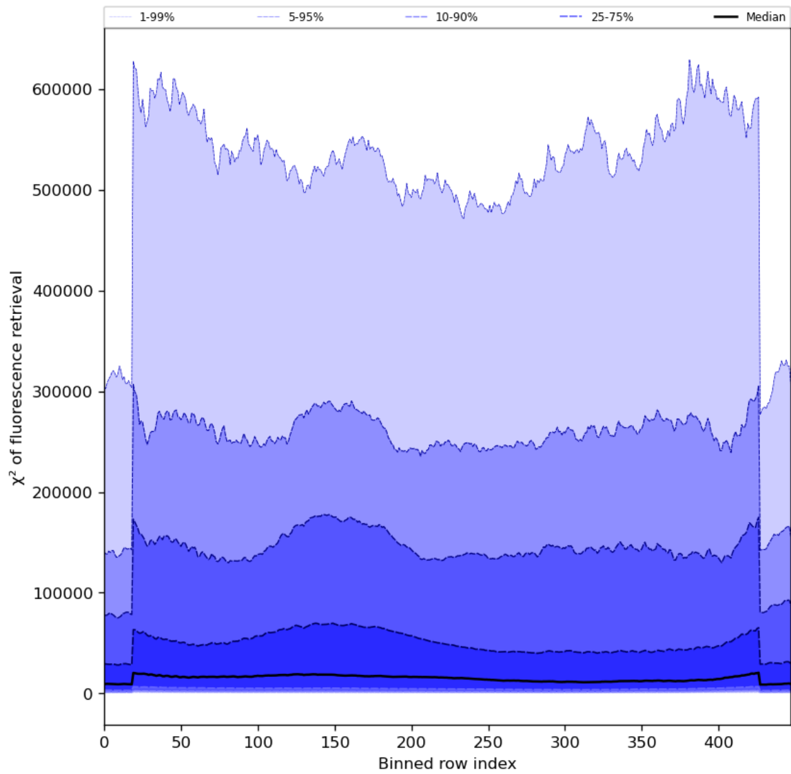
Figure 59: Along track statistics of “ \chi^2 of fluorescence retrieval” for 2024-03-14 to 2024-03-15
