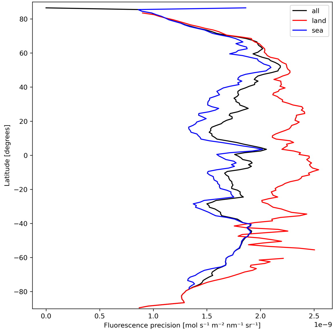
Figure 24: Zonal average of “Fluorescence precision” for 2024-03-14 to 2024-03-15.
