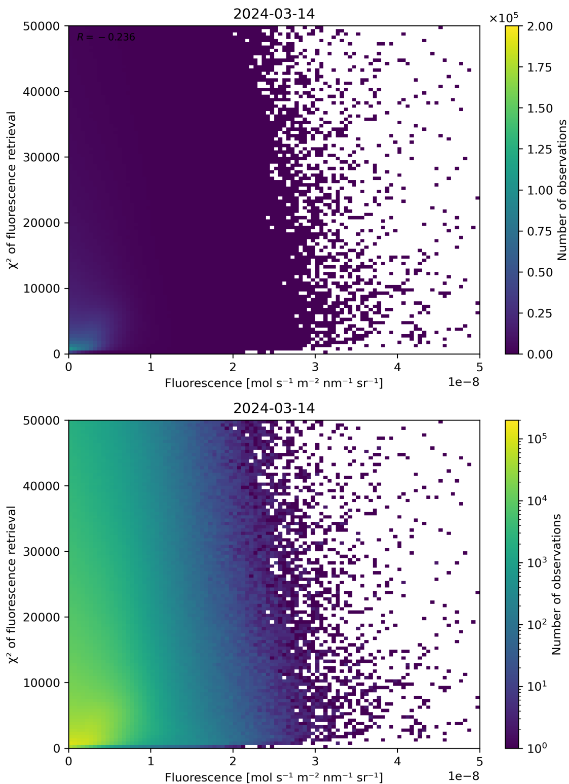
Figure 85: Scatter density plot of “Fluorescence” against “ \chi^2 of fluorescence retrieval” for 2024-03-14 to 2024-03-15.
