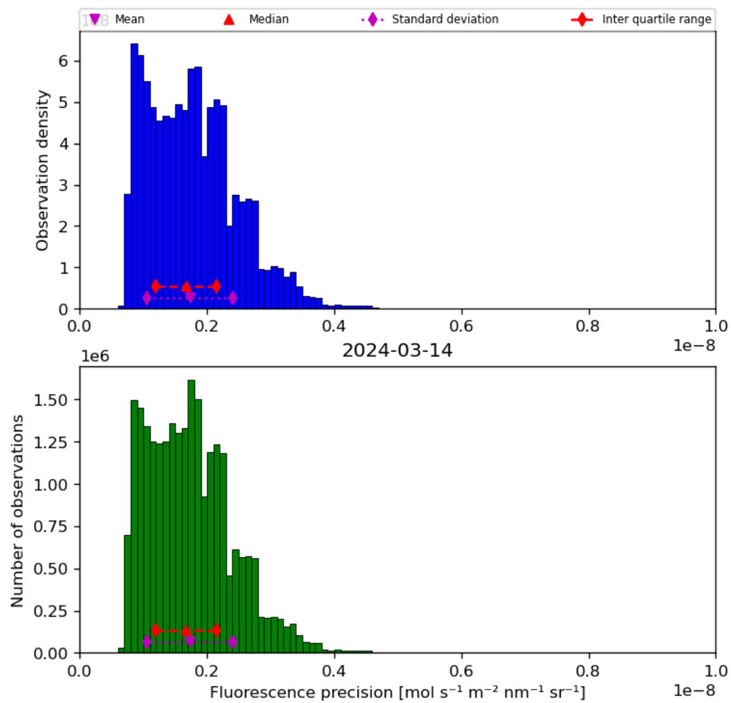
Figure 41: Histogram of “Fluorescence precision” for 2024-03-14 to 2024-03-15
