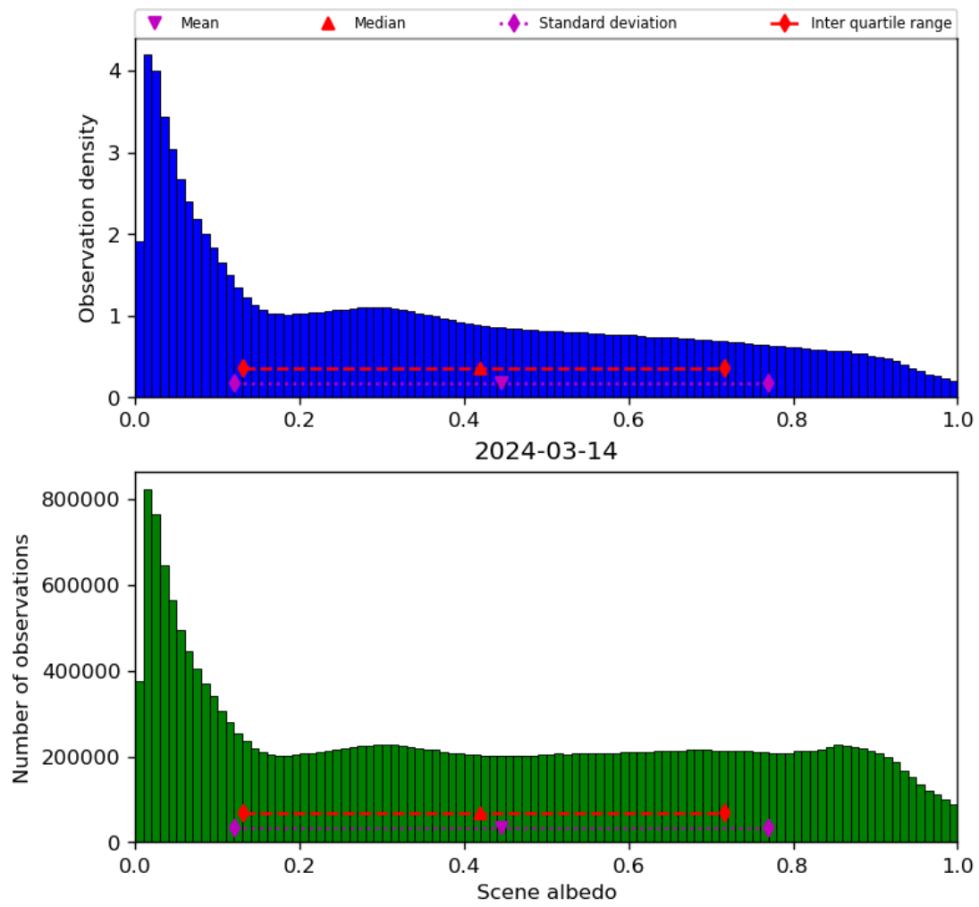
Figure 34: Histogram of “Scene albedo” for 2024-03-14 to 2024-03-15
