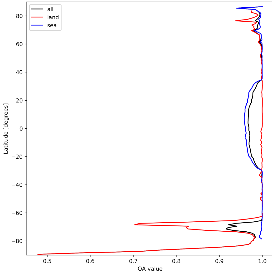
Figure 12: Zonal average of “QA value” for 2024-03-14 to 2024-03-15.
