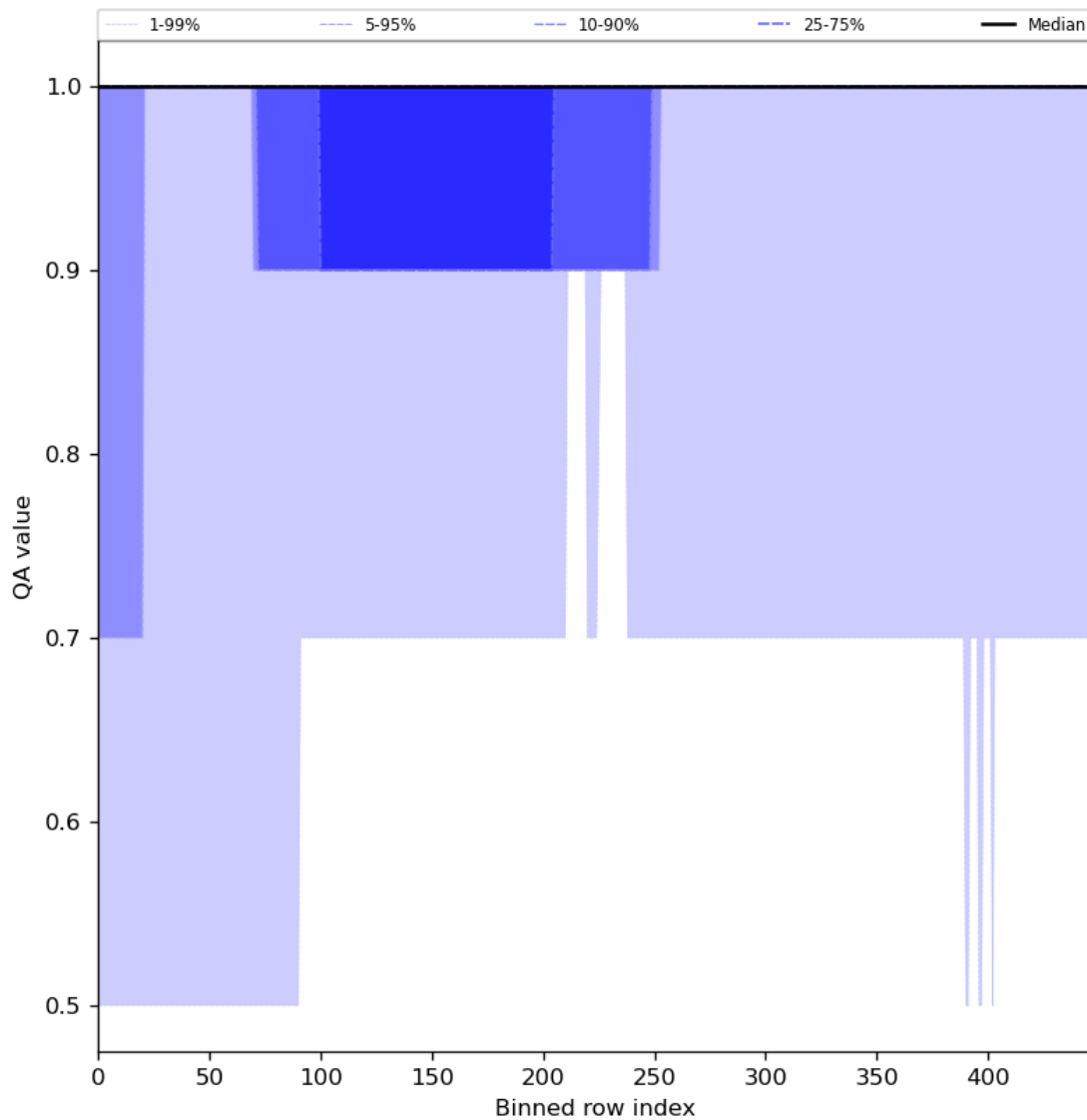
Figure 46: Along track statistics of “QA value” for 2024-03-14 to 2024-03-15
