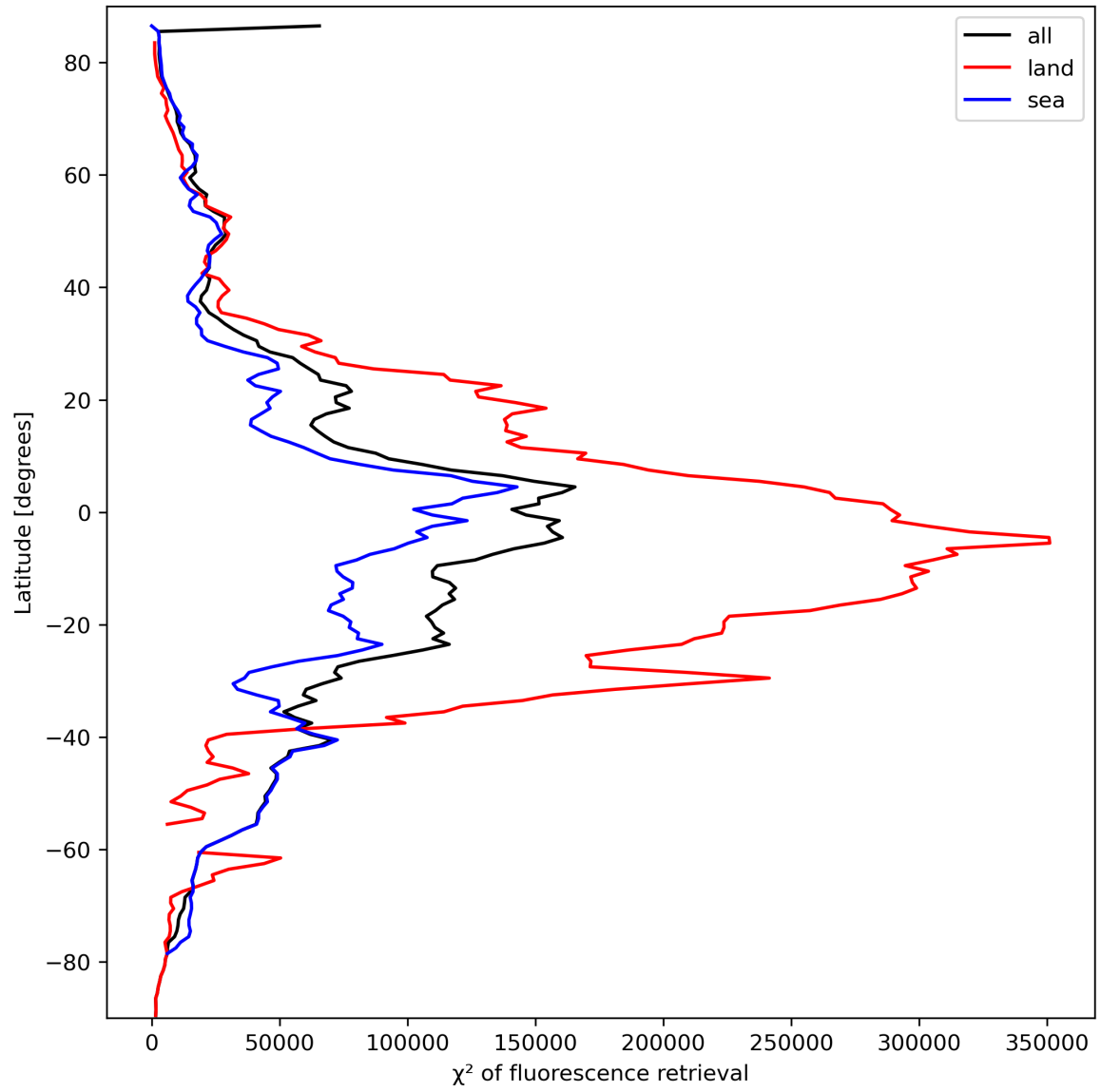
Figure 25: Zonal average of “ \chi^2 of fluorescence retrieval” for 2024-03-14 to 2024-03-15.
