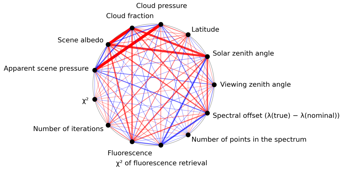
Figure 1: Map of correlation graph for 2024-03-14 to 2024-03-15.
