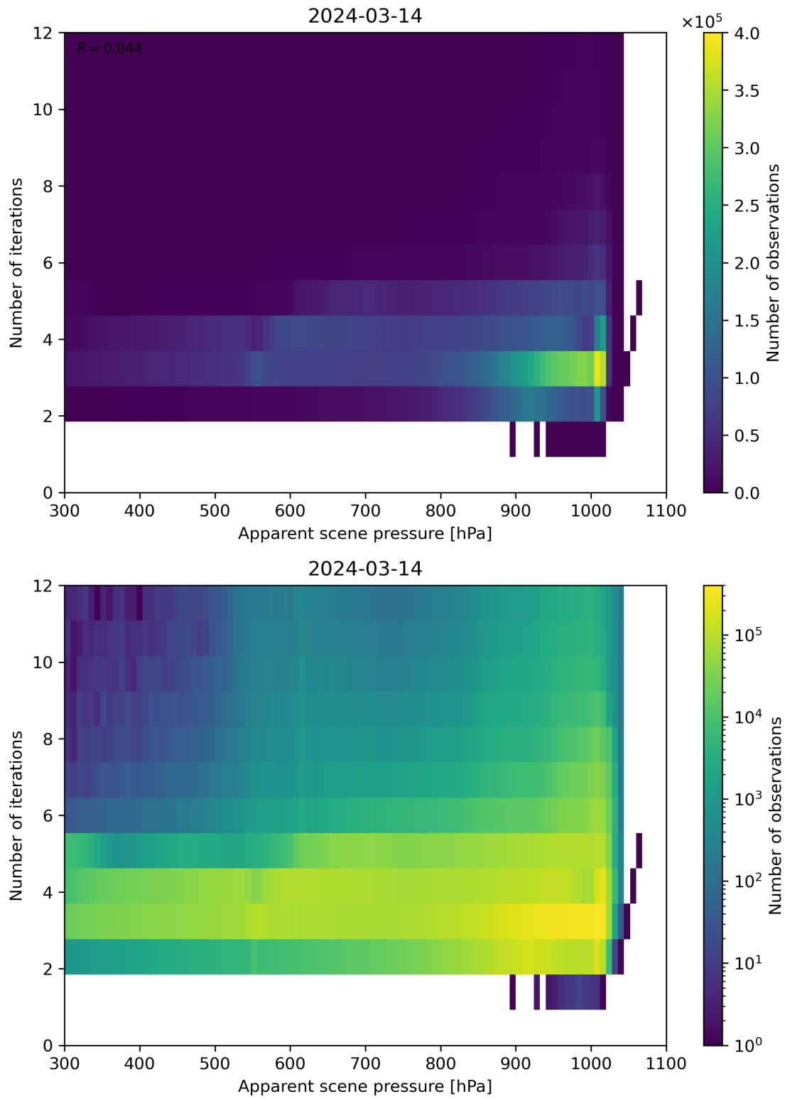
Figure 65: Scatter density plot of “Apparent scene pressure” against “Number of iterations” for 2024-03-14 to 2024-03-15.
