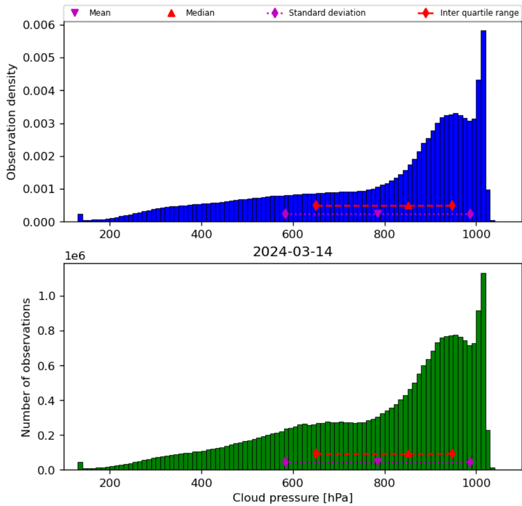
Figure 30: Histogram of “Cloud pressure” for 2024-03-14 to 2024-03-15
