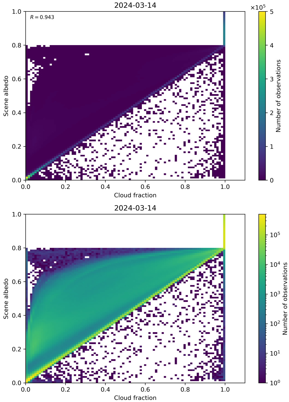
Figure 75: Scatter density plot of “Cloud fraction” against “Scene albedo” for 2024-03-14 to 2024-03-15.
