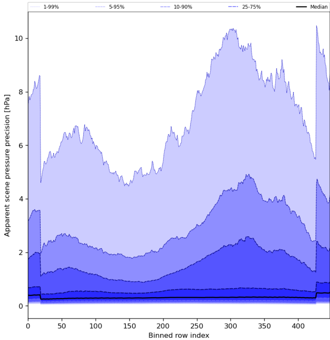
Figure 54: Along track statistics of “Apparent scene pressure precision” for 2024-03-14 to 2024-03-15
