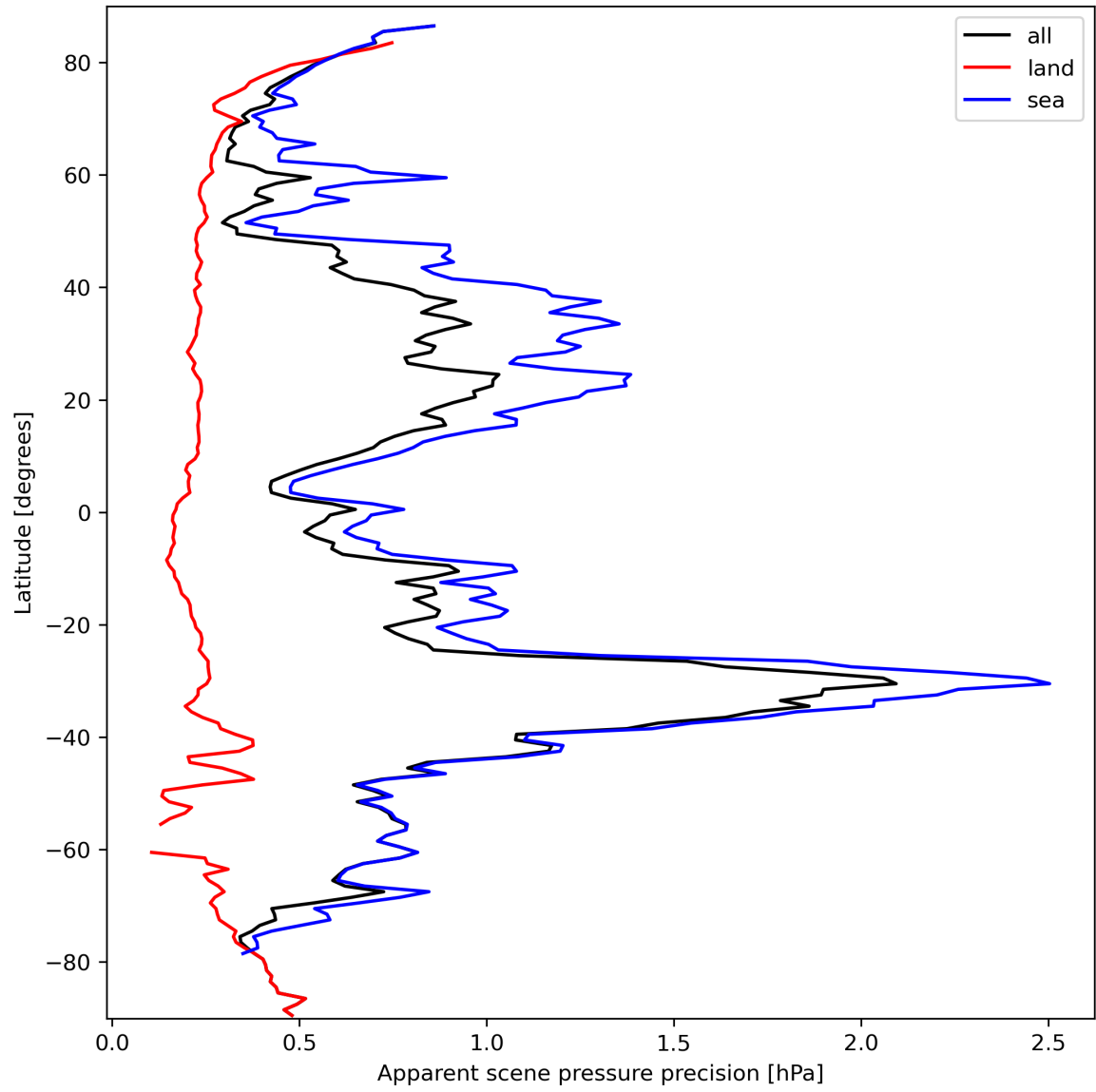
Figure 20: Zonal average of “Apparent scene pressure precision” for 2024-03-14 to 2024-03-15.
