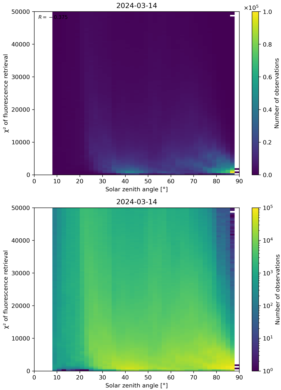
Figure 109: Scatter density plot of “Solar zenith angle” against “ \chi^2 of fluorescence retrieval” for 2024-03-14 to 2024-03-15.
