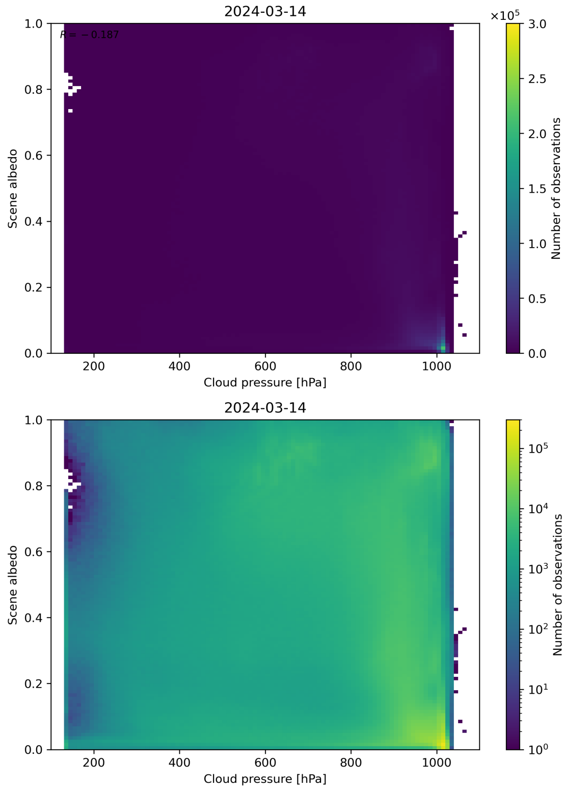
Figure 83: Scatter density plot of “Cloud pressure” against “Scene albedo” for 2024-03-14 to 2024-03-15.
