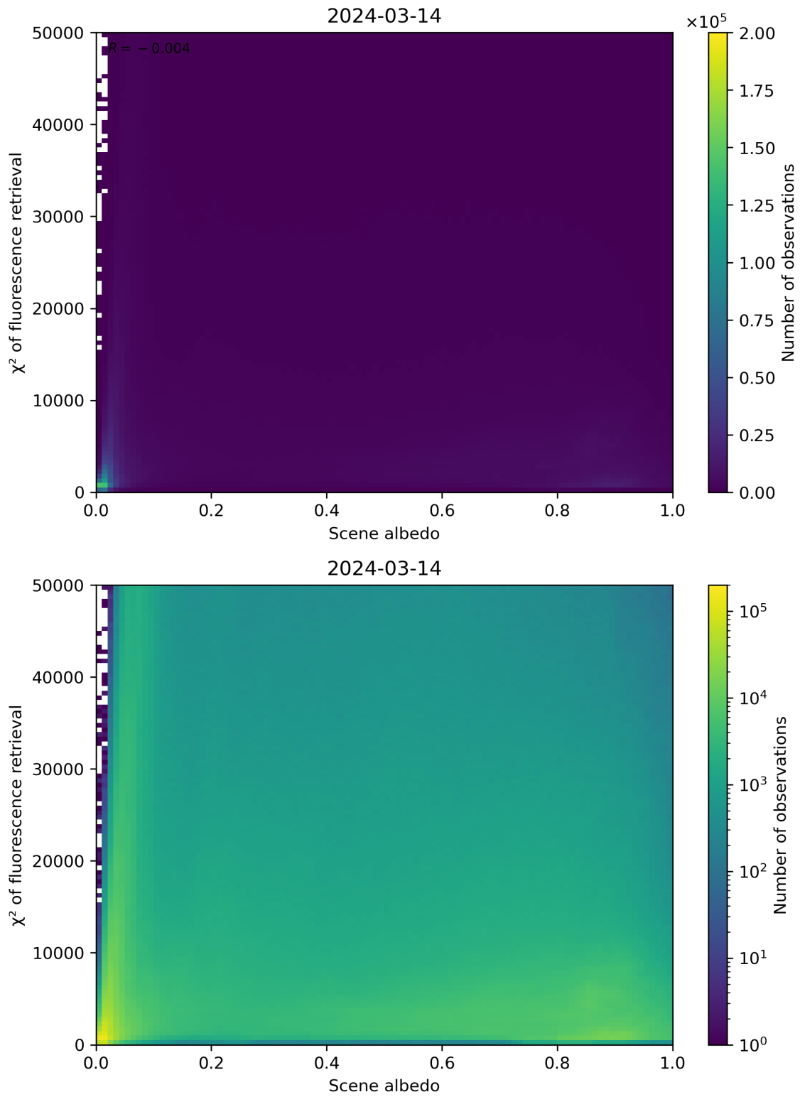
Figure 103: Scatter density plot of “Scene albedo” against “ \chi^2 of fluorescence retrieval” for 2024-03-14 to 2024-03-15.
