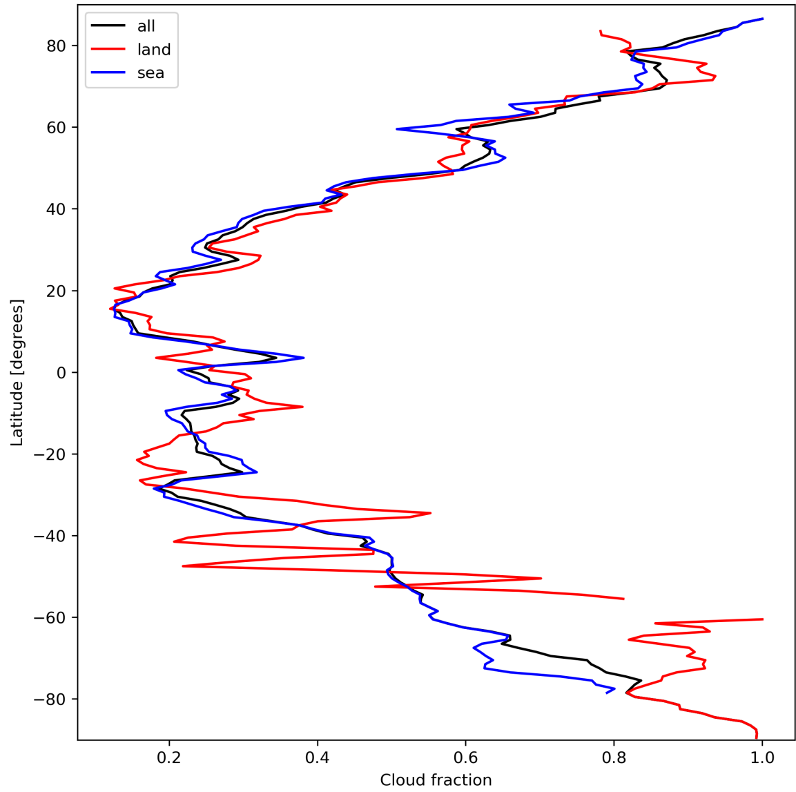
Figure 15: Zonal average of “Cloud fraction” for 2024-03-14 to 2024-03-15.
