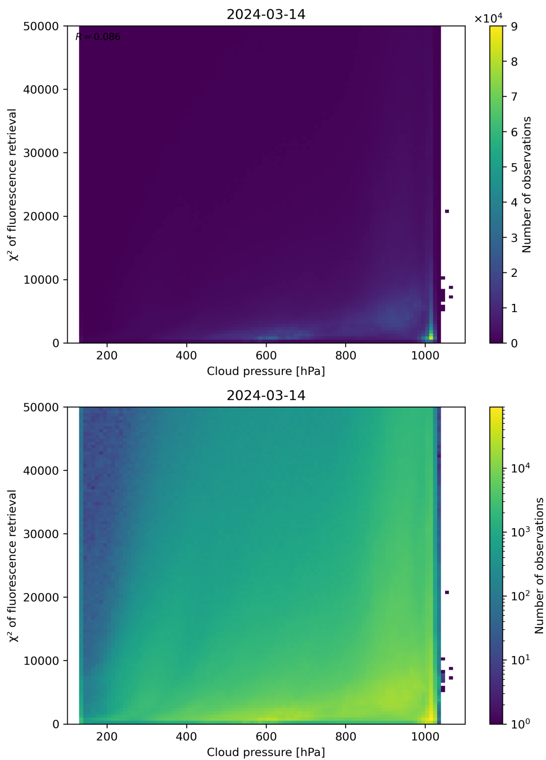
Figure 78: Scatter density plot of “Cloud pressure” against “ \chi^2 of fluorescence retrieval” for 2024-03-14 to 2024-03-15.
