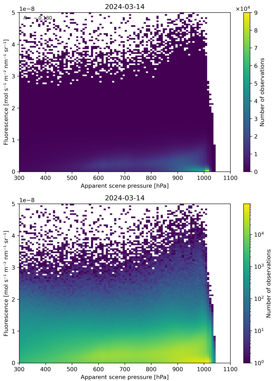
Figure 64: Scatter density plot of “Apparent scene pressure” against “Fluorescence” for 2024-03-14 to 2024-03-15.
