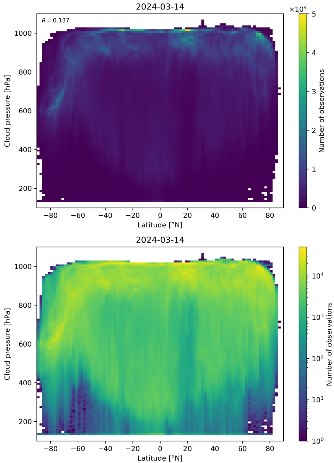
Figure 91: Scatter density plot of “Latitude” against “Cloud pressure” for 2024-03-14 to 2024-03-15.
