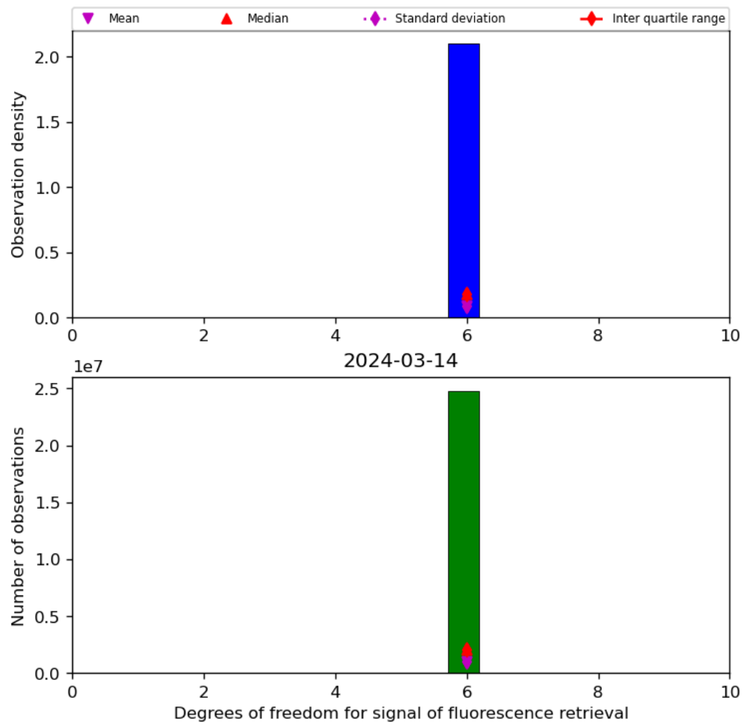
Figure 43: Histogram of “Degrees of freedom for signal of fluorescence retrieval” for 2024-03-14 to 2024-03-15
