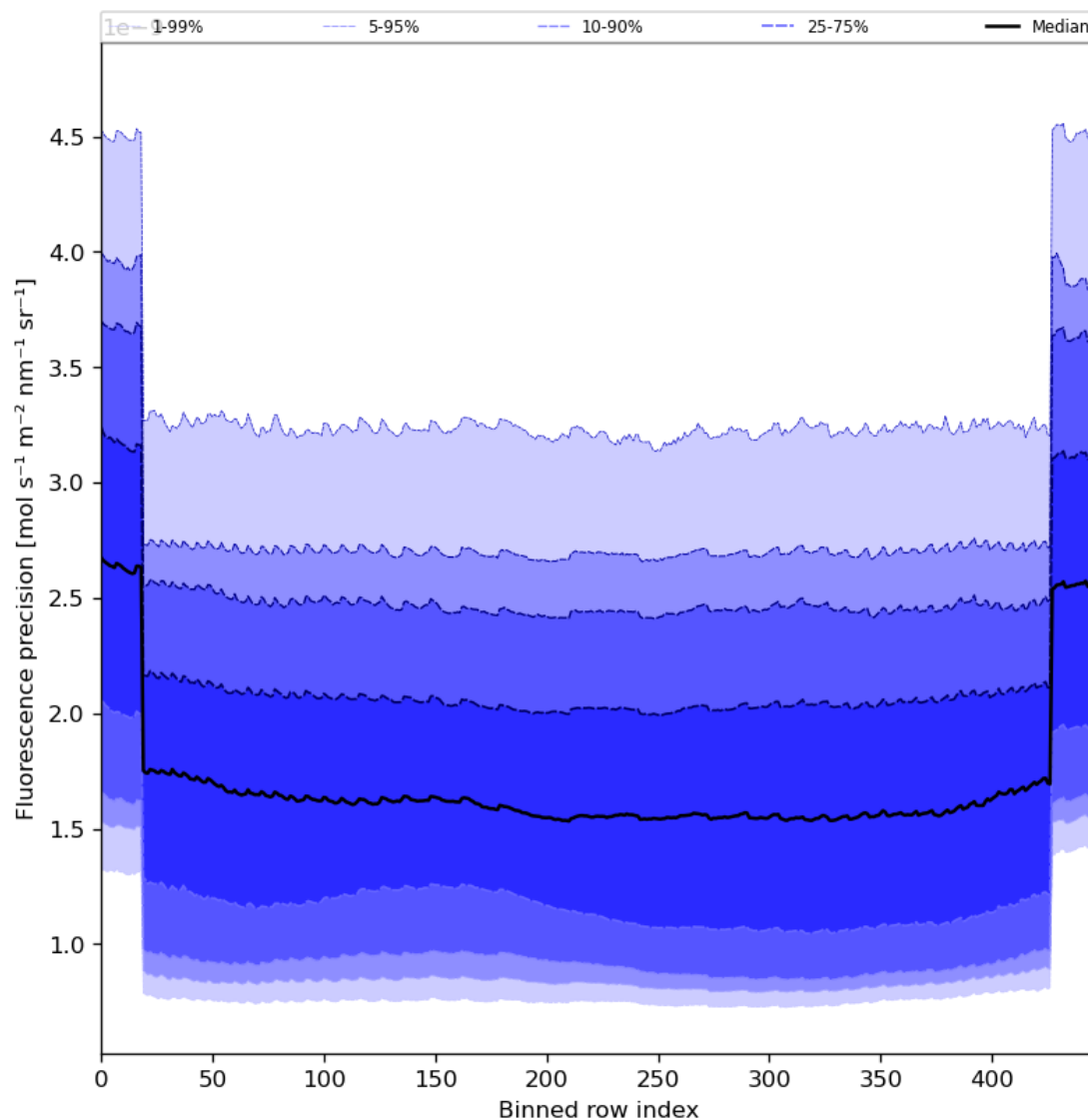
Figure 58: Along track statistics of “Fluorescence precision” for 2024-03-14 to 2024-03-15
