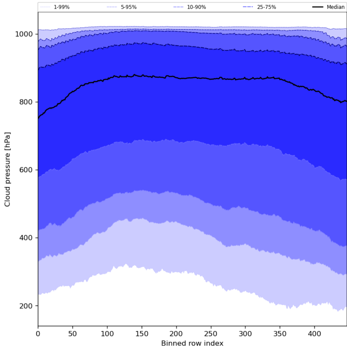
Figure 47: Along track statistics of “Cloud pressure” for 2024-03-14 to 2024-03-15
