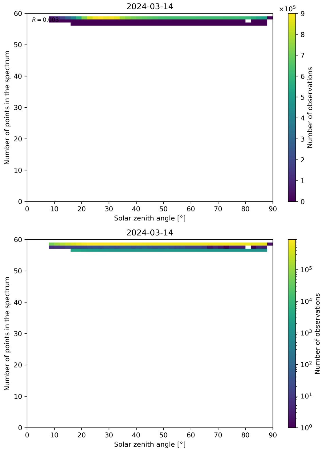
Figure 115: Scatter density plot of “Solar zenith angle” against “Number of points in the spectrum” for 2024-03-14 to 2024-03-15.
