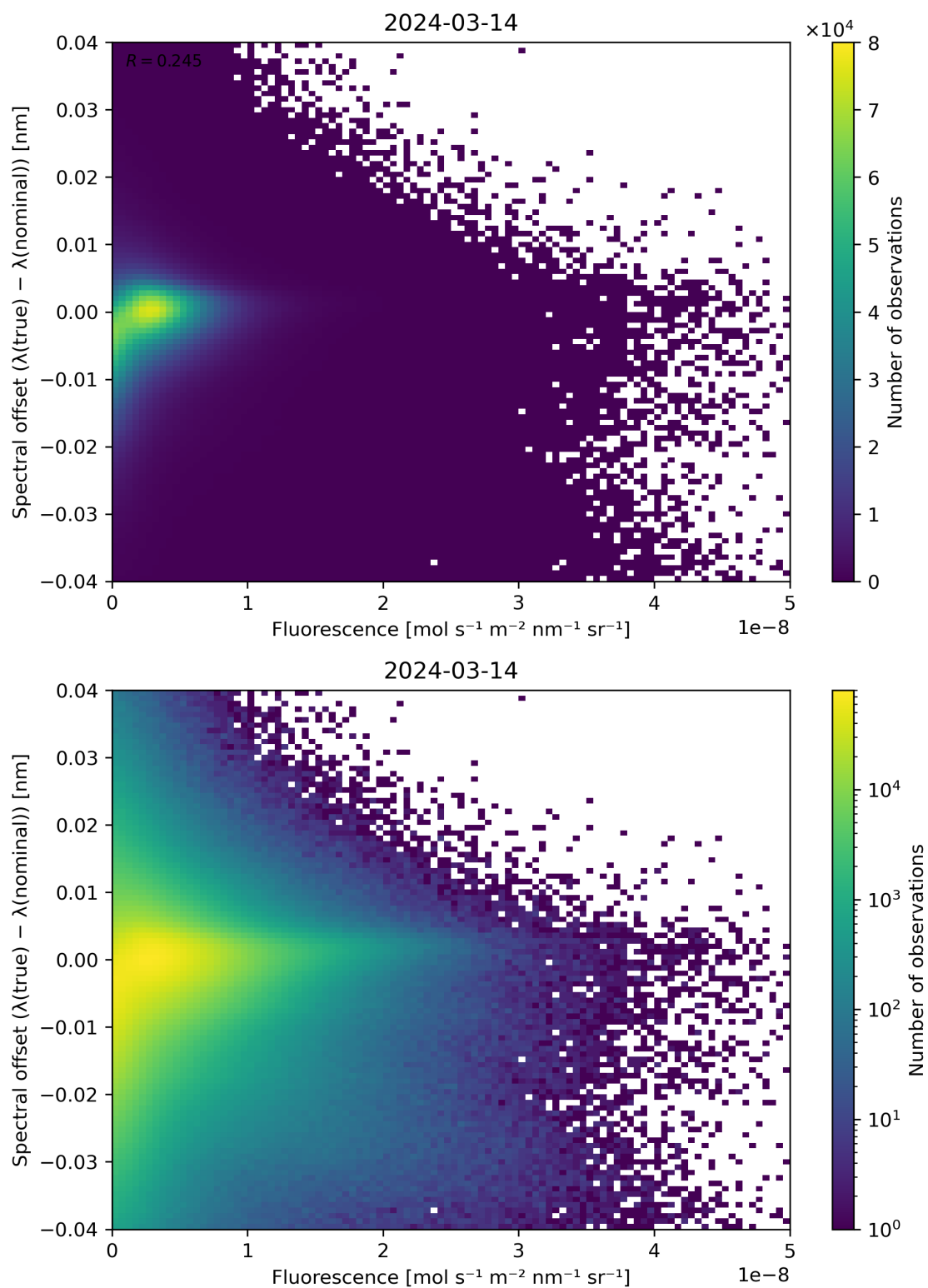
Figure 87: Scatter density plot of “Fluorescence” against “Spectral offset ( \lambda(\text{true}) - \lambda(\text{nominal}) )” for 2024-03-14 to 2024-03-15.
