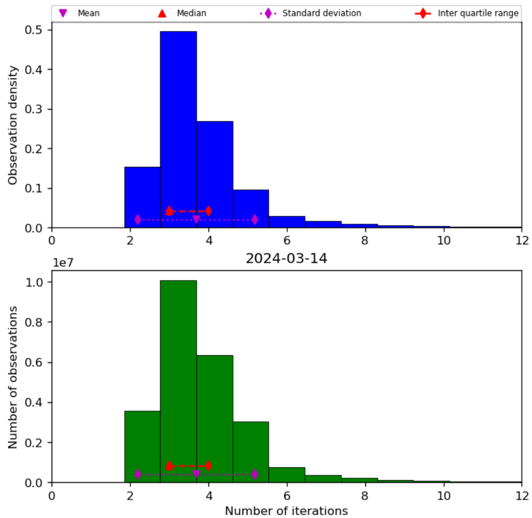
Figure 39: Histogram of “Number of iterations” for 2024-03-14 to 2024-03-15
