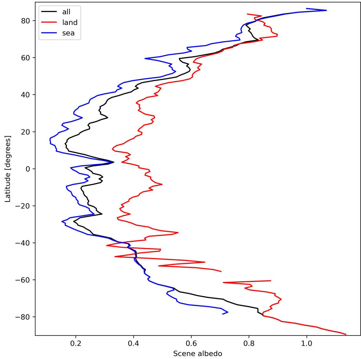
Figure 17: Zonal average of “Scene albedo” for 2024-03-14 to 2024-03-15.
