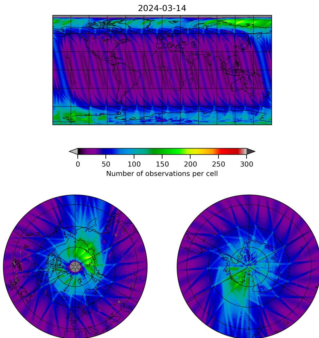
Figure 11: Map of the number of observations for 2024-03-14 to 2024-03-15
