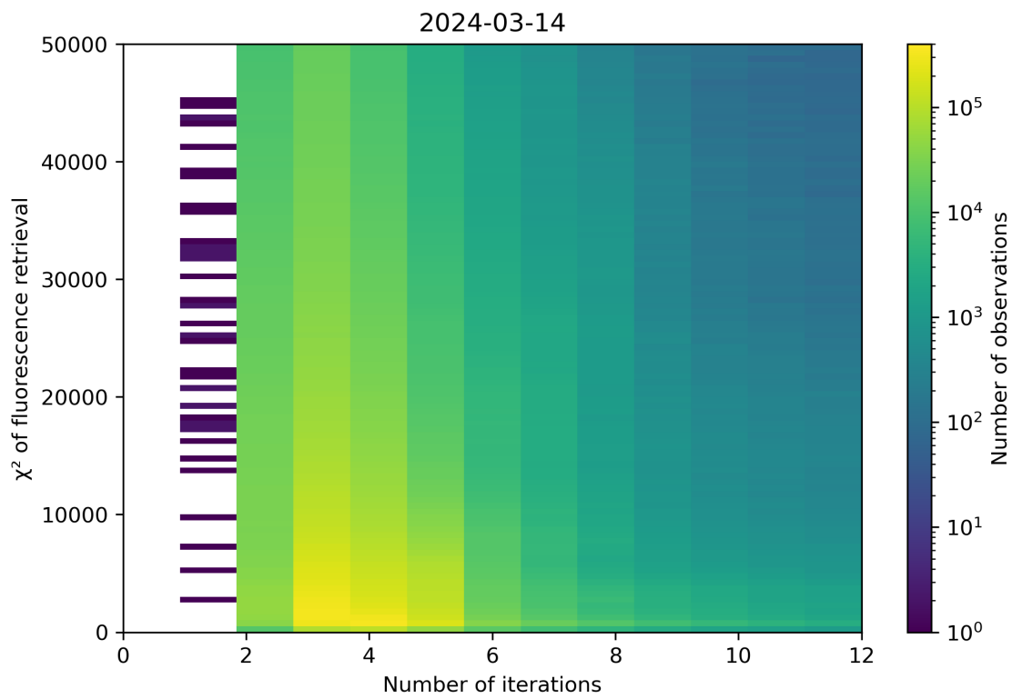
Figure 97: Scatter density plot of “Number of iterations” against “ \chi^2 of fluorescence retrieval” for 2024-03-14 to 2024-03-15.
