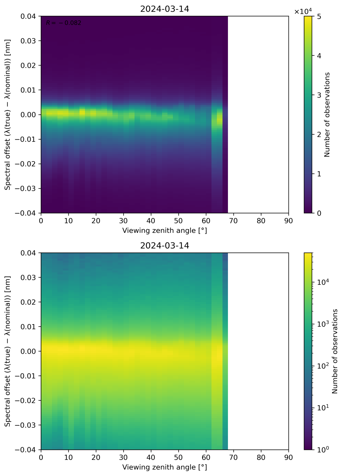
Figure 128: Scatter density plot of “Viewing zenith angle” against “Spectral offset ( \lambda(\text{true}) - \lambda(\text{nominal}) )” for 2024-03-14 to 2024-03-15.
