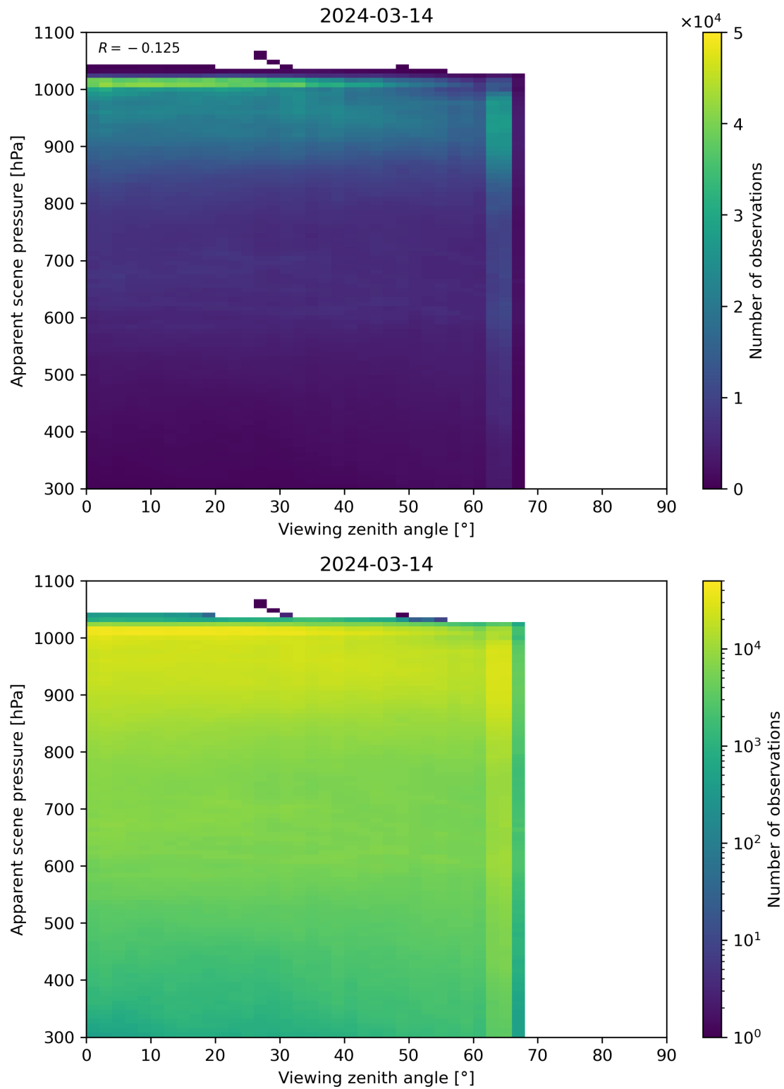
Figure 118: Scatter density plot of “Viewing zenith angle” against “Apparent scene pressure” for 2024-03-14 to 2024-03-15.
