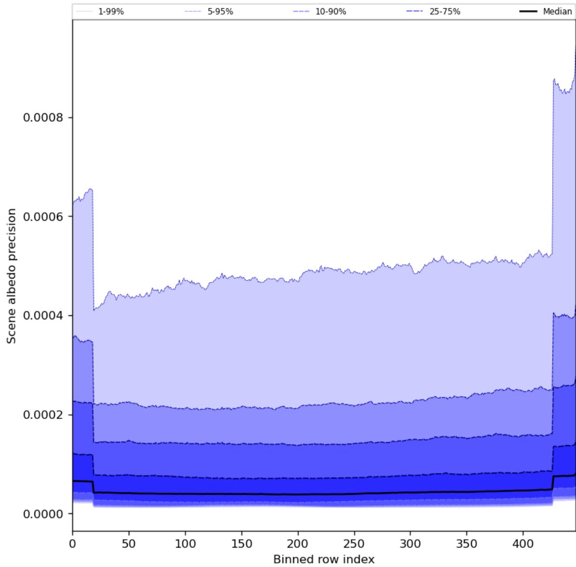
Figure 52: Along track statistics of “Scene albedo precision” for 2024-03-14 to 2024-03-15
