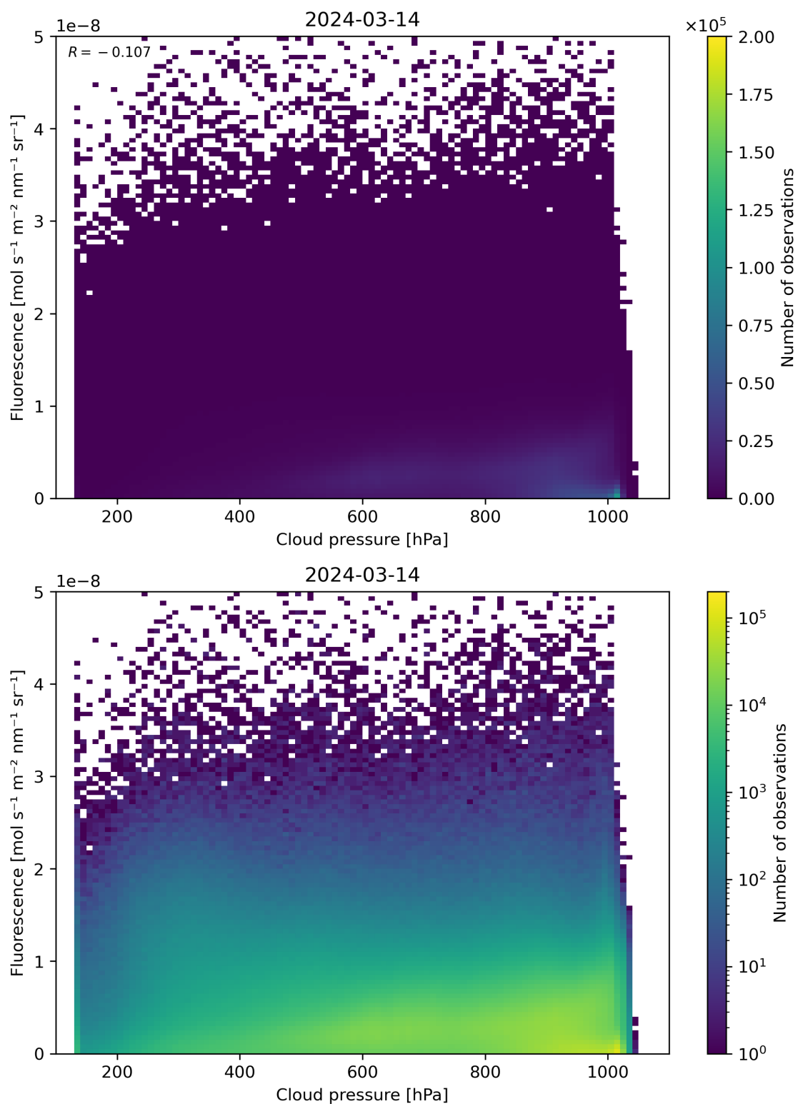
Figure 80: Scatter density plot of “Cloud pressure” against “Fluorescence” for 2024-03-14 to 2024-03-15.
