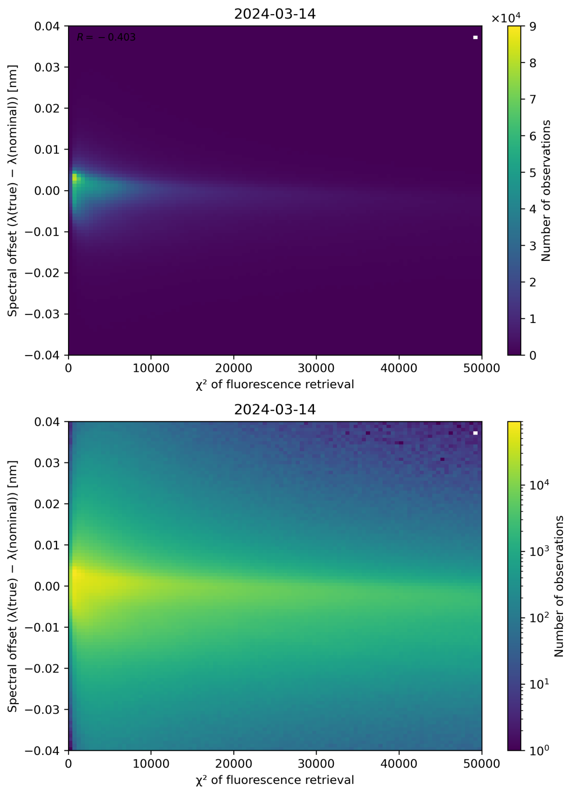
Figure 69: Scatter density plot of “ \chi^2 of fluorescence retrieval” against “Spectral offset ( \lambda(\text{true}) - \lambda(\text{nominal}) )” for 2024-03-14 to 2024-03-15.
