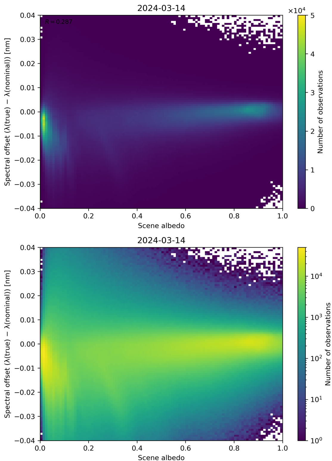
Figure 107: Scatter density plot of “Scene albedo” against “Spectral offset ( \lambda(\text{true}) - \lambda(\text{nominal}) )” for 2024-03-14 to 2024-03-15.
