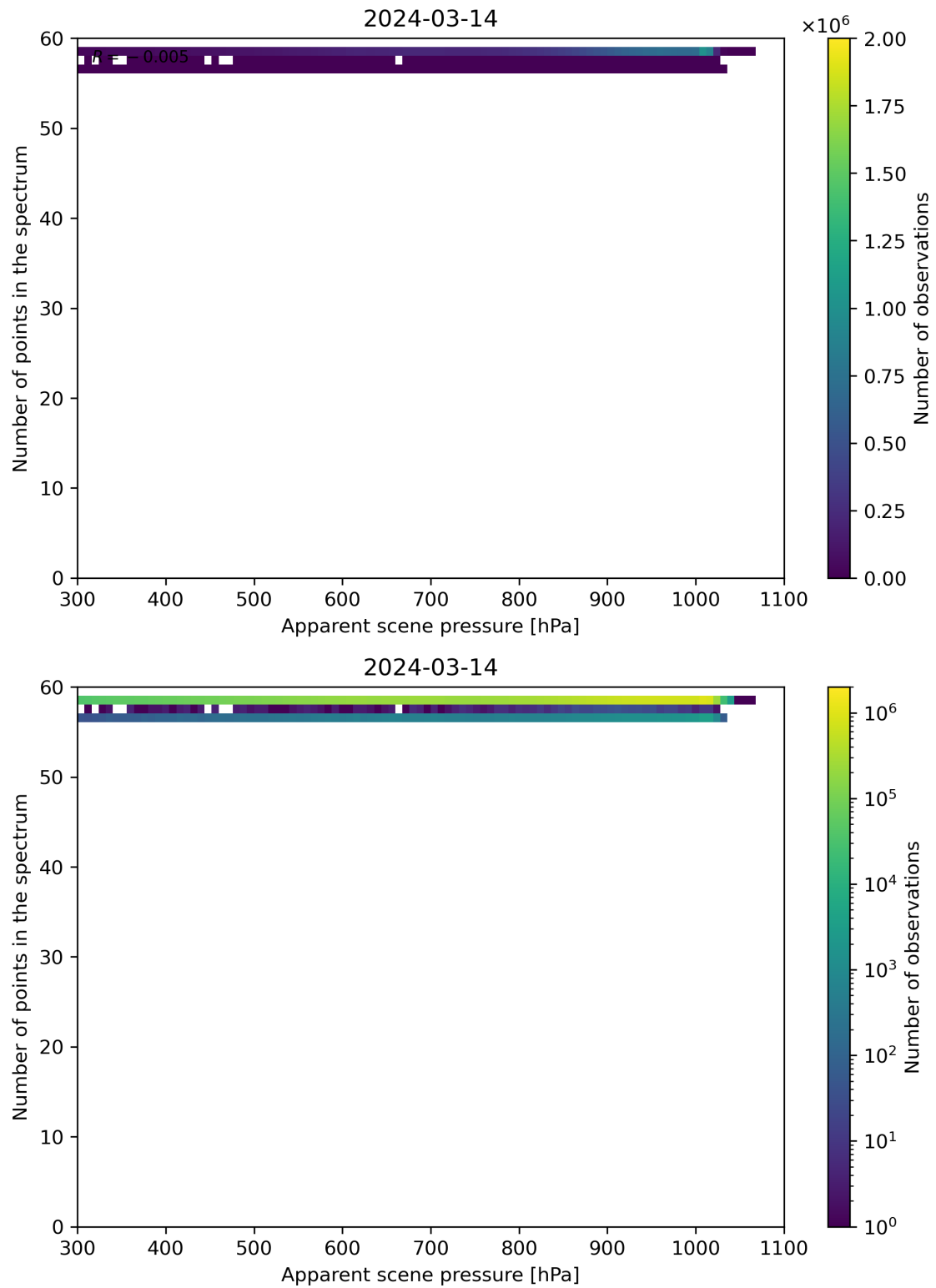
Figure 66: Scatter density plot of “Apparent scene pressure” against “Number of points in the spectrum” for 2024-03-14 to 2024-03-15.
