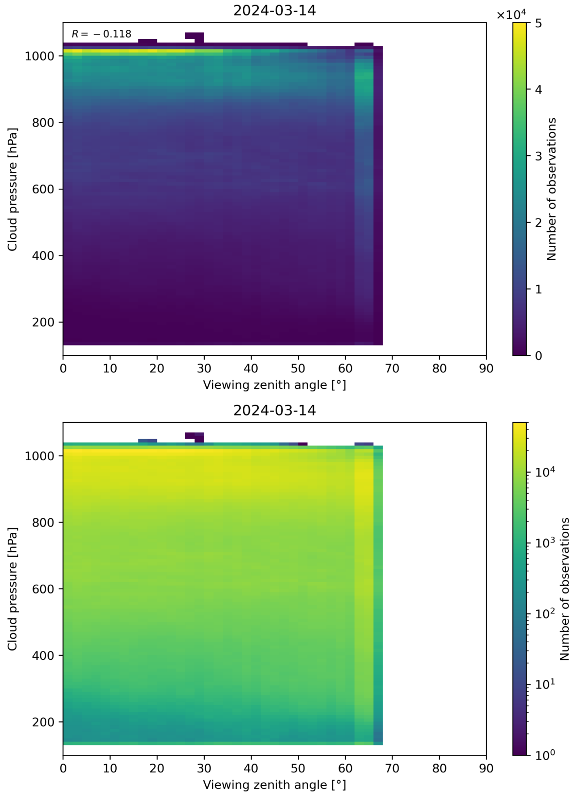
Figure 121: Scatter density plot of “Viewing zenith angle” against “Cloud pressure” for 2024-03-14 to 2024-03-15.
