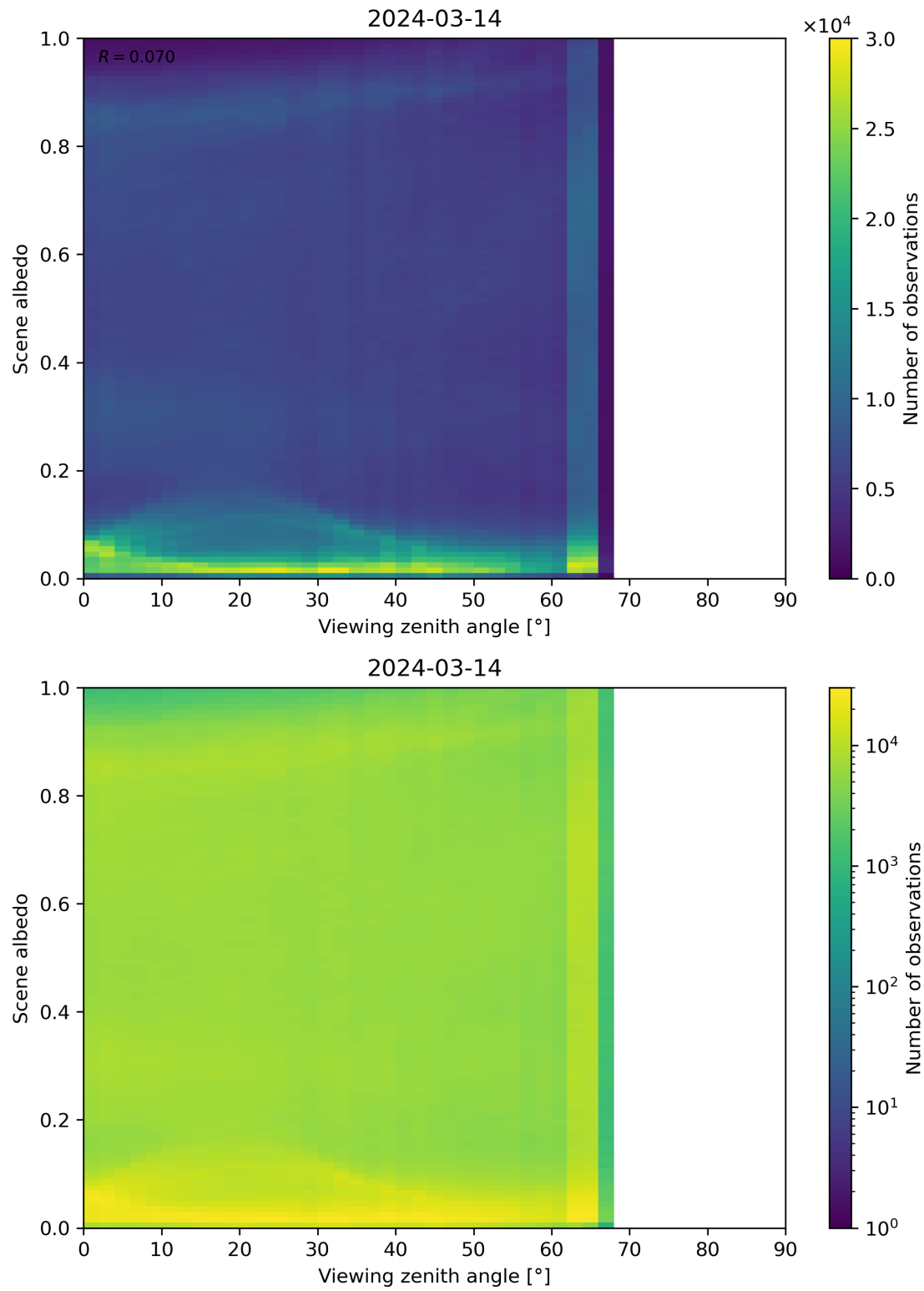
Figure 126: Scatter density plot of “Viewing zenith angle” against “Scene albedo” for 2024-03-14 to 2024-03-15.
