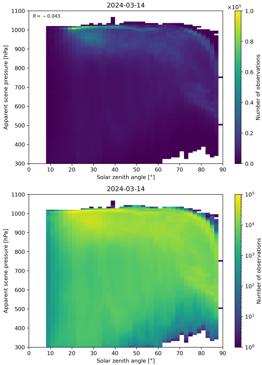
Figure 108: Scatter density plot of “Solar zenith angle” against “Apparent scene pressure” for 2024-03-14 to 2024-03-15.
