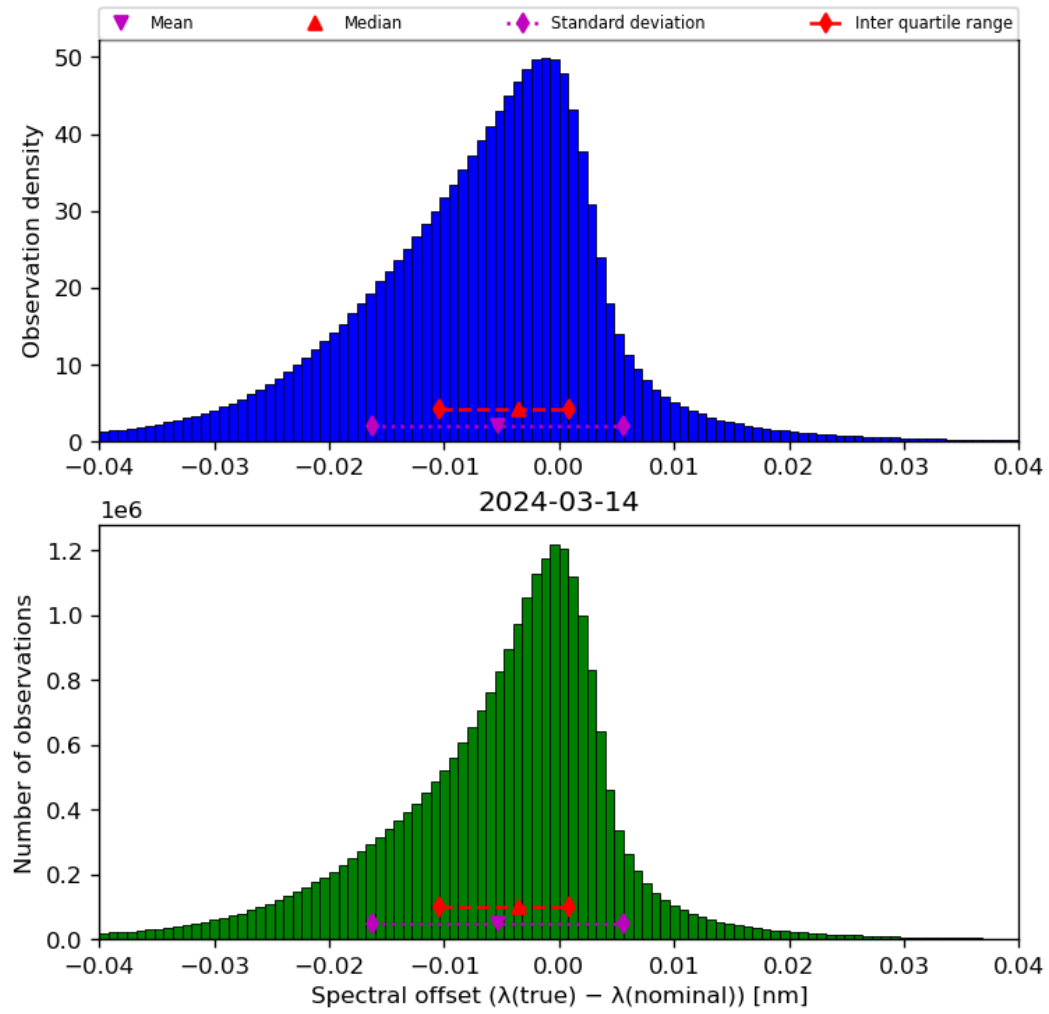
Figure 45: Histogram of “Spectral offset ( \lambda(\text{true}) - \lambda(\text{nominal}) )” for 2024-03-14 to 2024-03-15
