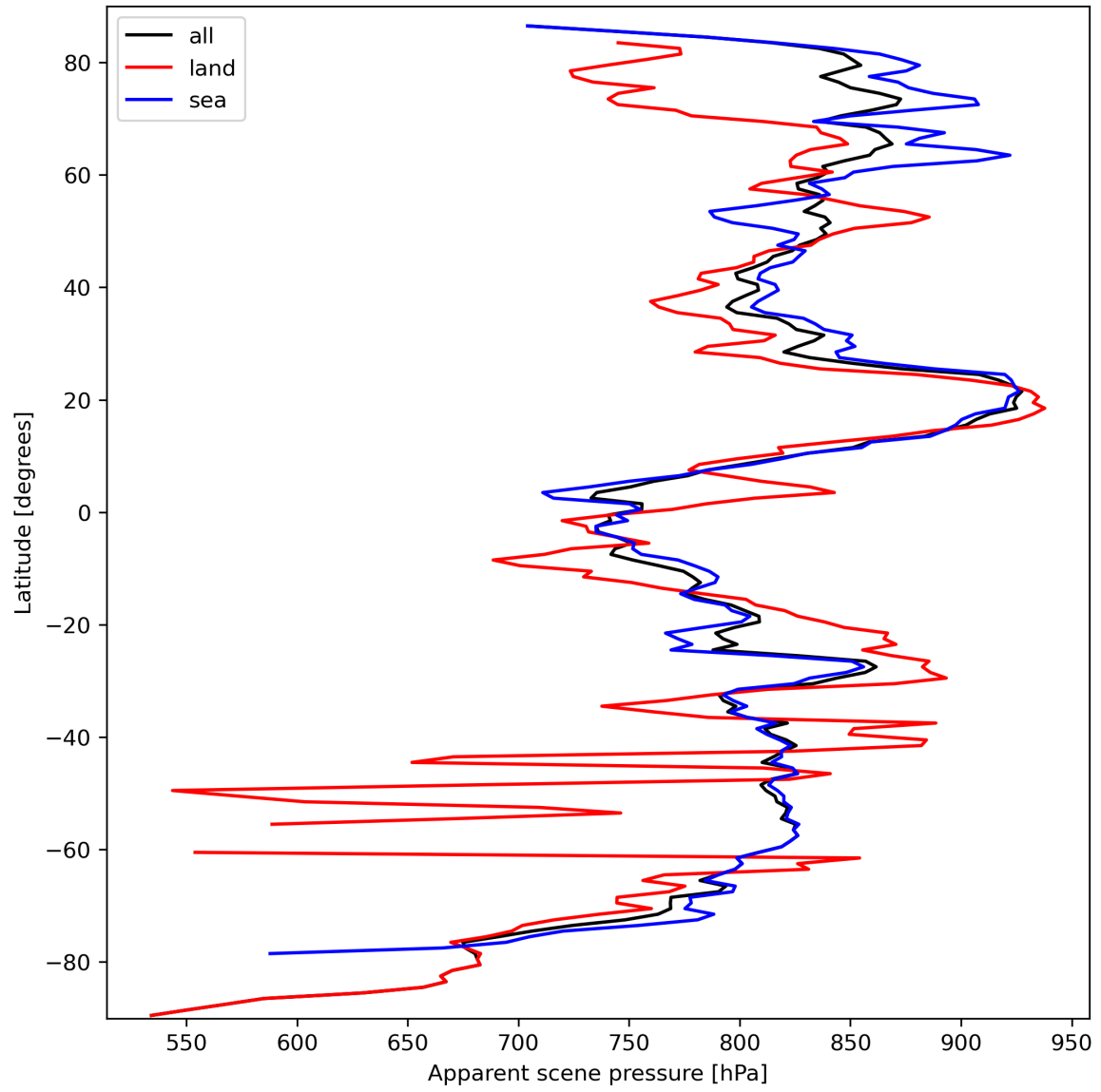
Figure 19: Zonal average of “Apparent scene pressure” for 2024-03-14 to 2024-03-15.
