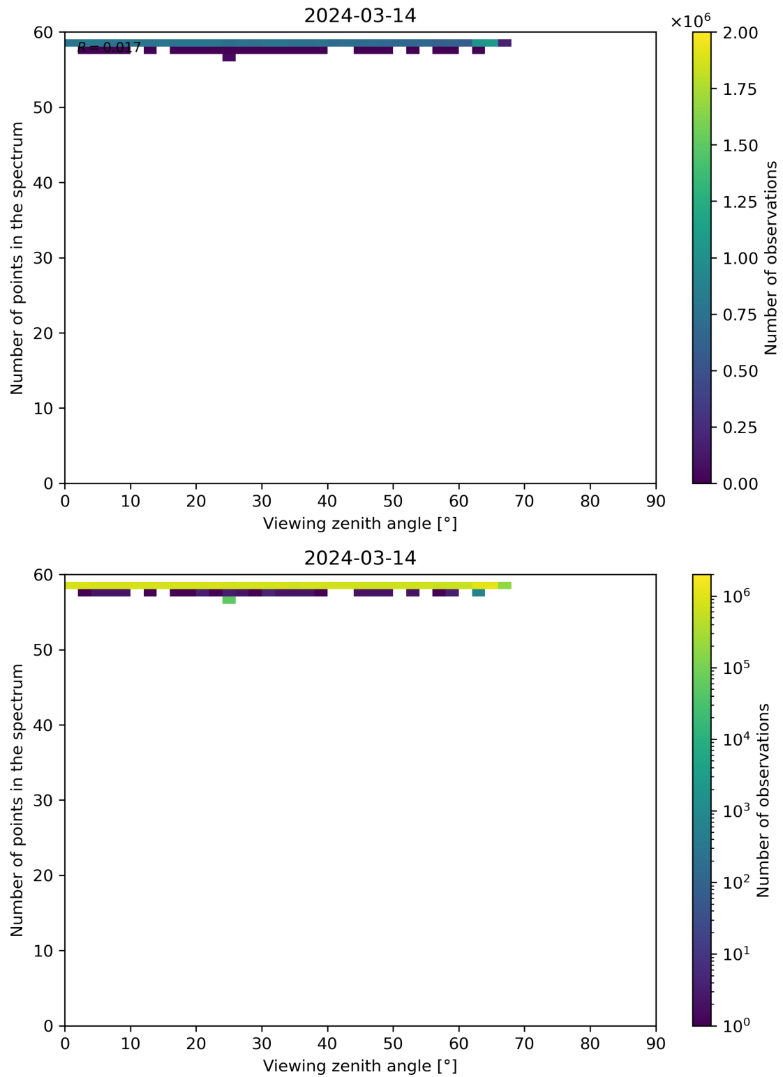
Figure 125: Scatter density plot of “Viewing zenith angle” against “Number of points in the spectrum” for 2024-03-14 to 2024-03-15.
