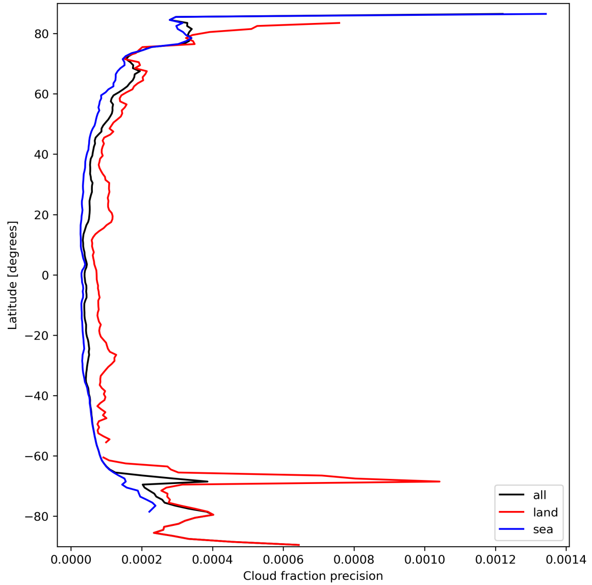
Figure 16: Zonal average of “Cloud fraction precision” for 2024-03-14 to 2024-03-15.
