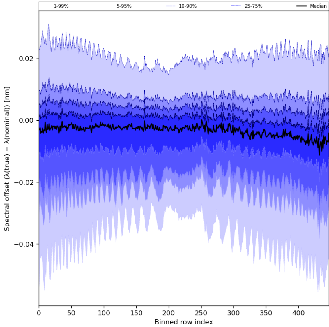
Figure 62: Along track statistics of “Spectral offset ( \lambda(\text{true}) - \lambda(\text{nominal}) )” for 2024-03-14 to 2024-03-15
