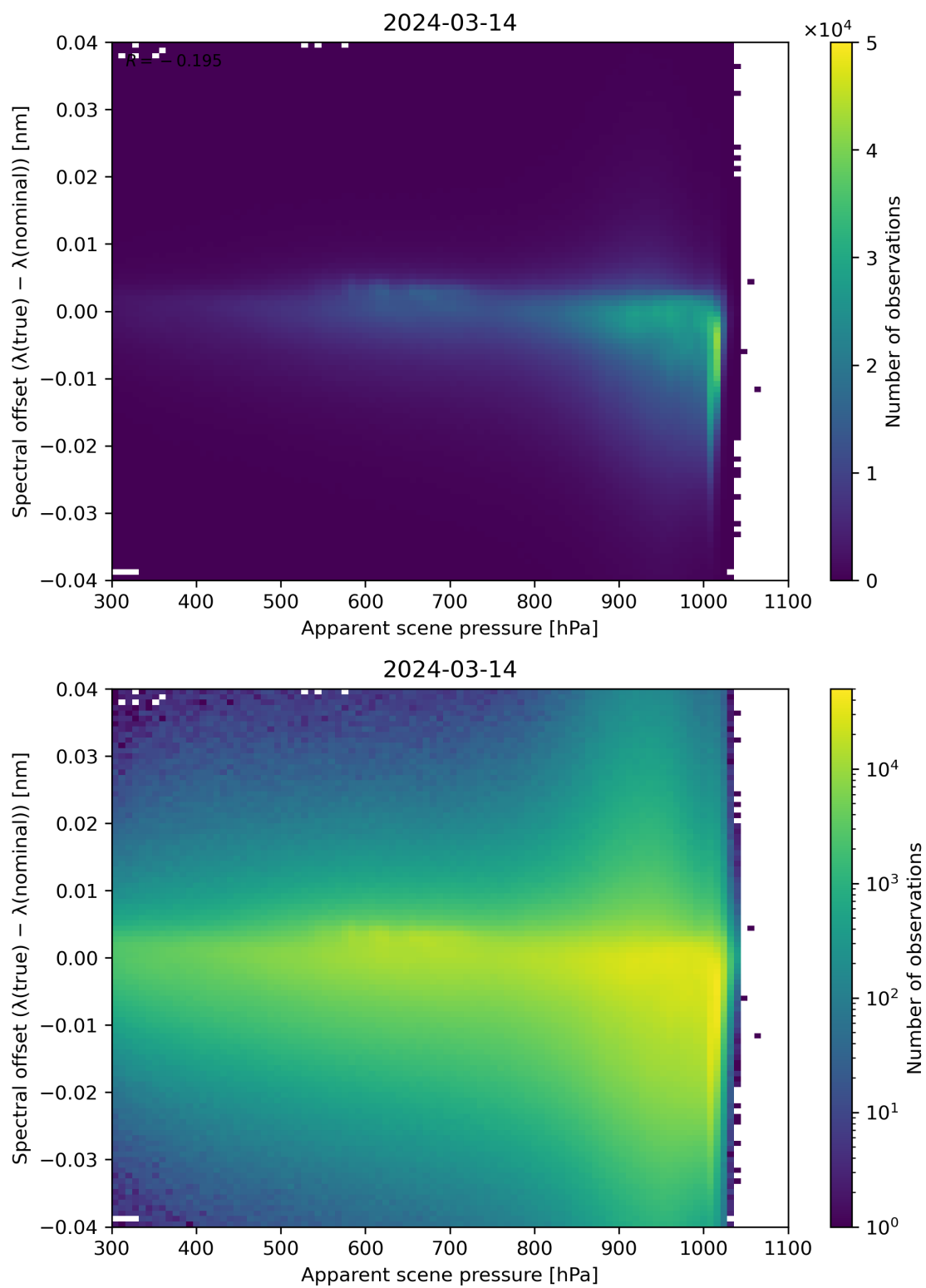
Figure 67: Scatter density plot of “Apparent scene pressure” against “Spectral offset ( \lambda(\text{true}) - \lambda(\text{nominal}) )” for 2024-03-14 to 2024-03-15.
