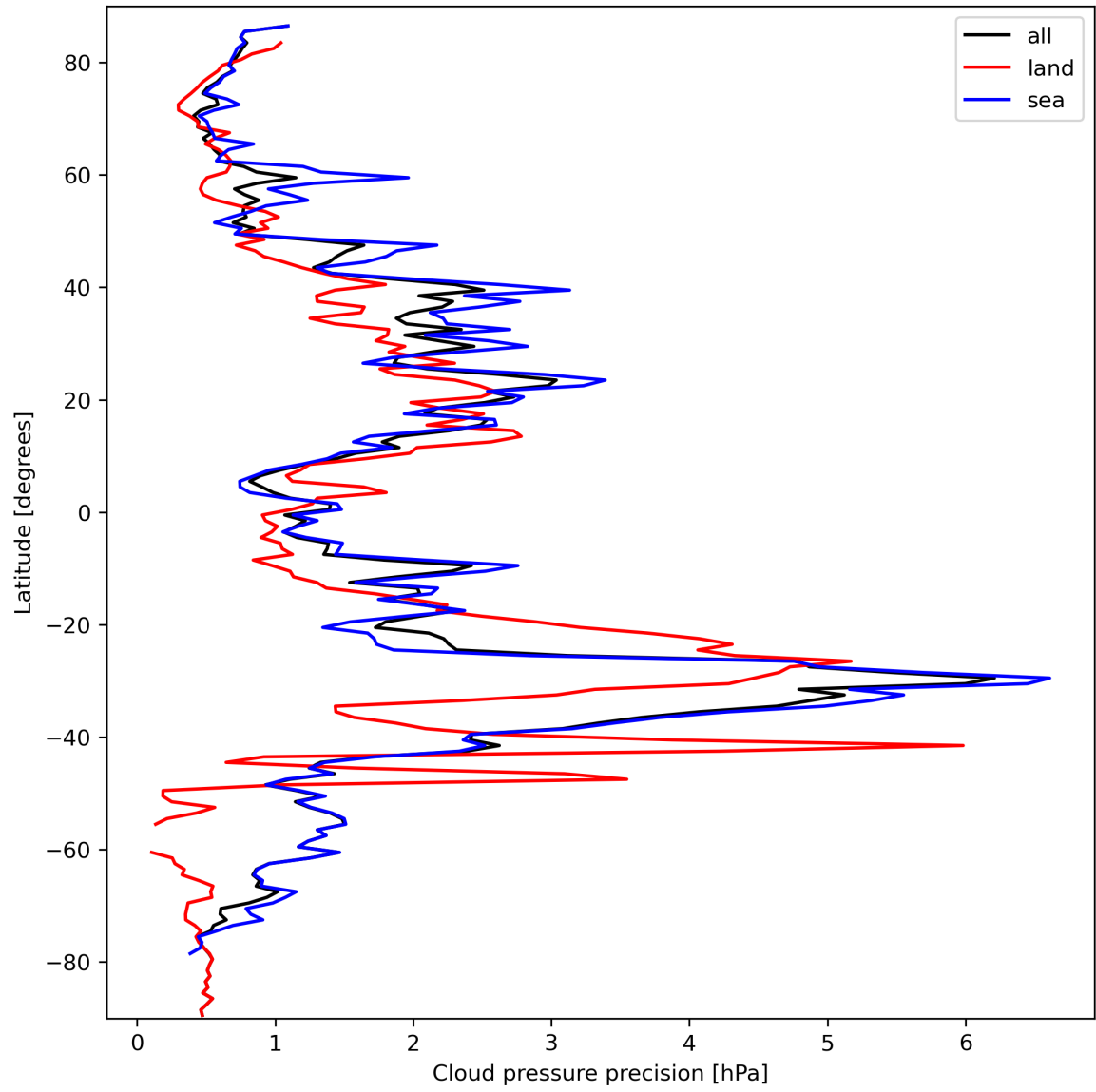
Figure 14: Zonal average of “Cloud pressure precision” for 2024-03-14 to 2024-03-15.
