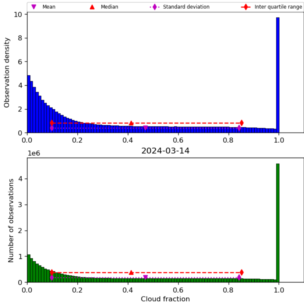
Figure 32: Histogram of “Cloud fraction” for 2024-03-14 to 2024-03-15
