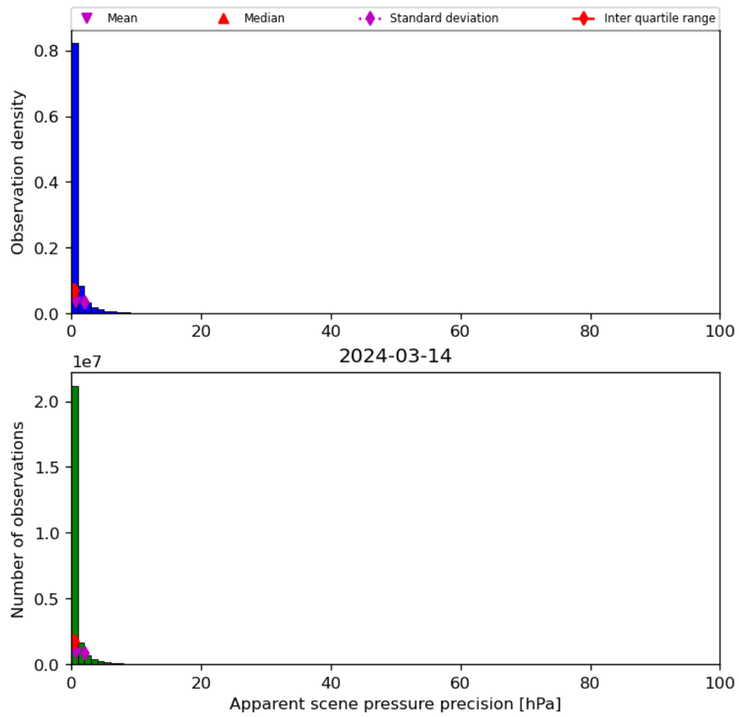
Figure 37: Histogram of “Apparent scene pressure precision” for 2024-03-14 to 2024-03-15
