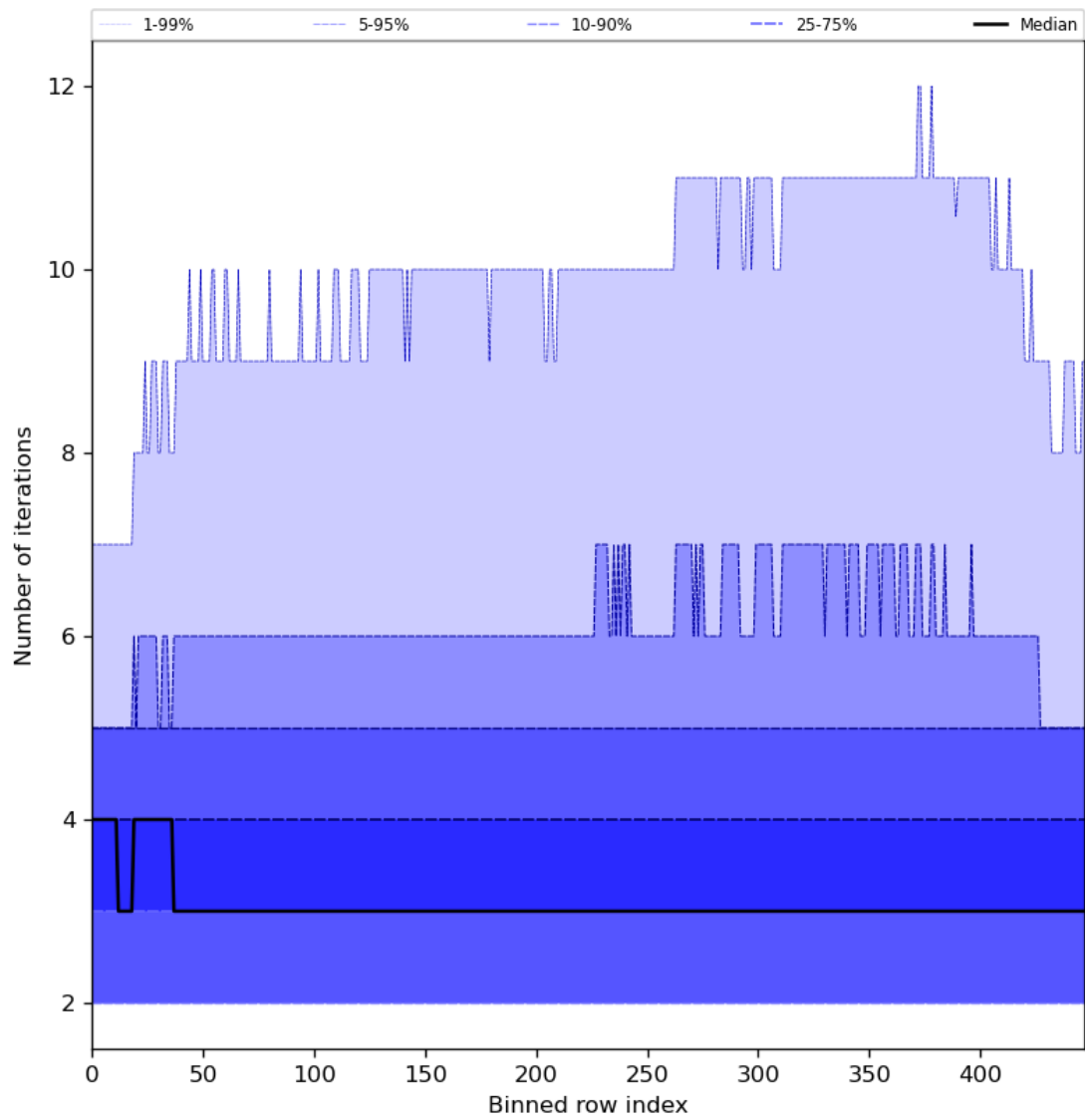
Figure 56: Along track statistics of “Number of iterations” for 2024-03-14 to 2024-03-15
