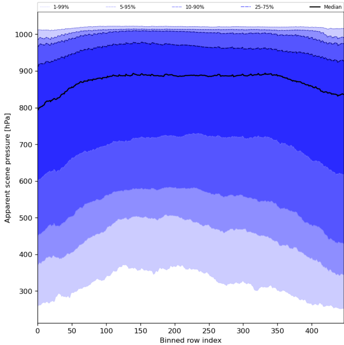
Figure 53: Along track statistics of “Apparent scene pressure” for 2024-03-14 to 2024-03-15
