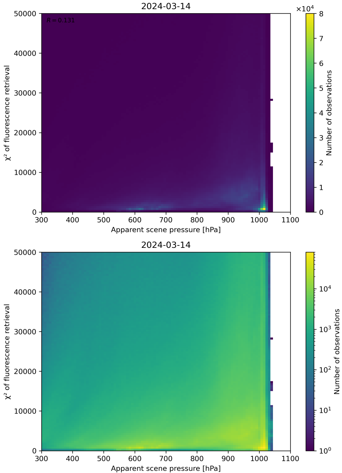
Figure 63: Scatter density plot of “Apparent scene pressure” against “ \chi^2 of fluorescence retrieval” for 2024-03-14 to 2024-03-15.
