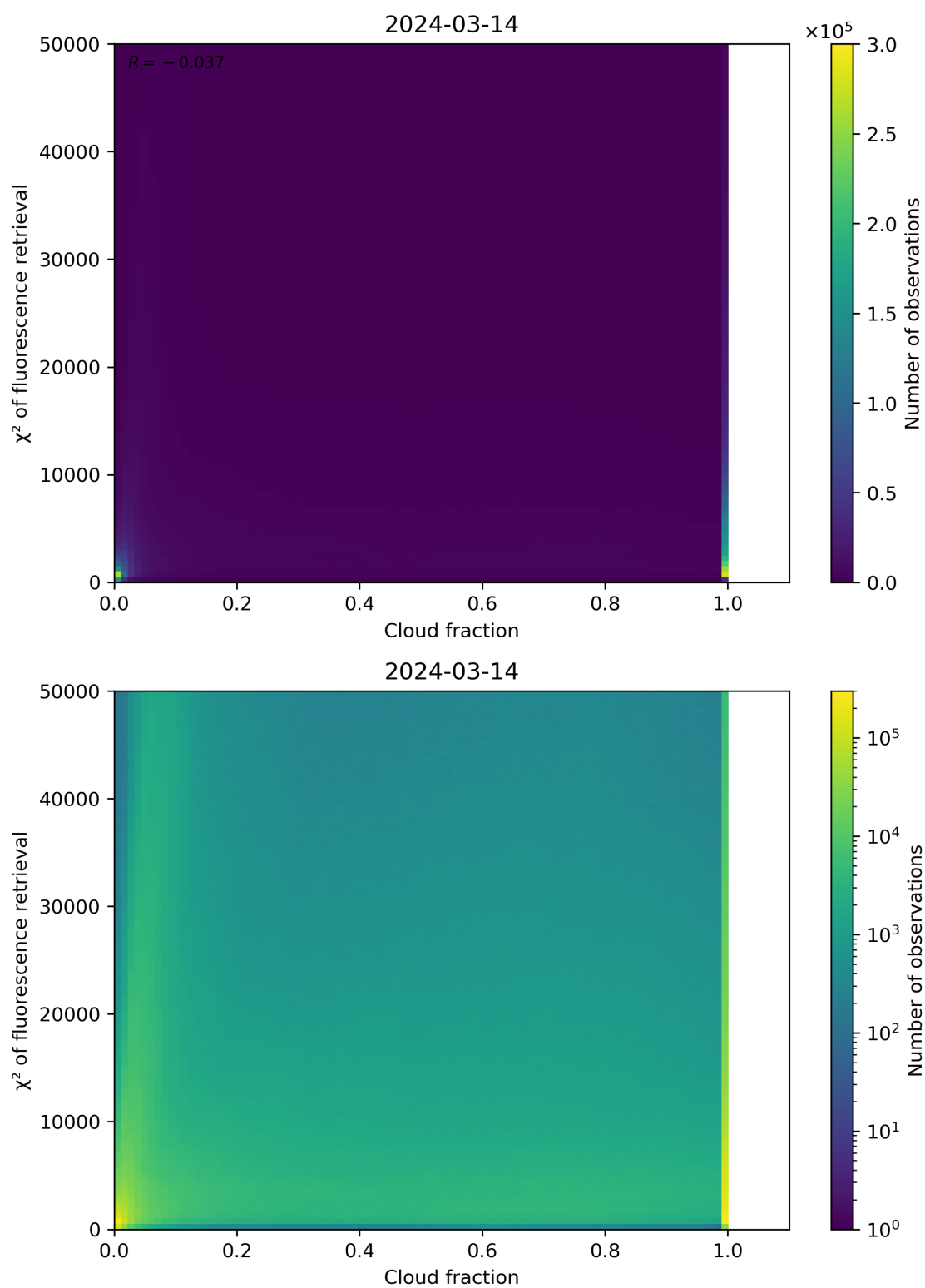
Figure 71: Scatter density plot of “Cloud fraction” against “ \chi^2 of fluorescence retrieval” for 2024-03-14 to 2024-03-15.
