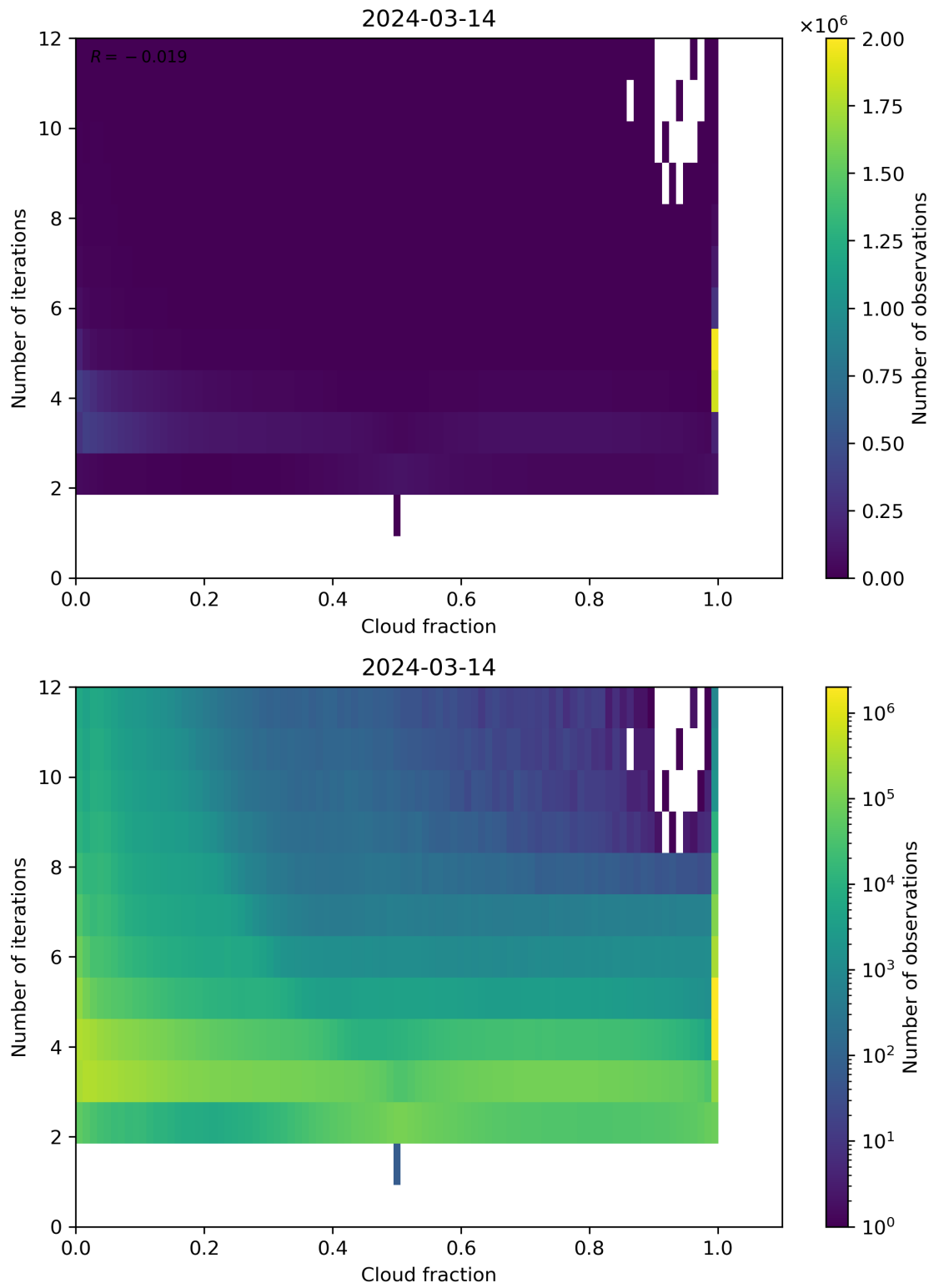
Figure 73: Scatter density plot of “Cloud fraction” against “Number of iterations” for 2024-03-14 to 2024-03-15.
