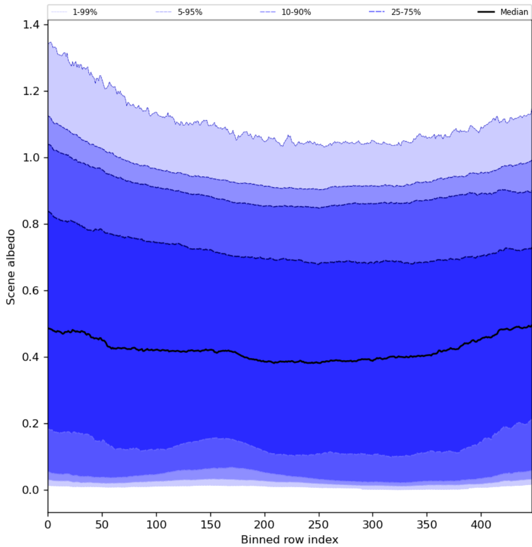
Figure 51: Along track statistics of “Scene albedo” for 2024-03-14 to 2024-03-15
