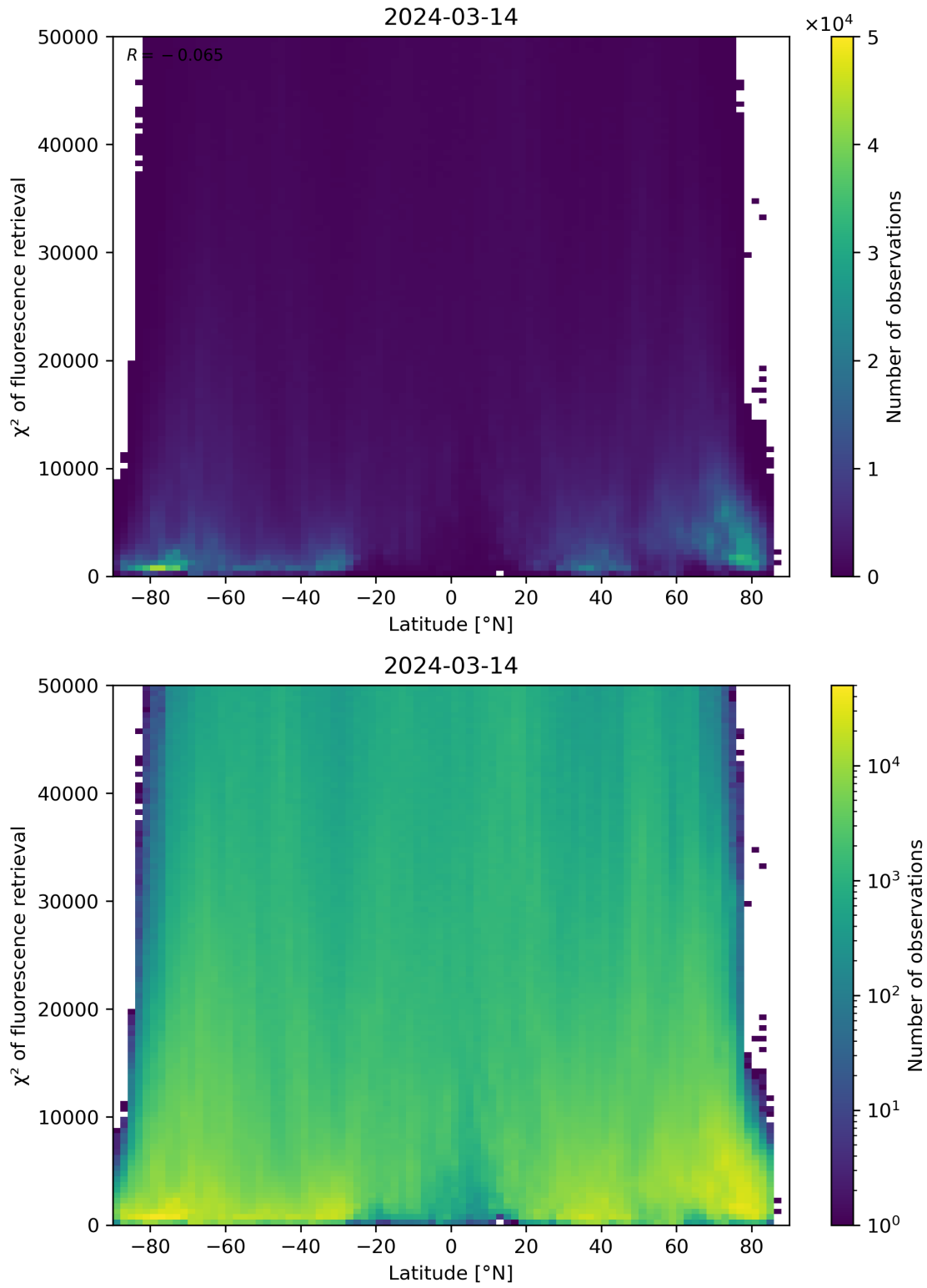
Figure 89: Scatter density plot of “Latitude” against “ \chi^2 of fluorescence retrieval” for 2024-03-14 to 2024-03-15.
