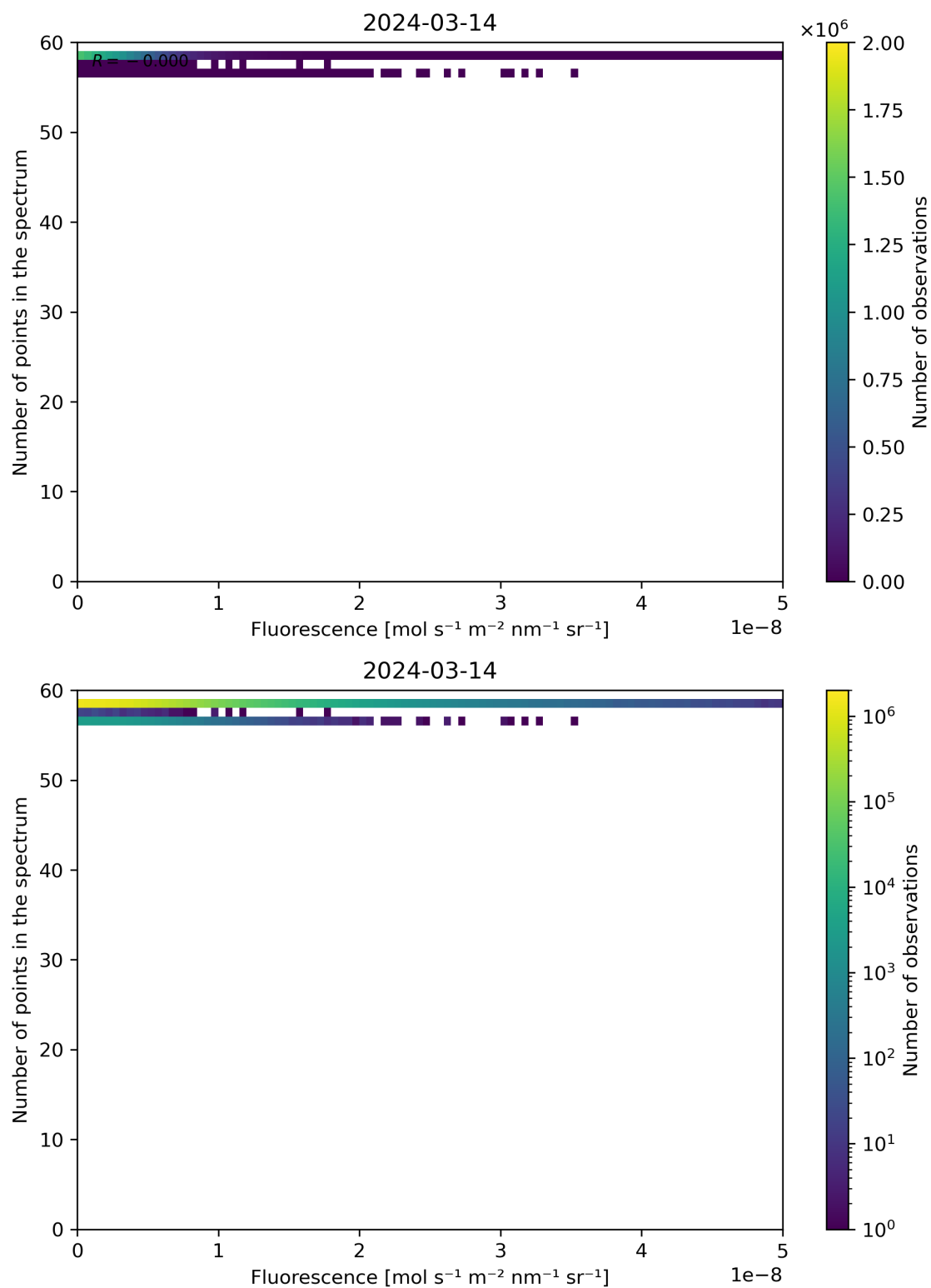
Figure 86: Scatter density plot of “Fluorescence” against “Number of points in the spectrum” for 2024-03-14 to 2024-03-15.
