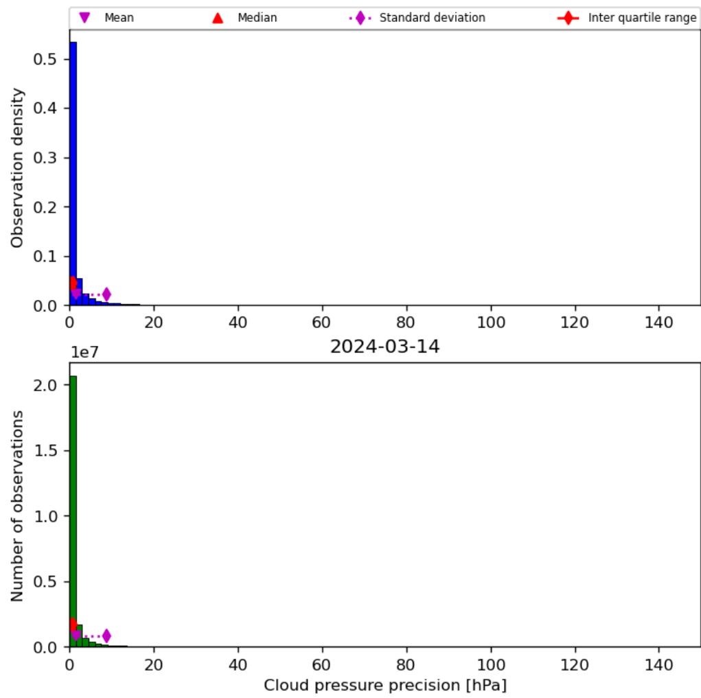
Figure 31: Histogram of “Cloud pressure precision” for 2024-03-14 to 2024-03-15
