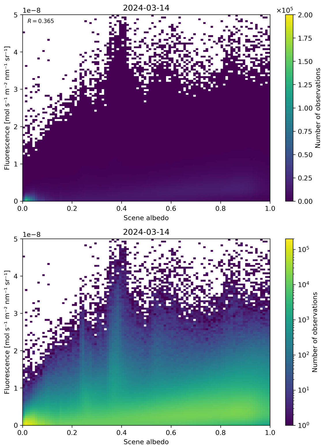
Figure 104: Scatter density plot of “Scene albedo” against “Fluorescence” for 2024-03-14 to 2024-03-15.
