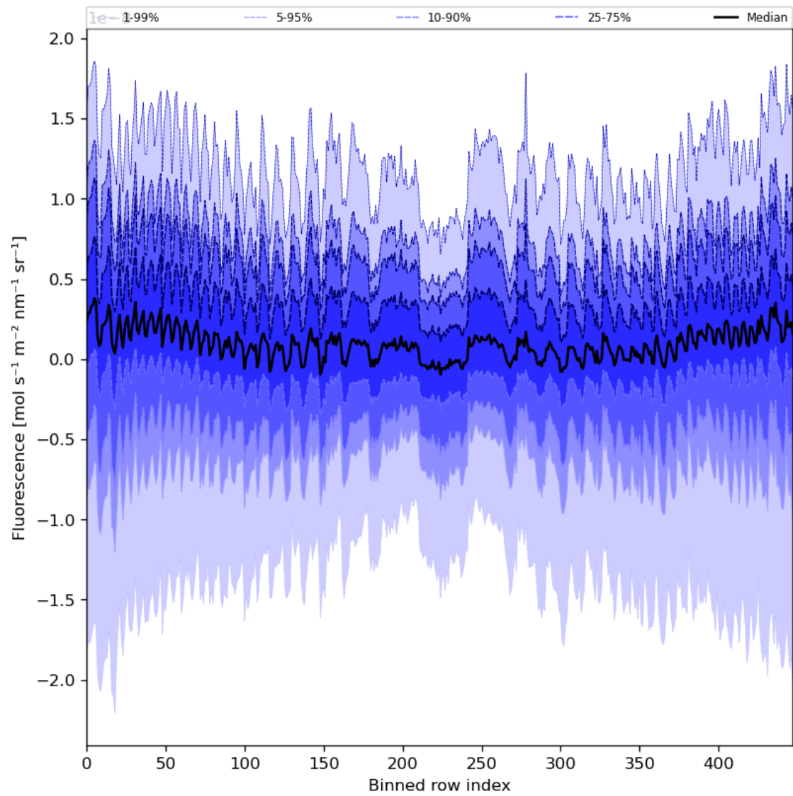
Figure 57: Along track statistics of “Fluorescence” for 2024-03-14 to 2024-03-15
