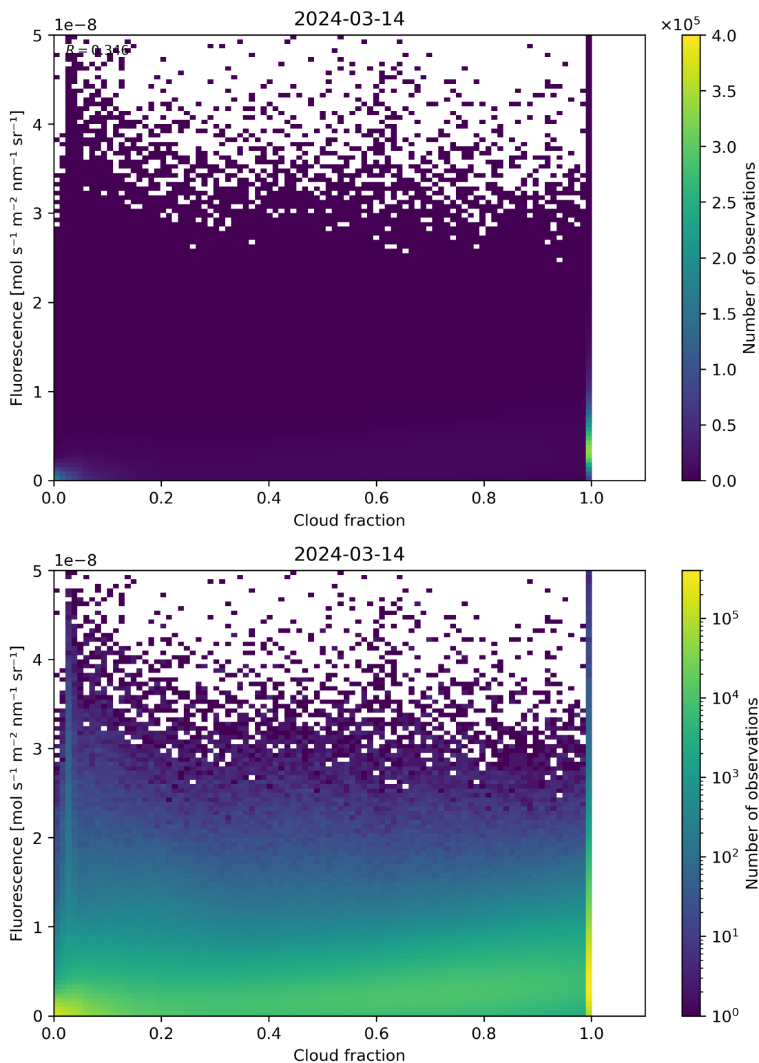
Figure 72: Scatter density plot of “Cloud fraction” against “Fluorescence” for 2024-03-14 to 2024-03-15.
