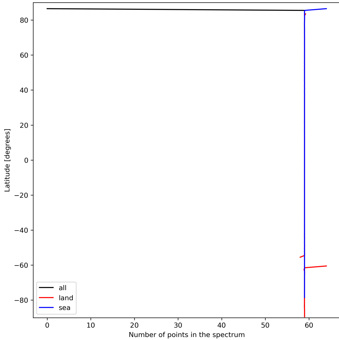
Figure 27: Zonal average of “Number of points in the spectrum” for 2024-03-14 to 2024-03-15.
