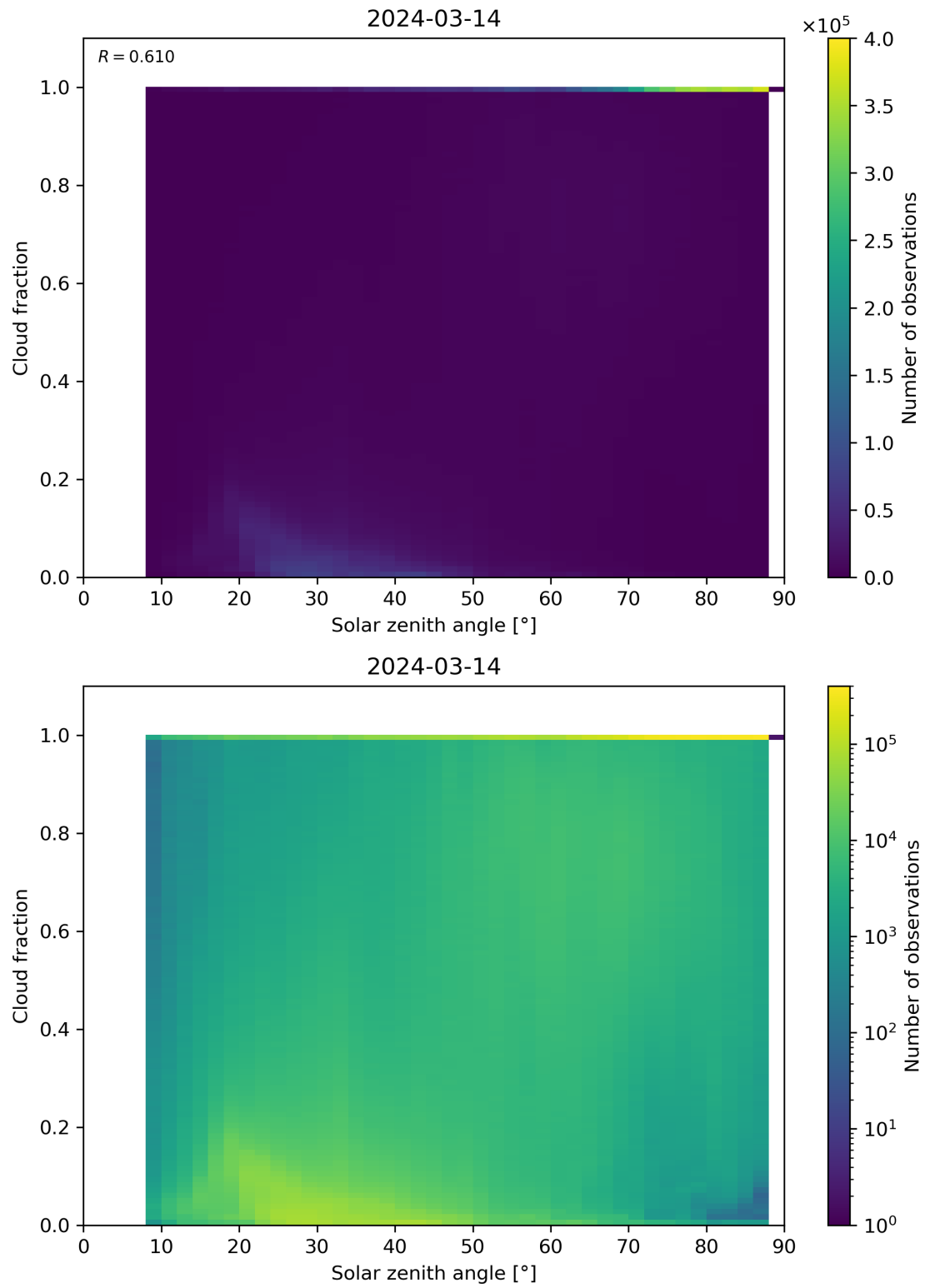
Figure 110: Scatter density plot of “Solar zenith angle” against “Cloud fraction” for 2024-03-14 to 2024-03-15.
