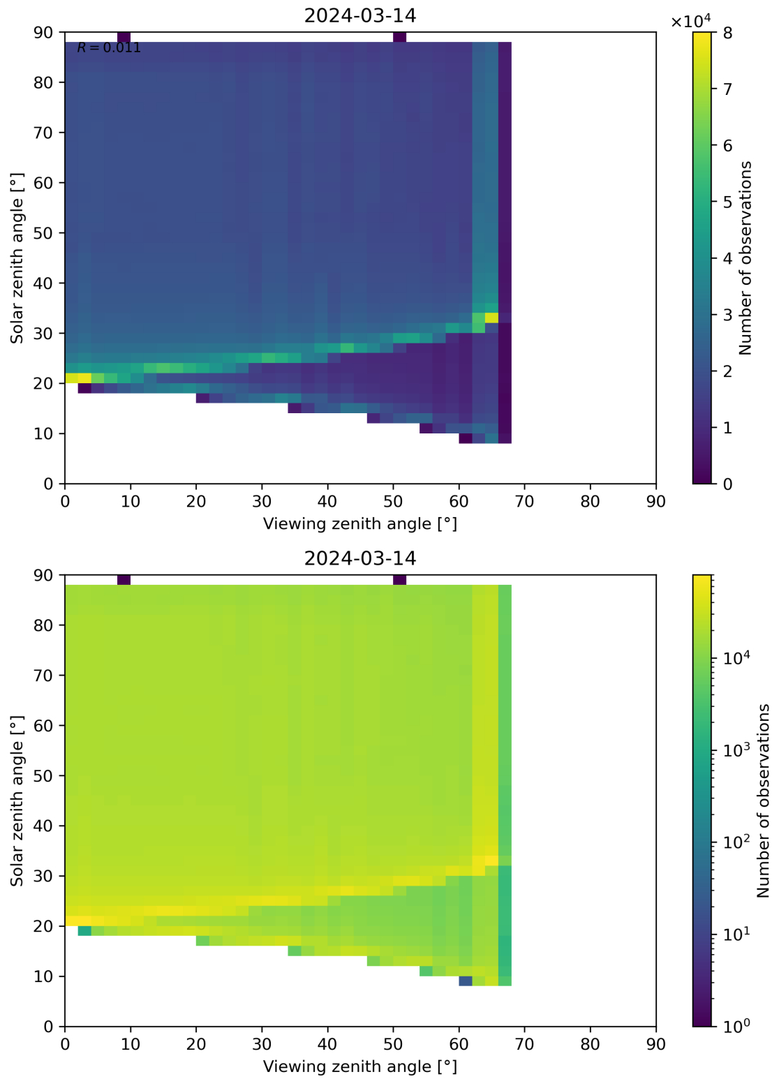
Figure 127: Scatter density plot of “Viewing zenith angle” against “Solar zenith angle” for 2024-03-14 to 2024-03-15.
