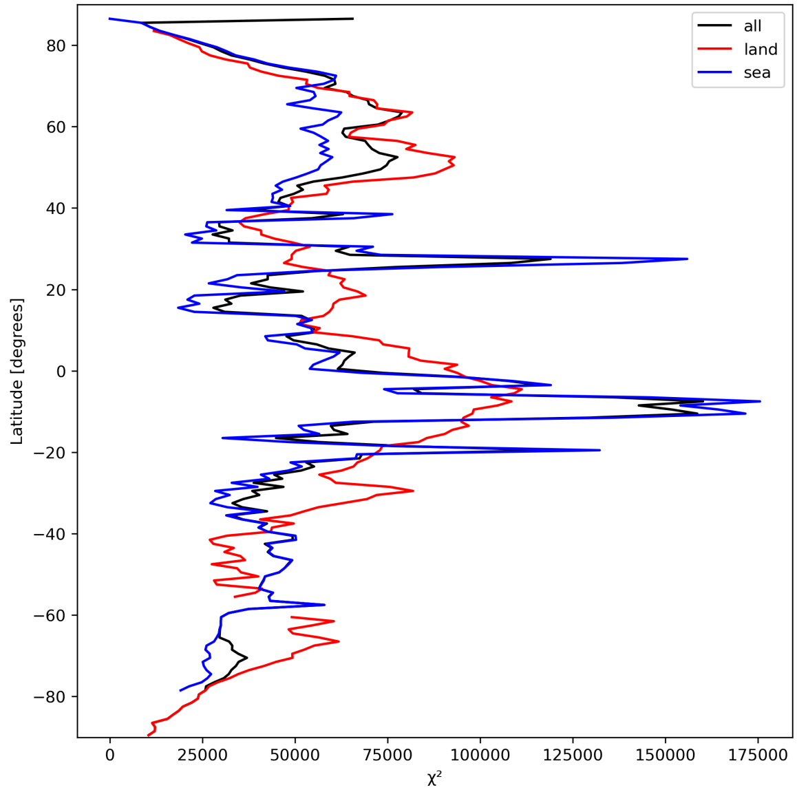
Figure 21: Zonal average of “ \chi^2 ” for 2024-03-14 to 2024-03-15.
