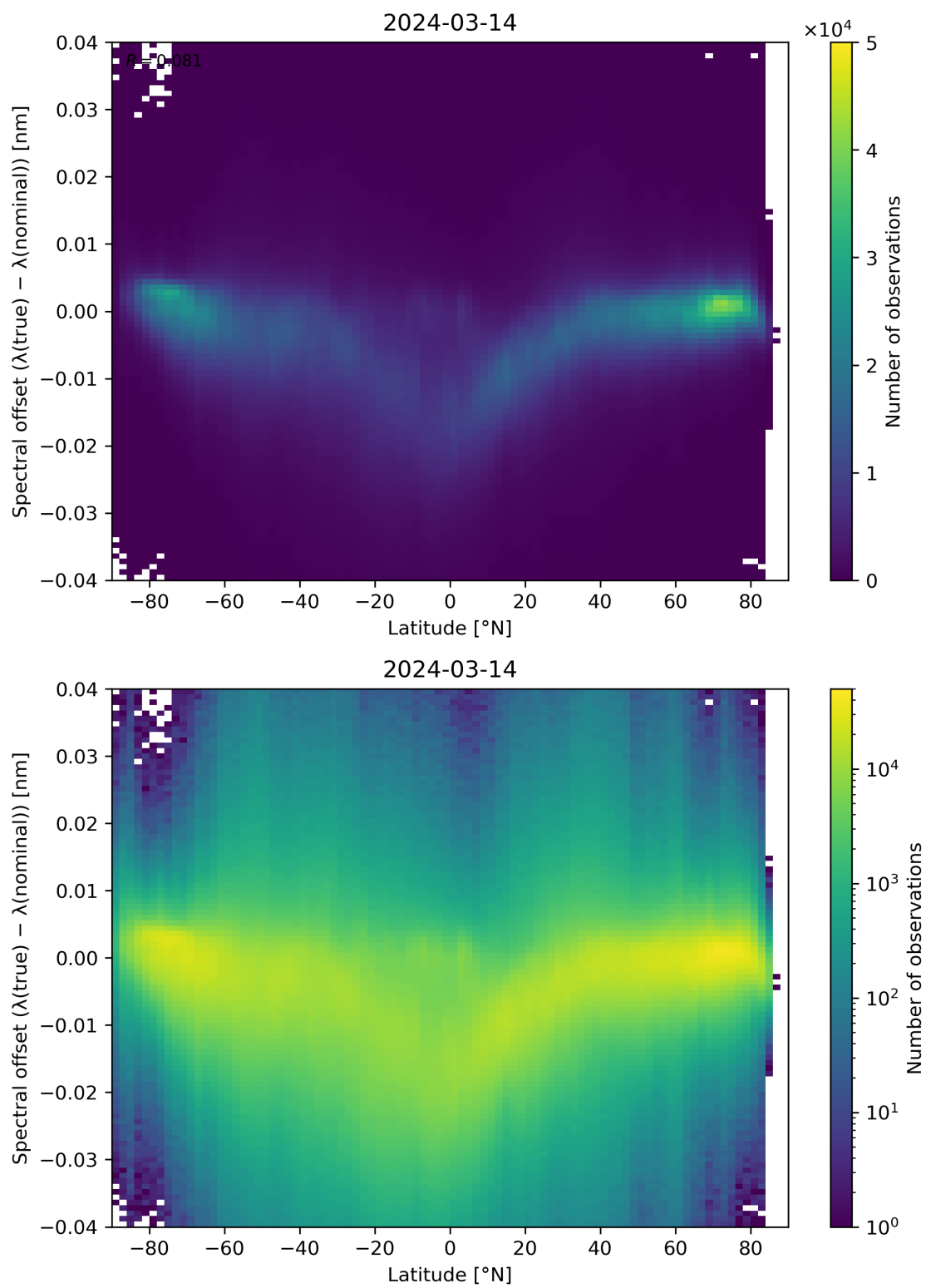
Figure 96: Scatter density plot of “Latitude” against “Spectral offset ( \lambda(\text{true}) - \lambda(\text{nominal}) )” for 2024-03-14 to 2024-03-15.
