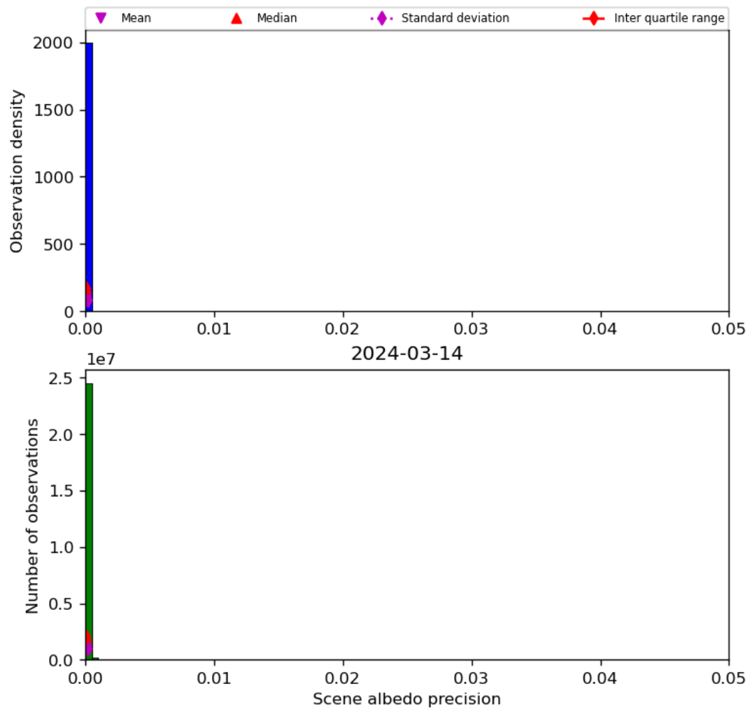
Figure 35: Histogram of “Scene albedo precision” for 2024-03-14 to 2024-03-15
