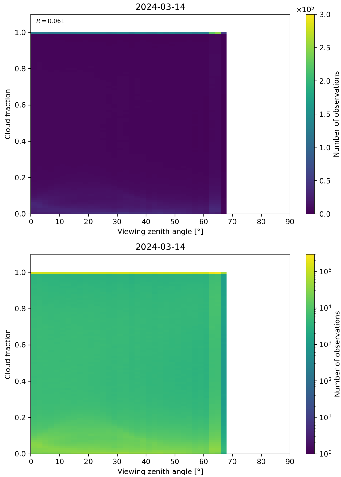
Figure 120: Scatter density plot of “Viewing zenith angle” against “Cloud fraction” for 2024-03-14 to 2024-03-15.
