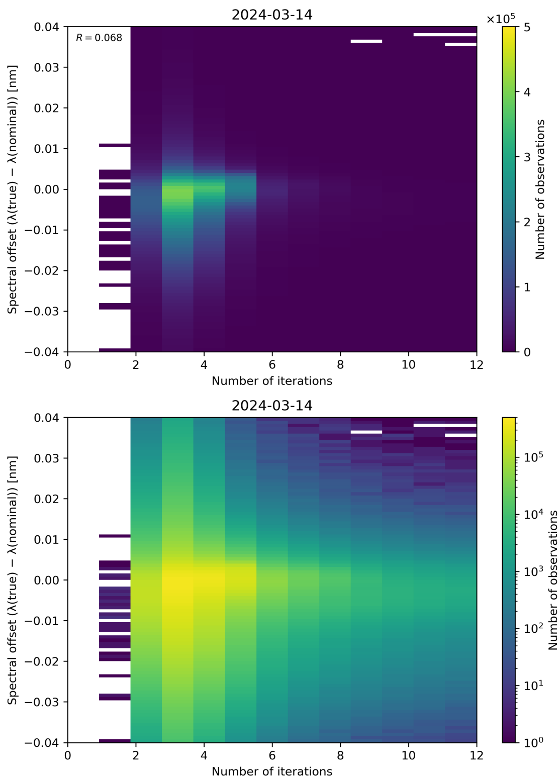
Figure 100: Scatter density plot of “Number of iterations” against “Spectral offset ( \lambda(\text{true}) - \lambda(\text{nominal}) )” for 2024-03-14 to 2024-03-15.
