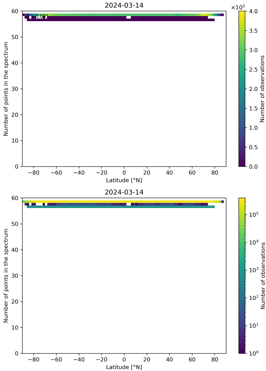
Figure 94: Scatter density plot of “Latitude” against “Number of points in the spectrum” for 2024-03-14 to 2024-03-15.
