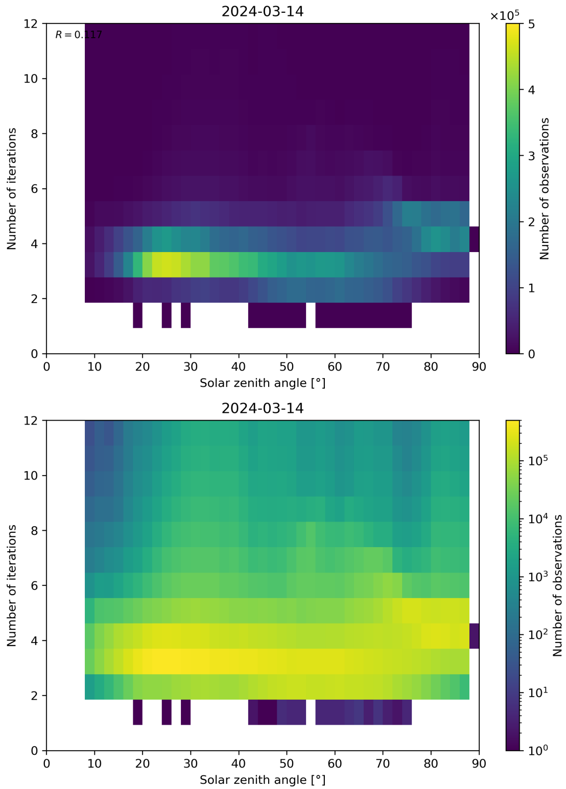
Figure 114: Scatter density plot of “Solar zenith angle” against “Number of iterations” for 2024-03-14 to 2024-03-15.
