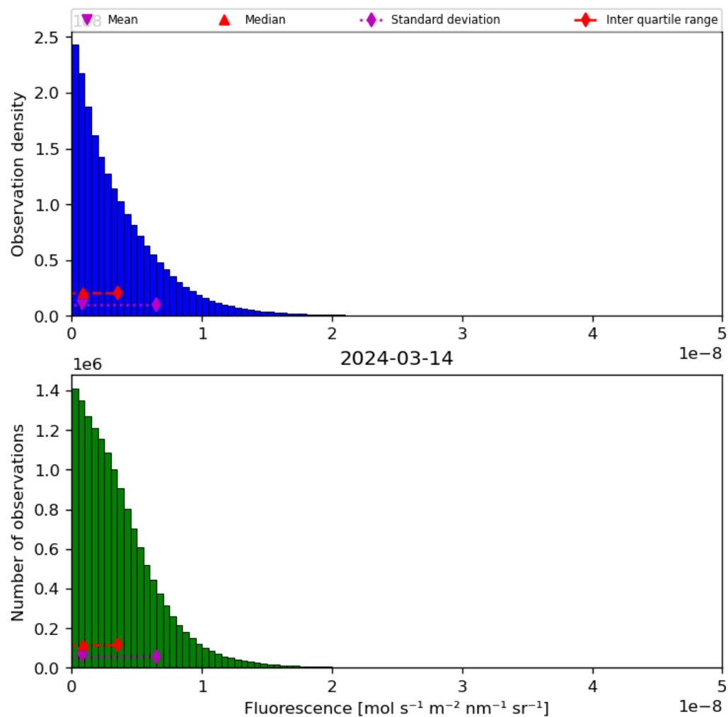
Figure 40: Histogram of “Fluorescence” for 2024-03-14 to 2024-03-15
