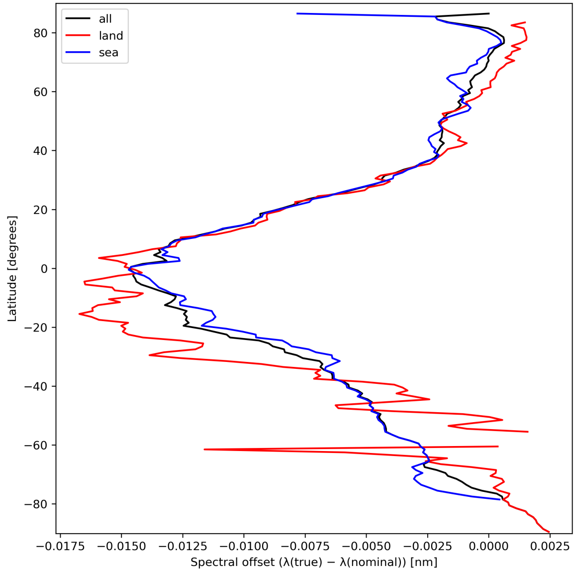
Figure 28: Zonal average of “Spectral offset ( \lambda(\text{true}) - \lambda(\text{nominal}) )” for 2024-03-14 to 2024-03-15.
