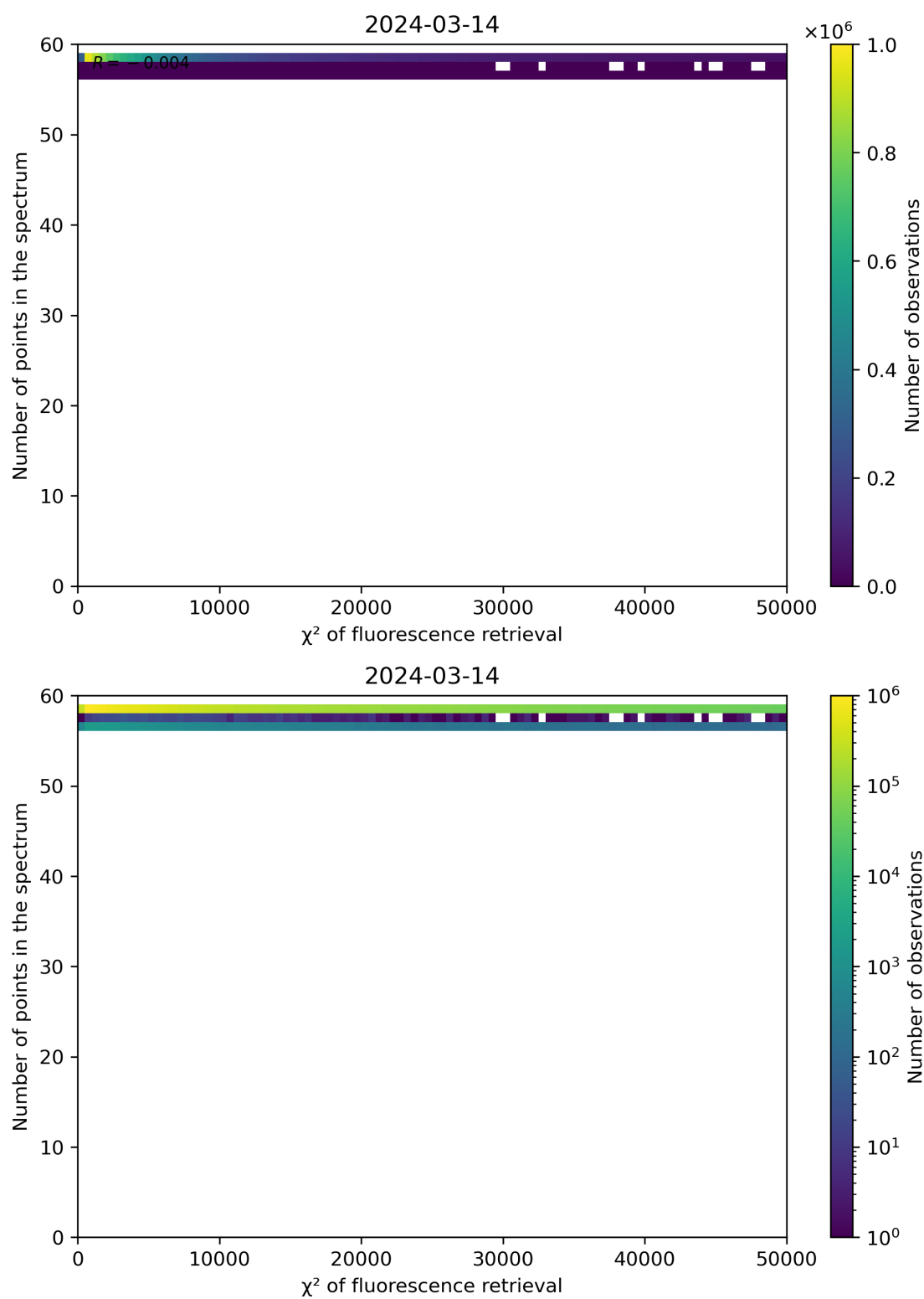
Figure 68: Scatter density plot of “ \chi^2 of fluorescence retrieval” against “Number of points in the spectrum” for 2024-03-14 to 2024-03-15.
