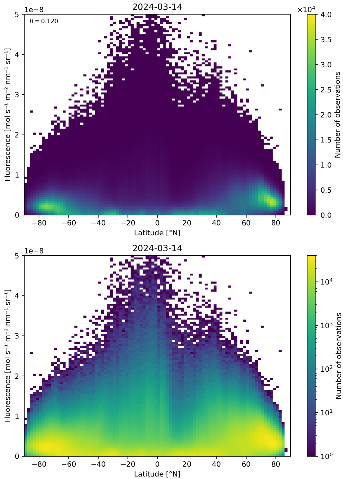
Figure 92: Scatter density plot of “Latitude” against “Fluorescence” for 2024-03-14 to 2024-03-15.
