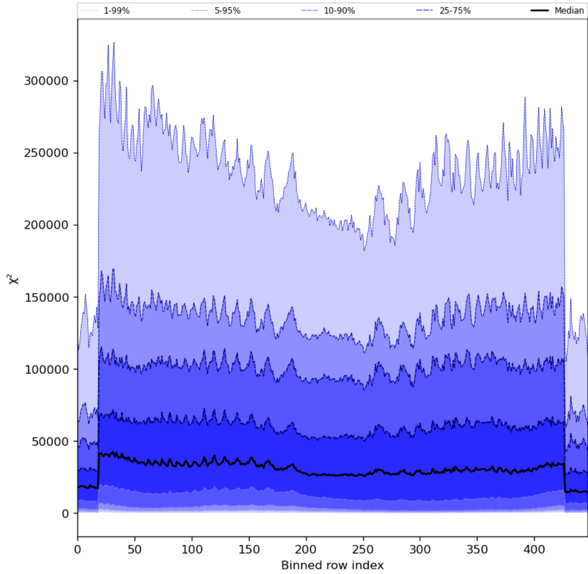
Figure 55: Along track statistics of “ \chi^2 ” for 2024-03-14 to 2024-03-15
