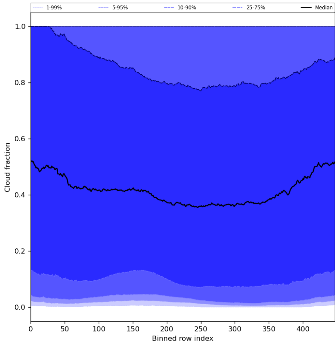
Figure 49: Along track statistics of “Cloud fraction” for 2024-03-14 to 2024-03-15
