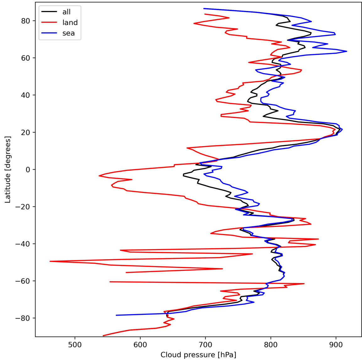
Figure 13: Zonal average of “Cloud pressure” for 2024-03-14 to 2024-03-15.
