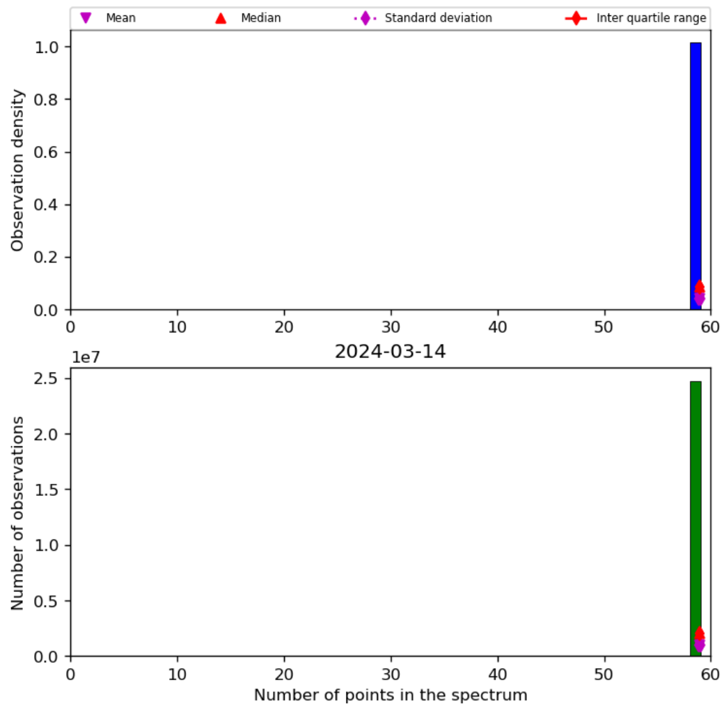
Figure 44: Histogram of “Number of points in the spectrum” for 2024-03-14 to 2024-03-15
