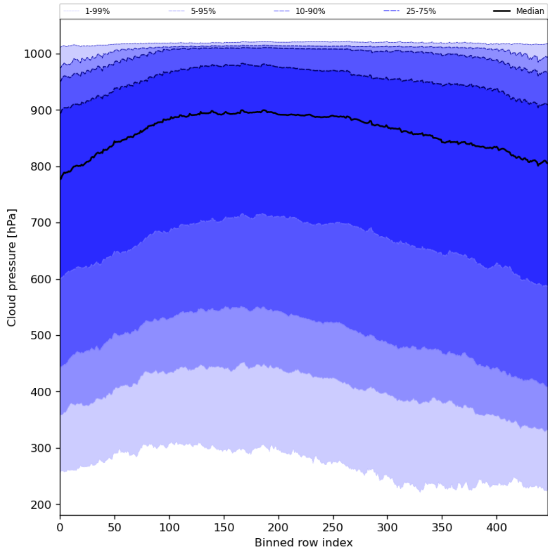
Figure 47: Along track statistics of “Cloud pressure” for 2024-03-15 to 2024-03-17
