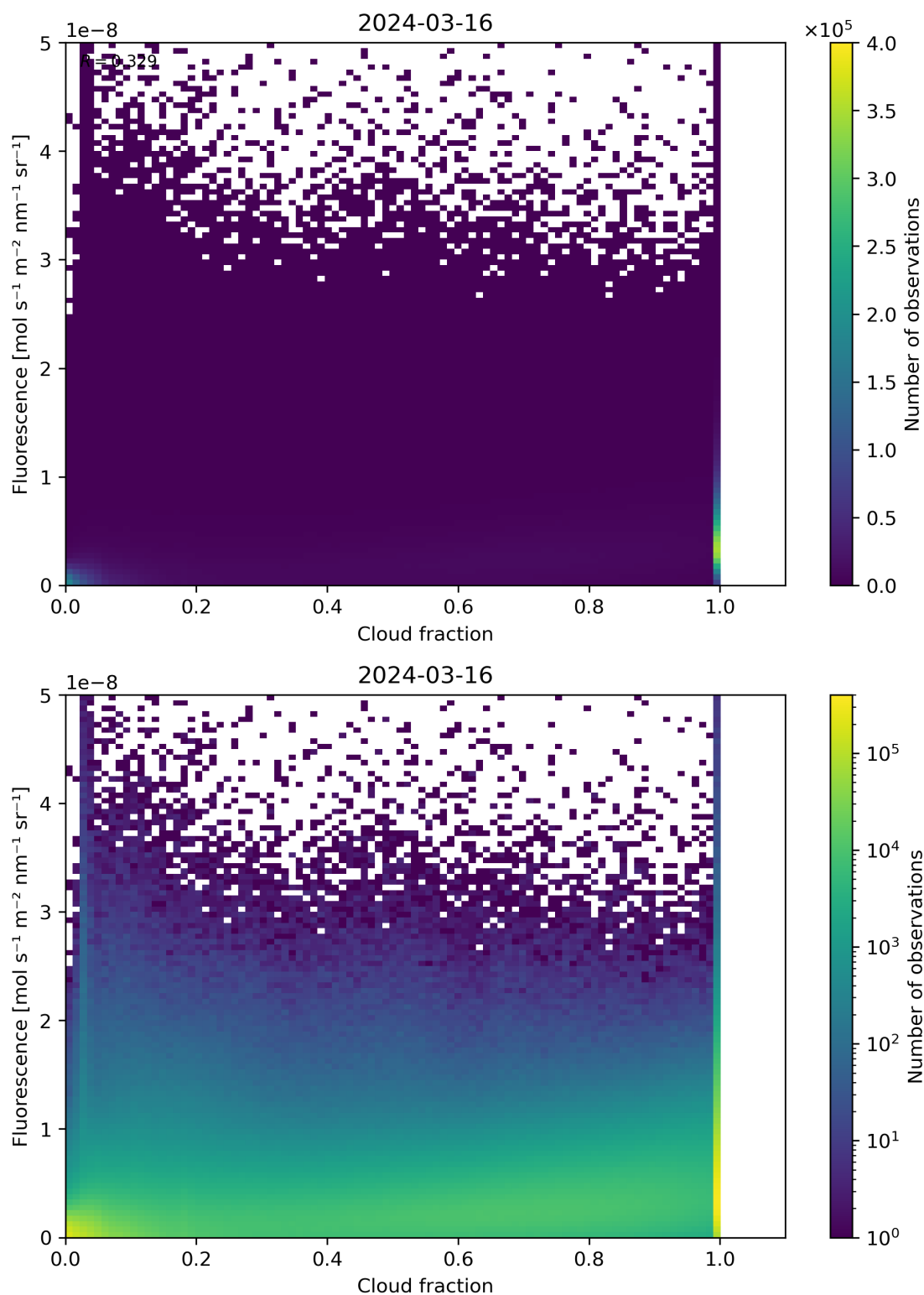
Figure 72: Scatter density plot of “Cloud fraction” against “Fluorescence” for 2024-03-15 to 2024-03-17.
