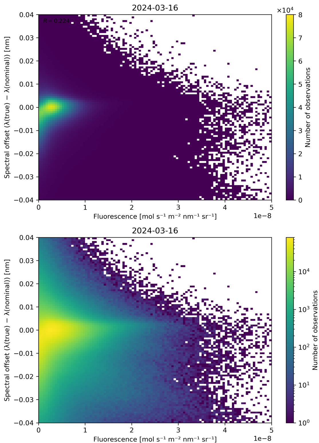
Figure 87: Scatter density plot of “Fluorescence” against “Spectral offset ( \lambda(\text{true}) - \lambda(\text{nominal}) )” for 2024-03-15 to 2024-03-17.
