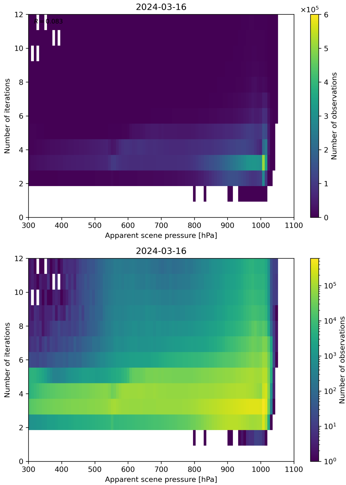
Figure 65: Scatter density plot of “Apparent scene pressure” against “Number of iterations” for 2024-03-15 to 2024-03-17.
