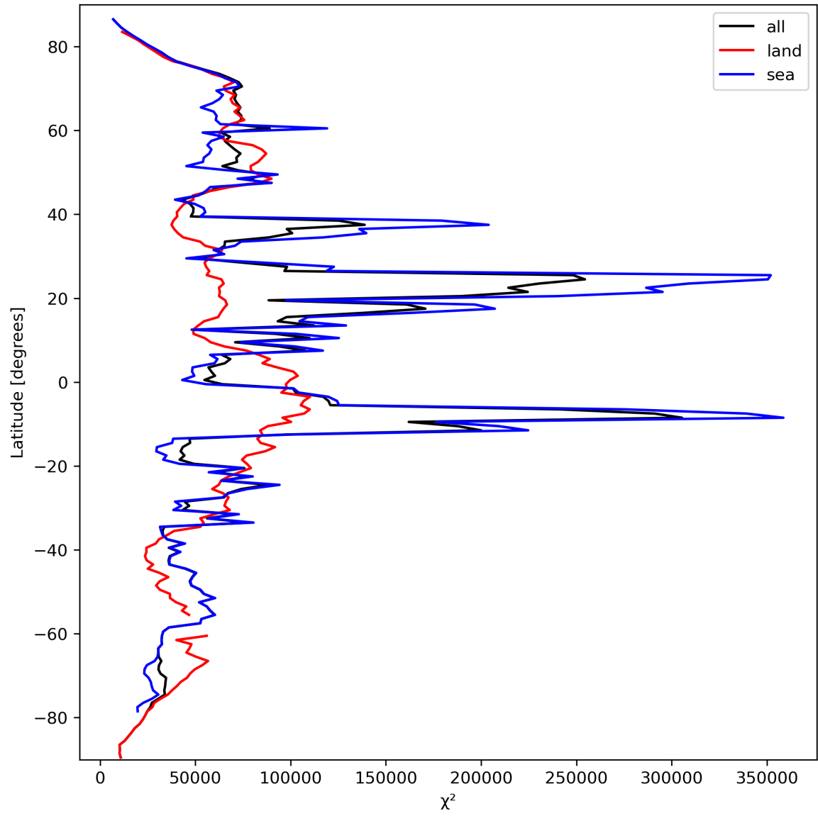
Figure 21: Zonal average of “ \chi^2 ” for 2024-03-15 to 2024-03-17.
