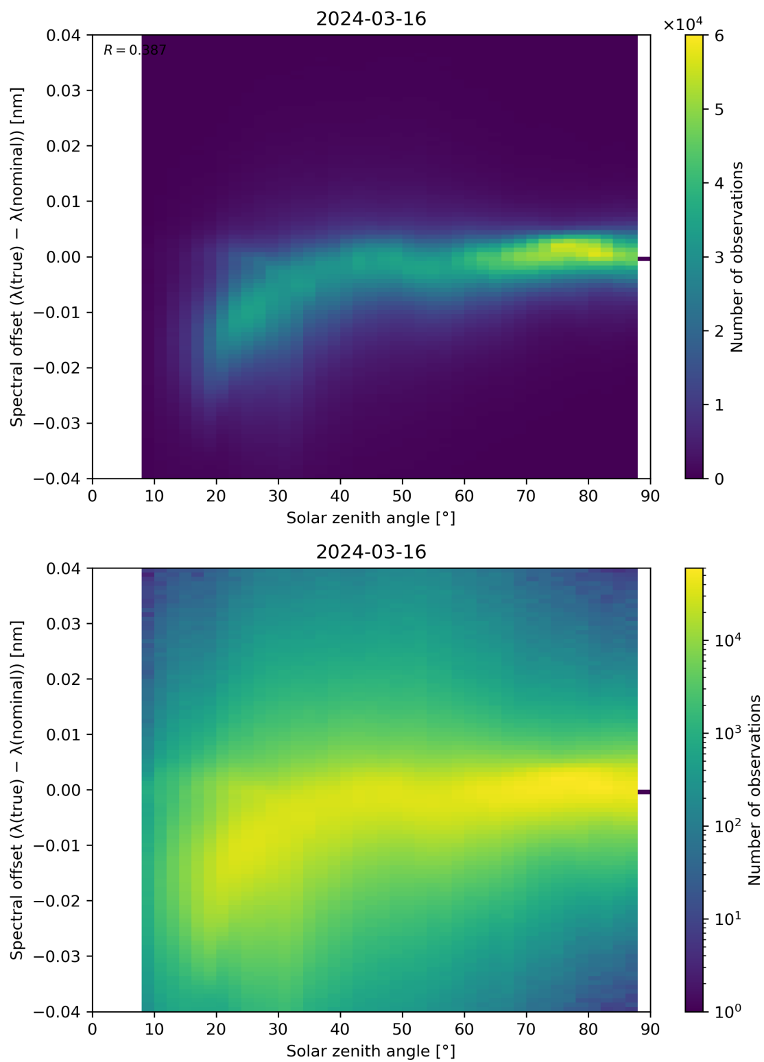
Figure 117: Scatter density plot of “Solar zenith angle” against “Spectral offset ( \lambda(\text{true}) - \lambda(\text{nominal}) )” for 2024-03-15 to 2024-03-17.
