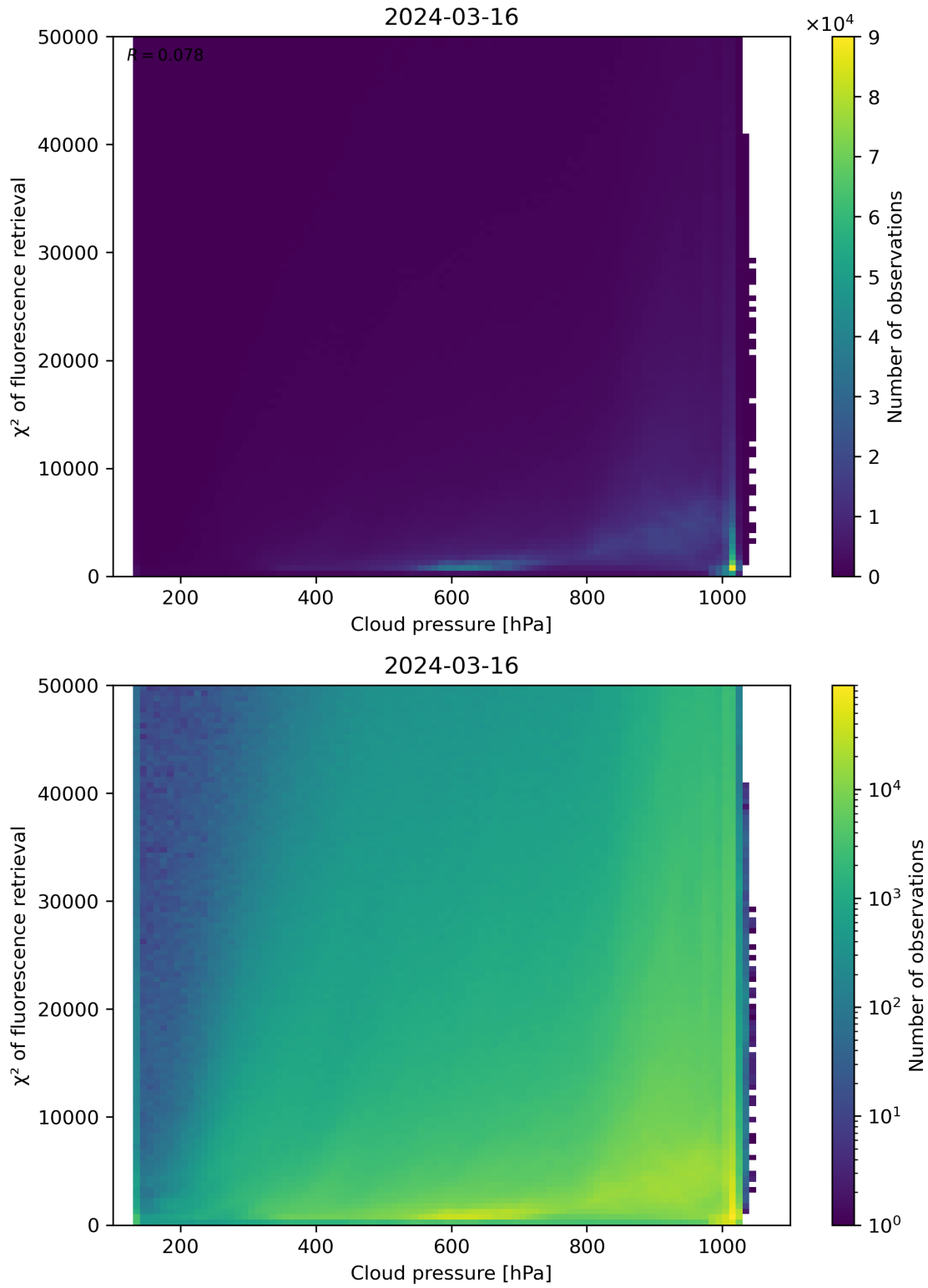
Figure 78: Scatter density plot of “Cloud pressure” against “ \chi^2 of fluorescence retrieval” for 2024-03-15 to 2024-03-17.
