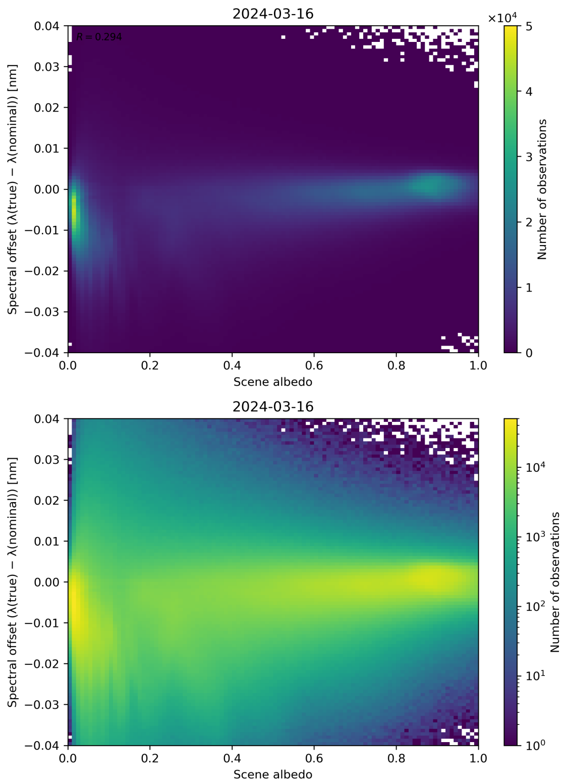
Figure 107: Scatter density plot of “Scene albedo” against “Spectral offset ( \lambda(\text{true}) - \lambda(\text{nominal}) )” for 2024-03-15 to 2024-03-17.
