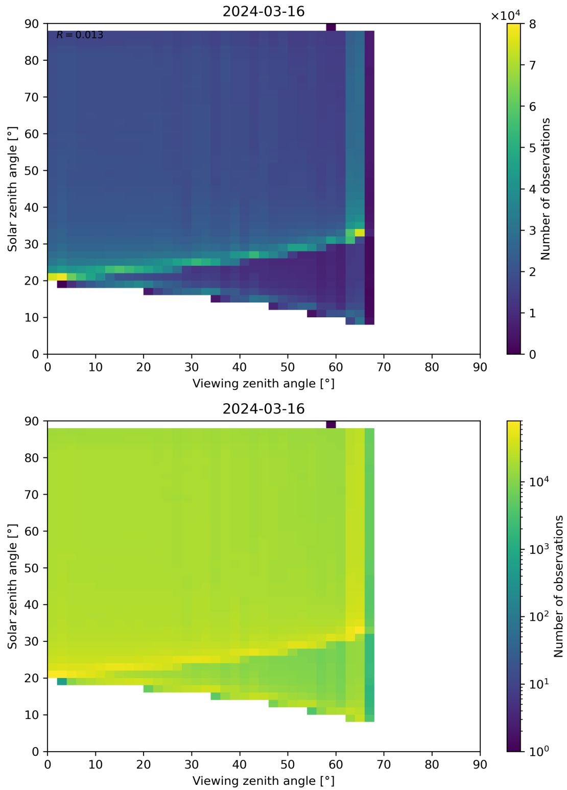
Figure 127: Scatter density plot of “Viewing zenith angle” against “Solar zenith angle” for 2024-03-15 to 2024-03-17.
