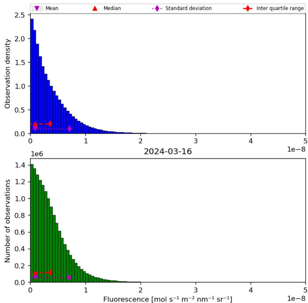
Figure 40: Histogram of “Fluorescence” for 2024-03-15 to 2024-03-17
