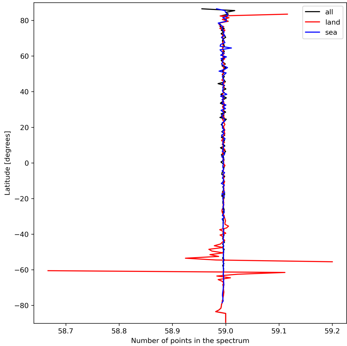
Figure 27: Zonal average of “Number of points in the spectrum” for 2024-03-15 to 2024-03-17.
