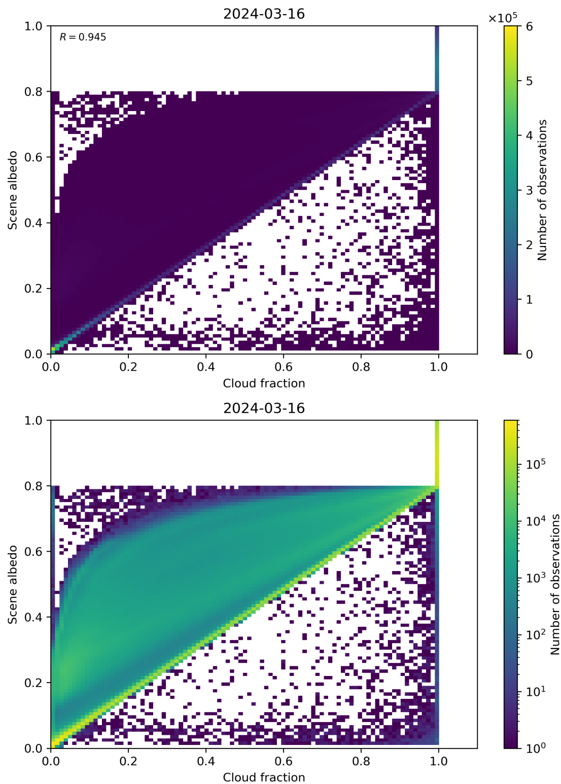
Figure 75: Scatter density plot of “Cloud fraction” against “Scene albedo” for 2024-03-15 to 2024-03-17.
