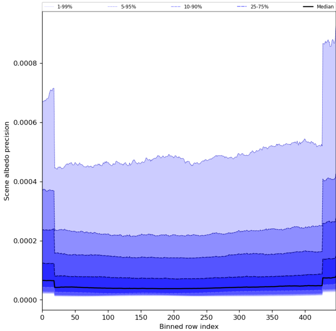
Figure 52: Along track statistics of “Scene albedo precision” for 2024-03-15 to 2024-03-17
