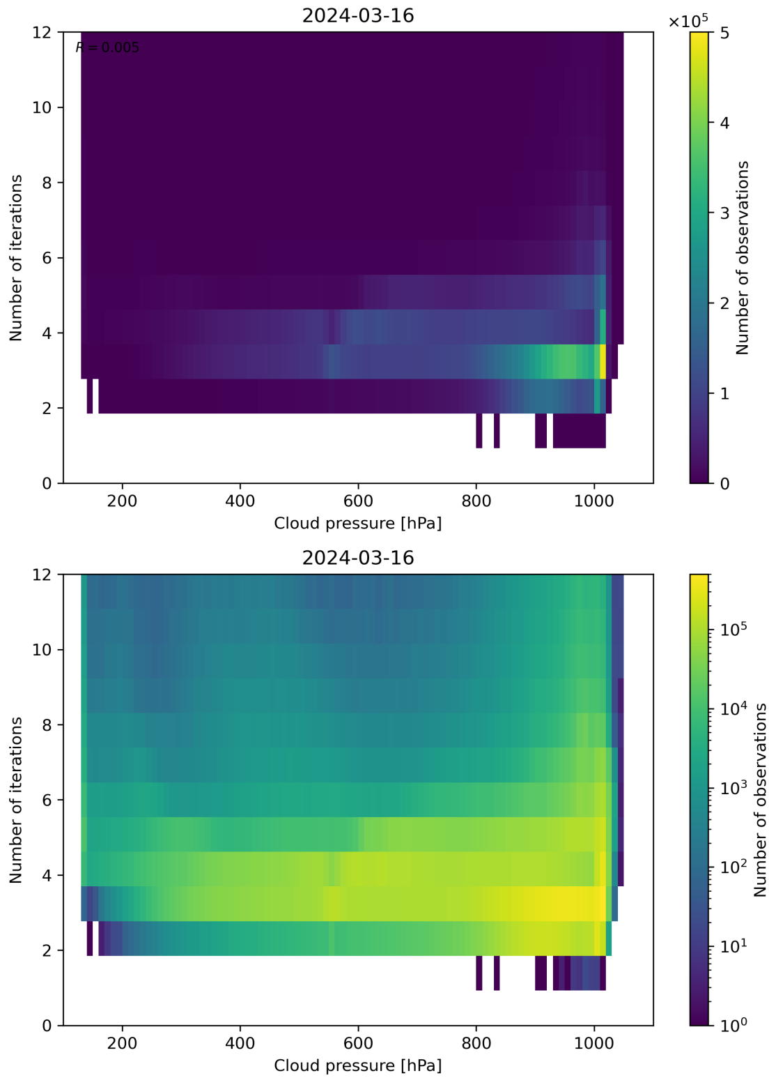
Figure 81: Scatter density plot of “Cloud pressure” against “Number of iterations” for 2024-03-15 to 2024-03-17.
