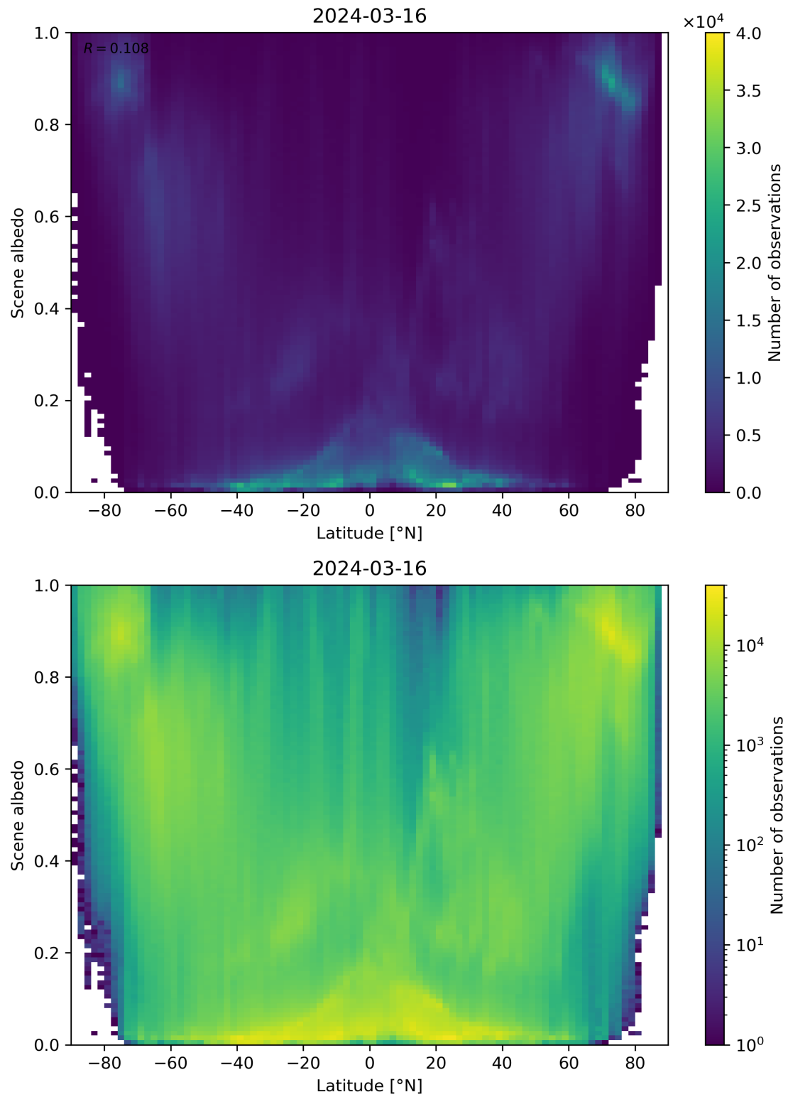
Figure 95: Scatter density plot of “Latitude” against “Scene albedo” for 2024-03-15 to 2024-03-17.
