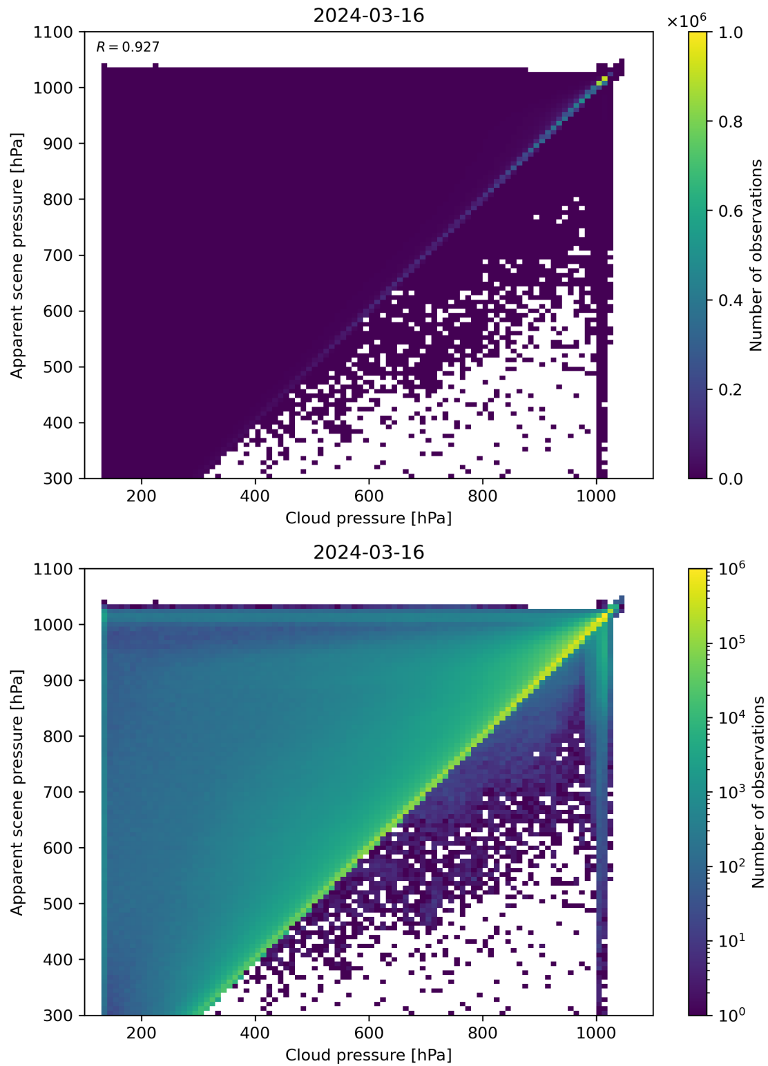
Figure 77: Scatter density plot of “Cloud pressure” against “Apparent scene pressure” for 2024-03-15 to 2024-03-17.
