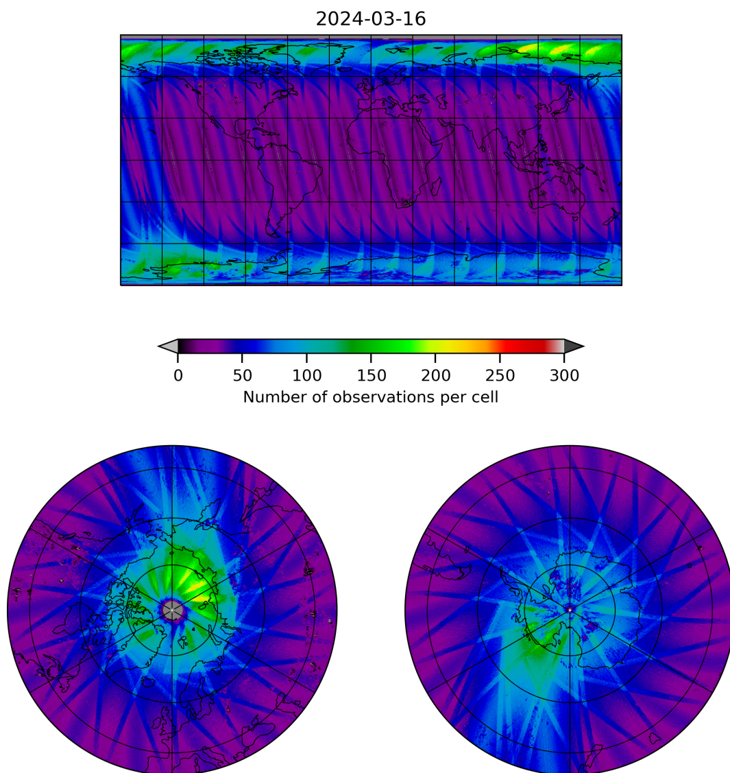
Figure 11: Map of the number of observations for 2024-03-15 to 2024-03-17
