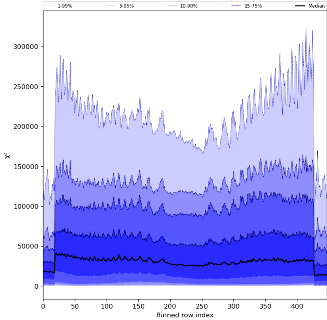
Figure 55: Along track statistics of “ \chi^2 ” for 2024-03-15 to 2024-03-17
