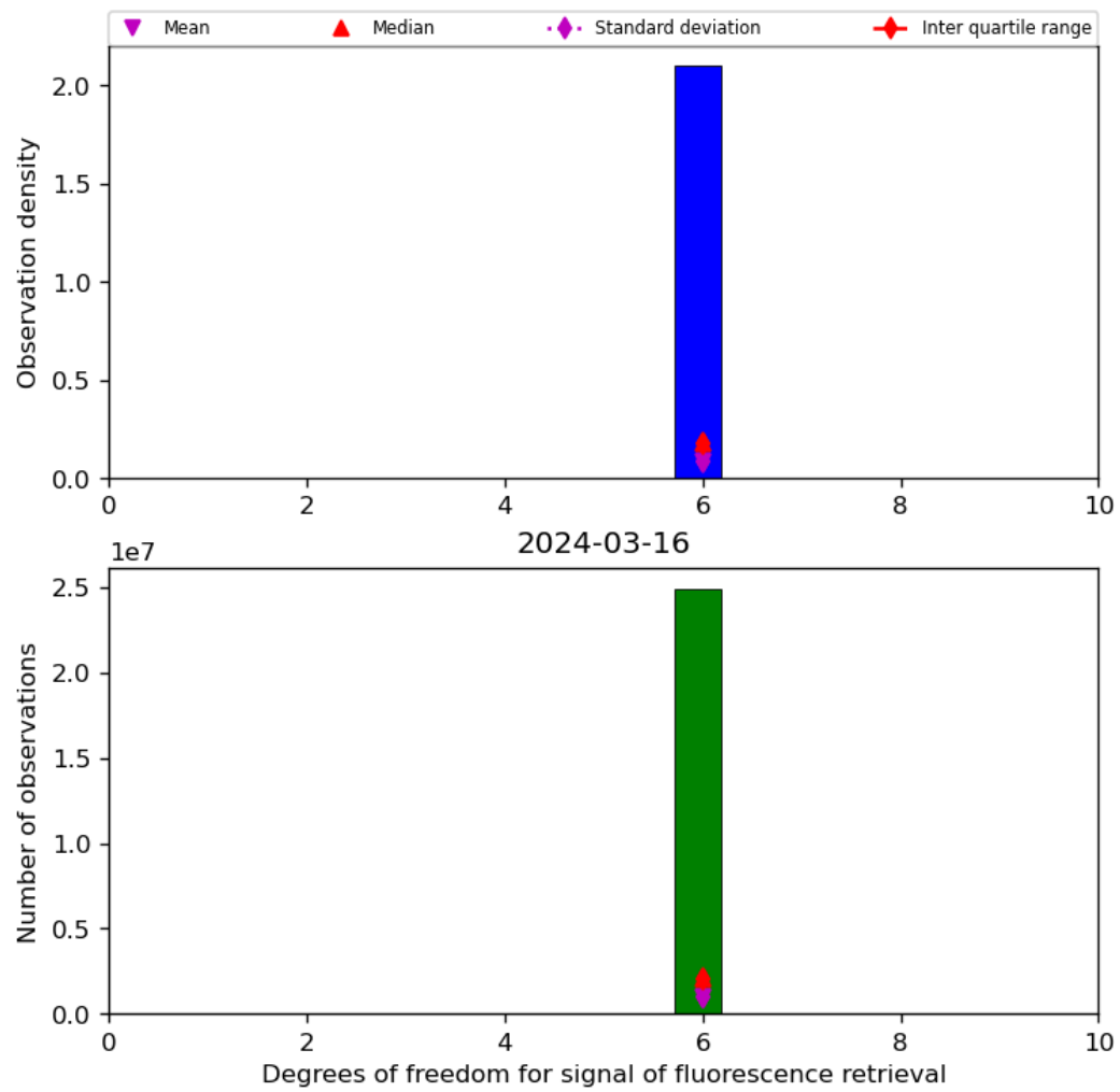
Figure 43: Histogram of “Degrees of freedom for signal of fluorescence retrieval” for 2024-03-15 to 2024-03-17
