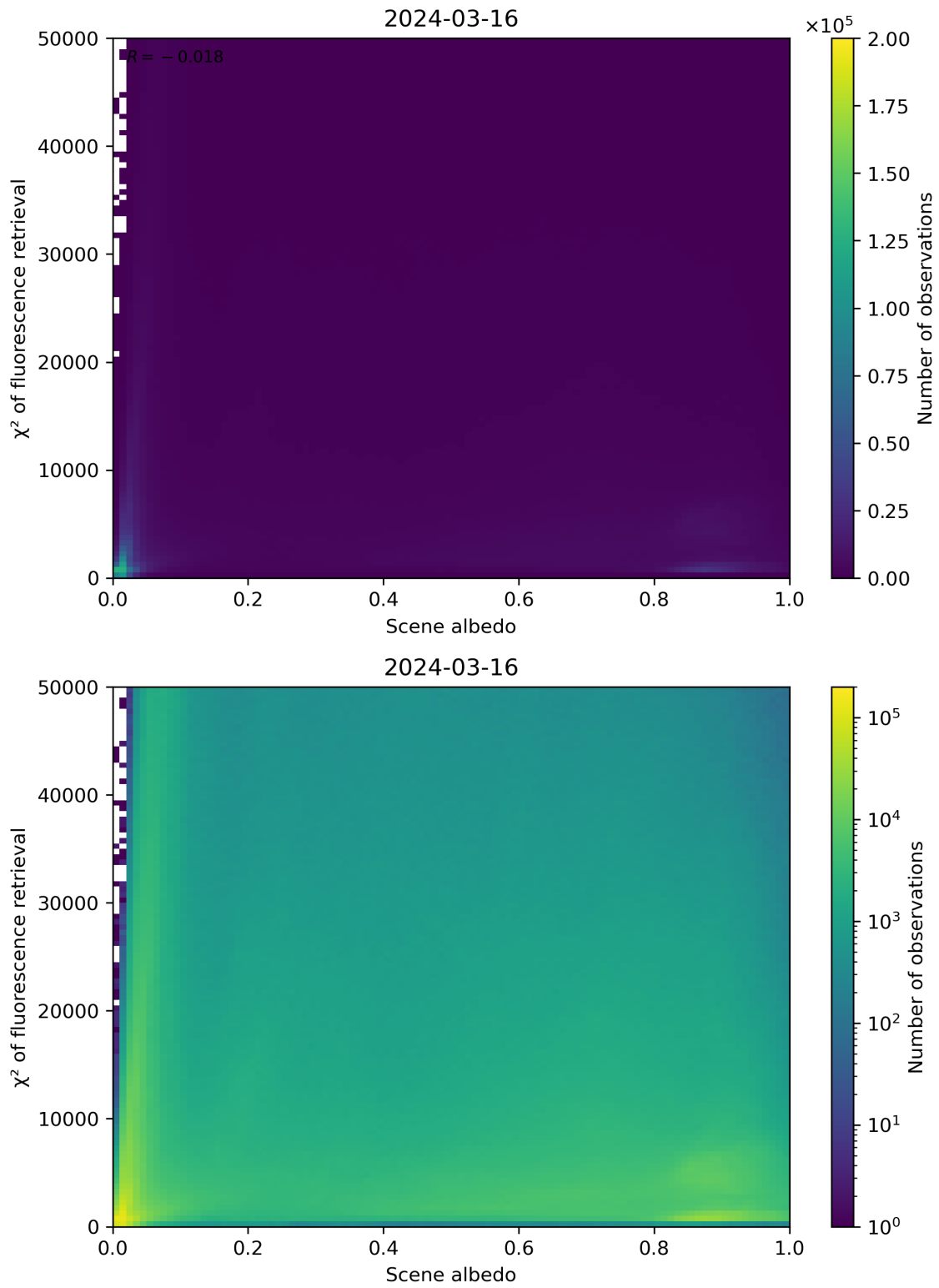
Figure 103: Scatter density plot of “Scene albedo” against “ \chi^2 of fluorescence retrieval” for 2024-03-15 to 2024-03-17.
