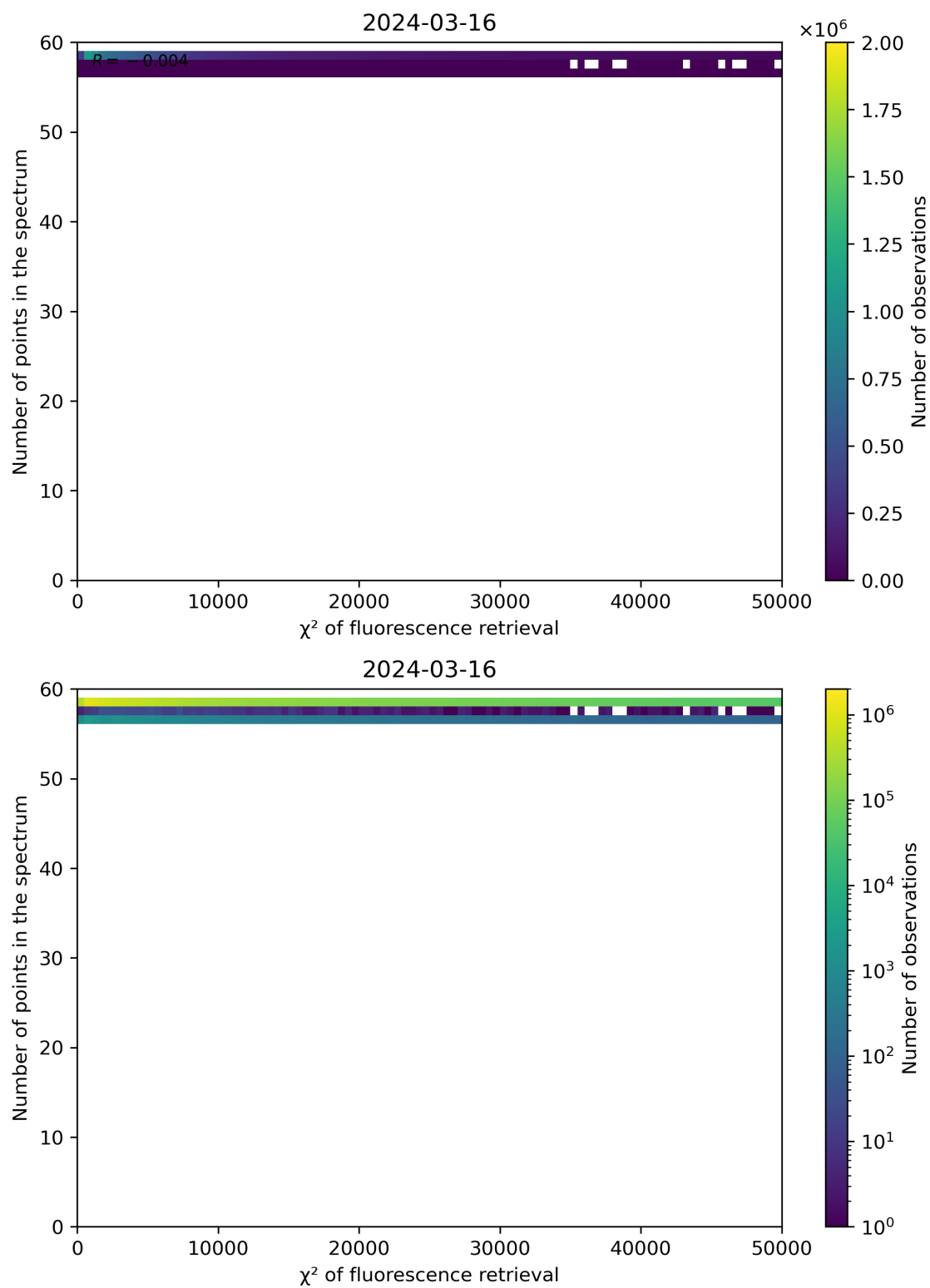
Figure 68: Scatter density plot of “ \chi^2 of fluorescence retrieval” against “Number of points in the spectrum” for 2024-03-15 to 2024-03-17.
