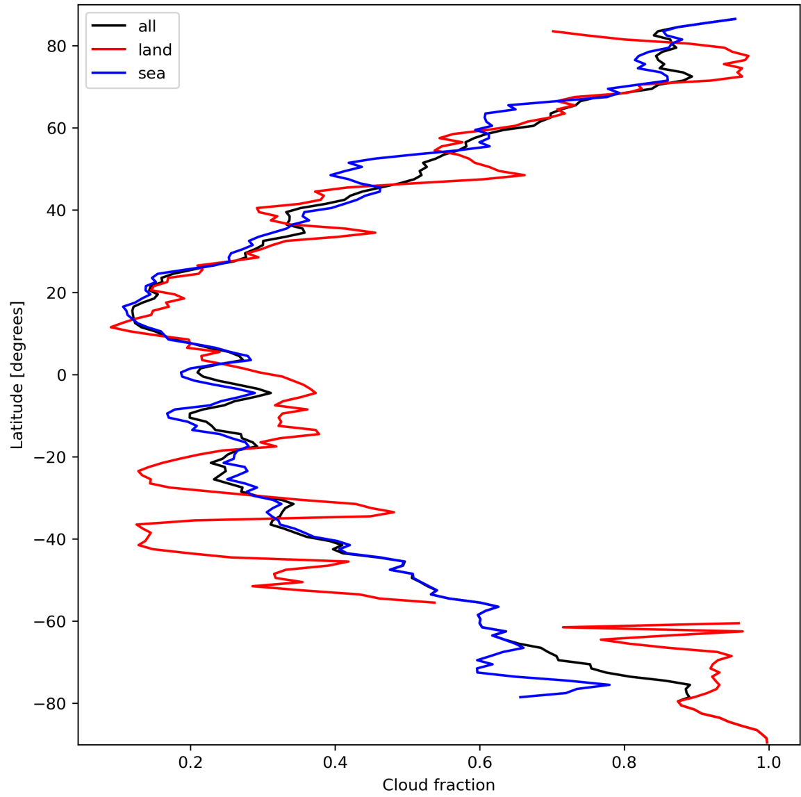
Figure 15: Zonal average of “Cloud fraction” for 2024-03-15 to 2024-03-17.
