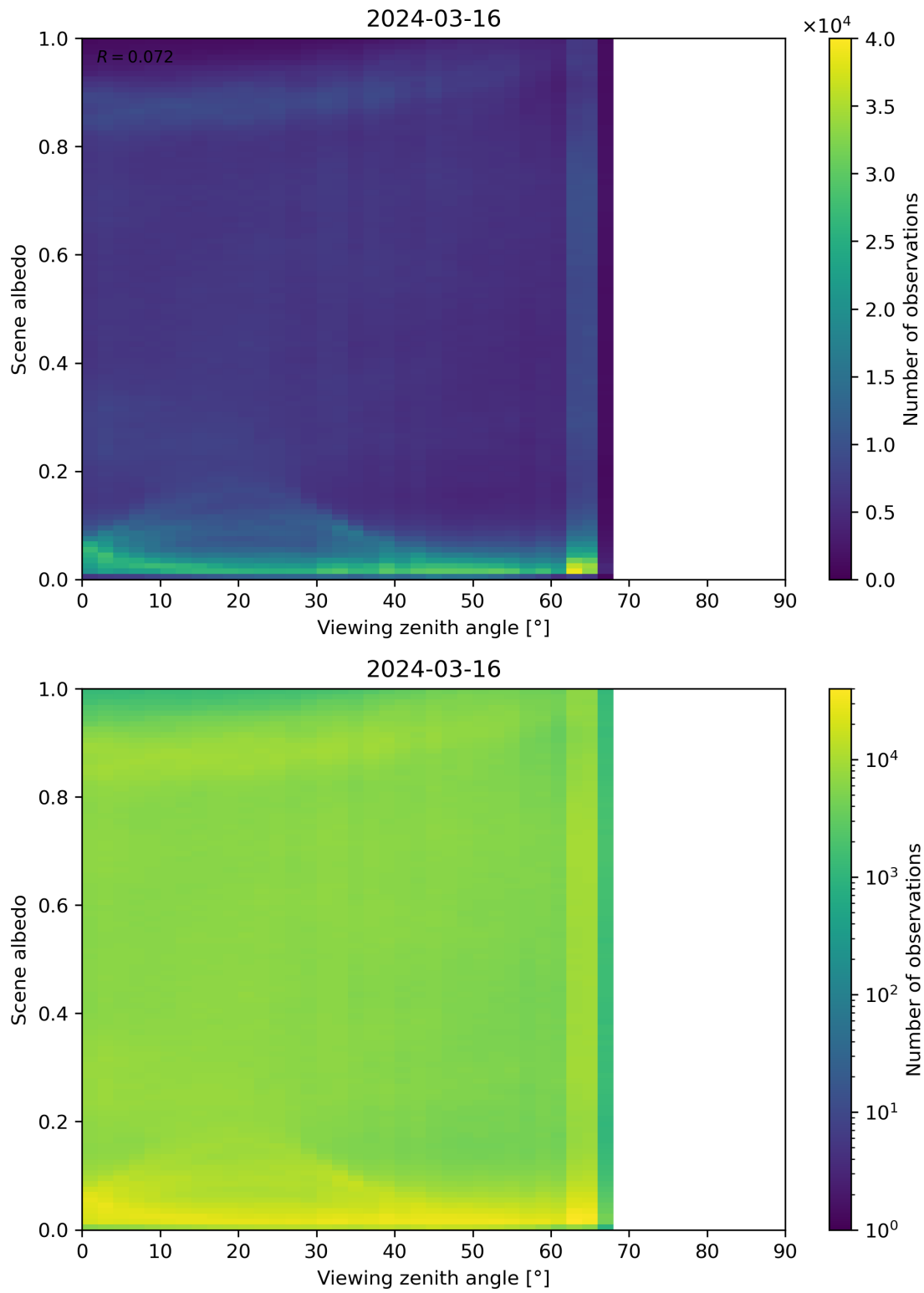
Figure 126: Scatter density plot of “Viewing zenith angle” against “Scene albedo” for 2024-03-15 to 2024-03-17.
