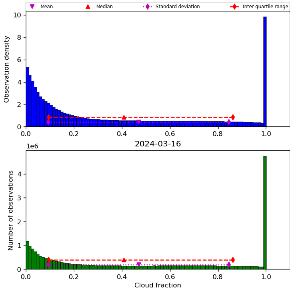
Figure 32: Histogram of “Cloud fraction” for 2024-03-15 to 2024-03-17
