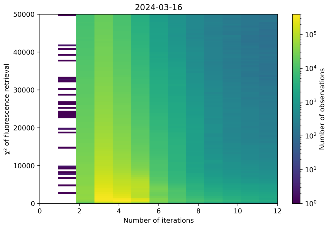
Figure 97: Scatter density plot of “Number of iterations” against “ \chi^2 of fluorescence retrieval” for 2024-03-15 to 2024-03-17.
