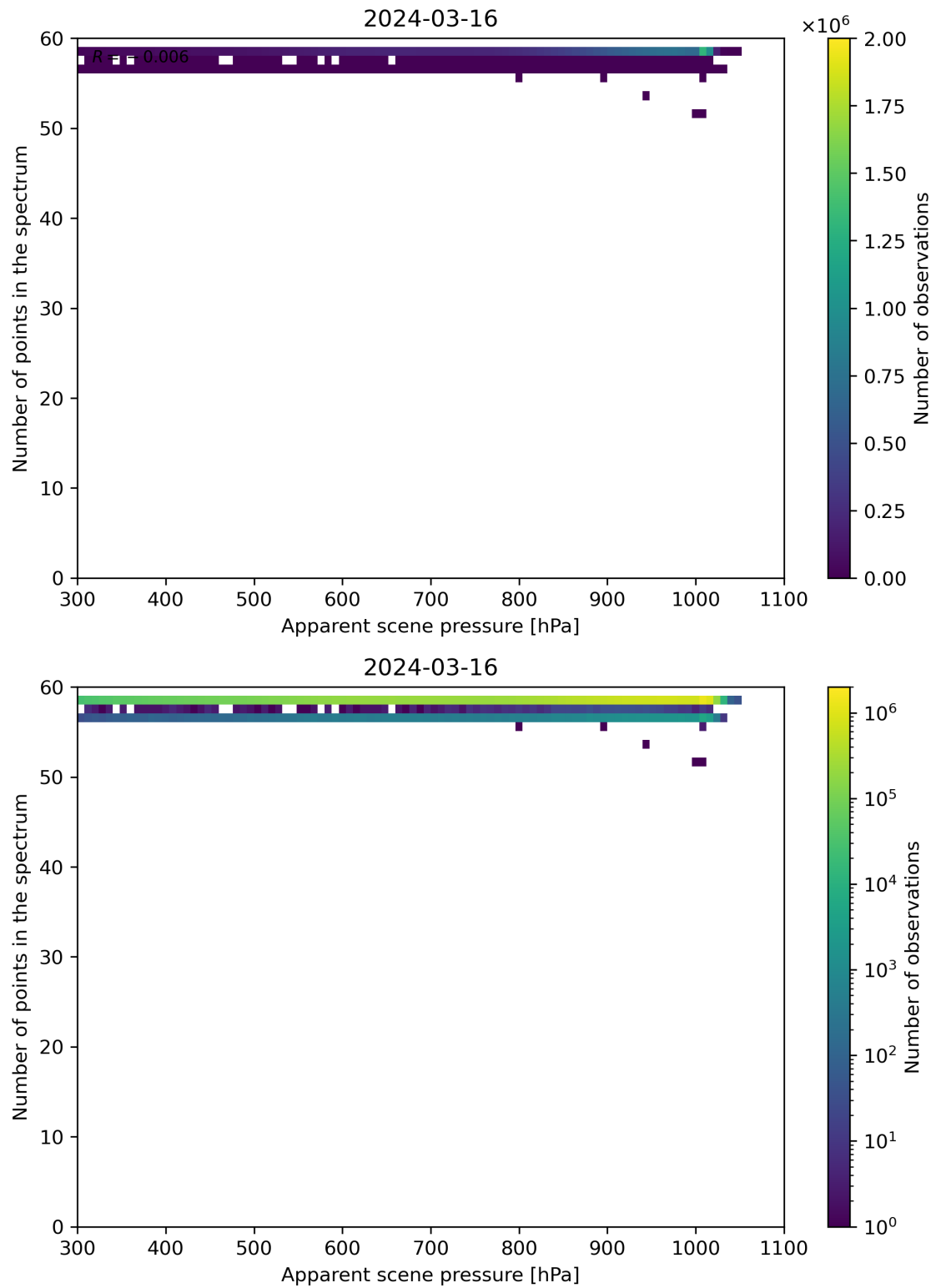
Figure 66: Scatter density plot of “Apparent scene pressure” against “Number of points in the spectrum” for 2024-03-15 to 2024-03-17.
