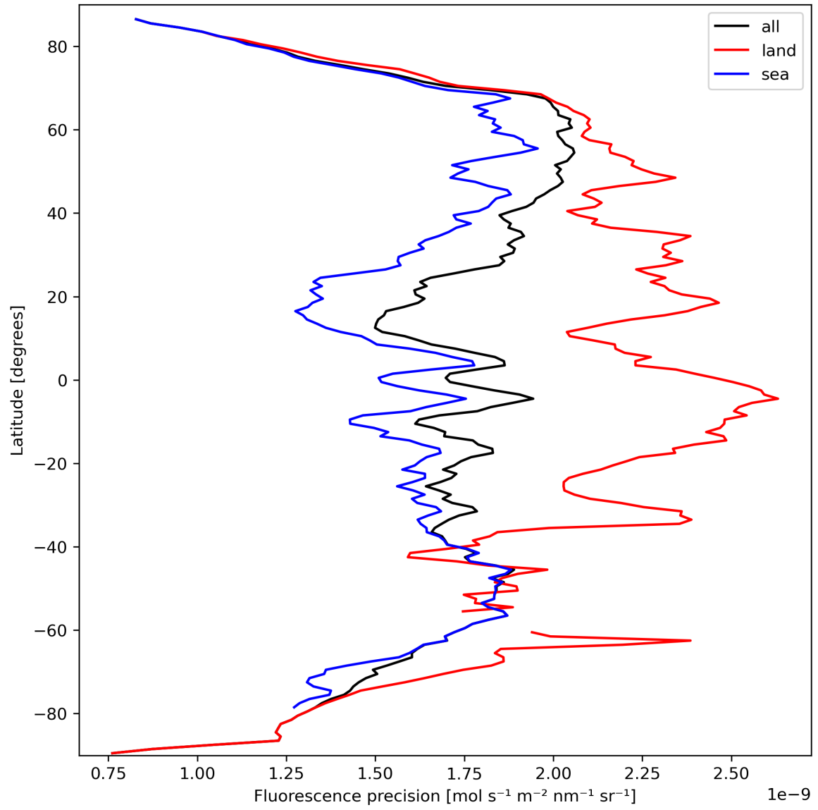
Figure 24: Zonal average of “Fluorescence precision” for 2024-03-15 to 2024-03-17.
