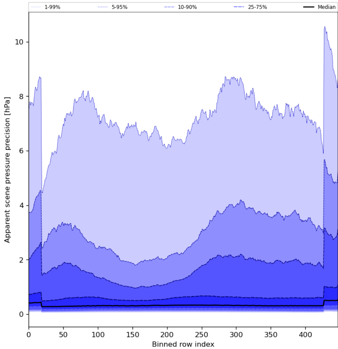
Figure 54: Along track statistics of “Apparent scene pressure precision” for 2024-03-15 to 2024-03-17
