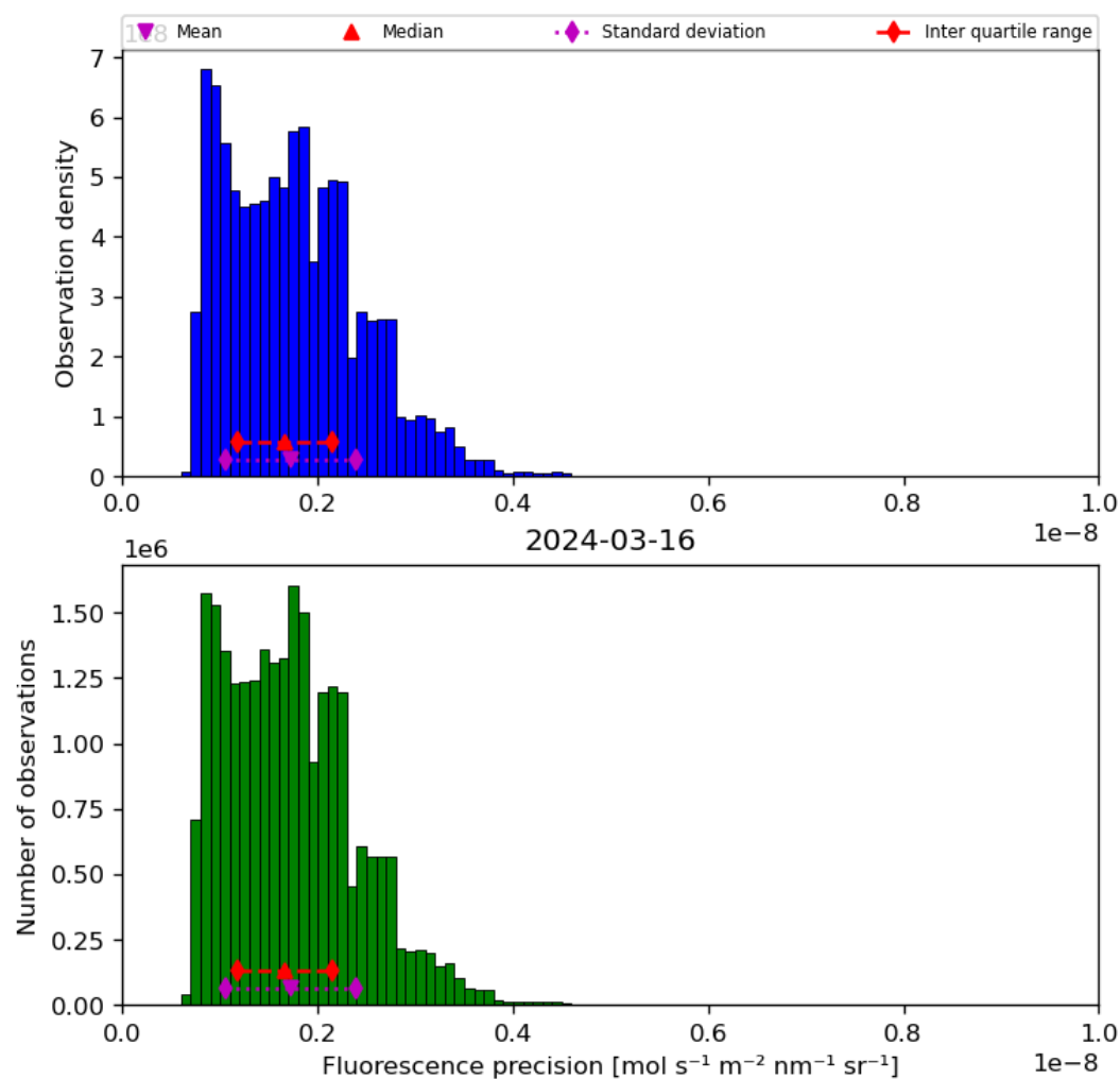
Figure 41: Histogram of “Fluorescence precision” for 2024-03-15 to 2024-03-17
