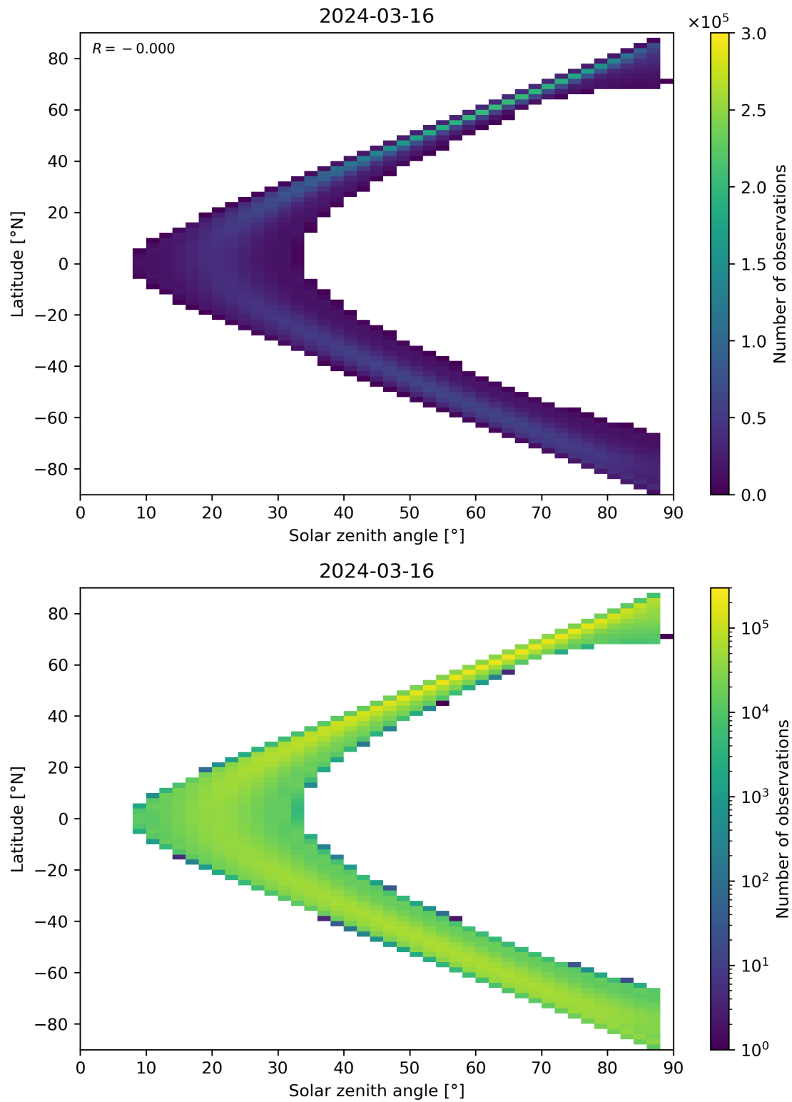
Figure 113: Scatter density plot of “Solar zenith angle” against “Latitude” for 2024-03-15 to 2024-03-17.
