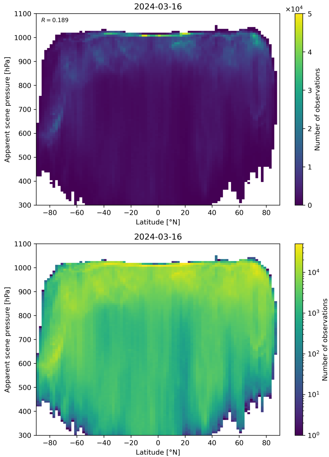
Figure 88: Scatter density plot of “Latitude” against “Apparent scene pressure” for 2024-03-15 to 2024-03-17.
