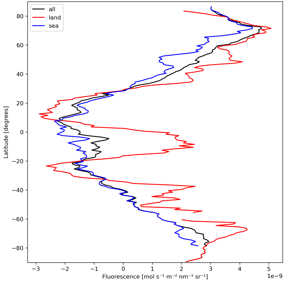
Figure 23: Zonal average of “Fluorescence” for 2024-03-15 to 2024-03-17.
