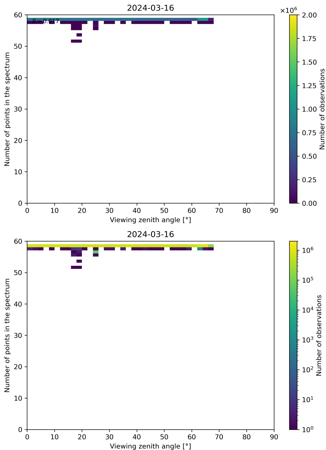
Figure 125: Scatter density plot of “Viewing zenith angle” against “Number of points in the spectrum” for 2024-03-15 to 2024-03-17.
