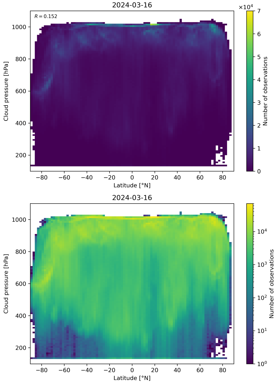
Figure 91: Scatter density plot of “Latitude” against “Cloud pressure” for 2024-03-15 to 2024-03-17.
