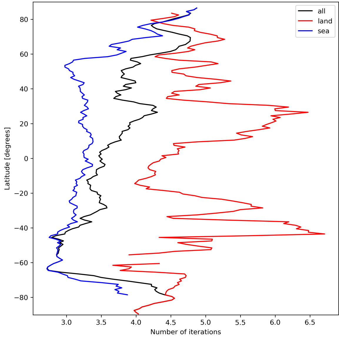
Figure 22: Zonal average of “Number of iterations” for 2024-03-15 to 2024-03-17.
