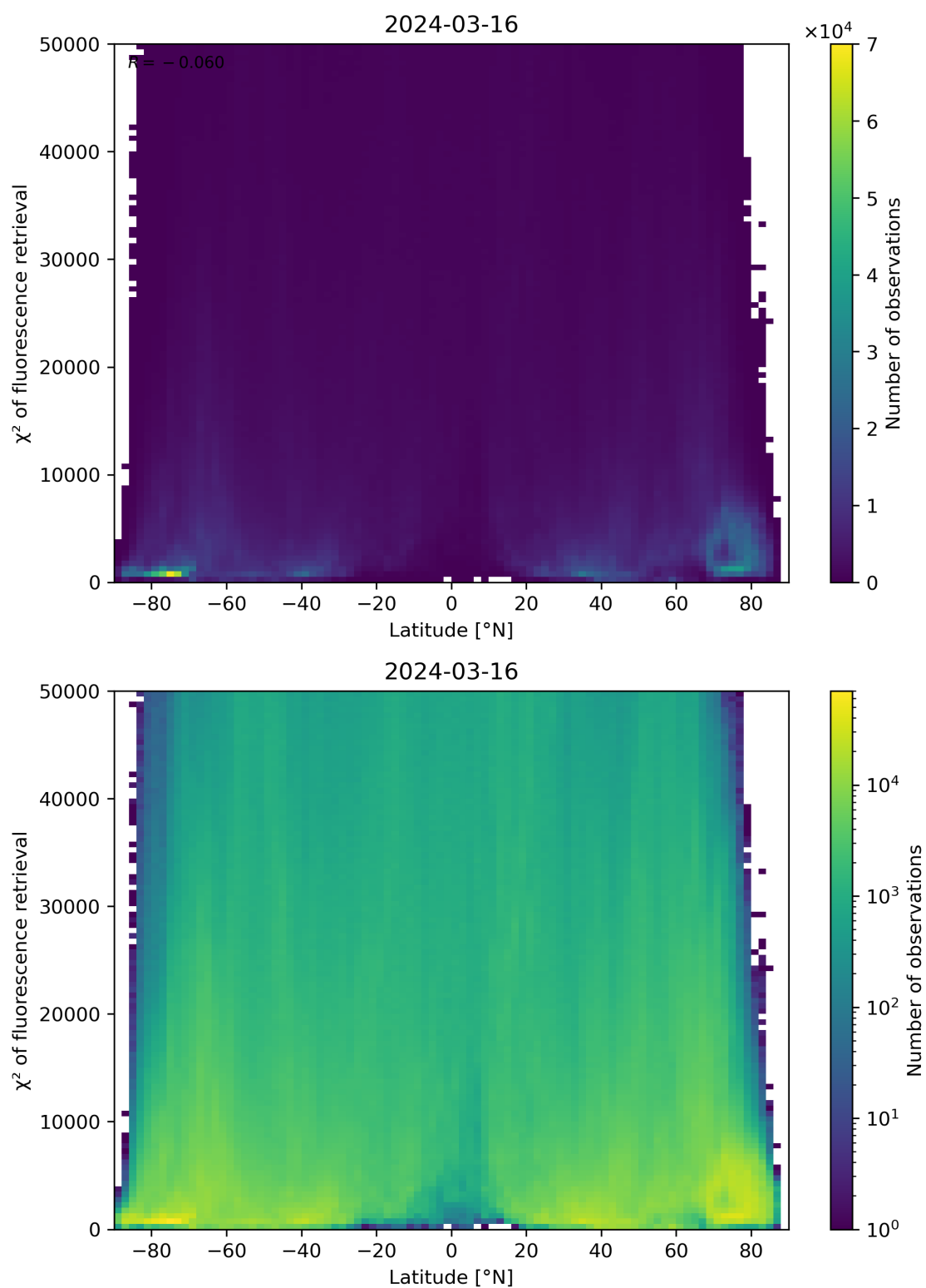
Figure 89: Scatter density plot of “Latitude” against “ \chi^2 of fluorescence retrieval” for 2024-03-15 to 2024-03-17.
