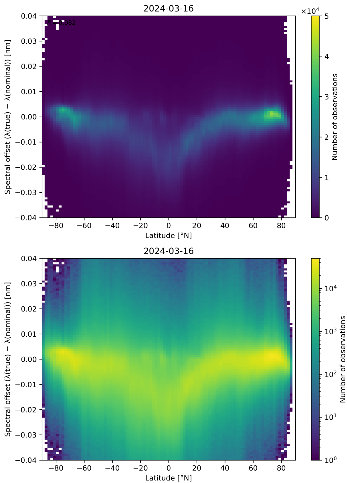
Figure 96: Scatter density plot of “Latitude” against “Spectral offset ( \lambda(\text{true}) - \lambda(\text{nominal}) )” for 2024-03-15 to 2024-03-17.
