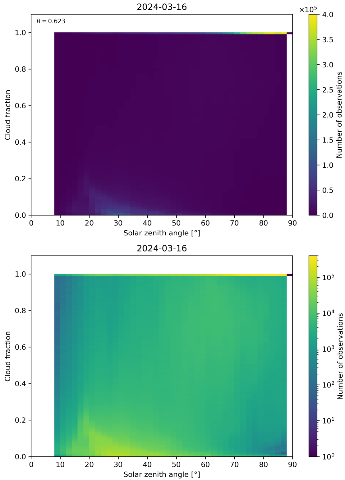
Figure 110: Scatter density plot of “Solar zenith angle” against “Cloud fraction” for 2024-03-15 to 2024-03-17.
