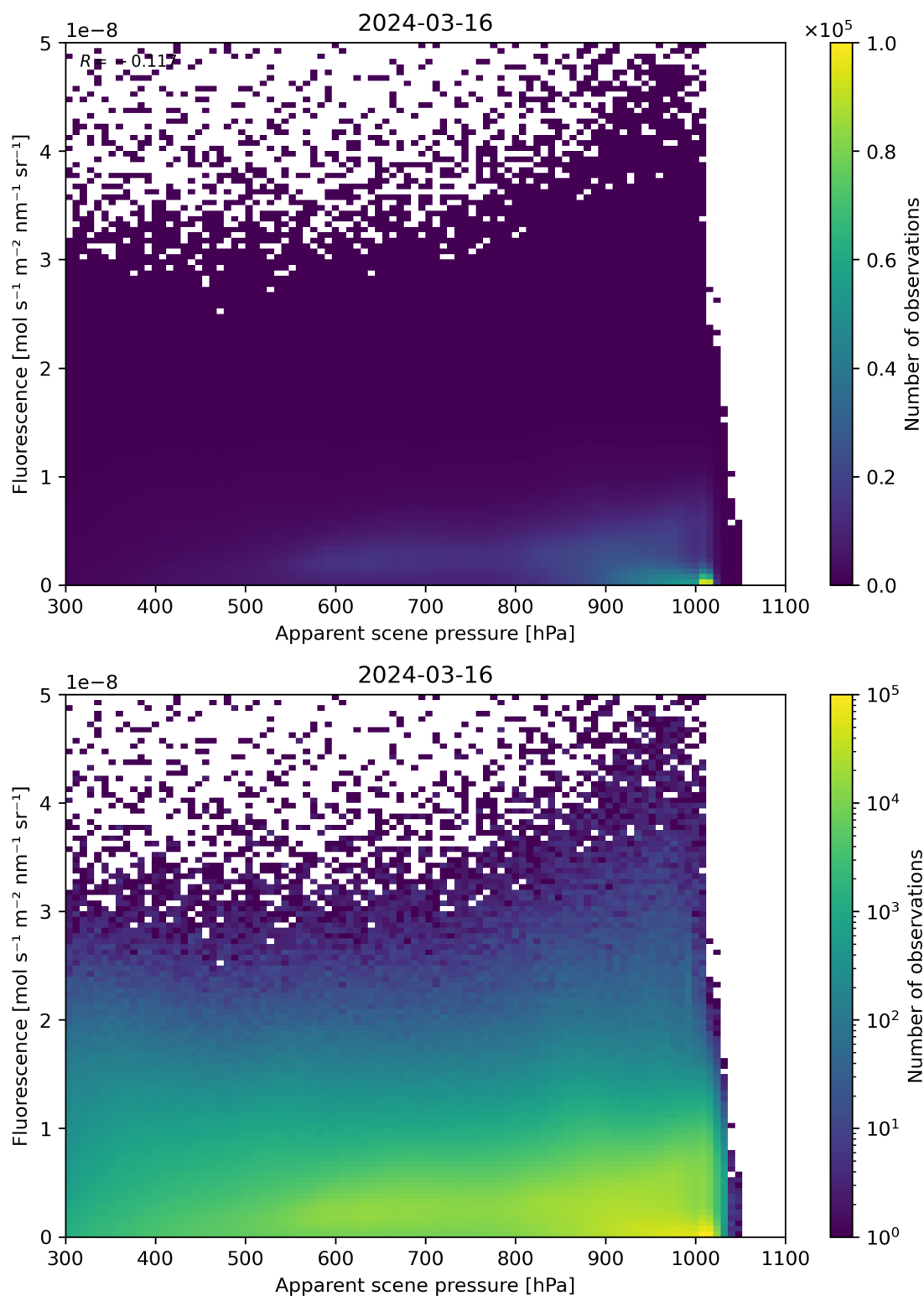
Figure 64: Scatter density plot of “Apparent scene pressure” against “Fluorescence” for 2024-03-15 to 2024-03-17.
