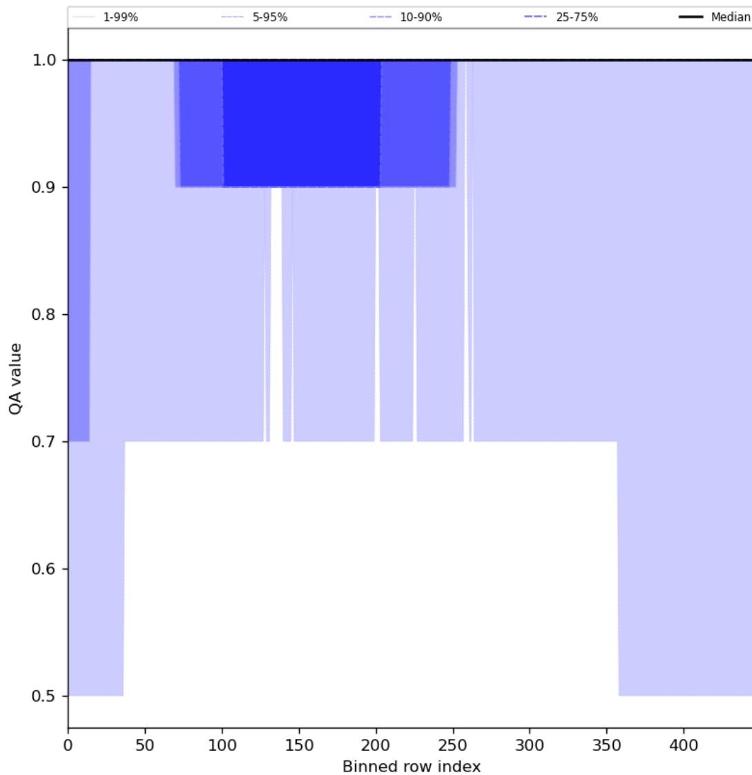
Figure 46: Along track statistics of “QA value” for 2024-03-15 to 2024-03-17
