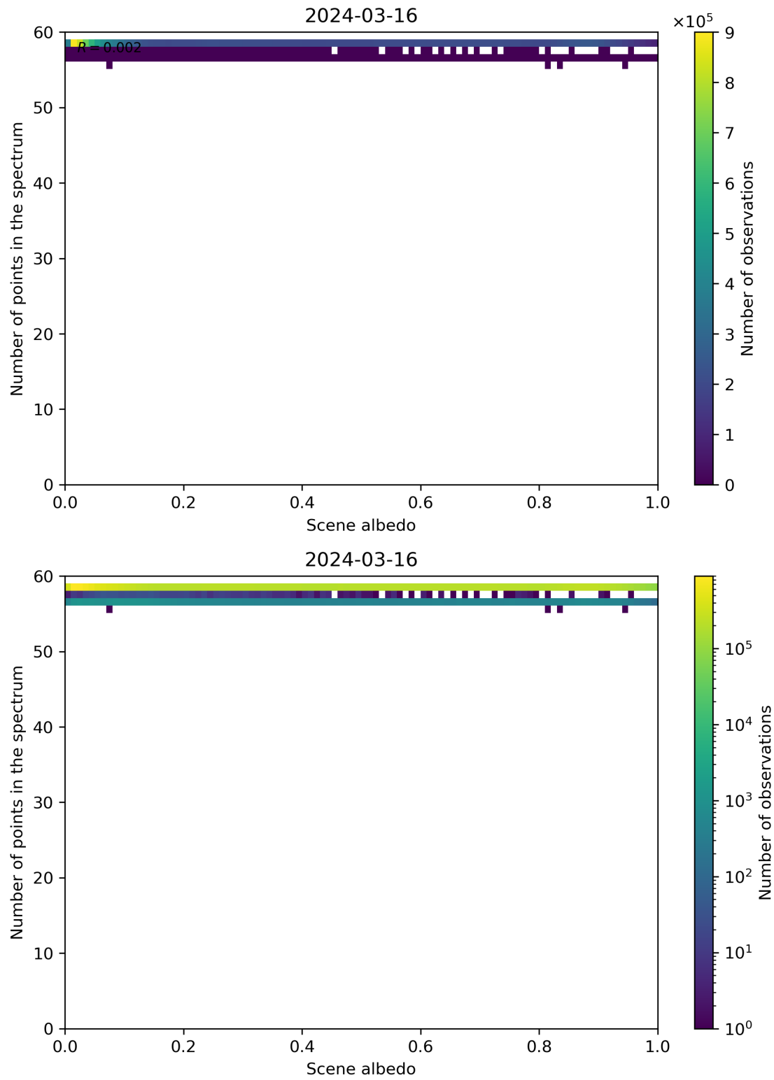
Figure 106: Scatter density plot of “Scene albedo” against “Number of points in the spectrum” for 2024-03-15 to 2024-03-17.
