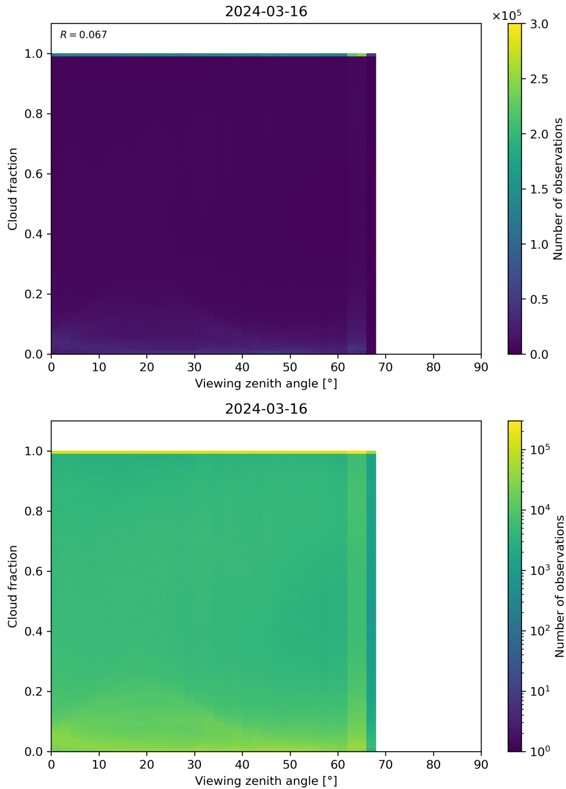
Figure 120: Scatter density plot of “Viewing zenith angle” against “Cloud fraction” for 2024-03-15 to 2024-03-17.
