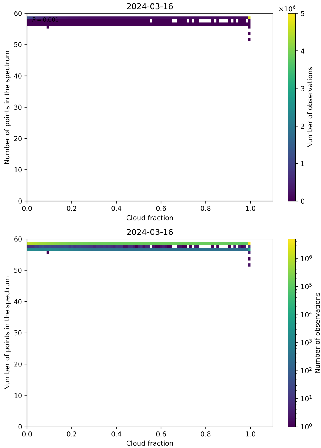
Figure 74: Scatter density plot of “Cloud fraction” against “Number of points in the spectrum” for 2024-03-15 to 2024-03-17.
