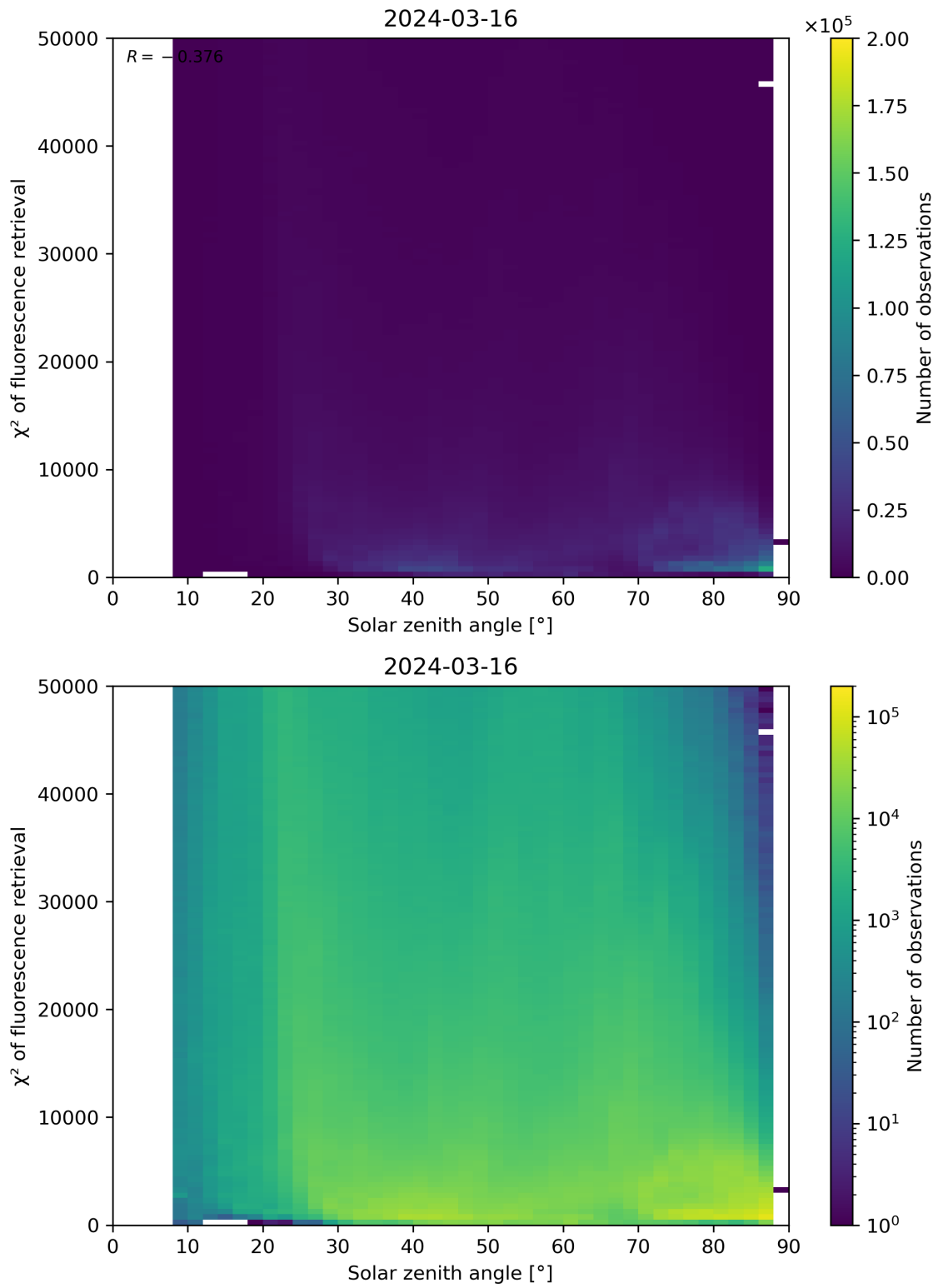
Figure 109: Scatter density plot of “Solar zenith angle” against “ \chi^2 of fluorescence retrieval” for 2024-03-15 to 2024-03-17.
