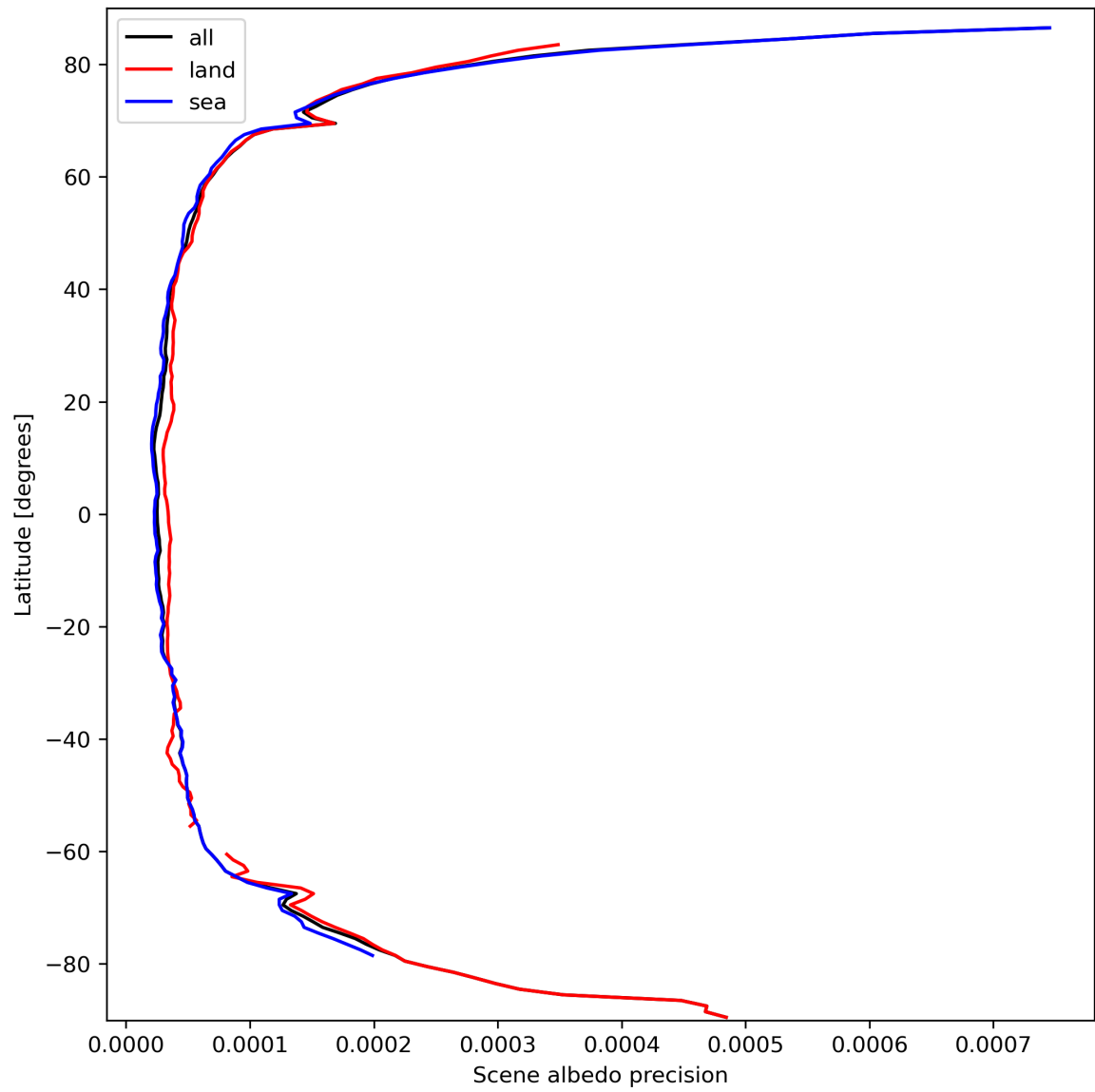
Figure 18: Zonal average of “Scene albedo precision” for 2024-03-15 to 2024-03-17.
