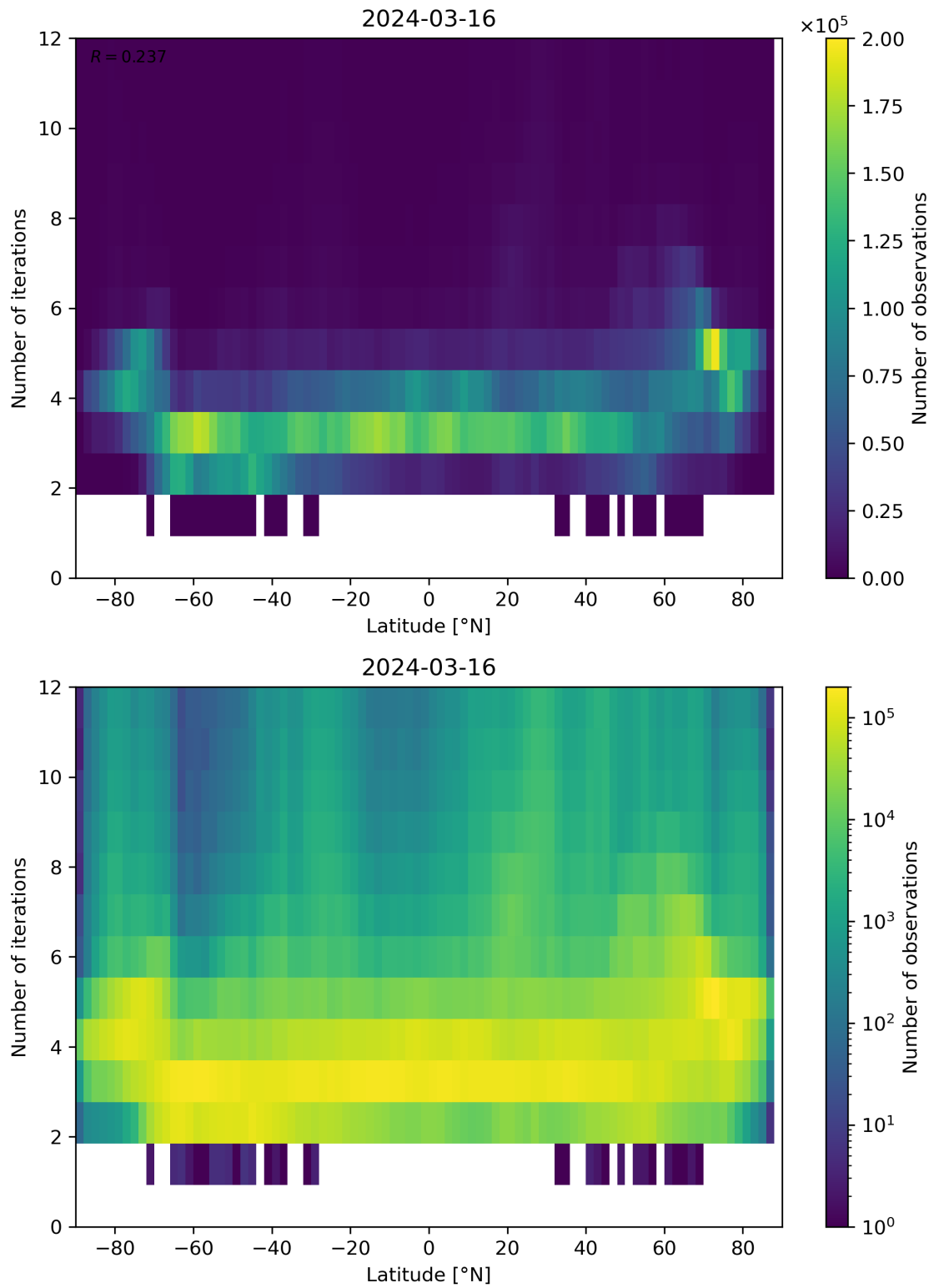
Figure 93: Scatter density plot of “Latitude” against “Number of iterations” for 2024-03-15 to 2024-03-17.
