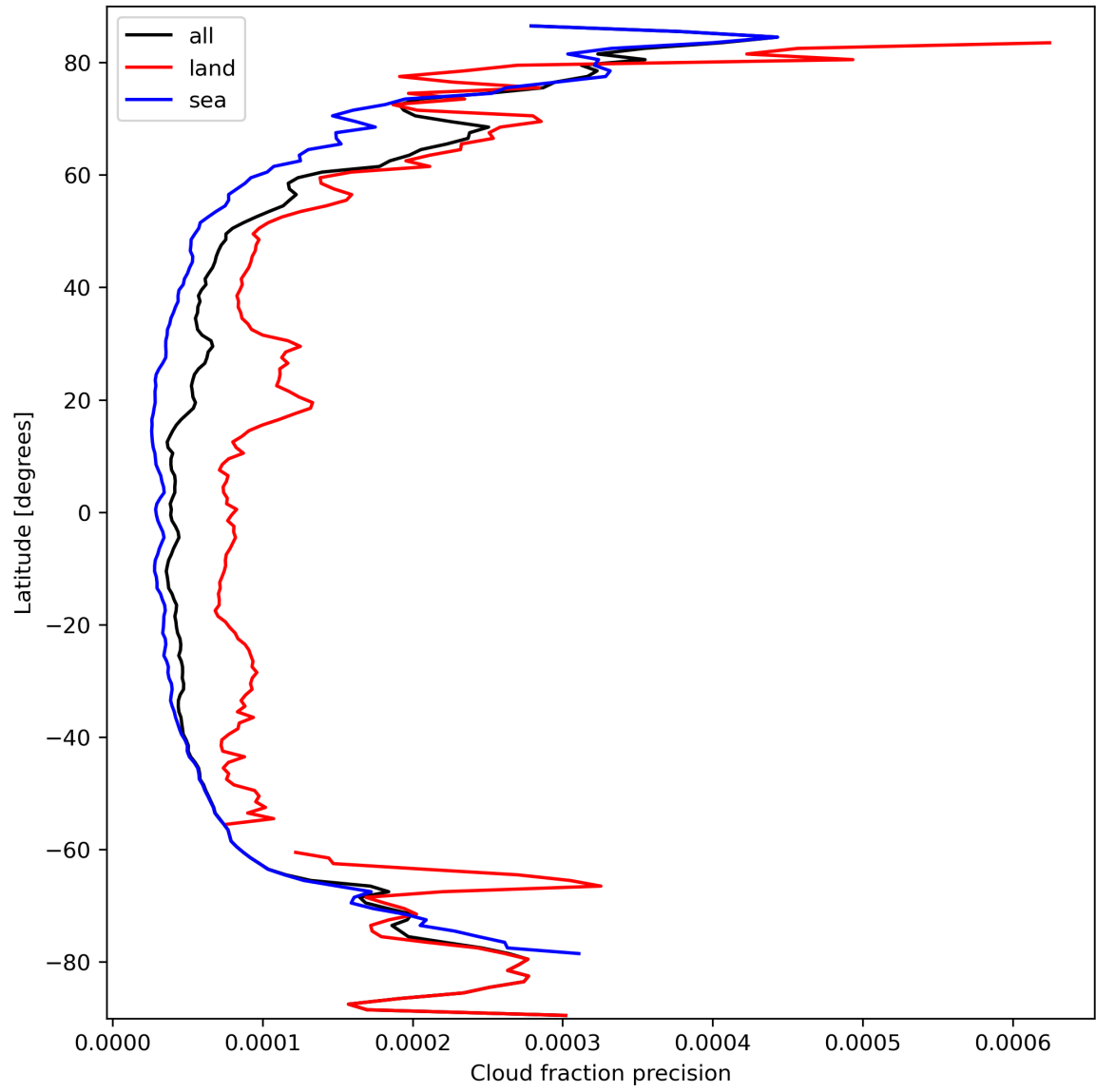
Figure 16: Zonal average of “Cloud fraction precision” for 2024-03-15 to 2024-03-17.
