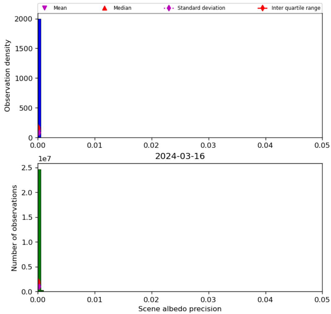
Figure 35: Histogram of “Scene albedo precision” for 2024-03-15 to 2024-03-17
