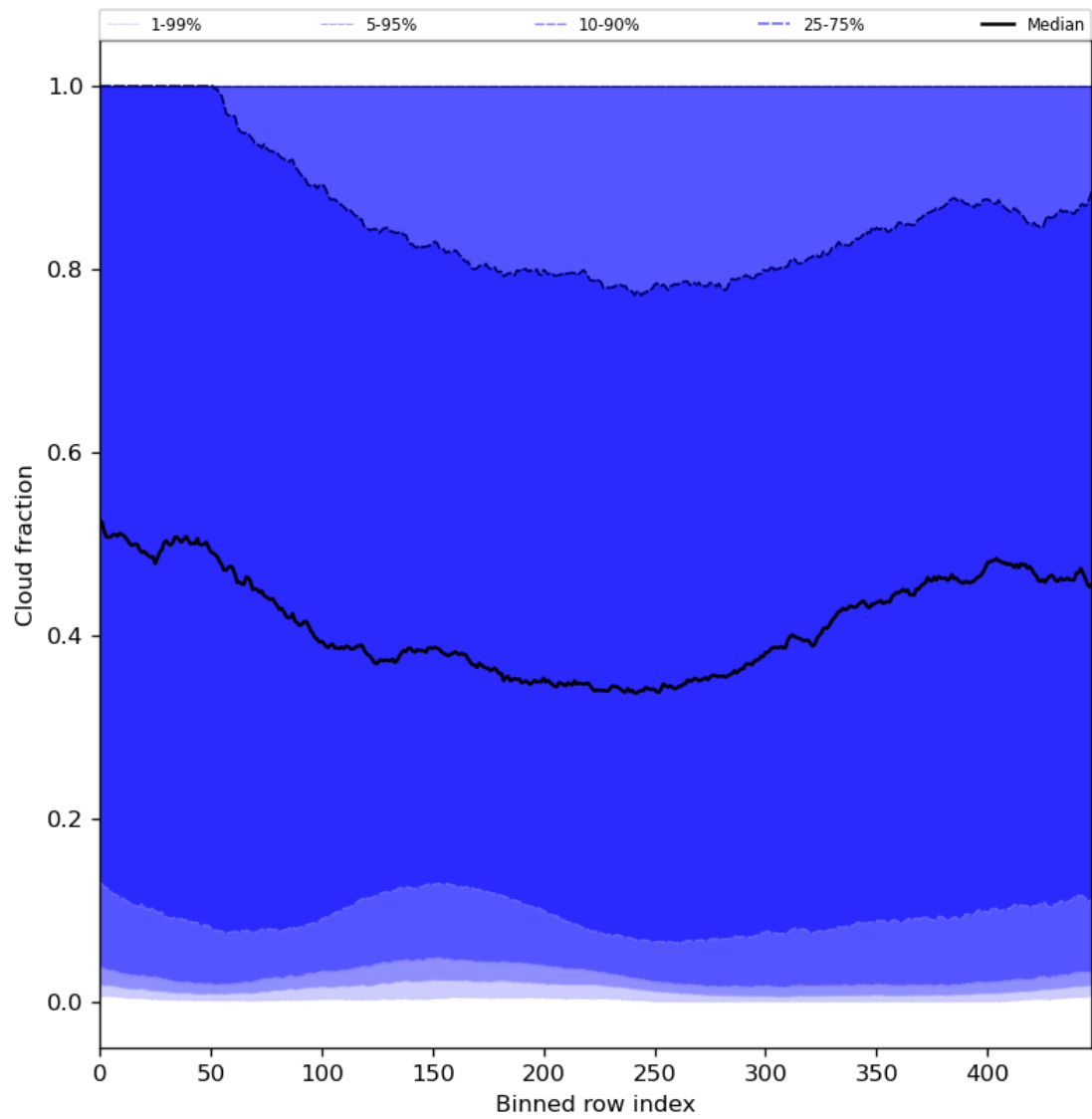
Figure 49: Along track statistics of “Cloud fraction” for 2024-03-15 to 2024-03-17
