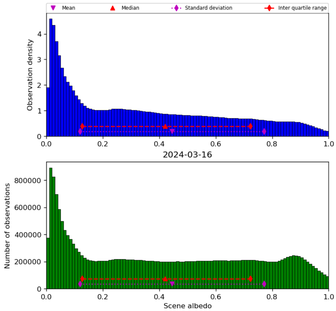
Figure 34: Histogram of “Scene albedo” for 2024-03-15 to 2024-03-17
