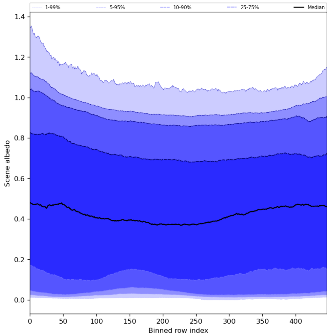
Figure 51: Along track statistics of “Scene albedo” for 2024-03-15 to 2024-03-17
