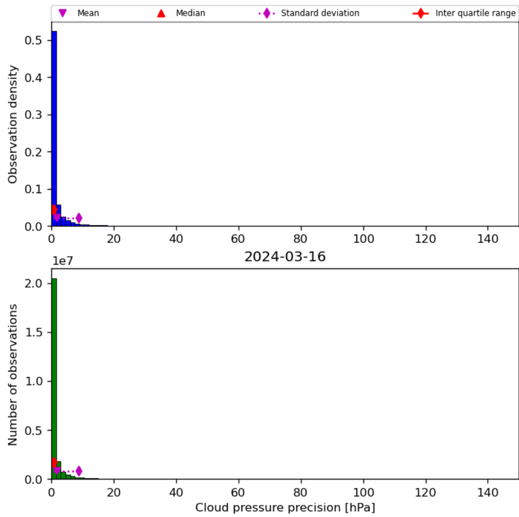
Figure 31: Histogram of “Cloud pressure precision” for 2024-03-15 to 2024-03-17
