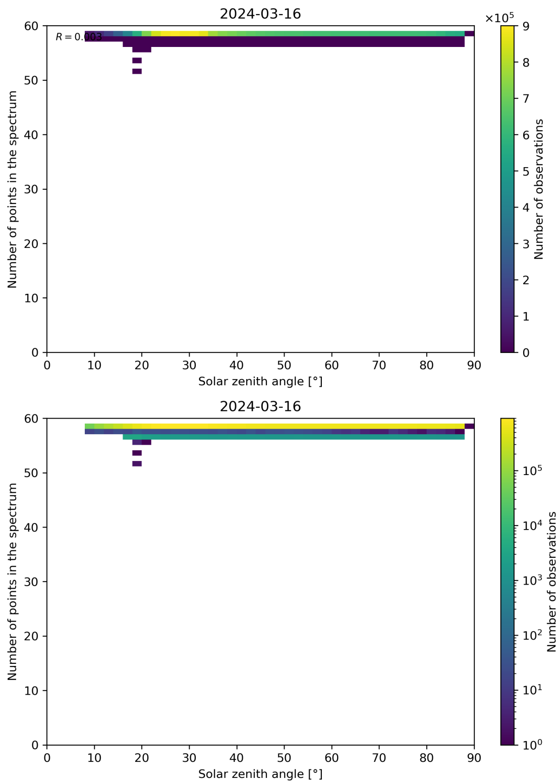
Figure 115: Scatter density plot of “Solar zenith angle” against “Number of points in the spectrum” for 2024-03-15 to 2024-03-17.
