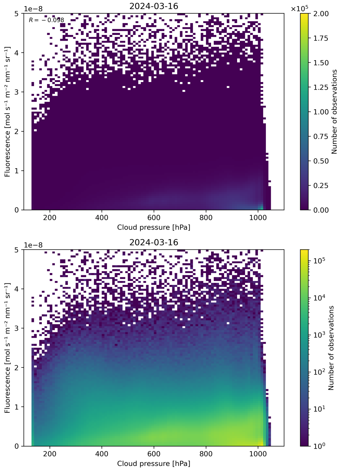
Figure 80: Scatter density plot of “Cloud pressure” against “Fluorescence” for 2024-03-15 to 2024-03-17.
