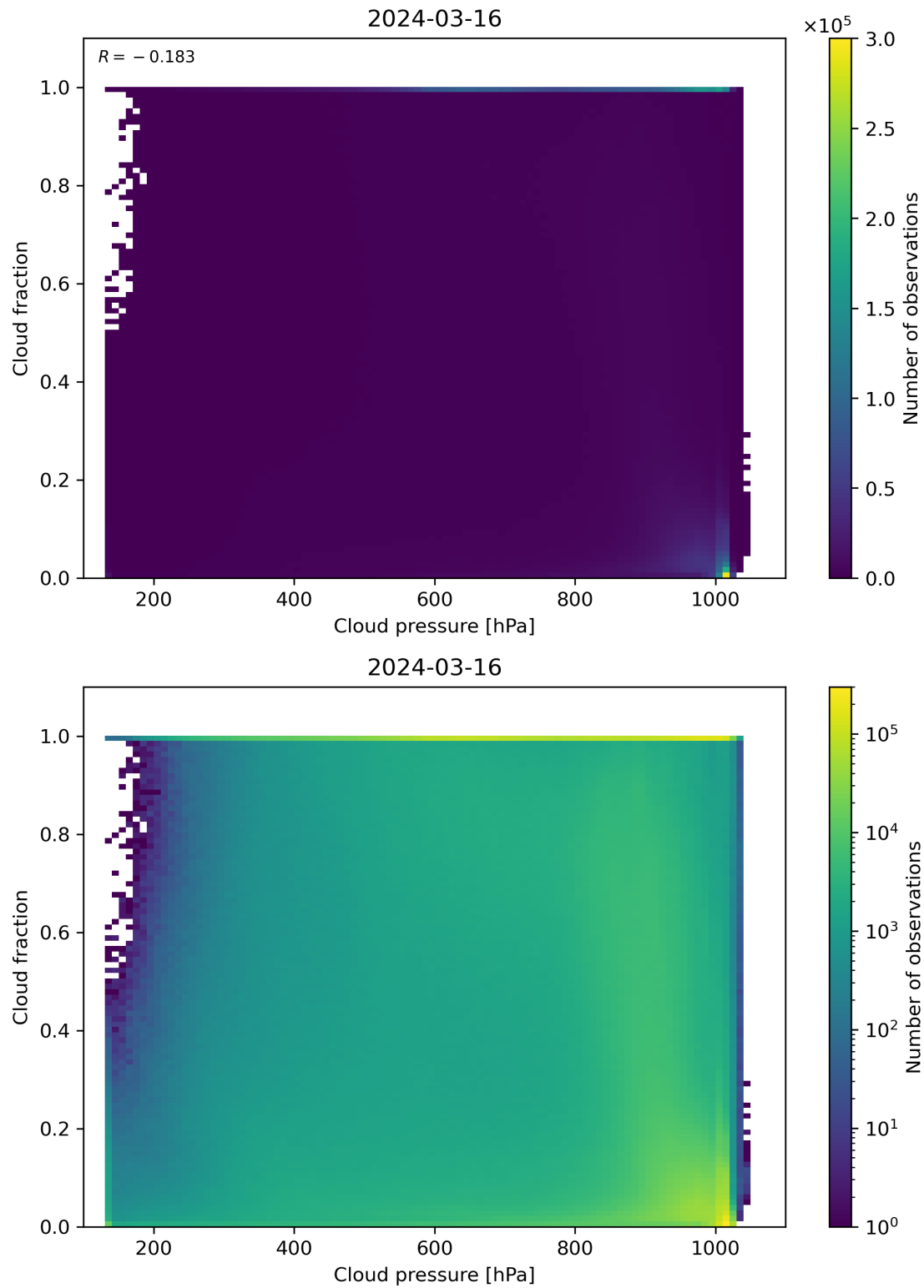
Figure 79: Scatter density plot of “Cloud pressure” against “Cloud fraction” for 2024-03-15 to 2024-03-17.
