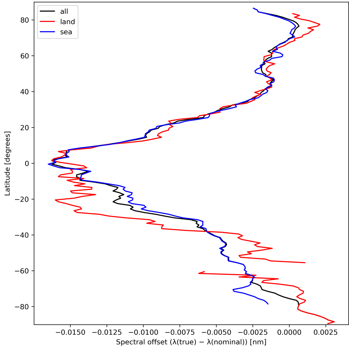
Figure 28: Zonal average of “Spectral offset ( \lambda(\text{true}) - \lambda(\text{nominal}) )” for 2024-03-15 to 2024-03-17.
