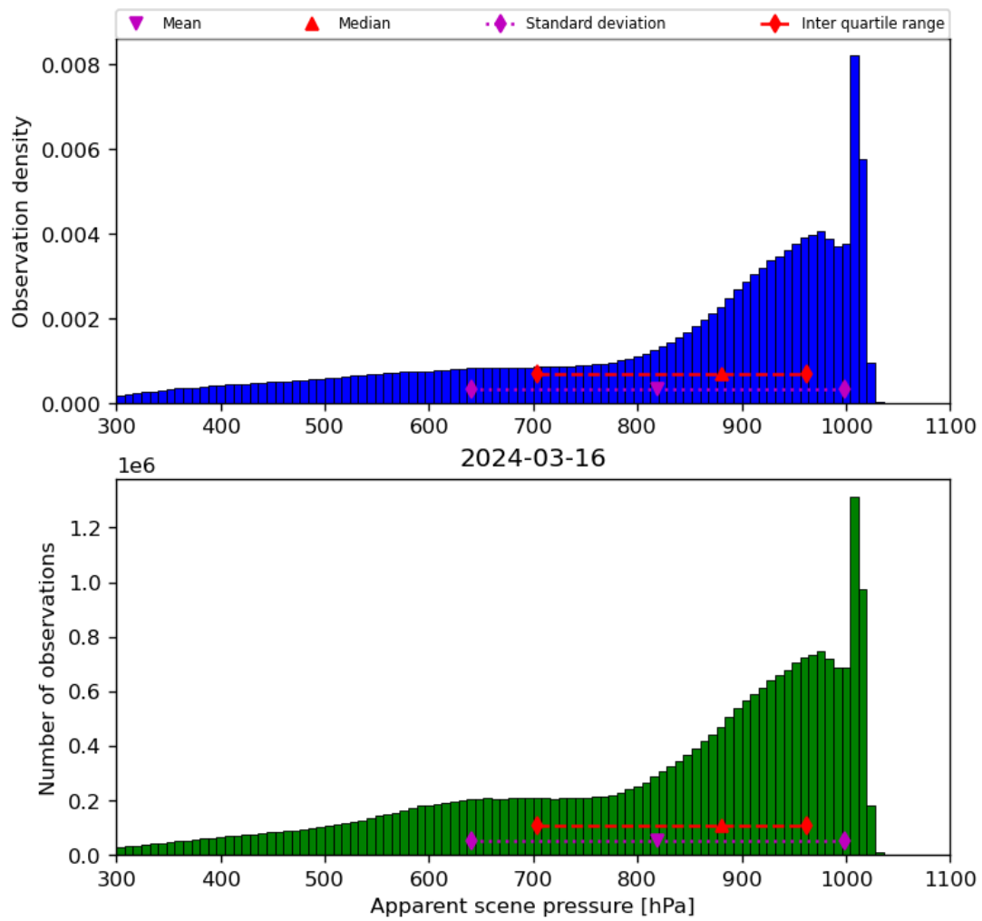
Figure 36: Histogram of “Apparent scene pressure” for 2024-03-15 to 2024-03-17
