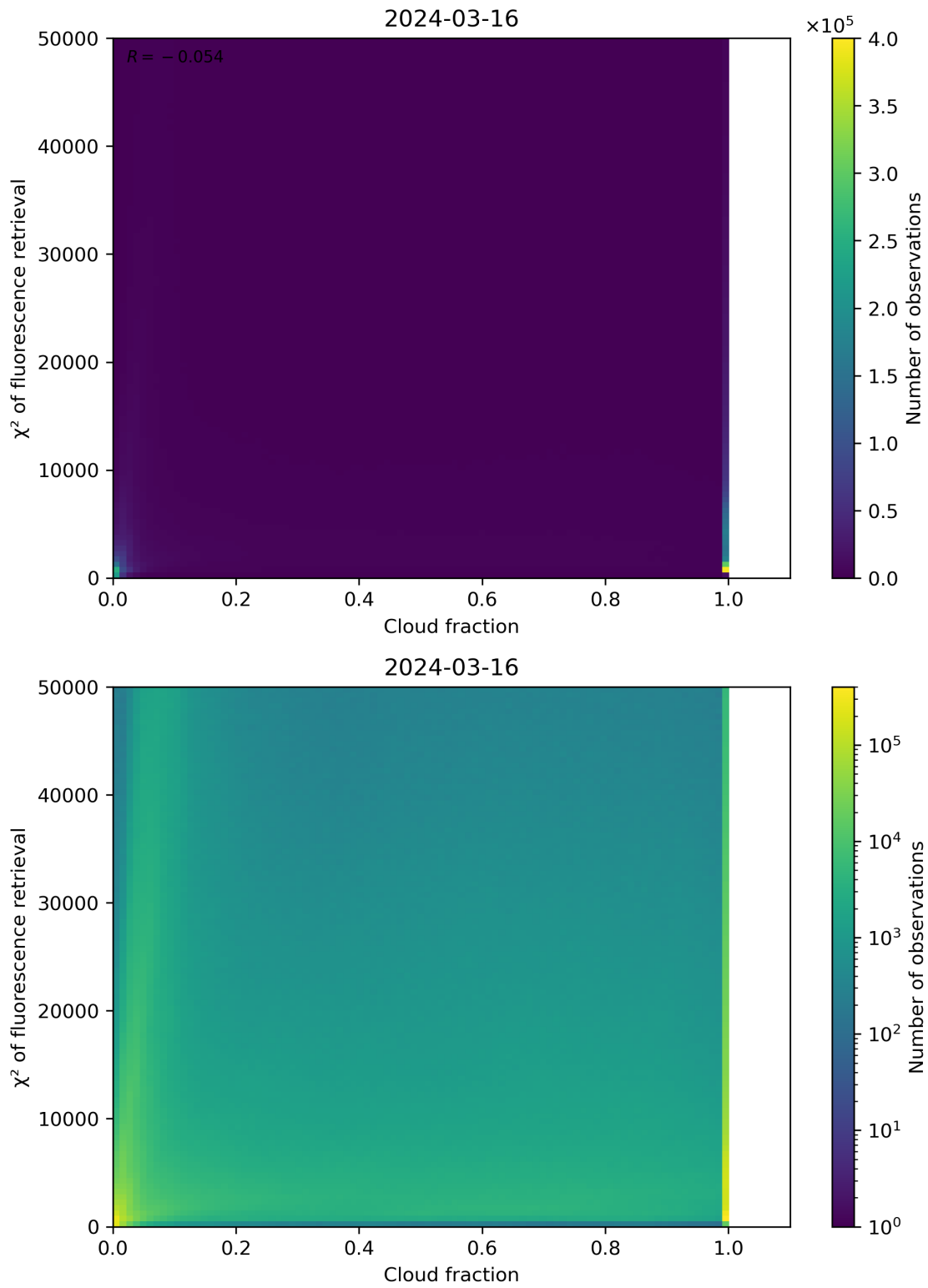
Figure 71: Scatter density plot of “Cloud fraction” against “ \chi^2 of fluorescence retrieval” for 2024-03-15 to 2024-03-17.
