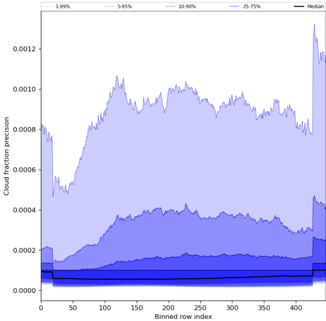
Figure 50: Along track statistics of “Cloud fraction precision” for 2024-03-15 to 2024-03-17
