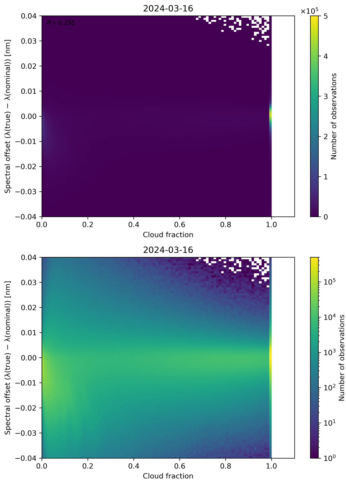
Figure 76: Scatter density plot of “Cloud fraction” against “Spectral offset ( \lambda(\text{true}) - \lambda(\text{nominal}) )” for 2024-03-15 to 2024-03-17.
