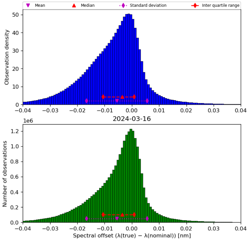
Figure 45: Histogram of “Spectral offset ( \lambda(\text{true}) - \lambda(\text{nominal}) )” for 2024-03-15 to 2024-03-17
