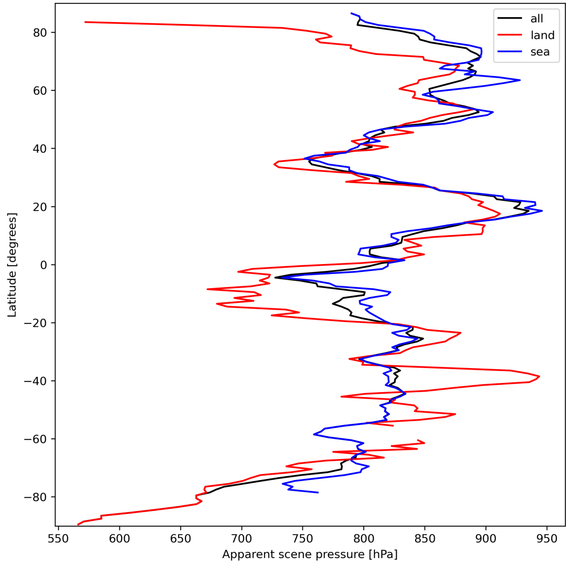
Figure 19: Zonal average of “Apparent scene pressure” for 2024-03-15 to 2024-03-17.
