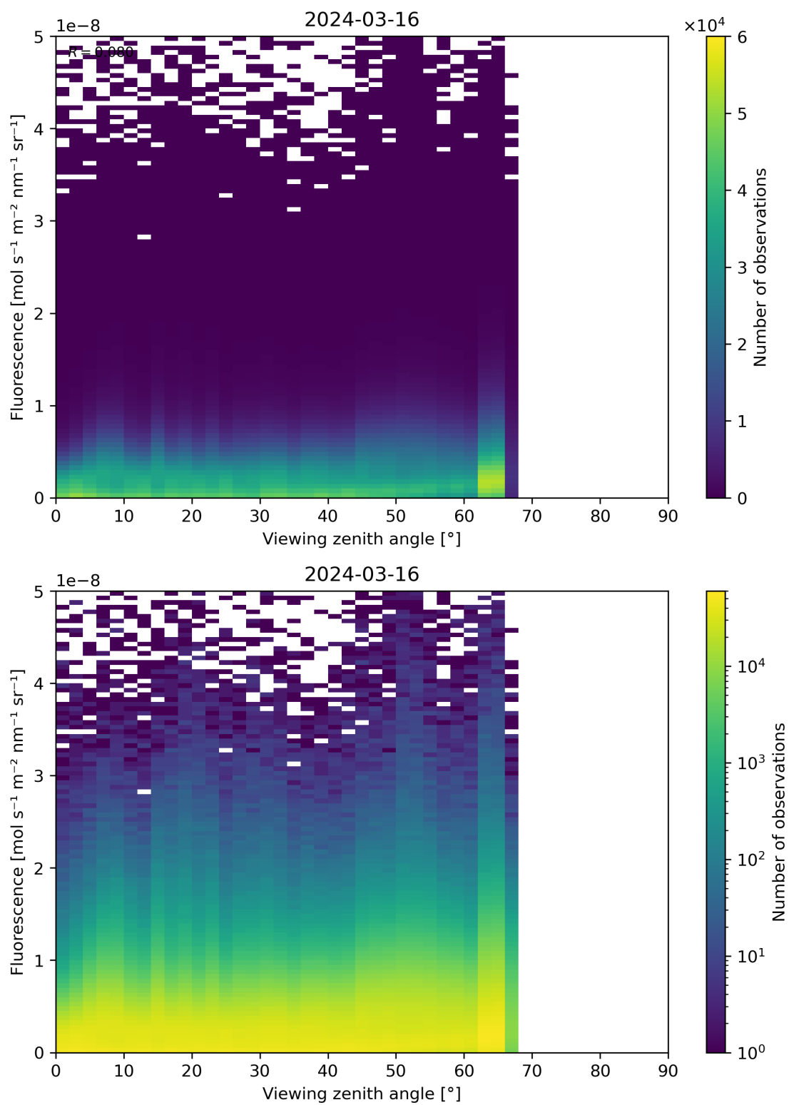
Figure 122: Scatter density plot of “Viewing zenith angle” against “Fluorescence” for 2024-03-15 to 2024-03-17.
