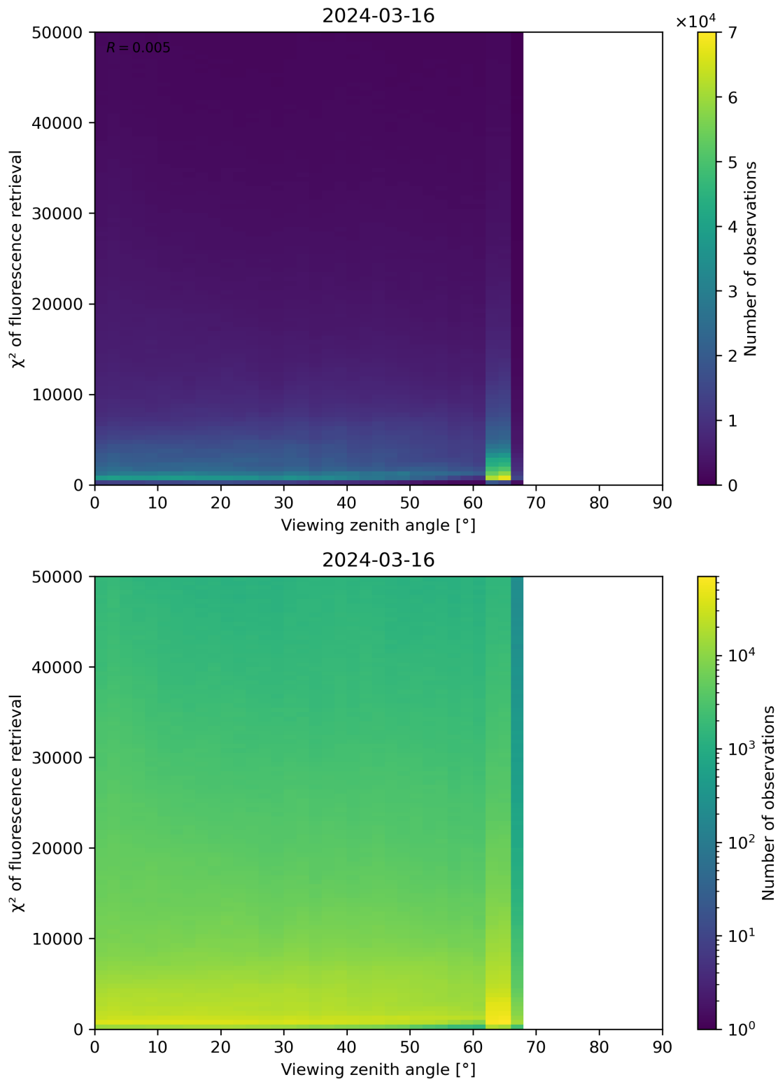
Figure 119: Scatter density plot of “Viewing zenith angle” against “ \chi^2 of fluorescence retrieval” for 2024-03-15 to 2024-03-17.
