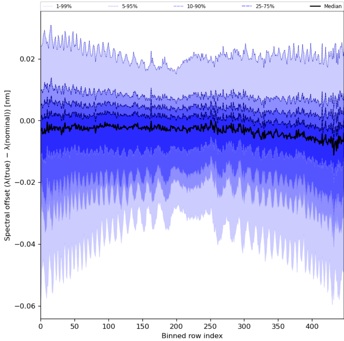
Figure 62: Along track statistics of “Spectral offset ( \lambda(\text{true}) - \lambda(\text{nominal}) )” for 2024-03-15 to 2024-03-17
