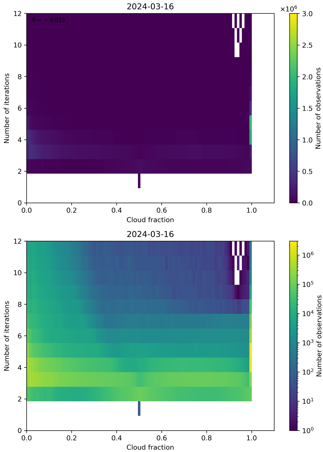
Figure 73: Scatter density plot of “Cloud fraction” against “Number of iterations” for 2024-03-15 to 2024-03-17.
