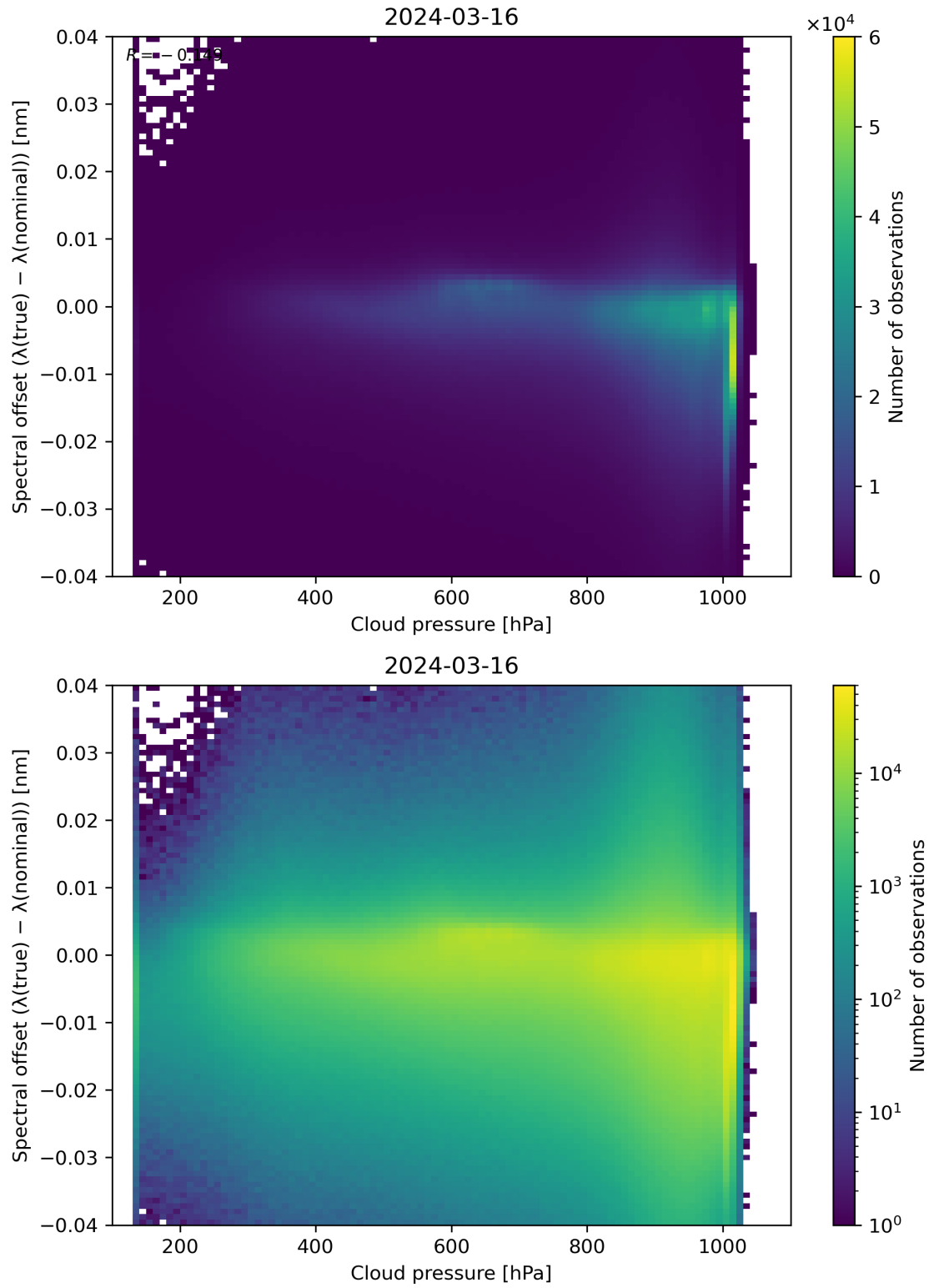
Figure 84: Scatter density plot of “Cloud pressure” against “Spectral offset ( \lambda(\text{true}) - \lambda(\text{nominal}) )” for 2024-03-15 to 2024-03-17.
