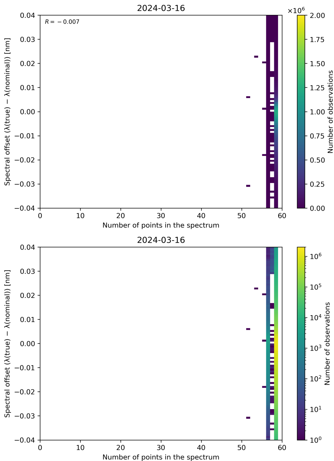
Figure 101: Scatter density plot of “Number of points in the spectrum” against “Spectral offset ( \lambda(\text{true}) - \lambda(\text{nominal}) )” for 2024-03-15 to 2024-03-17.
