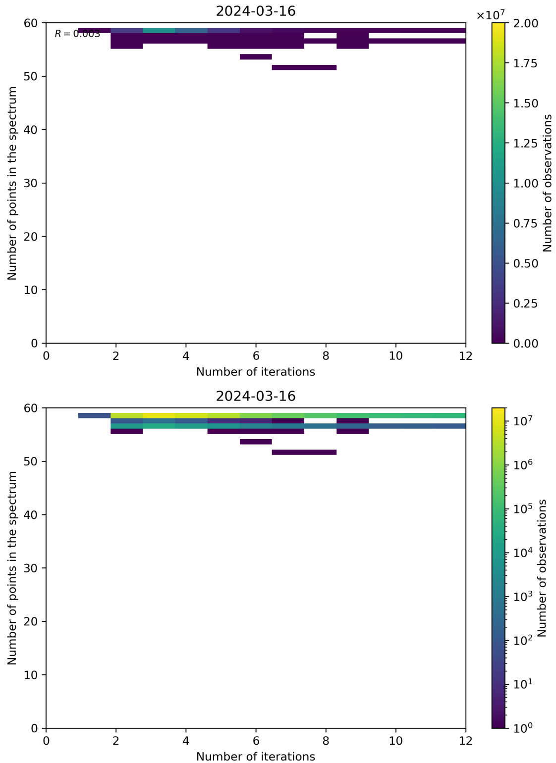
Figure 99: Scatter density plot of “Number of iterations” against “Number of points in the spectrum” for 2024-03-15 to 2024-03-17.
