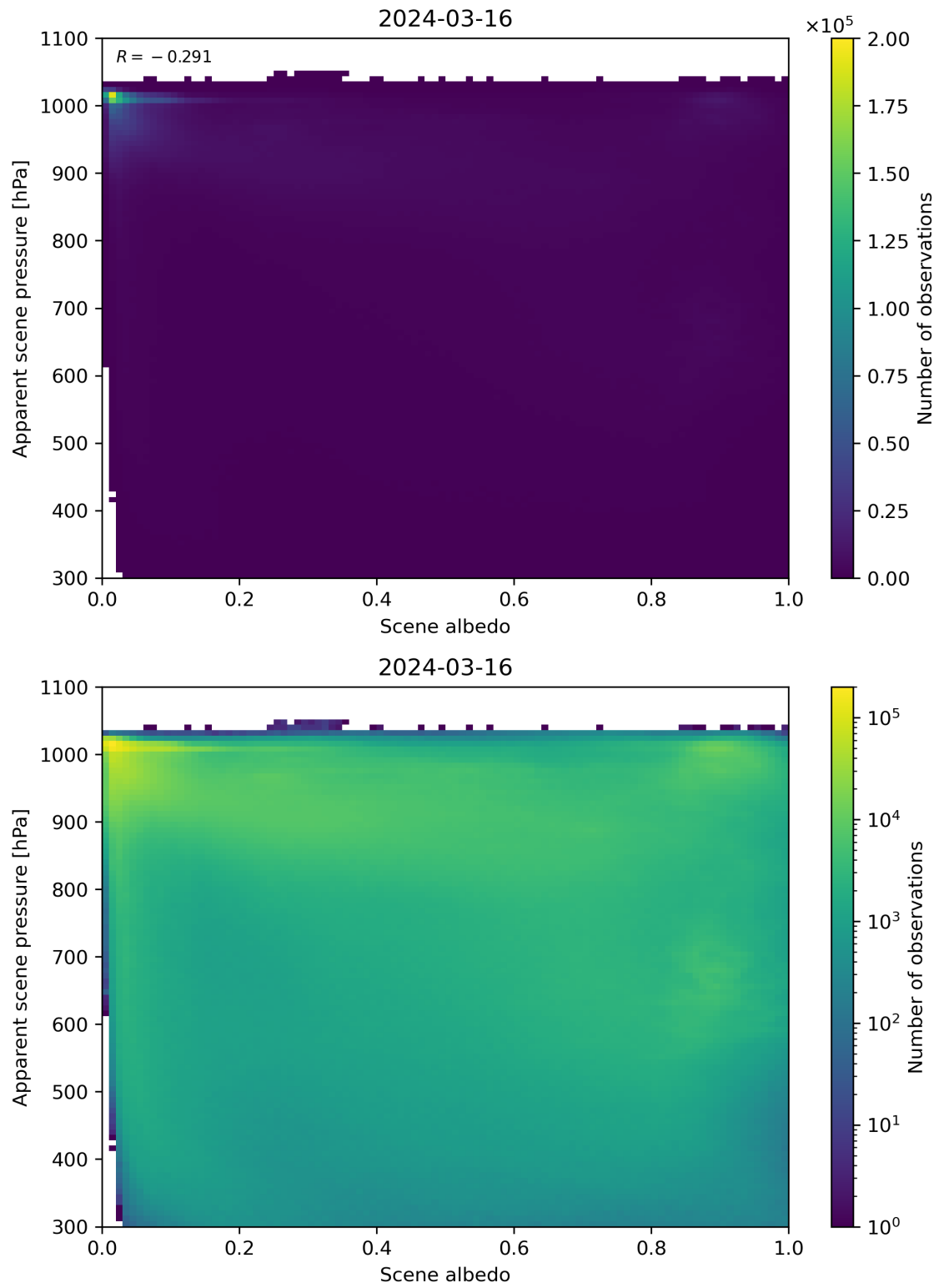
Figure 102: Scatter density plot of “Scene albedo” against “Apparent scene pressure” for 2024-03-15 to 2024-03-17.
