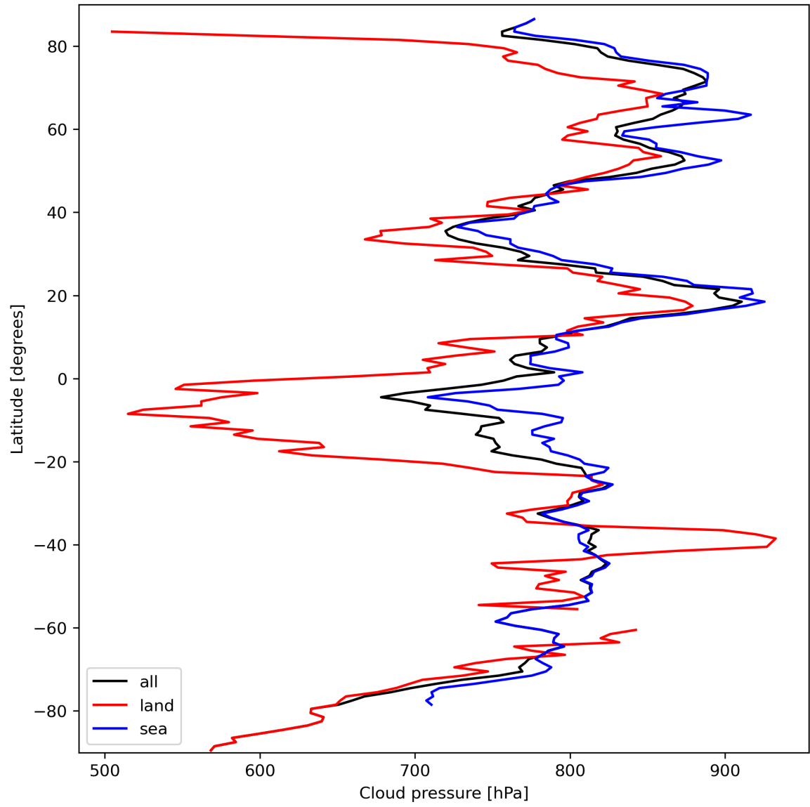
Figure 13: Zonal average of “Cloud pressure” for 2024-03-15 to 2024-03-17.
