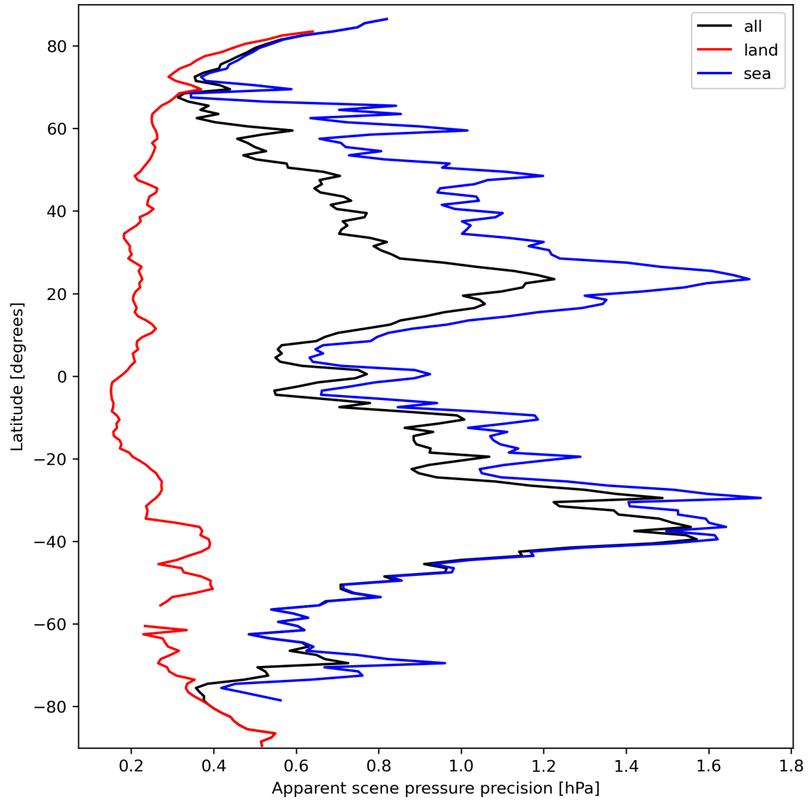
Figure 20: Zonal average of “Apparent scene pressure precision” for 2024-03-15 to 2024-03-17.
