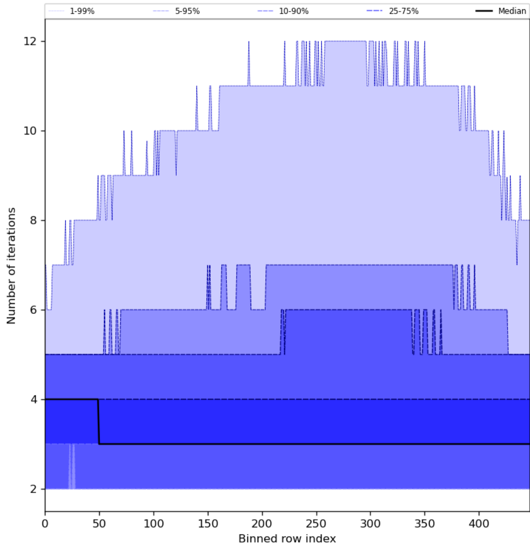
Figure 56: Along track statistics of “Number of iterations” for 2024-03-15 to 2024-03-17
