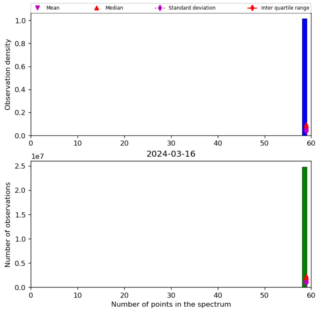
Figure 44: Histogram of “Number of points in the spectrum” for 2024-03-15 to 2024-03-17
