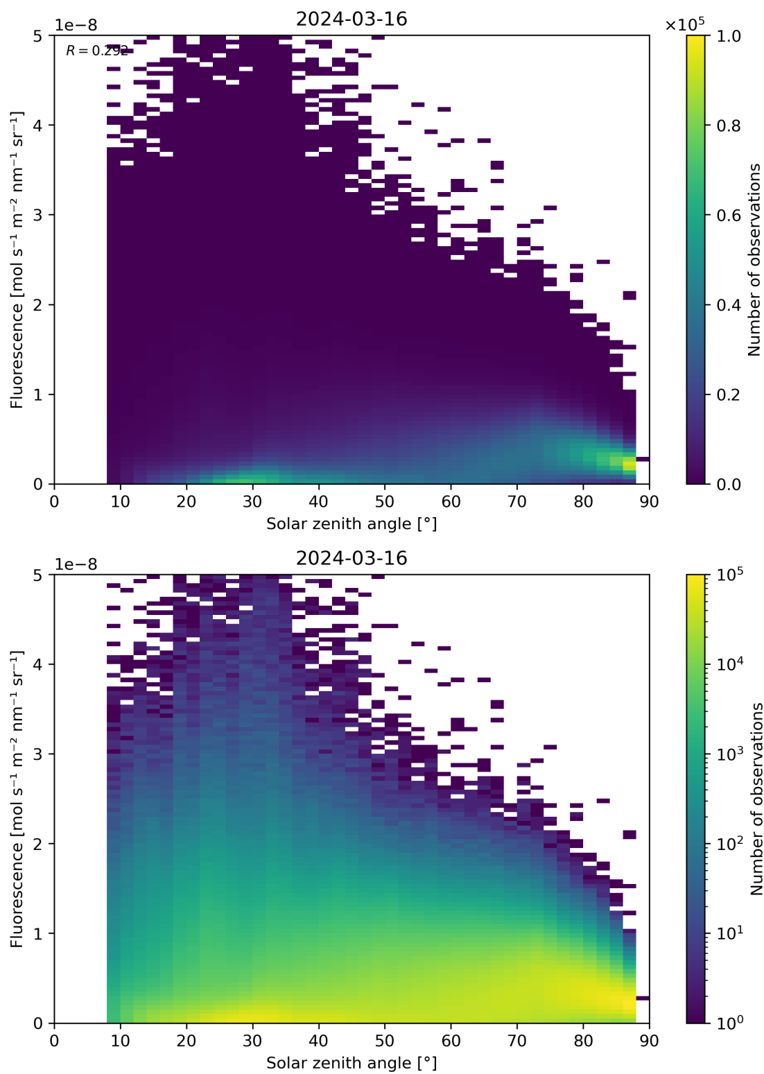
Figure 112: Scatter density plot of “Solar zenith angle” against “Fluorescence” for 2024-03-15 to 2024-03-17.
