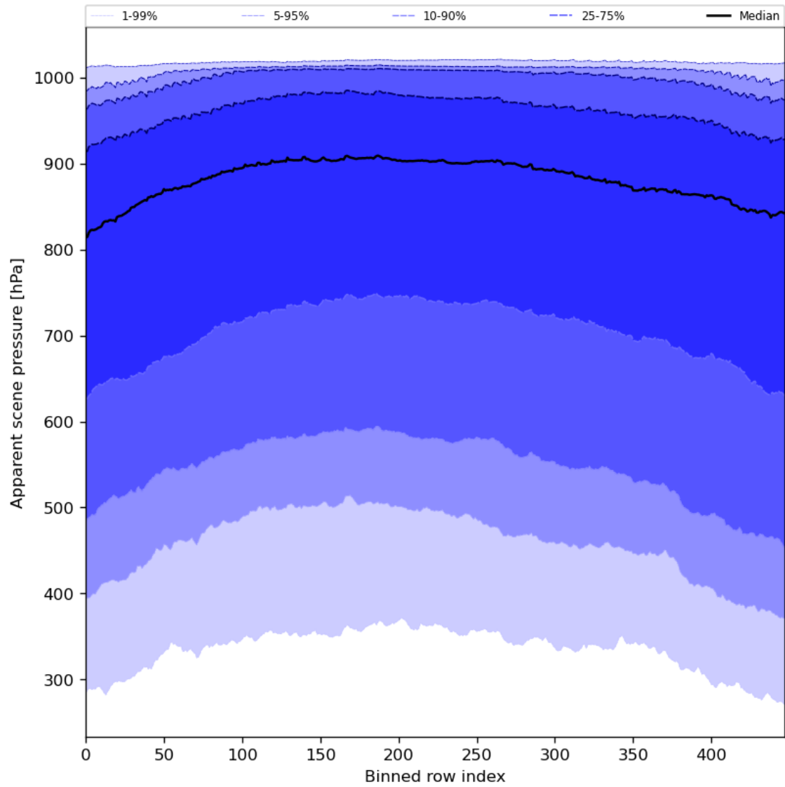
Figure 53: Along track statistics of “Apparent scene pressure” for 2024-03-15 to 2024-03-17
