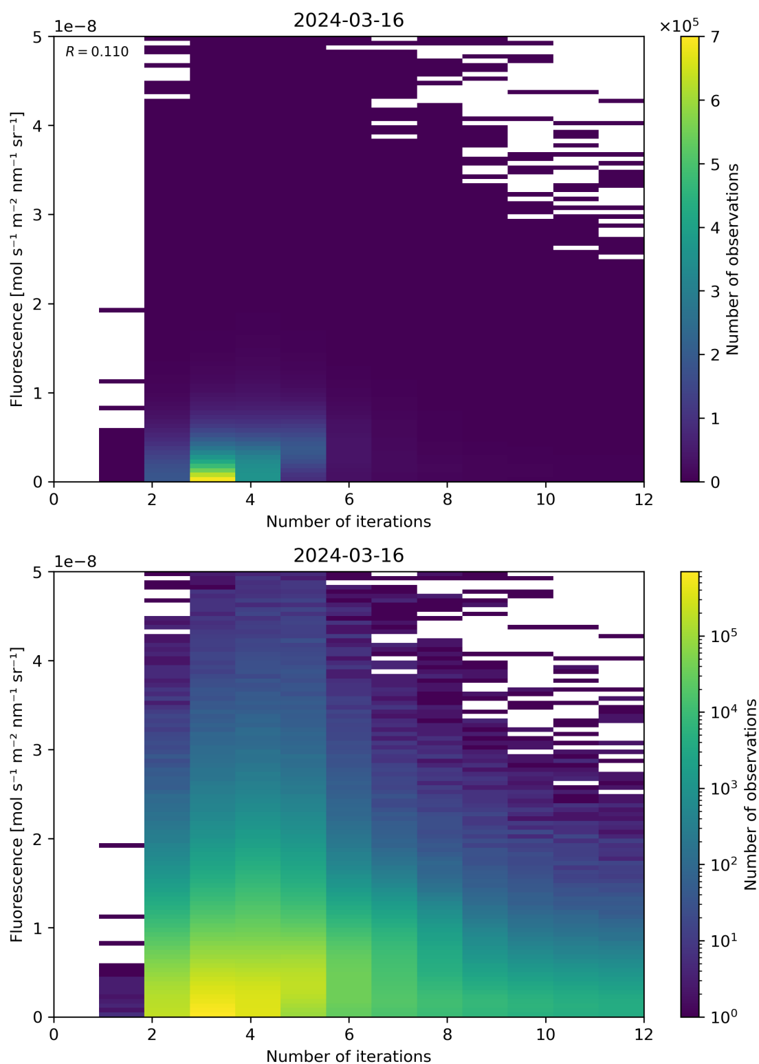
Figure 98: Scatter density plot of “Number of iterations” against “Fluorescence” for 2024-03-15 to 2024-03-17.
