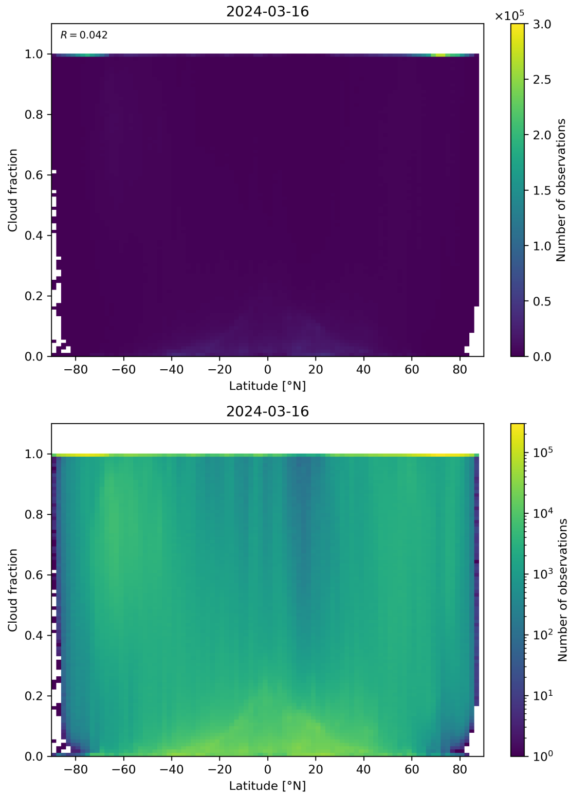
Figure 90: Scatter density plot of “Latitude” against “Cloud fraction” for 2024-03-15 to 2024-03-17.
