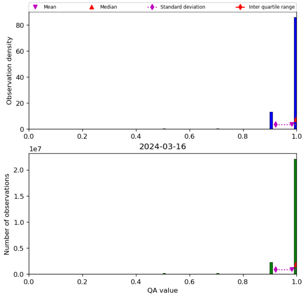
Figure 29: Histogram of “QA value” for 2024-03-15 to 2024-03-17
