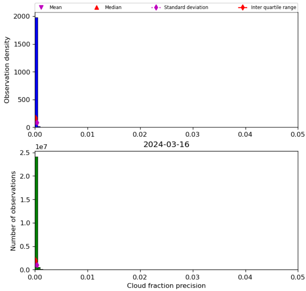
Figure 33: Histogram of “Cloud fraction precision” for 2024-03-15 to 2024-03-17
