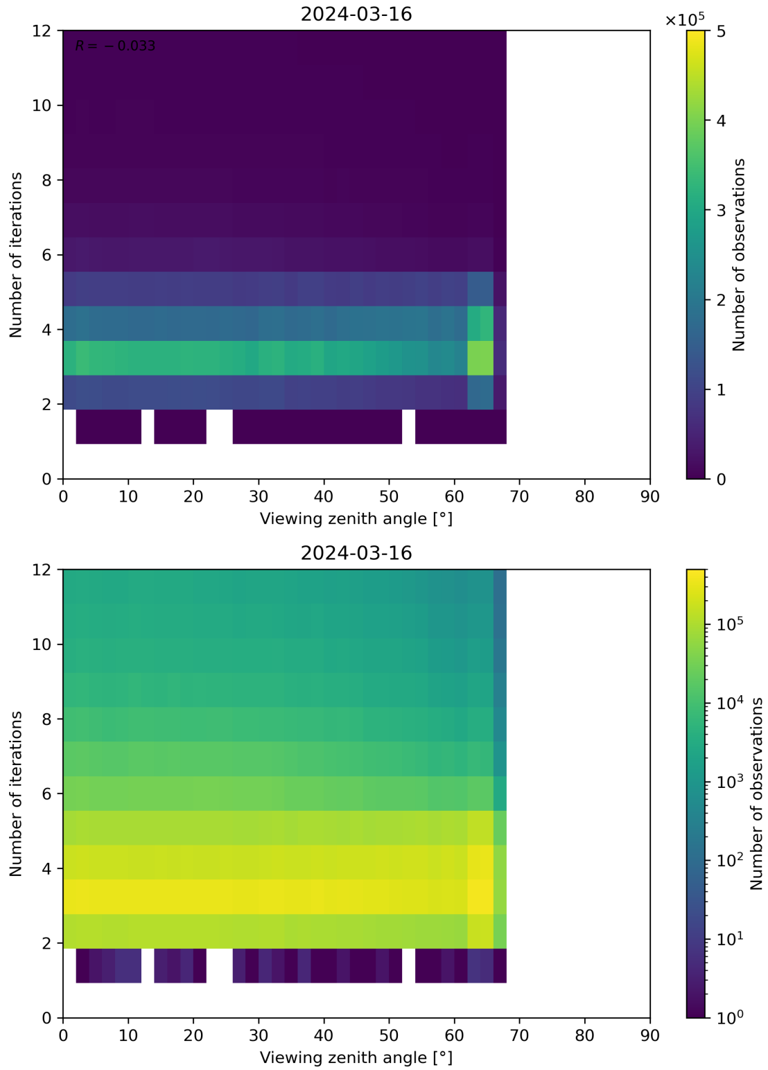
Figure 124: Scatter density plot of “Viewing zenith angle” against “Number of iterations” for 2024-03-15 to 2024-03-17.
