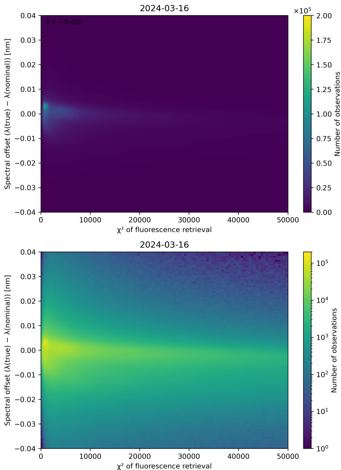
Figure 69: Scatter density plot of " \chi^2 of fluorescence retrieval" against "Spectral offset ( \lambda(\text{true}) - \lambda(\text{nominal}) )" for 2024-03-15 to 2024-03-17.
