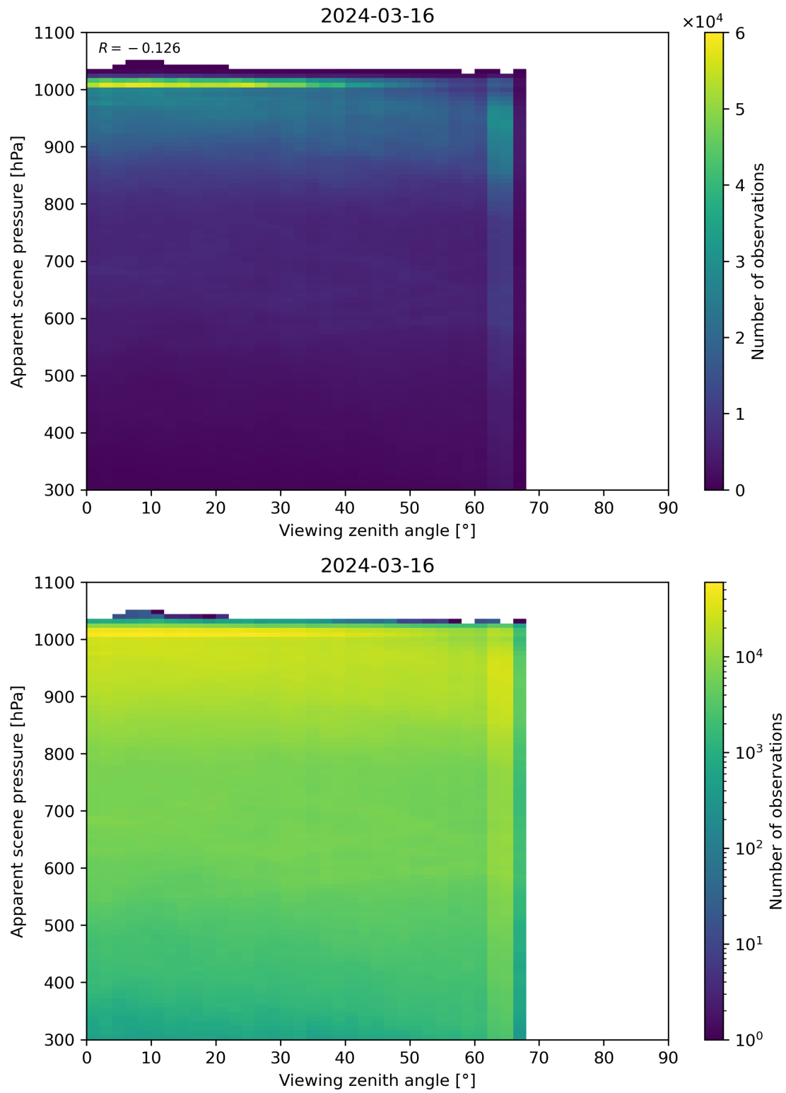
Figure 118: Scatter density plot of “Viewing zenith angle” against “Apparent scene pressure” for 2024-03-15 to 2024-03-17.
