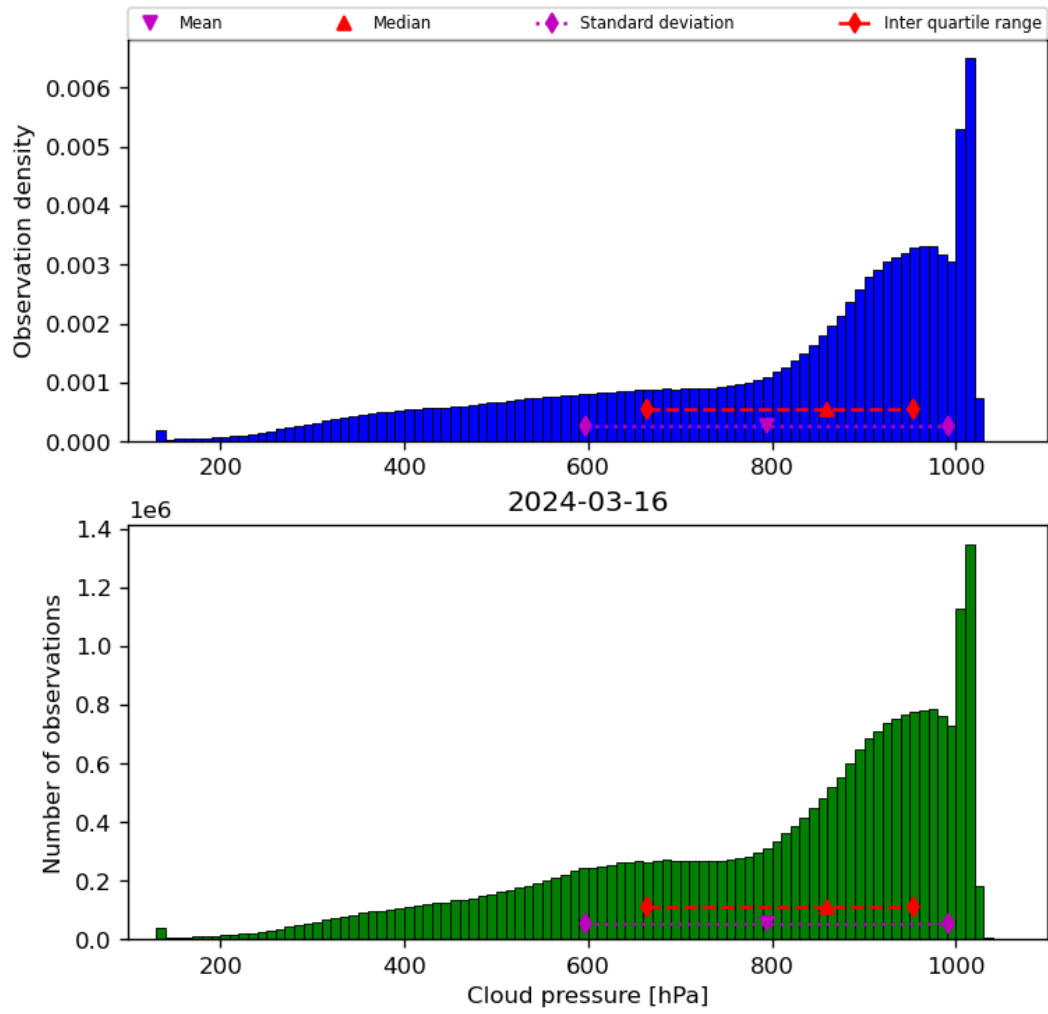
Figure 30: Histogram of “Cloud pressure” for 2024-03-15 to 2024-03-17
