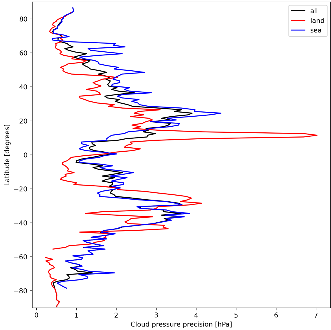
Figure 14: Zonal average of “Cloud pressure precision” for 2024-03-15 to 2024-03-17.
