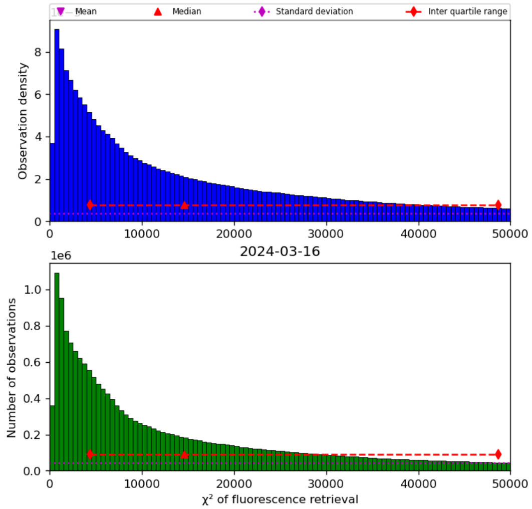
Figure 42: Histogram of “ \chi^2 of fluorescence retrieval” for 2024-03-15 to 2024-03-17
