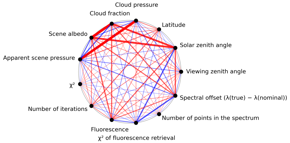
Figure 1: Map of correlation graph for 2024-03-15 to 2024-03-17.
