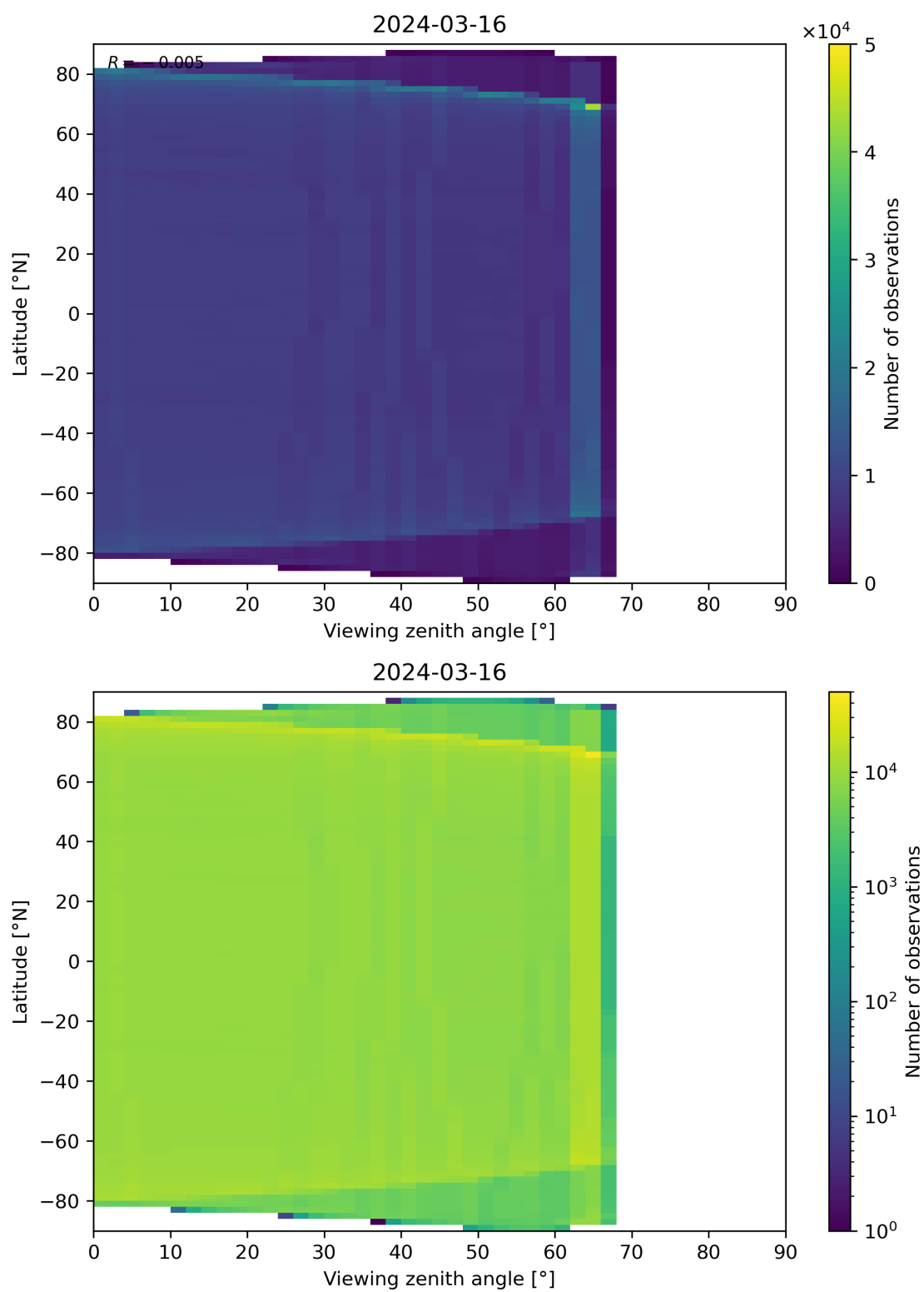
Figure 123: Scatter density plot of “Viewing zenith angle” against “Latitude” for 2024-03-15 to 2024-03-17.
