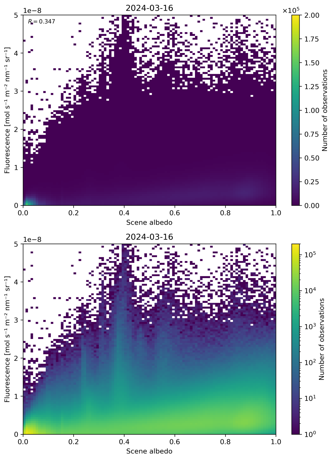
Figure 104: Scatter density plot of “Scene albedo” against “Fluorescence” for 2024-03-15 to 2024-03-17.
