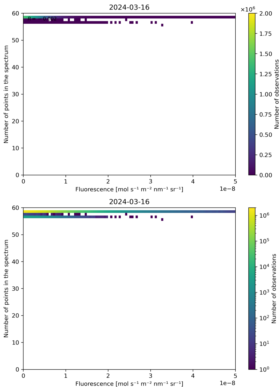
Figure 86: Scatter density plot of “Fluorescence” against “Number of points in the spectrum” for 2024-03-15 to 2024-03-17.
