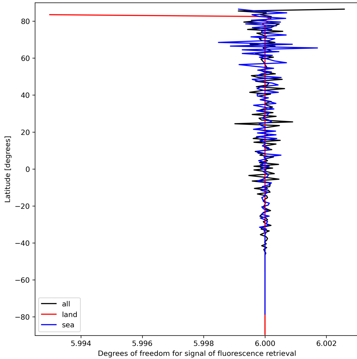
Figure 26: Zonal average of “Degrees of freedom for signal of fluorescence retrieval” for 2024-03-15 to 2024-03-17.
