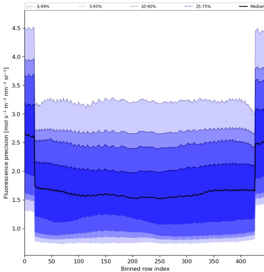
Figure 58: Along track statistics of “Fluorescence precision” for 2024-03-15 to 2024-03-17
