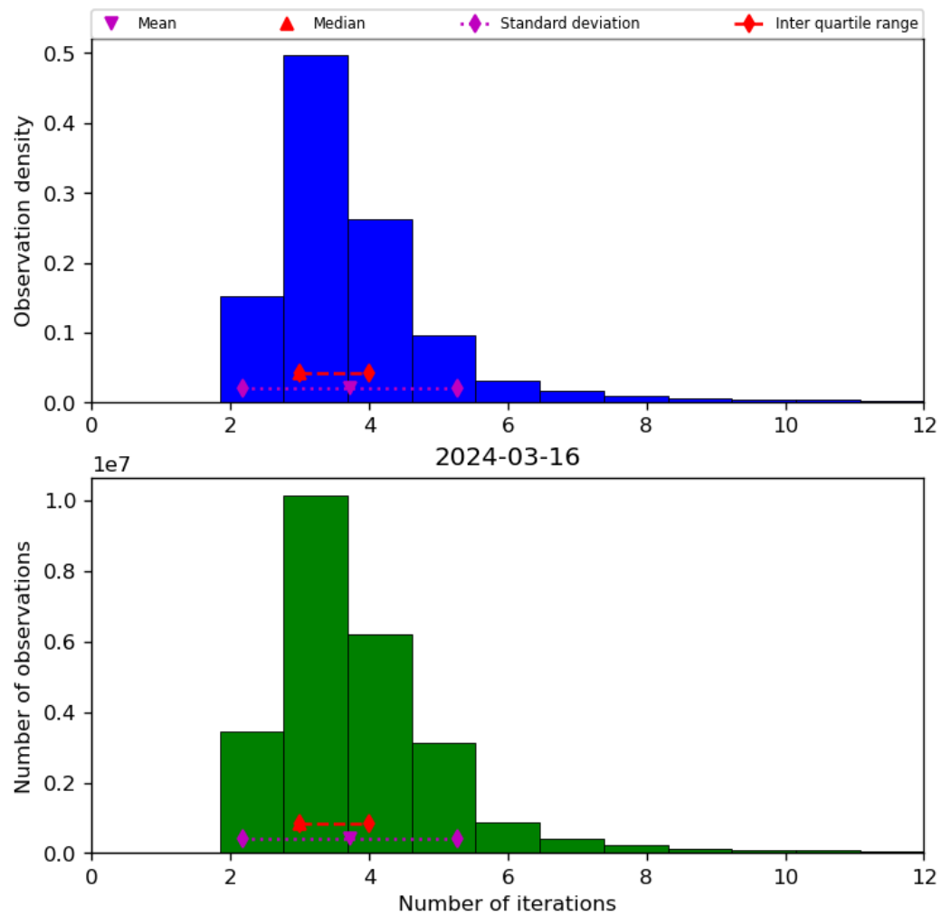
Figure 39: Histogram of “Number of iterations” for 2024-03-15 to 2024-03-17
