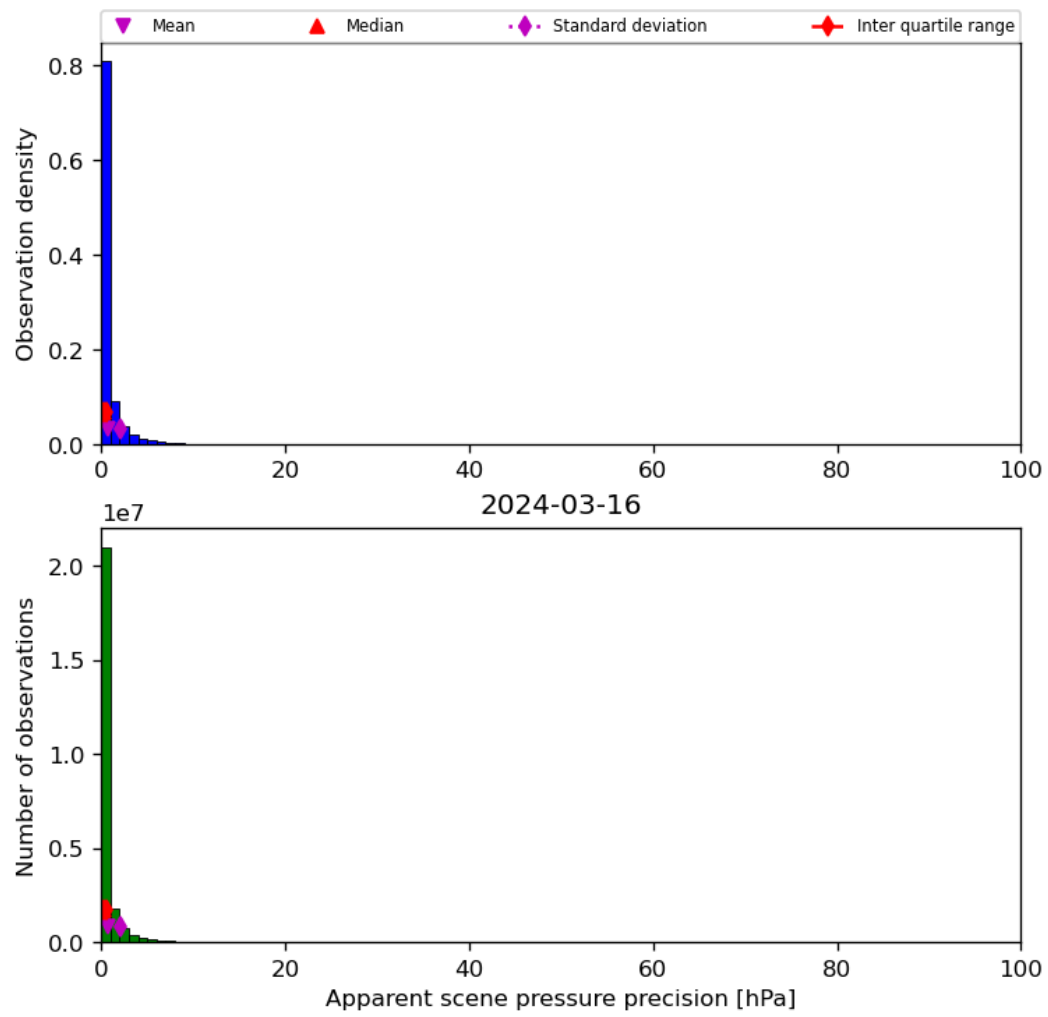
Figure 37: Histogram of “Apparent scene pressure precision” for 2024-03-15 to 2024-03-17
