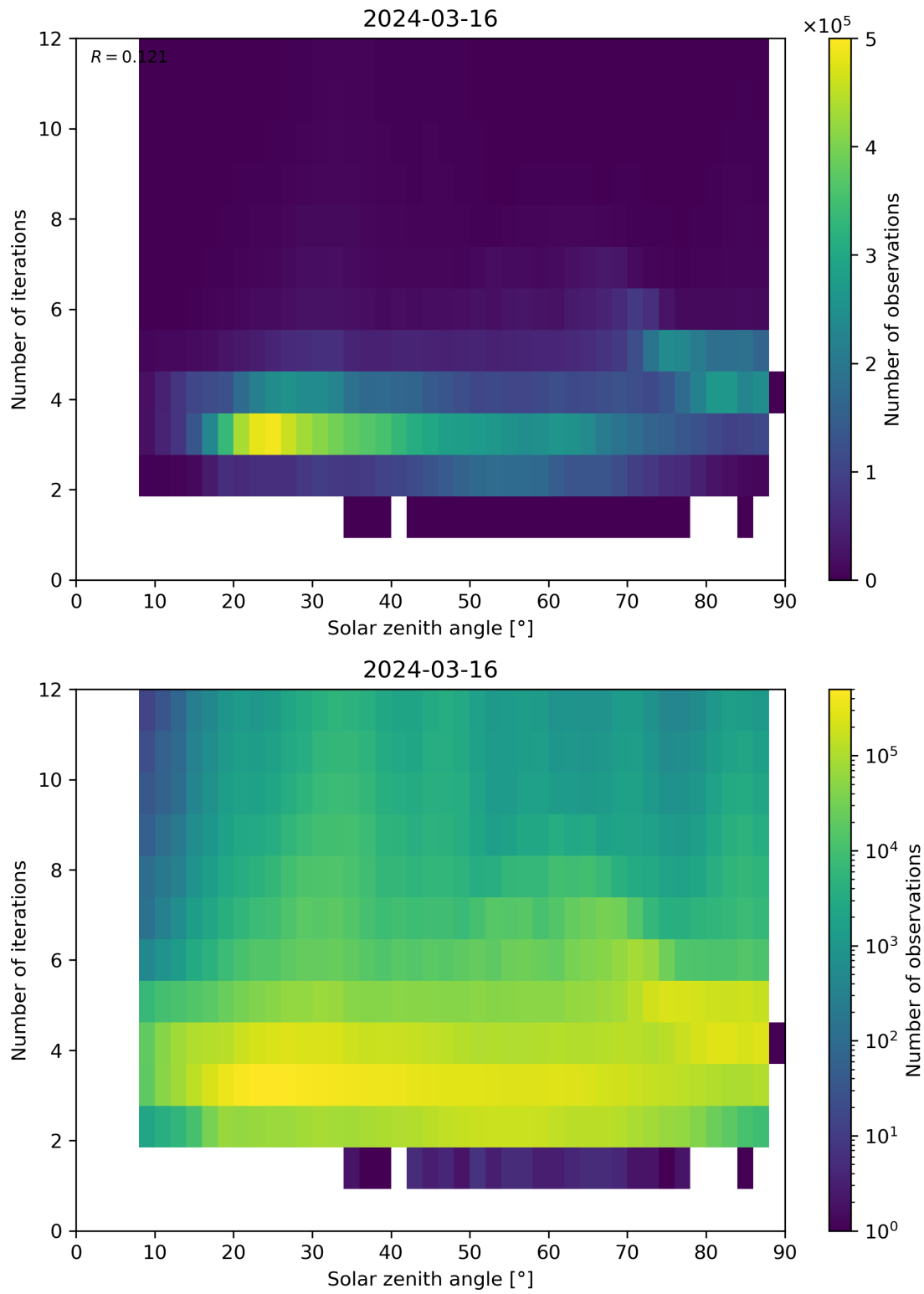
Figure 114: Scatter density plot of “Solar zenith angle” against “Number of iterations” for 2024-03-15 to 2024-03-17.
