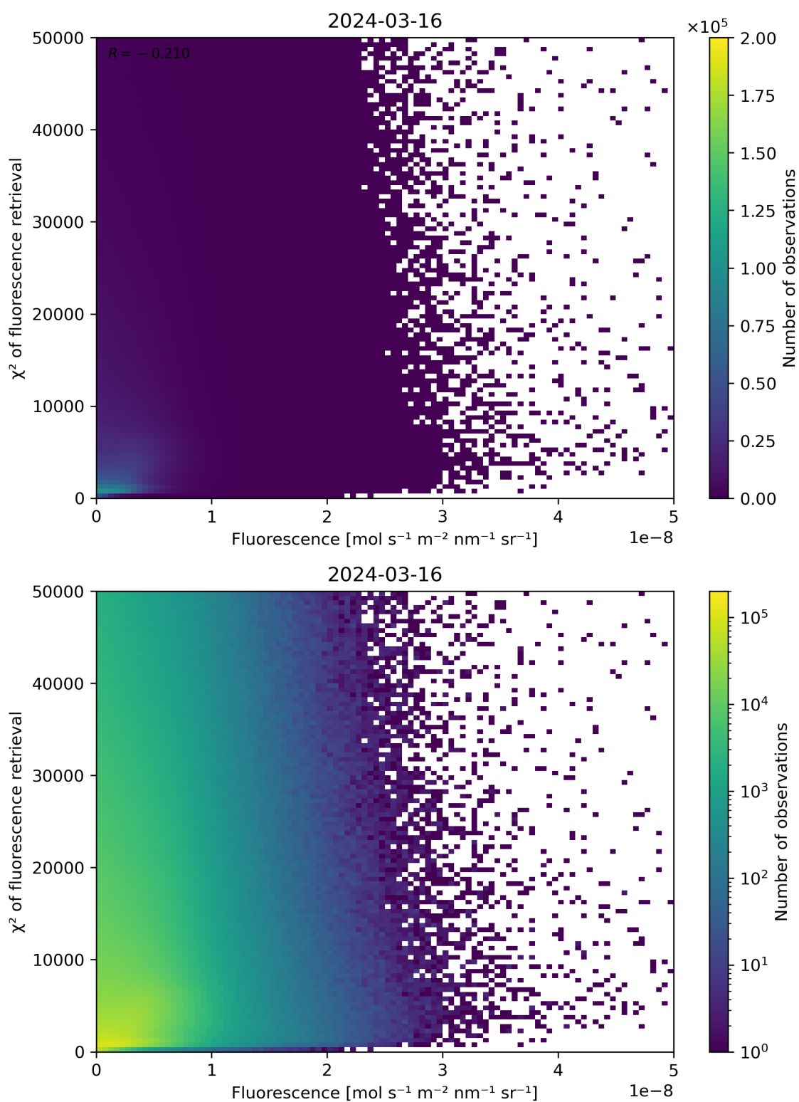
Figure 85: Scatter density plot of “Fluorescence” against “ \chi^2 of fluorescence retrieval” for 2024-03-15 to 2024-03-17.
