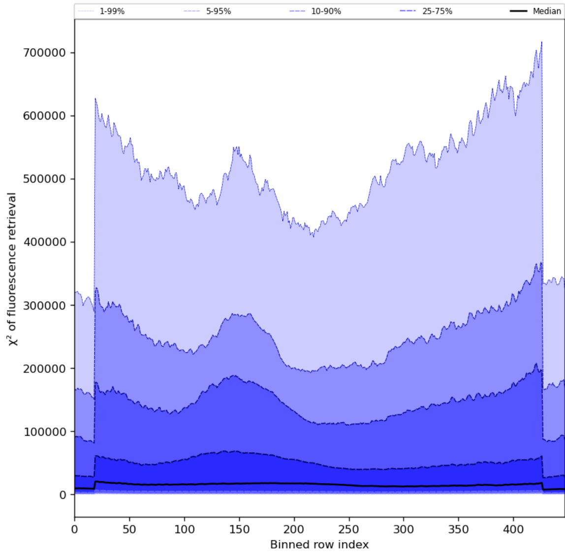
Figure 59: Along track statistics of “ \chi^2 of fluorescence retrieval” for 2024-03-15 to 2024-03-17
