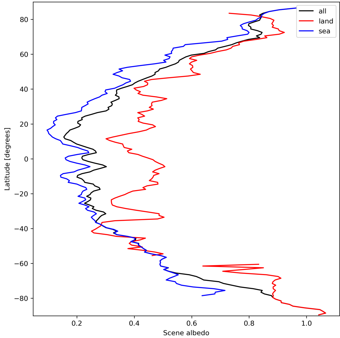
Figure 17: Zonal average of “Scene albedo” for 2024-03-15 to 2024-03-17.
