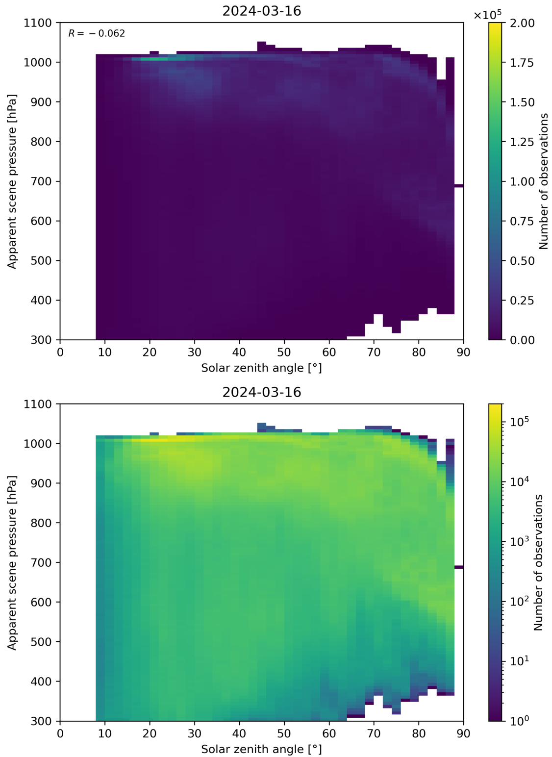
Figure 108: Scatter density plot of “Solar zenith angle” against “Apparent scene pressure” for 2024-03-15 to 2024-03-17.
