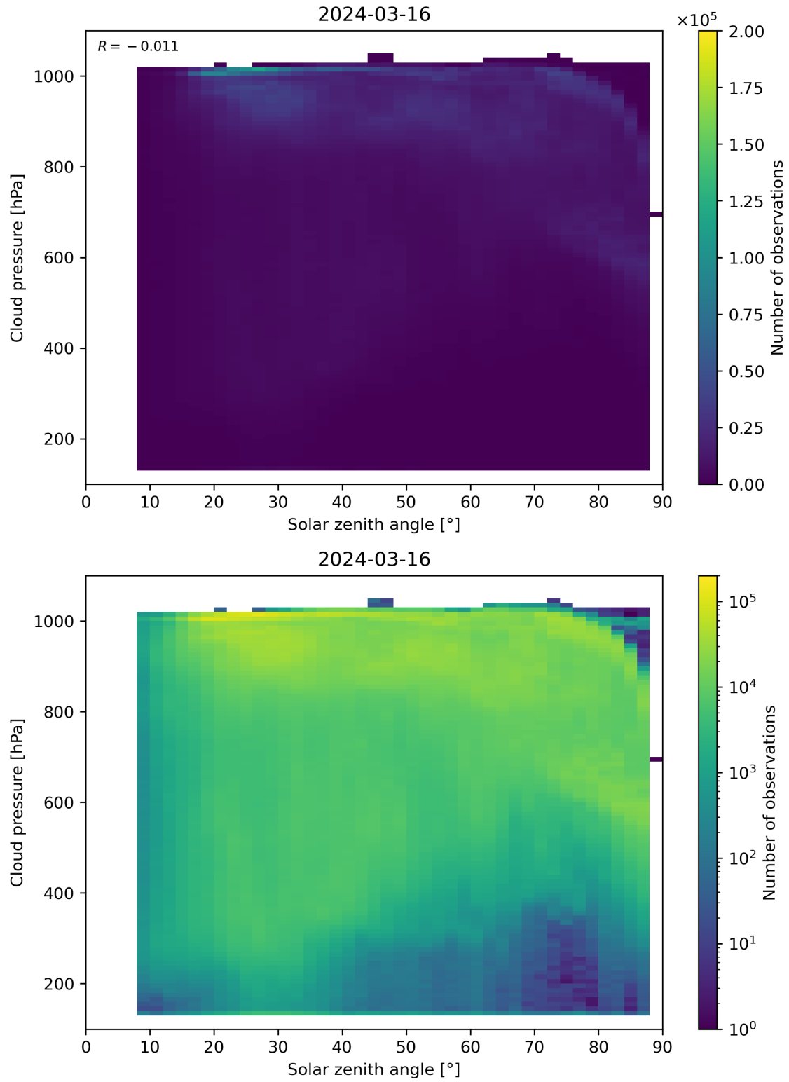
Figure 111: Scatter density plot of “Solar zenith angle” against “Cloud pressure” for 2024-03-15 to 2024-03-17.
