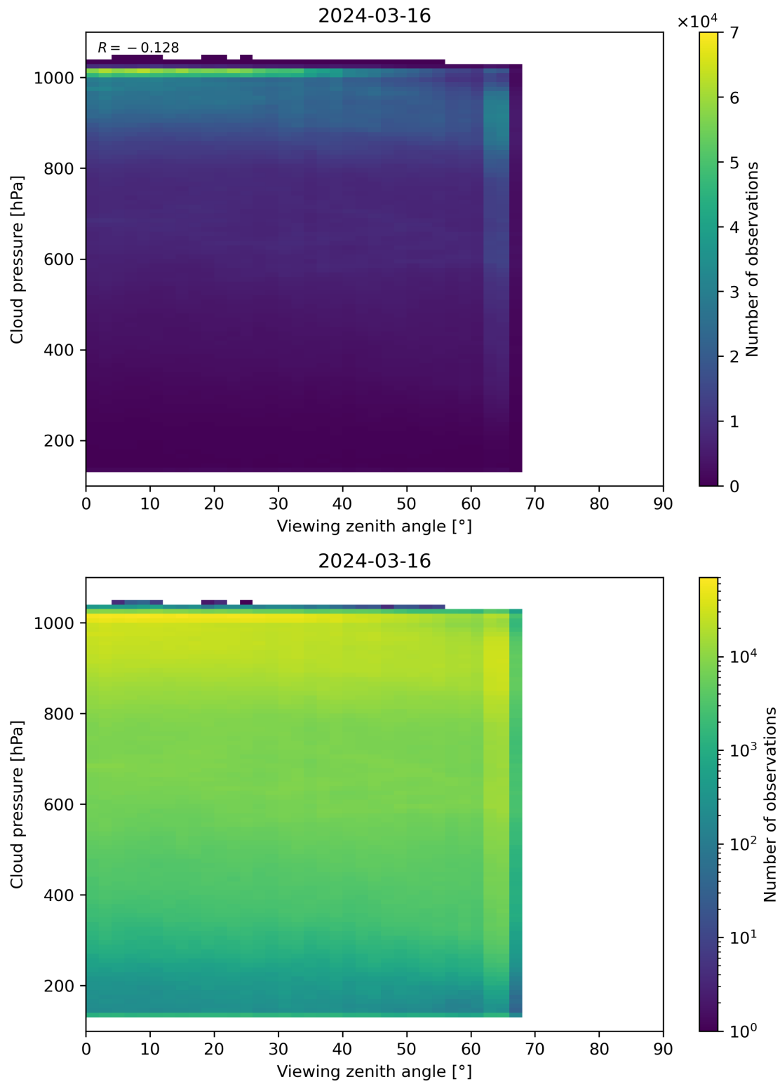
Figure 121: Scatter density plot of “Viewing zenith angle” against “Cloud pressure” for 2024-03-15 to 2024-03-17.
