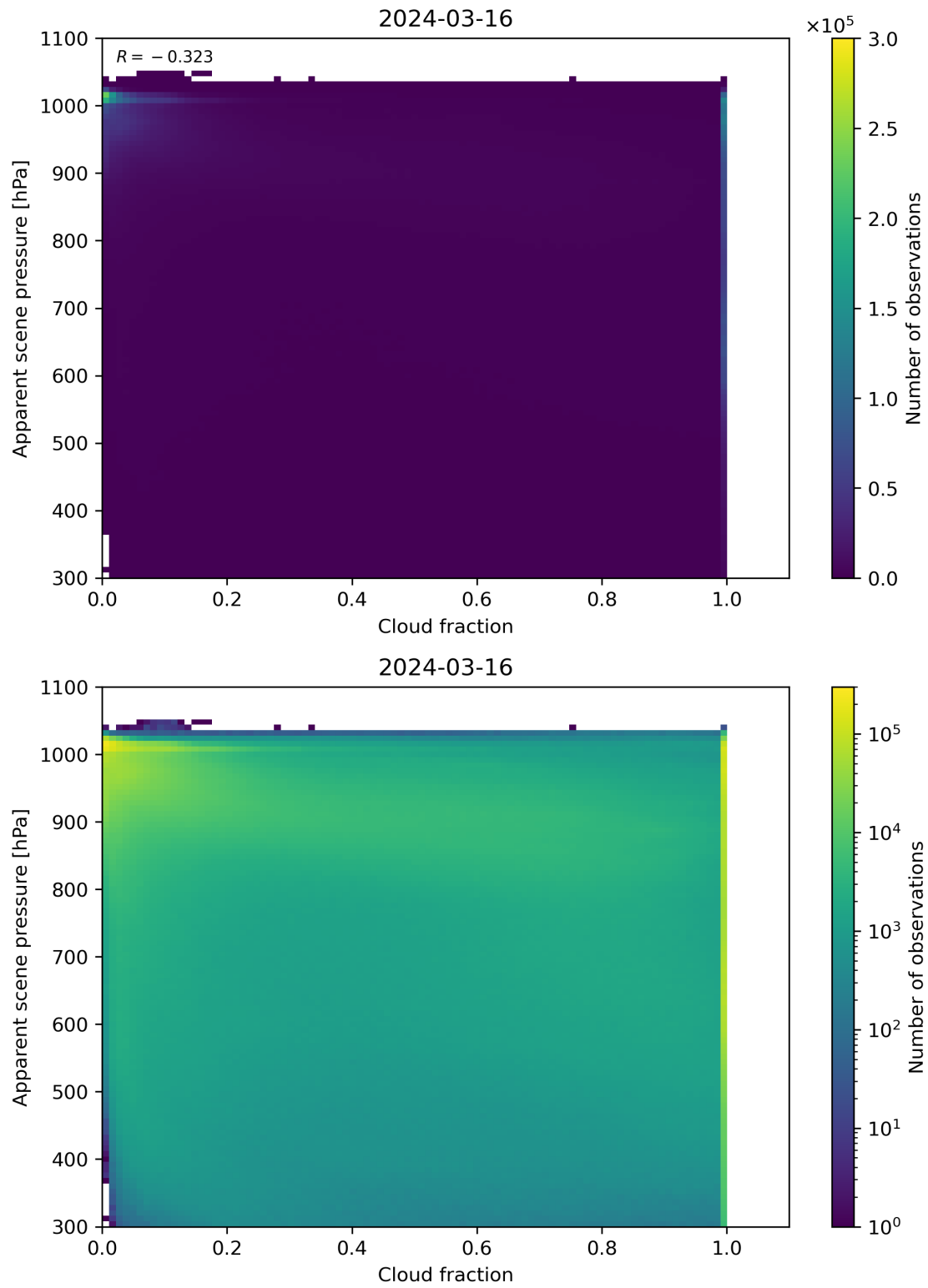
Figure 70: Scatter density plot of “Cloud fraction” against “Apparent scene pressure” for 2024-03-15 to 2024-03-17.
