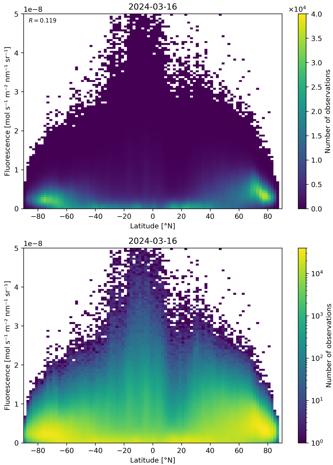
Figure 92: Scatter density plot of “Latitude” against “Fluorescence” for 2024-03-15 to 2024-03-17.
