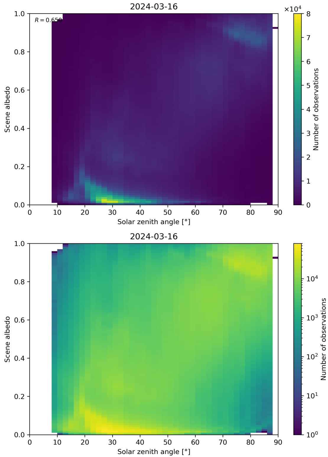
Figure 116: Scatter density plot of “Solar zenith angle” against “Scene albedo” for 2024-03-15 to 2024-03-17.
