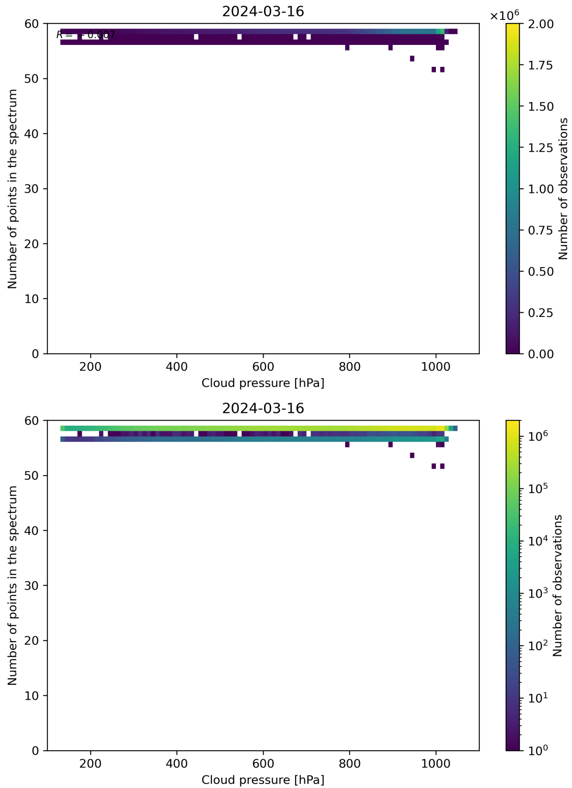
Figure 82: Scatter density plot of “Cloud pressure” against “Number of points in the spectrum” for 2024-03-15 to 2024-03-17.
