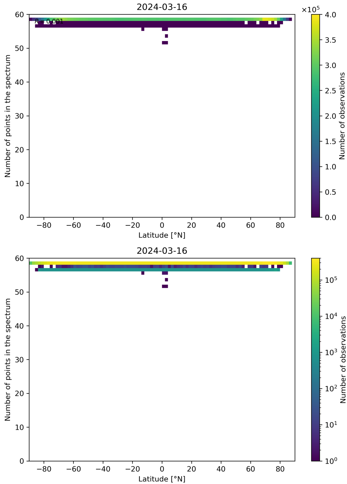
Figure 94: Scatter density plot of “Latitude” against “Number of points in the spectrum” for 2024-03-15 to 2024-03-17.
