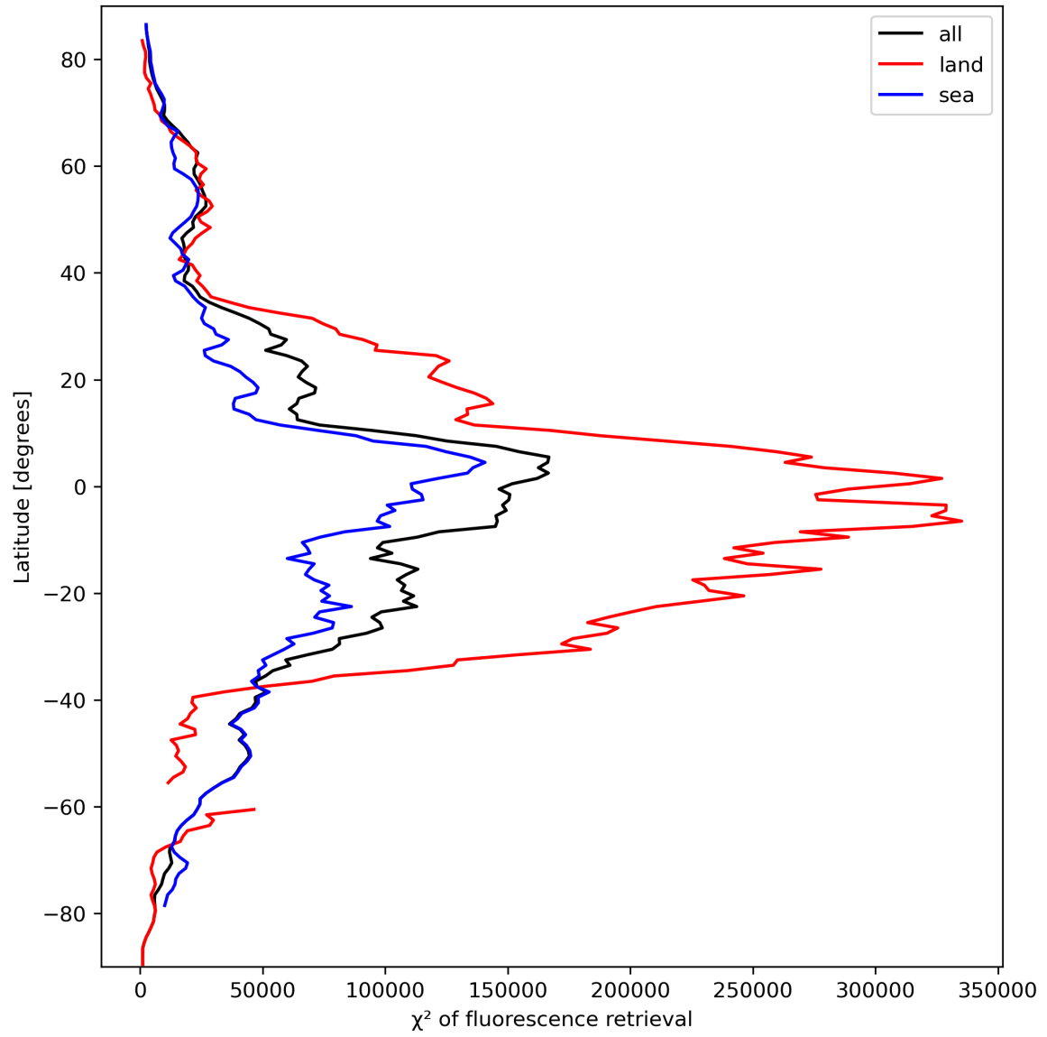
Figure 25: Zonal average of “ \chi^2 of fluorescence retrieval” for 2024-03-15 to 2024-03-17.
