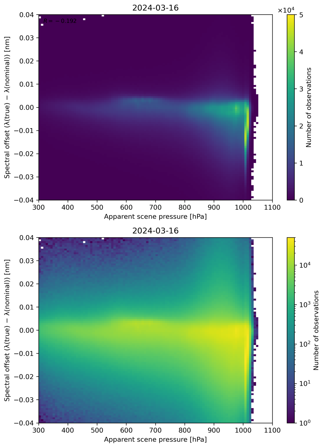
Figure 67: Scatter density plot of “Apparent scene pressure” against “Spectral offset ( \lambda(\text{true}) - \lambda(\text{nominal}) )” for 2024-03-15 to 2024-03-17.
