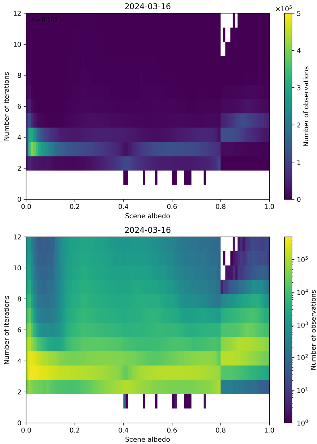
Figure 105: Scatter density plot of “Scene albedo” against “Number of iterations” for 2024-03-15 to 2024-03-17.
