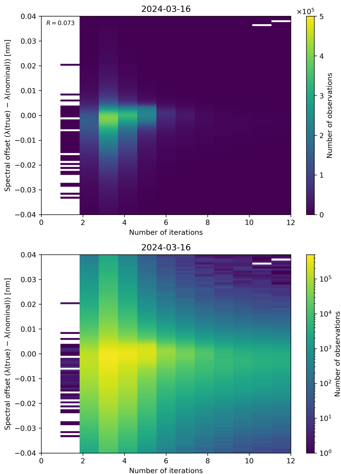
Figure 100: Scatter density plot of “Number of iterations” against “Spectral offset ( \lambda(\text{true}) - \lambda(\text{nominal}) )” for 2024-03-15 to 2024-03-17.
