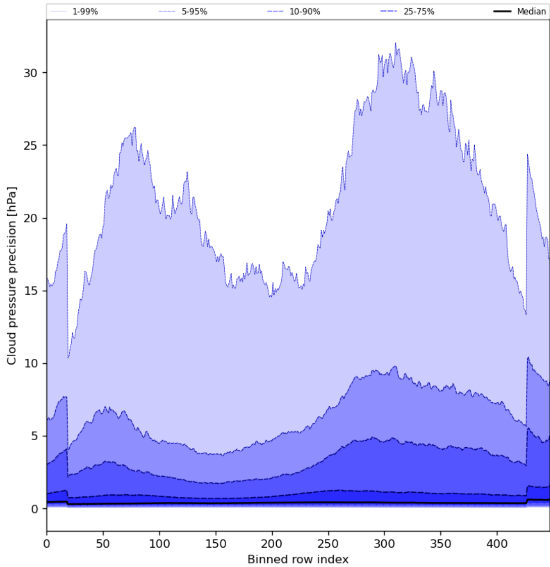
Figure 48: Along track statistics of “Cloud pressure precision” for 2024-03-15 to 2024-03-17
