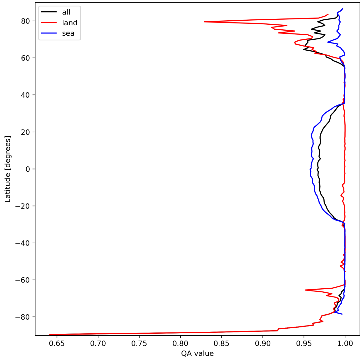
Figure 12: Zonal average of “QA value” for 2024-03-15 to 2024-03-17.
