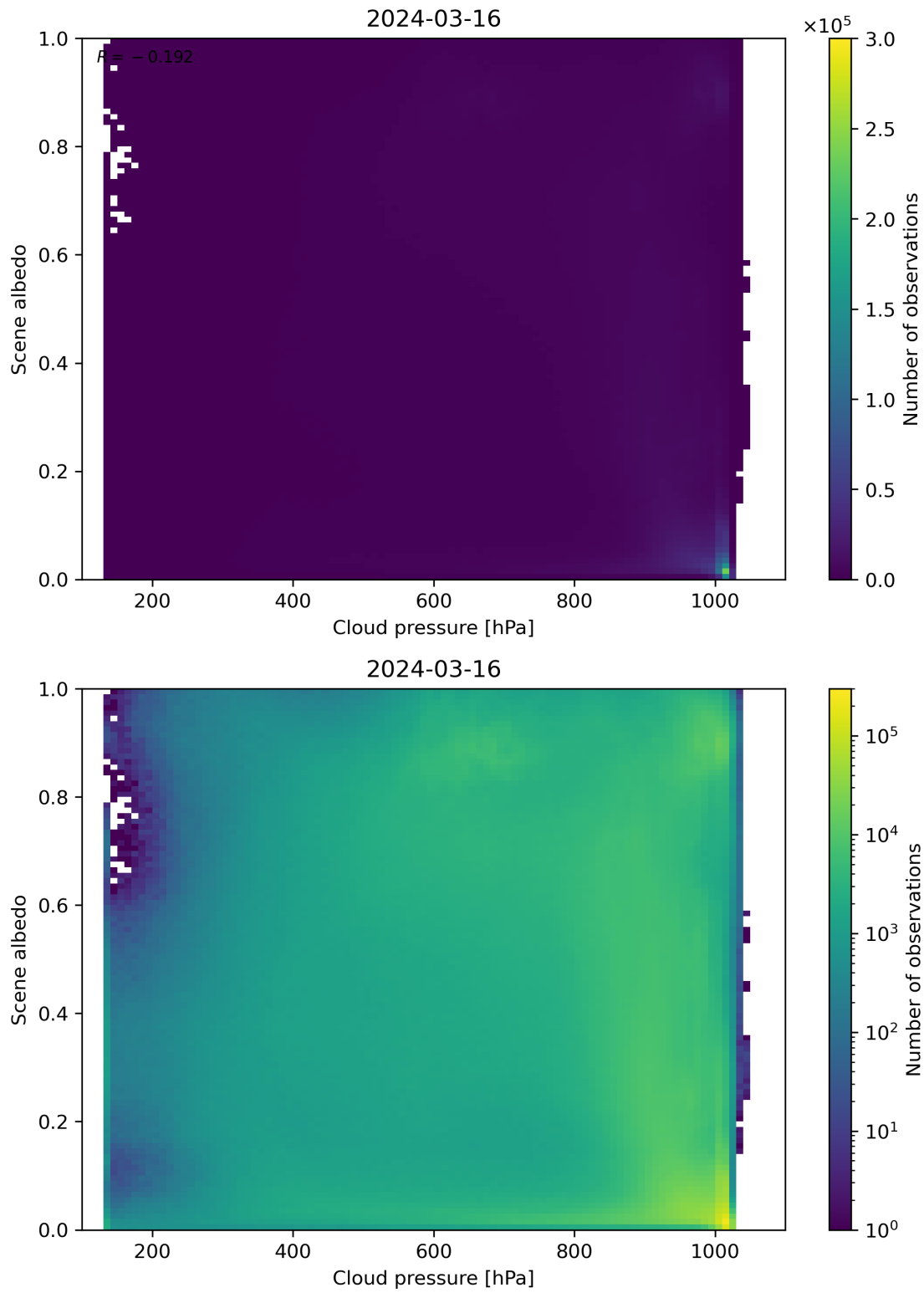
Figure 83: Scatter density plot of “Cloud pressure” against “Scene albedo” for 2024-03-15 to 2024-03-17.
