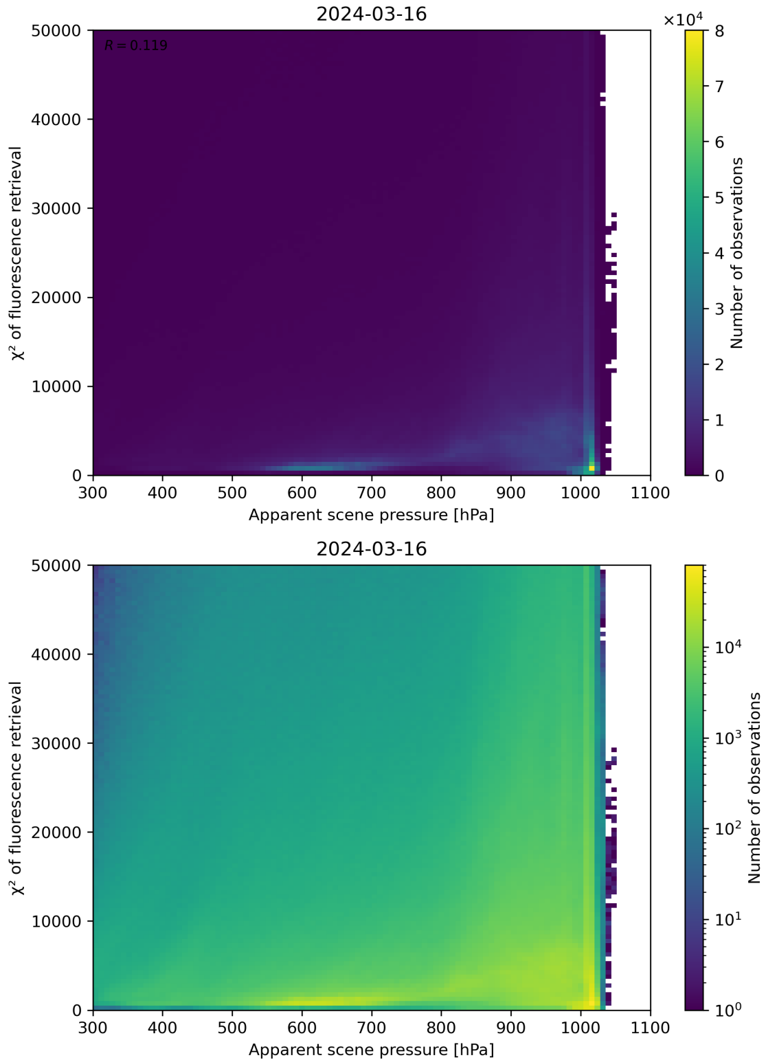
Figure 63: Scatter density plot of “Apparent scene pressure” against “ \chi^2 of fluorescence retrieval” for 2024-03-15 to 2024-03-17.
