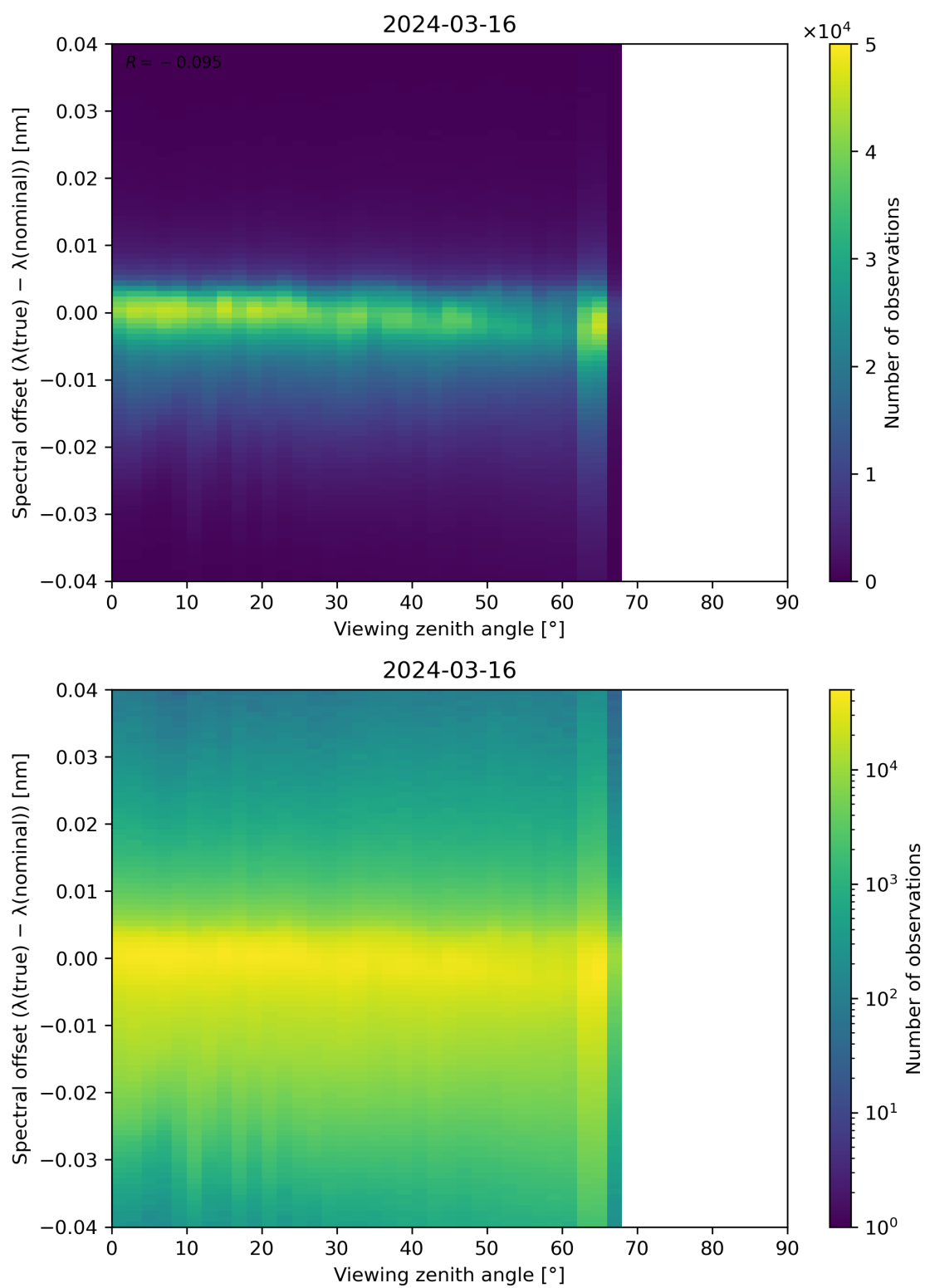
Figure 128: Scatter density plot of “Viewing zenith angle” against “Spectral offset ( \lambda(\text{true}) - \lambda(\text{nominal}) )” for 2024-03-15 to 2024-03-17.
