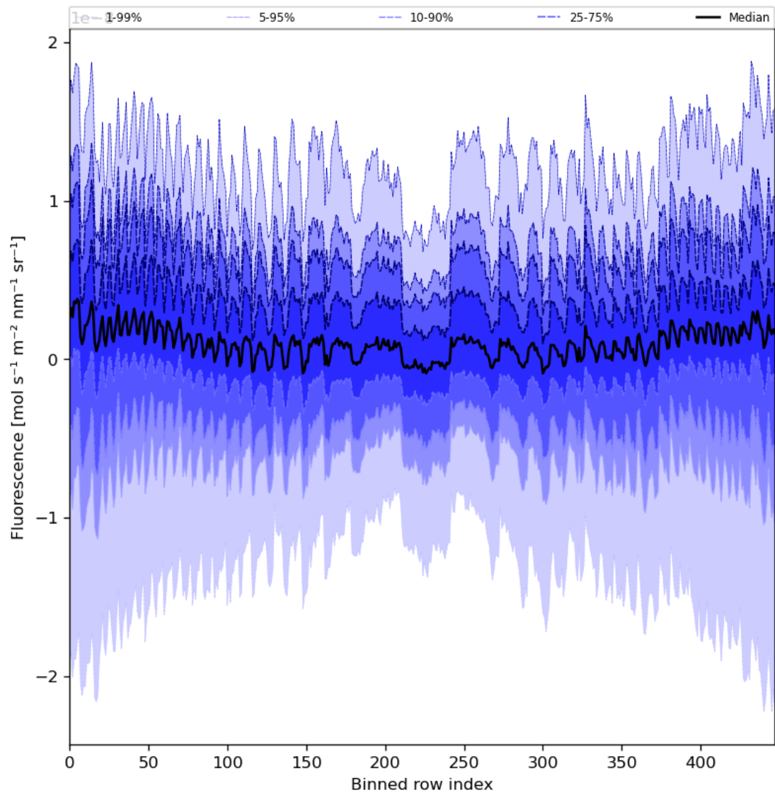
Figure 57: Along track statistics of “Fluorescence” for 2024-03-15 to 2024-03-17
