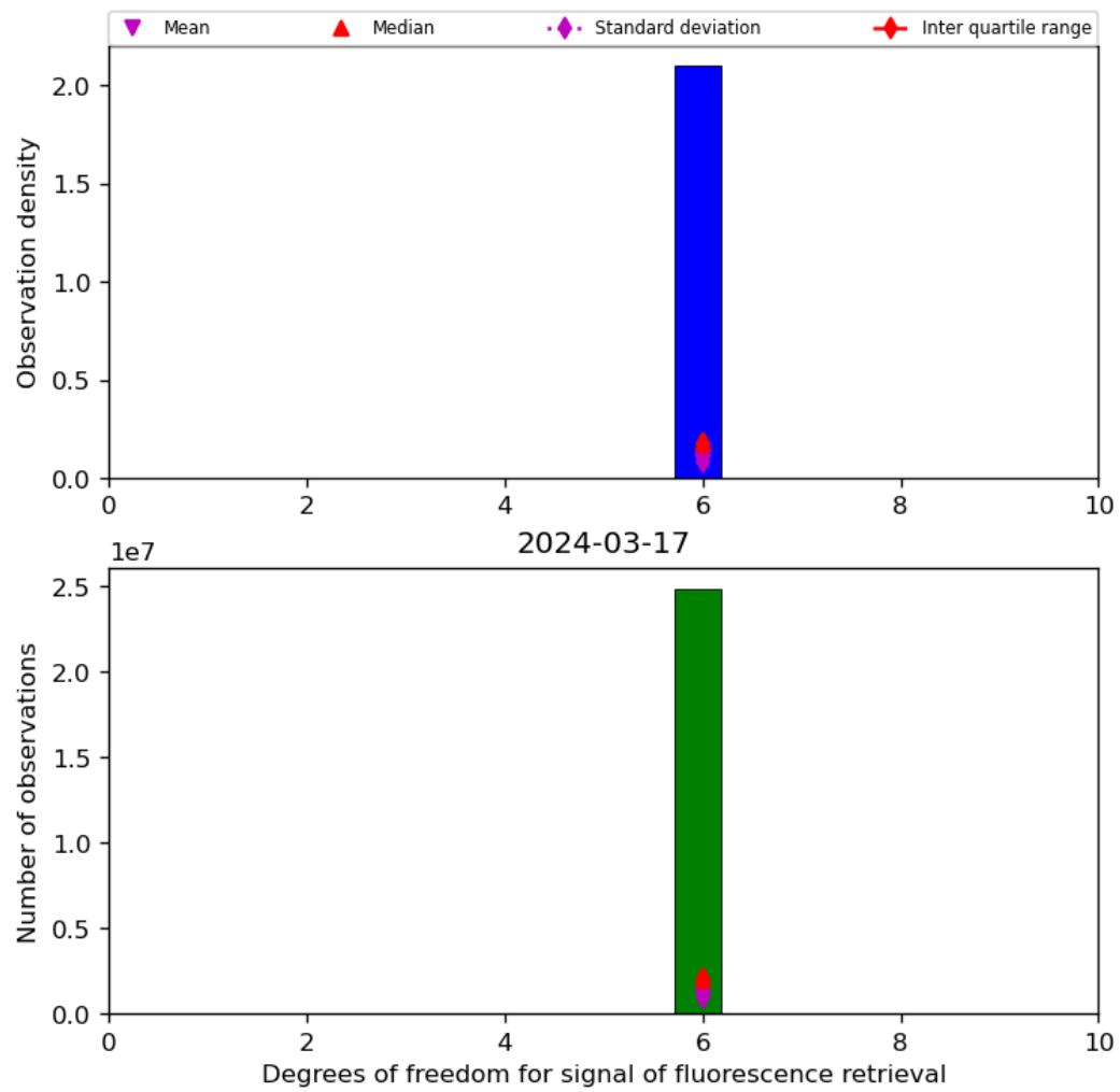
Figure 43: Histogram of “Degrees of freedom for signal of fluorescence retrieval” for 2024-03-16 to 2024-03-18
