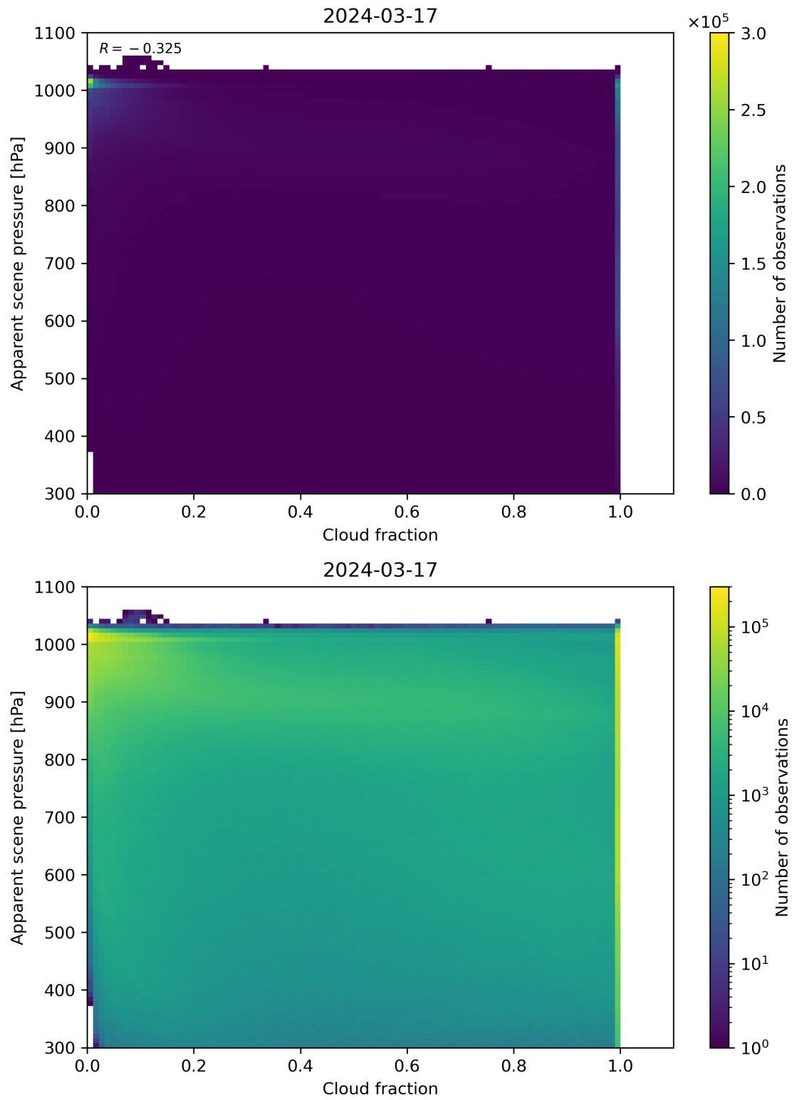
Figure 70: Scatter density plot of “Cloud fraction” against “Apparent scene pressure” for 2024-03-16 to 2024-03-18.
