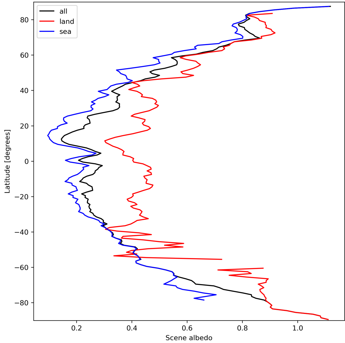
Figure 17: Zonal average of “Scene albedo” for 2024-03-16 to 2024-03-18.
