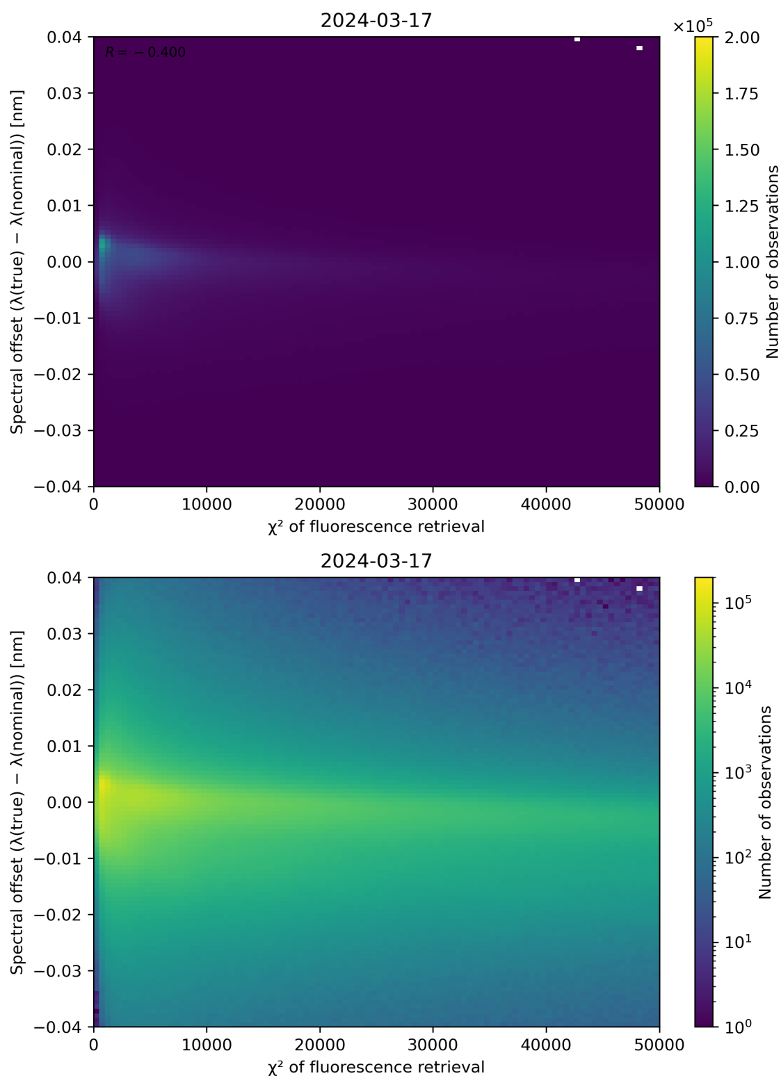
Figure 69: Scatter density plot of “ \chi^2 of fluorescence retrieval” against “Spectral offset ( \lambda(\text{true}) - \lambda(\text{nominal}) )” for 2024-03-16 to 2024-03-18.
