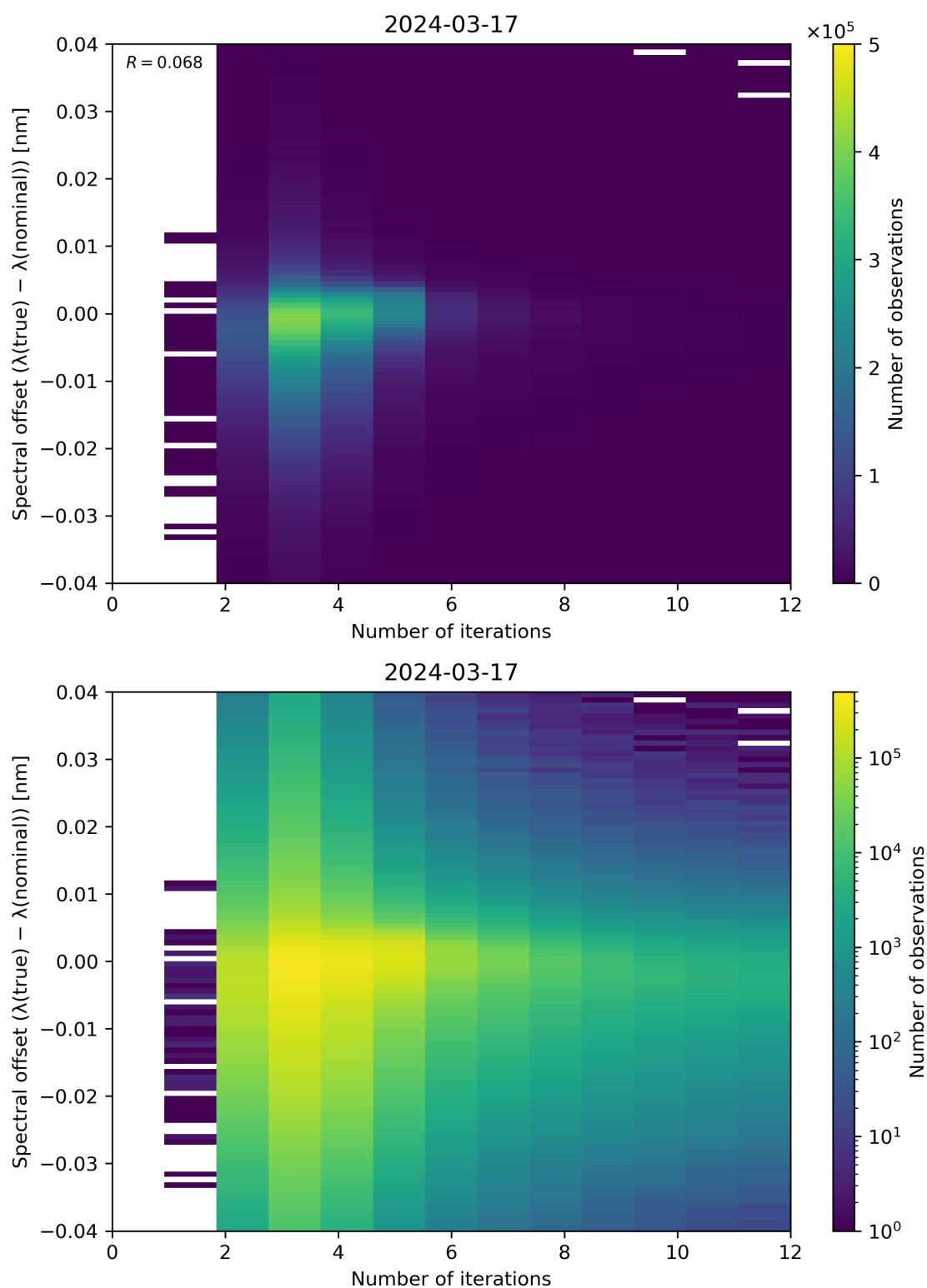
Figure 100: Scatter density plot of “Number of iterations” against “Spectral offset ( \lambda(\text{true}) - \lambda(\text{nominal}) )” for 2024-03-16 to 2024-03-18.
