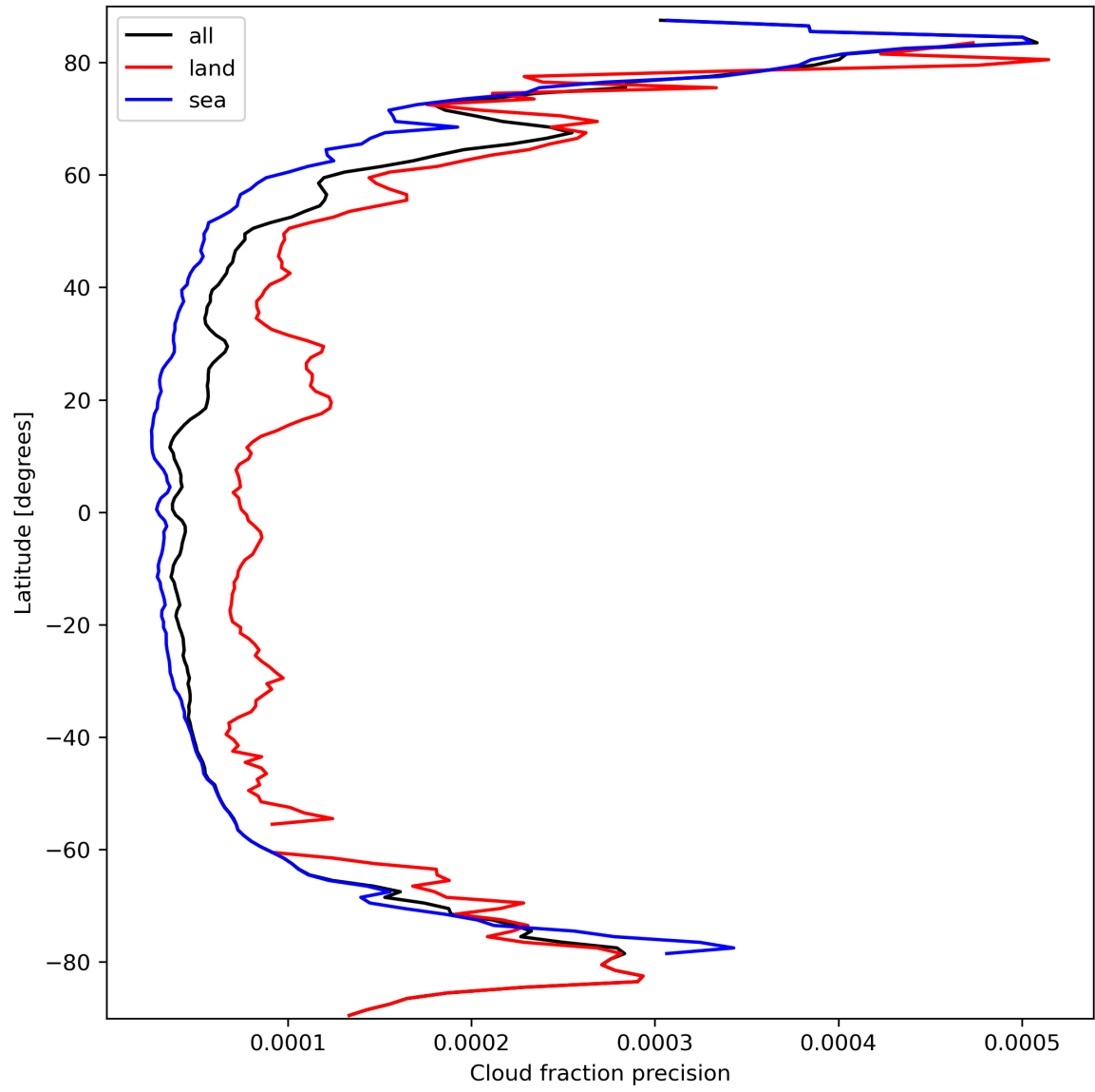
Figure 16: Zonal average of “Cloud fraction precision” for 2024-03-16 to 2024-03-18.
