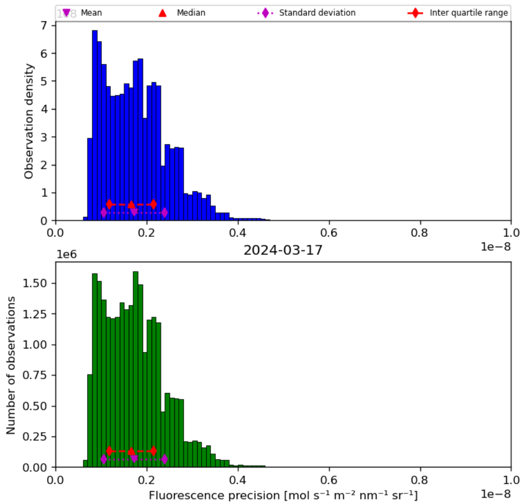
Figure 41: Histogram of “Fluorescence precision” for 2024-03-16 to 2024-03-18
