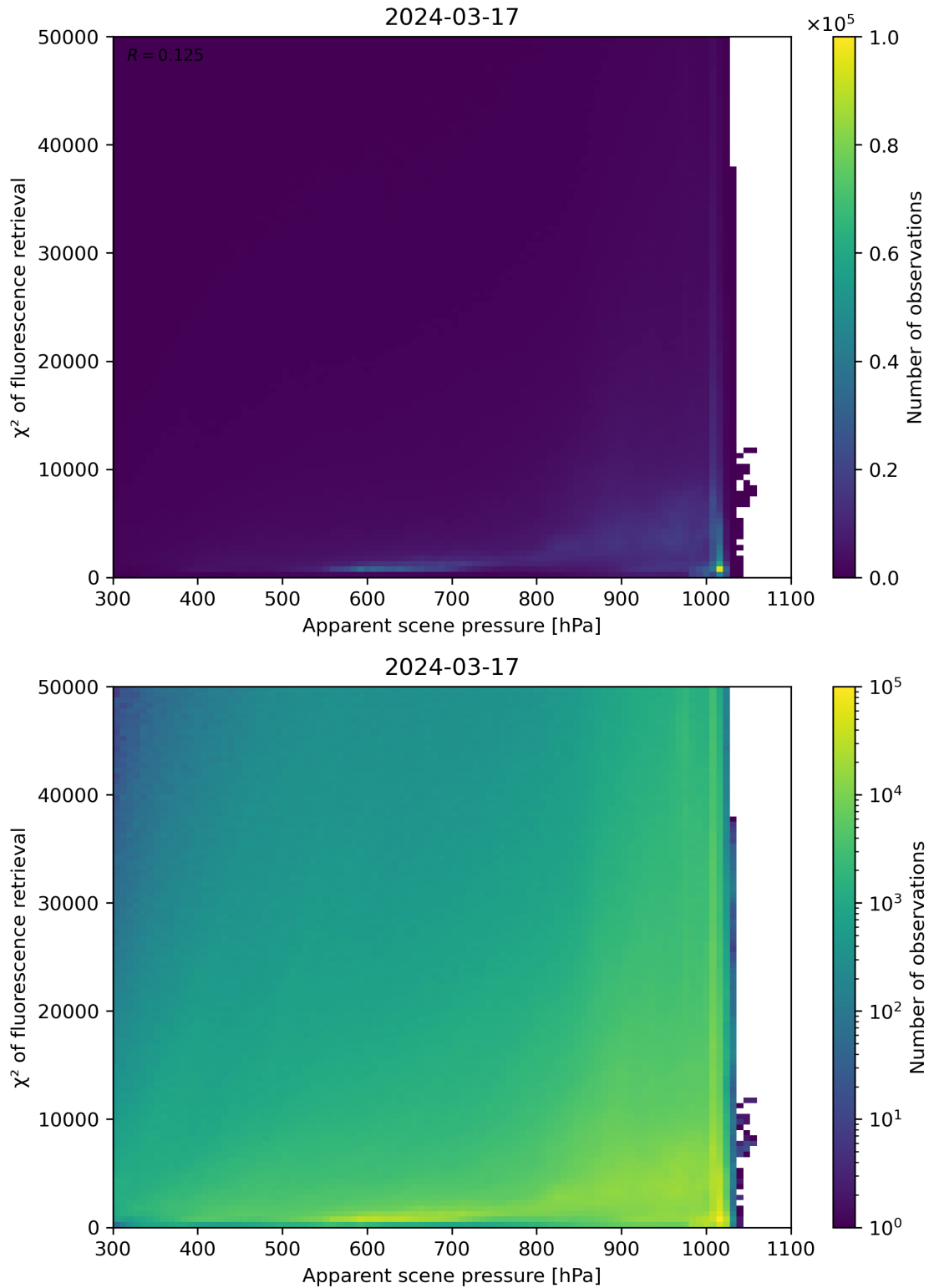
Figure 63: Scatter density plot of “Apparent scene pressure” against “ \chi^2 of fluorescence retrieval” for 2024-03-16 to 2024-03-18.
