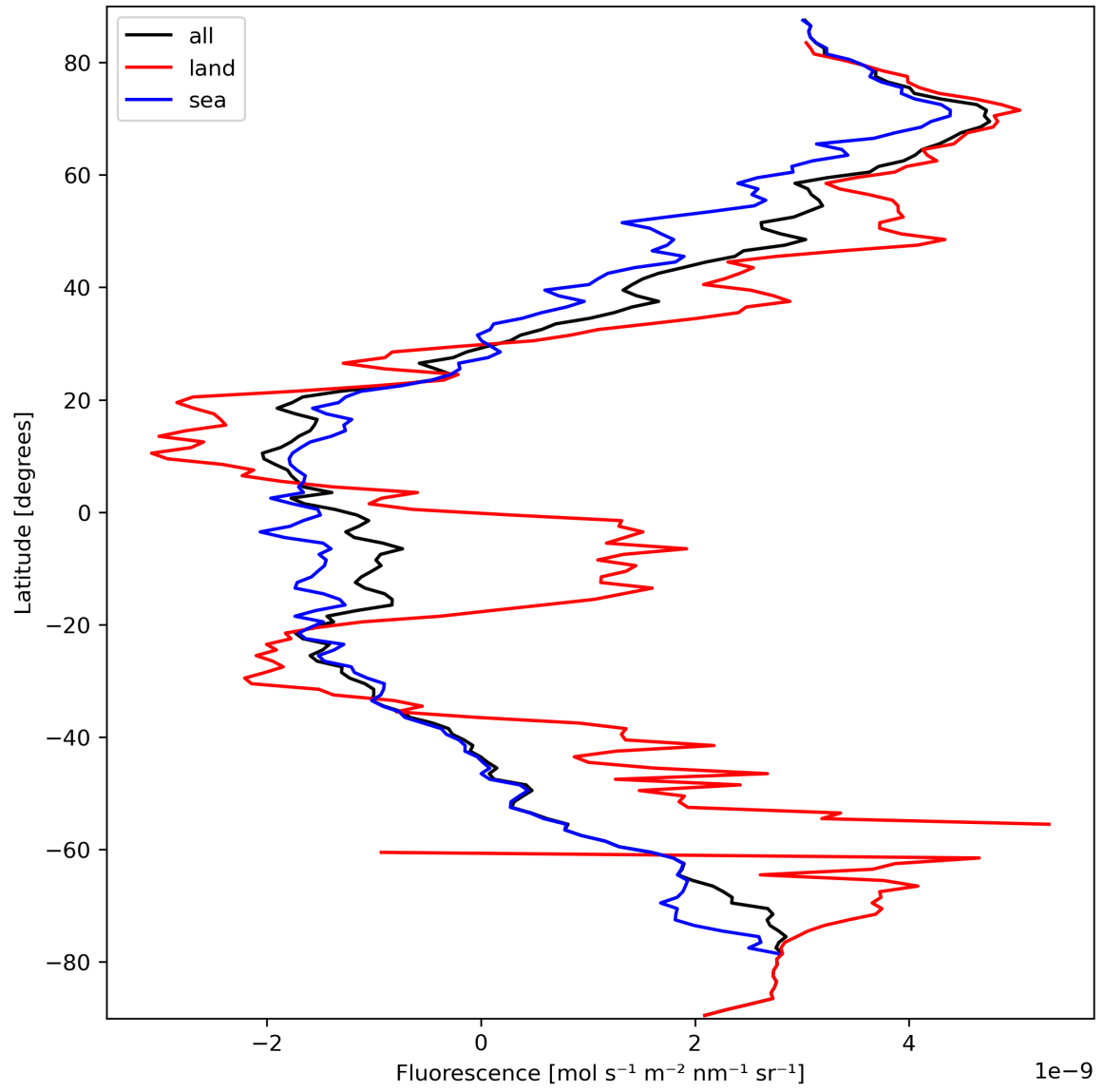
Figure 23: Zonal average of “Fluorescence” for 2024-03-16 to 2024-03-18.
