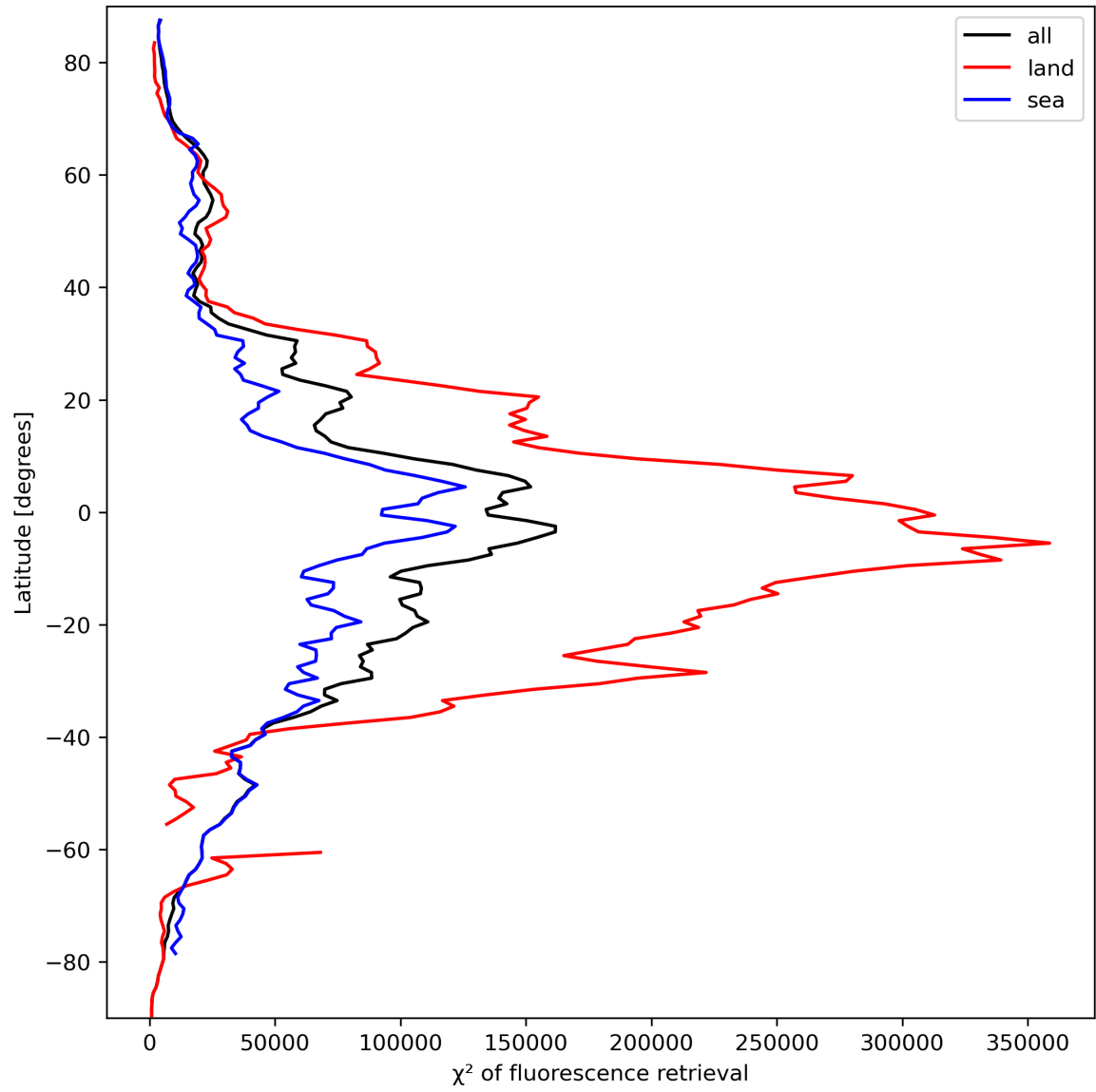
Figure 25: Zonal average of “ \chi^2 of fluorescence retrieval” for 2024-03-16 to 2024-03-18.
