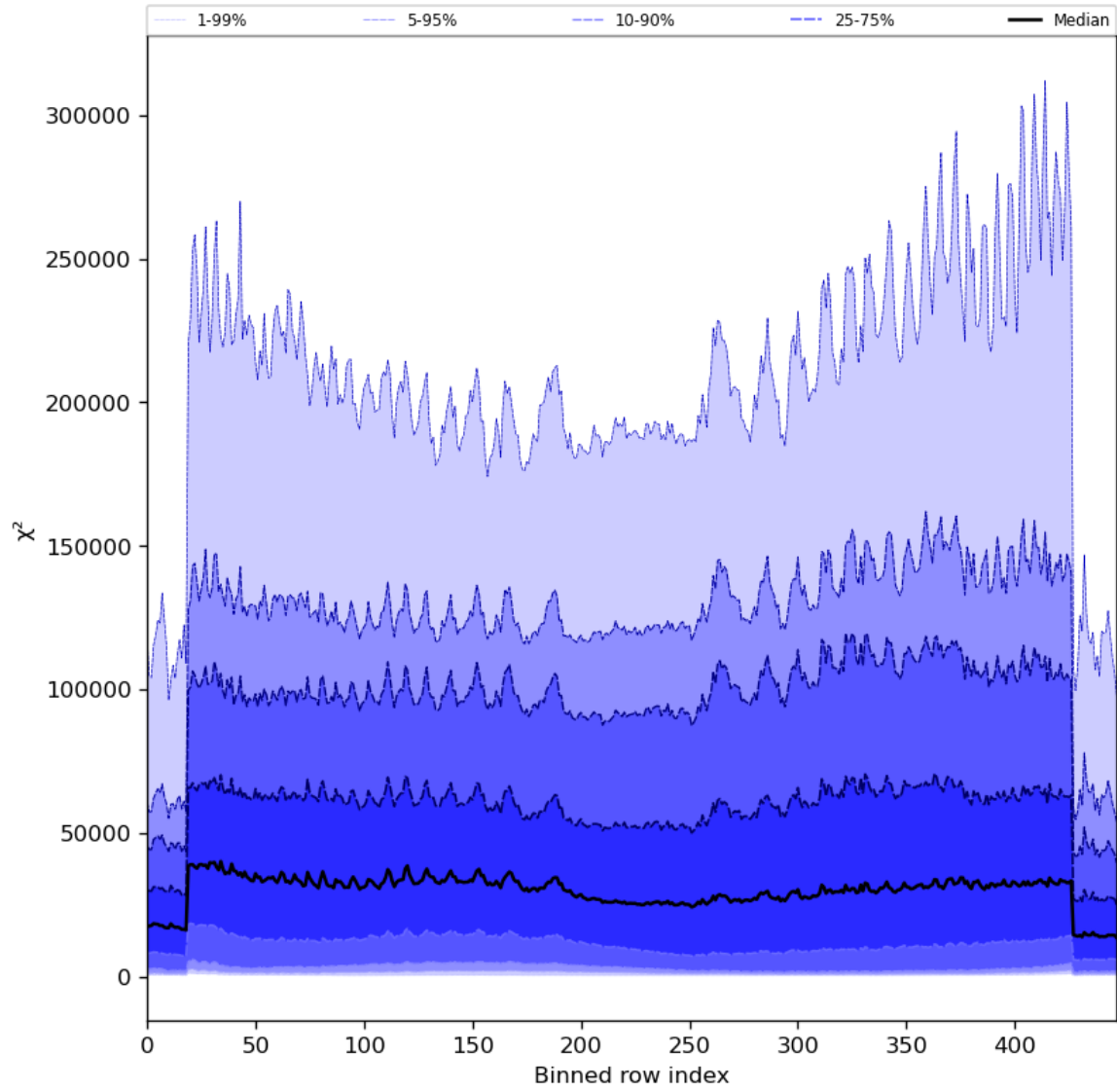
Figure 55: Along track statistics of “ \chi^2 ” for 2024-03-16 to 2024-03-18
