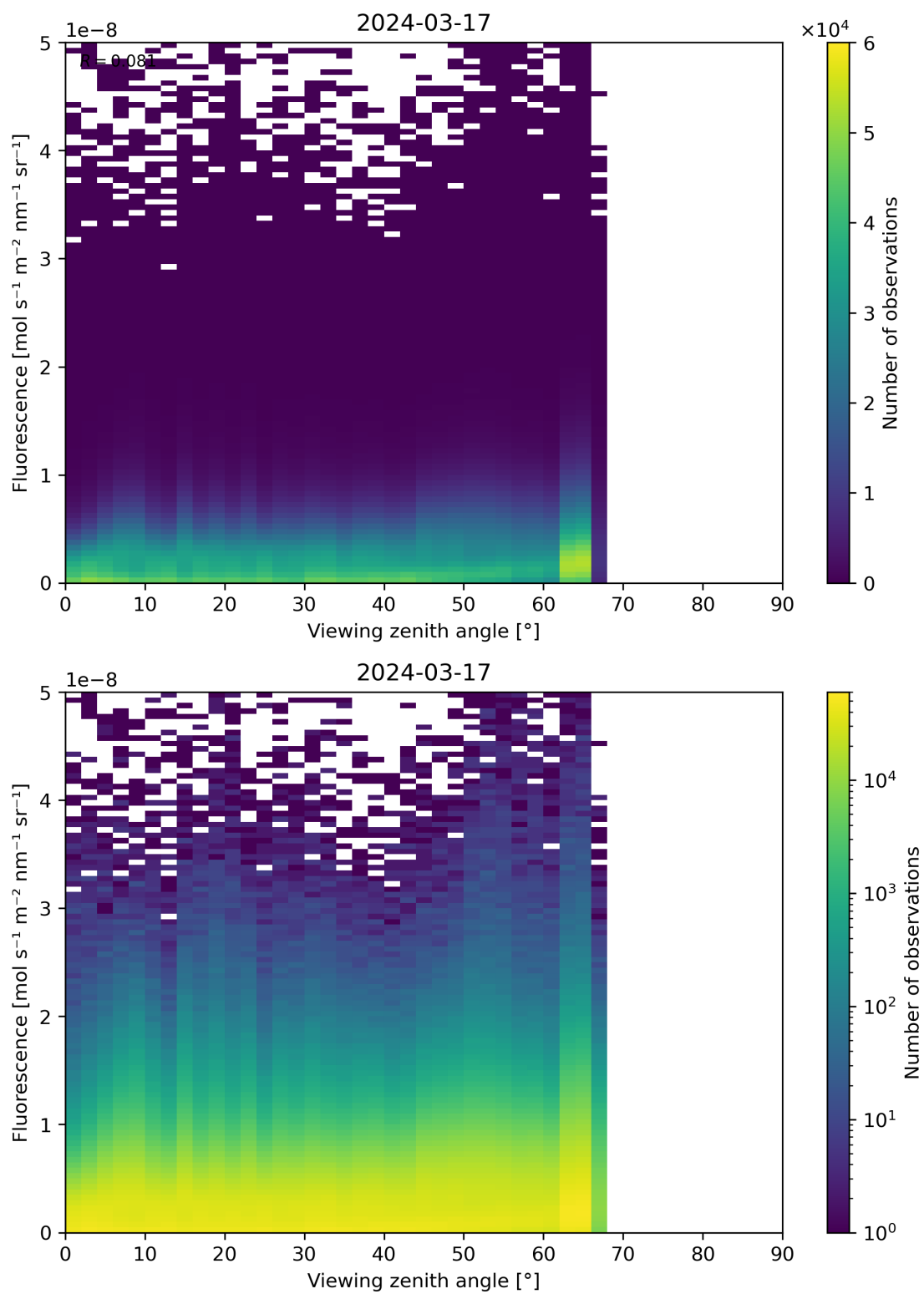
Figure 122: Scatter density plot of “Viewing zenith angle” against “Fluorescence” for 2024-03-16 to 2024-03-18.
