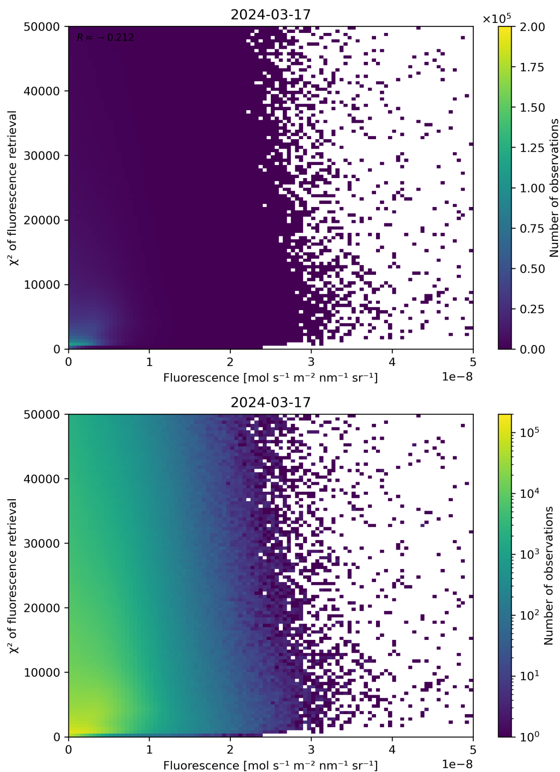
Figure 85: Scatter density plot of “Fluorescence” against “ \chi^2 of fluorescence retrieval” for 2024-03-16 to 2024-03-18.
