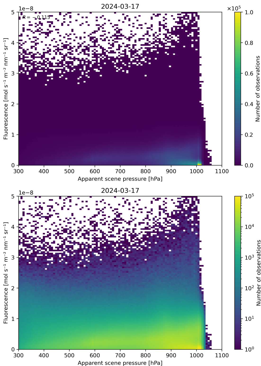
Figure 64: Scatter density plot of “Apparent scene pressure” against “Fluorescence” for 2024-03-16 to 2024-03-18.
