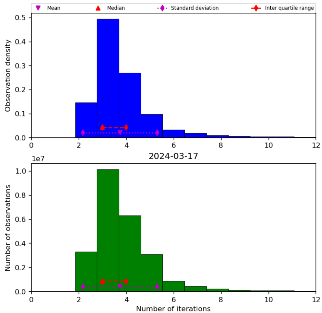
Figure 39: Histogram of “Number of iterations” for 2024-03-16 to 2024-03-18
