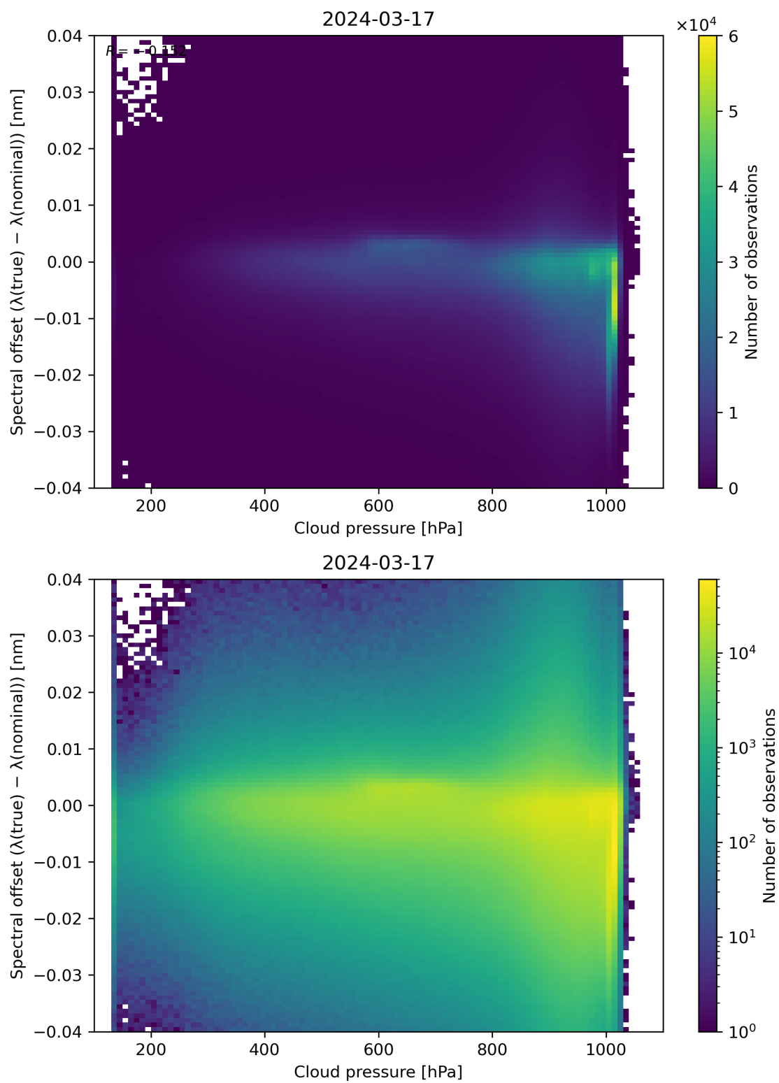
Figure 84: Scatter density plot of “Cloud pressure” against “Spectral offset ( \lambda(\text{true}) - \lambda(\text{nominal}) )” for 2024-03-16 to 2024-03-18.
