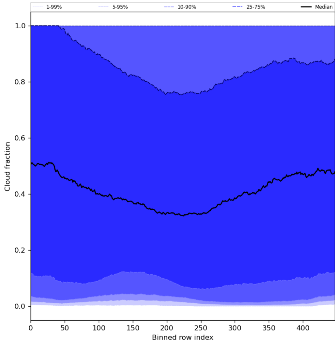
Figure 49: Along track statistics of “Cloud fraction” for 2024-03-16 to 2024-03-18
