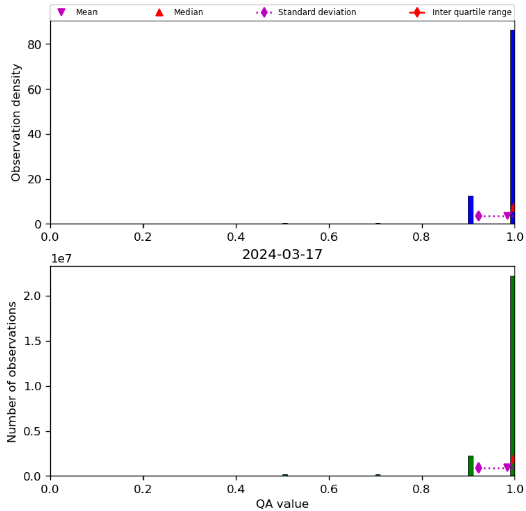
Figure 29: Histogram of “QA value” for 2024-03-16 to 2024-03-18
