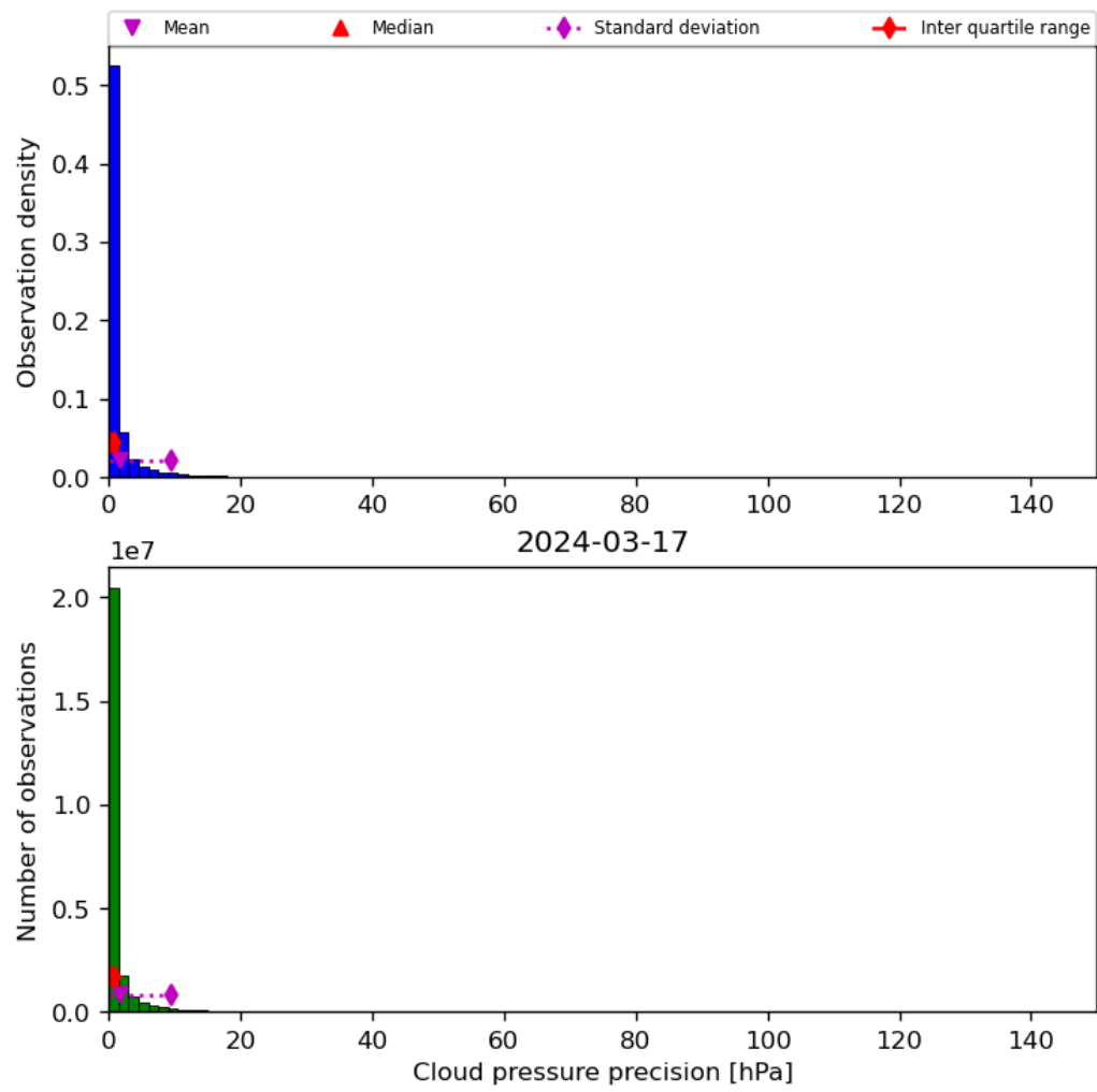
Figure 31: Histogram of “Cloud pressure precision” for 2024-03-16 to 2024-03-18
