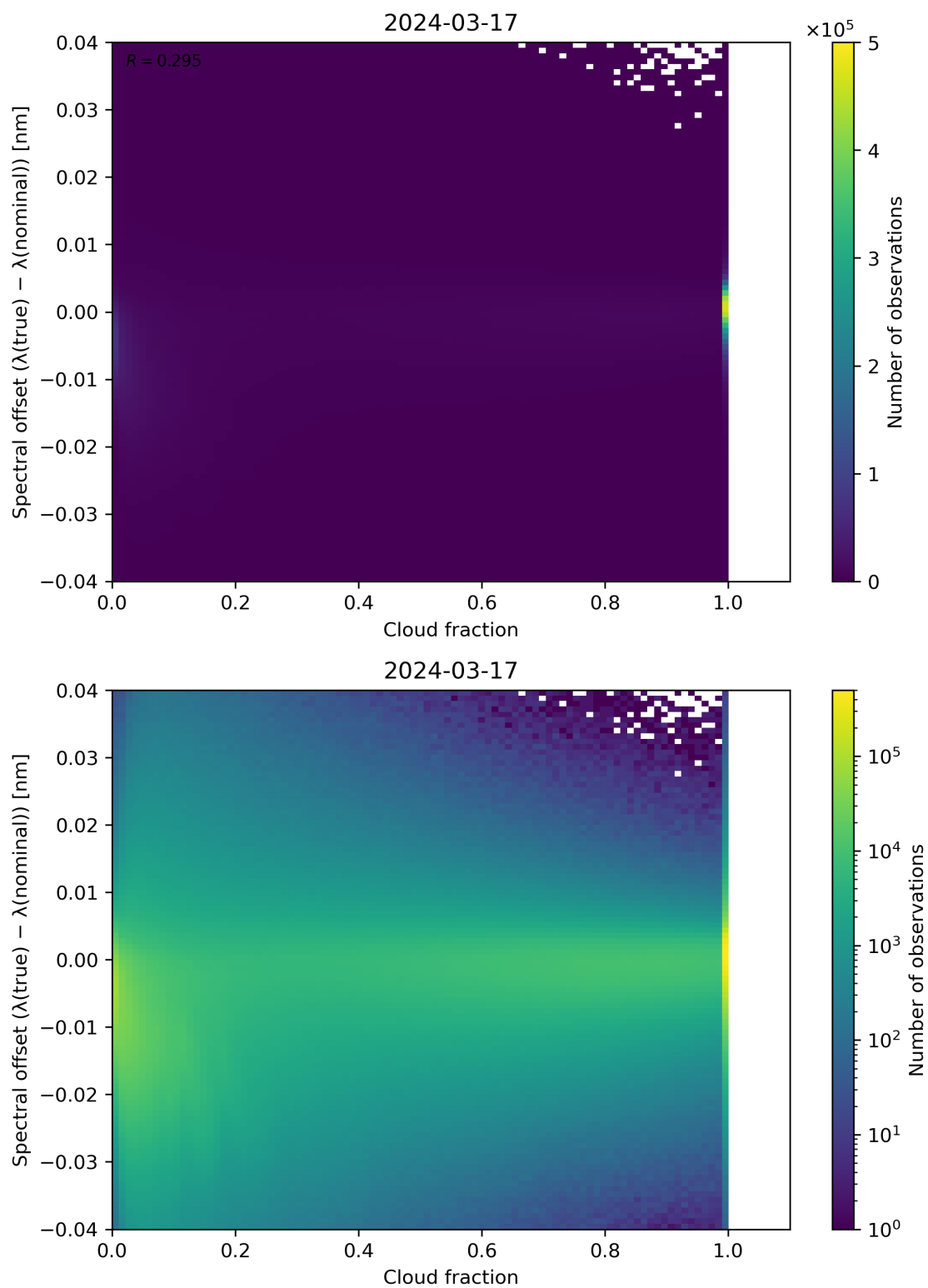
Figure 76: Scatter density plot of “Cloud fraction” against “Spectral offset ( \lambda(\text{true}) - \lambda(\text{nominal}) )” for 2024-03-16 to 2024-03-18.
