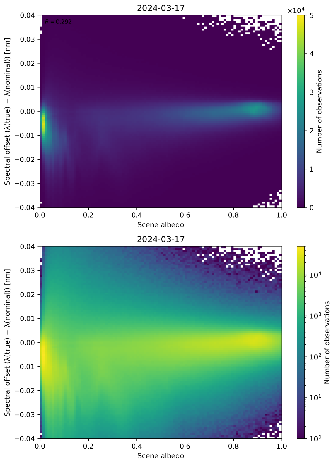
Figure 107: Scatter density plot of “Scene albedo” against “Spectral offset ( \lambda(\text{true}) - \lambda(\text{nominal}) )” for 2024-03-16 to 2024-03-18.
