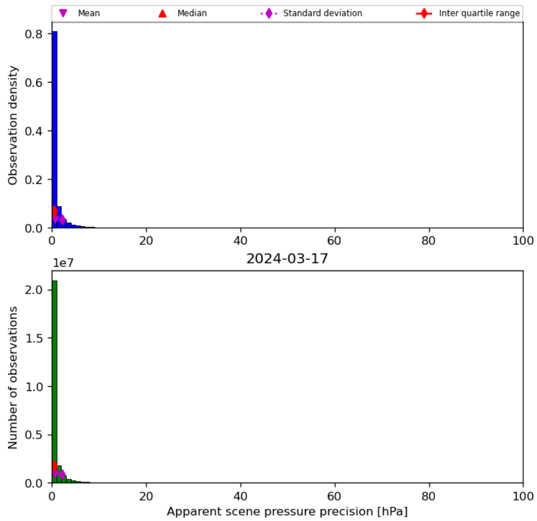
Figure 37: Histogram of “Apparent scene pressure precision” for 2024-03-16 to 2024-03-18
