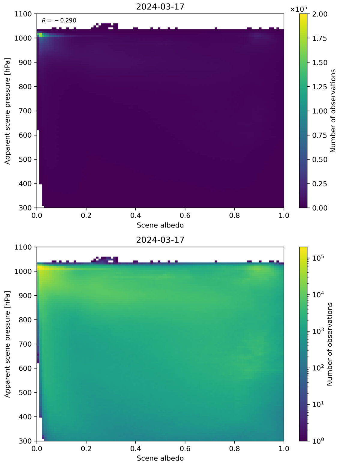
Figure 102: Scatter density plot of “Scene albedo” against “Apparent scene pressure” for 2024-03-16 to 2024-03-18.
