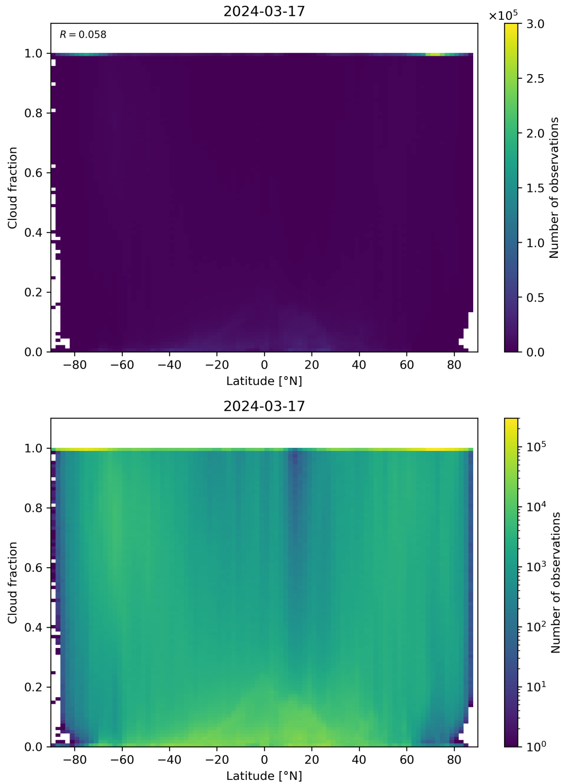
Figure 90: Scatter density plot of “Latitude” against “Cloud fraction” for 2024-03-16 to 2024-03-18.
