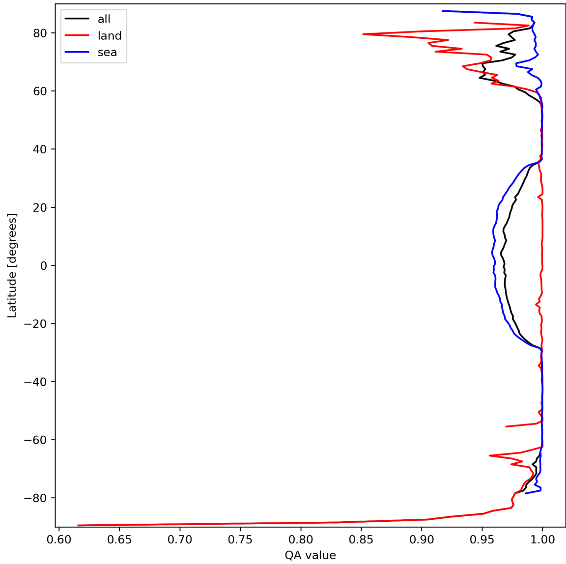
Figure 12: Zonal average of “QA value” for 2024-03-16 to 2024-03-18.
