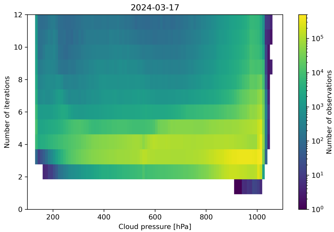
Figure 81: Scatter density plot of “Cloud pressure” against “Number of iterations” for 2024-03-16 to 2024-03-18.
