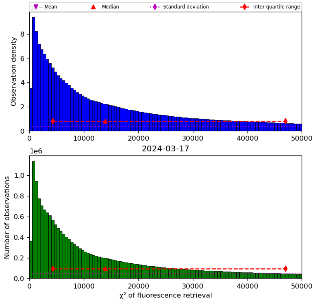
Figure 42: Histogram of “ \chi^2 of fluorescence retrieval” for 2024-03-16 to 2024-03-18
