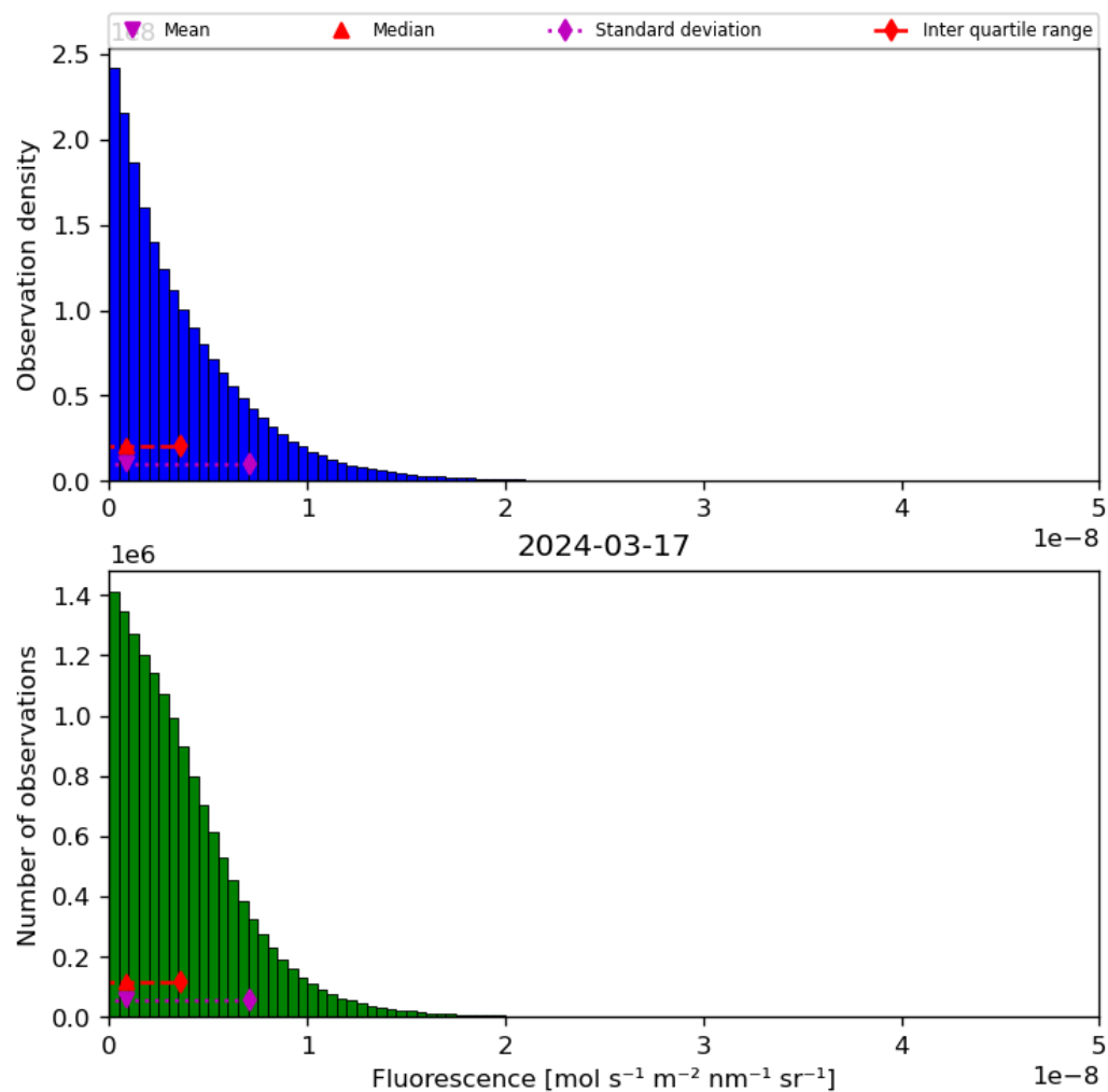
Figure 40: Histogram of “Fluorescence” for 2024-03-16 to 2024-03-18
