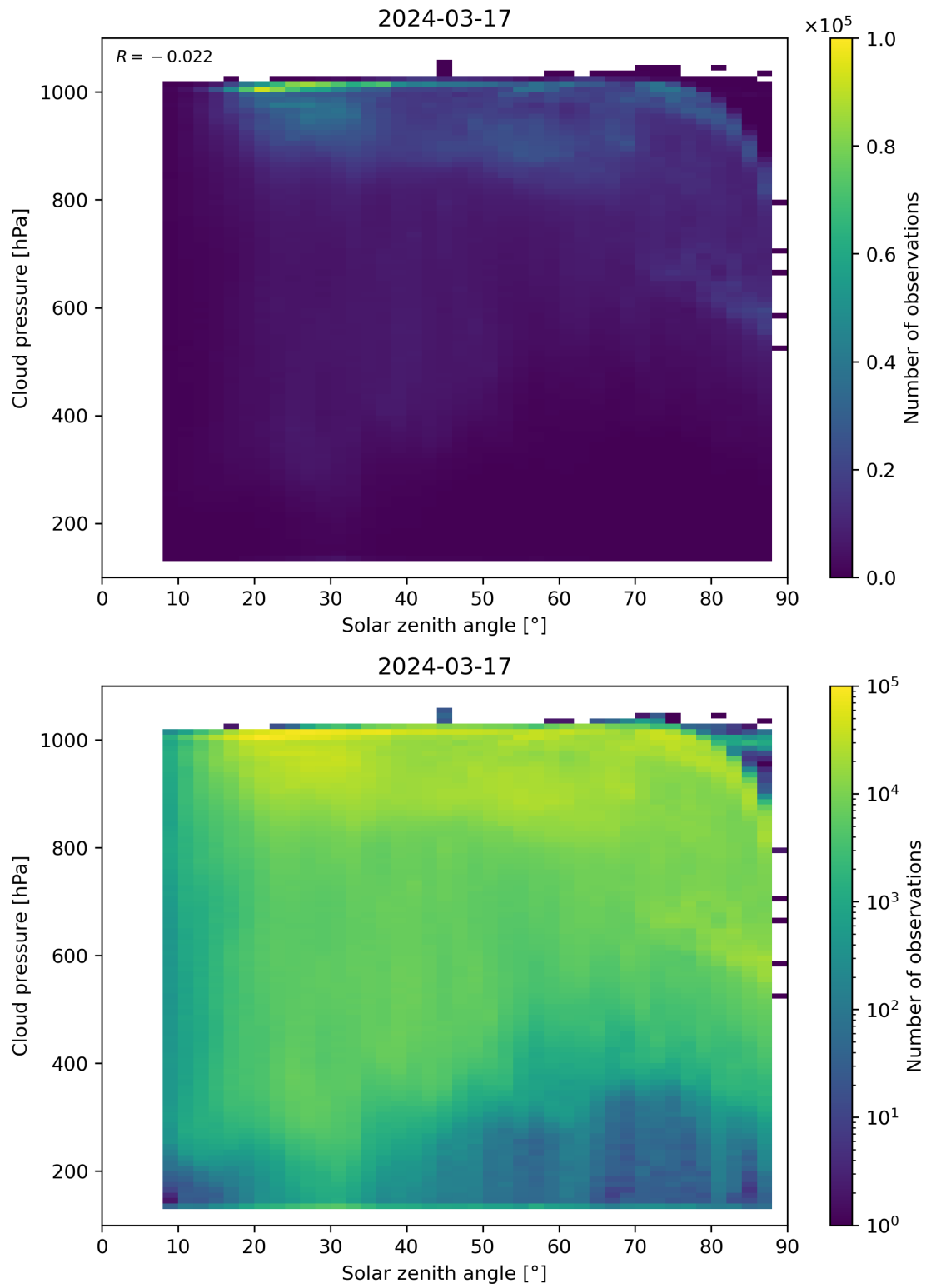
Figure 111: Scatter density plot of “Solar zenith angle” against “Cloud pressure” for 2024-03-16 to 2024-03-18.
