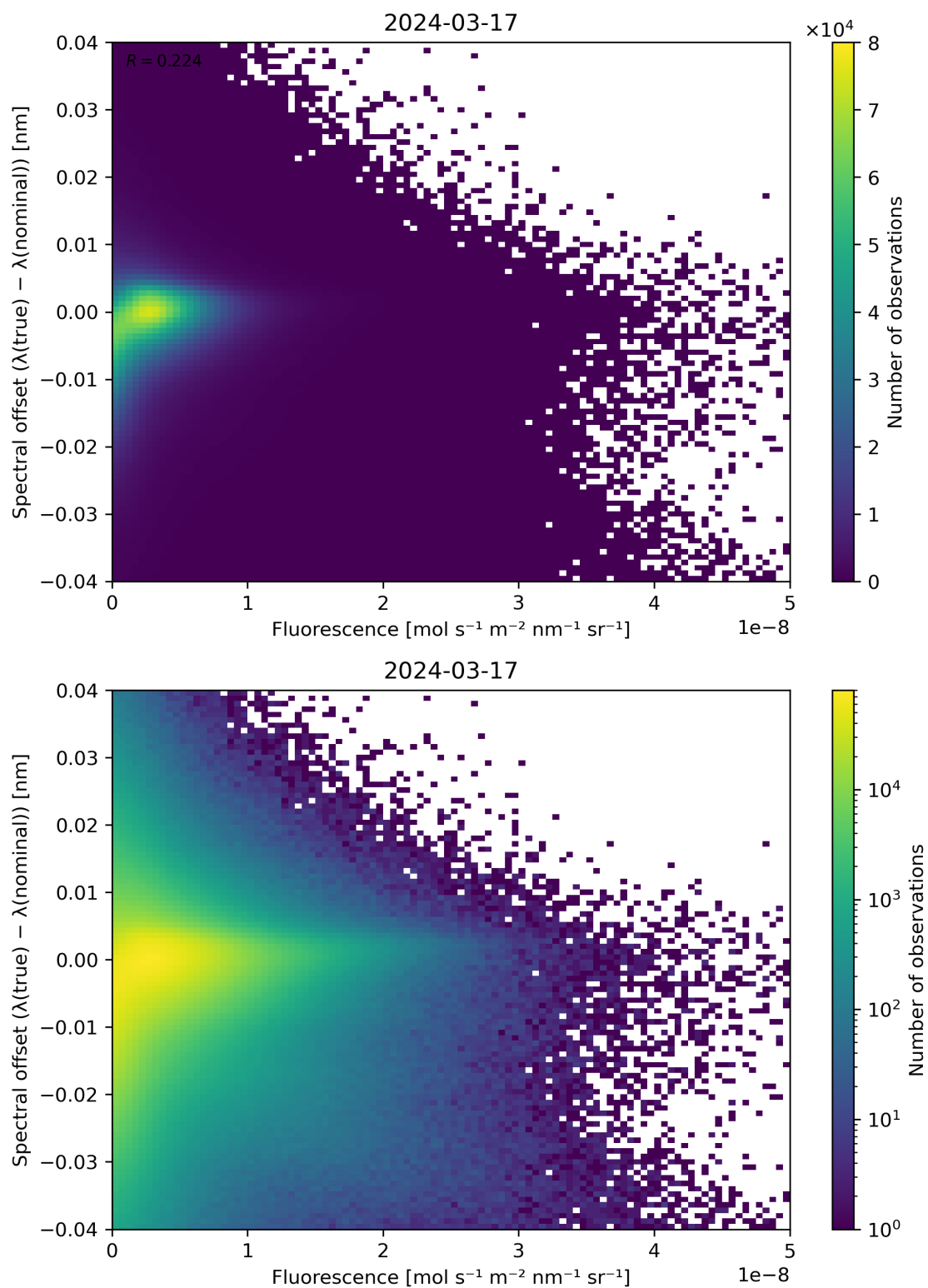
Figure 87: Scatter density plot of “Fluorescence” against “Spectral offset ( \lambda(\text{true}) - \lambda(\text{nominal}) )” for 2024-03-16 to 2024-03-18.
