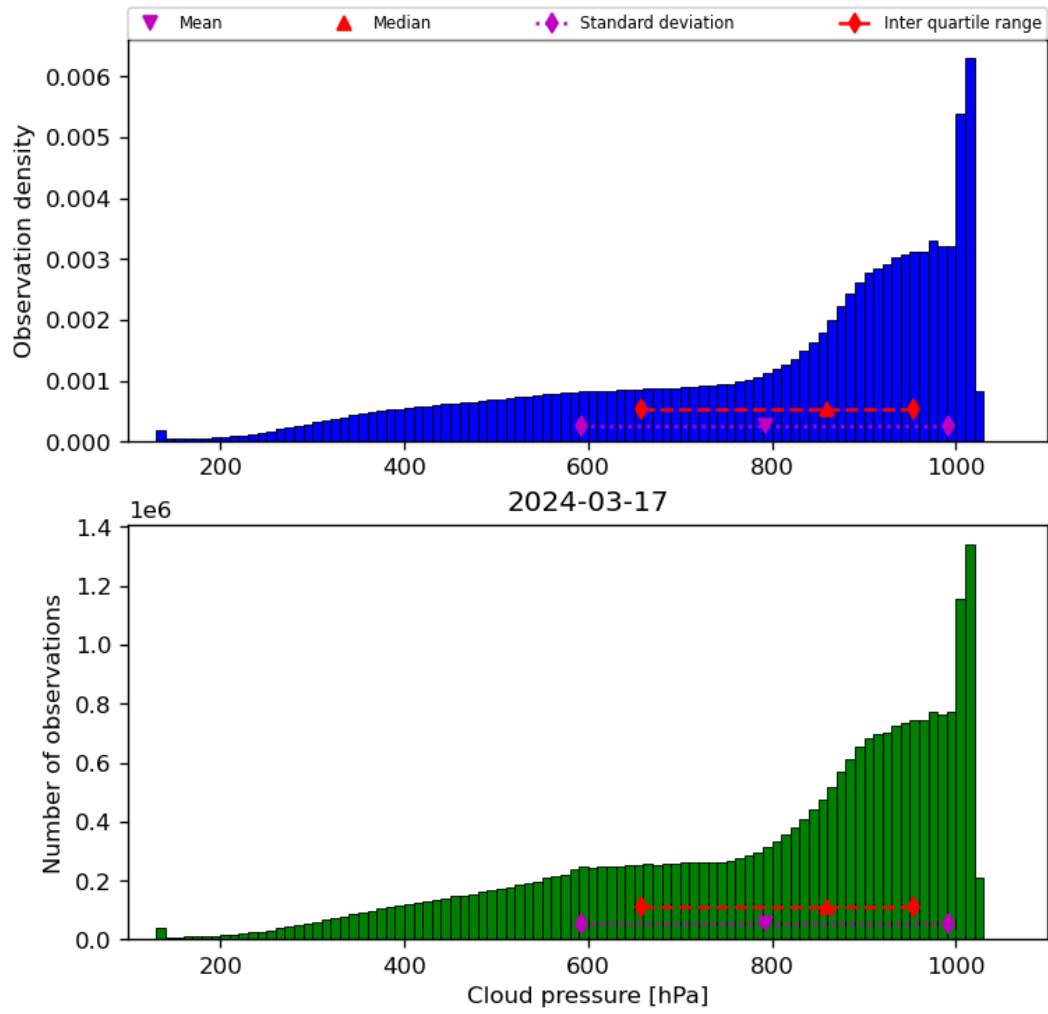
Figure 30: Histogram of “Cloud pressure” for 2024-03-16 to 2024-03-18
