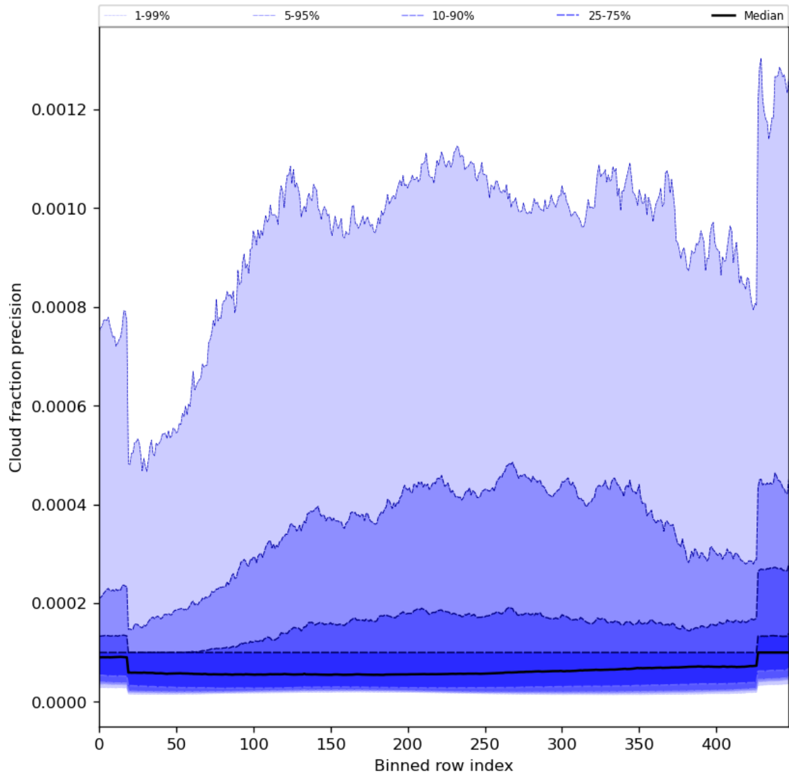
Figure 50: Along track statistics of “Cloud fraction precision” for 2024-03-16 to 2024-03-18
