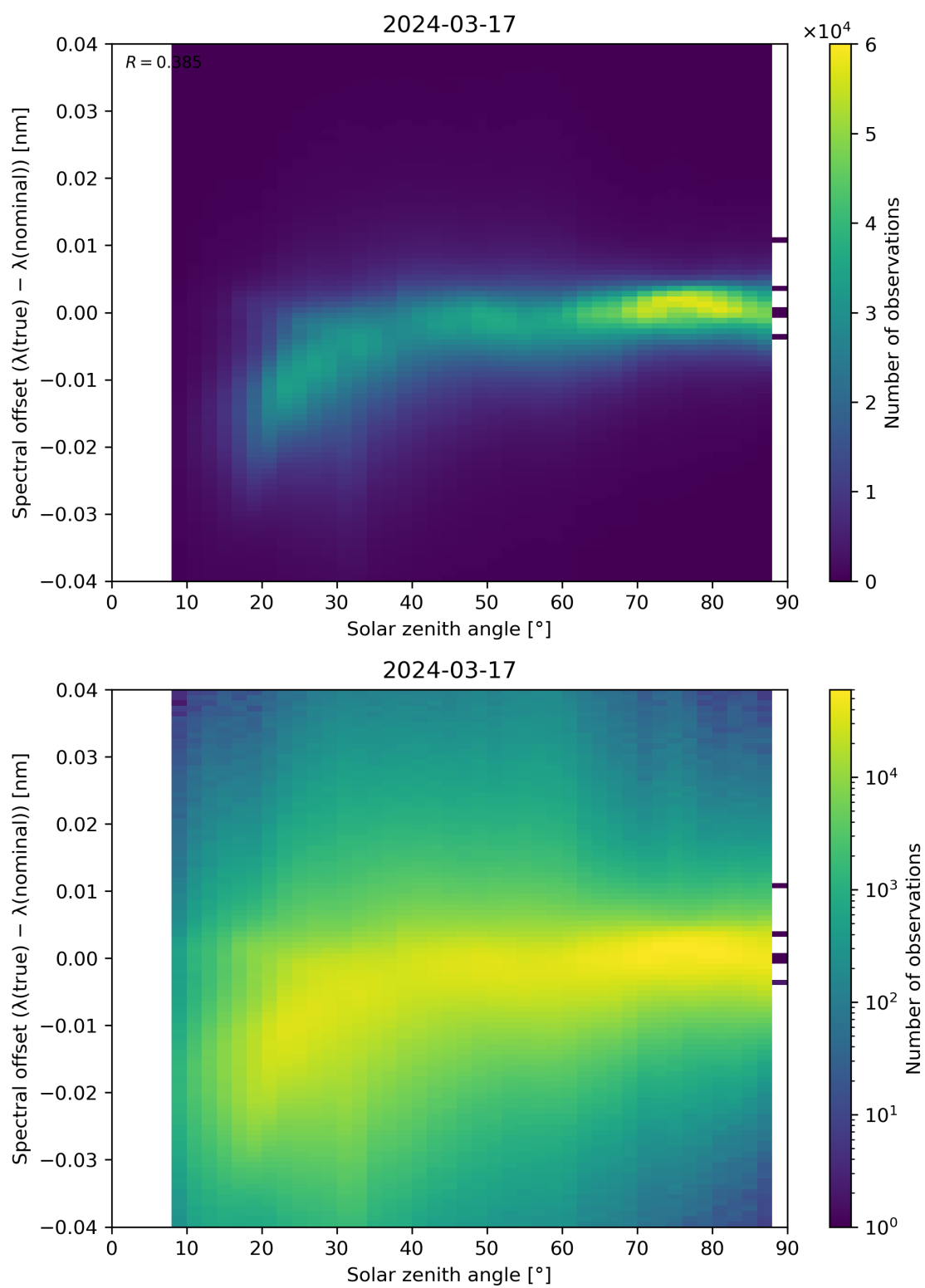
Figure 117: Scatter density plot of “Solar zenith angle” against “Spectral offset ( \lambda(\text{true}) - \lambda(\text{nominal}) )” for 2024-03-16 to 2024-03-18.
