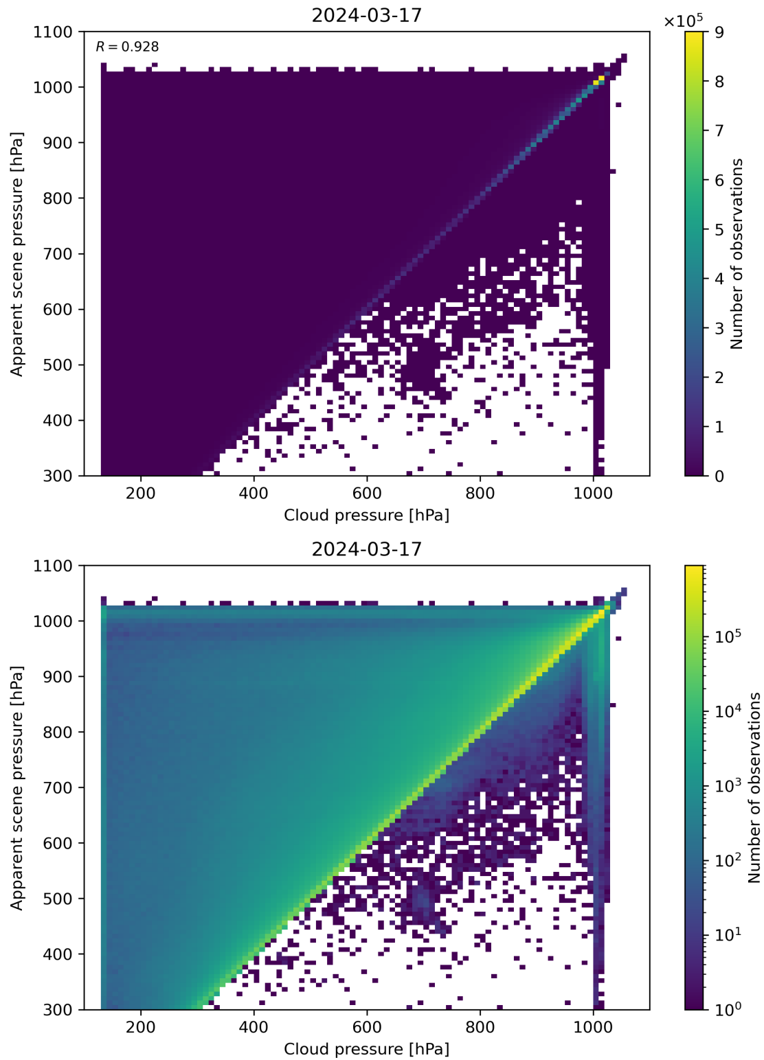
Figure 77: Scatter density plot of “Cloud pressure” against “Apparent scene pressure” for 2024-03-16 to 2024-03-18.
