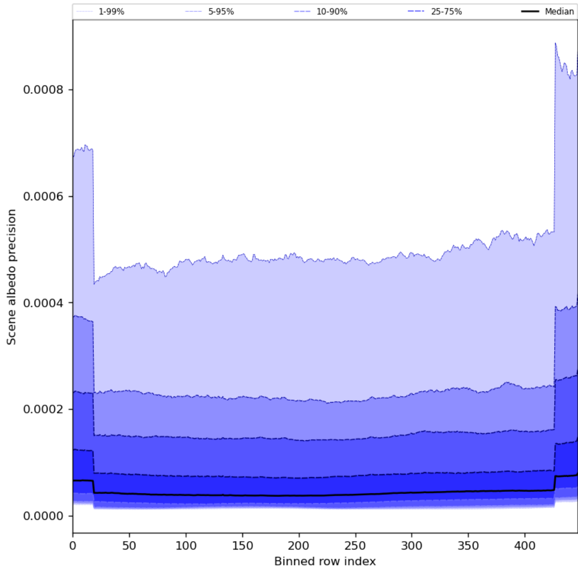
Figure 52: Along track statistics of “Scene albedo precision” for 2024-03-16 to 2024-03-18
