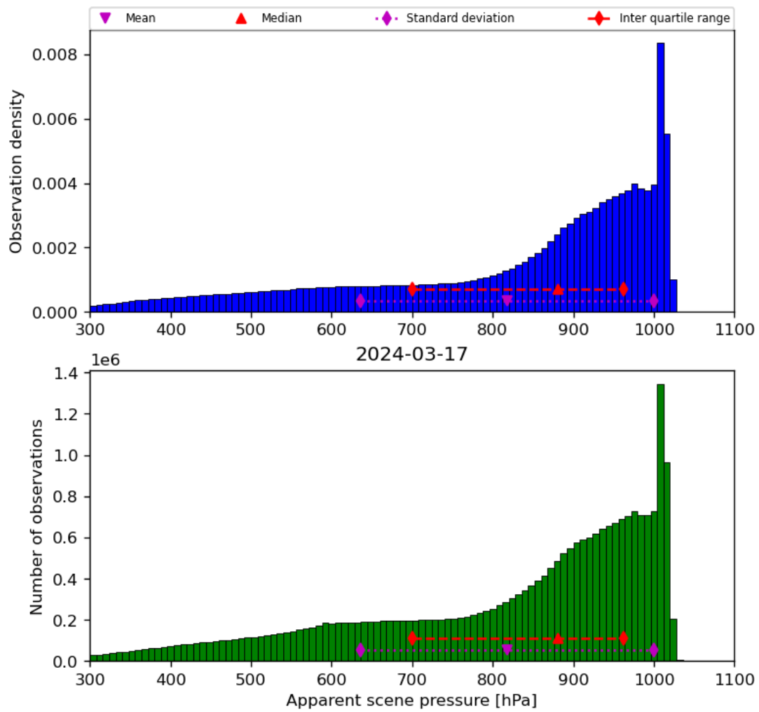
Figure 36: Histogram of “Apparent scene pressure” for 2024-03-16 to 2024-03-18
