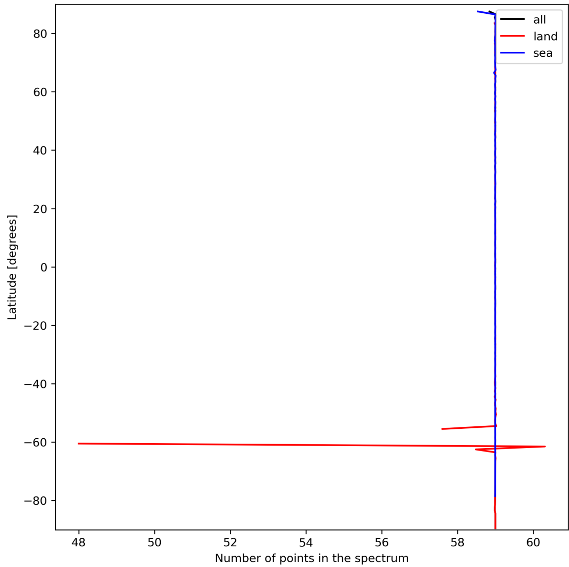
Figure 27: Zonal average of “Number of points in the spectrum” for 2024-03-16 to 2024-03-18.
