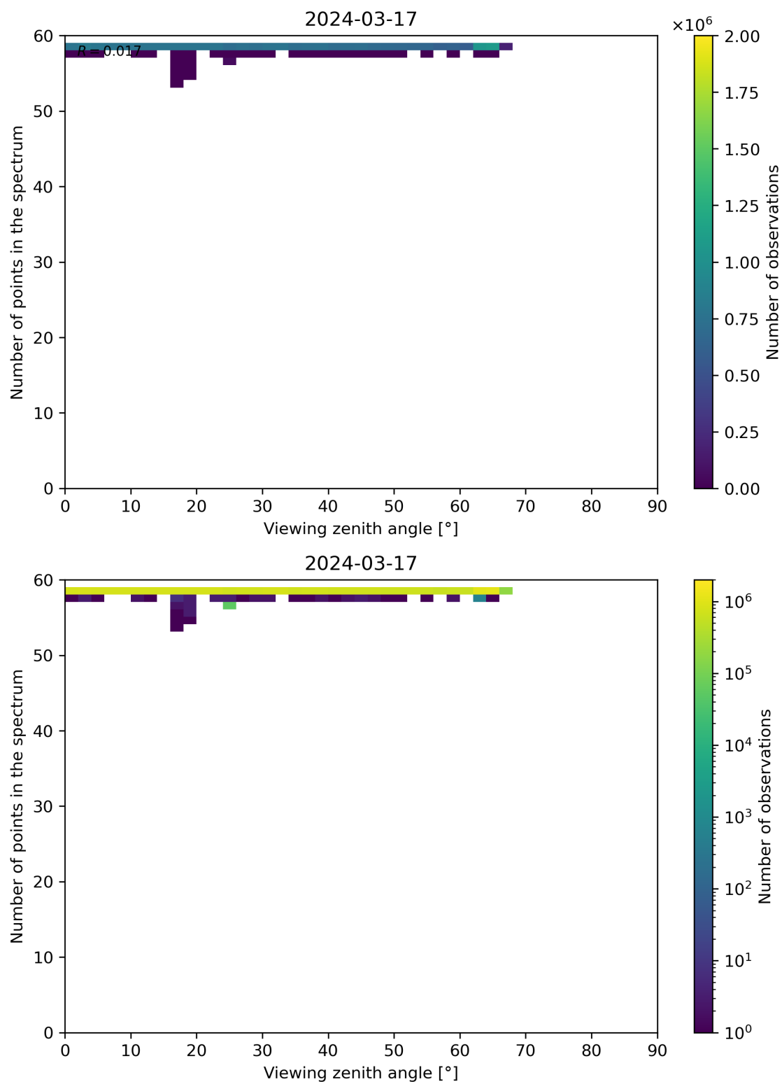
Figure 125: Scatter density plot of “Viewing zenith angle” against “Number of points in the spectrum” for 2024-03-16 to 2024-03-18.
