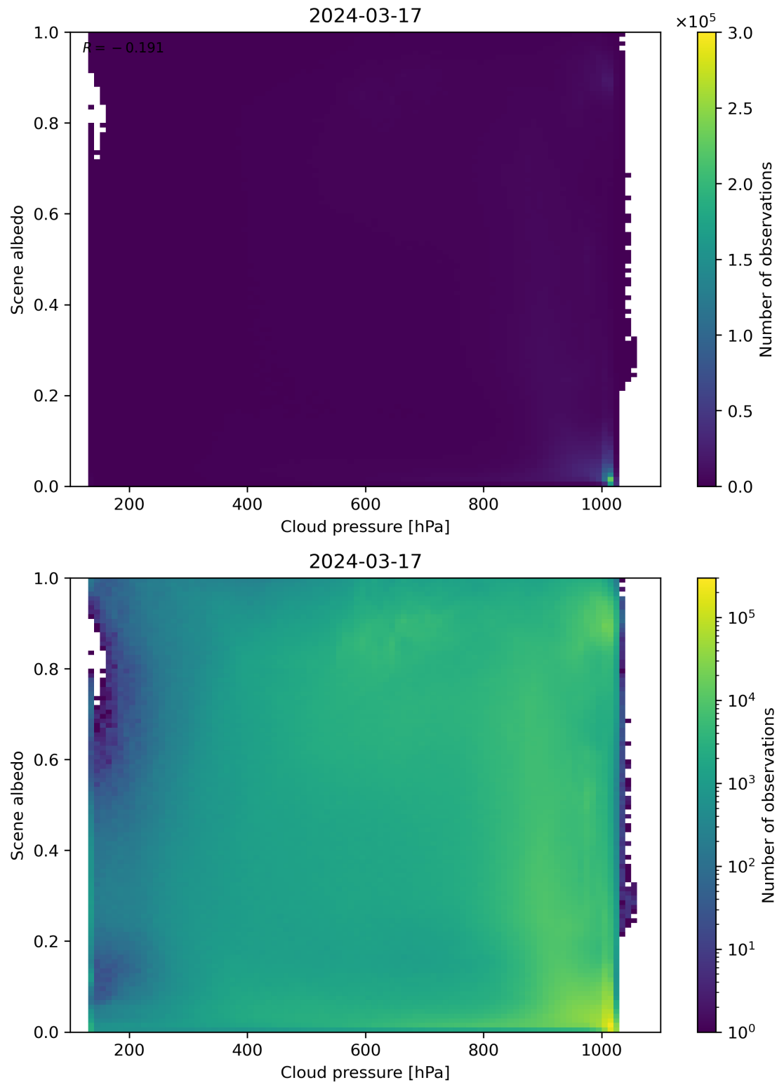
Figure 83: Scatter density plot of “Cloud pressure” against “Scene albedo” for 2024-03-16 to 2024-03-18.
