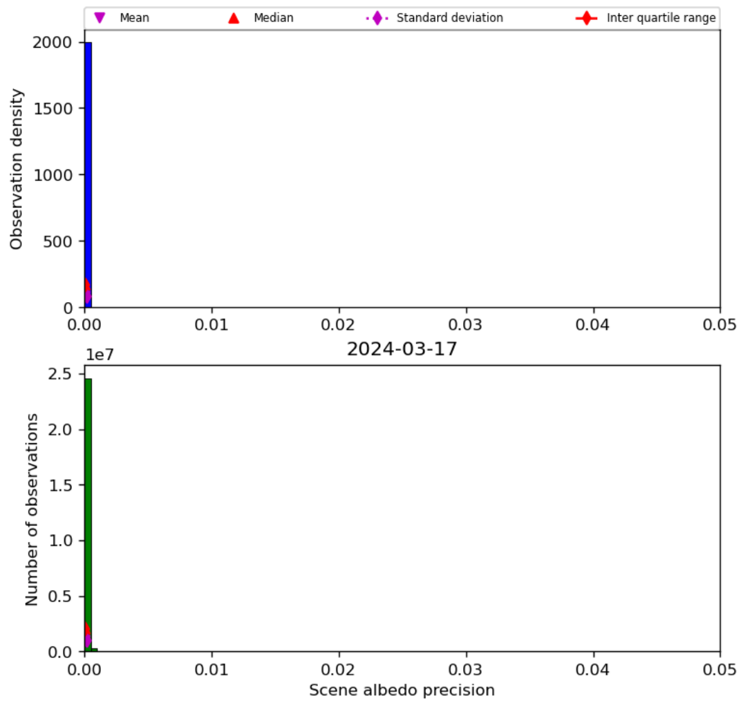
Figure 35: Histogram of “Scene albedo precision” for 2024-03-16 to 2024-03-18
