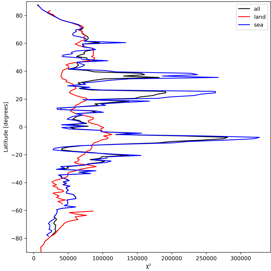
Figure 21: Zonal average of “ \chi^2 ” for 2024-03-16 to 2024-03-18.
