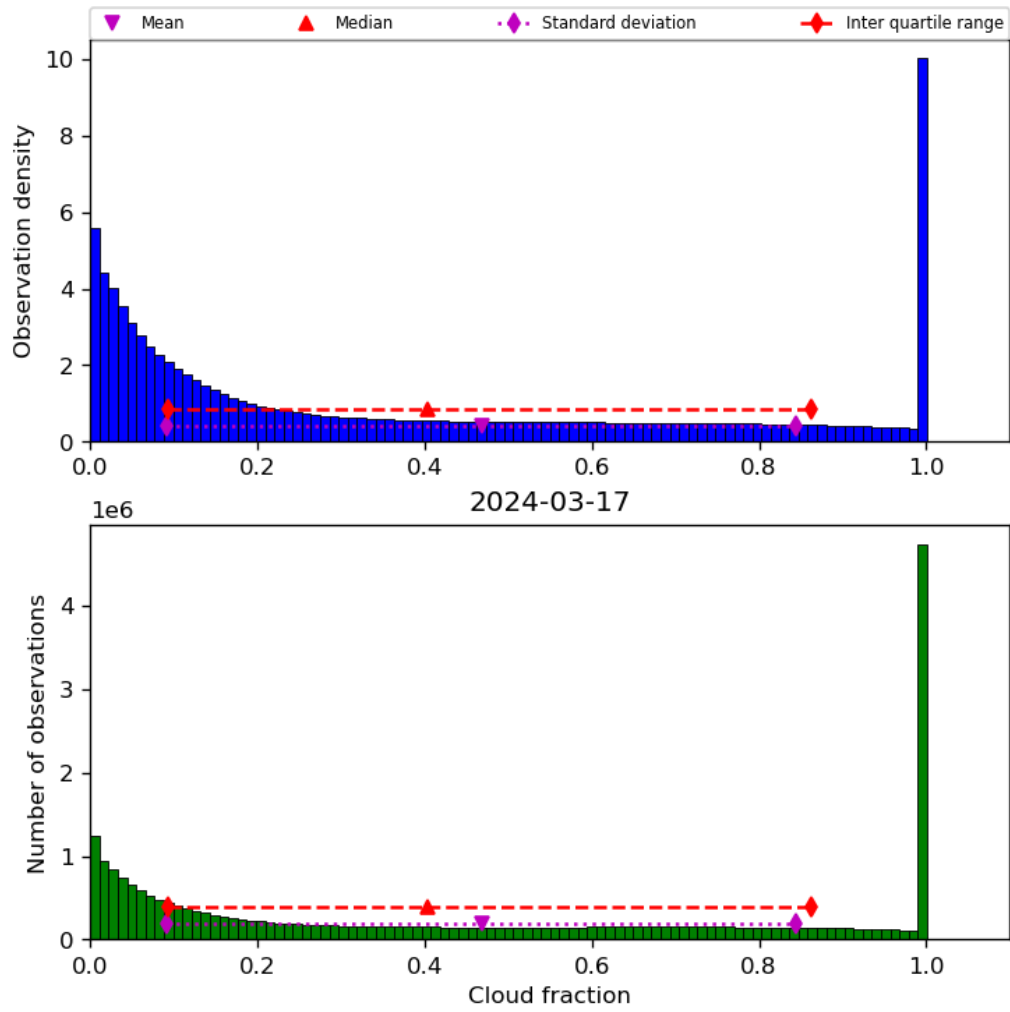
Figure 32: Histogram of “Cloud fraction” for 2024-03-16 to 2024-03-18
