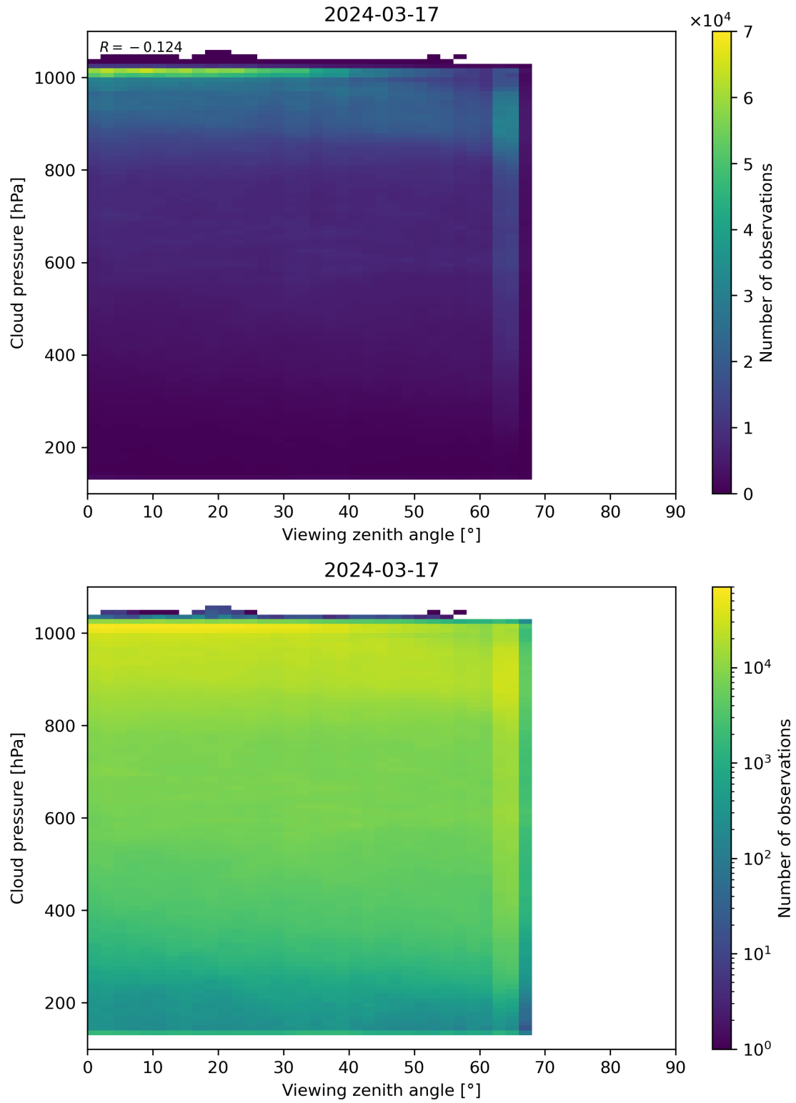
Figure 121: Scatter density plot of “Viewing zenith angle” against “Cloud pressure” for 2024-03-16 to 2024-03-18.
