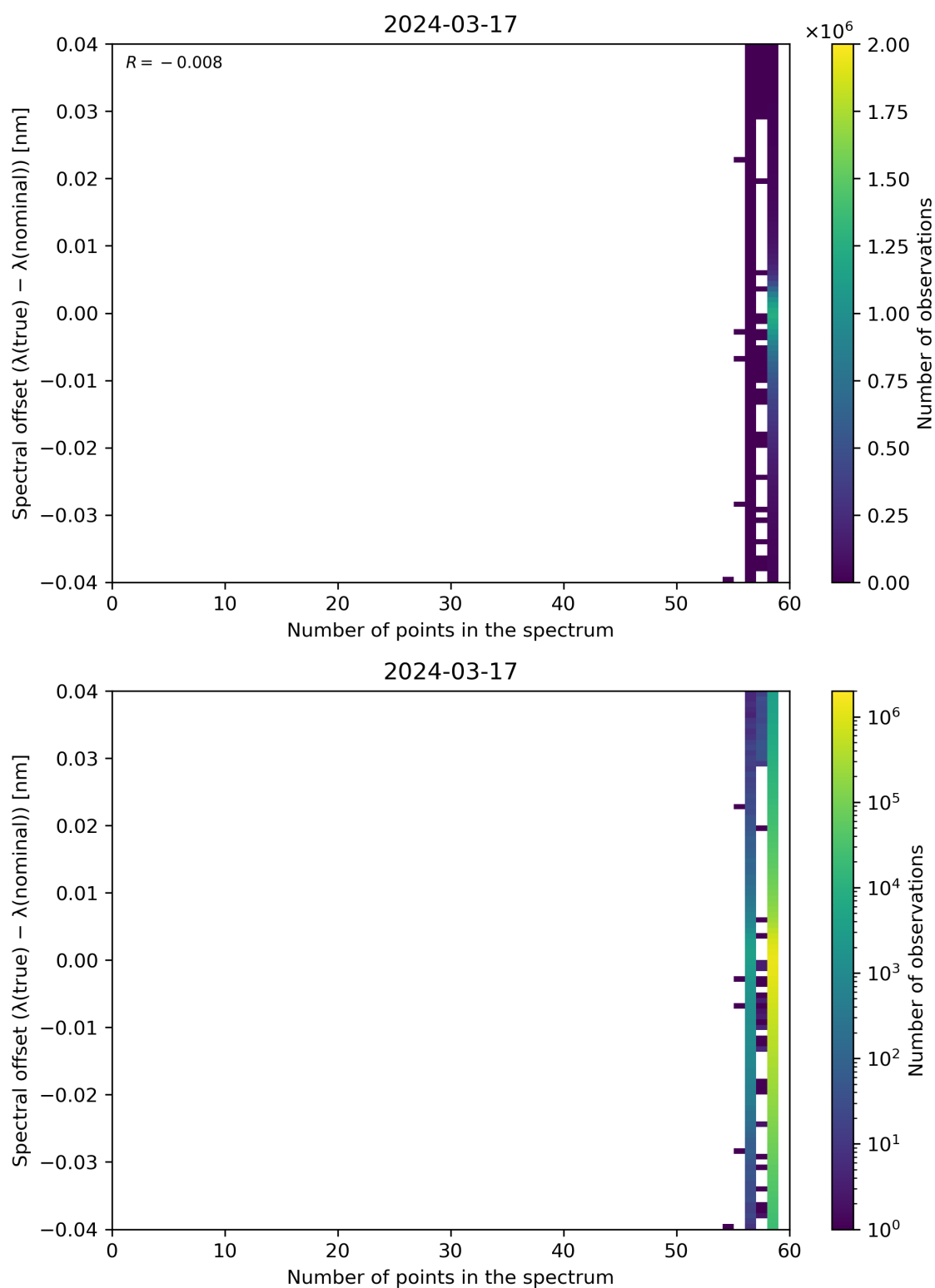
Figure 101: Scatter density plot of “Number of points in the spectrum” against “Spectral offset ( \lambda(\text{true}) - \lambda(\text{nominal}) )” for 2024-03-16 to 2024-03-18.
