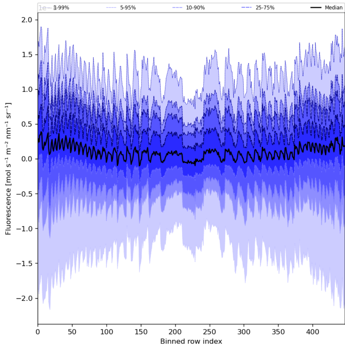
Figure 57: Along track statistics of “Fluorescence” for 2024-03-16 to 2024-03-18
