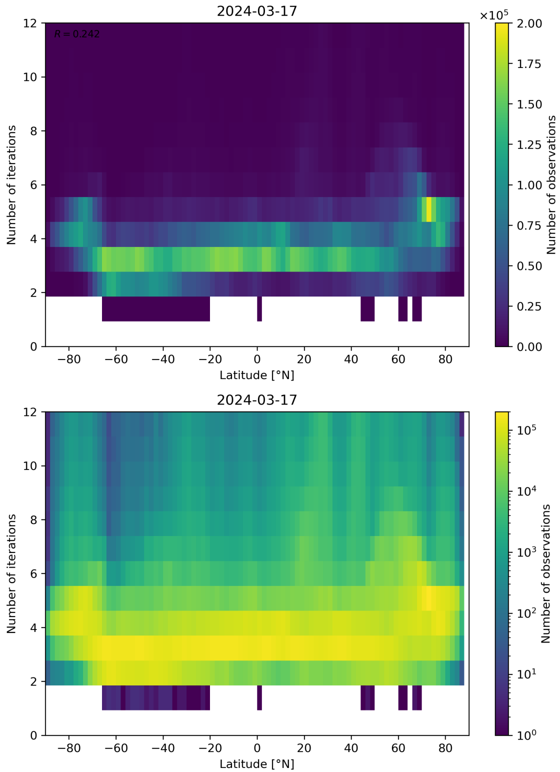
Figure 93: Scatter density plot of “Latitude” against “Number of iterations” for 2024-03-16 to 2024-03-18.
