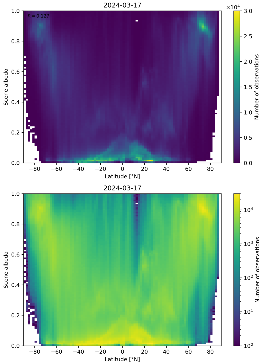
Figure 95: Scatter density plot of “Latitude” against “Scene albedo” for 2024-03-16 to 2024-03-18.
