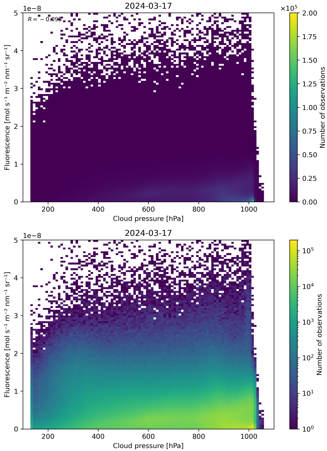
Figure 80: Scatter density plot of “Cloud pressure” against “Fluorescence” for 2024-03-16 to 2024-03-18.
