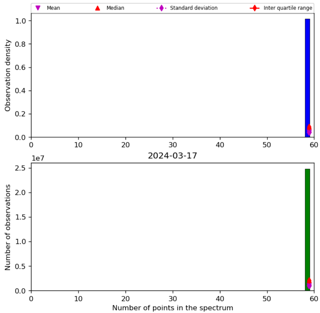
Figure 44: Histogram of “Number of points in the spectrum” for 2024-03-16 to 2024-03-18
