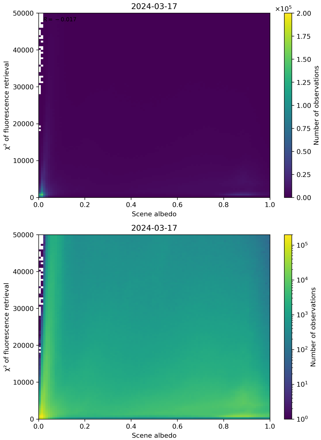
Figure 103: Scatter density plot of “Scene albedo” against “ \chi^2 of fluorescence retrieval” for 2024-03-16 to 2024-03-18.
