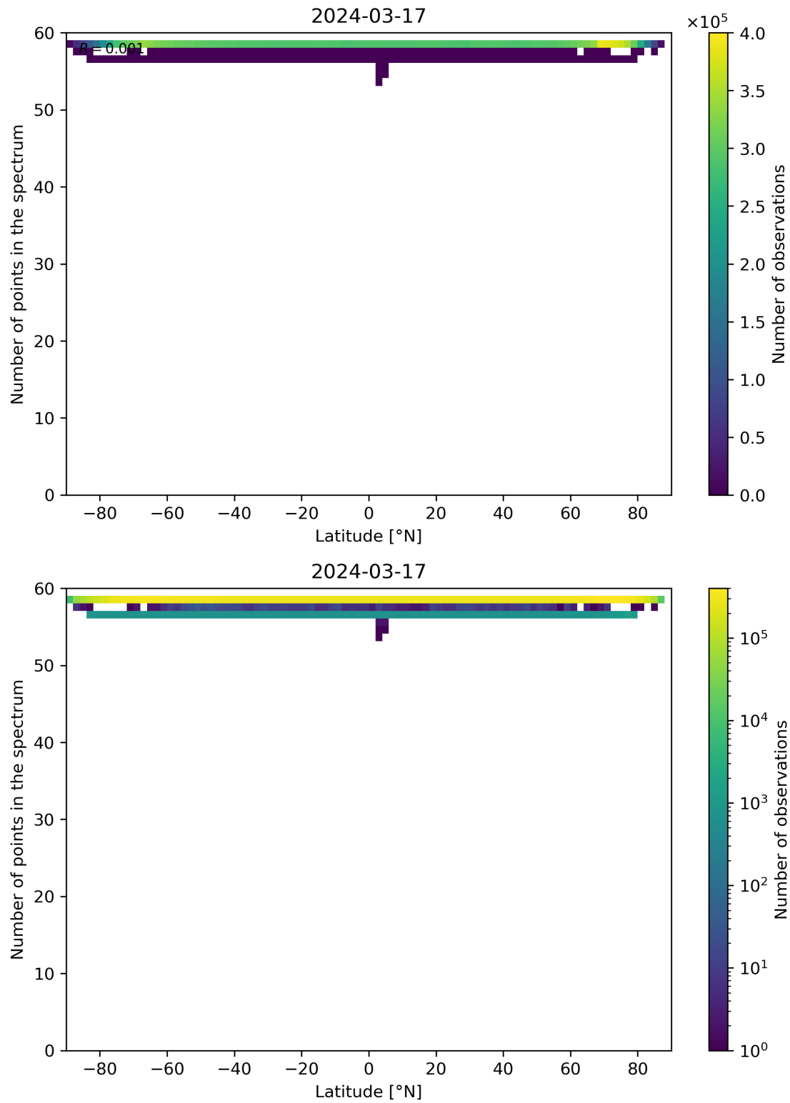
Figure 94: Scatter density plot of “Latitude” against “Number of points in the spectrum” for 2024-03-16 to 2024-03-18.
