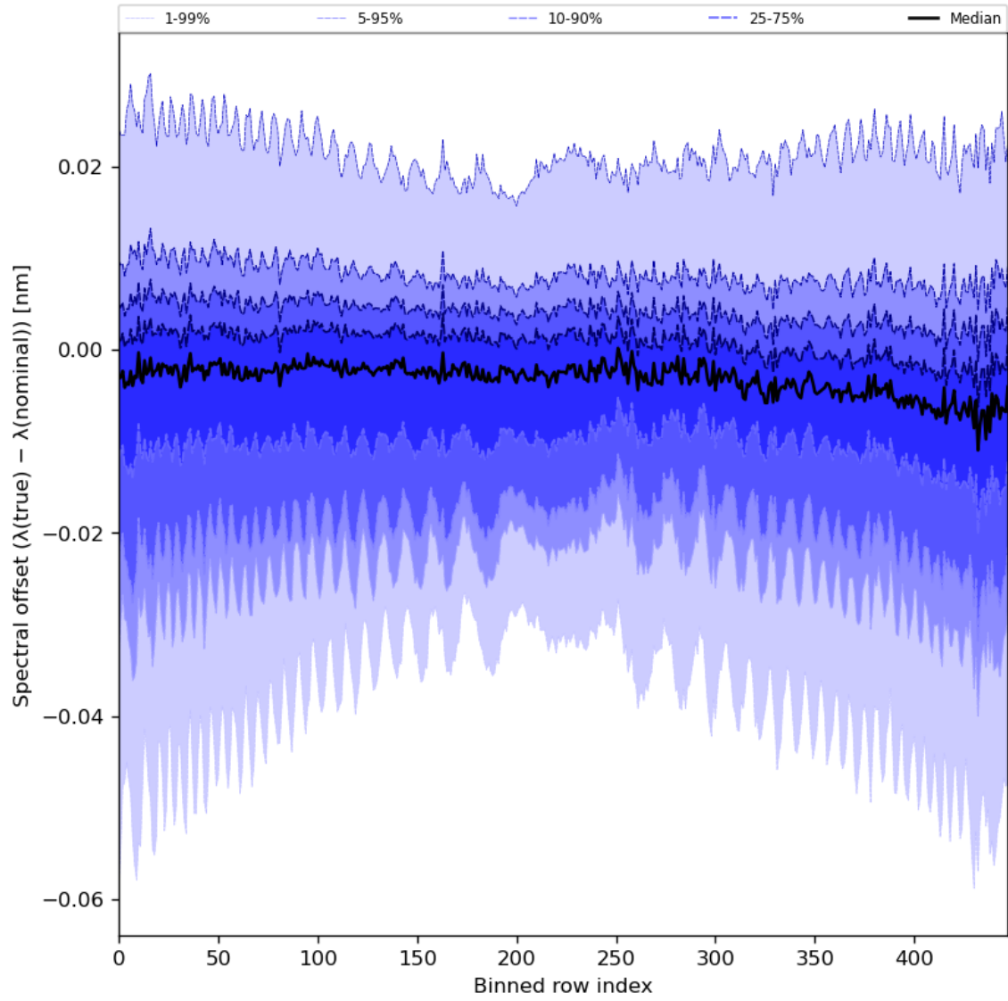
Figure 62: Along track statistics of “Spectral offset ( \lambda(\text{true}) - \lambda(\text{nominal}) )” for 2024-03-16 to 2024-03-18
