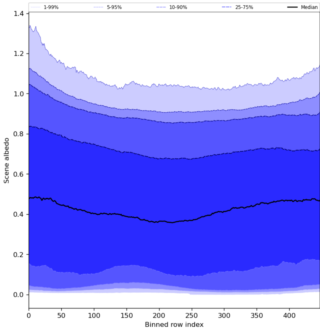
Figure 51: Along track statistics of “Scene albedo” for 2024-03-16 to 2024-03-18
