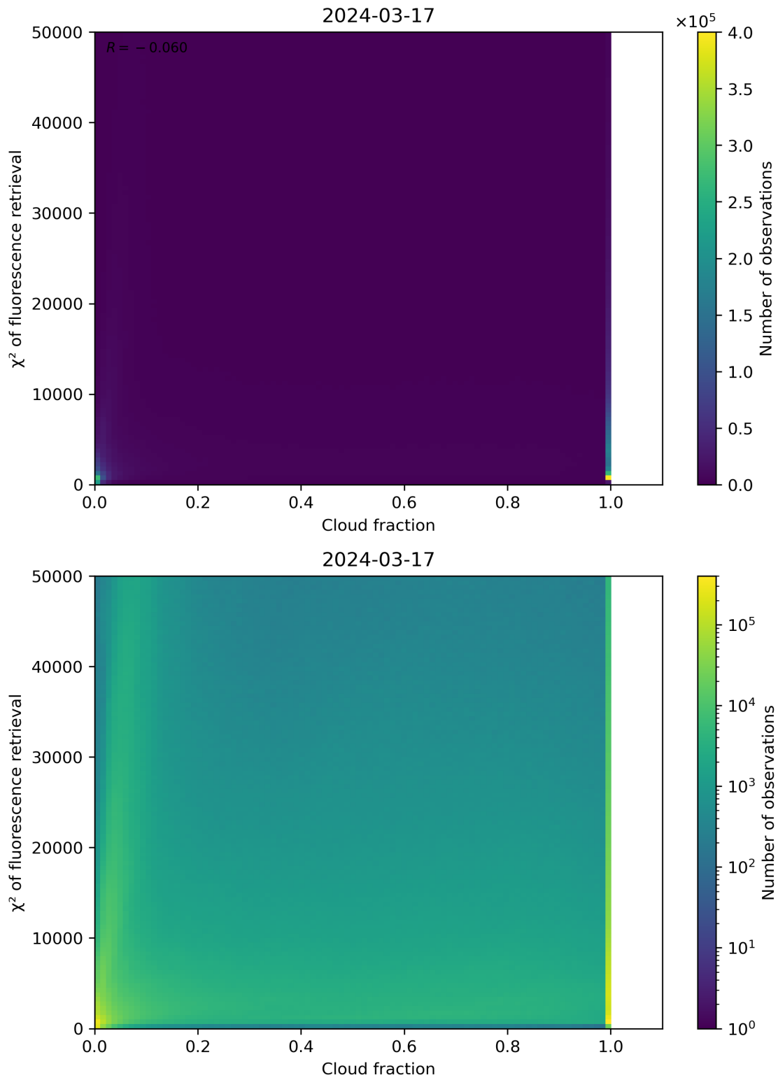
Figure 71: Scatter density plot of “Cloud fraction” against “ \chi^2 of fluorescence retrieval” for 2024-03-16 to 2024-03-18.
