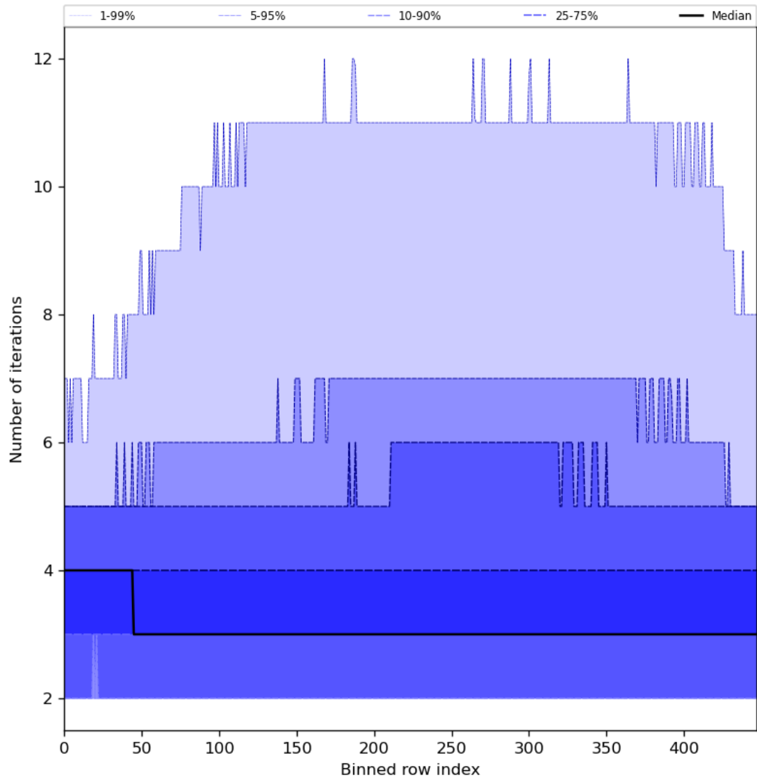
Figure 56: Along track statistics of “Number of iterations” for 2024-03-16 to 2024-03-18
