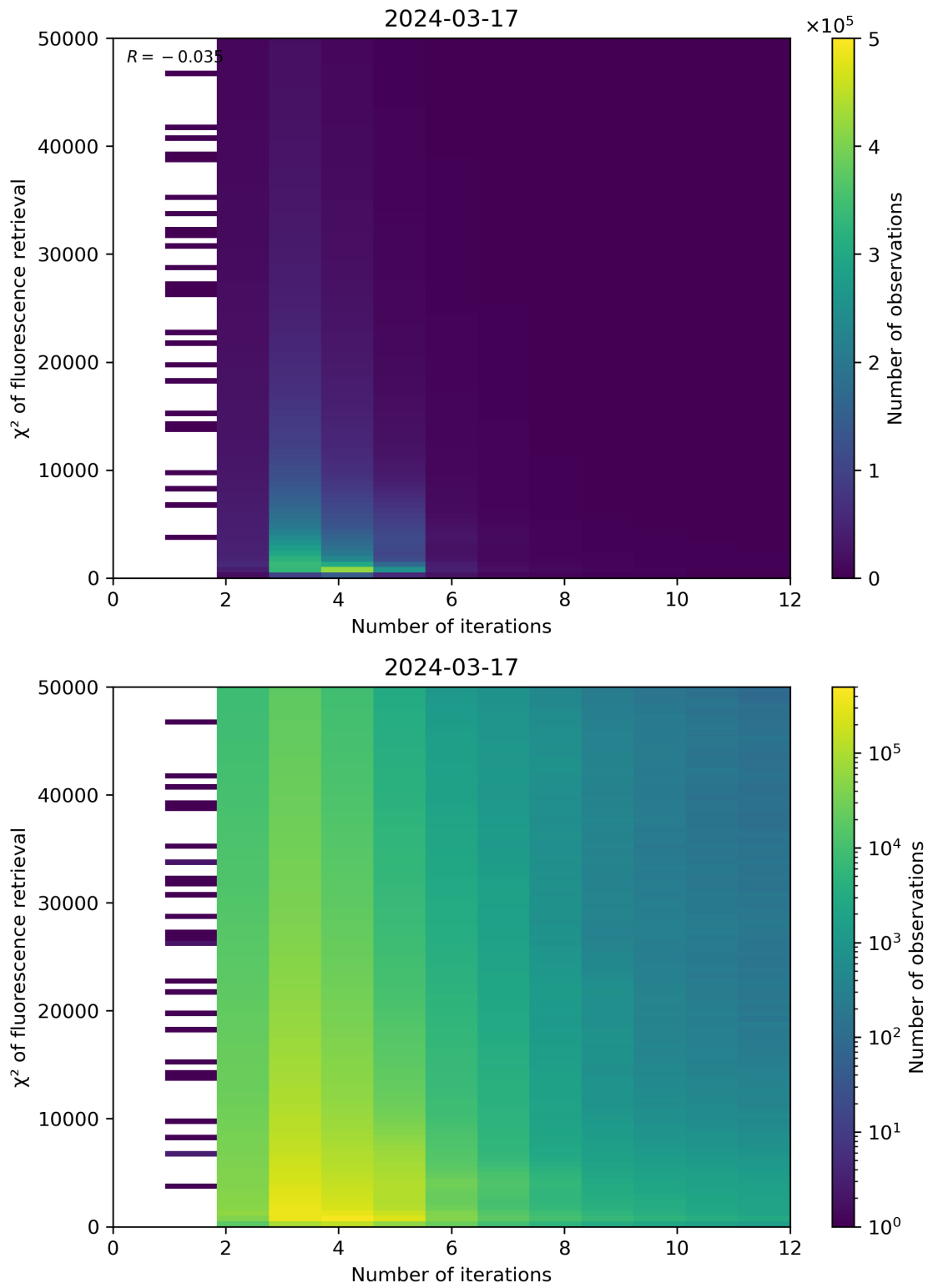
Figure 97: Scatter density plot of “Number of iterations” against “ \chi^2 of fluorescence retrieval” for 2024-03-16 to 2024-03-18.
