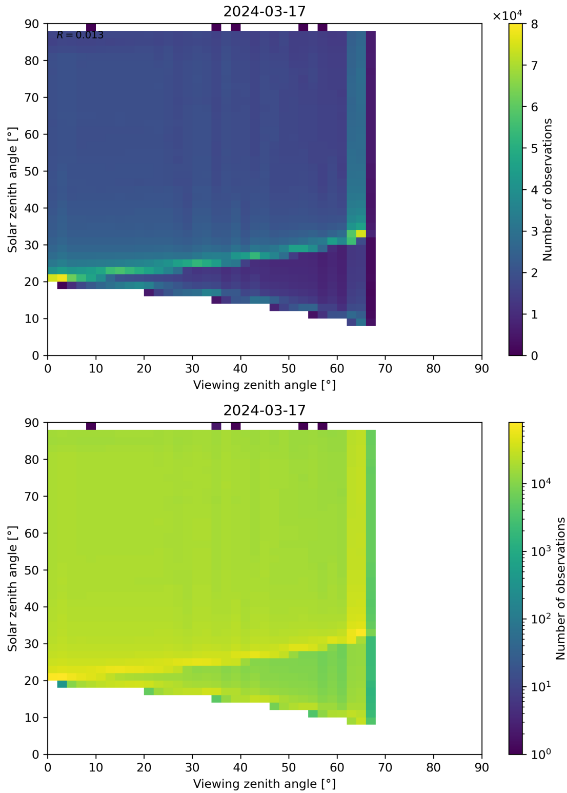
Figure 127: Scatter density plot of “Viewing zenith angle” against “Solar zenith angle” for 2024-03-16 to 2024-03-18.
