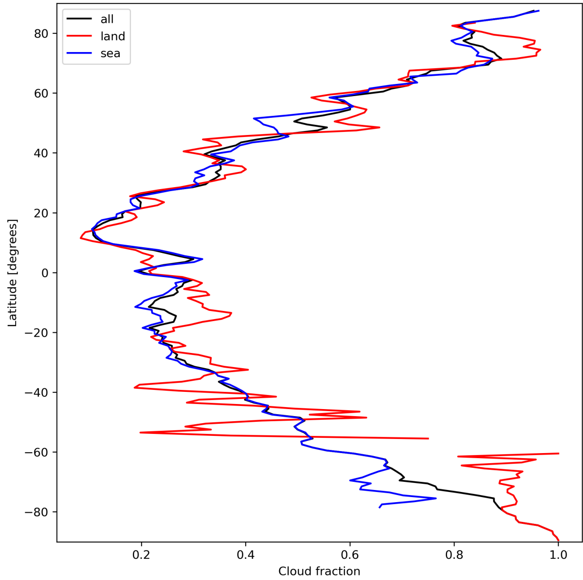
Figure 15: Zonal average of “Cloud fraction” for 2024-03-16 to 2024-03-18.
