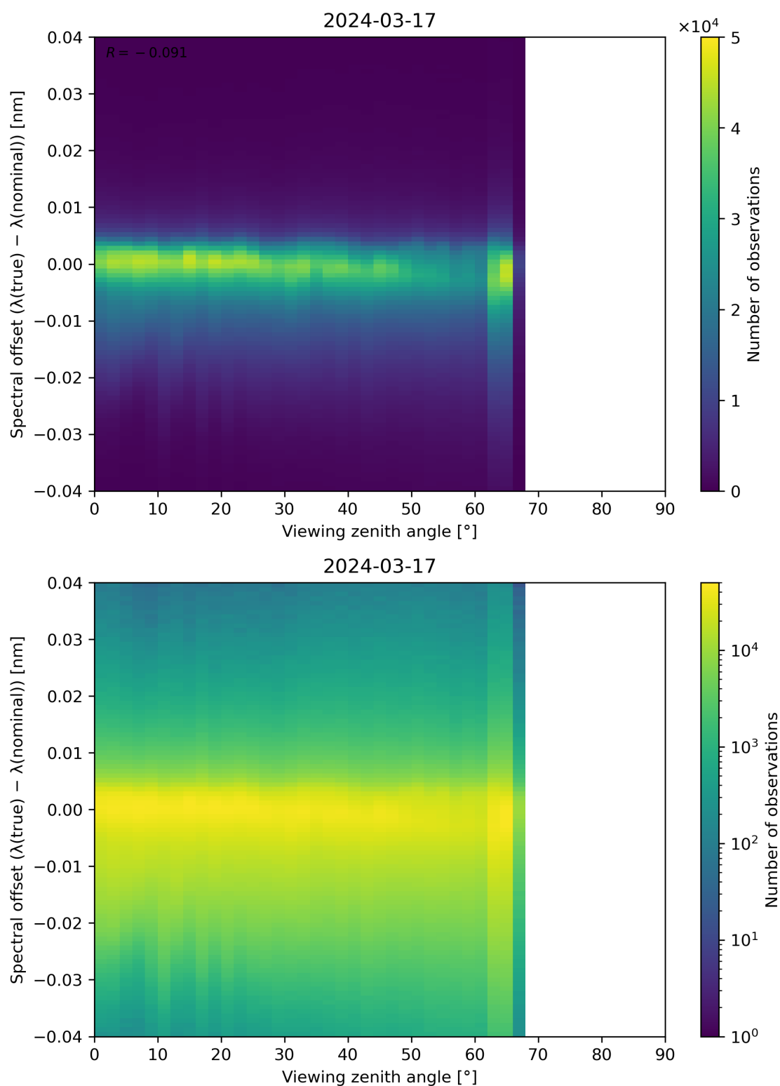
Figure 128: Scatter density plot of “Viewing zenith angle” against “Spectral offset ( \lambda(\text{true}) - \lambda(\text{nominal}) )” for 2024-03-16 to 2024-03-18.
