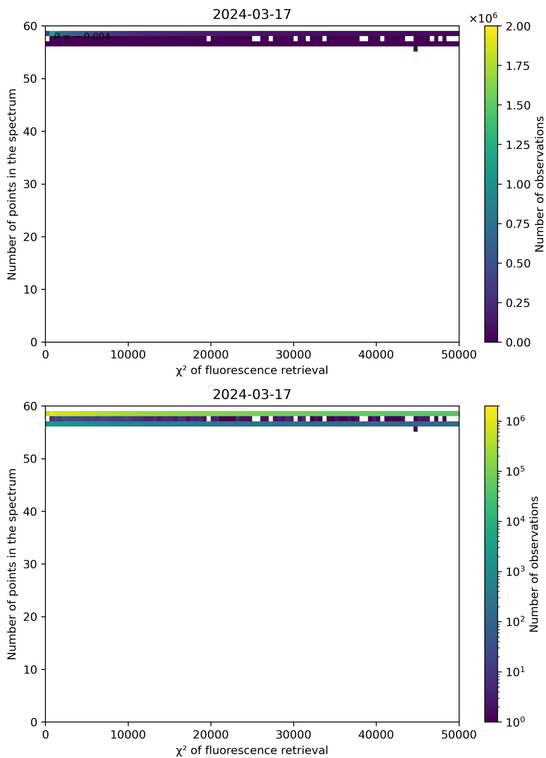
Figure 68: Scatter density plot of “ \chi^2 of fluorescence retrieval” against “Number of points in the spectrum” for 2024-03-16 to 2024-03-18.
