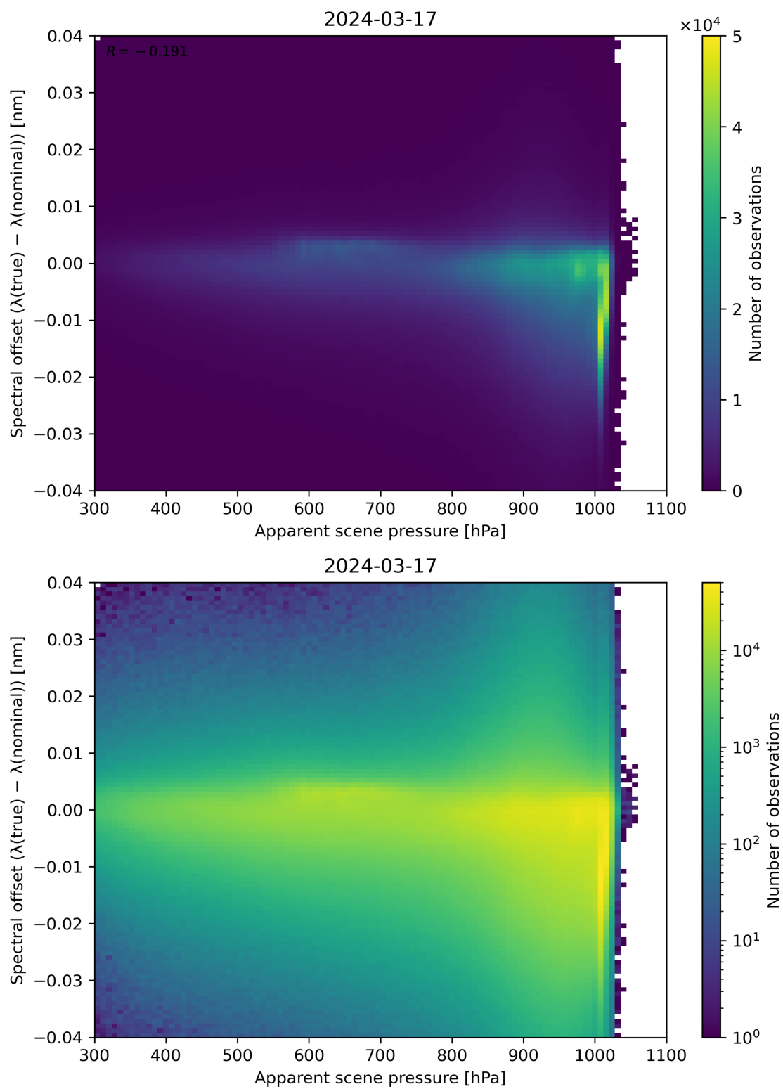
Figure 67: Scatter density plot of “Apparent scene pressure” against “Spectral offset ( \lambda(\text{true}) - \lambda(\text{nominal}) )” for 2024-03-16 to 2024-03-18.
