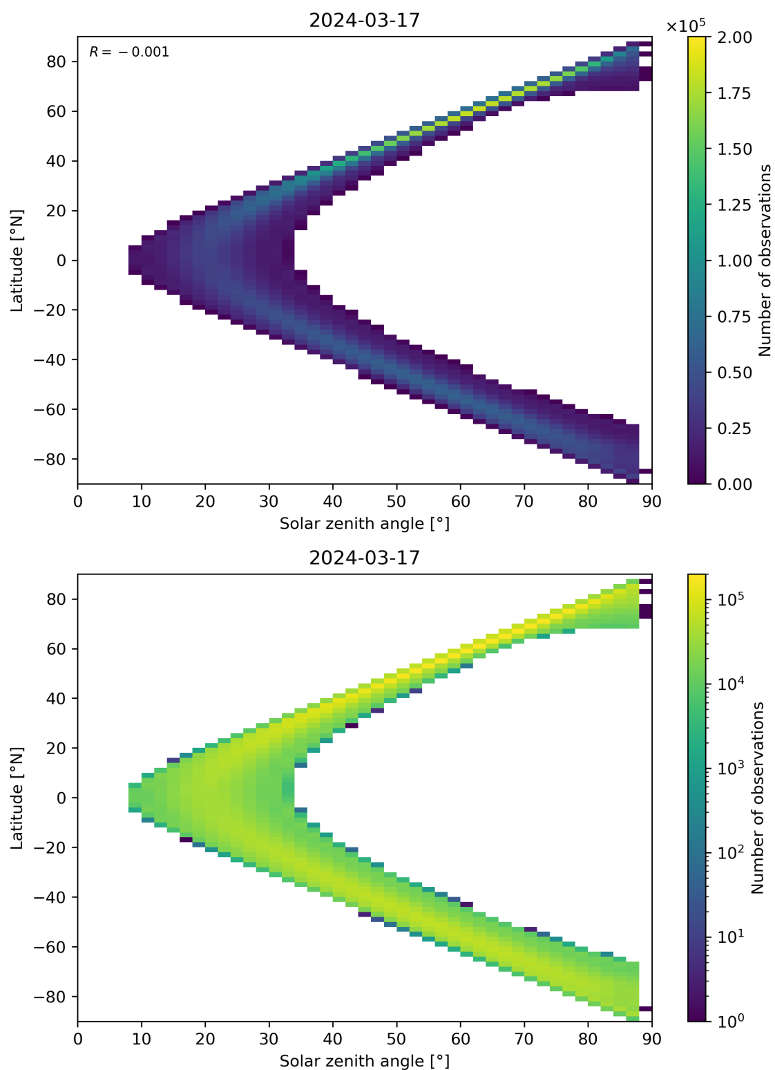
Figure 113: Scatter density plot of “Solar zenith angle” against “Latitude” for 2024-03-16 to 2024-03-18.
