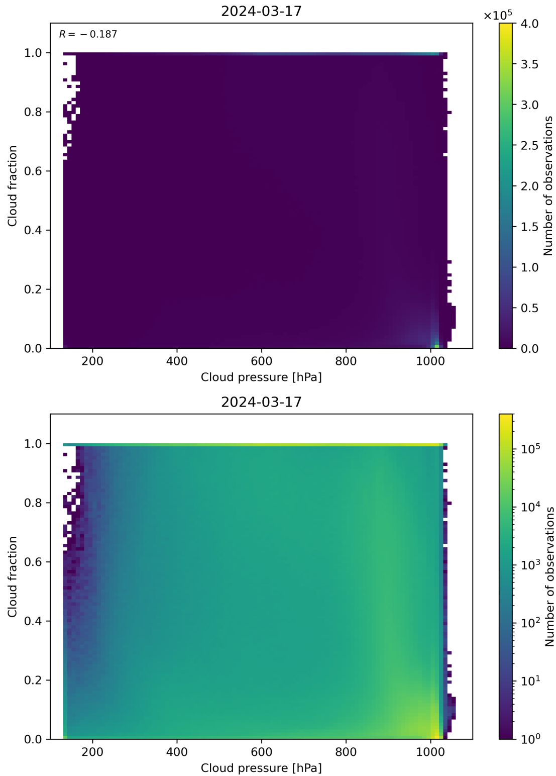
Figure 79: Scatter density plot of “Cloud pressure” against “Cloud fraction” for 2024-03-16 to 2024-03-18.
