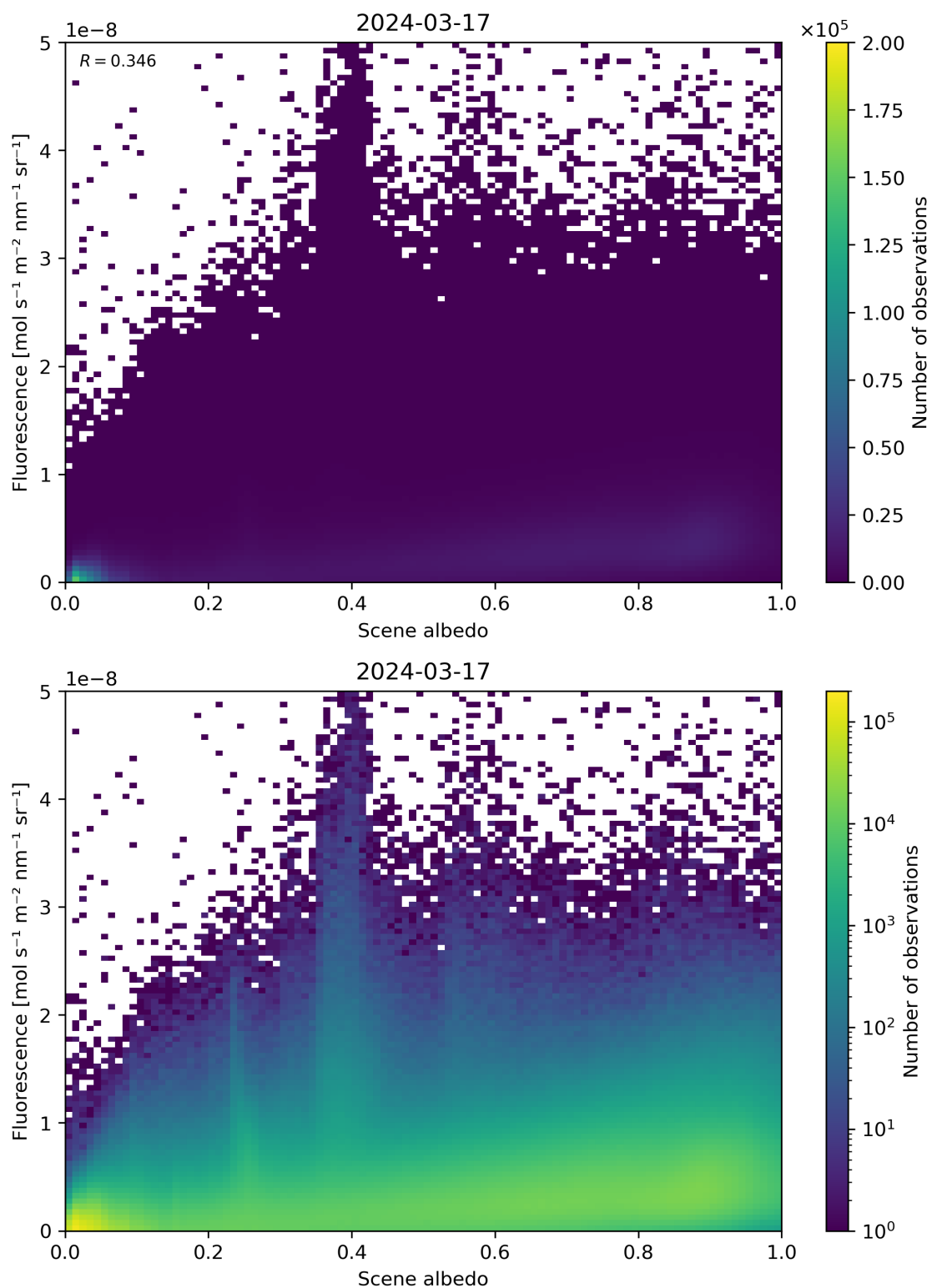
Figure 104: Scatter density plot of “Scene albedo” against “Fluorescence” for 2024-03-16 to 2024-03-18.
