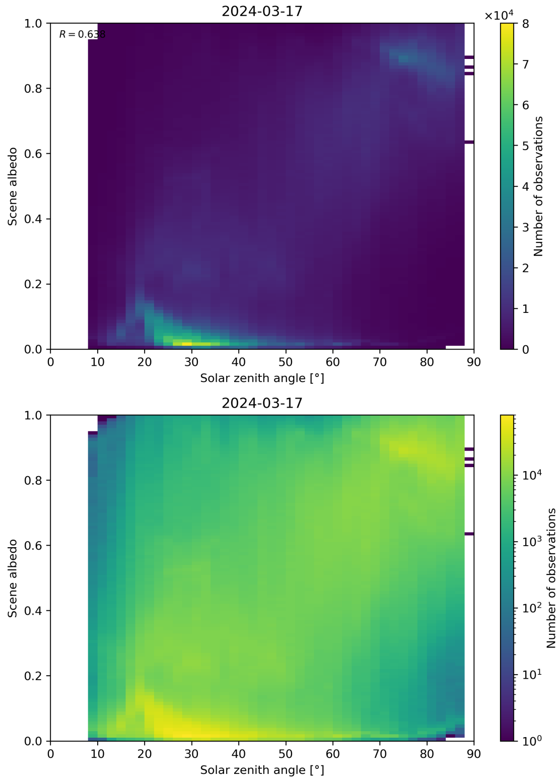
Figure 116: Scatter density plot of “Solar zenith angle” against “Scene albedo” for 2024-03-16 to 2024-03-18.
