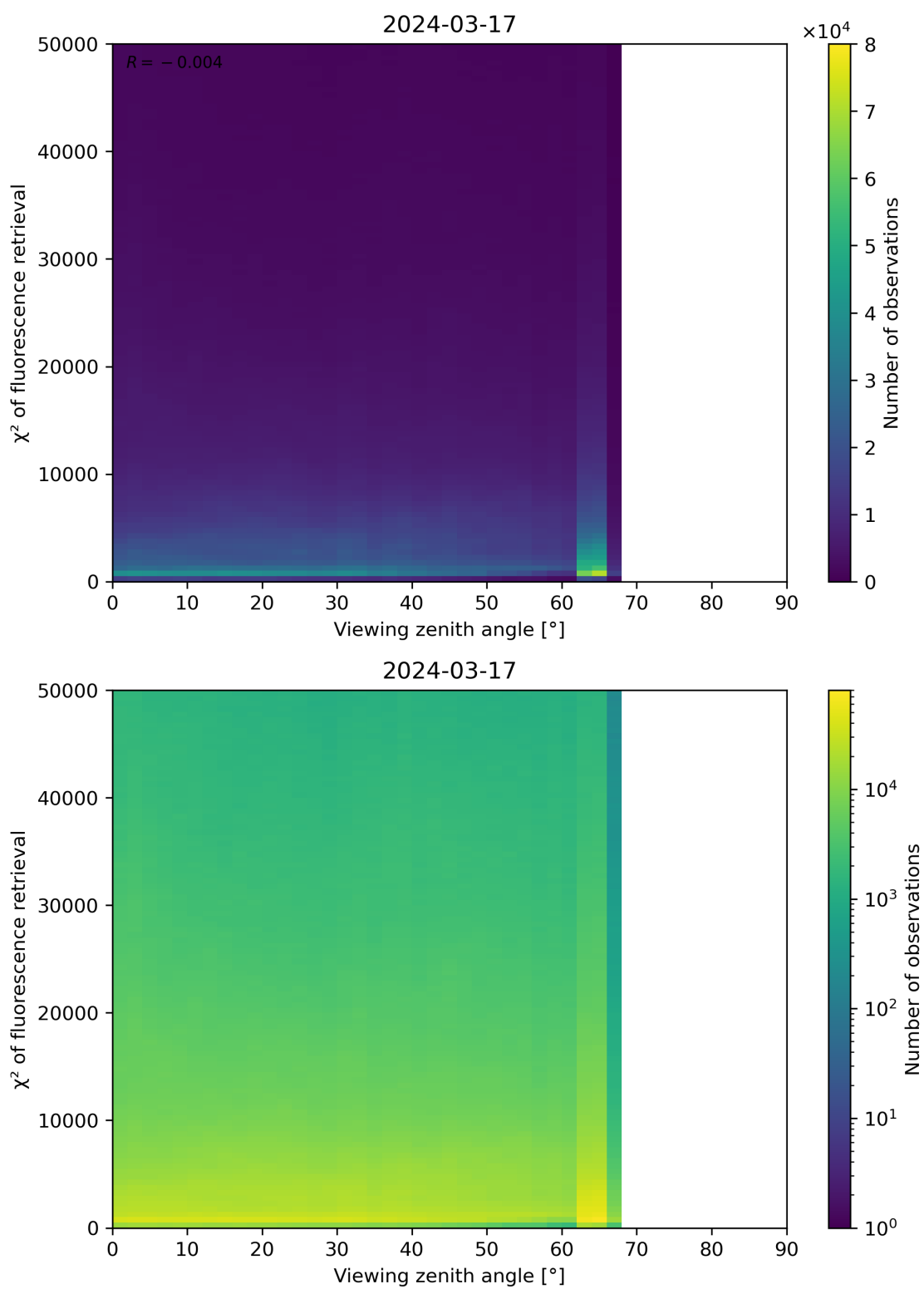
Figure 119: Scatter density plot of “Viewing zenith angle” against “ \chi^2 of fluorescence retrieval” for 2024-03-16 to 2024-03-18.
