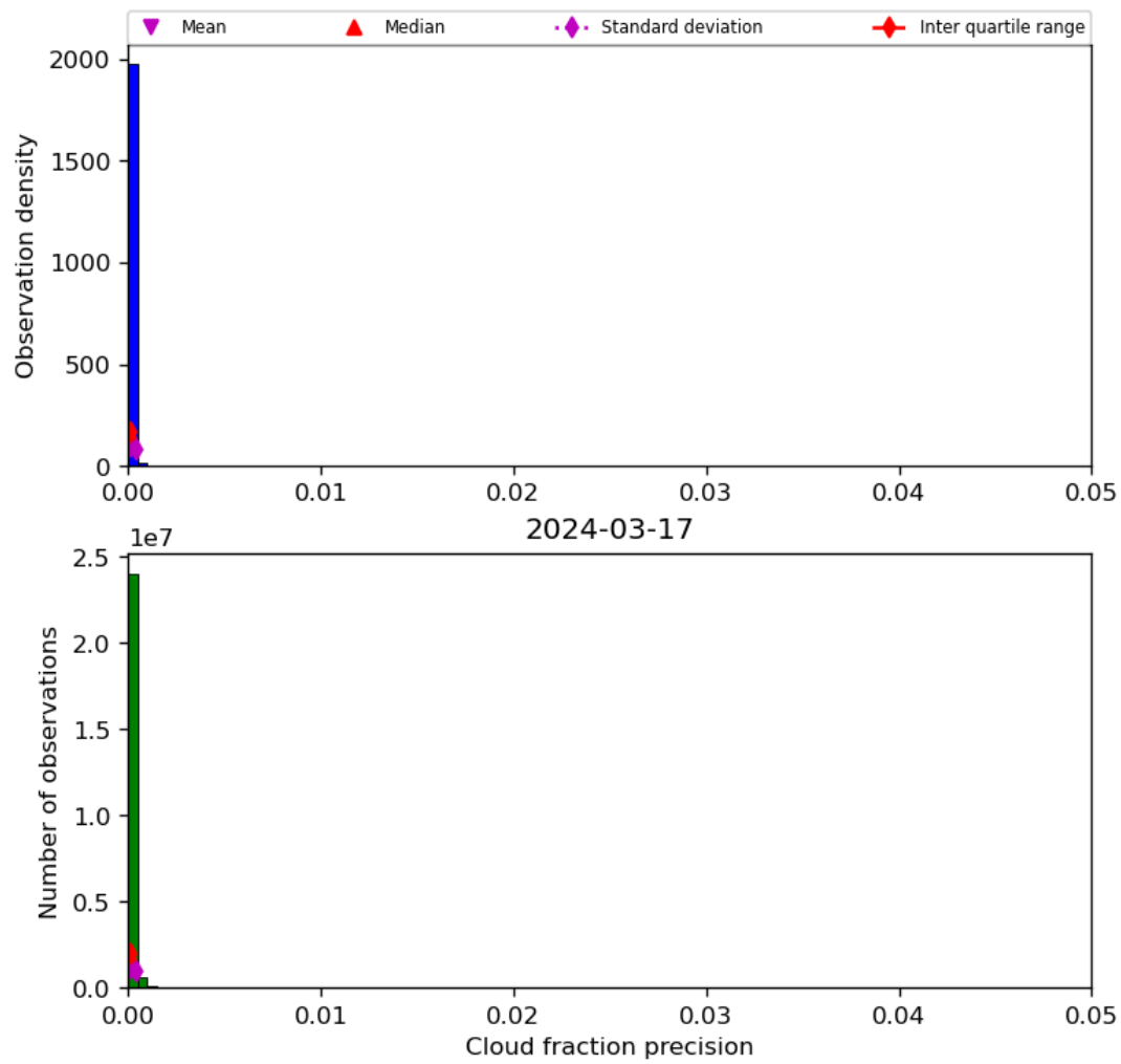
Figure 33: Histogram of “Cloud fraction precision” for 2024-03-16 to 2024-03-18
