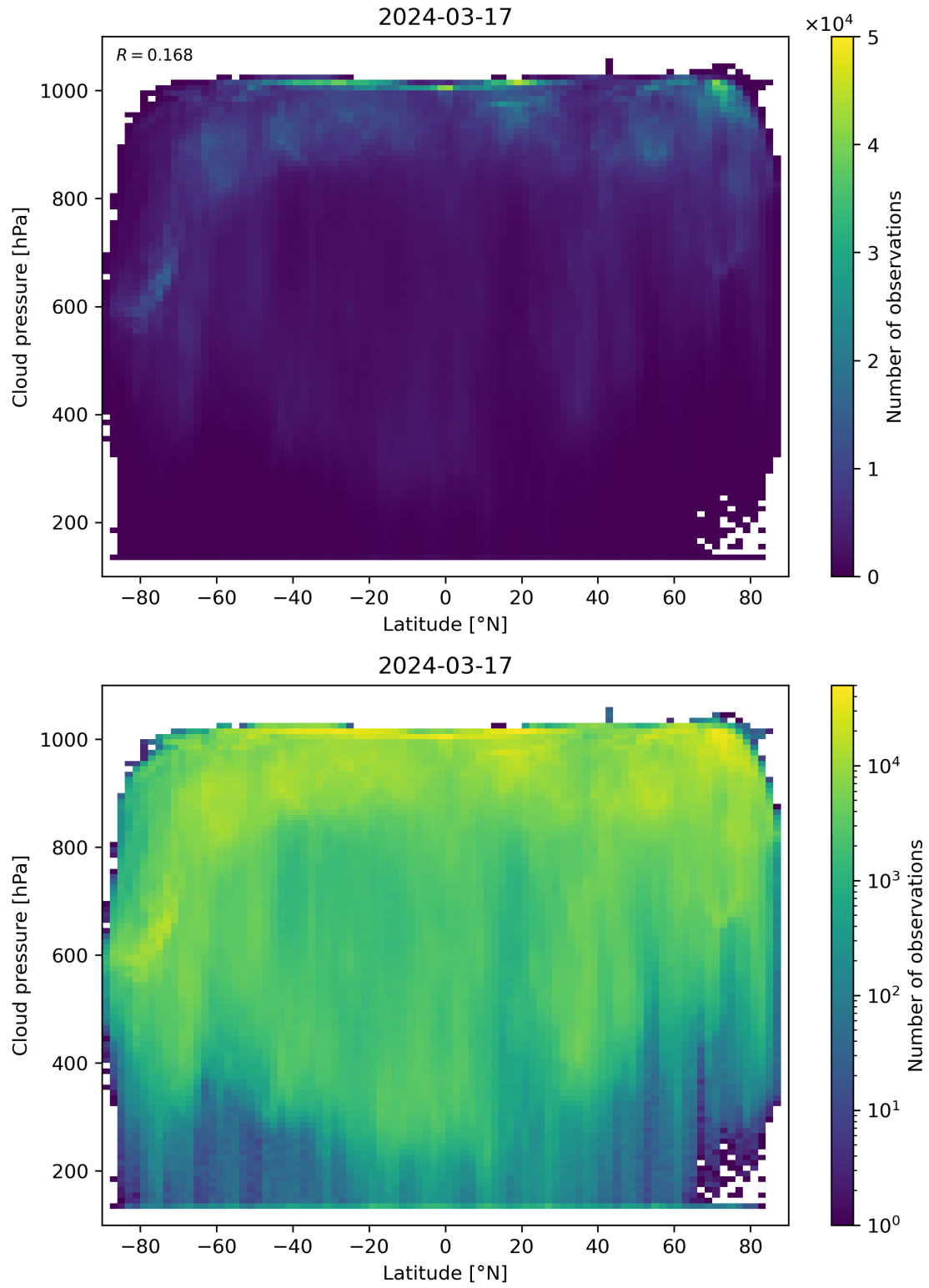
Figure 91: Scatter density plot of “Latitude” against “Cloud pressure” for 2024-03-16 to 2024-03-18.
