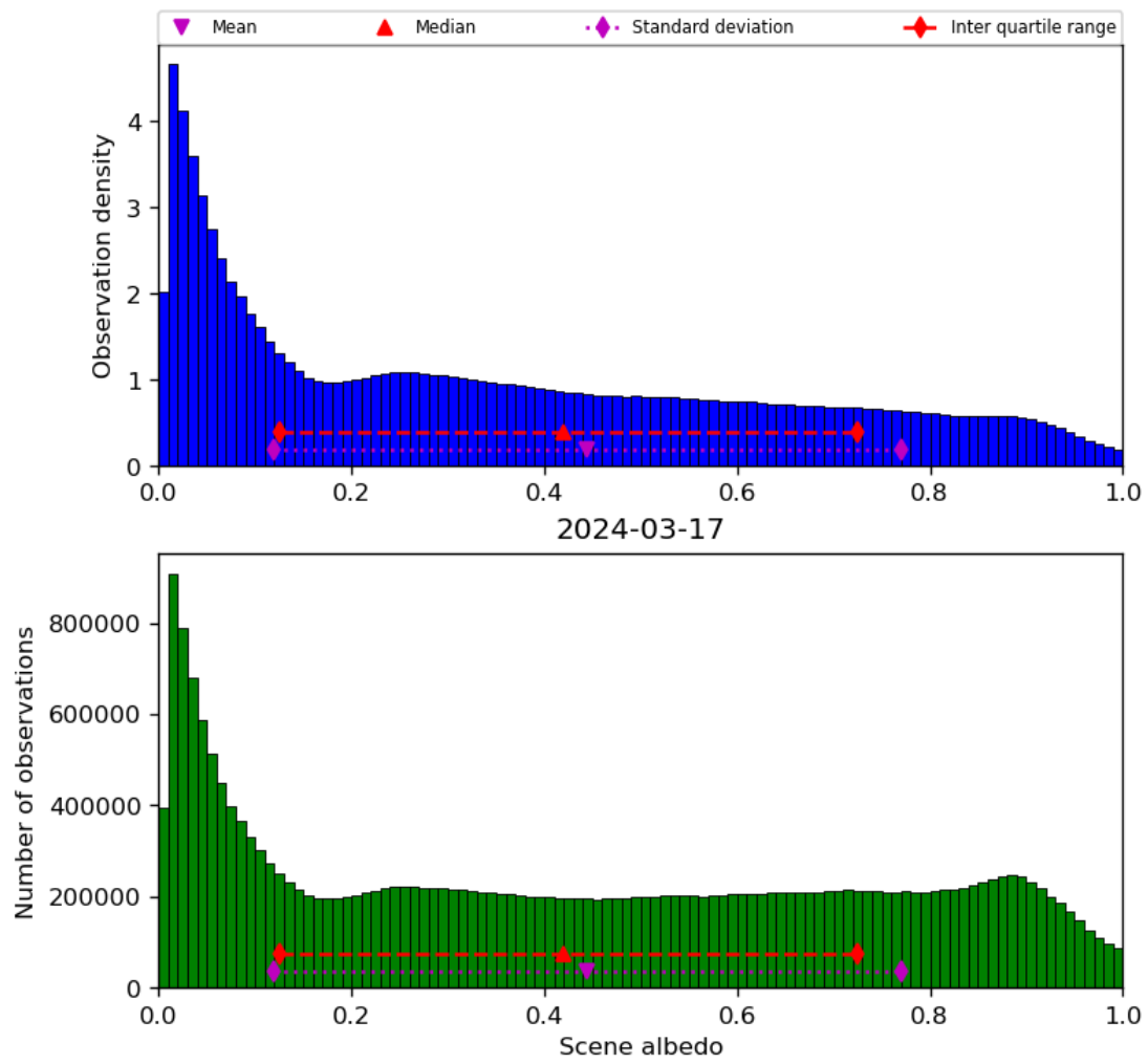
Figure 34: Histogram of “Scene albedo” for 2024-03-16 to 2024-03-18
