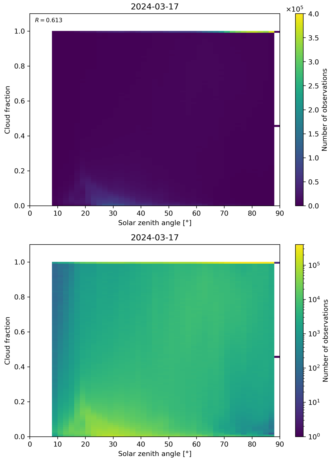
Figure 110: Scatter density plot of “Solar zenith angle” against “Cloud fraction” for 2024-03-16 to 2024-03-18.
