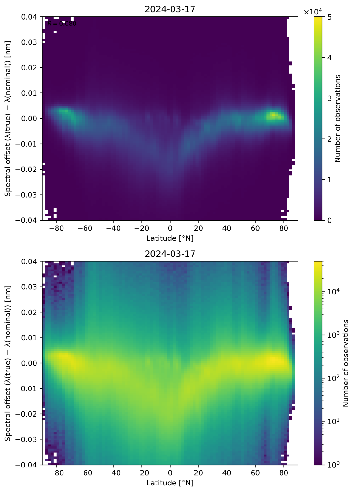
Figure 96: Scatter density plot of “Latitude” against “Spectral offset ( \lambda(\text{true}) - \lambda(\text{nominal}) )” for 2024-03-16 to 2024-03-18.
