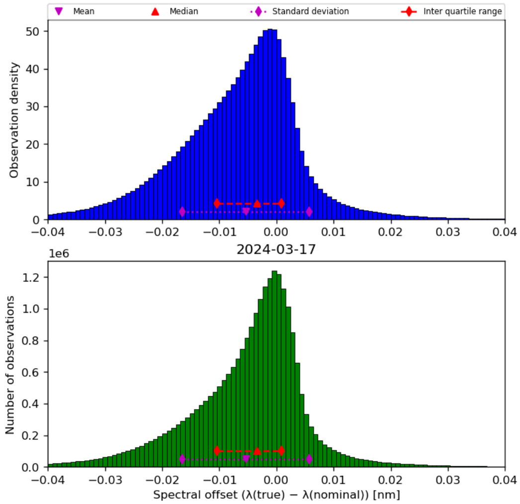
Figure 45: Histogram of “Spectral offset ( \lambda(\text{true}) - \lambda(\text{nominal}) )” for 2024-03-16 to 2024-03-18
