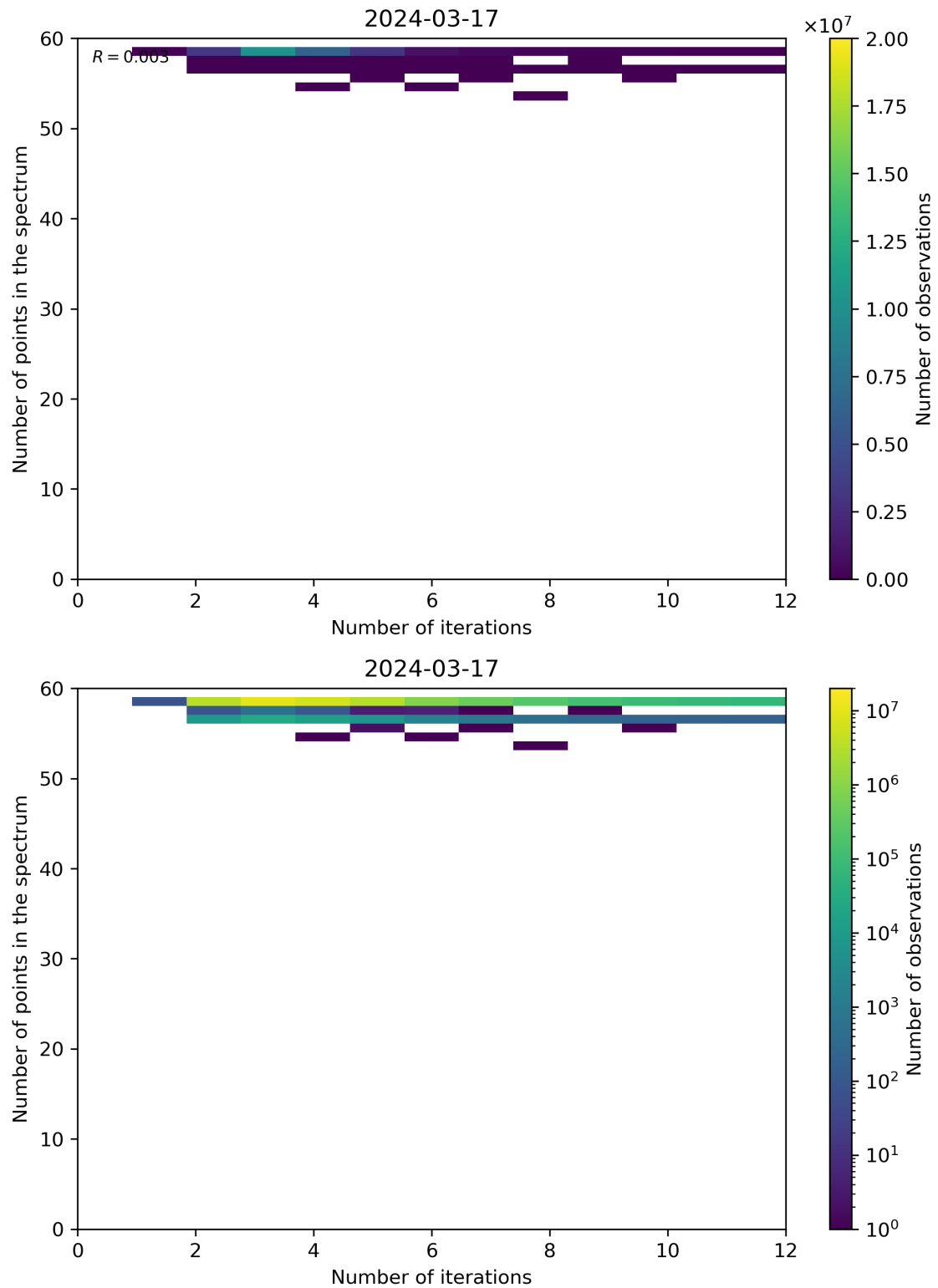
Figure 99: Scatter density plot of “Number of iterations” against “Number of points in the spectrum” for 2024-03-16 to 2024-03-18.
