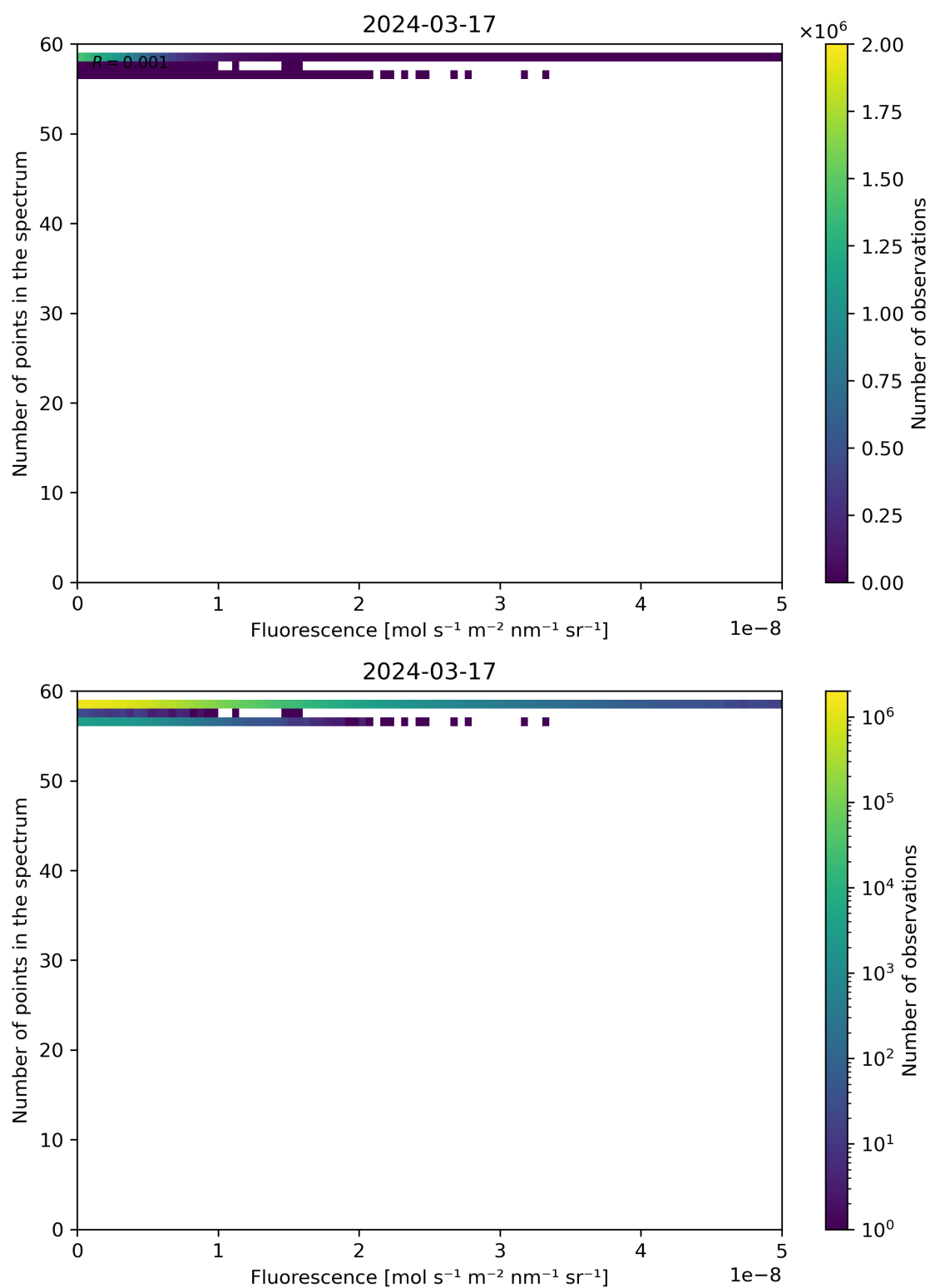
Figure 86: Scatter density plot of “Fluorescence” against “Number of points in the spectrum” for 2024-03-16 to 2024-03-18.
