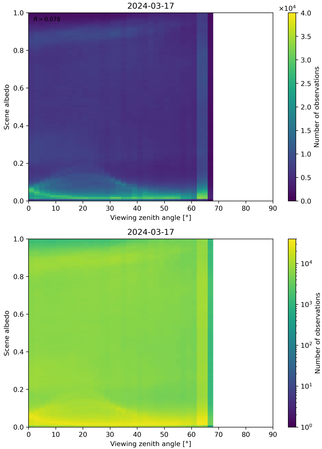
Figure 126: Scatter density plot of “Viewing zenith angle” against “Scene albedo” for 2024-03-16 to 2024-03-18.
