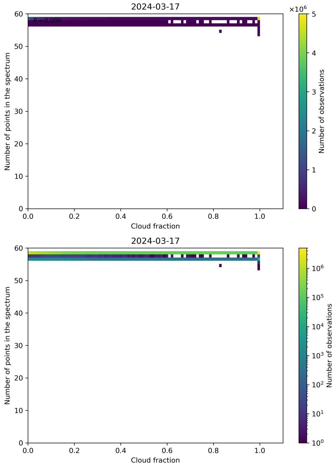
Figure 74: Scatter density plot of “Cloud fraction” against “Number of points in the spectrum” for 2024-03-16 to 2024-03-18.
