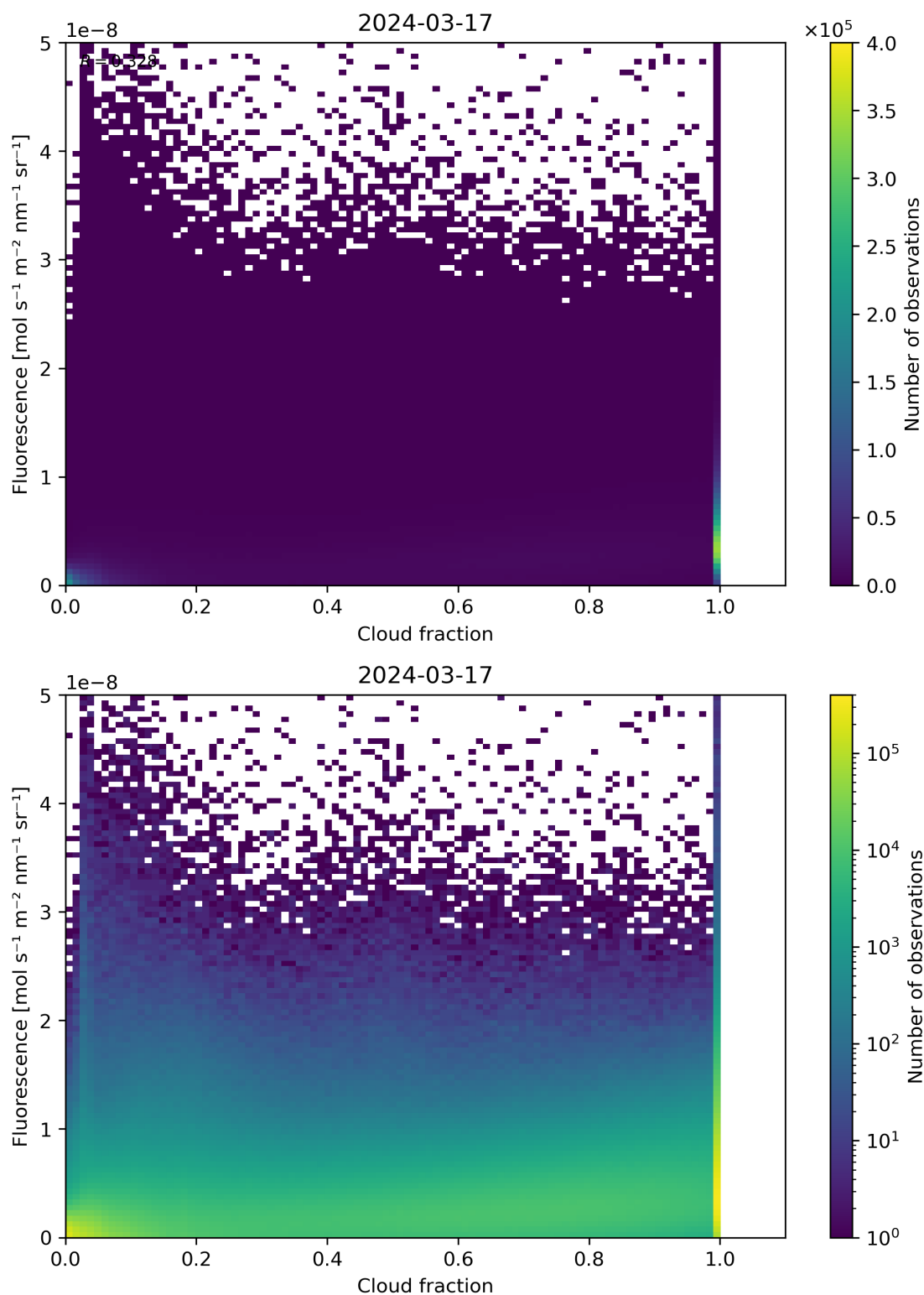
Figure 72: Scatter density plot of “Cloud fraction” against “Fluorescence” for 2024-03-16 to 2024-03-18.
