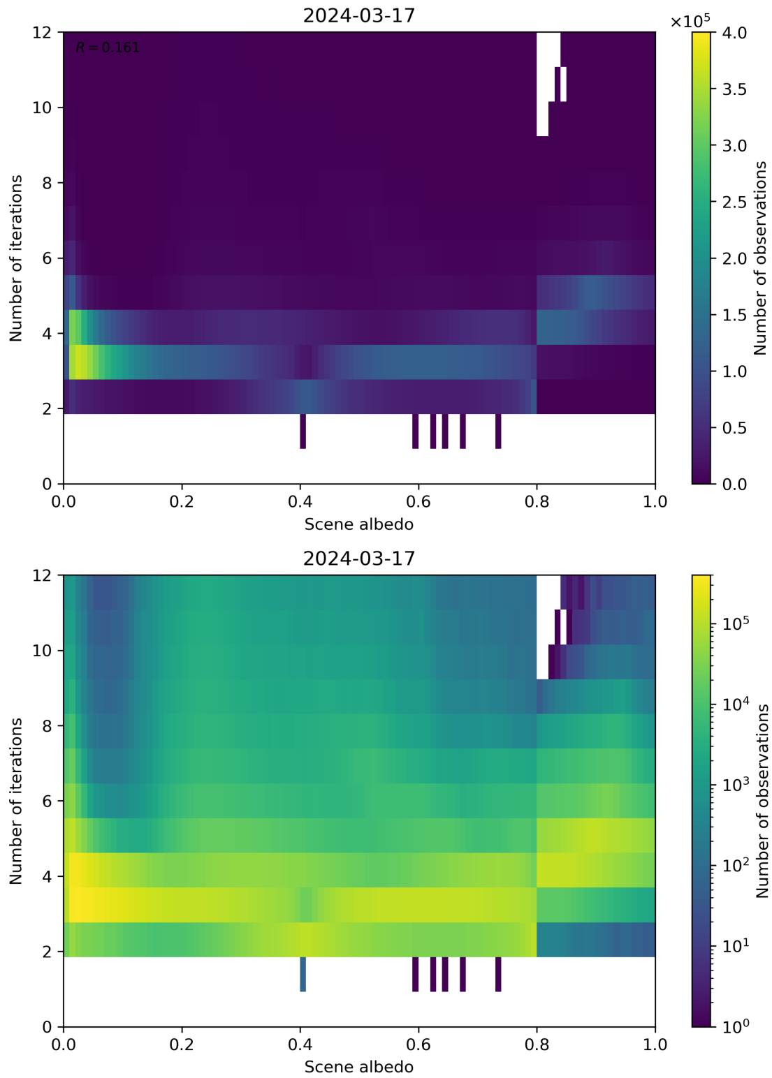
Figure 105: Scatter density plot of “Scene albedo” against “Number of iterations” for 2024-03-16 to 2024-03-18.
