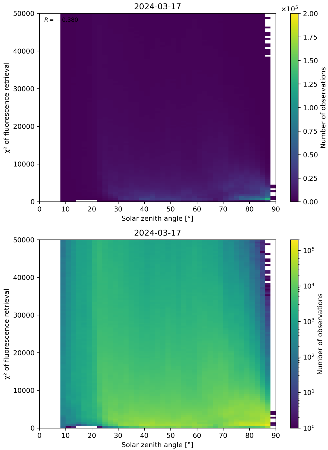
Figure 109: Scatter density plot of “Solar zenith angle” against “ \chi^2 of fluorescence retrieval” for 2024-03-16 to 2024-03-18.
