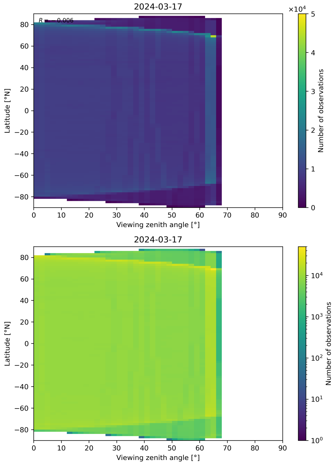
Figure 123: Scatter density plot of “Viewing zenith angle” against “Latitude” for 2024-03-16 to 2024-03-18.
