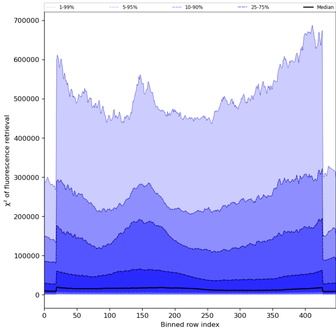
Figure 59: Along track statistics of “ \chi^2 of fluorescence retrieval” for 2024-03-16 to 2024-03-18
