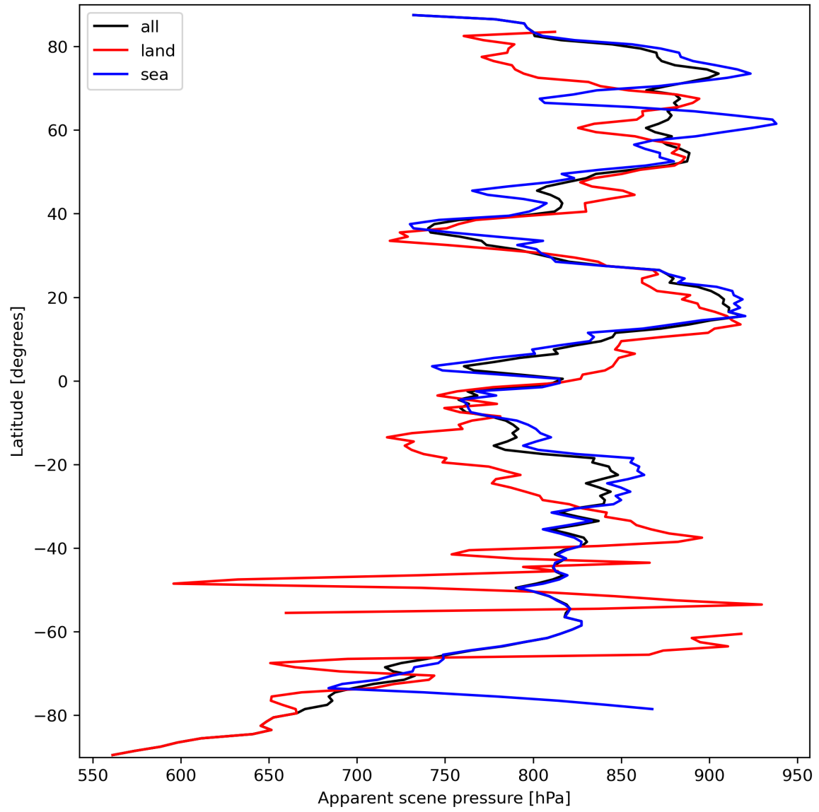
Figure 19: Zonal average of “Apparent scene pressure” for 2024-03-16 to 2024-03-18.
