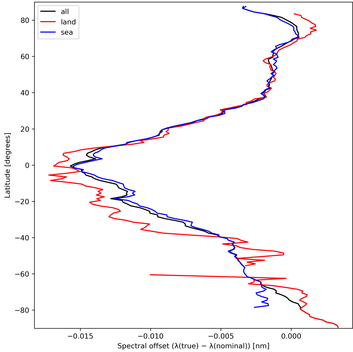
Figure 28: Zonal average of “Spectral offset ( \lambda(\text{true}) - \lambda(\text{nominal}) )” for 2024-03-16 to 2024-03-18.
