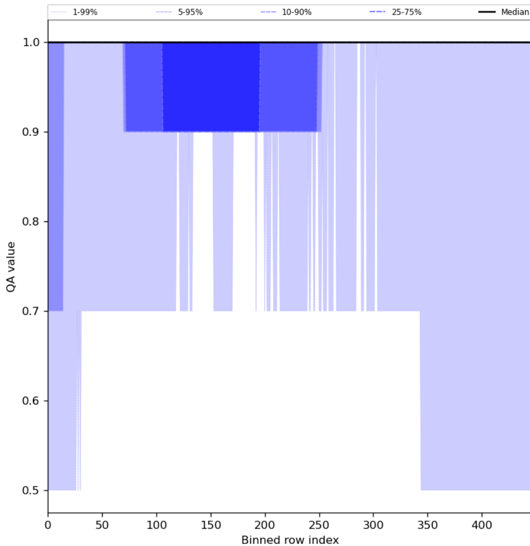
Figure 46: Along track statistics of “QA value” for 2024-03-16 to 2024-03-18
