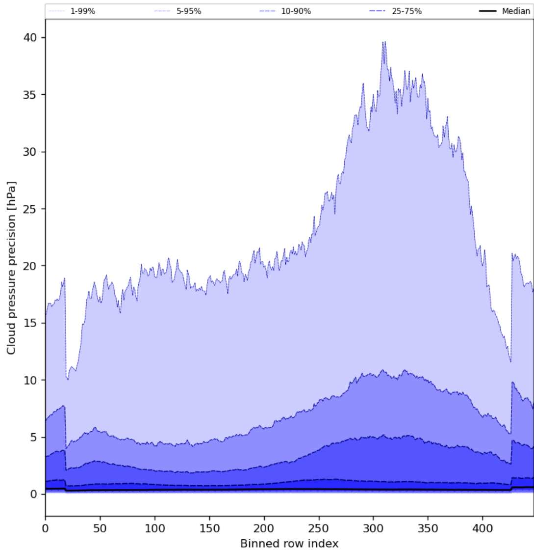
Figure 48: Along track statistics of “Cloud pressure precision” for 2024-03-16 to 2024-03-18
