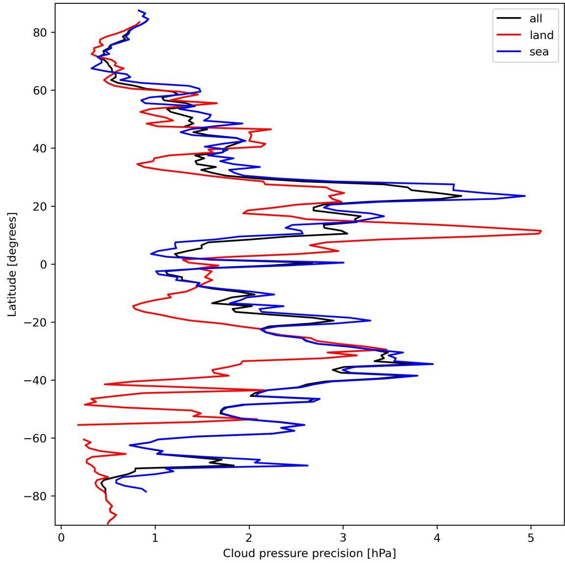
Figure 14: Zonal average of “Cloud pressure precision” for 2024-03-16 to 2024-03-18.
