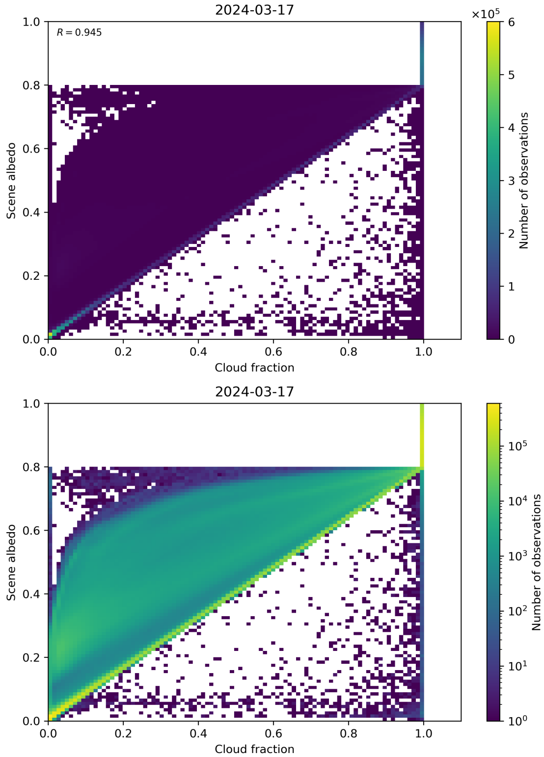
Figure 75: Scatter density plot of “Cloud fraction” against “Scene albedo” for 2024-03-16 to 2024-03-18.
