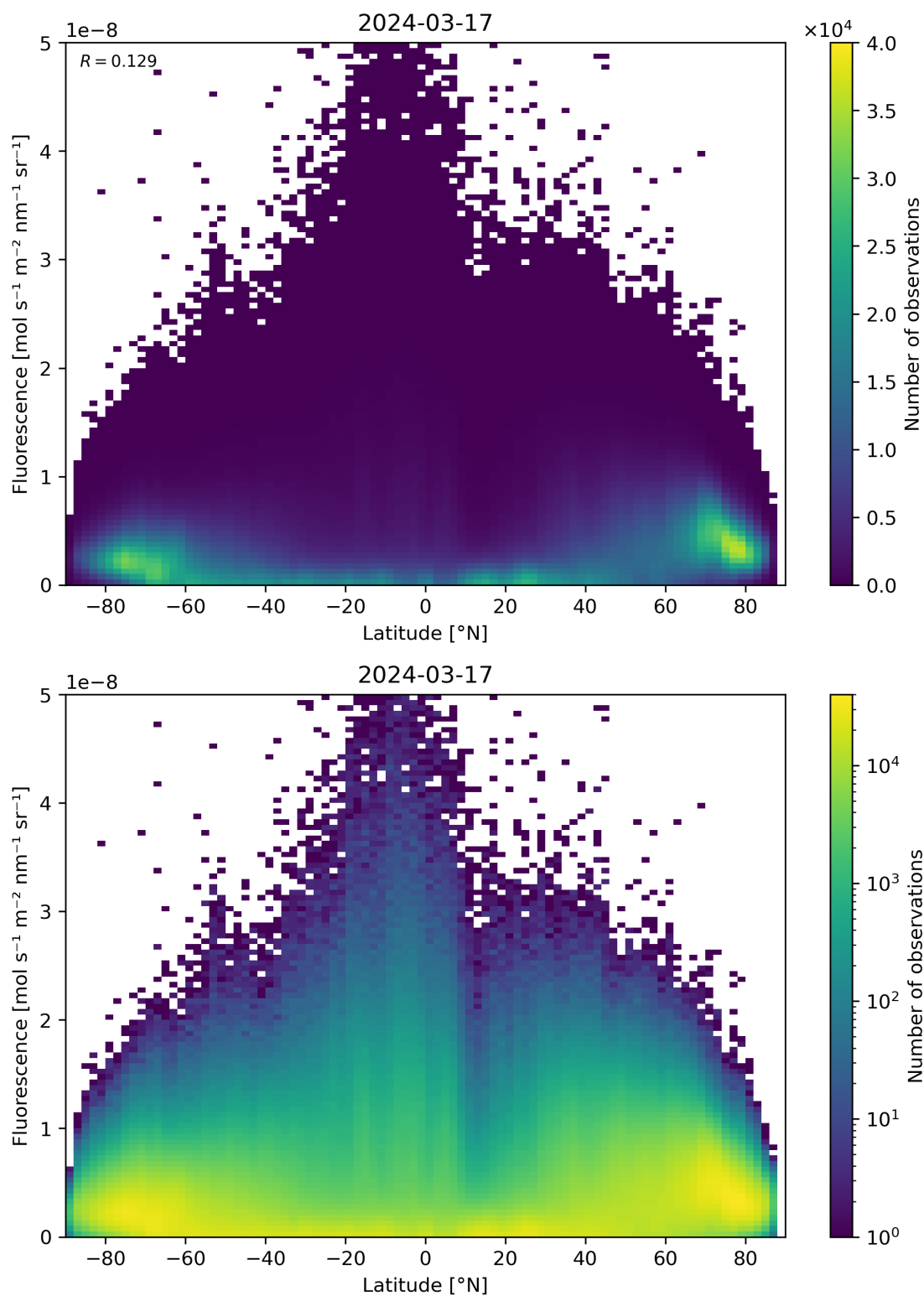
Figure 92: Scatter density plot of “Latitude” against “Fluorescence” for 2024-03-16 to 2024-03-18.
