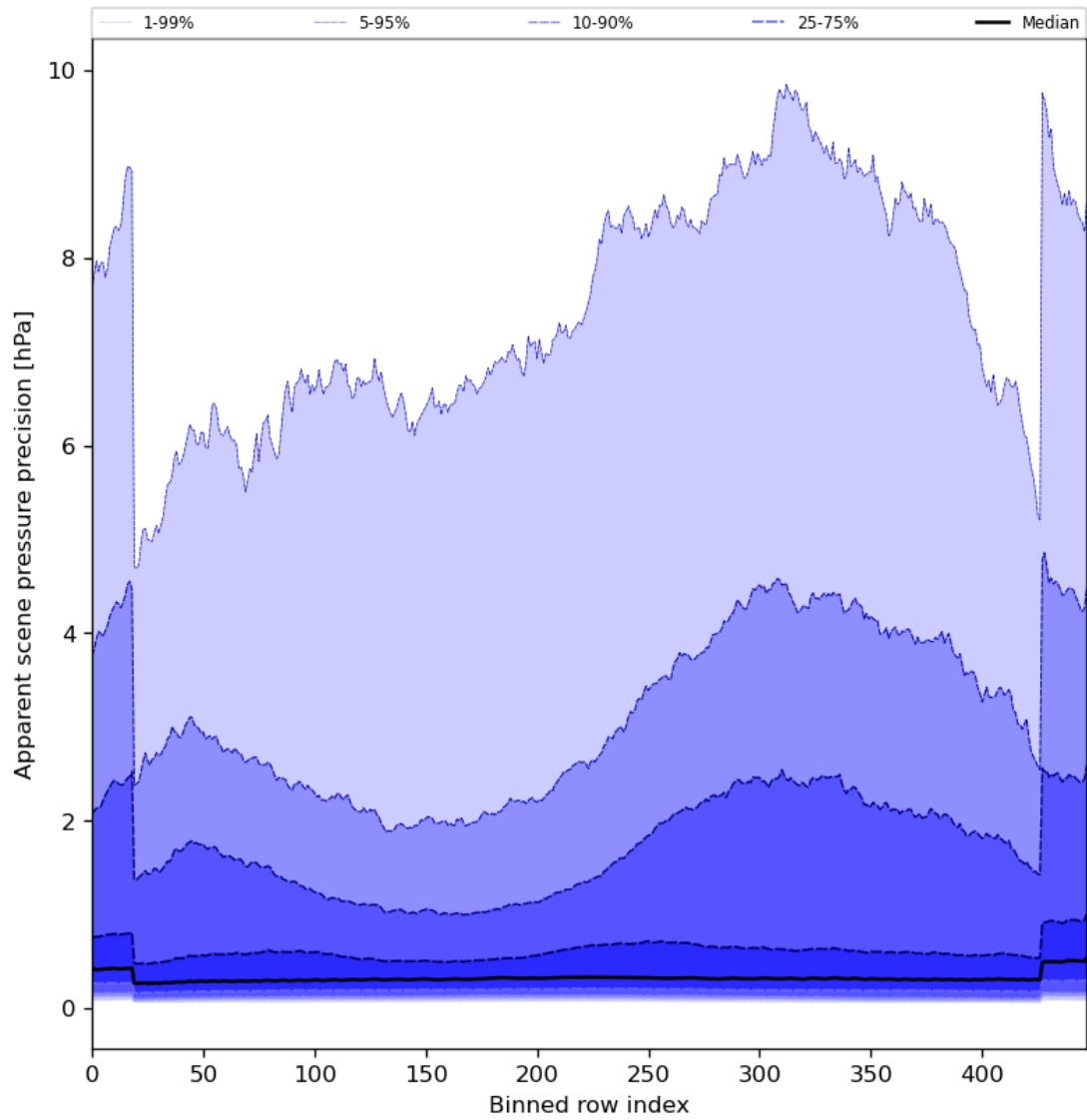
Figure 54: Along track statistics of “Apparent scene pressure precision” for 2024-03-16 to 2024-03-18
