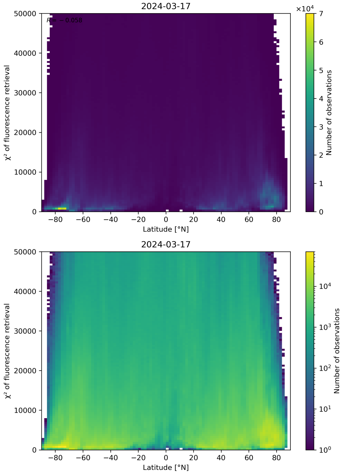
Figure 89: Scatter density plot of “Latitude” against “ \chi^2 of fluorescence retrieval” for 2024-03-16 to 2024-03-18.
