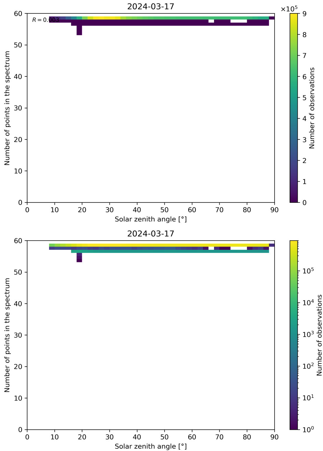
Figure 115: Scatter density plot of “Solar zenith angle” against “Number of points in the spectrum” for 2024-03-16 to 2024-03-18.
