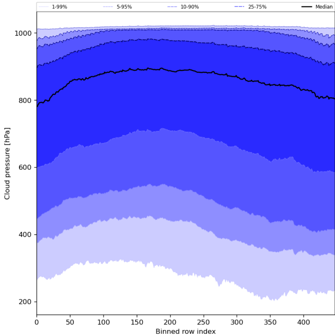
Figure 47: Along track statistics of “Cloud pressure” for 2024-03-16 to 2024-03-18
