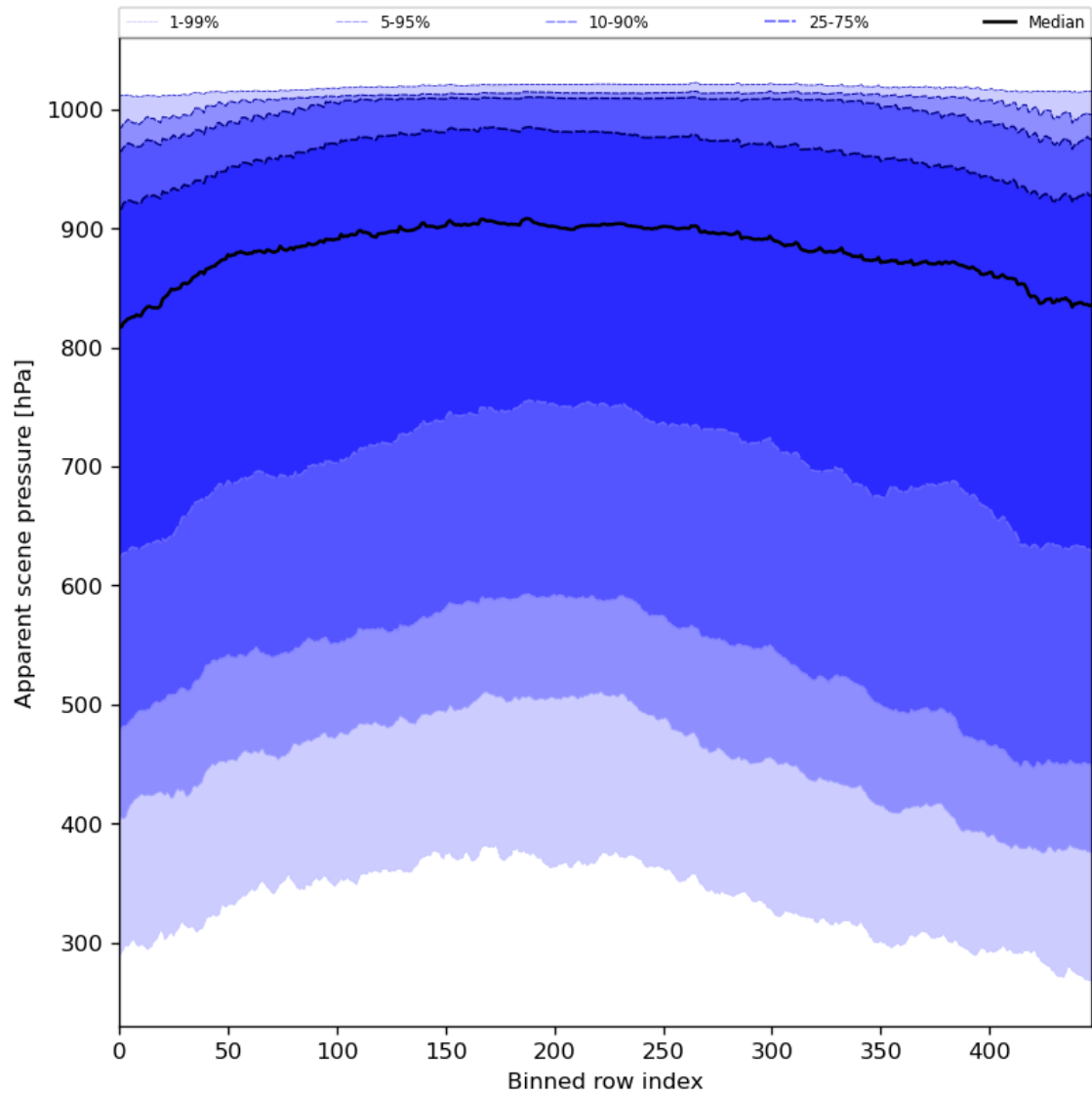
Figure 53: Along track statistics of “Apparent scene pressure” for 2024-03-16 to 2024-03-18
