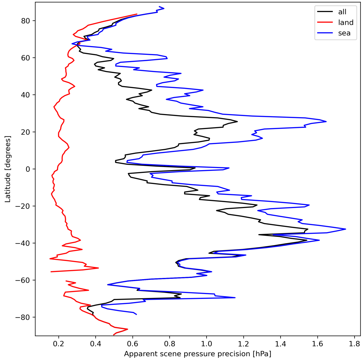
Figure 20: Zonal average of “Apparent scene pressure precision” for 2024-03-16 to 2024-03-18.
