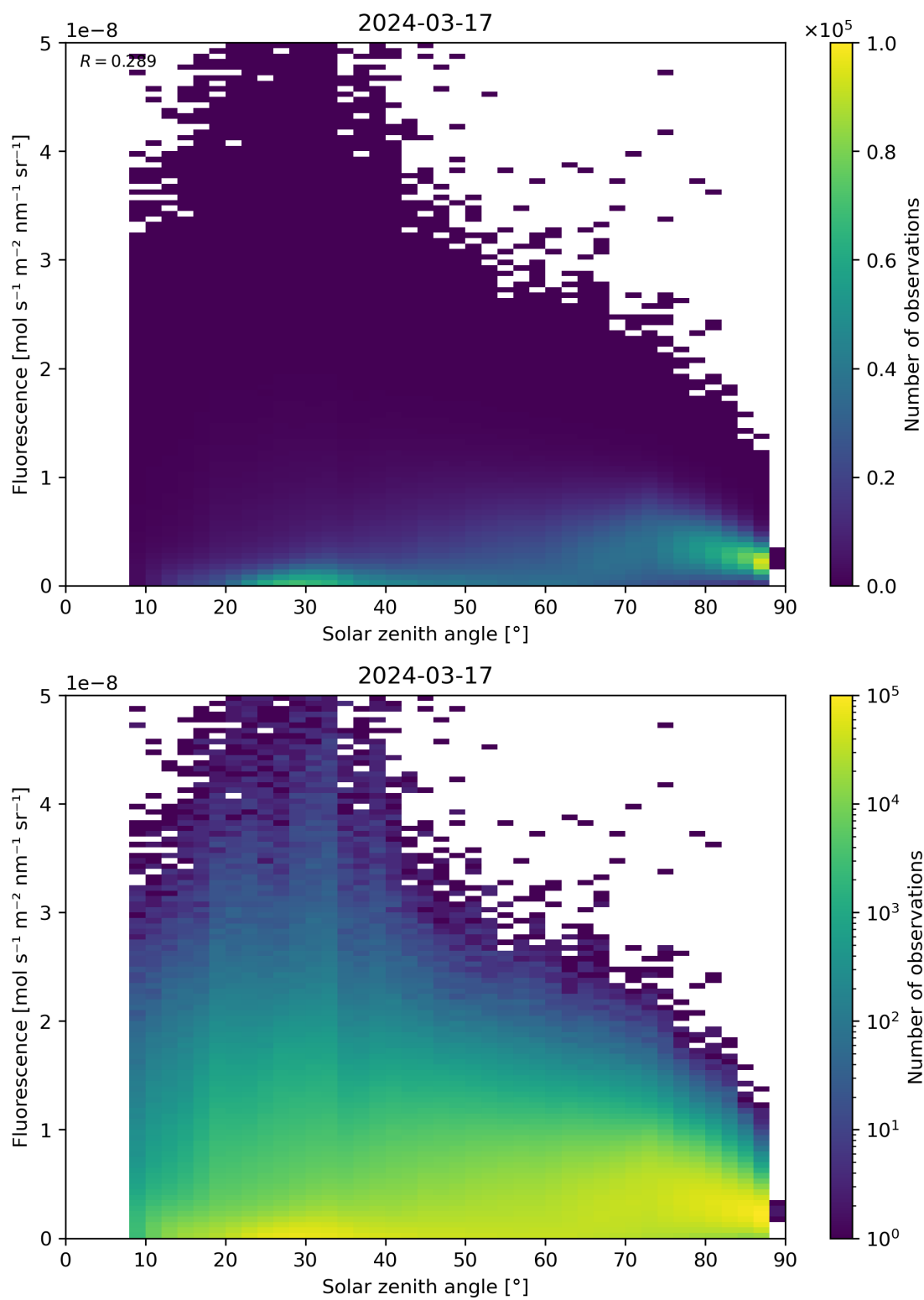
Figure 112: Scatter density plot of “Solar zenith angle” against “Fluorescence” for 2024-03-16 to 2024-03-18.
