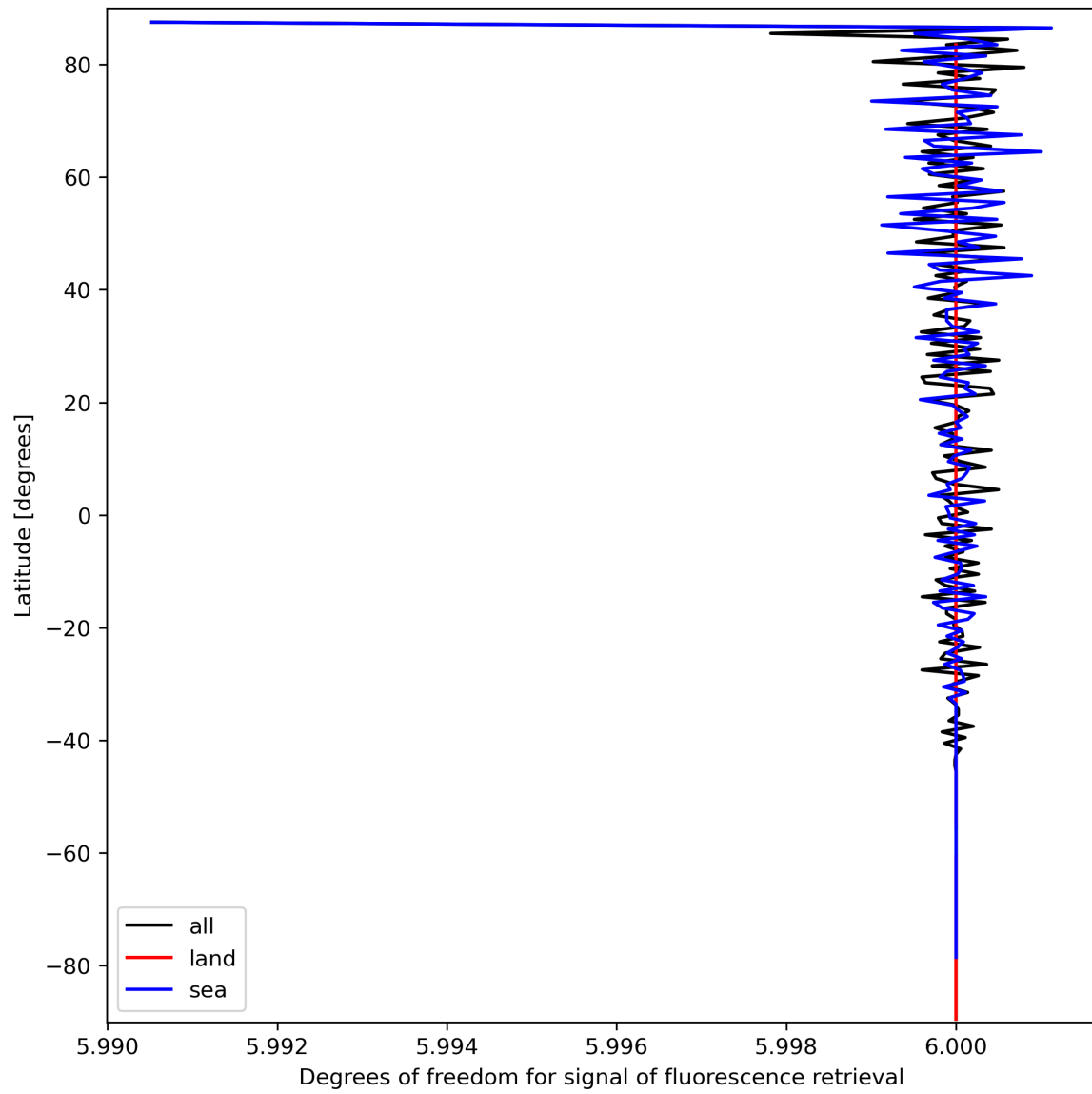
Figure 26: Zonal average of “Degrees of freedom for signal of fluorescence retrieval” for 2024-03-16 to 2024-03-18.
