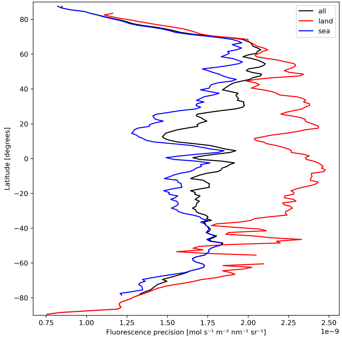
Figure 24: Zonal average of “Fluorescence precision” for 2024-03-16 to 2024-03-18.
