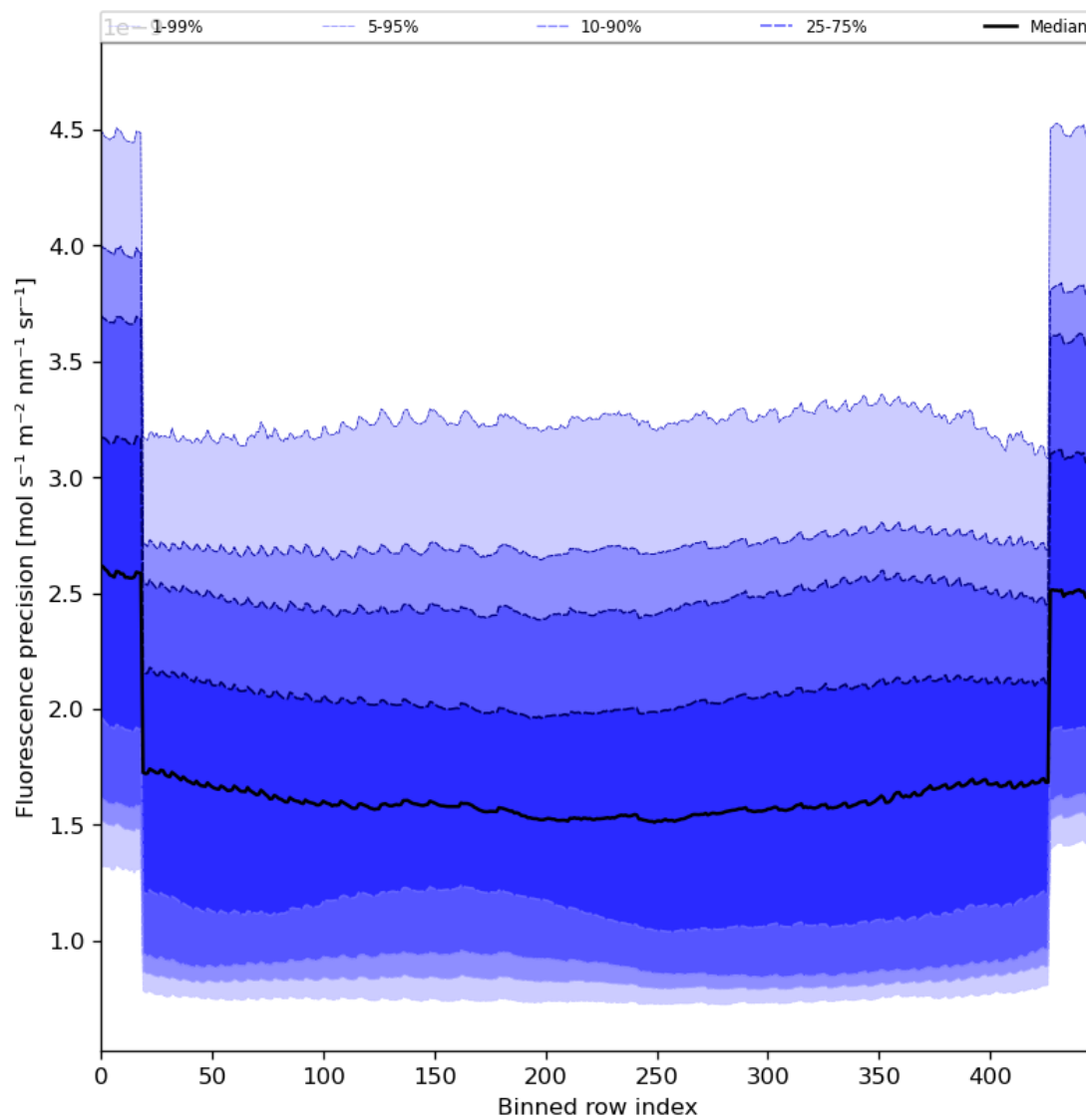
Figure 58: Along track statistics of “Fluorescence precision” for 2024-03-16 to 2024-03-18
