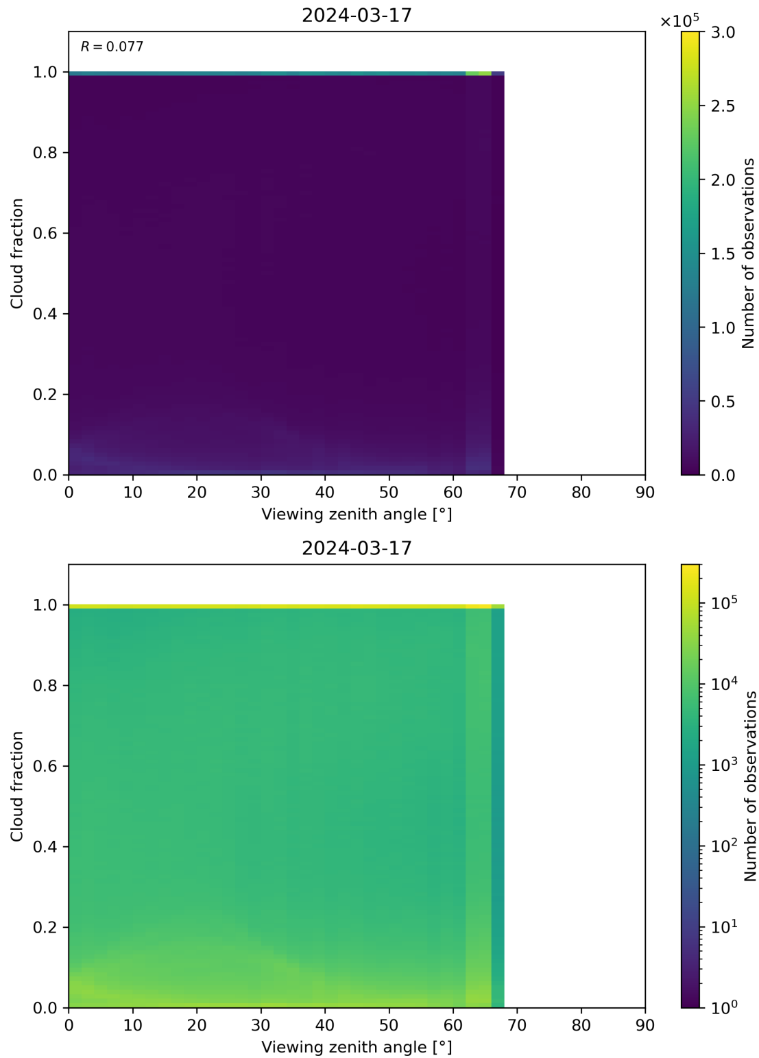
Figure 120: Scatter density plot of “Viewing zenith angle” against “Cloud fraction” for 2024-03-16 to 2024-03-18.
