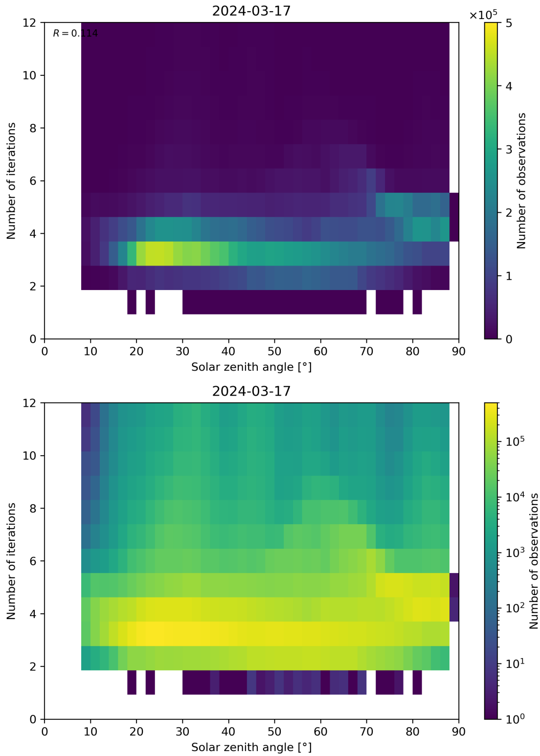
Figure 114: Scatter density plot of “Solar zenith angle” against “Number of iterations” for 2024-03-16 to 2024-03-18.
