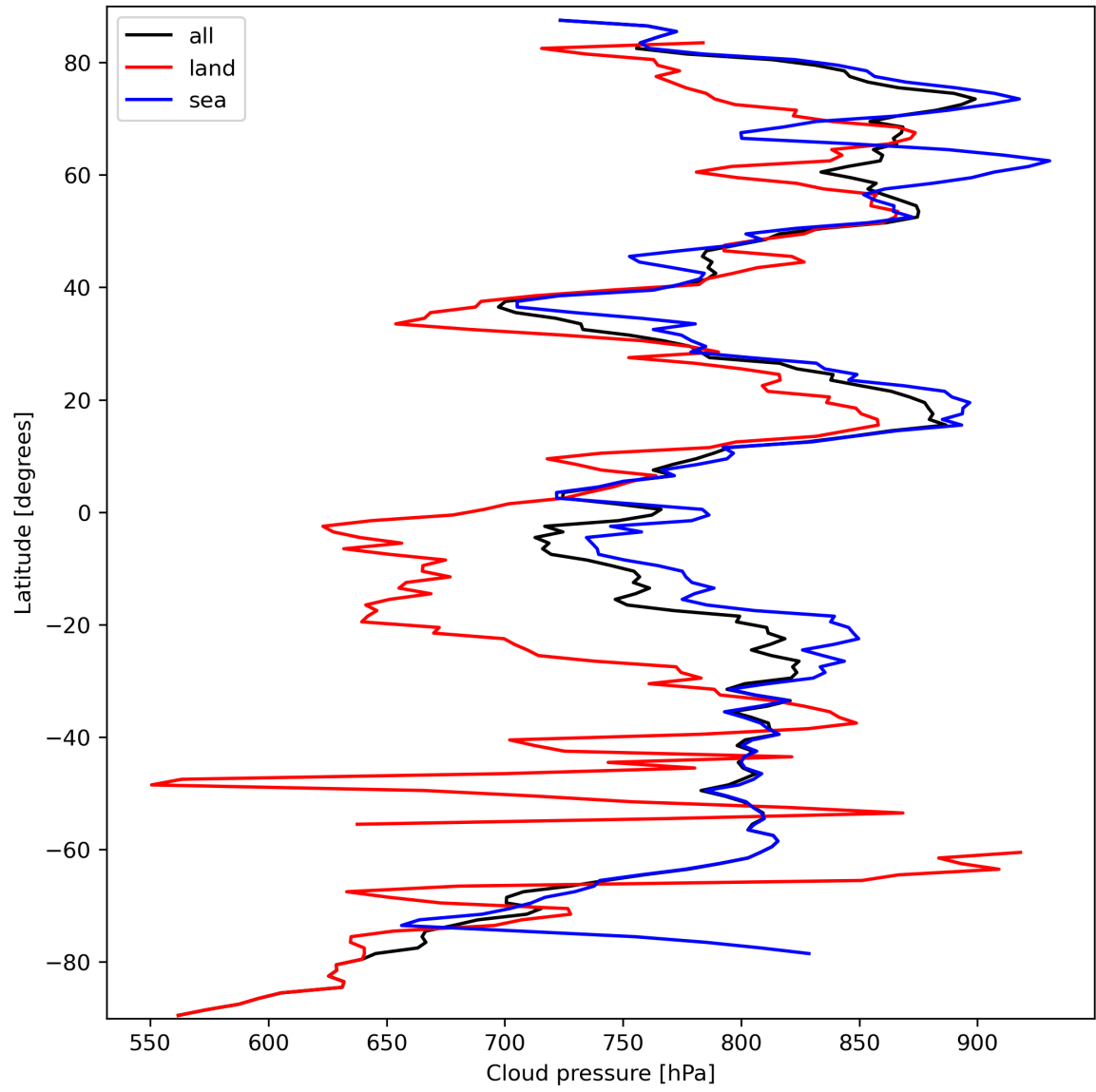
Figure 13: Zonal average of “Cloud pressure” for 2024-03-16 to 2024-03-18.
