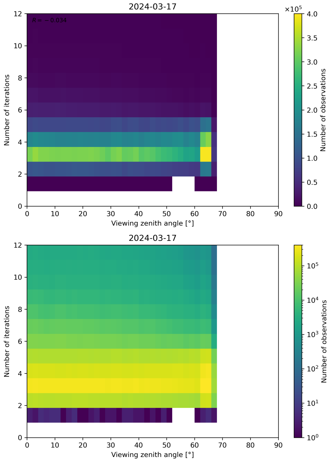
Figure 124: Scatter density plot of “Viewing zenith angle” against “Number of iterations” for 2024-03-16 to 2024-03-18.
