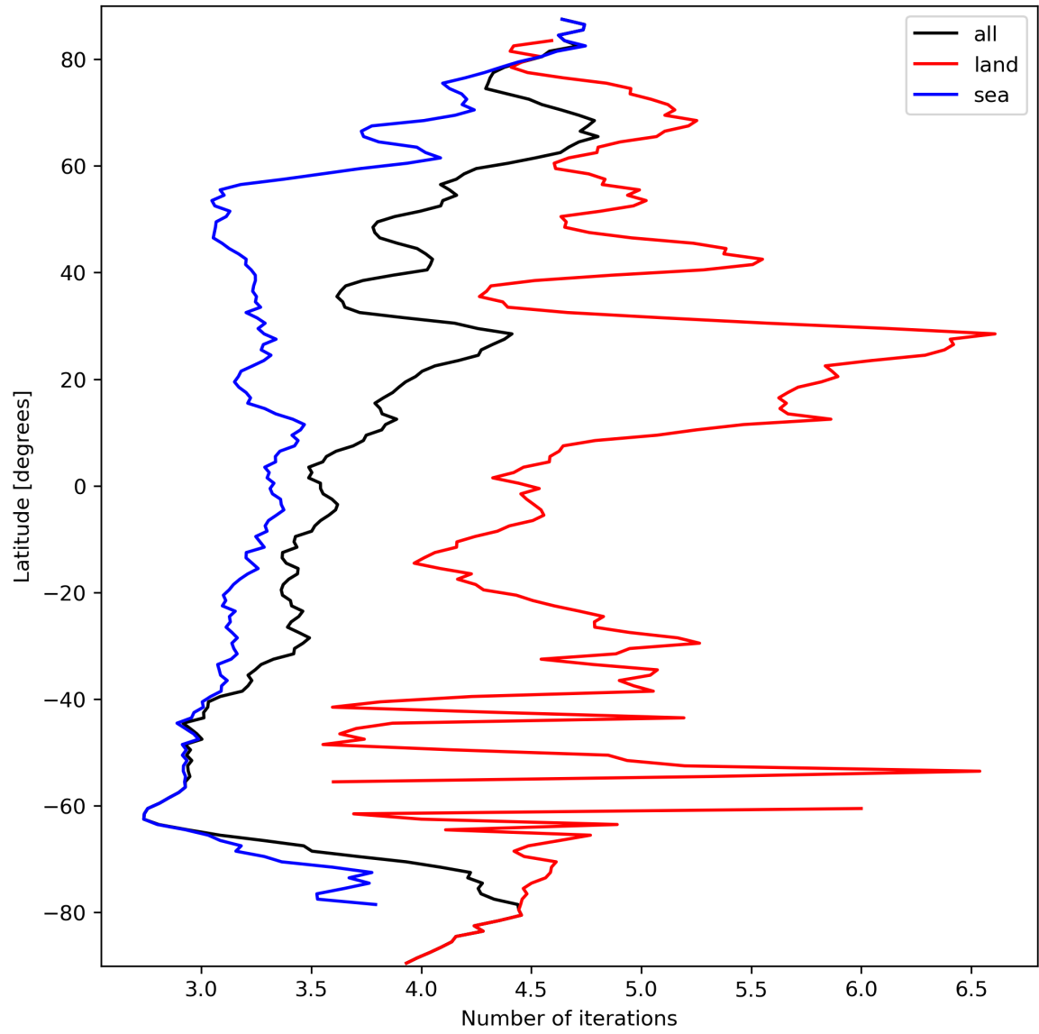
Figure 22: Zonal average of “Number of iterations” for 2024-03-16 to 2024-03-18.
