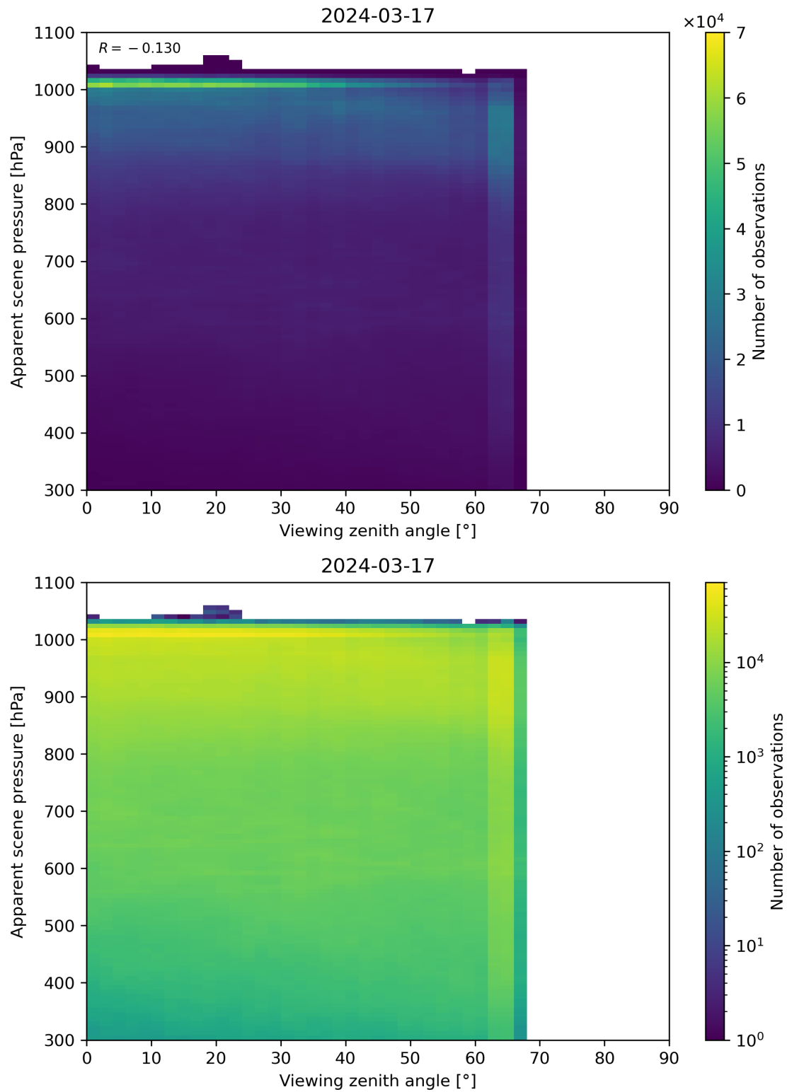
Figure 118: Scatter density plot of “Viewing zenith angle” against “Apparent scene pressure” for 2024-03-16 to 2024-03-18.
