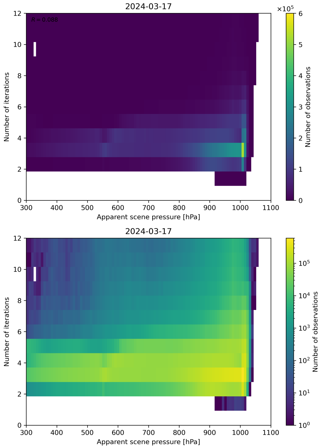
Figure 65: Scatter density plot of “Apparent scene pressure” against “Number of iterations” for 2024-03-16 to 2024-03-18.
