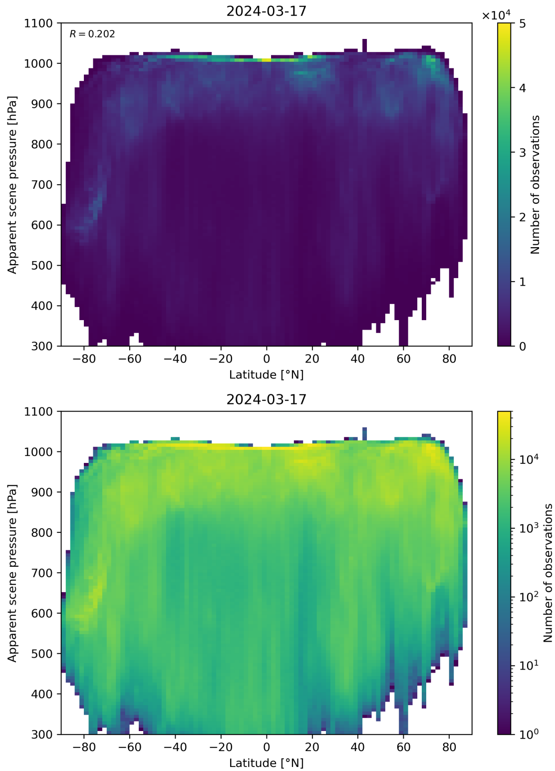
Figure 88: Scatter density plot of “Latitude” against “Apparent scene pressure” for 2024-03-16 to 2024-03-18.
