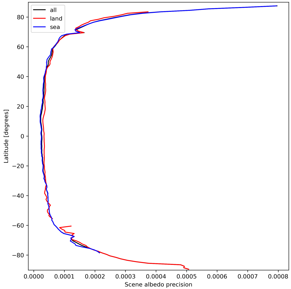
Figure 18: Zonal average of “Scene albedo precision” for 2024-03-16 to 2024-03-18.
