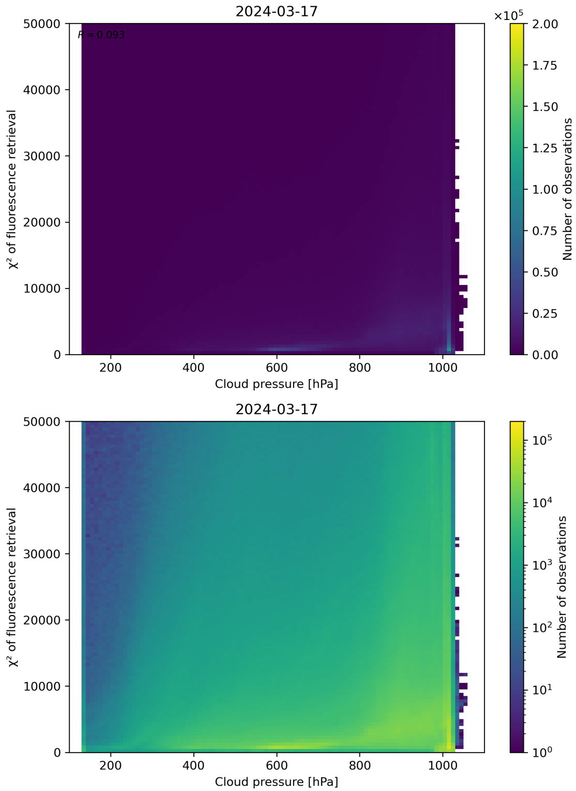
Figure 78: Scatter density plot of “Cloud pressure” against “ \chi^2 of fluorescence retrieval” for 2024-03-16 to 2024-03-18.
