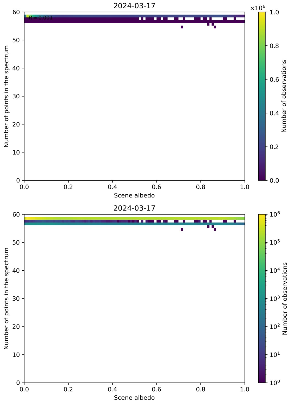
Figure 106: Scatter density plot of “Scene albedo” against “Number of points in the spectrum” for 2024-03-16 to 2024-03-18.
