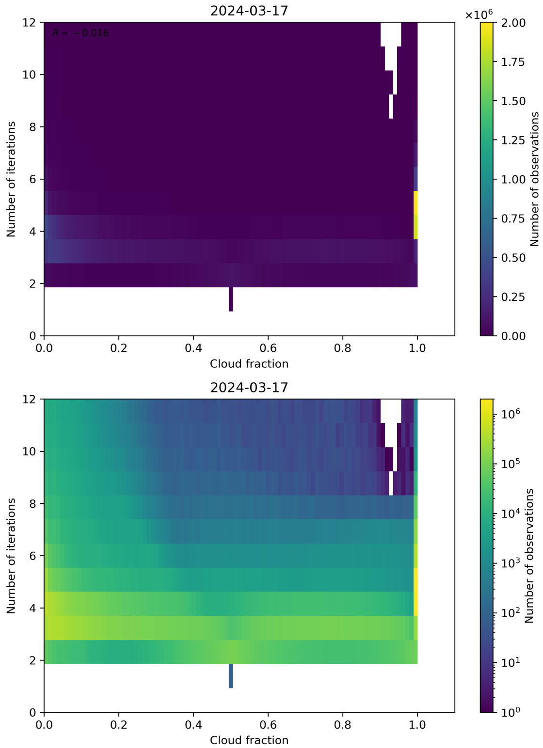
Figure 73: Scatter density plot of “Cloud fraction” against “Number of iterations” for 2024-03-16 to 2024-03-18.
