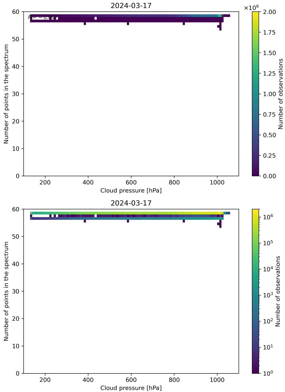
Figure 82: Scatter density plot of “Cloud pressure” against “Number of points in the spectrum” for 2024-03-16 to 2024-03-18.
