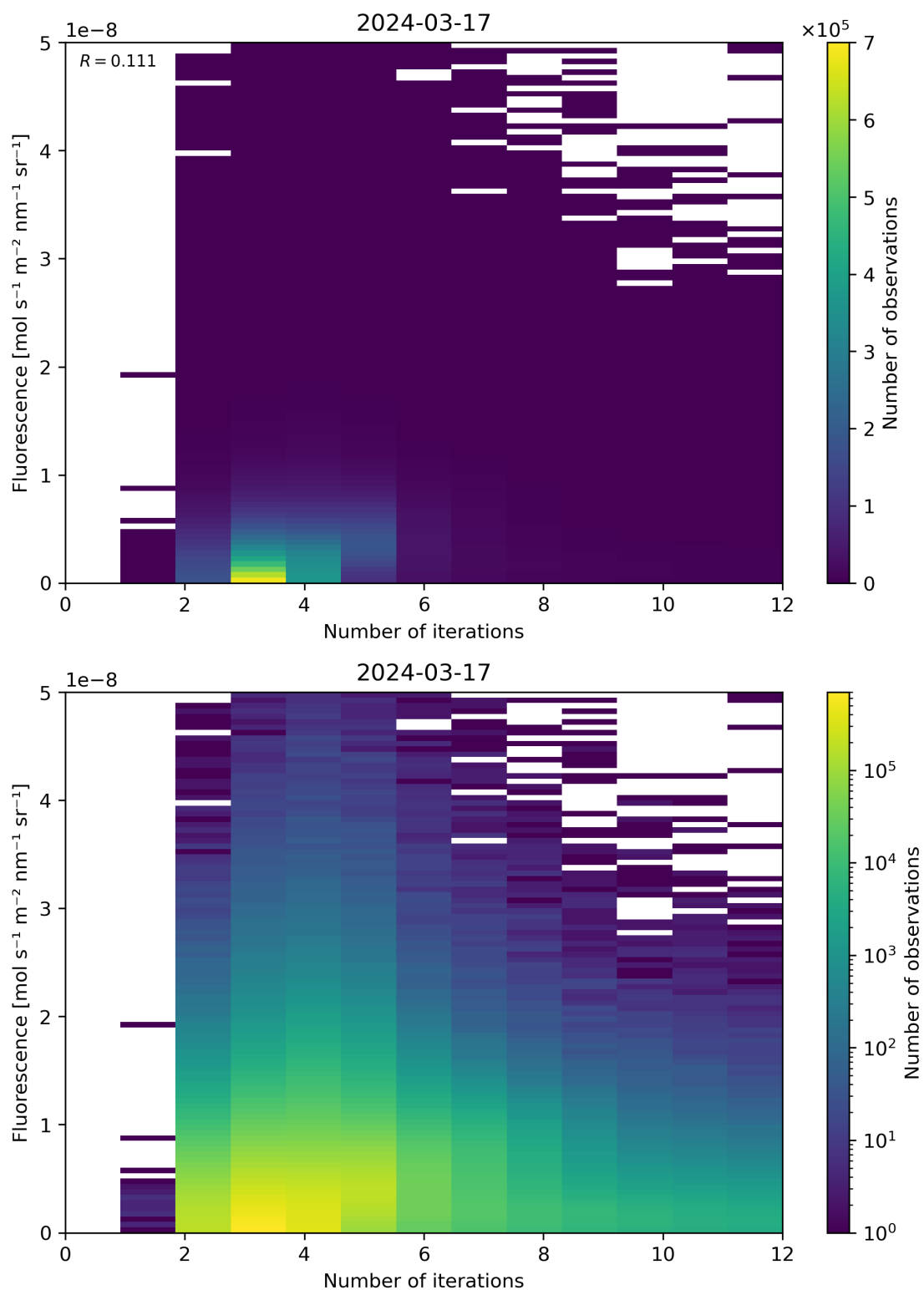
Figure 98: Scatter density plot of “Number of iterations” against “Fluorescence” for 2024-03-16 to 2024-03-18.
