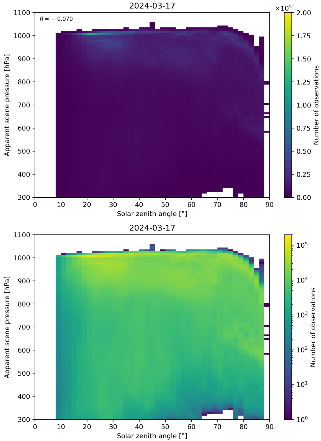
Figure 108: Scatter density plot of “Solar zenith angle” against “Apparent scene pressure” for 2024-03-16 to 2024-03-18.
