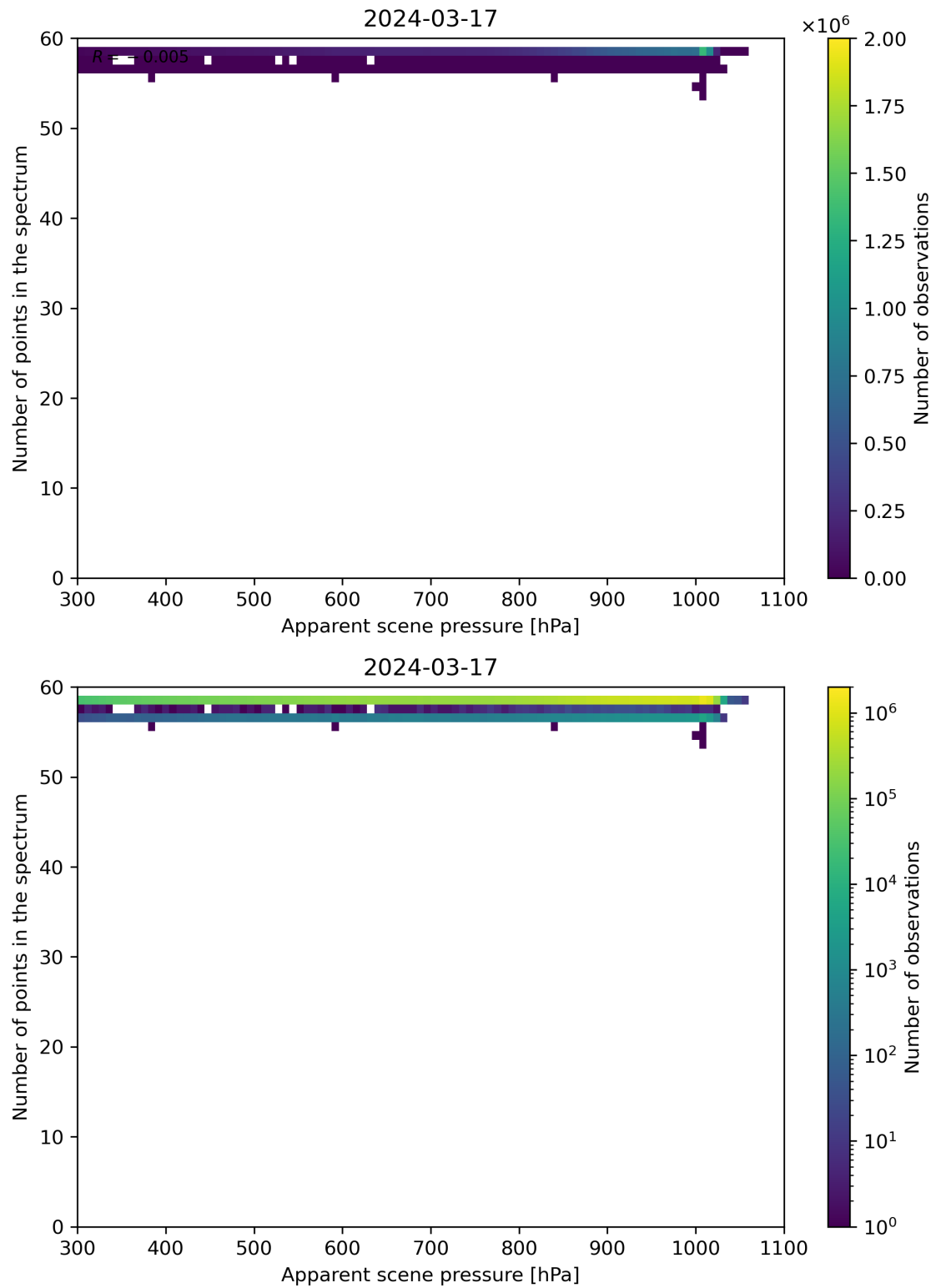
Figure 66: Scatter density plot of “Apparent scene pressure” against “Number of points in the spectrum” for 2024-03-16 to 2024-03-18.
