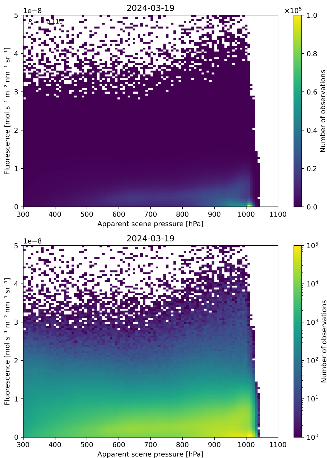
Figure 64: Scatter density plot of “Apparent scene pressure” against “Fluorescence” for 2024-03-18 to 2024-03-20.
