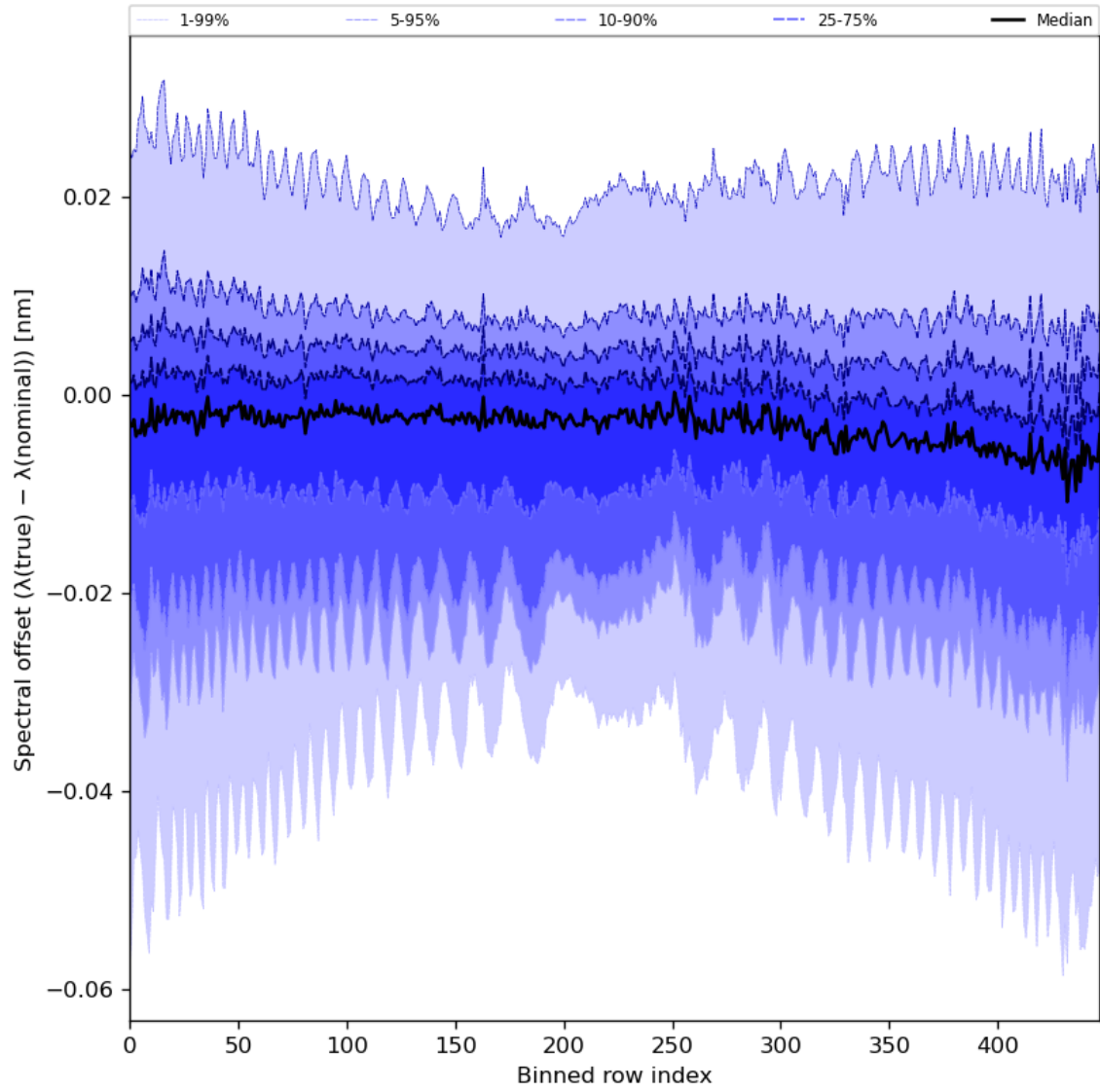
Figure 62: Along track statistics of “Spectral offset ( \lambda(\text{true}) - \lambda(\text{nominal}) )” for 2024-03-18 to 2024-03-20
