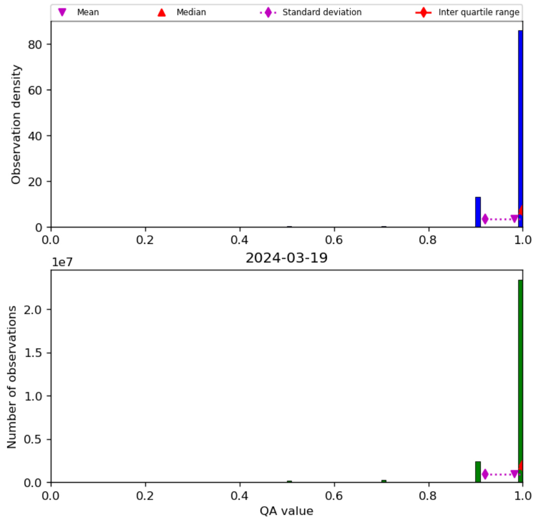
Figure 29: Histogram of “QA value” for 2024-03-18 to 2024-03-20
