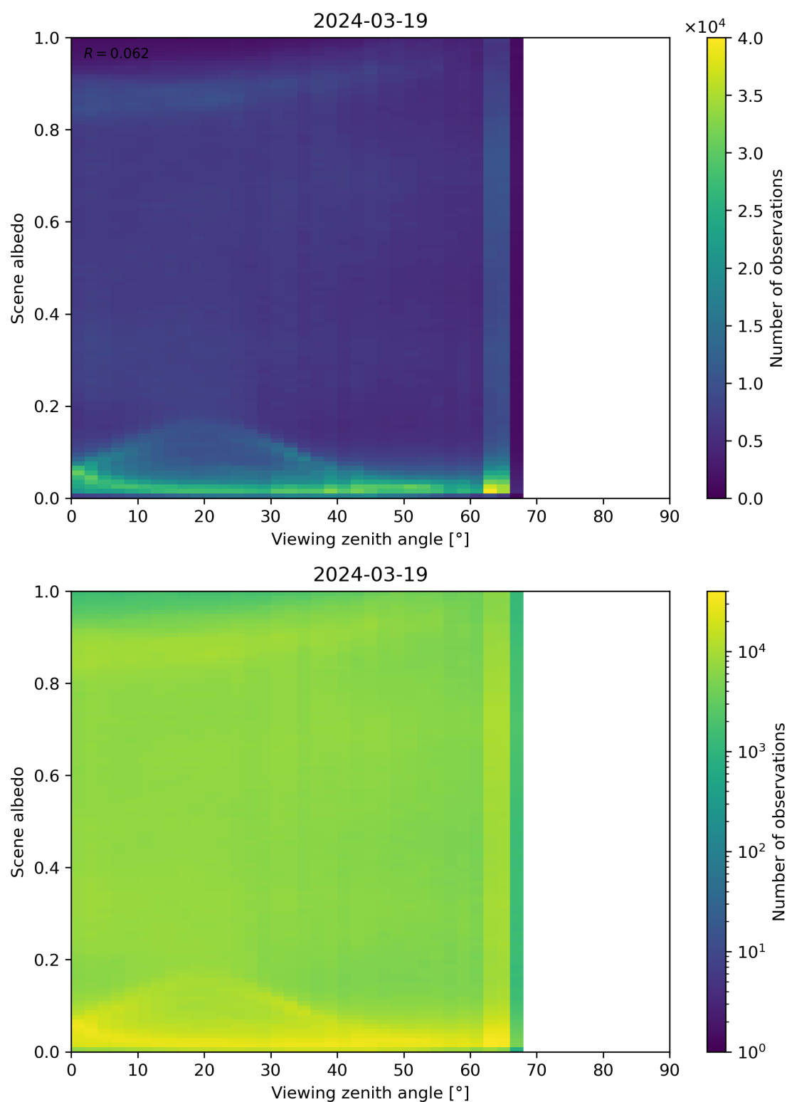
Figure 126: Scatter density plot of “Viewing zenith angle” against “Scene albedo” for 2024-03-18 to 2024-03-20.
