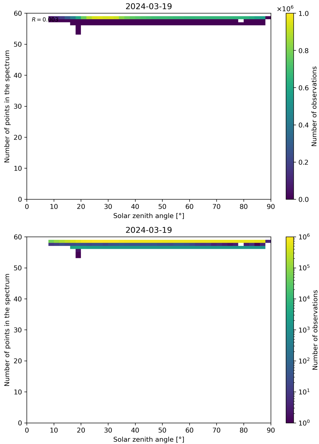
Figure 115: Scatter density plot of “Solar zenith angle” against “Number of points in the spectrum” for 2024-03-18 to 2024-03-20.
