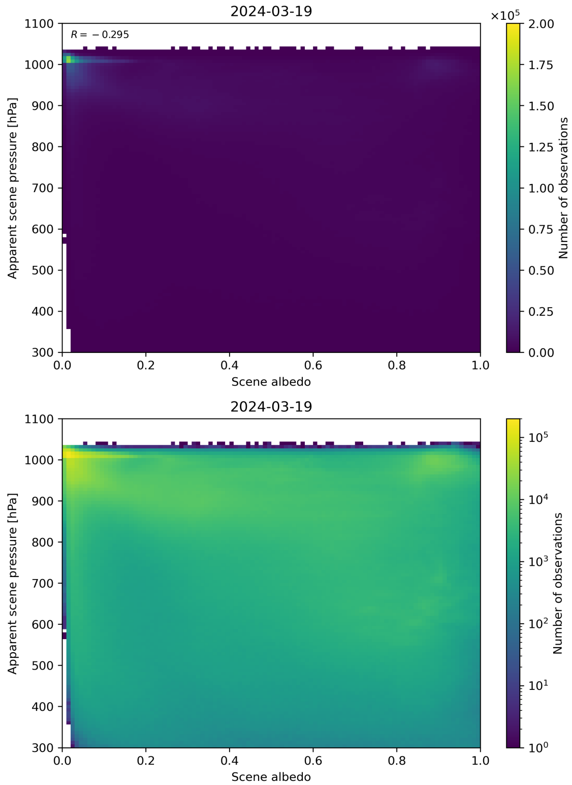
Figure 102: Scatter density plot of “Scene albedo” against “Apparent scene pressure” for 2024-03-18 to 2024-03-20.
