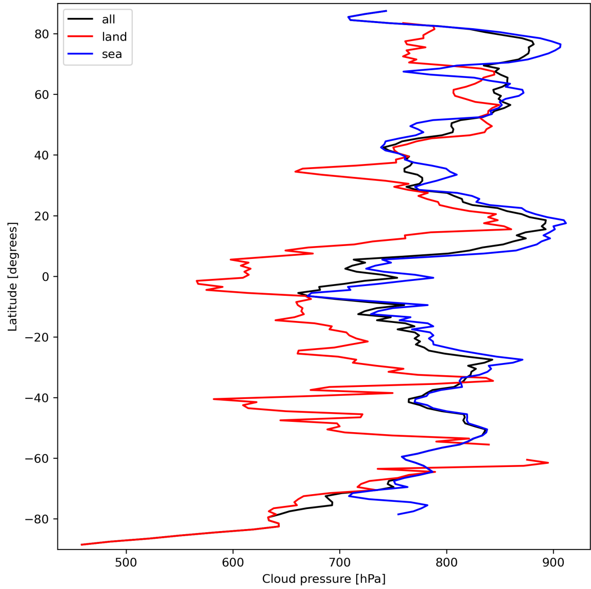
Figure 13: Zonal average of “Cloud pressure” for 2024-03-18 to 2024-03-20.
