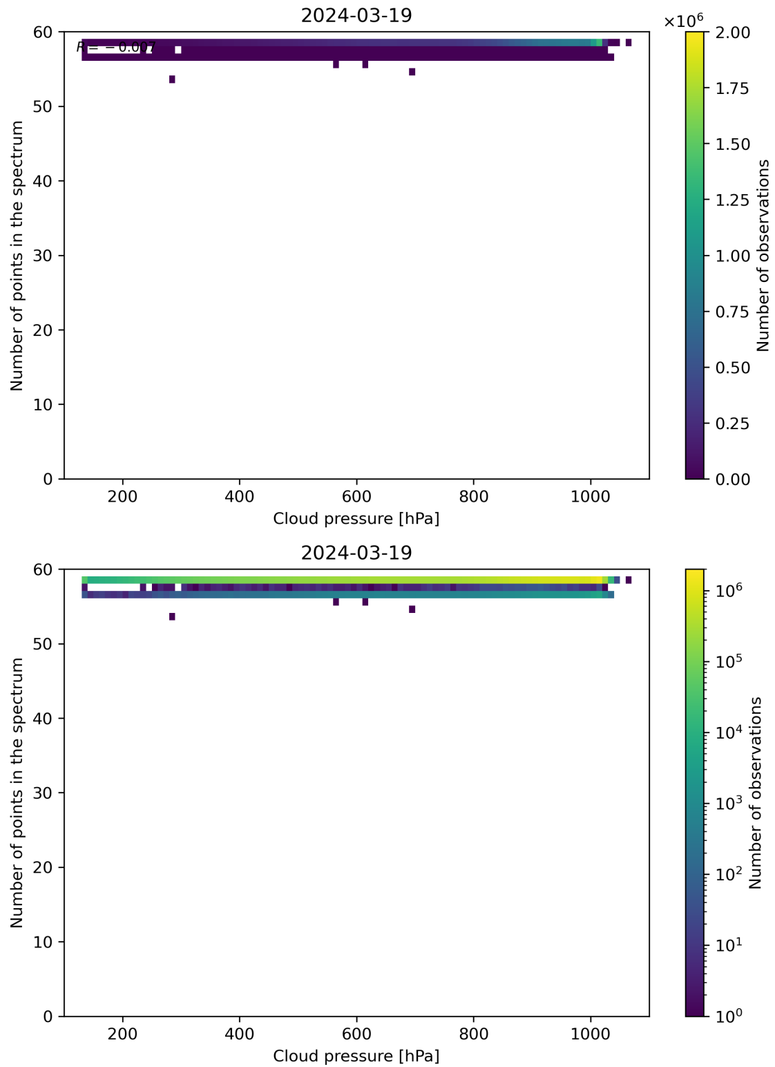
Figure 82: Scatter density plot of “Cloud pressure” against “Number of points in the spectrum” for 2024-03-18 to 2024-03-20.
