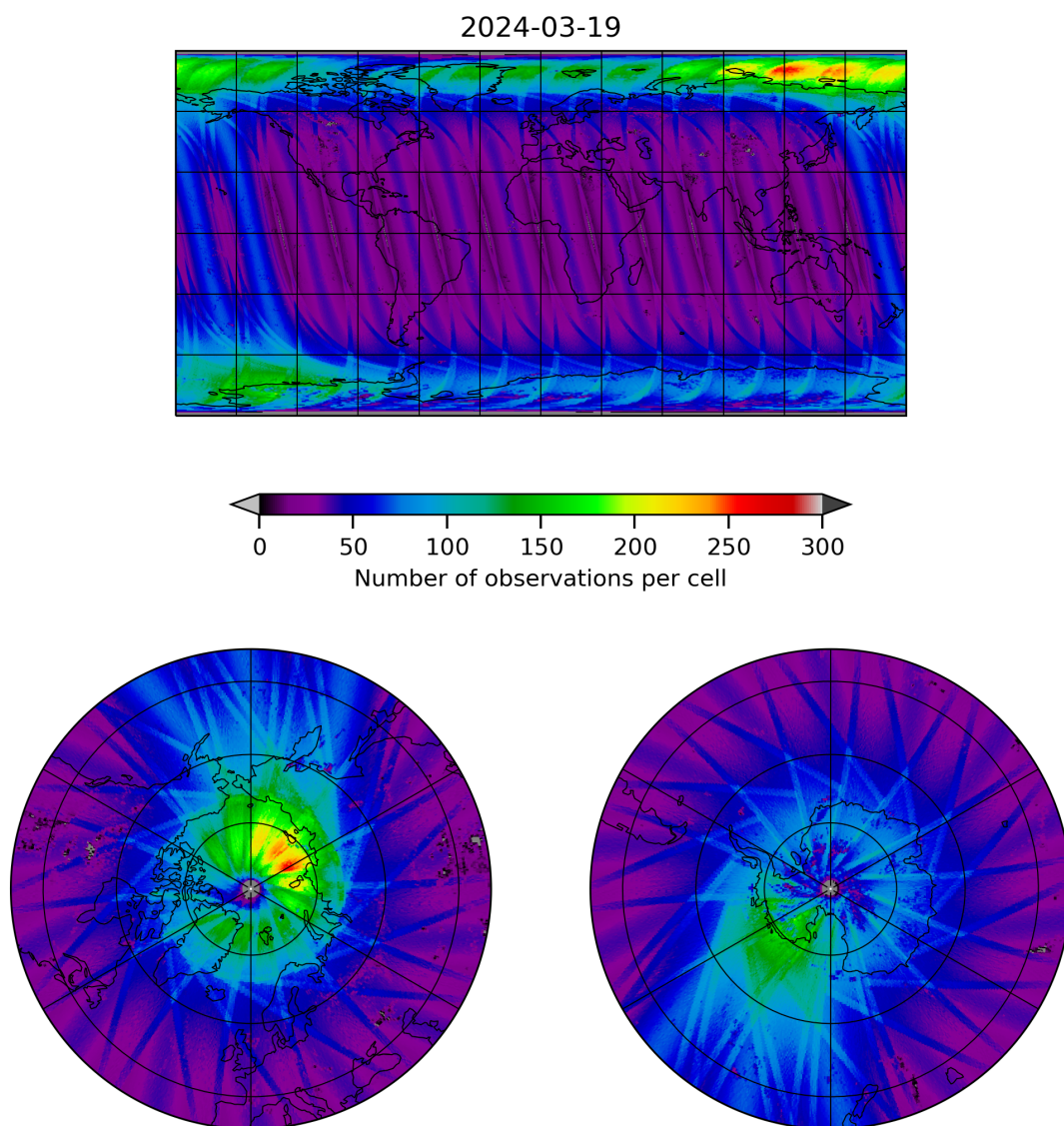
Figure 11: Map of the number of observations for 2024-03-18 to 2024-03-20
