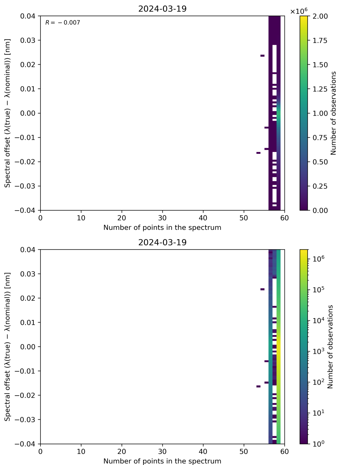
Figure 101: Scatter density plot of “Number of points in the spectrum” against “Spectral offset ( \lambda(\text{true}) - \lambda(\text{nominal}) )” for 2024-03-18 to 2024-03-20.
