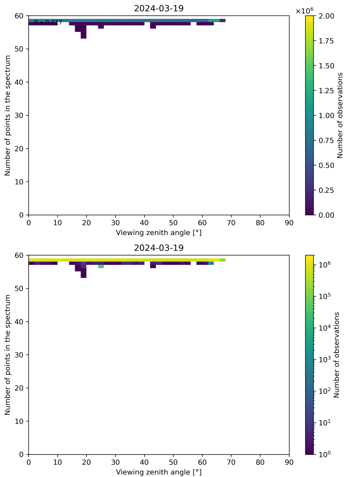
Figure 125: Scatter density plot of “Viewing zenith angle” against “Number of points in the spectrum” for 2024-03-18 to 2024-03-20.
