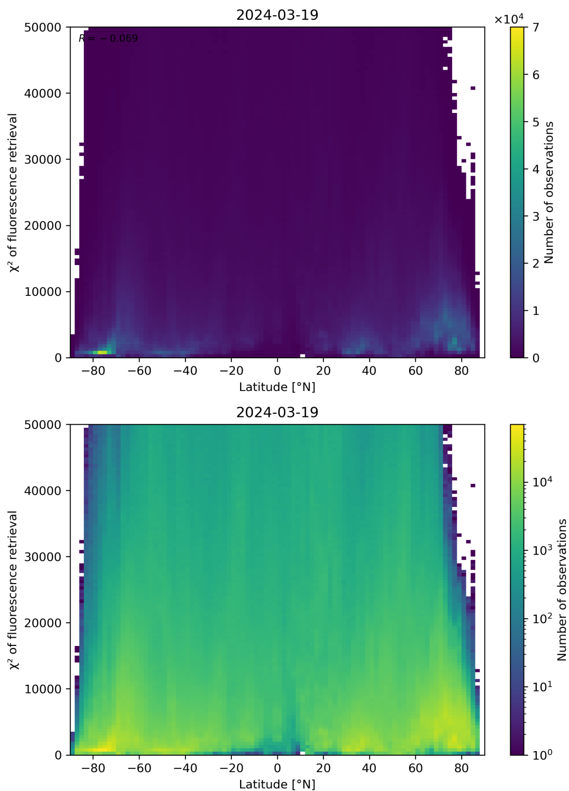
Figure 89: Scatter density plot of “Latitude” against “ \chi^2 of fluorescence retrieval” for 2024-03-18 to 2024-03-20.
