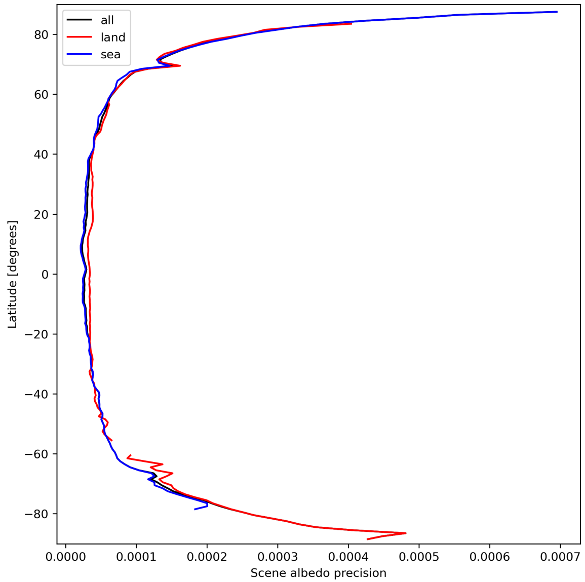
Figure 18: Zonal average of “Scene albedo precision” for 2024-03-18 to 2024-03-20.
