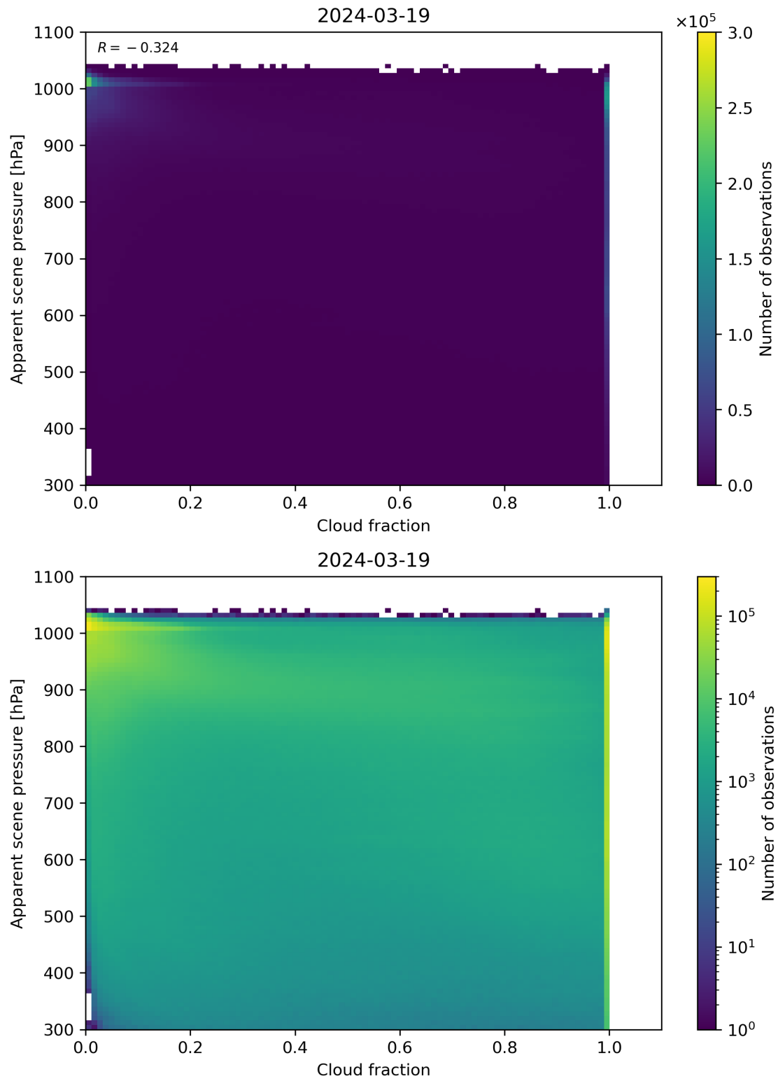
Figure 70: Scatter density plot of “Cloud fraction” against “Apparent scene pressure” for 2024-03-18 to 2024-03-20.
