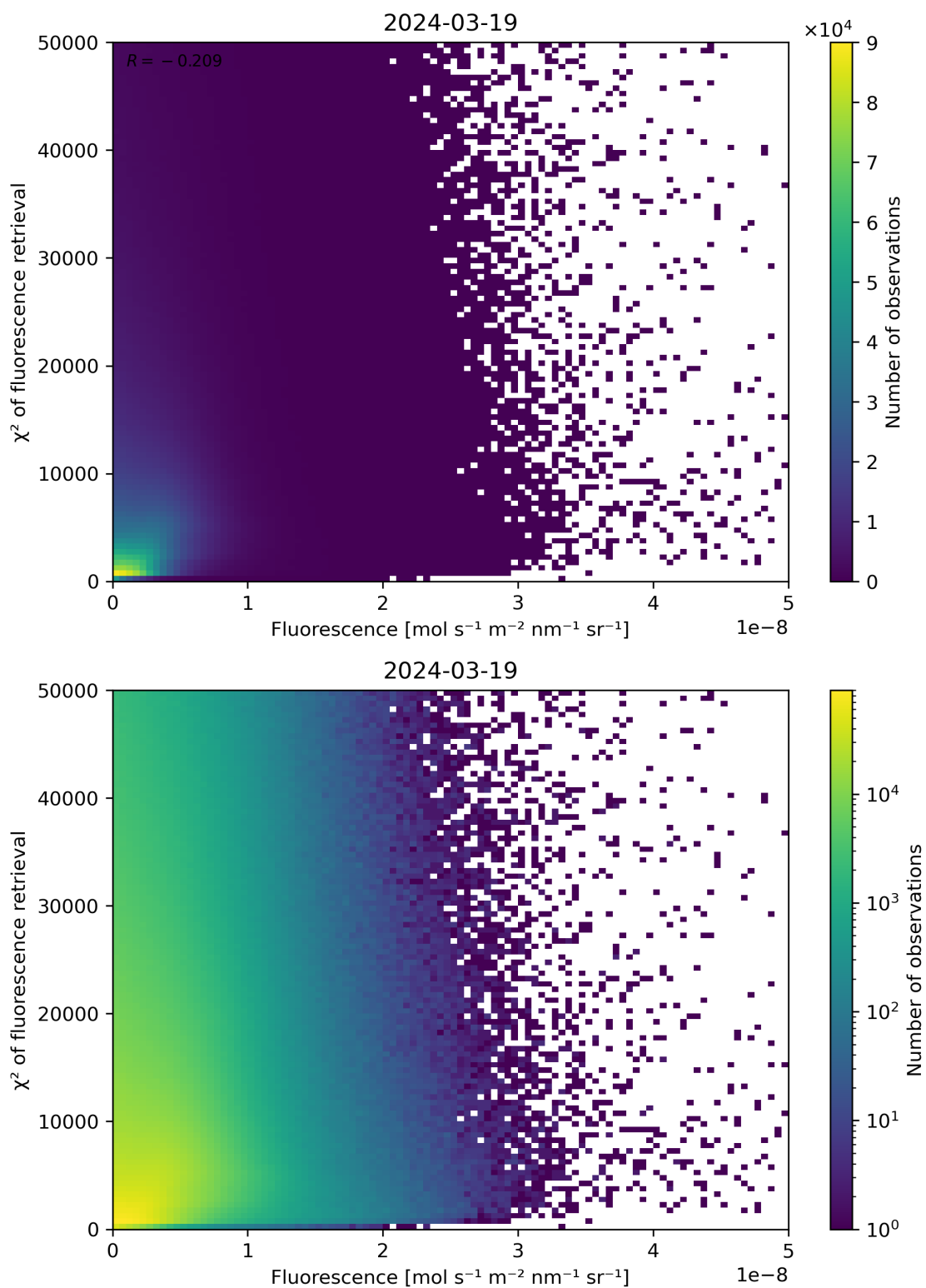
Figure 85: Scatter density plot of “Fluorescence” against “ \chi^2 of fluorescence retrieval” for 2024-03-18 to 2024-03-20.
