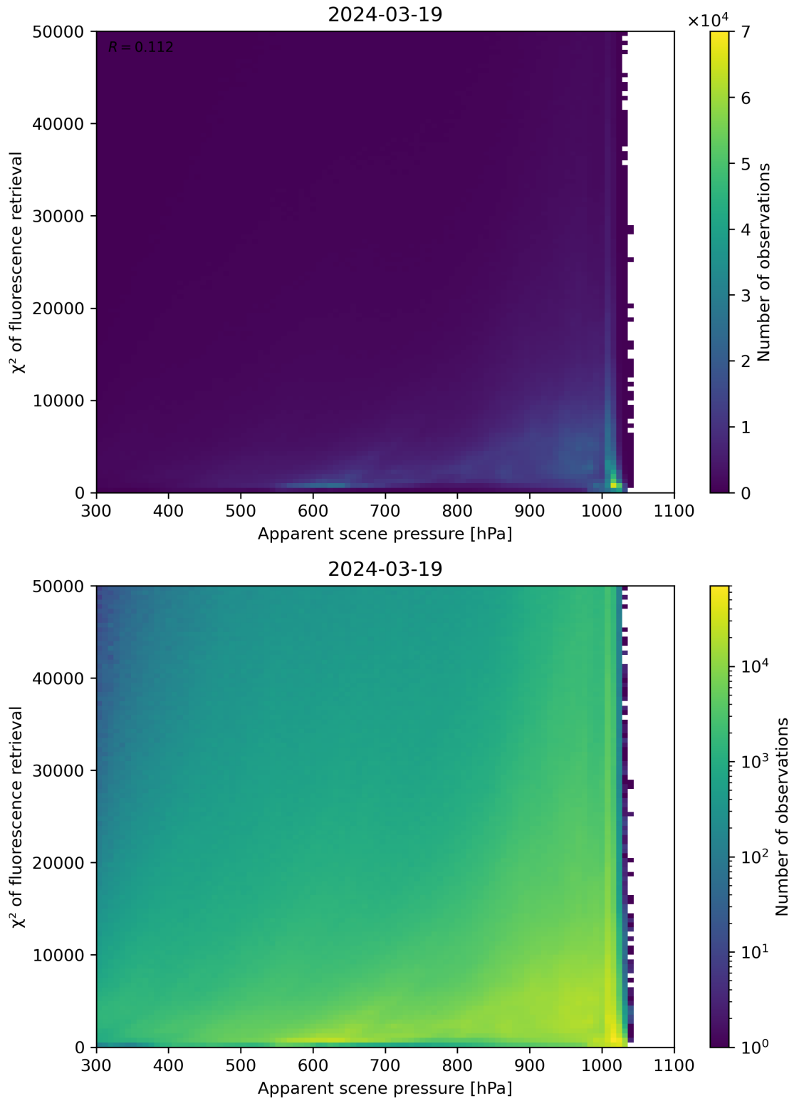
Figure 63: Scatter density plot of “Apparent scene pressure” against “ \chi^2 of fluorescence retrieval” for 2024-03-18 to 2024-03-20.
