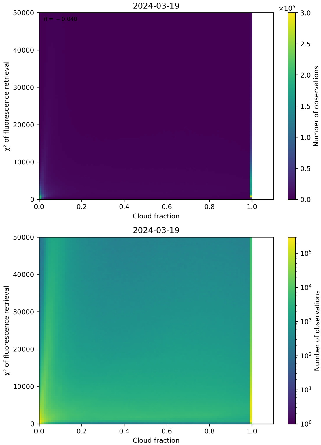
Figure 71: Scatter density plot of “Cloud fraction” against “ \chi^2 of fluorescence retrieval” for 2024-03-18 to 2024-03-20.
