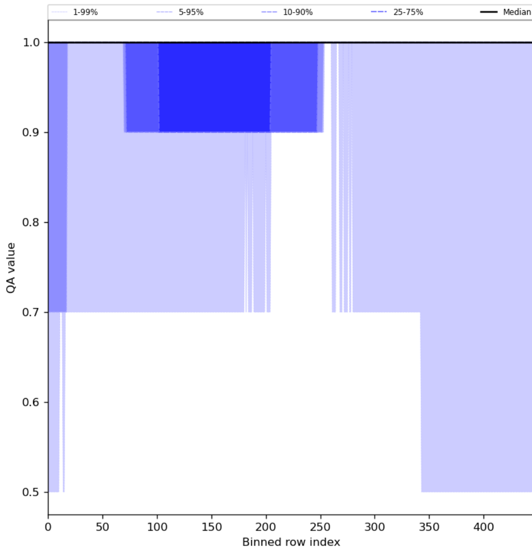
Figure 46: Along track statistics of “QA value” for 2024-03-18 to 2024-03-20
