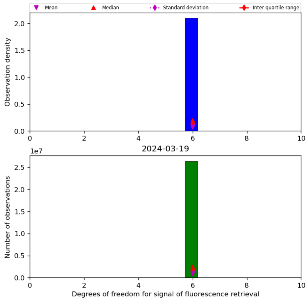
Figure 43: Histogram of “Degrees of freedom for signal of fluorescence retrieval” for 2024-03-18 to 2024-03-20
