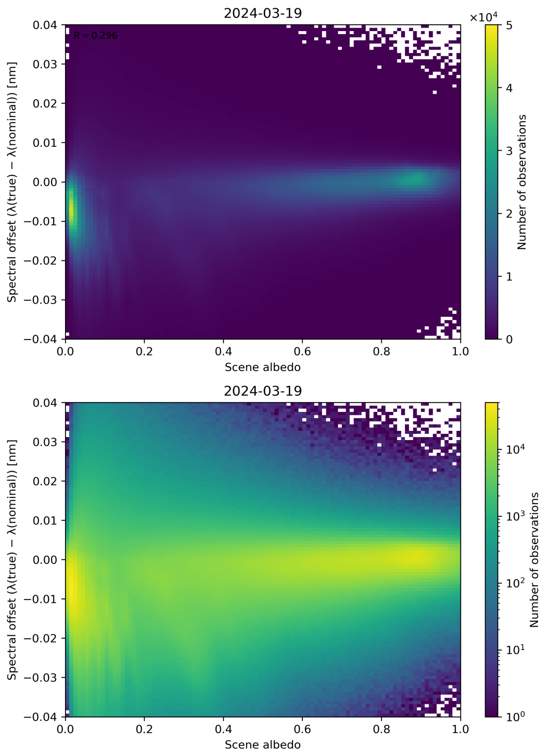
Figure 107: Scatter density plot of “Scene albedo” against “Spectral offset ( \lambda(\text{true}) - \lambda(\text{nominal}) )” for 2024-03-18 to 2024-03-20.
