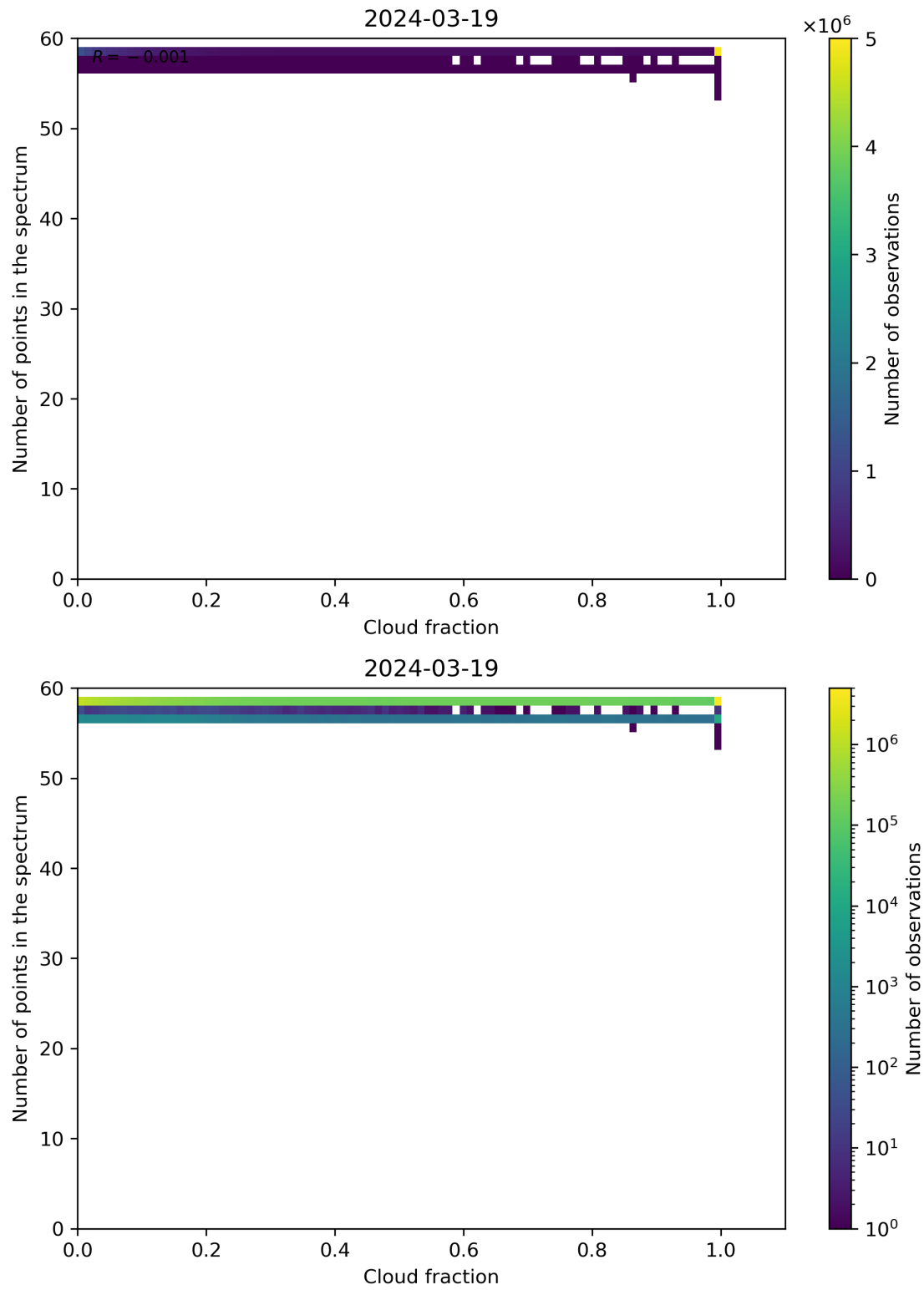
Figure 74: Scatter density plot of “Cloud fraction” against “Number of points in the spectrum” for 2024-03-18 to 2024-03-20.
