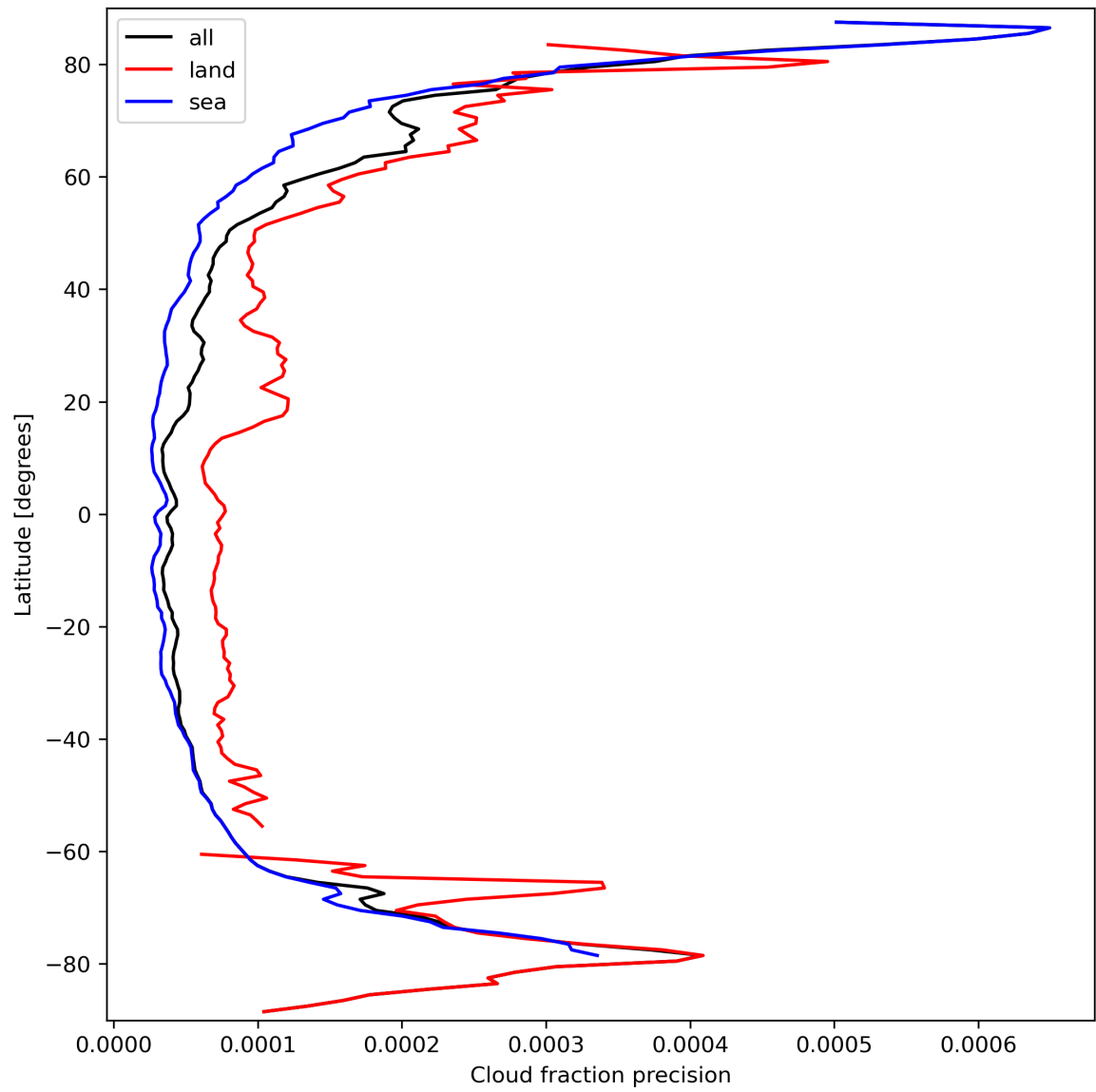
Figure 16: Zonal average of “Cloud fraction precision” for 2024-03-18 to 2024-03-20.
