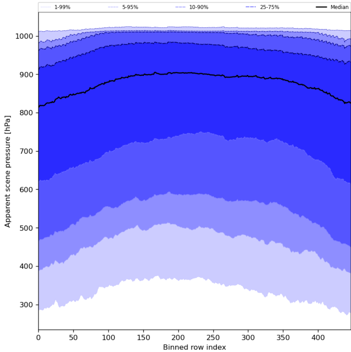
Figure 53: Along track statistics of “Apparent scene pressure” for 2024-03-18 to 2024-03-20
