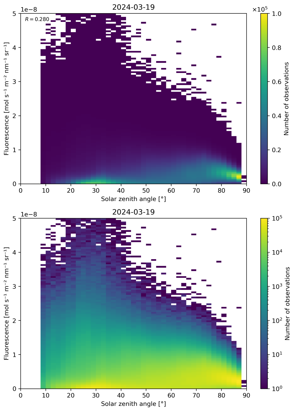
Figure 112: Scatter density plot of “Solar zenith angle” against “Fluorescence” for 2024-03-18 to 2024-03-20.
