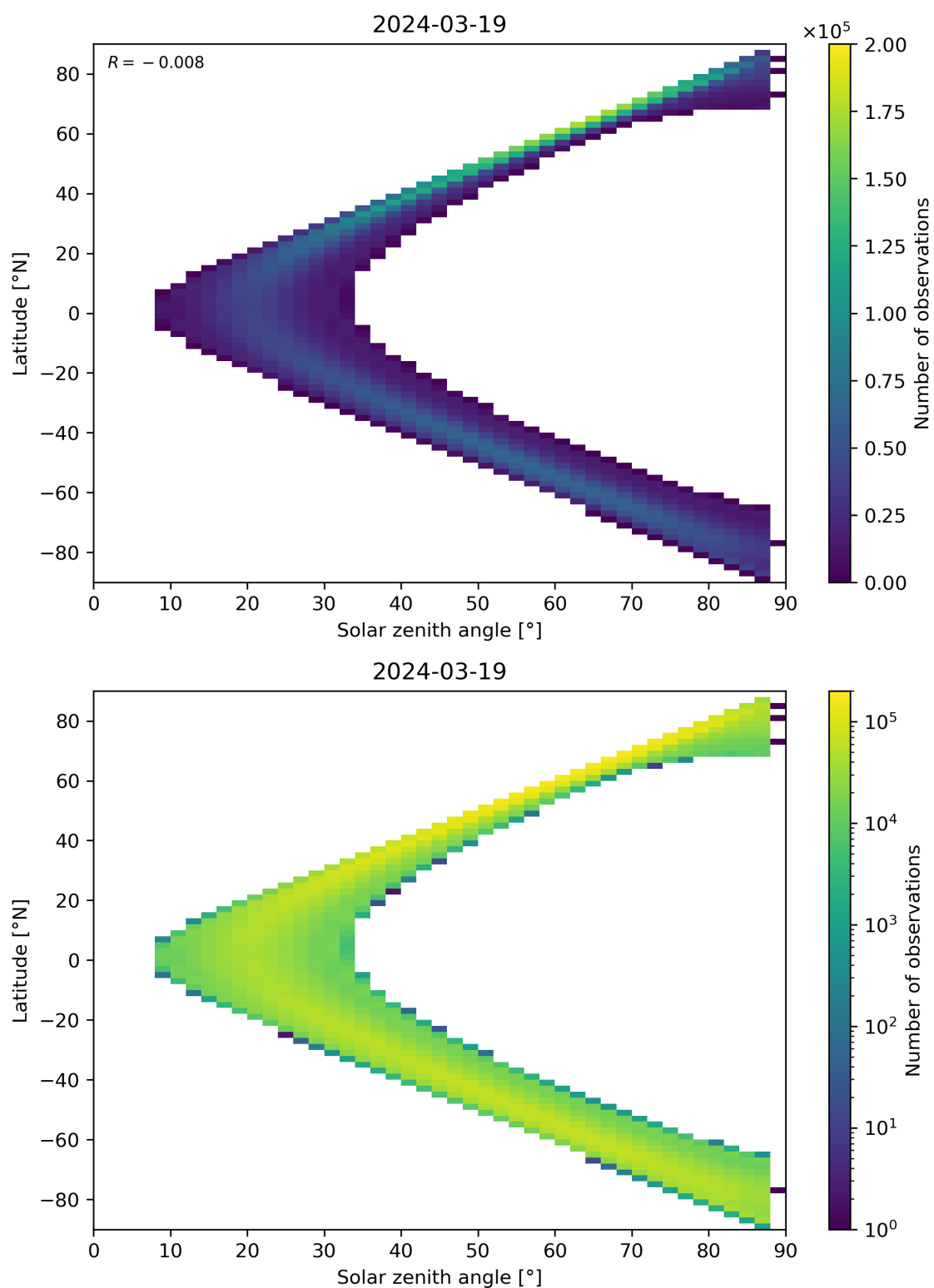
Figure 113: Scatter density plot of “Solar zenith angle” against “Latitude” for 2024-03-18 to 2024-03-20.
