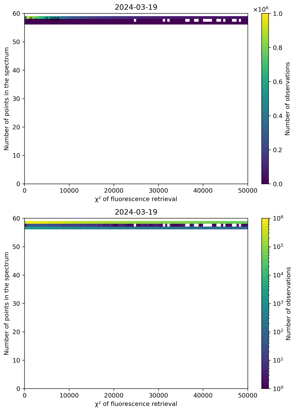
Figure 68: Scatter density plot of " \chi^2 of fluorescence retrieval" against "Number of points in the spectrum" for 2024-03-18 to 2024-03-20.
