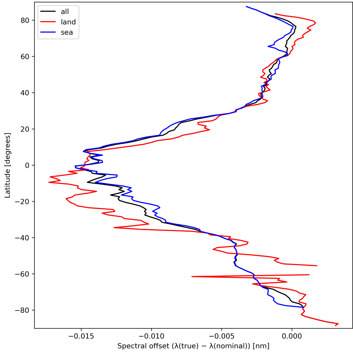
Figure 28: Zonal average of “Spectral offset ( \lambda(\text{true}) - \lambda(\text{nominal}) )” for 2024-03-18 to 2024-03-20.
