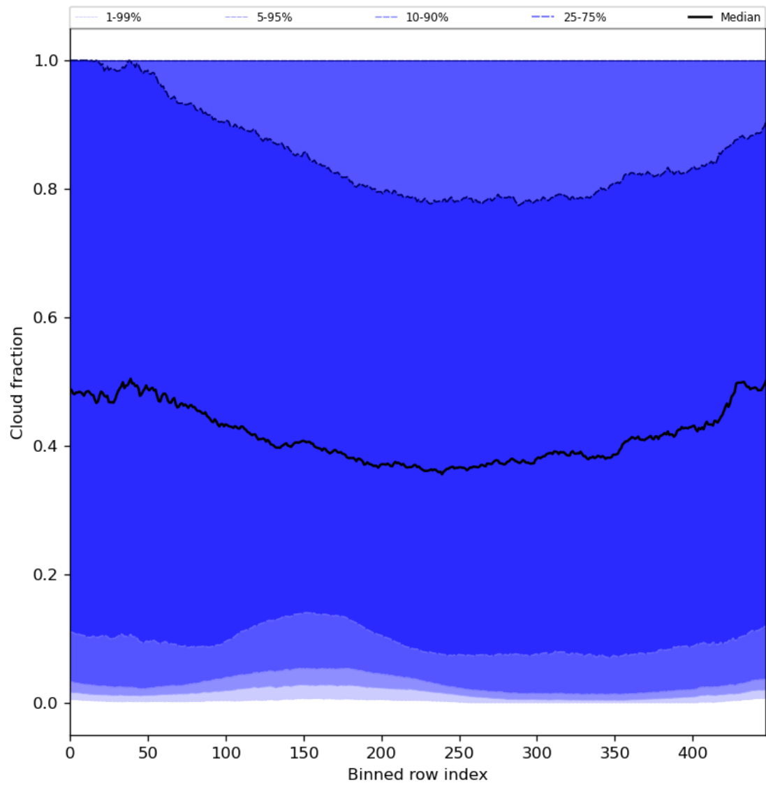
Figure 49: Along track statistics of “Cloud fraction” for 2024-03-18 to 2024-03-20
