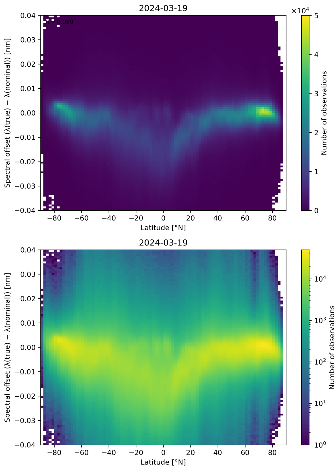
Figure 96: Scatter density plot of “Latitude” against “Spectral offset ( \lambda(\text{true}) - \lambda(\text{nominal}) )” for 2024-03-18 to 2024-03-20.
