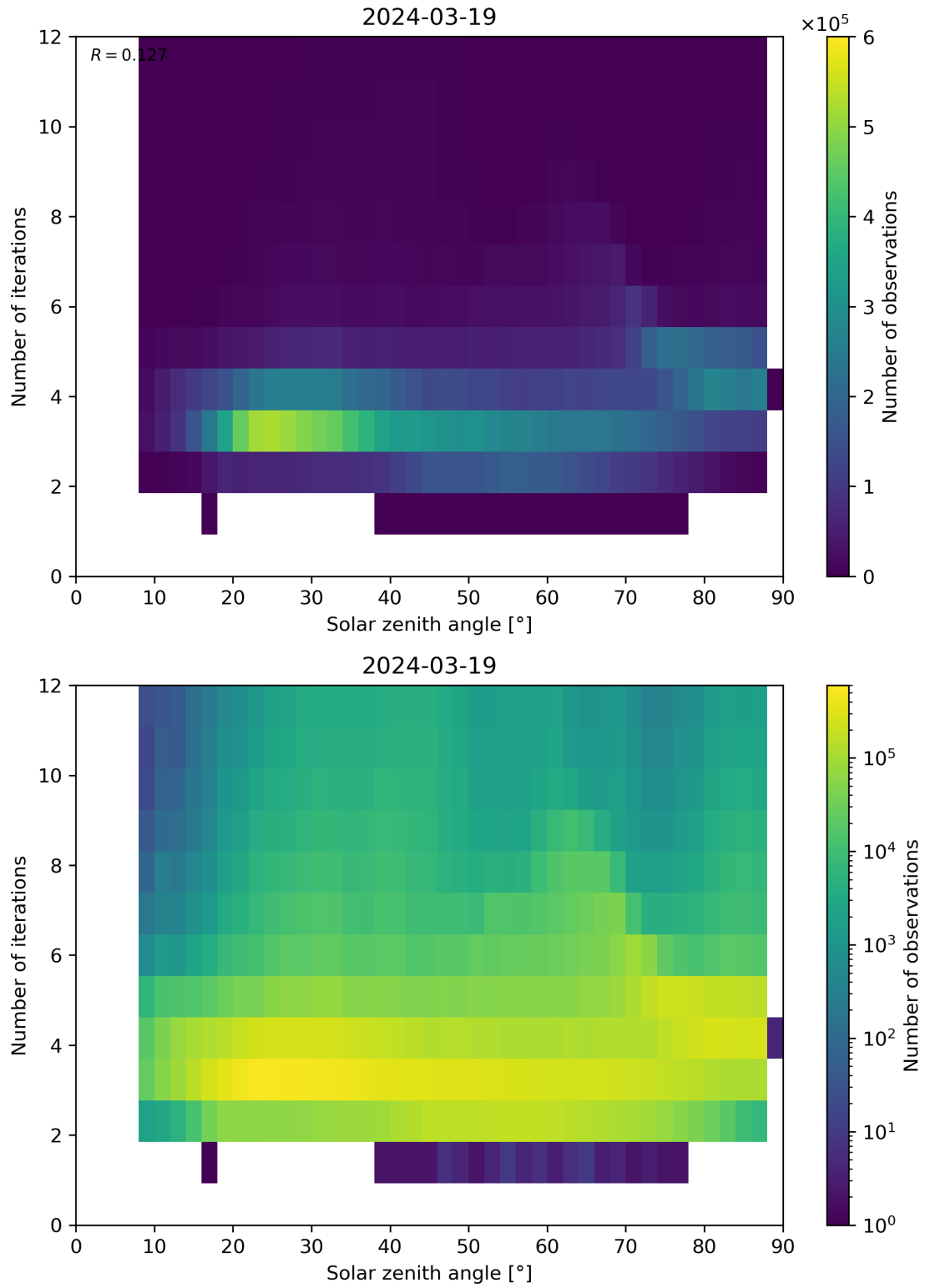
Figure 114: Scatter density plot of “Solar zenith angle” against “Number of iterations” for 2024-03-18 to 2024-03-20.
