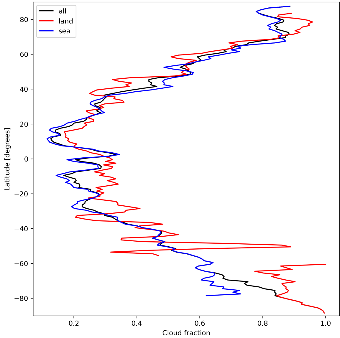
Figure 15: Zonal average of “Cloud fraction” for 2024-03-18 to 2024-03-20.
