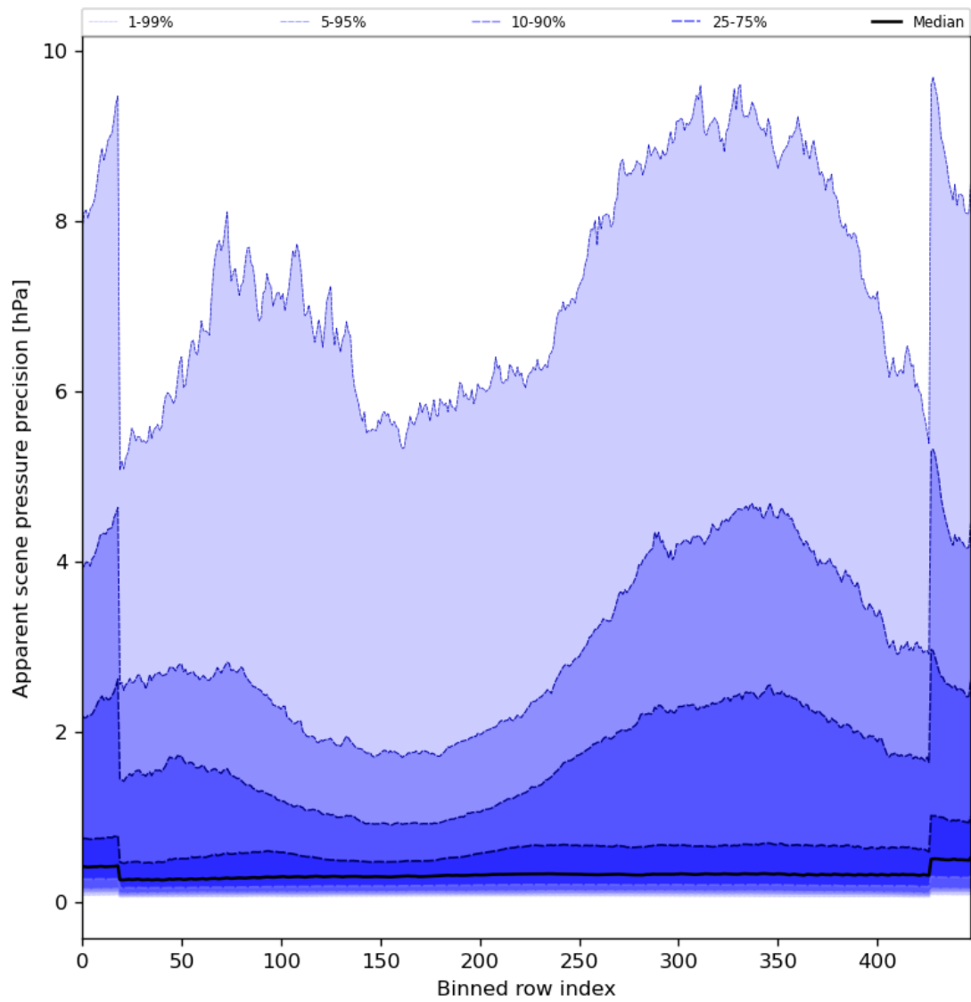
Figure 54: Along track statistics of “Apparent scene pressure precision” for 2024-03-18 to 2024-03-20
