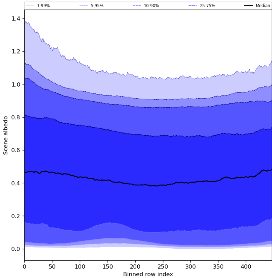
Figure 51: Along track statistics of “Scene albedo” for 2024-03-18 to 2024-03-20
