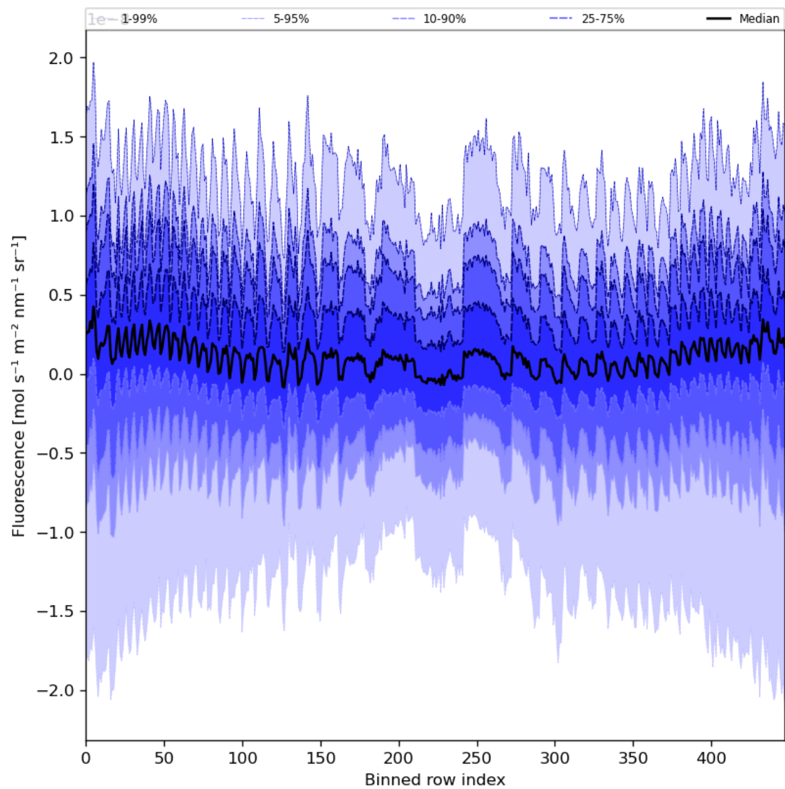
Figure 57: Along track statistics of “Fluorescence” for 2024-03-18 to 2024-03-20
