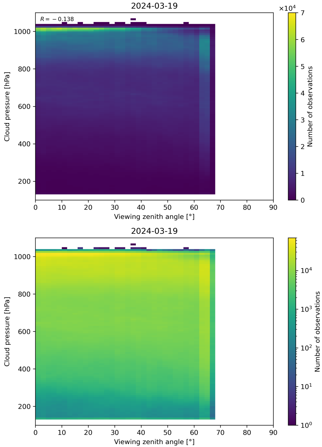
Figure 121: Scatter density plot of “Viewing zenith angle” against “Cloud pressure” for 2024-03-18 to 2024-03-20.
