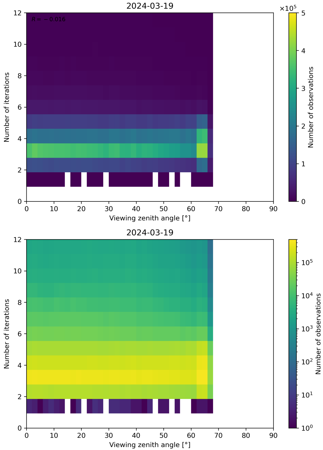
Figure 124: Scatter density plot of “Viewing zenith angle” against “Number of iterations” for 2024-03-18 to 2024-03-20.
