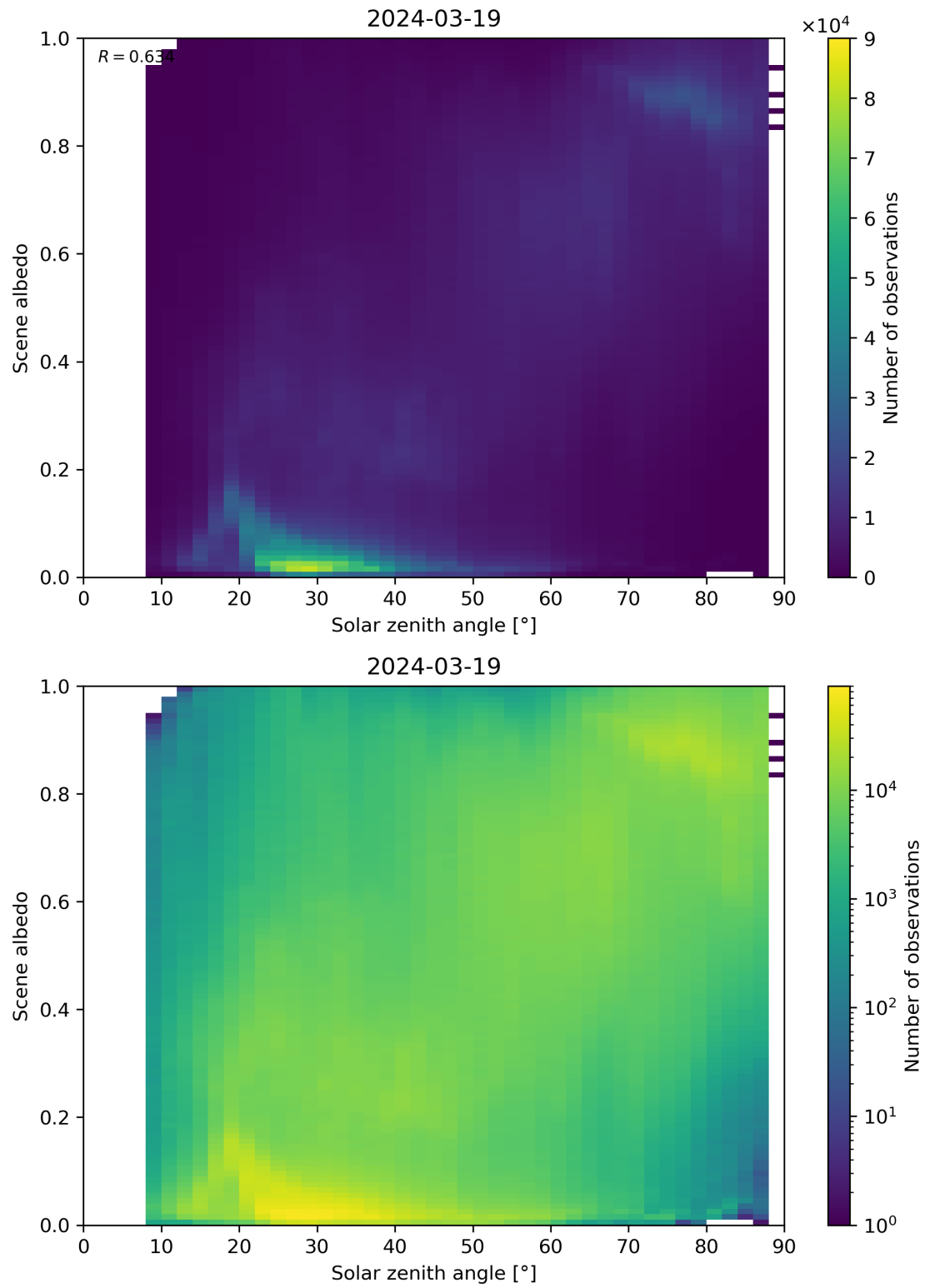
Figure 116: Scatter density plot of “Solar zenith angle” against “Scene albedo” for 2024-03-18 to 2024-03-20.
