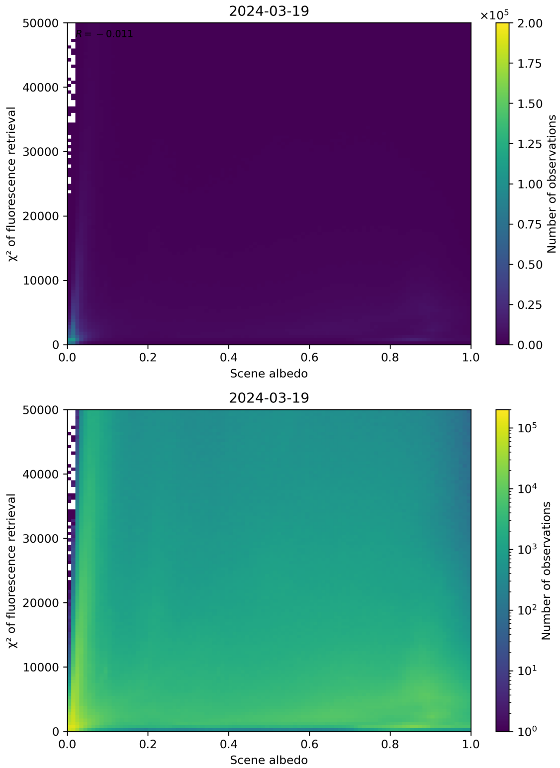
Figure 103: Scatter density plot of “Scene albedo” against “ \chi^2 of fluorescence retrieval” for 2024-03-18 to 2024-03-20.
