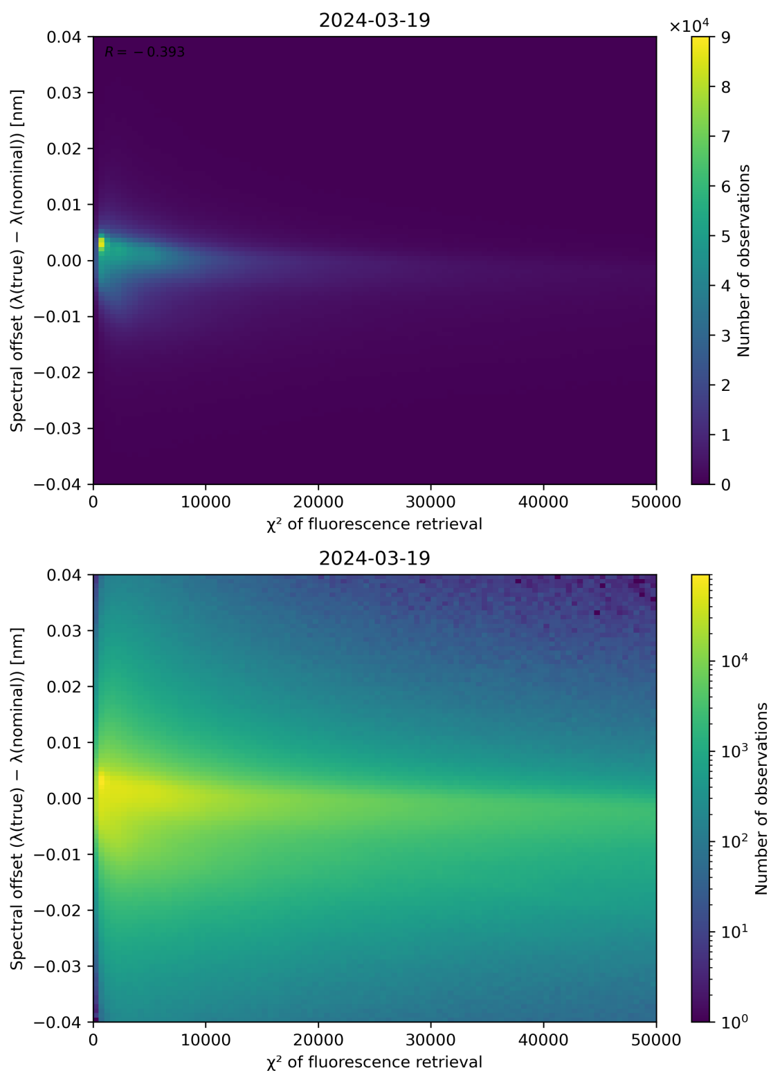
Figure 69: Scatter density plot of " \chi^2 of fluorescence retrieval" against "Spectral offset ( \lambda(\text{true}) - \lambda(\text{nominal}) )" for 2024-03-18 to 2024-03-20.
