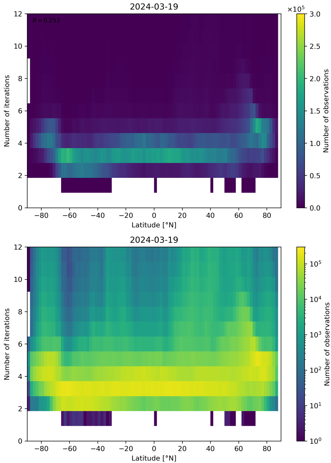
Figure 93: Scatter density plot of “Latitude” against “Number of iterations” for 2024-03-18 to 2024-03-20.
