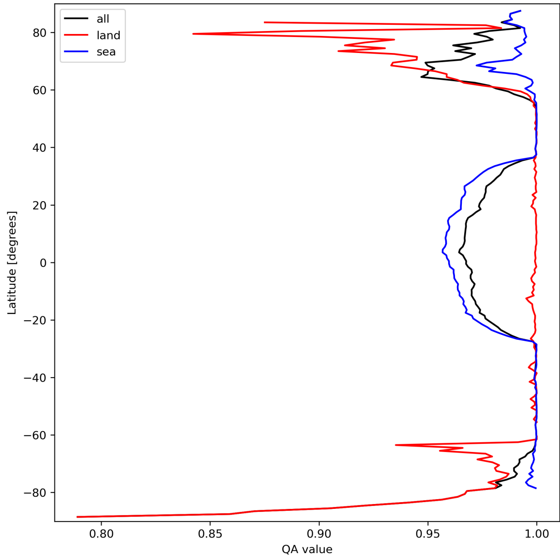
Figure 12: Zonal average of “QA value” for 2024-03-18 to 2024-03-20.
