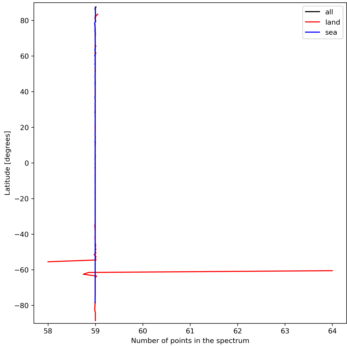
Figure 27: Zonal average of “Number of points in the spectrum” for 2024-03-18 to 2024-03-20.
