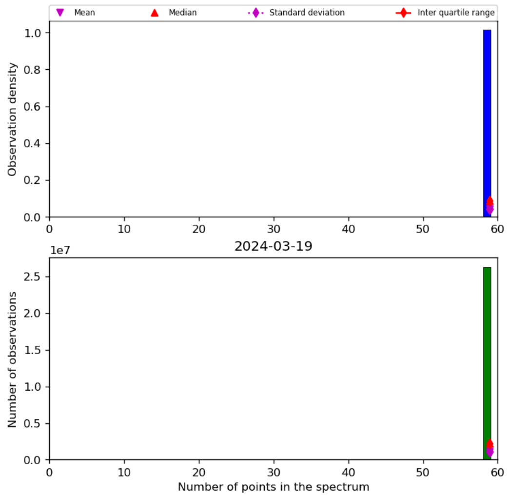
Figure 44: Histogram of “Number of points in the spectrum” for 2024-03-18 to 2024-03-20
