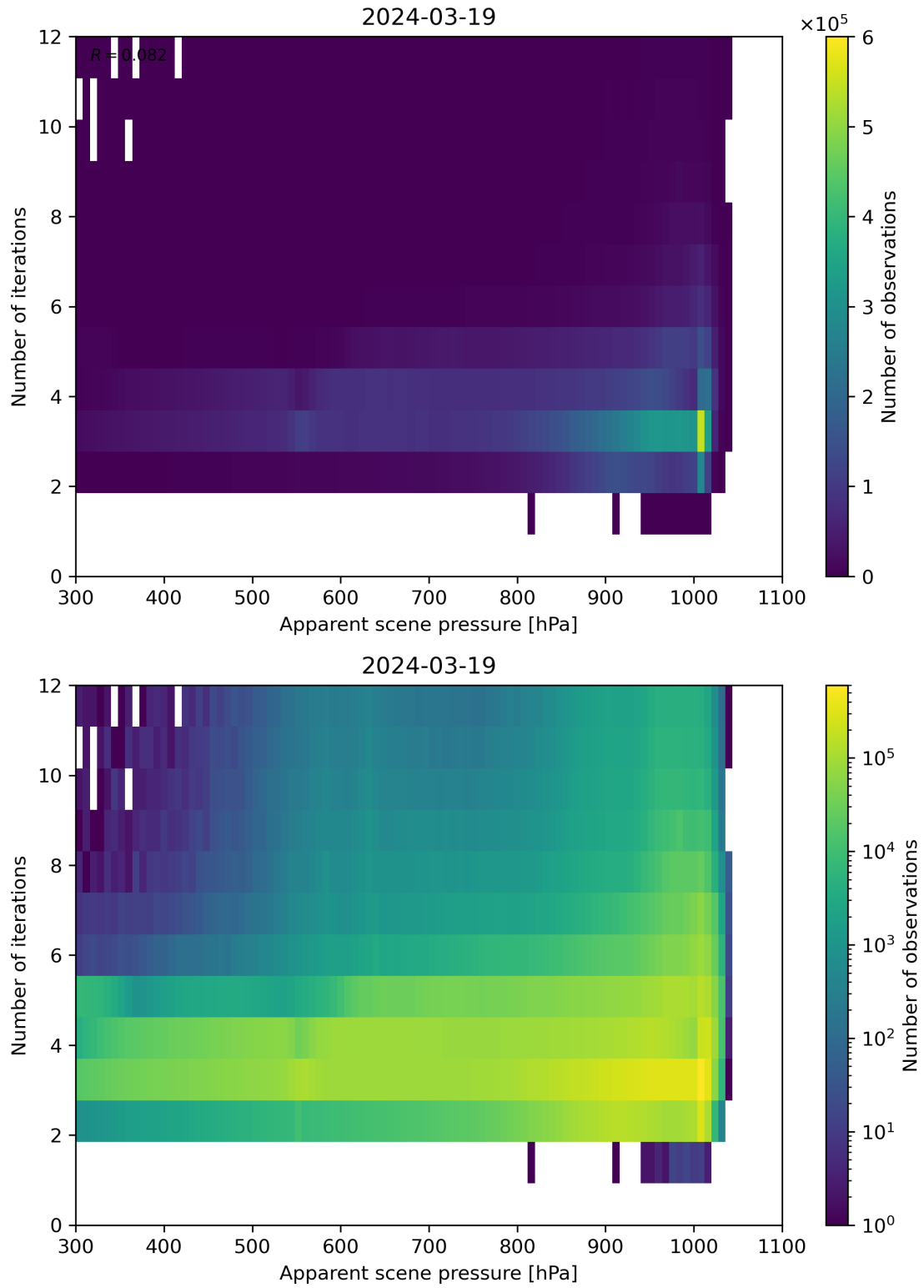
Figure 65: Scatter density plot of “Apparent scene pressure” against “Number of iterations” for 2024-03-18 to 2024-03-20.
