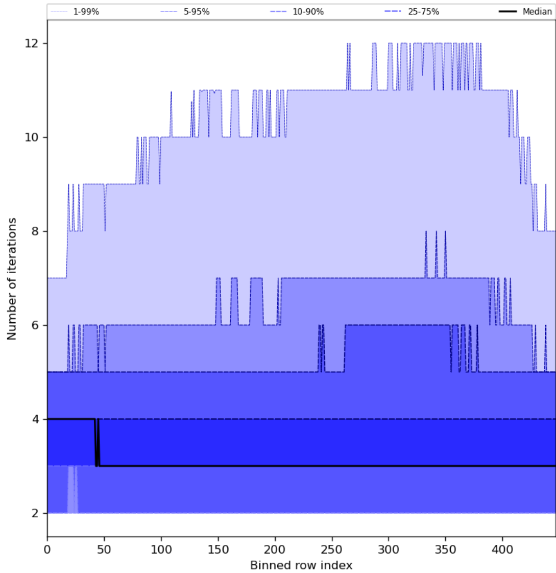
Figure 56: Along track statistics of “Number of iterations” for 2024-03-18 to 2024-03-20
