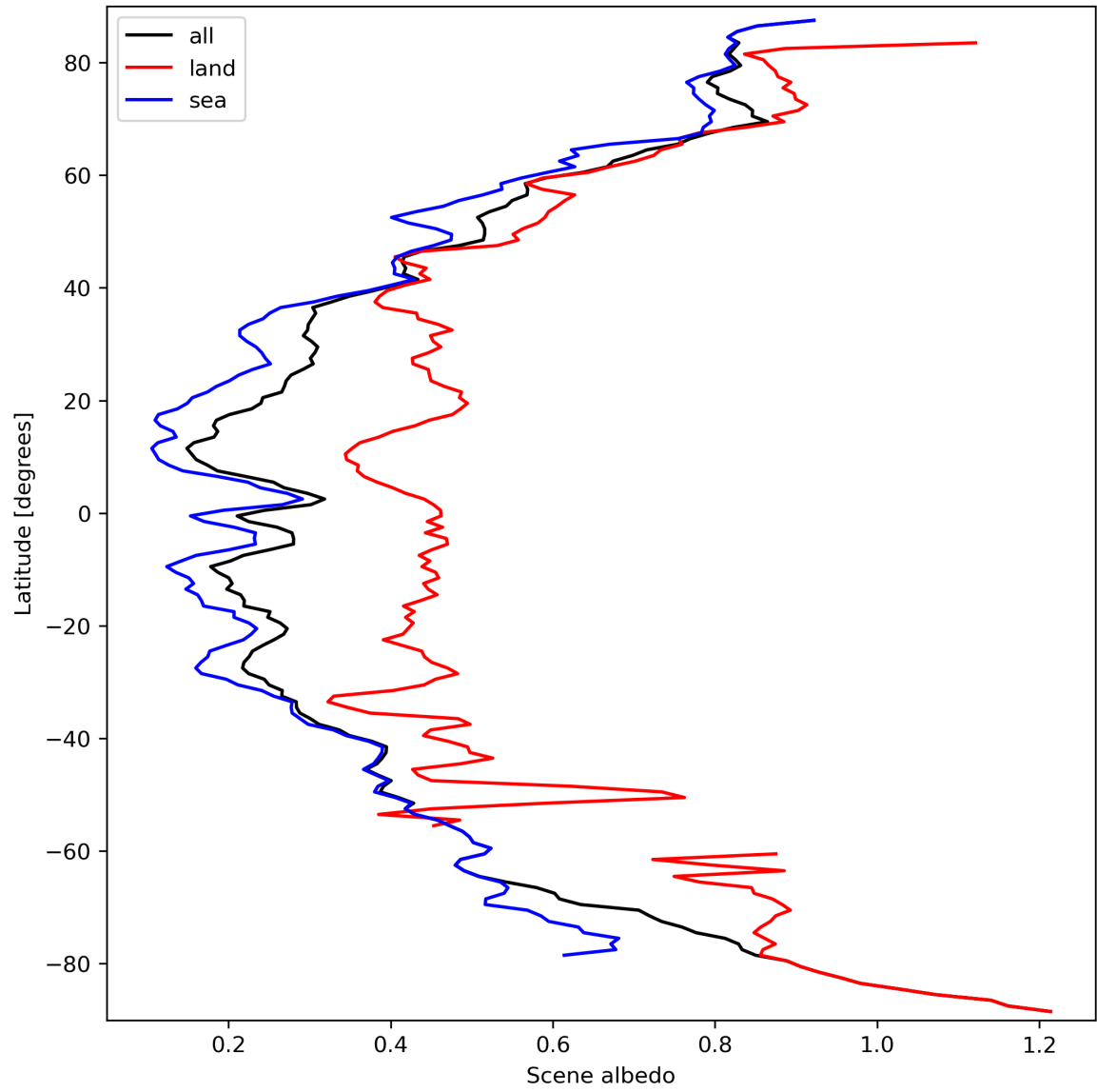
Figure 17: Zonal average of “Scene albedo” for 2024-03-18 to 2024-03-20.
