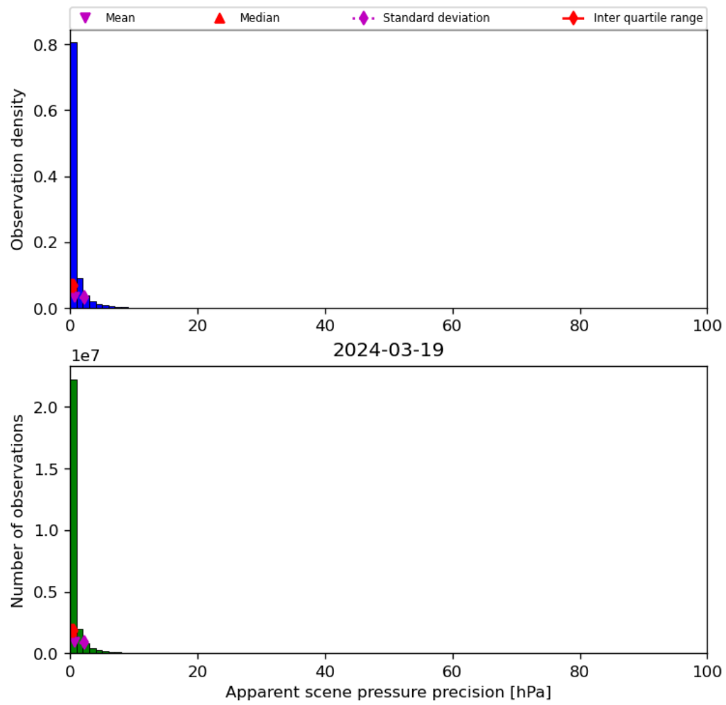
Figure 37: Histogram of “Apparent scene pressure precision” for 2024-03-18 to 2024-03-20
