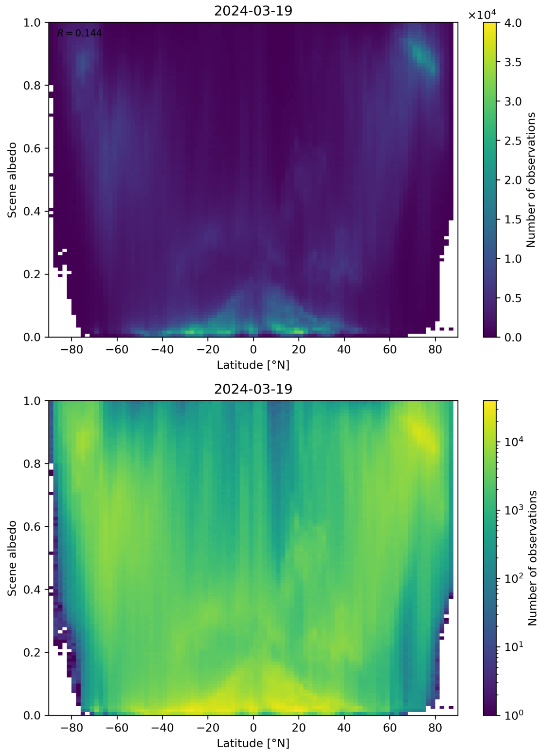
Figure 95: Scatter density plot of “Latitude” against “Scene albedo” for 2024-03-18 to 2024-03-20.
