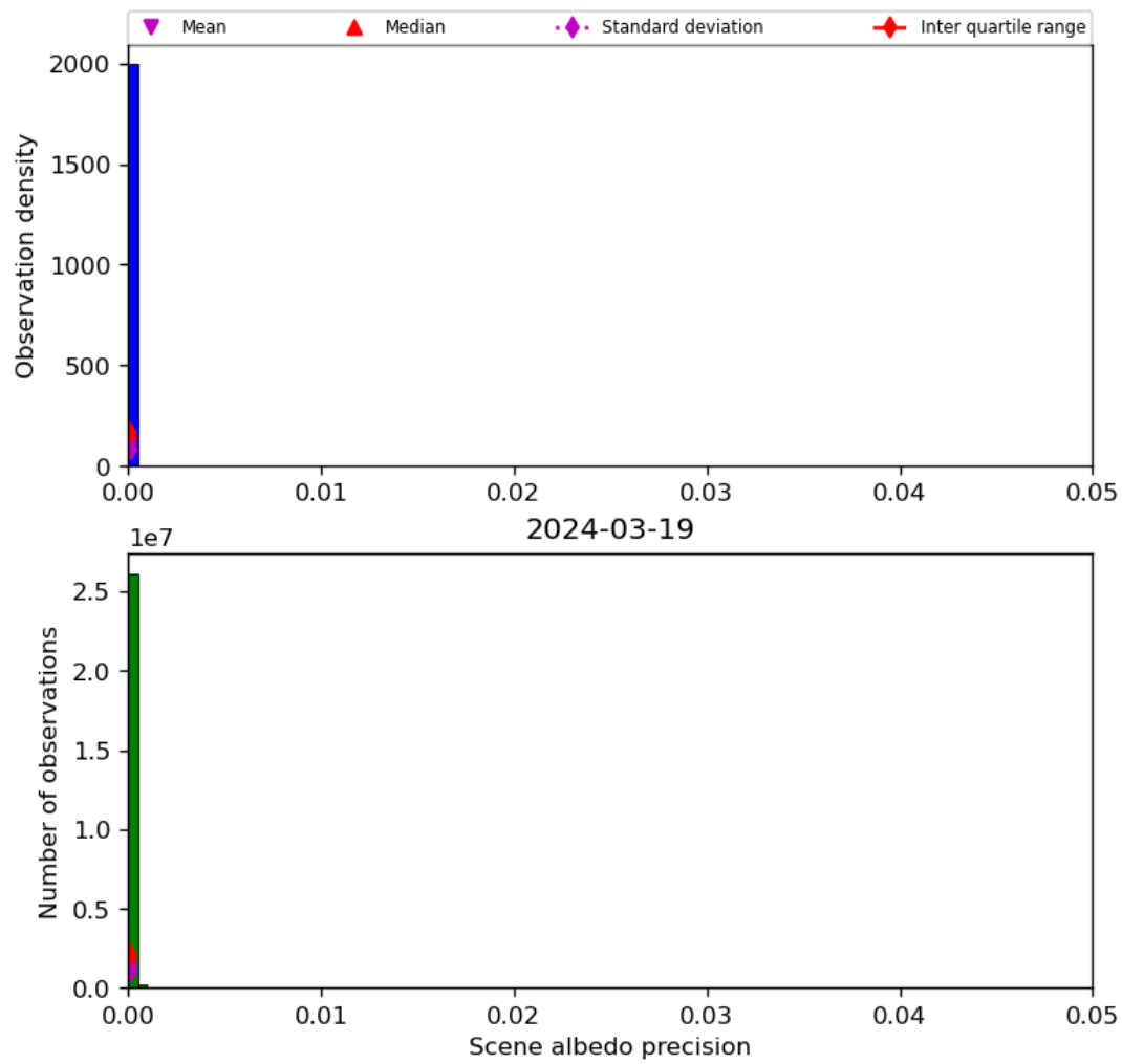
Figure 35: Histogram of “Scene albedo precision” for 2024-03-18 to 2024-03-20
