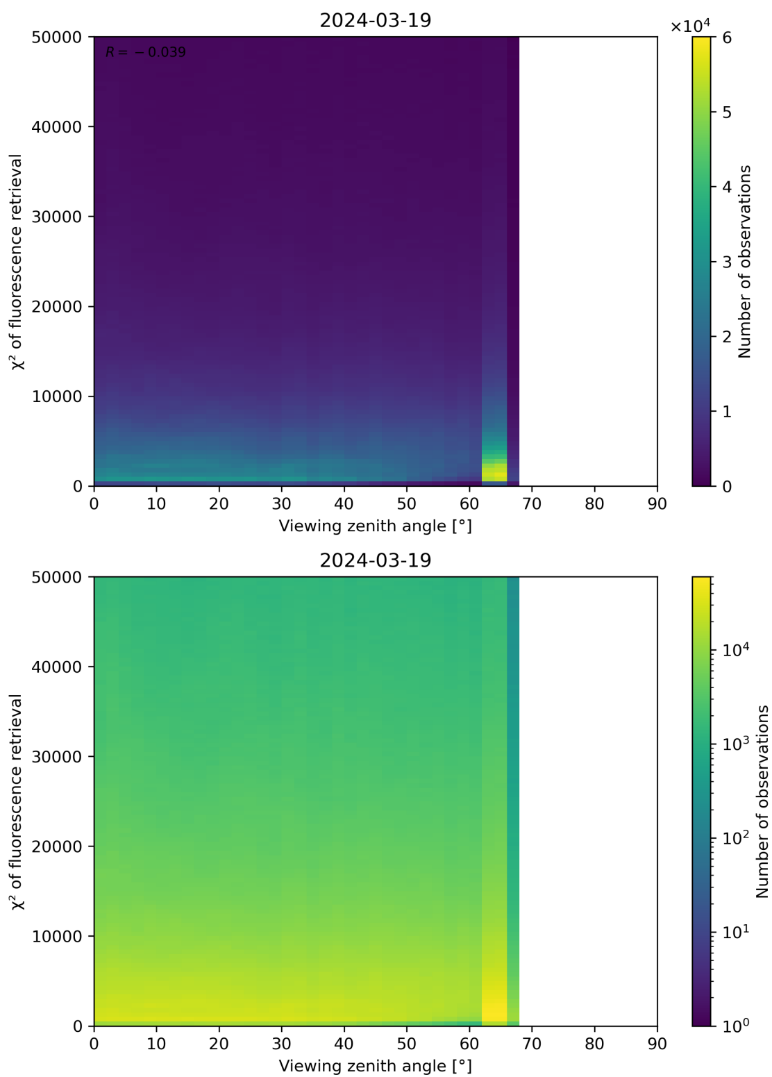
Figure 119: Scatter density plot of “Viewing zenith angle” against “ \chi^2 of fluorescence retrieval” for 2024-03-18 to 2024-03-20.
