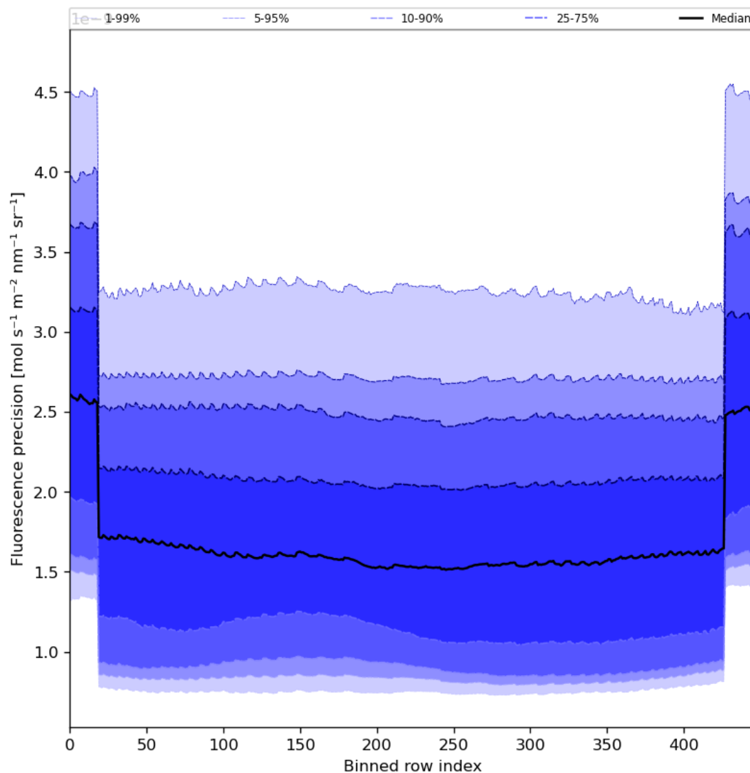
Figure 58: Along track statistics of “Fluorescence precision” for 2024-03-18 to 2024-03-20
