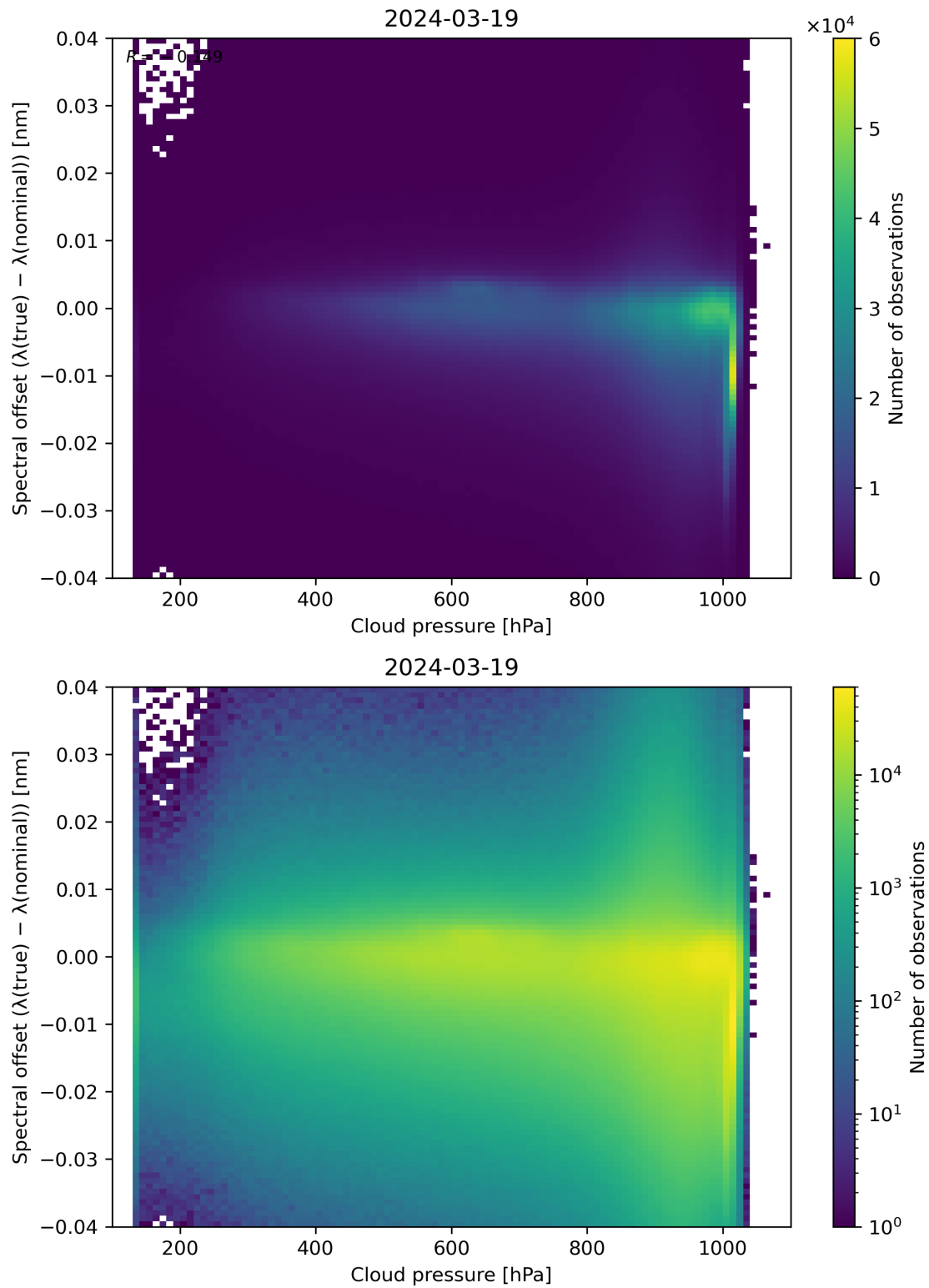
Figure 84: Scatter density plot of “Cloud pressure” against “Spectral offset ( \lambda(\text{true}) - \lambda(\text{nominal}) )” for 2024-03-18 to 2024-03-20.
