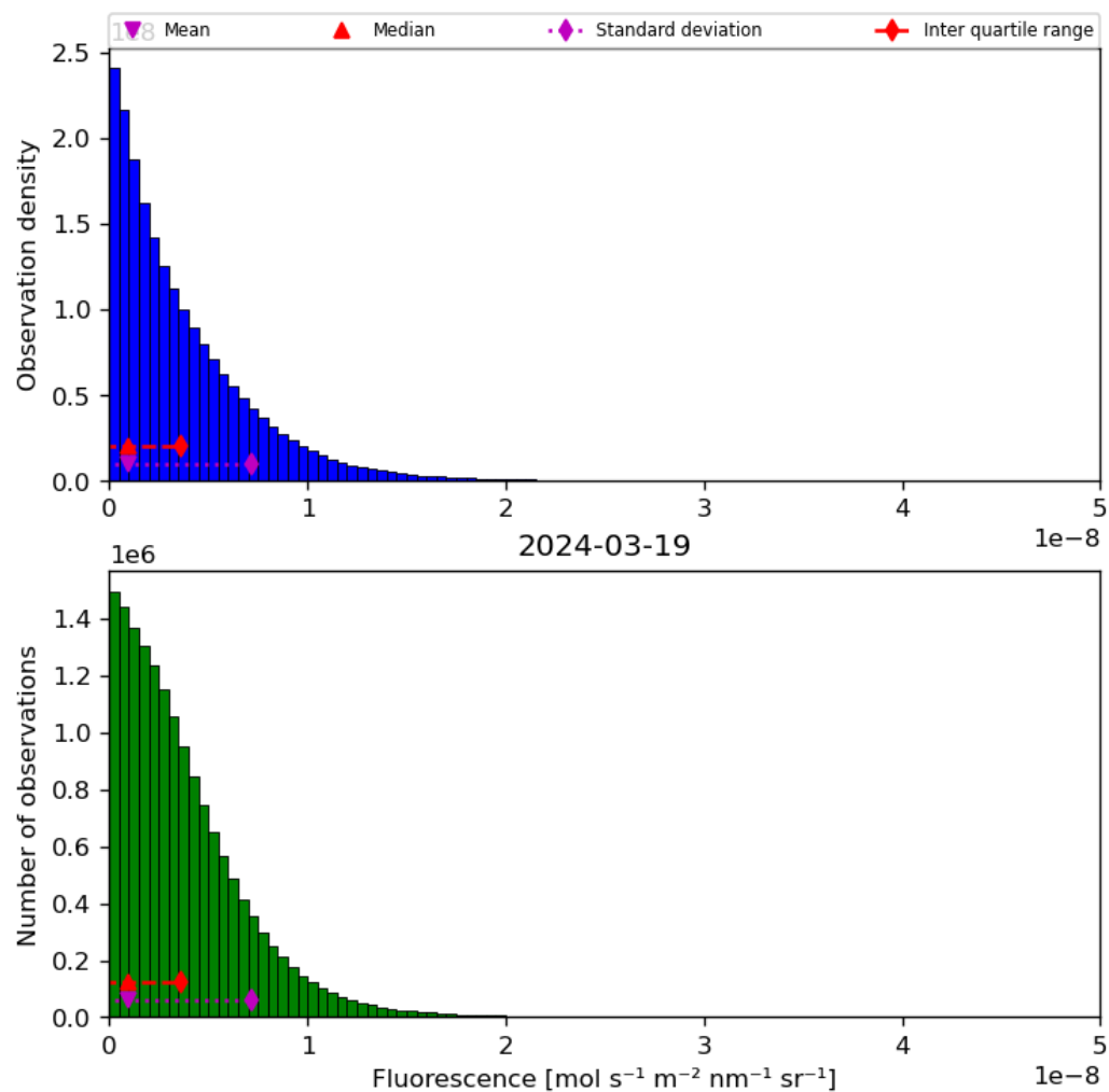
Figure 40: Histogram of “Fluorescence” for 2024-03-18 to 2024-03-20
