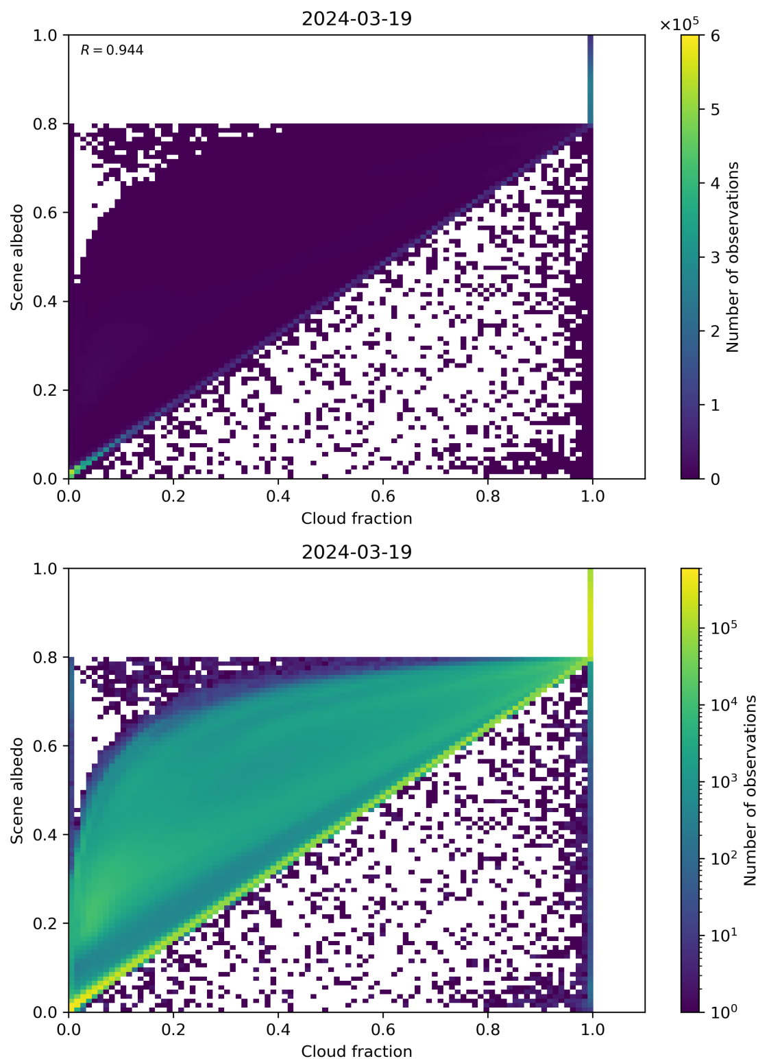
Figure 75: Scatter density plot of “Cloud fraction” against “Scene albedo” for 2024-03-18 to 2024-03-20.
