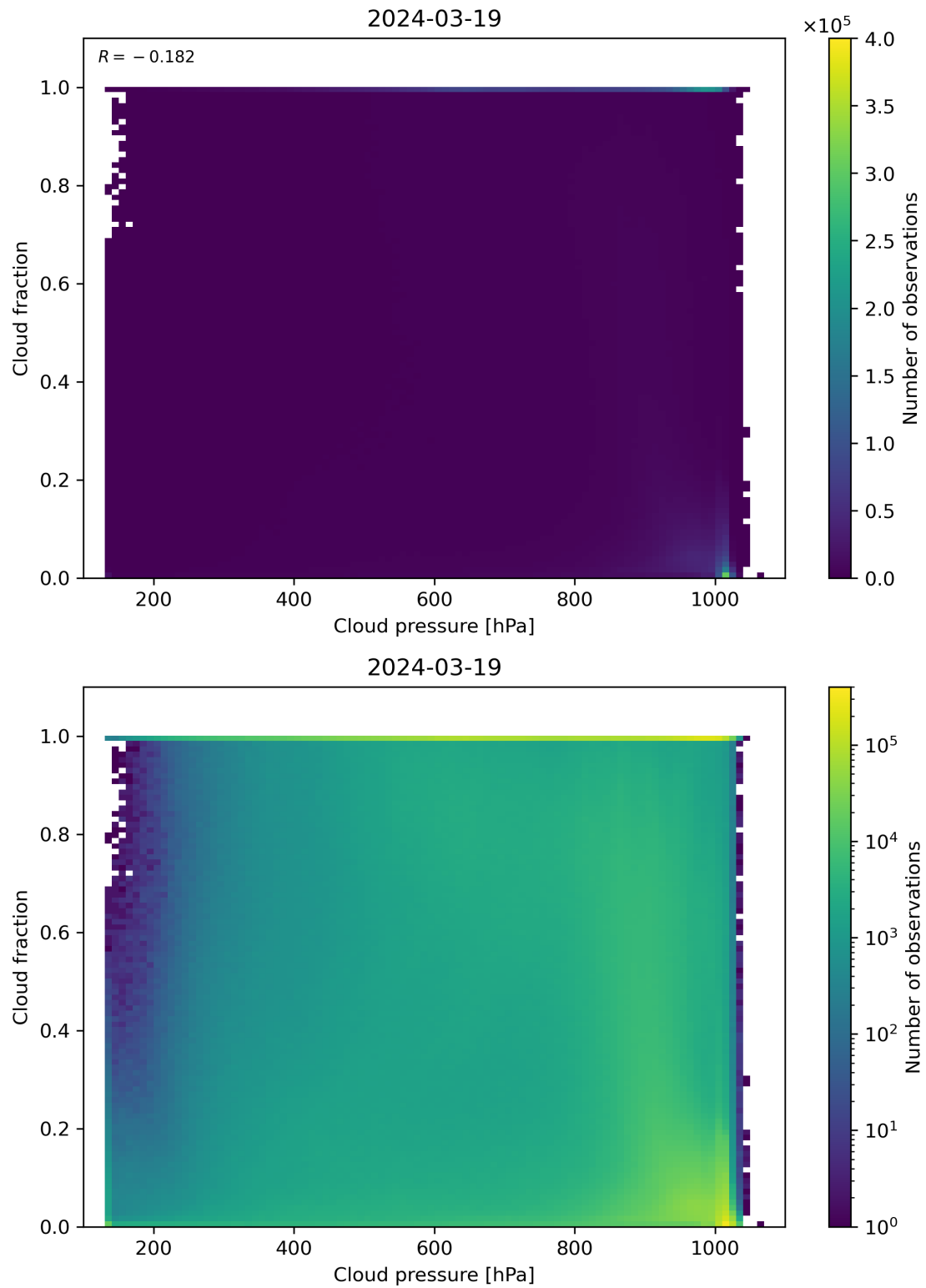
Figure 79: Scatter density plot of “Cloud pressure” against “Cloud fraction” for 2024-03-18 to 2024-03-20.
