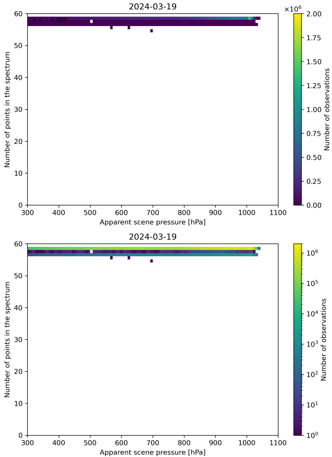
Figure 66: Scatter density plot of “Apparent scene pressure” against “Number of points in the spectrum” for 2024-03-18 to 2024-03-20.
