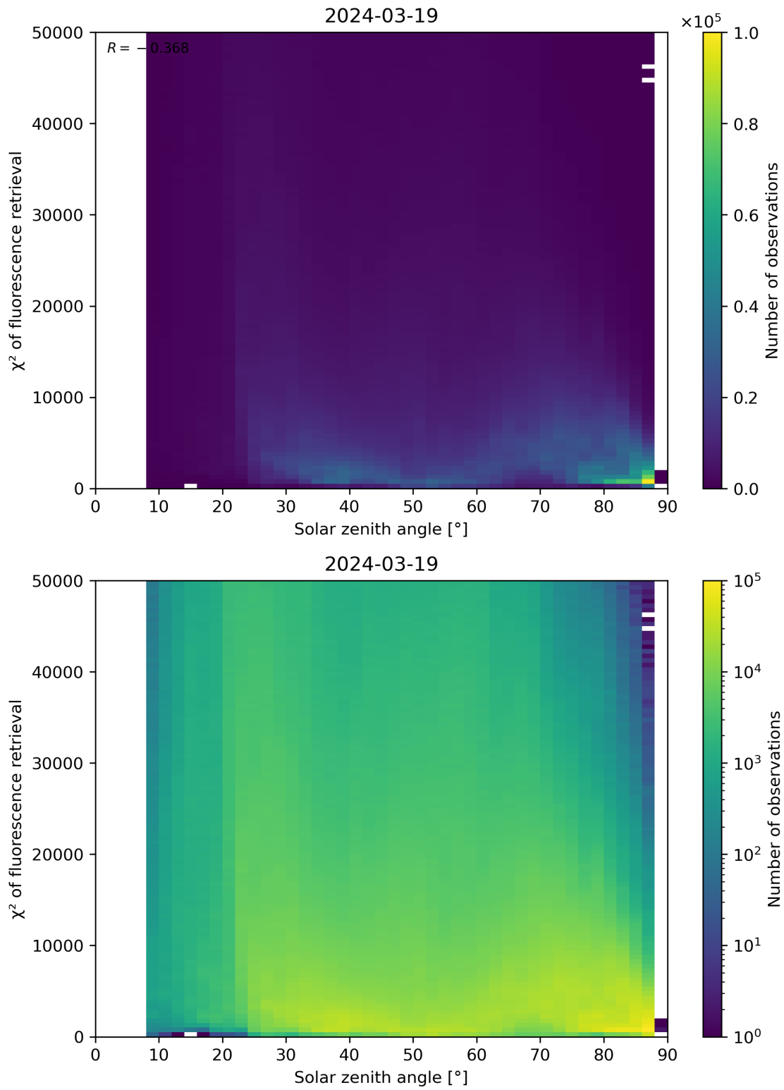
Figure 109: Scatter density plot of “Solar zenith angle” against “ \chi^2 of fluorescence retrieval” for 2024-03-18 to 2024-03-20.
