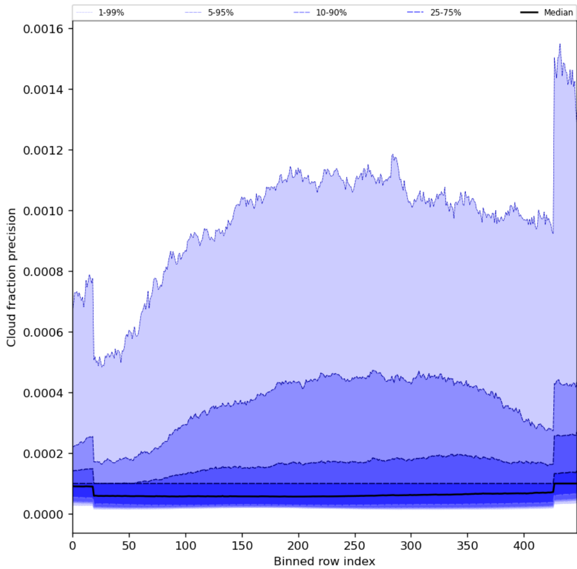
Figure 50: Along track statistics of “Cloud fraction precision” for 2024-03-18 to 2024-03-20
