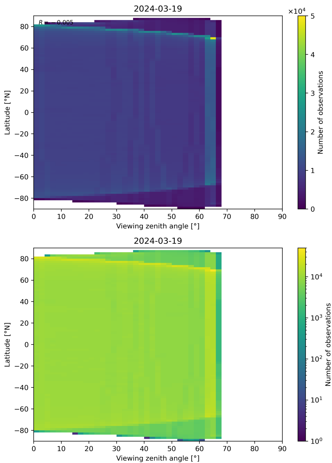
Figure 123: Scatter density plot of “Viewing zenith angle” against “Latitude” for 2024-03-18 to 2024-03-20.
