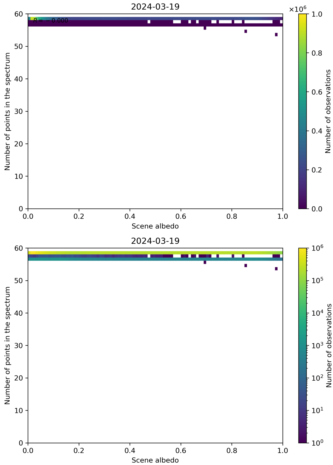
Figure 106: Scatter density plot of “Scene albedo” against “Number of points in the spectrum” for 2024-03-18 to 2024-03-20.
