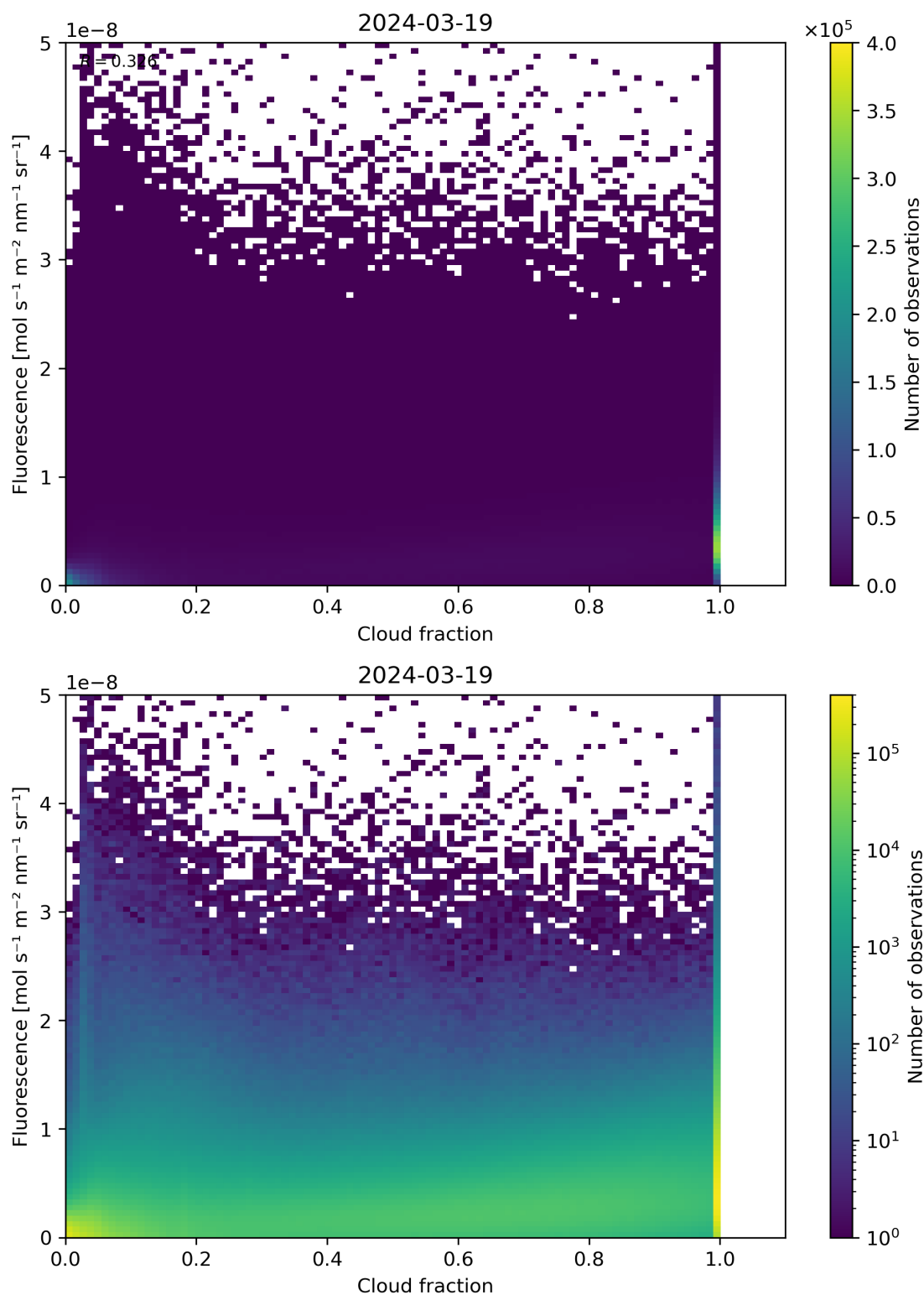
Figure 72: Scatter density plot of “Cloud fraction” against “Fluorescence” for 2024-03-18 to 2024-03-20.
