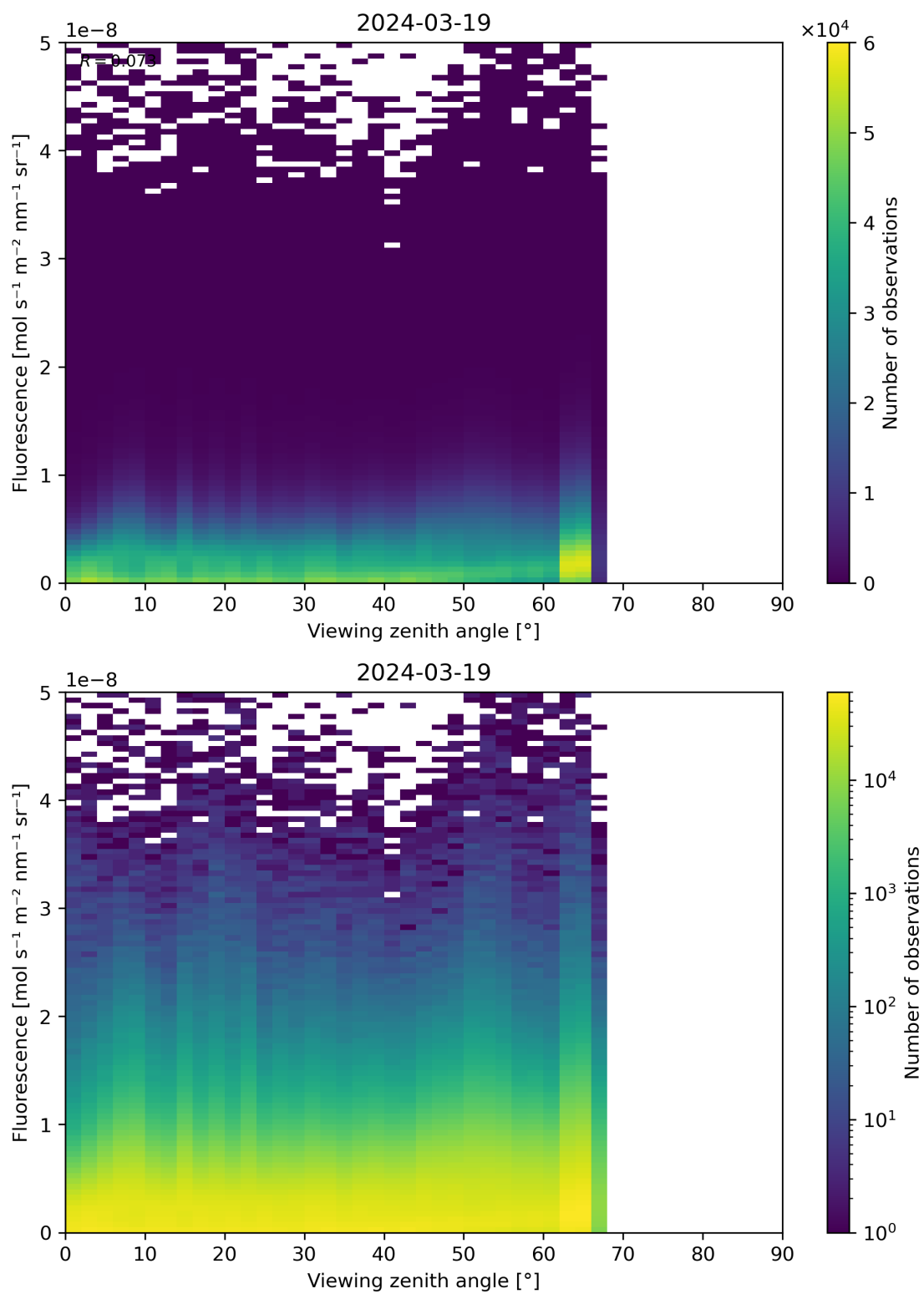
Figure 122: Scatter density plot of “Viewing zenith angle” against “Fluorescence” for 2024-03-18 to 2024-03-20.
