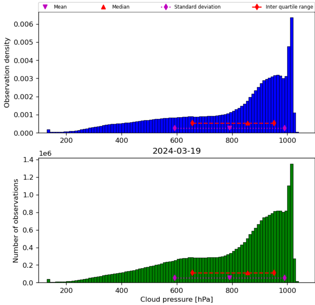
Figure 30: Histogram of “Cloud pressure” for 2024-03-18 to 2024-03-20
