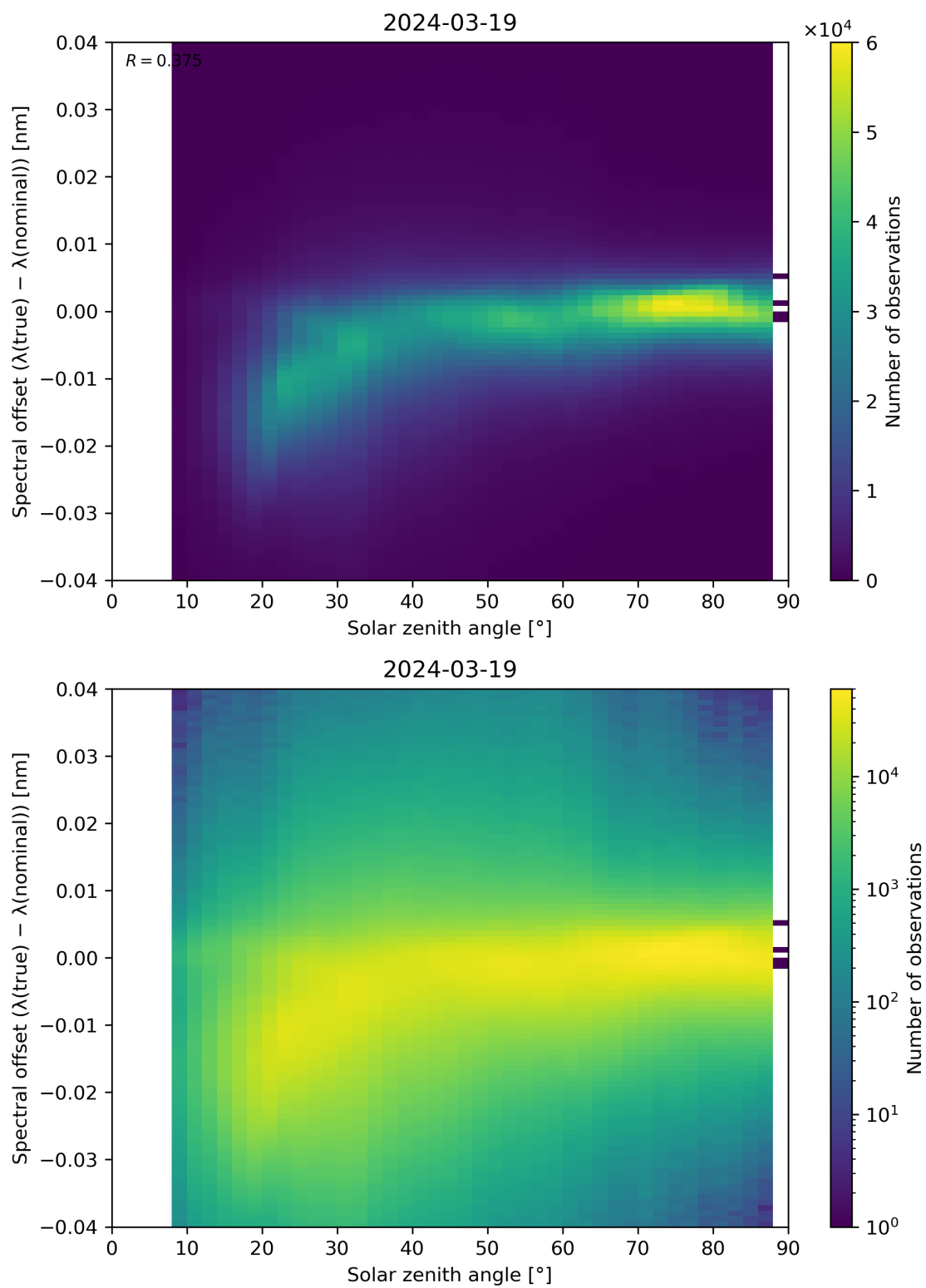
Figure 117: Scatter density plot of “Solar zenith angle” against “Spectral offset ( \lambda(\text{true}) - \lambda(\text{nominal}) )” for 2024-03-18 to 2024-03-20.
