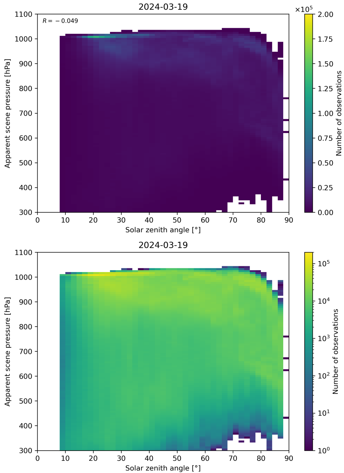
Figure 108: Scatter density plot of “Solar zenith angle” against “Apparent scene pressure” for 2024-03-18 to 2024-03-20.
