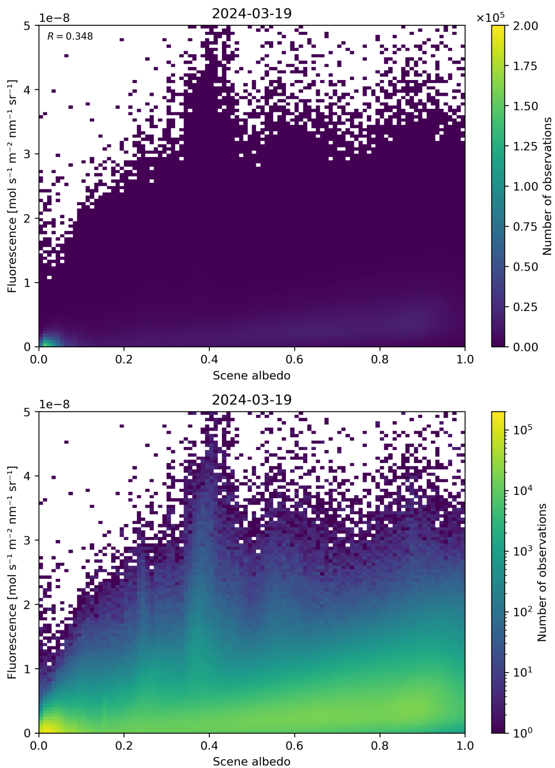
Figure 104: Scatter density plot of “Scene albedo” against “Fluorescence” for 2024-03-18 to 2024-03-20.
