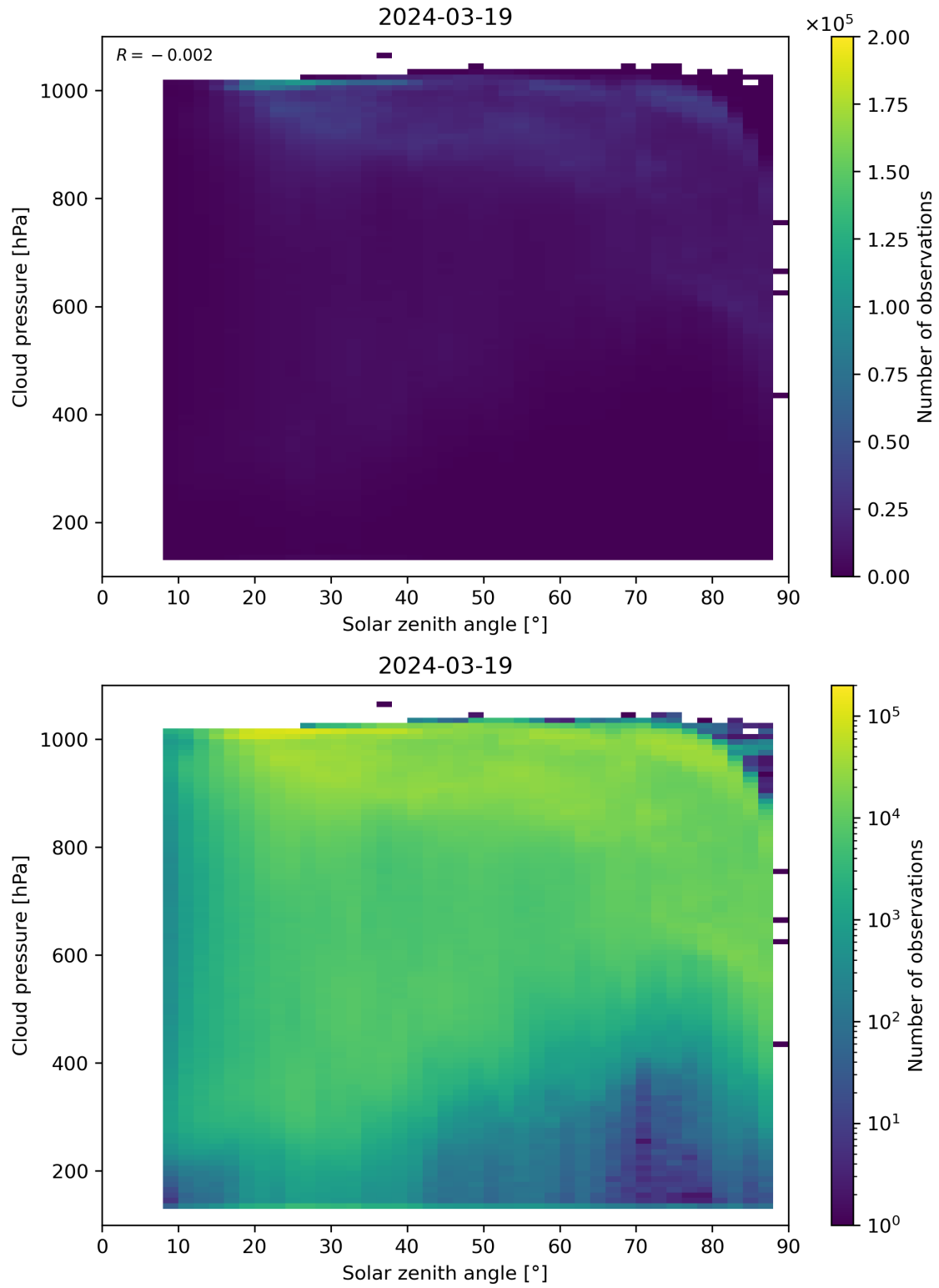
Figure 111: Scatter density plot of “Solar zenith angle” against “Cloud pressure” for 2024-03-18 to 2024-03-20.
