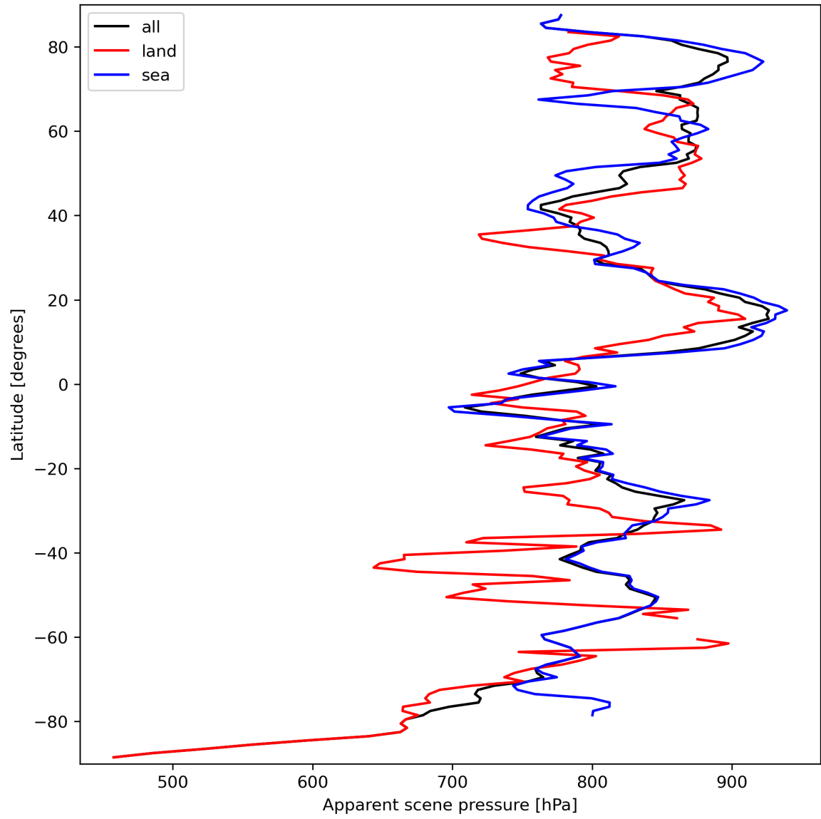
Figure 19: Zonal average of “Apparent scene pressure” for 2024-03-18 to 2024-03-20.
