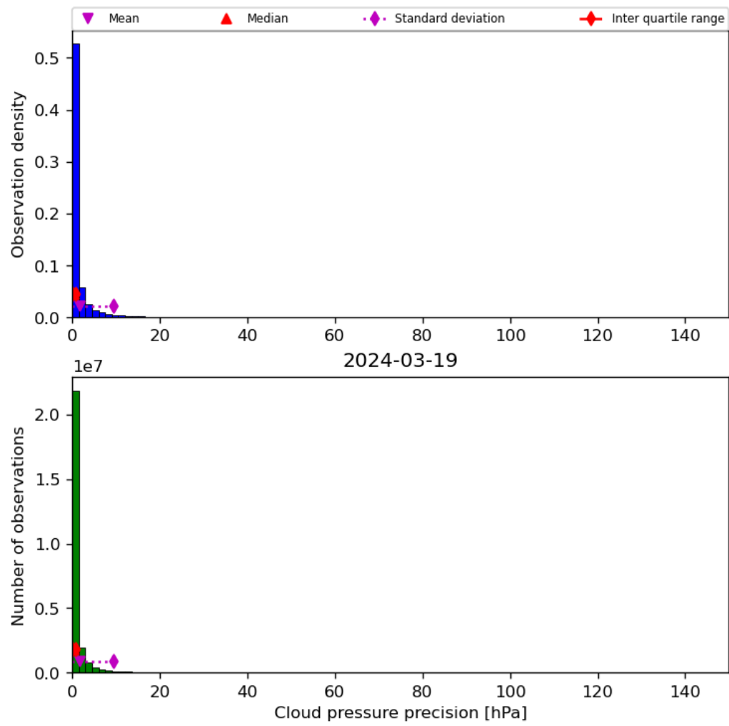
Figure 31: Histogram of “Cloud pressure precision” for 2024-03-18 to 2024-03-20
