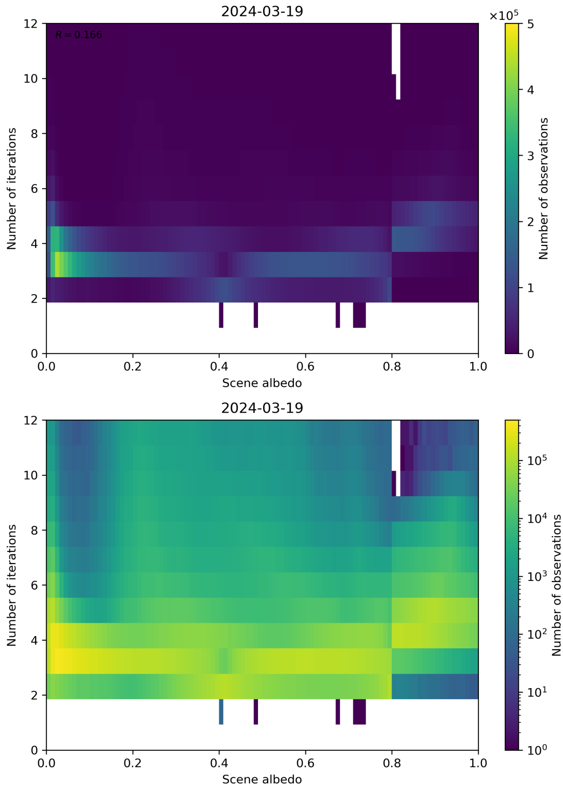
Figure 105: Scatter density plot of “Scene albedo” against “Number of iterations” for 2024-03-18 to 2024-03-20.
