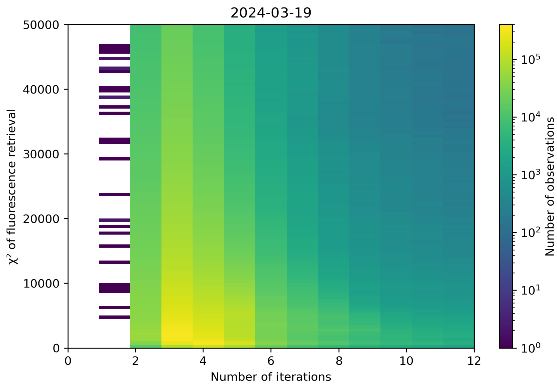
Figure 97: Scatter density plot of “Number of iterations” against “ \chi^2 of fluorescence retrieval” for 2024-03-18 to 2024-03-20.
