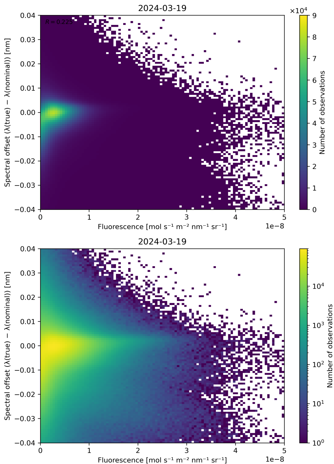
Figure 87: Scatter density plot of “Fluorescence” against “Spectral offset ( \lambda(\text{true}) - \lambda(\text{nominal}) )” for 2024-03-18 to 2024-03-20.
