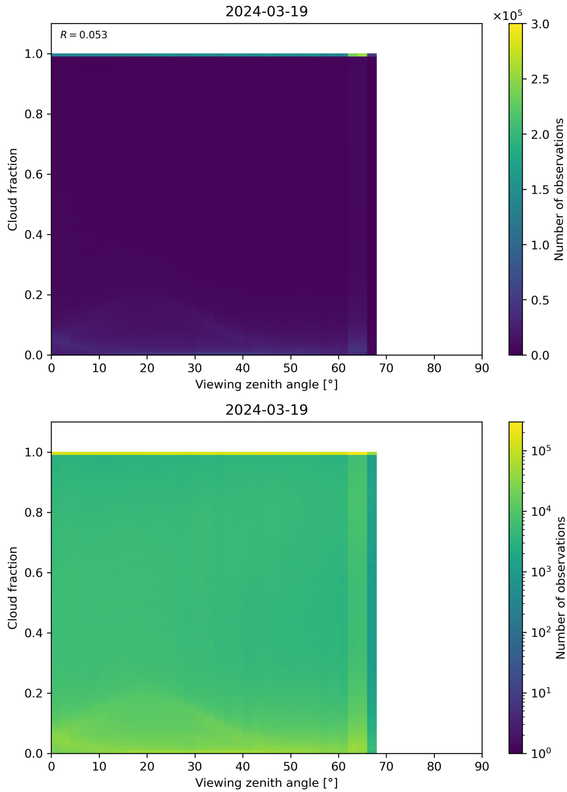
Figure 120: Scatter density plot of “Viewing zenith angle” against “Cloud fraction” for 2024-03-18 to 2024-03-20.
