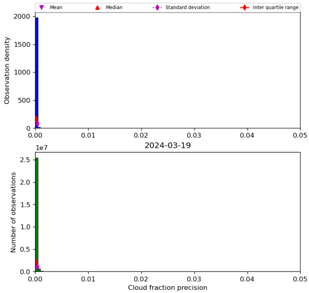
Figure 33: Histogram of “Cloud fraction precision” for 2024-03-18 to 2024-03-20
