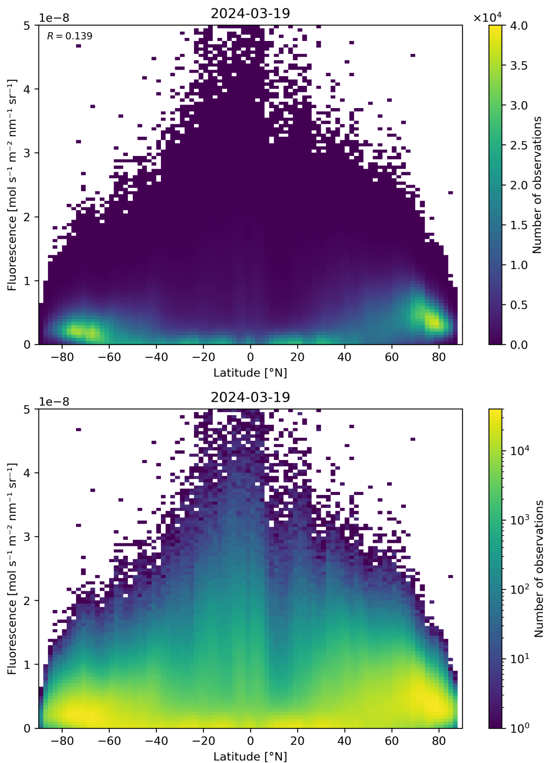
Figure 92: Scatter density plot of “Latitude” against “Fluorescence” for 2024-03-18 to 2024-03-20.
