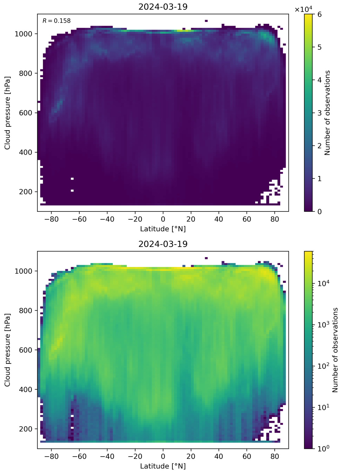
Figure 91: Scatter density plot of “Latitude” against “Cloud pressure” for 2024-03-18 to 2024-03-20.
