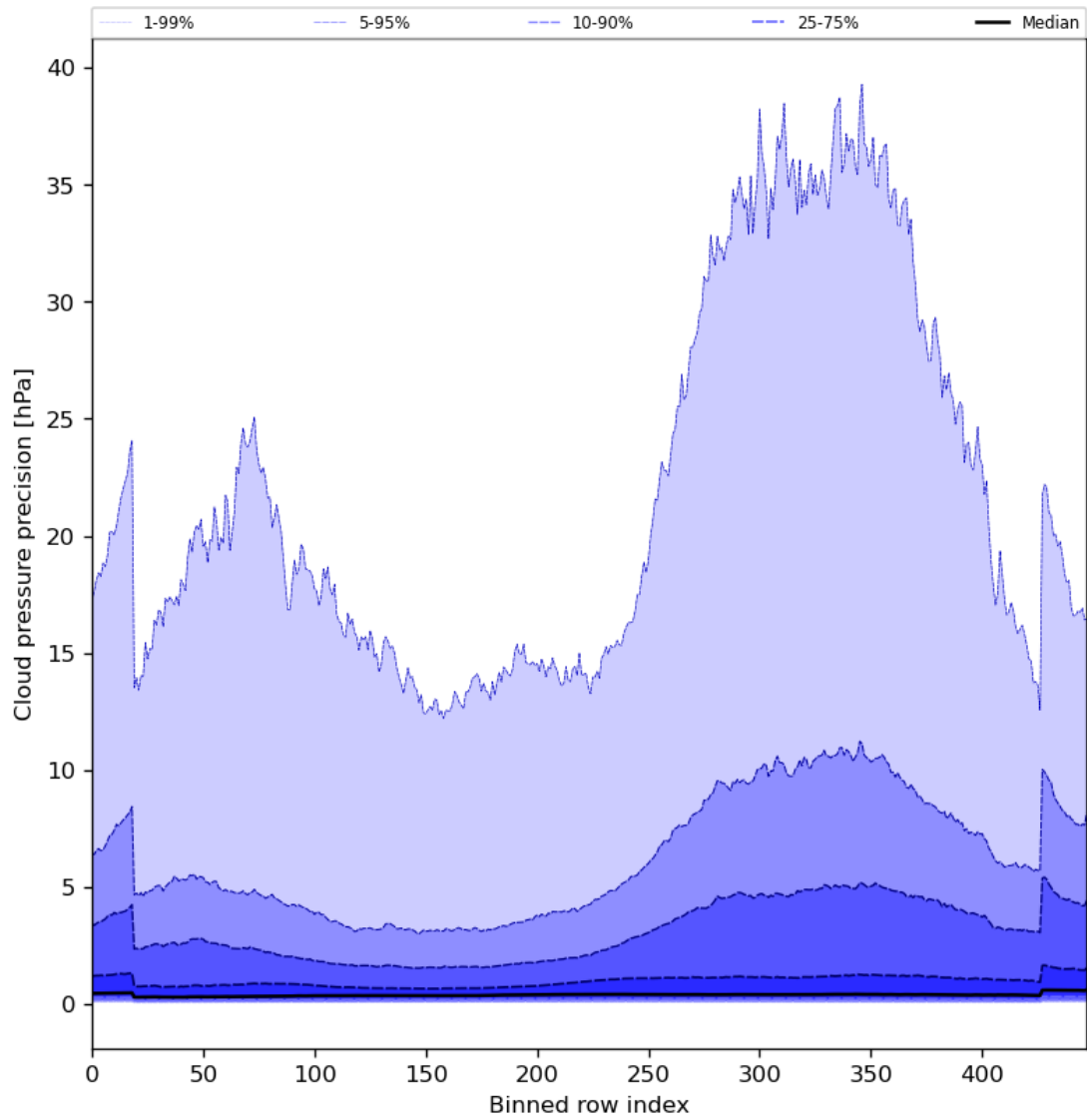
Figure 48: Along track statistics of “Cloud pressure precision” for 2024-03-18 to 2024-03-20
