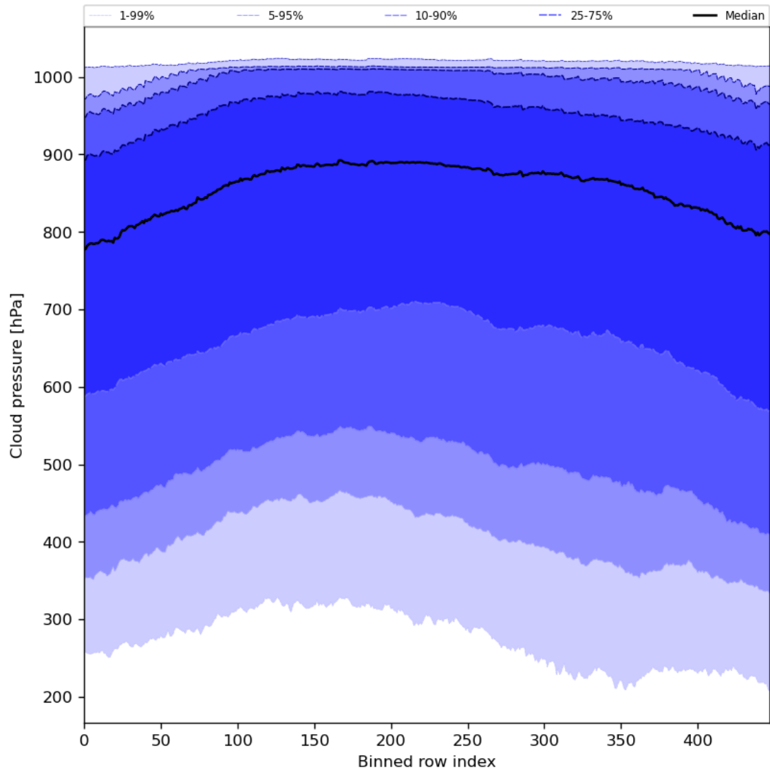
Figure 47: Along track statistics of “Cloud pressure” for 2024-03-18 to 2024-03-20
