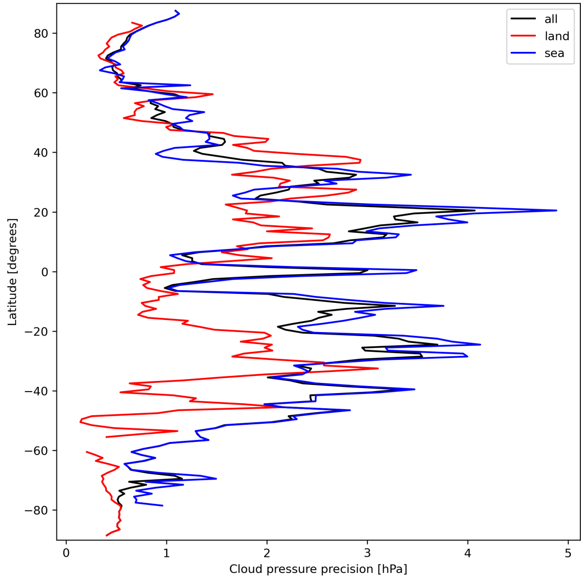
Figure 14: Zonal average of “Cloud pressure precision” for 2024-03-18 to 2024-03-20.
