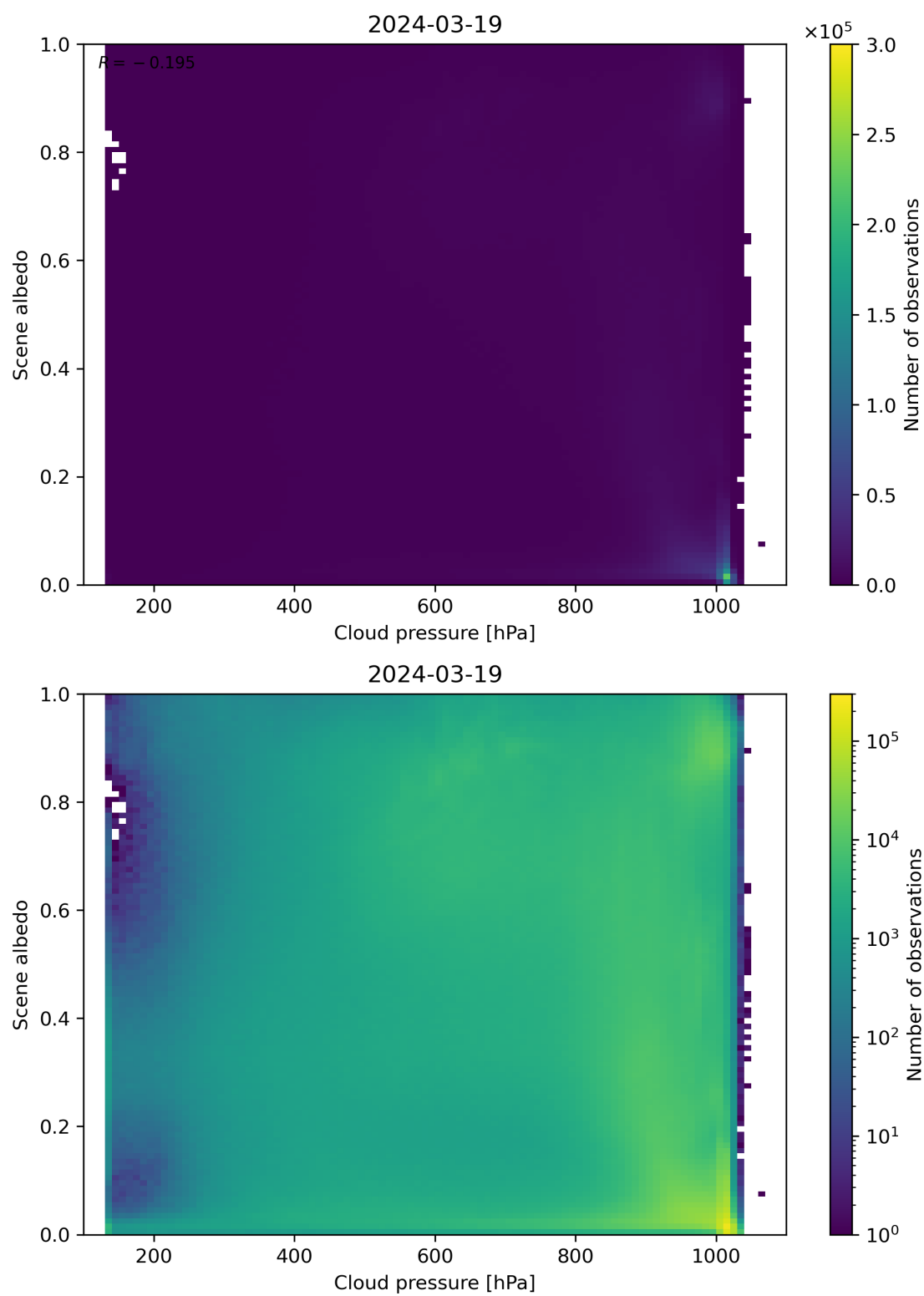
Figure 83: Scatter density plot of “Cloud pressure” against “Scene albedo” for 2024-03-18 to 2024-03-20.
