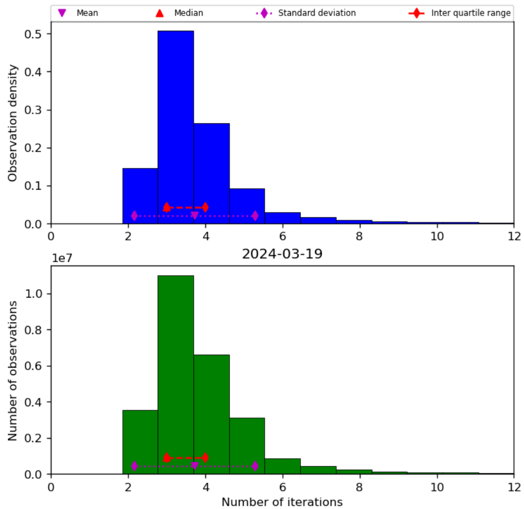
Figure 39: Histogram of “Number of iterations” for 2024-03-18 to 2024-03-20
