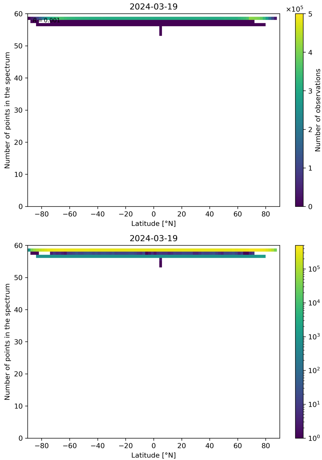
Figure 94: Scatter density plot of “Latitude” against “Number of points in the spectrum” for 2024-03-18 to 2024-03-20.
