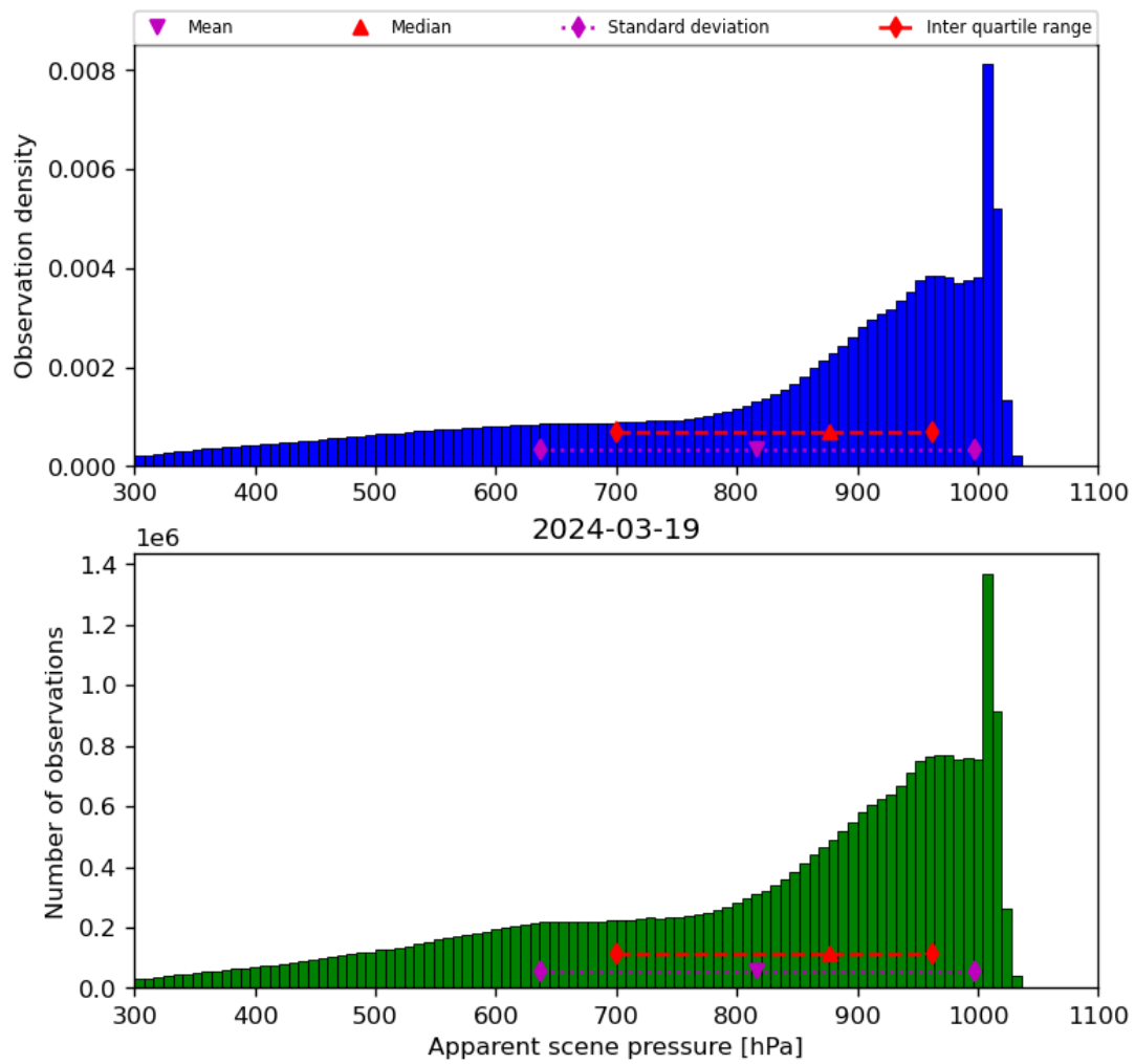
Figure 36: Histogram of “Apparent scene pressure” for 2024-03-18 to 2024-03-20
