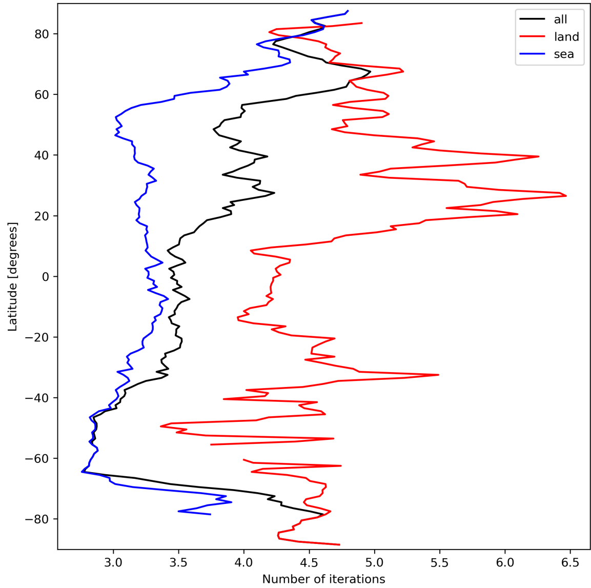
Figure 22: Zonal average of “Number of iterations” for 2024-03-18 to 2024-03-20.
