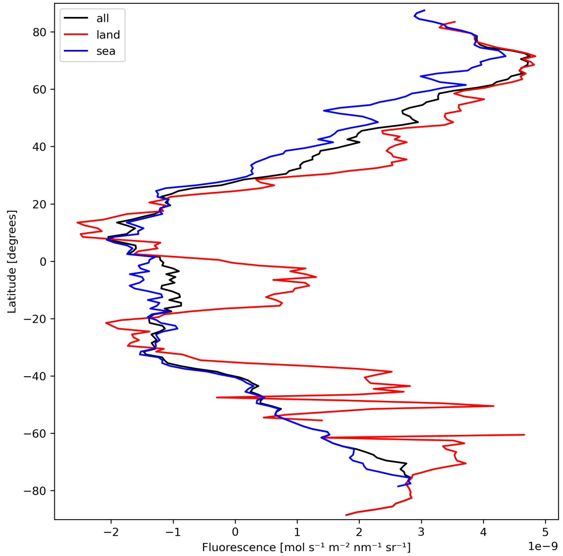
Figure 23: Zonal average of “Fluorescence” for 2024-03-18 to 2024-03-20.
