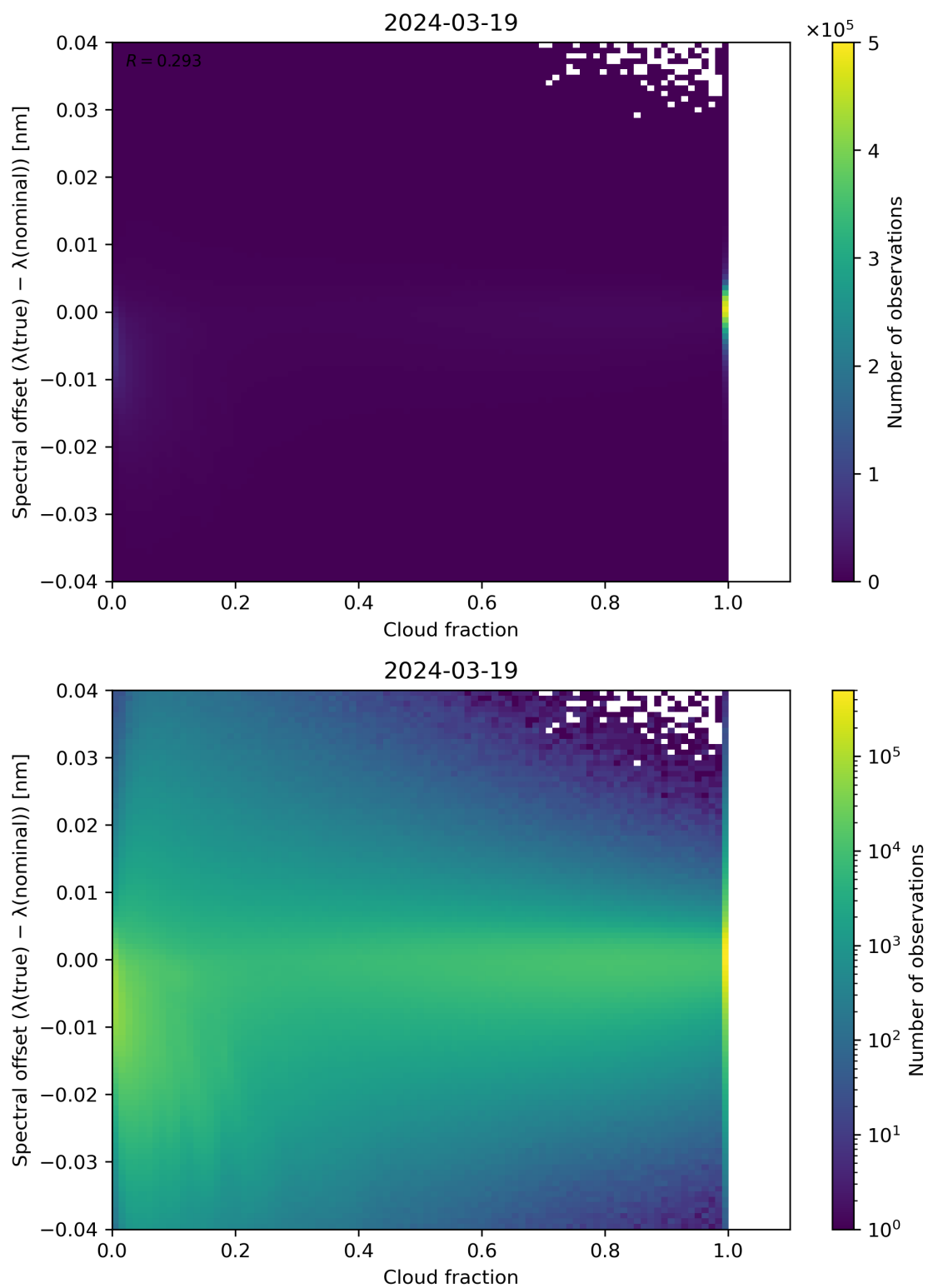
Figure 76: Scatter density plot of “Cloud fraction” against “Spectral offset ( \lambda(\text{true}) - \lambda(\text{nominal}) )” for 2024-03-18 to 2024-03-20.
