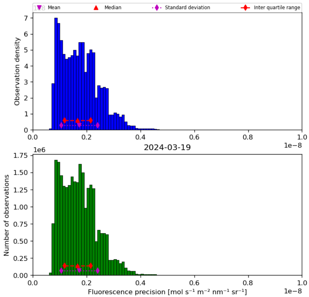
Figure 41: Histogram of “Fluorescence precision” for 2024-03-18 to 2024-03-20
