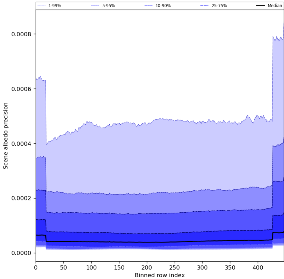
Figure 52: Along track statistics of “Scene albedo precision” for 2024-03-18 to 2024-03-20
