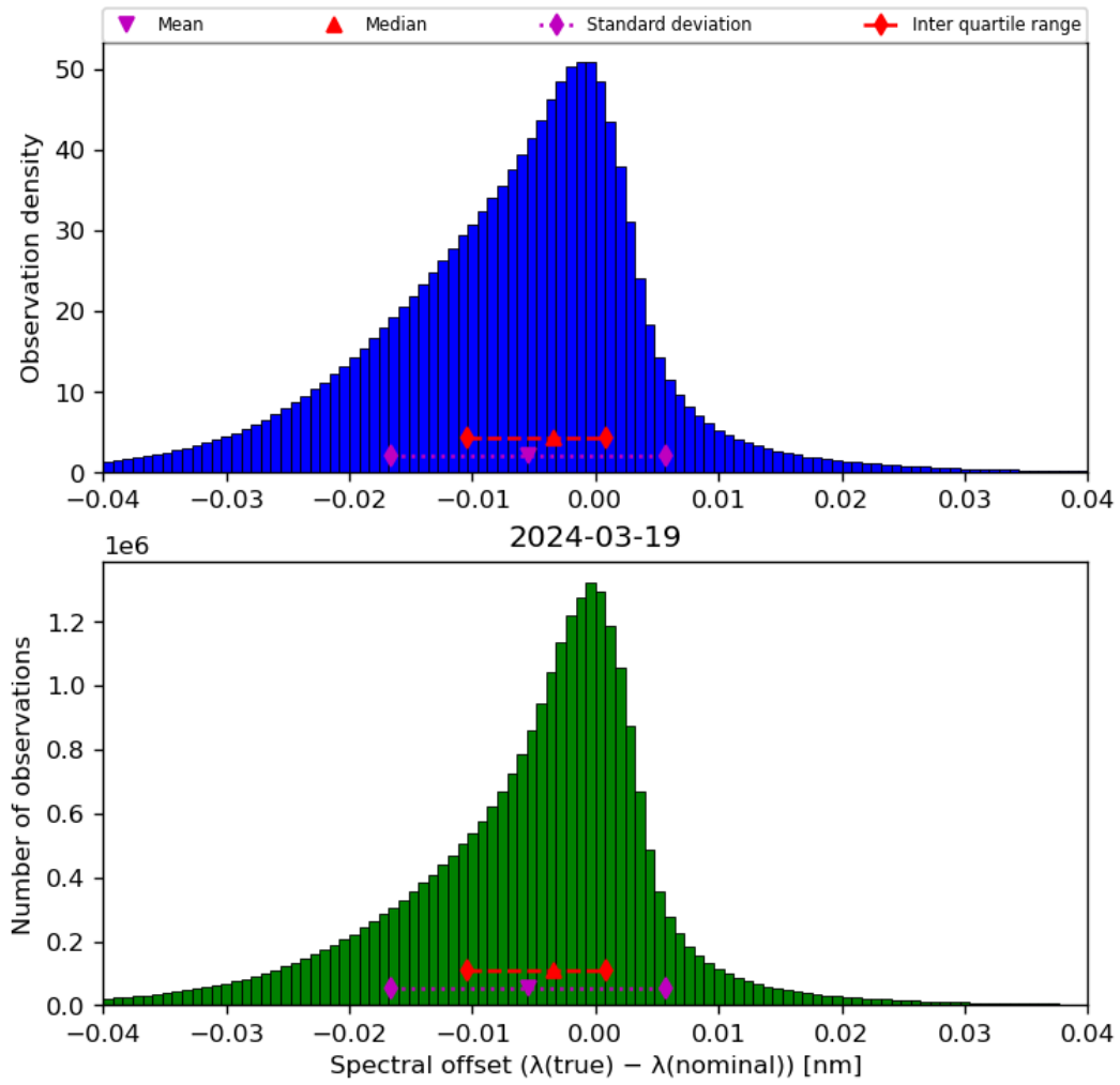
Figure 45: Histogram of “Spectral offset ( \lambda(\text{true}) - \lambda(\text{nominal}) )” for 2024-03-18 to 2024-03-20
