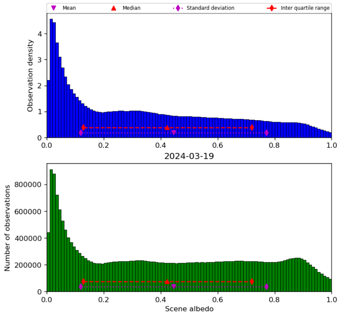
Figure 34: Histogram of “Scene albedo” for 2024-03-18 to 2024-03-20
