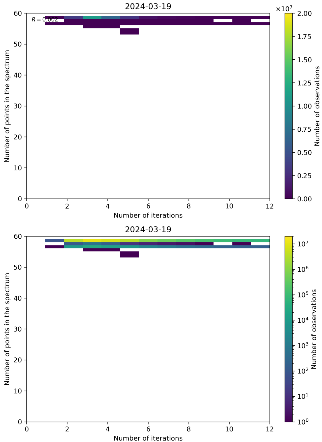
Figure 99: Scatter density plot of “Number of iterations” against “Number of points in the spectrum” for 2024-03-18 to 2024-03-20.
