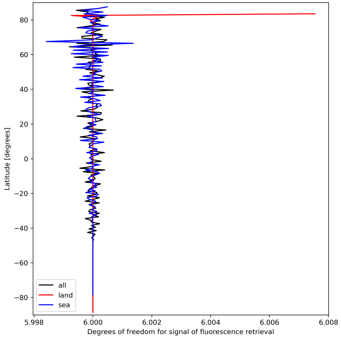
Figure 26: Zonal average of “Degrees of freedom for signal of fluorescence retrieval” for 2024-03-18 to 2024-03-20.
