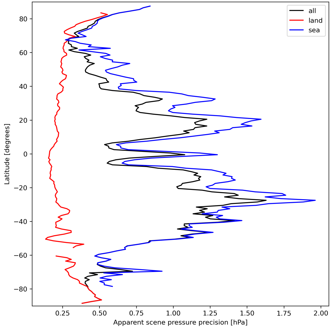
Figure 20: Zonal average of “Apparent scene pressure precision” for 2024-03-18 to 2024-03-20.
