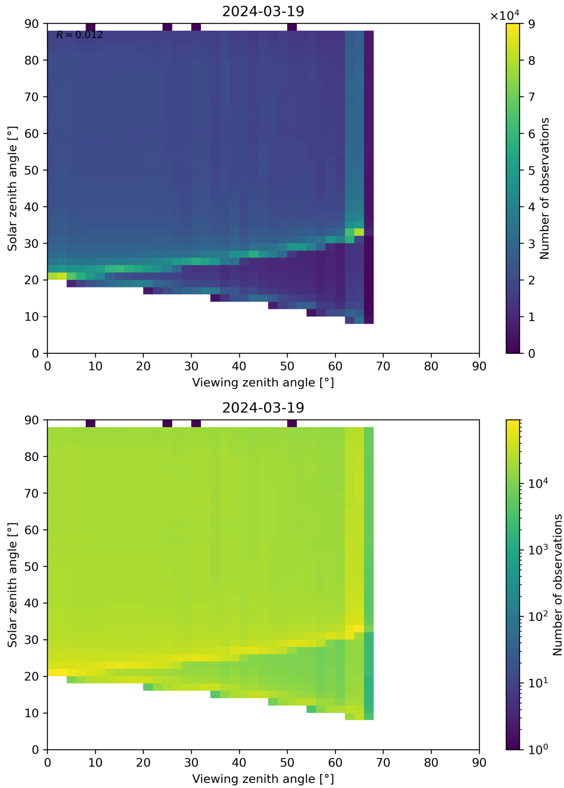
Figure 127: Scatter density plot of “Viewing zenith angle” against “Solar zenith angle” for 2024-03-18 to 2024-03-20.
