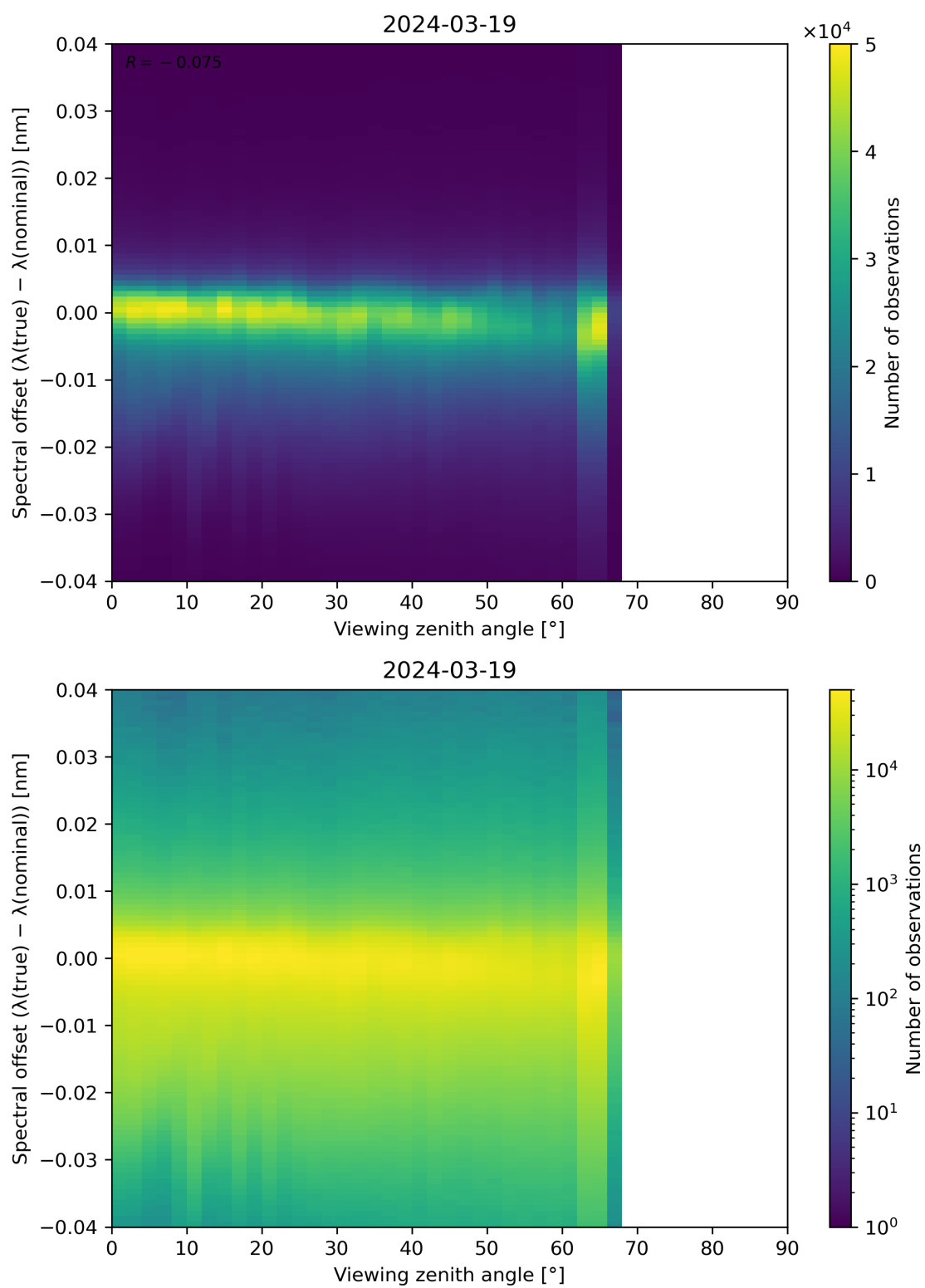
Figure 128: Scatter density plot of “Viewing zenith angle” against “Spectral offset ( \lambda(\text{true}) - \lambda(\text{nominal}) )” for 2024-03-18 to 2024-03-20.
