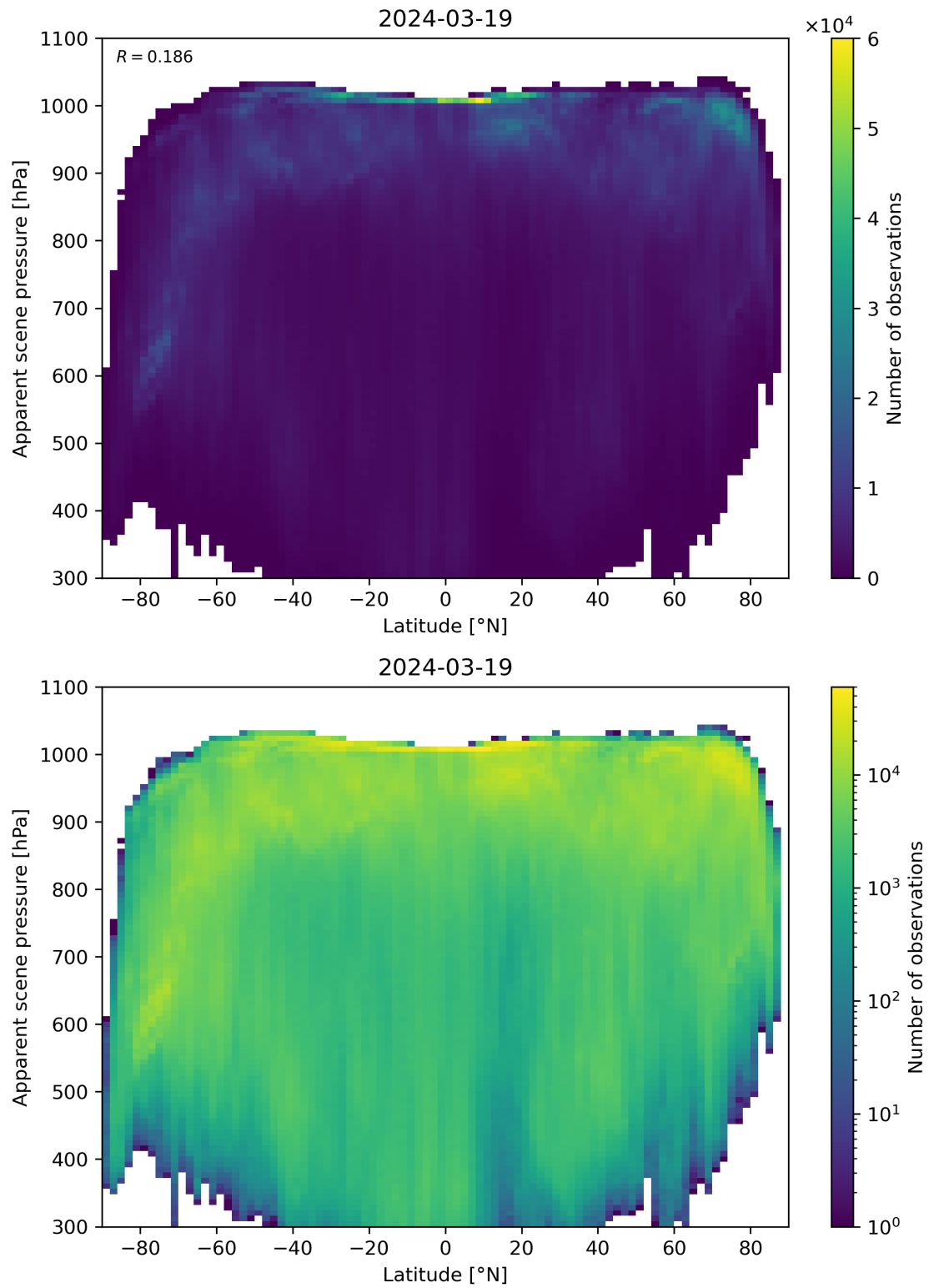
Figure 88: Scatter density plot of “Latitude” against “Apparent scene pressure” for 2024-03-18 to 2024-03-20.
