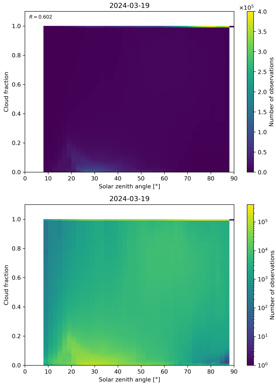
Figure 110: Scatter density plot of “Solar zenith angle” against “Cloud fraction” for 2024-03-18 to 2024-03-20.
