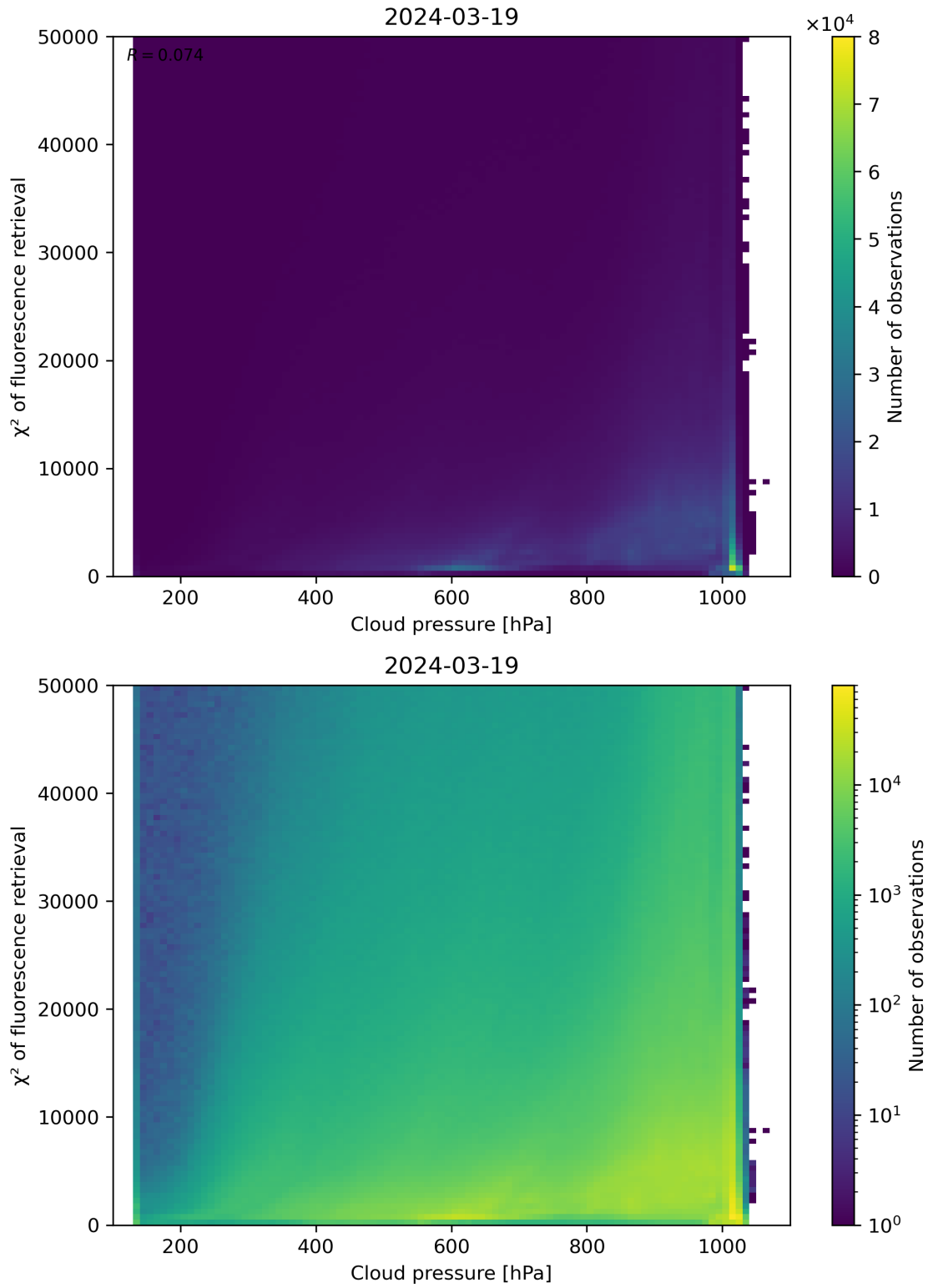
Figure 78: Scatter density plot of “Cloud pressure” against “ \chi^2 of fluorescence retrieval” for 2024-03-18 to 2024-03-20.
