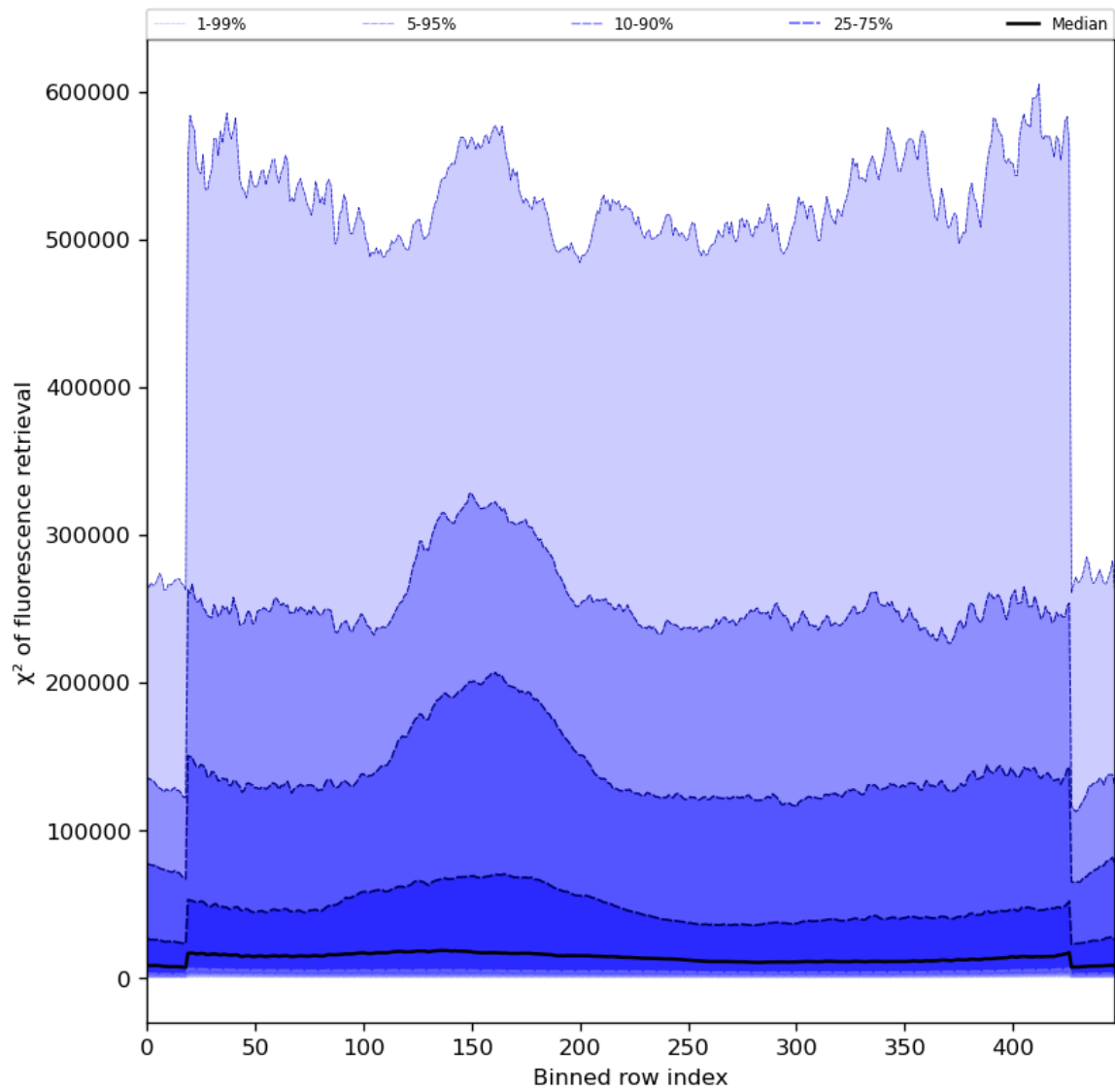
Figure 59: Along track statistics of “ \chi^2 of fluorescence retrieval” for 2024-03-18 to 2024-03-20
