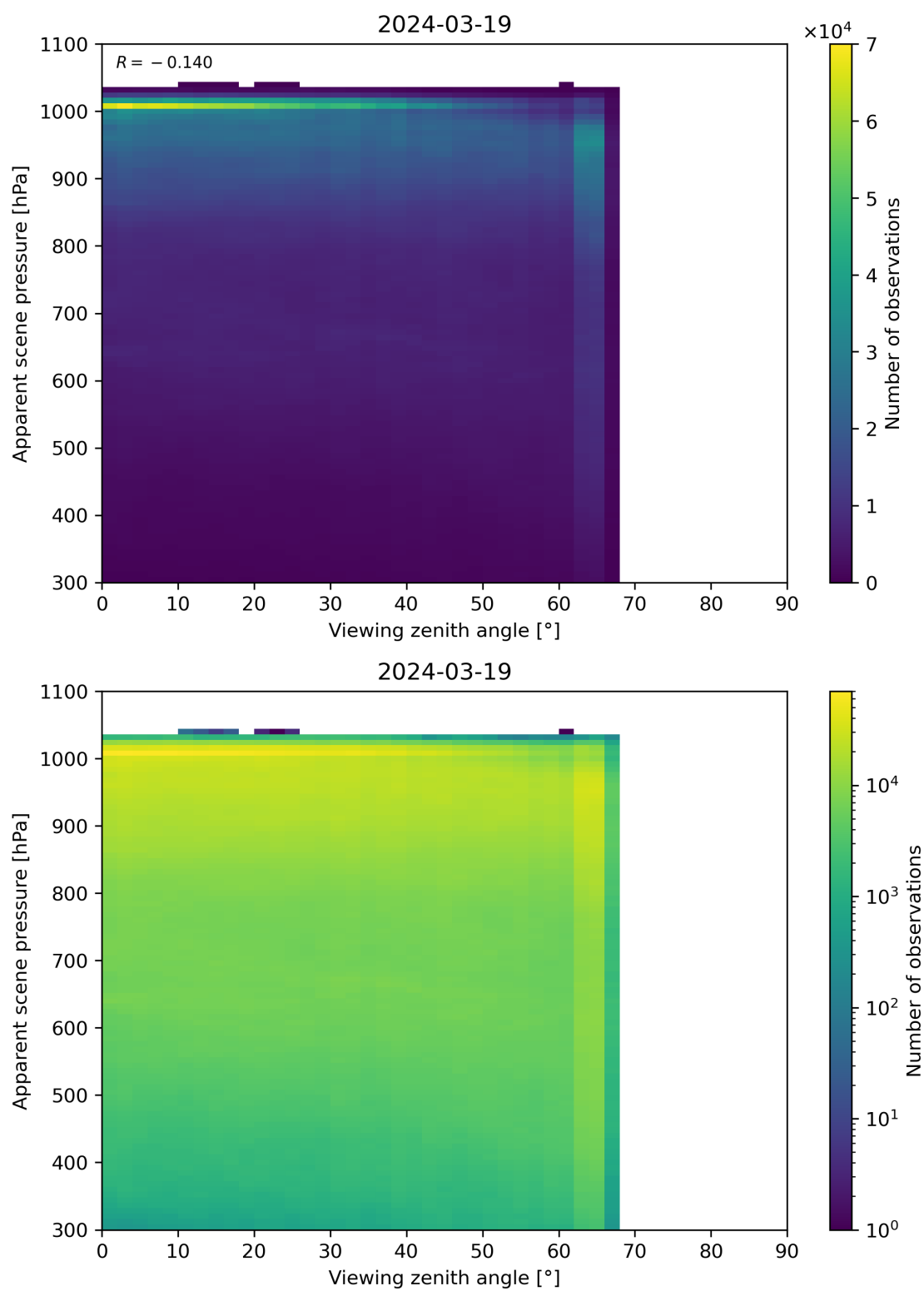
Figure 118: Scatter density plot of “Viewing zenith angle” against “Apparent scene pressure” for 2024-03-18 to 2024-03-20.
