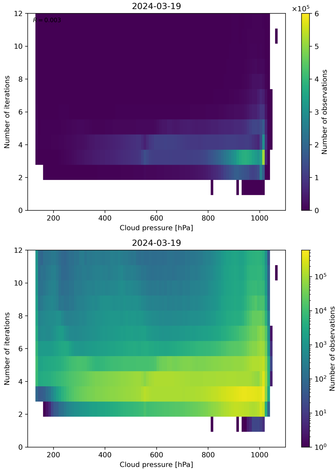
Figure 81: Scatter density plot of “Cloud pressure” against “Number of iterations” for 2024-03-18 to 2024-03-20.
