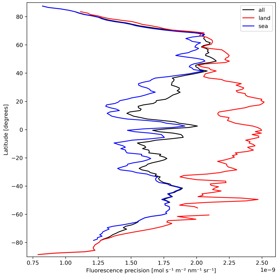
Figure 24: Zonal average of “Fluorescence precision” for 2024-03-18 to 2024-03-20.
