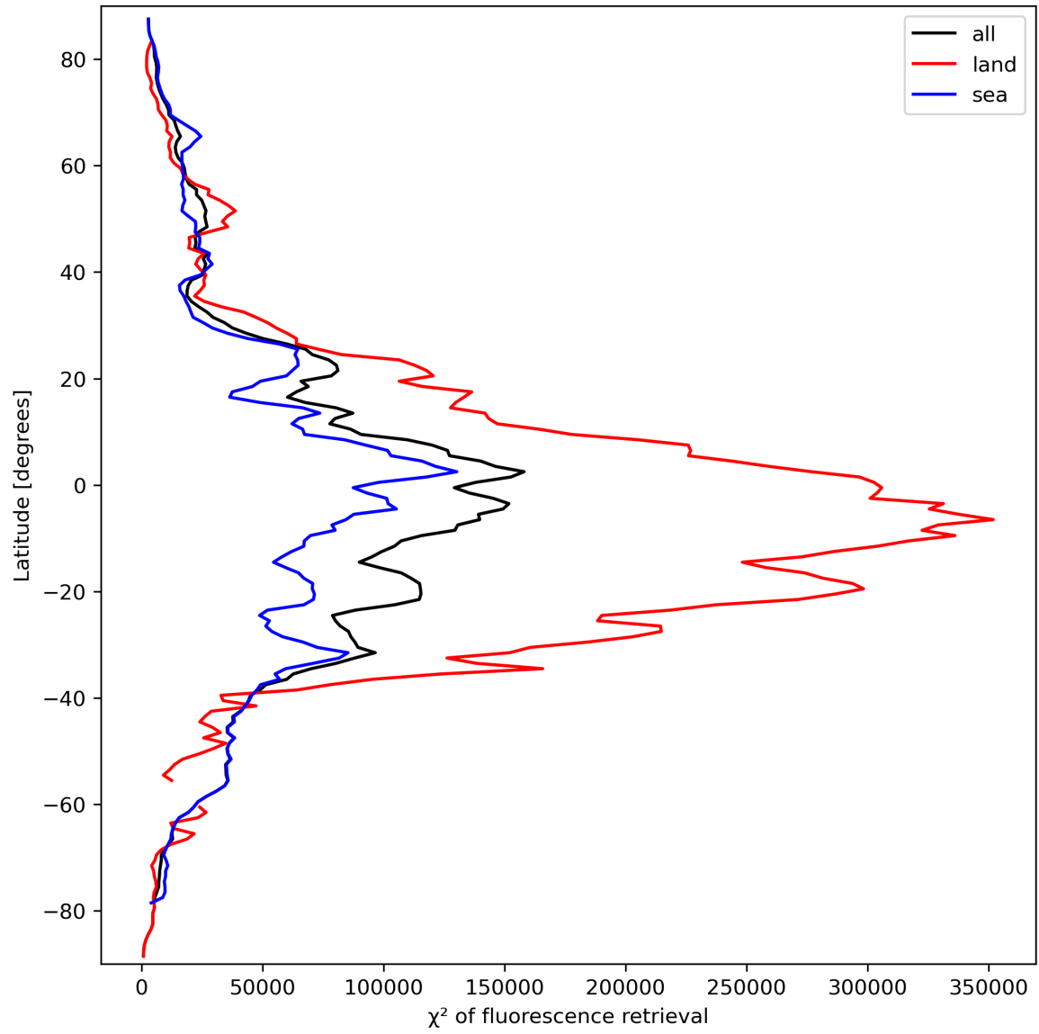
Figure 25: Zonal average of “ \chi^2 of fluorescence retrieval” for 2024-03-18 to 2024-03-20.
