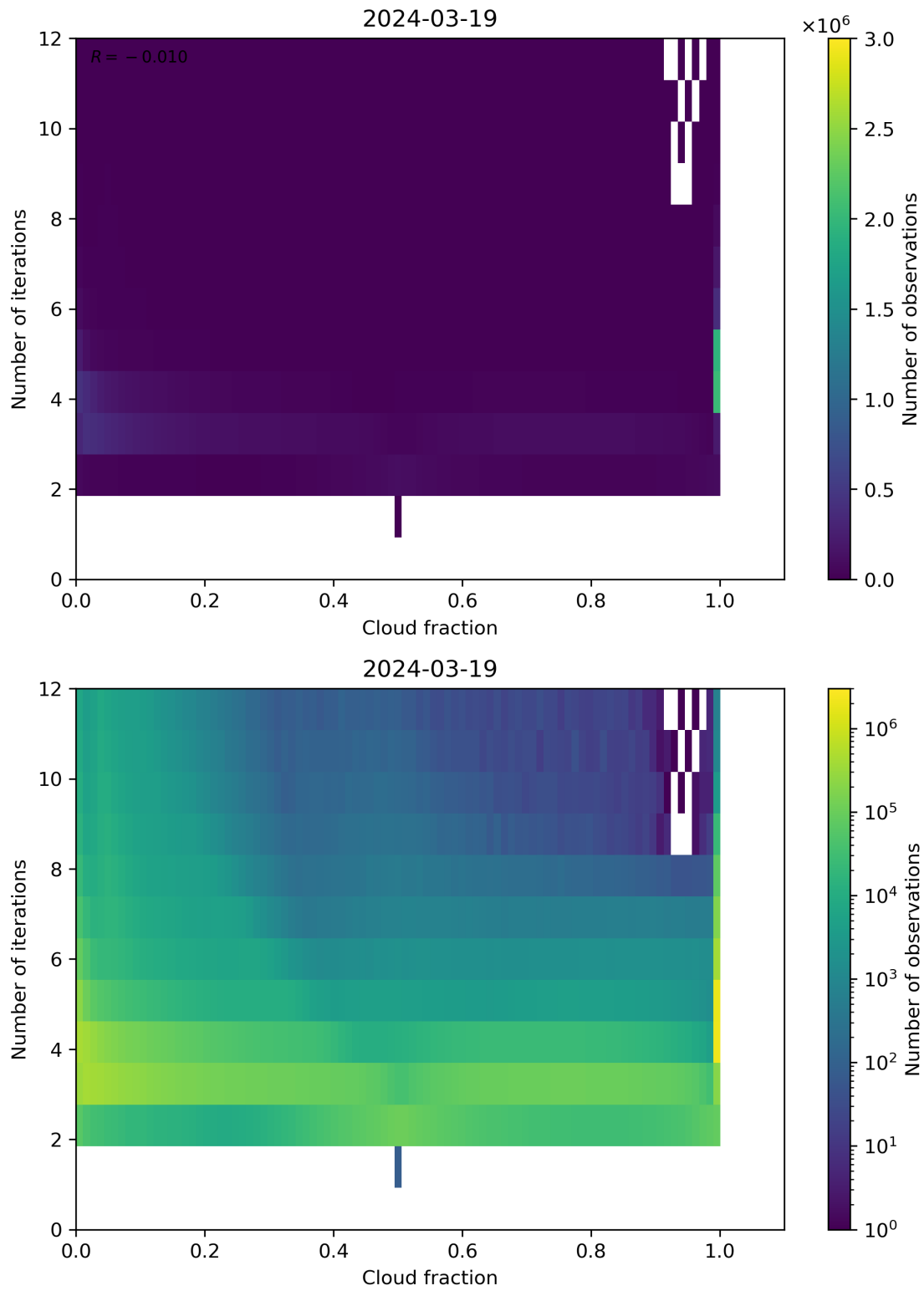
Figure 73: Scatter density plot of “Cloud fraction” against “Number of iterations” for 2024-03-18 to 2024-03-20.
