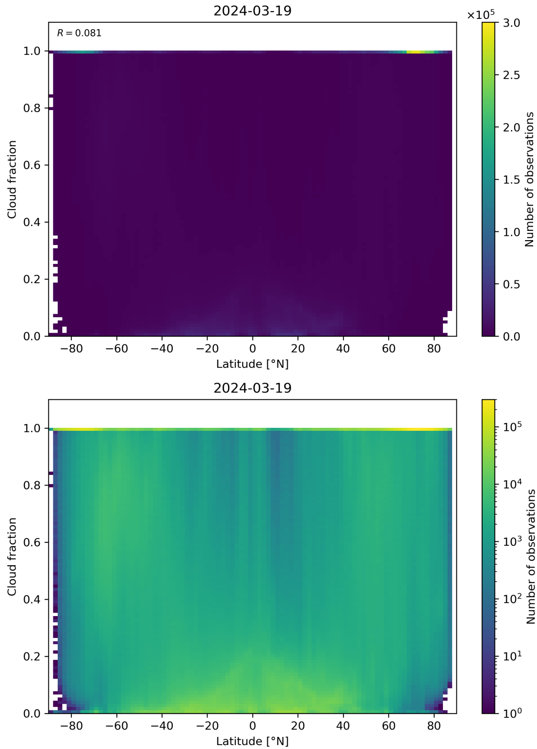
Figure 90: Scatter density plot of “Latitude” against “Cloud fraction” for 2024-03-18 to 2024-03-20.
