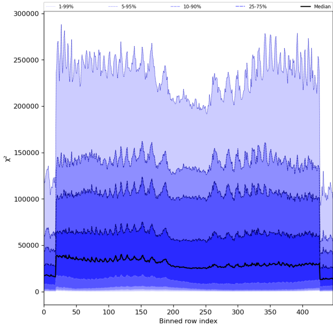
Figure 55: Along track statistics of “ \chi^2 ” for 2024-03-18 to 2024-03-20
