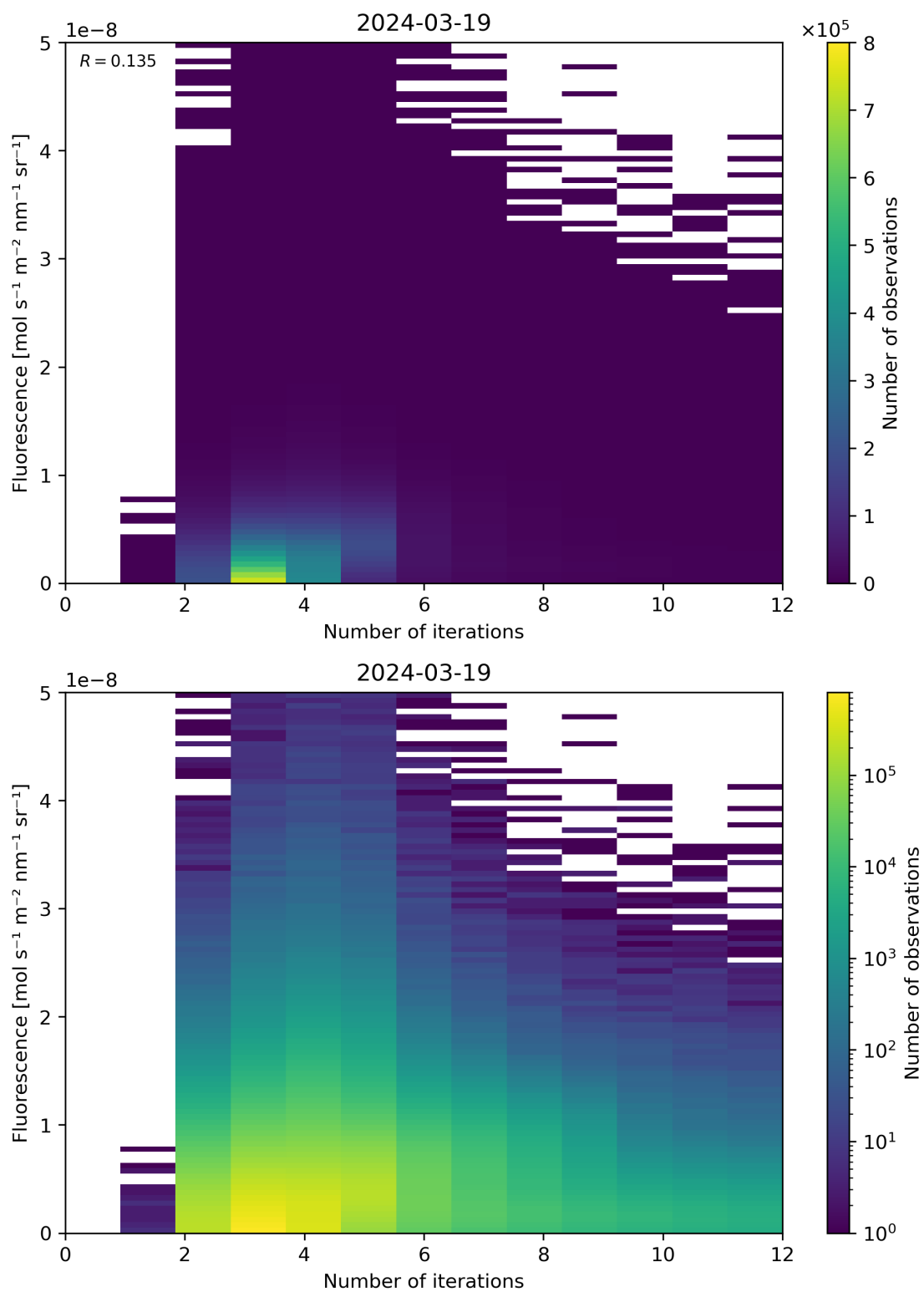
Figure 98: Scatter density plot of “Number of iterations” against “Fluorescence” for 2024-03-18 to 2024-03-20.
