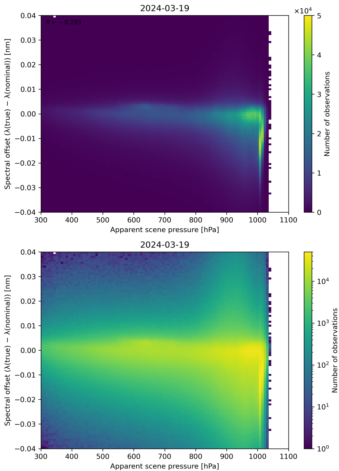
Figure 67: Scatter density plot of “Apparent scene pressure” against “Spectral offset ( \lambda(\text{true}) - \lambda(\text{nominal}) )” for 2024-03-18 to 2024-03-20.
