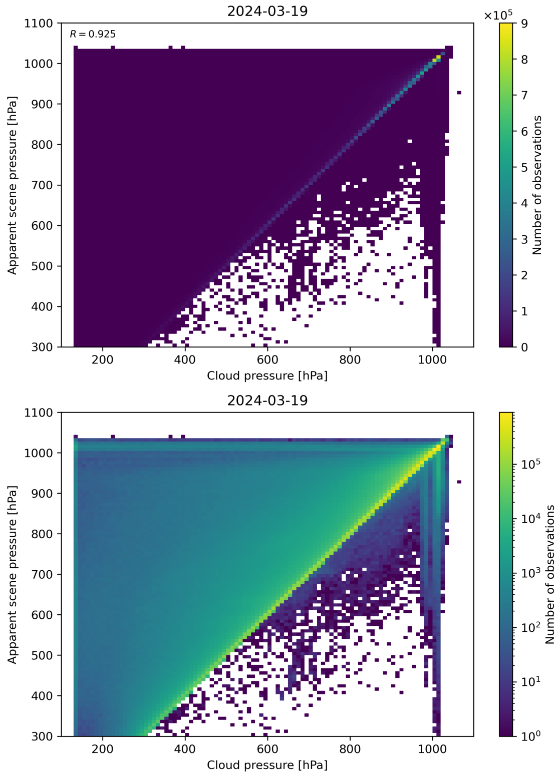
Figure 77: Scatter density plot of “Cloud pressure” against “Apparent scene pressure” for 2024-03-18 to 2024-03-20.
