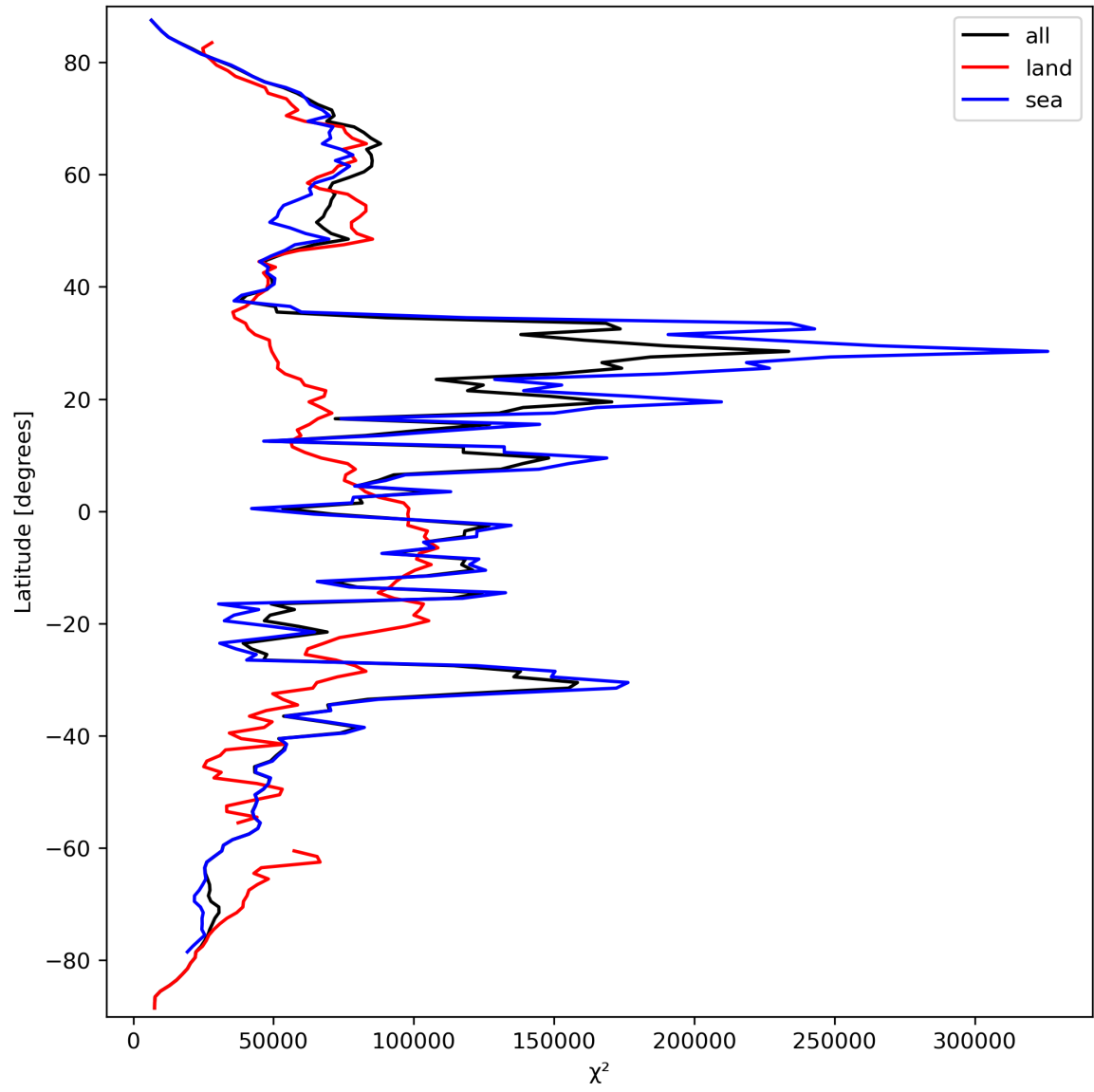
Figure 21: Zonal average of “ \chi^2 ” for 2024-03-18 to 2024-03-20.
