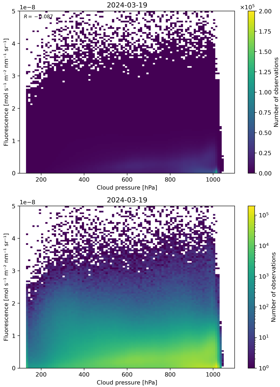
Figure 80: Scatter density plot of “Cloud pressure” against “Fluorescence” for 2024-03-18 to 2024-03-20.
