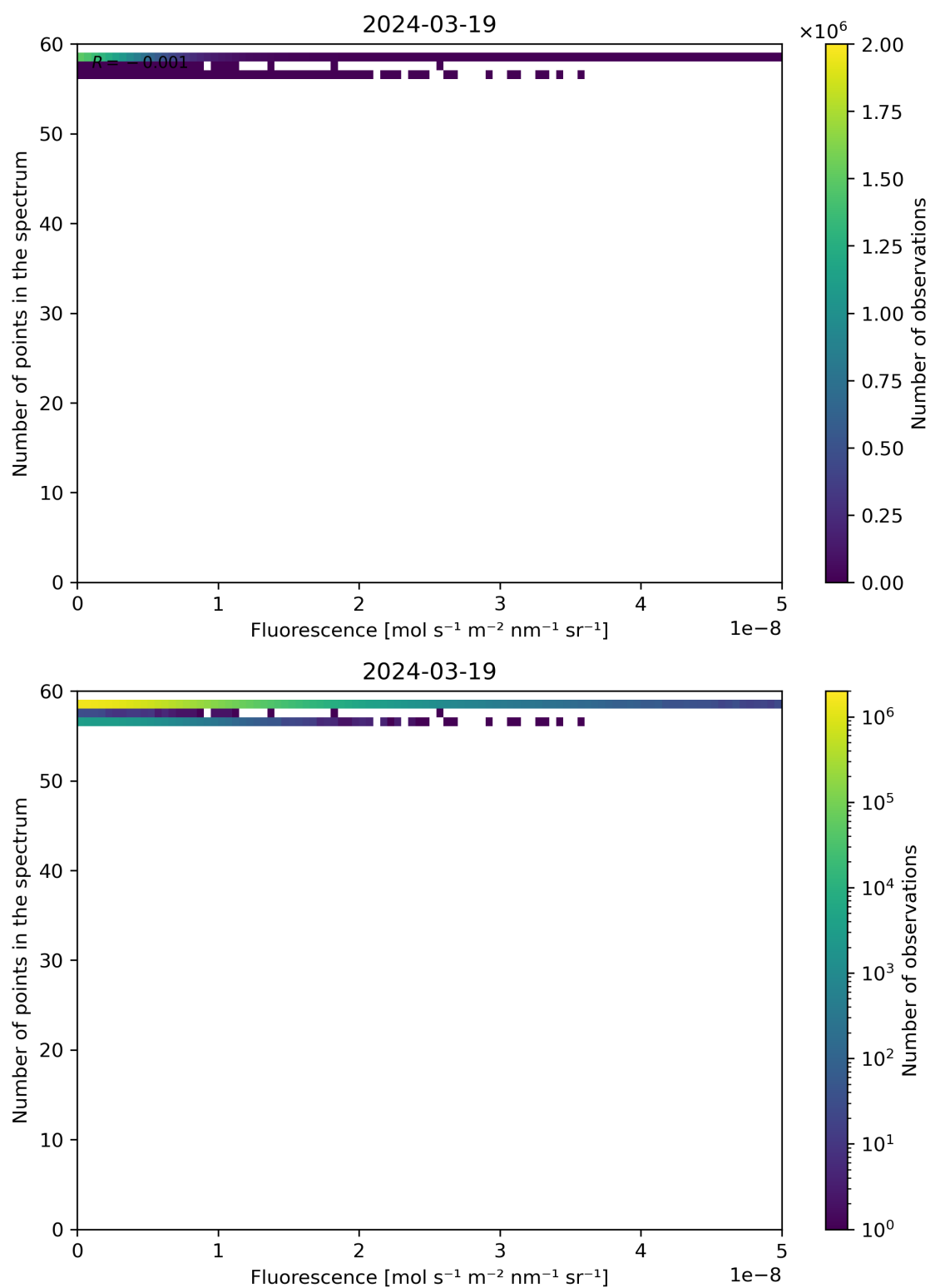
Figure 86: Scatter density plot of “Fluorescence” against “Number of points in the spectrum” for 2024-03-18 to 2024-03-20.
