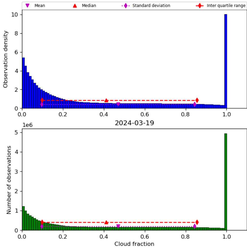
Figure 32: Histogram of “Cloud fraction” for 2024-03-18 to 2024-03-20
