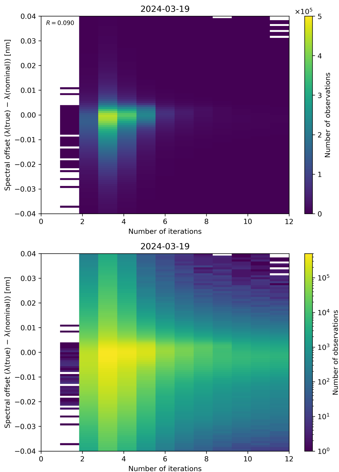
Figure 100: Scatter density plot of “Number of iterations” against “Spectral offset ( \lambda(\text{true}) - \lambda(\text{nominal}) )” for 2024-03-18 to 2024-03-20.
