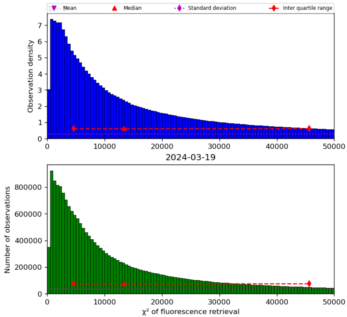
Figure 42: Histogram of “ \chi^2 of fluorescence retrieval” for 2024-03-18 to 2024-03-20
