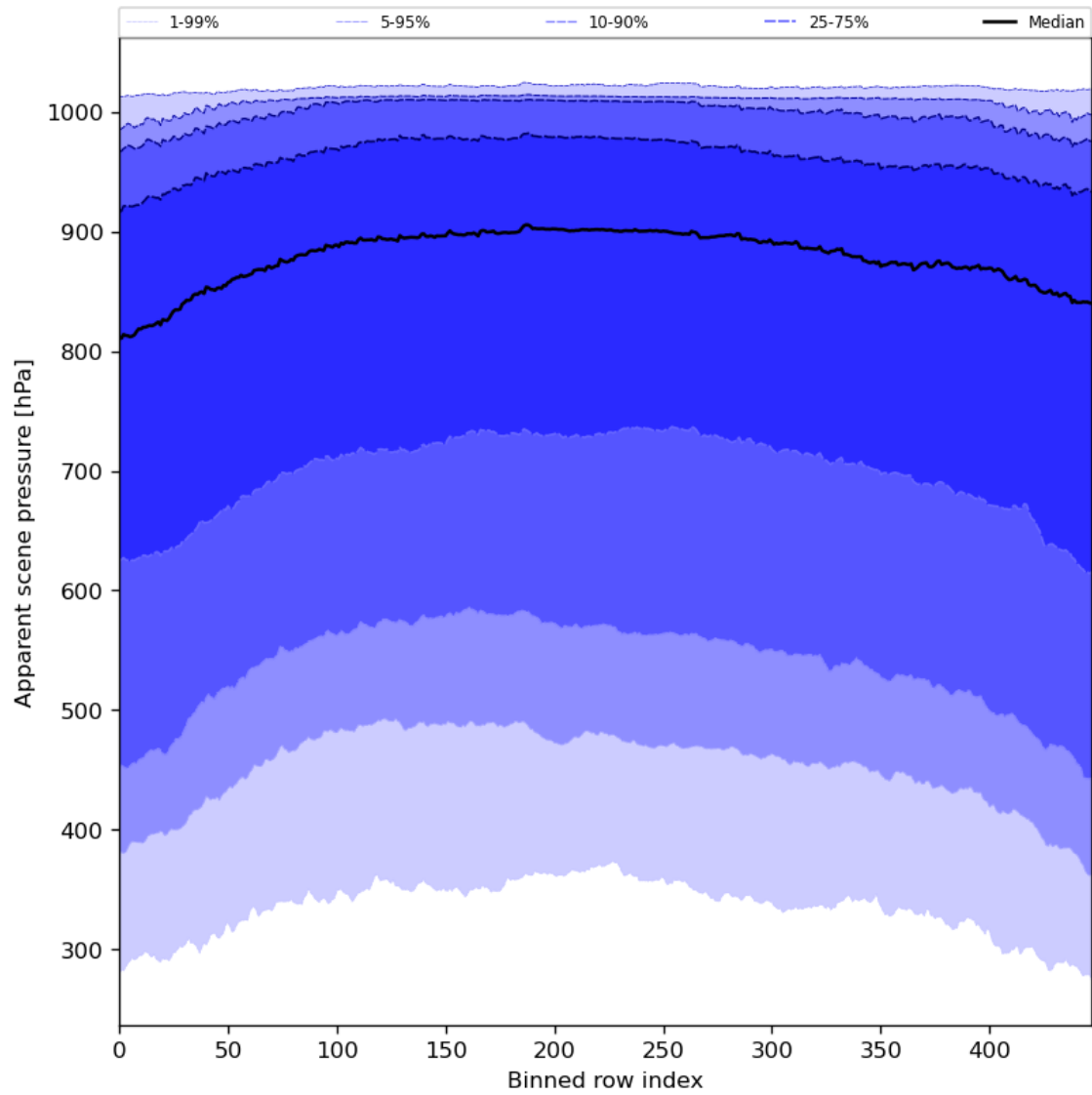
Figure 53: Along track statistics of “Apparent scene pressure” for 2024-03-20 to 2024-03-21
