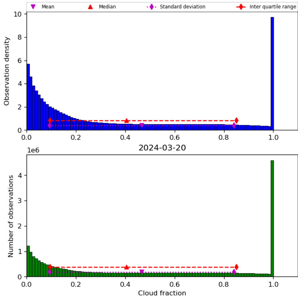
Figure 32: Histogram of “Cloud fraction” for 2024-03-20 to 2024-03-21
