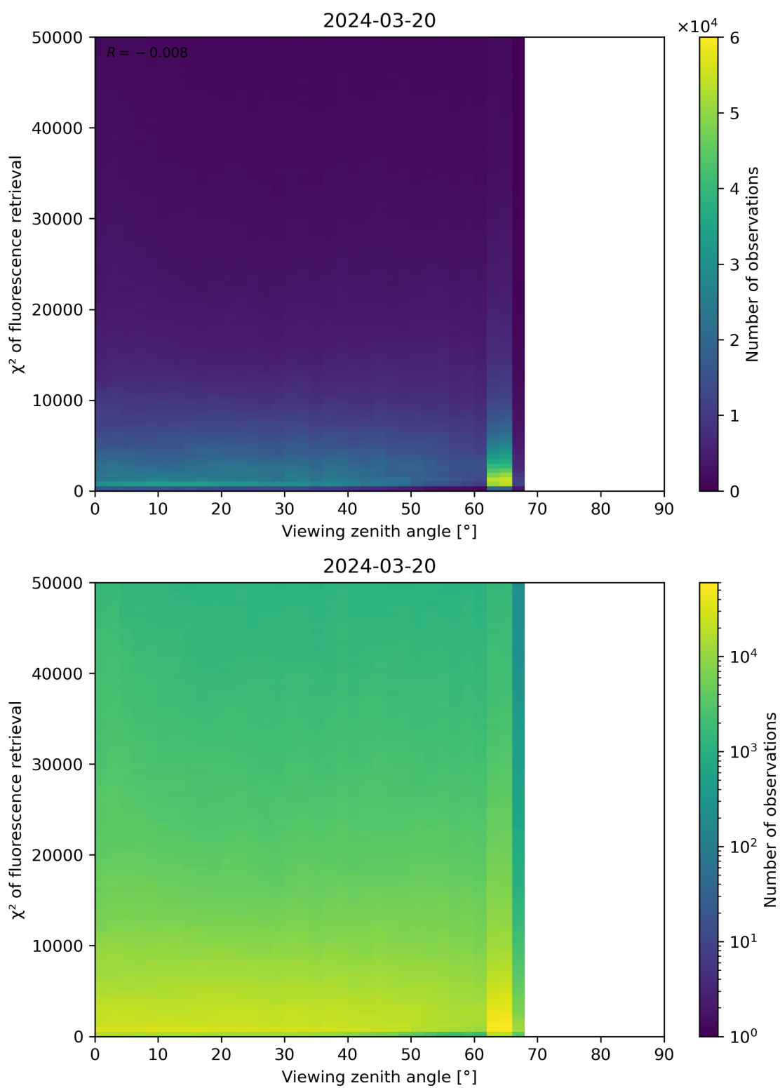
Figure 119: Scatter density plot of “Viewing zenith angle” against “ \chi^2 of fluorescence retrieval” for 2024-03-20 to 2024-03-21.
