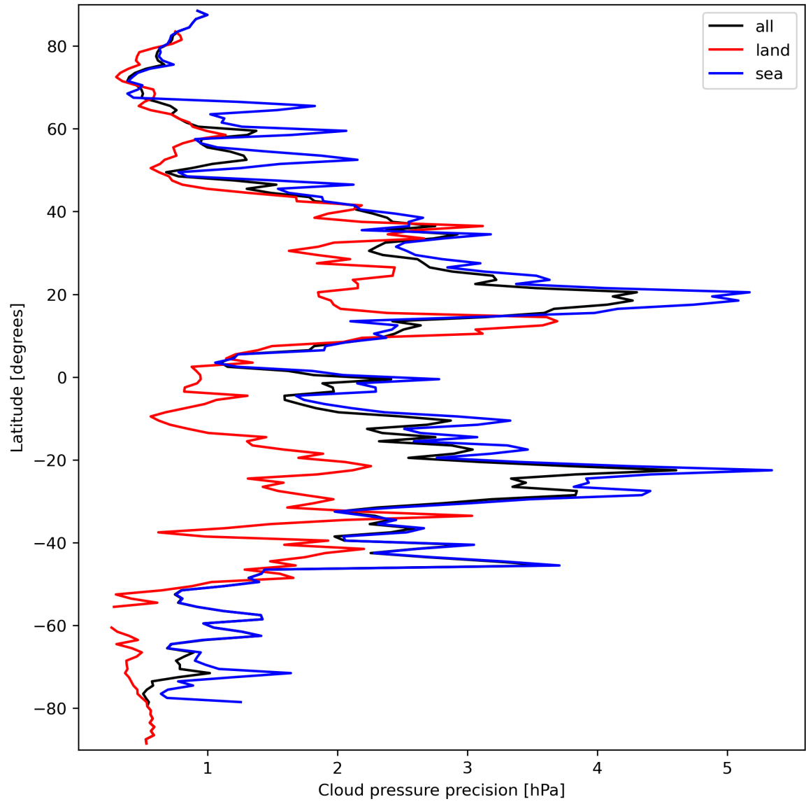
Figure 14: Zonal average of “Cloud pressure precision” for 2024-03-20 to 2024-03-21.
