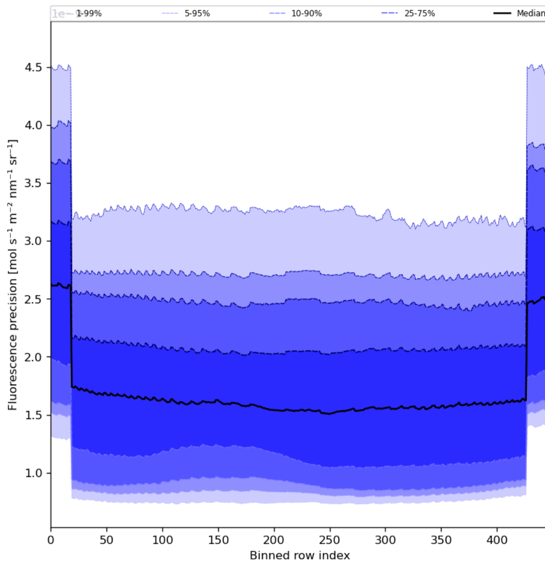
Figure 58: Along track statistics of “Fluorescence precision” for 2024-03-20 to 2024-03-21
