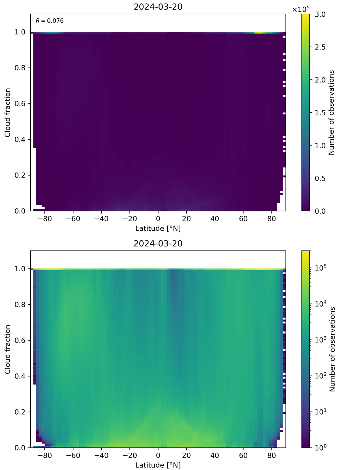
Figure 90: Scatter density plot of “Latitude” against “Cloud fraction” for 2024-03-20 to 2024-03-21.
