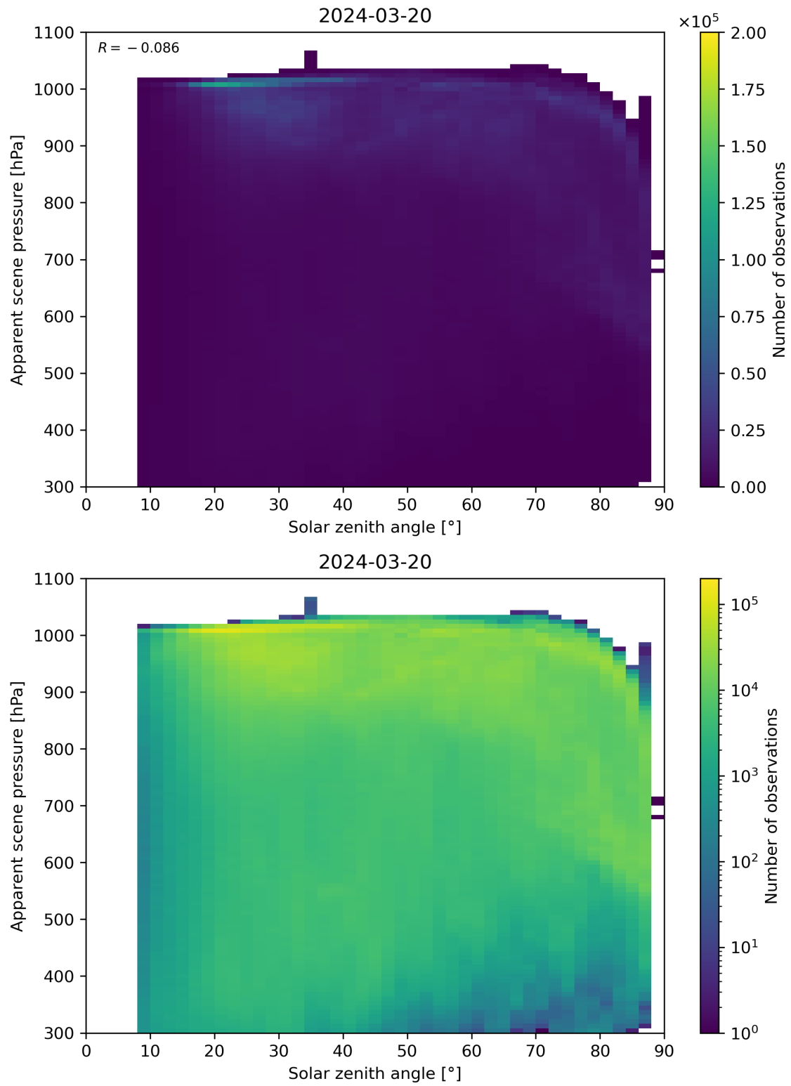
Figure 108: Scatter density plot of “Solar zenith angle” against “Apparent scene pressure” for 2024-03-20 to 2024-03-21.
