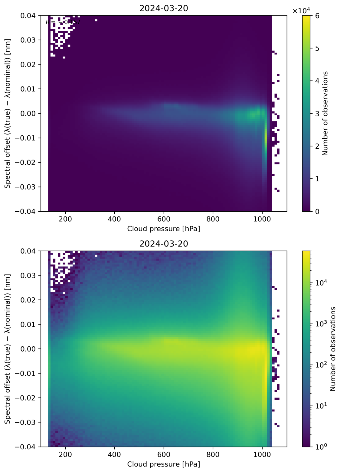
Figure 84: Scatter density plot of “Cloud pressure” against “Spectral offset ( \lambda(\text{true}) - \lambda(\text{nominal}) )” for 2024-03-20 to 2024-03-21.
