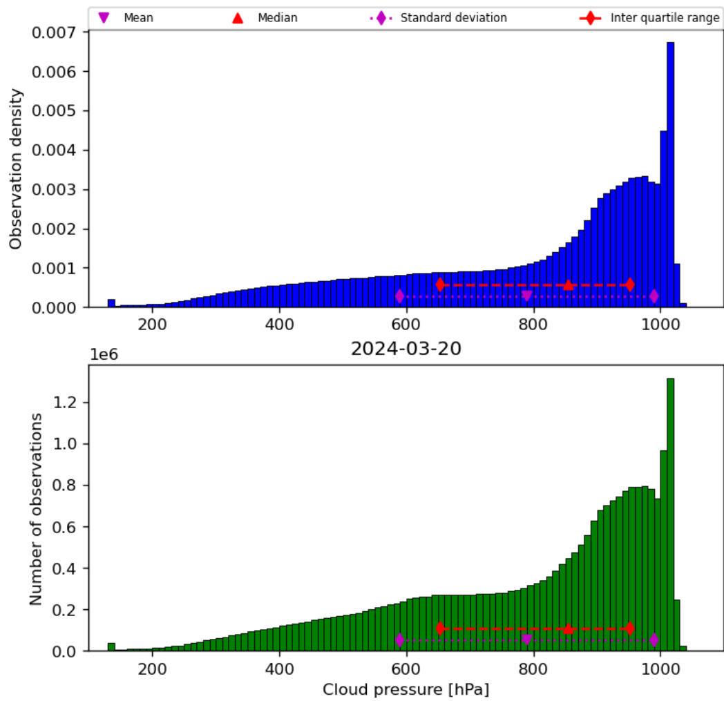
Figure 30: Histogram of “Cloud pressure” for 2024-03-20 to 2024-03-21
