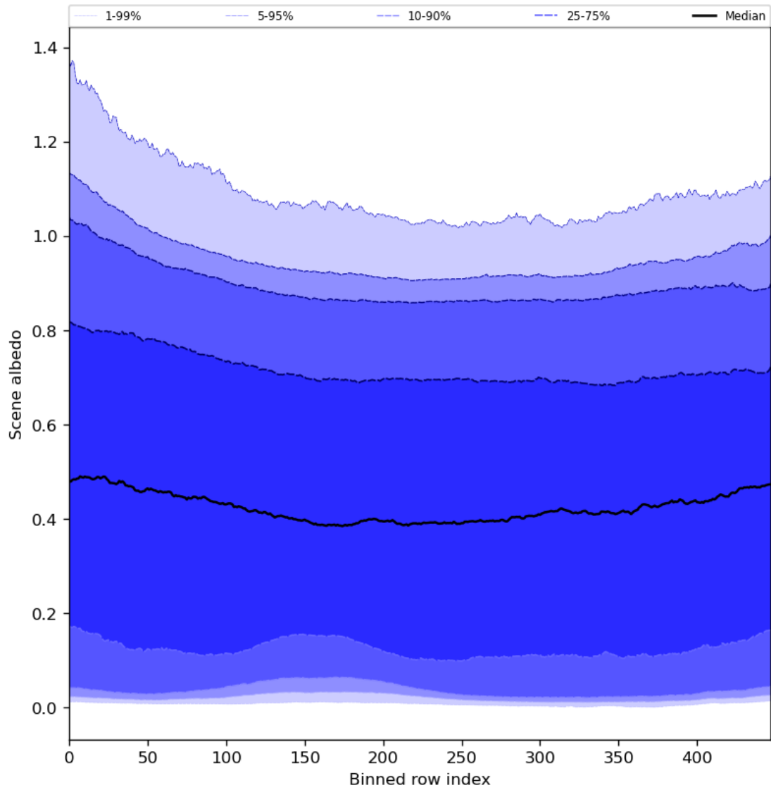
Figure 51: Along track statistics of “Scene albedo” for 2024-03-20 to 2024-03-21
