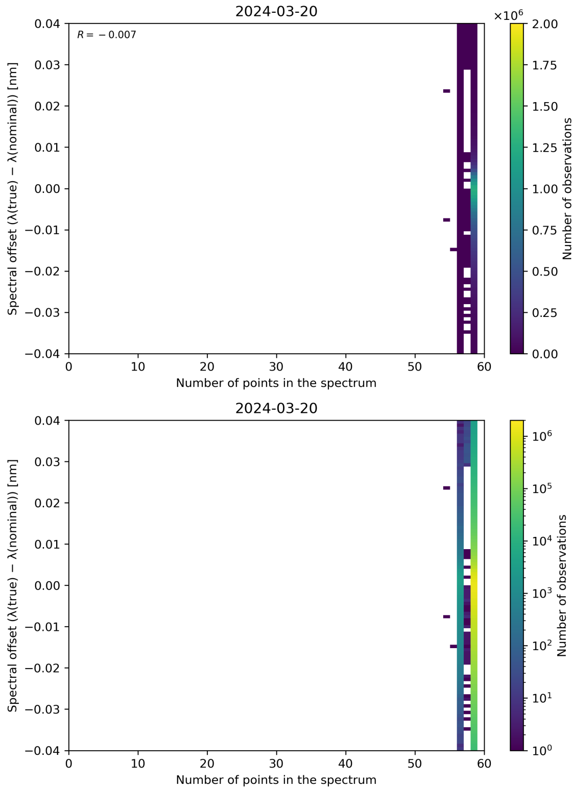
Figure 101: Scatter density plot of “Number of points in the spectrum” against “Spectral offset ( \lambda(\text{true}) - \lambda(\text{nominal}) )” for 2024-03-20 to 2024-03-21.
