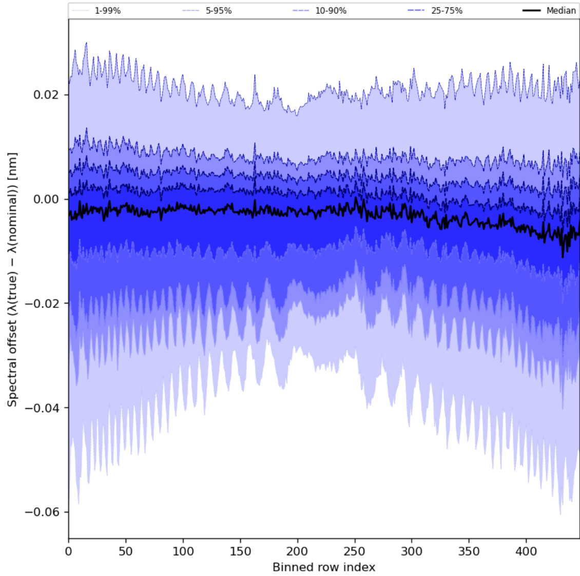
Figure 62: Along track statistics of “Spectral offset ( \lambda(\text{true}) - \lambda(\text{nominal}) )” for 2024-03-20 to 2024-03-21
