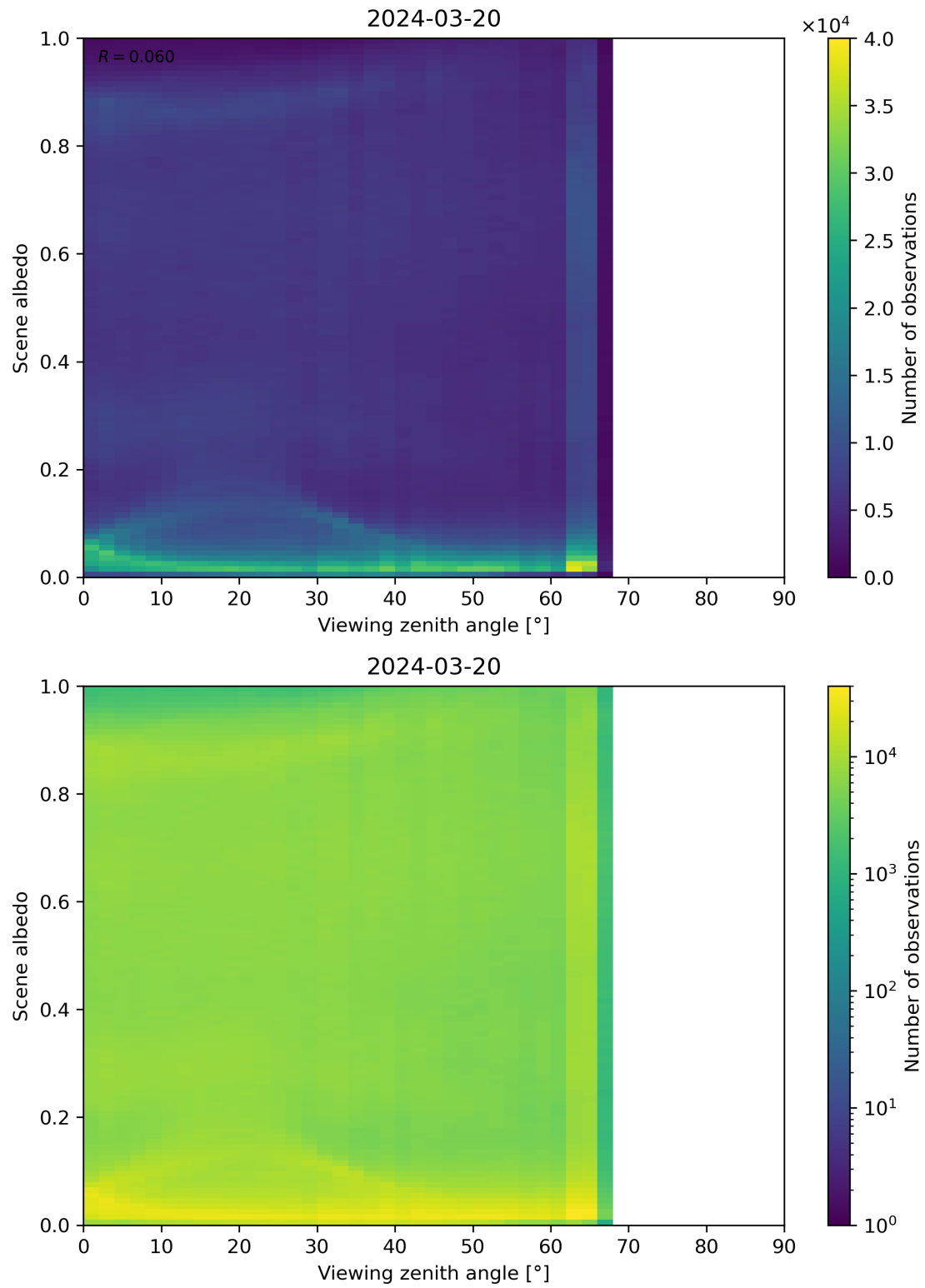
Figure 126: Scatter density plot of “Viewing zenith angle” against “Scene albedo” for 2024-03-20 to 2024-03-21.
