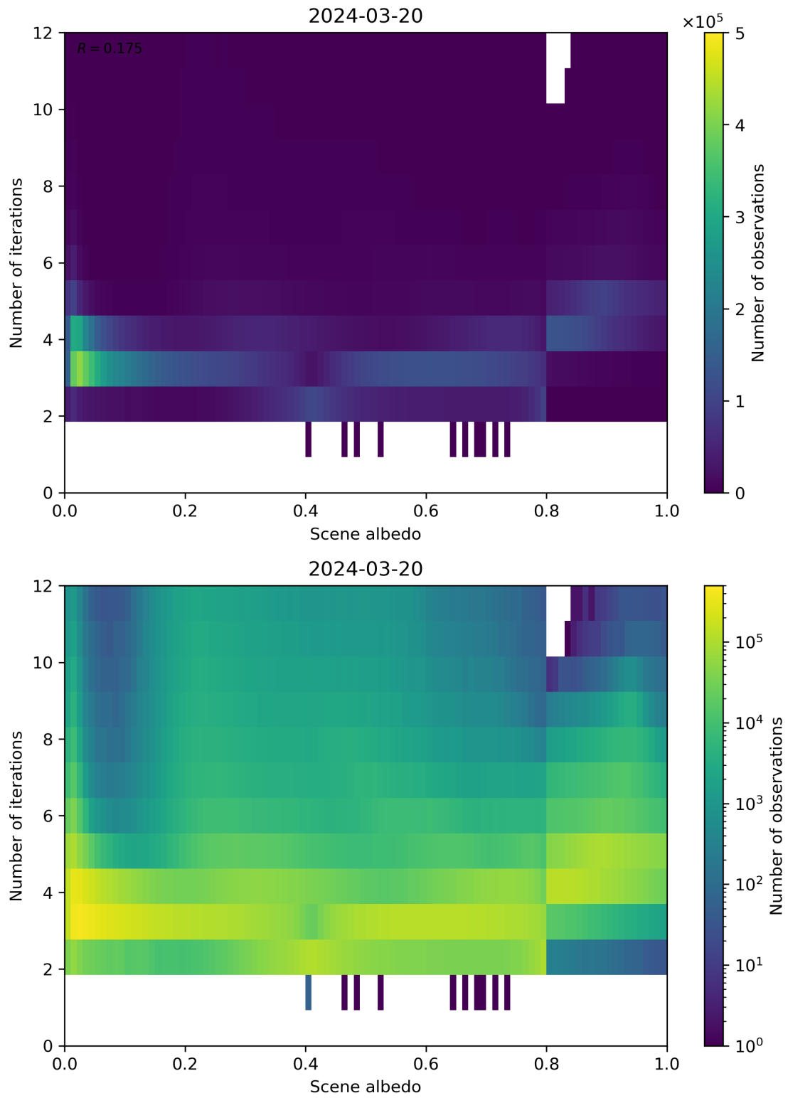
Figure 105: Scatter density plot of “Scene albedo” against “Number of iterations” for 2024-03-20 to 2024-03-21.
