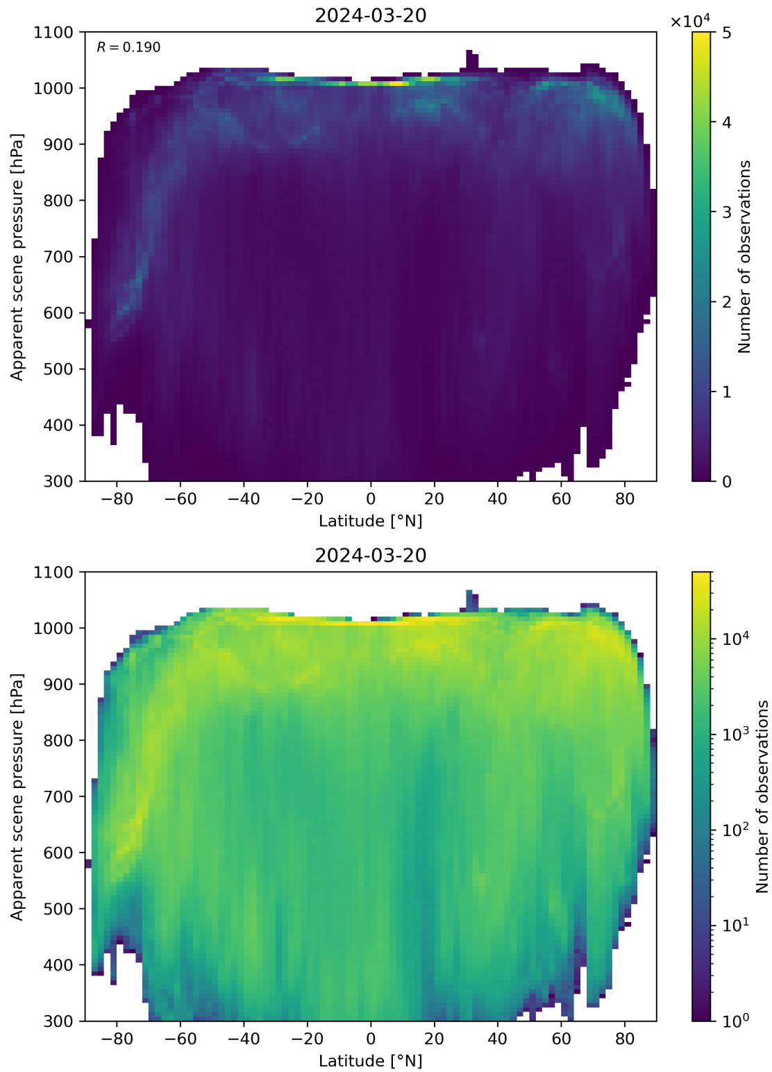
Figure 88: Scatter density plot of “Latitude” against “Apparent scene pressure” for 2024-03-20 to 2024-03-21.
