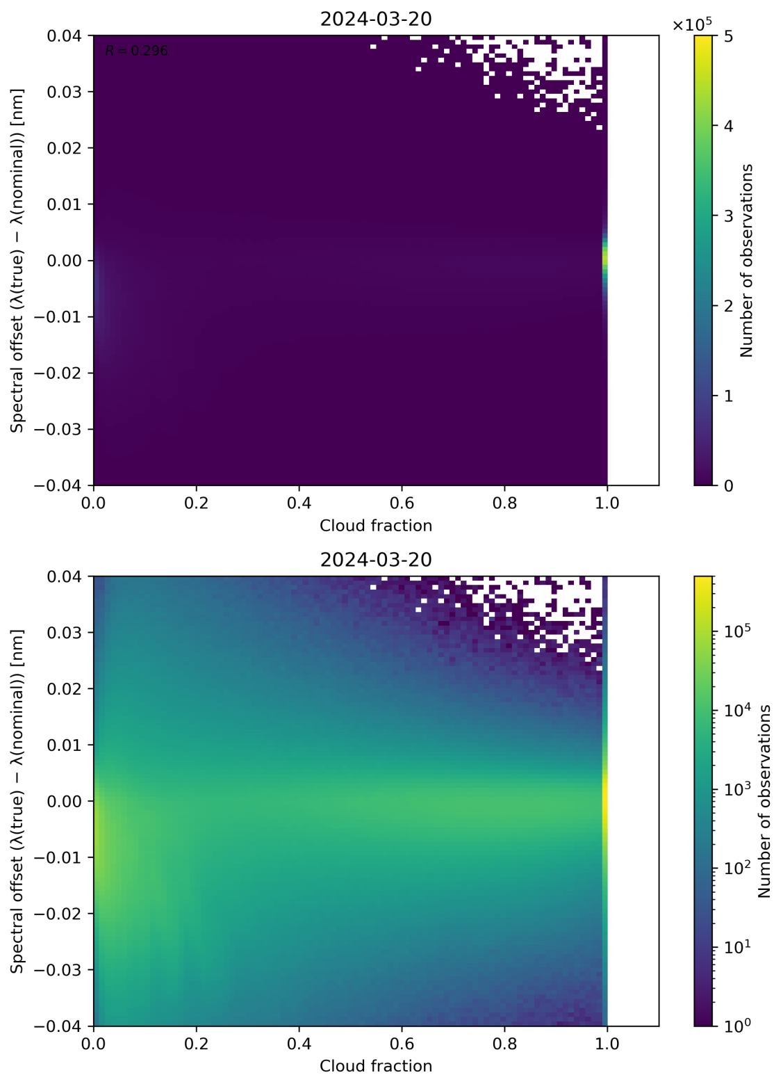
Figure 76: Scatter density plot of “Cloud fraction” against “Spectral offset ( \lambda(\text{true}) - \lambda(\text{nominal}) )” for 2024-03-20 to 2024-03-21.
