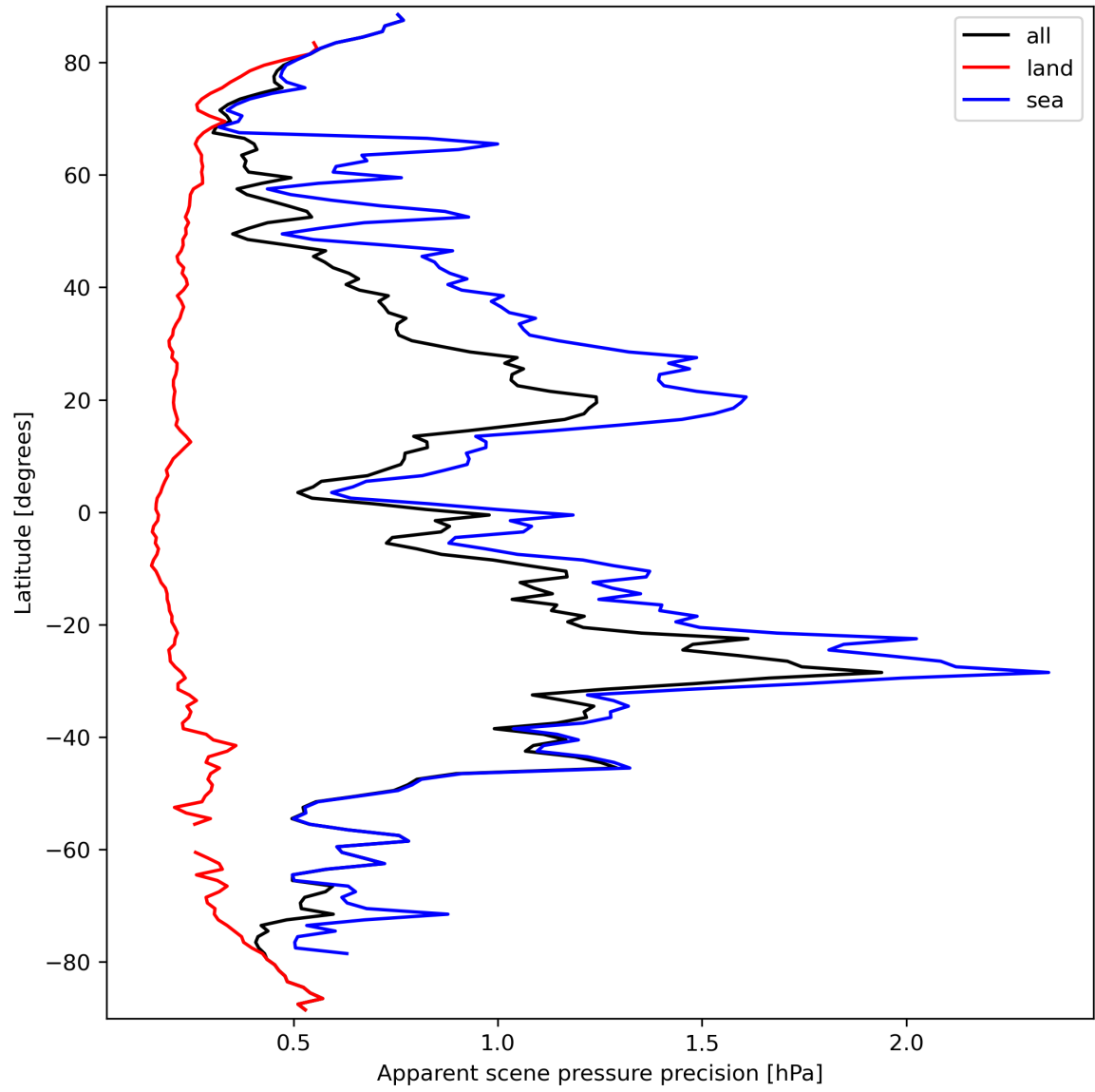
Figure 20: Zonal average of “Apparent scene pressure precision” for 2024-03-20 to 2024-03-21.
