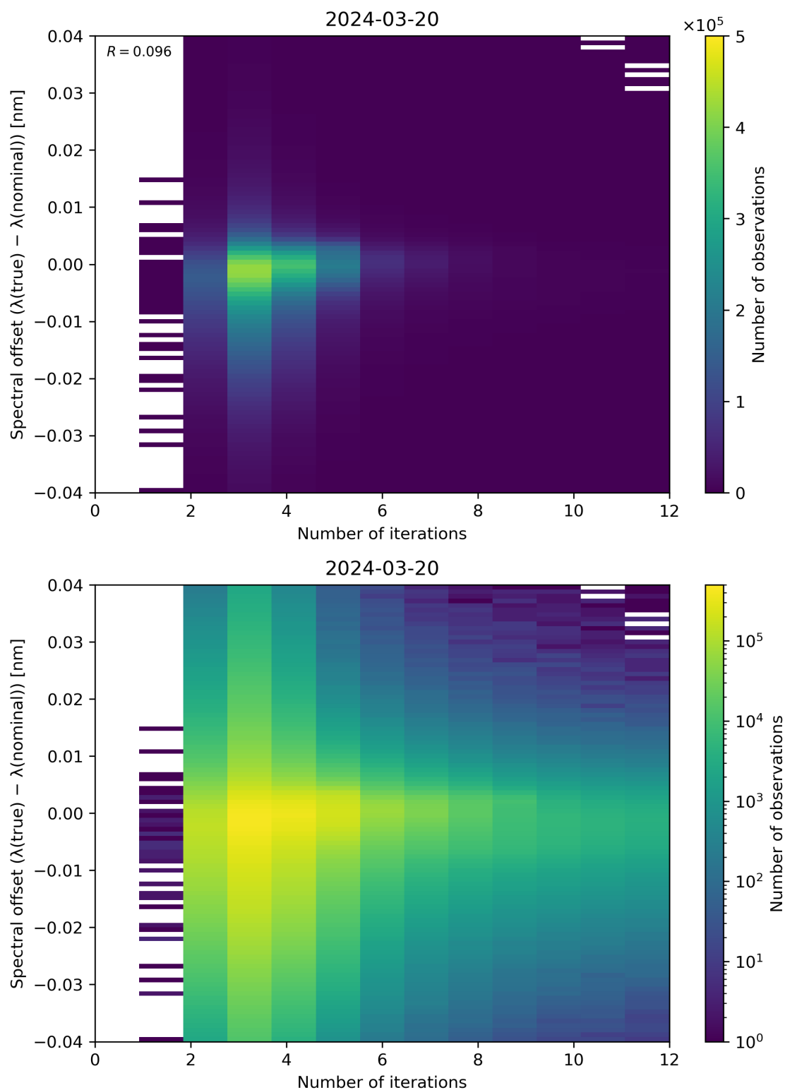
Figure 100: Scatter density plot of “Number of iterations” against “Spectral offset ( \lambda(\text{true}) - \lambda(\text{nominal}) )” for 2024-03-20 to 2024-03-21.
