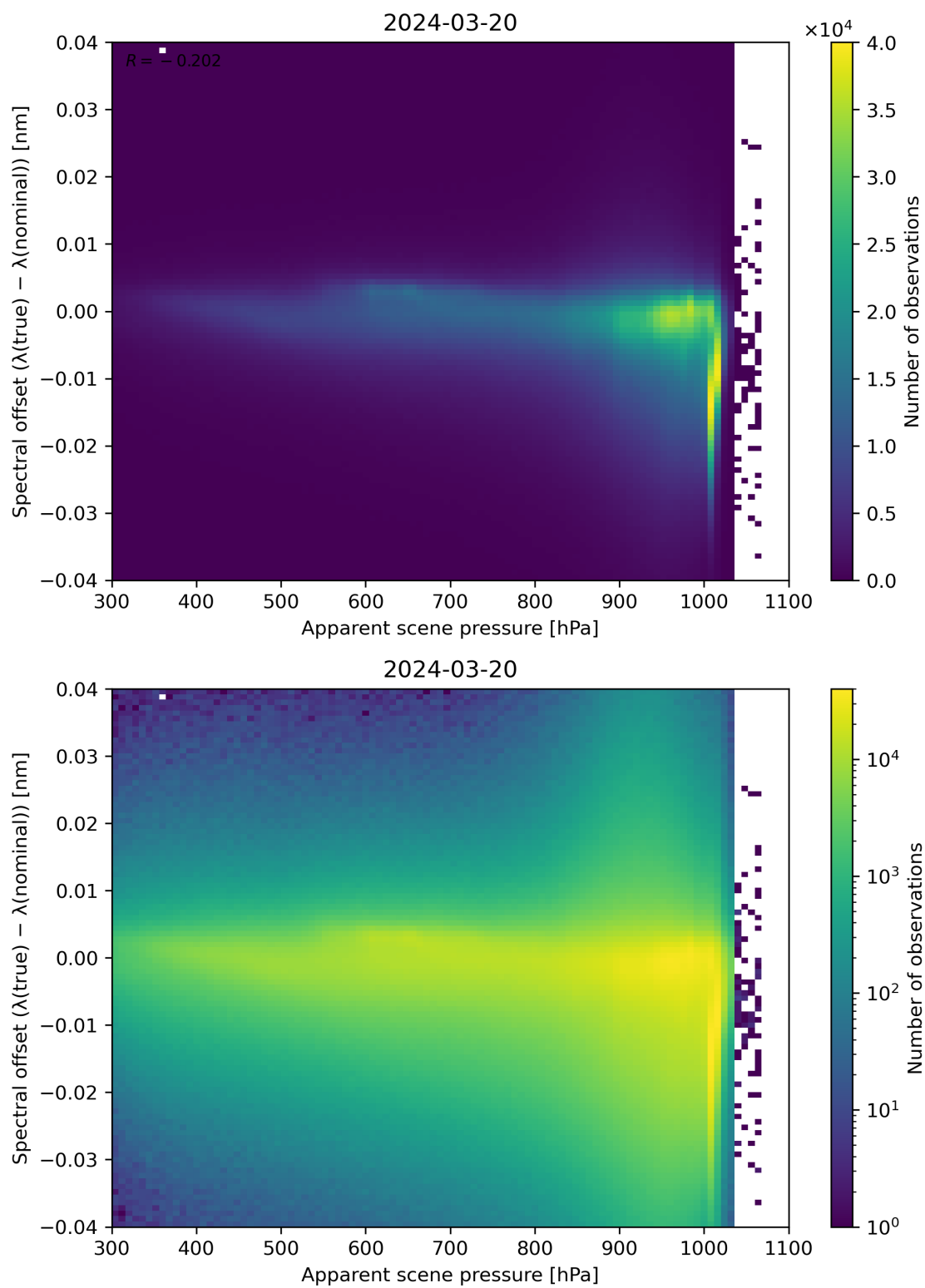
Figure 67: Scatter density plot of “Apparent scene pressure” against “Spectral offset ( \lambda(\text{true}) - \lambda(\text{nominal}) )” for 2024-03-20 to 2024-03-21.
