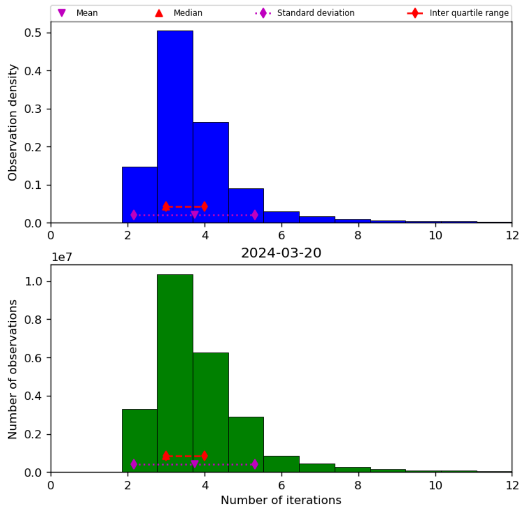
Figure 39: Histogram of “Number of iterations” for 2024-03-20 to 2024-03-21
