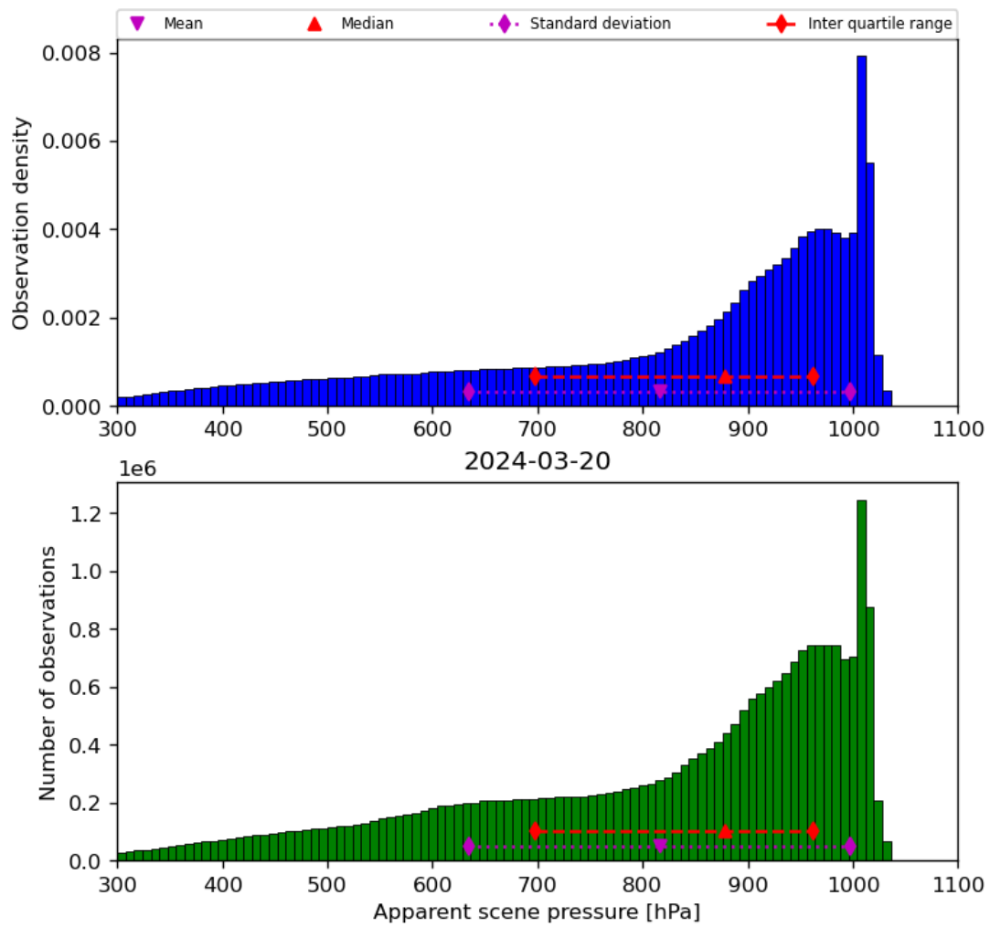
Figure 36: Histogram of “Apparent scene pressure” for 2024-03-20 to 2024-03-21
