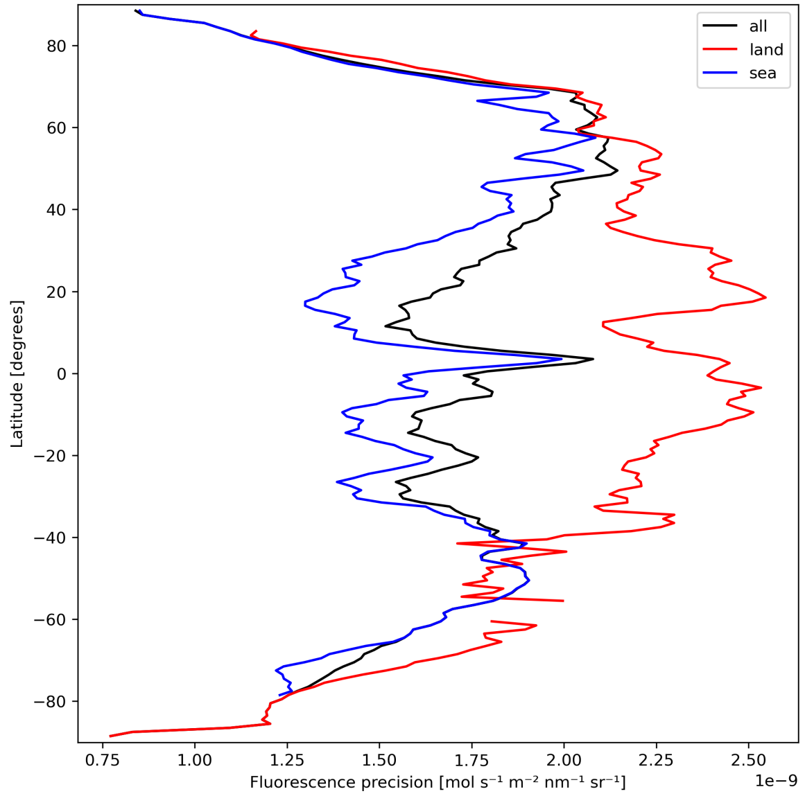
Figure 24: Zonal average of “Fluorescence precision” for 2024-03-20 to 2024-03-21.
