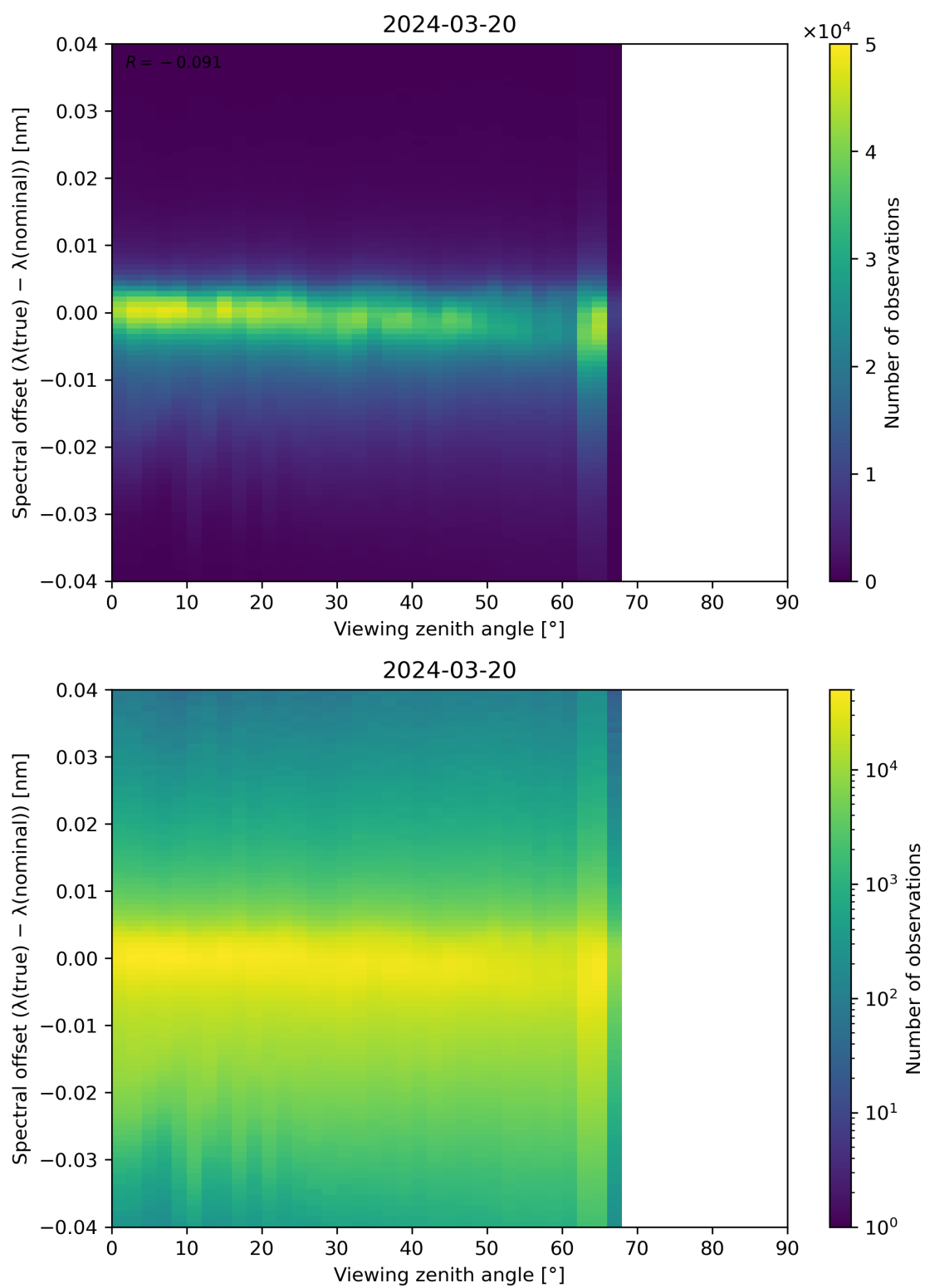
Figure 128: Scatter density plot of “Viewing zenith angle” against “Spectral offset ( \lambda(\text{true}) - \lambda(\text{nominal}) )” for 2024-03-20 to 2024-03-21.
