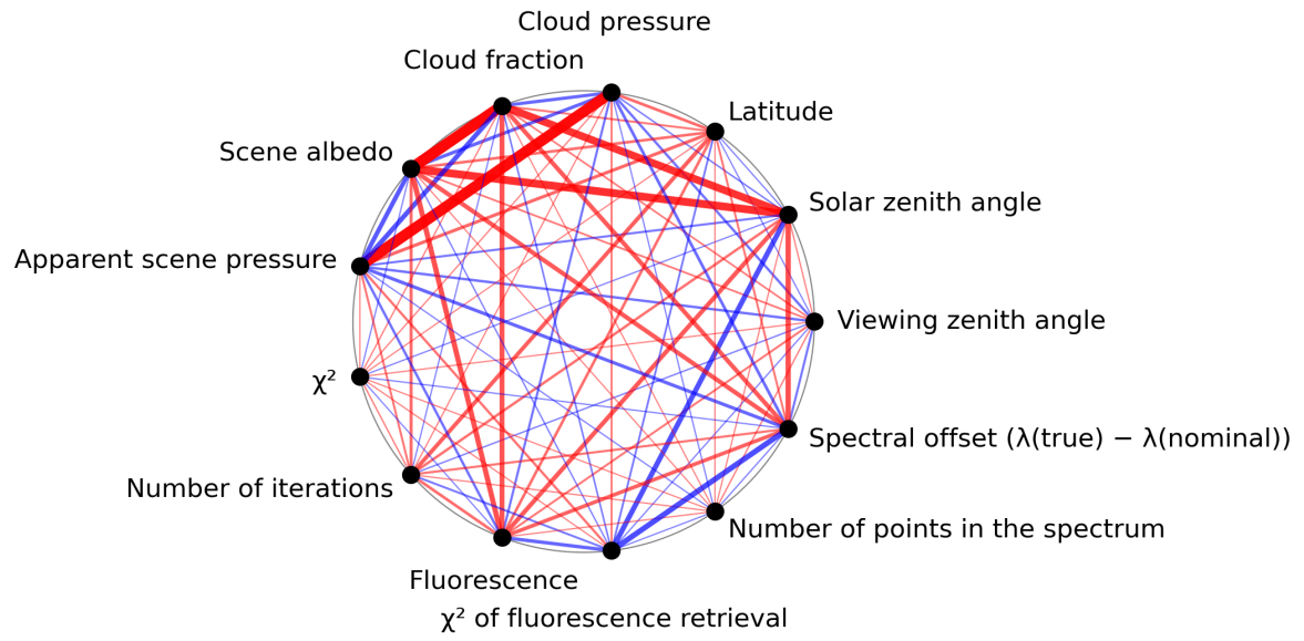
Figure 1: Map of correlation graph for 2024-03-20 to 2024-03-21.
