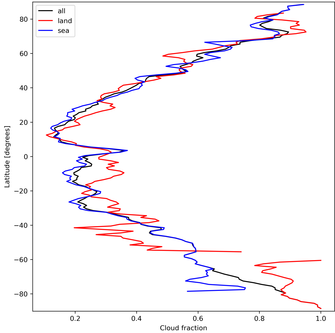
Figure 15: Zonal average of “Cloud fraction” for 2024-03-20 to 2024-03-21.
