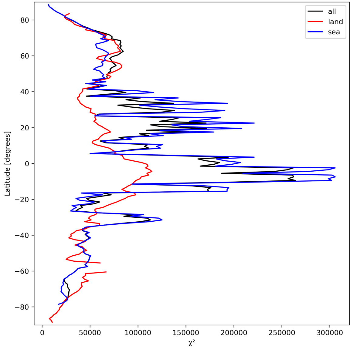
Figure 21: Zonal average of “ \chi^2 ” for 2024-03-20 to 2024-03-21.
