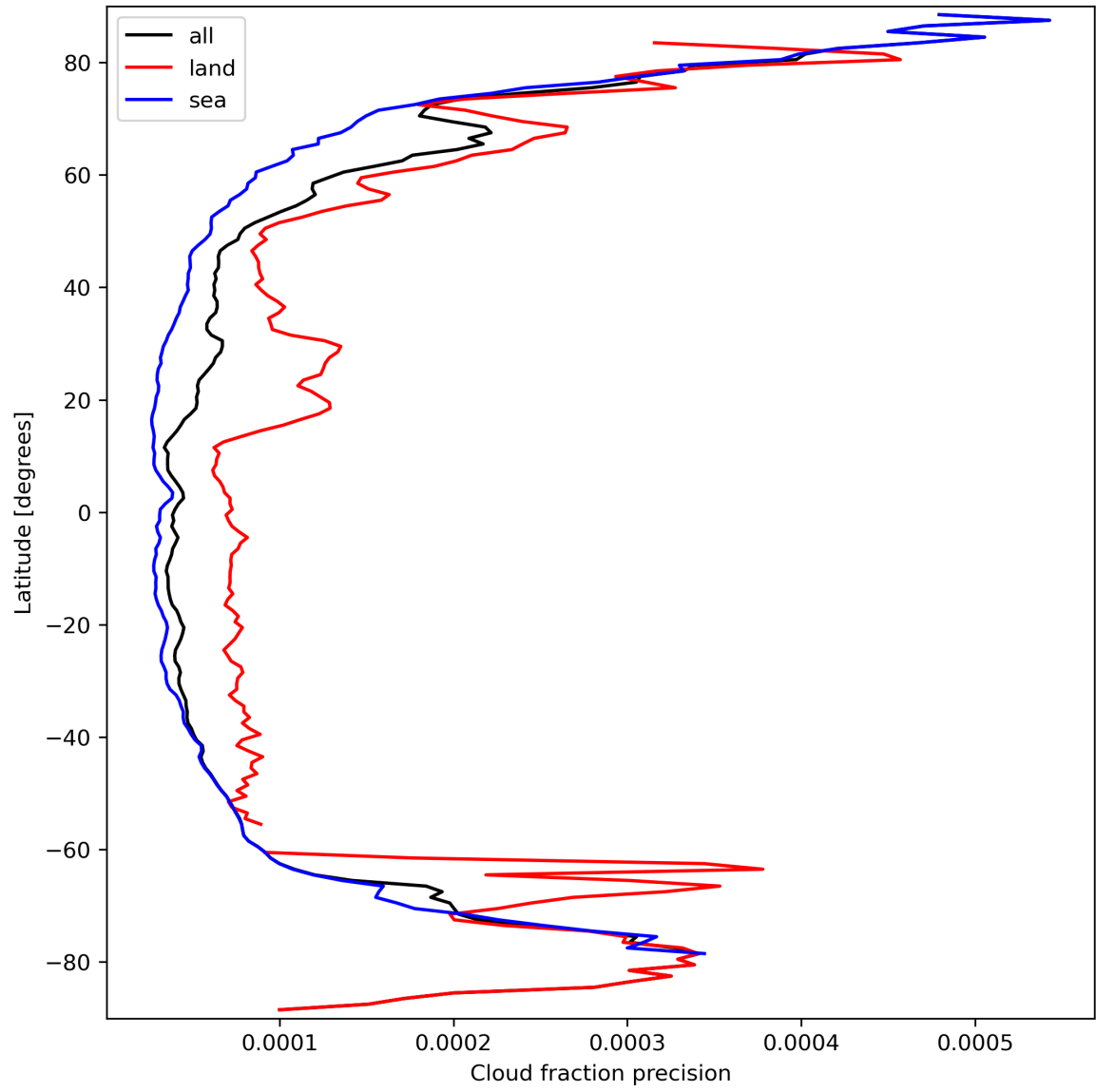
Figure 16: Zonal average of “Cloud fraction precision” for 2024-03-20 to 2024-03-21.
