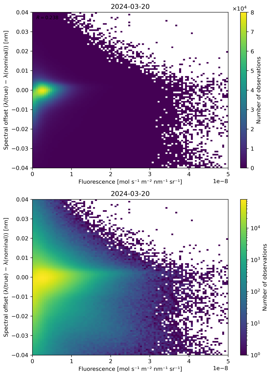
Figure 87: Scatter density plot of “Fluorescence” against “Spectral offset ( \lambda(\text{true}) - \lambda(\text{nominal}) )” for 2024-03-20 to 2024-03-21.
