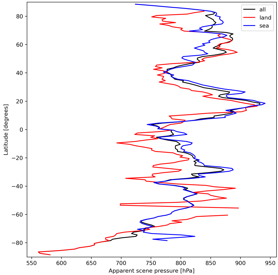
Figure 19: Zonal average of “Apparent scene pressure” for 2024-03-20 to 2024-03-21.
