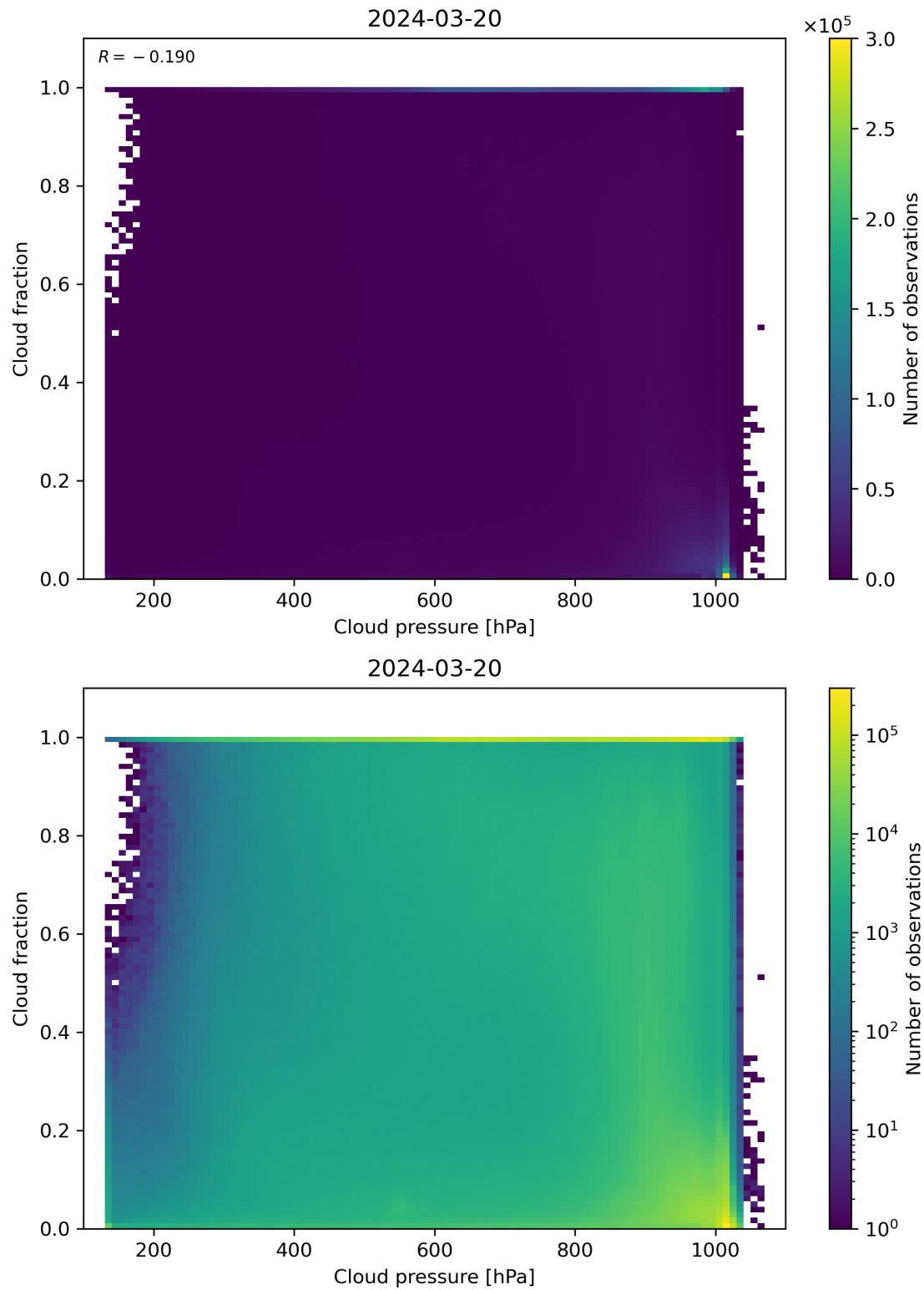
Figure 79: Scatter density plot of “Cloud pressure” against “Cloud fraction” for 2024-03-20 to 2024-03-21.
