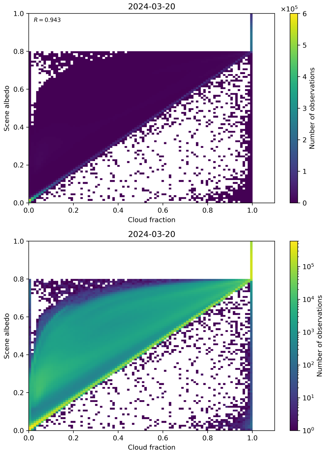
Figure 75: Scatter density plot of “Cloud fraction” against “Scene albedo” for 2024-03-20 to 2024-03-21.
