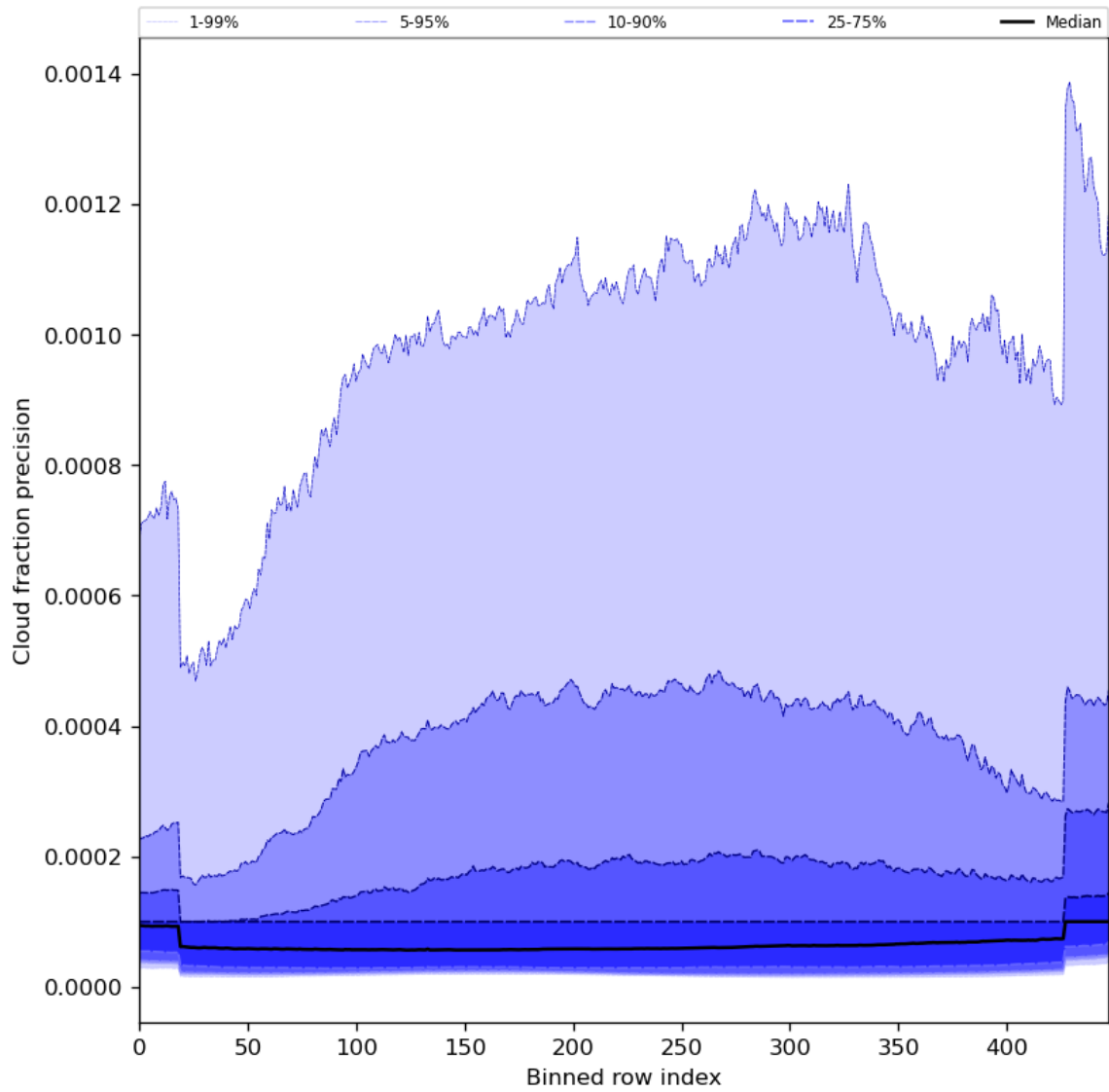
Figure 50: Along track statistics of “Cloud fraction precision” for 2024-03-20 to 2024-03-21
