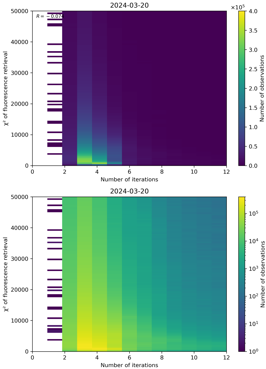
Figure 97: Scatter density plot of “Number of iterations” against “ \chi^2 of fluorescence retrieval” for 2024-03-20 to 2024-03-21.
