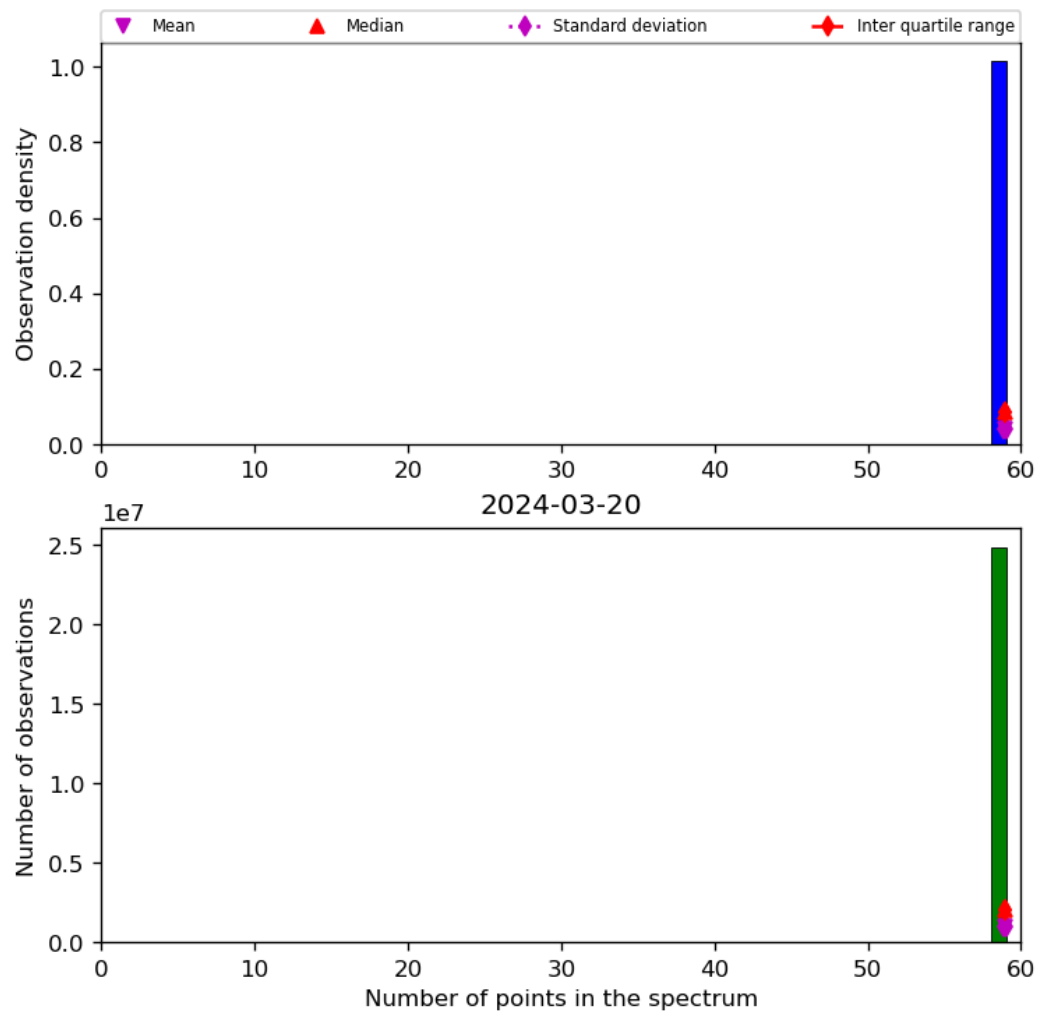
Figure 44: Histogram of “Number of points in the spectrum” for 2024-03-20 to 2024-03-21
