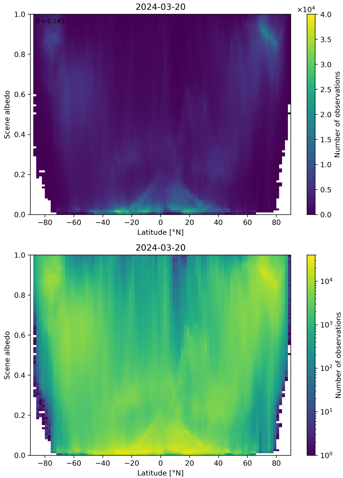
Figure 95: Scatter density plot of “Latitude” against “Scene albedo” for 2024-03-20 to 2024-03-21.
