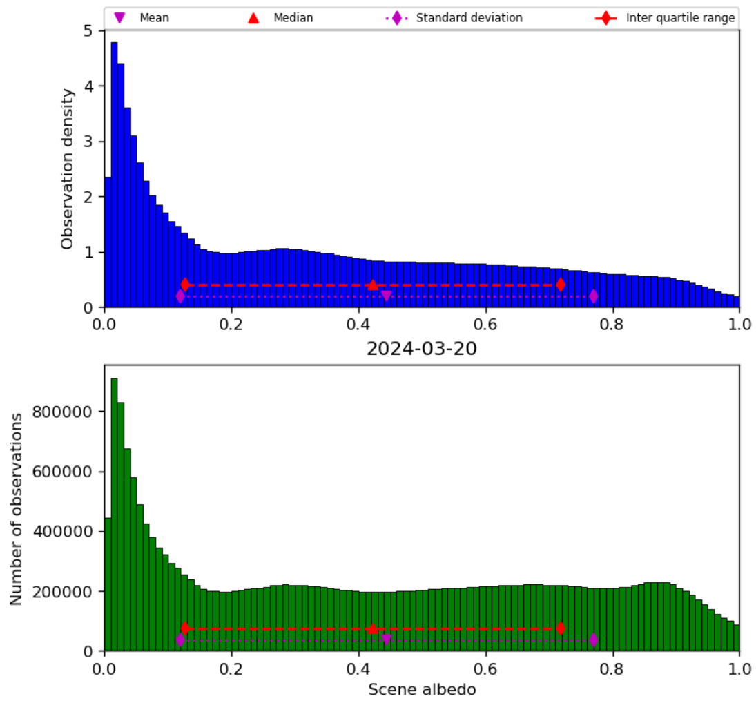
Figure 34: Histogram of “Scene albedo” for 2024-03-20 to 2024-03-21
