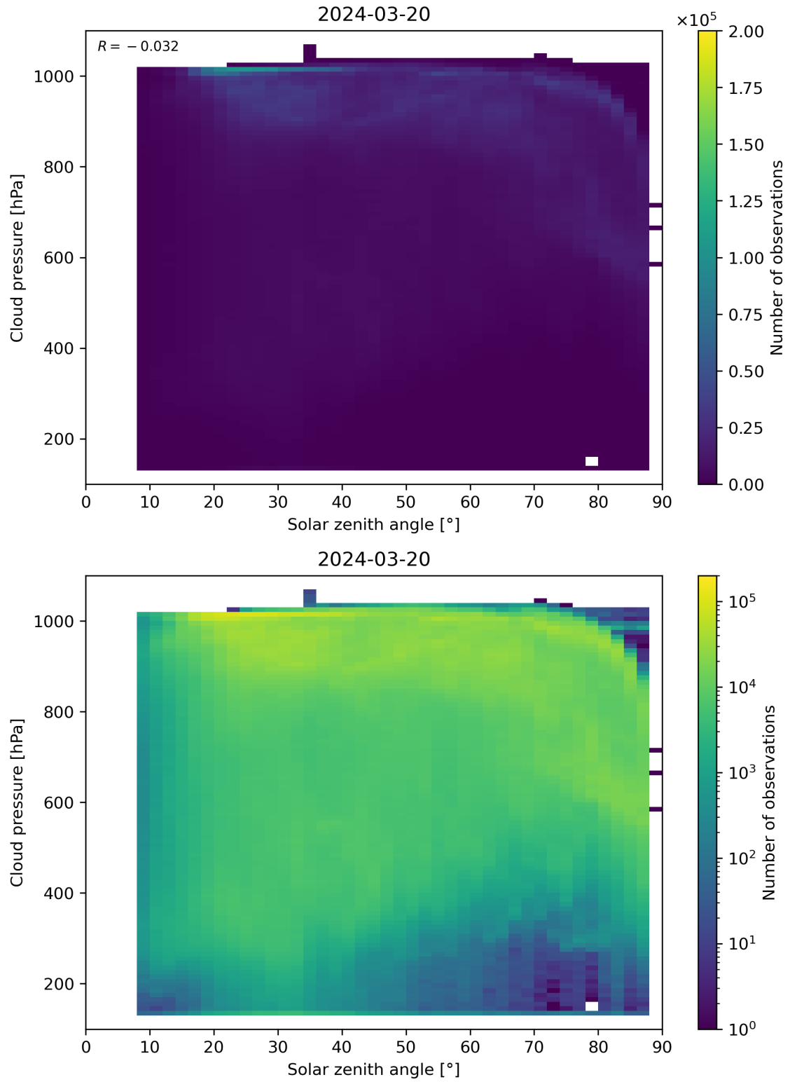
Figure 111: Scatter density plot of “Solar zenith angle” against “Cloud pressure” for 2024-03-20 to 2024-03-21.
