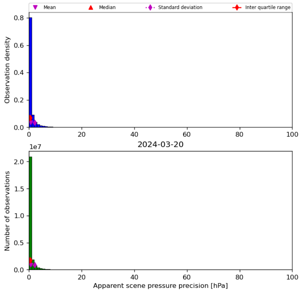
Figure 37: Histogram of “Apparent scene pressure precision” for 2024-03-20 to 2024-03-21
