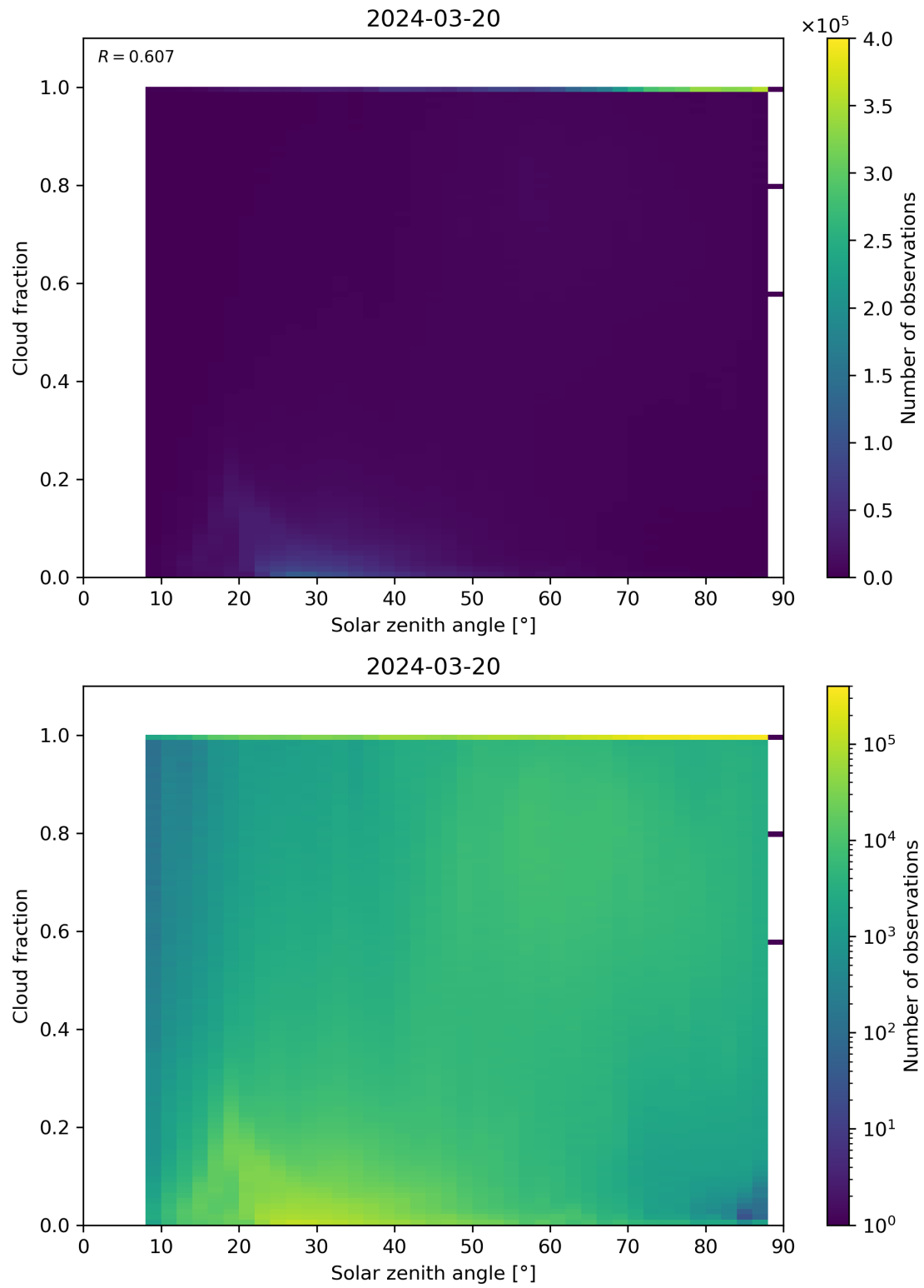
Figure 110: Scatter density plot of “Solar zenith angle” against “Cloud fraction” for 2024-03-20 to 2024-03-21.
