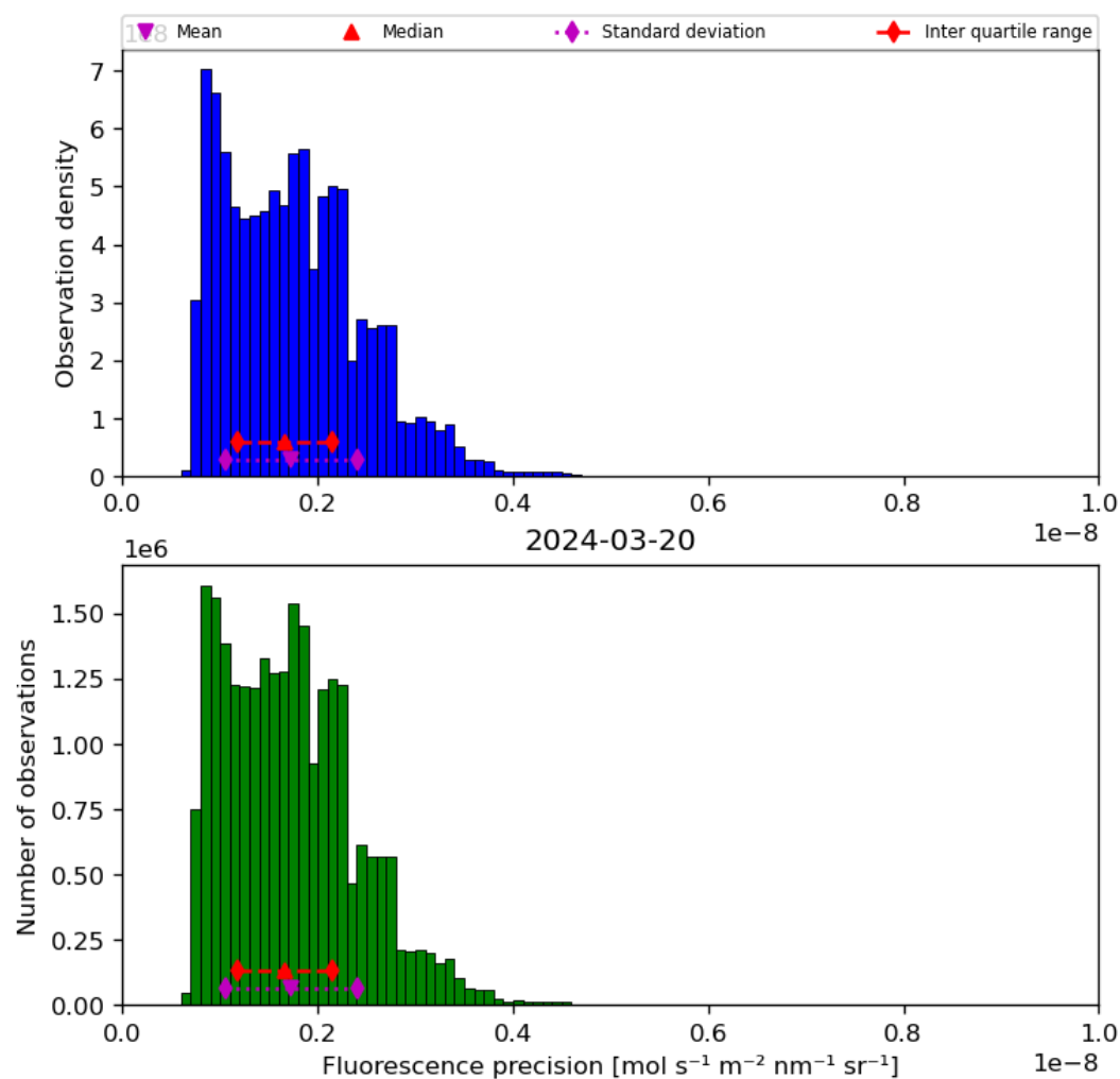
Figure 41: Histogram of “Fluorescence precision” for 2024-03-20 to 2024-03-21
