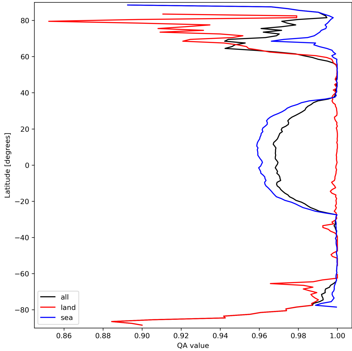
Figure 12: Zonal average of “QA value” for 2024-03-20 to 2024-03-21.
