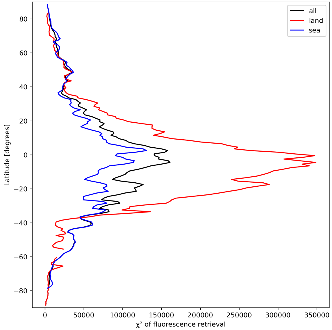
Figure 25: Zonal average of “ \chi^2 of fluorescence retrieval” for 2024-03-20 to 2024-03-21.
