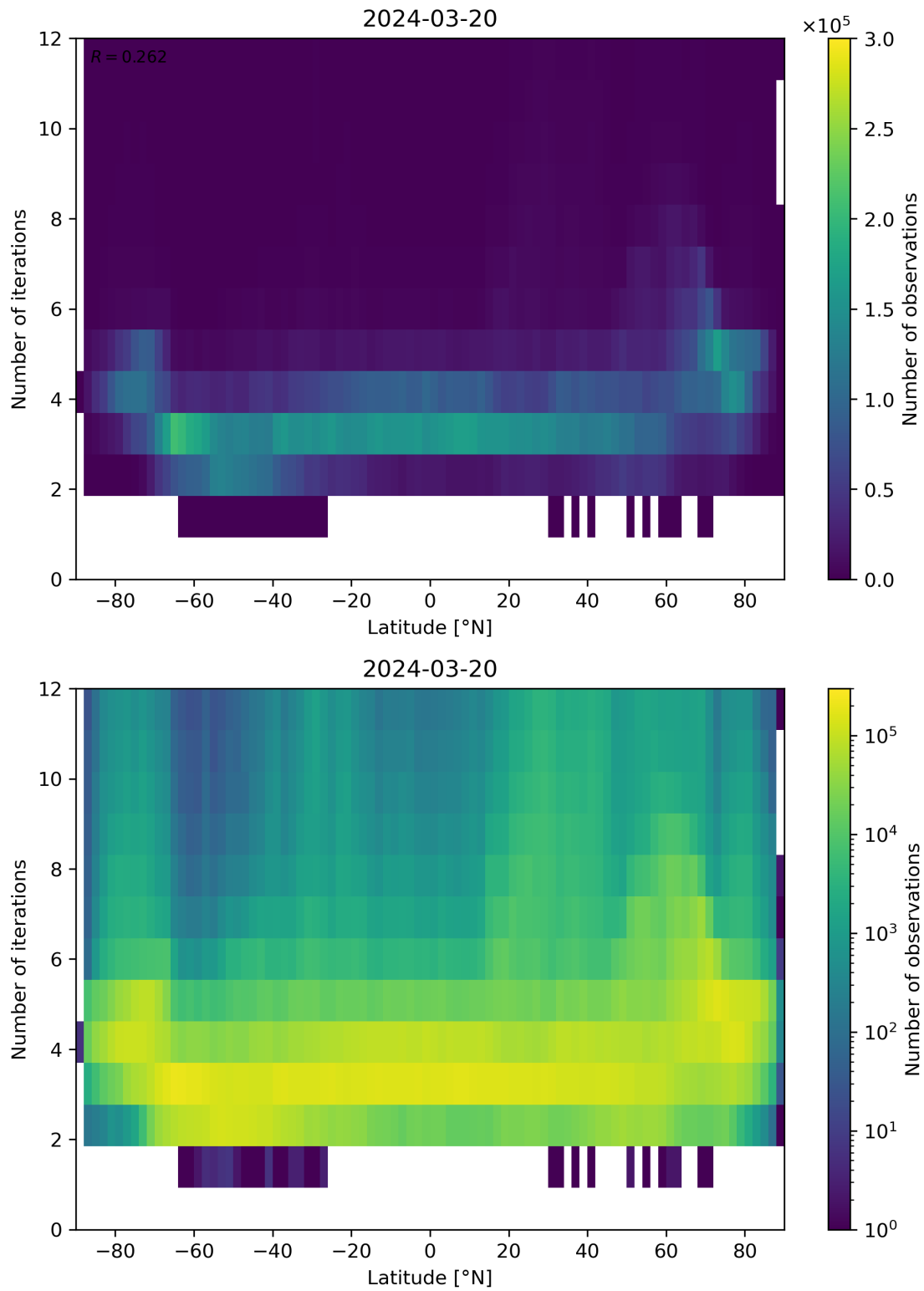
Figure 93: Scatter density plot of “Latitude” against “Number of iterations” for 2024-03-20 to 2024-03-21.
