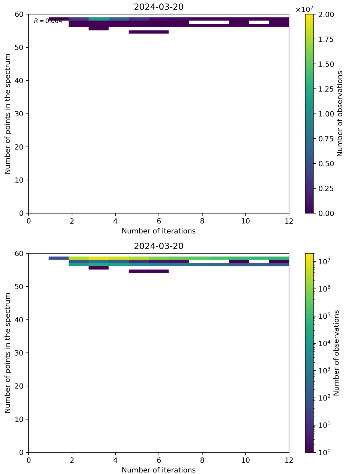
Figure 99: Scatter density plot of “Number of iterations” against “Number of points in the spectrum” for 2024-03-20 to 2024-03-21.
