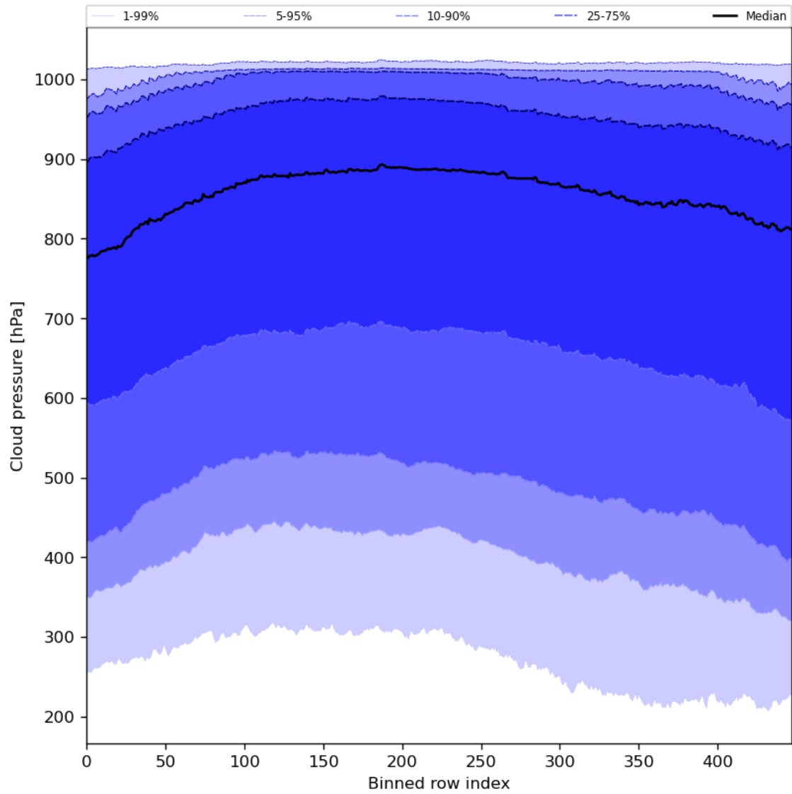
Figure 47: Along track statistics of “Cloud pressure” for 2024-03-20 to 2024-03-21
