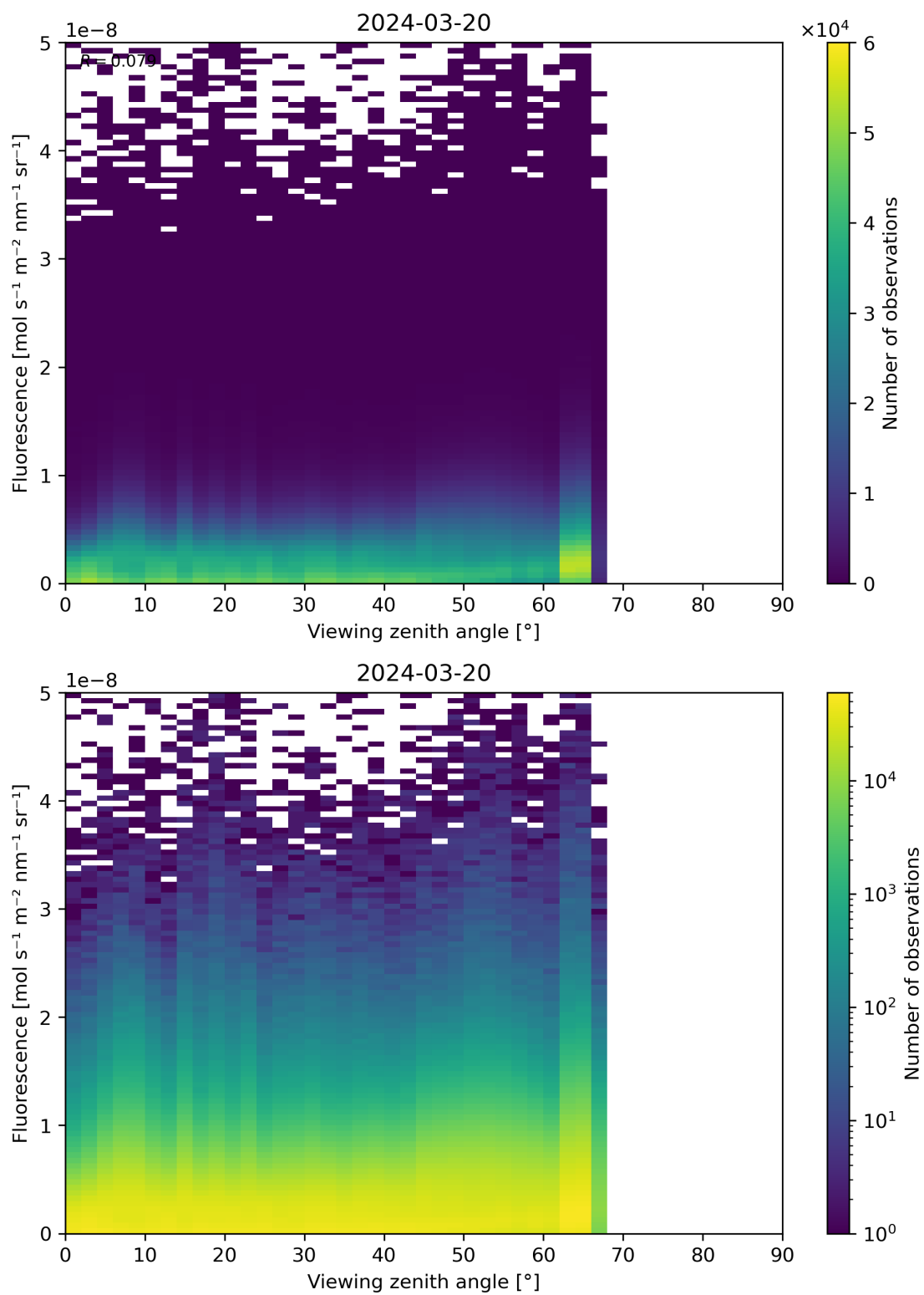
Figure 122: Scatter density plot of “Viewing zenith angle” against “Fluorescence” for 2024-03-20 to 2024-03-21.
