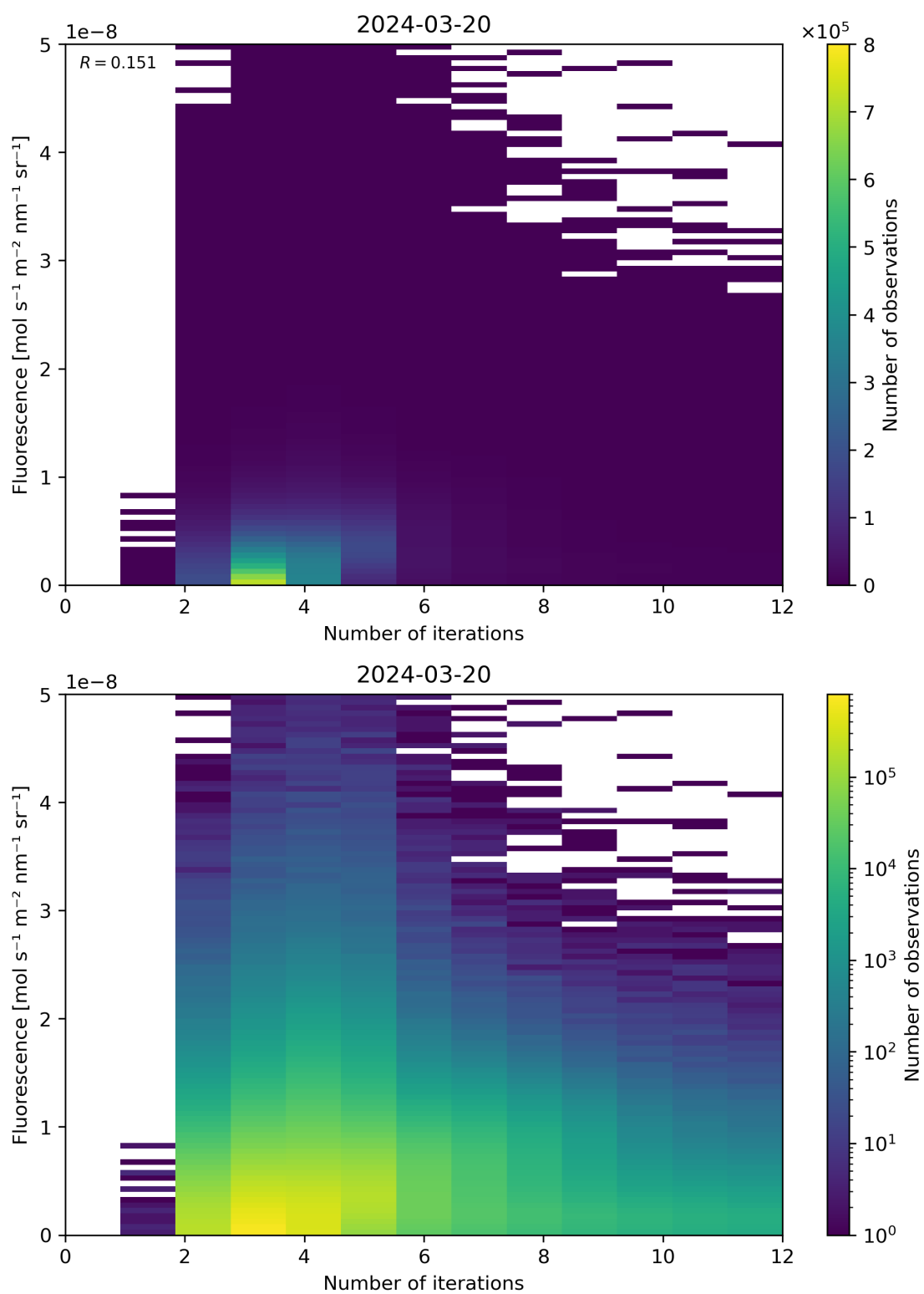
Figure 98: Scatter density plot of “Number of iterations” against “Fluorescence” for 2024-03-20 to 2024-03-21.
