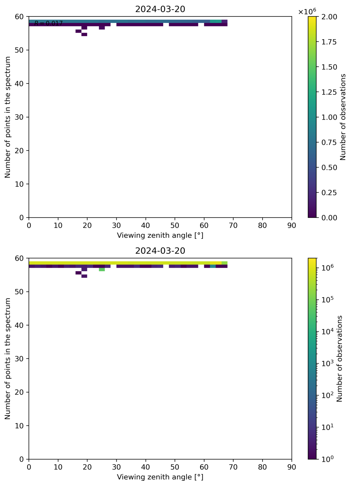
Figure 125: Scatter density plot of “Viewing zenith angle” against “Number of points in the spectrum” for 2024-03-20 to 2024-03-21.
