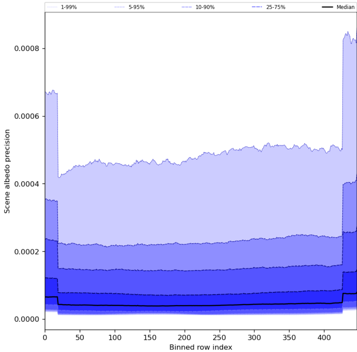
Figure 52: Along track statistics of “Scene albedo precision” for 2024-03-20 to 2024-03-21
