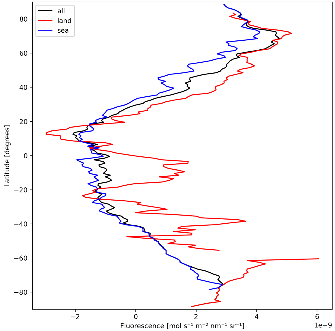
Figure 23: Zonal average of “Fluorescence” for 2024-03-20 to 2024-03-21.
