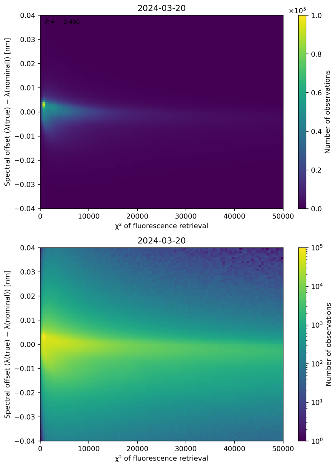
Figure 69: Scatter density plot of " \chi^2 of fluorescence retrieval" against "Spectral offset ( \lambda(\text{true}) - \lambda(\text{nominal})) " for 2024-03-20 to 2024-03-21.
