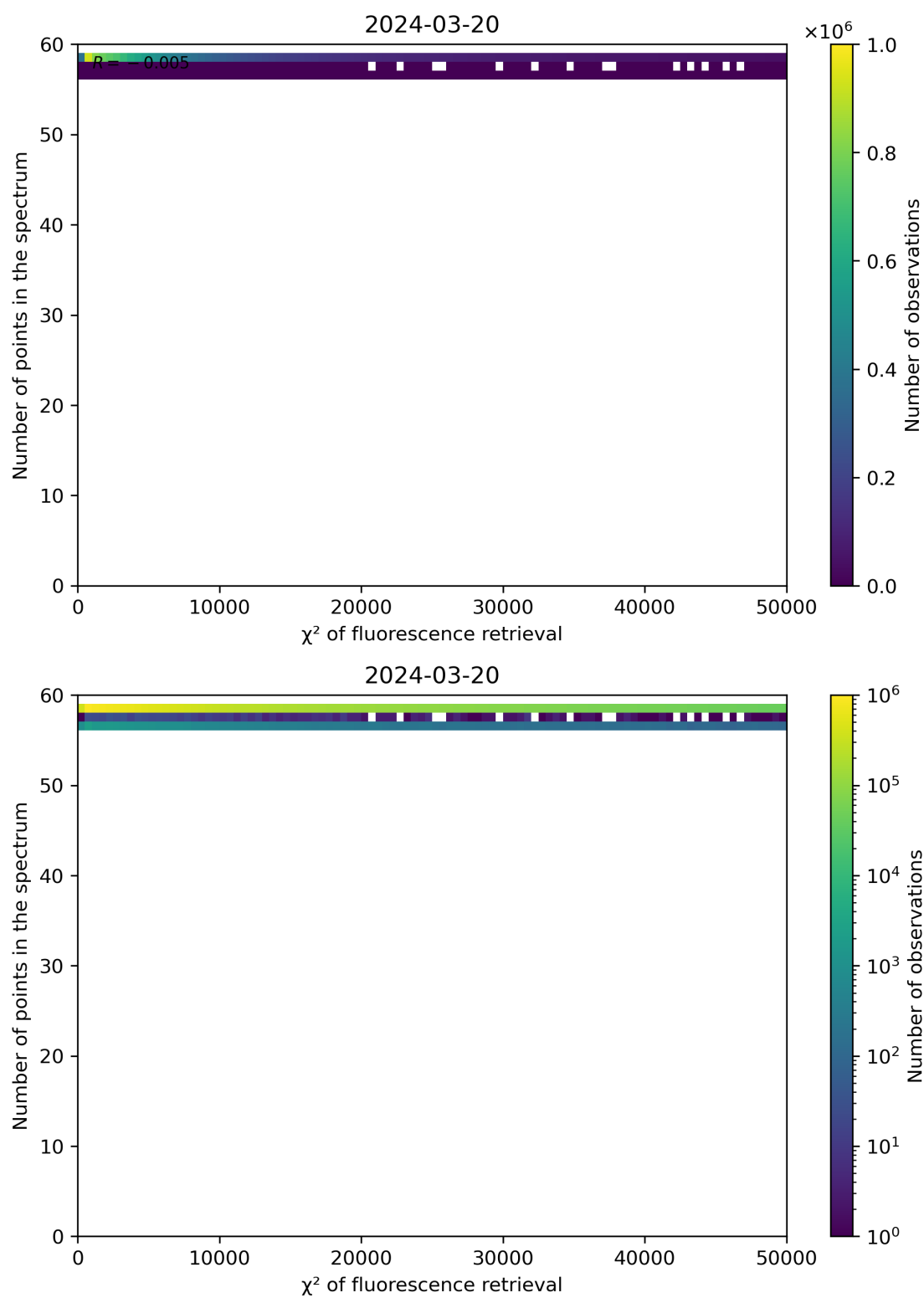
Figure 68: Scatter density plot of “ \chi^2 of fluorescence retrieval” against “Number of points in the spectrum” for 2024-03-20 to 2024-03-21.
