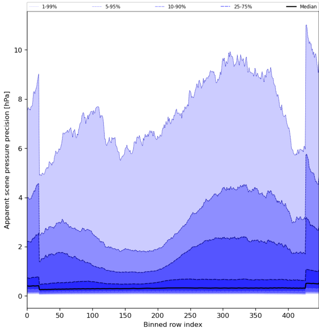
Figure 54: Along track statistics of “Apparent scene pressure precision” for 2024-03-20 to 2024-03-21
