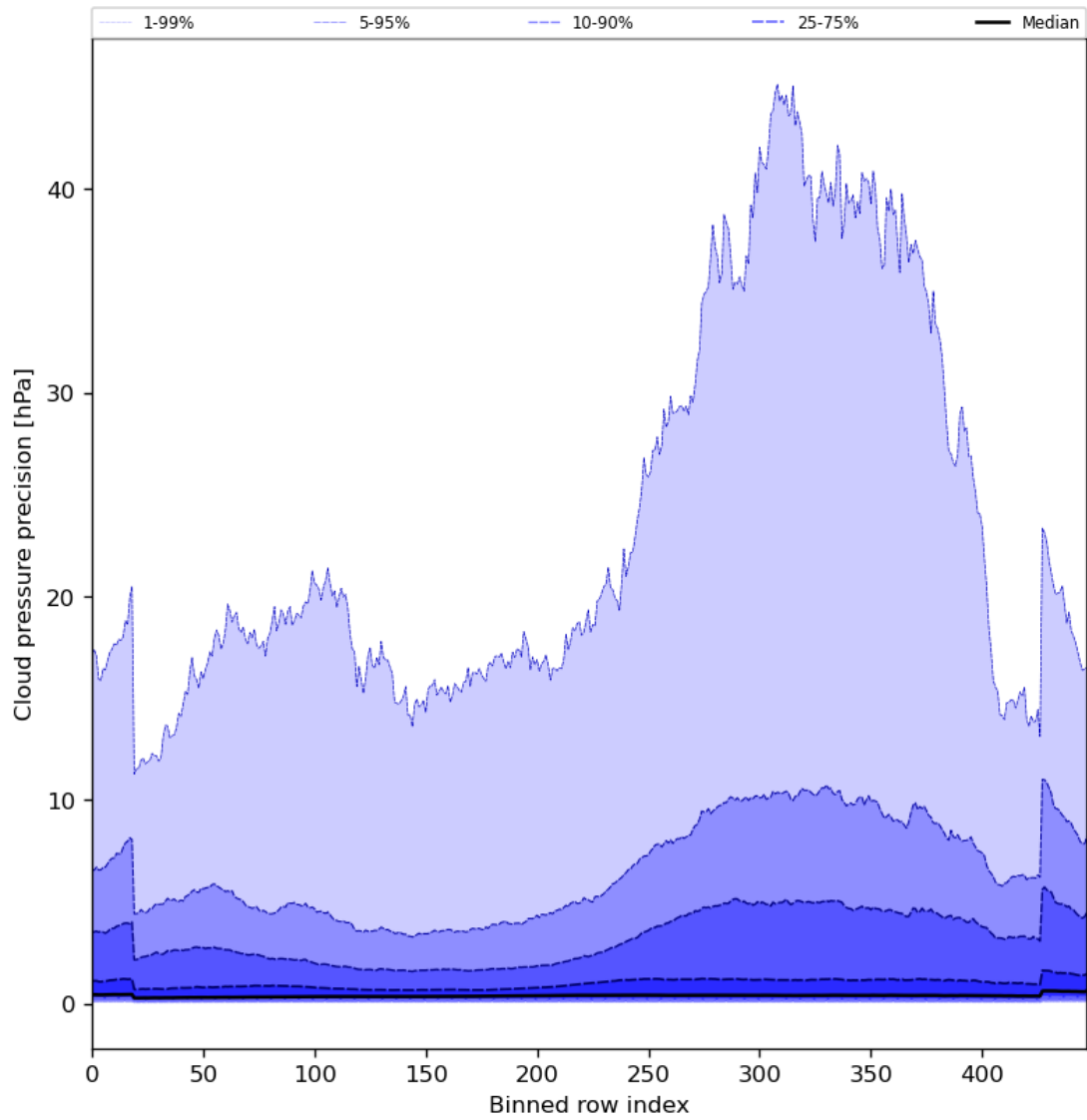
Figure 48: Along track statistics of “Cloud pressure precision” for 2024-03-20 to 2024-03-21
