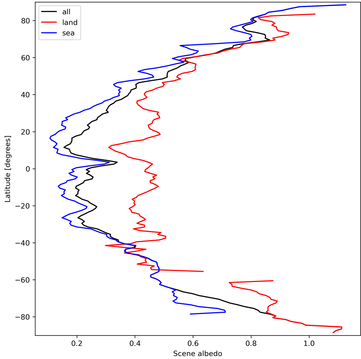
Figure 17: Zonal average of “Scene albedo” for 2024-03-20 to 2024-03-21.
