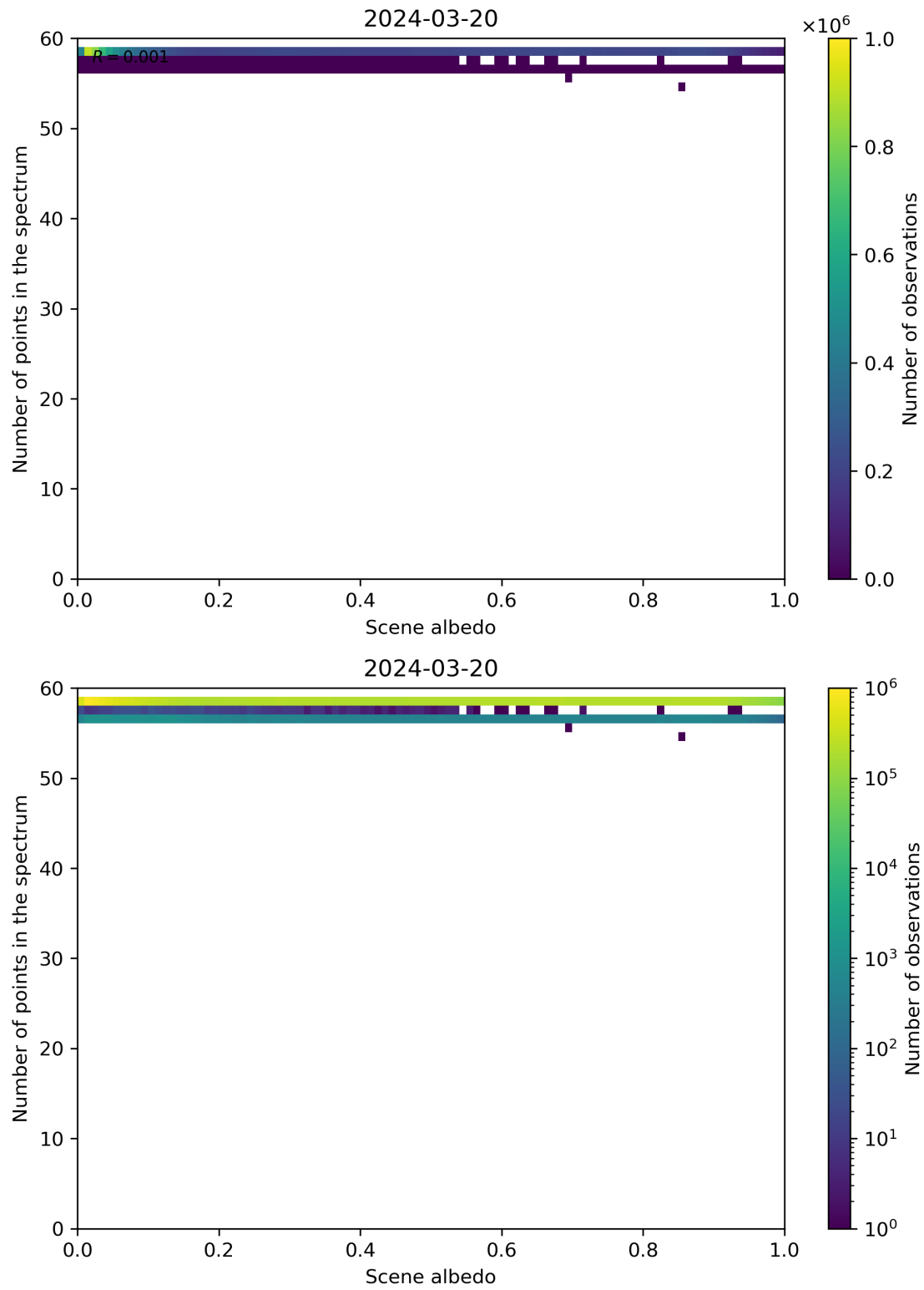
Figure 106: Scatter density plot of “Scene albedo” against “Number of points in the spectrum” for 2024-03-20 to 2024-03-21.
