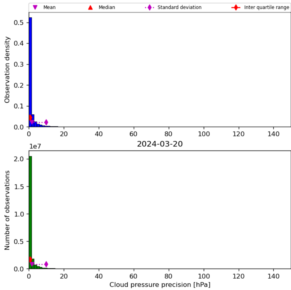
Figure 31: Histogram of “Cloud pressure precision” for 2024-03-20 to 2024-03-21
