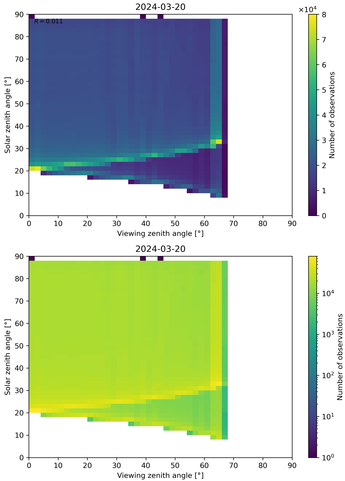
Figure 127: Scatter density plot of “Viewing zenith angle” against “Solar zenith angle” for 2024-03-20 to 2024-03-21.
