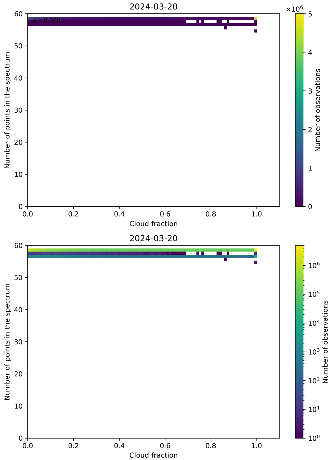
Figure 74: Scatter density plot of “Cloud fraction” against “Number of points in the spectrum” for 2024-03-20 to 2024-03-21.
