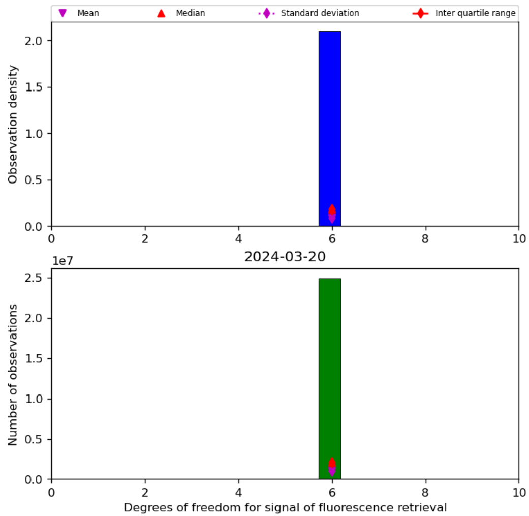
Figure 43: Histogram of “Degrees of freedom for signal of fluorescence retrieval” for 2024-03-20 to 2024-03-21
