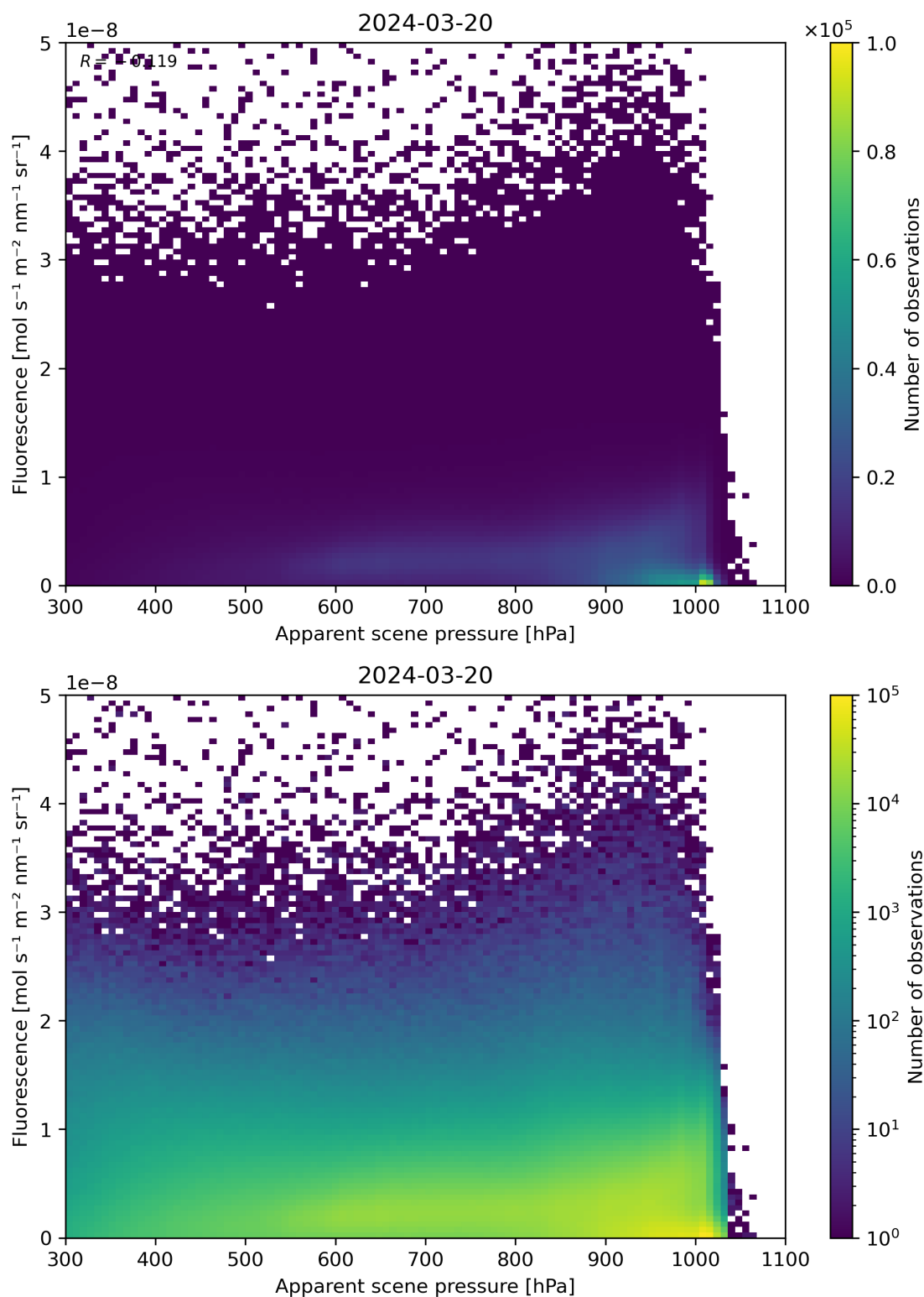
Figure 64: Scatter density plot of “Apparent scene pressure” against “Fluorescence” for 2024-03-20 to 2024-03-21.
