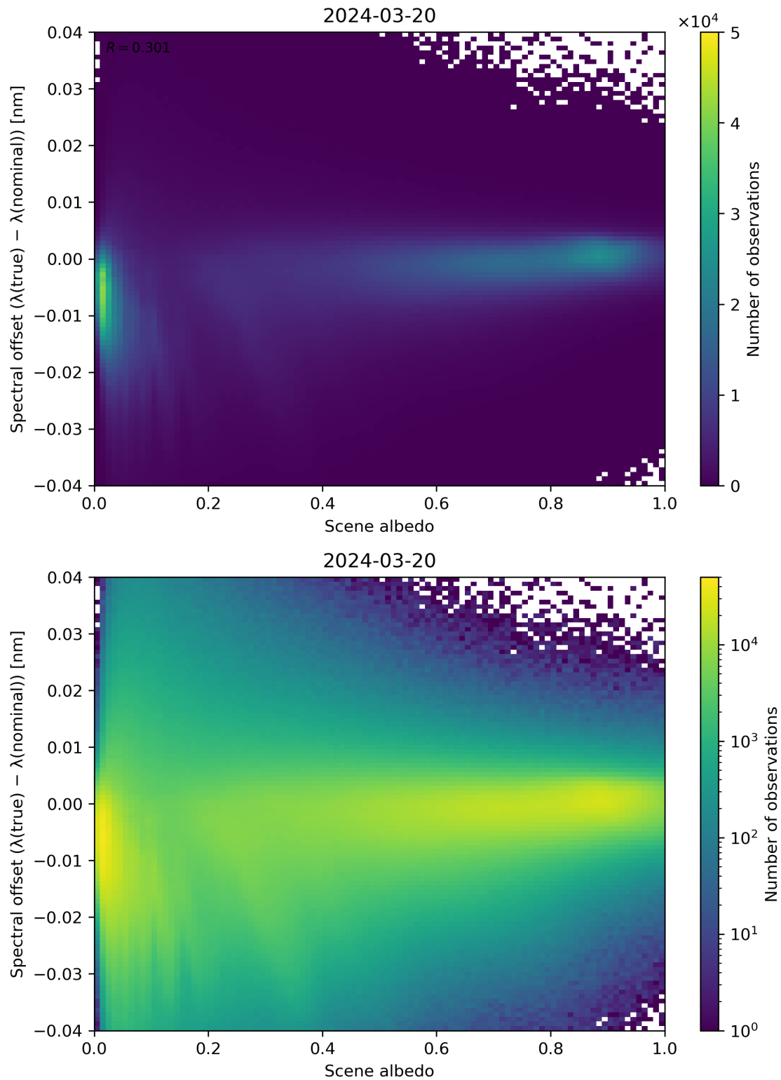
Figure 107: Scatter density plot of “Scene albedo” against “Spectral offset ( \lambda(\text{true}) - \lambda(\text{nominal}) )” for 2024-03-20 to 2024-03-21.
