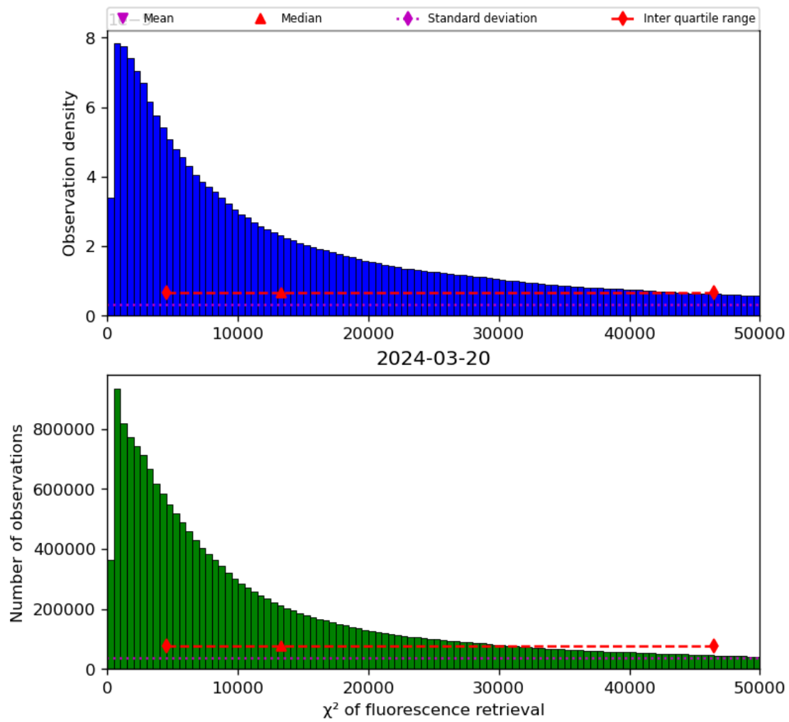
Figure 42: Histogram of “ \chi^2 of fluorescence retrieval” for 2024-03-20 to 2024-03-21
