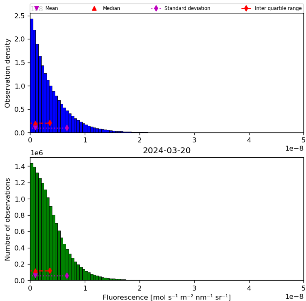
Figure 40: Histogram of “Fluorescence” for 2024-03-20 to 2024-03-21
