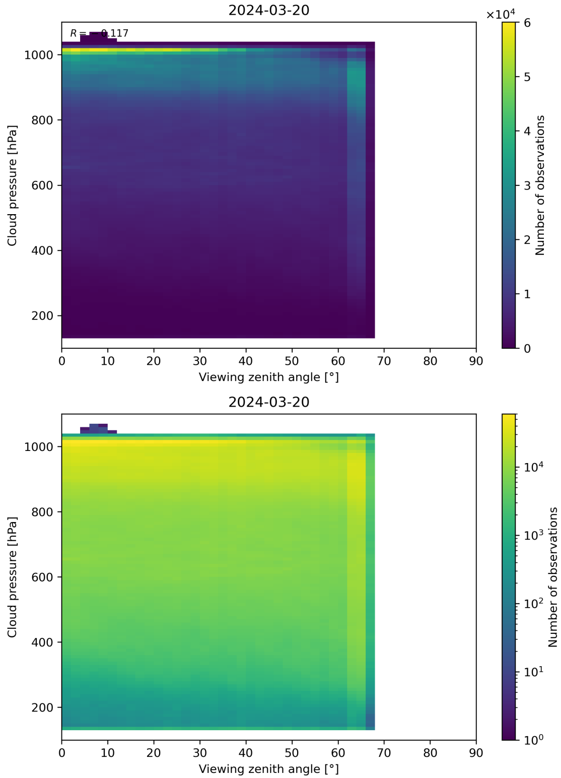
Figure 121: Scatter density plot of “Viewing zenith angle” against “Cloud pressure” for 2024-03-20 to 2024-03-21.
