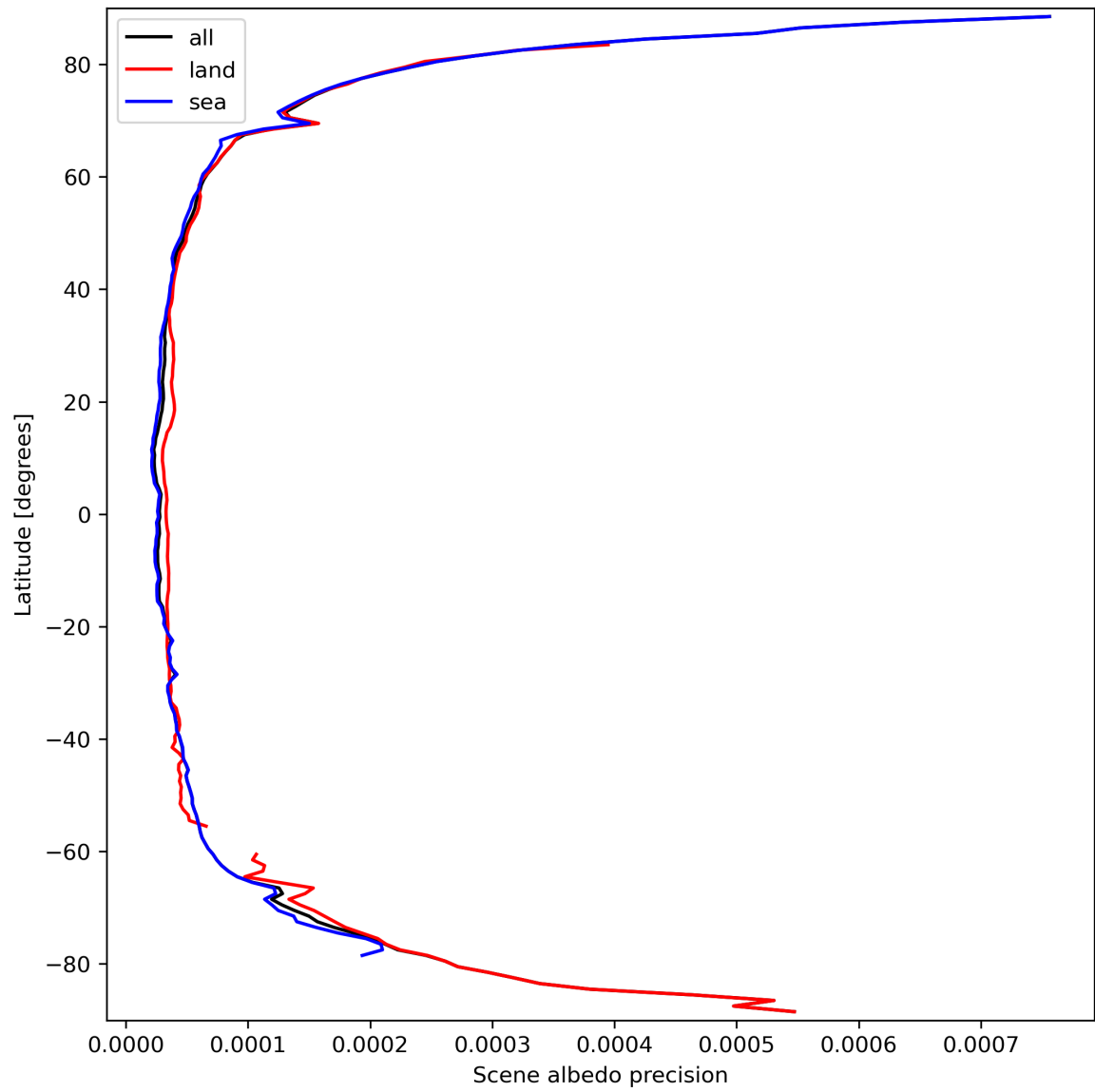
Figure 18: Zonal average of “Scene albedo precision” for 2024-03-20 to 2024-03-21.
