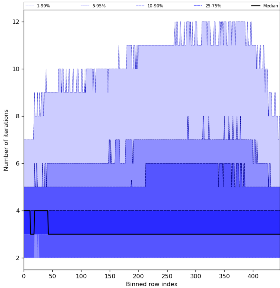
Figure 56: Along track statistics of “Number of iterations” for 2024-03-20 to 2024-03-21
