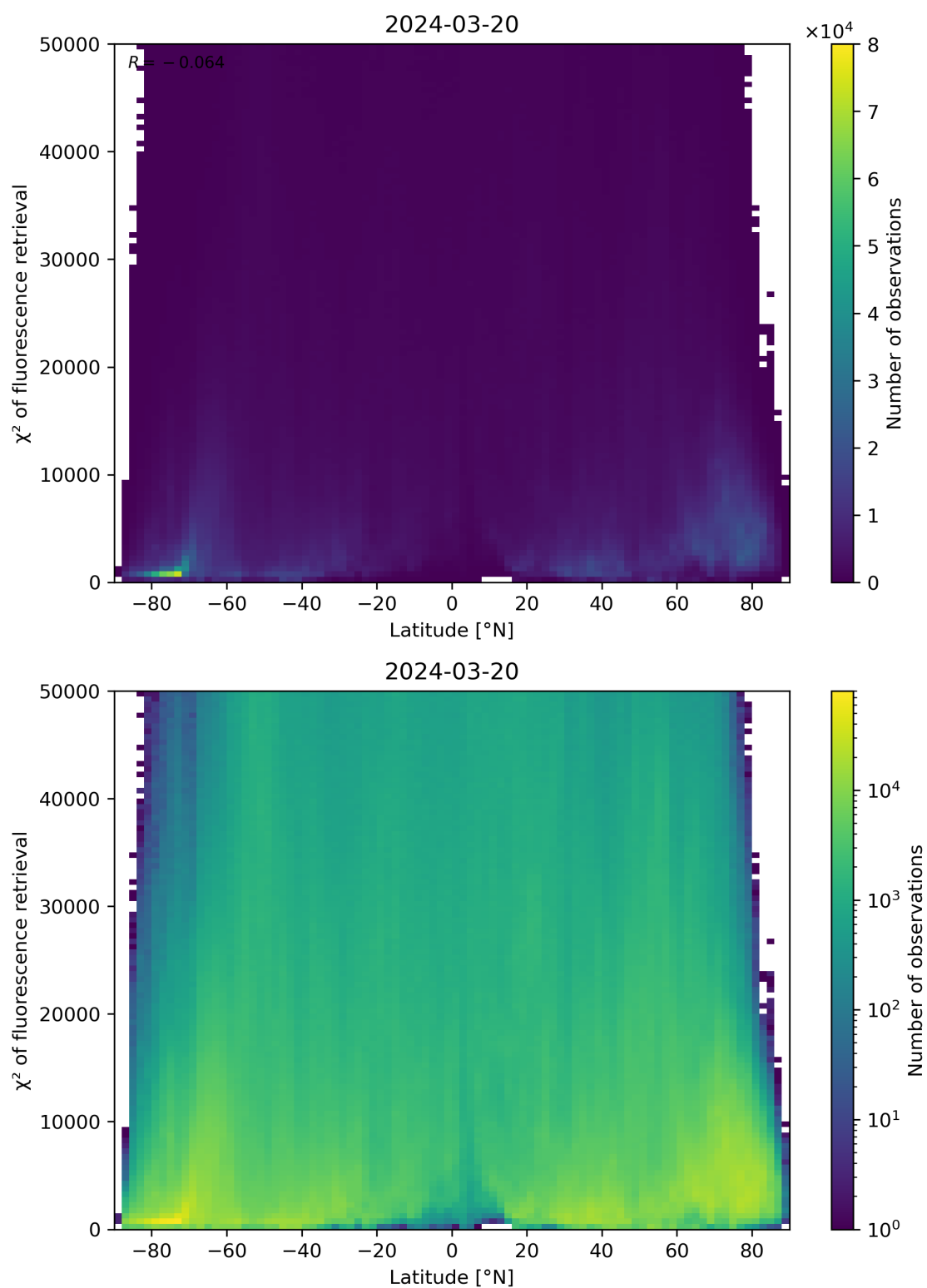
Figure 89: Scatter density plot of “Latitude” against “ \chi^2 of fluorescence retrieval” for 2024-03-20 to 2024-03-21.
