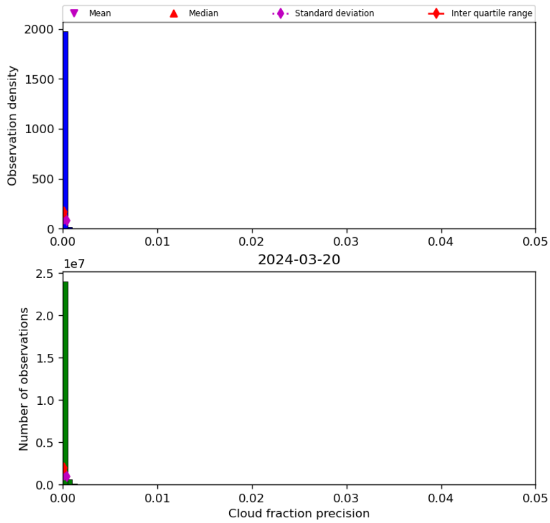
Figure 33: Histogram of “Cloud fraction precision” for 2024-03-20 to 2024-03-21
