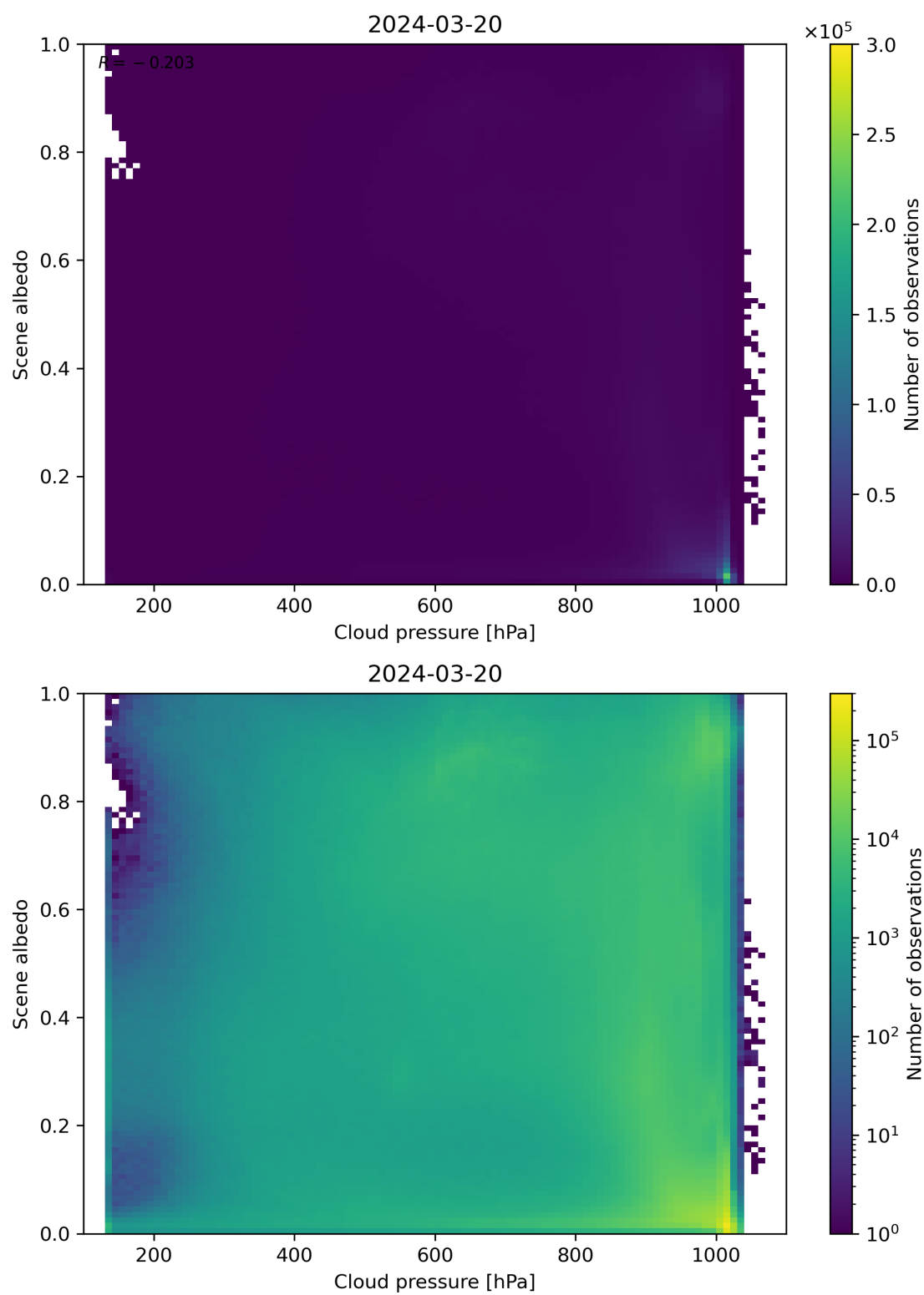
Figure 83: Scatter density plot of “Cloud pressure” against “Scene albedo” for 2024-03-20 to 2024-03-21.
