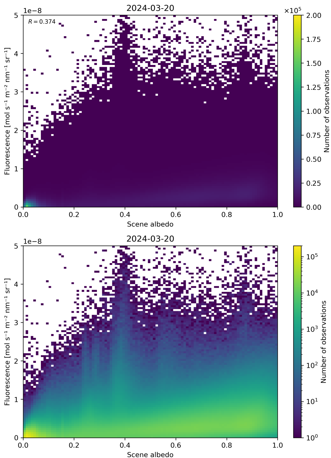
Figure 104: Scatter density plot of “Scene albedo” against “Fluorescence” for 2024-03-20 to 2024-03-21.
