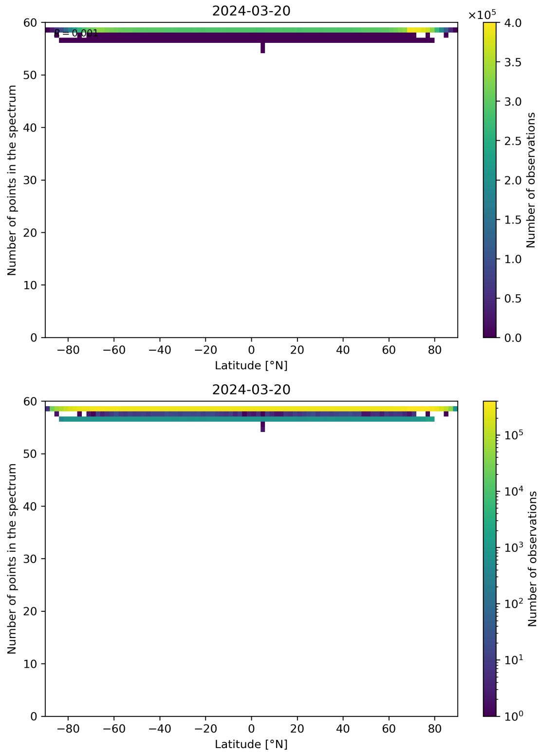
Figure 94: Scatter density plot of “Latitude” against “Number of points in the spectrum” for 2024-03-20 to 2024-03-21.
