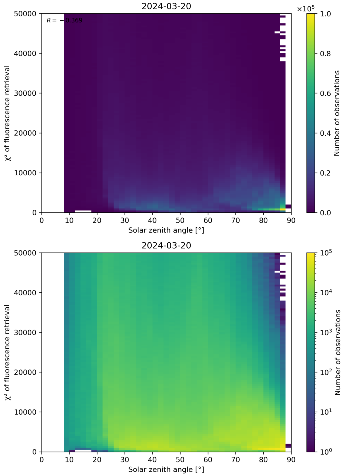
Figure 109: Scatter density plot of “Solar zenith angle” against “ \chi^2 of fluorescence retrieval” for 2024-03-20 to 2024-03-21.
