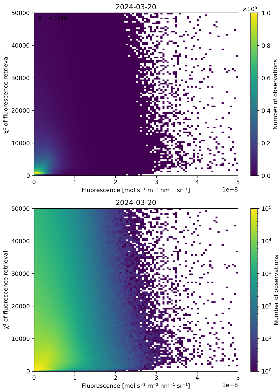
Figure 85: Scatter density plot of “Fluorescence” against “ \chi^2 of fluorescence retrieval” for 2024-03-20 to 2024-03-21.
