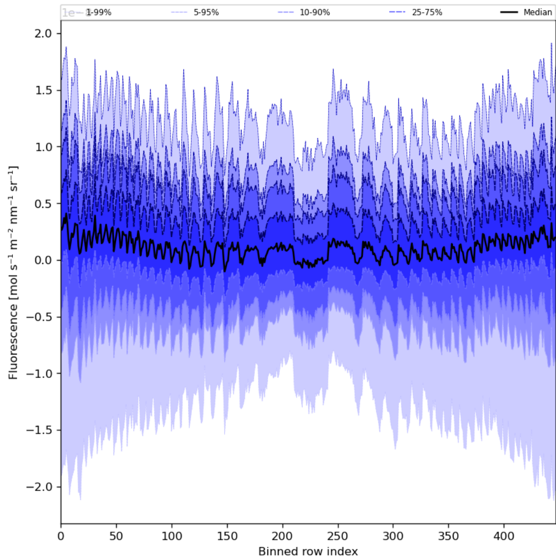
Figure 57: Along track statistics of “Fluorescence” for 2024-03-20 to 2024-03-21
