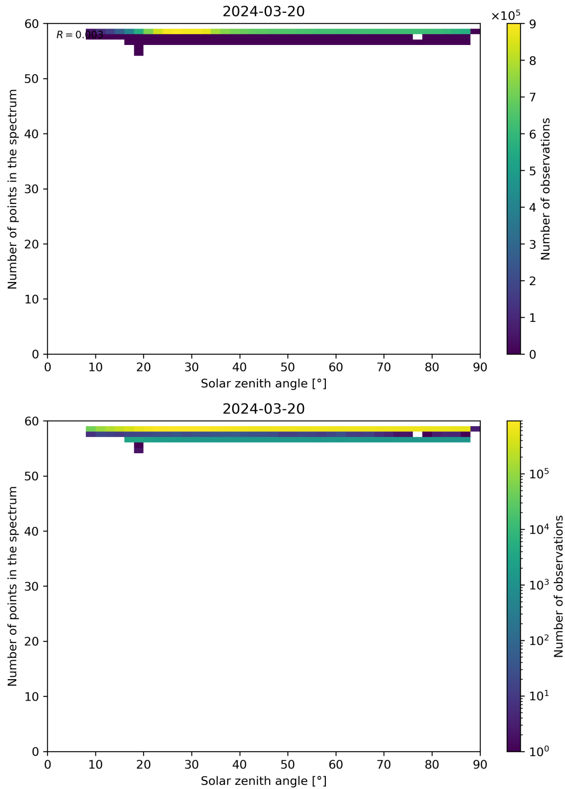
Figure 115: Scatter density plot of “Solar zenith angle” against “Number of points in the spectrum” for 2024-03-20 to 2024-03-21.
