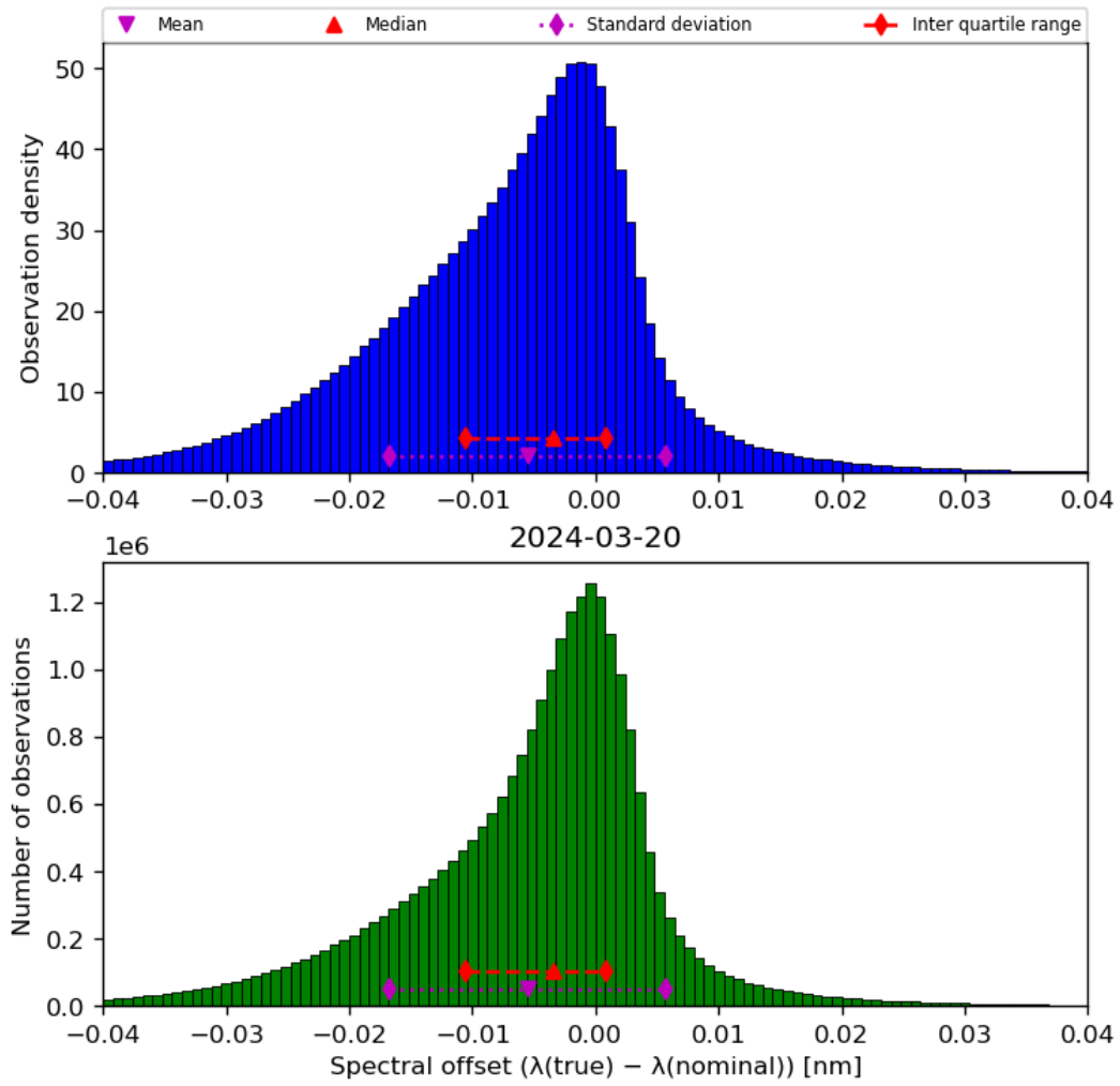
Figure 45: Histogram of “Spectral offset ( \lambda(\text{true}) - \lambda(\text{nominal}) )” for 2024-03-20 to 2024-03-21
