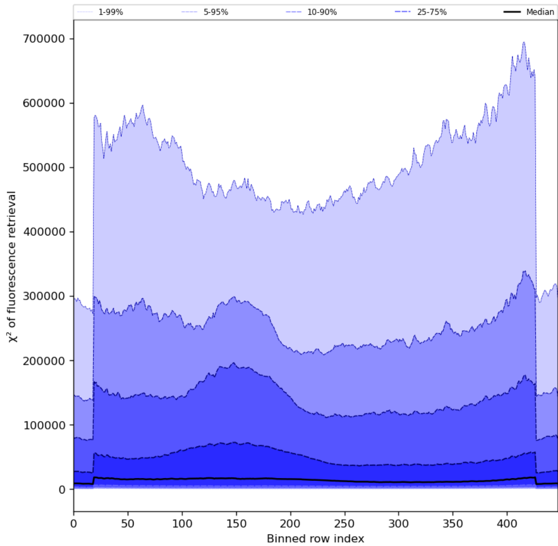
Figure 59: Along track statistics of “ \chi^2 of fluorescence retrieval” for 2024-03-20 to 2024-03-21
