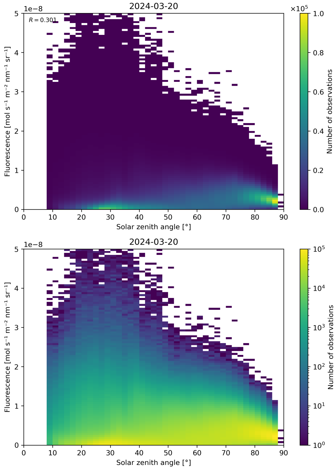
Figure 112: Scatter density plot of “Solar zenith angle” against “Fluorescence” for 2024-03-20 to 2024-03-21.
