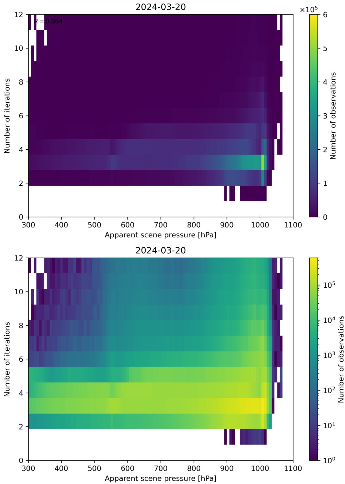
Figure 65: Scatter density plot of “Apparent scene pressure” against “Number of iterations” for 2024-03-20 to 2024-03-21.
