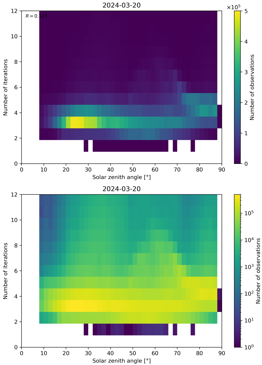
Figure 114: Scatter density plot of “Solar zenith angle” against “Number of iterations” for 2024-03-20 to 2024-03-21.
