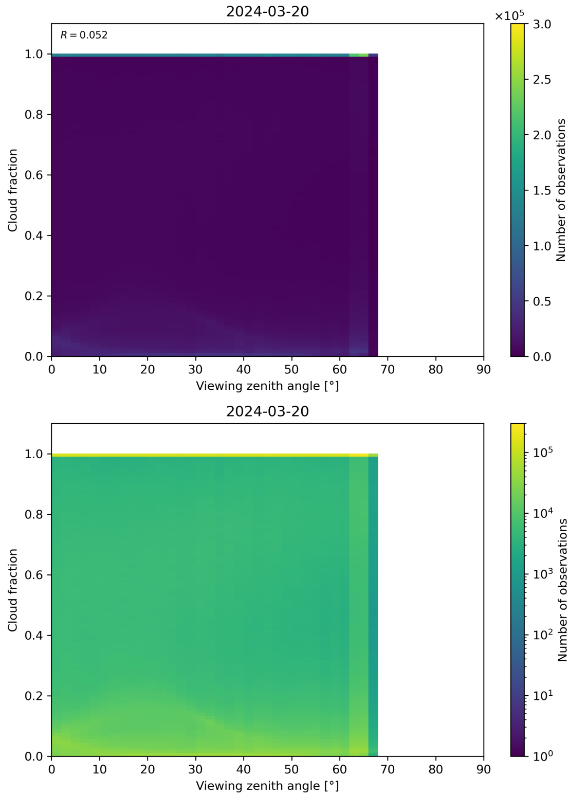
Figure 120: Scatter density plot of “Viewing zenith angle” against “Cloud fraction” for 2024-03-20 to 2024-03-21.
