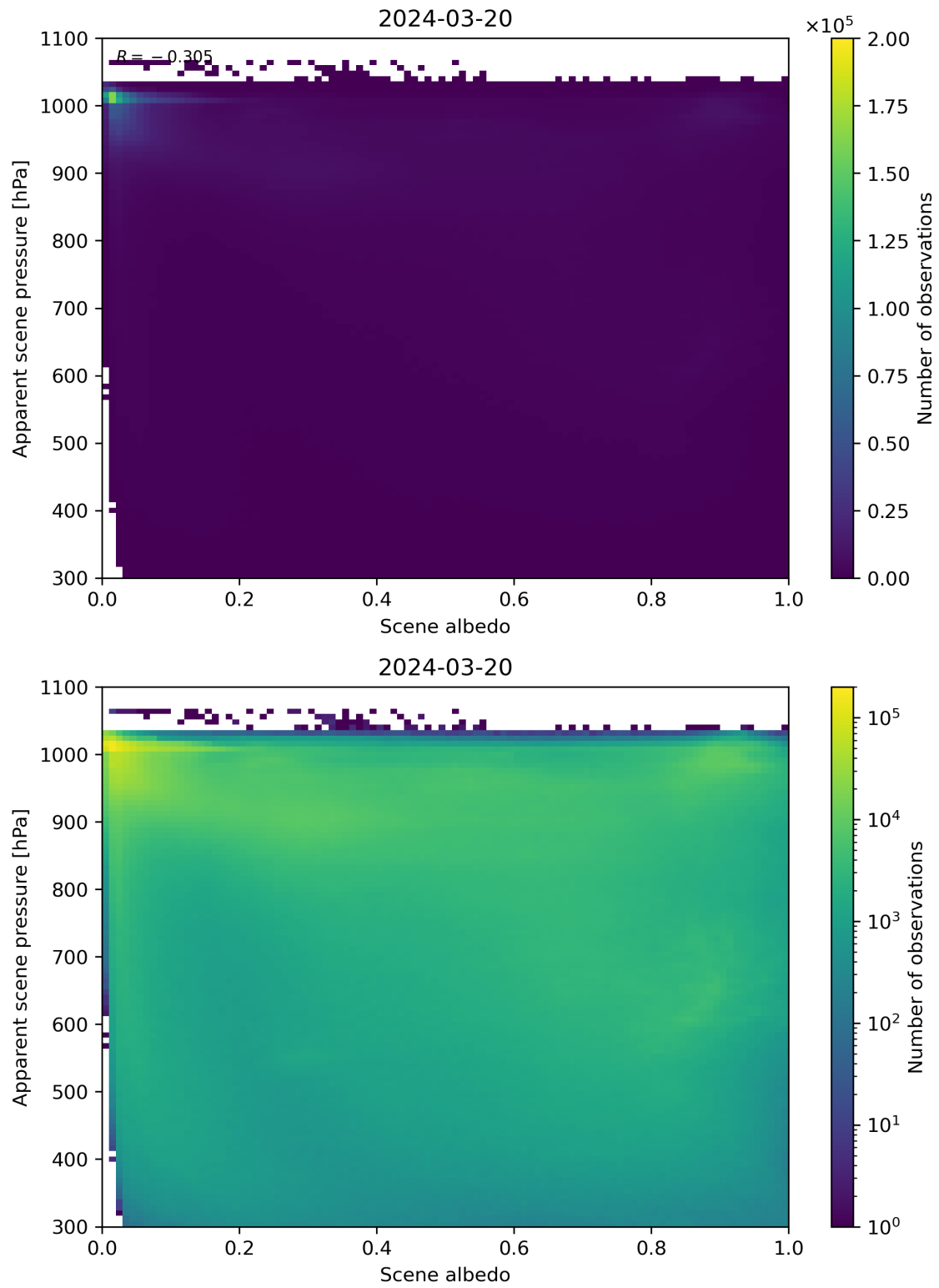
Figure 102: Scatter density plot of “Scene albedo” against “Apparent scene pressure” for 2024-03-20 to 2024-03-21.
