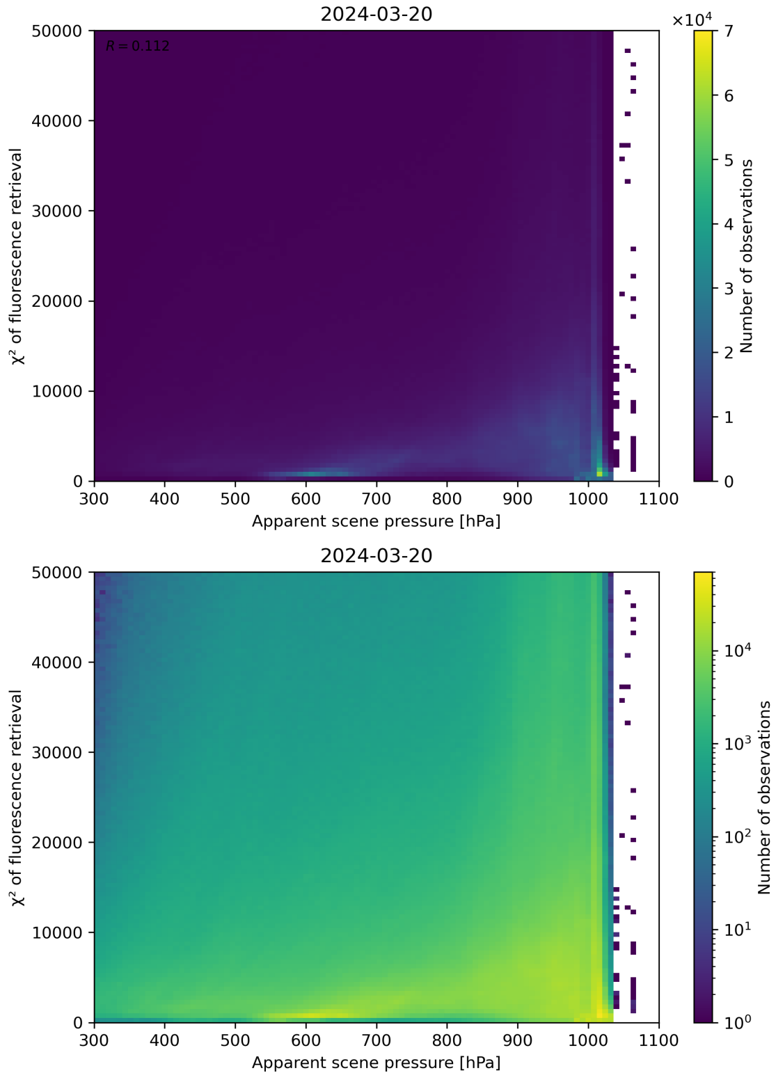
Figure 63: Scatter density plot of “Apparent scene pressure” against “ \chi^2 of fluorescence retrieval” for 2024-03-20 to 2024-03-21.
