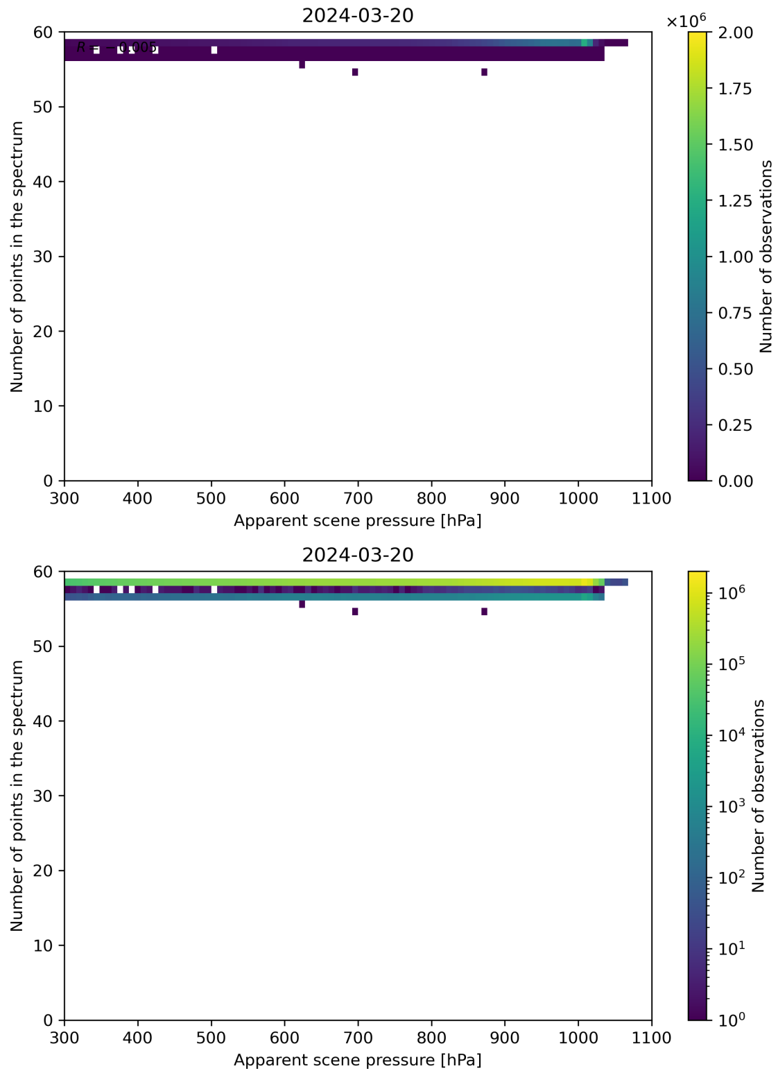
Figure 66: Scatter density plot of “Apparent scene pressure” against “Number of points in the spectrum” for 2024-03-20 to 2024-03-21.
