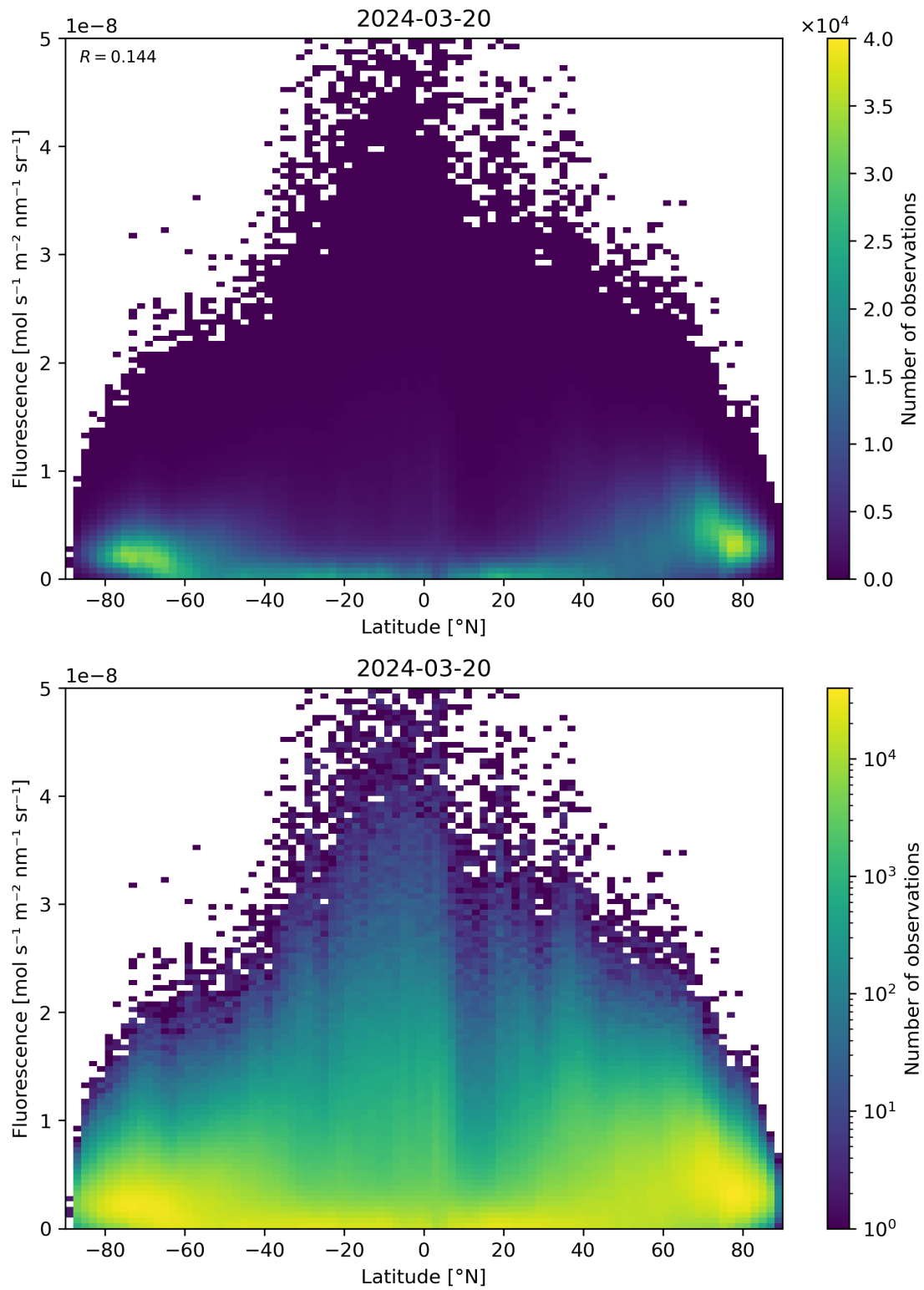
Figure 92: Scatter density plot of “Latitude” against “Fluorescence” for 2024-03-20 to 2024-03-21.
