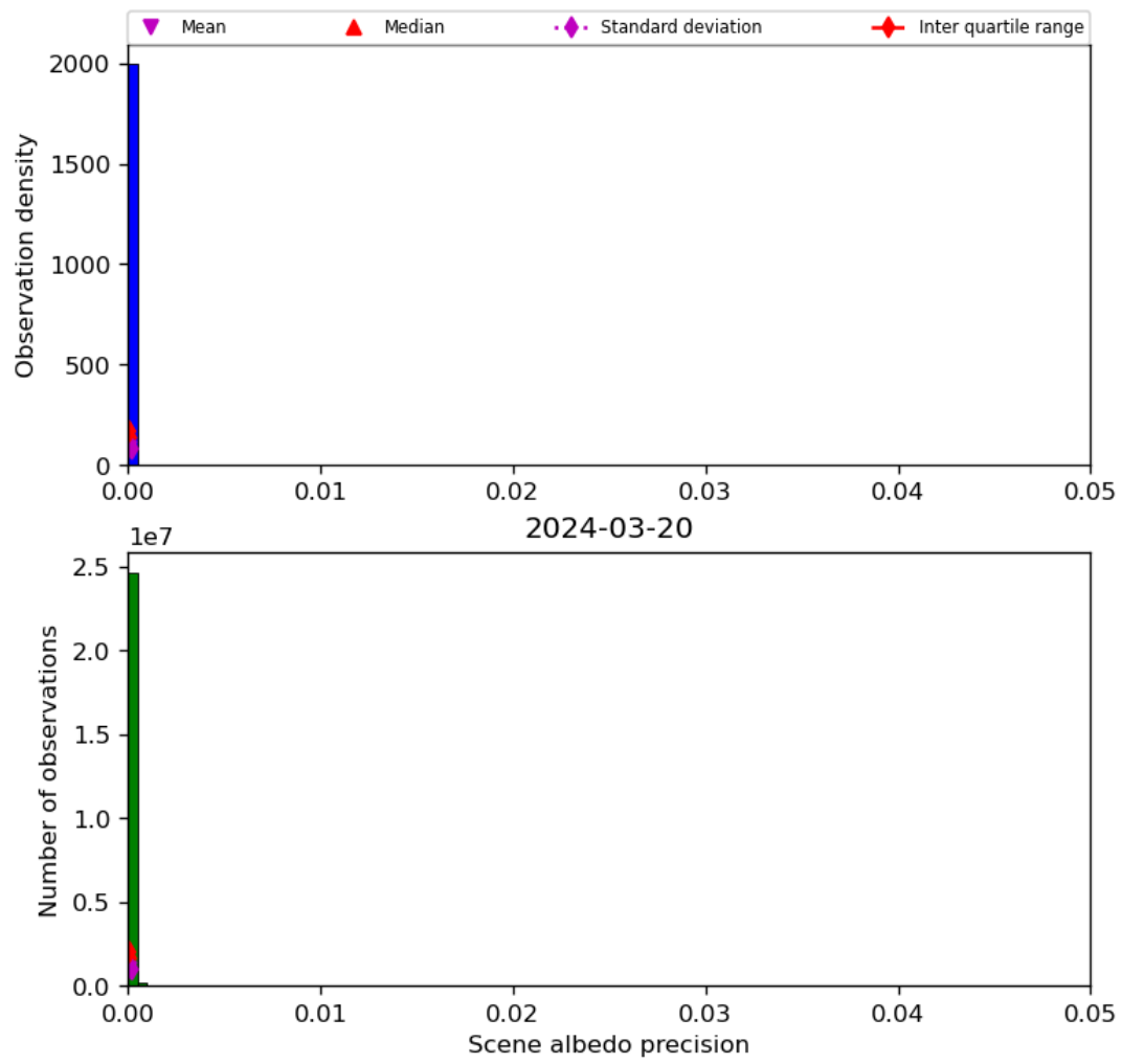
Figure 35: Histogram of “Scene albedo precision” for 2024-03-20 to 2024-03-21
