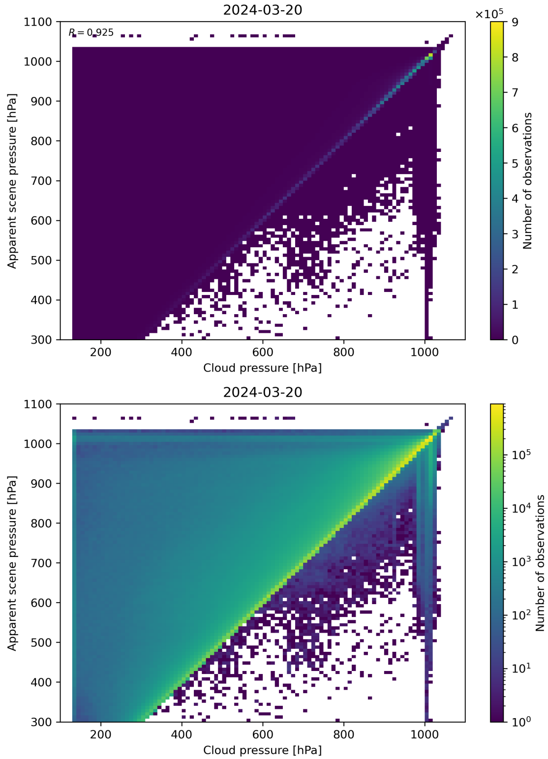
Figure 77: Scatter density plot of “Cloud pressure” against “Apparent scene pressure” for 2024-03-20 to 2024-03-21.
