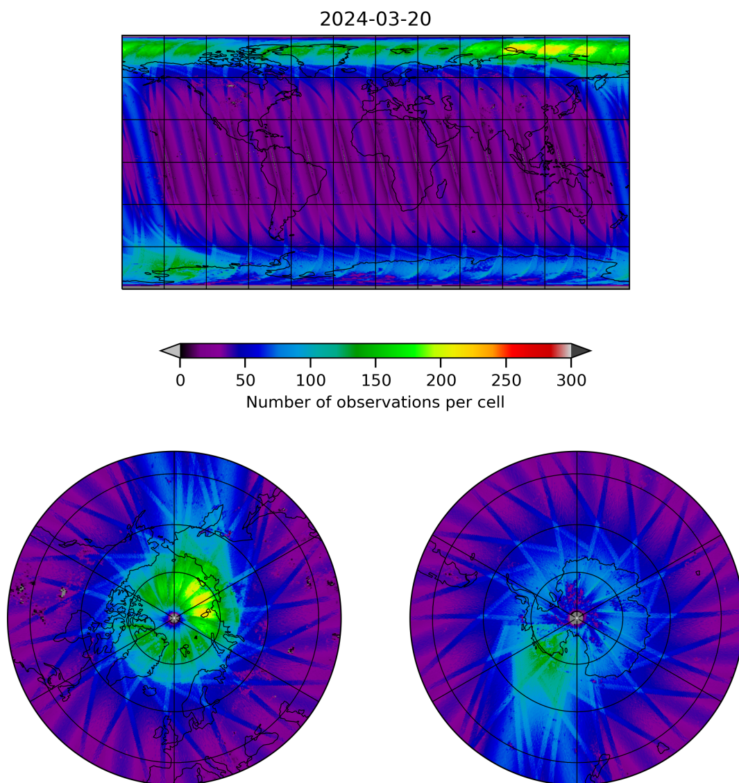
Figure 11: Map of the number of observations for 2024-03-20 to 2024-03-21
