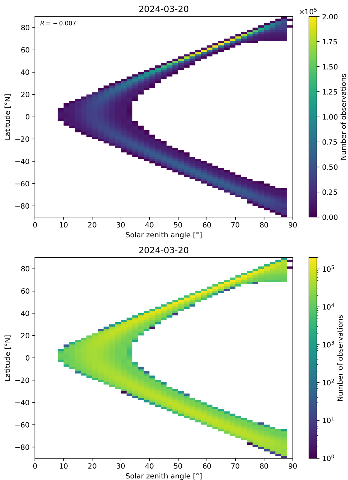
Figure 113: Scatter density plot of “Solar zenith angle” against “Latitude” for 2024-03-20 to 2024-03-21.
