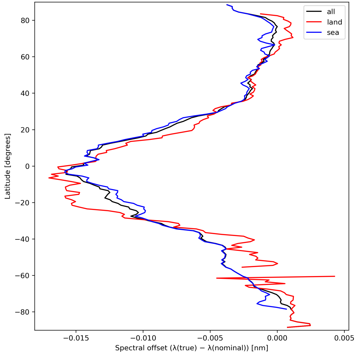
Figure 28: Zonal average of “Spectral offset ( \lambda(\text{true}) - \lambda(\text{nominal}) )” for 2024-03-20 to 2024-03-21.
