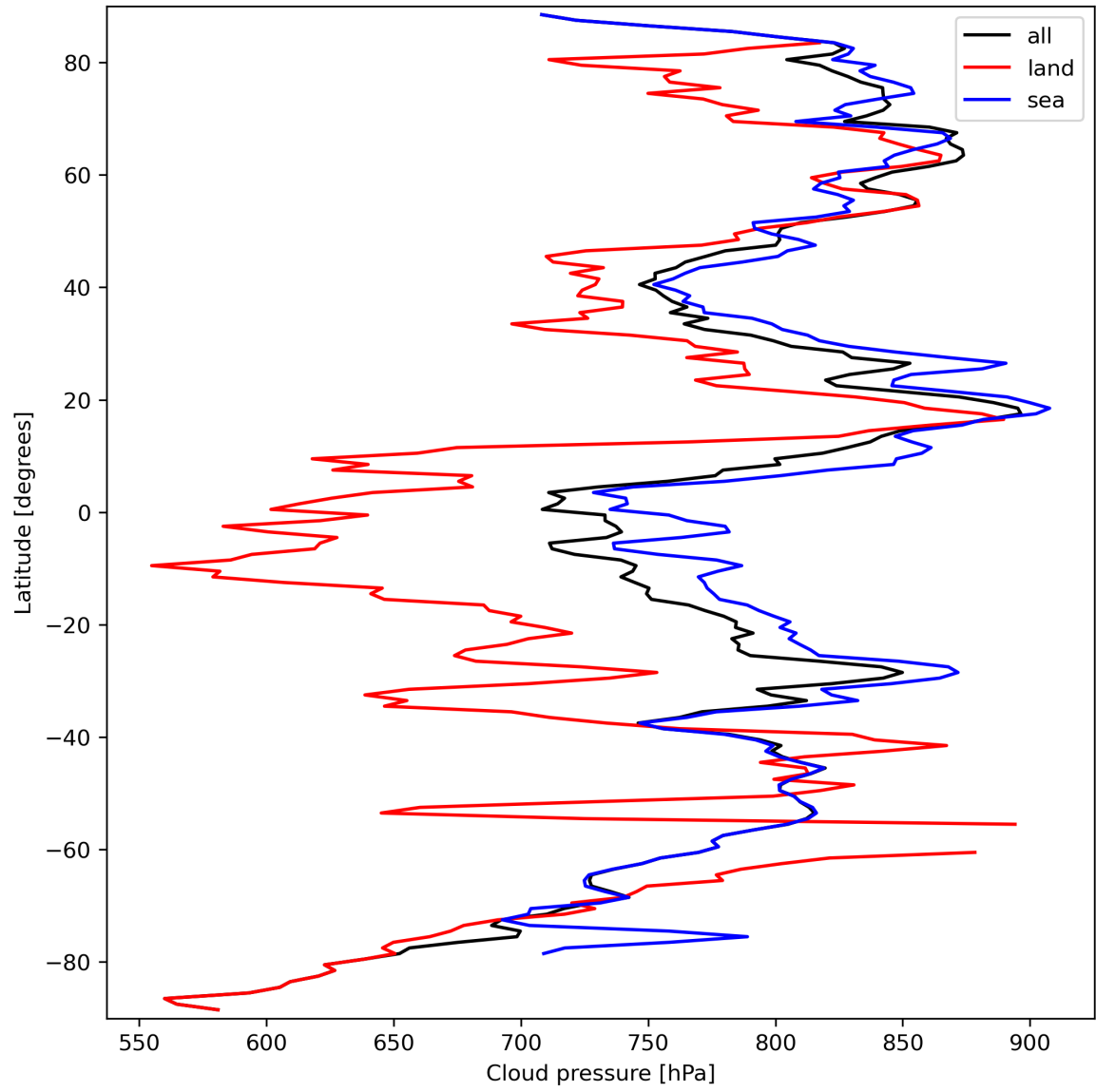
Figure 13: Zonal average of “Cloud pressure” for 2024-03-20 to 2024-03-21.
