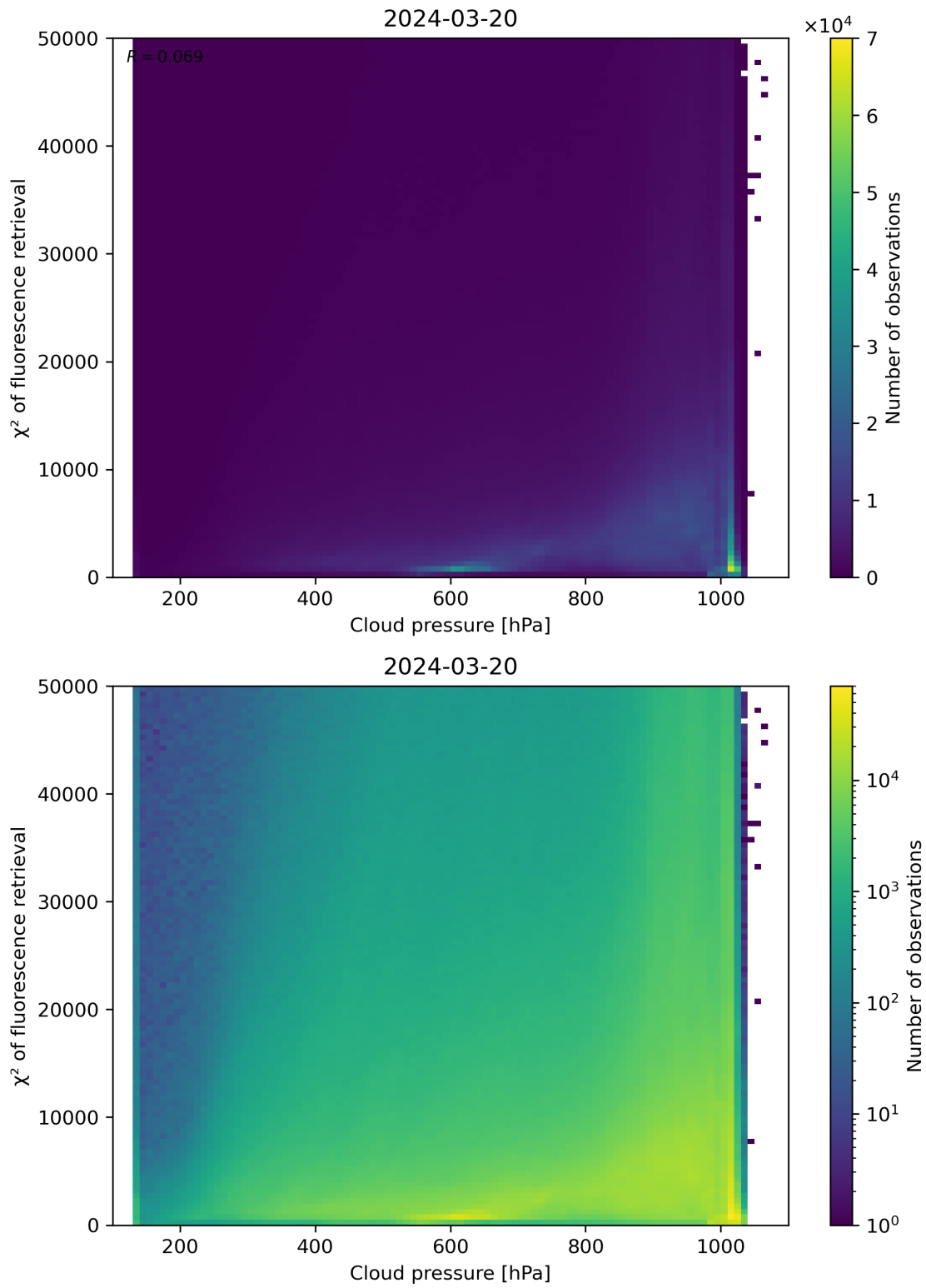
Figure 78: Scatter density plot of “Cloud pressure” against “ \chi^2 of fluorescence retrieval” for 2024-03-20 to 2024-03-21.
