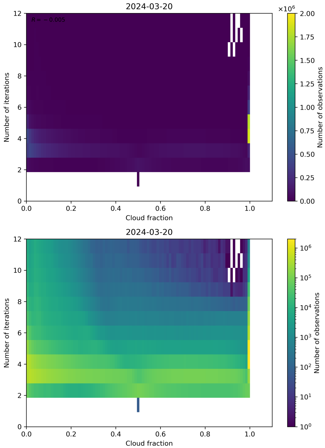
Figure 73: Scatter density plot of “Cloud fraction” against “Number of iterations” for 2024-03-20 to 2024-03-21.
