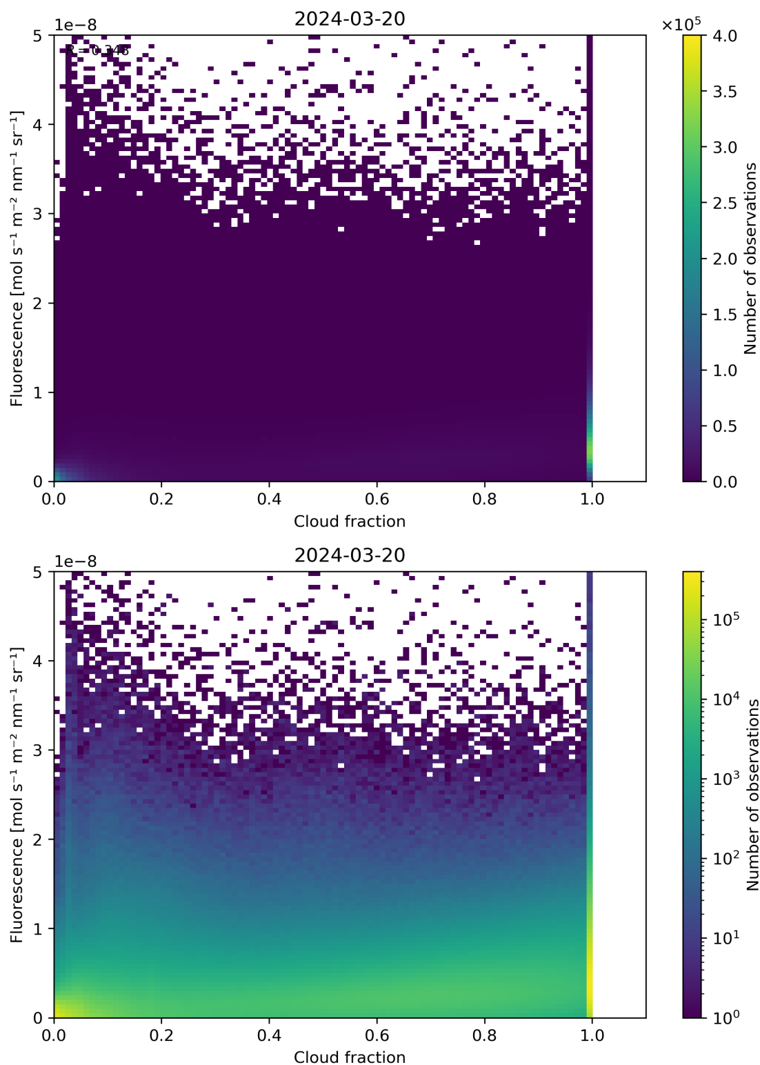
Figure 72: Scatter density plot of “Cloud fraction” against “Fluorescence” for 2024-03-20 to 2024-03-21.
