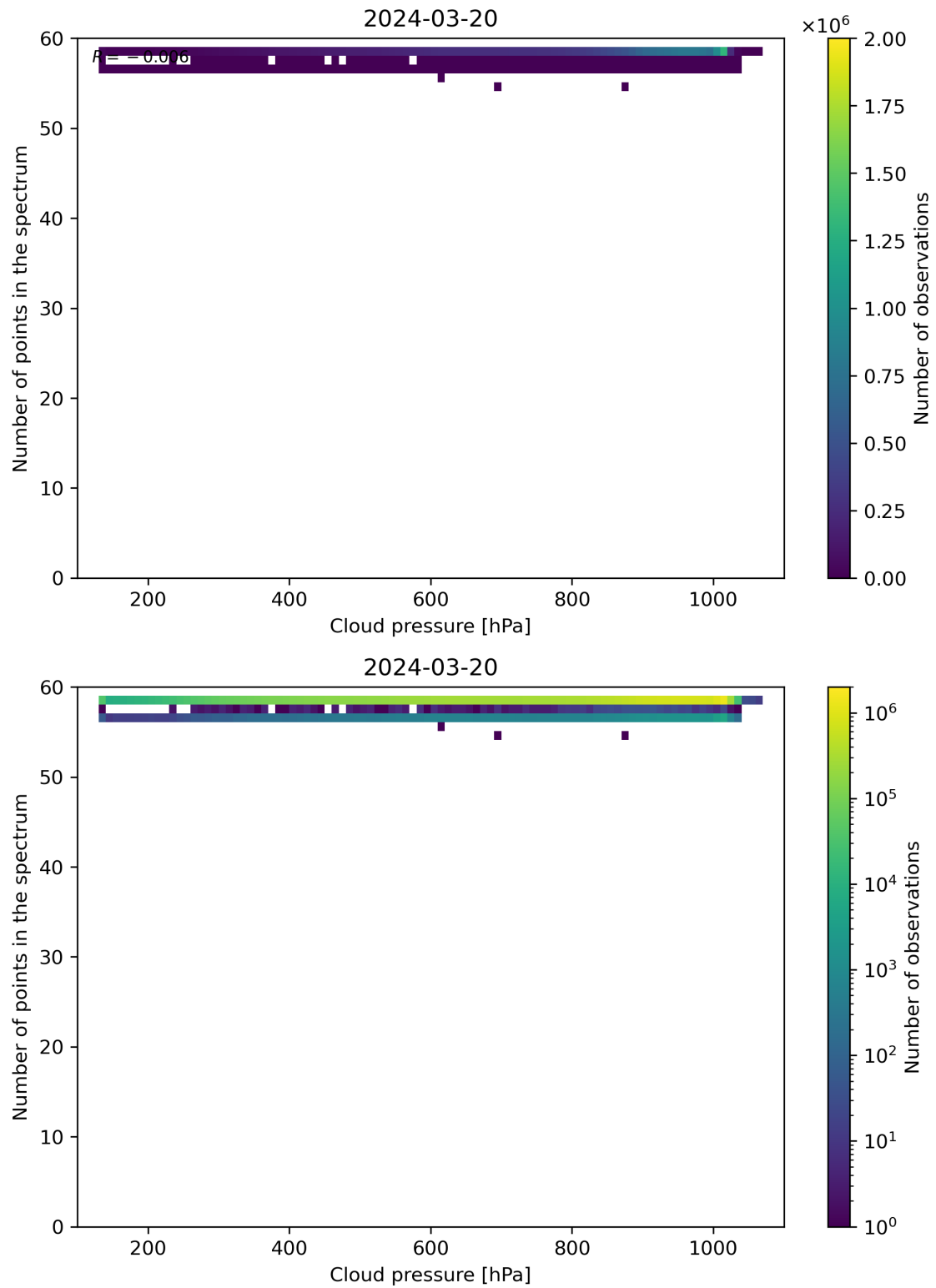
Figure 82: Scatter density plot of “Cloud pressure” against “Number of points in the spectrum” for 2024-03-20 to 2024-03-21.
