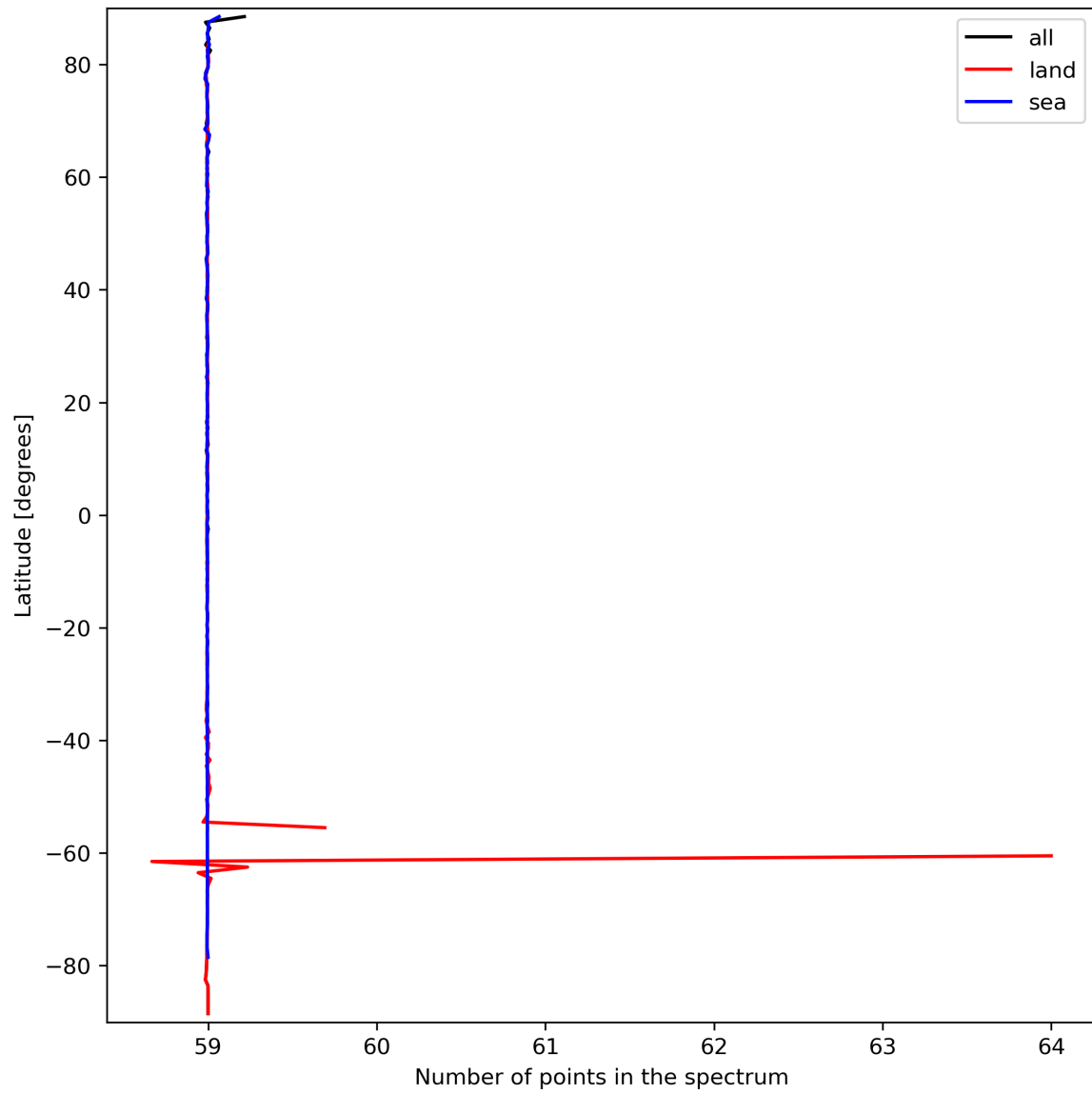
Figure 27: Zonal average of “Number of points in the spectrum” for 2024-03-20 to 2024-03-21.
