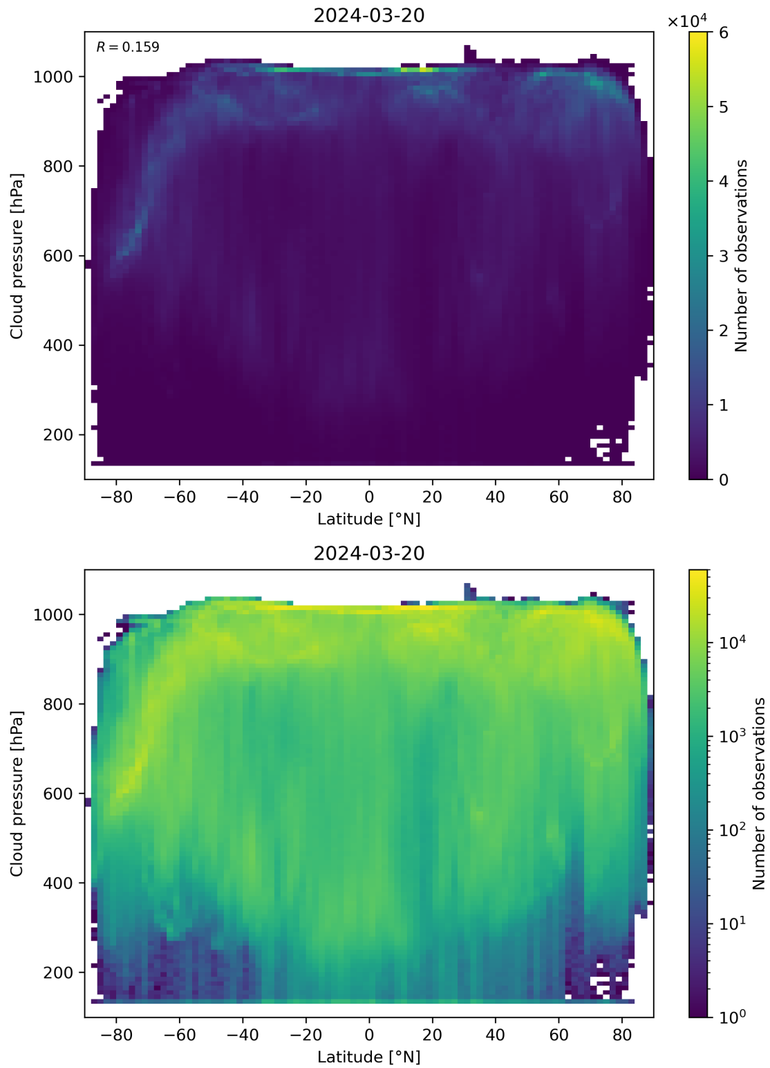
Figure 91: Scatter density plot of “Latitude” against “Cloud pressure” for 2024-03-20 to 2024-03-21.
