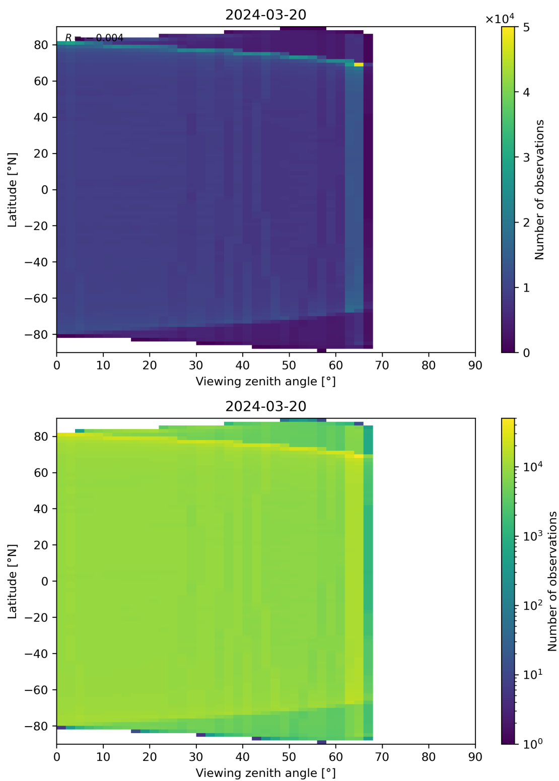
Figure 123: Scatter density plot of “Viewing zenith angle” against “Latitude” for 2024-03-20 to 2024-03-21.
