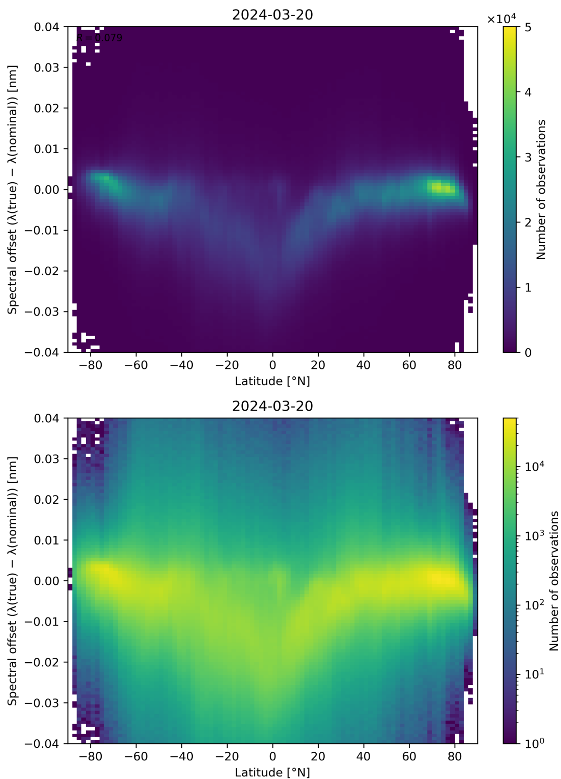
Figure 96: Scatter density plot of “Latitude” against “Spectral offset ( \lambda(\text{true}) - \lambda(\text{nominal}) )” for 2024-03-20 to 2024-03-21.
