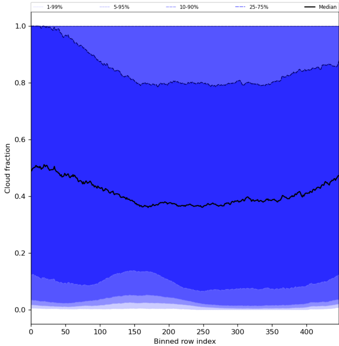
Figure 49: Along track statistics of “Cloud fraction” for 2024-03-20 to 2024-03-21
