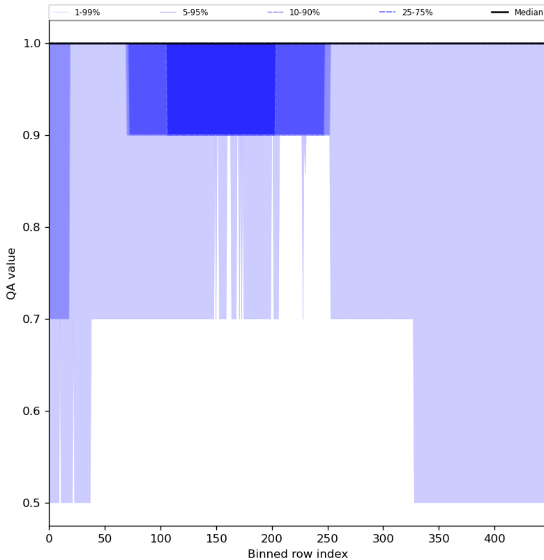
Figure 46: Along track statistics of “QA value” for 2024-03-20 to 2024-03-21
