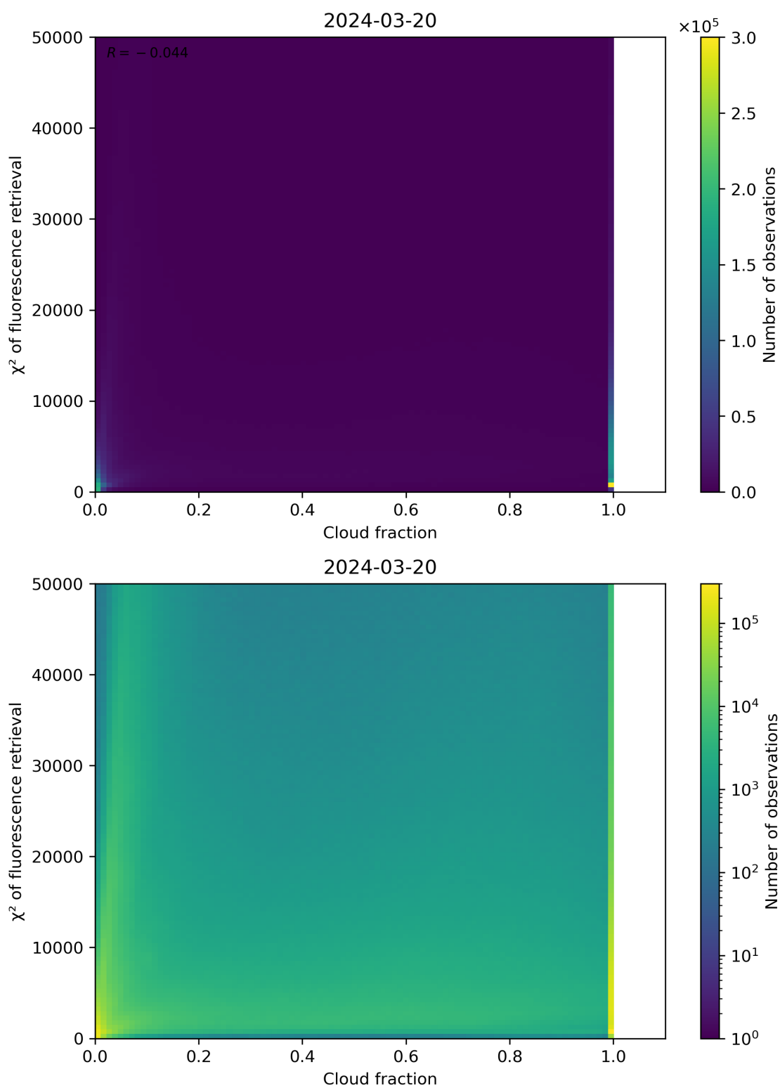
Figure 71: Scatter density plot of “Cloud fraction” against “ \chi^2 of fluorescence retrieval” for 2024-03-20 to 2024-03-21.
