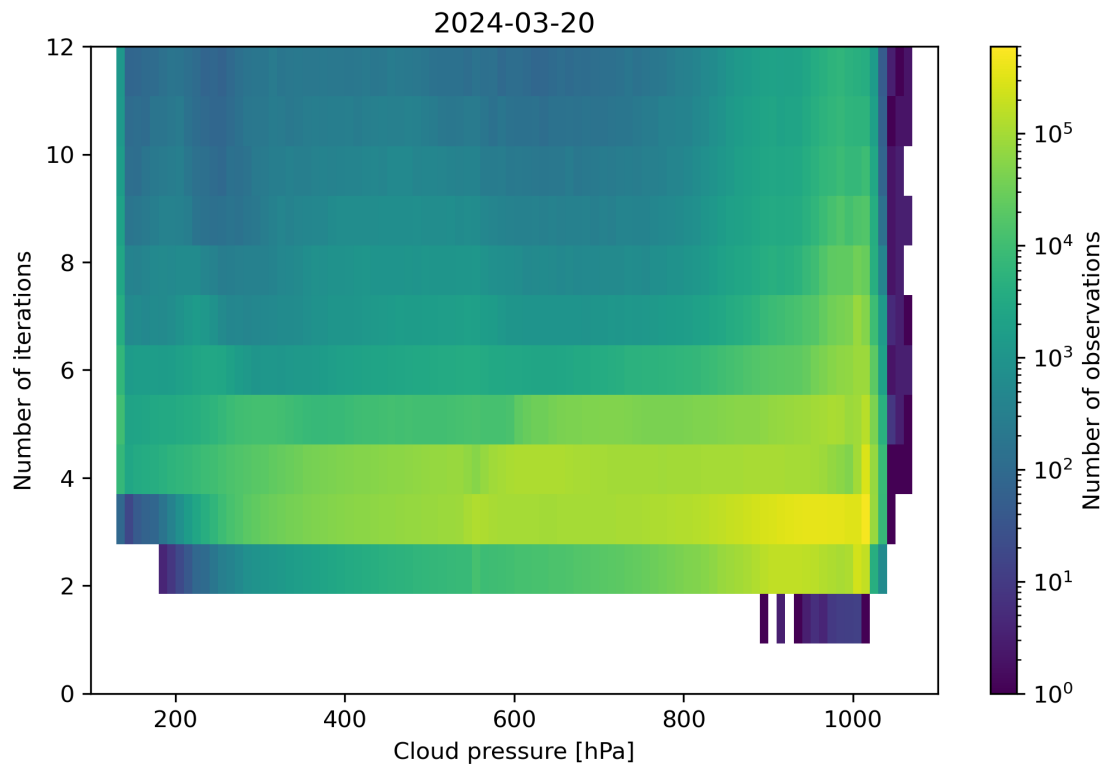
Figure 81: Scatter density plot of “Cloud pressure” against “Number of iterations” for 2024-03-20 to 2024-03-21.
