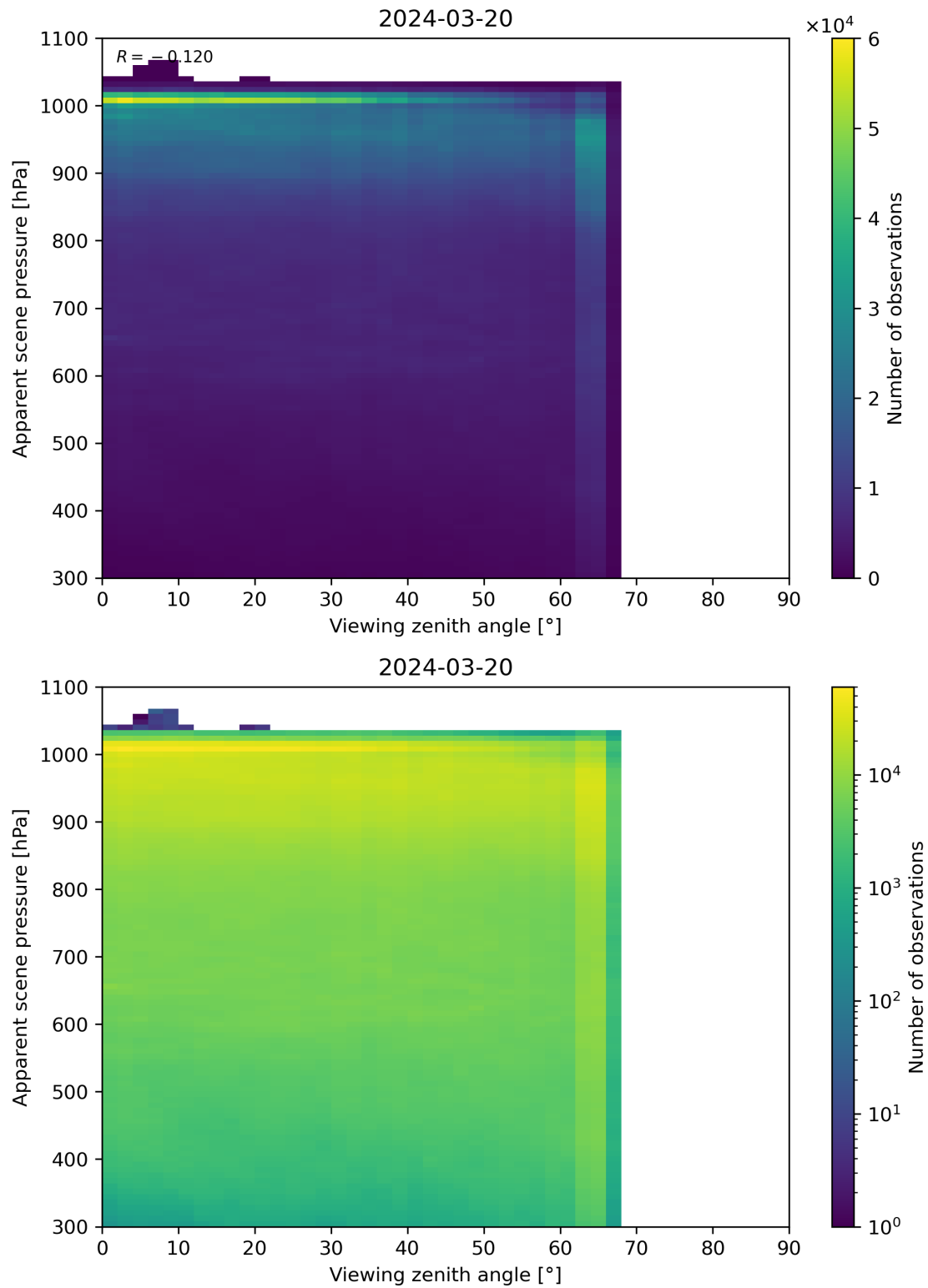
Figure 118: Scatter density plot of “Viewing zenith angle” against “Apparent scene pressure” for 2024-03-20 to 2024-03-21.
