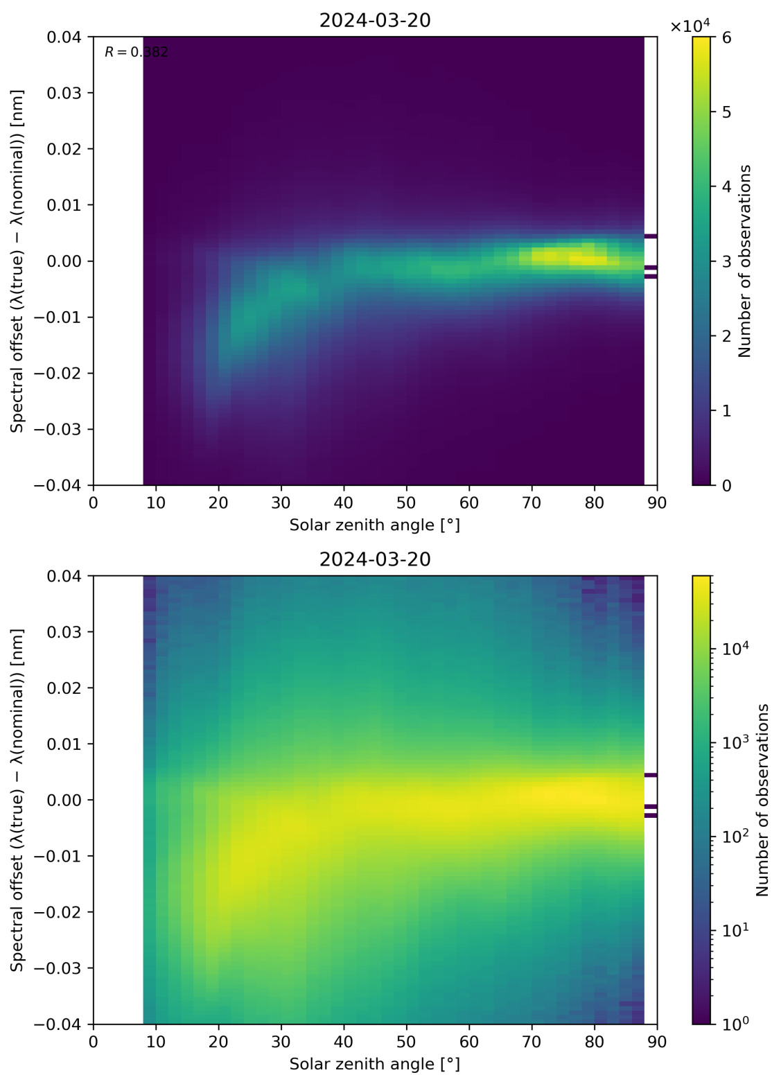
Figure 117: Scatter density plot of “Solar zenith angle” against “Spectral offset ( \lambda(\text{true}) - \lambda(\text{nominal}) )” for 2024-03-20 to 2024-03-21.
