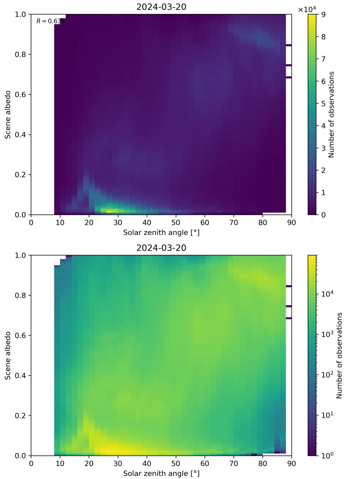
Figure 116: Scatter density plot of “Solar zenith angle” against “Scene albedo” for 2024-03-20 to 2024-03-21.
