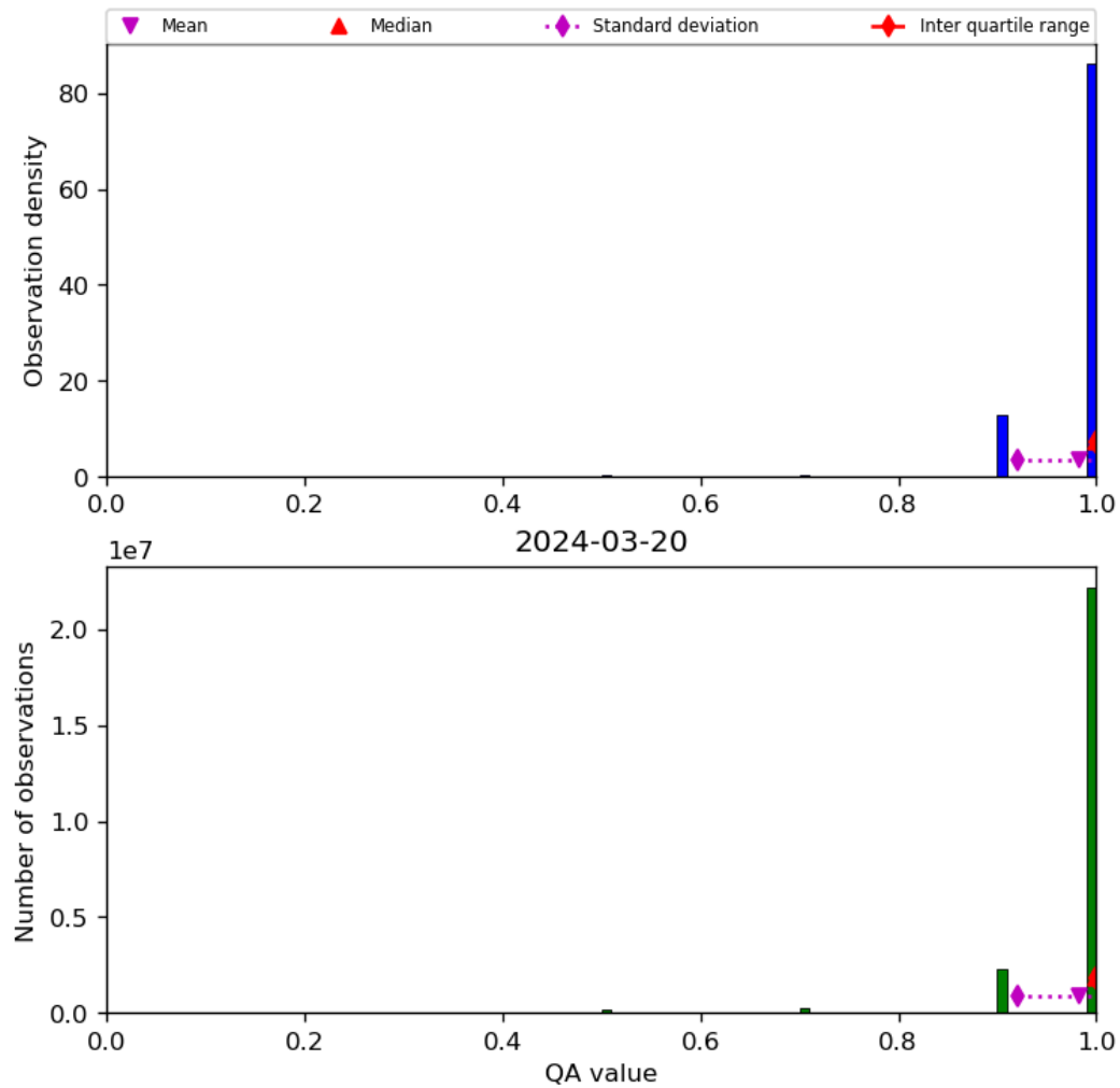
Figure 29: Histogram of “QA value” for 2024-03-20 to 2024-03-21
