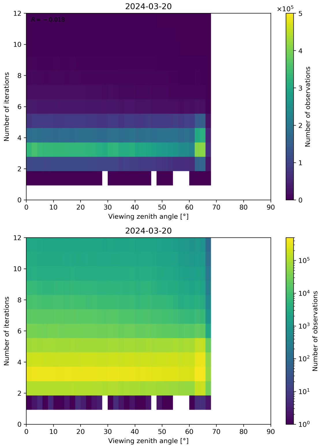
Figure 124: Scatter density plot of “Viewing zenith angle” against “Number of iterations” for 2024-03-20 to 2024-03-21.
