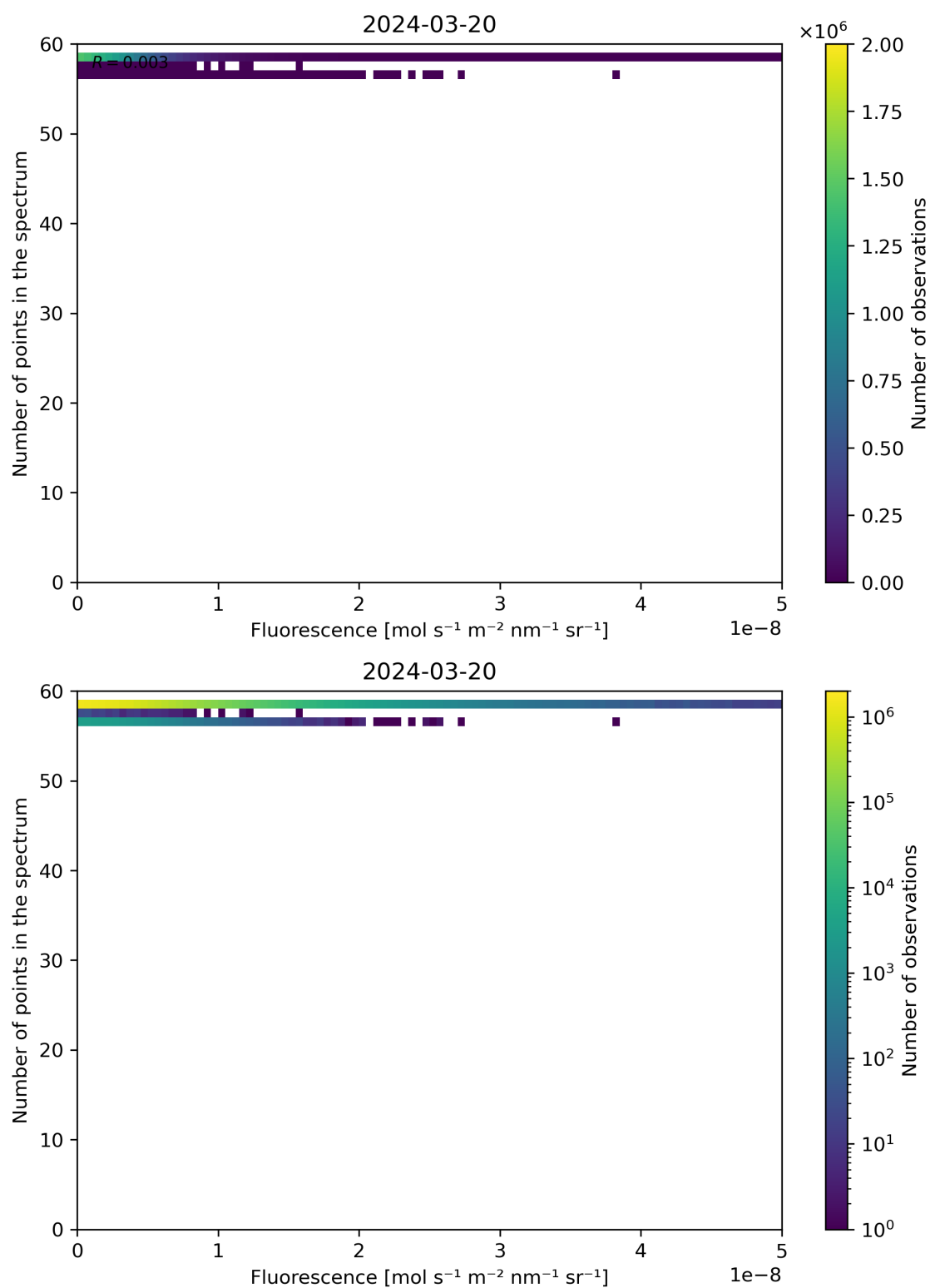
Figure 86: Scatter density plot of “Fluorescence” against “Number of points in the spectrum” for 2024-03-20 to 2024-03-21.
