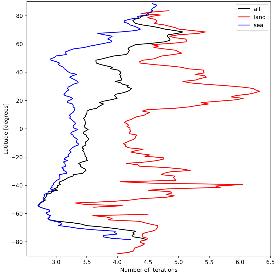
Figure 22: Zonal average of “Number of iterations” for 2024-03-20 to 2024-03-21.
