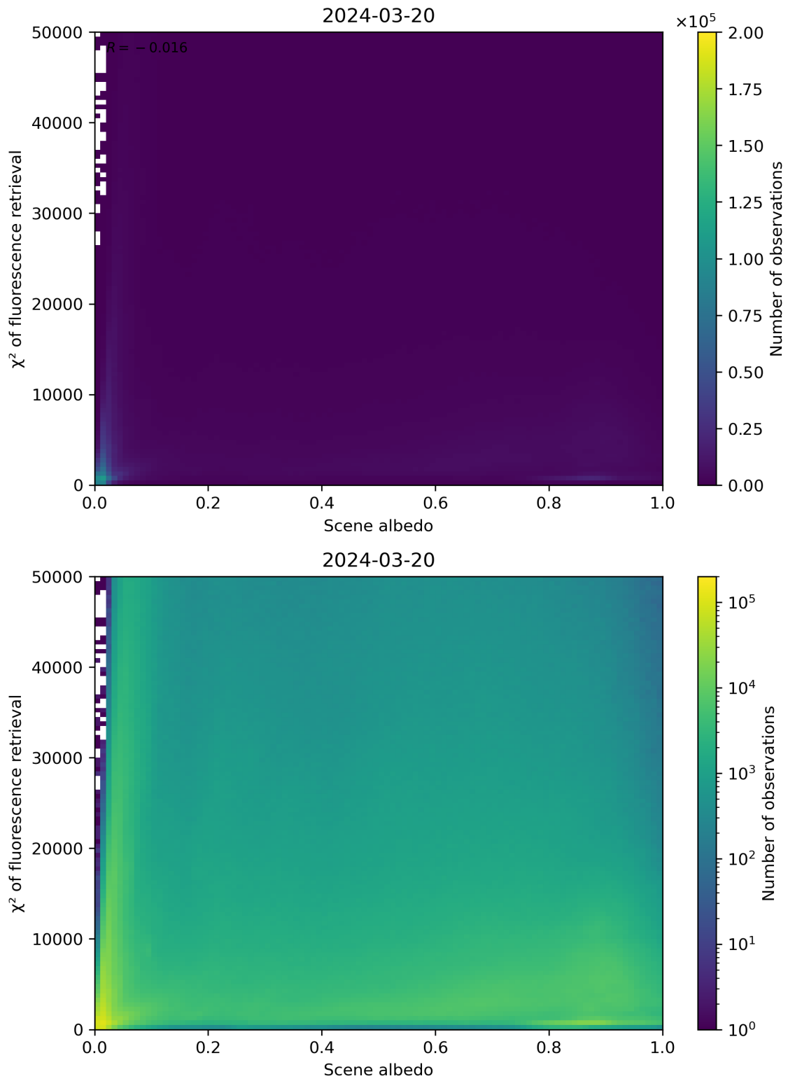
Figure 103: Scatter density plot of “Scene albedo” against “ \chi^2 of fluorescence retrieval” for 2024-03-20 to 2024-03-21.
