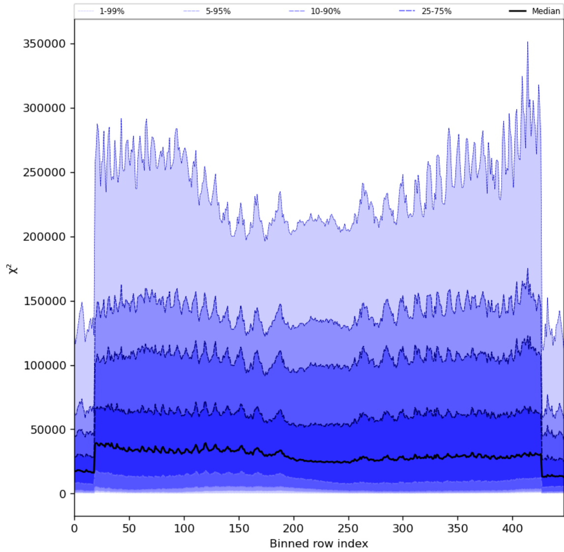
Figure 55: Along track statistics of “ \chi^2 ” for 2024-03-20 to 2024-03-21
