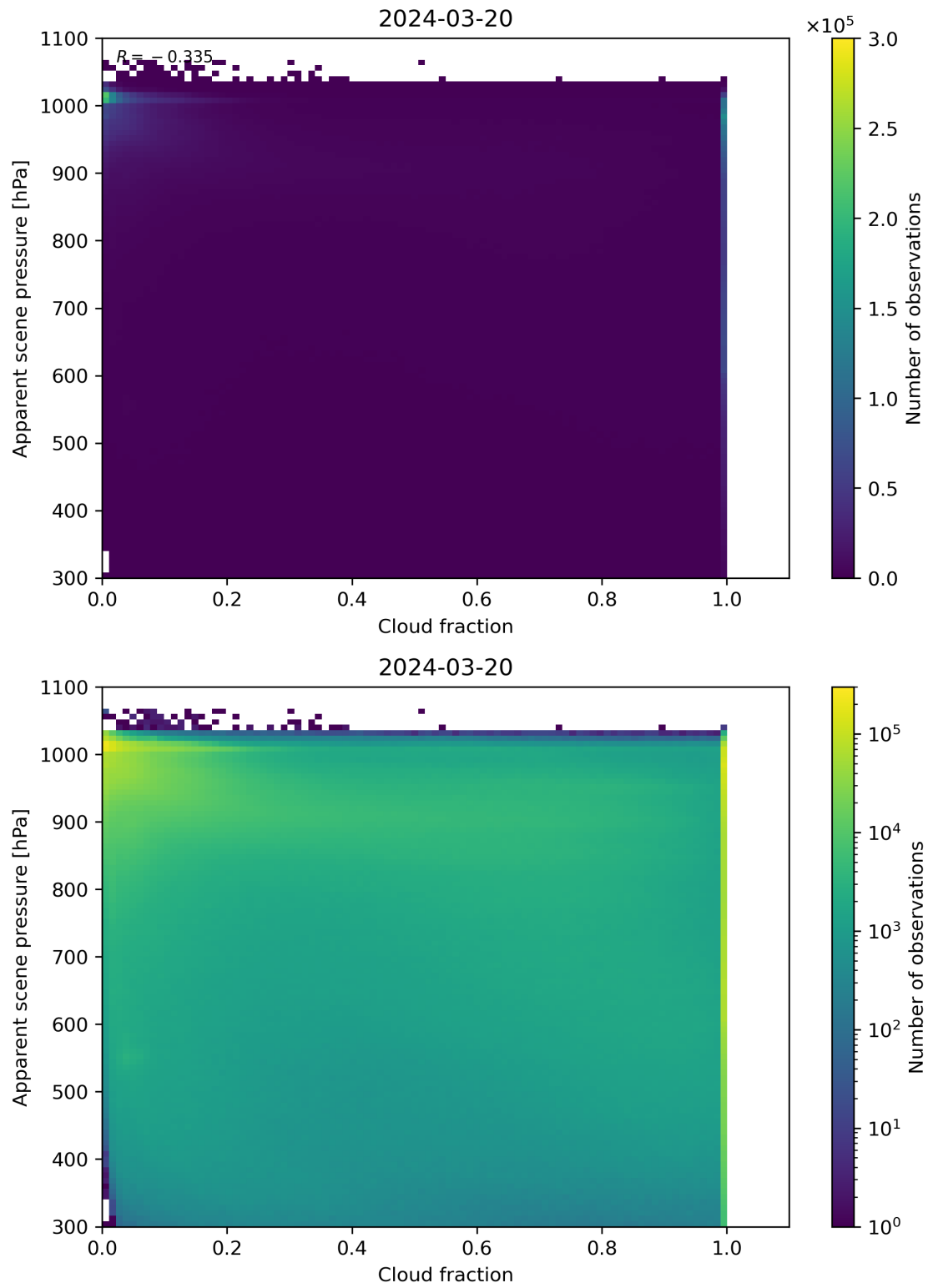
Figure 70: Scatter density plot of “Cloud fraction” against “Apparent scene pressure” for 2024-03-20 to 2024-03-21.
