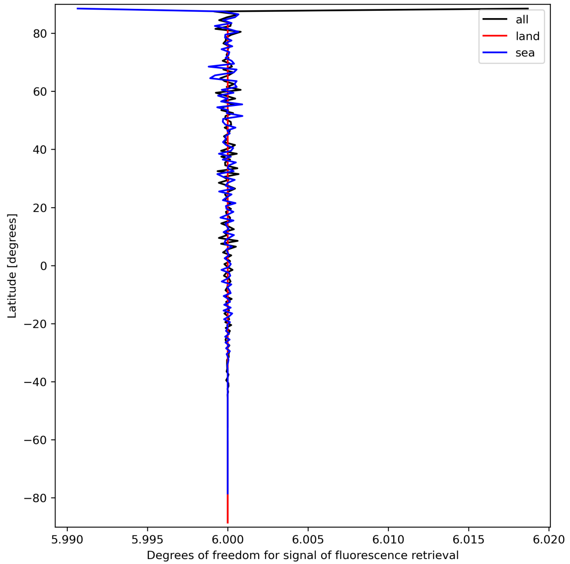
Figure 26: Zonal average of “Degrees of freedom for signal of fluorescence retrieval” for 2024-03-20 to 2024-03-21.
