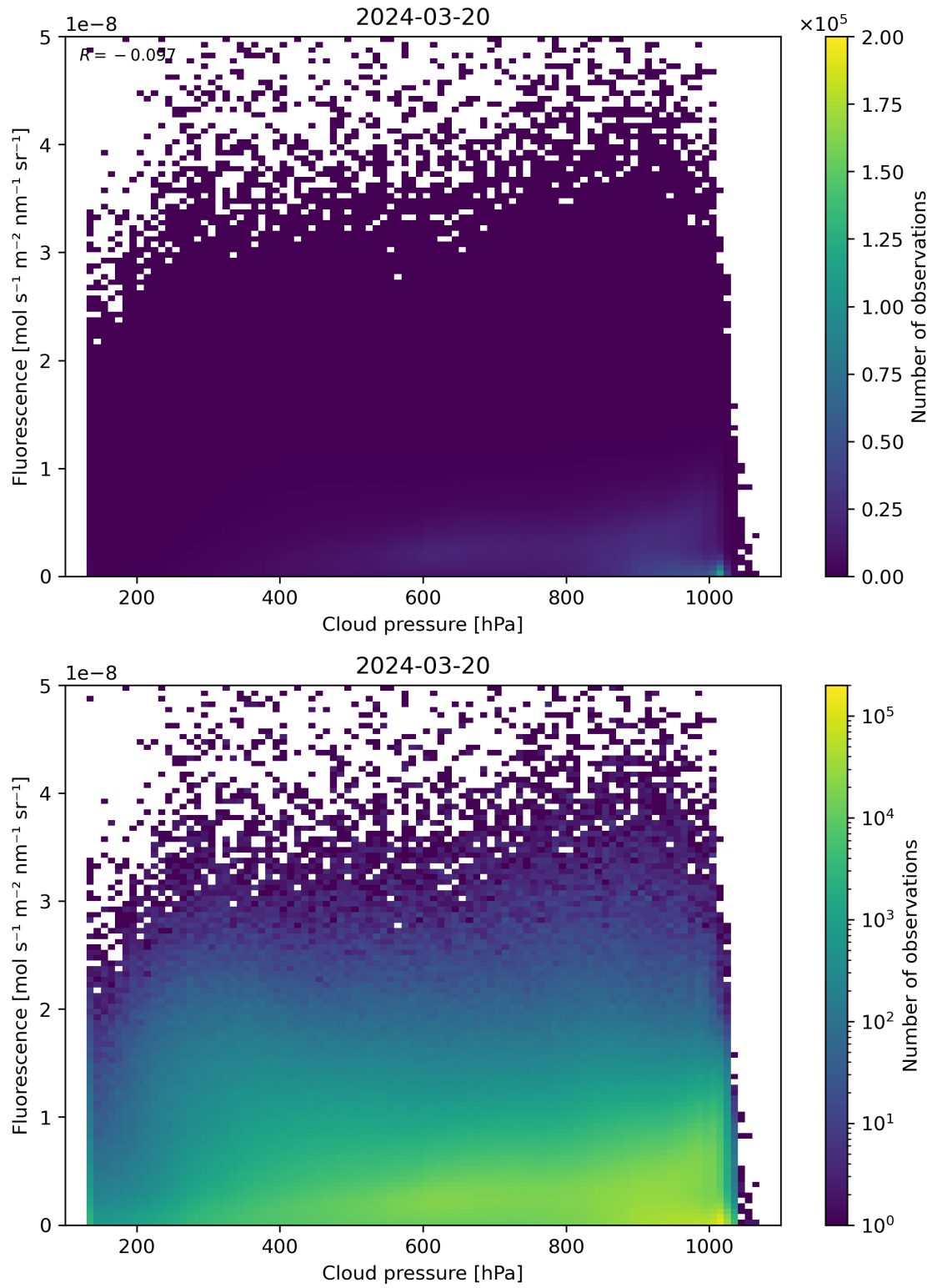
Figure 80: Scatter density plot of “Cloud pressure” against “Fluorescence” for 2024-03-20 to 2024-03-21.
