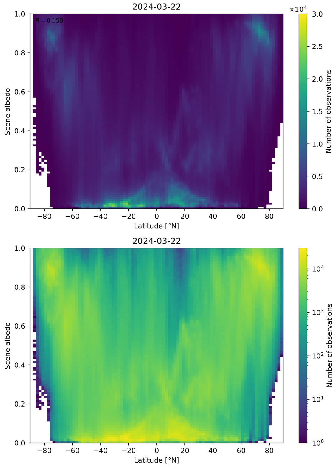
Figure 95: Scatter density plot of “Latitude” against “Scene albedo” for 2024-03-21 to 2024-03-22.
