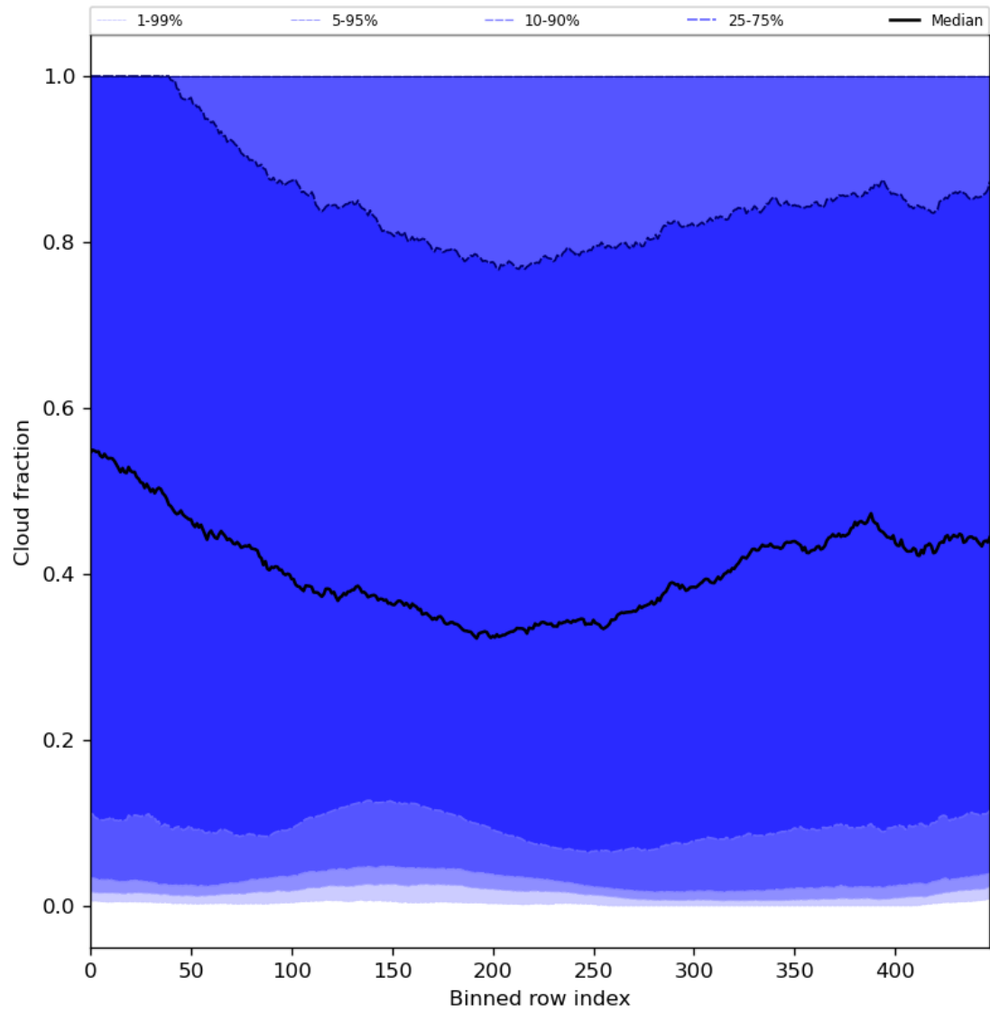
Figure 49: Along track statistics of “Cloud fraction” for 2024-03-21 to 2024-03-22
