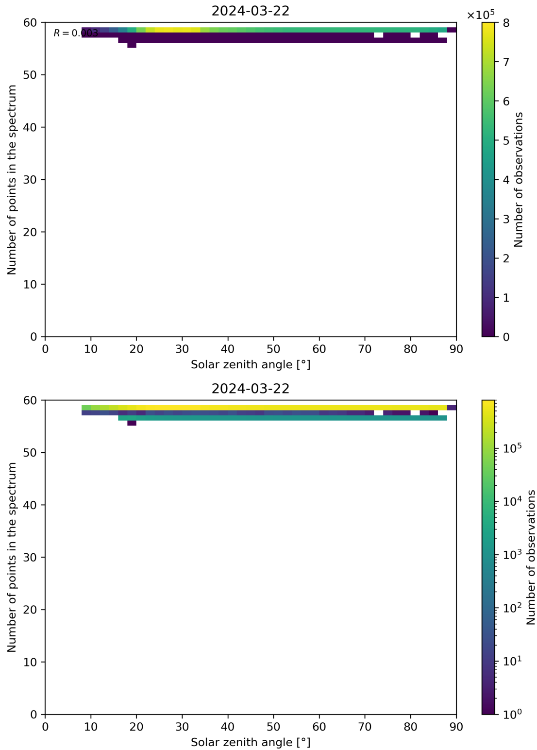
Figure 115: Scatter density plot of “Solar zenith angle” against “Number of points in the spectrum” for 2024-03-21 to 2024-03-22.
