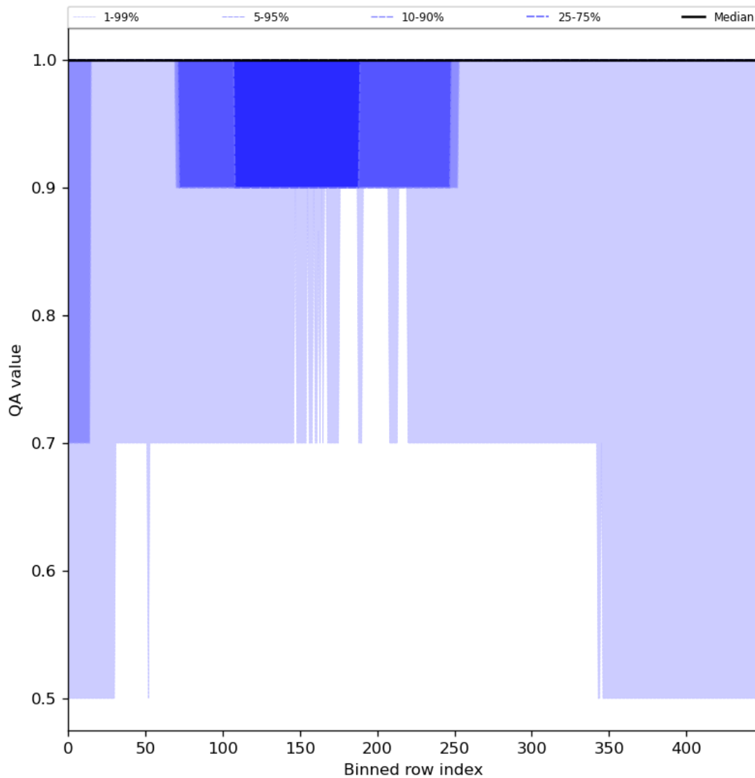
Figure 46: Along track statistics of “QA value” for 2024-03-21 to 2024-03-22
