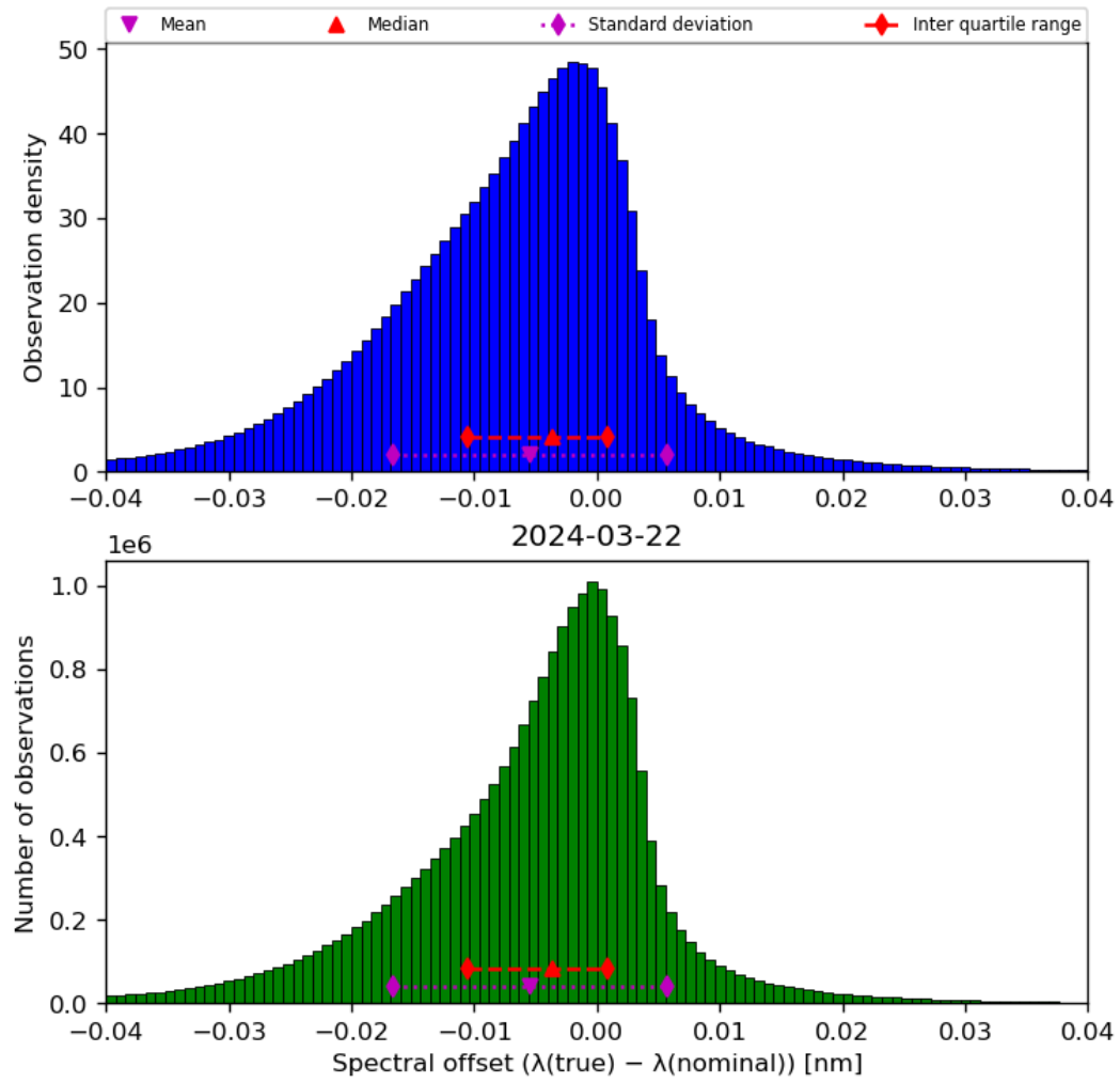
Figure 45: Histogram of “Spectral offset ( \lambda(\text{true}) - \lambda(\text{nominal}) )” for 2024-03-21 to 2024-03-22
