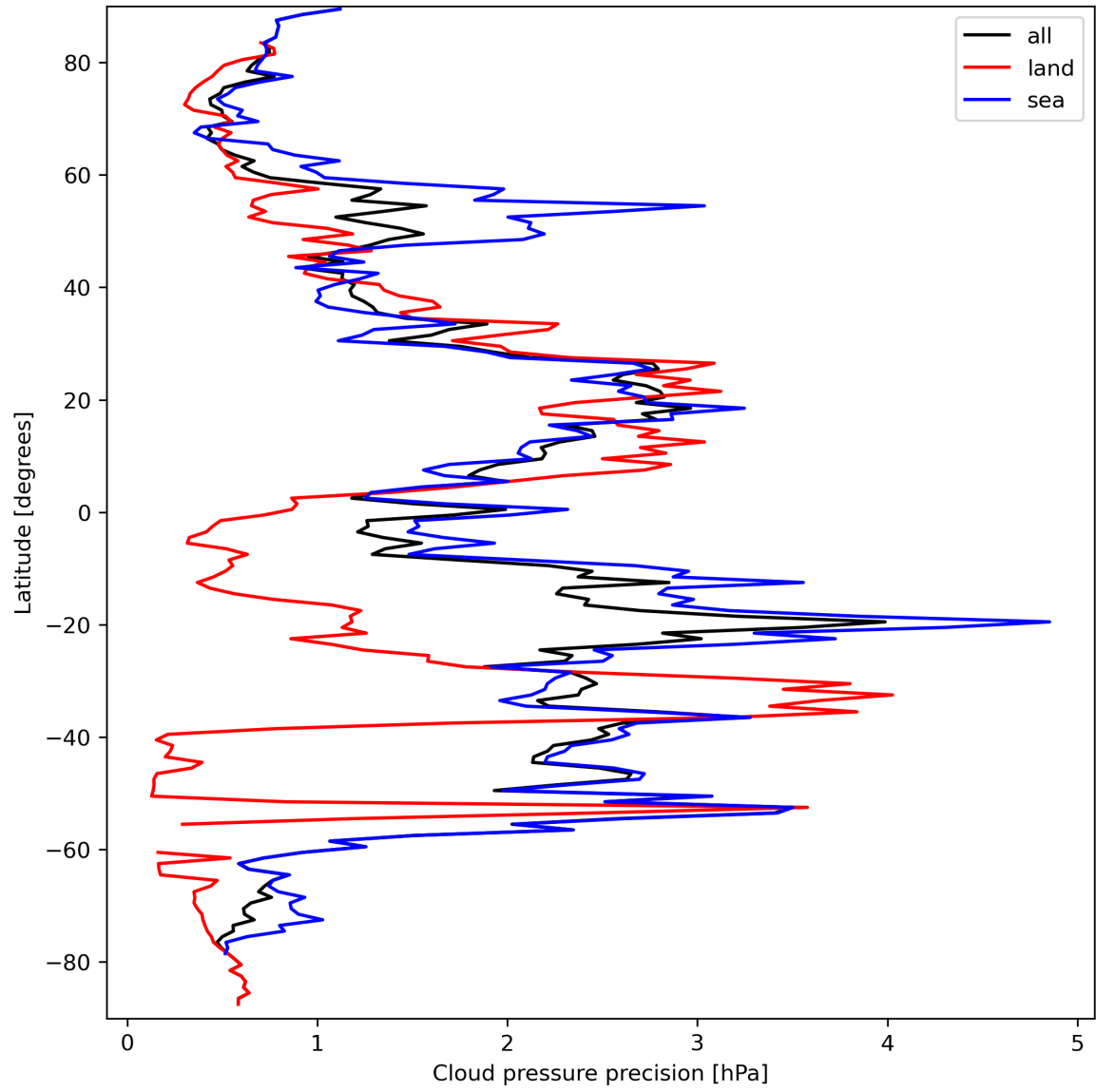
Figure 14: Zonal average of “Cloud pressure precision” for 2024-03-21 to 2024-03-22.
