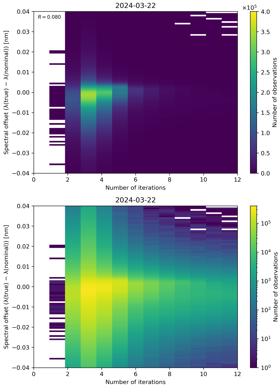
Figure 100: Scatter density plot of “Number of iterations” against “Spectral offset ( \lambda(\text{true}) - \lambda(\text{nominal}) )” for 2024-03-21 to 2024-03-22.
