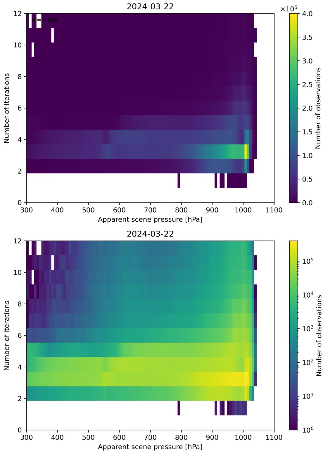
Figure 65: Scatter density plot of “Apparent scene pressure” against “Number of iterations” for 2024-03-21 to 2024-03-22.
