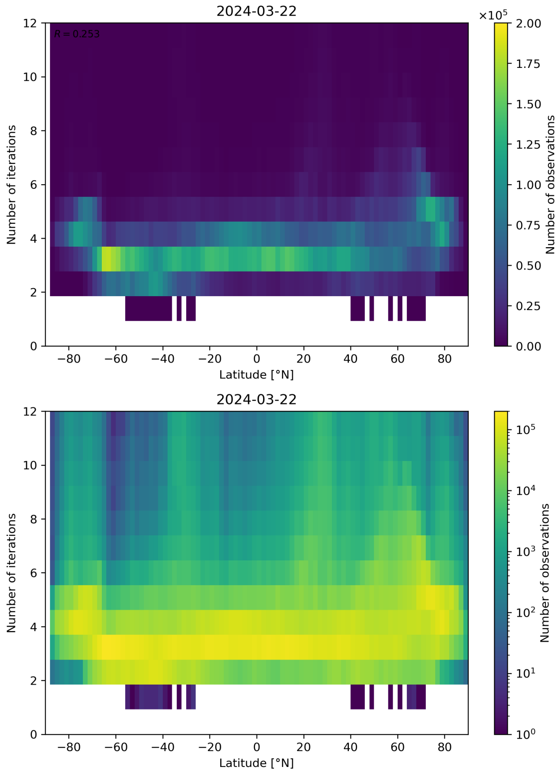
Figure 93: Scatter density plot of “Latitude” against “Number of iterations” for 2024-03-21 to 2024-03-22.
