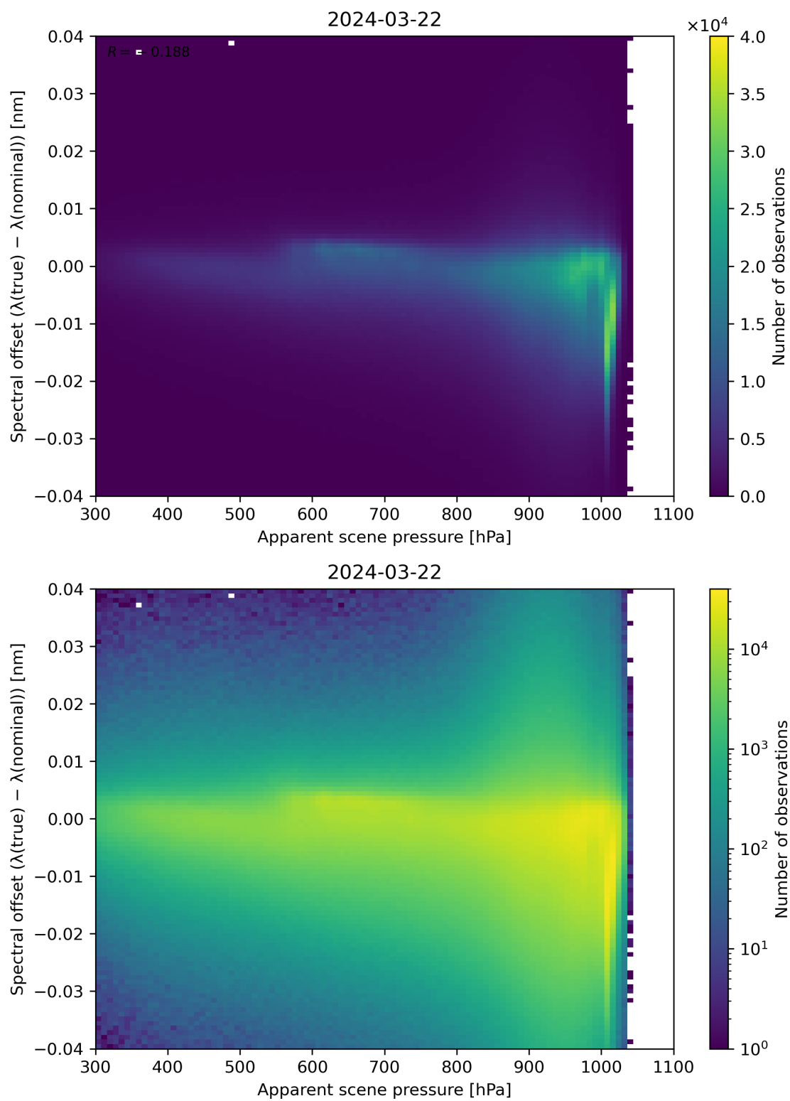
Figure 67: Scatter density plot of “Apparent scene pressure” against “Spectral offset ( \lambda(\text{true}) - \lambda(\text{nominal}) )” for 2024-03-21 to 2024-03-22.
