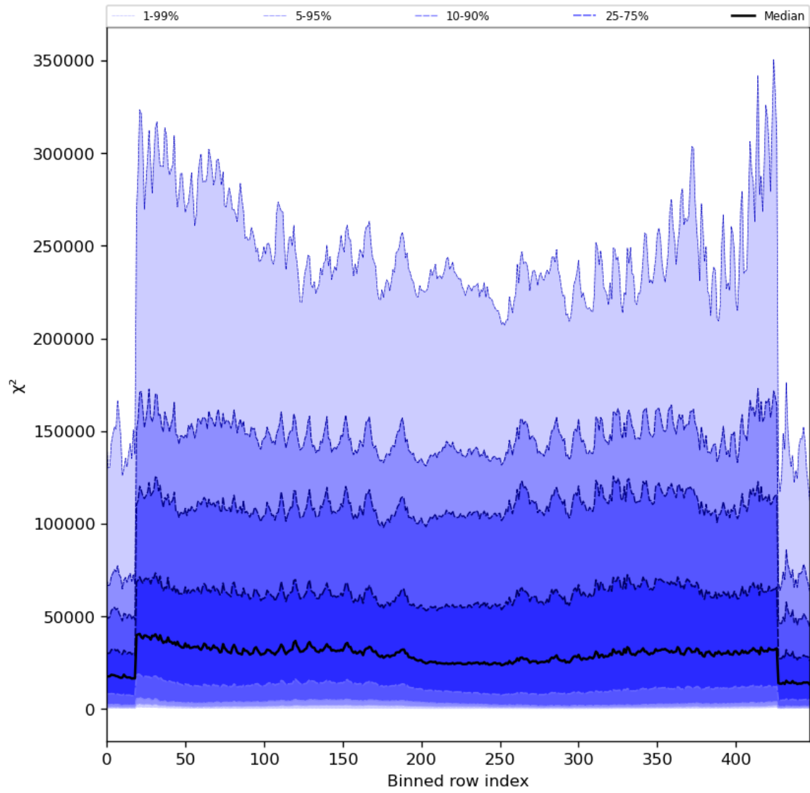
Figure 55: Along track statistics of “ \chi^2 ” for 2024-03-21 to 2024-03-22
