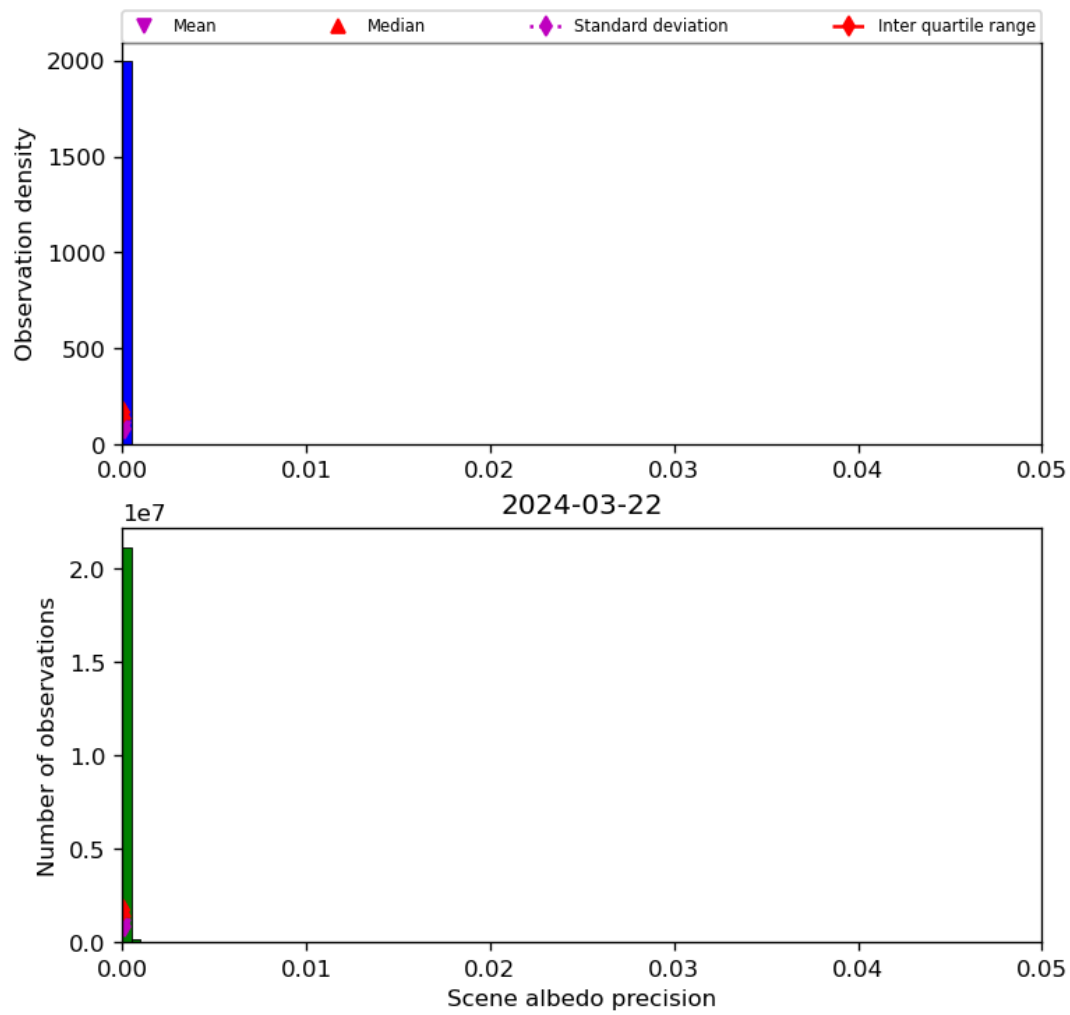
Figure 35: Histogram of “Scene albedo precision” for 2024-03-21 to 2024-03-22
