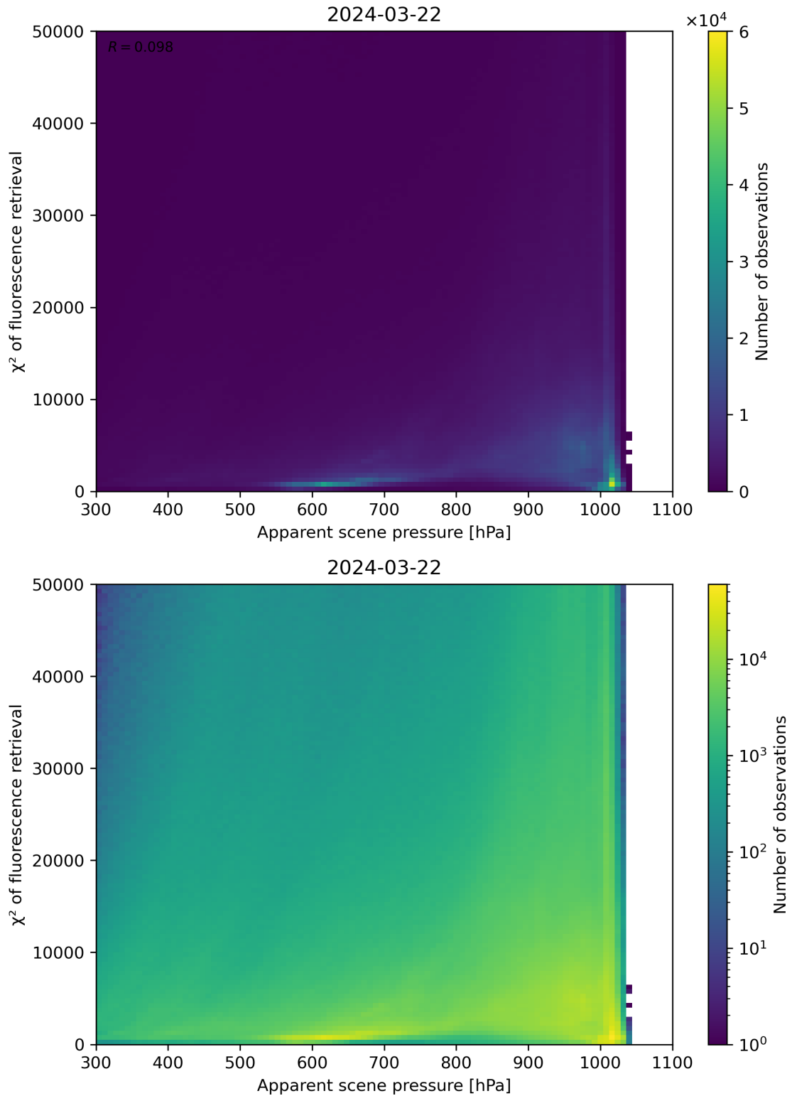
Figure 63: Scatter density plot of “Apparent scene pressure” against “ \chi^2 of fluorescence retrieval” for 2024-03-21 to 2024-03-22.
