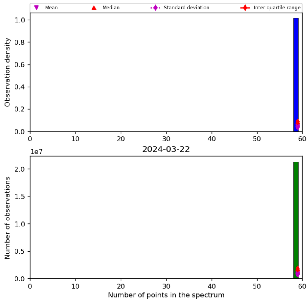
Figure 44: Histogram of “Number of points in the spectrum” for 2024-03-21 to 2024-03-22
