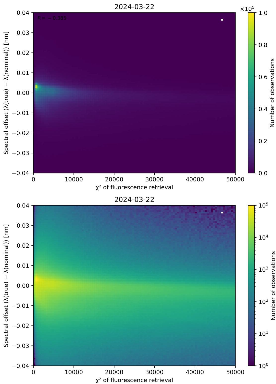
Figure 69: Scatter density plot of " \chi^2 of fluorescence retrieval" against "Spectral offset ( \lambda(\text{true}) - \lambda(\text{nominal})) " for 2024-03-21 to 2024-03-22.
