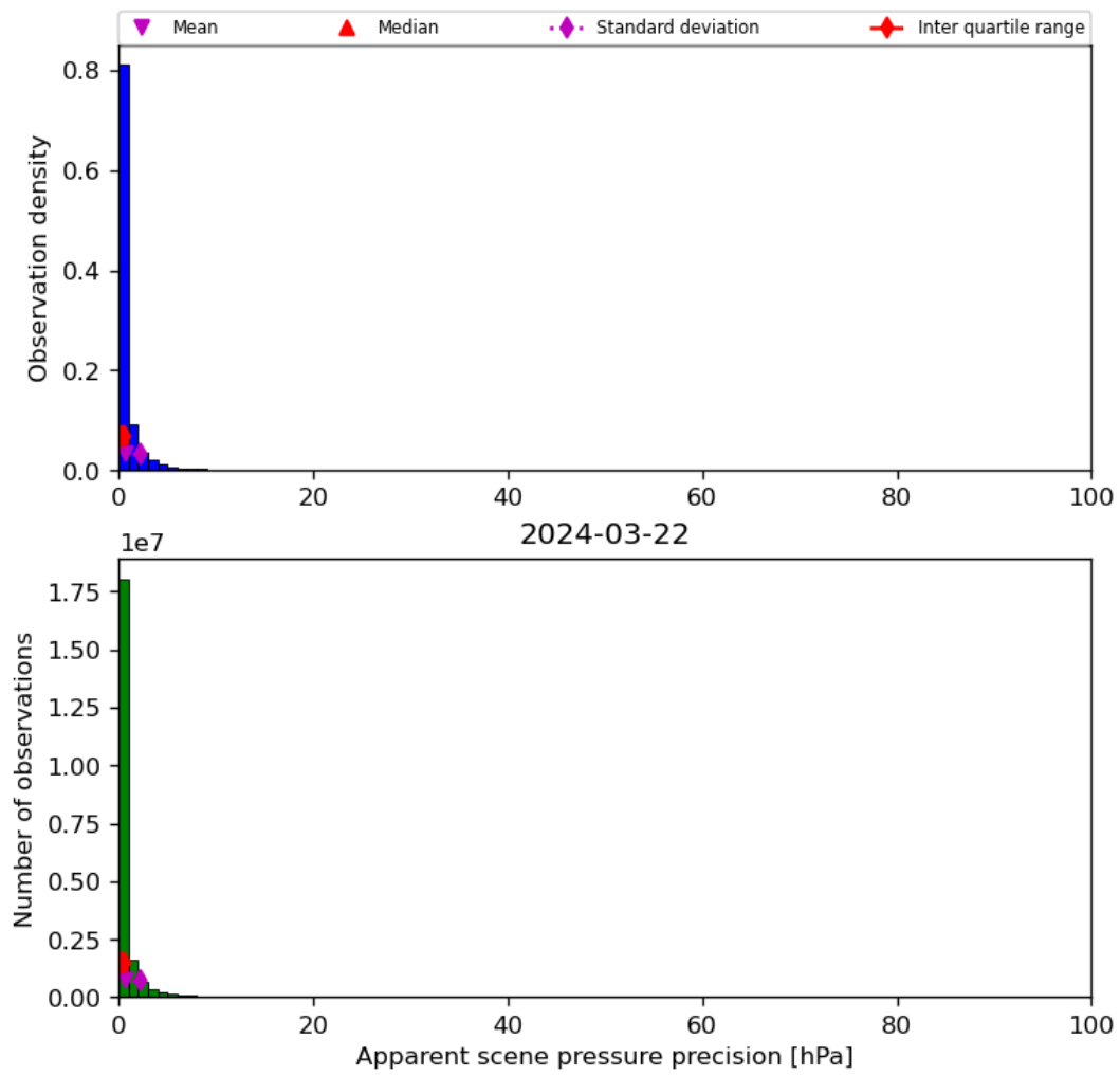
Figure 37: Histogram of “Apparent scene pressure precision” for 2024-03-21 to 2024-03-22
