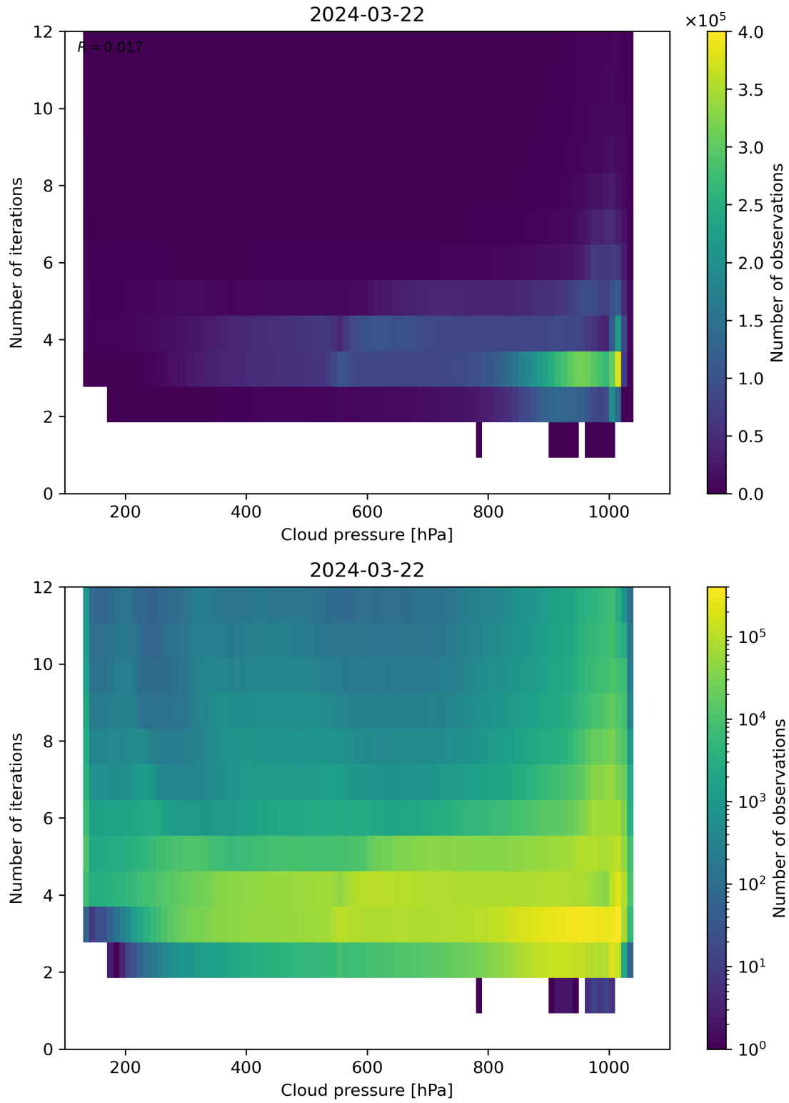
Figure 81: Scatter density plot of “Cloud pressure” against “Number of iterations” for 2024-03-21 to 2024-03-22.
