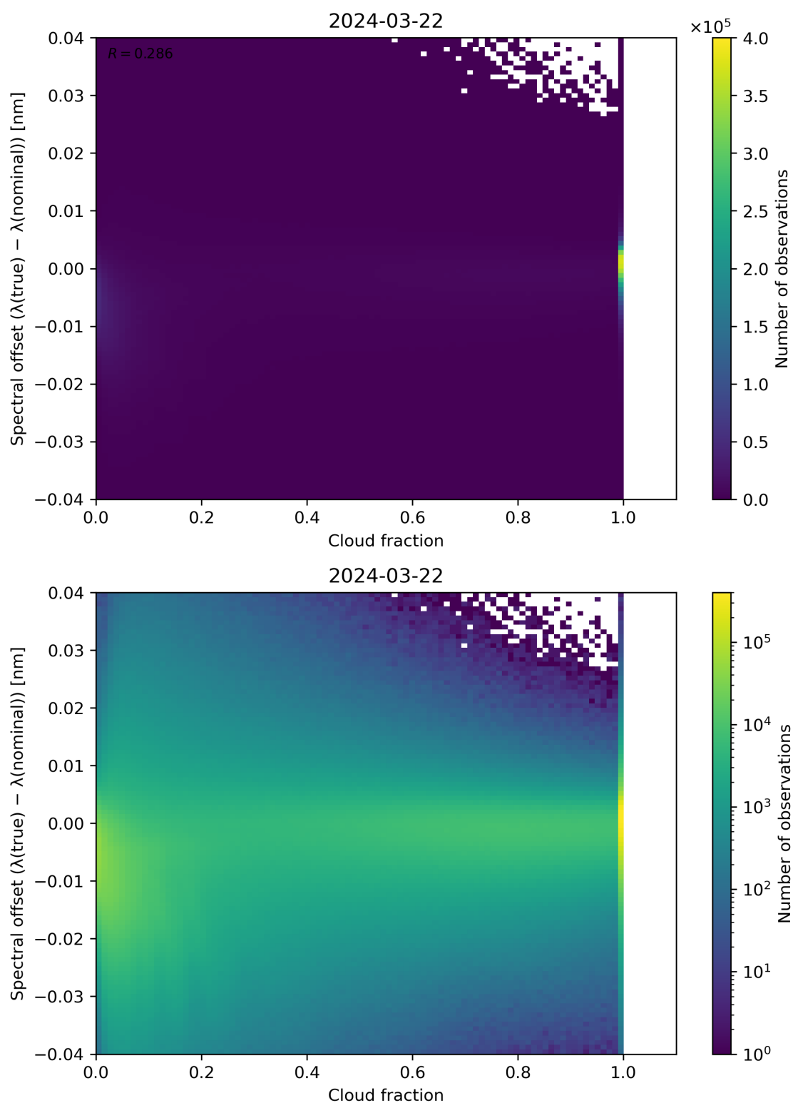
Figure 76: Scatter density plot of “Cloud fraction” against “Spectral offset ( \lambda(\text{true}) - \lambda(\text{nominal}) )” for 2024-03-21 to 2024-03-22.
