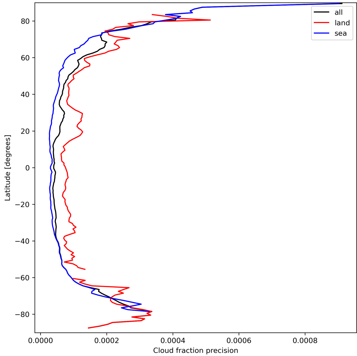
Figure 16: Zonal average of “Cloud fraction precision” for 2024-03-21 to 2024-03-22.
