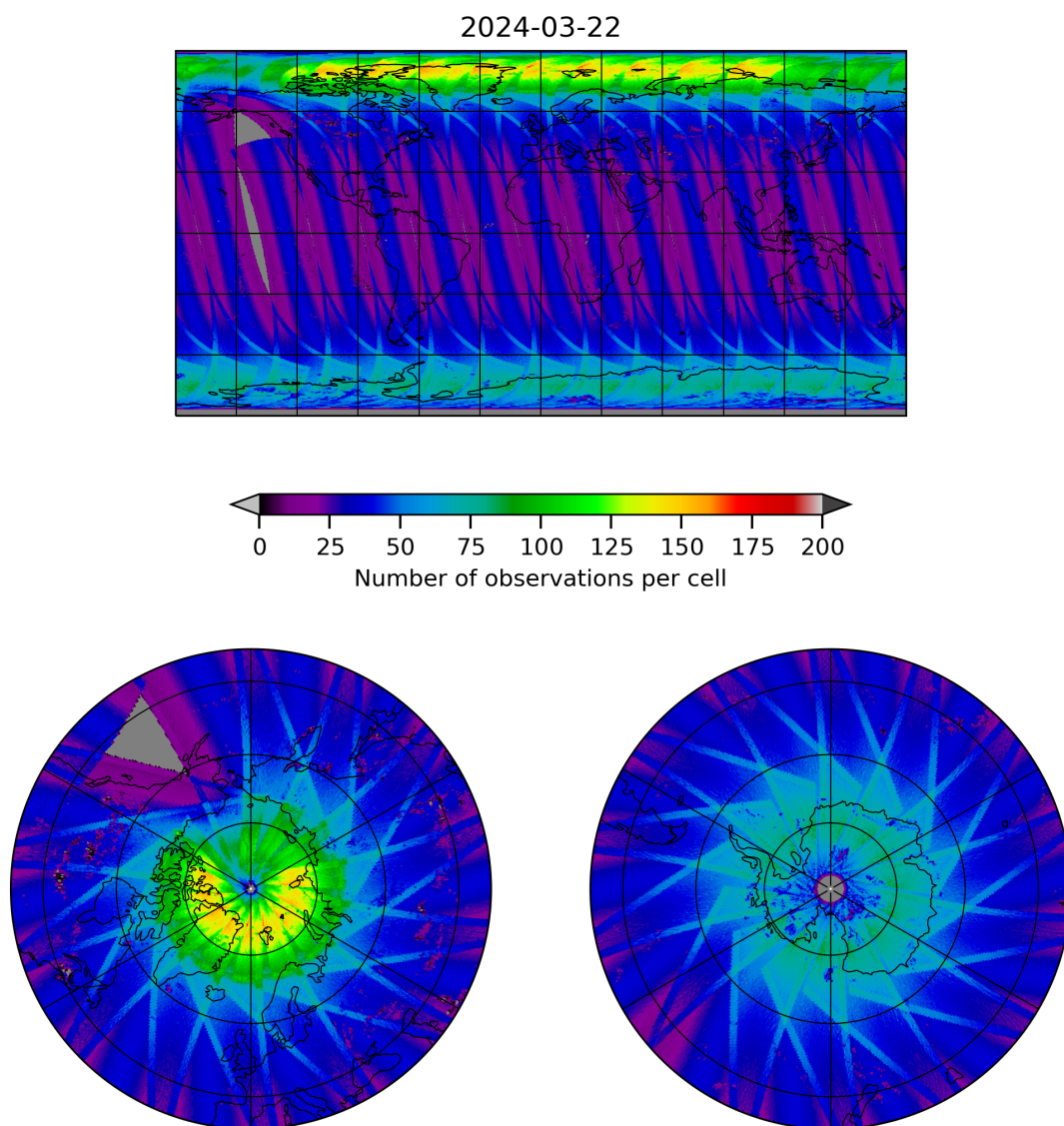
Figure 11: Map of the number of observations for 2024-03-21 to 2024-03-22
