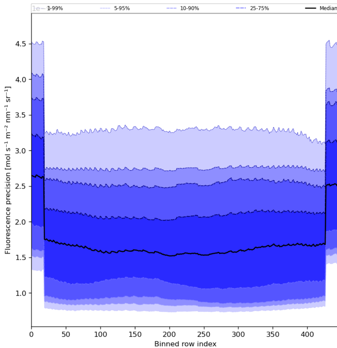
Figure 58: Along track statistics of “Fluorescence precision” for 2024-03-21 to 2024-03-22
