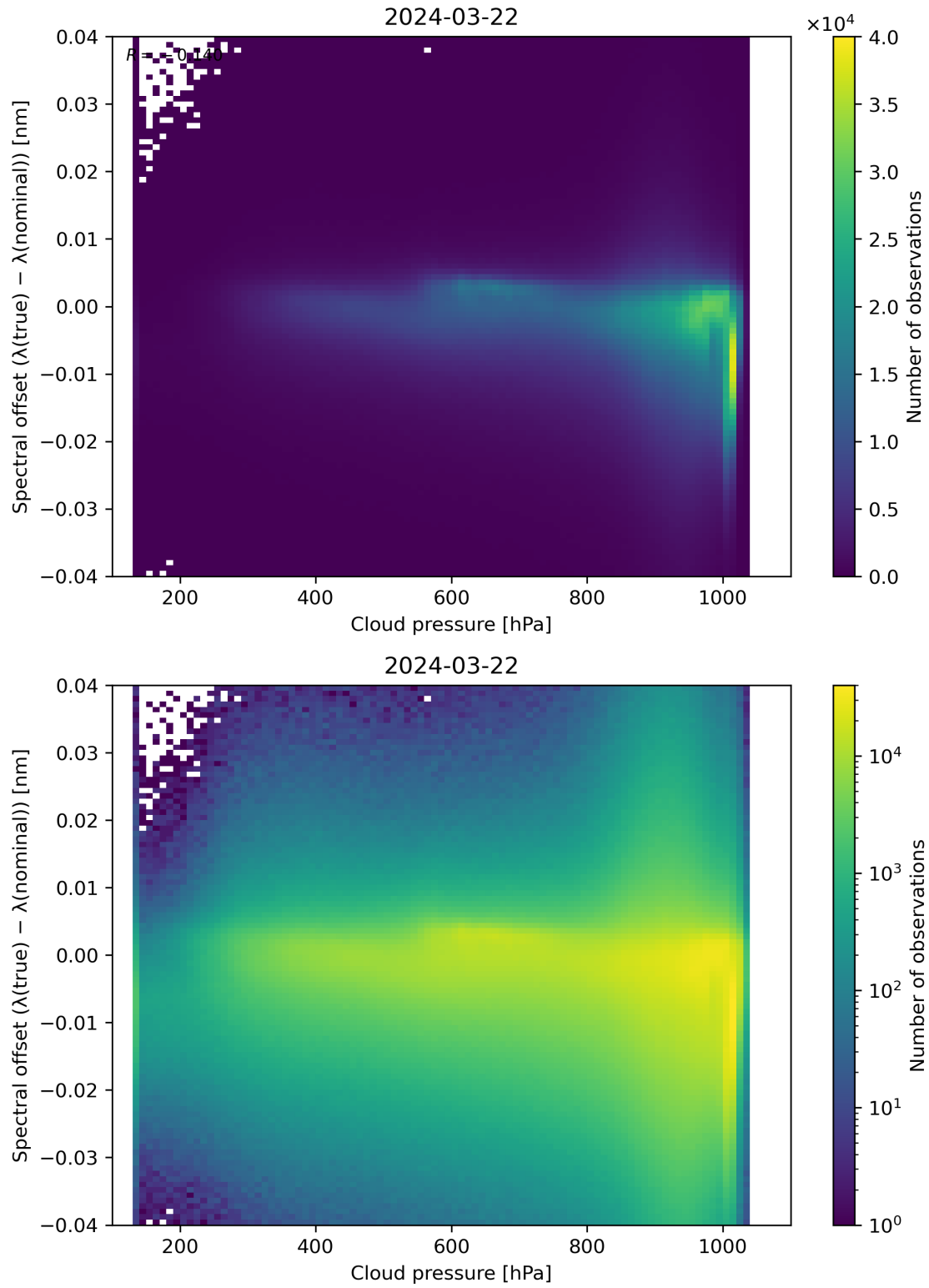
Figure 84: Scatter density plot of “Cloud pressure” against “Spectral offset ( \lambda(\text{true}) - \lambda(\text{nominal}) )” for 2024-03-21 to 2024-03-22.
