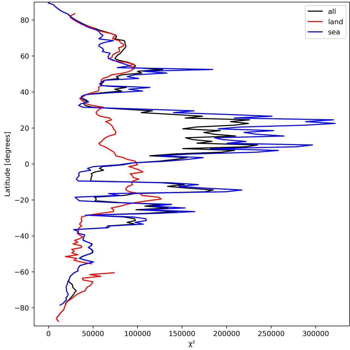
Figure 21: Zonal average of “ \chi^2 ” for 2024-03-21 to 2024-03-22.
