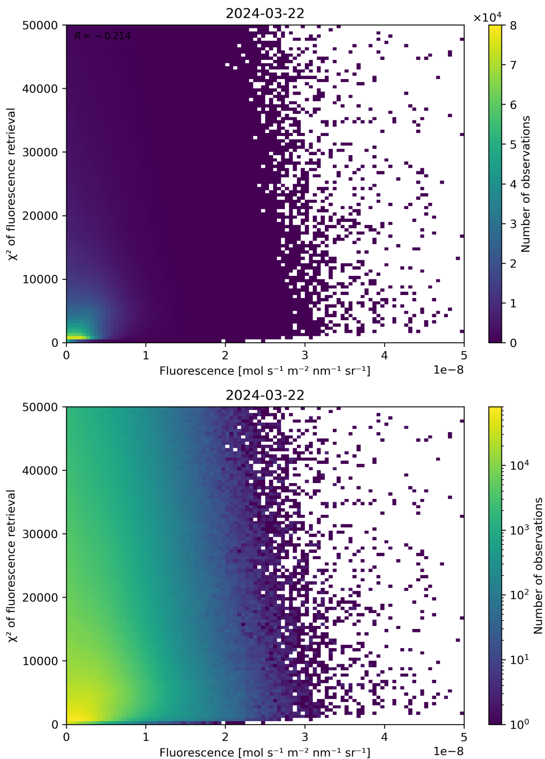
Figure 85: Scatter density plot of “Fluorescence” against “ \chi^2 of fluorescence retrieval” for 2024-03-21 to 2024-03-22.
