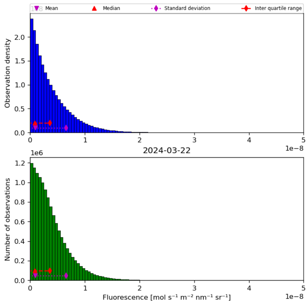
Figure 40: Histogram of “Fluorescence” for 2024-03-21 to 2024-03-22
