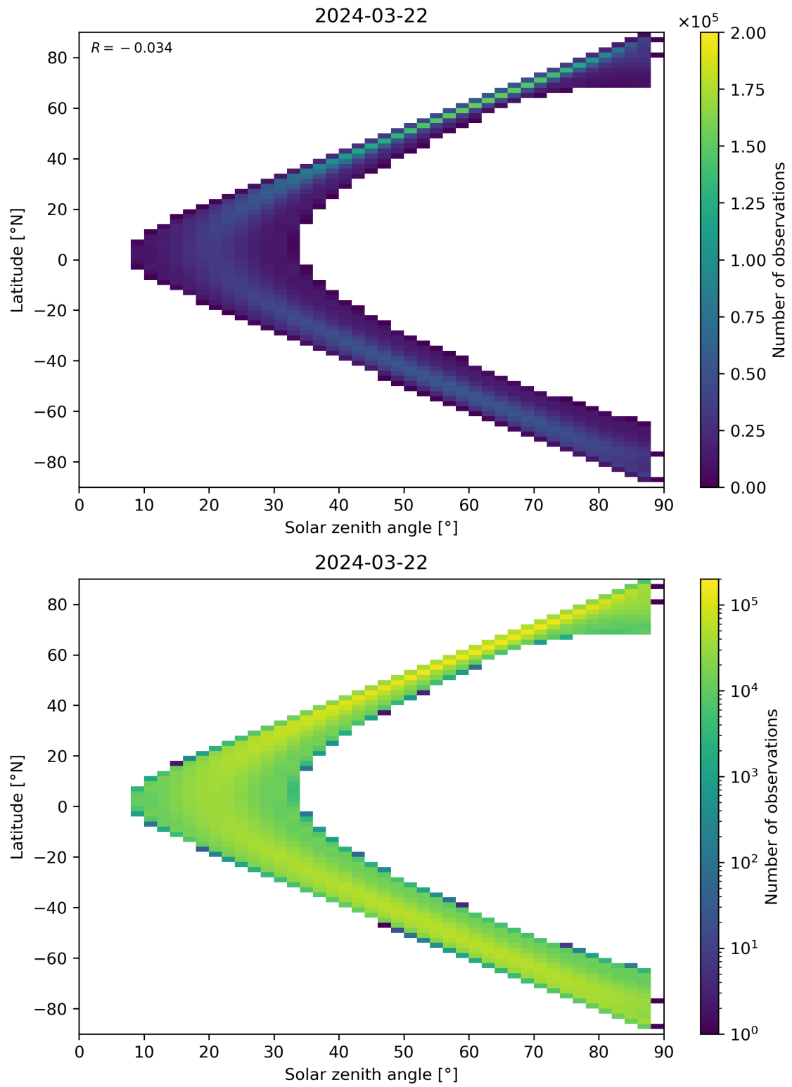
Figure 113: Scatter density plot of “Solar zenith angle” against “Latitude” for 2024-03-21 to 2024-03-22.
