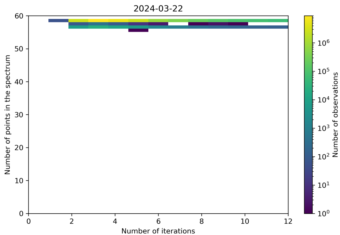
Figure 99: Scatter density plot of “Number of iterations” against “Number of points in the spectrum” for 2024-03-21 to 2024-03-22.
