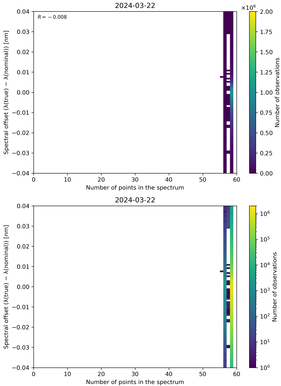
Figure 101: Scatter density plot of “Number of points in the spectrum” against “Spectral offset ( \lambda(\text{true}) - \lambda(\text{nominal}) )” for 2024-03-21 to 2024-03-22.
