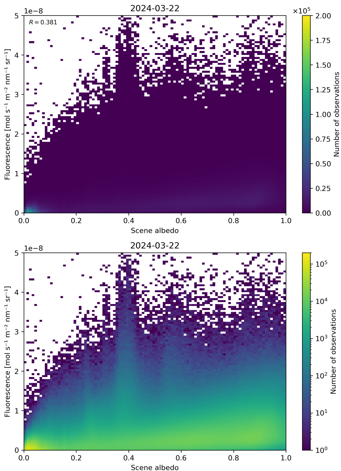
Figure 104: Scatter density plot of “Scene albedo” against “Fluorescence” for 2024-03-21 to 2024-03-22.
