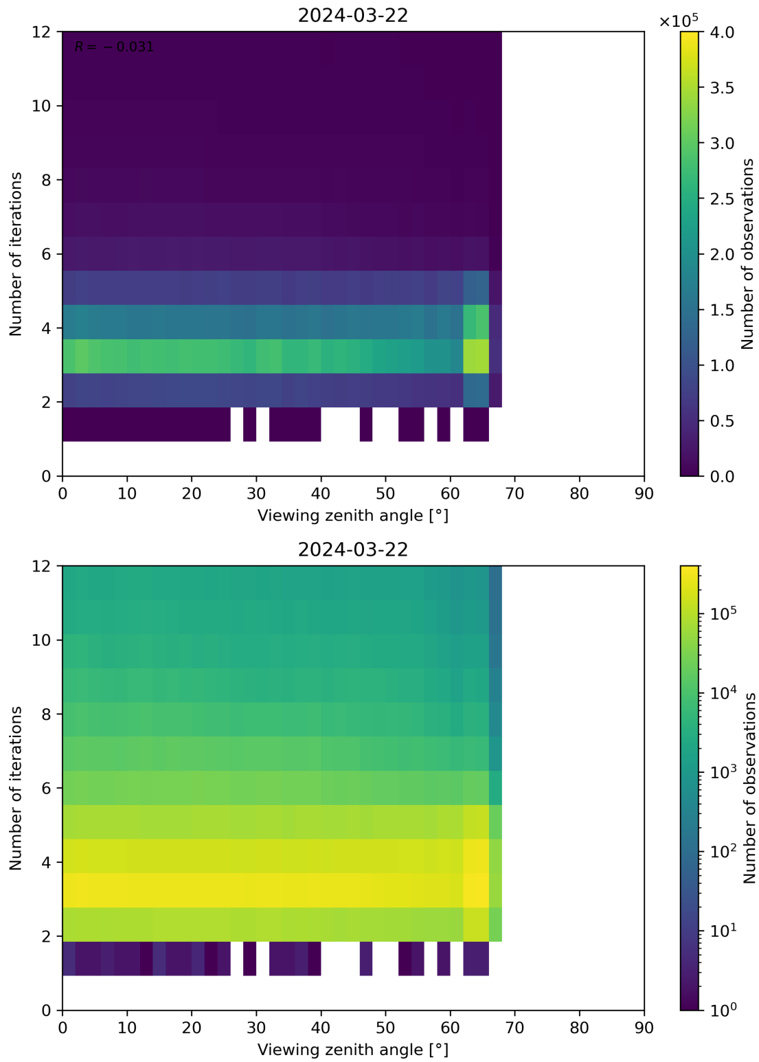
Figure 124: Scatter density plot of “Viewing zenith angle” against “Number of iterations” for 2024-03-21 to 2024-03-22.
