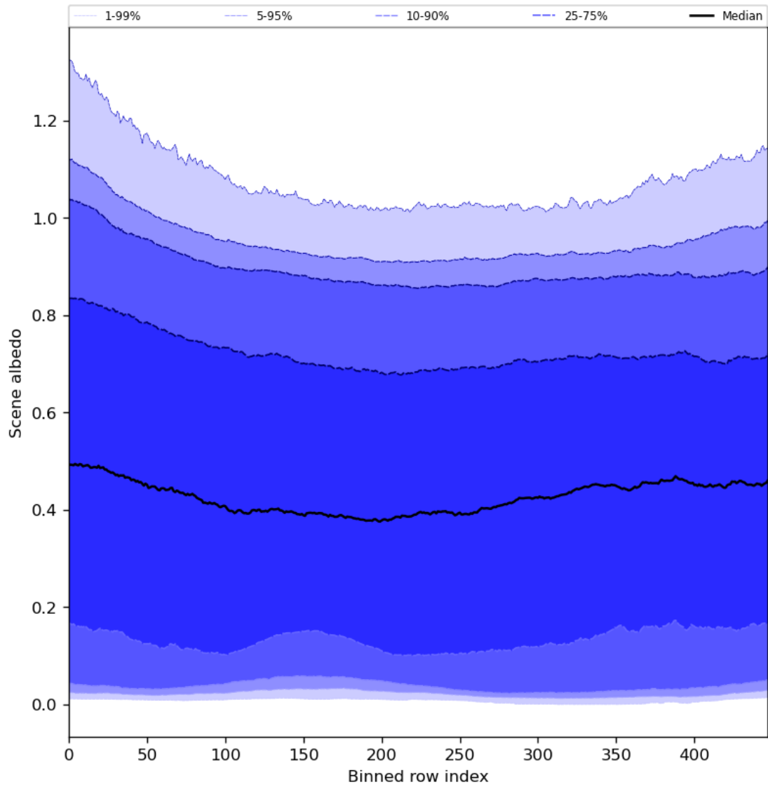
Figure 51: Along track statistics of “Scene albedo” for 2024-03-21 to 2024-03-22
