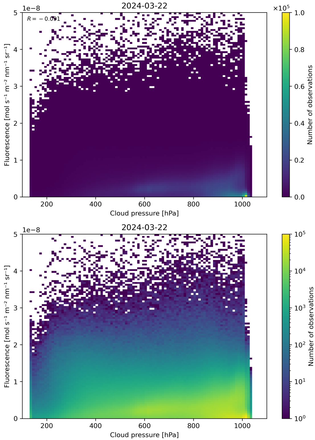
Figure 80: Scatter density plot of “Cloud pressure” against “Fluorescence” for 2024-03-21 to 2024-03-22.
