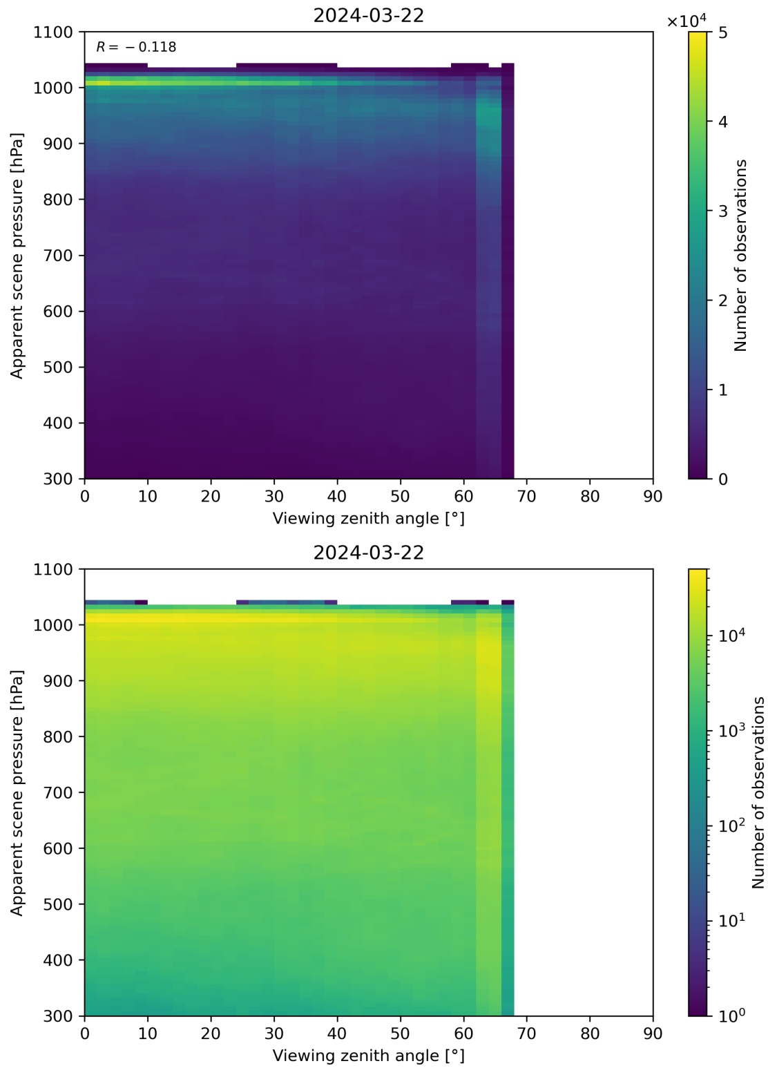
Figure 118: Scatter density plot of “Viewing zenith angle” against “Apparent scene pressure” for 2024-03-21 to 2024-03-22.
