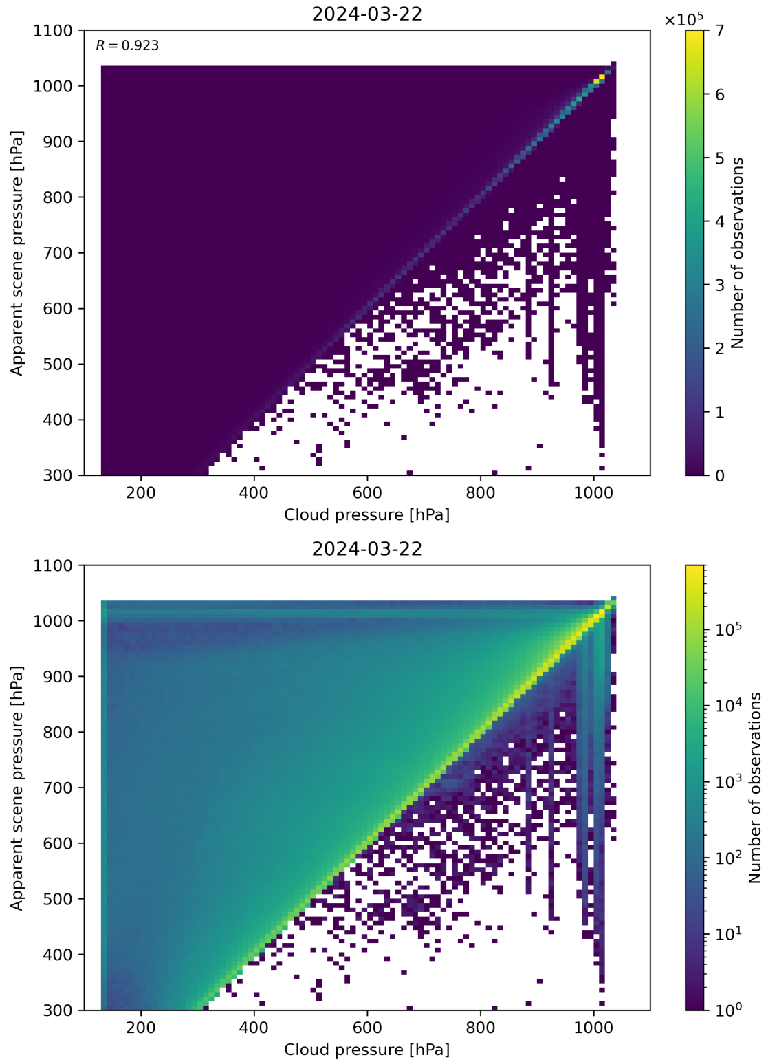
Figure 77: Scatter density plot of “Cloud pressure” against “Apparent scene pressure” for 2024-03-21 to 2024-03-22.
