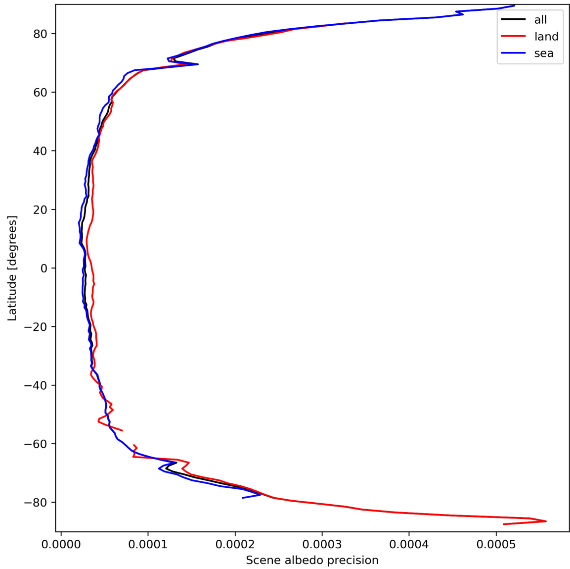
Figure 18: Zonal average of “Scene albedo precision” for 2024-03-21 to 2024-03-22.
