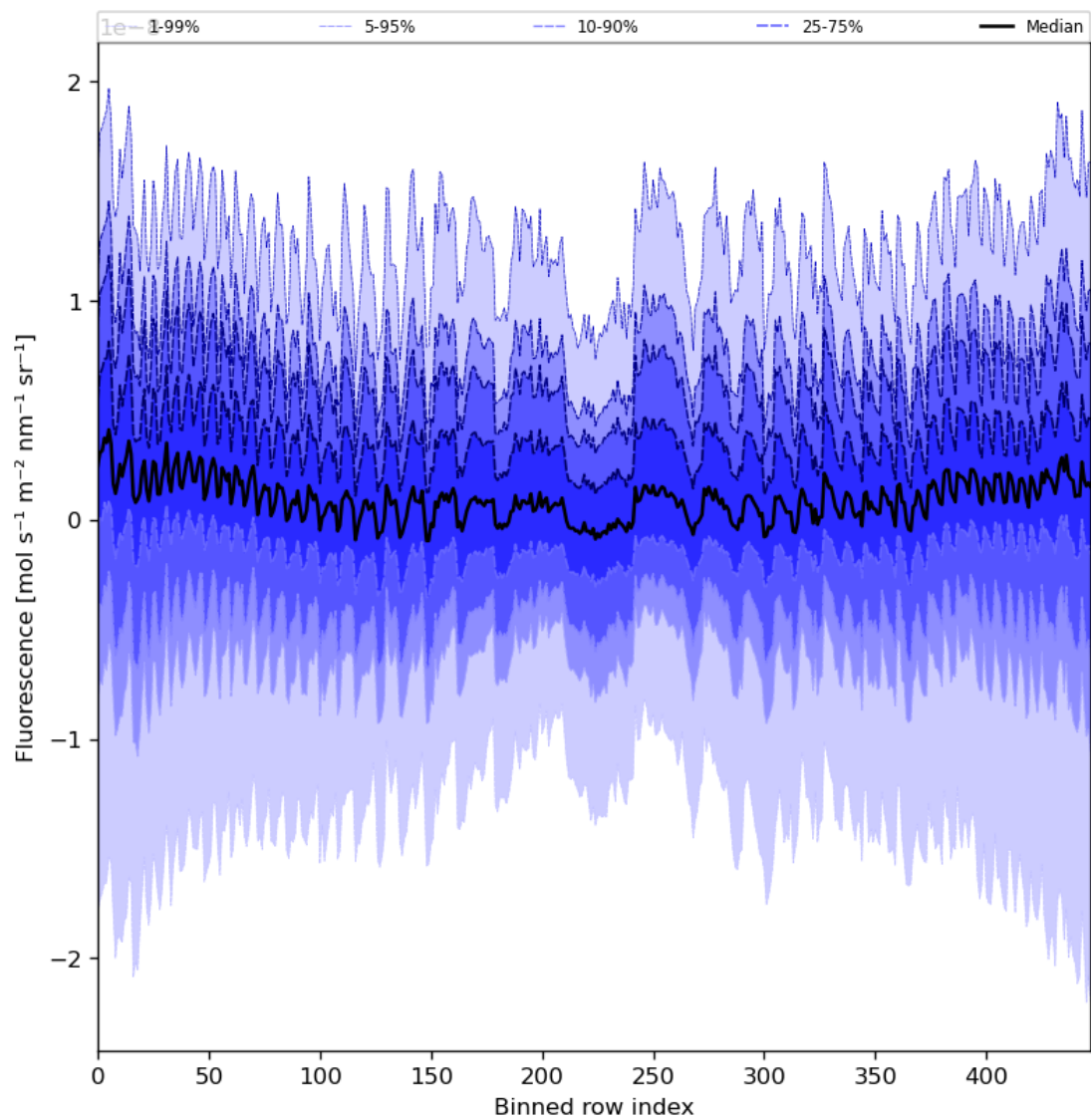
Figure 57: Along track statistics of “Fluorescence” for 2024-03-21 to 2024-03-22
