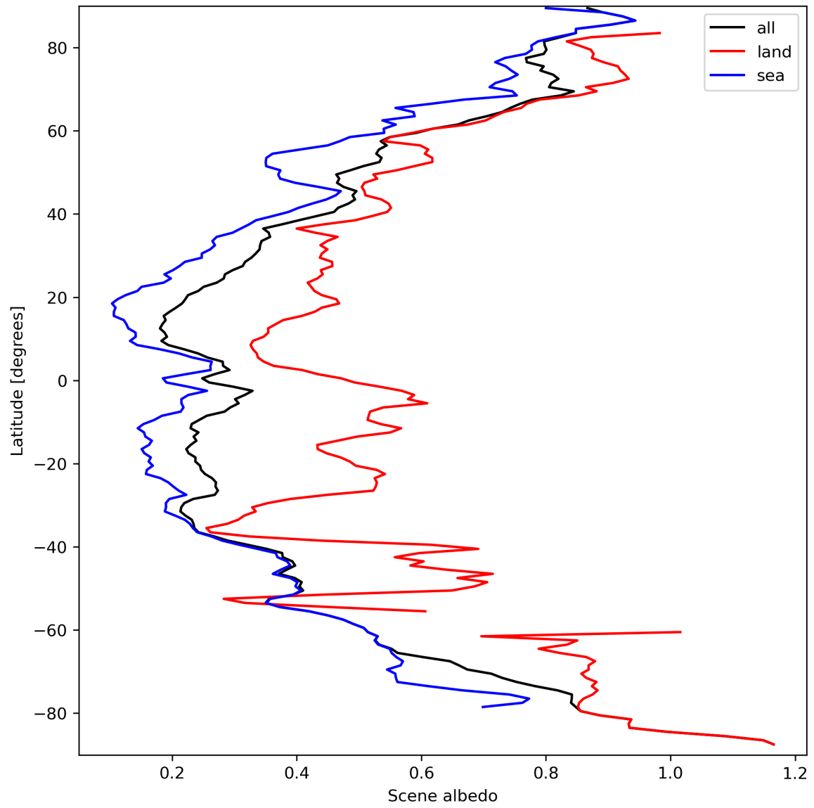
Figure 17: Zonal average of “Scene albedo” for 2024-03-21 to 2024-03-22.
