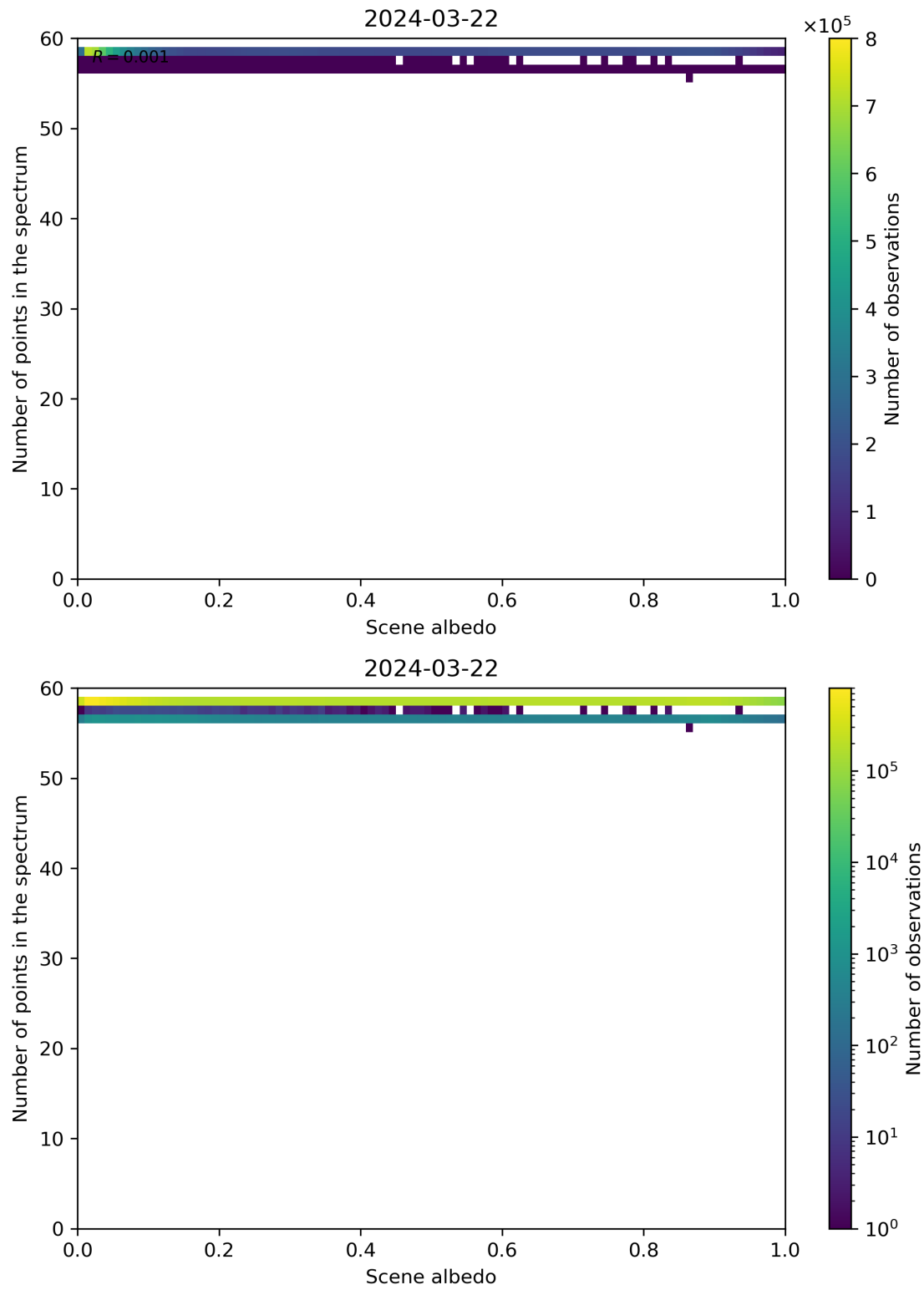
Figure 106: Scatter density plot of “Scene albedo” against “Number of points in the spectrum” for 2024-03-21 to 2024-03-22.
