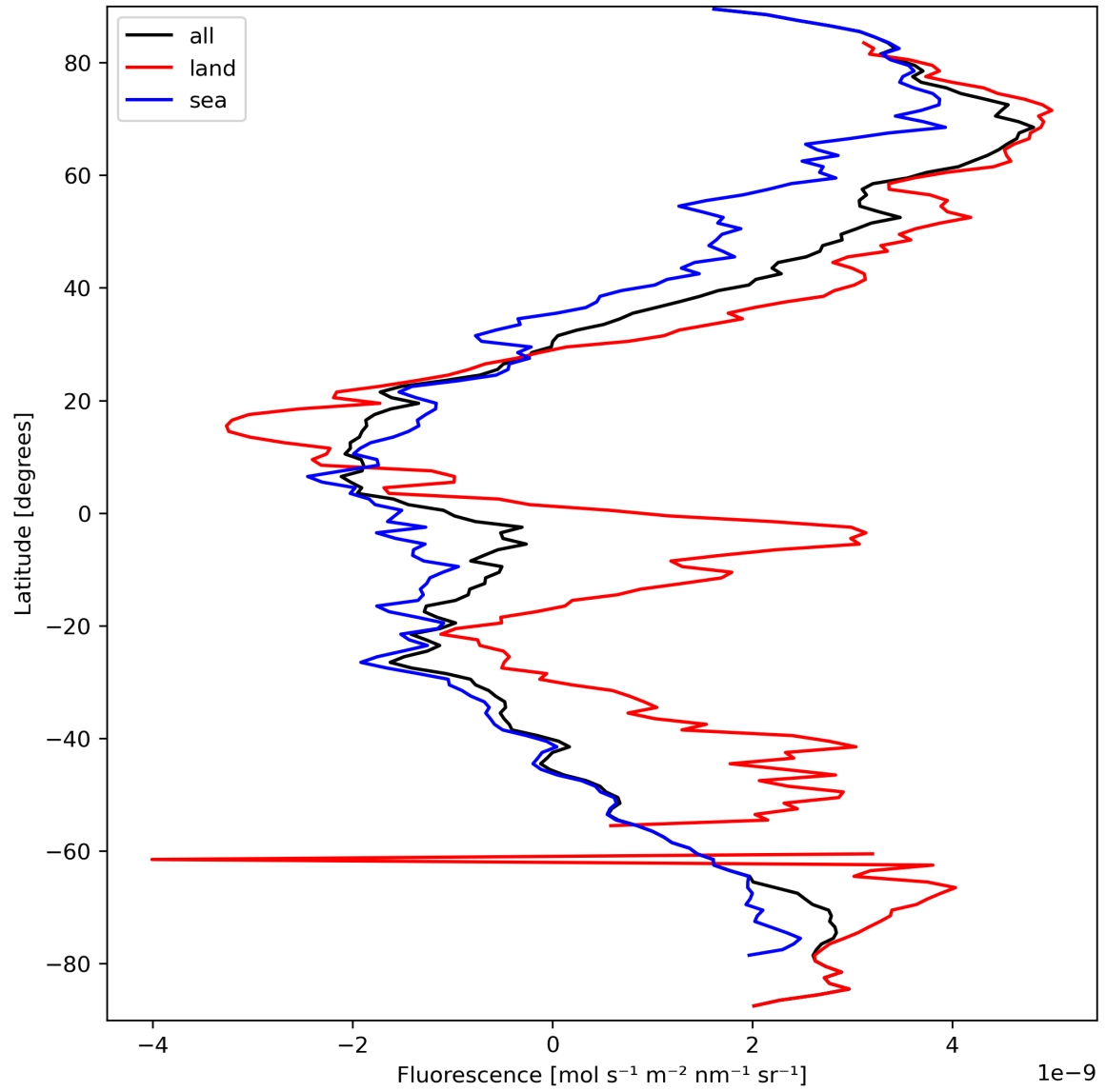
Figure 23: Zonal average of “Fluorescence” for 2024-03-21 to 2024-03-22.
