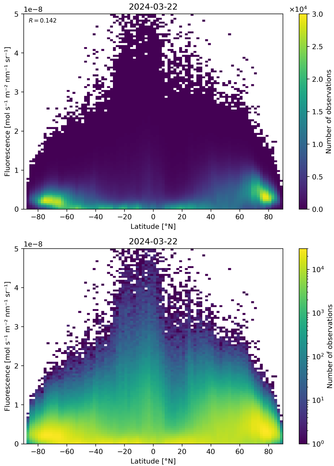
Figure 92: Scatter density plot of “Latitude” against “Fluorescence” for 2024-03-21 to 2024-03-22.
