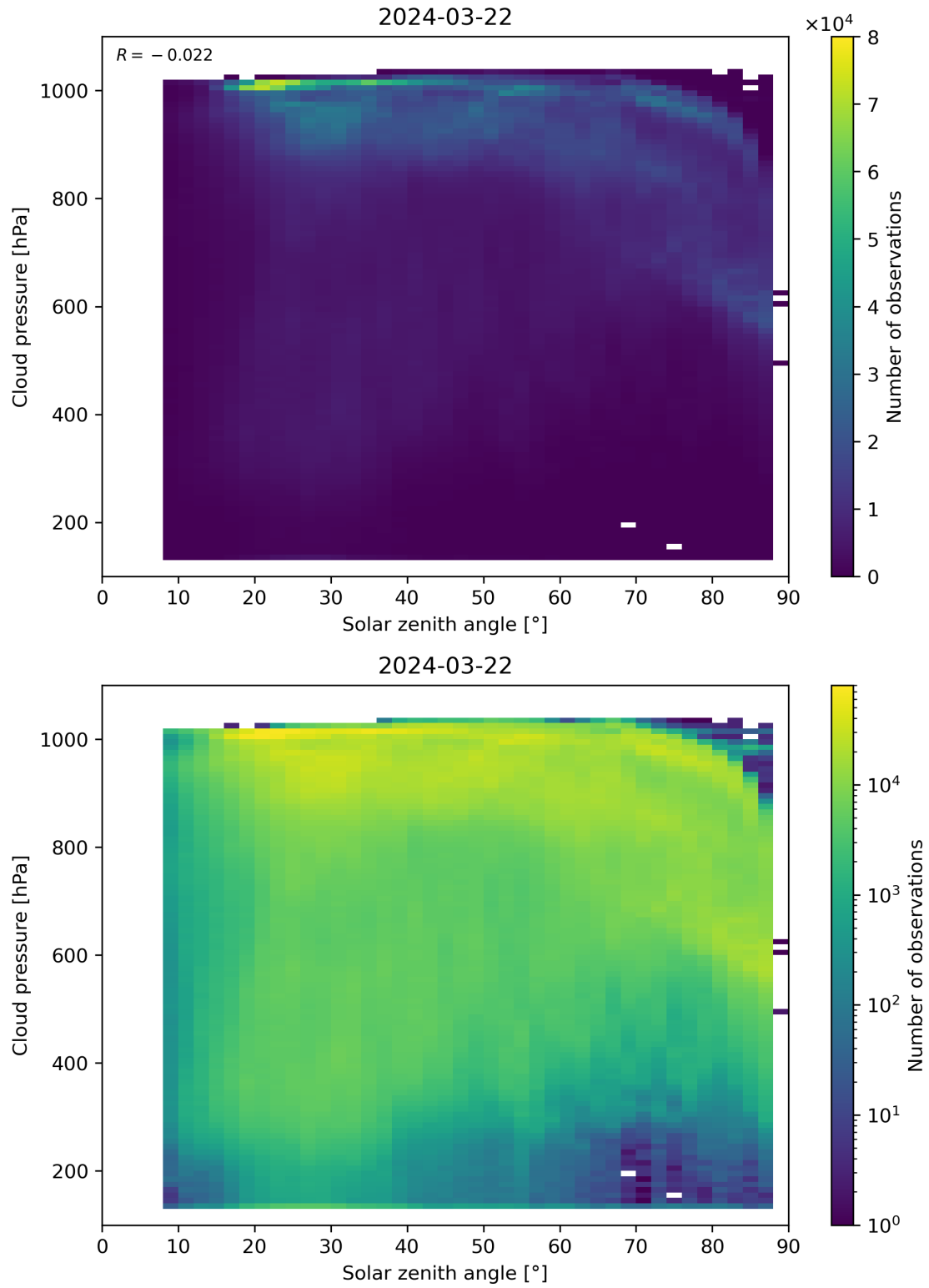
Figure 111: Scatter density plot of “Solar zenith angle” against “Cloud pressure” for 2024-03-21 to 2024-03-22.
