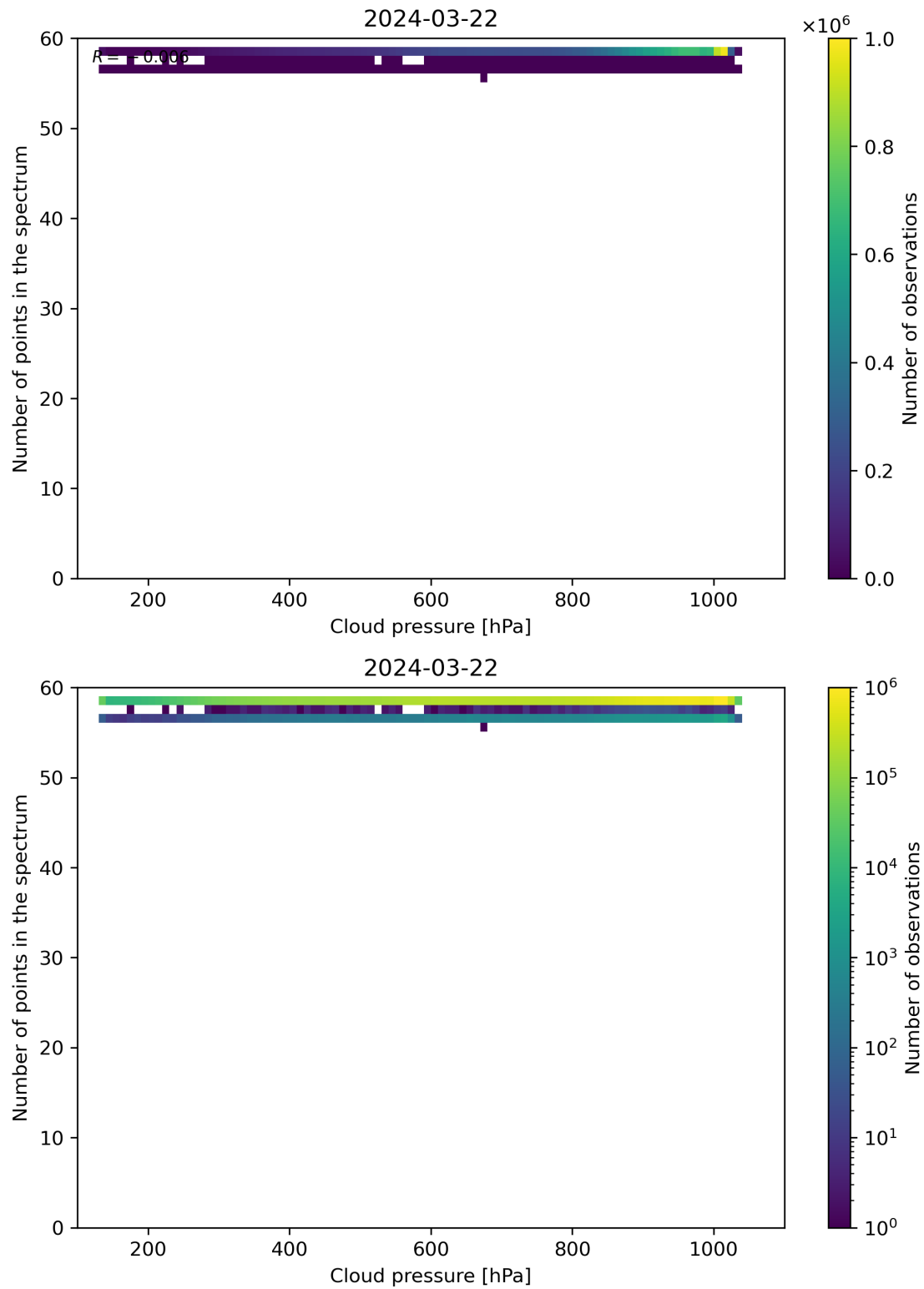
Figure 82: Scatter density plot of “Cloud pressure” against “Number of points in the spectrum” for 2024-03-21 to 2024-03-22.
