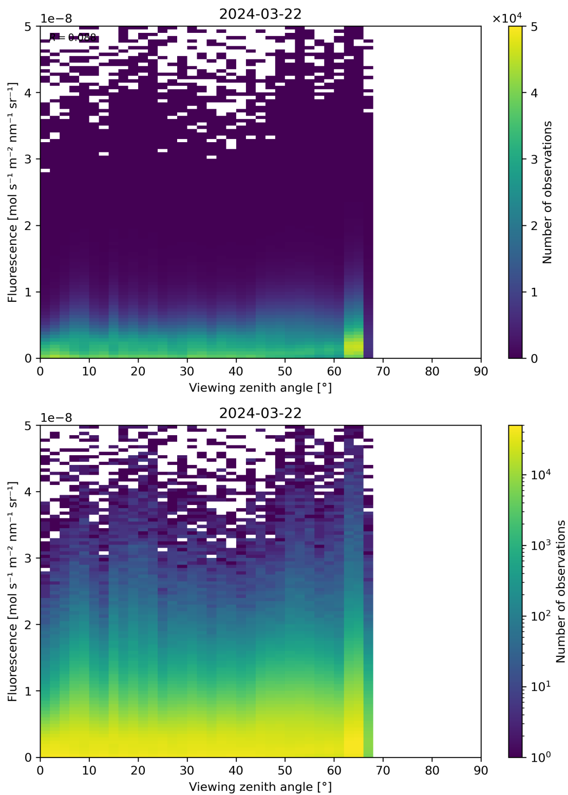
Figure 122: Scatter density plot of “Viewing zenith angle” against “Fluorescence” for 2024-03-21 to 2024-03-22.
