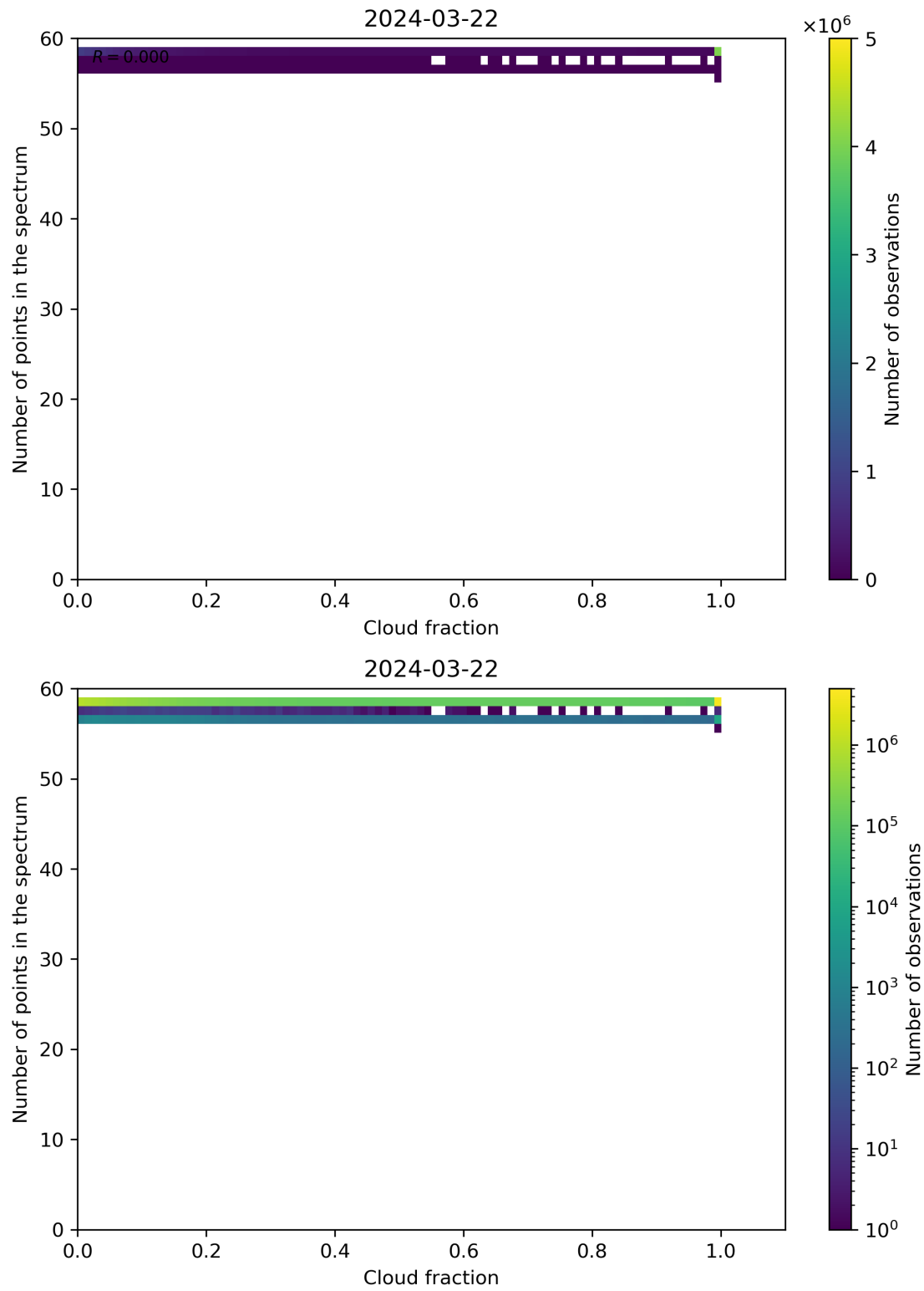
Figure 74: Scatter density plot of “Cloud fraction” against “Number of points in the spectrum” for 2024-03-21 to 2024-03-22.
