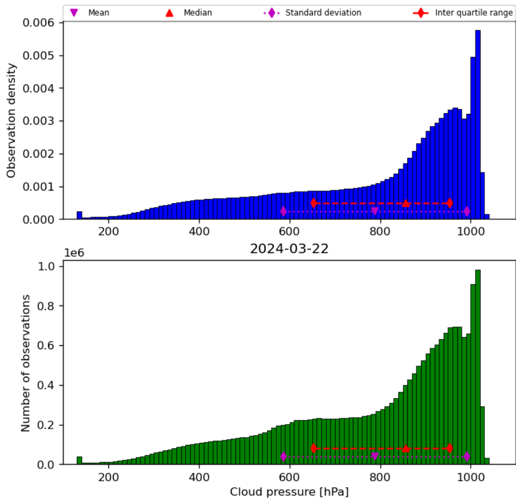
Figure 30: Histogram of “Cloud pressure” for 2024-03-21 to 2024-03-22
