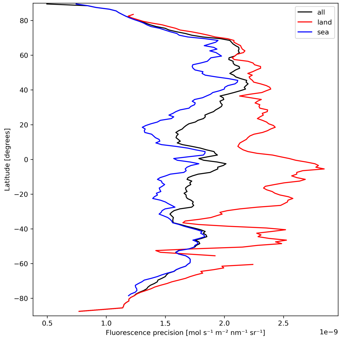
Figure 24: Zonal average of “Fluorescence precision” for 2024-03-21 to 2024-03-22.
