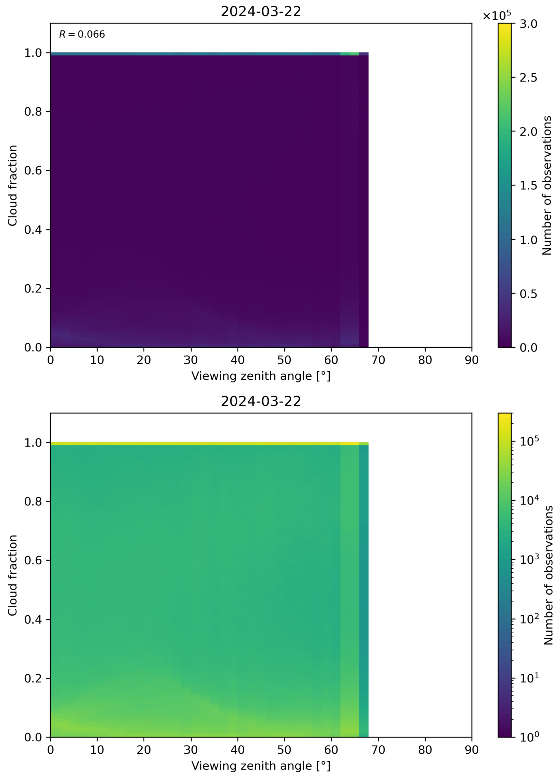
Figure 120: Scatter density plot of “Viewing zenith angle” against “Cloud fraction” for 2024-03-21 to 2024-03-22.
