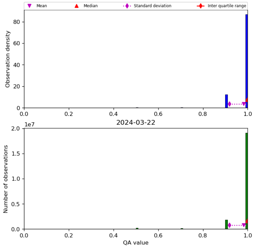
Figure 29: Histogram of “QA value” for 2024-03-21 to 2024-03-22
