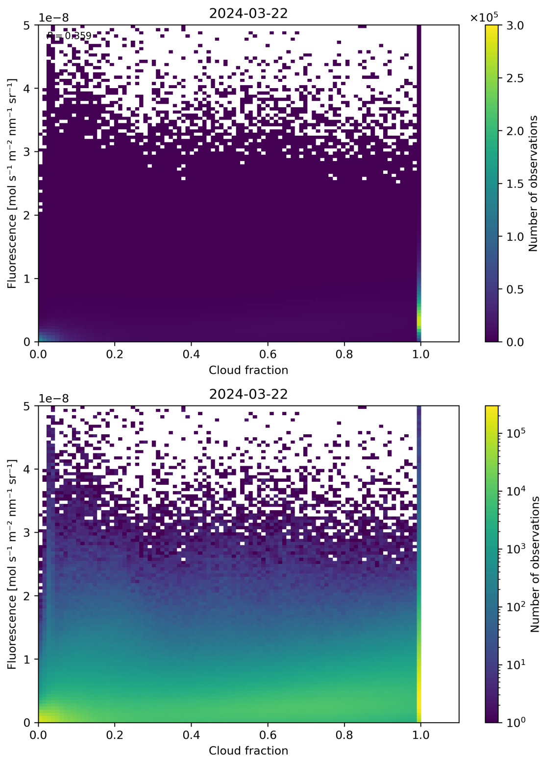
Figure 72: Scatter density plot of “Cloud fraction” against “Fluorescence” for 2024-03-21 to 2024-03-22.
