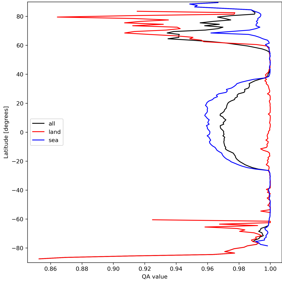
Figure 12: Zonal average of "QA value" for 2024-03-21 to 2024-03-22.
