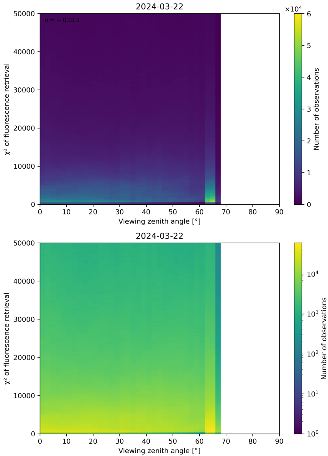
Figure 119: Scatter density plot of “Viewing zenith angle” against “ \chi^2 of fluorescence retrieval” for 2024-03-21 to 2024-03-22.
