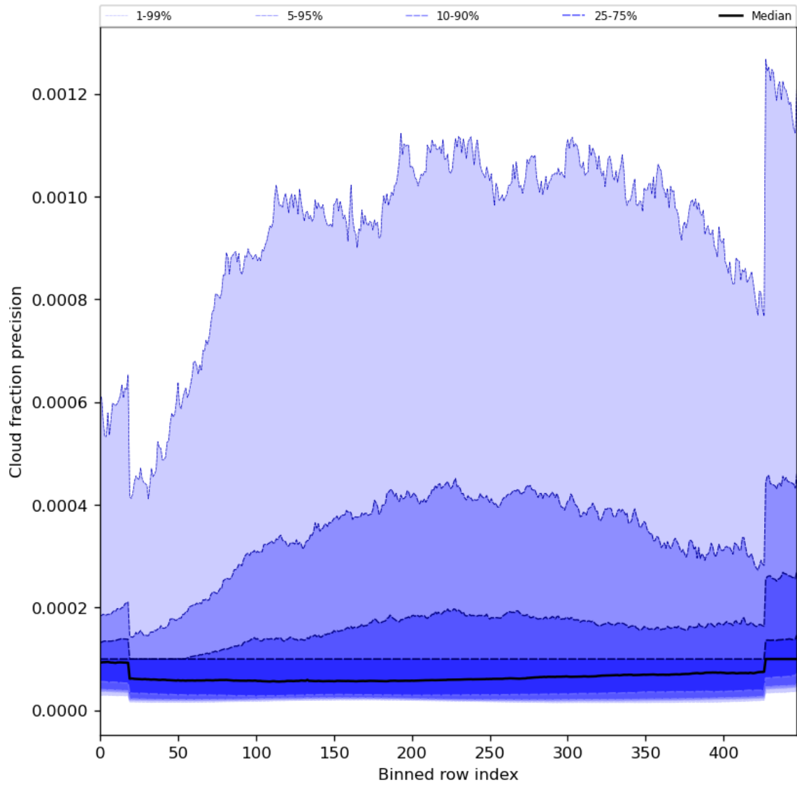
Figure 50: Along track statistics of “Cloud fraction precision” for 2024-03-21 to 2024-03-22
