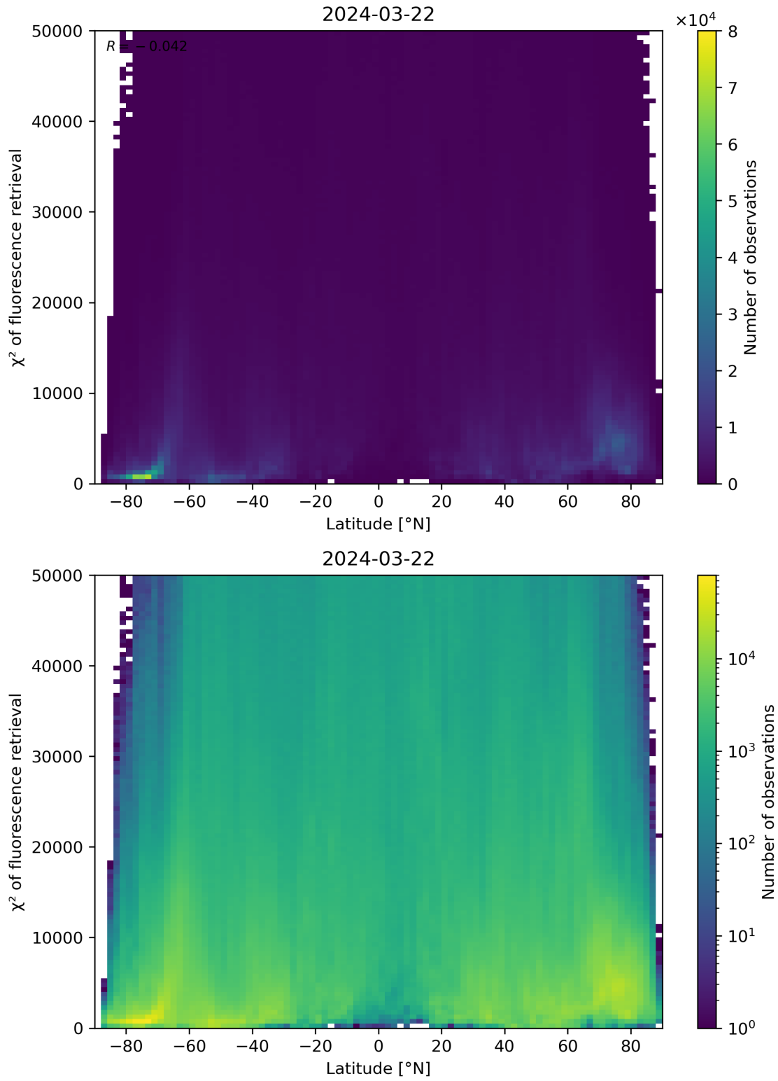
Figure 89: Scatter density plot of “Latitude” against “ \chi^2 of fluorescence retrieval” for 2024-03-21 to 2024-03-22.
