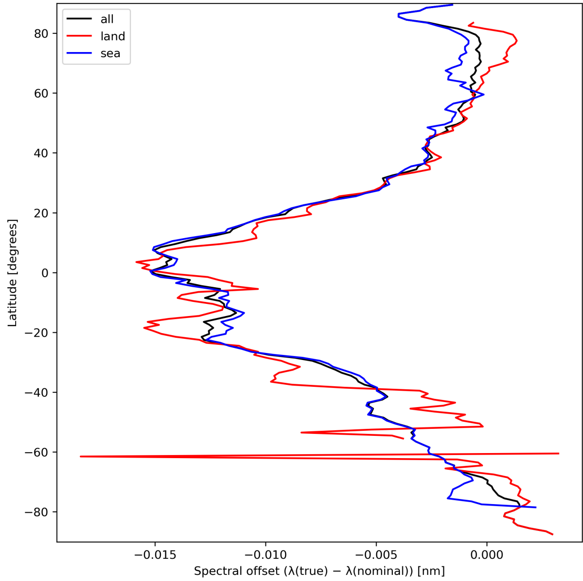
Figure 28: Zonal average of “Spectral offset ( \lambda(\text{true}) - \lambda(\text{nominal}) )” for 2024-03-21 to 2024-03-22.
