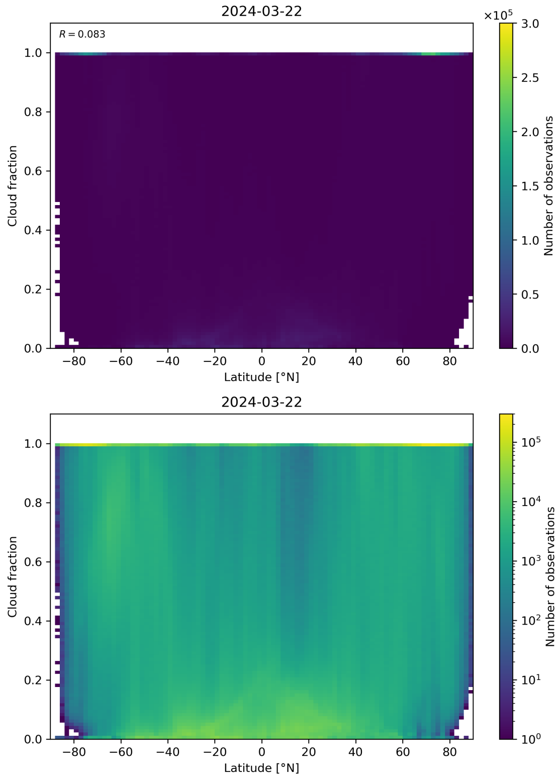
Figure 90: Scatter density plot of “Latitude” against “Cloud fraction” for 2024-03-21 to 2024-03-22.
