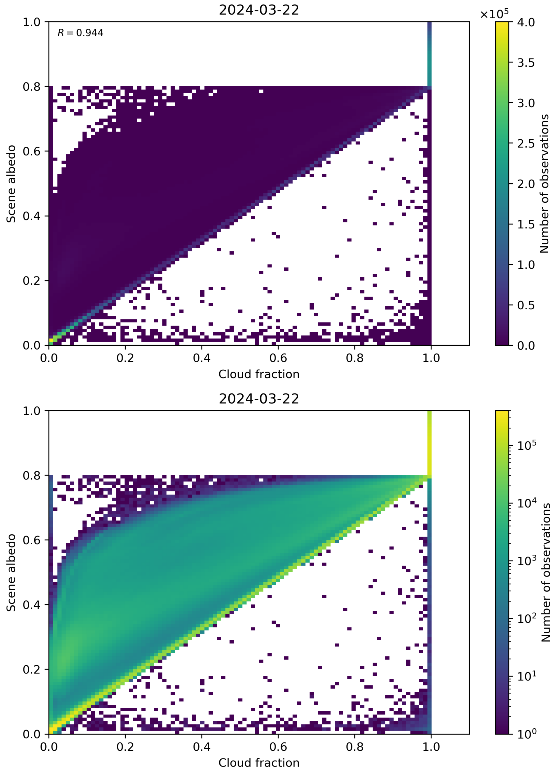
Figure 75: Scatter density plot of “Cloud fraction” against “Scene albedo” for 2024-03-21 to 2024-03-22.
