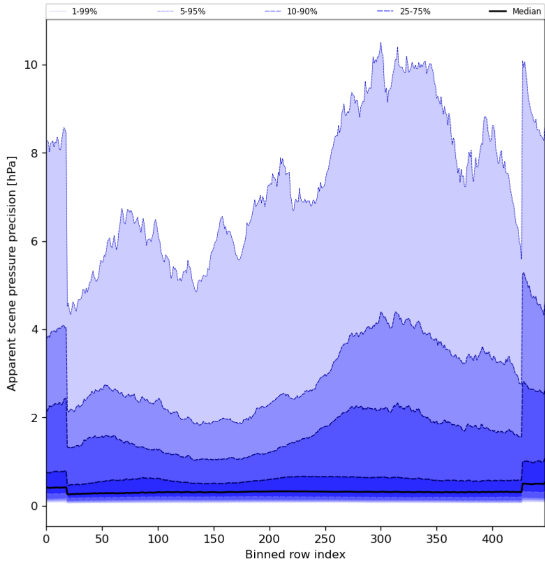
Figure 54: Along track statistics of “Apparent scene pressure precision” for 2024-03-21 to 2024-03-22
