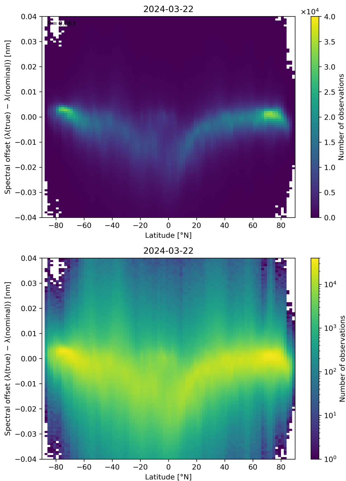
Figure 96: Scatter density plot of “Latitude” against “Spectral offset ( \lambda(\text{true}) - \lambda(\text{nominal}) )” for 2024-03-21 to 2024-03-22.
