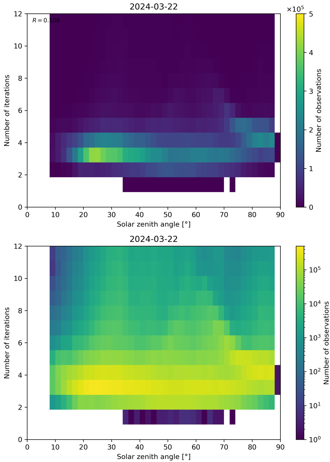
Figure 114: Scatter density plot of “Solar zenith angle” against “Number of iterations” for 2024-03-21 to 2024-03-22.
