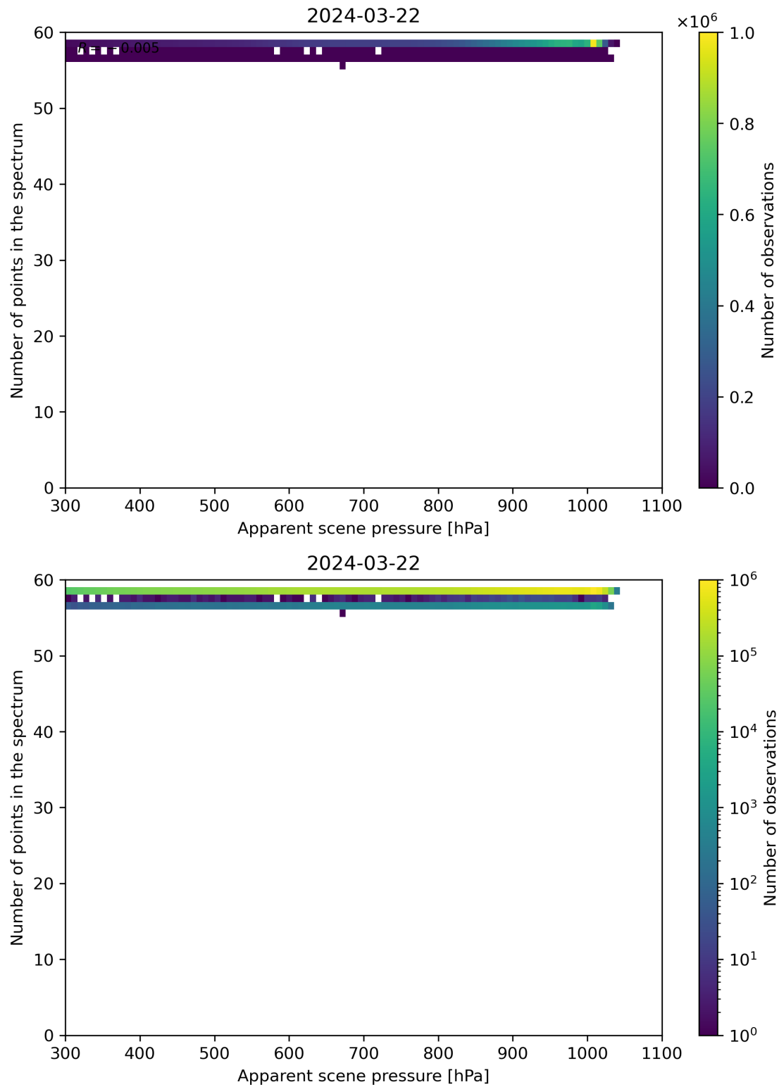
Figure 66: Scatter density plot of “Apparent scene pressure” against “Number of points in the spectrum” for 2024-03-21 to 2024-03-22.
