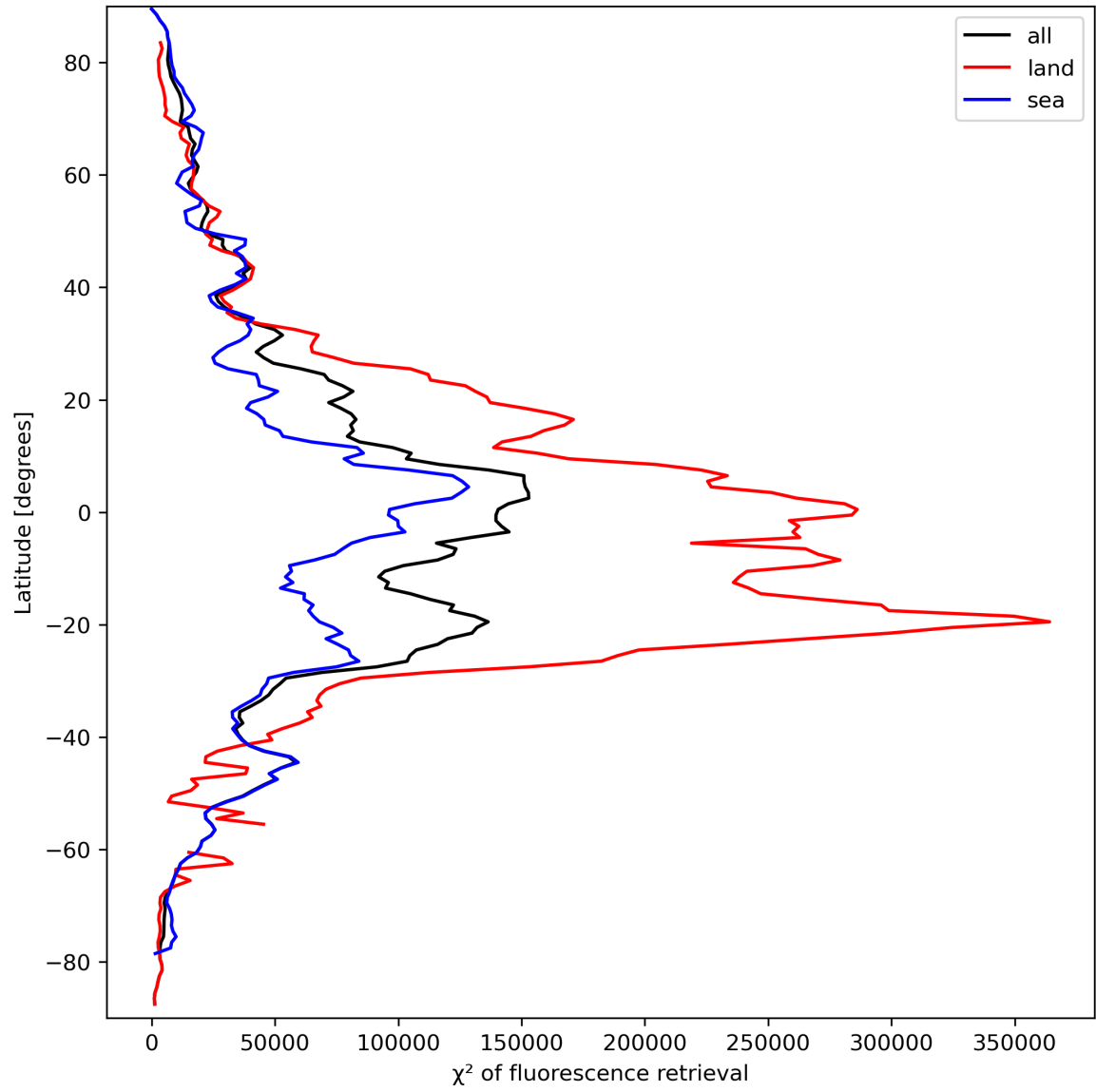
Figure 25: Zonal average of “ \chi^2 of fluorescence retrieval” for 2024-03-21 to 2024-03-22.
