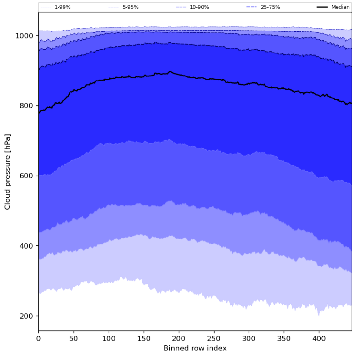
Figure 47: Along track statistics of “Cloud pressure” for 2024-03-21 to 2024-03-22
