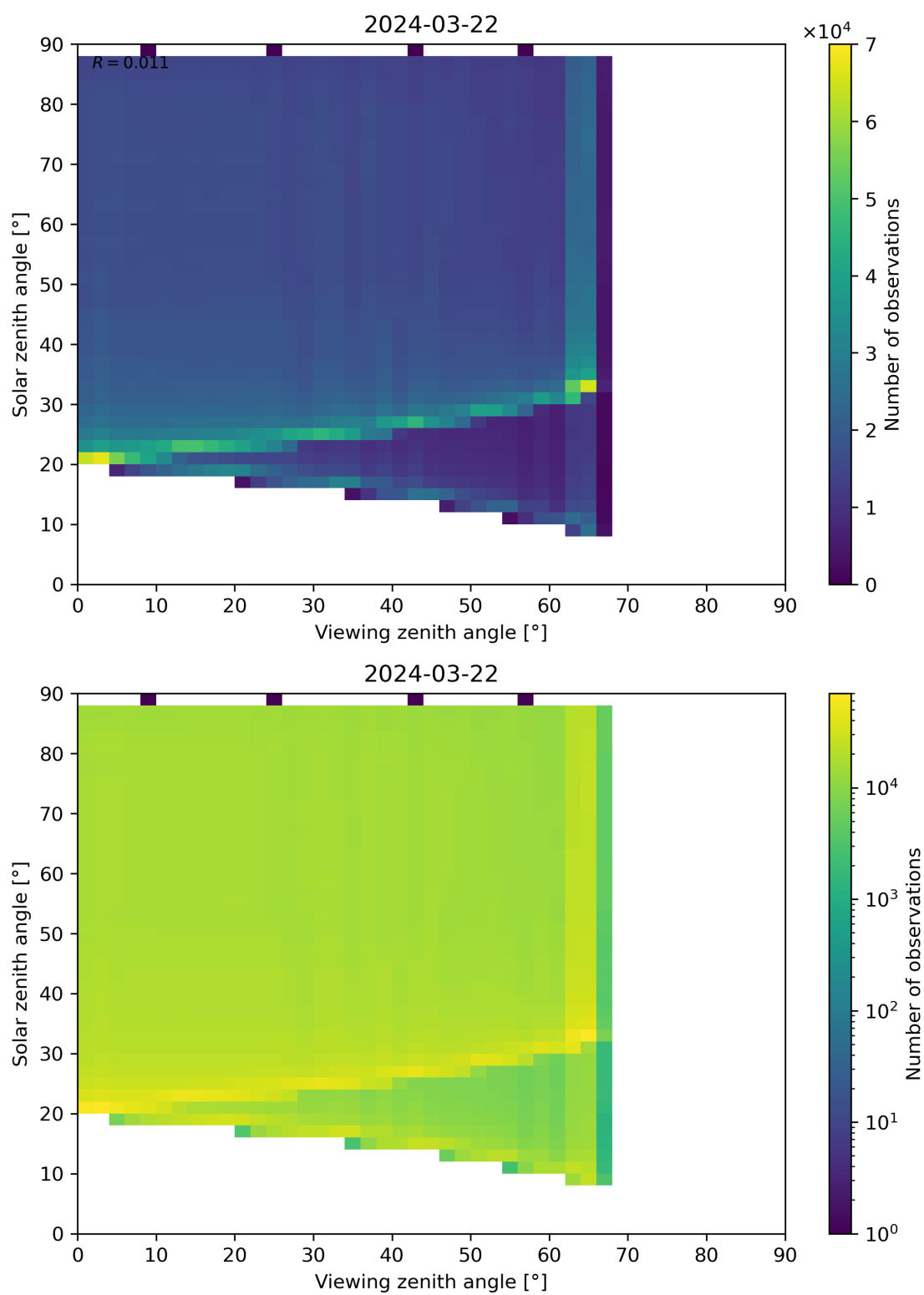
Figure 127: Scatter density plot of “Viewing zenith angle” against “Solar zenith angle” for 2024-03-21 to 2024-03-22.
