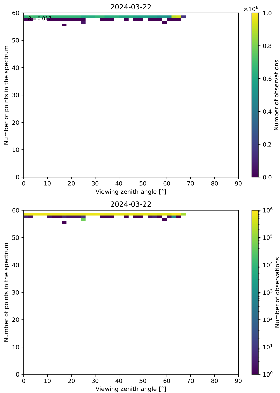
Figure 125: Scatter density plot of “Viewing zenith angle” against “Number of points in the spectrum” for 2024-03-21 to 2024-03-22.
