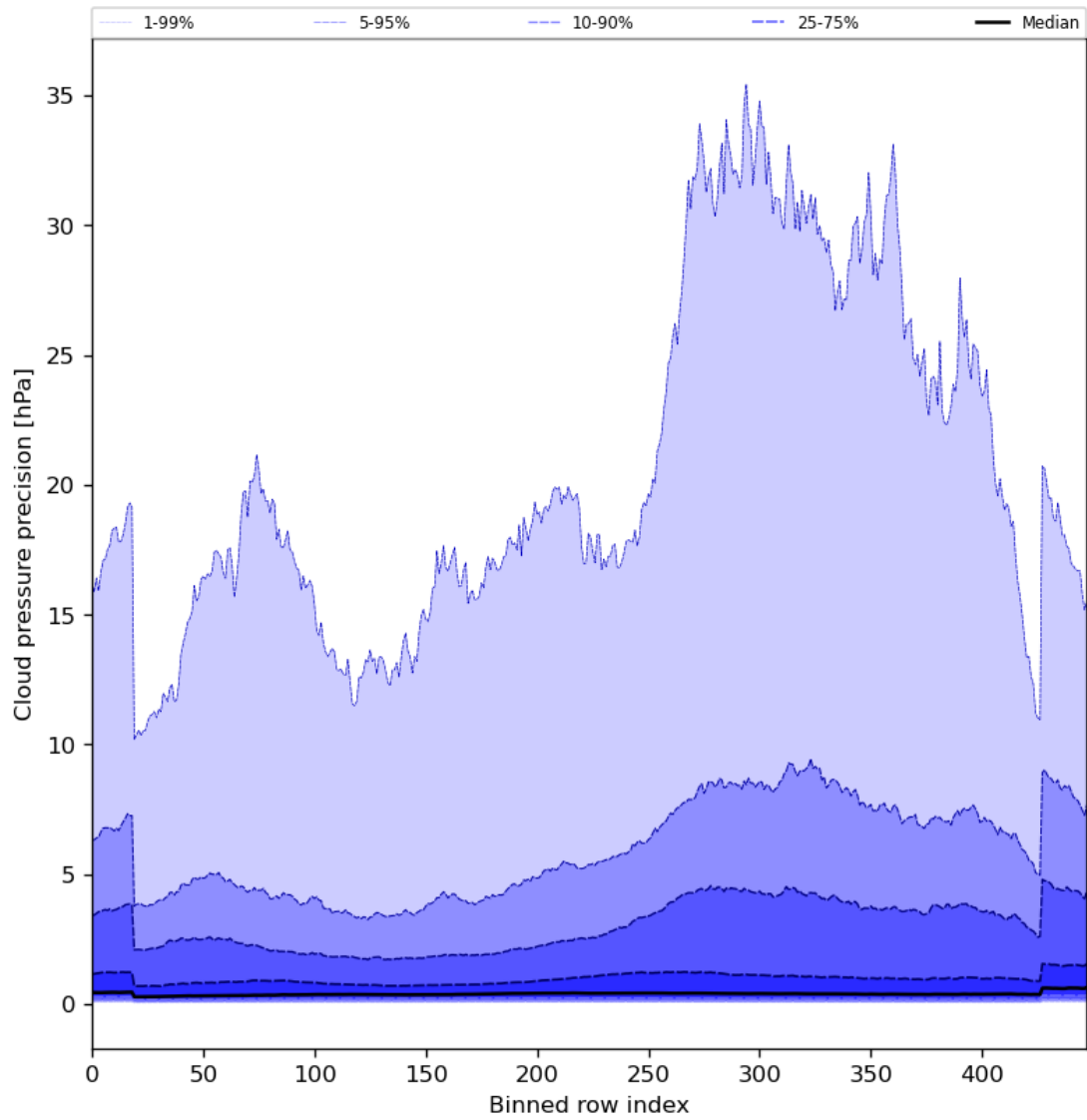
Figure 48: Along track statistics of “Cloud pressure precision” for 2024-03-21 to 2024-03-22
