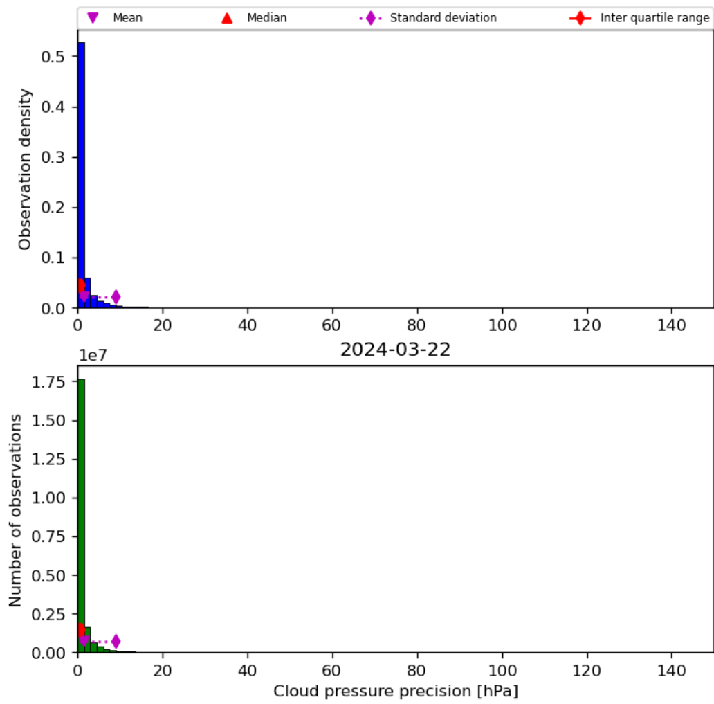
Figure 31: Histogram of “Cloud pressure precision” for 2024-03-21 to 2024-03-22
