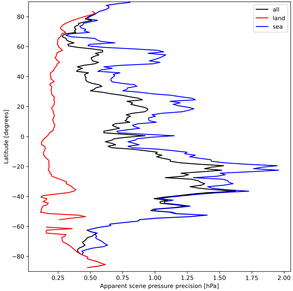
Figure 20: Zonal average of “Apparent scene pressure precision” for 2024-03-21 to 2024-03-22.
