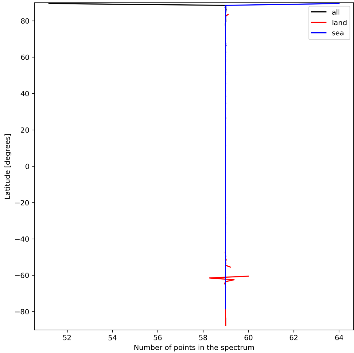
Figure 27: Zonal average of “Number of points in the spectrum” for 2024-03-21 to 2024-03-22.
