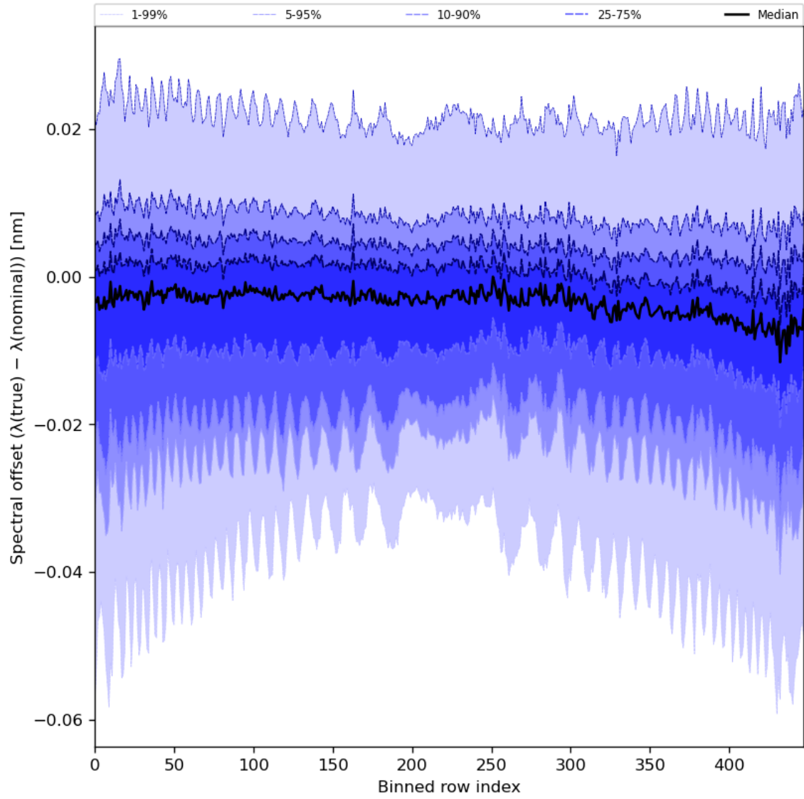
Figure 62: Along track statistics of “Spectral offset ( \lambda(\text{true}) - \lambda(\text{nominal}) )” for 2024-03-21 to 2024-03-22
