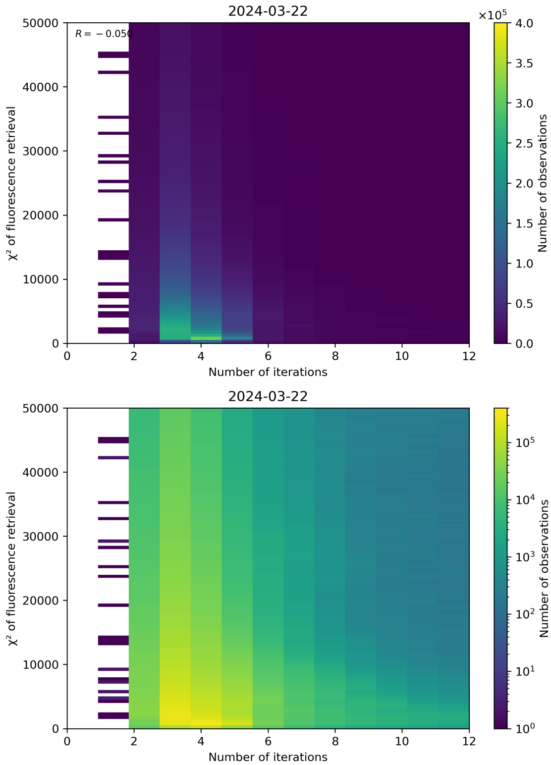
Figure 97: Scatter density plot of “Number of iterations” against “ \chi^2 of fluorescence retrieval” for 2024-03-21 to 2024-03-22.
