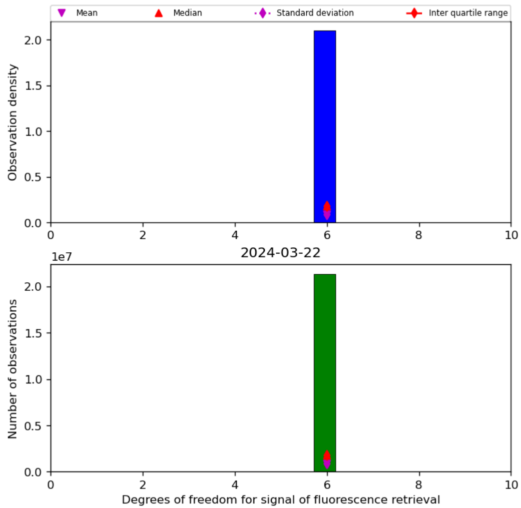
Figure 43: Histogram of “Degrees of freedom for signal of fluorescence retrieval” for 2024-03-21 to 2024-03-22
