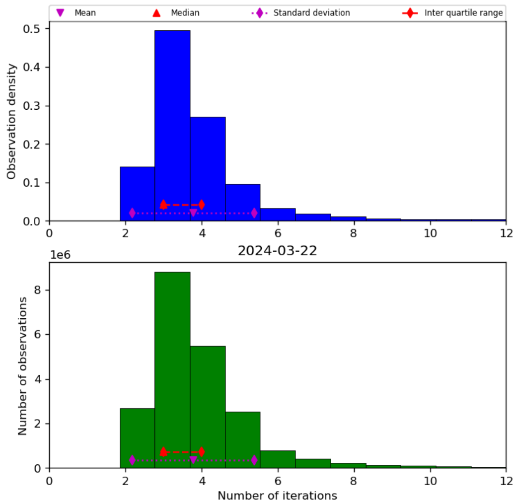
Figure 39: Histogram of “Number of iterations” for 2024-03-21 to 2024-03-22
