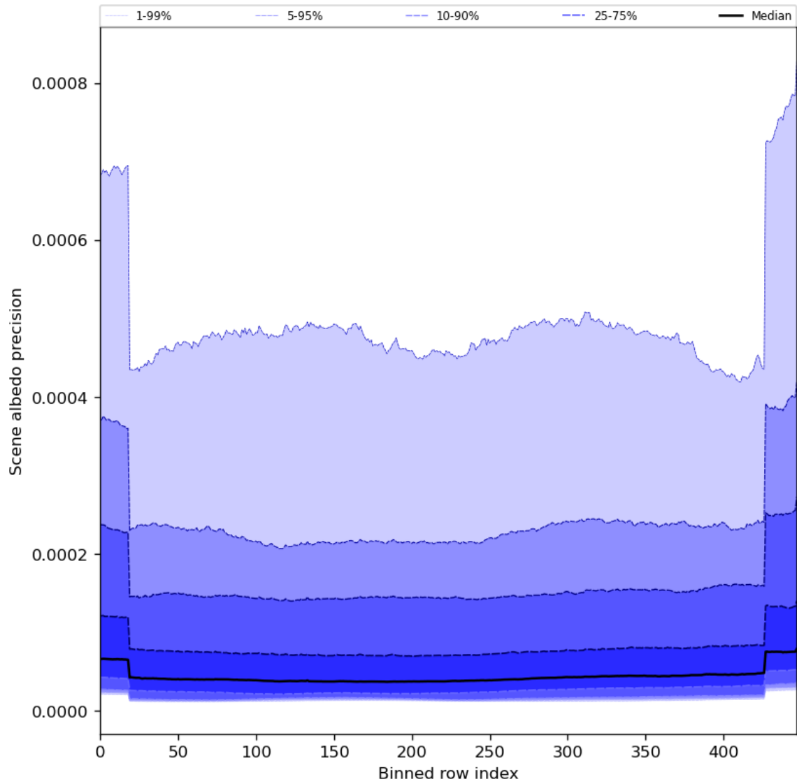
Figure 52: Along track statistics of “Scene albedo precision” for 2024-03-21 to 2024-03-22
