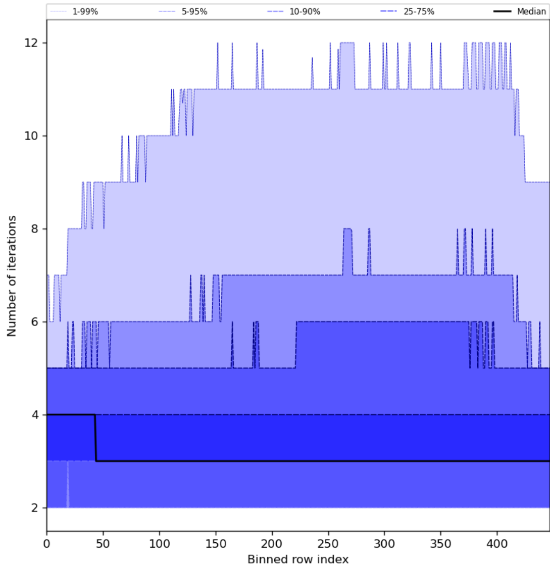
Figure 56: Along track statistics of “Number of iterations” for 2024-03-21 to 2024-03-22
