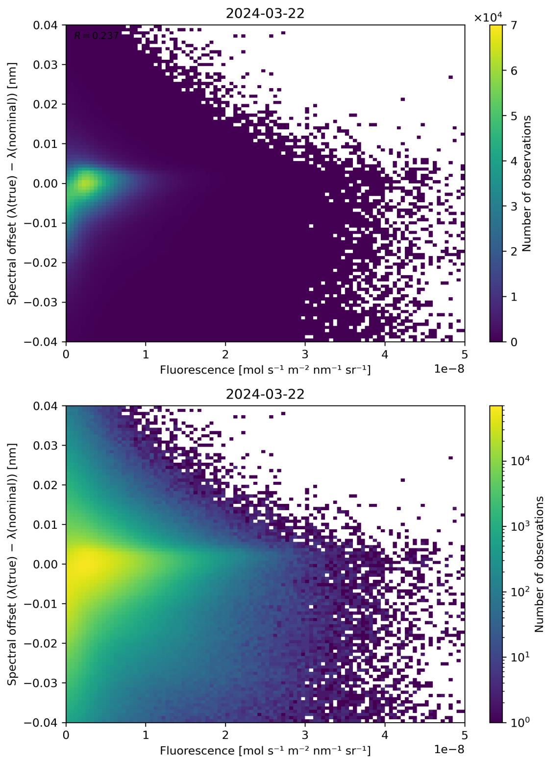
Figure 87: Scatter density plot of “Fluorescence” against “Spectral offset ( \lambda(\text{true}) - \lambda(\text{nominal}) )” for 2024-03-21 to 2024-03-22.
