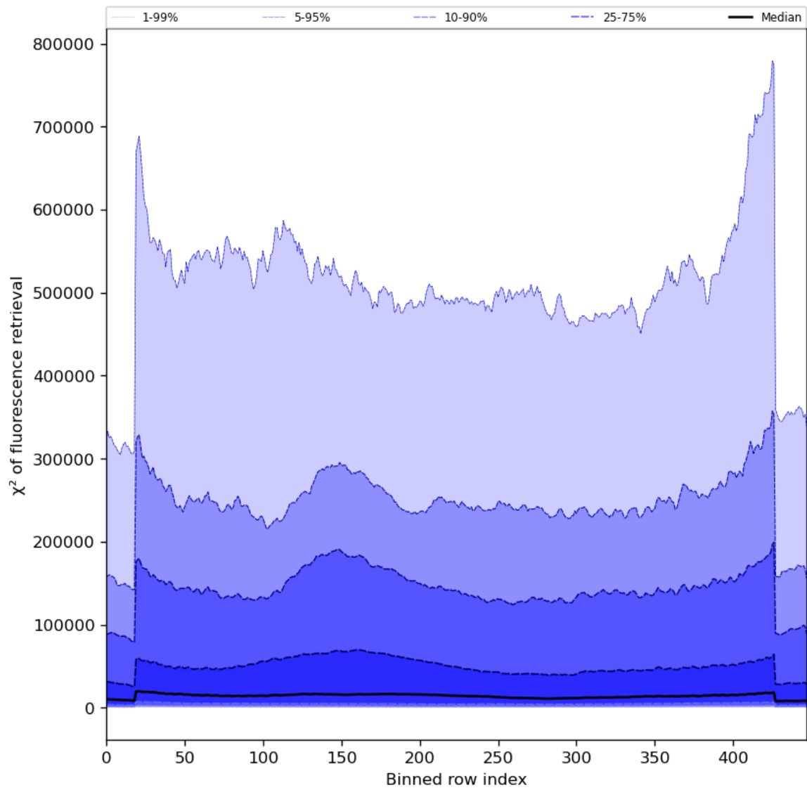
Figure 59: Along track statistics of " \chi^2 of fluorescence retrieval" for 2024-03-21 to 2024-03-22
