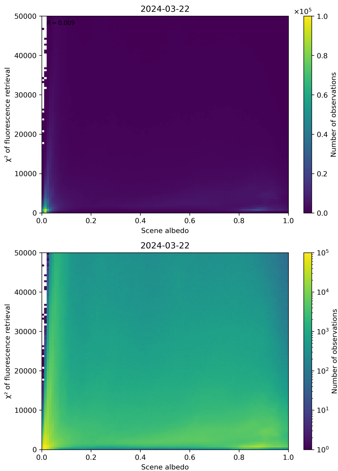
Figure 103: Scatter density plot of “Scene albedo” against “ \chi^2 of fluorescence retrieval” for 2024-03-21 to 2024-03-22.
