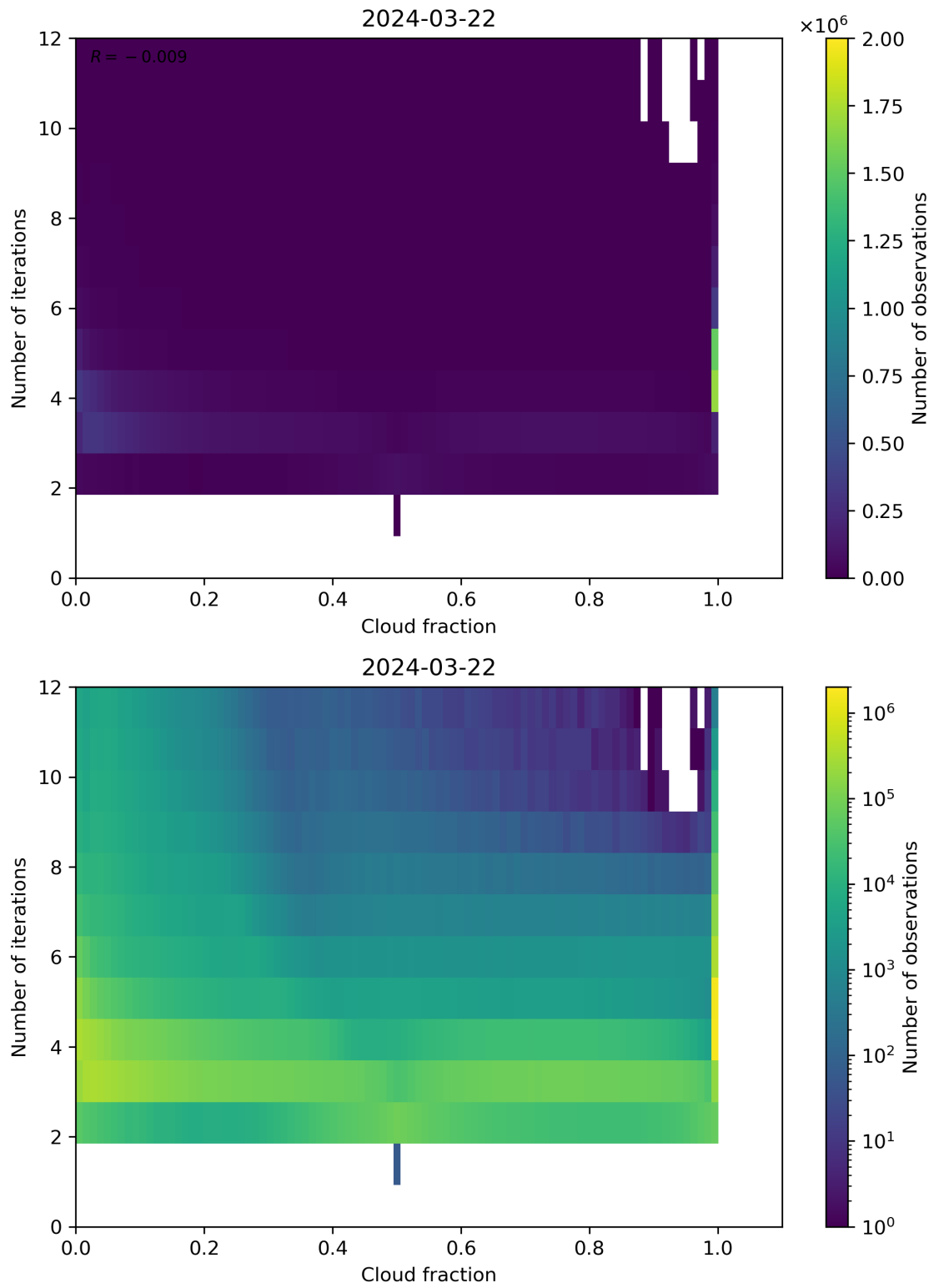
Figure 73: Scatter density plot of “Cloud fraction” against “Number of iterations” for 2024-03-21 to 2024-03-22.
