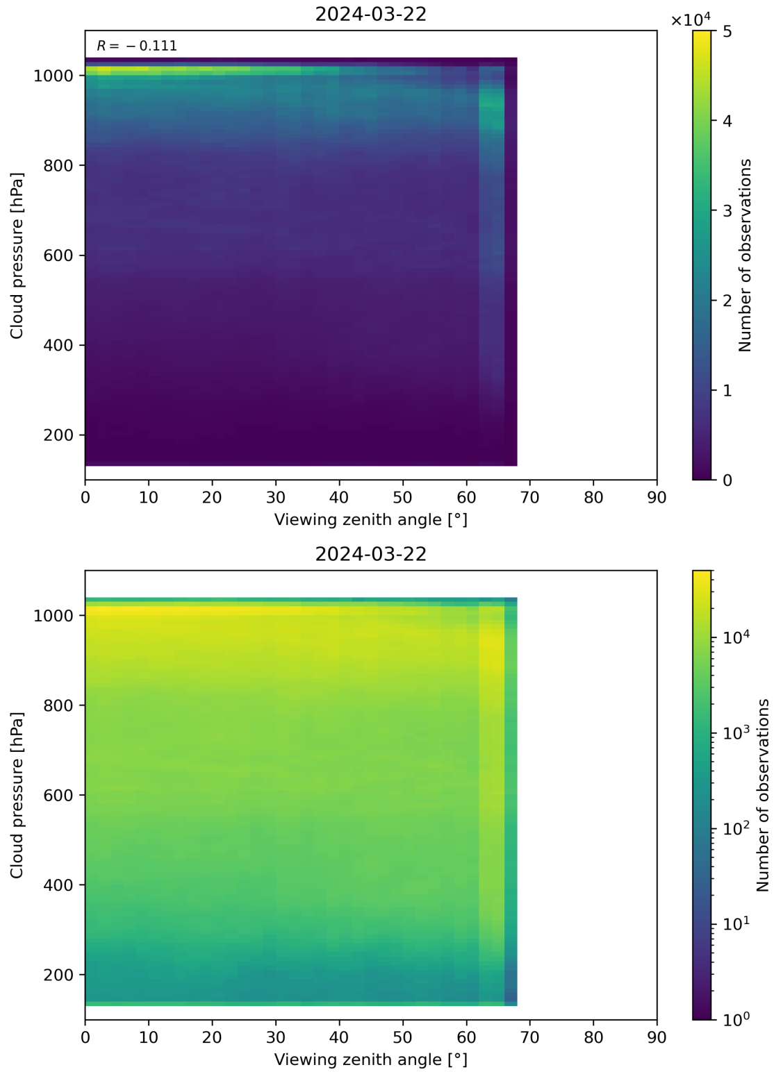
Figure 121: Scatter density plot of “Viewing zenith angle” against “Cloud pressure” for 2024-03-21 to 2024-03-22.
