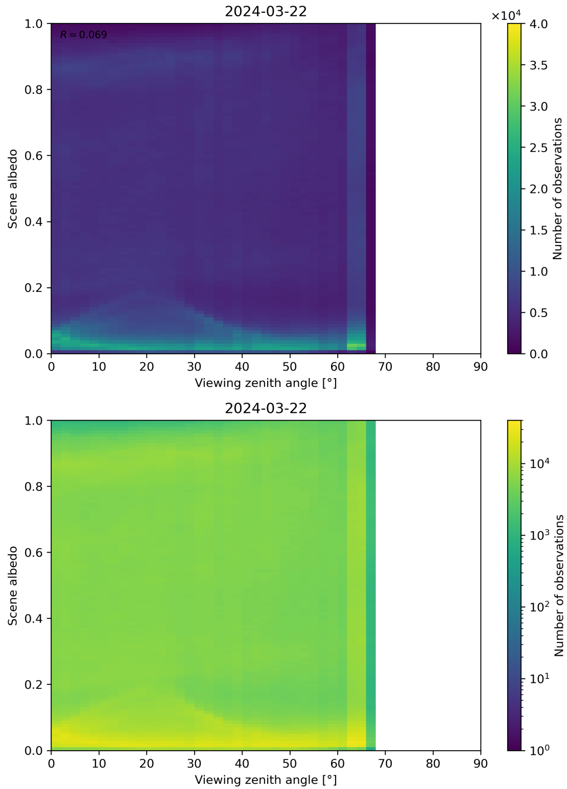
Figure 126: Scatter density plot of “Viewing zenith angle” against “Scene albedo” for 2024-03-21 to 2024-03-22.
