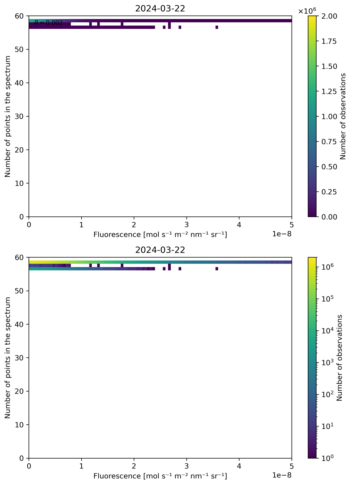
Figure 86: Scatter density plot of “Fluorescence” against “Number of points in the spectrum” for 2024-03-21 to 2024-03-22.
