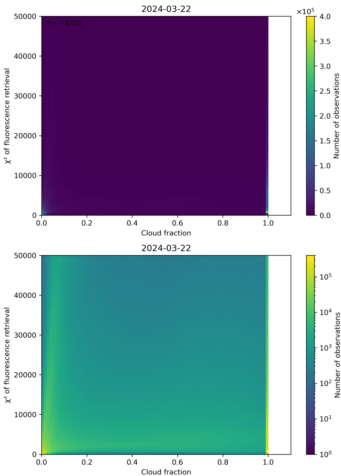
Figure 71: Scatter density plot of “Cloud fraction” against “ \chi^2 of fluorescence retrieval” for 2024-03-21 to 2024-03-22.
