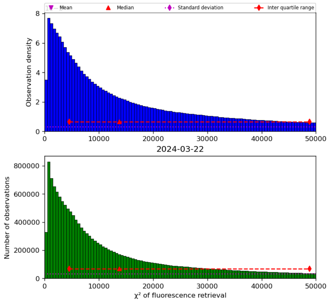
Figure 42: Histogram of “ \chi^2 of fluorescence retrieval” for 2024-03-21 to 2024-03-22
