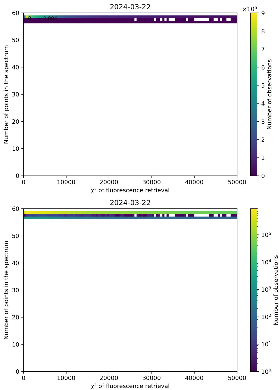
Figure 68: Scatter density plot of “ \chi^2 of fluorescence retrieval” against “Number of points in the spectrum” for 2024-03-21 to 2024-03-22.
