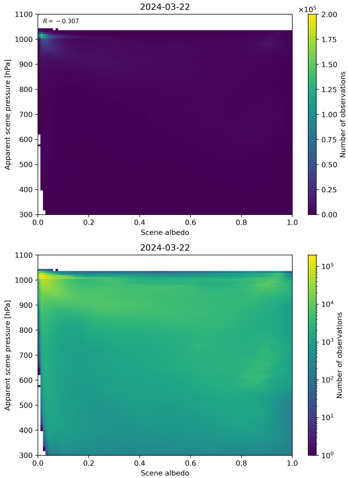
Figure 102: Scatter density plot of “Scene albedo” against “Apparent scene pressure” for 2024-03-21 to 2024-03-22.
