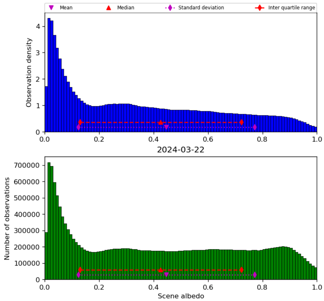
Figure 34: Histogram of “Scene albedo” for 2024-03-21 to 2024-03-22
