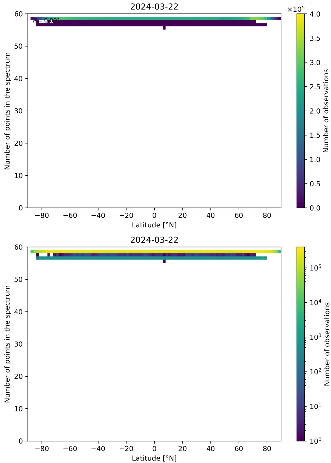
Figure 94: Scatter density plot of “Latitude” against “Number of points in the spectrum” for 2024-03-21 to 2024-03-22.
