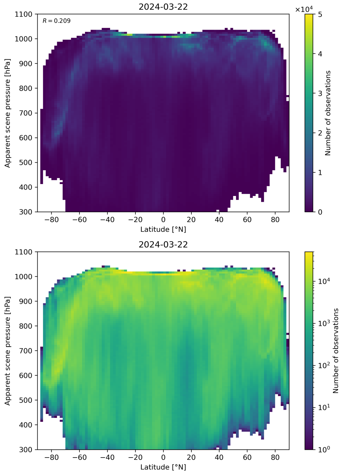
Figure 88: Scatter density plot of “Latitude” against “Apparent scene pressure” for 2024-03-21 to 2024-03-22.
