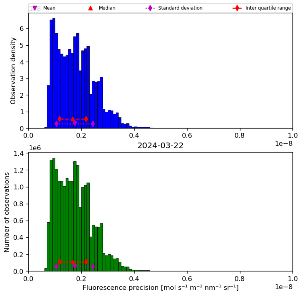
Figure 41: Histogram of “Fluorescence precision” for 2024-03-21 to 2024-03-22
