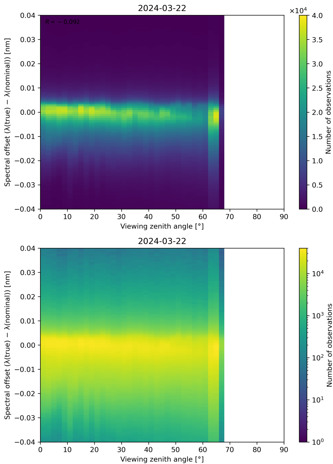
Figure 128: Scatter density plot of “Viewing zenith angle” against “Spectral offset ( \lambda(\text{true}) - \lambda(\text{nominal}) )” for 2024-03-21 to 2024-03-22.
