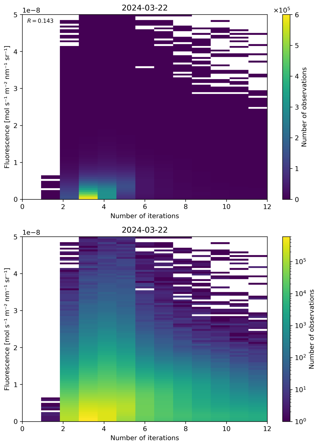
Figure 98: Scatter density plot of “Number of iterations” against “Fluorescence” for 2024-03-21 to 2024-03-22.
