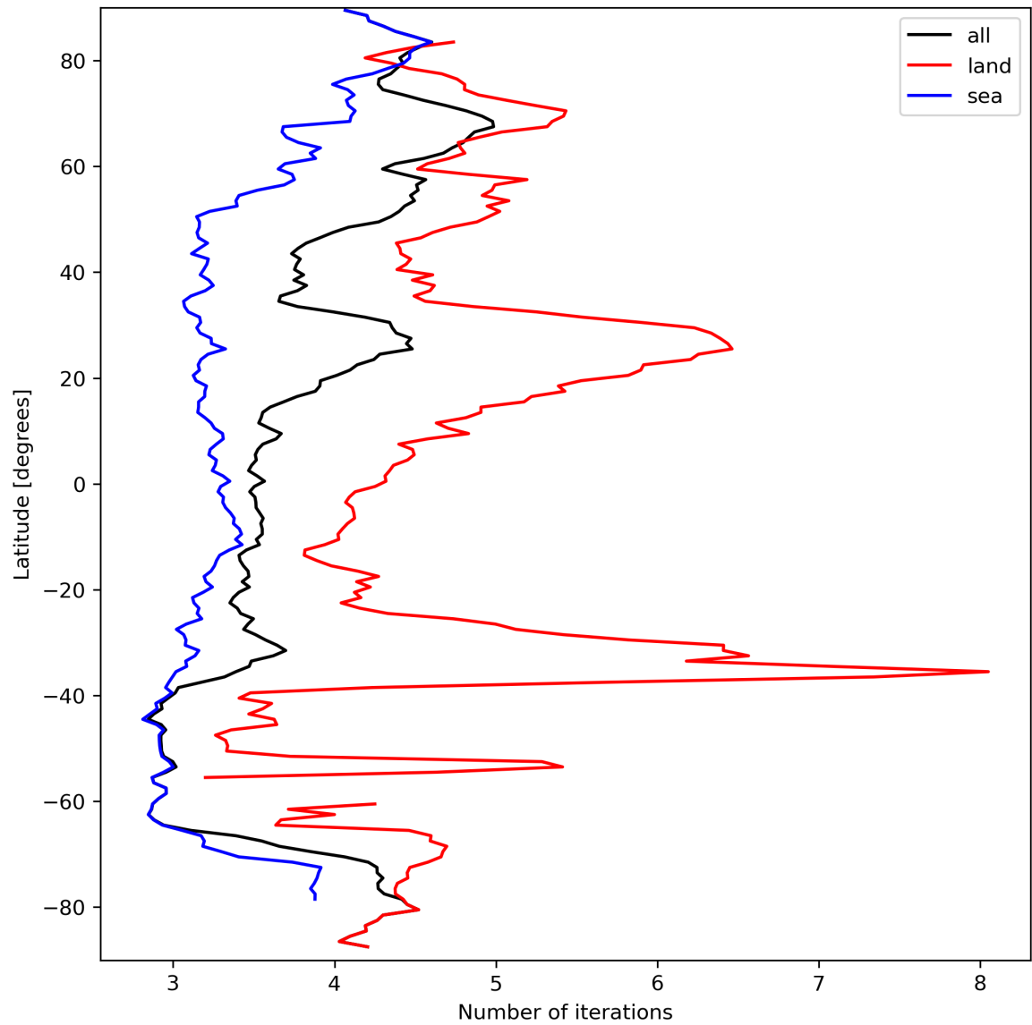
Figure 22: Zonal average of “Number of iterations” for 2024-03-21 to 2024-03-22.
