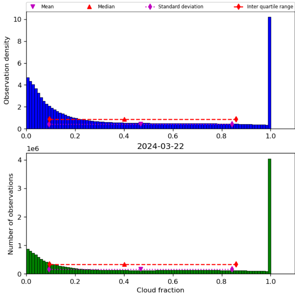
Figure 32: Histogram of “Cloud fraction” for 2024-03-21 to 2024-03-22
