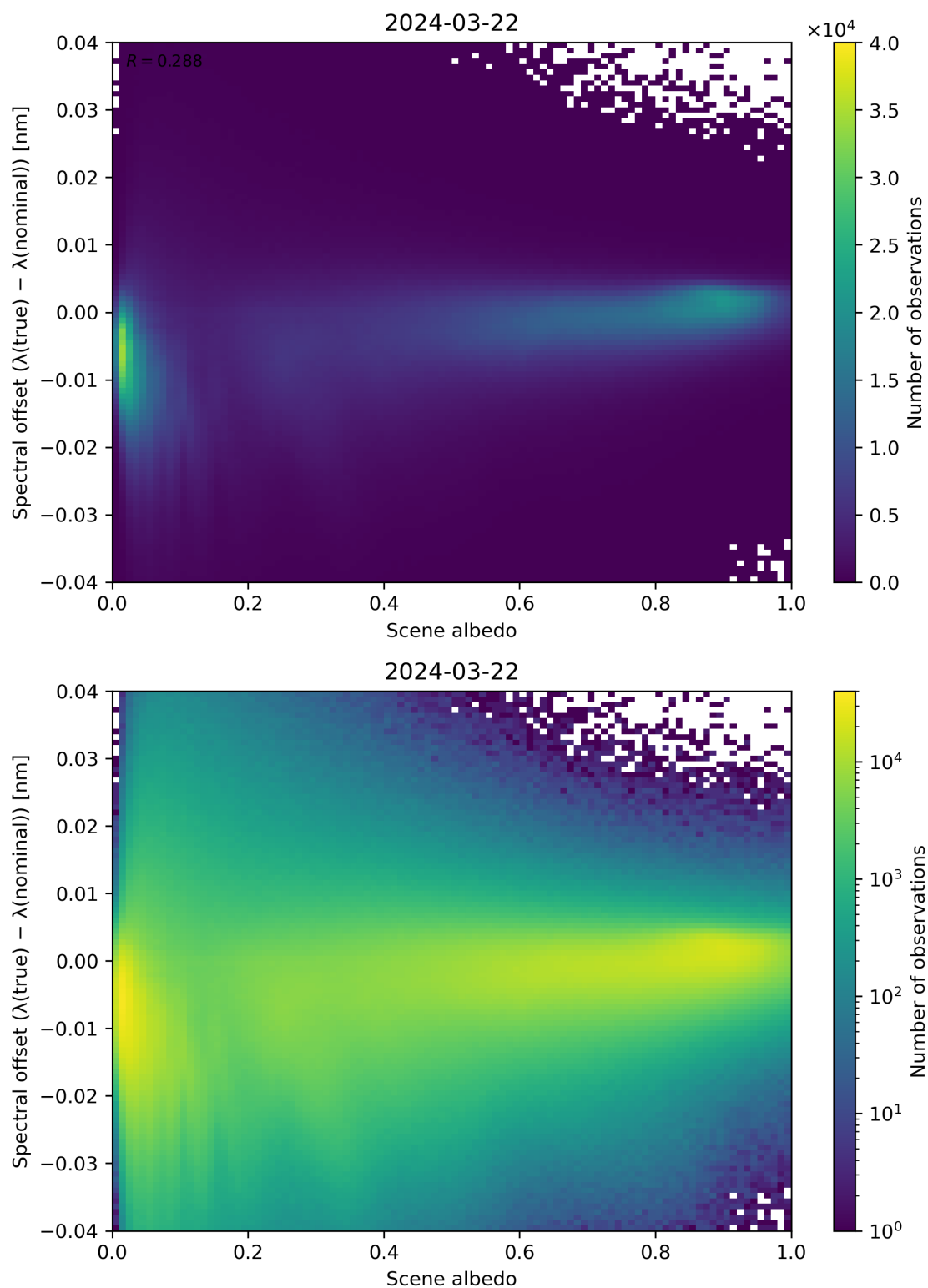
Figure 107: Scatter density plot of “Scene albedo” against “Spectral offset ( \lambda(\text{true}) - \lambda(\text{nominal}) )” for 2024-03-21 to 2024-03-22.
