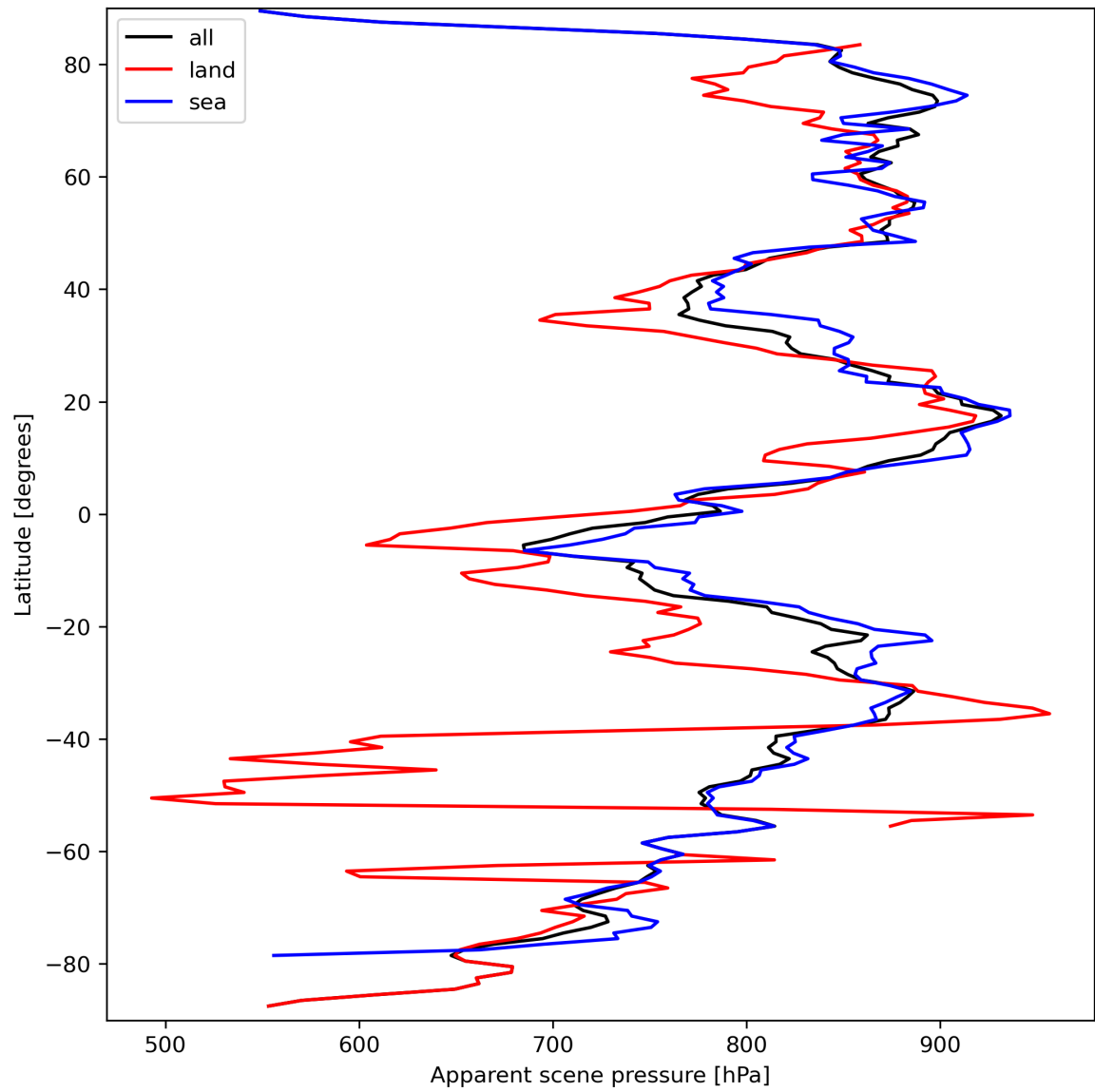
Figure 19: Zonal average of “Apparent scene pressure” for 2024-03-21 to 2024-03-22.
