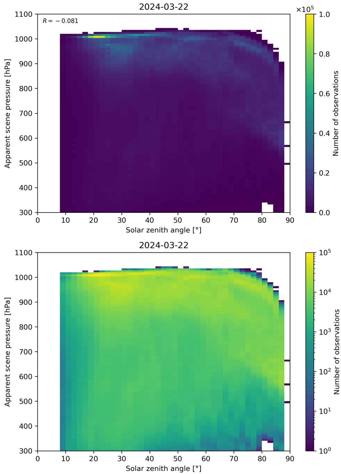
Figure 108: Scatter density plot of “Solar zenith angle” against “Apparent scene pressure” for 2024-03-21 to 2024-03-22.
