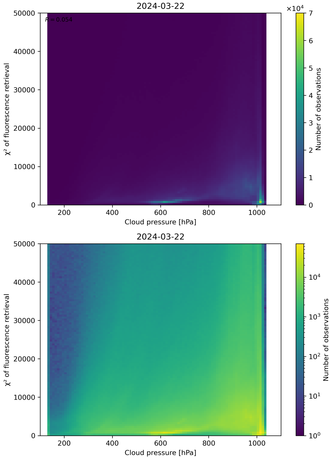
Figure 78: Scatter density plot of “Cloud pressure” against “ \chi^2 of fluorescence retrieval” for 2024-03-21 to 2024-03-22.
