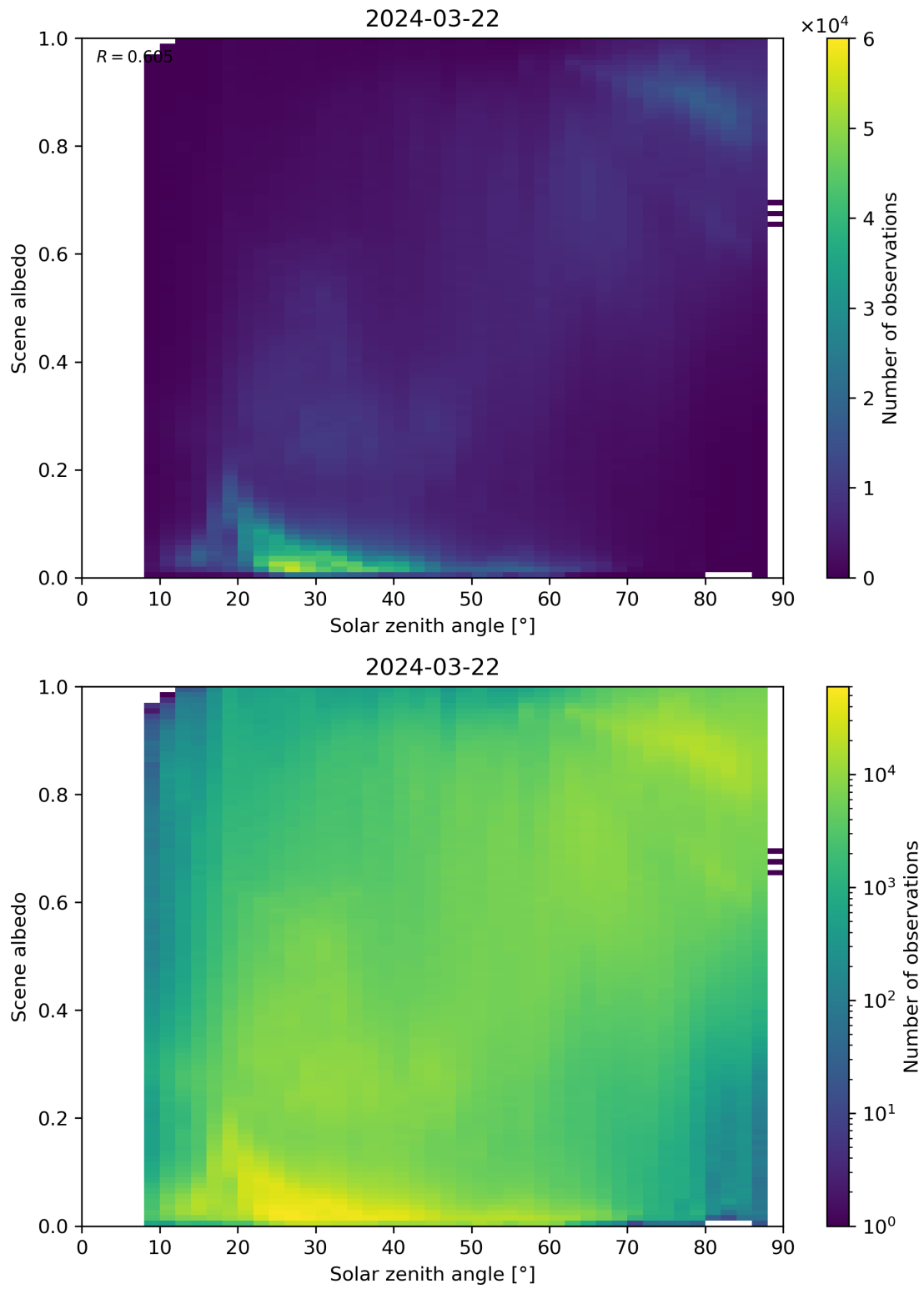
Figure 116: Scatter density plot of “Solar zenith angle” against “Scene albedo” for 2024-03-21 to 2024-03-22.
