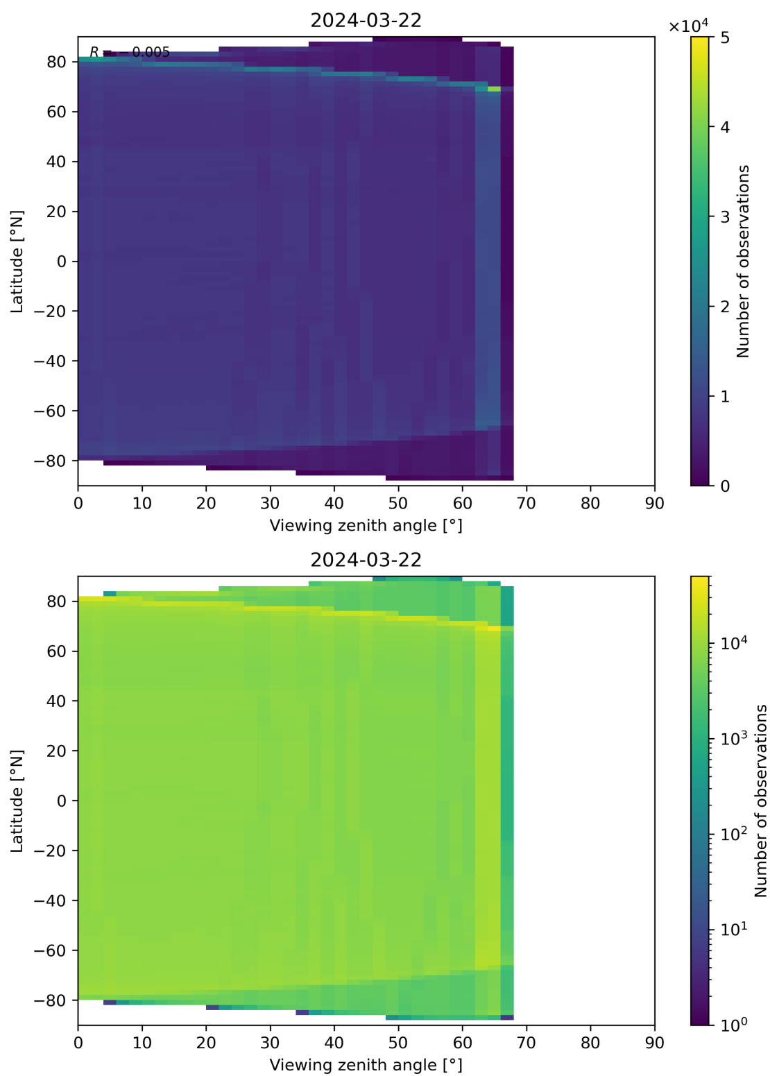
Figure 123: Scatter density plot of “Viewing zenith angle” against “Latitude” for 2024-03-21 to 2024-03-22.
