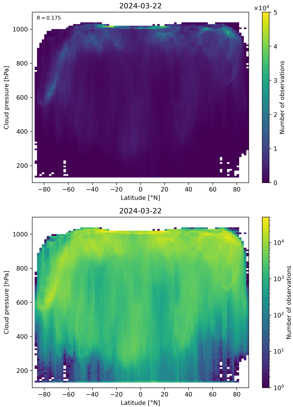
Figure 91: Scatter density plot of “Latitude” against “Cloud pressure” for 2024-03-21 to 2024-03-22.
