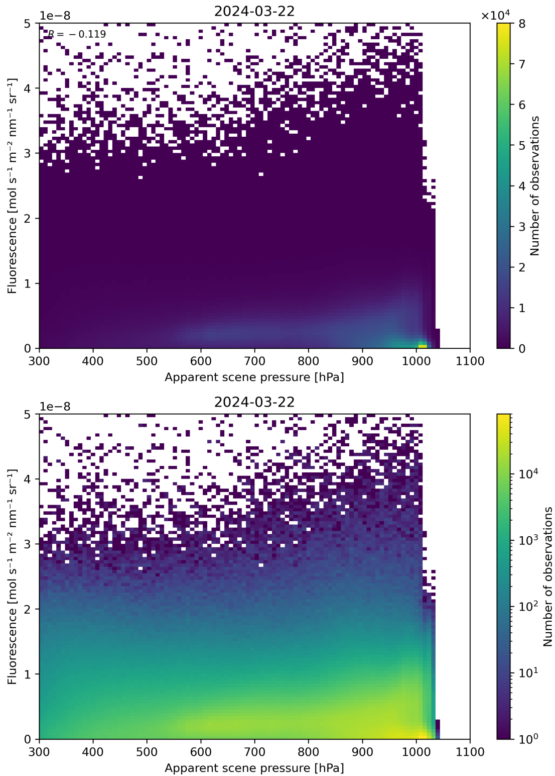
Figure 64: Scatter density plot of “Apparent scene pressure” against “Fluorescence” for 2024-03-21 to 2024-03-22.
