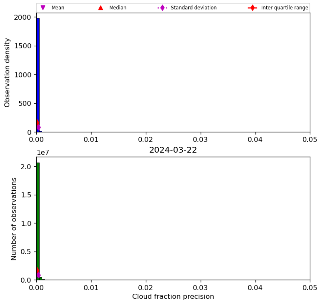
Figure 33: Histogram of “Cloud fraction precision” for 2024-03-21 to 2024-03-22
