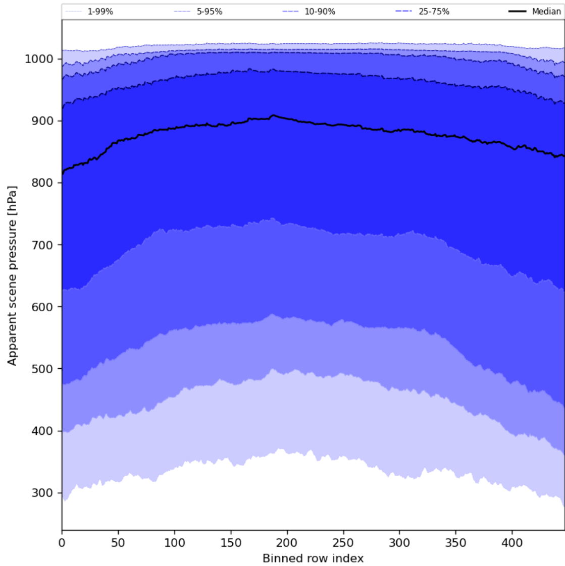
Figure 53: Along track statistics of “Apparent scene pressure” for 2024-03-21 to 2024-03-22
