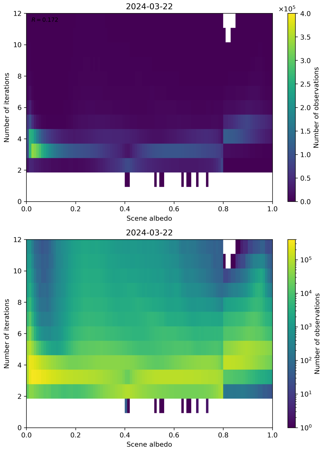
Figure 105: Scatter density plot of “Scene albedo” against “Number of iterations” for 2024-03-21 to 2024-03-22.
