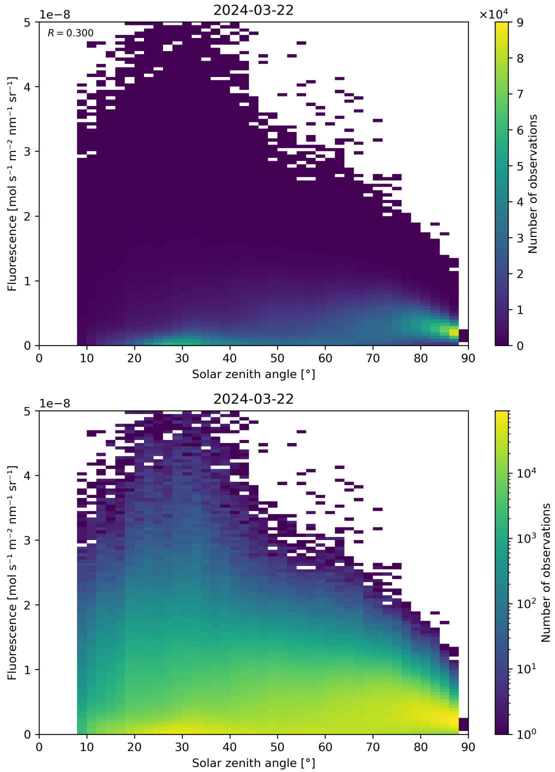
Figure 112: Scatter density plot of “Solar zenith angle” against “Fluorescence” for 2024-03-21 to 2024-03-22.
