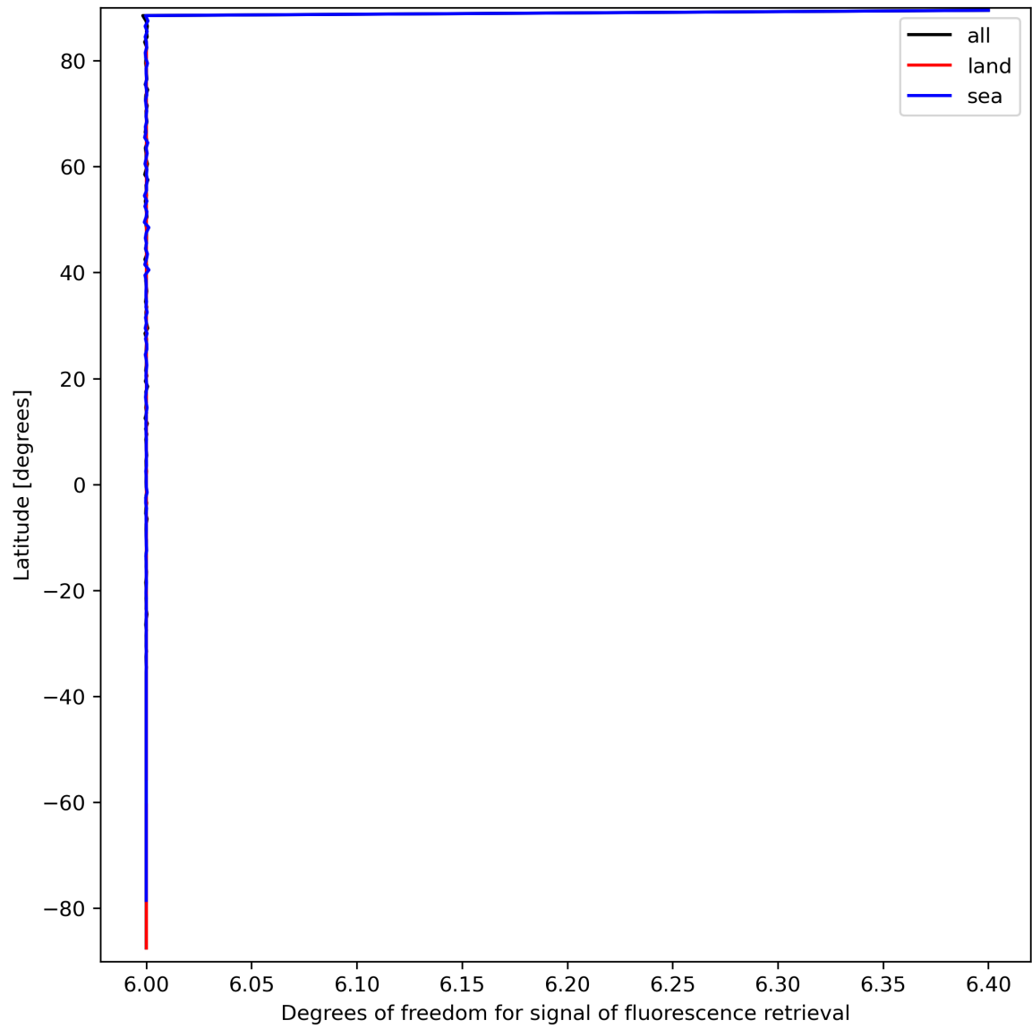
Figure 26: Zonal average of “Degrees of freedom for signal of fluorescence retrieval” for 2024-03-21 to 2024-03-22.
