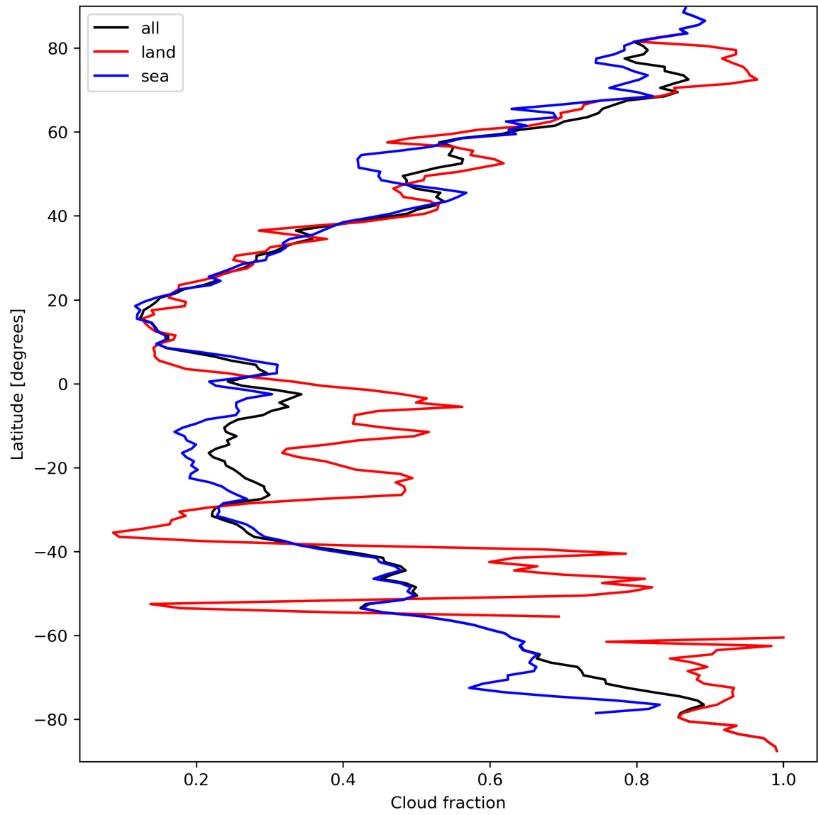
Figure 15: Zonal average of “Cloud fraction” for 2024-03-21 to 2024-03-22.
