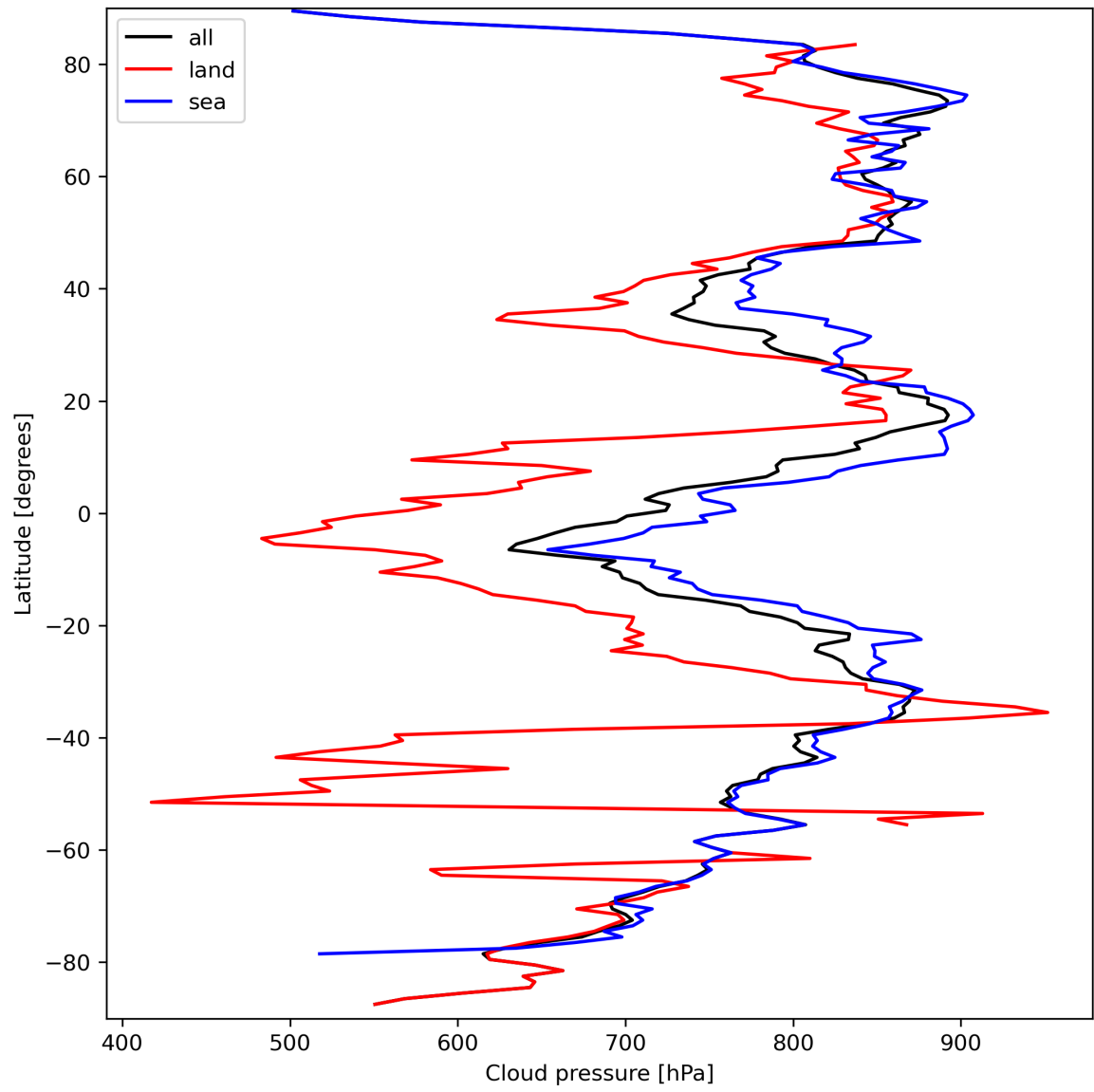
Figure 13: Zonal average of “Cloud pressure” for 2024-03-21 to 2024-03-22.
