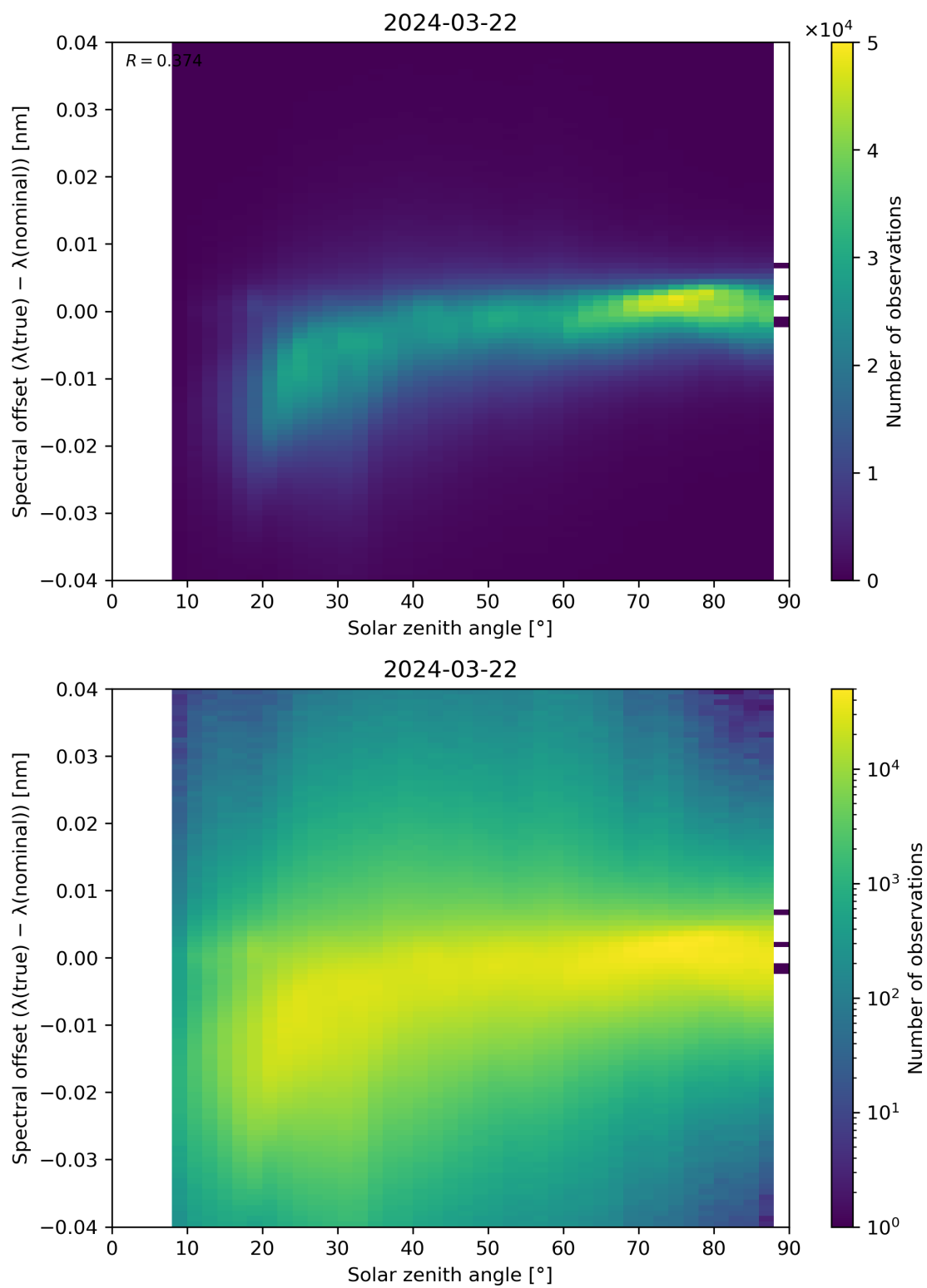
Figure 117: Scatter density plot of “Solar zenith angle” against “Spectral offset ( \lambda(\text{true}) - \lambda(\text{nominal}) )” for 2024-03-21 to 2024-03-22.
