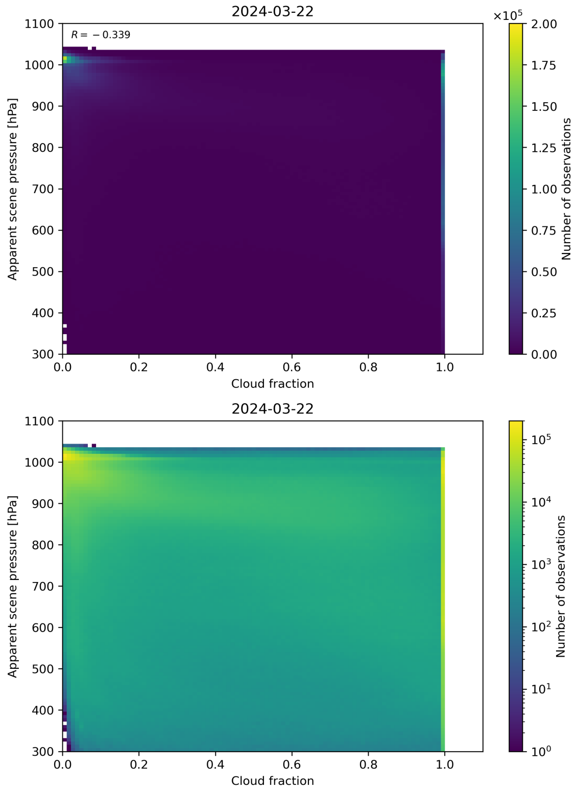
Figure 70: Scatter density plot of “Cloud fraction” against “Apparent scene pressure” for 2024-03-21 to 2024-03-22.
