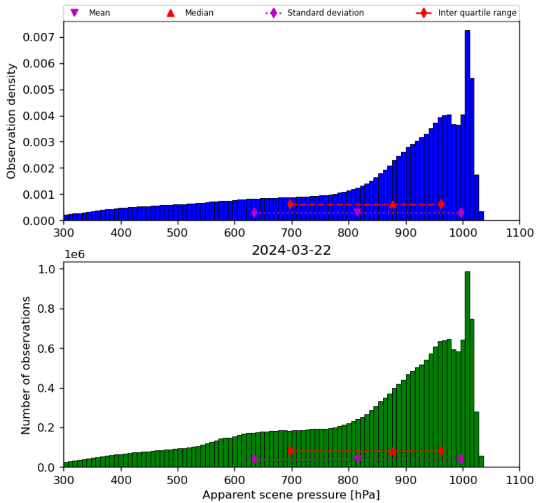
Figure 36: Histogram of “Apparent scene pressure” for 2024-03-21 to 2024-03-22
