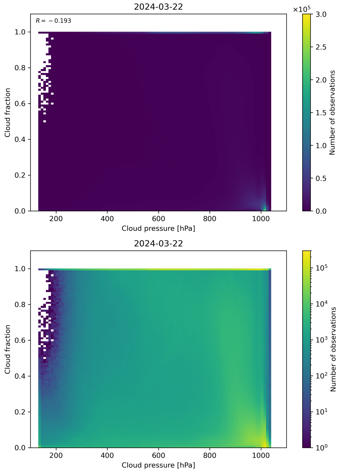
Figure 79: Scatter density plot of “Cloud pressure” against “Cloud fraction” for 2024-03-21 to 2024-03-22.
