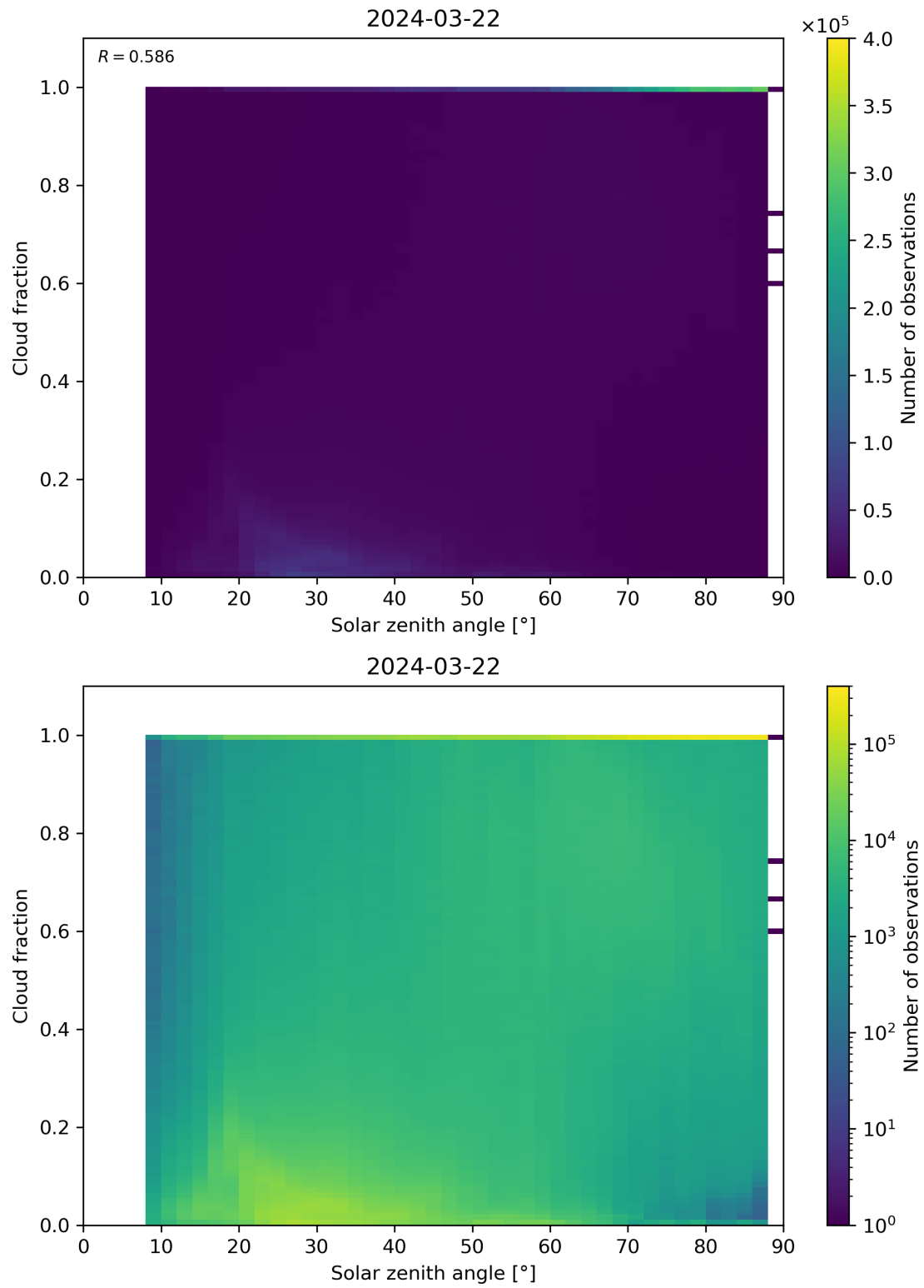
Figure 110: Scatter density plot of “Solar zenith angle” against “Cloud fraction” for 2024-03-21 to 2024-03-22.
