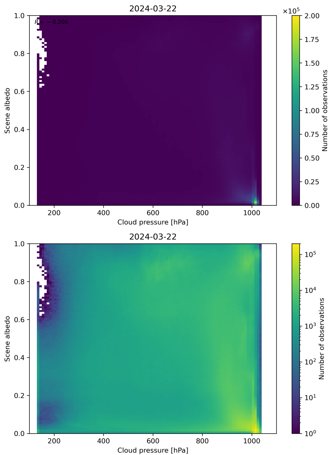
Figure 83: Scatter density plot of “Cloud pressure” against “Scene albedo” for 2024-03-21 to 2024-03-22.
