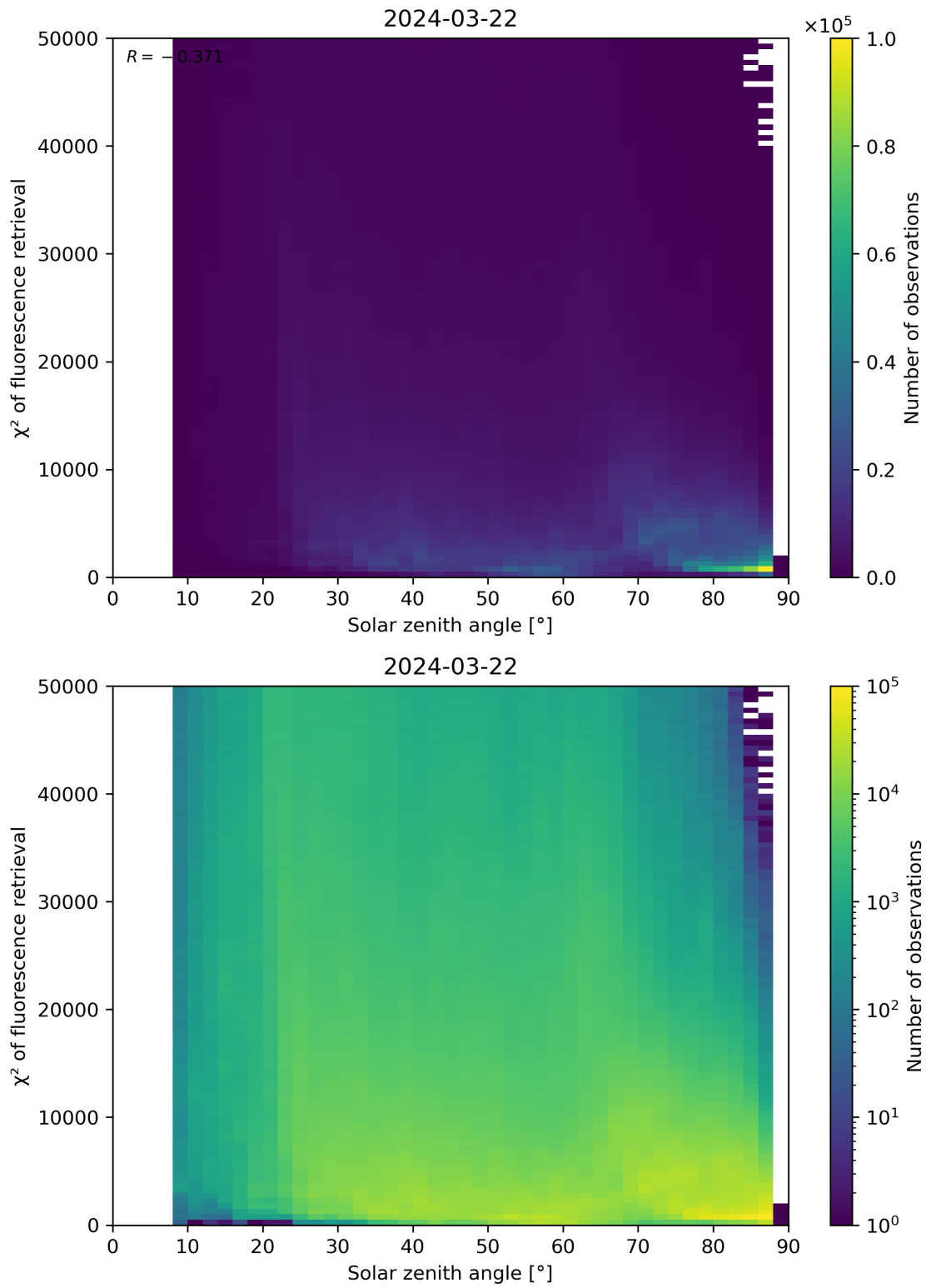
Figure 109: Scatter density plot of “Solar zenith angle” against “ \chi^2 of fluorescence retrieval” for 2024-03-21 to 2024-03-22.
