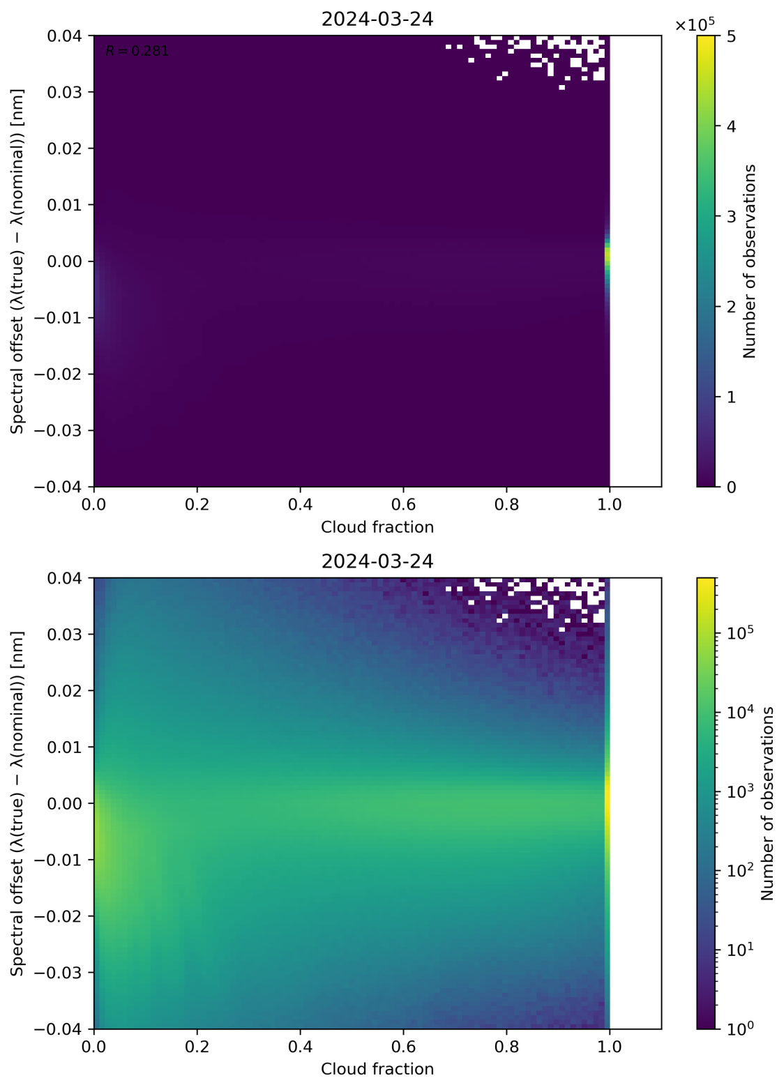
Figure 76: Scatter density plot of “Cloud fraction” against “Spectral offset ( \lambda(\text{true}) - \lambda(\text{nominal}) )” for 2024-03-23 to 2024-03-25.
