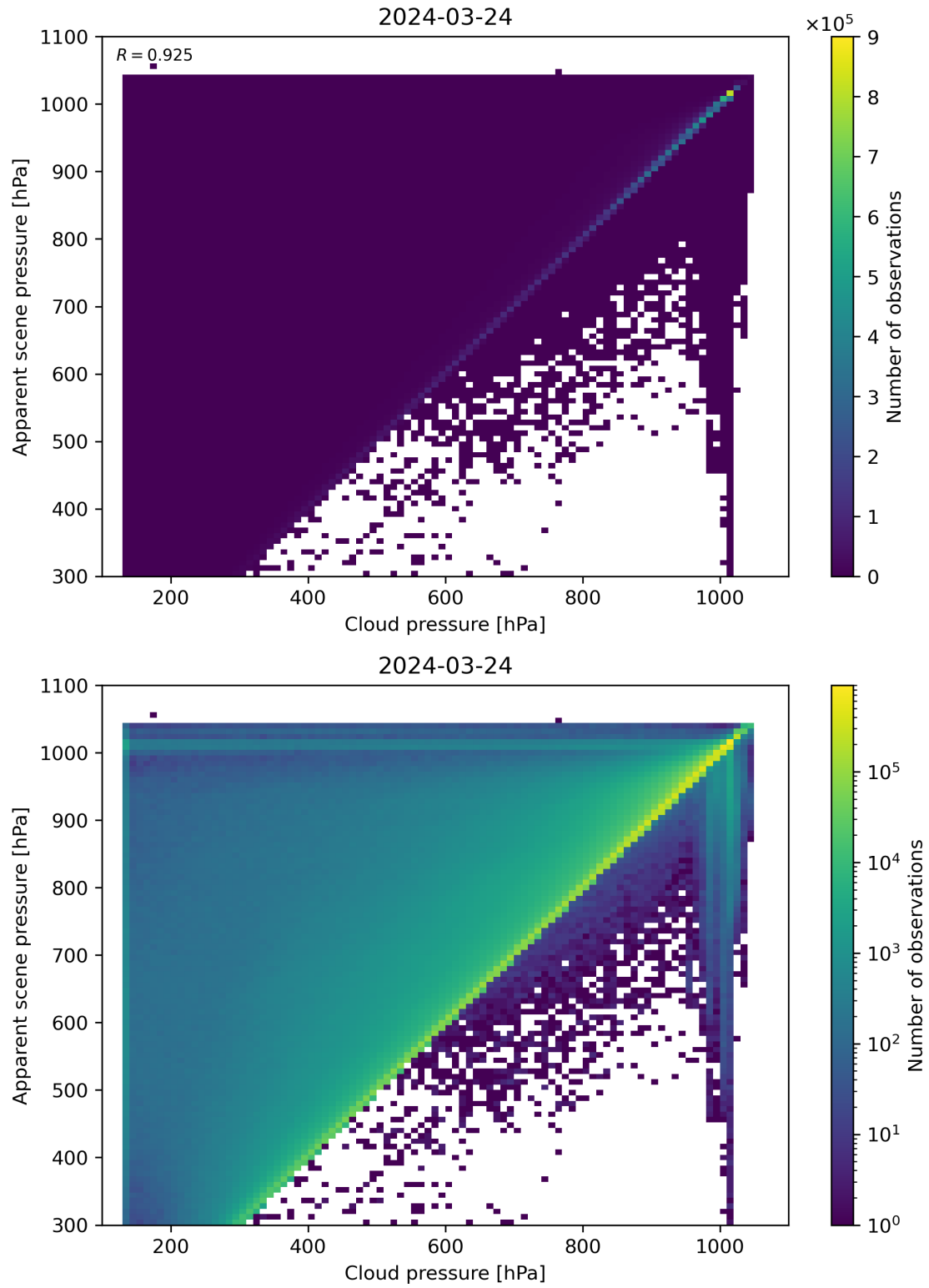
Figure 77: Scatter density plot of “Cloud pressure” against “Apparent scene pressure” for 2024-03-23 to 2024-03-25.
