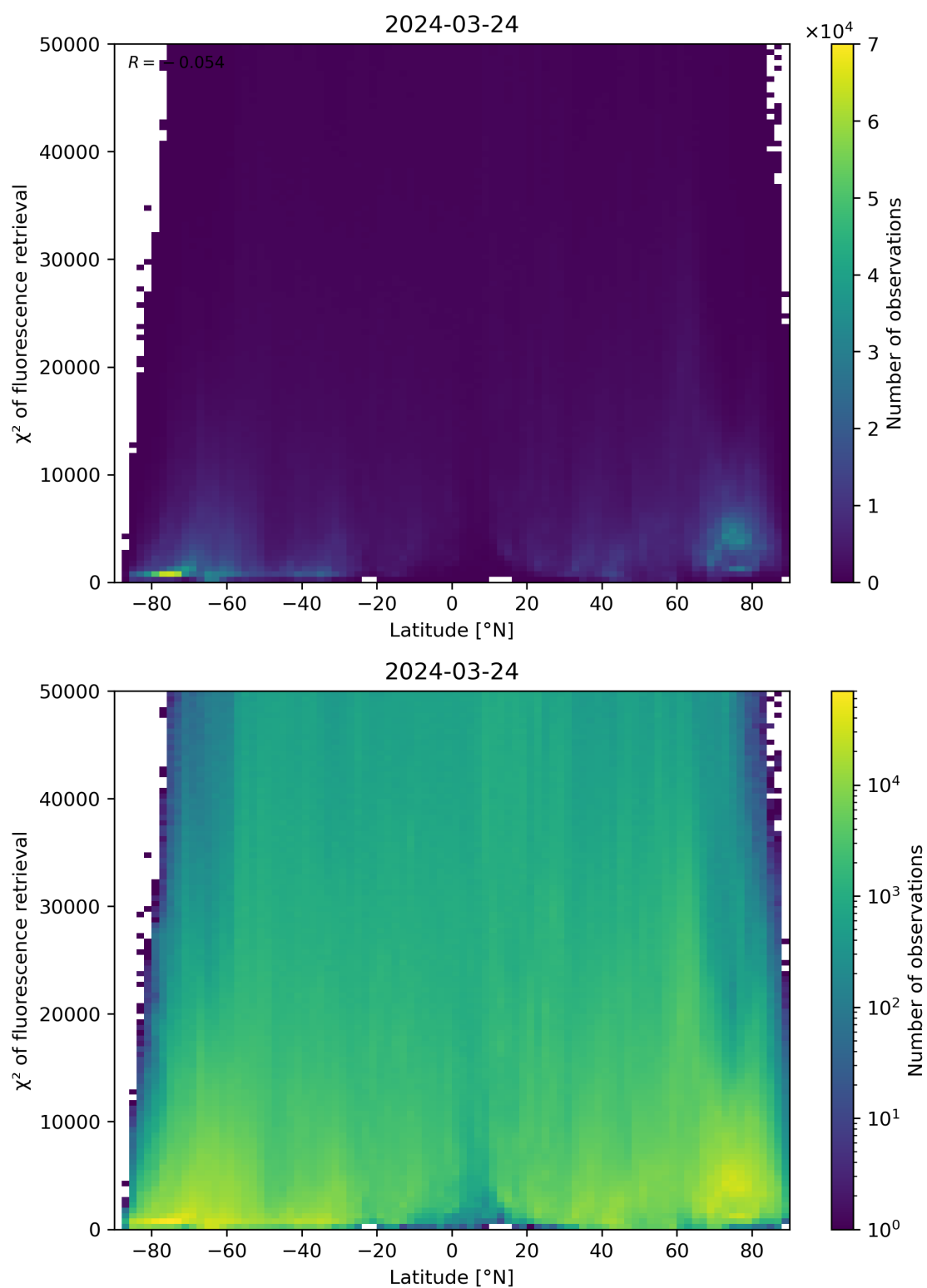
Figure 89: Scatter density plot of “Latitude” against “ \chi^2 of fluorescence retrieval” for 2024-03-23 to 2024-03-25.
