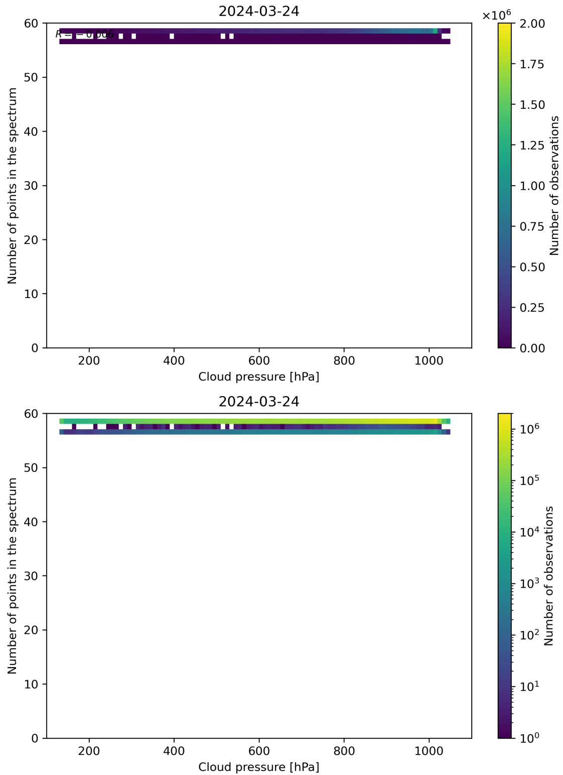
Figure 82: Scatter density plot of “Cloud pressure” against “Number of points in the spectrum” for 2024-03-23 to 2024-03-25.
