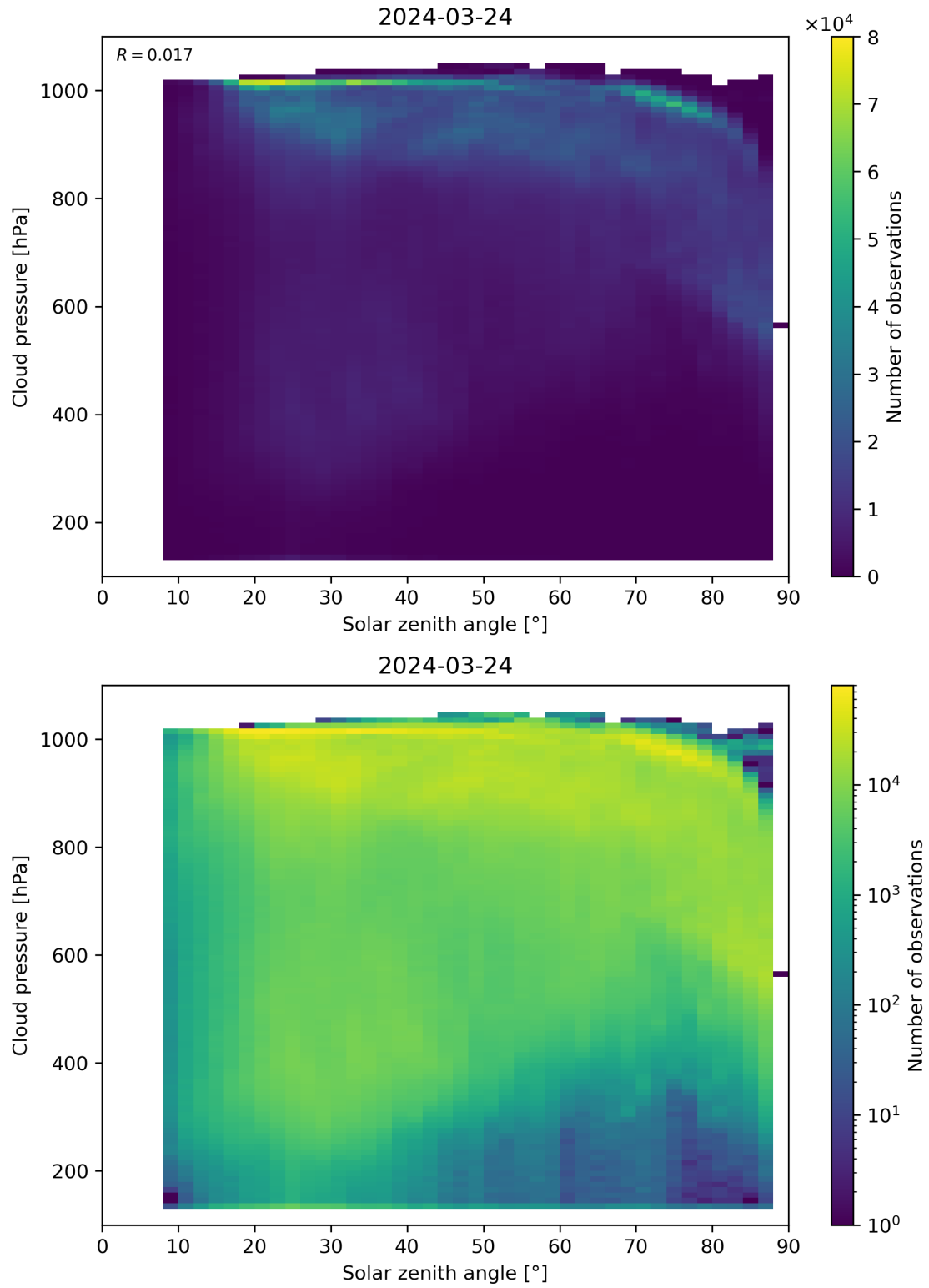
Figure 111: Scatter density plot of “Solar zenith angle” against “Cloud pressure” for 2024-03-23 to 2024-03-25.
