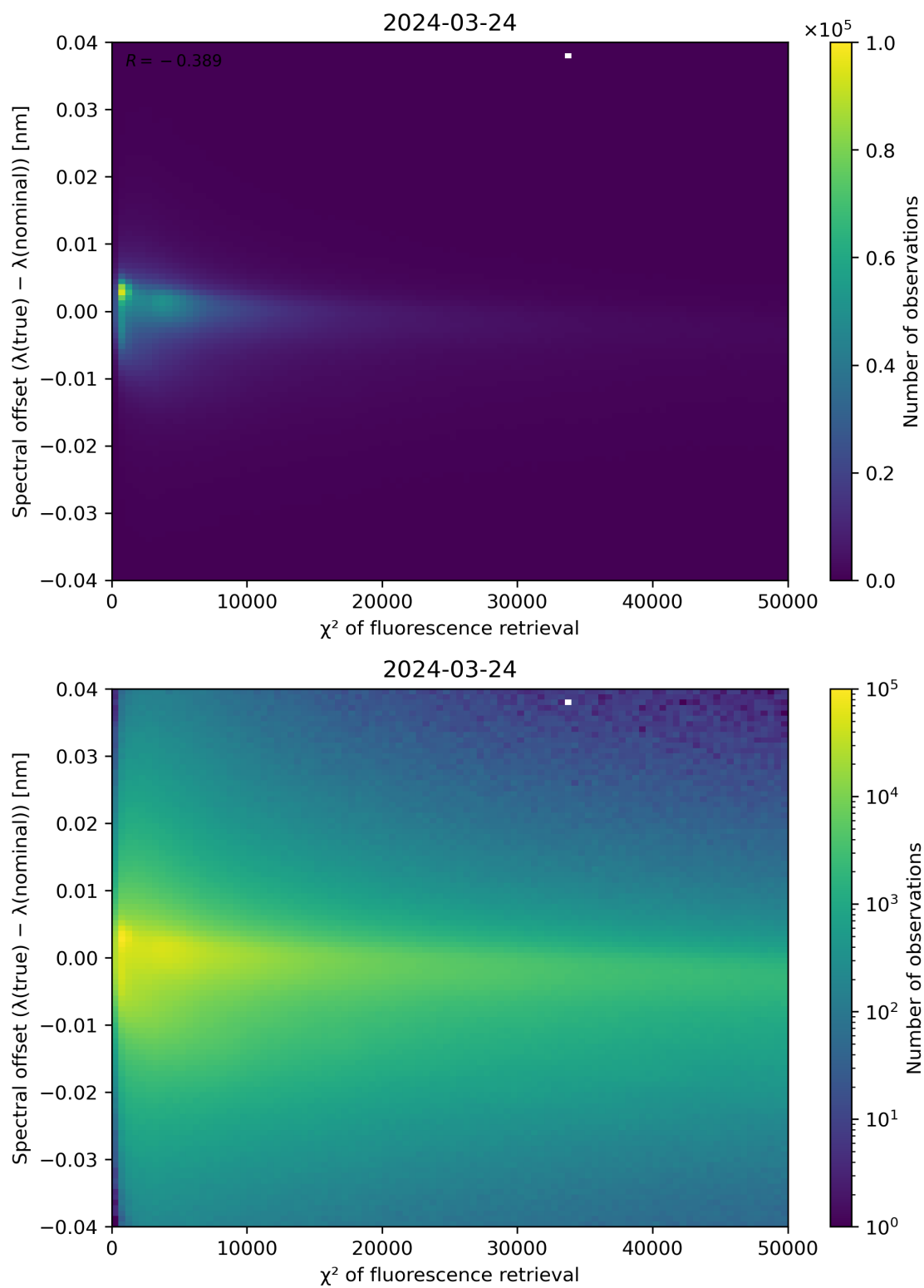
Figure 69: Scatter density plot of " \chi^2 of fluorescence retrieval" against "Spectral offset ( \lambda(\text{true}) - \lambda(\text{nominal}) )" for 2024-03-23 to 2024-03-25.
