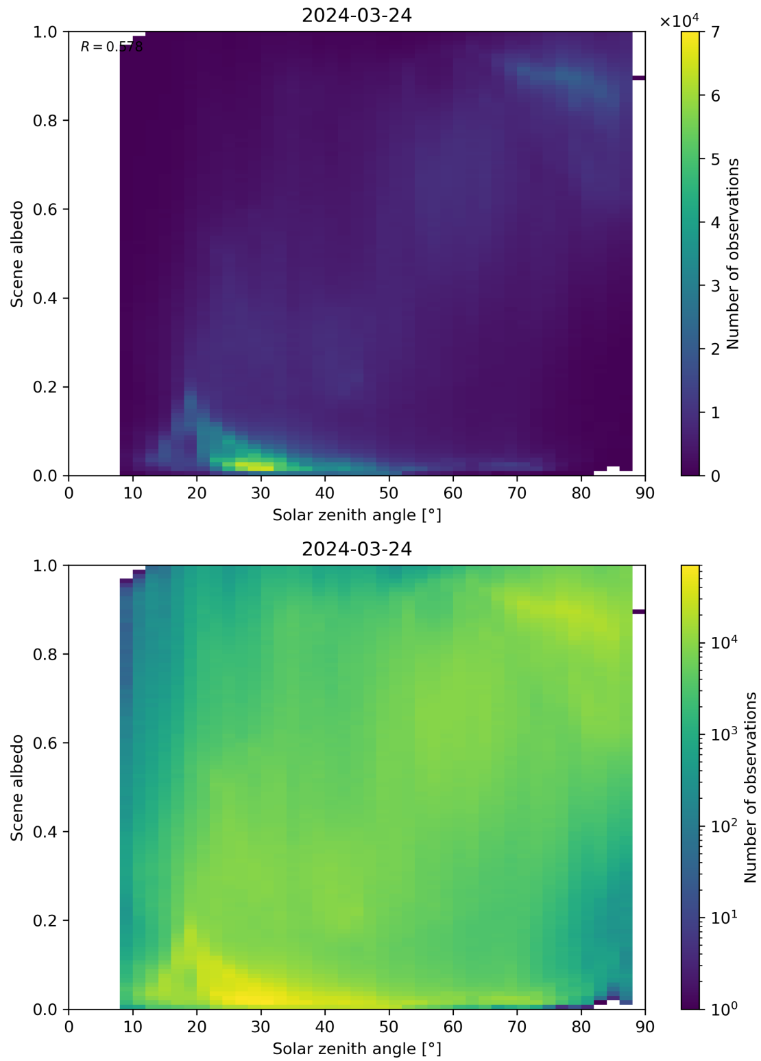
Figure 116: Scatter density plot of “Solar zenith angle” against “Scene albedo” for 2024-03-23 to 2024-03-25.
