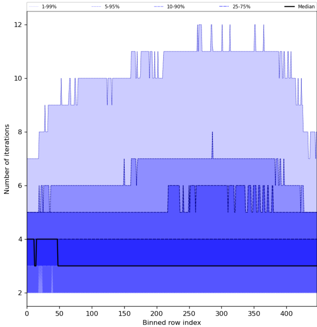
Figure 56: Along track statistics of “Number of iterations” for 2024-03-23 to 2024-03-25
