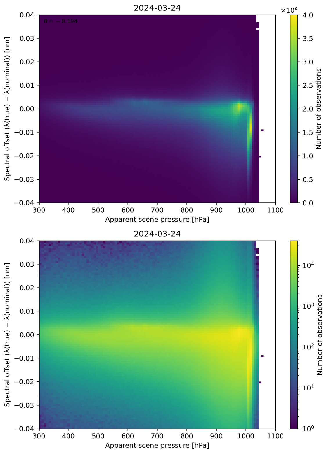
Figure 67: Scatter density plot of “Apparent scene pressure” against “Spectral offset ( \lambda(\text{true}) - \lambda(\text{nominal}) )” for 2024-03-23 to 2024-03-25.
