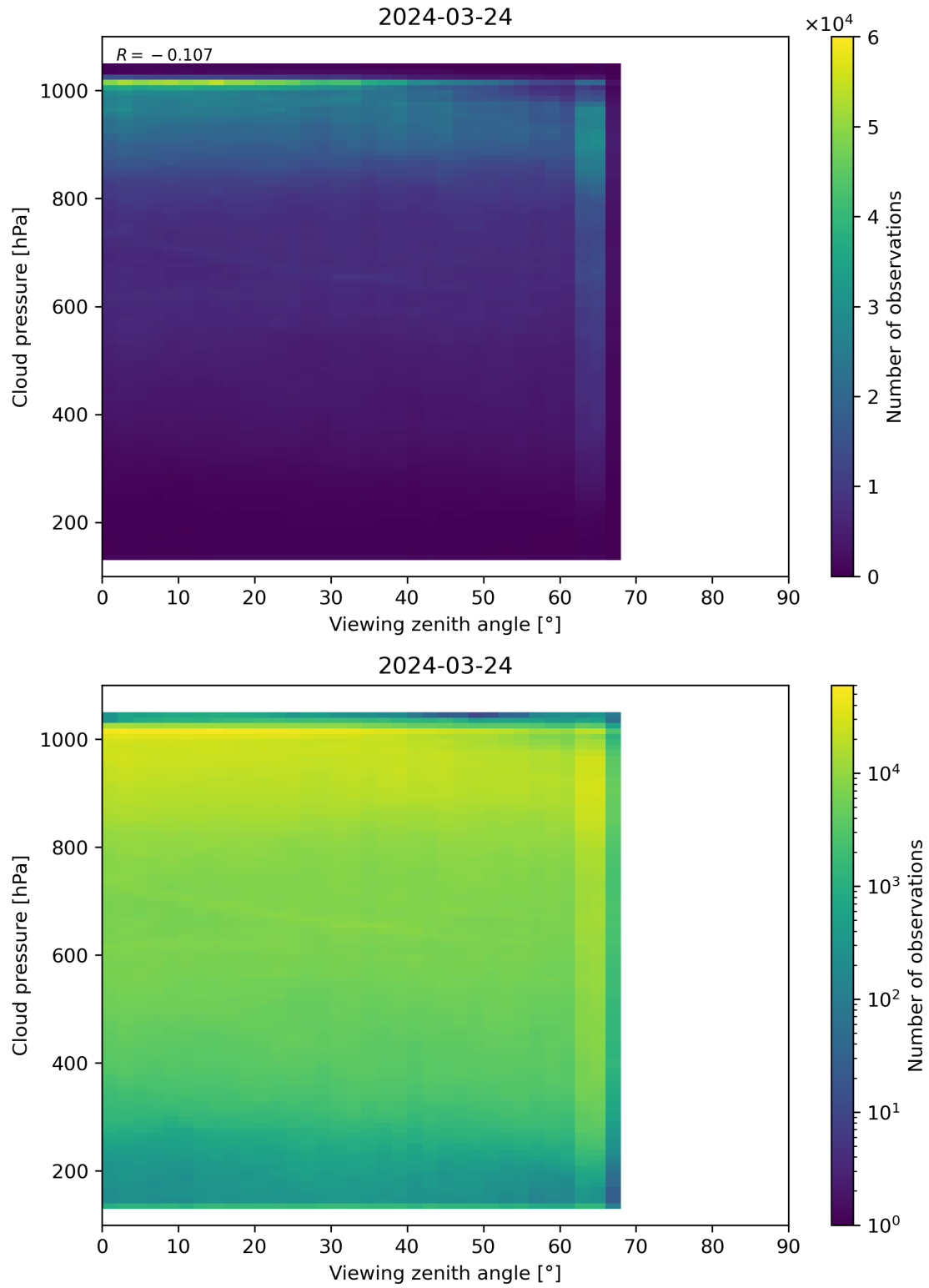
Figure 121: Scatter density plot of “Viewing zenith angle” against “Cloud pressure” for 2024-03-23 to 2024-03-25.
