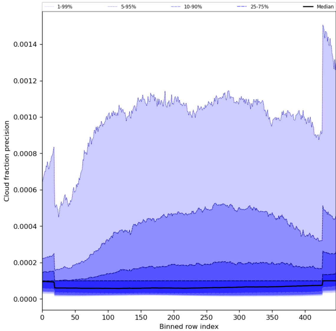
Figure 50: Along track statistics of “Cloud fraction precision” for 2024-03-23 to 2024-03-25
