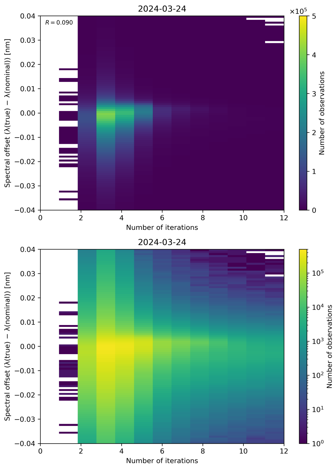
Figure 100: Scatter density plot of “Number of iterations” against “Spectral offset ( \lambda(\text{true}) - \lambda(\text{nominal}) )” for 2024-03-23 to 2024-03-25.
