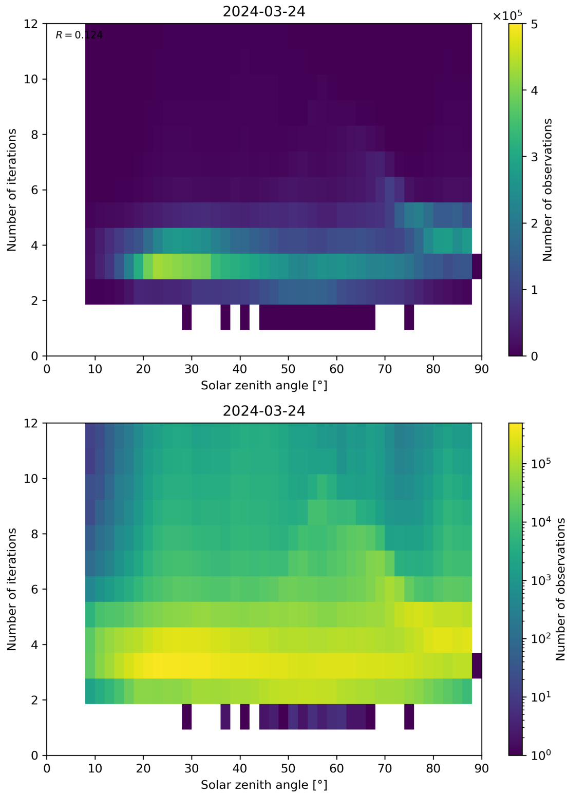
Figure 114: Scatter density plot of “Solar zenith angle” against “Number of iterations” for 2024-03-23 to 2024-03-25.
