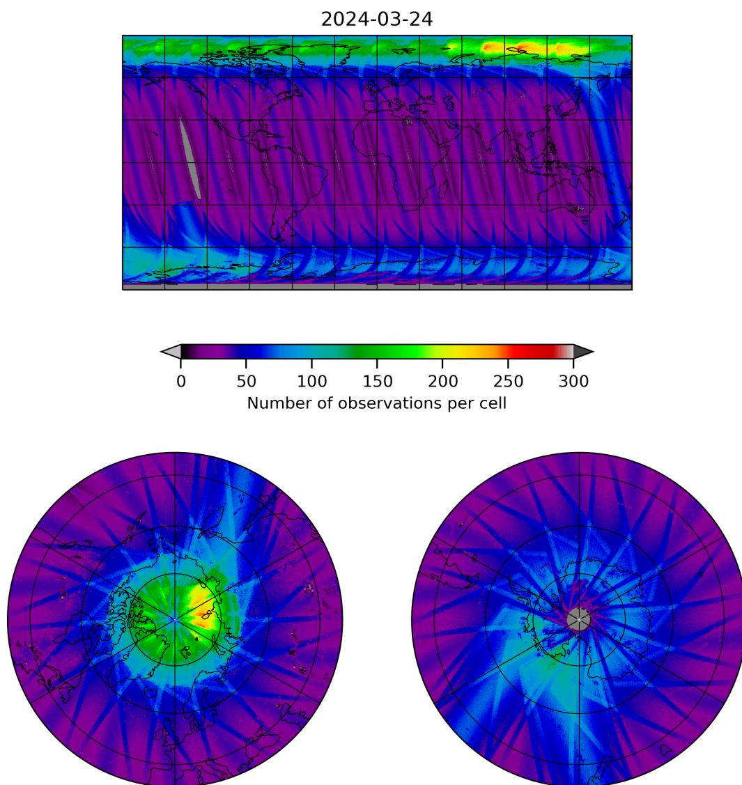
Figure 11: Map of the number of observations for 2024-03-23 to 2024-03-25
