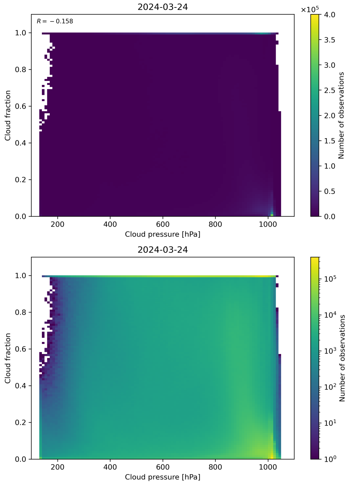
Figure 79: Scatter density plot of “Cloud pressure” against “Cloud fraction” for 2024-03-23 to 2024-03-25.
