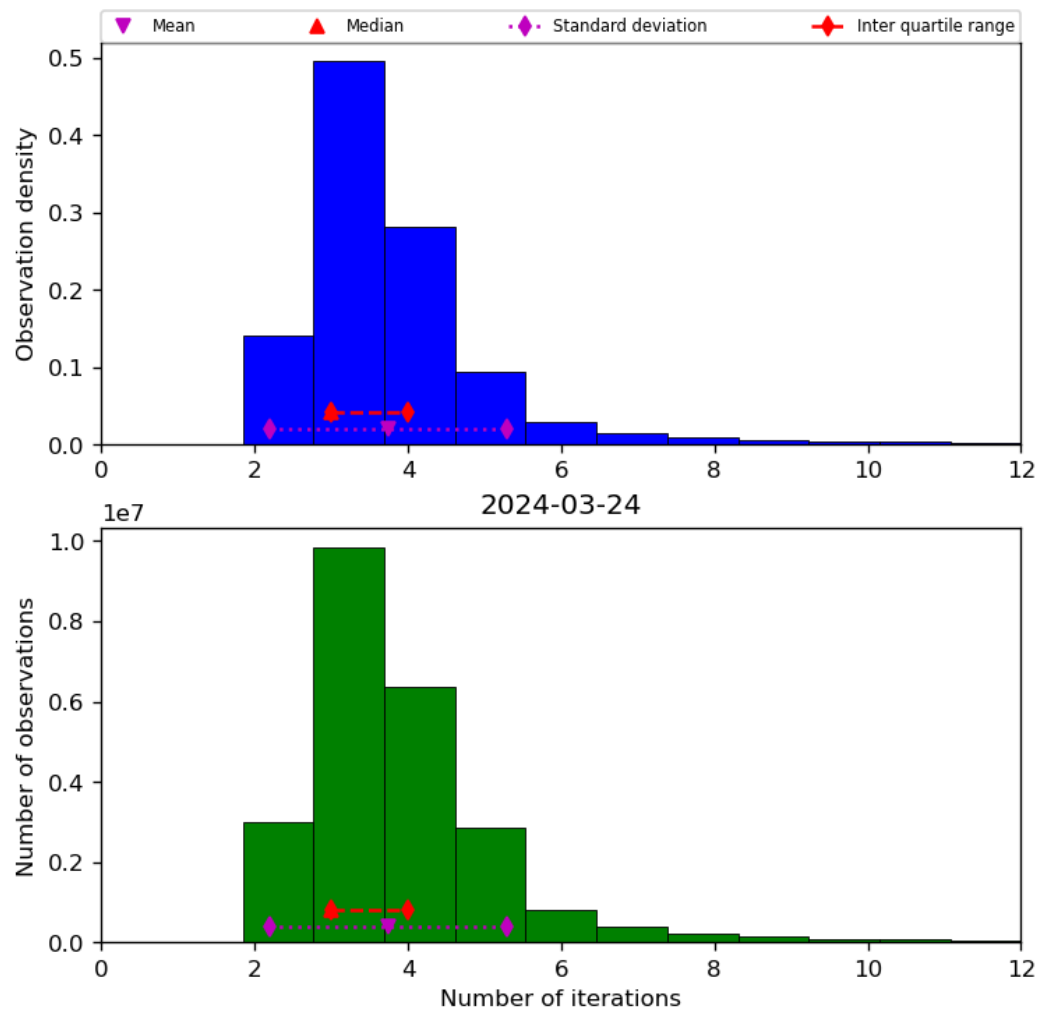
Figure 39: Histogram of “Number of iterations” for 2024-03-23 to 2024-03-25
