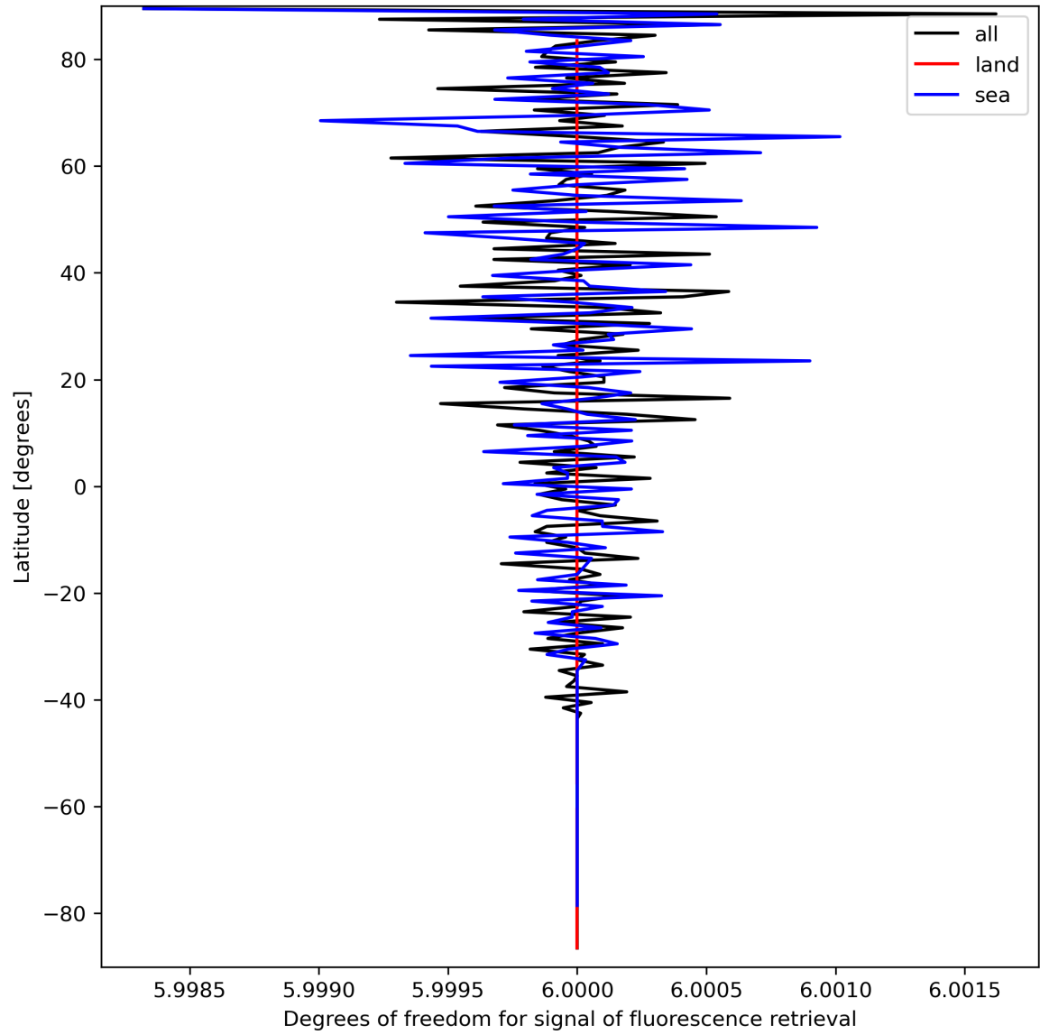
Figure 26: Zonal average of “Degrees of freedom for signal of fluorescence retrieval” for 2024-03-23 to 2024-03-25.
