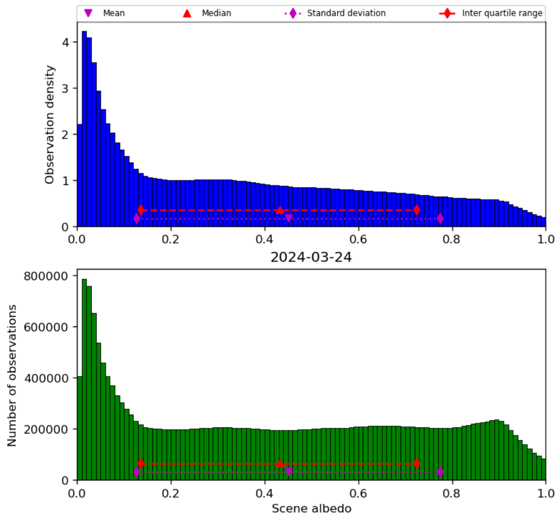
Figure 34: Histogram of “Scene albedo” for 2024-03-23 to 2024-03-25
