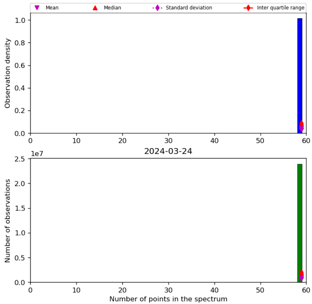
Figure 44: Histogram of “Number of points in the spectrum” for 2024-03-23 to 2024-03-25
