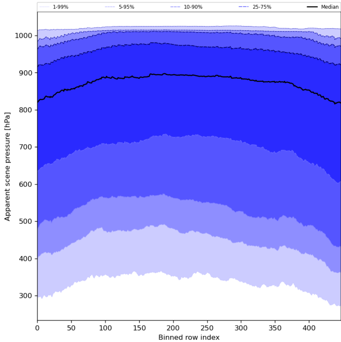
Figure 53: Along track statistics of “Apparent scene pressure” for 2024-03-23 to 2024-03-25
