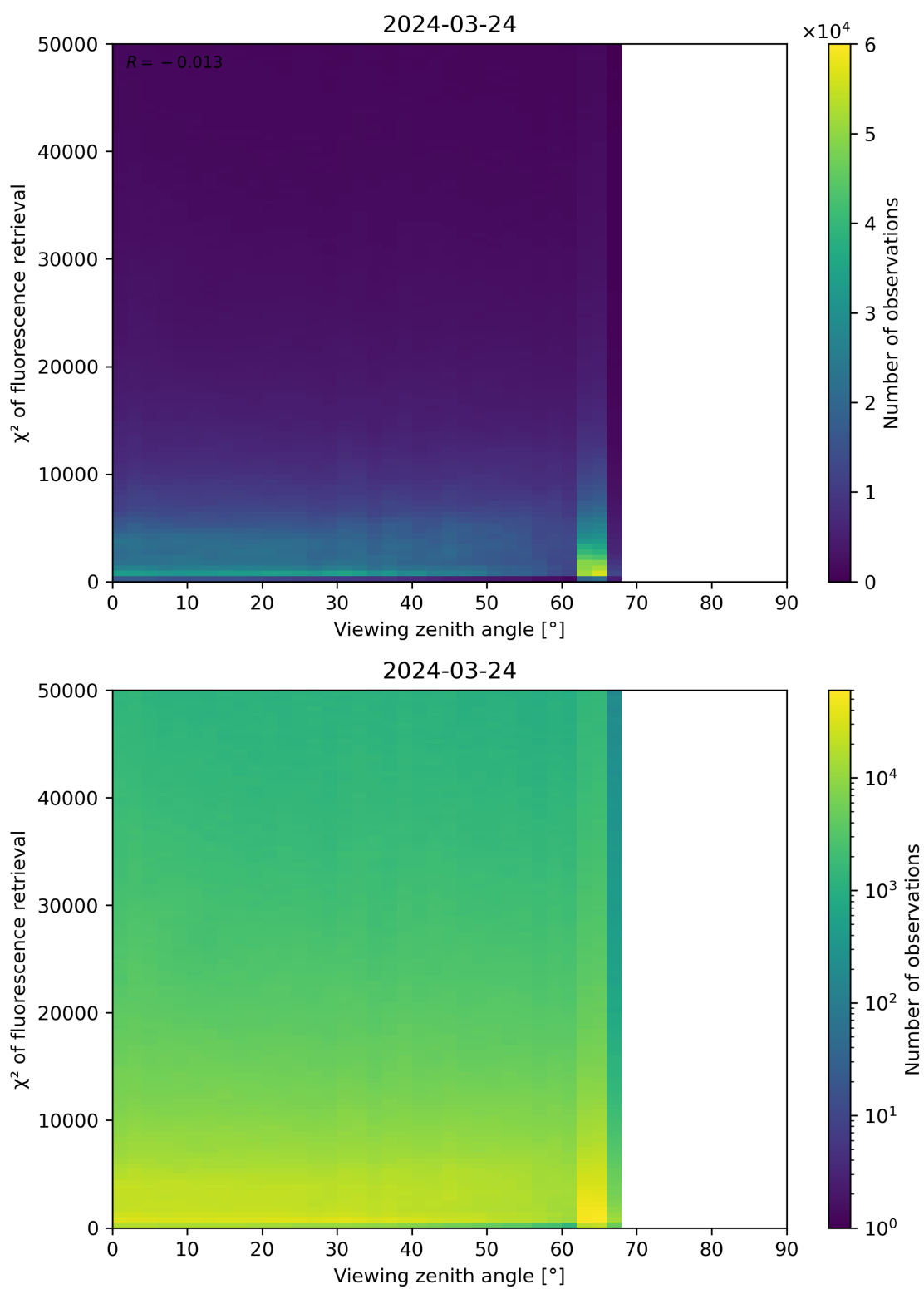
Figure 119: Scatter density plot of “Viewing zenith angle” against “ \chi^2 of fluorescence retrieval” for 2024-03-23 to 2024-03-25.
