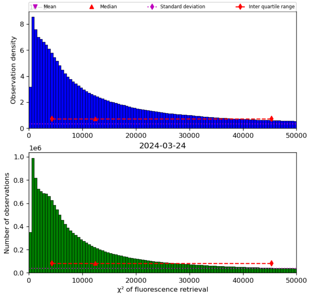
Figure 42: Histogram of “ \chi^2 of fluorescence retrieval” for 2024-03-23 to 2024-03-25
