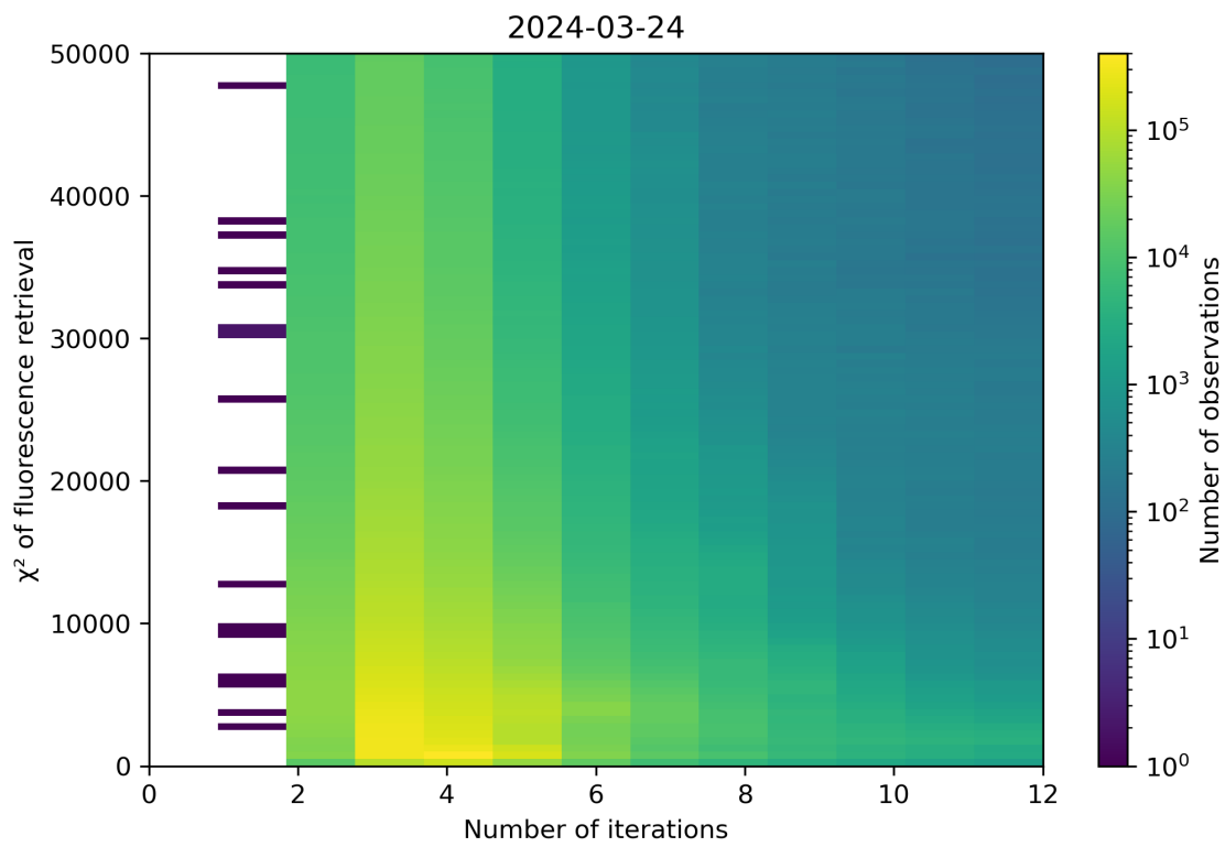
Figure 97: Scatter density plot of “Number of iterations” against “ \chi^2 of fluorescence retrieval” for 2024-03-23 to 2024-03-25.
