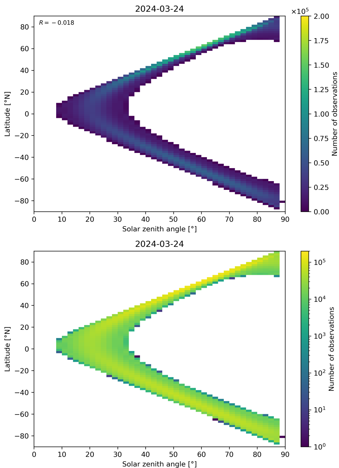
Figure 113: Scatter density plot of “Solar zenith angle” against “Latitude” for 2024-03-23 to 2024-03-25.
