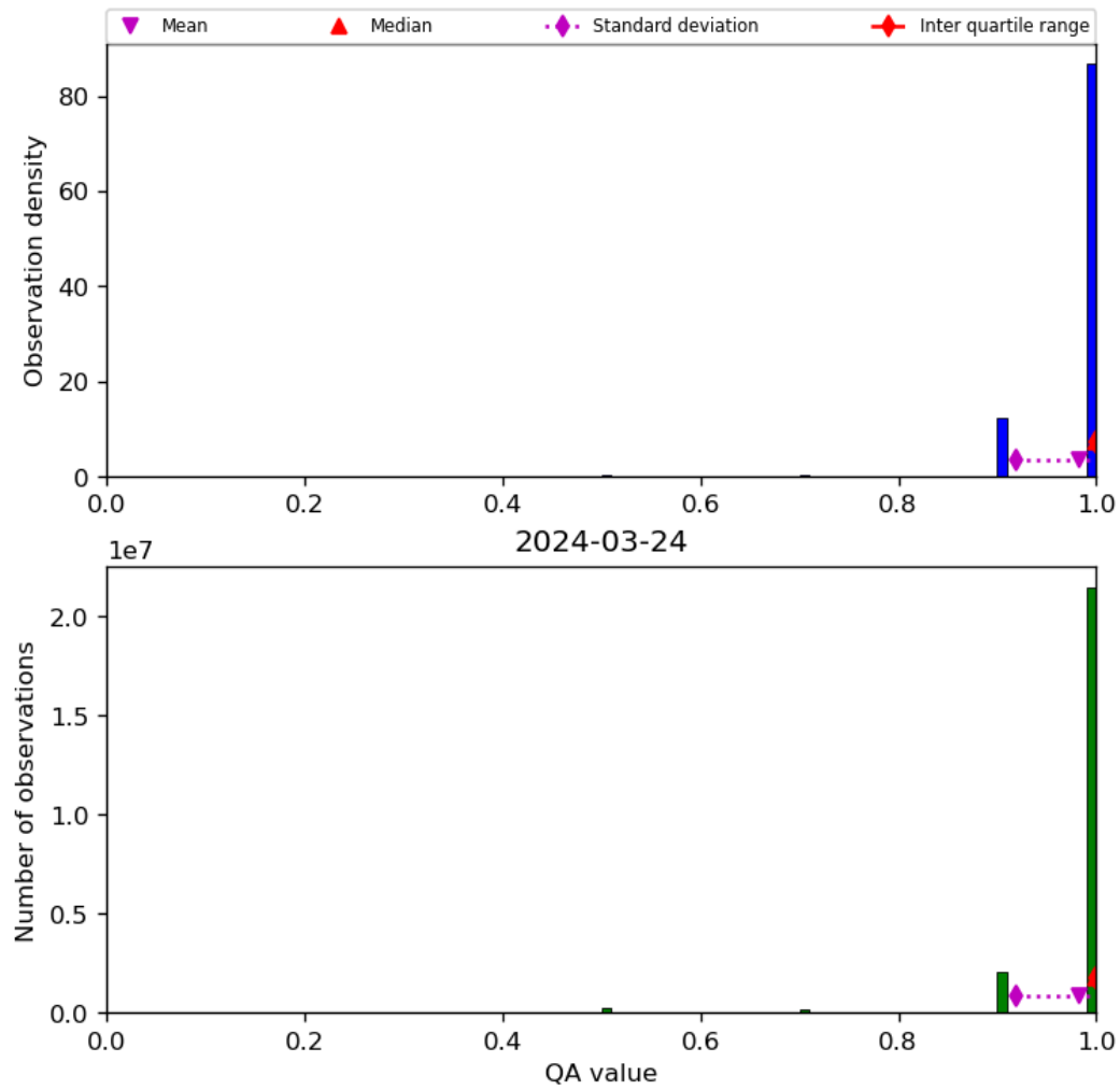
Figure 29: Histogram of “QA value” for 2024-03-23 to 2024-03-25
