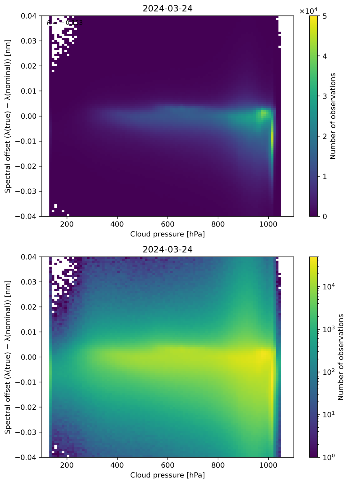
Figure 84: Scatter density plot of “Cloud pressure” against “Spectral offset ( \lambda(\text{true}) - \lambda(\text{nominal}) )” for 2024-03-23 to 2024-03-25.
