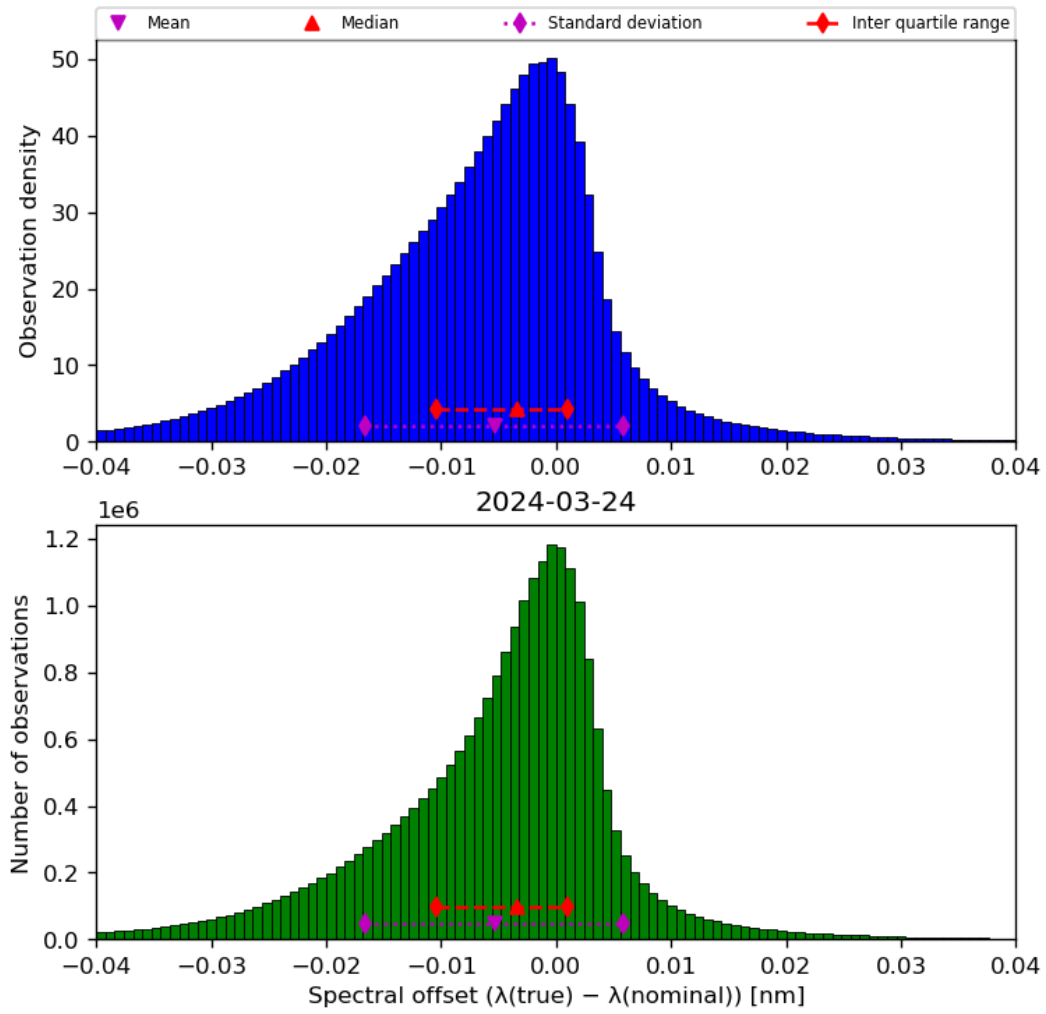
Figure 45: Histogram of “Spectral offset ( \lambda(\text{true}) - \lambda(\text{nominal}) )” for 2024-03-23 to 2024-03-25
