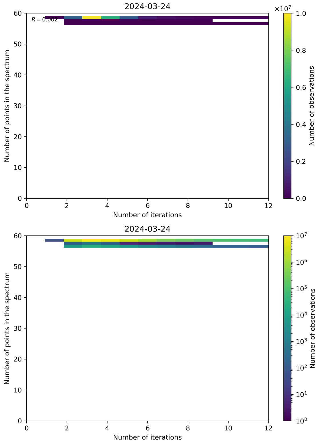
Figure 99: Scatter density plot of “Number of iterations” against “Number of points in the spectrum” for 2024-03-23 to 2024-03-25.
