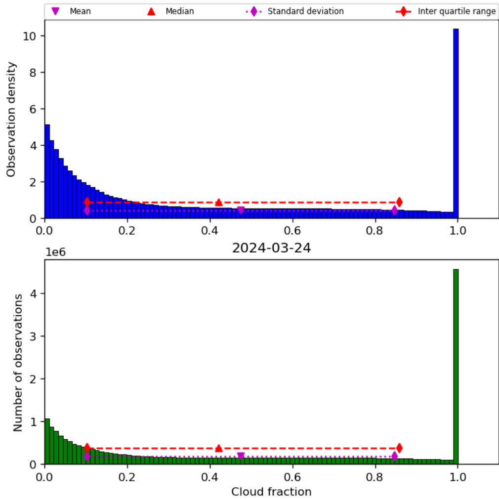
Figure 32: Histogram of “Cloud fraction” for 2024-03-23 to 2024-03-25
