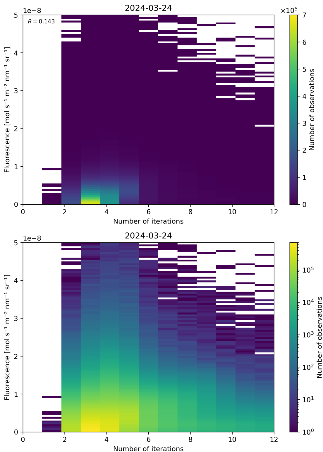
Figure 98: Scatter density plot of “Number of iterations” against “Fluorescence” for 2024-03-23 to 2024-03-25.
