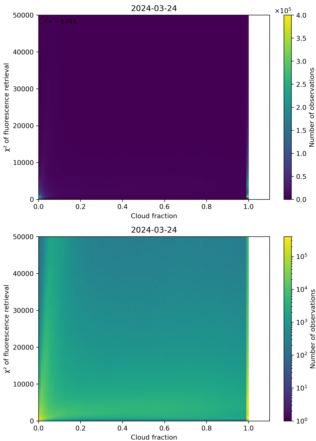
Figure 71: Scatter density plot of “Cloud fraction” against “ \chi^2 of fluorescence retrieval” for 2024-03-23 to 2024-03-25.
