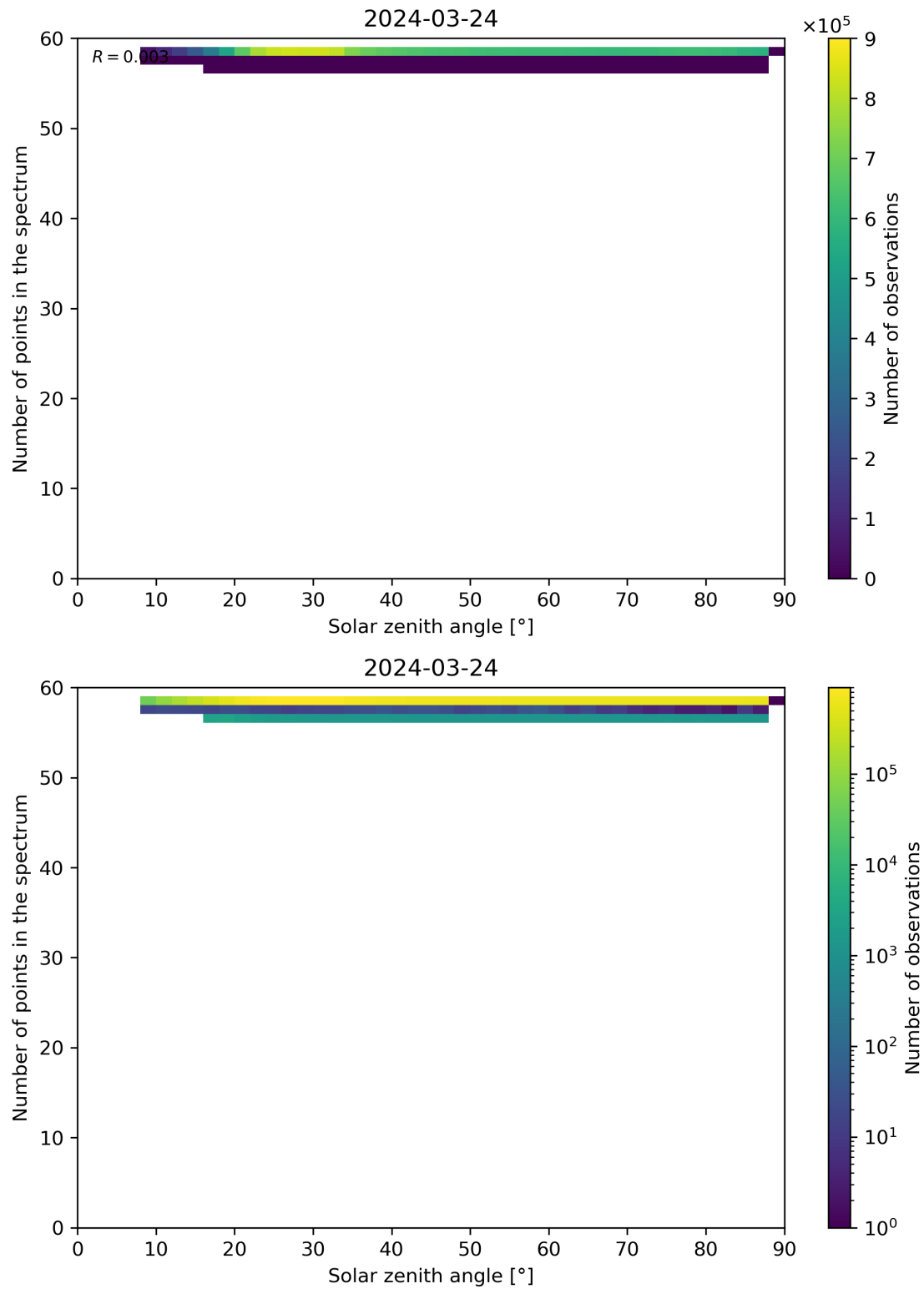
Figure 115: Scatter density plot of “Solar zenith angle” against “Number of points in the spectrum” for 2024-03-23 to 2024-03-25.
