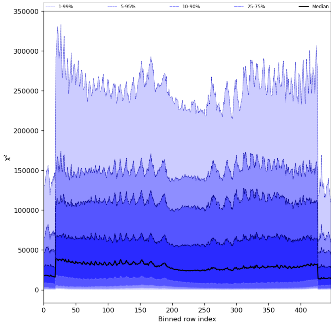
Figure 55: Along track statistics of “ \chi^2 ” for 2024-03-23 to 2024-03-25
