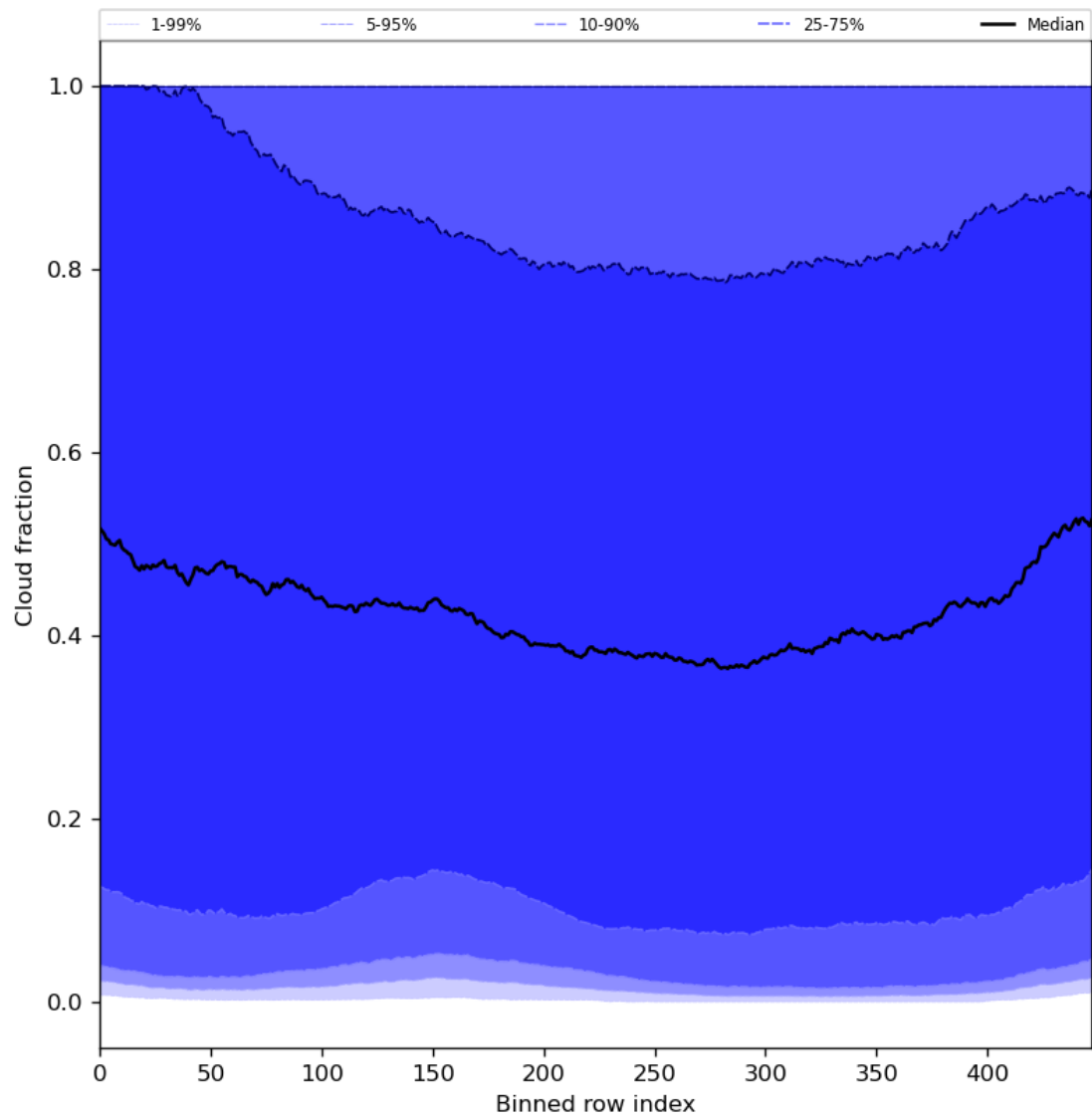
Figure 49: Along track statistics of “Cloud fraction” for 2024-03-23 to 2024-03-25
