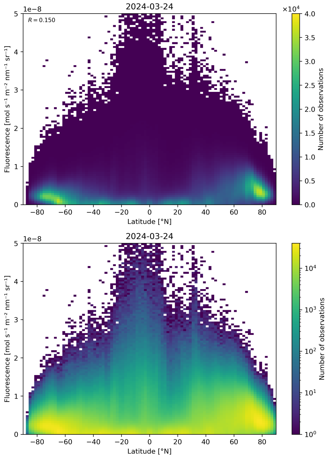
Figure 92: Scatter density plot of “Latitude” against “Fluorescence” for 2024-03-23 to 2024-03-25.
