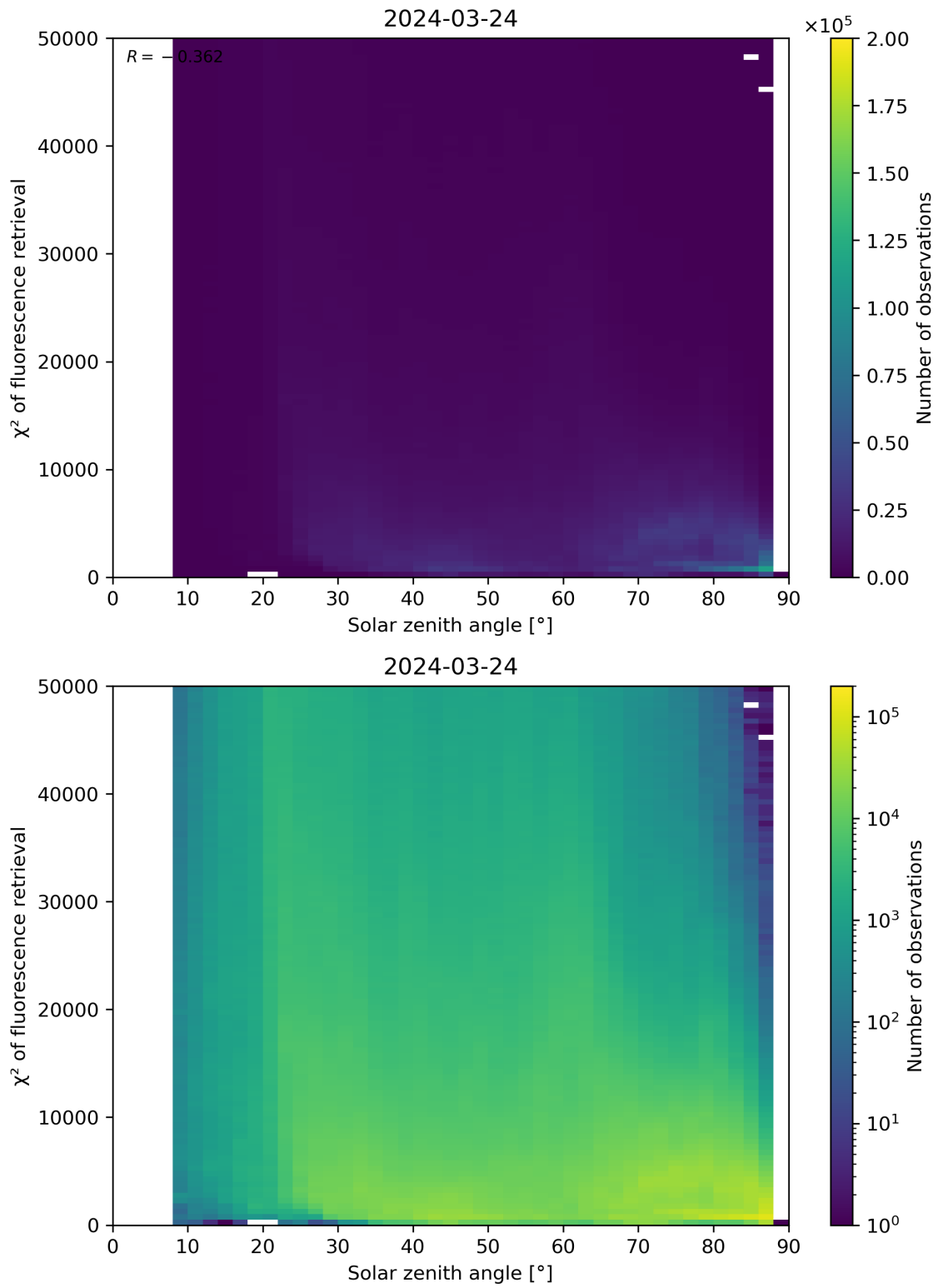
Figure 109: Scatter density plot of “Solar zenith angle” against “ \chi^2 of fluorescence retrieval” for 2024-03-23 to 2024-03-25.
