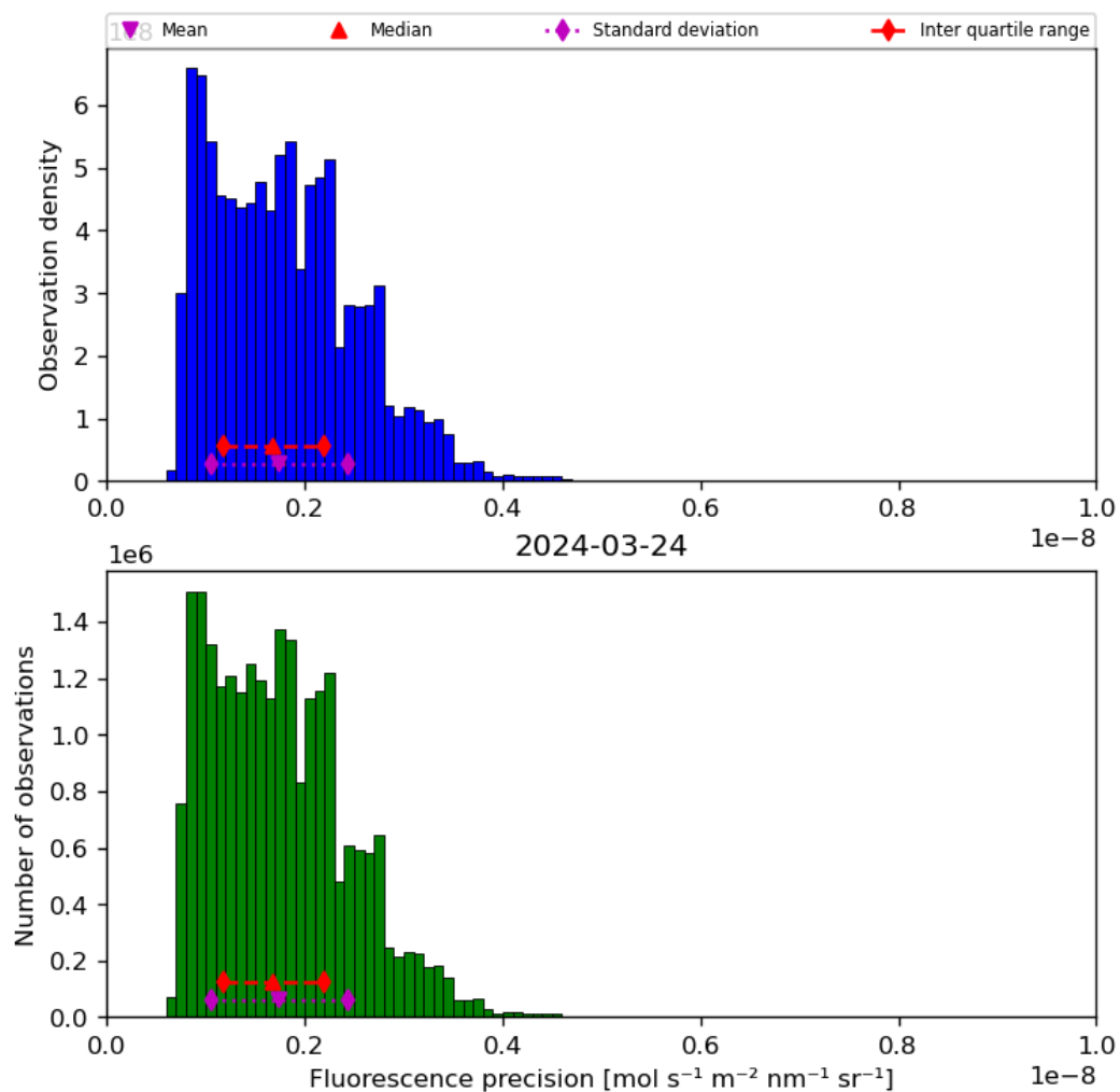
Figure 41: Histogram of “Fluorescence precision” for 2024-03-23 to 2024-03-25
