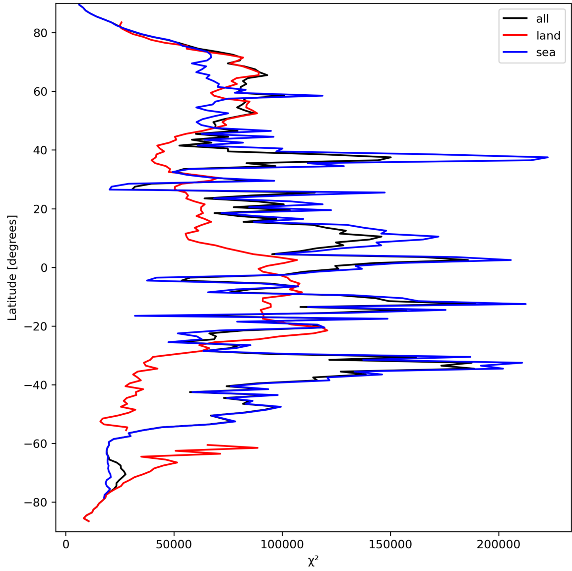
Figure 21: Zonal average of “ \chi^2 ” for 2024-03-23 to 2024-03-25.
