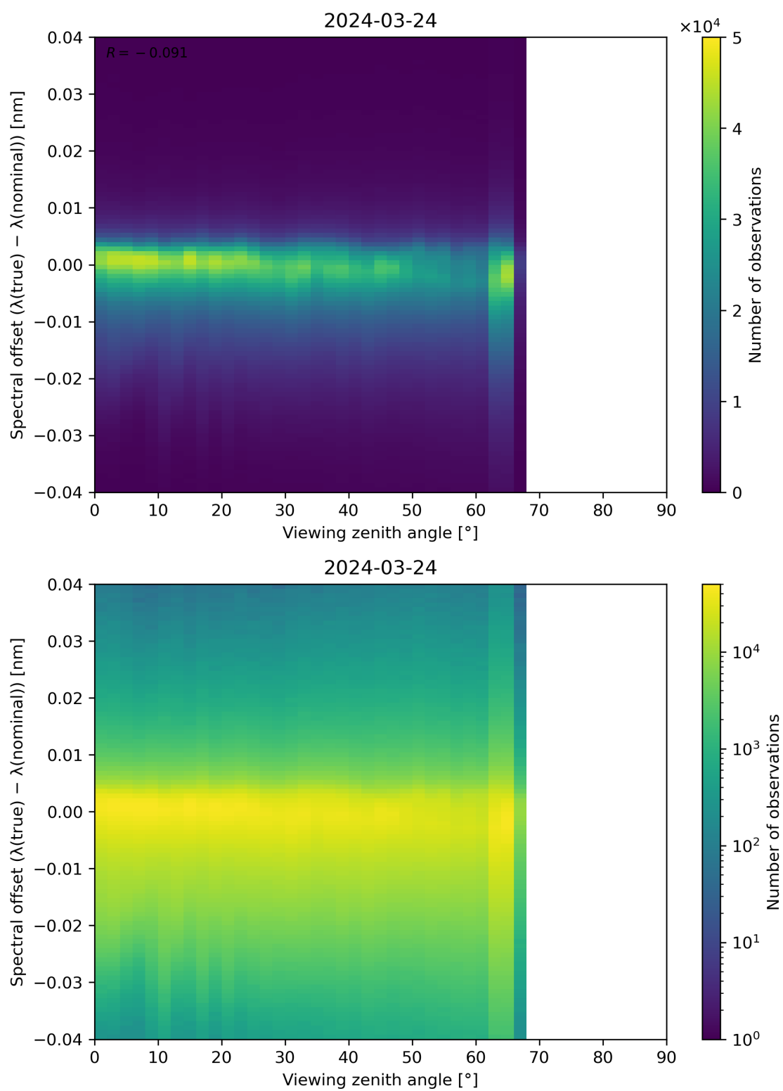
Figure 128: Scatter density plot of “Viewing zenith angle” against “Spectral offset ( \lambda(\text{true}) - \lambda(\text{nominal}) )” for 2024-03-23 to 2024-03-25.
