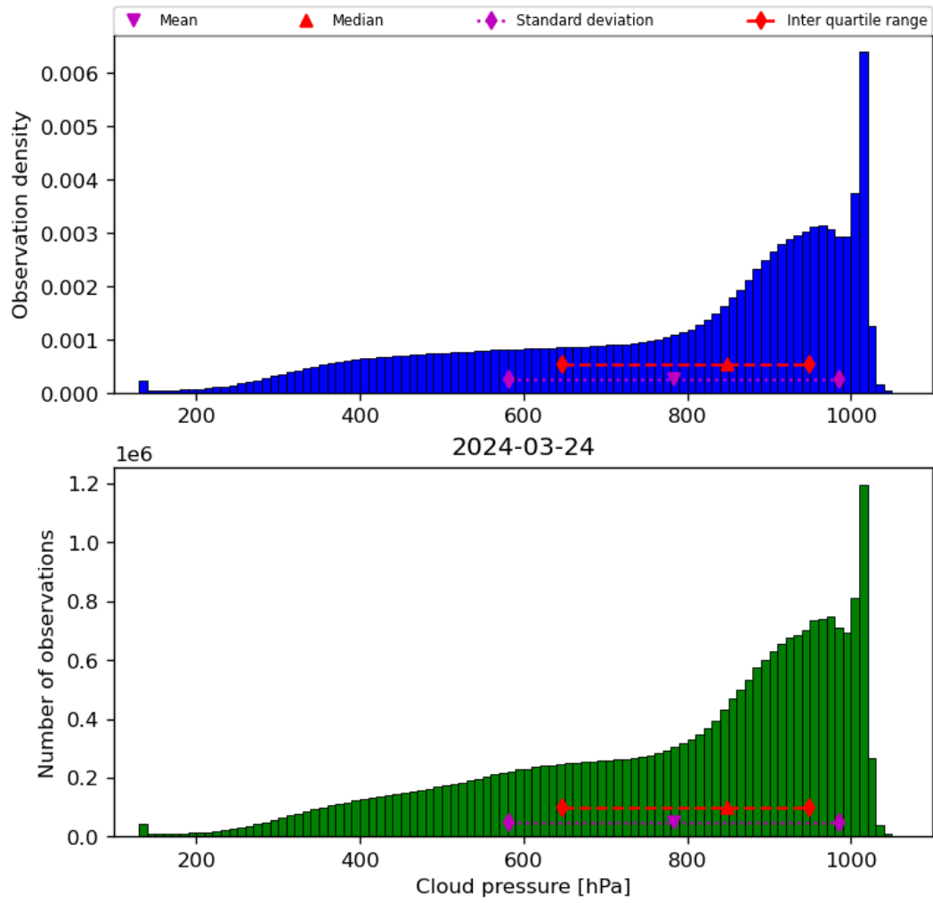
Figure 30: Histogram of “Cloud pressure” for 2024-03-23 to 2024-03-25
