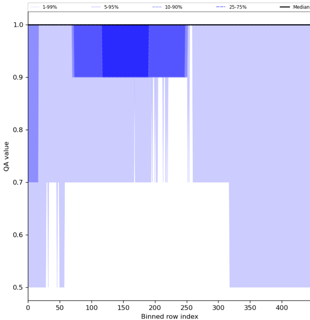
Figure 46: Along track statistics of “QA value” for 2024-03-23 to 2024-03-25
