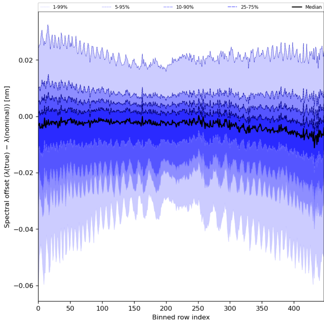
Figure 62: Along track statistics of “Spectral offset ( \lambda(\text{true}) - \lambda(\text{nominal}) )” for 2024-03-23 to 2024-03-25
