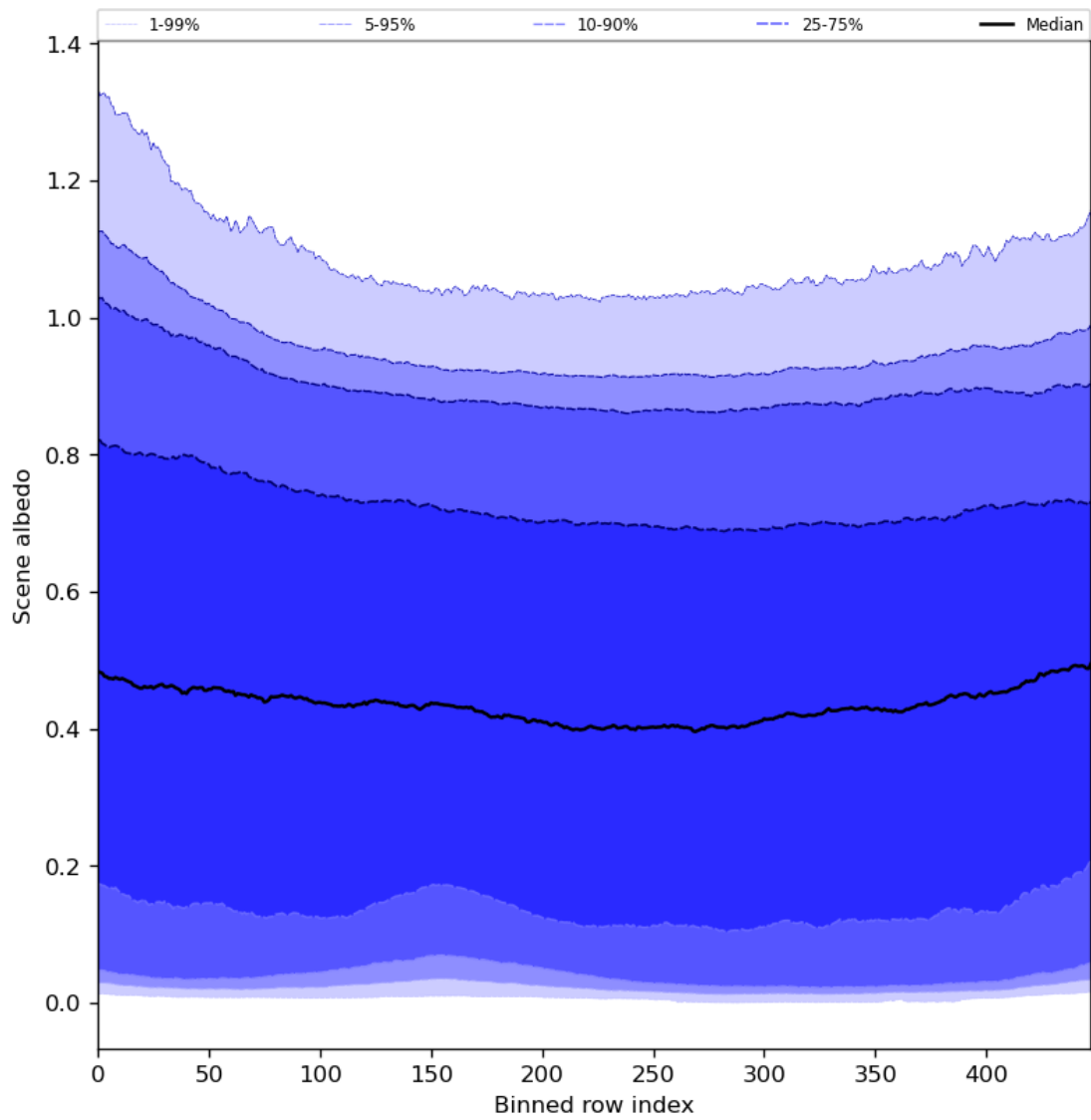
Figure 51: Along track statistics of “Scene albedo” for 2024-03-23 to 2024-03-25
