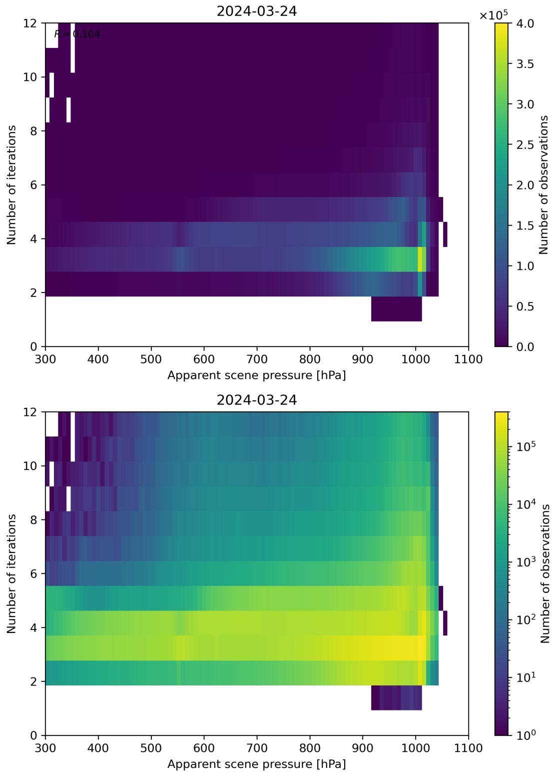
Figure 65: Scatter density plot of “Apparent scene pressure” against “Number of iterations” for 2024-03-23 to 2024-03-25.
