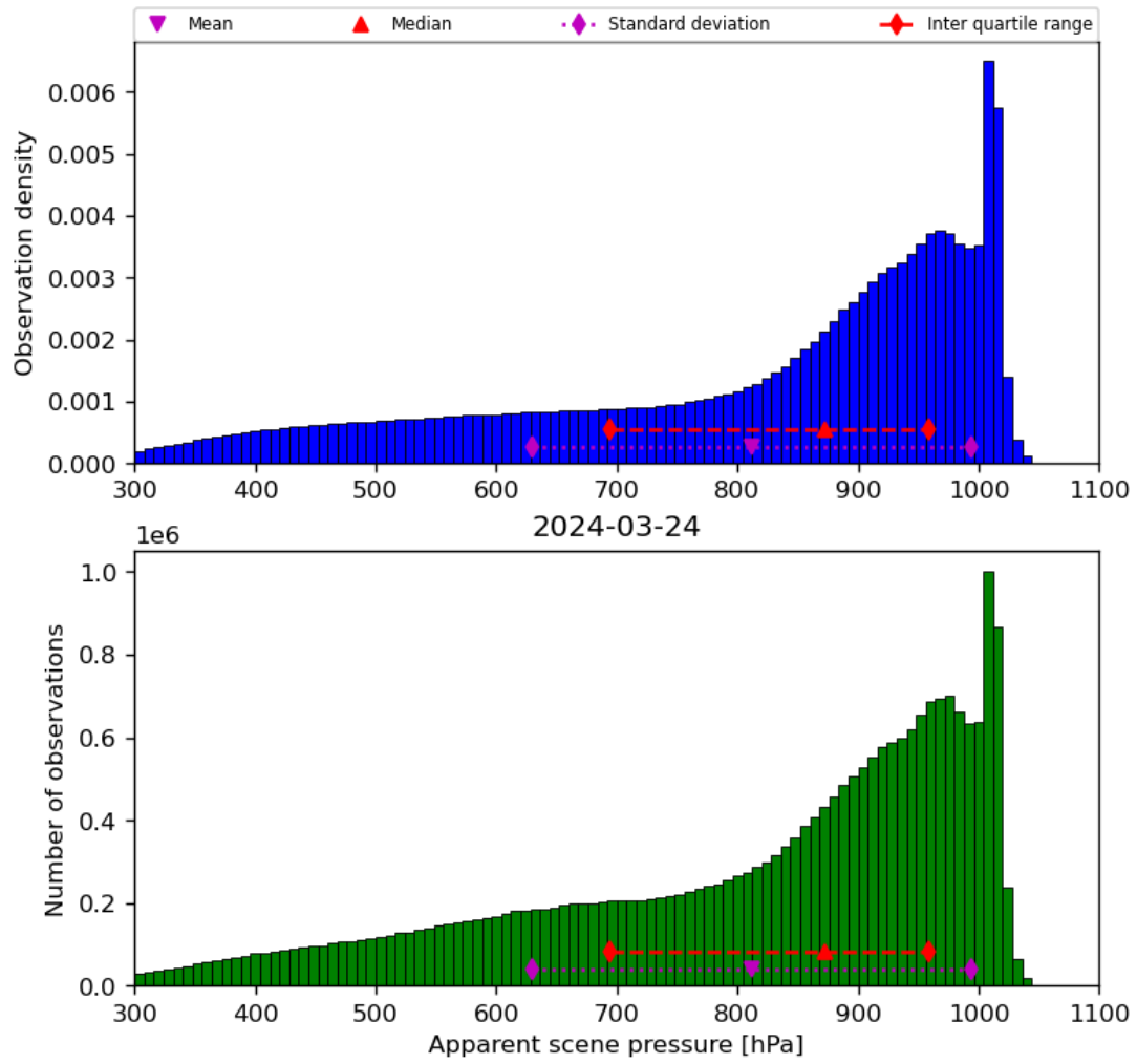
Figure 36: Histogram of “Apparent scene pressure” for 2024-03-23 to 2024-03-25
