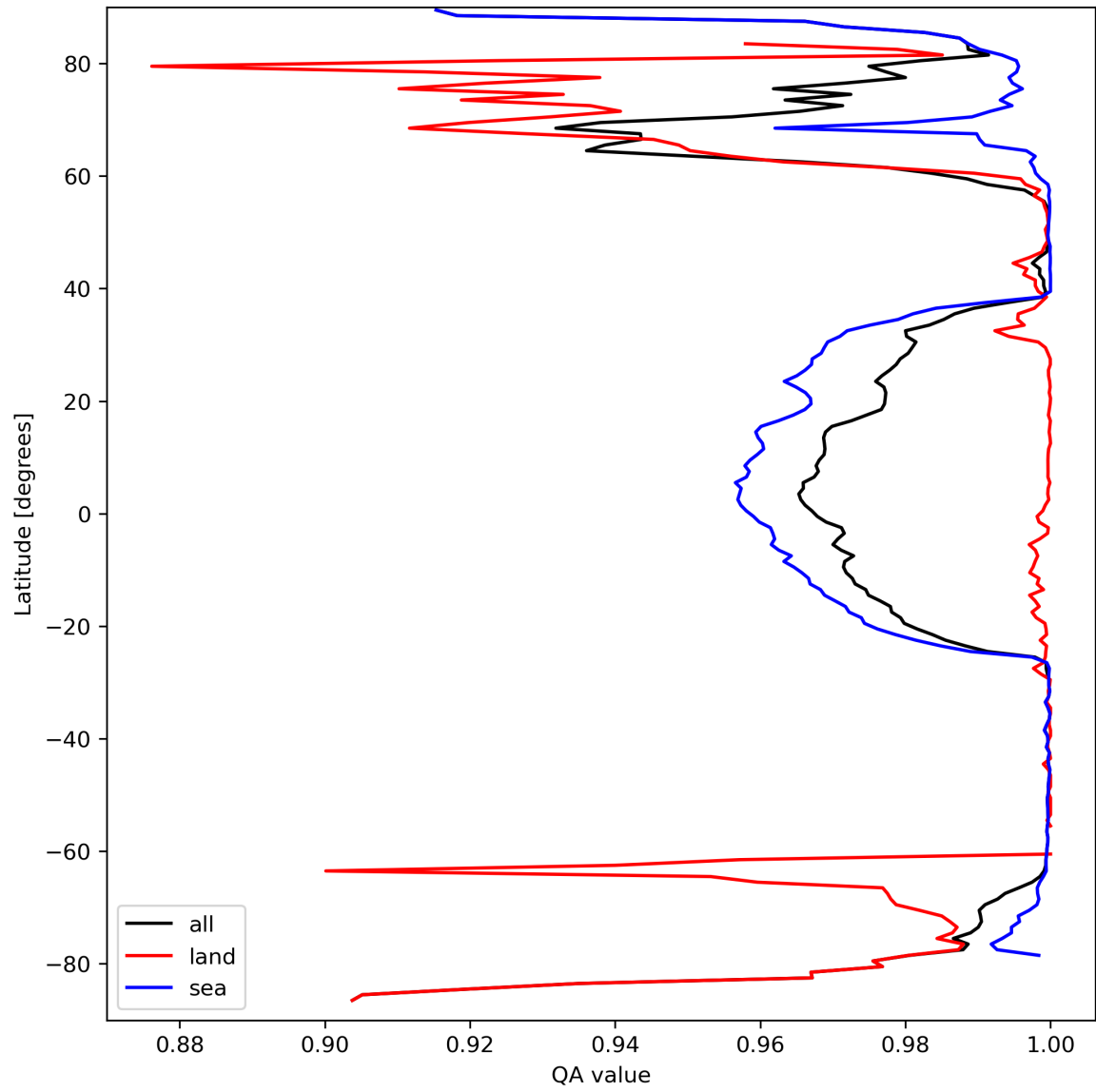
Figure 12: Zonal average of “QA value” for 2024-03-23 to 2024-03-25.
