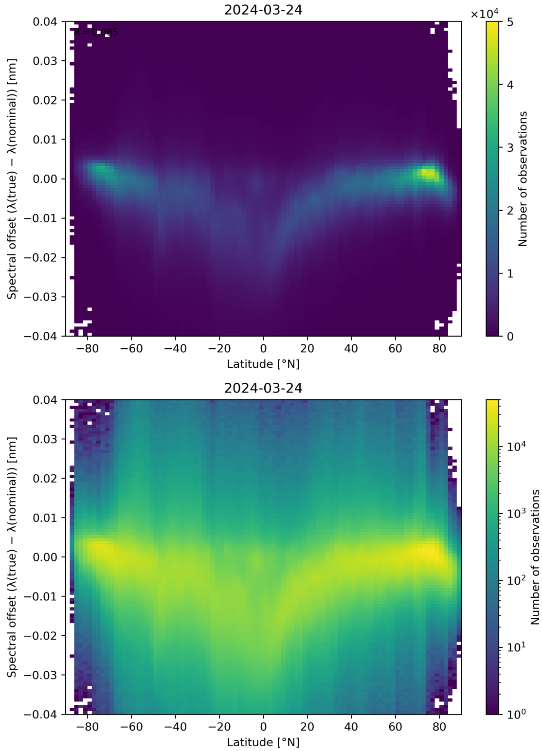
Figure 96: Scatter density plot of “Latitude” against “Spectral offset ( \lambda(\text{true}) - \lambda(\text{nominal}) )” for 2024-03-23 to 2024-03-25.
