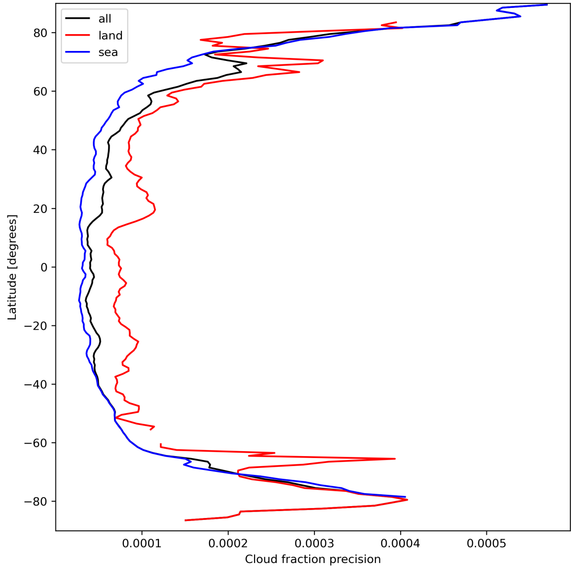
Figure 16: Zonal average of “Cloud fraction precision” for 2024-03-23 to 2024-03-25.
