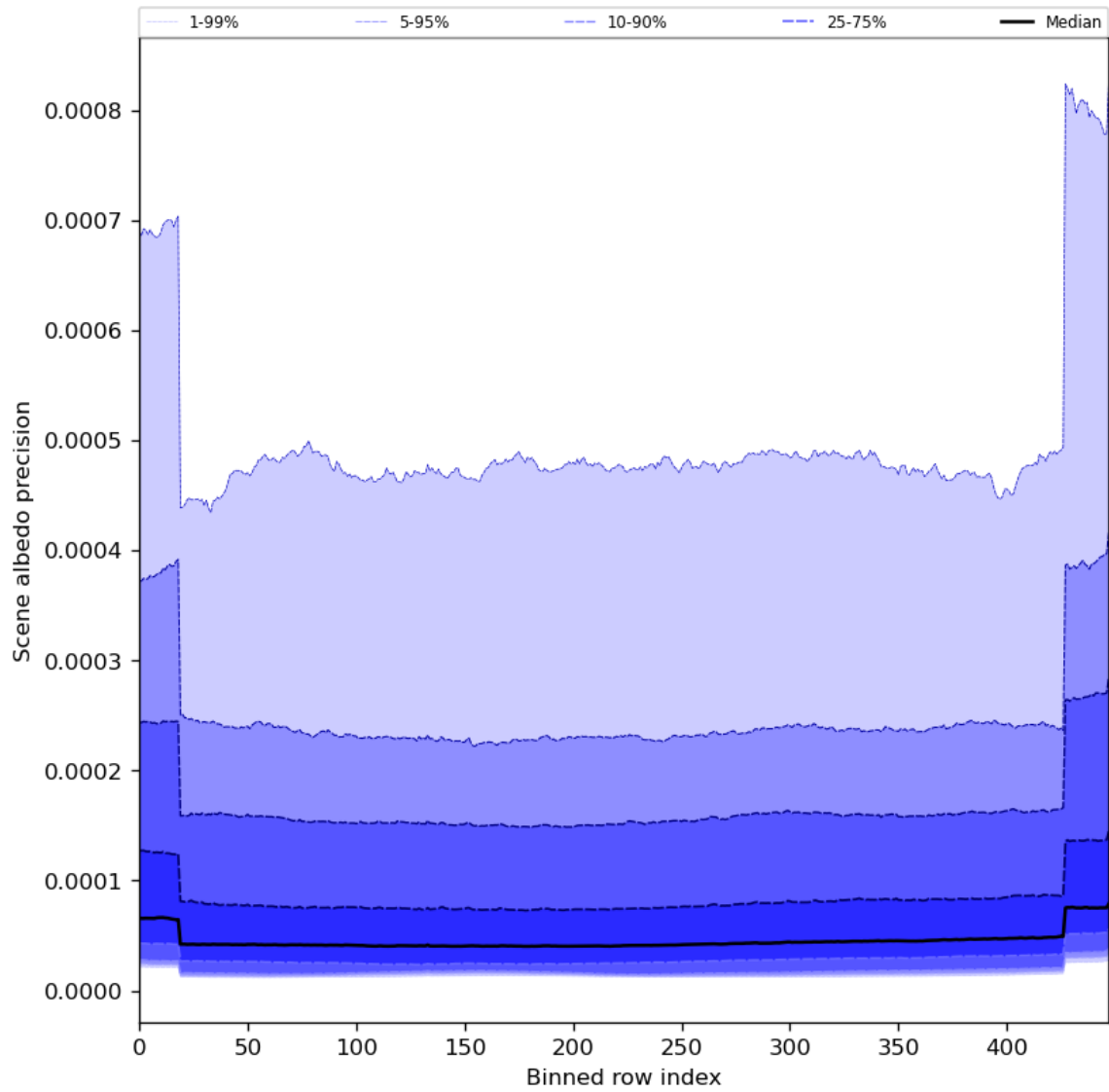
Figure 52: Along track statistics of “Scene albedo precision” for 2024-03-23 to 2024-03-25
