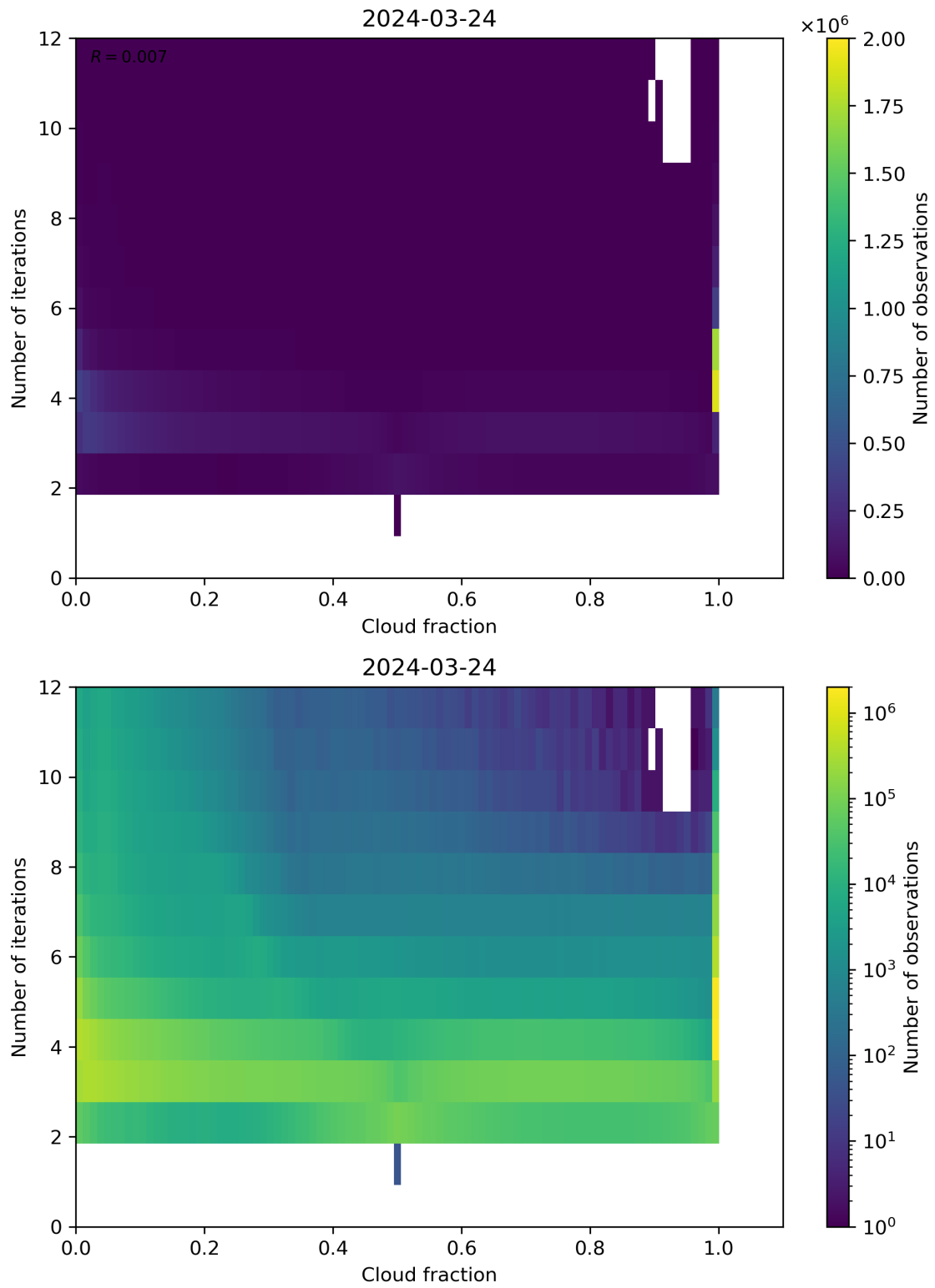
Figure 73: Scatter density plot of “Cloud fraction” against “Number of iterations” for 2024-03-23 to 2024-03-25.
