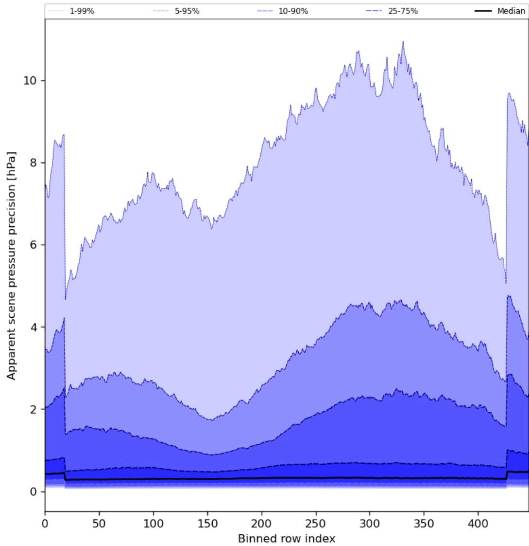
Figure 54: Along track statistics of “Apparent scene pressure precision” for 2024-03-23 to 2024-03-25
