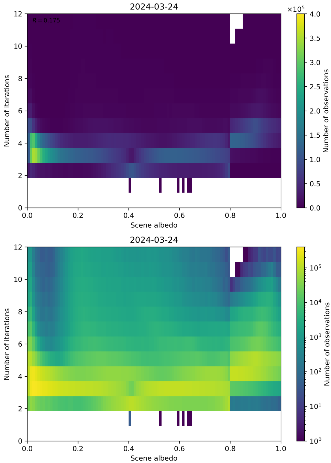
Figure 105: Scatter density plot of “Scene albedo” against “Number of iterations” for 2024-03-23 to 2024-03-25.
