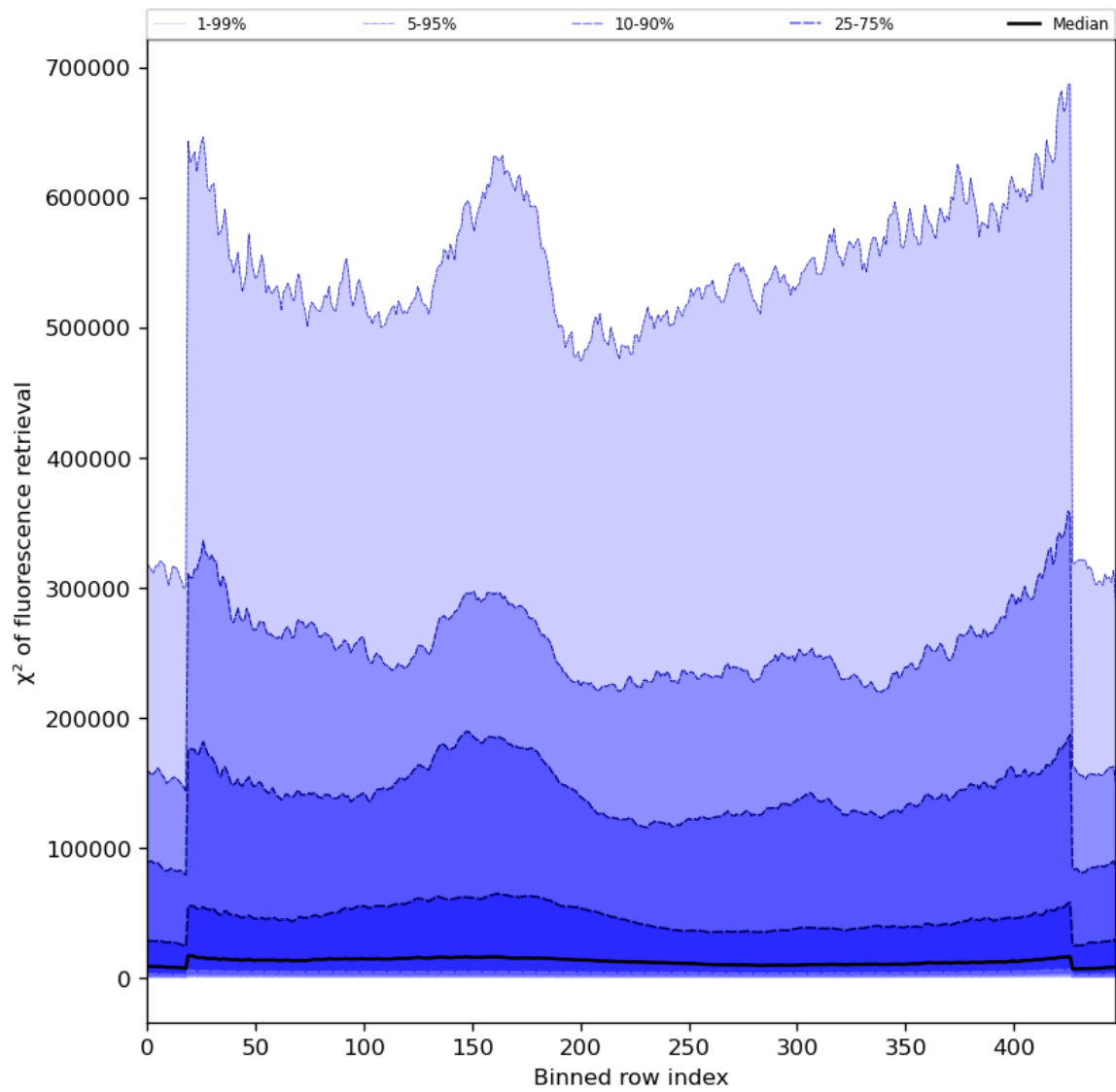
Figure 59: Along track statistics of “ \chi^2 of fluorescence retrieval” for 2024-03-23 to 2024-03-25
