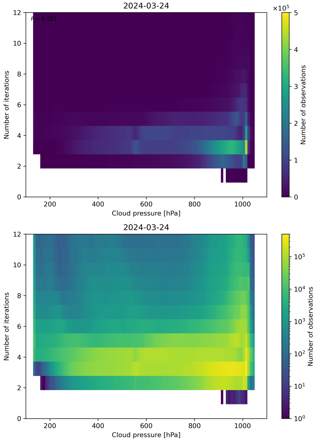
Figure 81: Scatter density plot of “Cloud pressure” against “Number of iterations” for 2024-03-23 to 2024-03-25.
