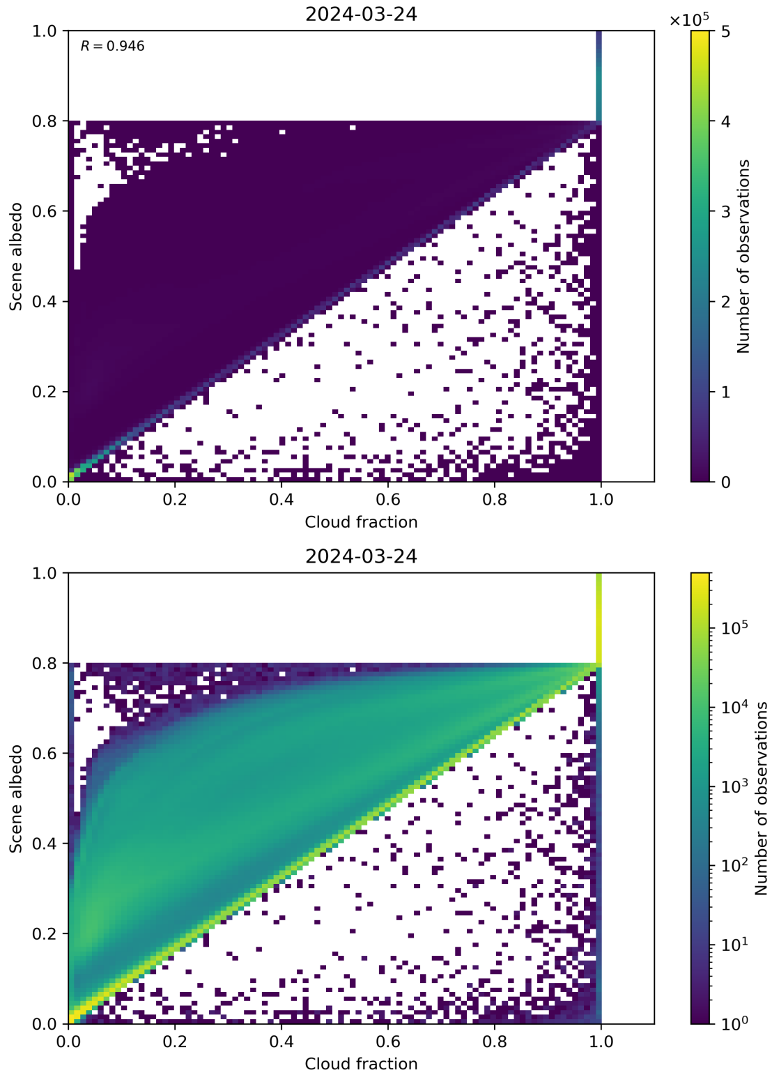
Figure 75: Scatter density plot of “Cloud fraction” against “Scene albedo” for 2024-03-23 to 2024-03-25.
