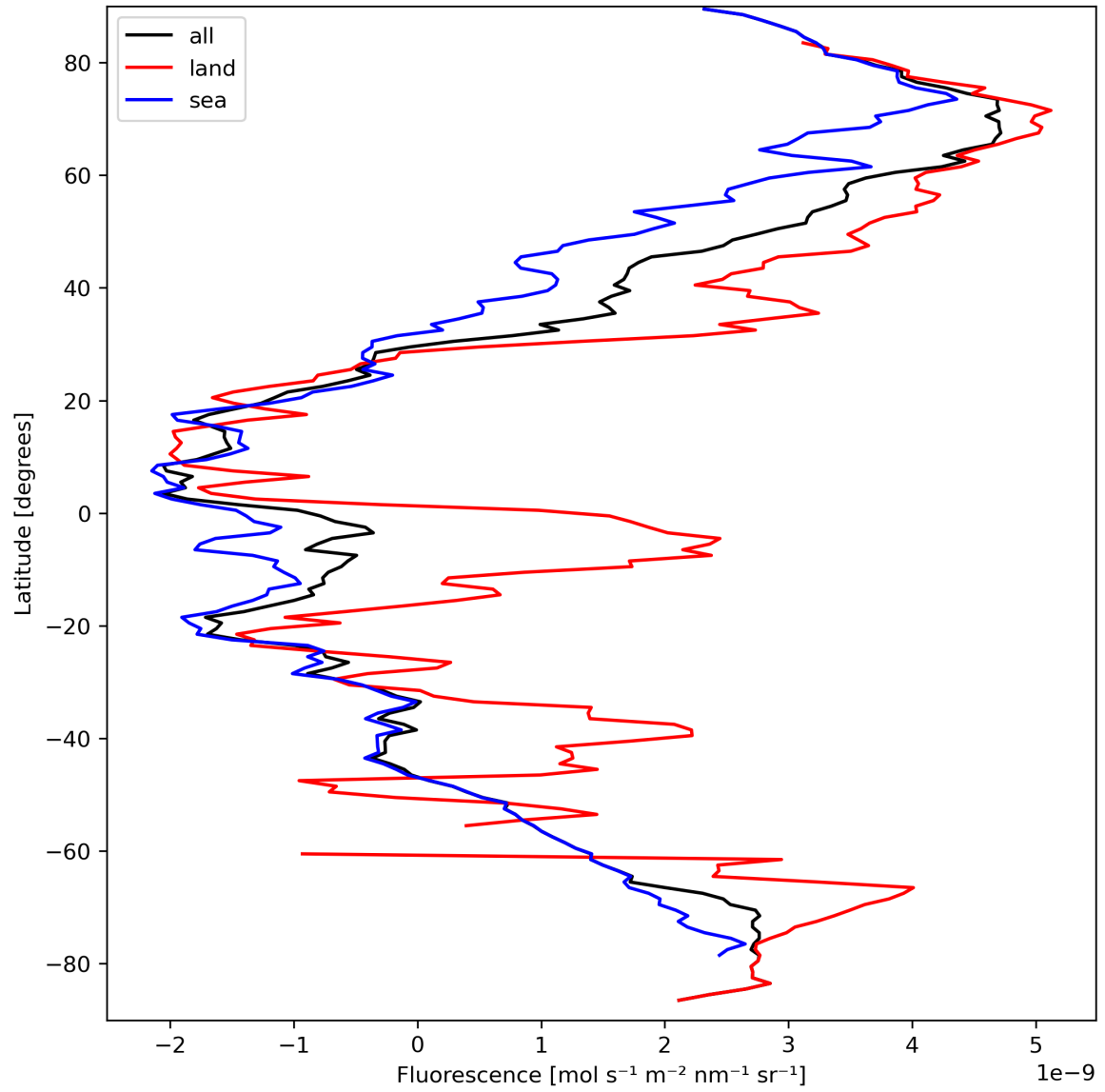
Figure 23: Zonal average of “Fluorescence” for 2024-03-23 to 2024-03-25.
