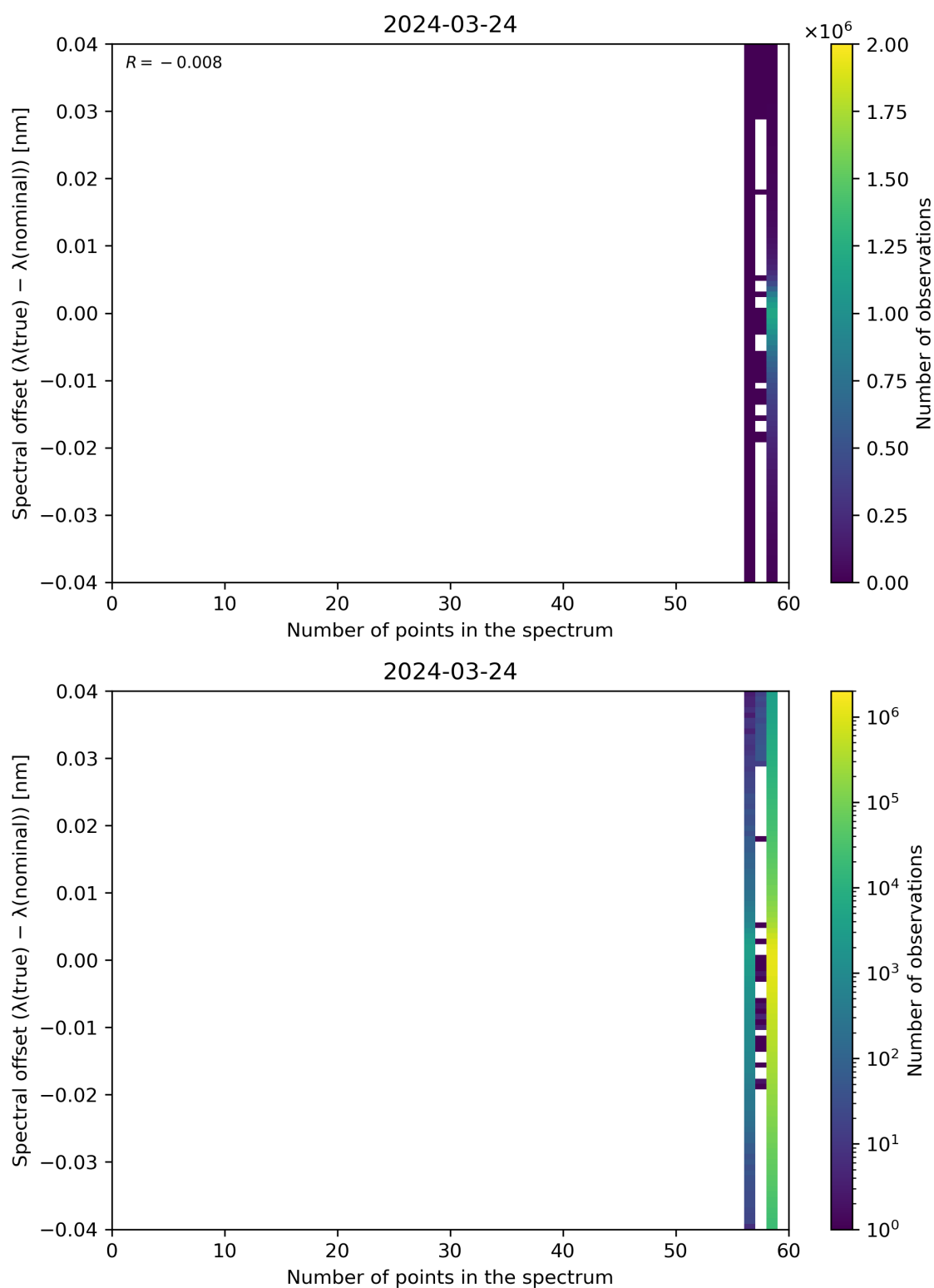
Figure 101: Scatter density plot of “Number of points in the spectrum” against “Spectral offset ( \lambda(\text{true}) - \lambda(\text{nominal}) )” for 2024-03-23 to 2024-03-25.
