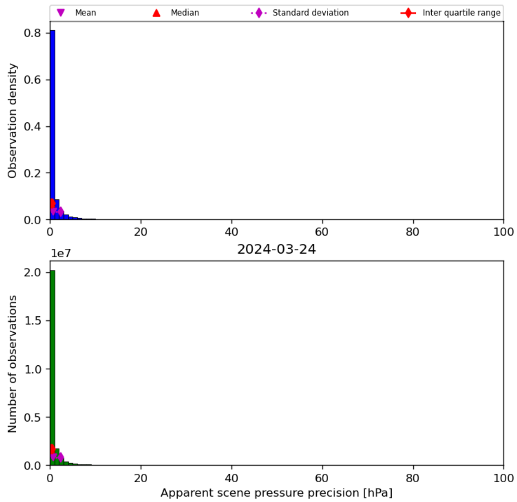
Figure 37: Histogram of “Apparent scene pressure precision” for 2024-03-23 to 2024-03-25
