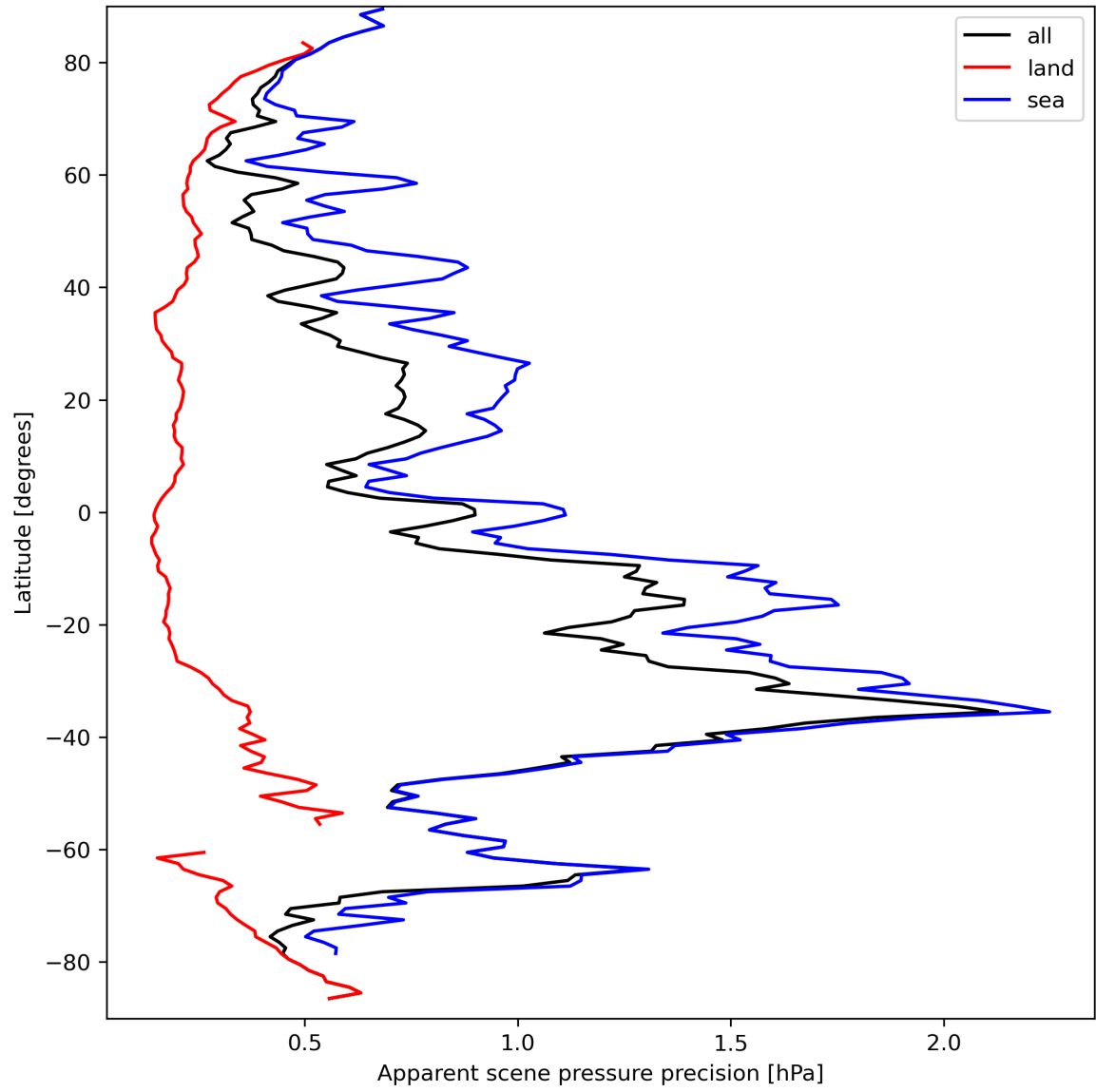
Figure 20: Zonal average of “Apparent scene pressure precision” for 2024-03-23 to 2024-03-25.
