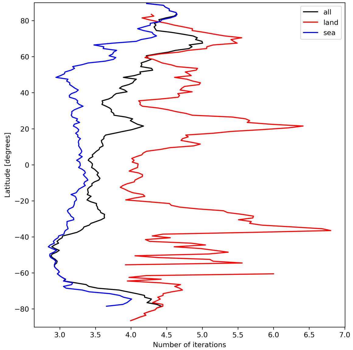
Figure 22: Zonal average of “Number of iterations” for 2024-03-23 to 2024-03-25.
