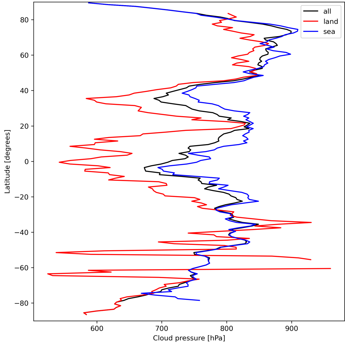
Figure 13: Zonal average of “Cloud pressure” for 2024-03-23 to 2024-03-25.
