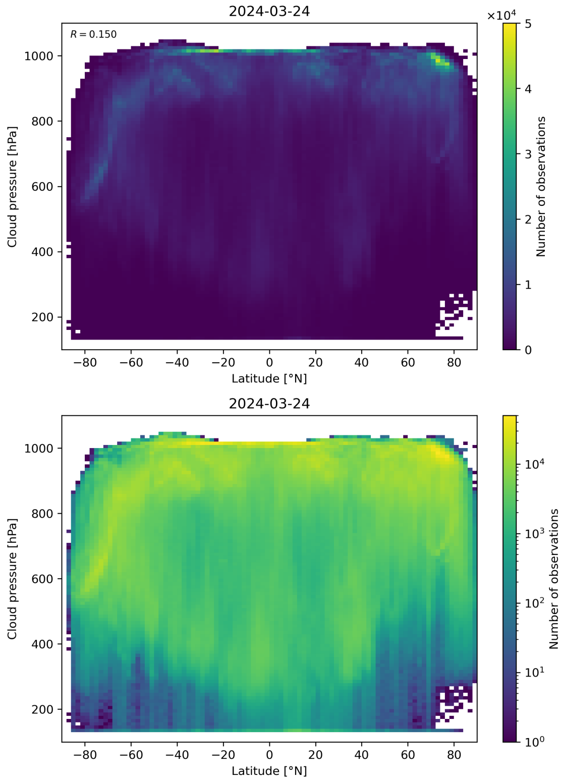
Figure 91: Scatter density plot of “Latitude” against “Cloud pressure” for 2024-03-23 to 2024-03-25.
