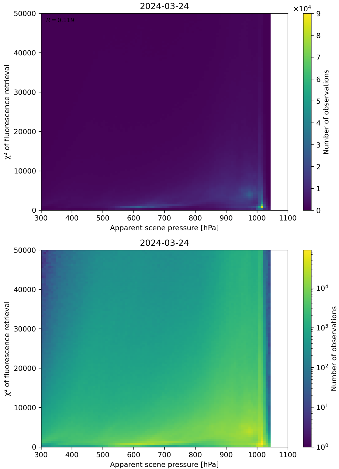
Figure 63: Scatter density plot of “Apparent scene pressure” against “ \chi^2 of fluorescence retrieval” for 2024-03-23 to 2024-03-25.
