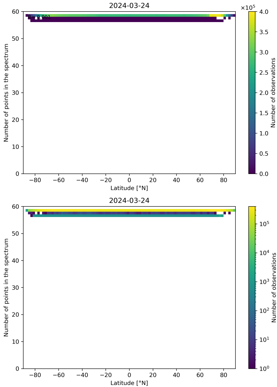
Figure 94: Scatter density plot of “Latitude” against “Number of points in the spectrum” for 2024-03-23 to 2024-03-25.
