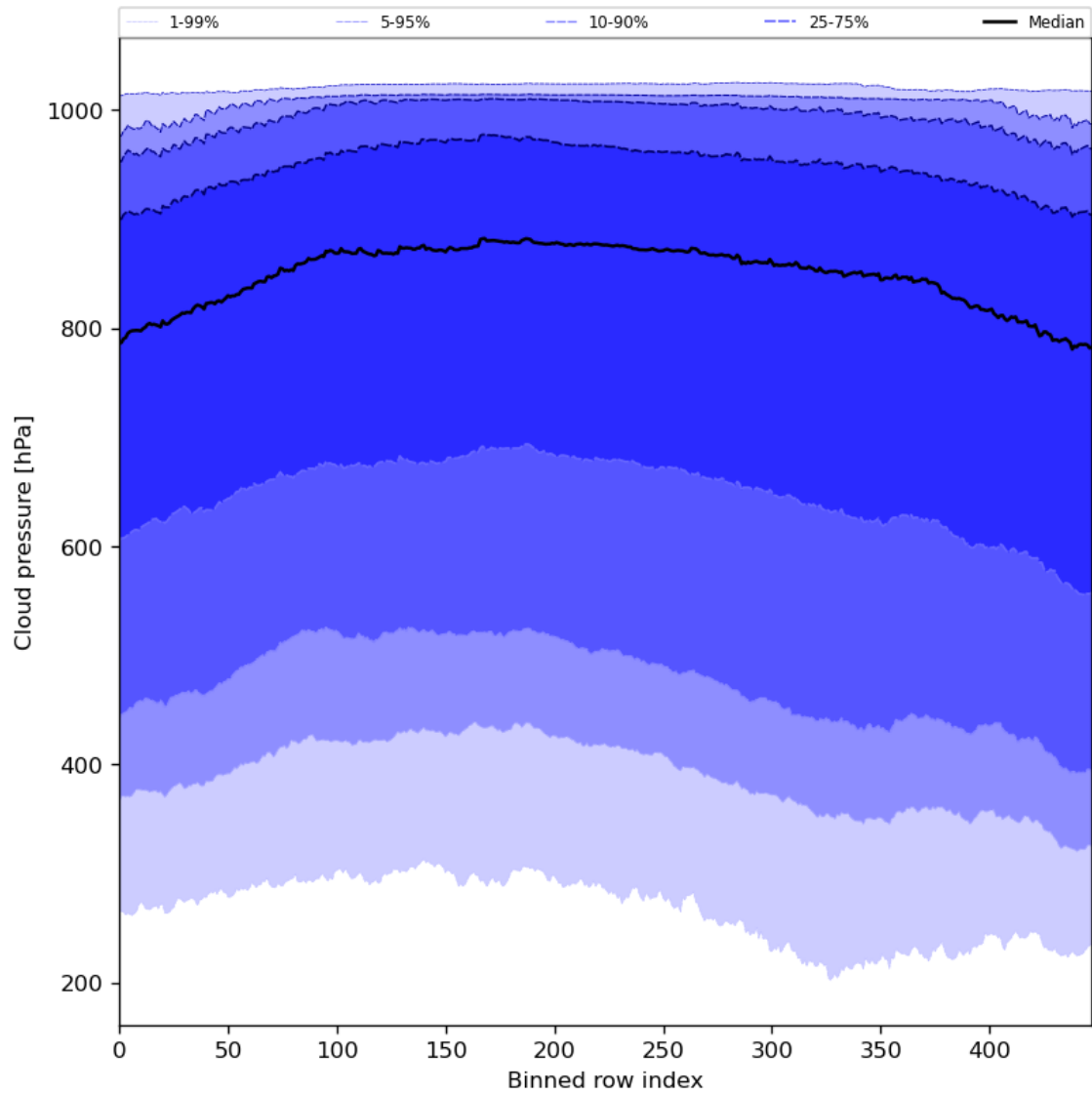
Figure 47: Along track statistics of “Cloud pressure” for 2024-03-23 to 2024-03-25
