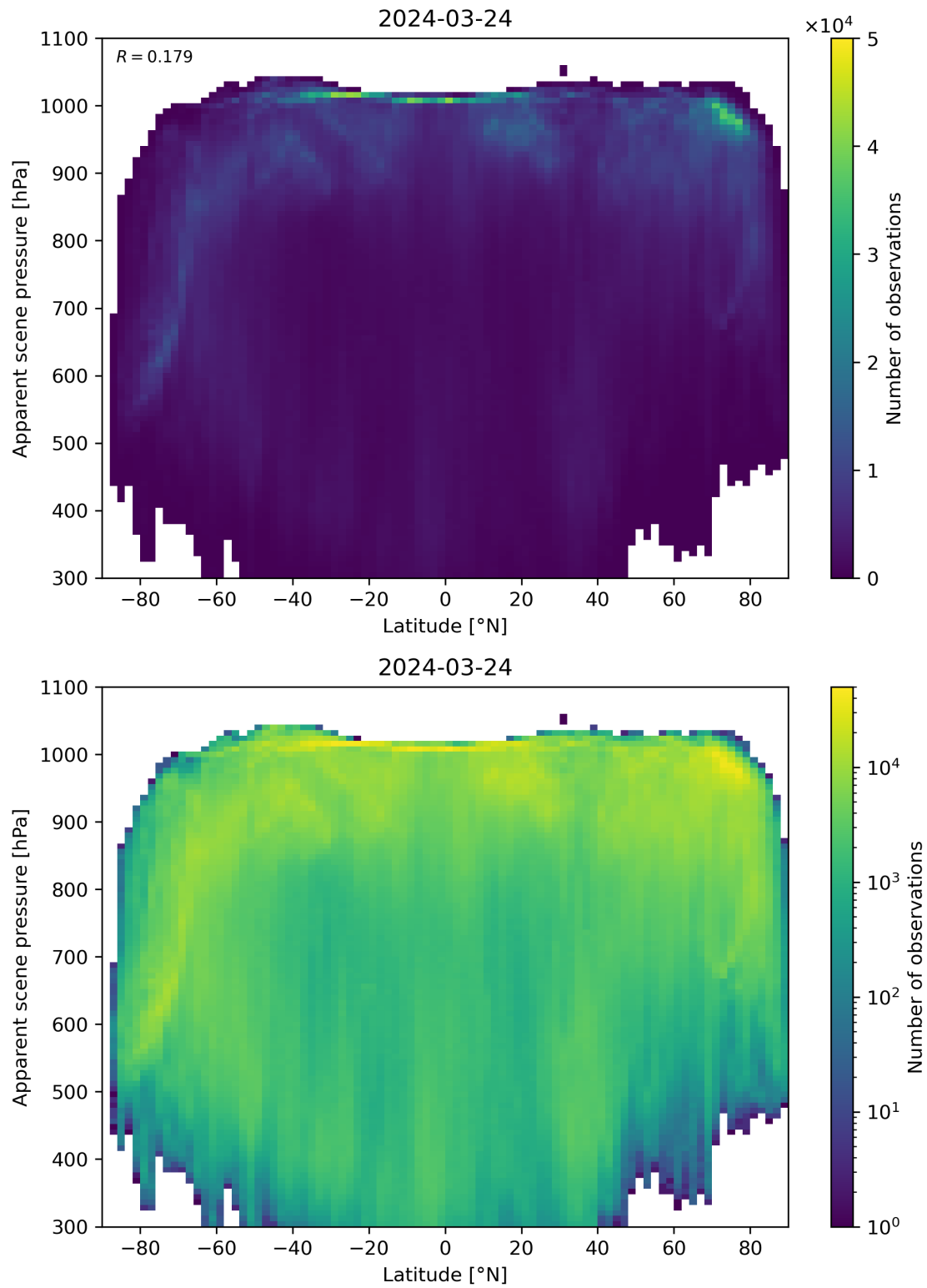
Figure 88: Scatter density plot of “Latitude” against “Apparent scene pressure” for 2024-03-23 to 2024-03-25.
