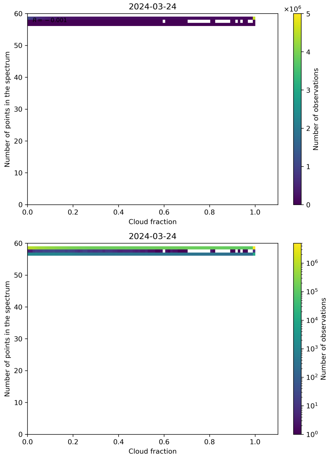
Figure 74: Scatter density plot of “Cloud fraction” against “Number of points in the spectrum” for 2024-03-23 to 2024-03-25.
