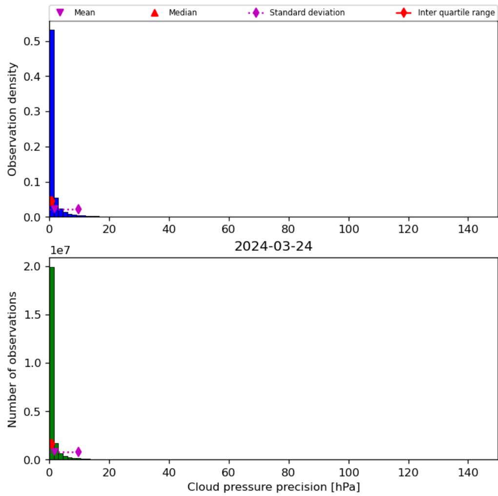
Figure 31: Histogram of “Cloud pressure precision” for 2024-03-23 to 2024-03-25
