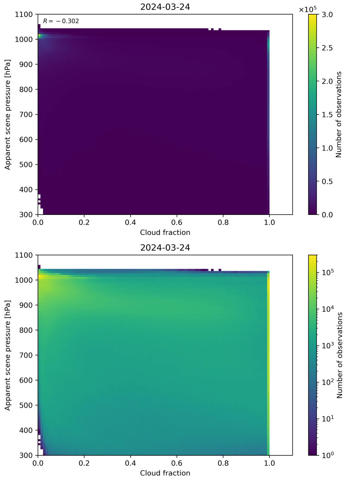
Figure 70: Scatter density plot of “Cloud fraction” against “Apparent scene pressure” for 2024-03-23 to 2024-03-25.
