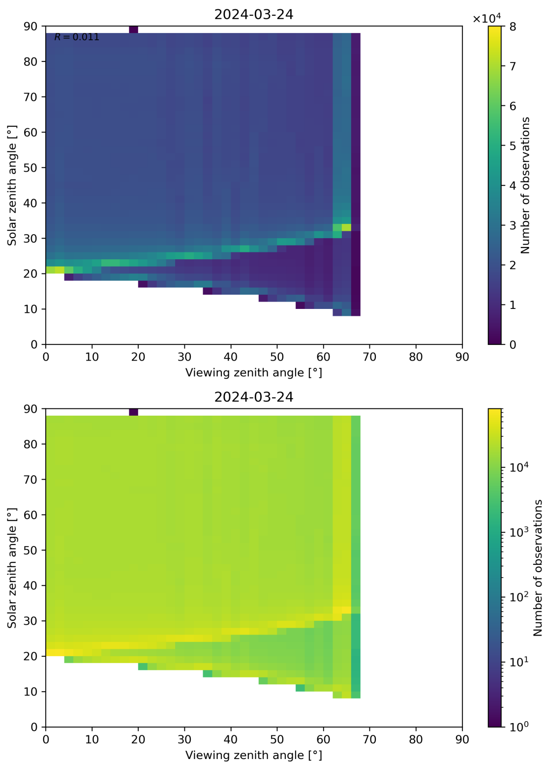
Figure 127: Scatter density plot of “Viewing zenith angle” against “Solar zenith angle” for 2024-03-23 to 2024-03-25.
