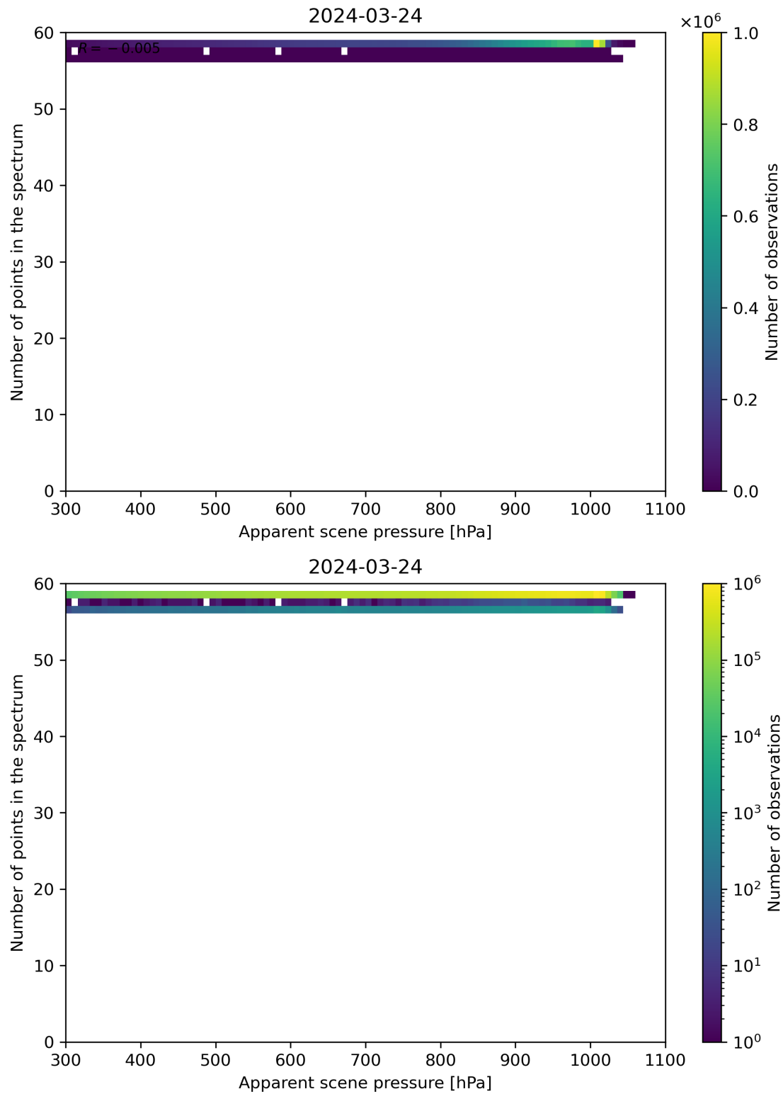
Figure 66: Scatter density plot of “Apparent scene pressure” against “Number of points in the spectrum” for 2024-03-23 to 2024-03-25.
