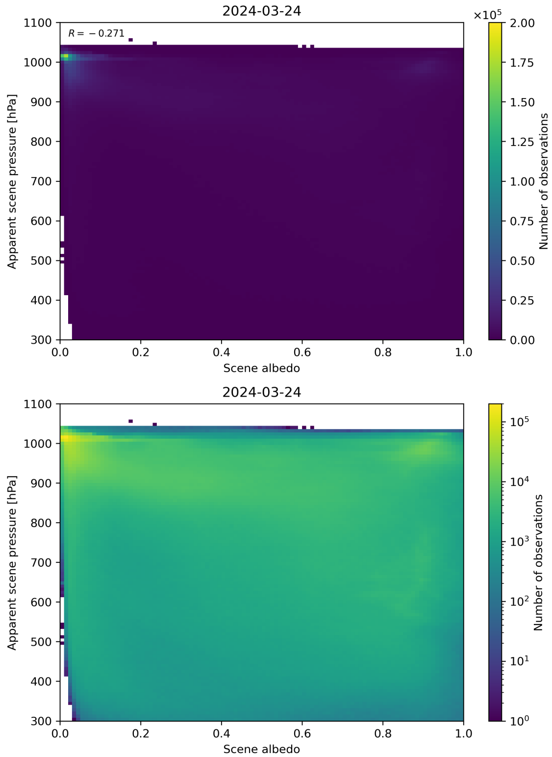
Figure 102: Scatter density plot of “Scene albedo” against “Apparent scene pressure” for 2024-03-23 to 2024-03-25.
