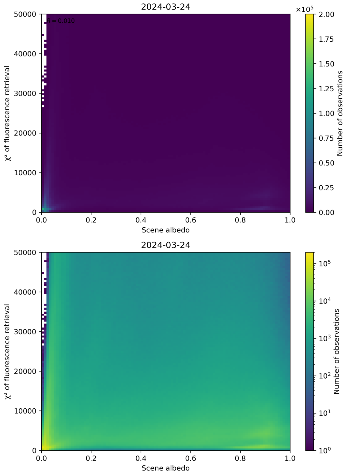
Figure 103: Scatter density plot of “Scene albedo” against “ \chi^2 of fluorescence retrieval” for 2024-03-23 to 2024-03-25.
