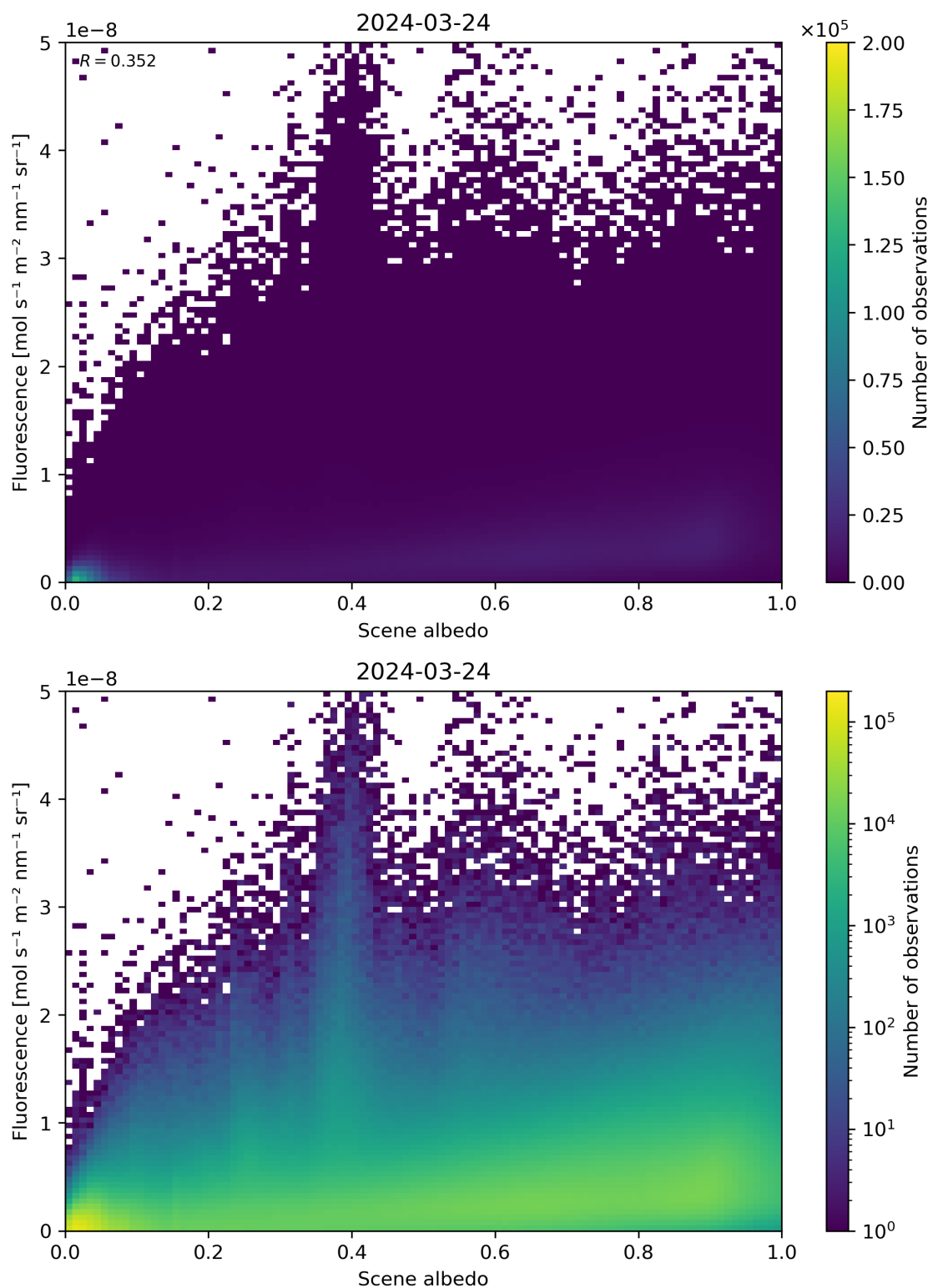
Figure 104: Scatter density plot of "Scene albedo" against "Fluorescence" for 2024-03-23 to 2024-03-25.
