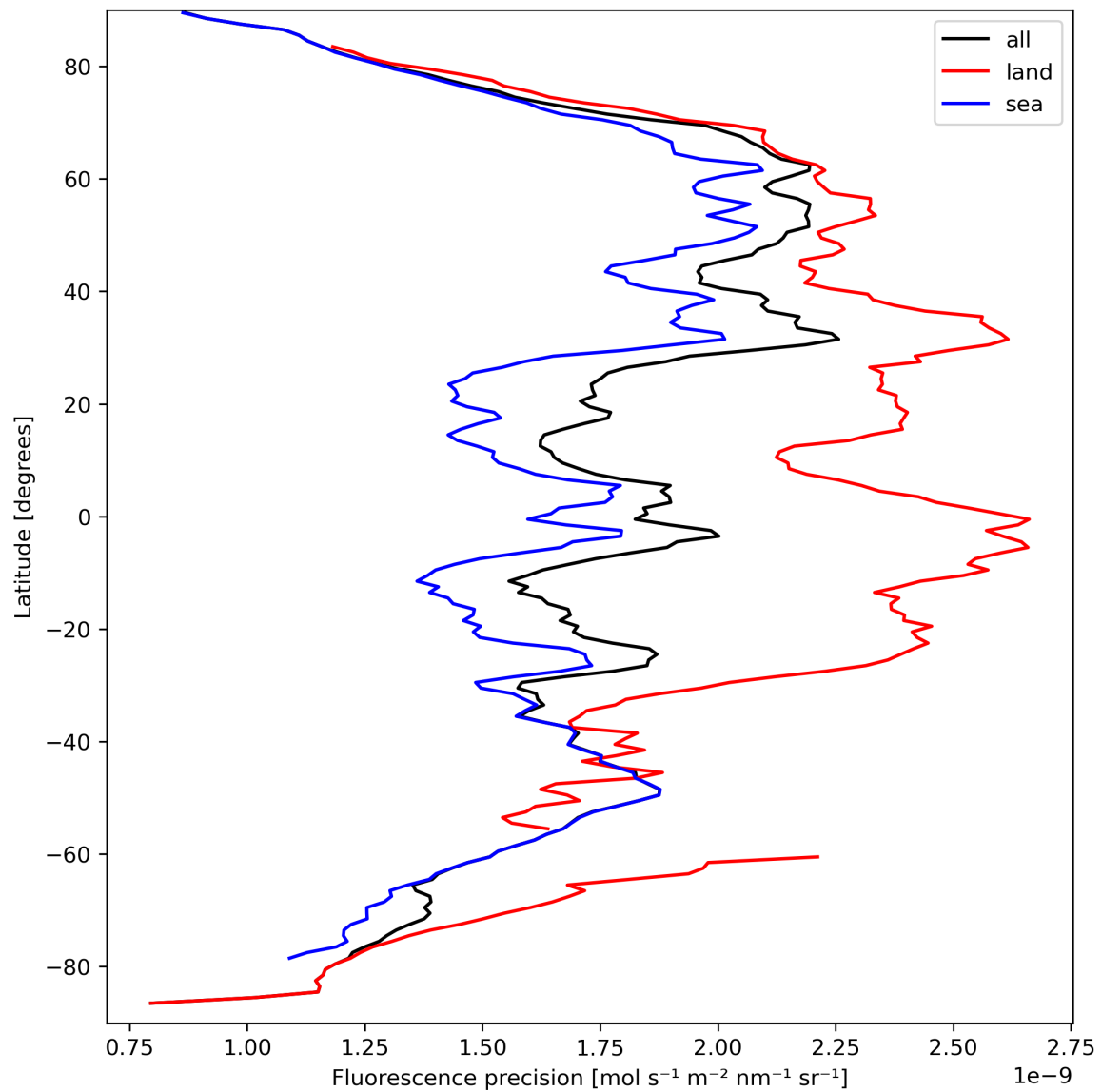
Figure 24: Zonal average of “Fluorescence precision” for 2024-03-23 to 2024-03-25.
