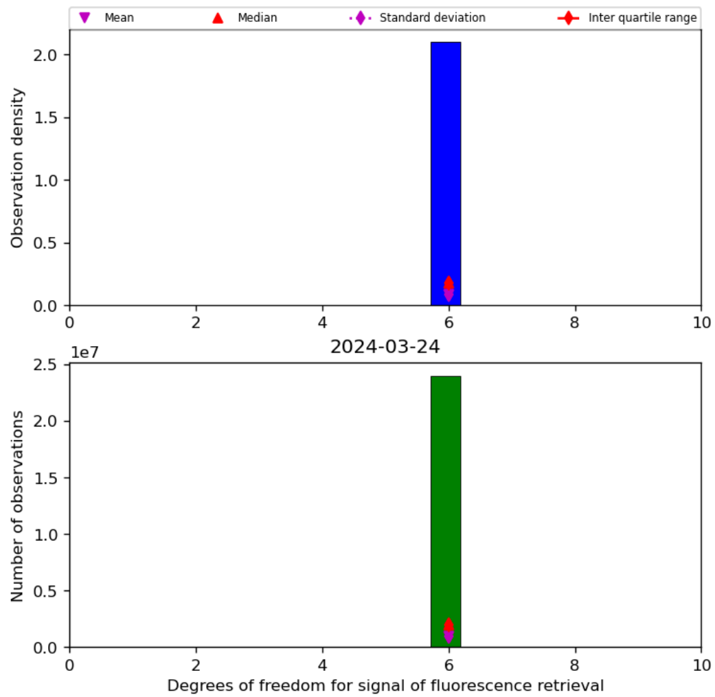
Figure 43: Histogram of "Degrees of freedom for signal of fluorescence retrieval" for 2024-03-23 to 2024-03-25
