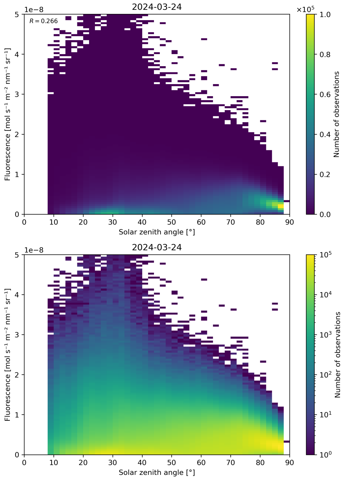
Figure 112: Scatter density plot of “Solar zenith angle” against “Fluorescence” for 2024-03-23 to 2024-03-25.
