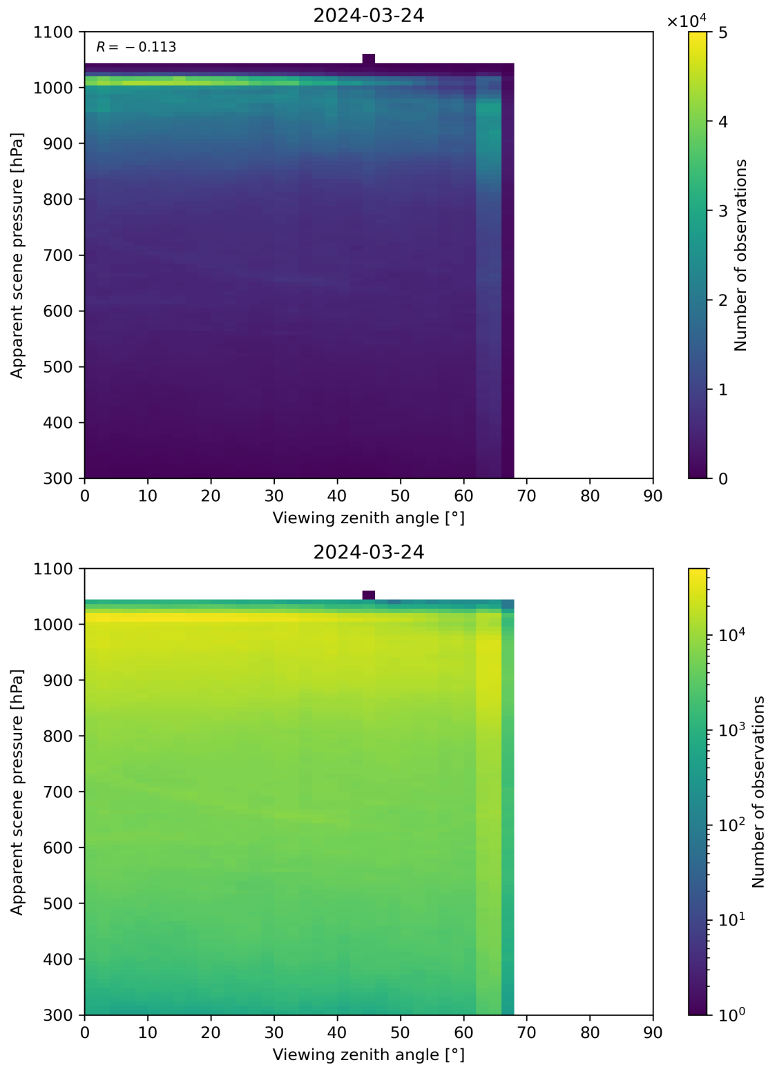
Figure 118: Scatter density plot of “Viewing zenith angle” against “Apparent scene pressure” for 2024-03-23 to 2024-03-25.
