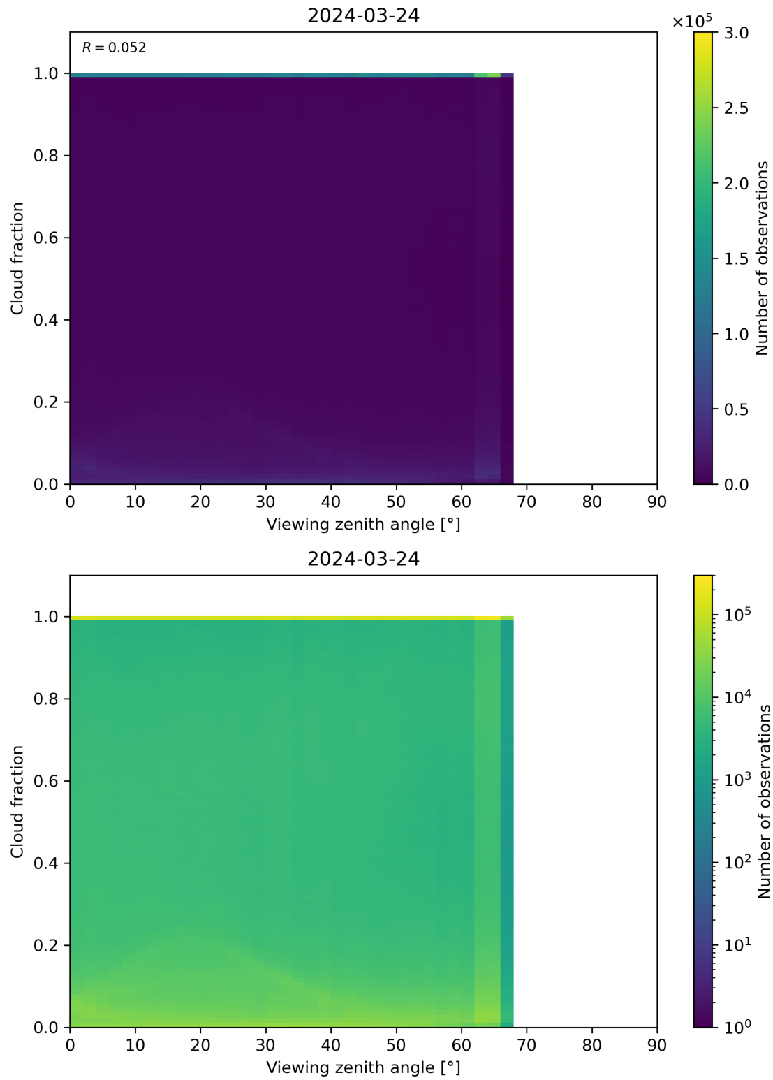
Figure 120: Scatter density plot of “Viewing zenith angle” against “Cloud fraction” for 2024-03-23 to 2024-03-25.
