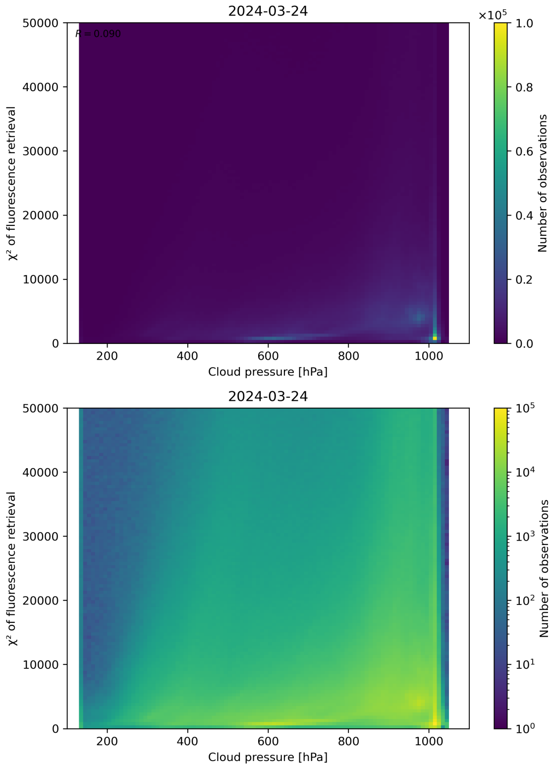
Figure 78: Scatter density plot of “Cloud pressure” against “ \chi^2 of fluorescence retrieval” for 2024-03-23 to 2024-03-25.
