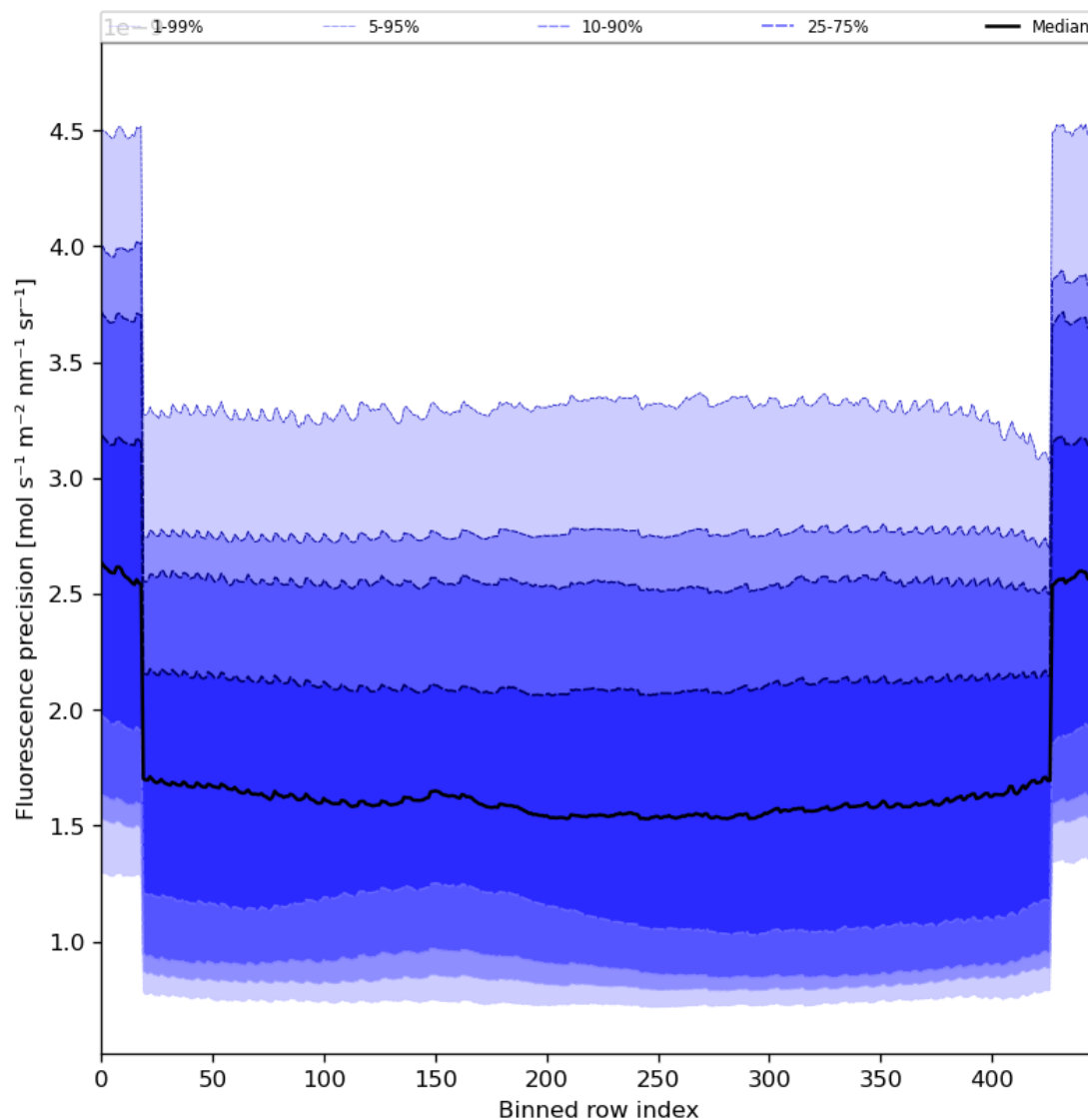
Figure 58: Along track statistics of “Fluorescence precision” for 2024-03-23 to 2024-03-25
