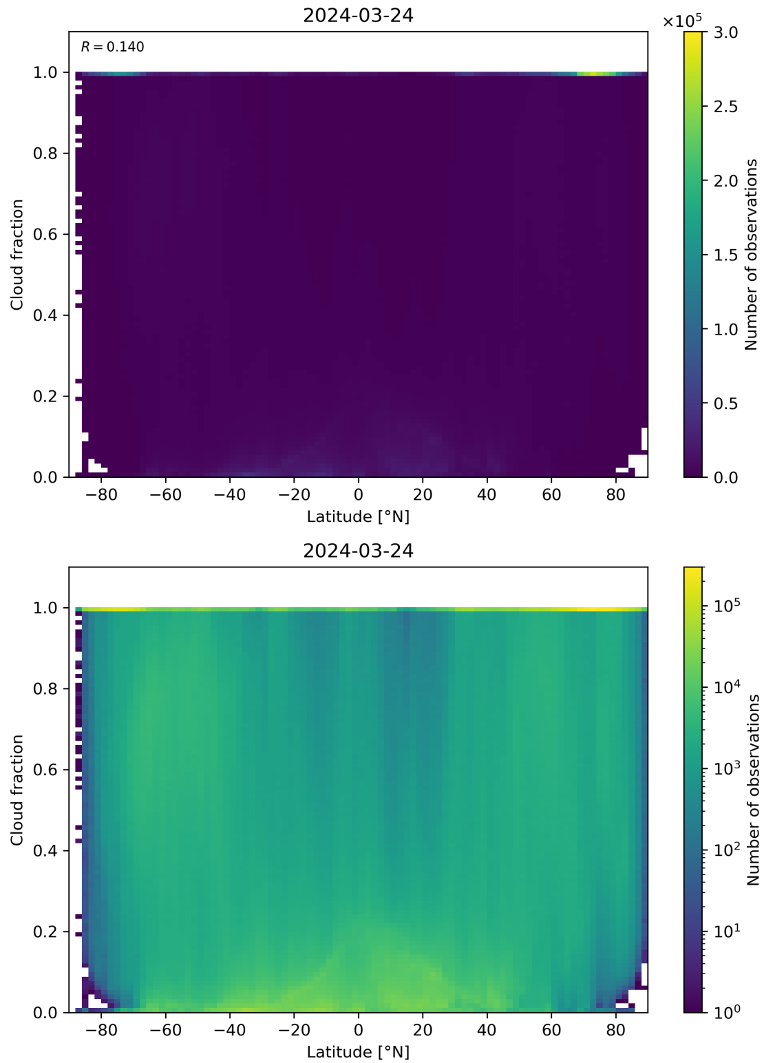
Figure 90: Scatter density plot of “Latitude” against “Cloud fraction” for 2024-03-23 to 2024-03-25.
