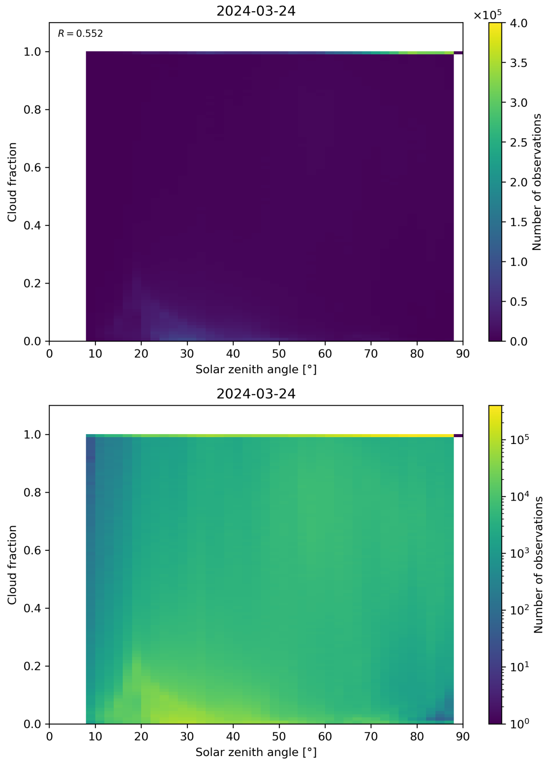
Figure 110: Scatter density plot of “Solar zenith angle” against “Cloud fraction” for 2024-03-23 to 2024-03-25.
