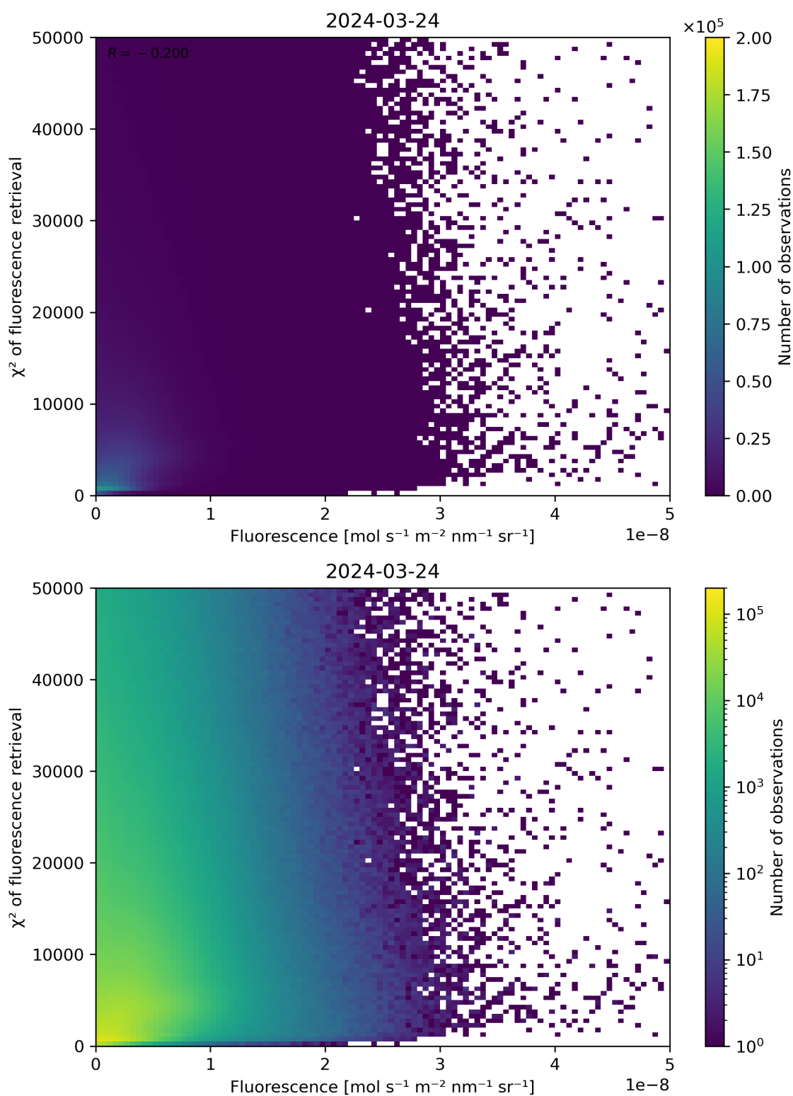
Figure 85: Scatter density plot of “Fluorescence” against “ \chi^2 of fluorescence retrieval” for 2024-03-23 to 2024-03-25.
