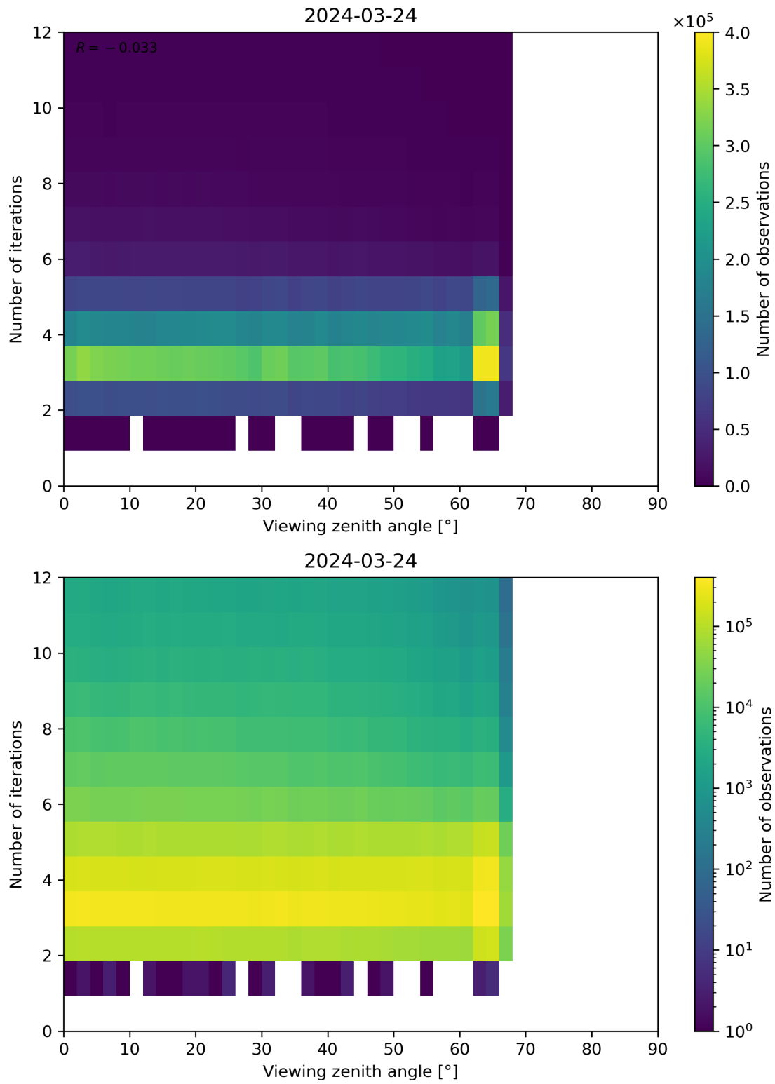
Figure 124: Scatter density plot of “Viewing zenith angle” against “Number of iterations” for 2024-03-23 to 2024-03-25.
