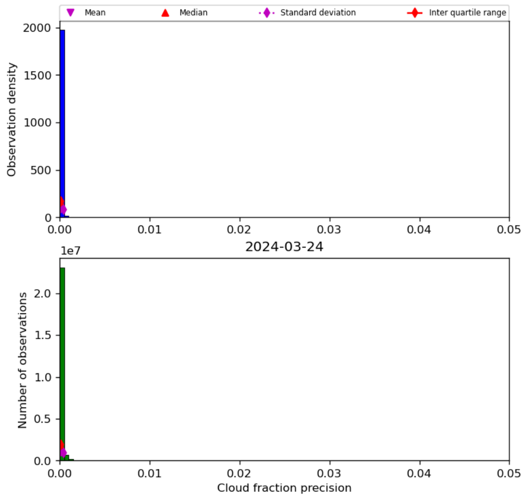
Figure 33: Histogram of “Cloud fraction precision” for 2024-03-23 to 2024-03-25
