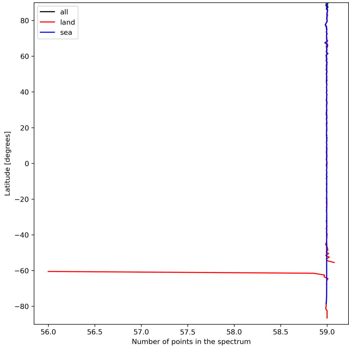
Figure 27: Zonal average of “Number of points in the spectrum” for 2024-03-23 to 2024-03-25.
