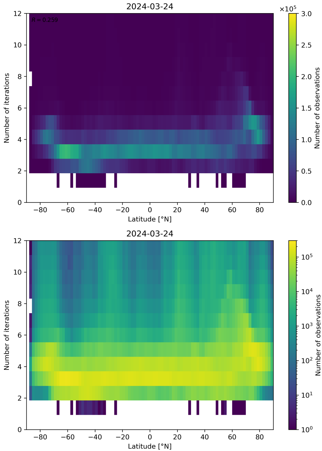
Figure 93: Scatter density plot of “Latitude” against “Number of iterations” for 2024-03-23 to 2024-03-25.
