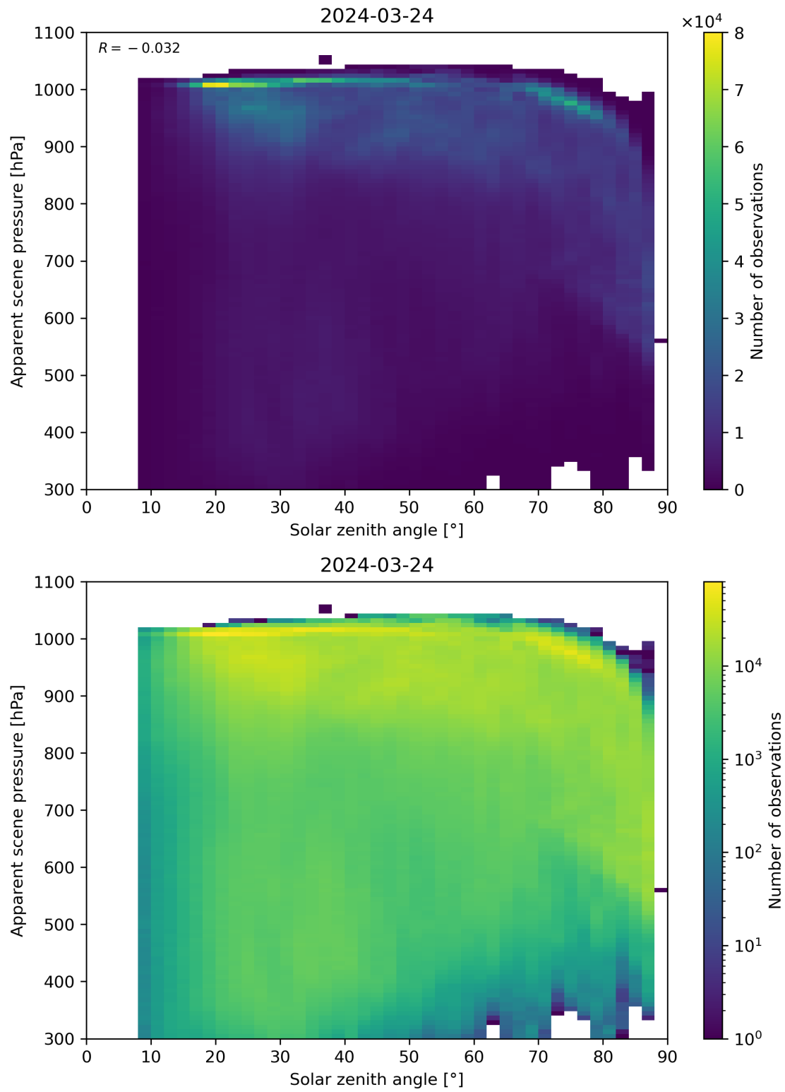
Figure 108: Scatter density plot of “Solar zenith angle” against “Apparent scene pressure” for 2024-03-23 to 2024-03-25.
