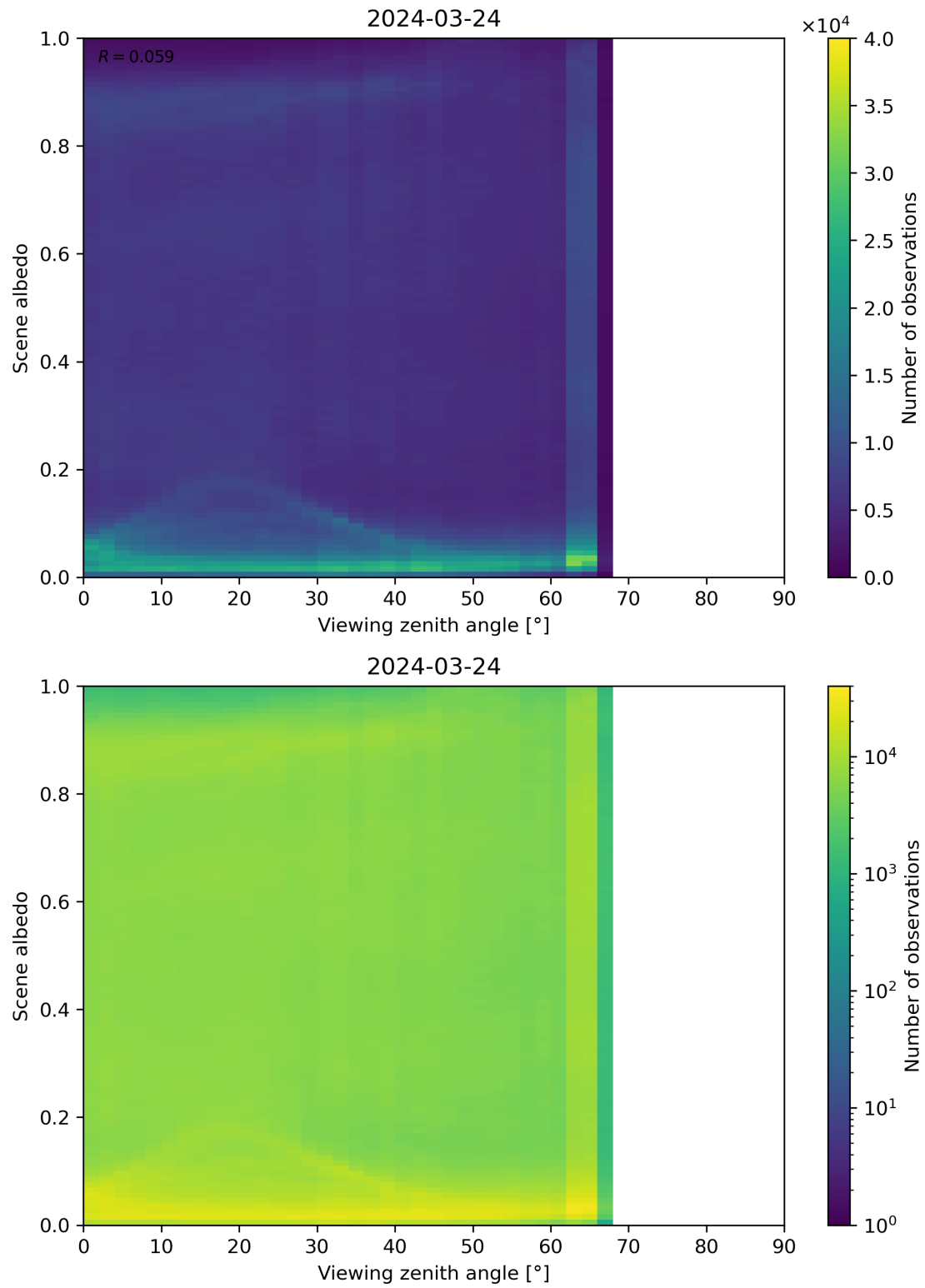
Figure 126: Scatter density plot of “Viewing zenith angle” against “Scene albedo” for 2024-03-23 to 2024-03-25.
