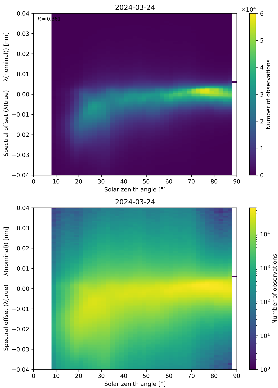
Figure 117: Scatter density plot of “Solar zenith angle” against “Spectral offset ( \lambda(\text{true}) - \lambda(\text{nominal}) )” for 2024-03-23 to 2024-03-25.
