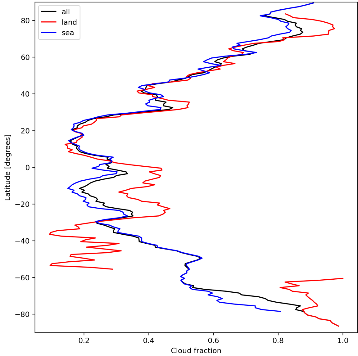
Figure 15: Zonal average of “Cloud fraction” for 2024-03-23 to 2024-03-25.
