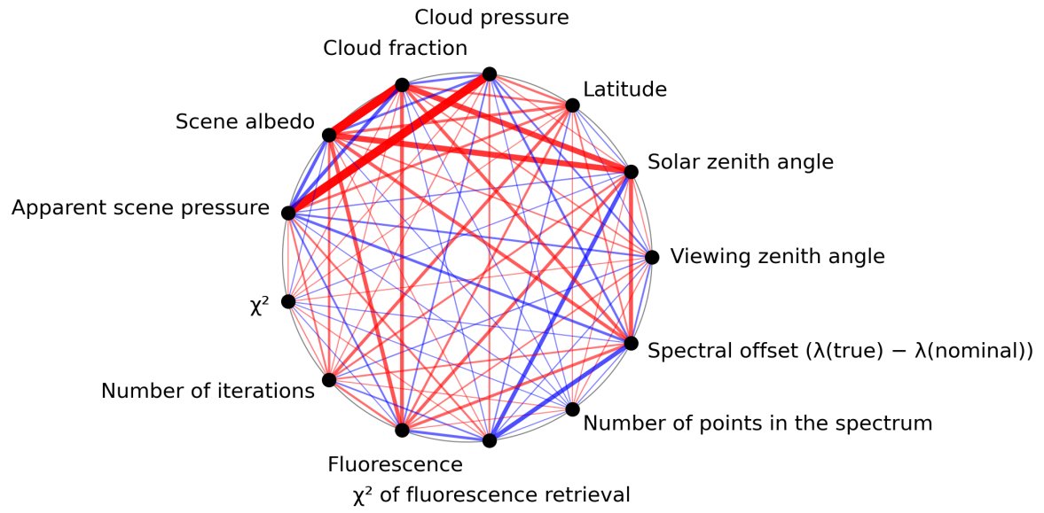
Figure 1: Map of correlation graph for 2024-03-23 to 2024-03-25.
