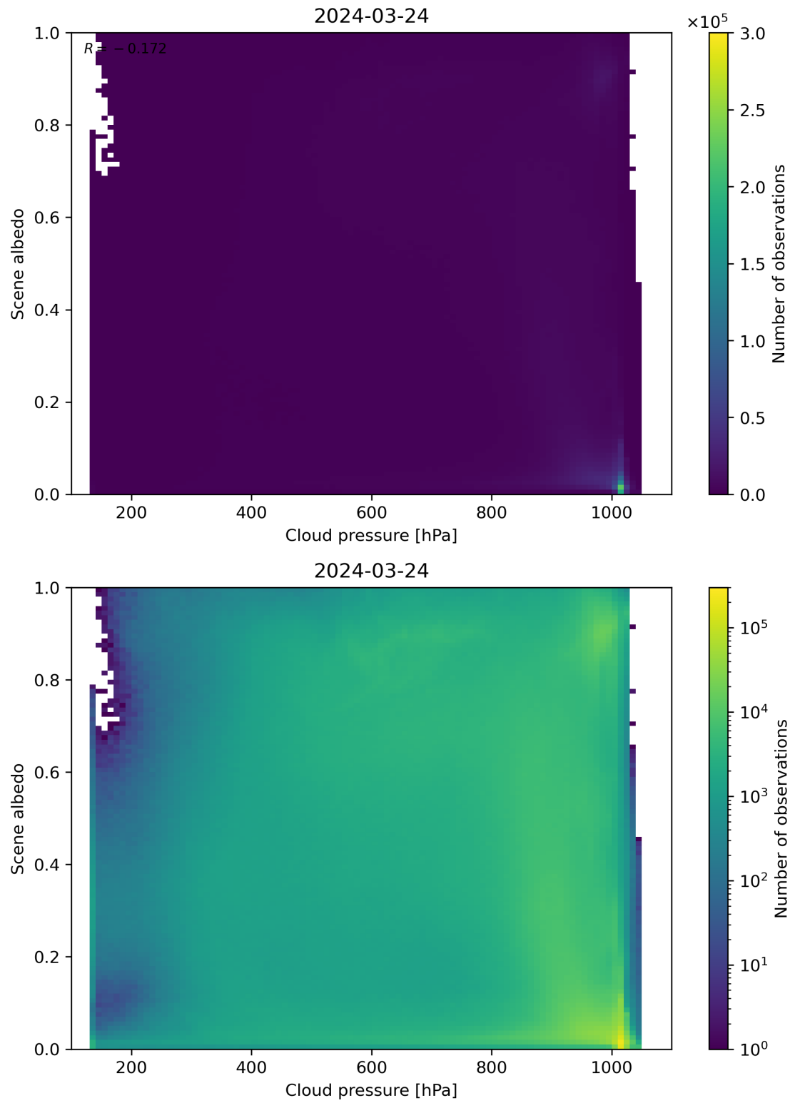
Figure 83: Scatter density plot of “Cloud pressure” against “Scene albedo” for 2024-03-23 to 2024-03-25.
