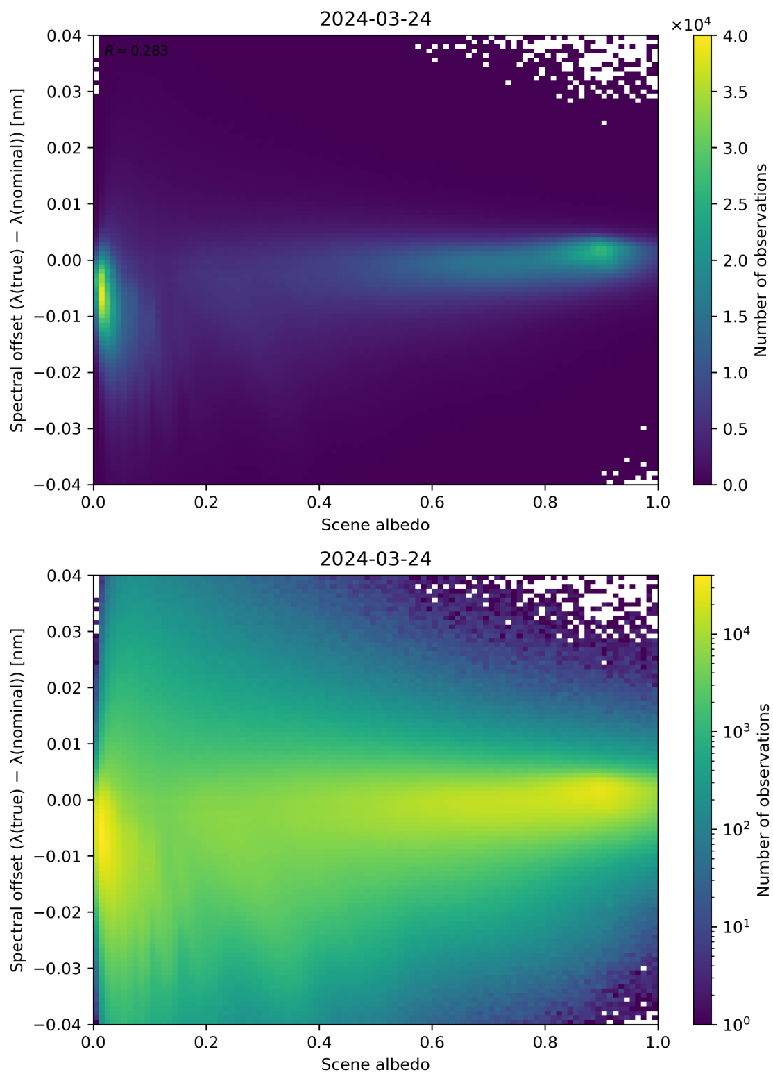
Figure 107: Scatter density plot of “Scene albedo” against “Spectral offset ( \lambda(\text{true}) - \lambda(\text{nominal}) )” for 2024-03-23 to 2024-03-25.
