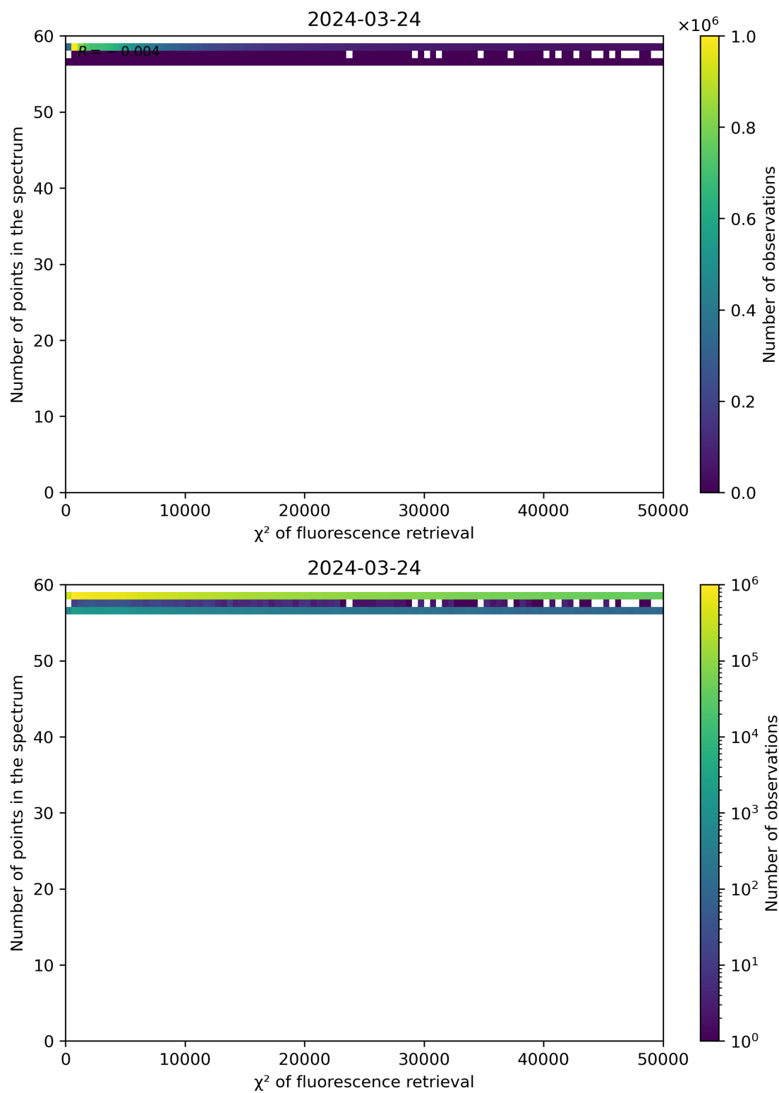
Figure 68: Scatter density plot of “ \chi^2 of fluorescence retrieval” against “Number of points in the spectrum” for 2024-03-23 to 2024-03-25.
