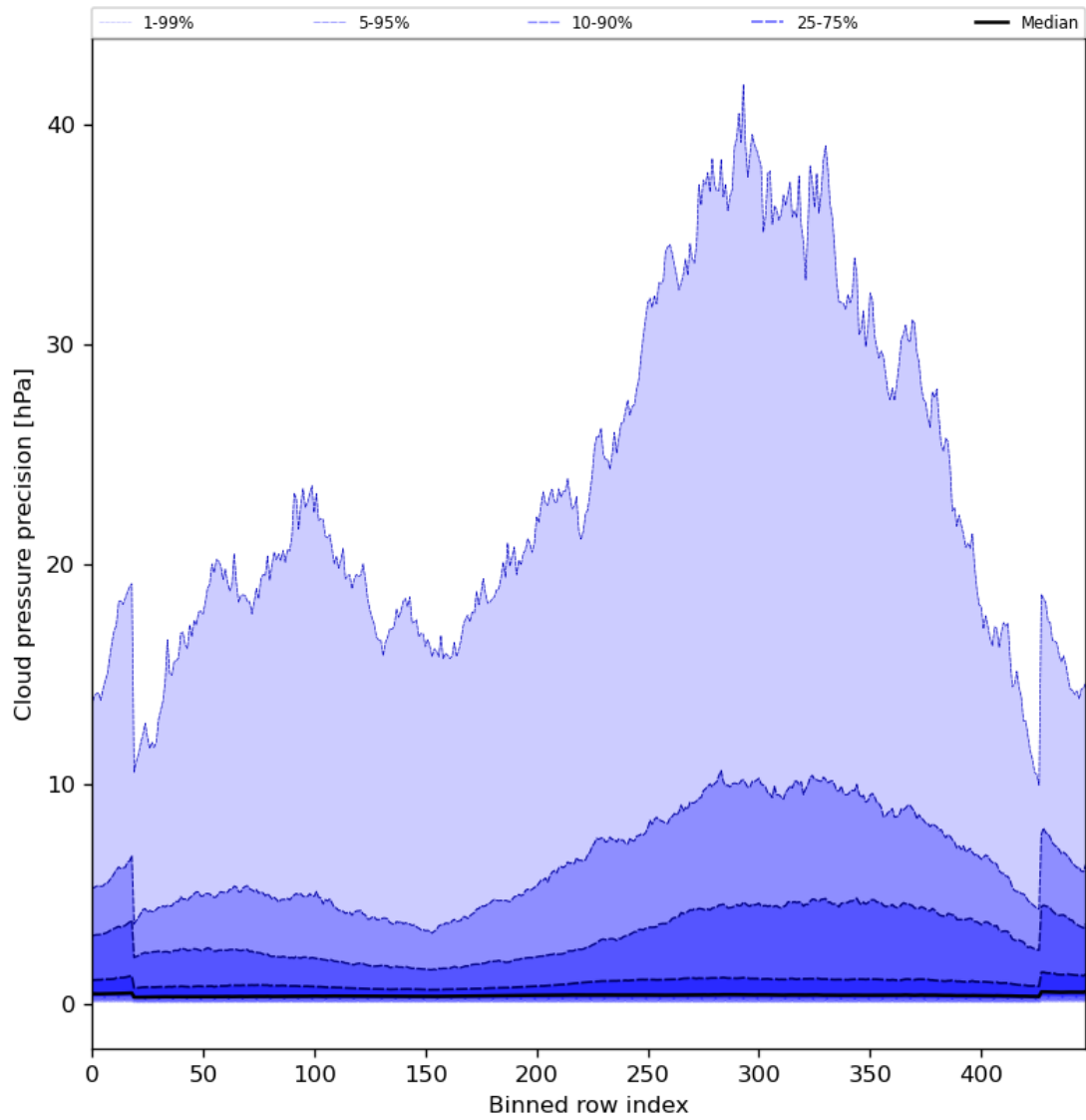
Figure 48: Along track statistics of “Cloud pressure precision” for 2024-03-23 to 2024-03-25
