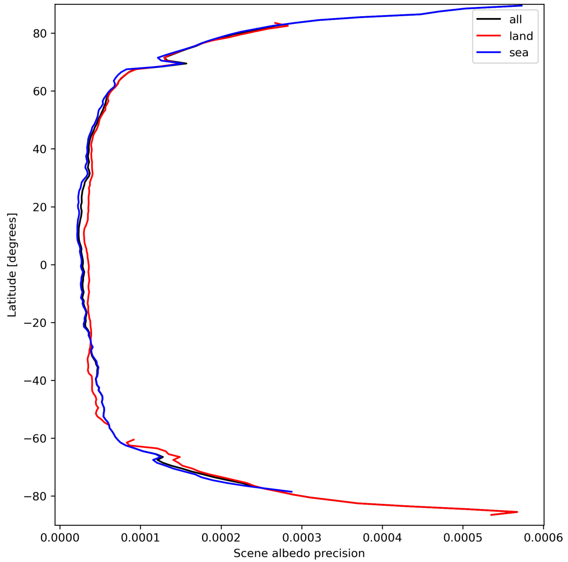
Figure 18: Zonal average of “Scene albedo precision” for 2024-03-23 to 2024-03-25.
