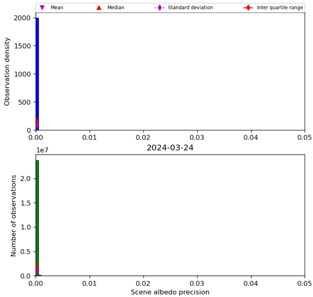
Figure 35: Histogram of “Scene albedo precision” for 2024-03-23 to 2024-03-25
