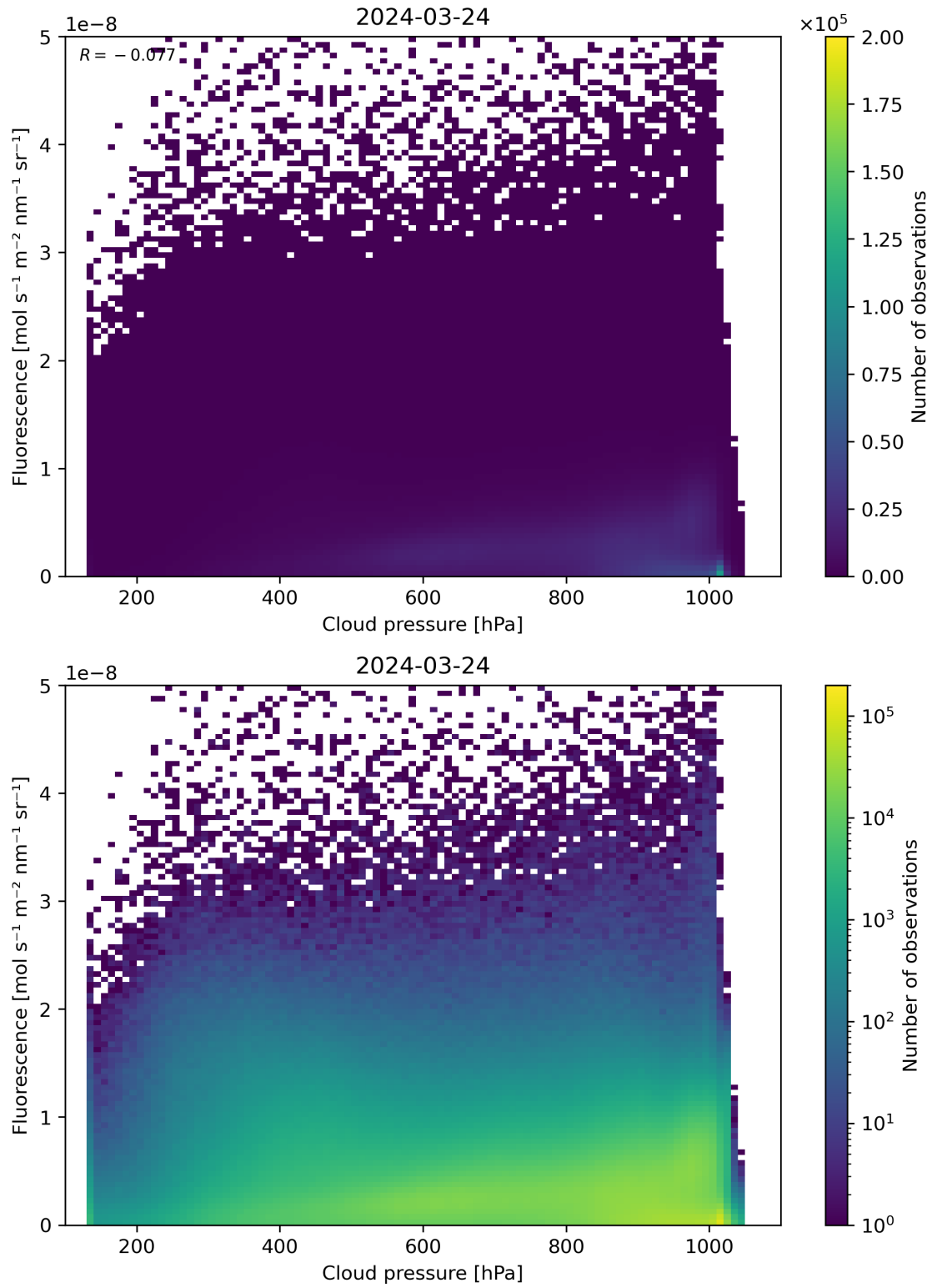
Figure 80: Scatter density plot of “Cloud pressure” against “Fluorescence” for 2024-03-23 to 2024-03-25.
