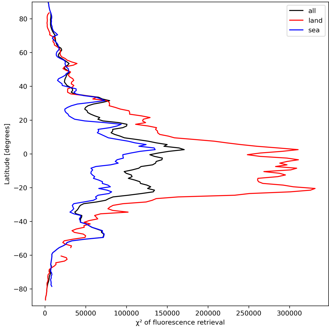
Figure 25: Zonal average of “ \chi^2 of fluorescence retrieval” for 2024-03-23 to 2024-03-25.
