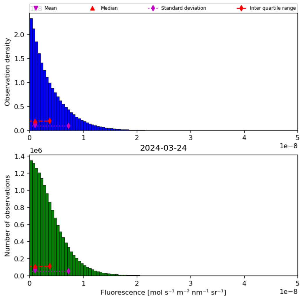
Figure 40: Histogram of “Fluorescence” for 2024-03-23 to 2024-03-25
