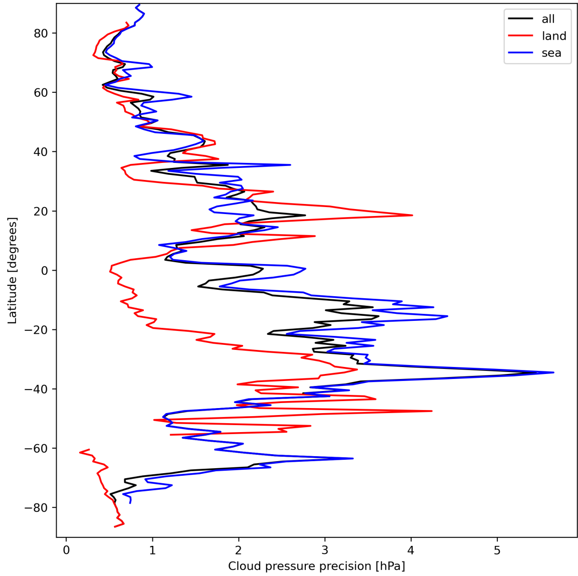
Figure 14: Zonal average of “Cloud pressure precision” for 2024-03-23 to 2024-03-25.
