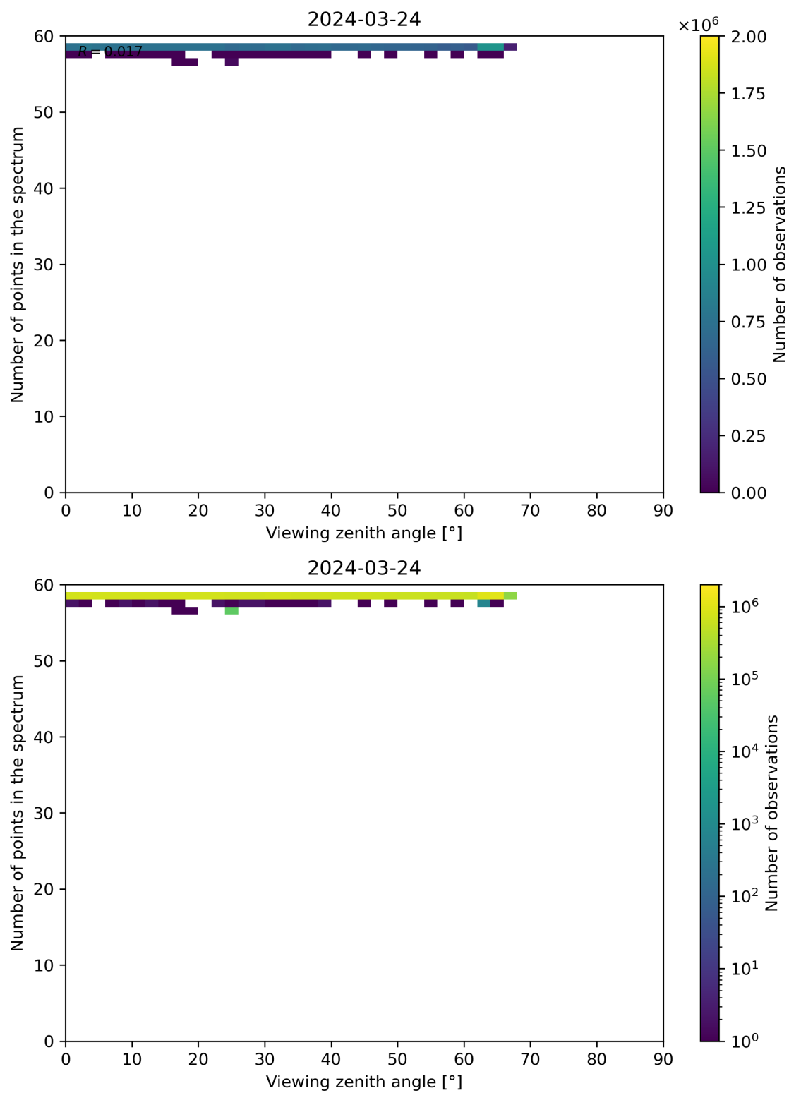
Figure 125: Scatter density plot of “Viewing zenith angle” against “Number of points in the spectrum” for 2024-03-23 to 2024-03-25.
