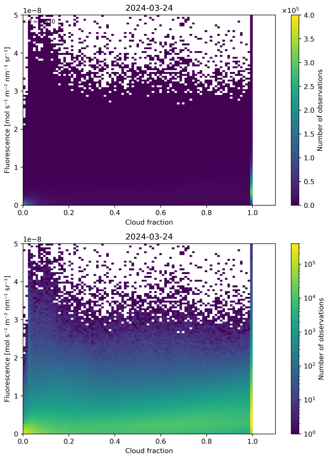
Figure 72: Scatter density plot of “Cloud fraction” against “Fluorescence” for 2024-03-23 to 2024-03-25.
