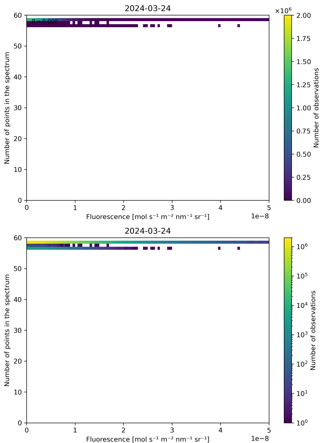
Figure 86: Scatter density plot of “Fluorescence” against “Number of points in the spectrum” for 2024-03-23 to 2024-03-25.
