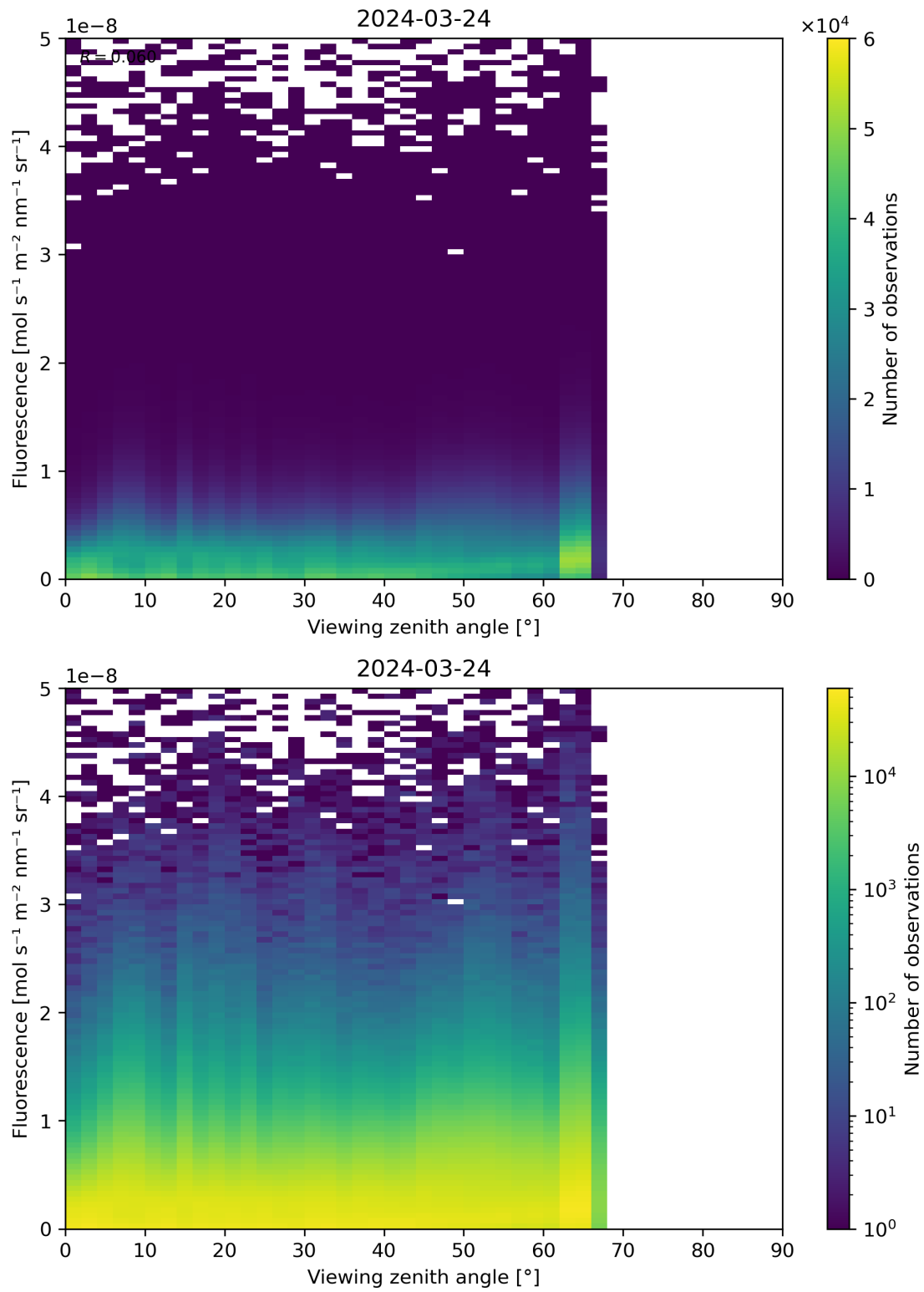
Figure 122: Scatter density plot of “Viewing zenith angle” against “Fluorescence” for 2024-03-23 to 2024-03-25.
