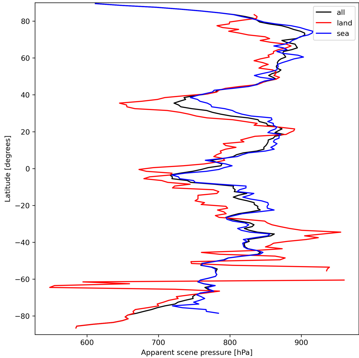
Figure 19: Zonal average of “Apparent scene pressure” for 2024-03-23 to 2024-03-25.
