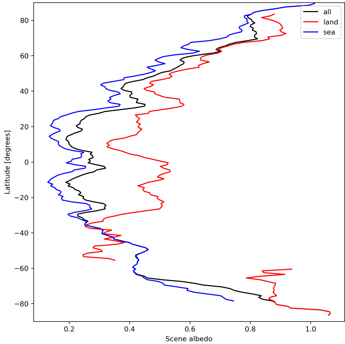
Figure 17: Zonal average of “Scene albedo” for 2024-03-23 to 2024-03-25.
