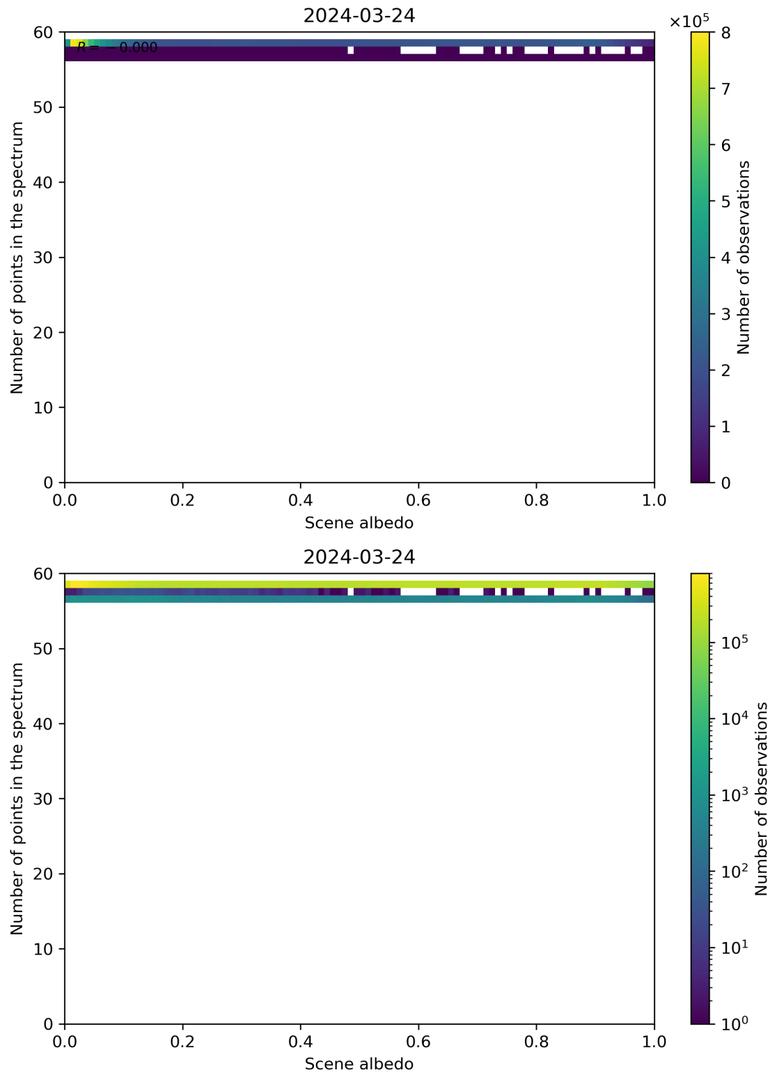
Figure 106: Scatter density plot of “Scene albedo” against “Number of points in the spectrum” for 2024-03-23 to 2024-03-25.
