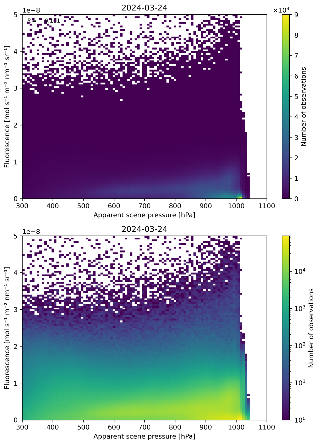
Figure 64: Scatter density plot of “Apparent scene pressure” against “Fluorescence” for 2024-03-23 to 2024-03-25.
