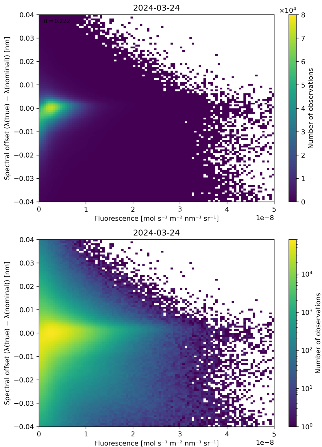
Figure 87: Scatter density plot of “Fluorescence” against “Spectral offset ( \lambda(\text{true}) - \lambda(\text{nominal}) )” for 2024-03-23 to 2024-03-25.
