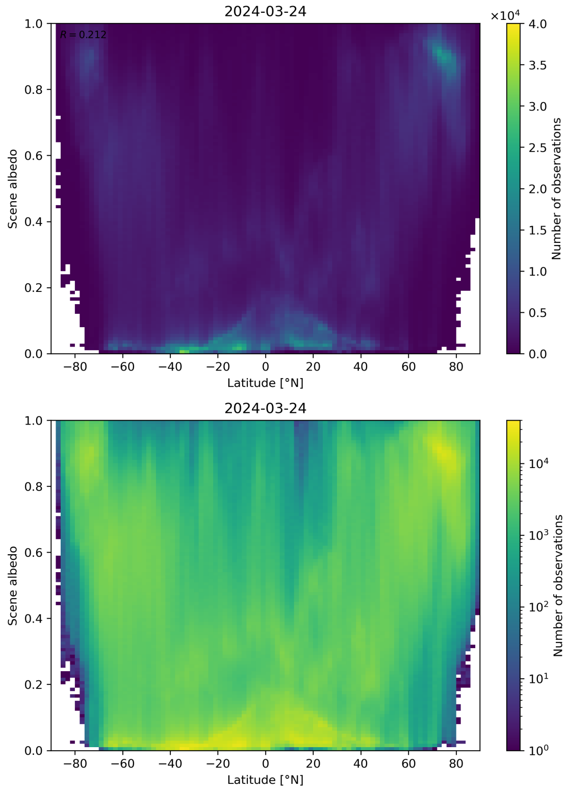
Figure 95: Scatter density plot of “Latitude” against “Scene albedo” for 2024-03-23 to 2024-03-25.
