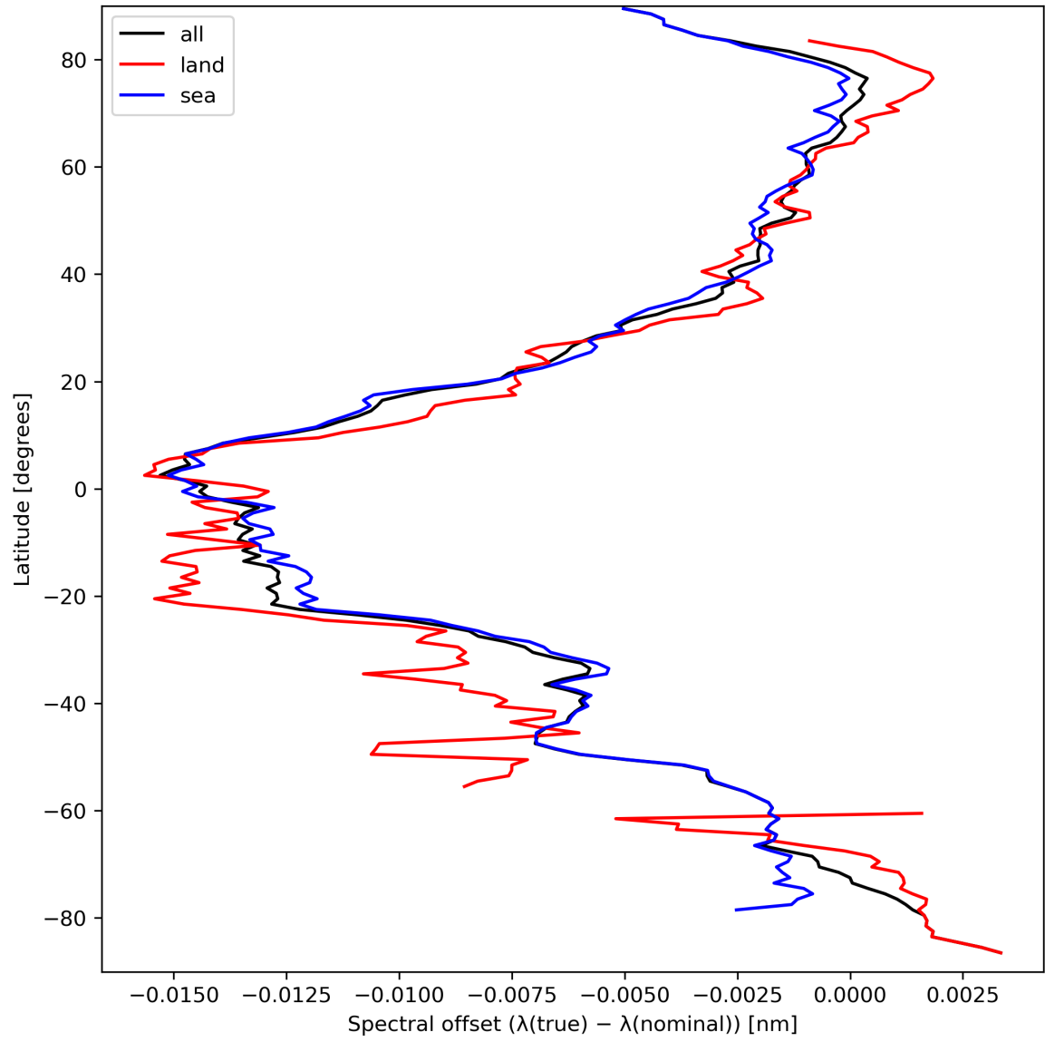
Figure 28: Zonal average of “Spectral offset ( \lambda(\text{true}) - \lambda(\text{nominal}) )” for 2024-03-23 to 2024-03-25.
