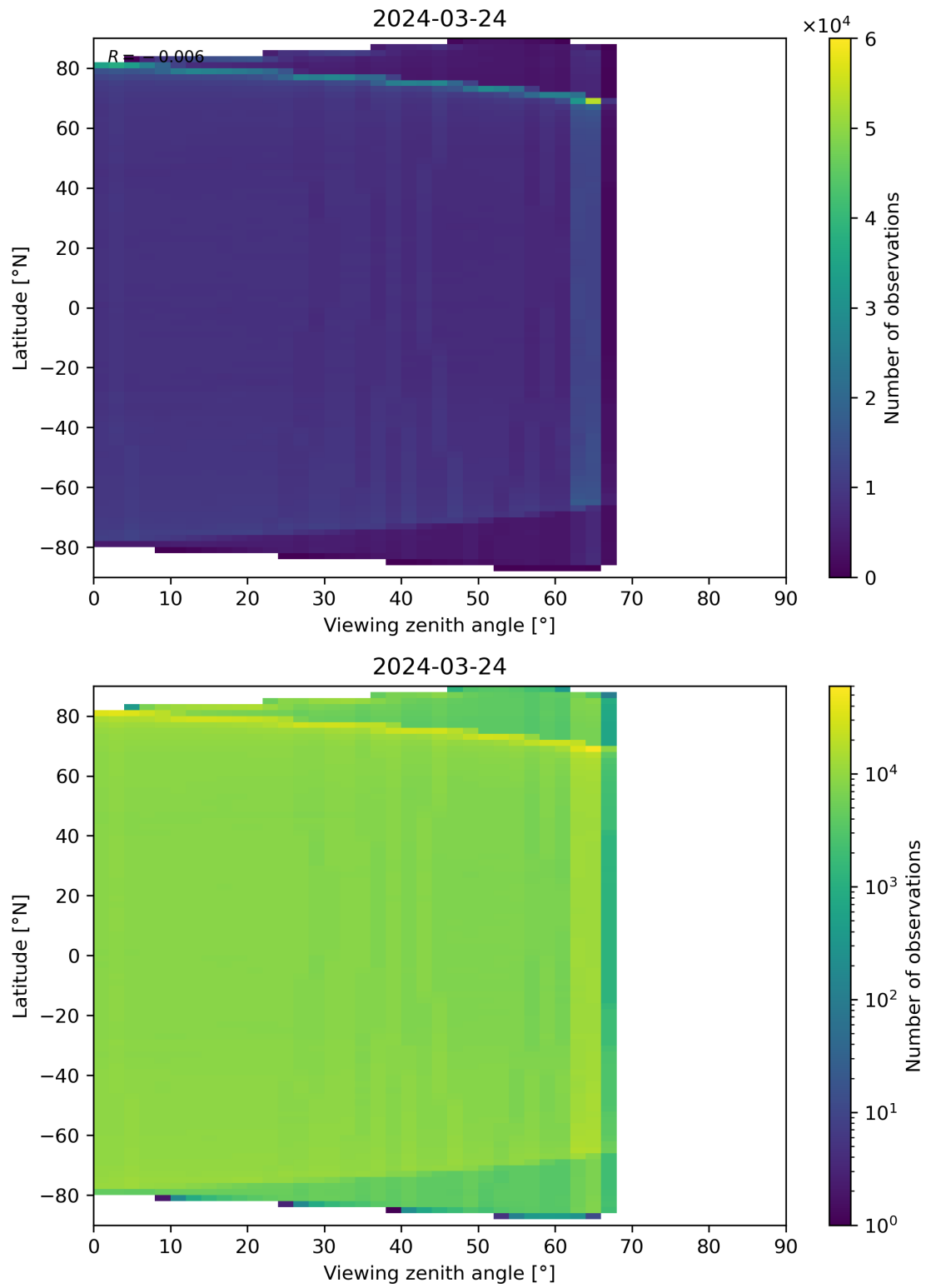
Figure 123: Scatter density plot of “Viewing zenith angle” against “Latitude” for 2024-03-23 to 2024-03-25.
