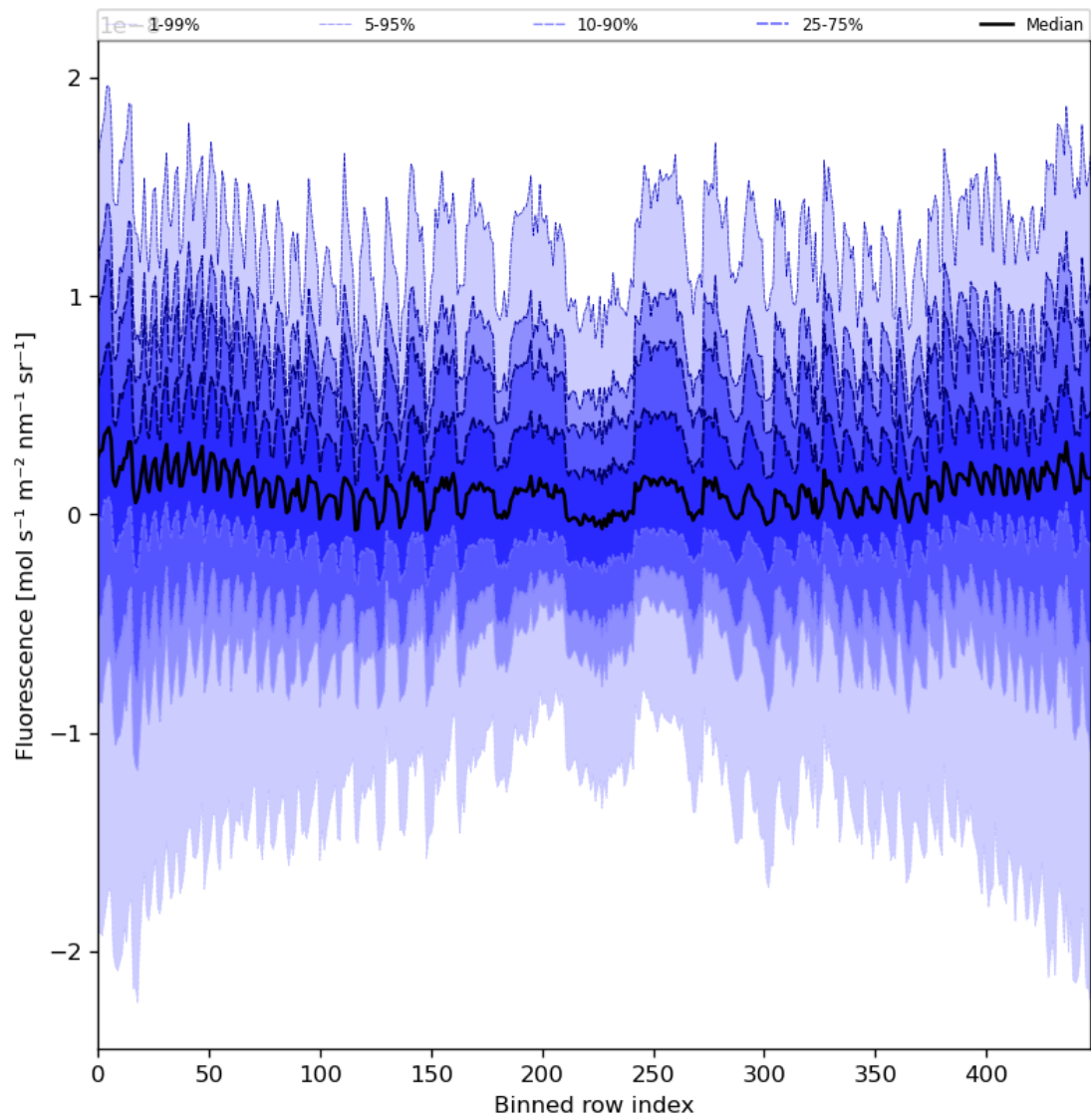
Figure 57: Along track statistics of “Fluorescence” for 2024-03-23 to 2024-03-25
