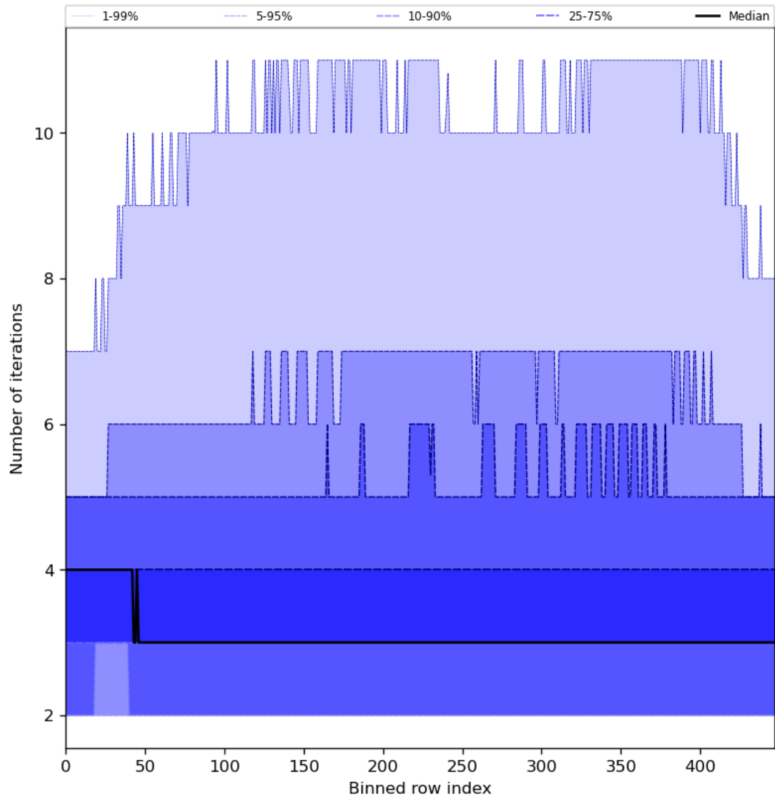
Figure 56: Along track statistics of “Number of iterations” for 2024-03-25 to 2024-03-26
