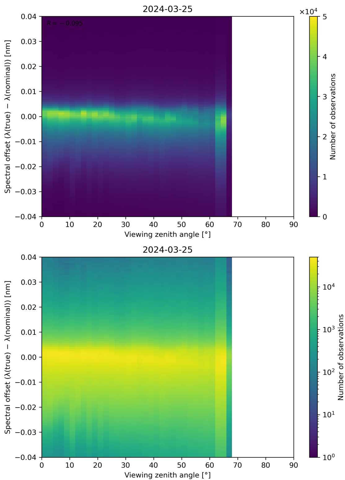
Figure 128: Scatter density plot of “Viewing zenith angle” against “Spectral offset ( \lambda(\text{true}) - \lambda(\text{nominal}) )” for 2024-03-25 to 2024-03-26.
