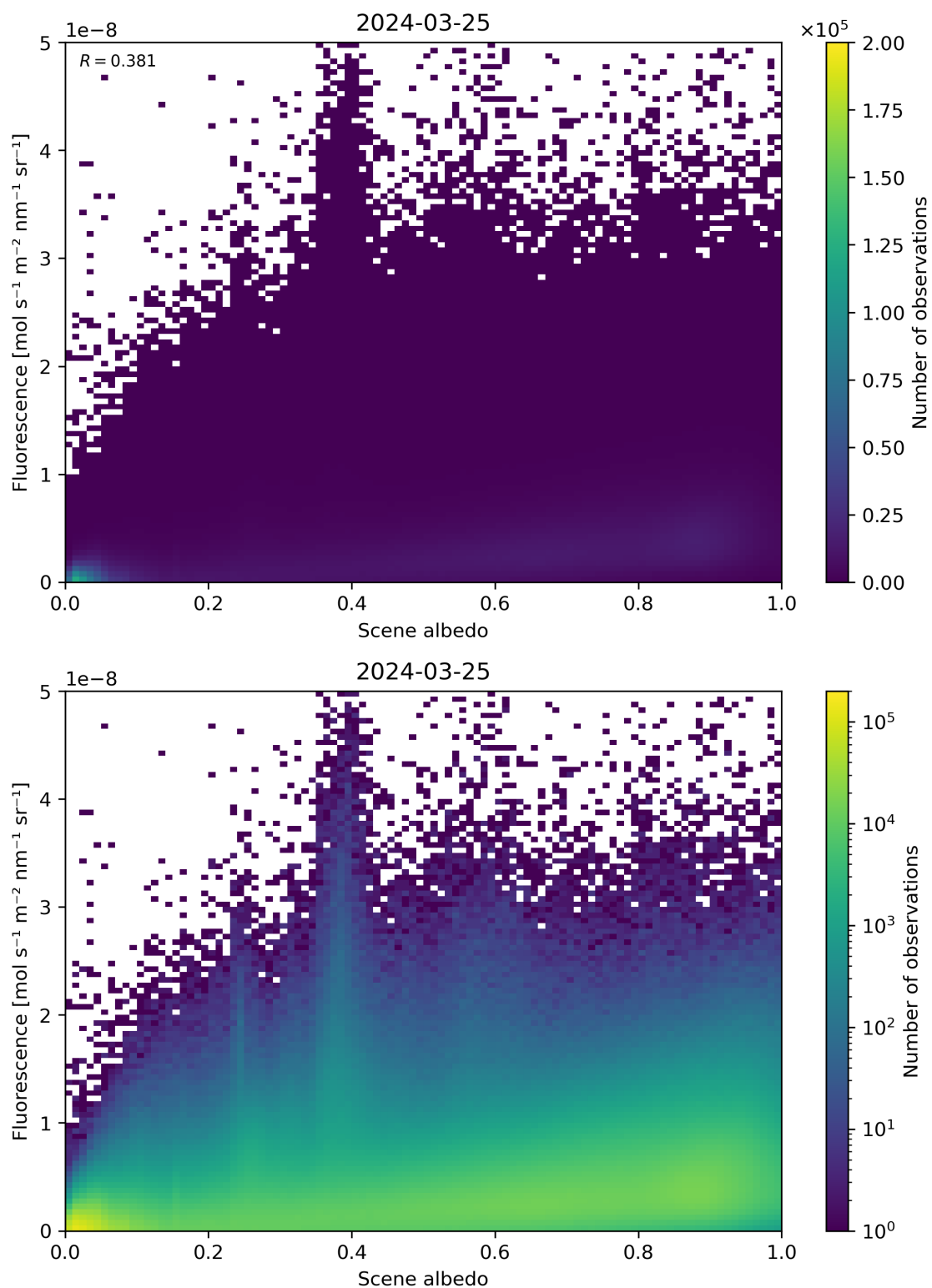
Figure 104: Scatter density plot of “Scene albedo” against “Fluorescence” for 2024-03-25 to 2024-03-26.
