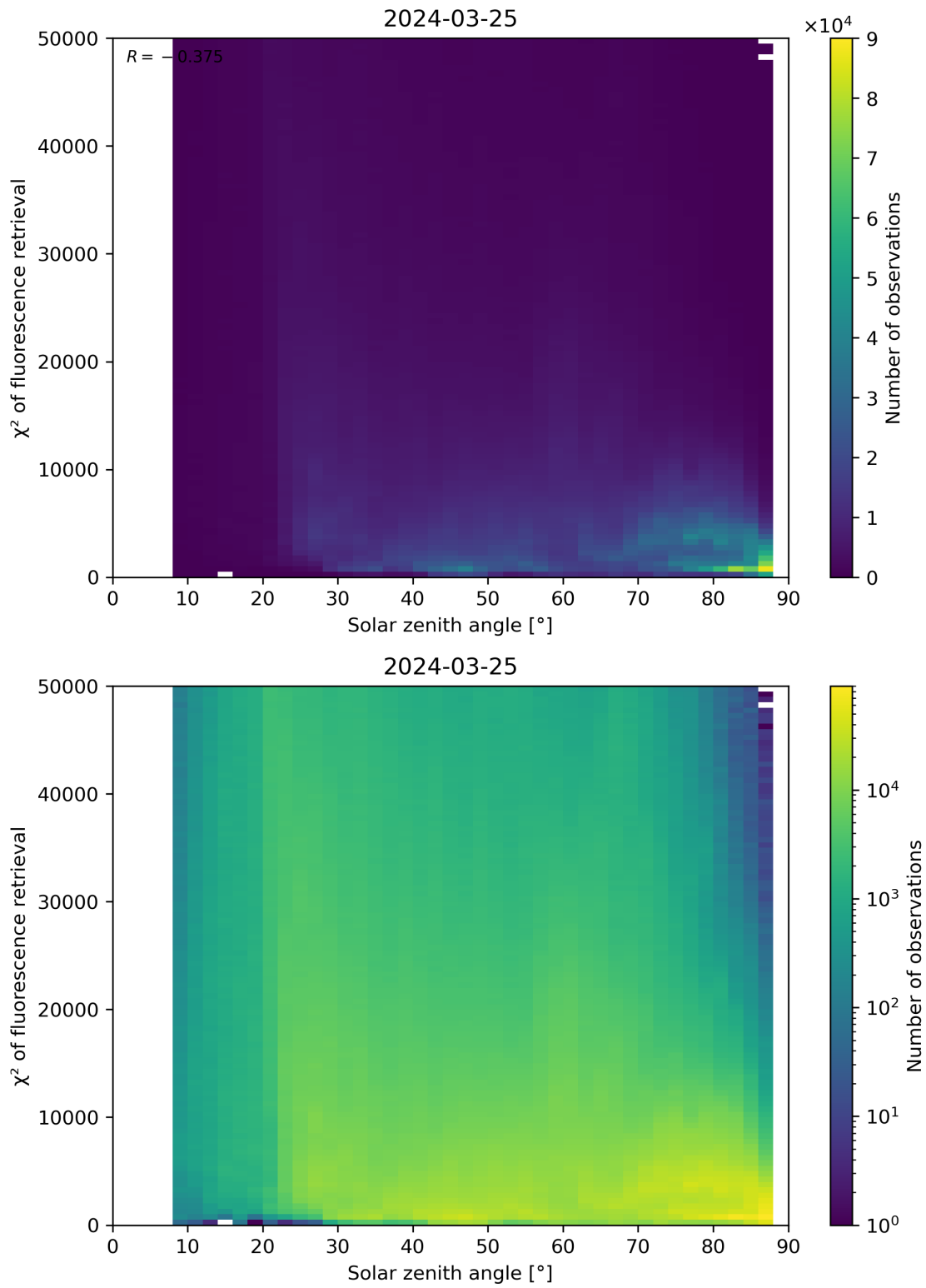
Figure 109: Scatter density plot of “Solar zenith angle” against “ \chi^2 of fluorescence retrieval” for 2024-03-25 to 2024-03-26.
