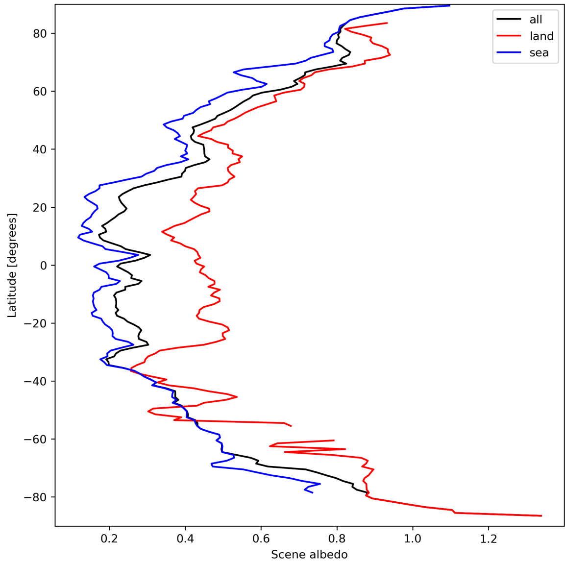
Figure 17: Zonal average of “Scene albedo” for 2024-03-25 to 2024-03-26.
