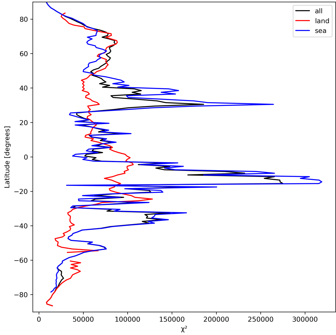
Figure 21: Zonal average of “ \chi^2 ” for 2024-03-25 to 2024-03-26.
