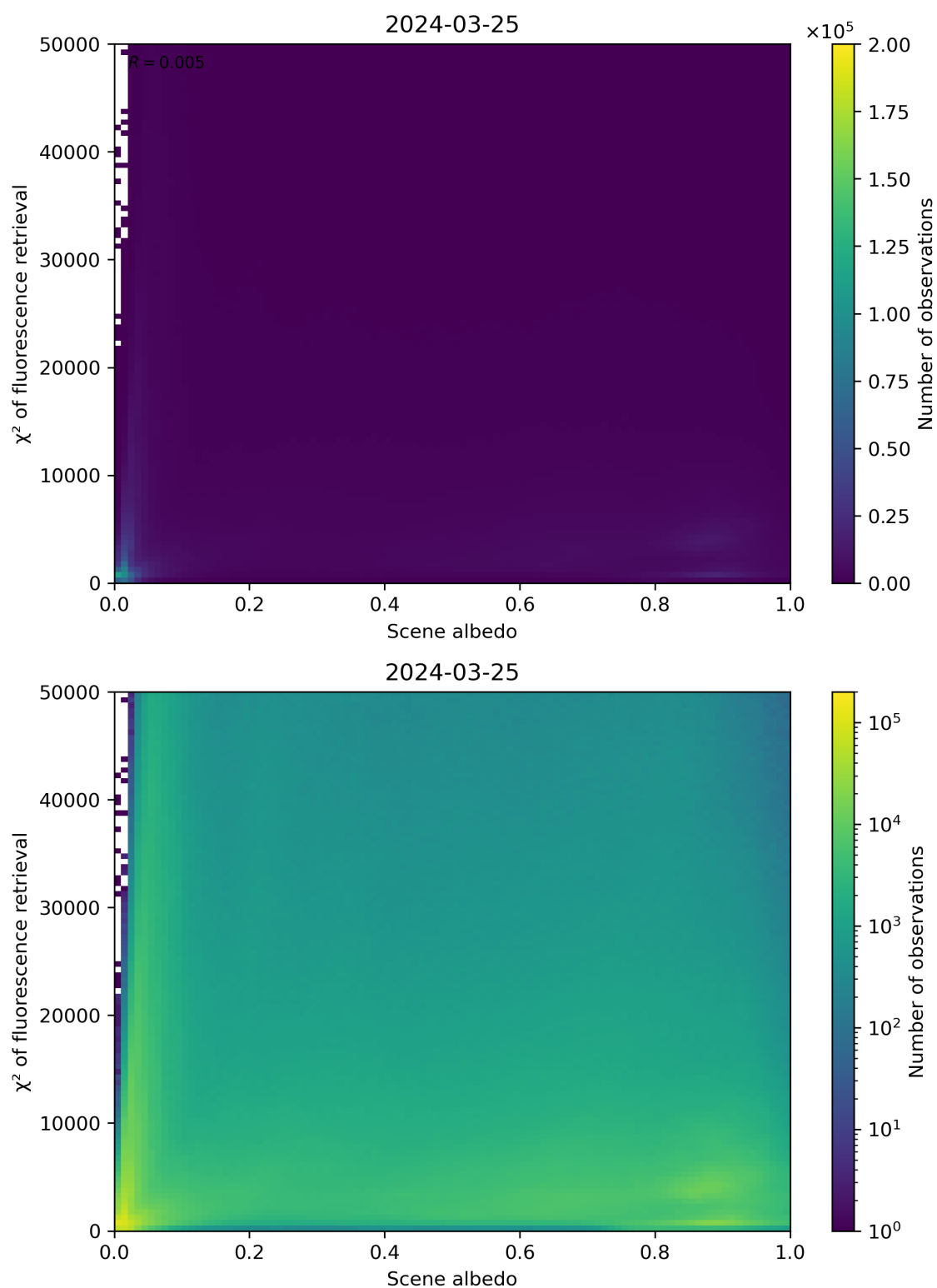
Figure 103: Scatter density plot of “Scene albedo” against “ \chi^2 of fluorescence retrieval” for 2024-03-25 to 2024-03-26.
