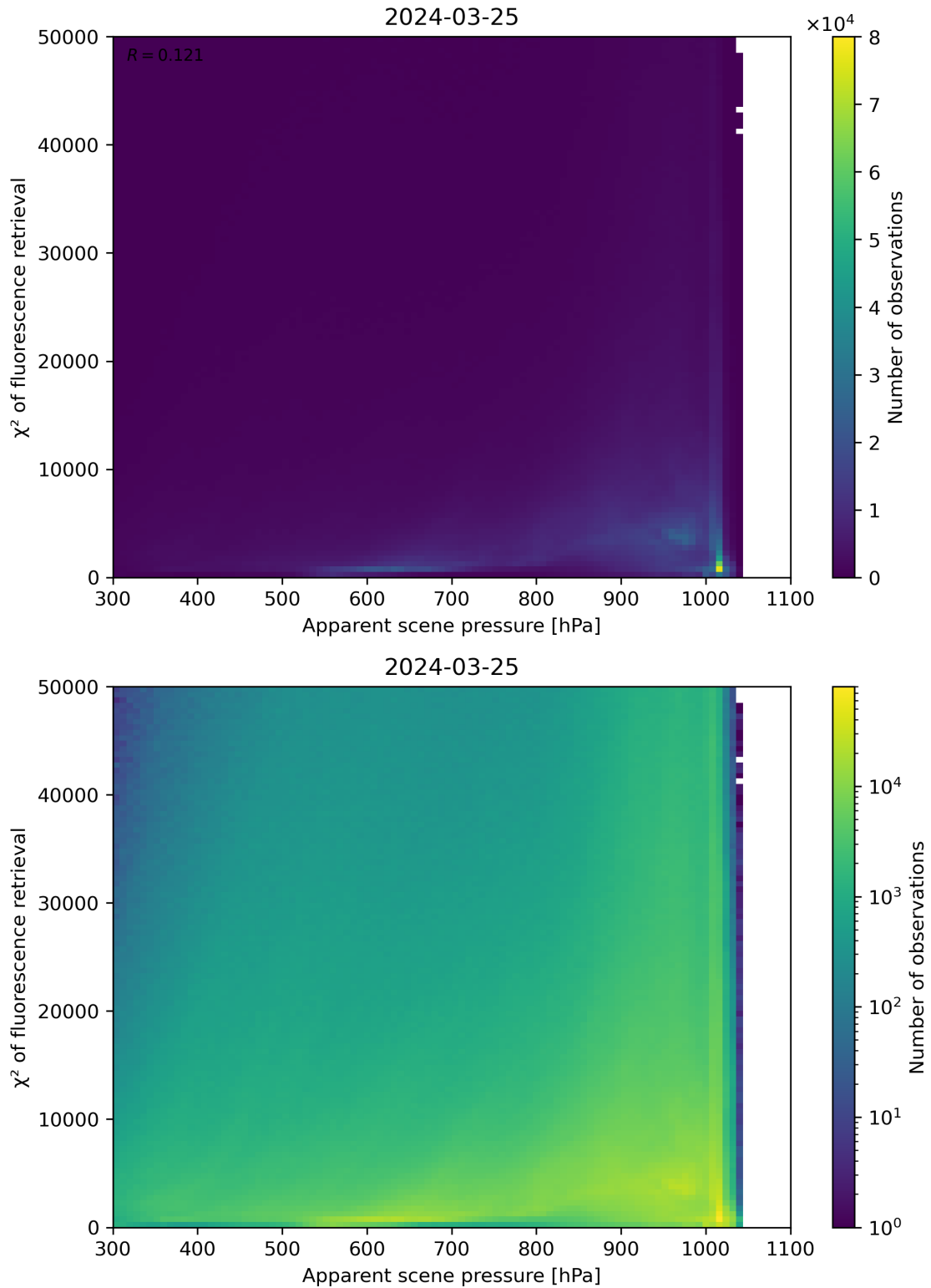
Figure 63: Scatter density plot of “Apparent scene pressure” against “ \chi^2 of fluorescence retrieval” for 2024-03-25 to 2024-03-26.
