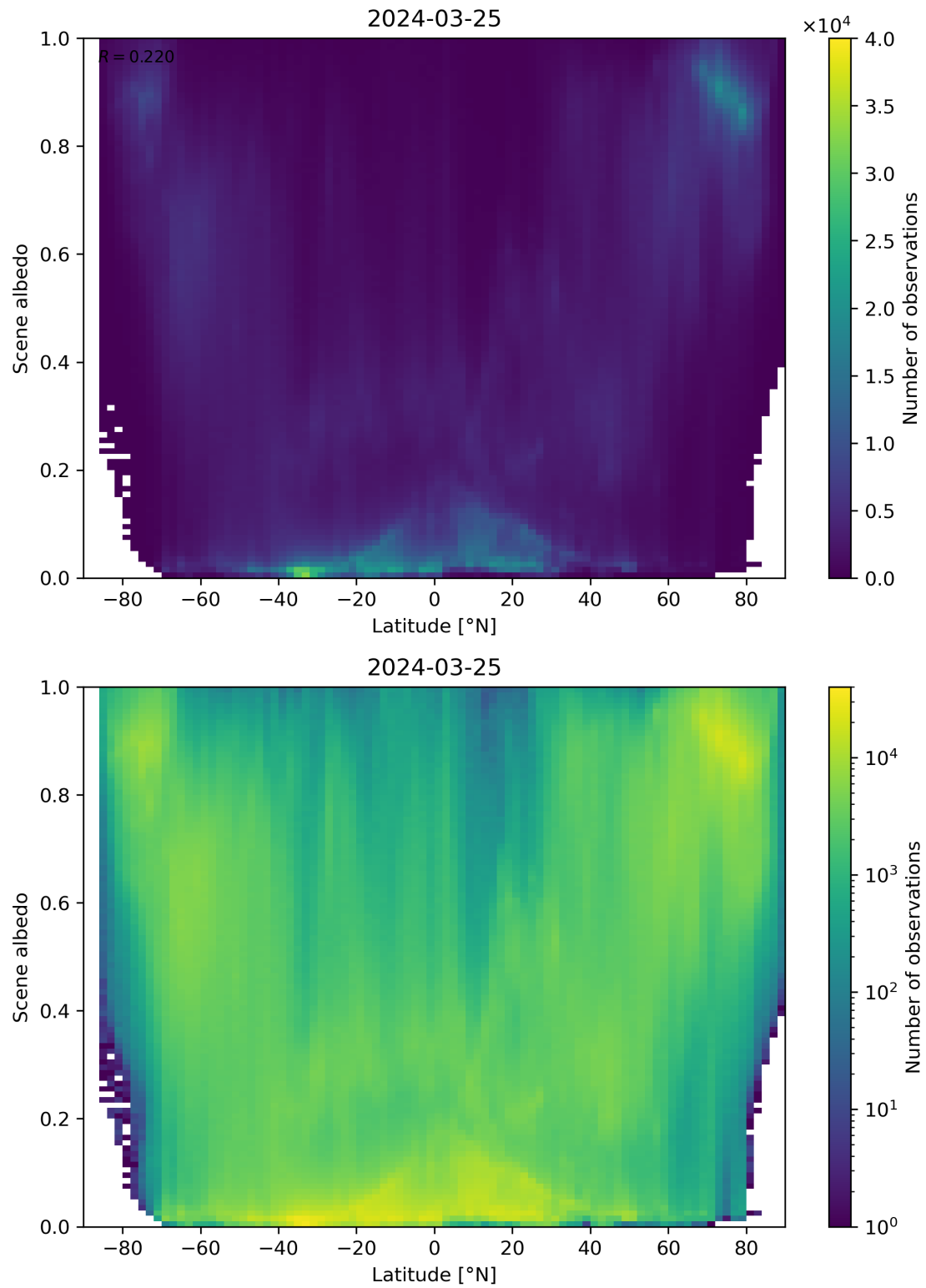
Figure 95: Scatter density plot of “Latitude” against “Scene albedo” for 2024-03-25 to 2024-03-26.
