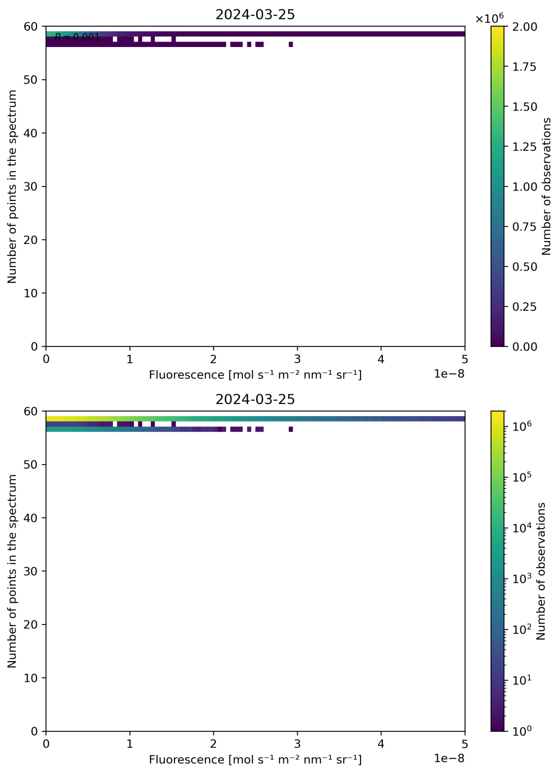
Figure 86: Scatter density plot of “Fluorescence” against “Number of points in the spectrum” for 2024-03-25 to 2024-03-26.
