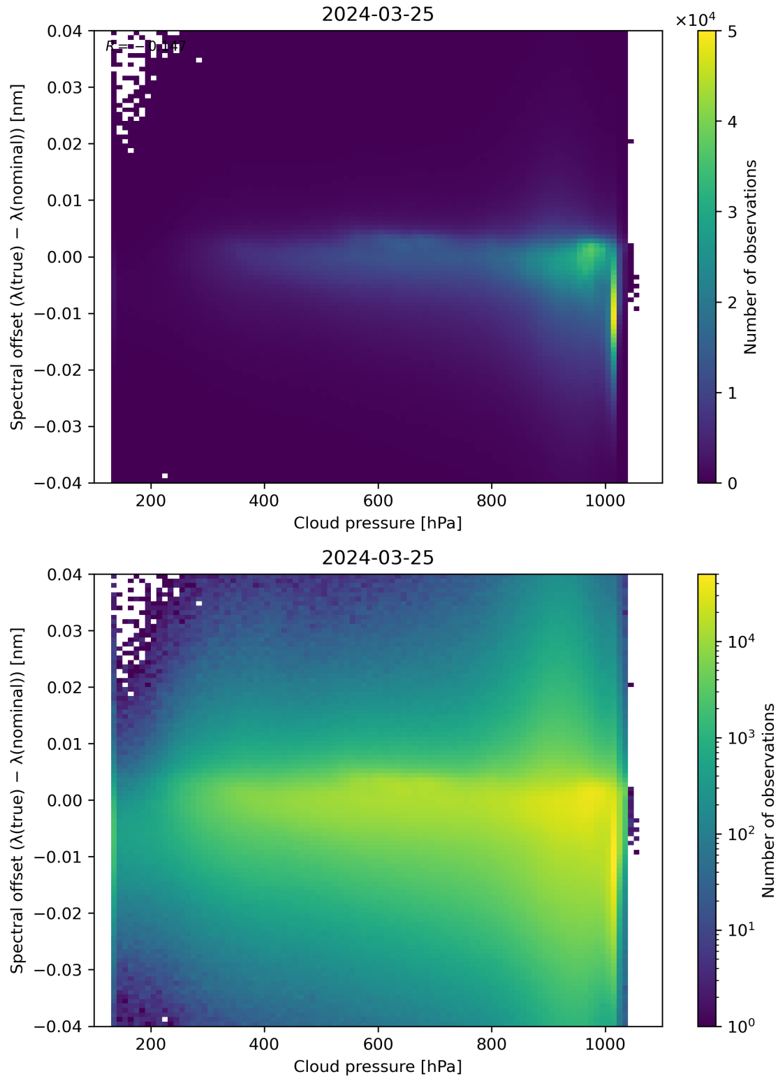
Figure 84: Scatter density plot of “Cloud pressure” against “Spectral offset ( \lambda(\text{true}) - \lambda(\text{nominal}) )” for 2024-03-25 to 2024-03-26.
