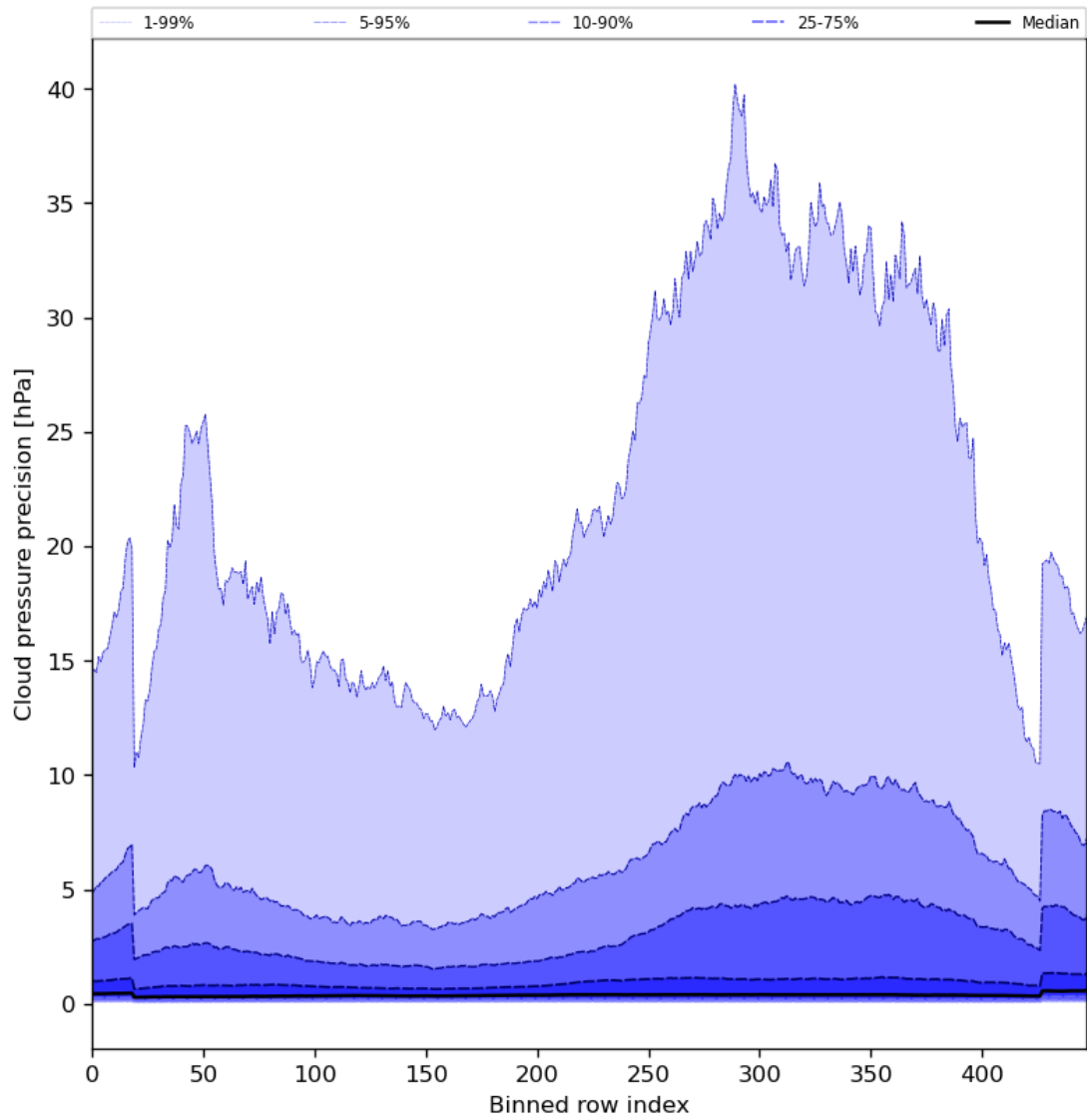
Figure 48: Along track statistics of “Cloud pressure precision” for 2024-03-25 to 2024-03-26
