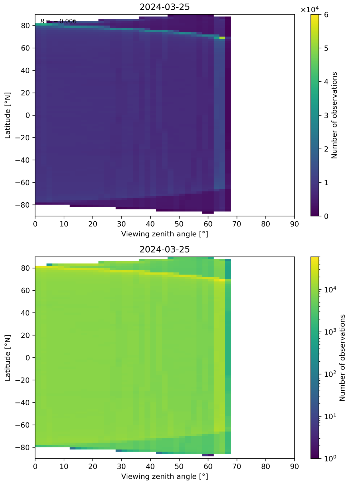
Figure 123: Scatter density plot of “Viewing zenith angle” against “Latitude” for 2024-03-25 to 2024-03-26.
