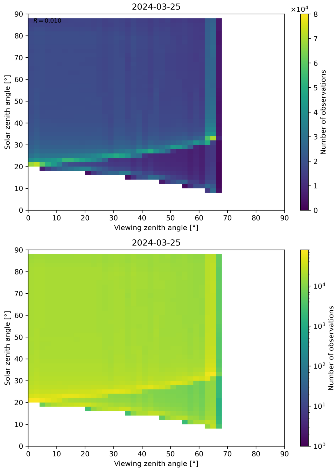
Figure 127: Scatter density plot of “Viewing zenith angle” against “Solar zenith angle” for 2024-03-25 to 2024-03-26.
