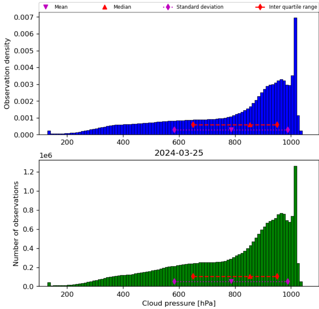
Figure 30: Histogram of “Cloud pressure” for 2024-03-25 to 2024-03-26
