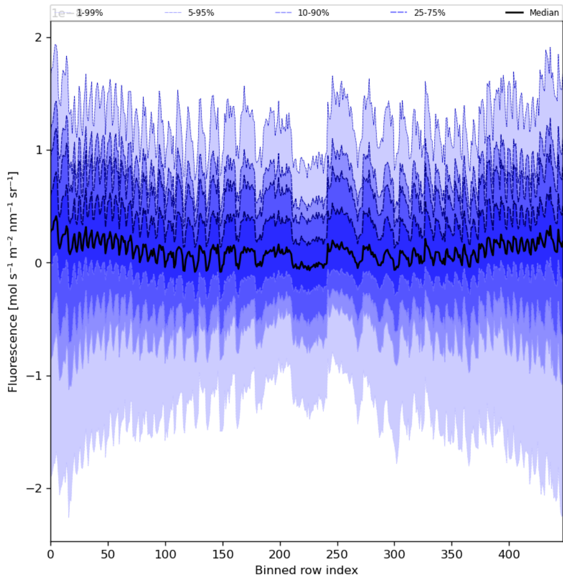
Figure 57: Along track statistics of “Fluorescence” for 2024-03-25 to 2024-03-26
