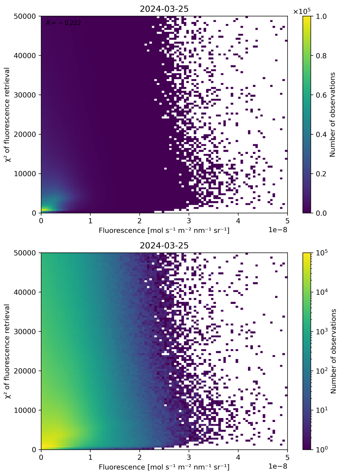
Figure 85: Scatter density plot of “Fluorescence” against “ \chi^2 of fluorescence retrieval” for 2024-03-25 to 2024-03-26.
