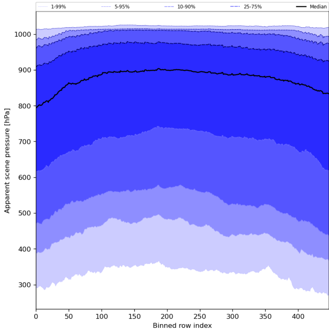
Figure 53: Along track statistics of “Apparent scene pressure” for 2024-03-25 to 2024-03-26
