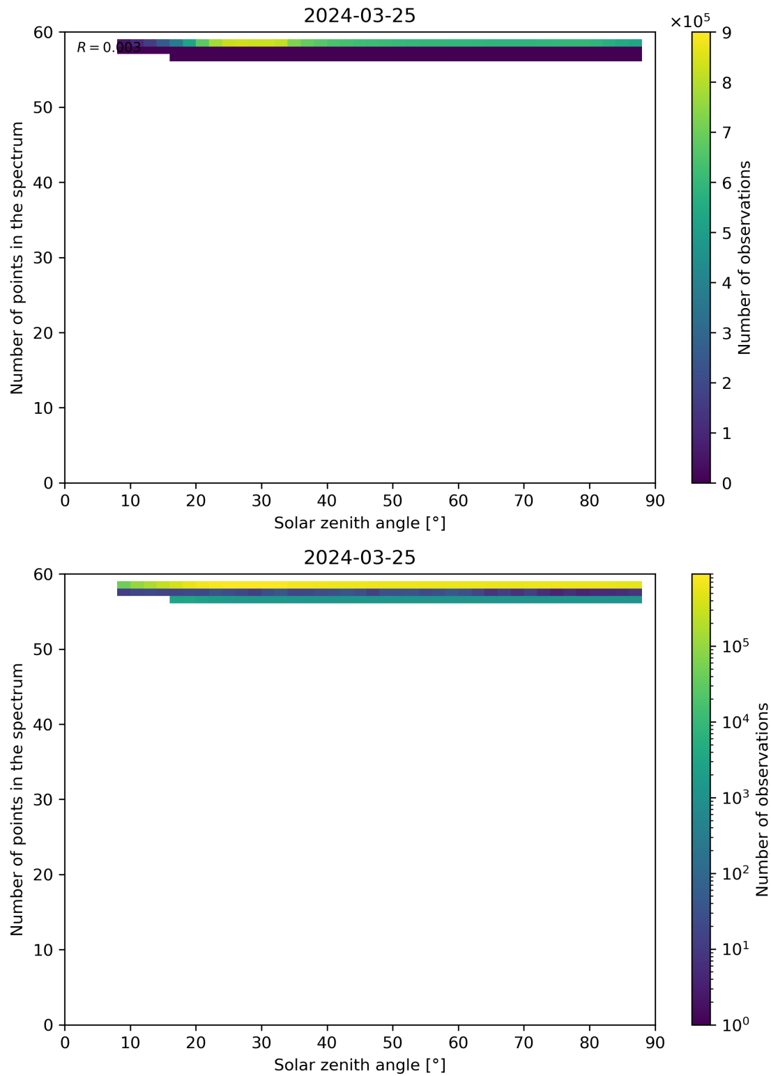
Figure 115: Scatter density plot of “Solar zenith angle” against “Number of points in the spectrum” for 2024-03-25 to 2024-03-26.
