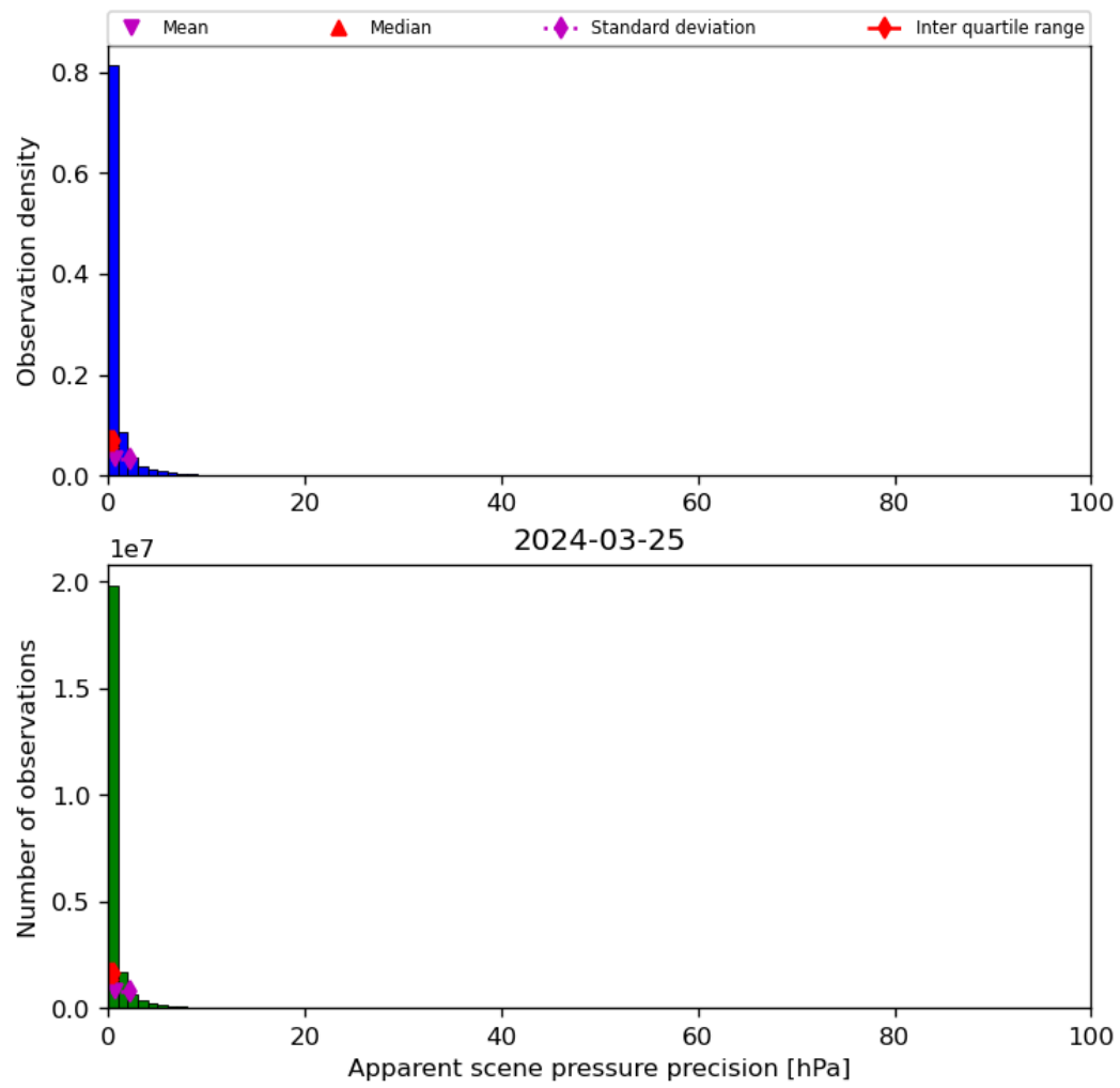
Figure 37: Histogram of “Apparent scene pressure precision” for 2024-03-25 to 2024-03-26
