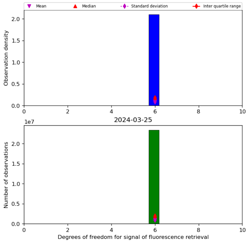
Figure 43: Histogram of “Degrees of freedom for signal of fluorescence retrieval” for 2024-03-25 to 2024-03-26
