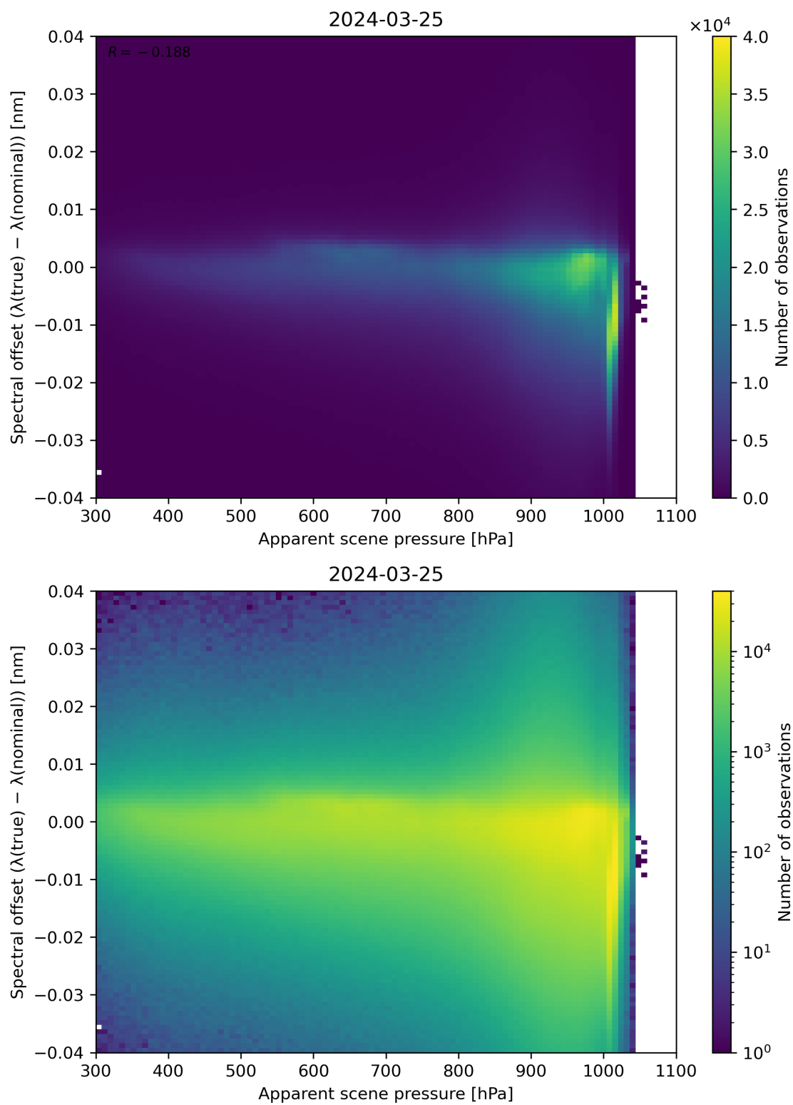
Figure 67: Scatter density plot of “Apparent scene pressure” against “Spectral offset ( \lambda(\text{true}) - \lambda(\text{nominal}) )” for 2024-03-25 to 2024-03-26.
