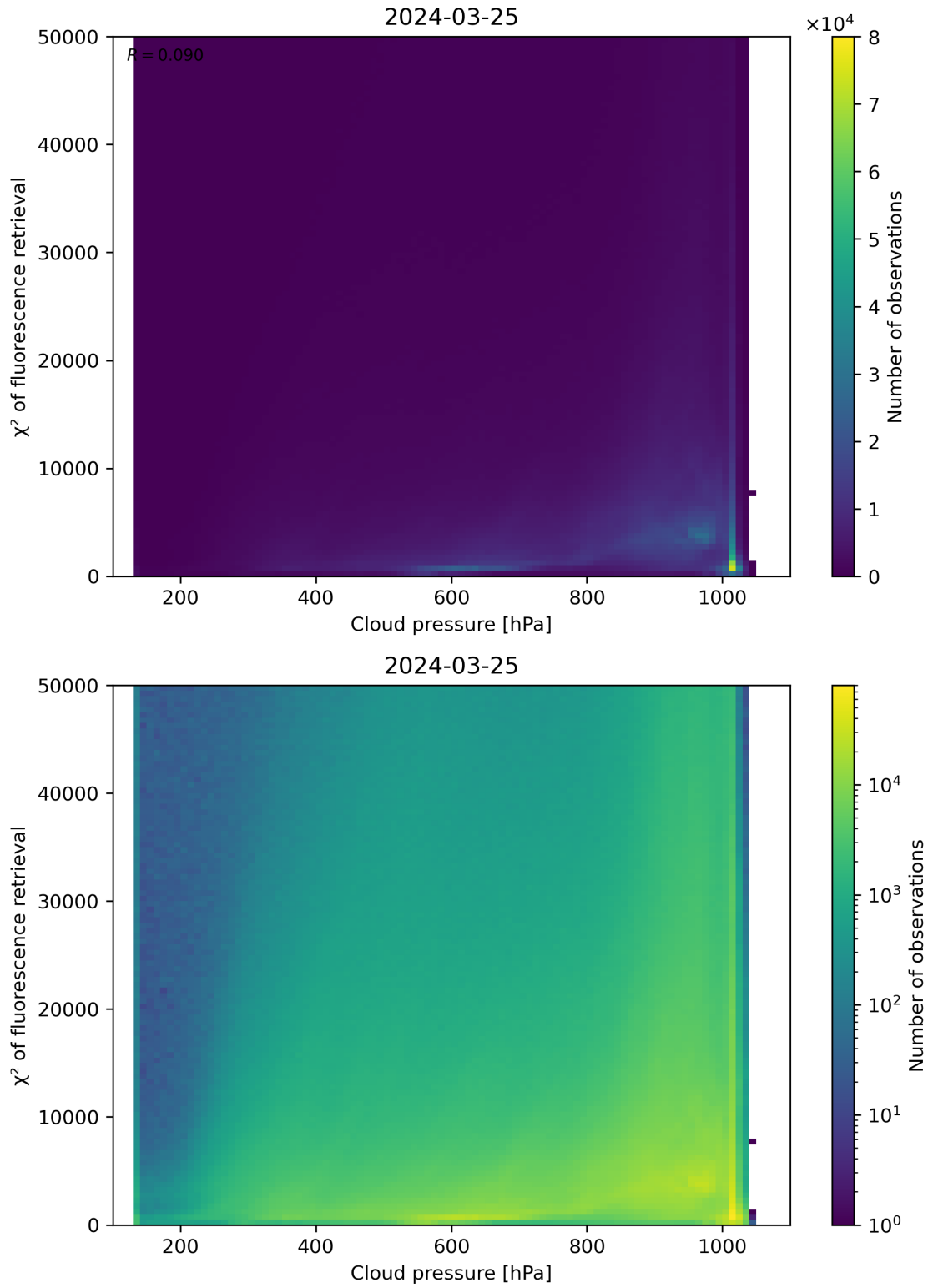
Figure 78: Scatter density plot of “Cloud pressure” against “ \chi^2 of fluorescence retrieval” for 2024-03-25 to 2024-03-26.
