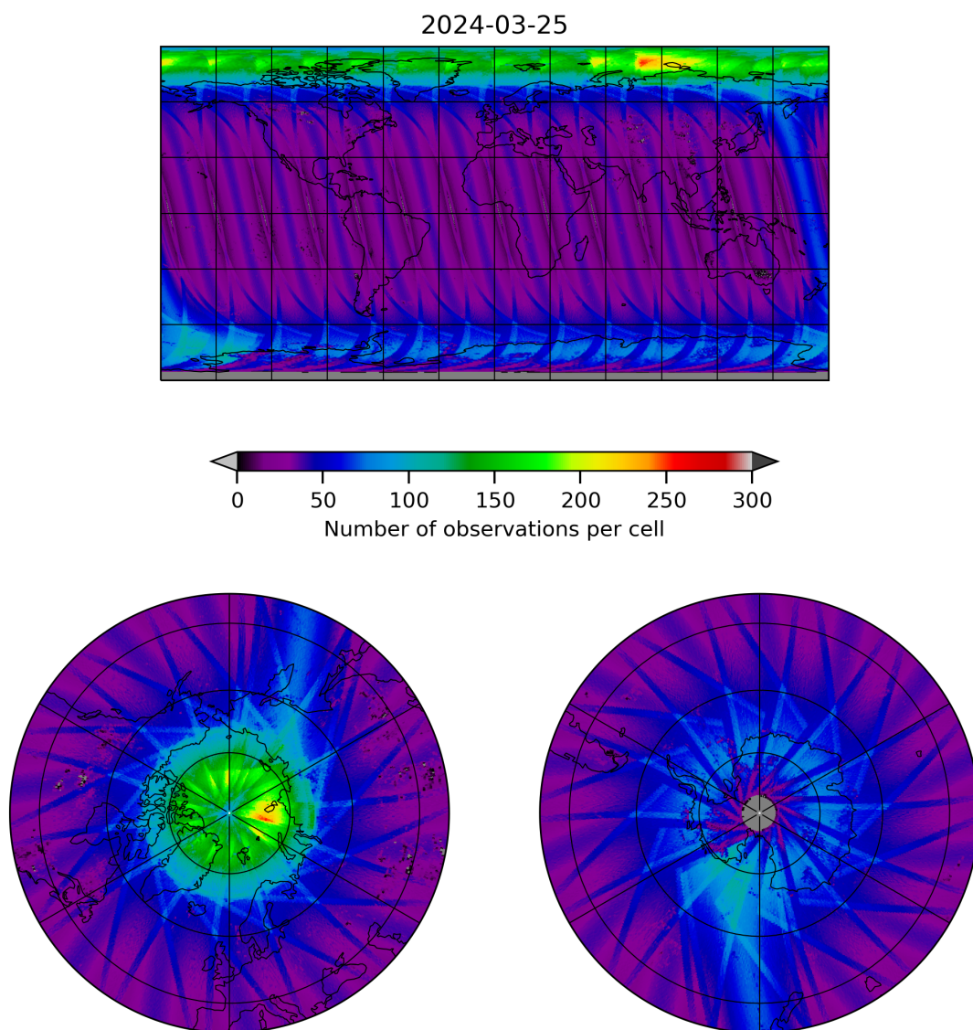
Figure 11: Map of the number of observations for 2024-03-25 to 2024-03-26
