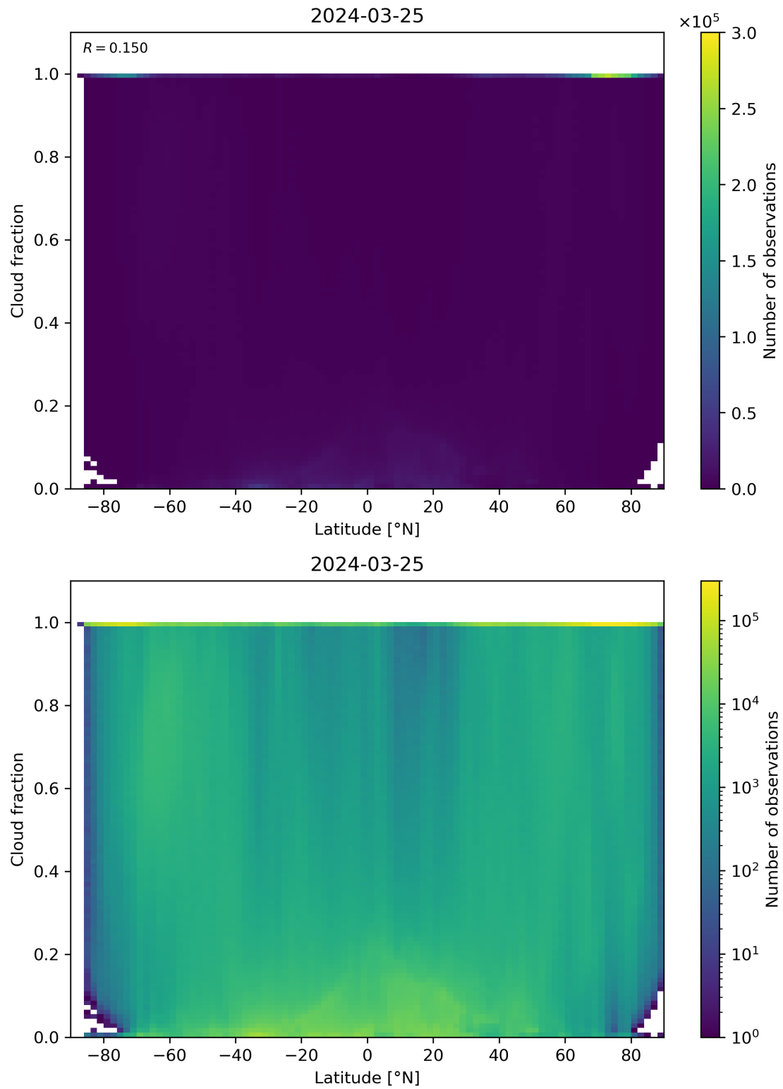
Figure 90: Scatter density plot of “Latitude” against “Cloud fraction” for 2024-03-25 to 2024-03-26.
