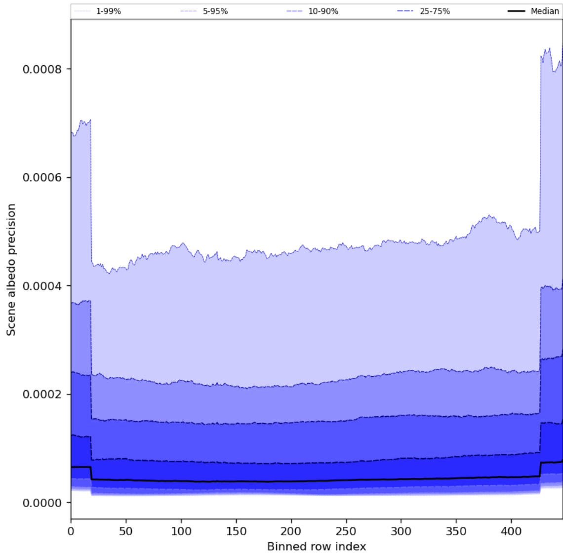
Figure 52: Along track statistics of “Scene albedo precision” for 2024-03-25 to 2024-03-26
