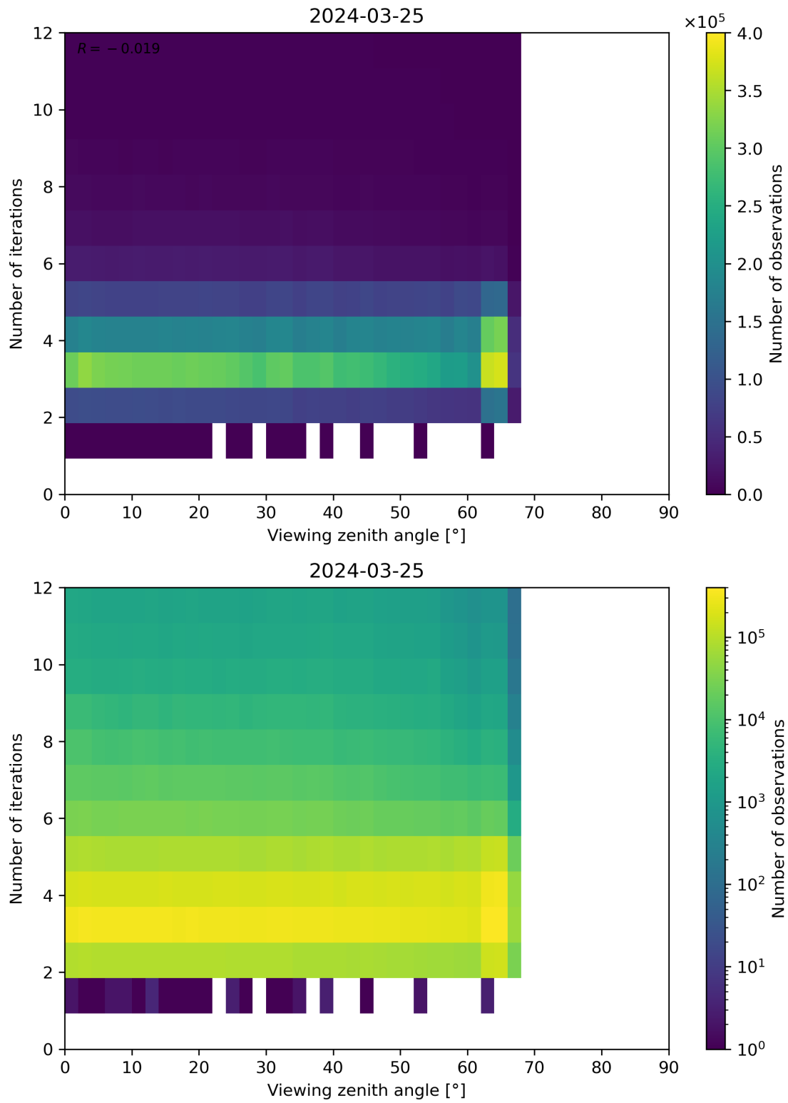
Figure 124: Scatter density plot of “Viewing zenith angle” against “Number of iterations” for 2024-03-25 to 2024-03-26.
