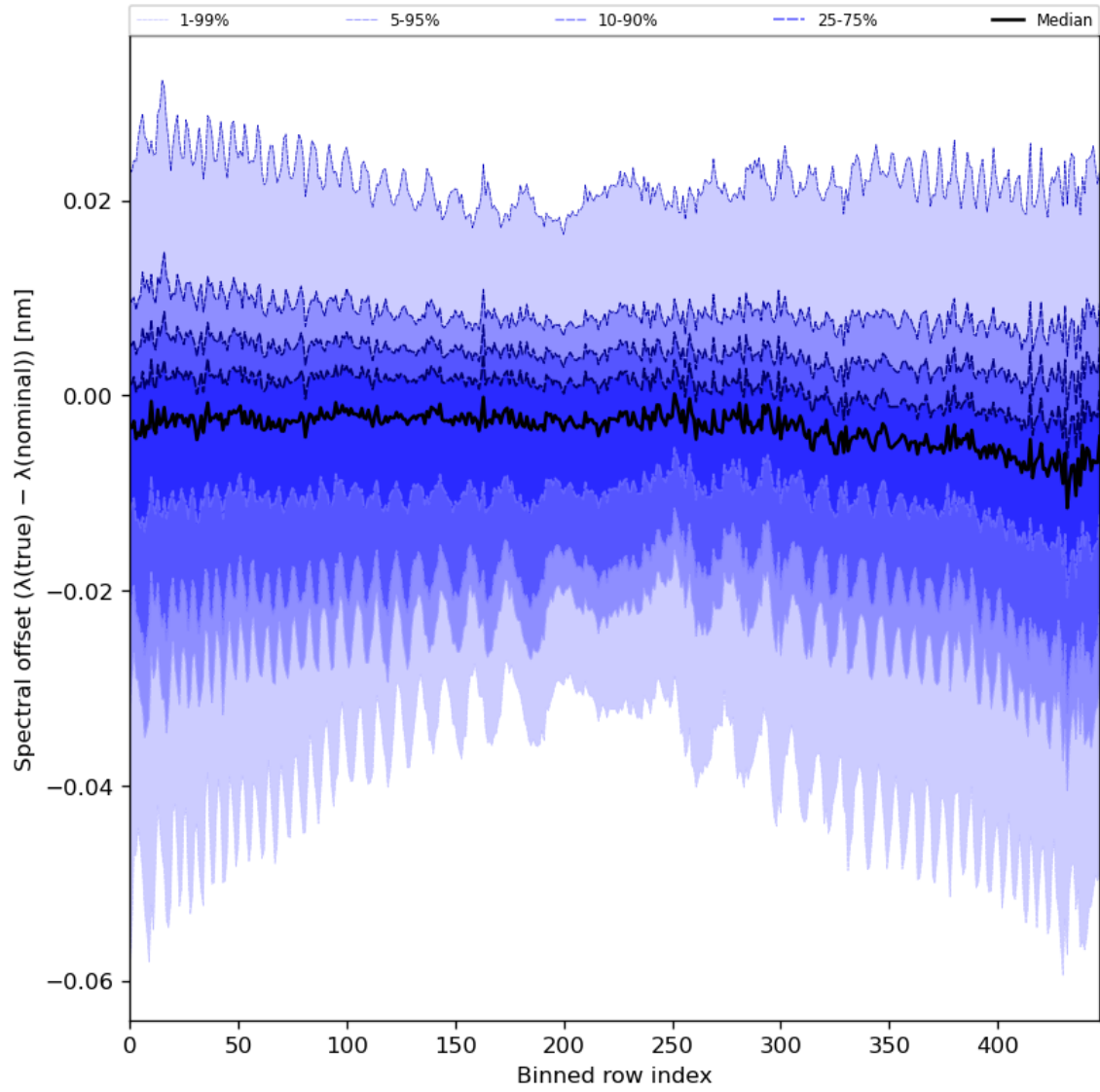
Figure 62: Along track statistics of “Spectral offset ( \lambda(\text{true}) - \lambda(\text{nominal}) )” for 2024-03-25 to 2024-03-26
