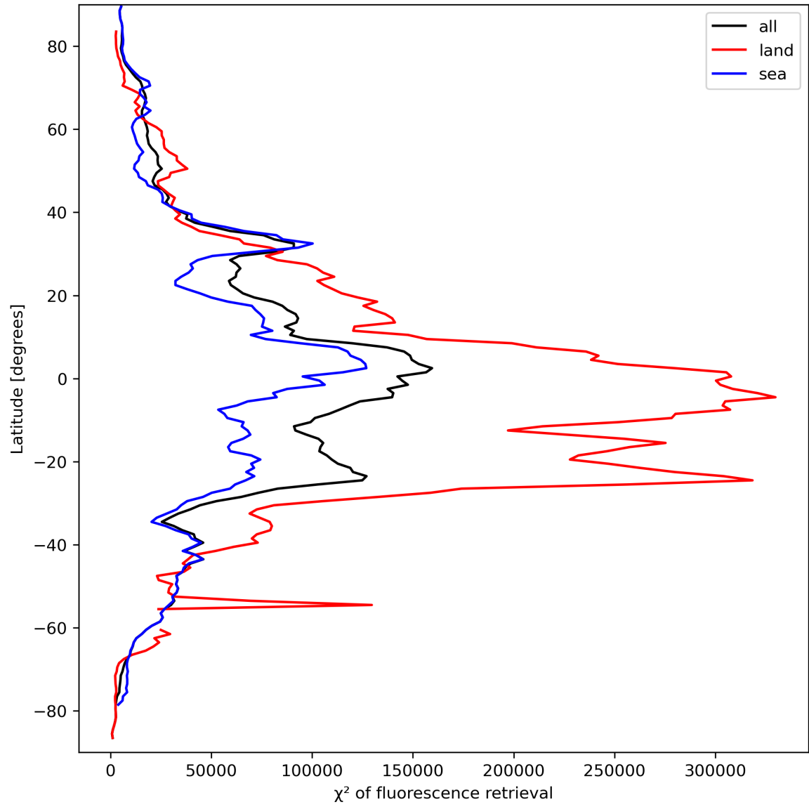
Figure 25: Zonal average of “ \chi^2 of fluorescence retrieval” for 2024-03-25 to 2024-03-26.
