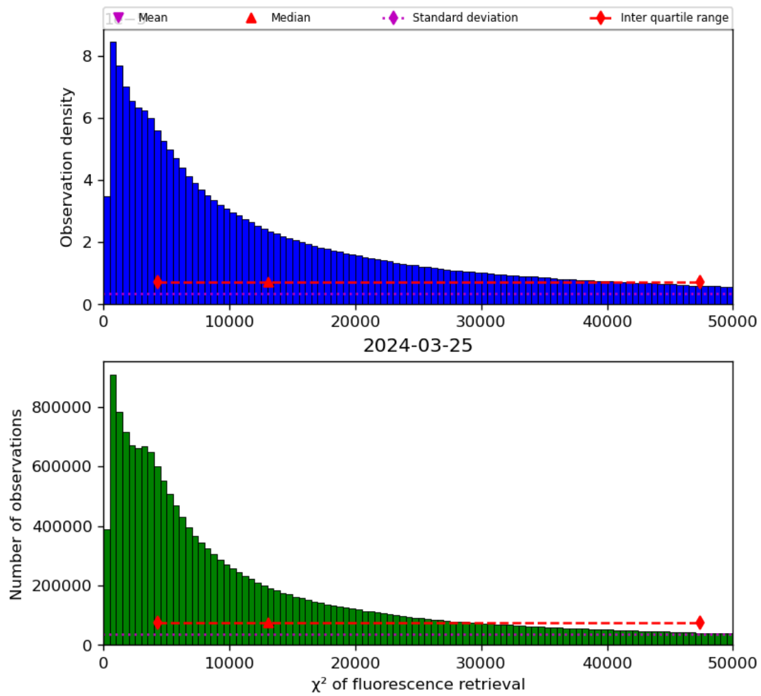
Figure 42: Histogram of “ \chi^2 of fluorescence retrieval” for 2024-03-25 to 2024-03-26
