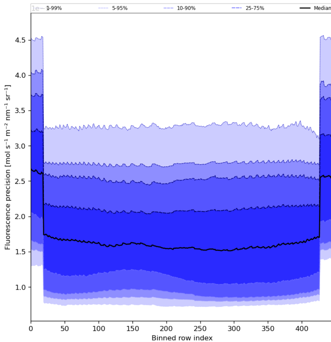
Figure 58: Along track statistics of “Fluorescence precision” for 2024-03-25 to 2024-03-26
