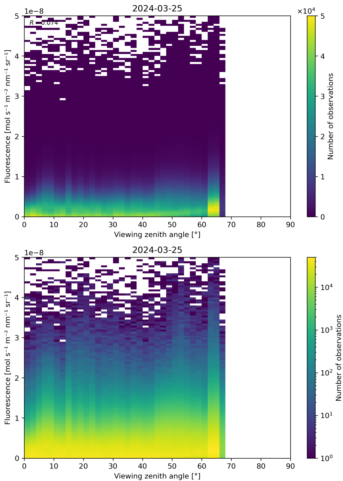
Figure 122: Scatter density plot of “Viewing zenith angle” against “Fluorescence” for 2024-03-25 to 2024-03-26.
