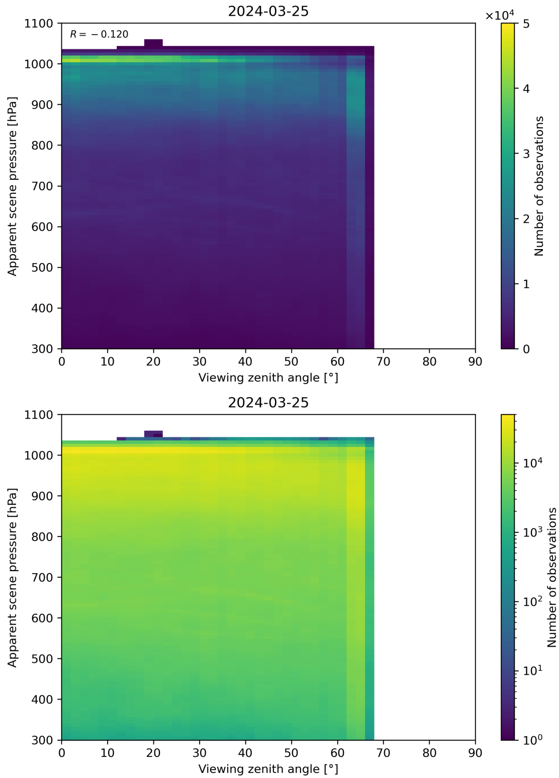
Figure 118: Scatter density plot of “Viewing zenith angle” against “Apparent scene pressure” for 2024-03-25 to 2024-03-26.
