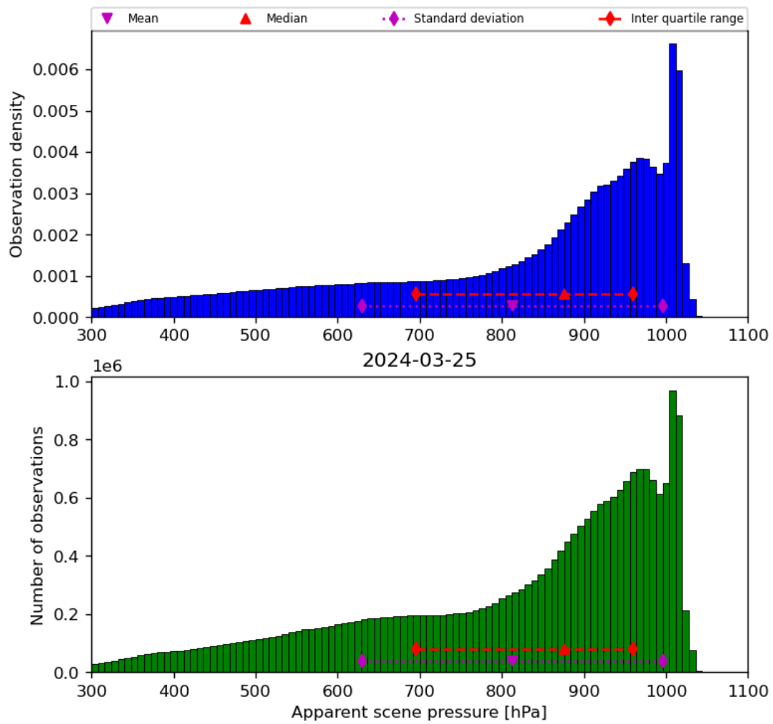
Figure 36: Histogram of “Apparent scene pressure” for 2024-03-25 to 2024-03-26
