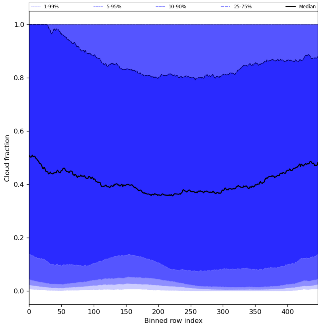
Figure 49: Along track statistics of “Cloud fraction” for 2024-03-25 to 2024-03-26
