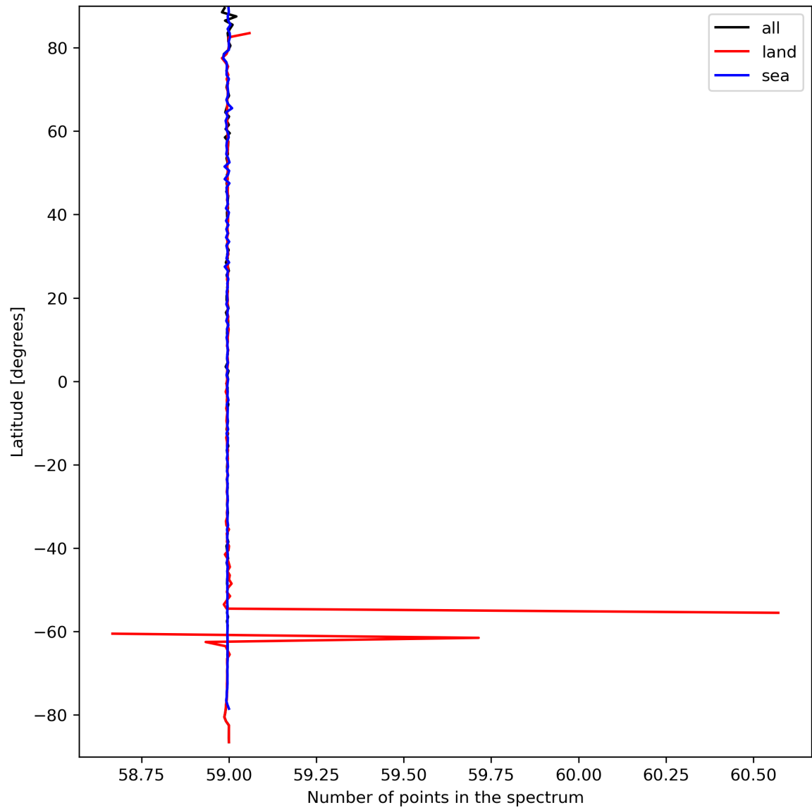
Figure 27: Zonal average of “Number of points in the spectrum” for 2024-03-25 to 2024-03-26.
