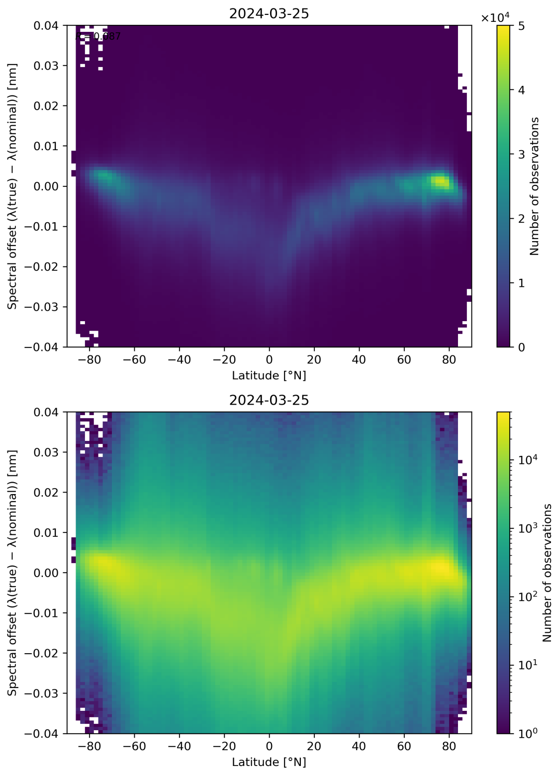
Figure 96: Scatter density plot of “Latitude” against “Spectral offset ( \lambda(\text{true}) - \lambda(\text{nominal}) )” for 2024-03-25 to 2024-03-26.
