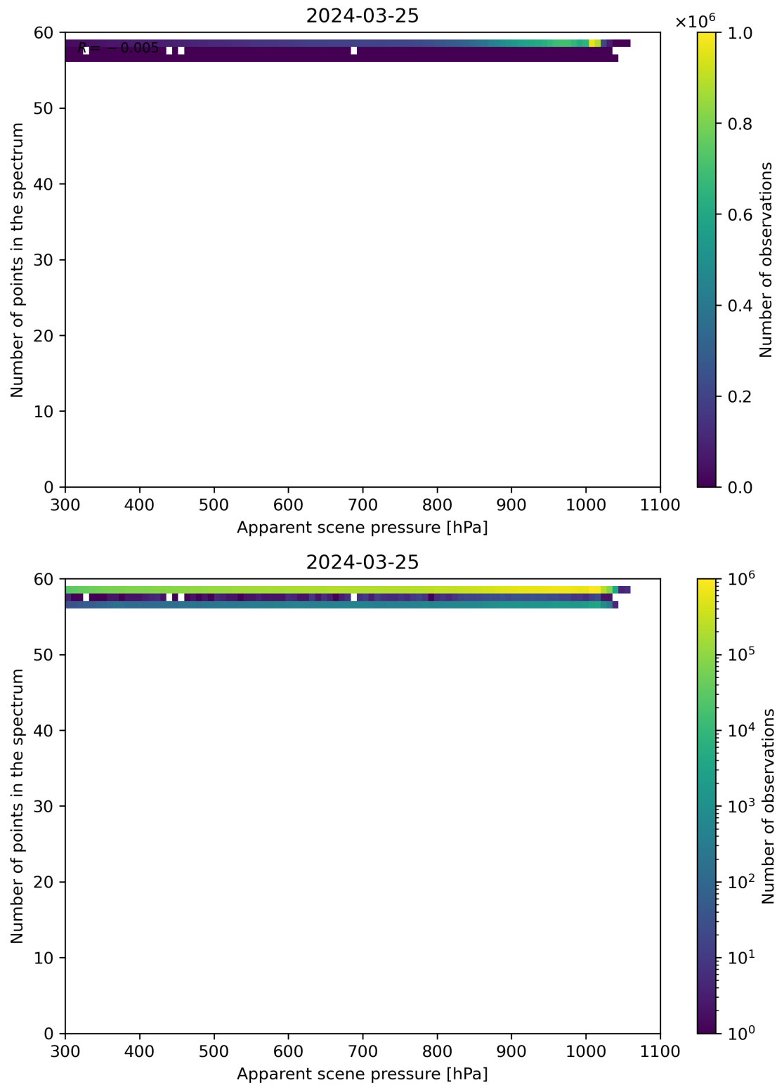
Figure 66: Scatter density plot of “Apparent scene pressure” against “Number of points in the spectrum” for 2024-03-25 to 2024-03-26.
