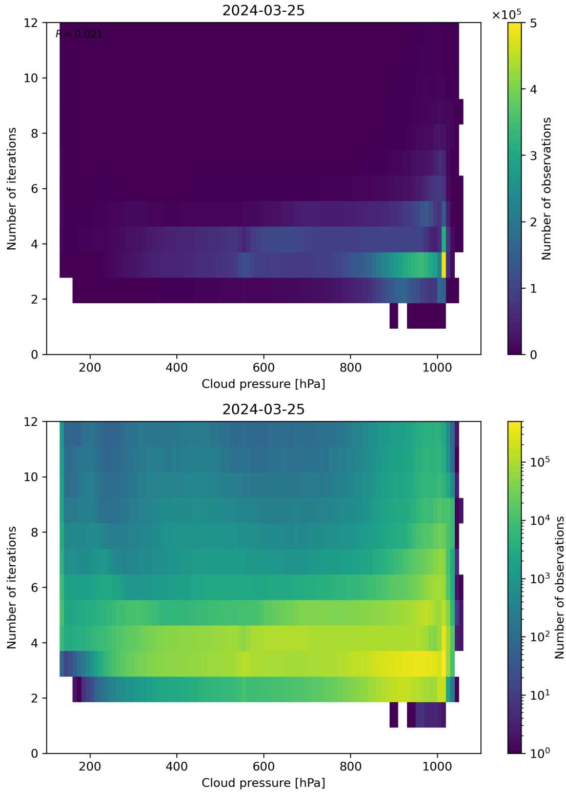
Figure 81: Scatter density plot of “Cloud pressure” against “Number of iterations” for 2024-03-25 to 2024-03-26.
