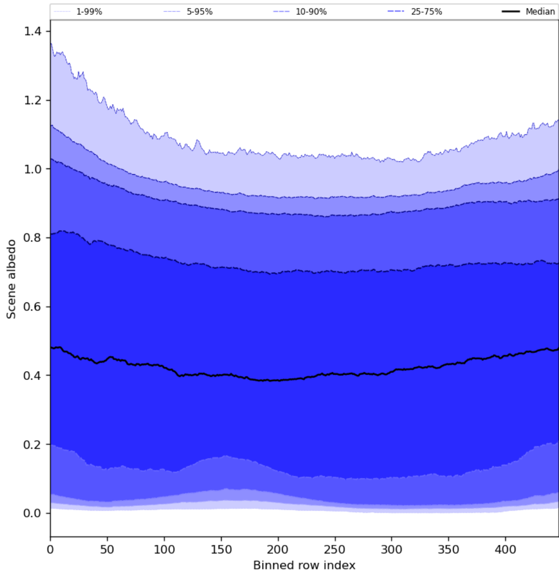
Figure 51: Along track statistics of “Scene albedo” for 2024-03-25 to 2024-03-26
