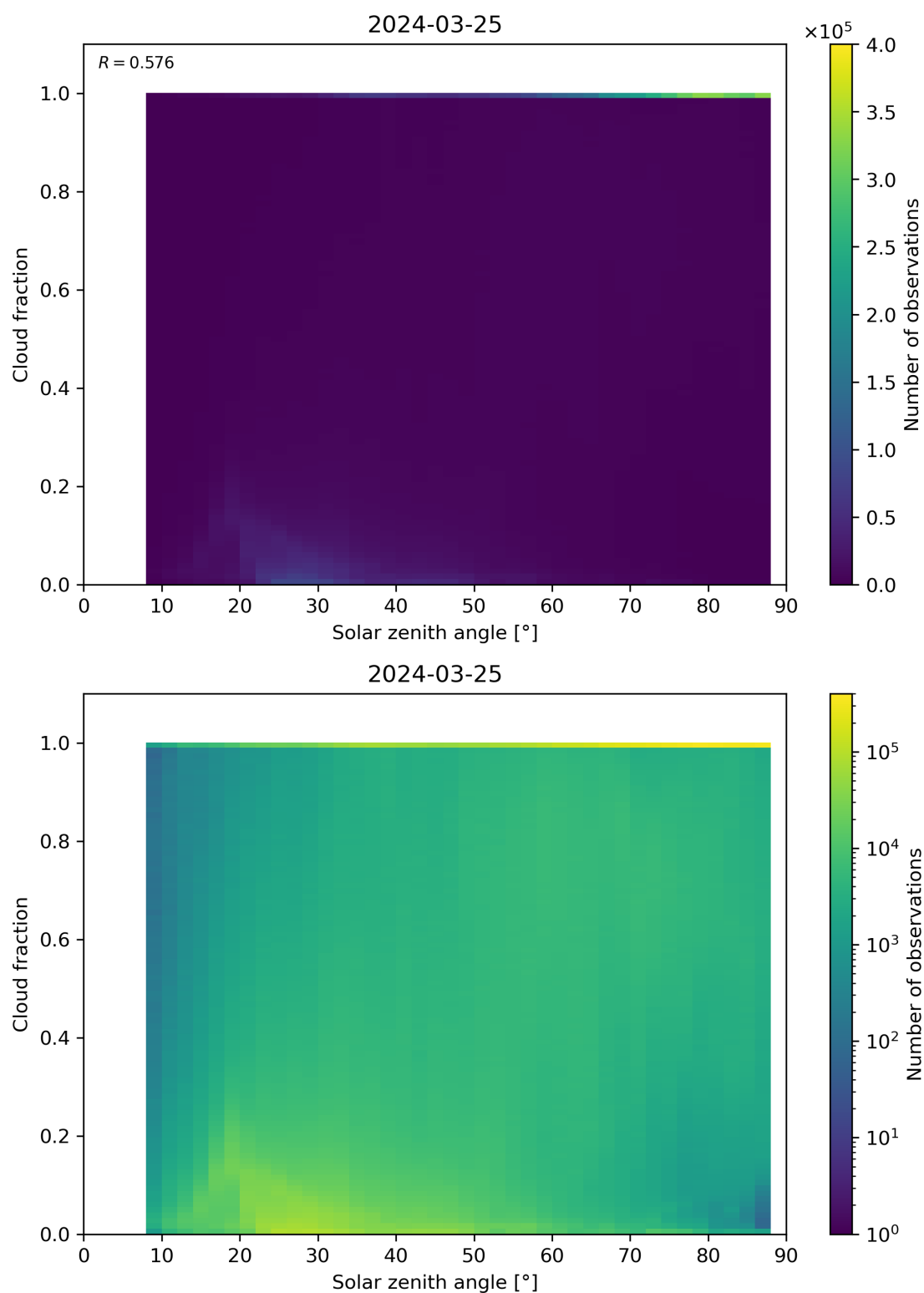
Figure 110: Scatter density plot of “Solar zenith angle” against “Cloud fraction” for 2024-03-25 to 2024-03-26.
