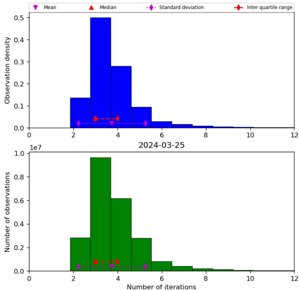
Figure 39: Histogram of “Number of iterations” for 2024-03-25 to 2024-03-26
