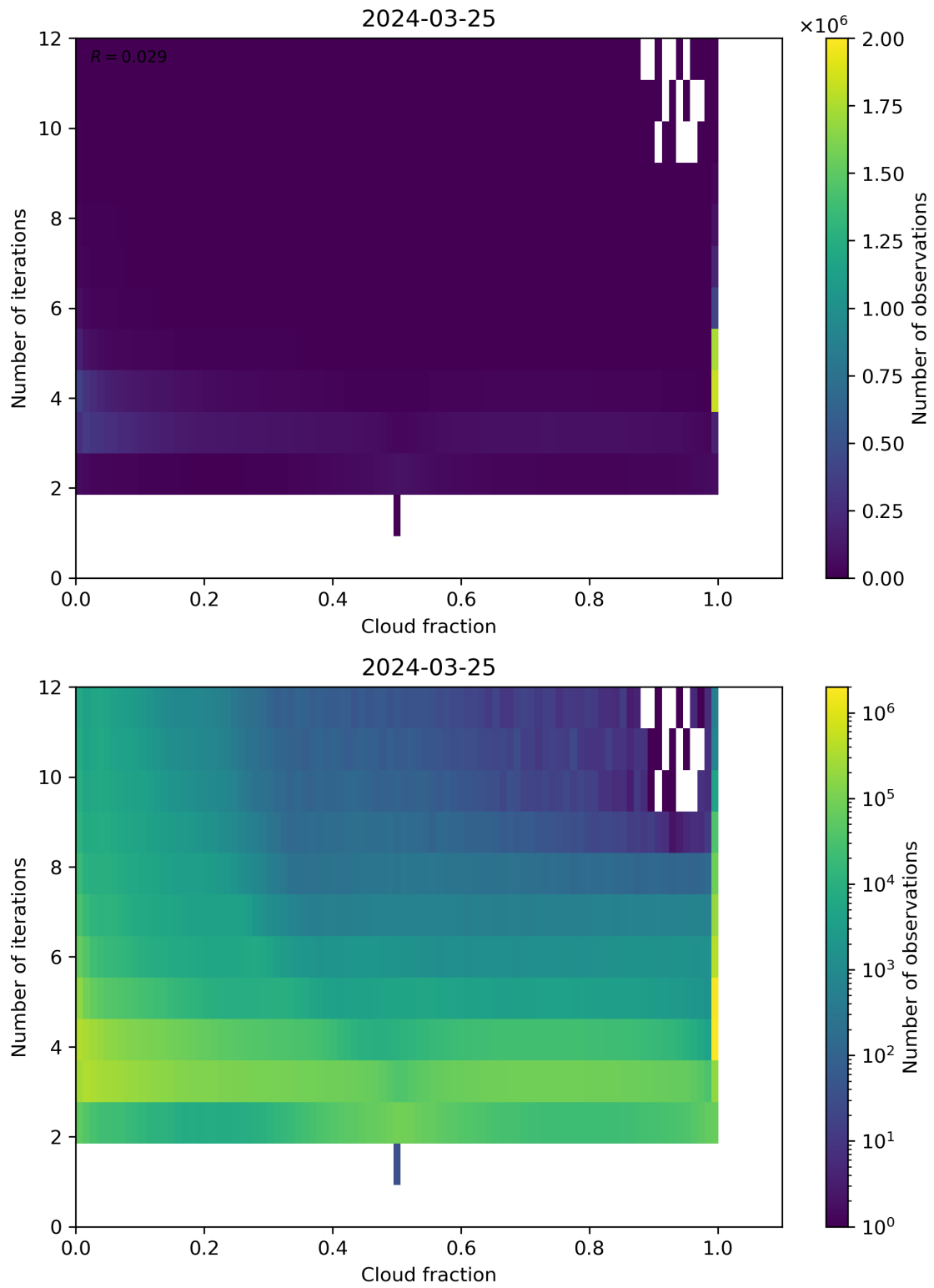
Figure 73: Scatter density plot of “Cloud fraction” against “Number of iterations” for 2024-03-25 to 2024-03-26.
