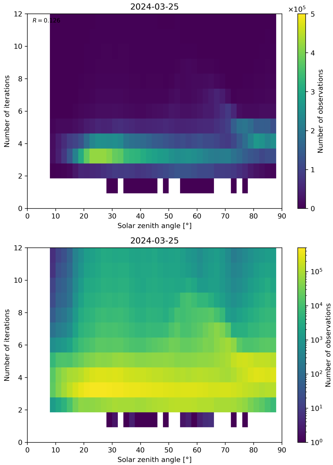
Figure 114: Scatter density plot of “Solar zenith angle” against “Number of iterations” for 2024-03-25 to 2024-03-26.
