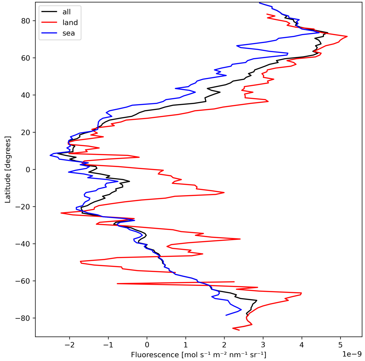
Figure 23: Zonal average of “Fluorescence” for 2024-03-25 to 2024-03-26.
