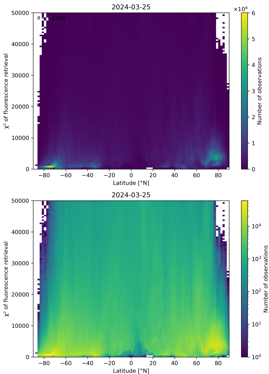
Figure 89: Scatter density plot of “Latitude” against “ \chi^2 of fluorescence retrieval” for 2024-03-25 to 2024-03-26.
