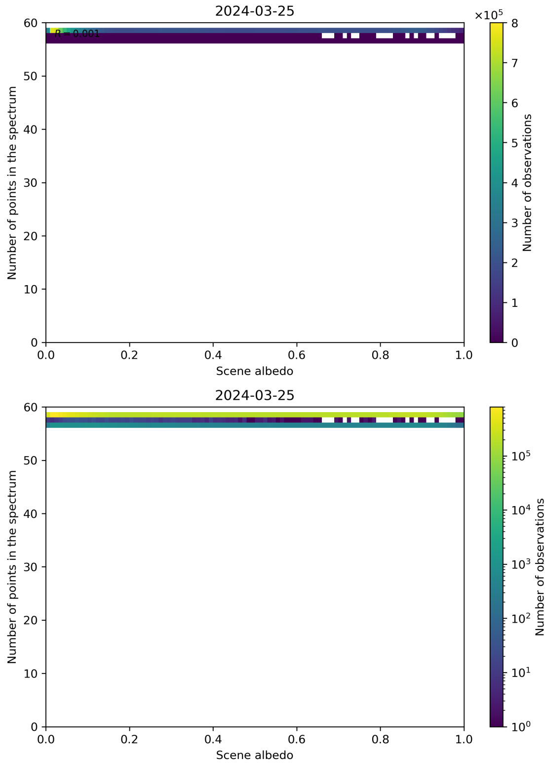
Figure 106: Scatter density plot of “Scene albedo” against “Number of points in the spectrum” for 2024-03-25 to 2024-03-26.
