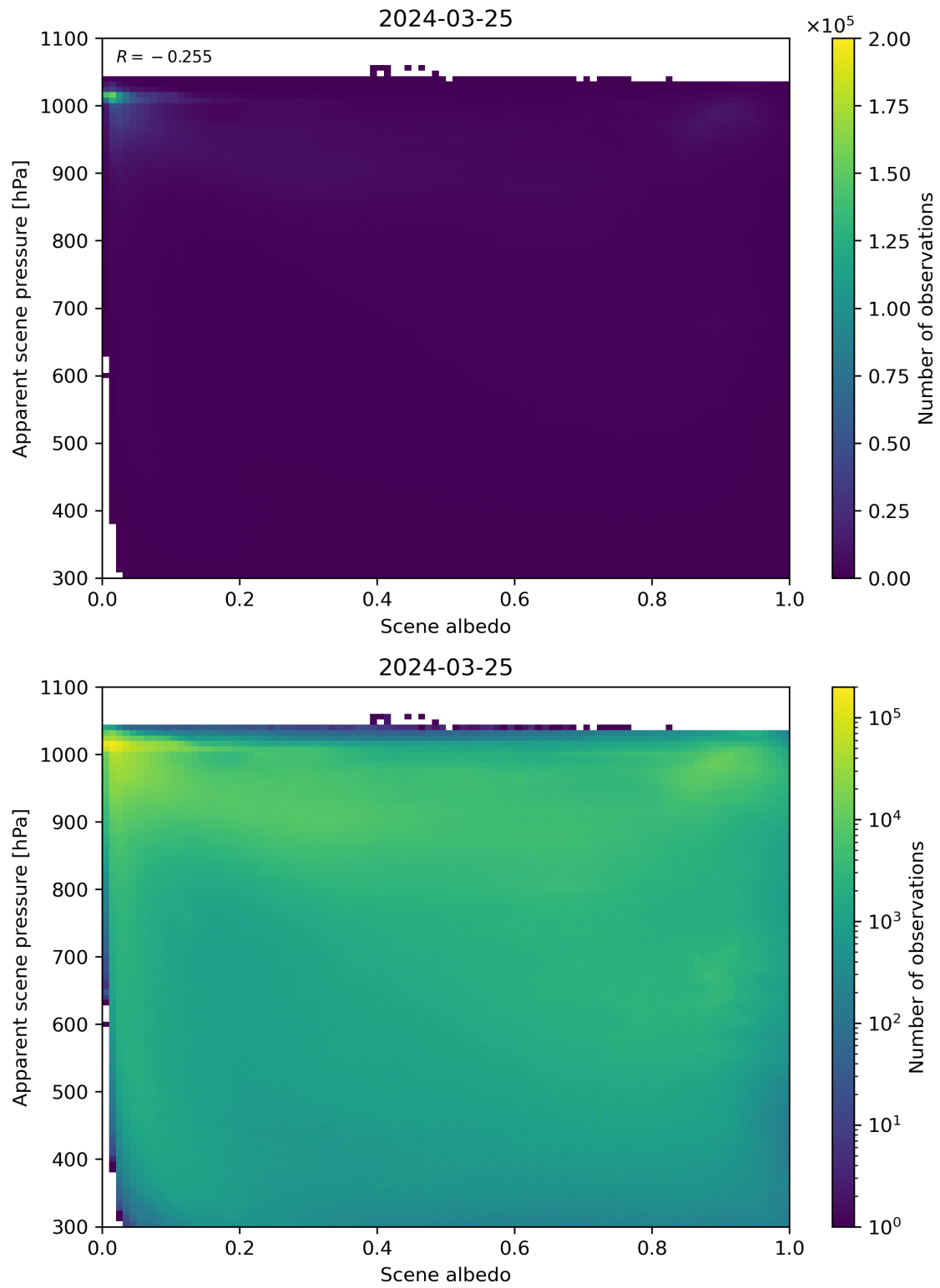
Figure 102: Scatter density plot of “Scene albedo” against “Apparent scene pressure” for 2024-03-25 to 2024-03-26.
