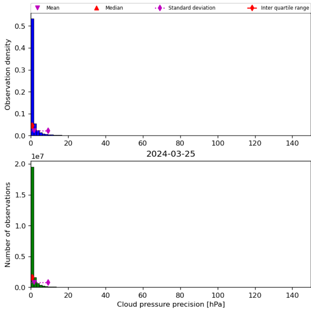
Figure 31: Histogram of “Cloud pressure precision” for 2024-03-25 to 2024-03-26
