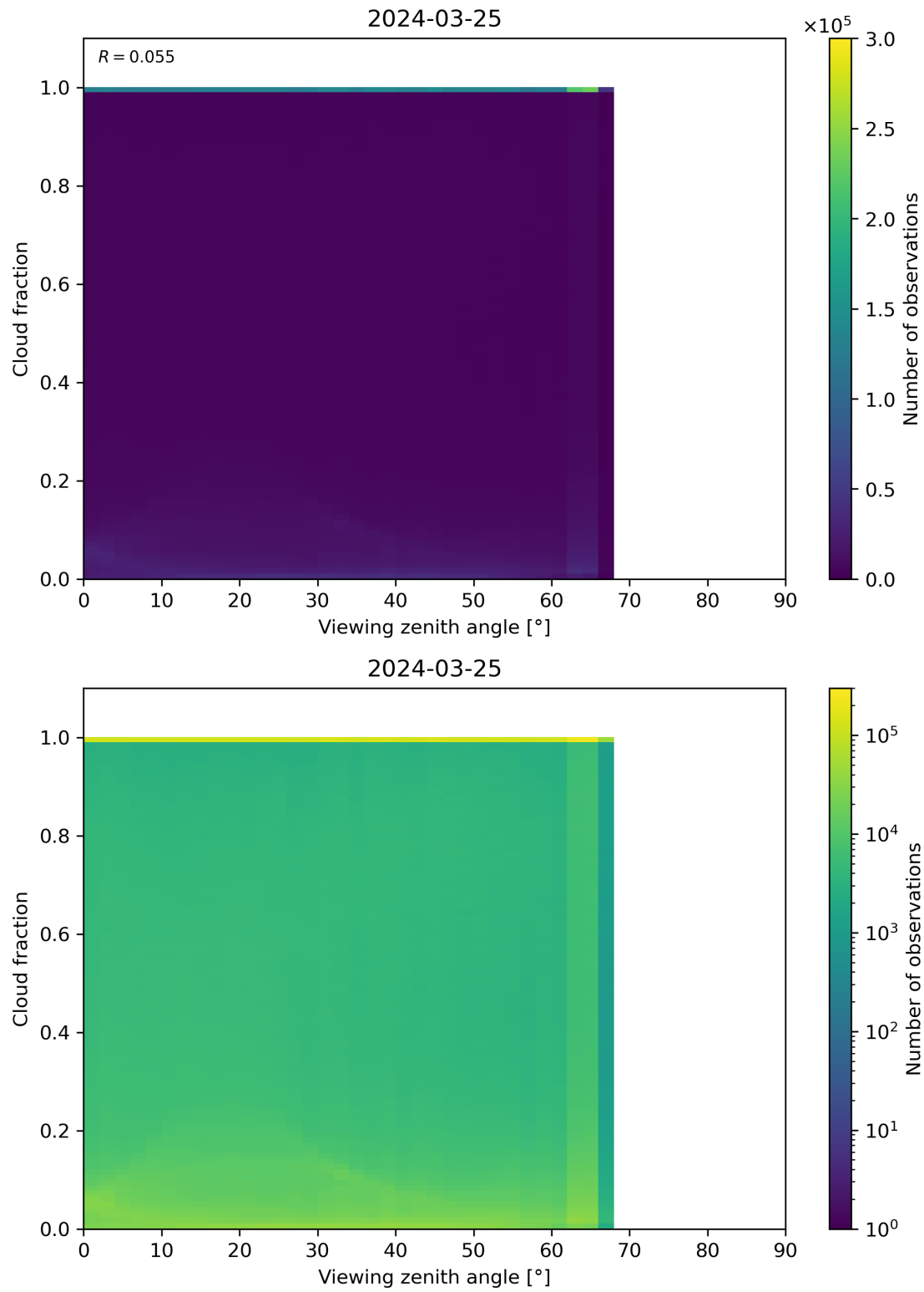
Figure 120: Scatter density plot of “Viewing zenith angle” against “Cloud fraction” for 2024-03-25 to 2024-03-26.
