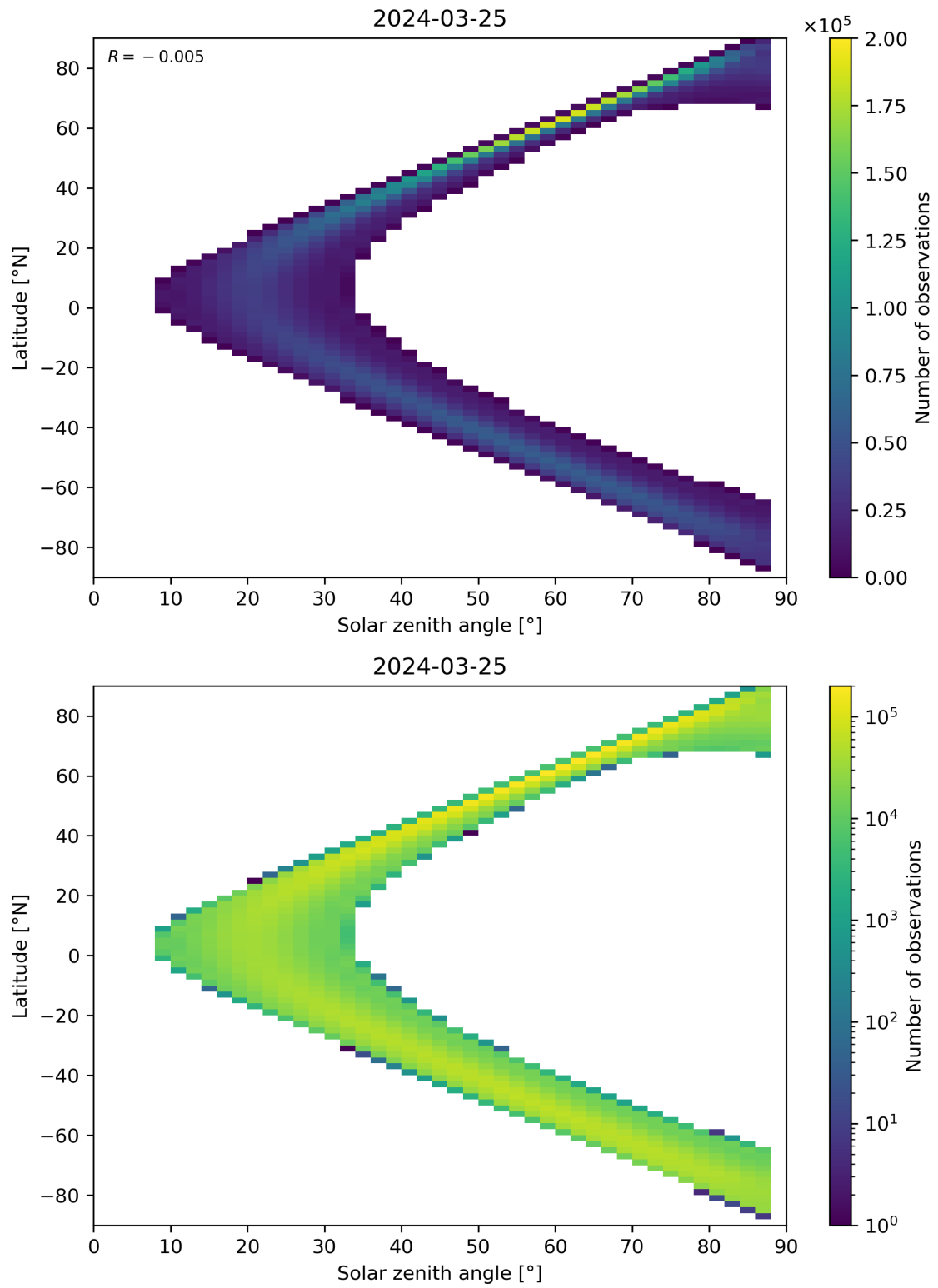
Figure 113: Scatter density plot of “Solar zenith angle” against “Latitude” for 2024-03-25 to 2024-03-26.
