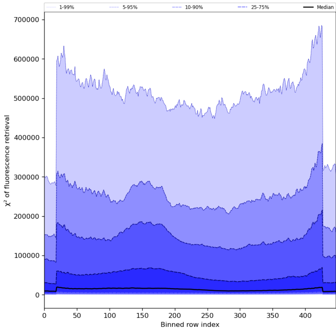
Figure 59: Along track statistics of “ \chi^2 of fluorescence retrieval” for 2024-03-25 to 2024-03-26
