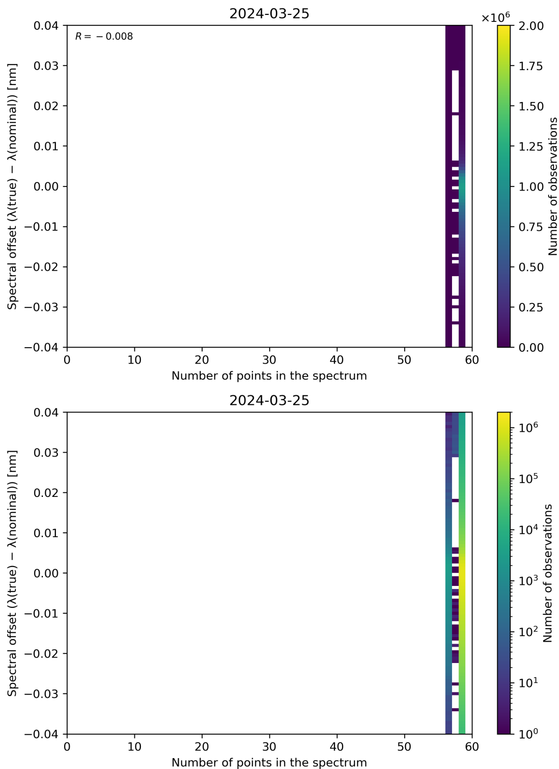
Figure 101: Scatter density plot of “Number of points in the spectrum” against “Spectral offset ( \lambda(\text{true}) - \lambda(\text{nominal}) )” for 2024-03-25 to 2024-03-26.
