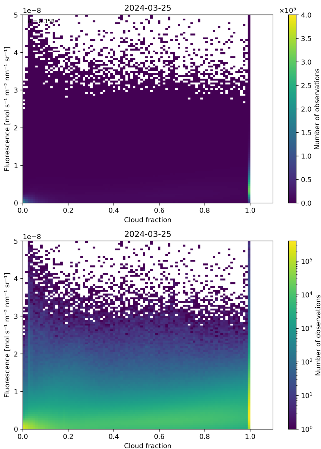
Figure 72: Scatter density plot of “Cloud fraction” against “Fluorescence” for 2024-03-25 to 2024-03-26.
