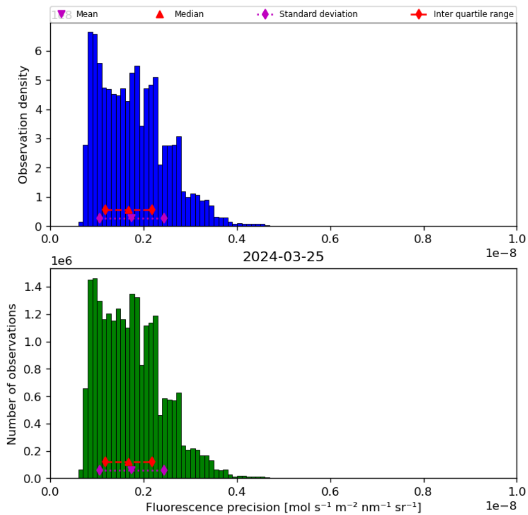
Figure 41: Histogram of “Fluorescence precision” for 2024-03-25 to 2024-03-26
