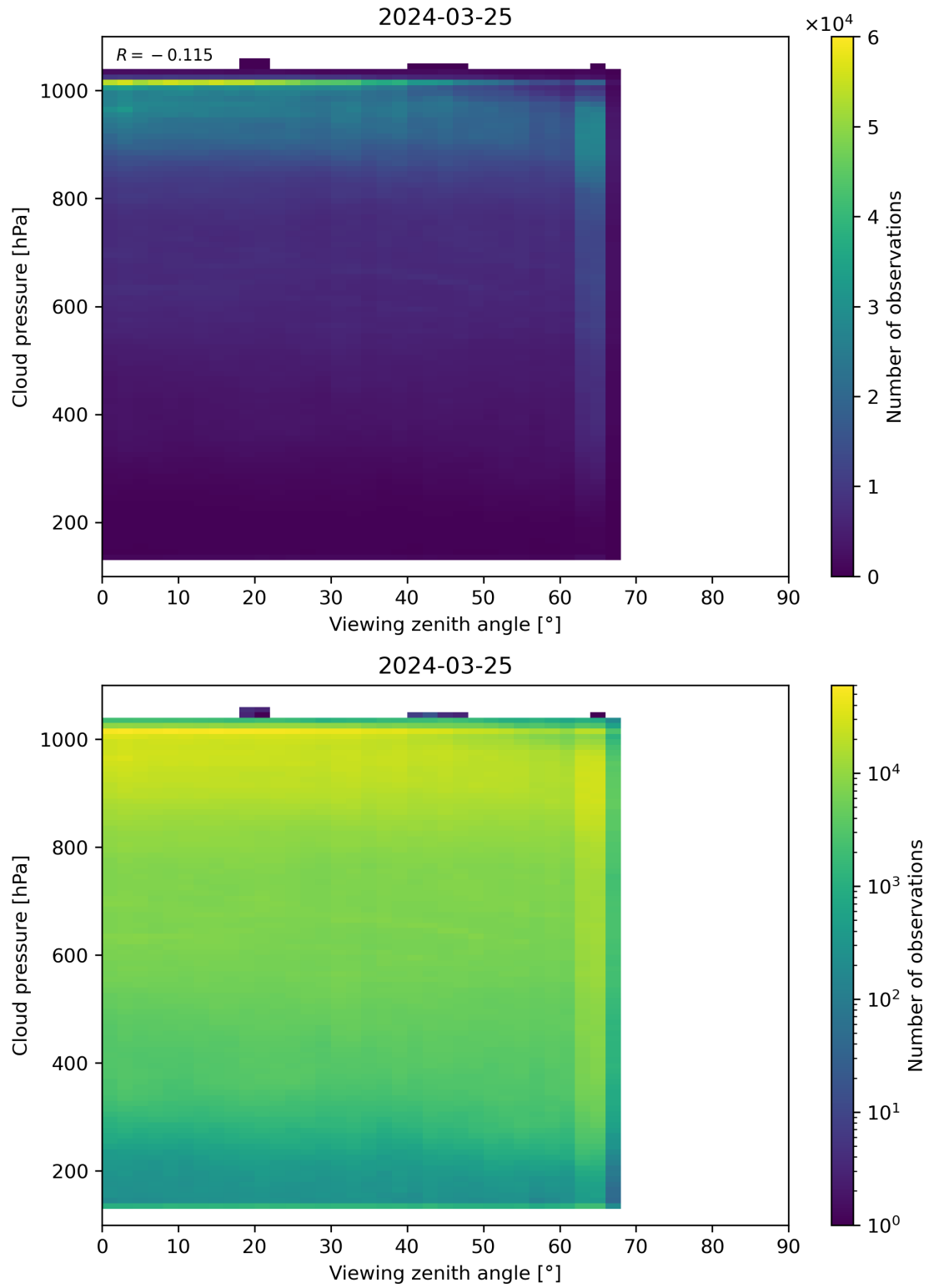
Figure 121: Scatter density plot of “Viewing zenith angle” against “Cloud pressure” for 2024-03-25 to 2024-03-26.
