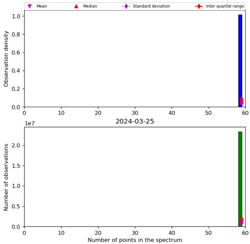
Figure 44: Histogram of “Number of points in the spectrum” for 2024-03-25 to 2024-03-26
