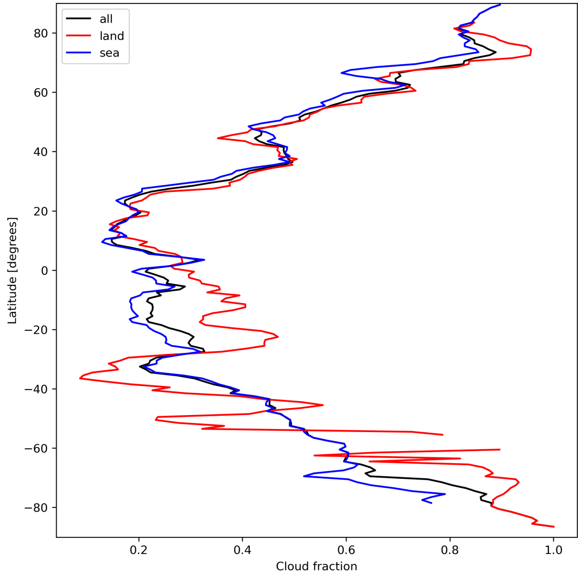
Figure 15: Zonal average of “Cloud fraction” for 2024-03-25 to 2024-03-26.
