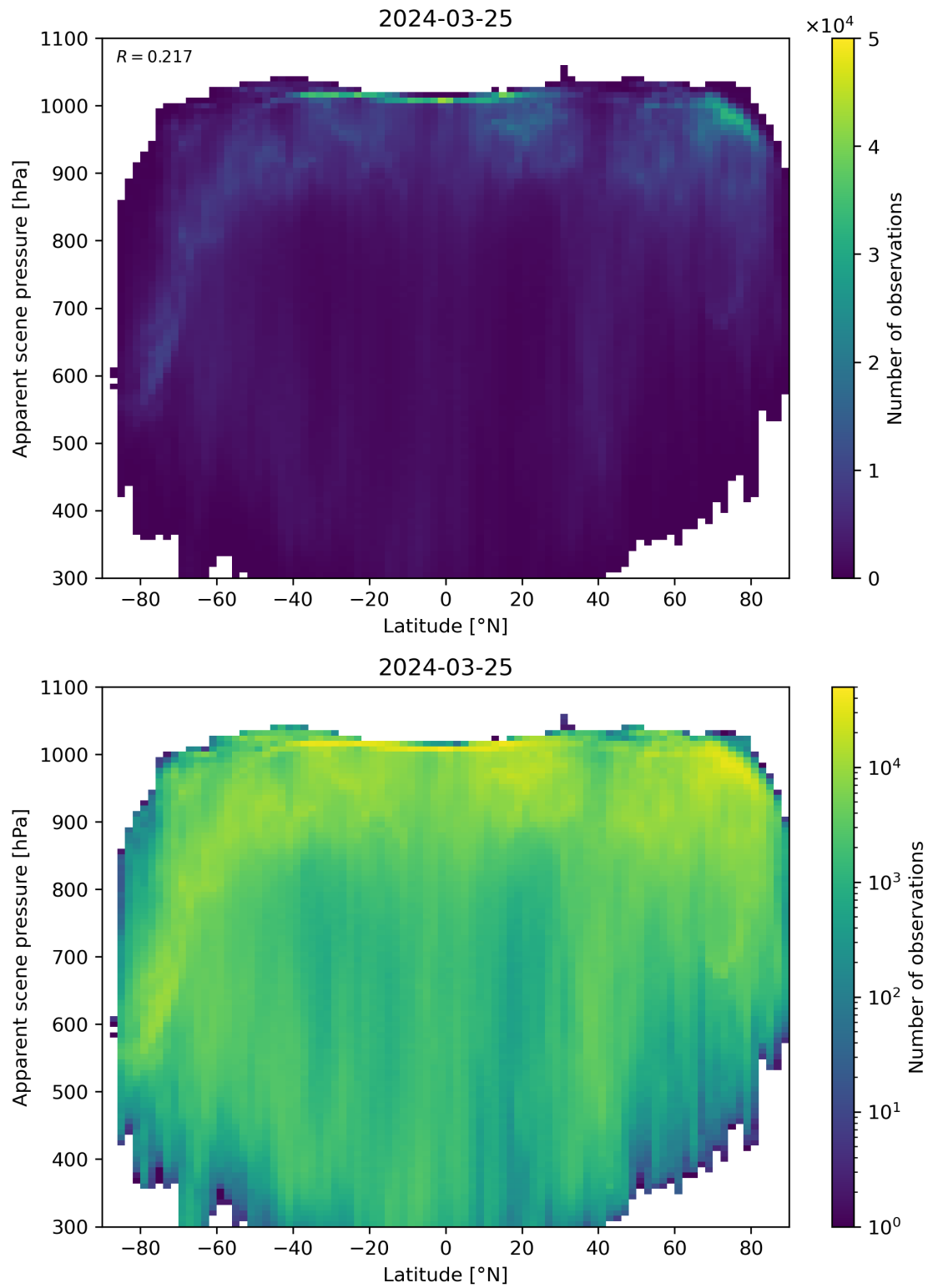
Figure 88: Scatter density plot of “Latitude” against “Apparent scene pressure” for 2024-03-25 to 2024-03-26.
