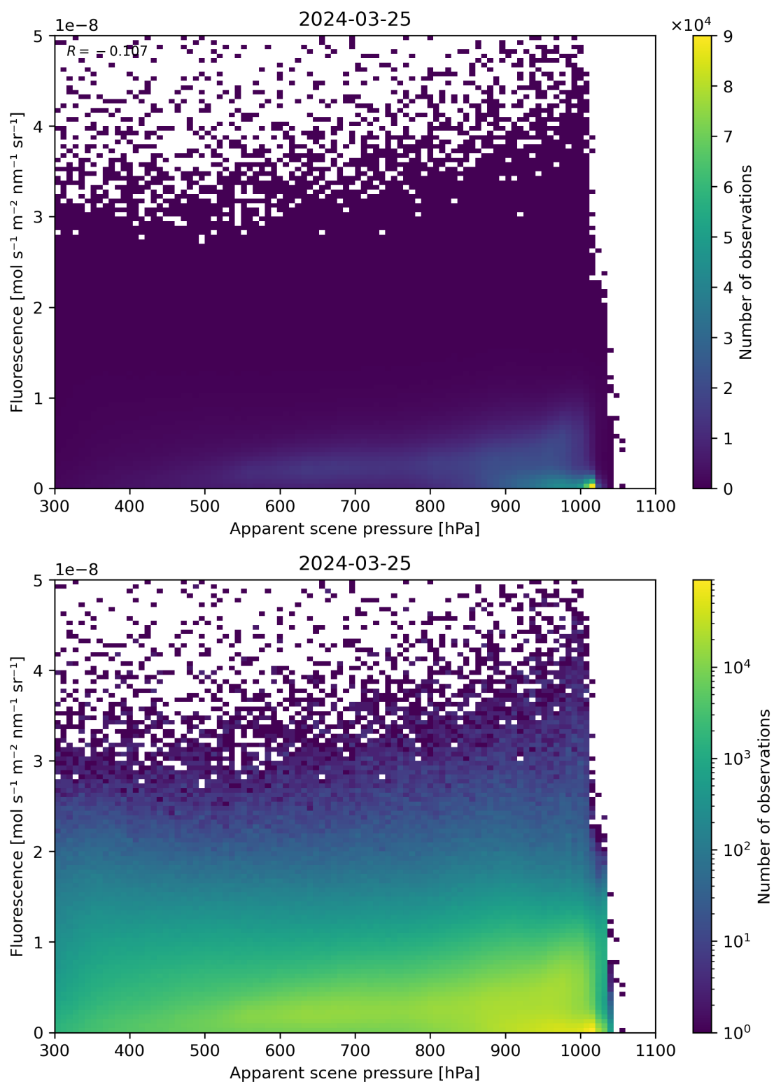
Figure 64: Scatter density plot of “Apparent scene pressure” against “Fluorescence” for 2024-03-25 to 2024-03-26.
