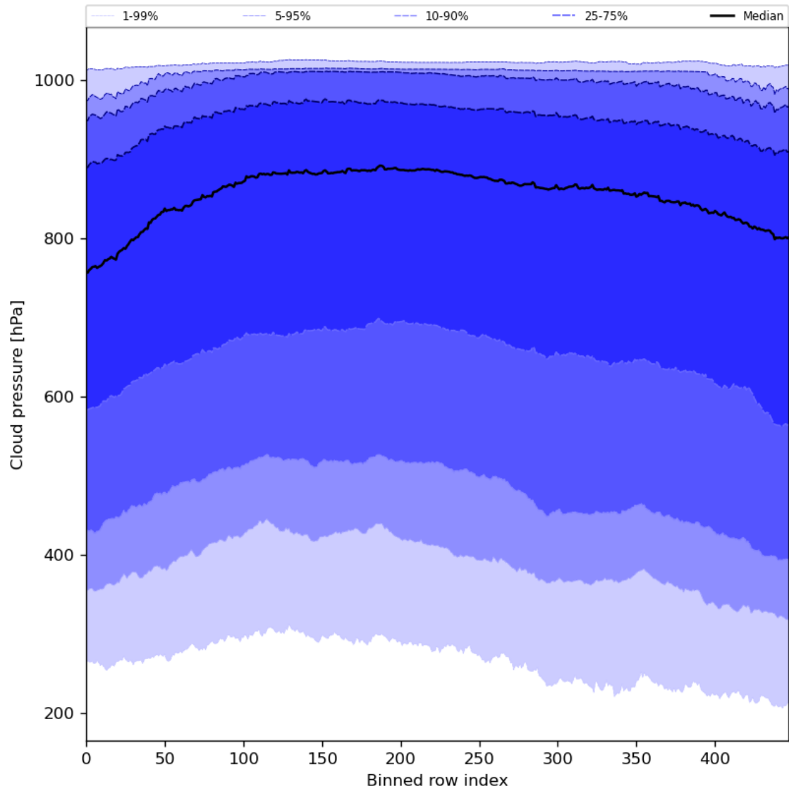
Figure 47: Along track statistics of “Cloud pressure” for 2024-03-25 to 2024-03-26
