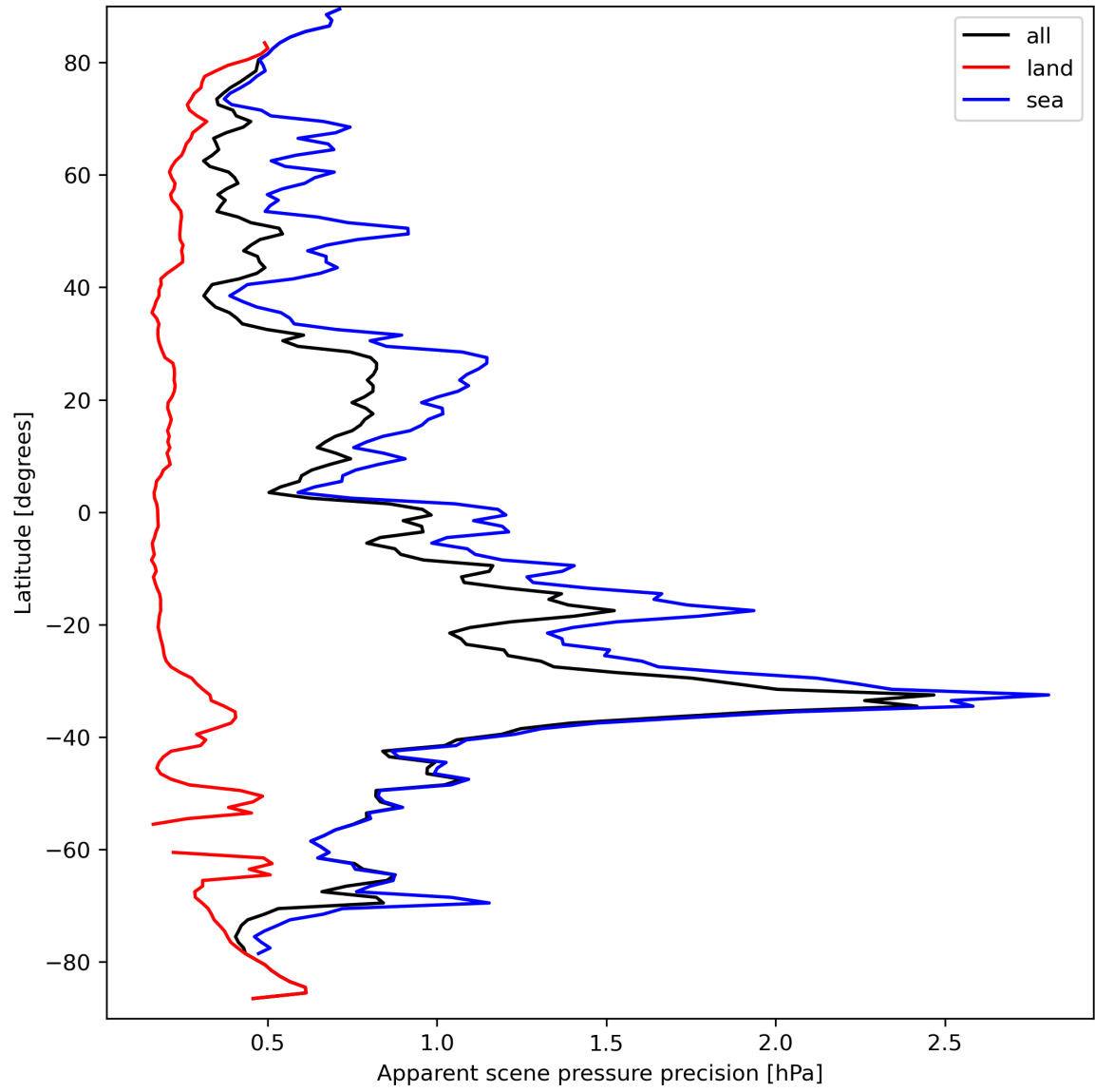
Figure 20: Zonal average of “Apparent scene pressure precision” for 2024-03-25 to 2024-03-26.
