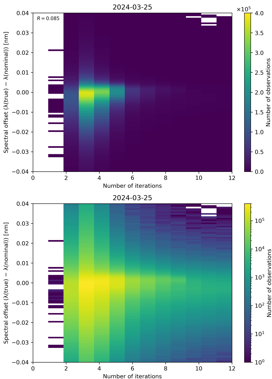
Figure 100: Scatter density plot of “Number of iterations” against “Spectral offset ( \lambda(\text{true}) - \lambda(\text{nominal}) )” for 2024-03-25 to 2024-03-26.
