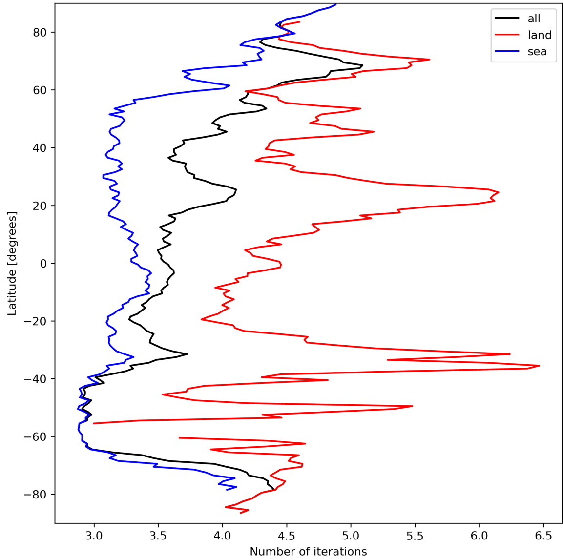
Figure 22: Zonal average of “Number of iterations” for 2024-03-25 to 2024-03-26.
