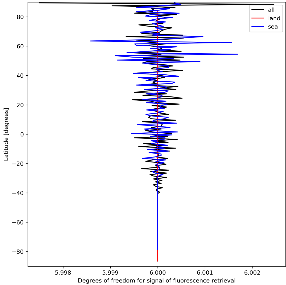
Figure 26: Zonal average of “Degrees of freedom for signal of fluorescence retrieval” for 2024-03-25 to 2024-03-26.
