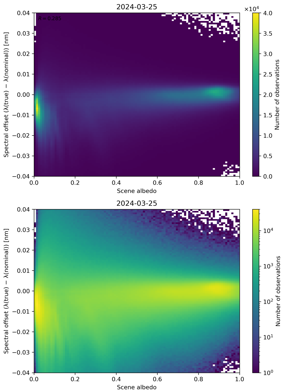
Figure 107: Scatter density plot of “Scene albedo” against “Spectral offset ( \lambda(\text{true}) - \lambda(\text{nominal}) )” for 2024-03-25 to 2024-03-26.
