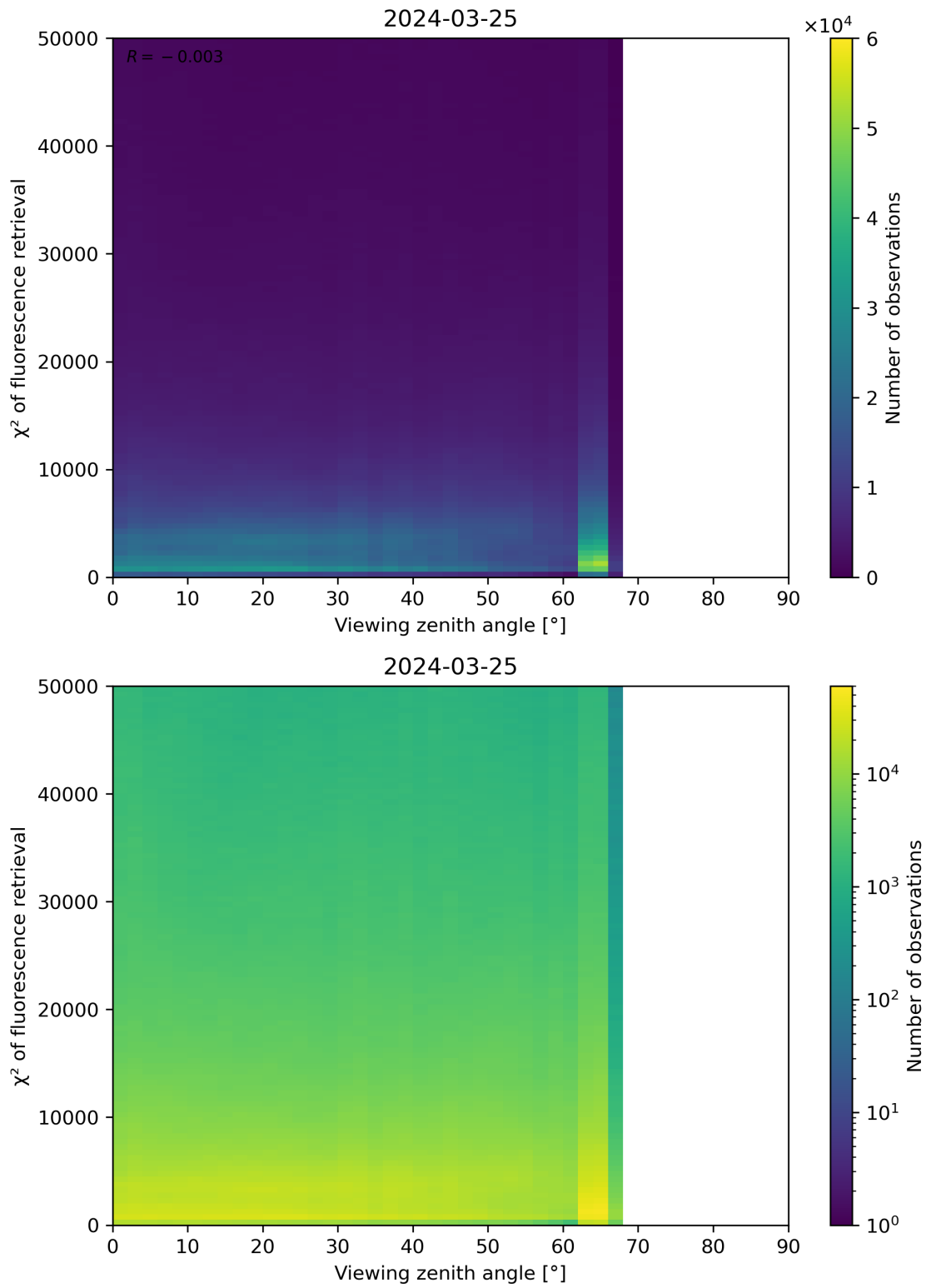
Figure 119: Scatter density plot of “Viewing zenith angle” against “ \chi^2 of fluorescence retrieval” for 2024-03-25 to 2024-03-26.
