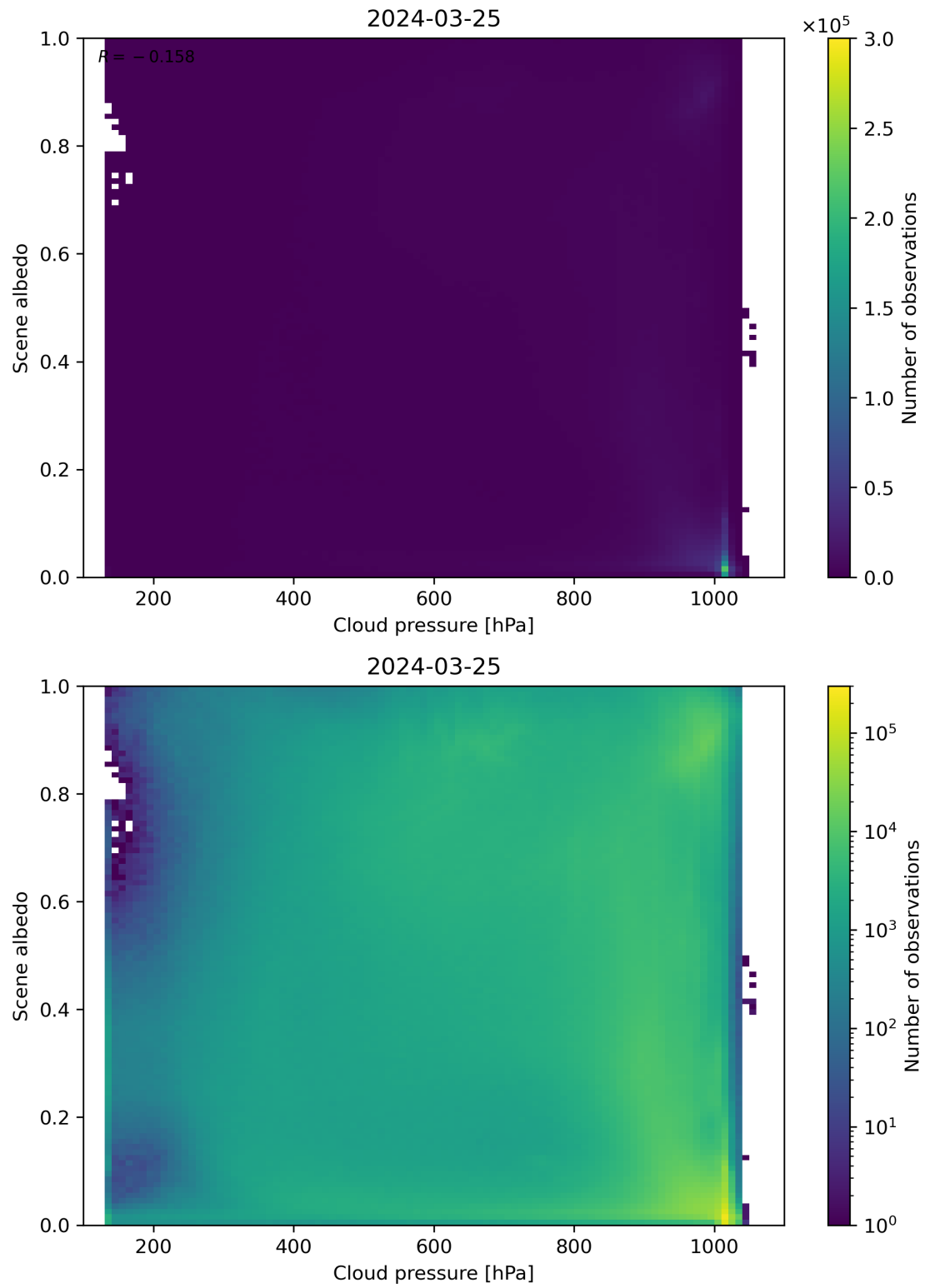
Figure 83: Scatter density plot of “Cloud pressure” against “Scene albedo” for 2024-03-25 to 2024-03-26.
