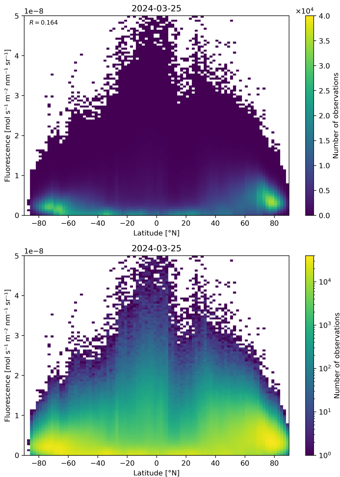
Figure 92: Scatter density plot of “Latitude” against “Fluorescence” for 2024-03-25 to 2024-03-26.
