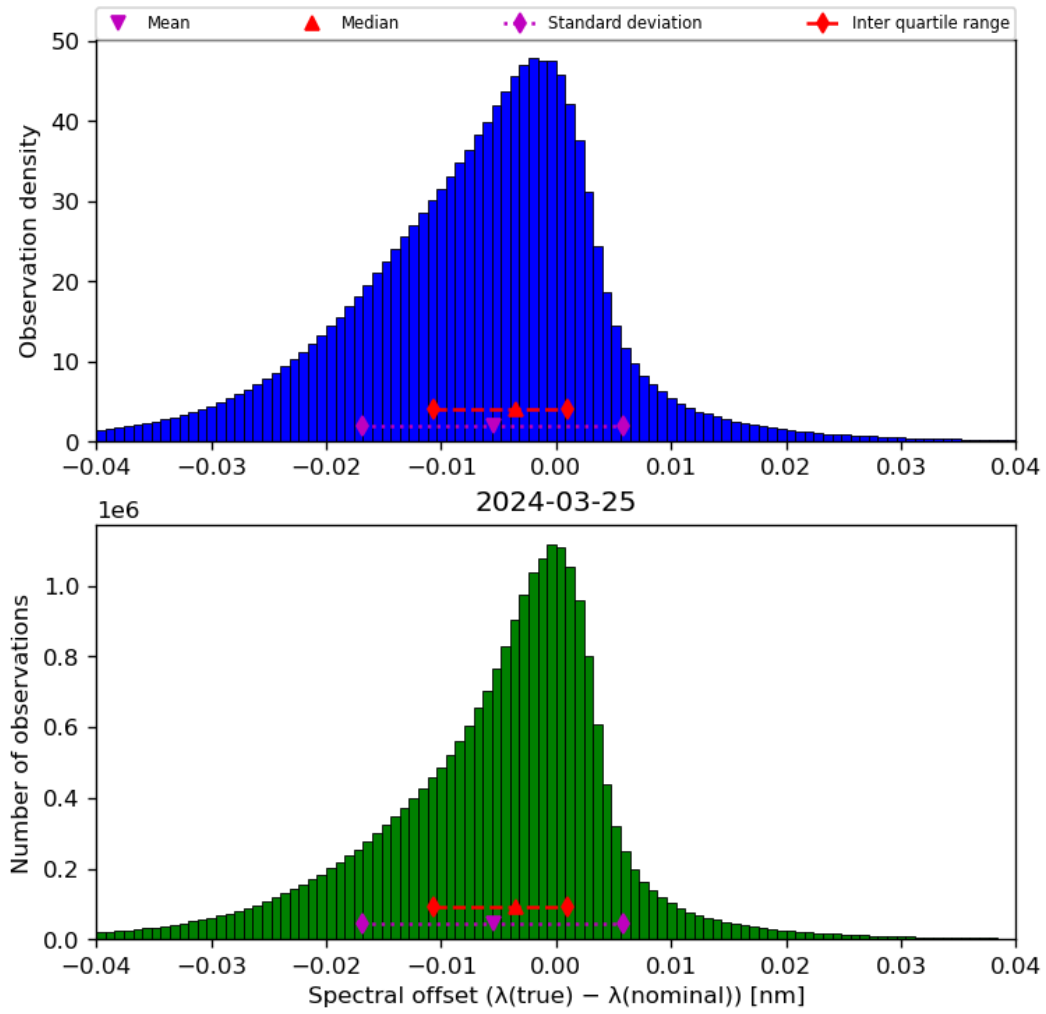
Figure 45: Histogram of “Spectral offset ( \lambda(\text{true}) - \lambda(\text{nominal}) )” for 2024-03-25 to 2024-03-26
