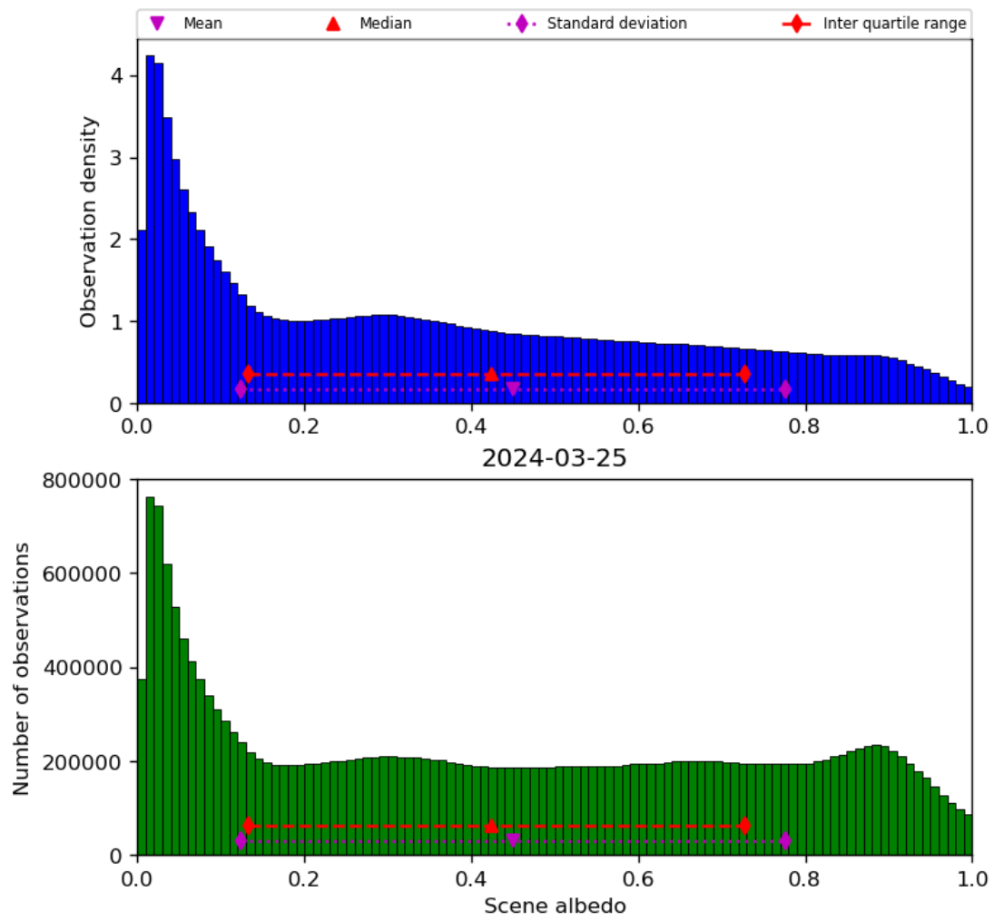
Figure 34: Histogram of “Scene albedo” for 2024-03-25 to 2024-03-26
