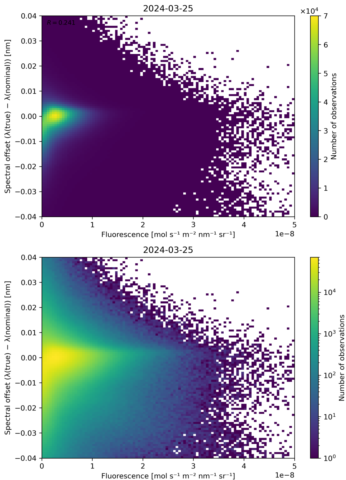
Figure 87: Scatter density plot of “Fluorescence” against “Spectral offset ( \lambda(\text{true}) - \lambda(\text{nominal}) )” for 2024-03-25 to 2024-03-26.
