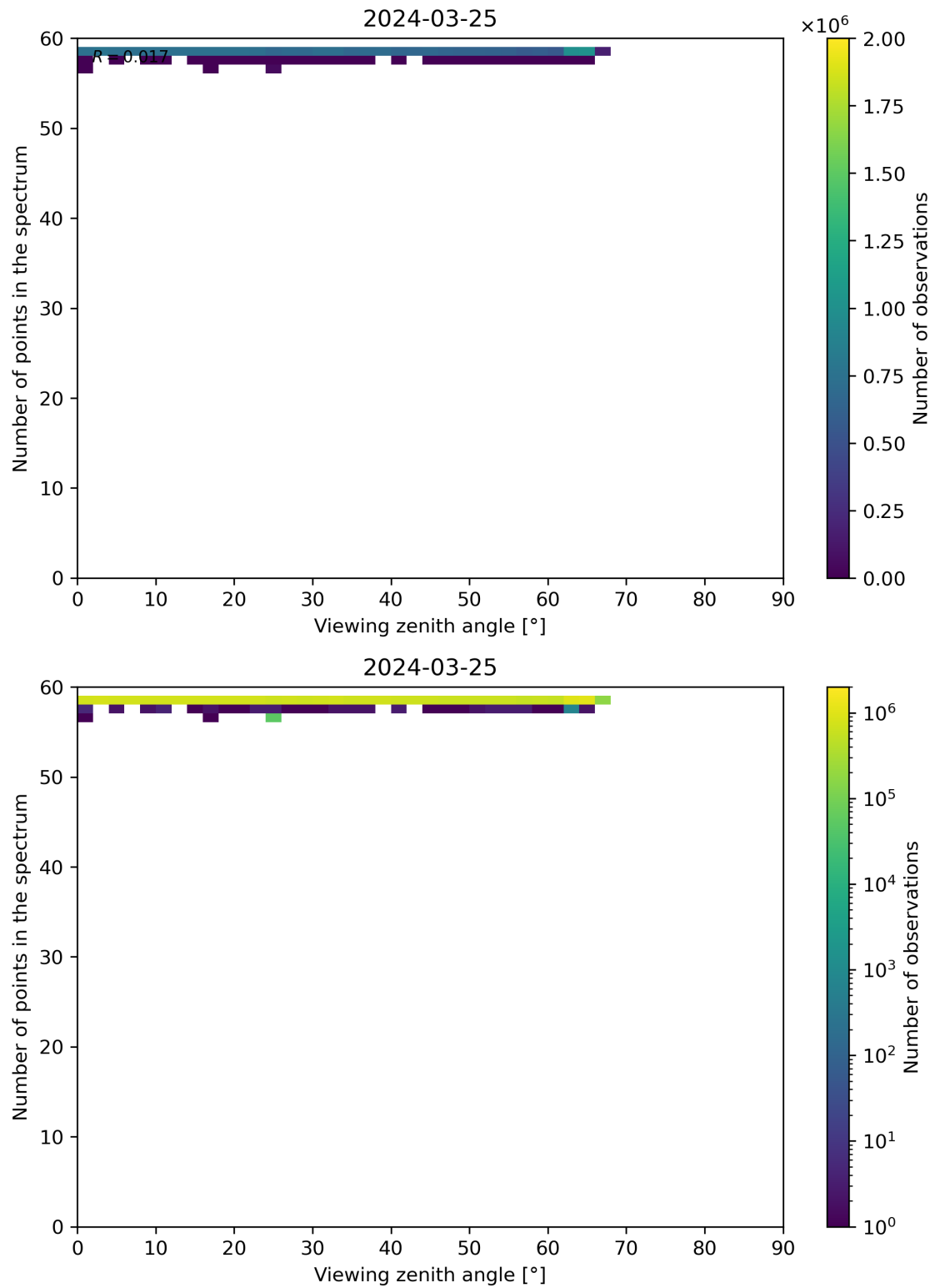
Figure 125: Scatter density plot of “Viewing zenith angle” against “Number of points in the spectrum” for 2024-03-25 to 2024-03-26.
