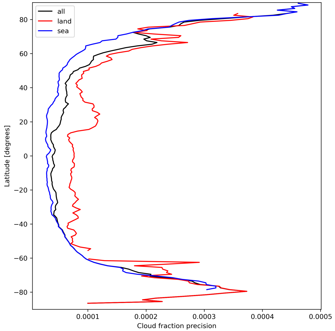
Figure 16: Zonal average of “Cloud fraction precision” for 2024-03-25 to 2024-03-26.
