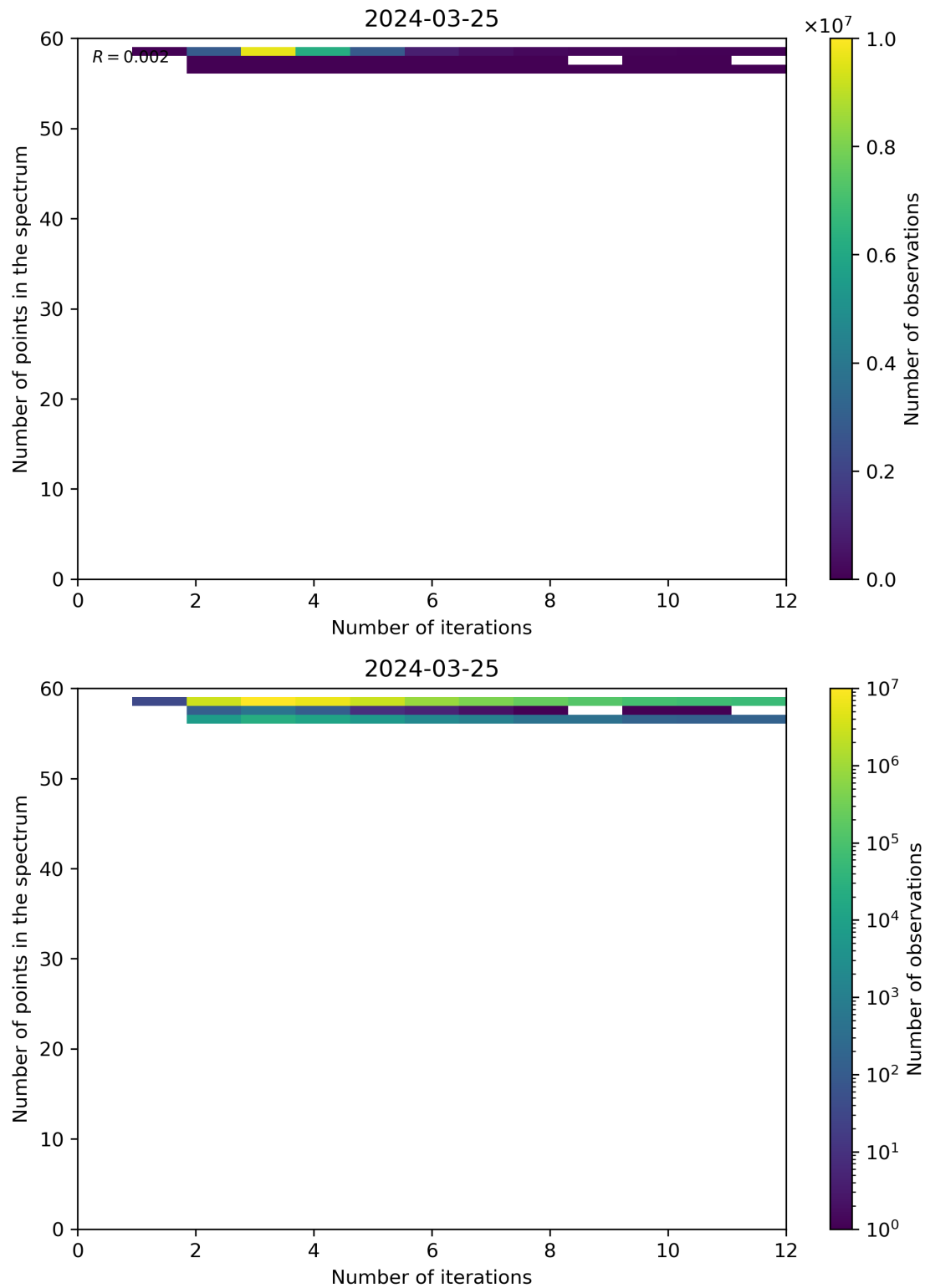
Figure 99: Scatter density plot of “Number of iterations” against “Number of points in the spectrum” for 2024-03-25 to 2024-03-26.
