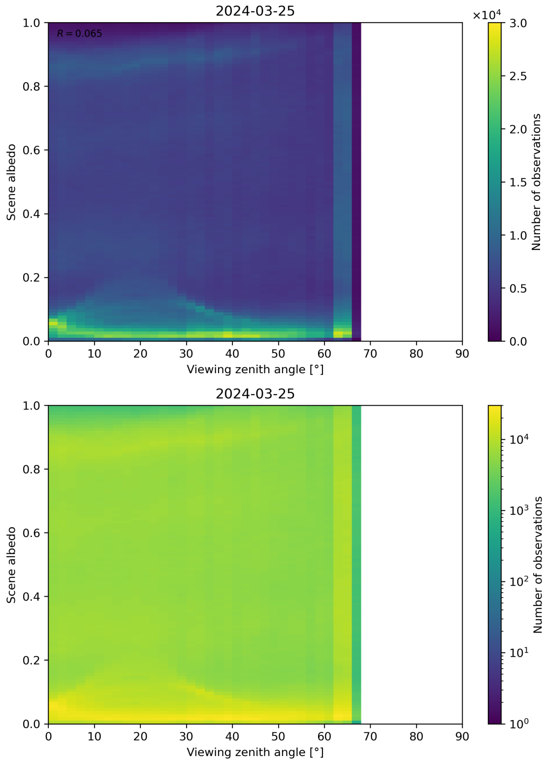
Figure 126: Scatter density plot of “Viewing zenith angle” against “Scene albedo” for 2024-03-25 to 2024-03-26.
