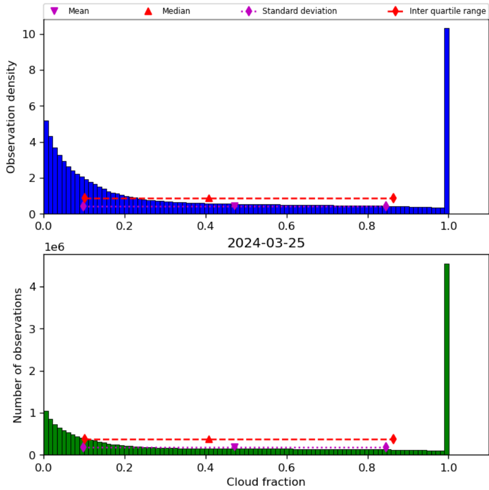
Figure 32: Histogram of “Cloud fraction” for 2024-03-25 to 2024-03-26
