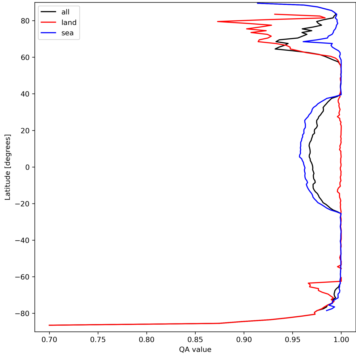
Figure 12: Zonal average of "QA value" for 2024-03-25 to 2024-03-26.
