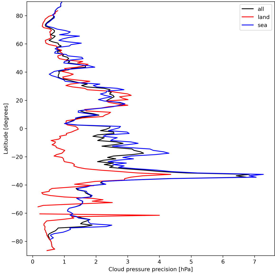
Figure 14: Zonal average of “Cloud pressure precision” for 2024-03-25 to 2024-03-26.
