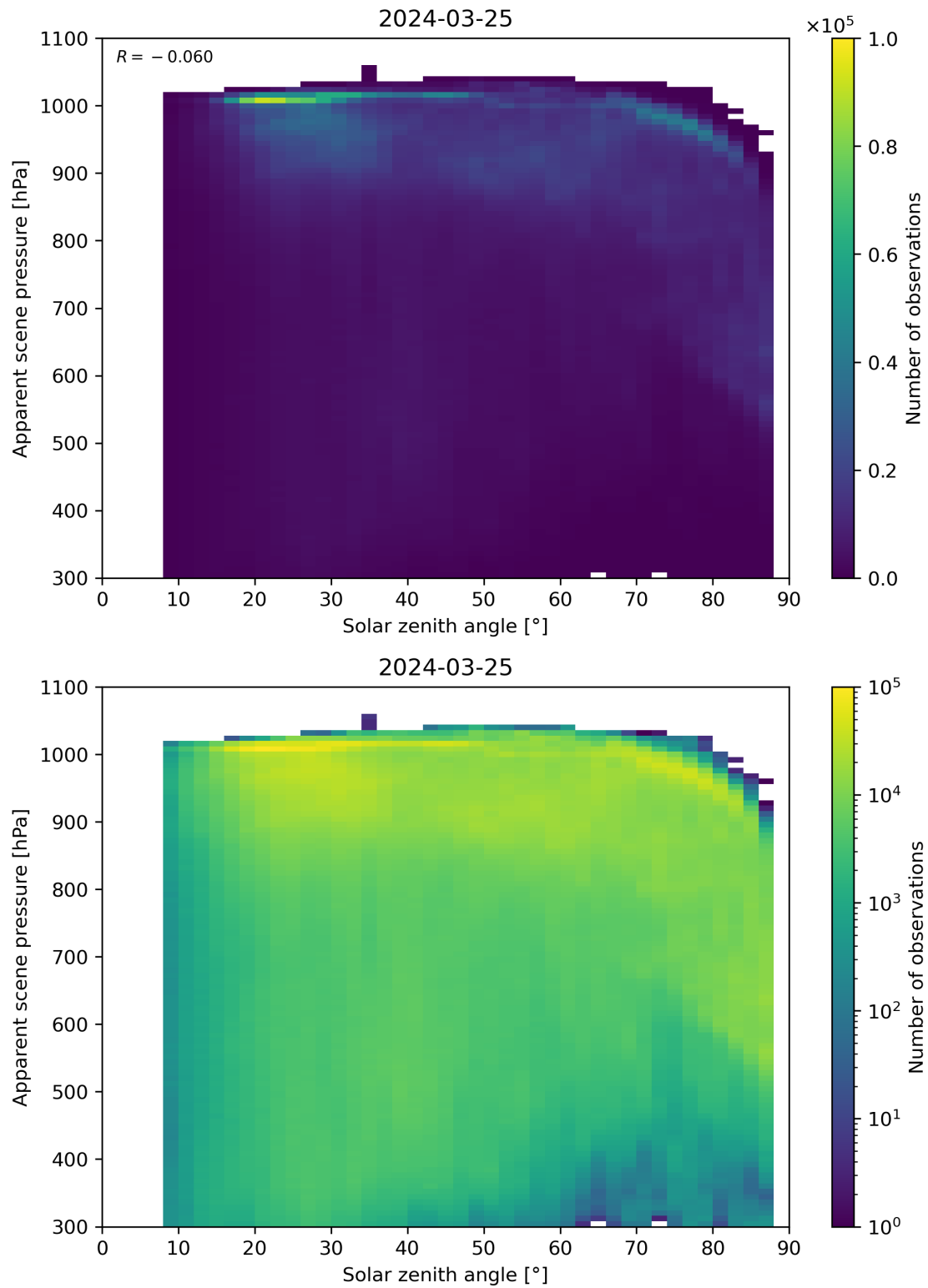
Figure 108: Scatter density plot of “Solar zenith angle” against “Apparent scene pressure” for 2024-03-25 to 2024-03-26.
