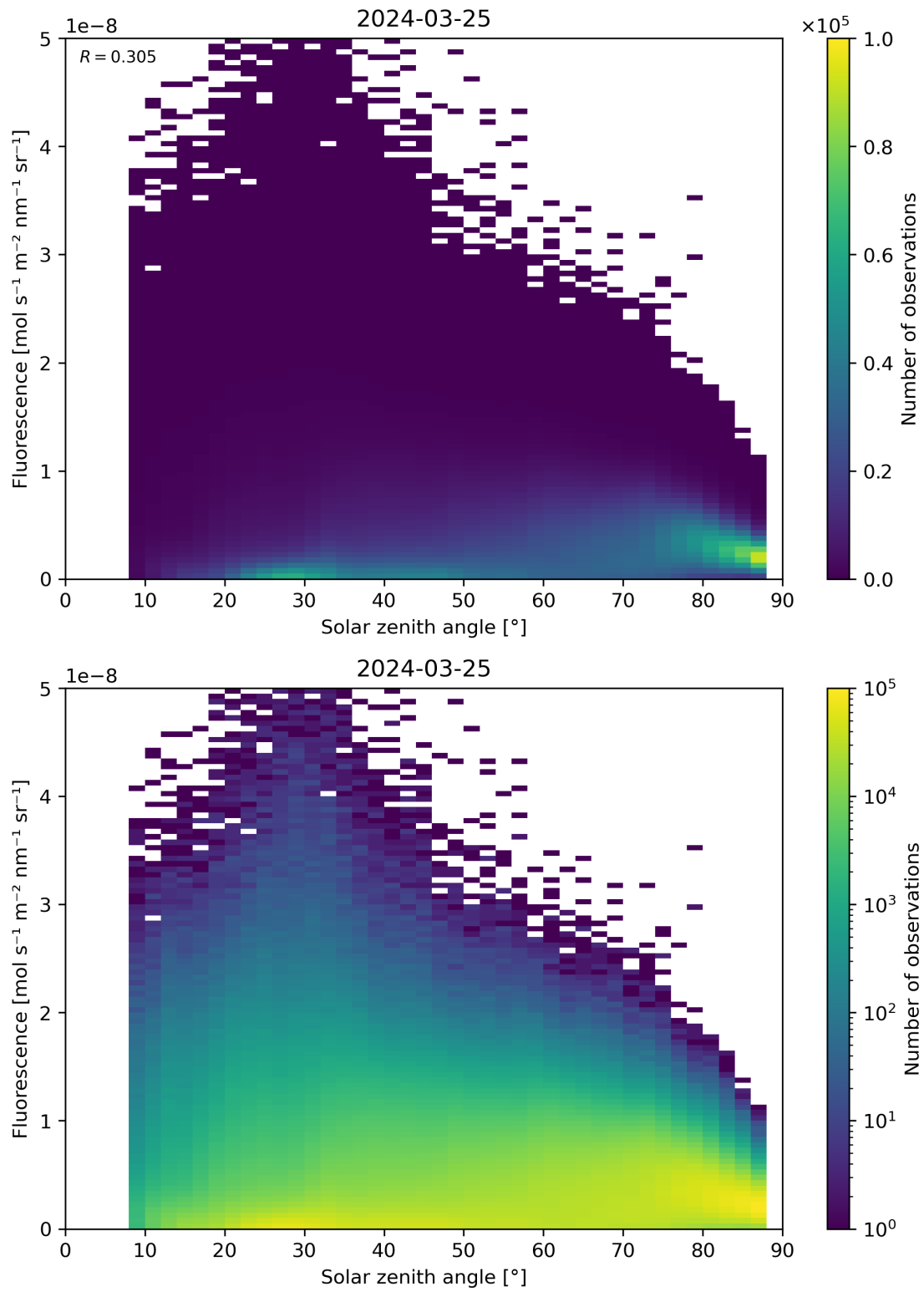
Figure 112: Scatter density plot of “Solar zenith angle” against “Fluorescence” for 2024-03-25 to 2024-03-26.
