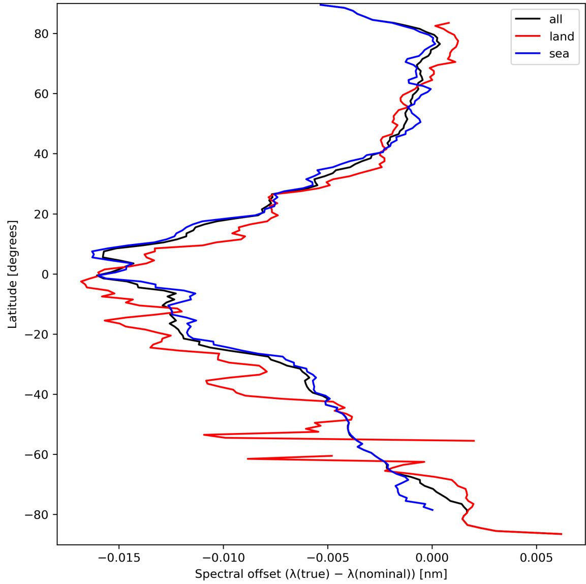
Figure 28: Zonal average of “Spectral offset ( \lambda(\text{true}) - \lambda(\text{nominal}) )” for 2024-03-25 to 2024-03-26.
