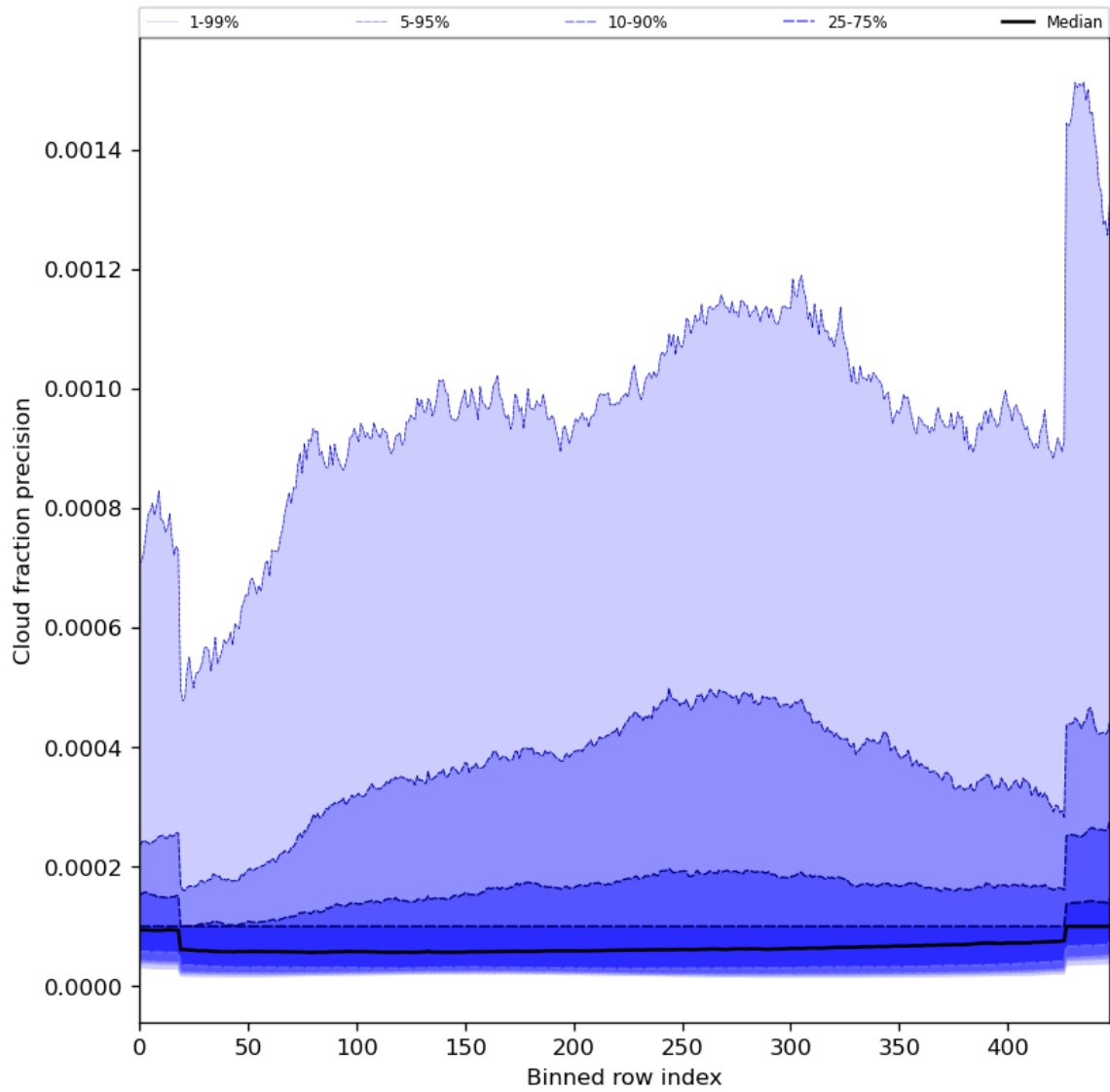
Figure 50: Along track statistics of “Cloud fraction precision” for 2024-03-25 to 2024-03-26
