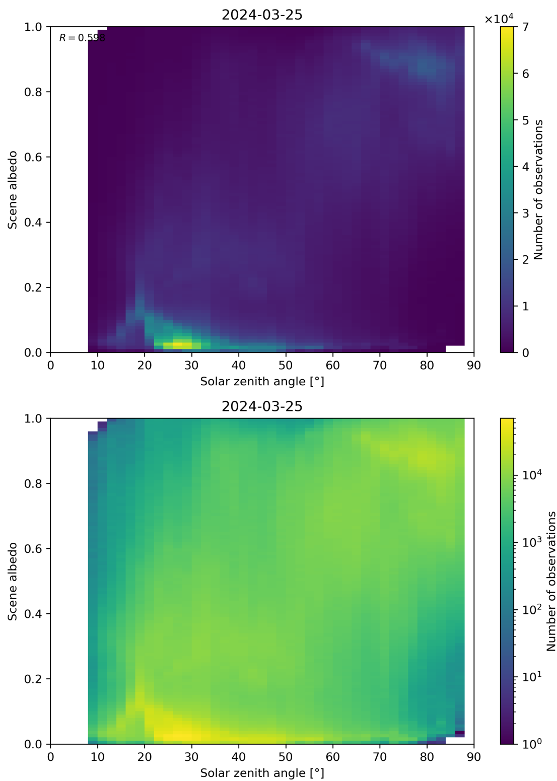
Figure 116: Scatter density plot of “Solar zenith angle” against “Scene albedo” for 2024-03-25 to 2024-03-26.
