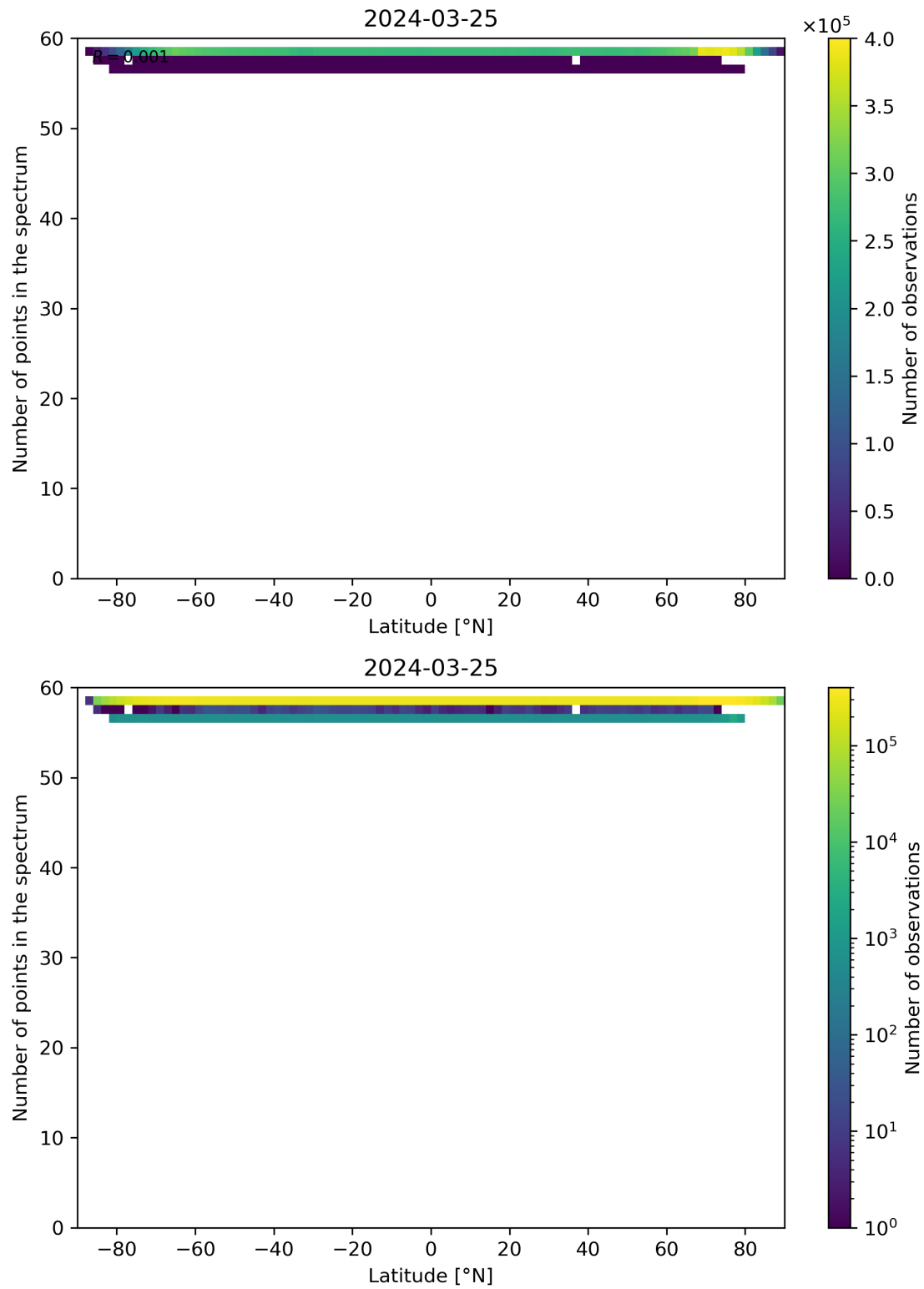
Figure 94: Scatter density plot of “Latitude” against “Number of points in the spectrum” for 2024-03-25 to 2024-03-26.
