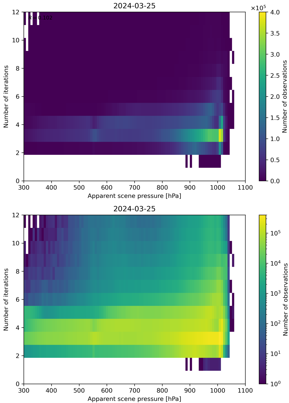
Figure 65: Scatter density plot of “Apparent scene pressure” against “Number of iterations” for 2024-03-25 to 2024-03-26.
