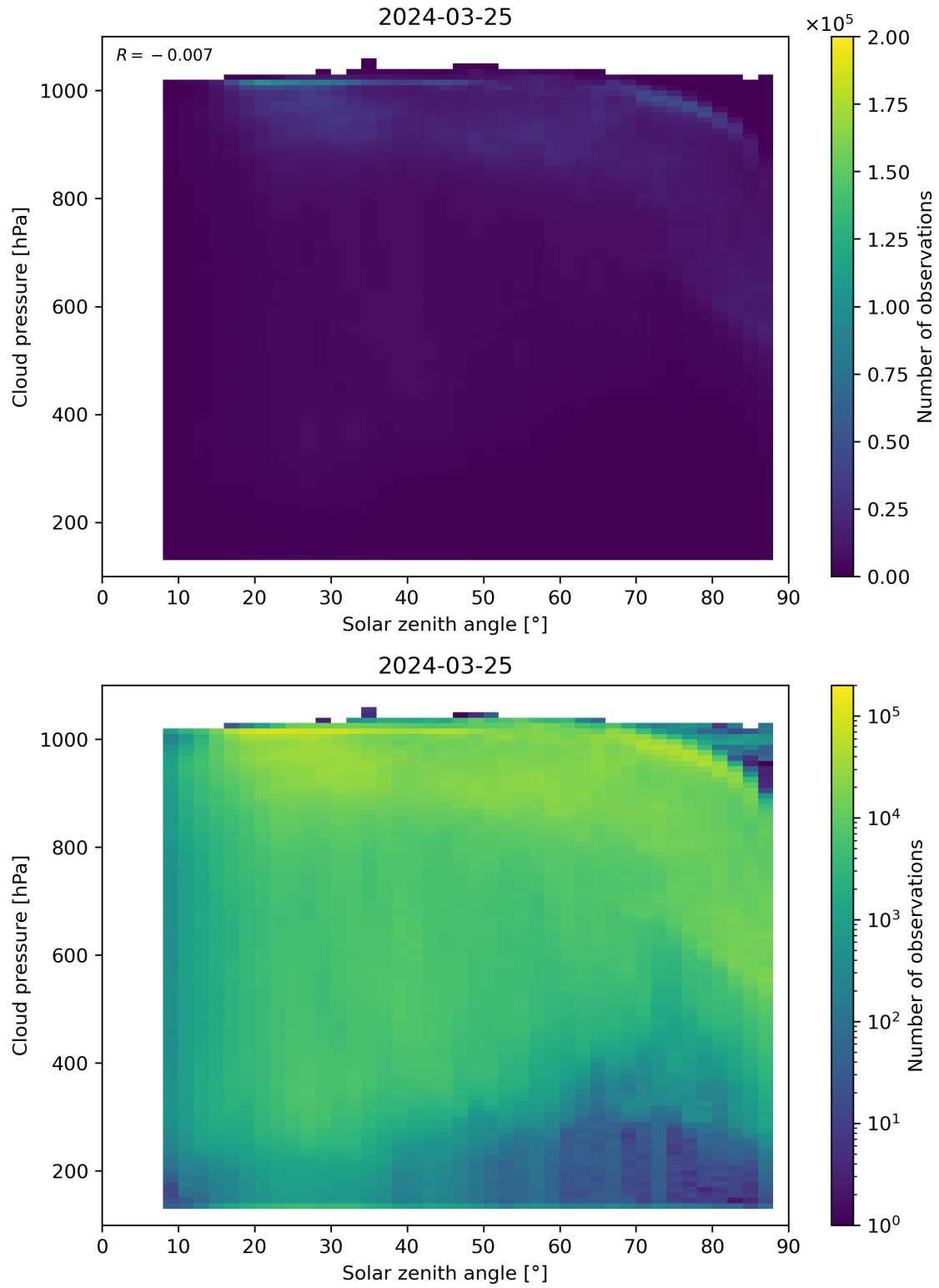
Figure 111: Scatter density plot of “Solar zenith angle” against “Cloud pressure” for 2024-03-25 to 2024-03-26.
