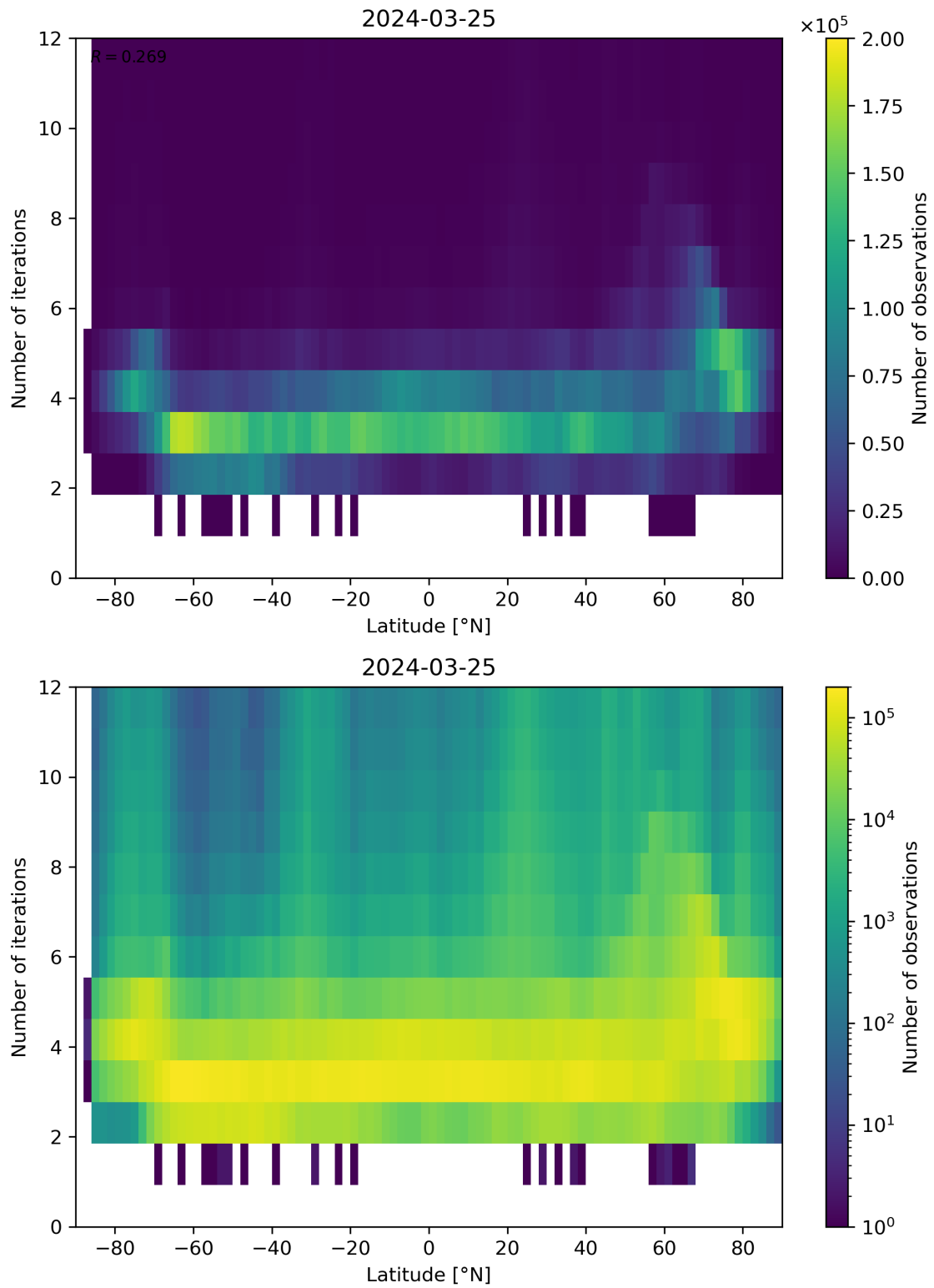
Figure 93: Scatter density plot of “Latitude” against “Number of iterations” for 2024-03-25 to 2024-03-26.
