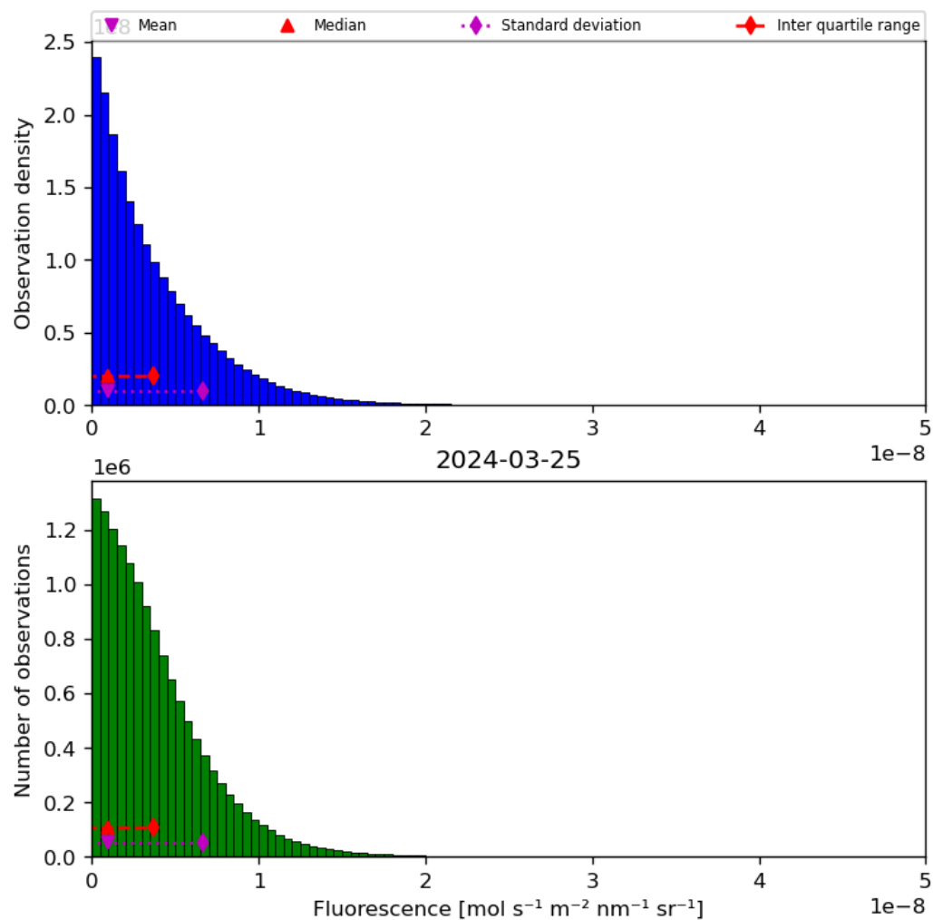
Figure 40: Histogram of “Fluorescence” for 2024-03-25 to 2024-03-26
