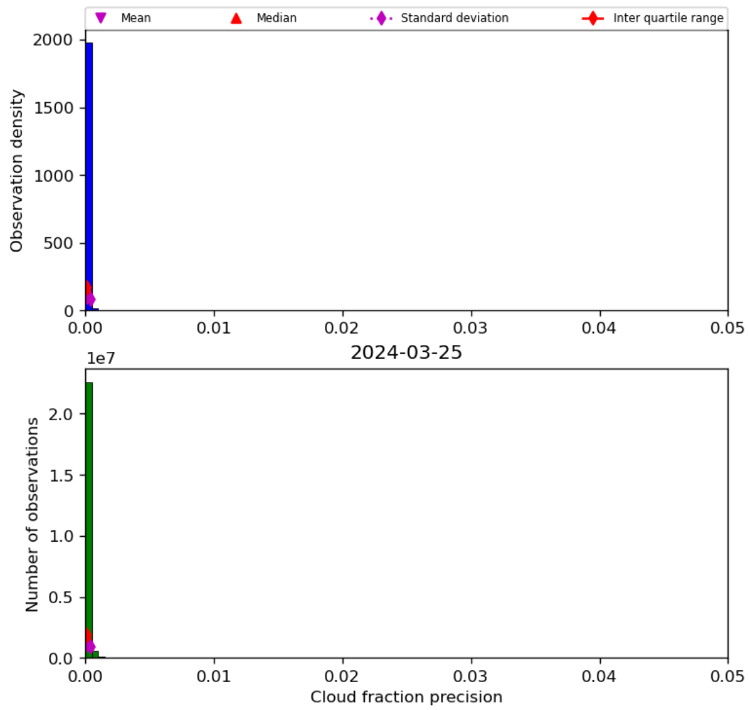
Figure 33: Histogram of “Cloud fraction precision” for 2024-03-25 to 2024-03-26
