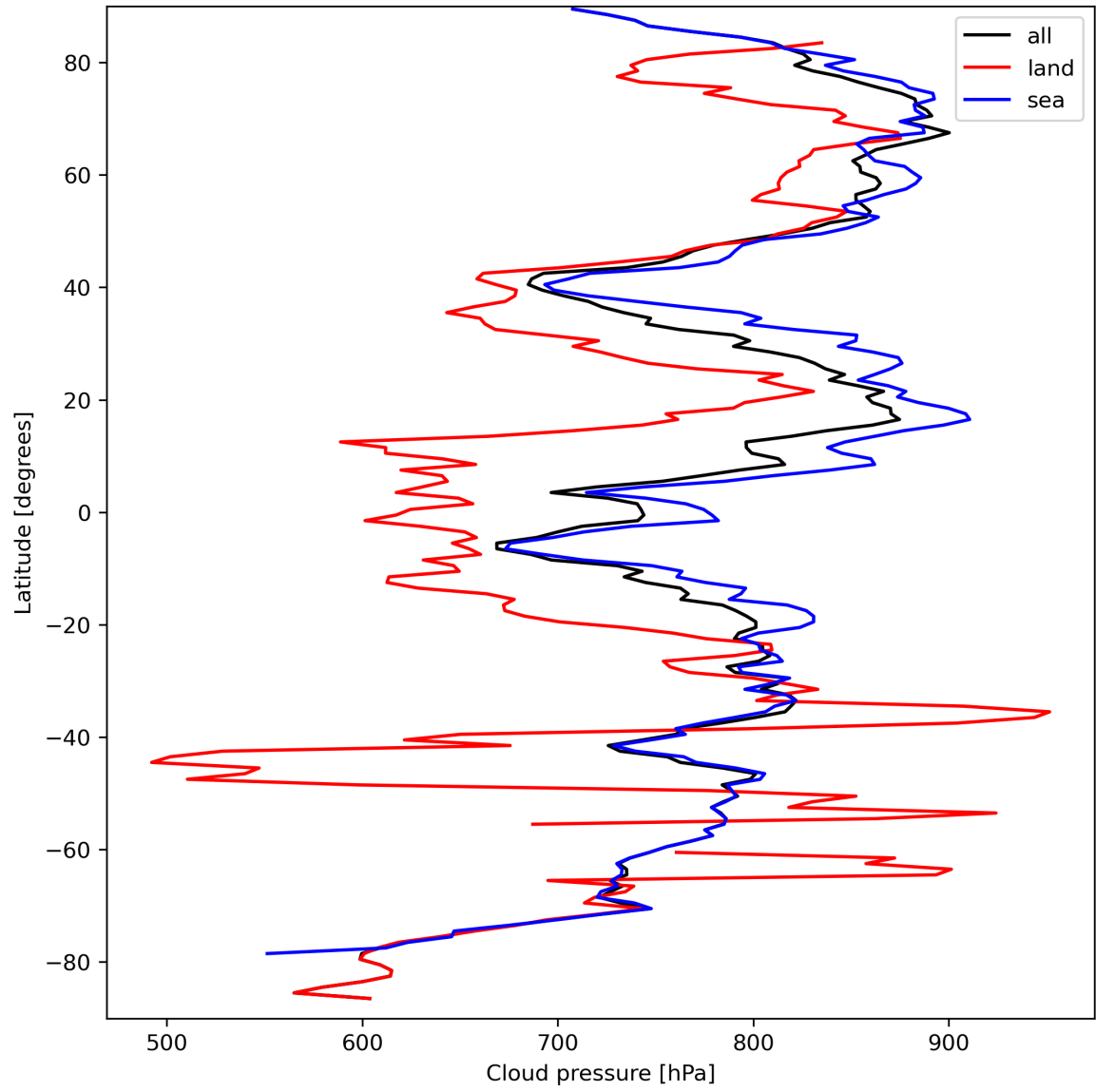
Figure 13: Zonal average of “Cloud pressure” for 2024-03-25 to 2024-03-26.
