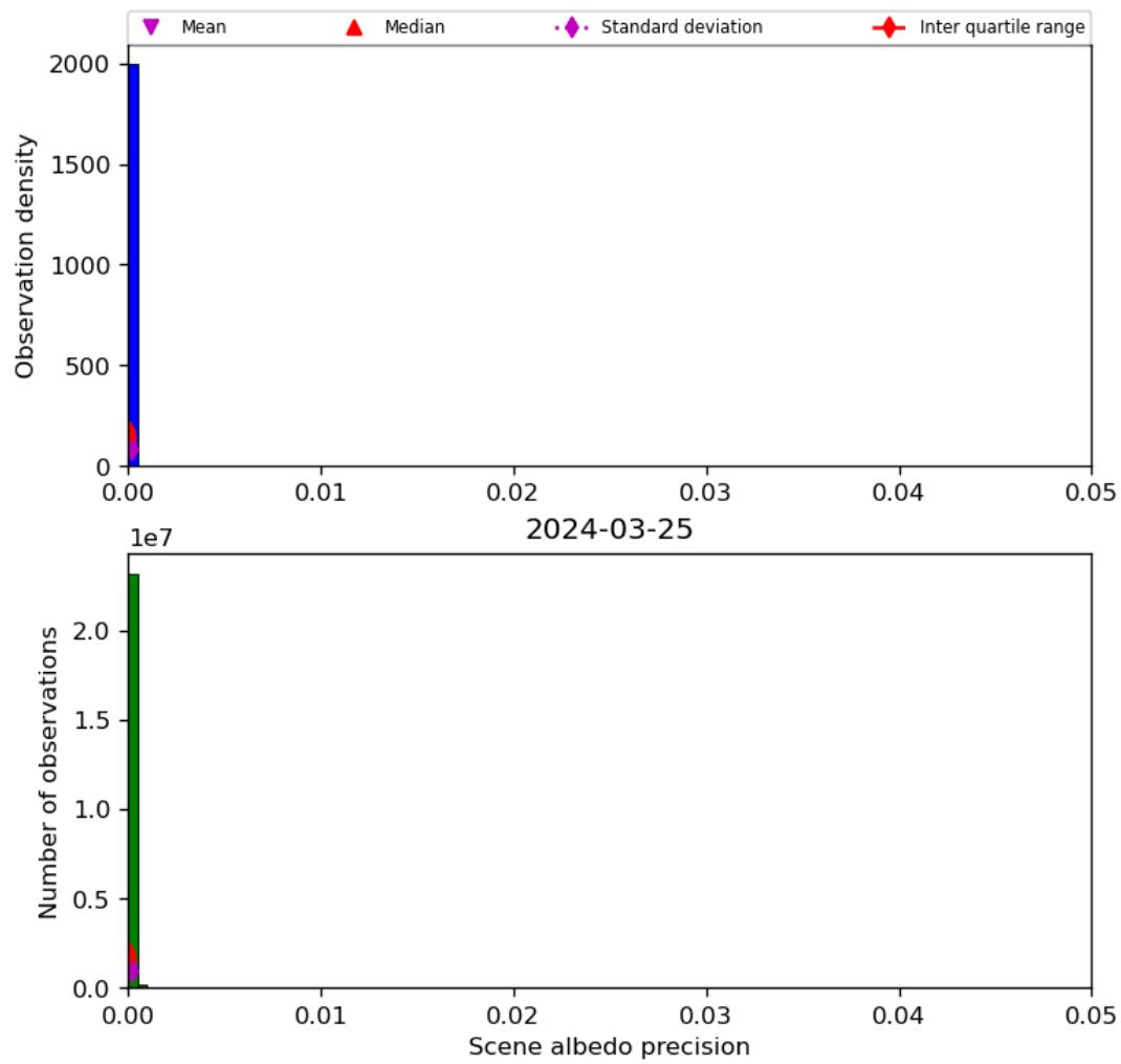
Figure 35: Histogram of “Scene albedo precision” for 2024-03-25 to 2024-03-26
