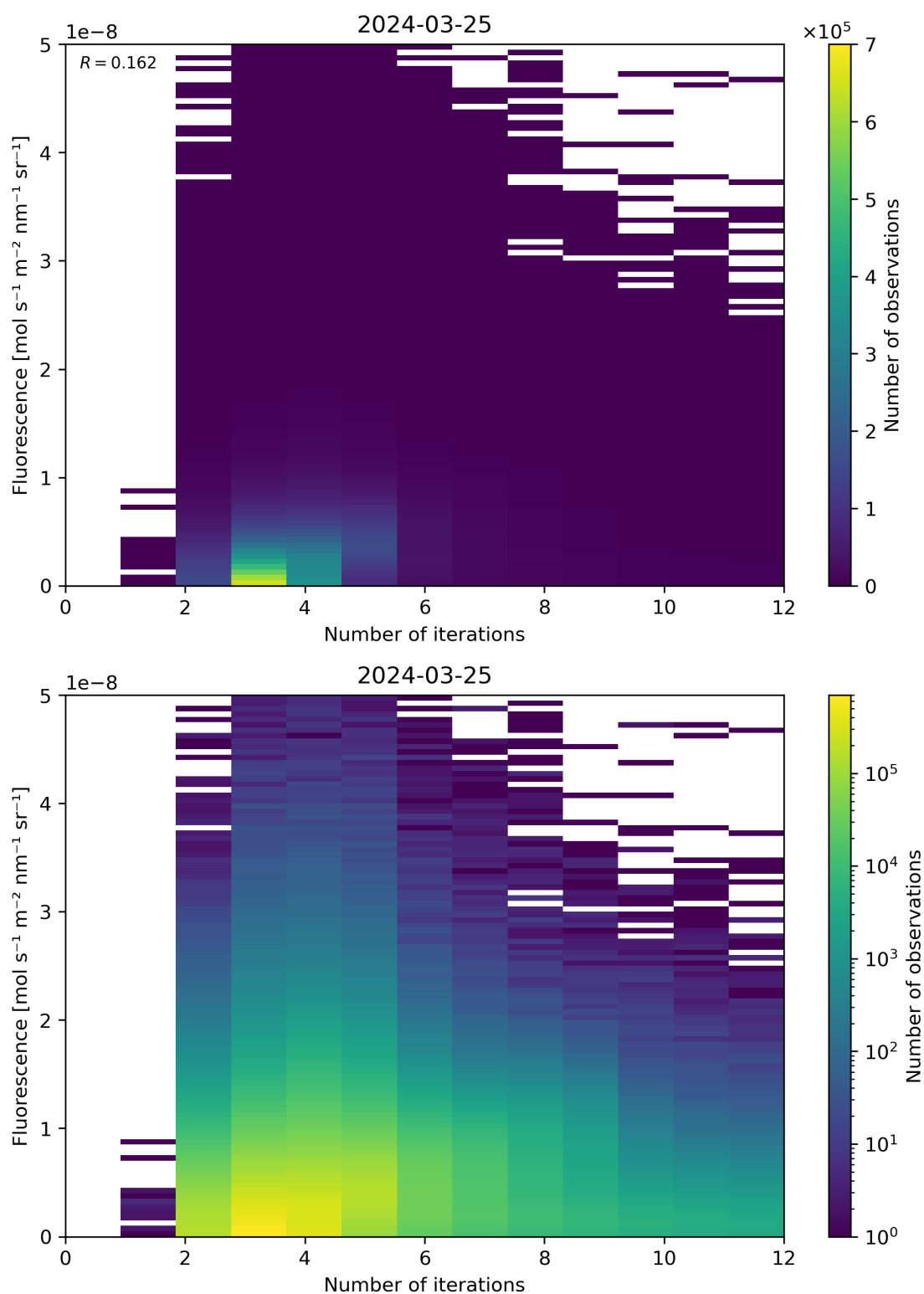
Figure 98: Scatter density plot of “Number of iterations” against “Fluorescence” for 2024-03-25 to 2024-03-26.
