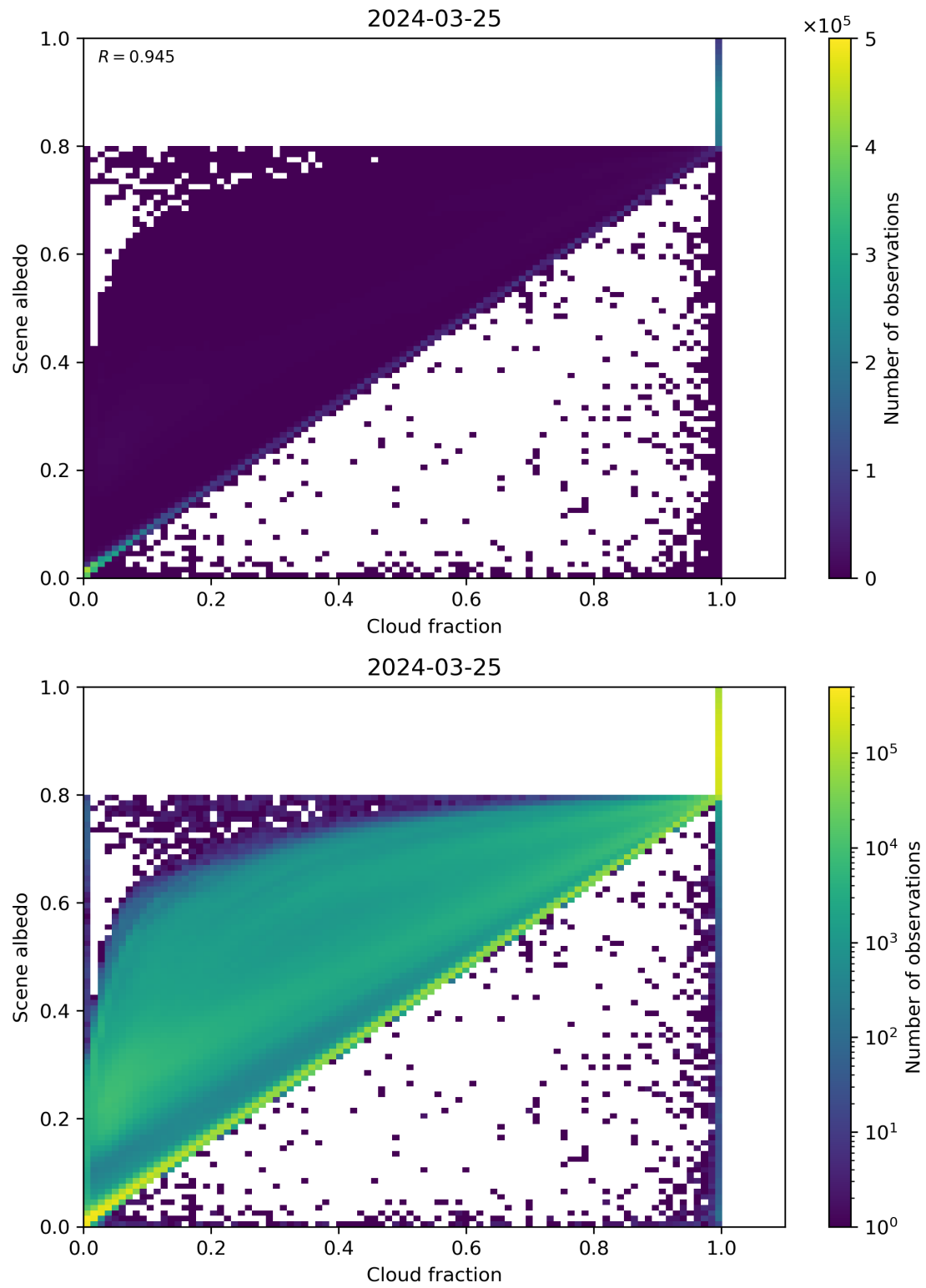
Figure 75: Scatter density plot of “Cloud fraction” against “Scene albedo” for 2024-03-25 to 2024-03-26.
