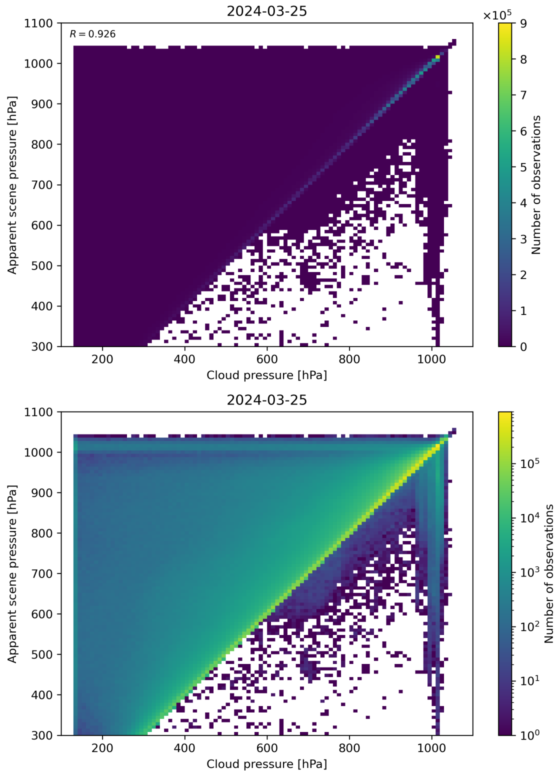
Figure 77: Scatter density plot of “Cloud pressure” against “Apparent scene pressure” for 2024-03-25 to 2024-03-26.
