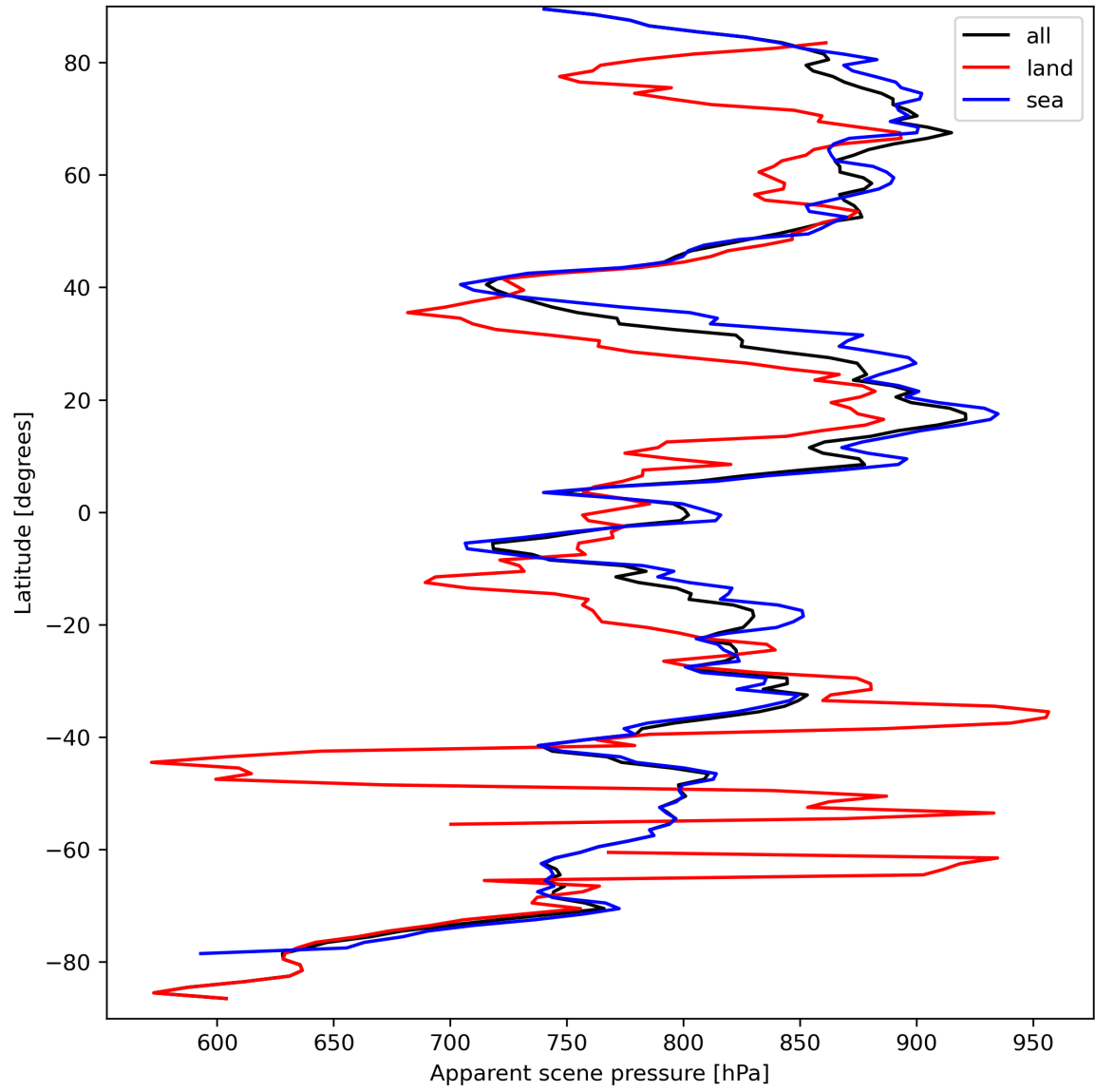
Figure 19: Zonal average of “Apparent scene pressure” for 2024-03-25 to 2024-03-26.
