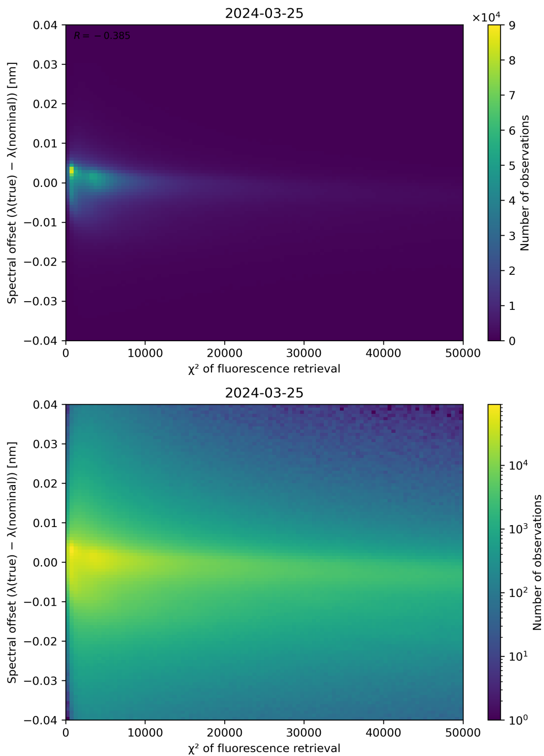
Figure 69: Scatter density plot of " \chi^2 of fluorescence retrieval" against "Spectral offset ( \lambda(\text{true}) - \lambda(\text{nominal}) )" for 2024-03-25 to 2024-03-26.
