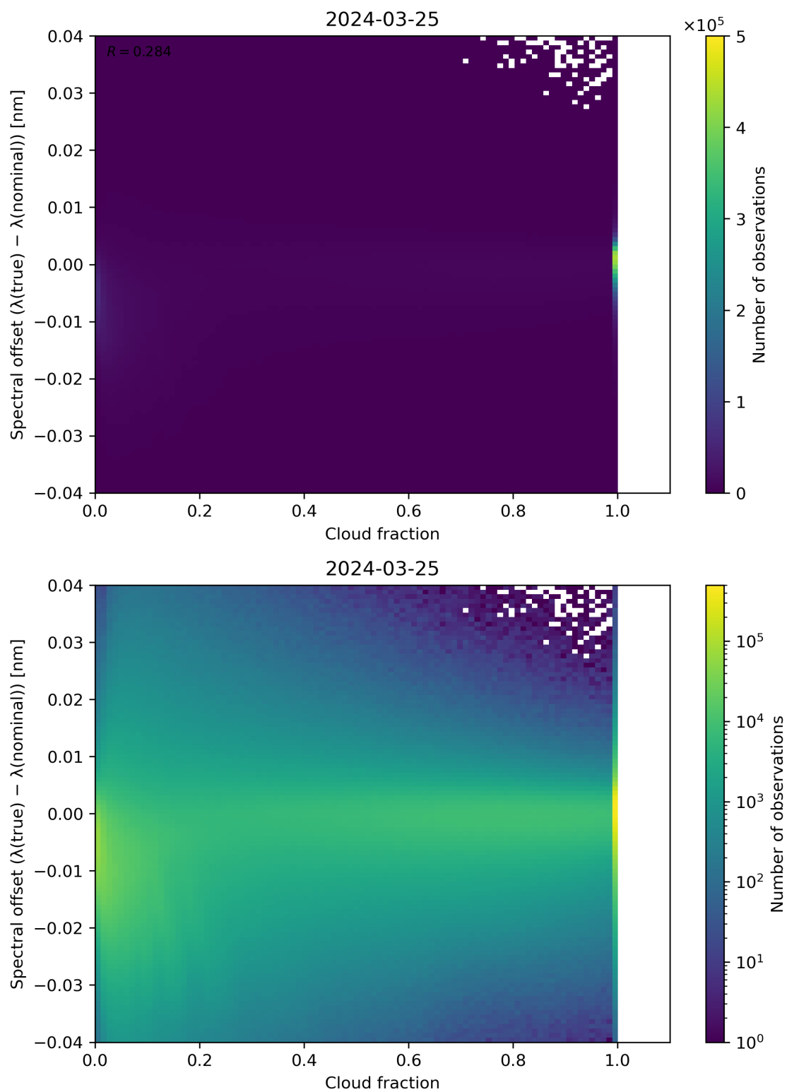
Figure 76: Scatter density plot of “Cloud fraction” against “Spectral offset ( \lambda(\text{true}) - \lambda(\text{nominal}) )” for 2024-03-25 to 2024-03-26.
