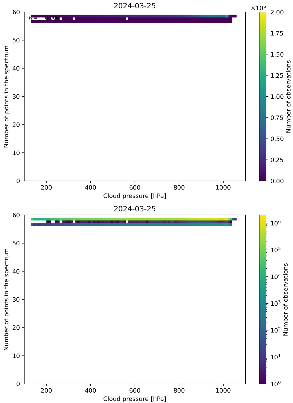
Figure 82: Scatter density plot of “Cloud pressure” against “Number of points in the spectrum” for 2024-03-25 to 2024-03-26.
