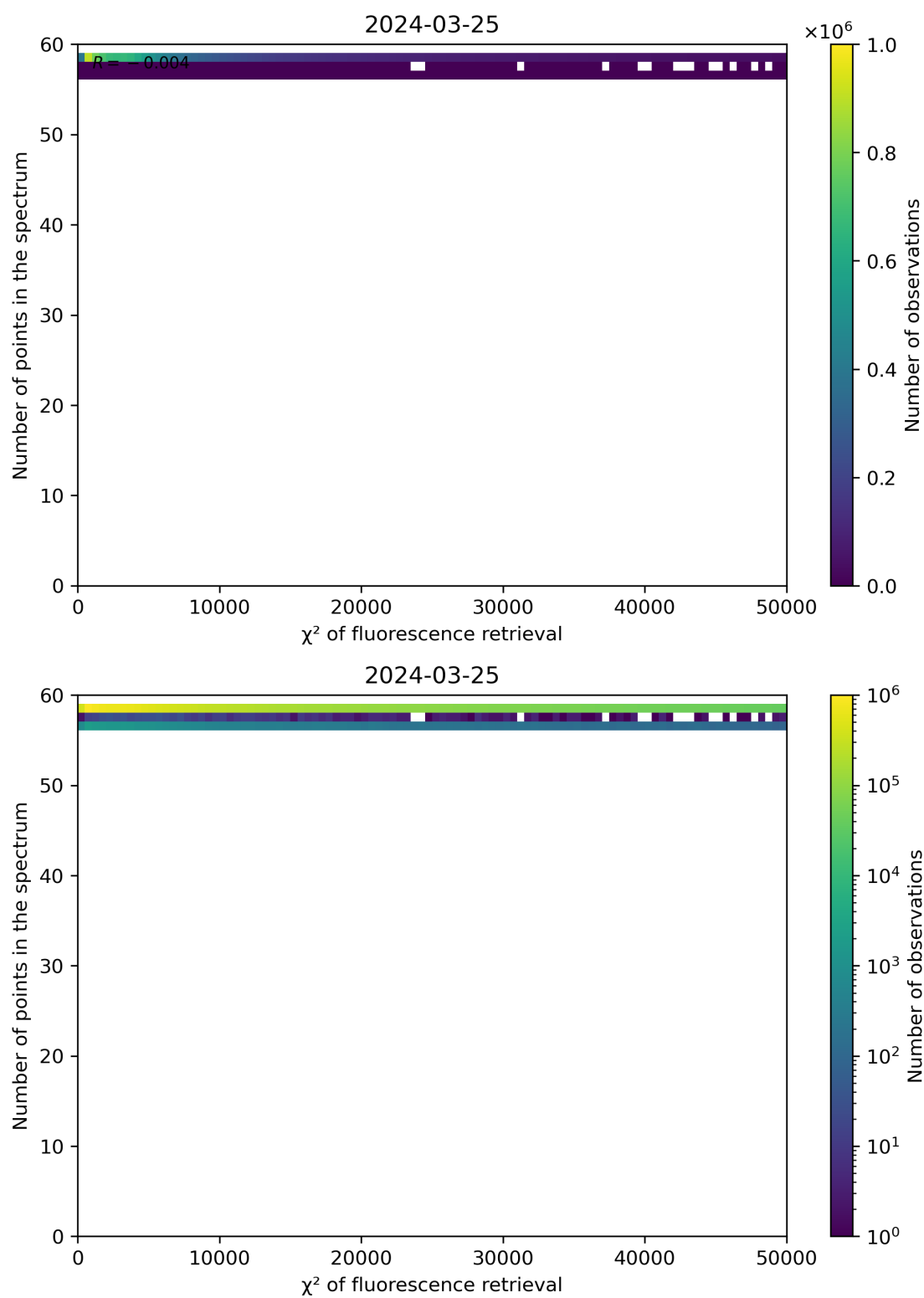
Figure 68: Scatter density plot of “ \chi^2 of fluorescence retrieval” against “Number of points in the spectrum” for 2024-03-25 to 2024-03-26.
