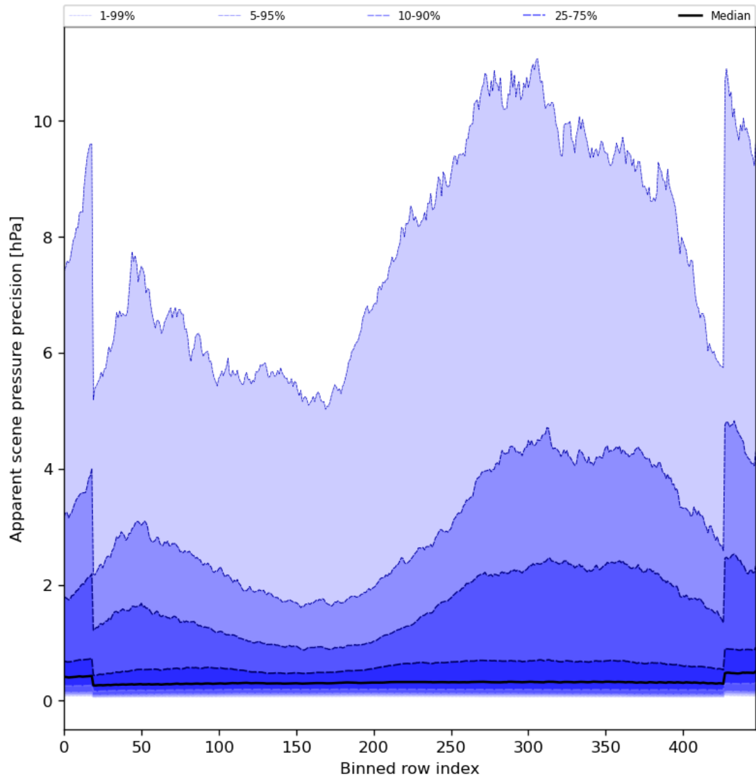
Figure 54: Along track statistics of “Apparent scene pressure precision” for 2024-03-25 to 2024-03-26
