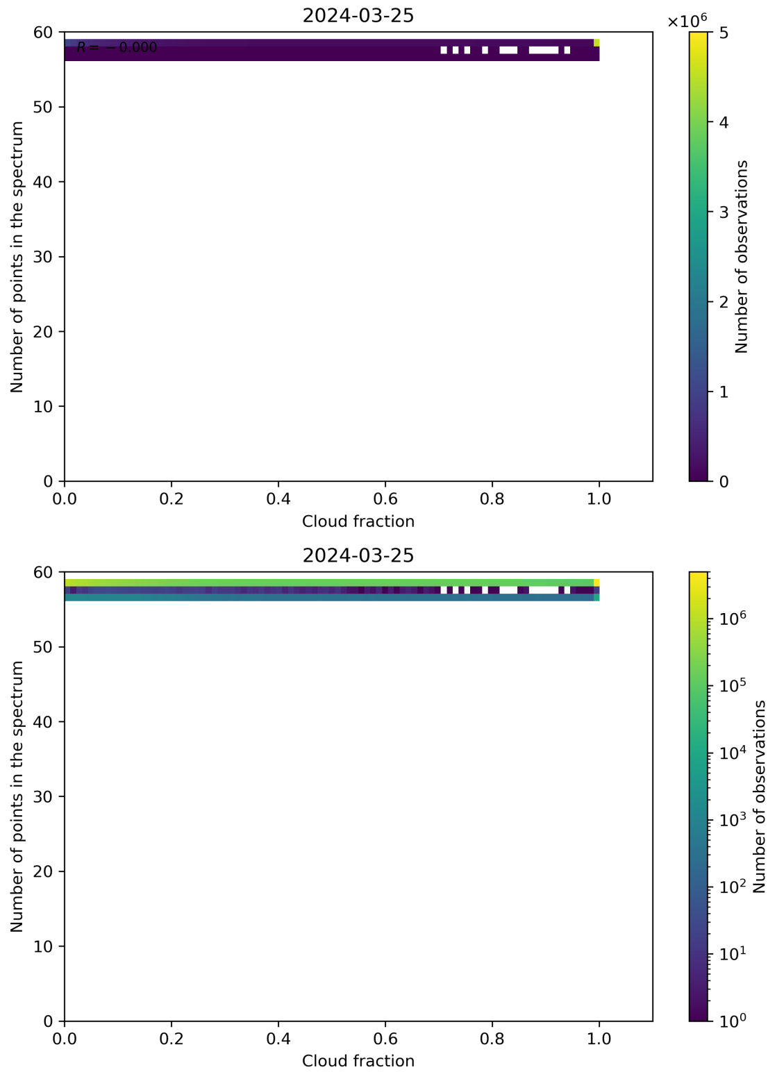
Figure 74: Scatter density plot of “Cloud fraction” against “Number of points in the spectrum” for 2024-03-25 to 2024-03-26.
