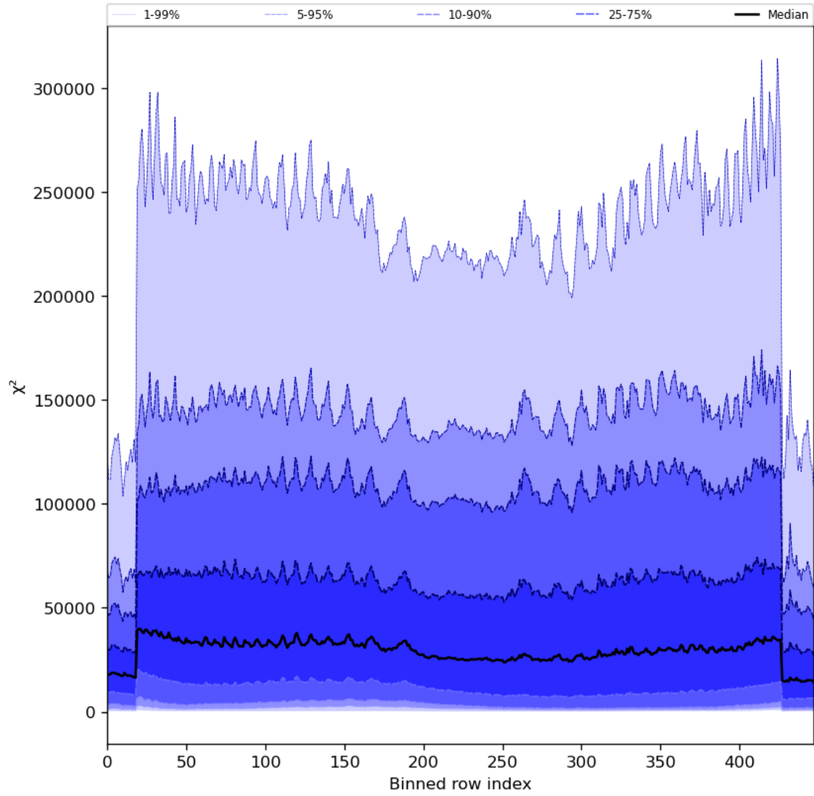
Figure 55: Along track statistics of “ \chi^2 ” for 2024-03-25 to 2024-03-26
