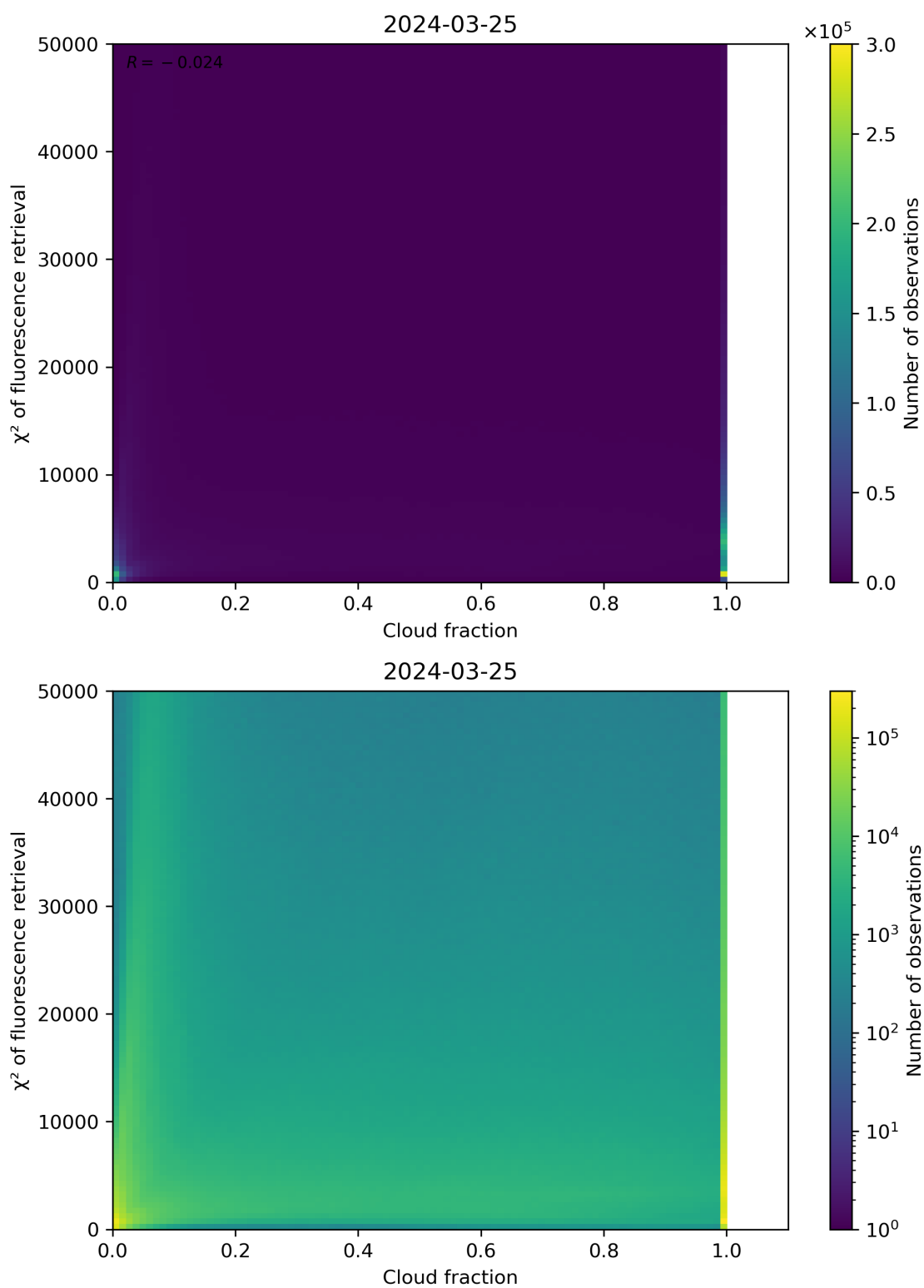
Figure 71: Scatter density plot of “Cloud fraction” against “ \chi^2 of fluorescence retrieval” for 2024-03-25 to 2024-03-26.
