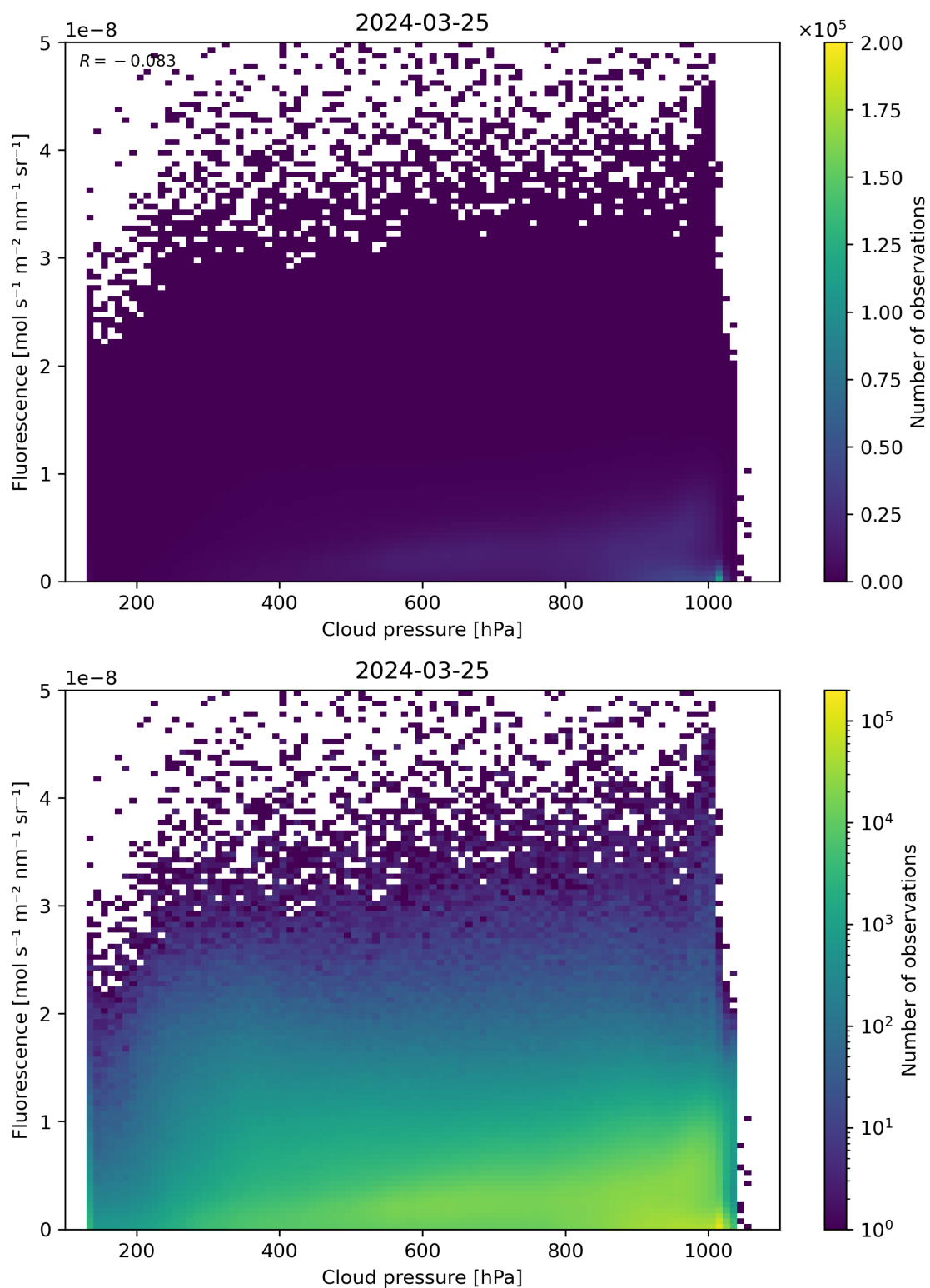
Figure 80: Scatter density plot of “Cloud pressure” against “Fluorescence” for 2024-03-25 to 2024-03-26.
