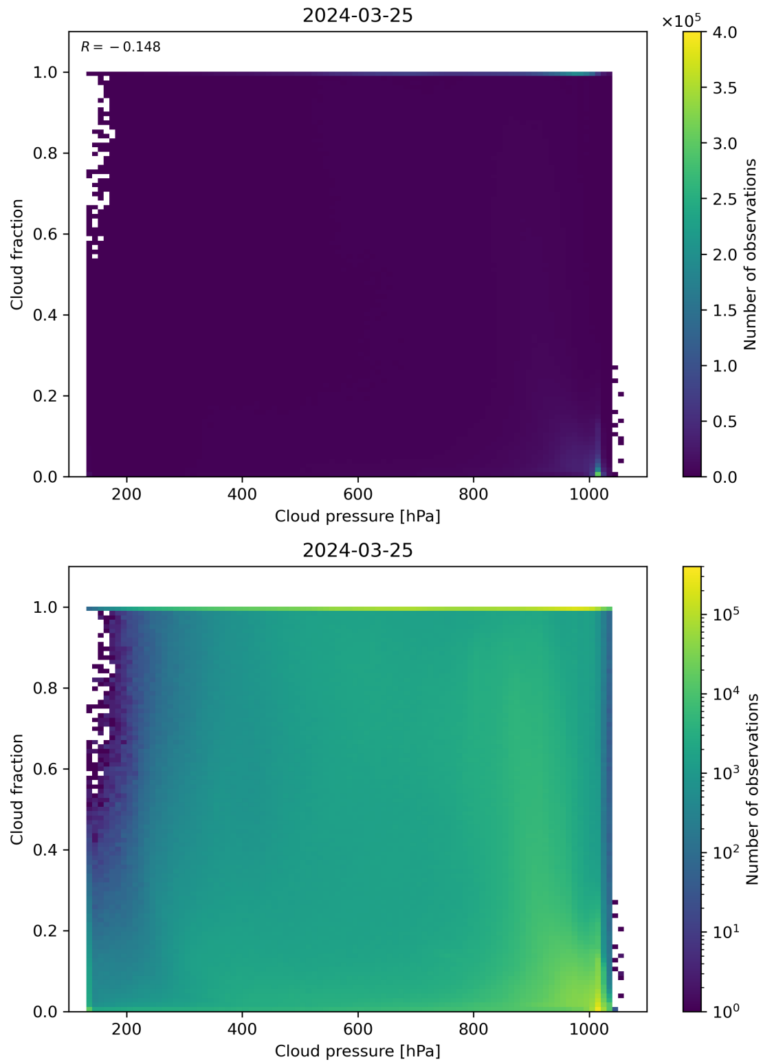
Figure 79: Scatter density plot of “Cloud pressure” against “Cloud fraction” for 2024-03-25 to 2024-03-26.
