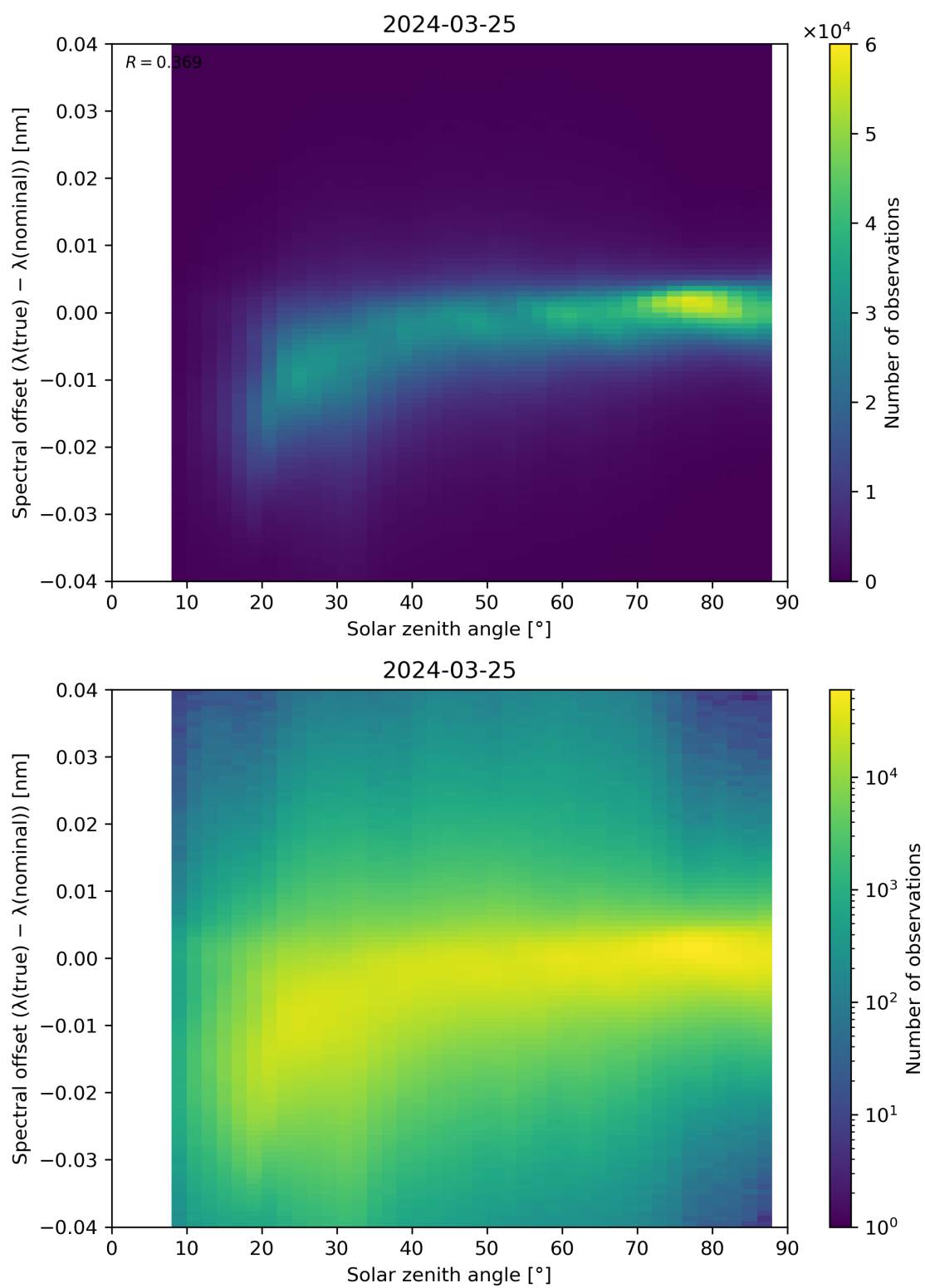
Figure 117: Scatter density plot of “Solar zenith angle” against “Spectral offset ( \lambda(\text{true}) - \lambda(\text{nominal}) )” for 2024-03-25 to 2024-03-26.
