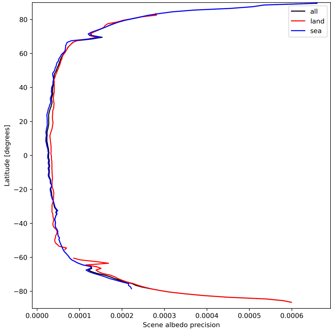
Figure 18: Zonal average of “Scene albedo precision” for 2024-03-25 to 2024-03-26.
