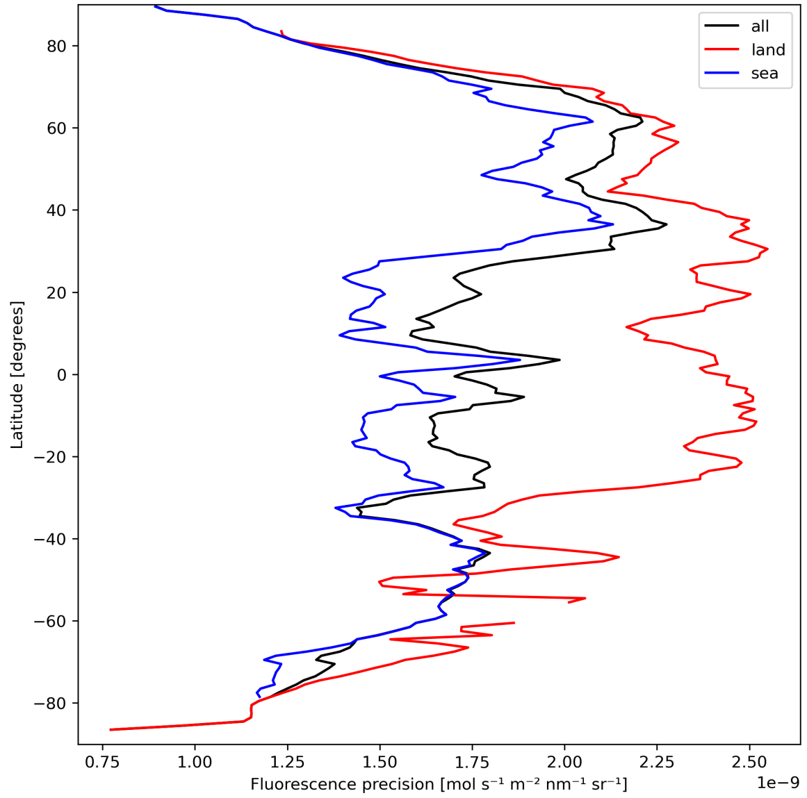
Figure 24: Zonal average of “Fluorescence precision” for 2024-03-25 to 2024-03-26.
