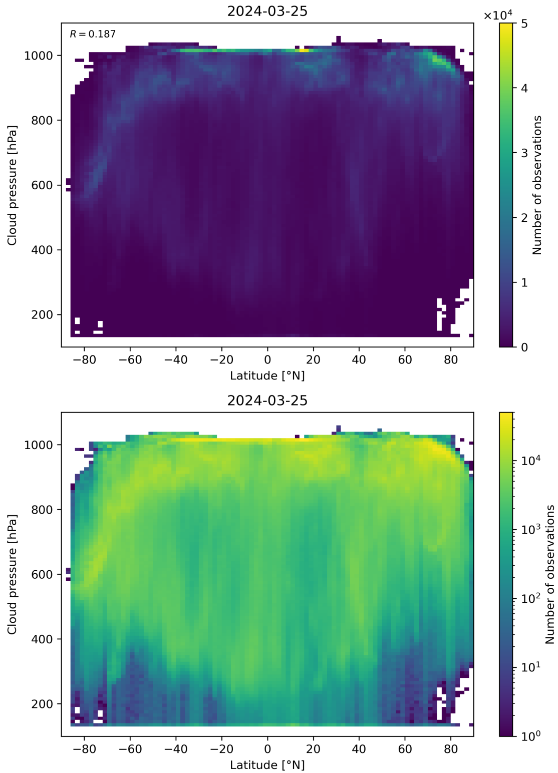
Figure 91: Scatter density plot of “Latitude” against “Cloud pressure” for 2024-03-25 to 2024-03-26.
