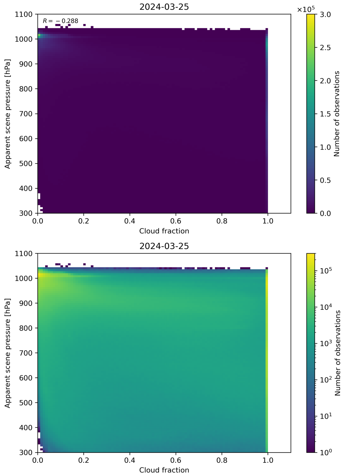
Figure 70: Scatter density plot of “Cloud fraction” against “Apparent scene pressure” for 2024-03-25 to 2024-03-26.
