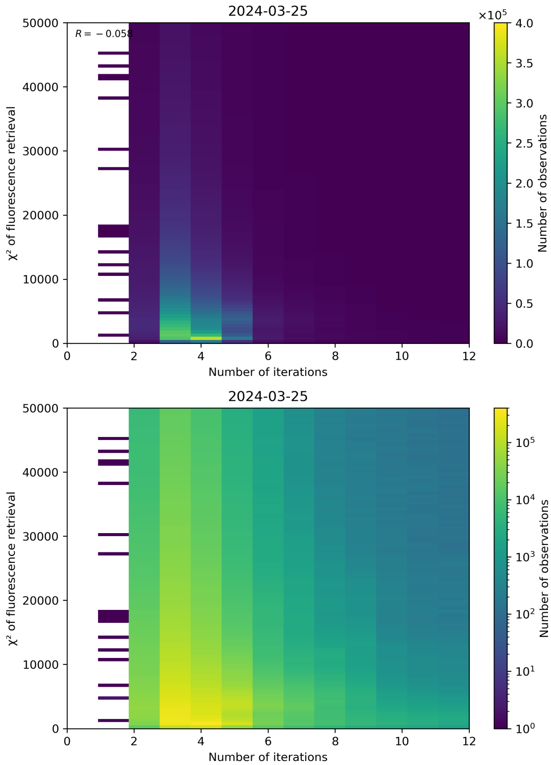
Figure 97: Scatter density plot of “Number of iterations” against “ \chi^2 of fluorescence retrieval” for 2024-03-25 to 2024-03-26.
