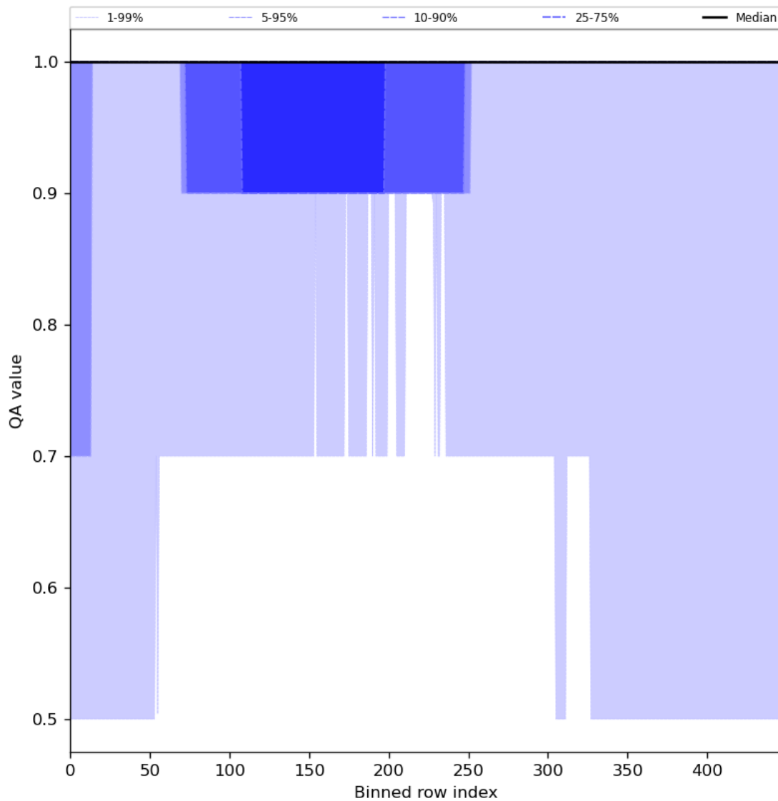
Figure 46: Along track statistics of “QA value” for 2024-03-25 to 2024-03-26
