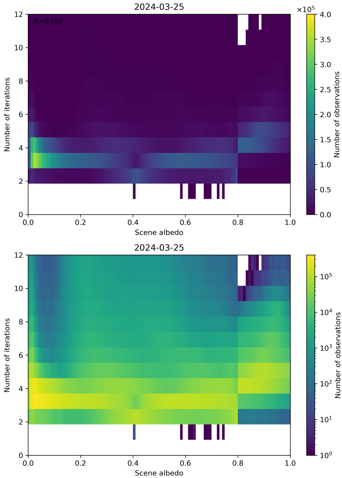
Figure 105: Scatter density plot of “Scene albedo” against “Number of iterations” for 2024-03-25 to 2024-03-26.
