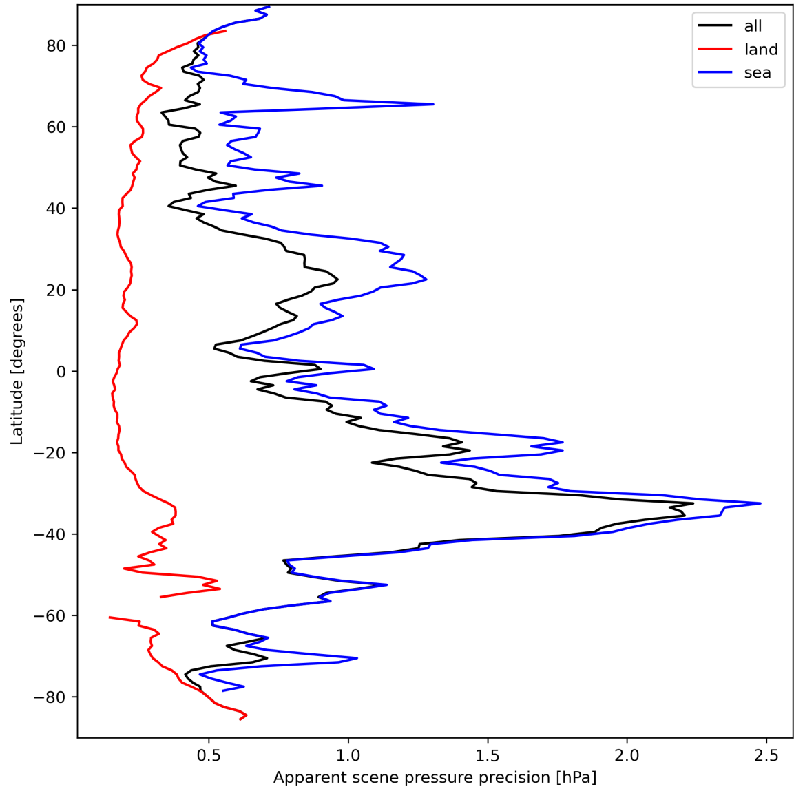
Figure 20: Zonal average of “Apparent scene pressure precision” for 2024-03-25 to 2024-03-27.
