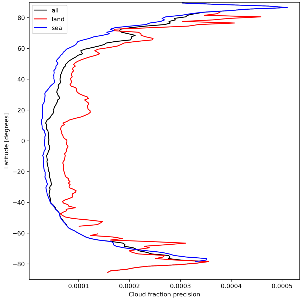
Figure 16: Zonal average of “Cloud fraction precision” for 2024-03-25 to 2024-03-27.
