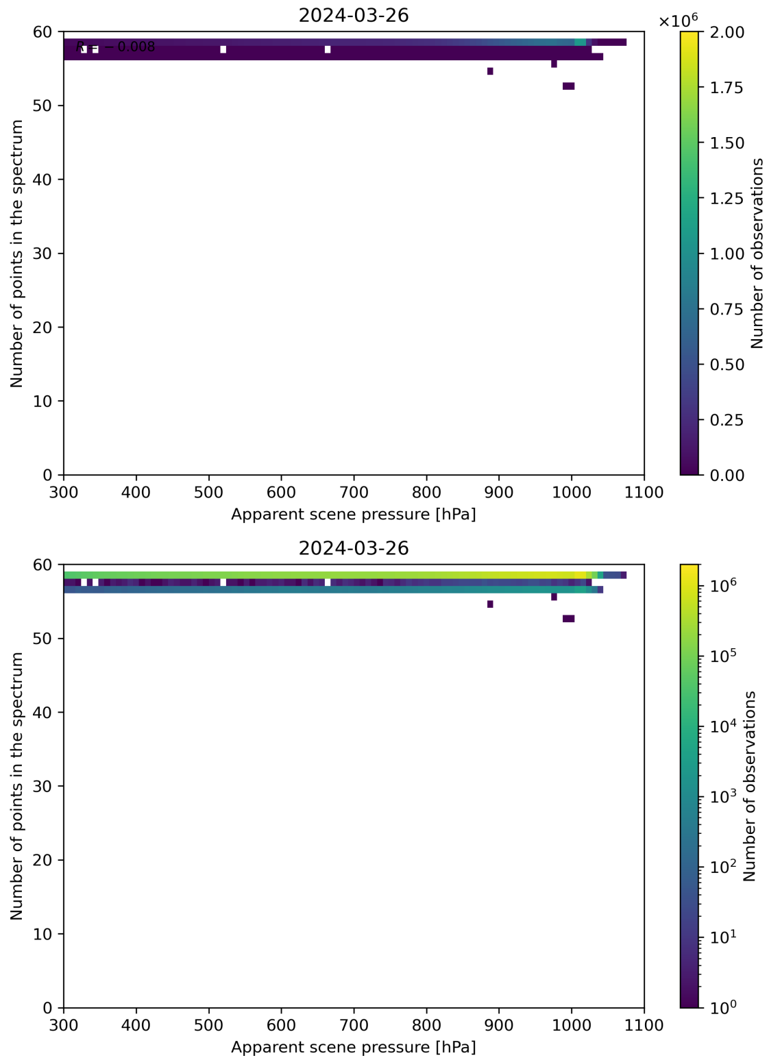
Figure 66: Scatter density plot of “Apparent scene pressure” against “Number of points in the spectrum” for 2024-03-25 to 2024-03-27.
