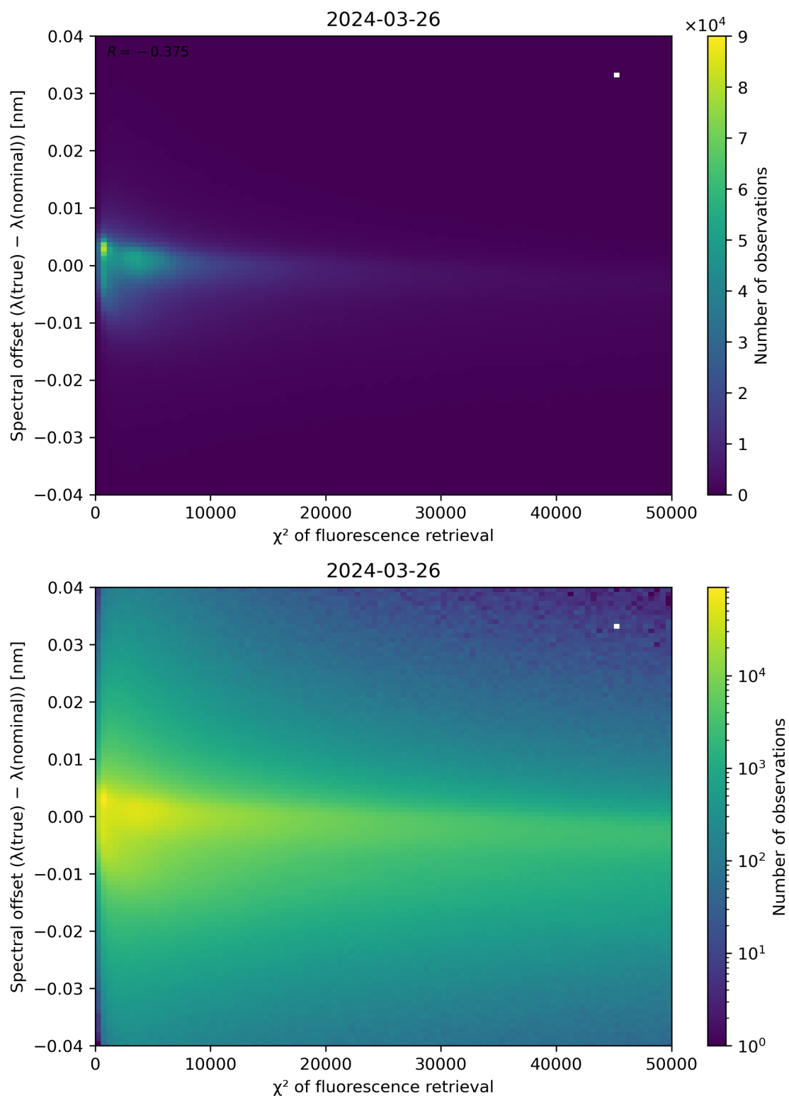
Figure 69: Scatter density plot of " \chi^2 of fluorescence retrieval" against "Spectral offset ( \lambda(\text{true}) - \lambda(\text{nominal}) )" for 2024-03-25 to 2024-03-27.
