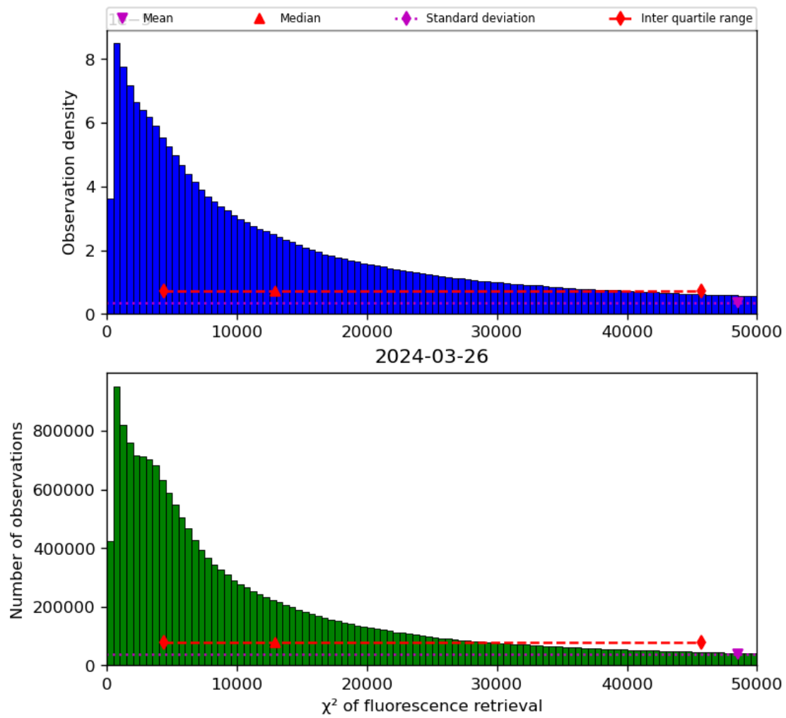
Figure 42: Histogram of “ \chi^2 of fluorescence retrieval” for 2024-03-25 to 2024-03-27
