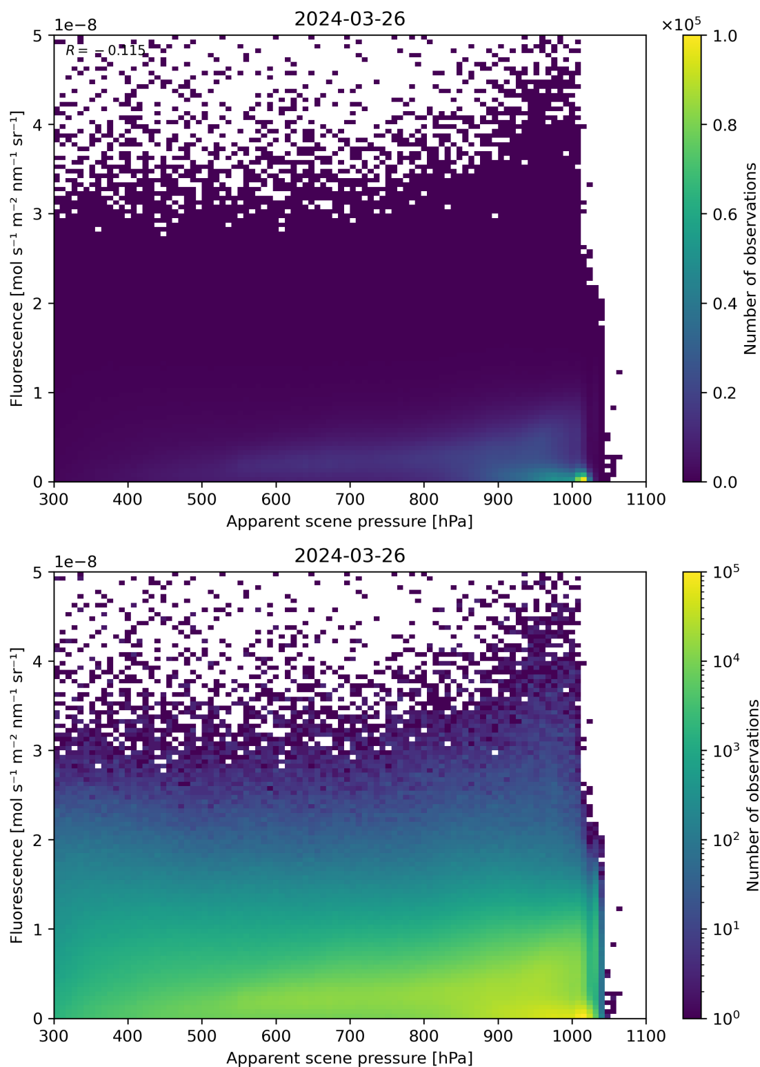
Figure 64: Scatter density plot of “Apparent scene pressure” against “Fluorescence” for 2024-03-25 to 2024-03-27.
