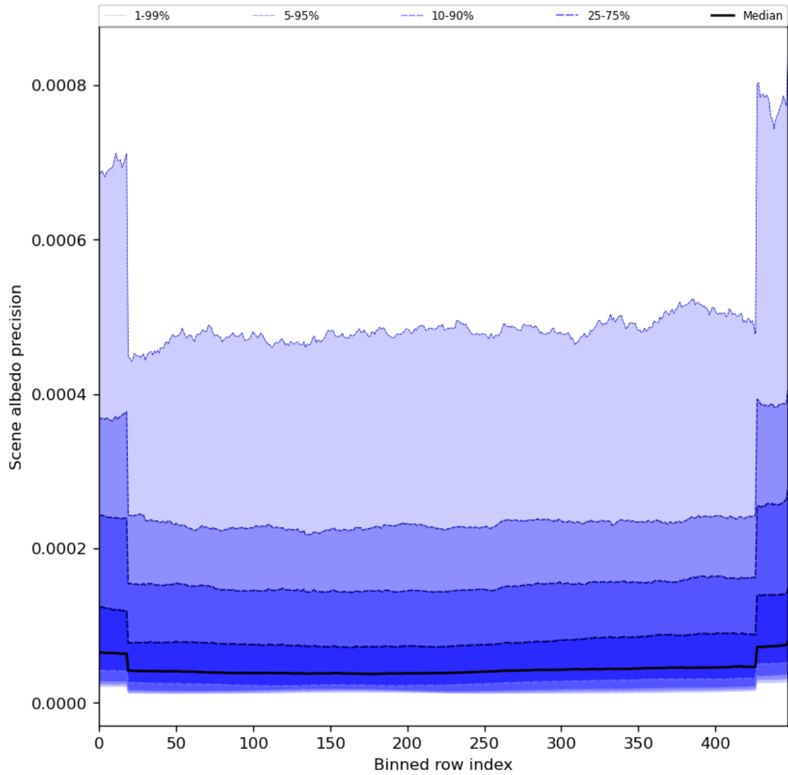
Figure 52: Along track statistics of “Scene albedo precision” for 2024-03-25 to 2024-03-27
