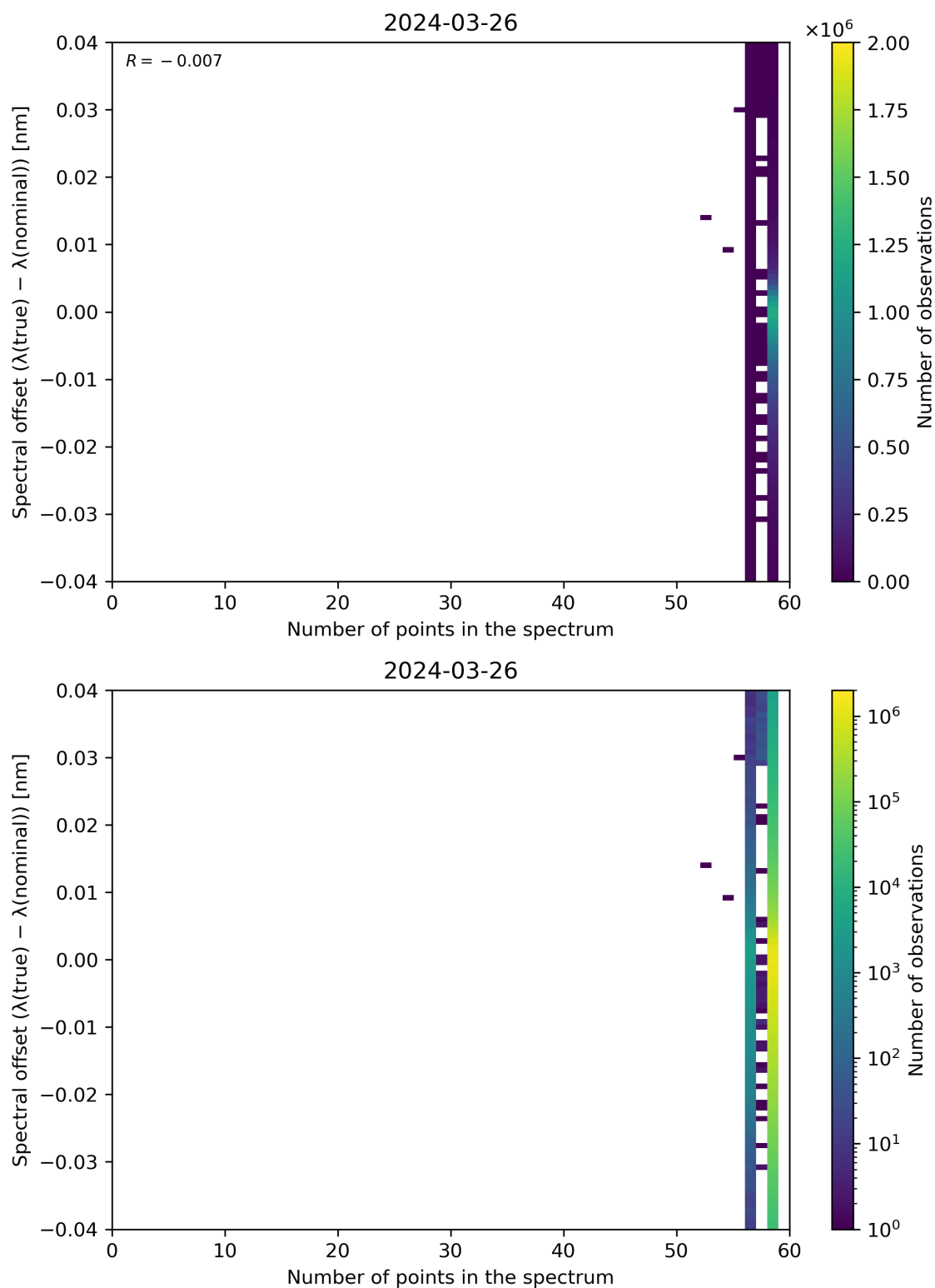
Figure 101: Scatter density plot of “Number of points in the spectrum” against “Spectral offset ( \lambda(\text{true}) - \lambda(\text{nominal}) )” for 2024-03-25 to 2024-03-27.
