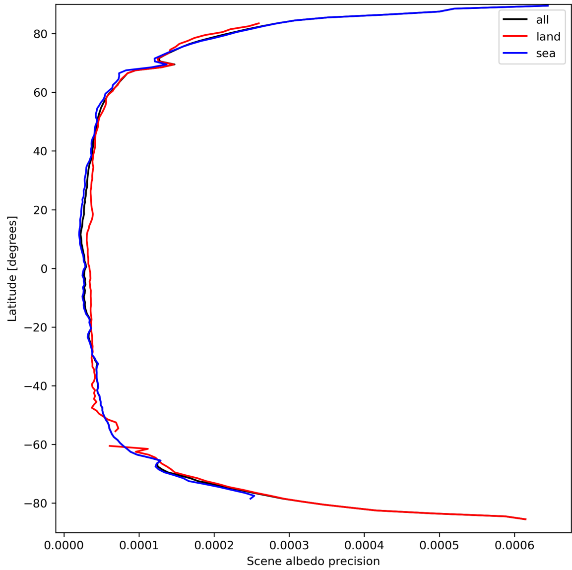
Figure 18: Zonal average of “Scene albedo precision” for 2024-03-25 to 2024-03-27.
