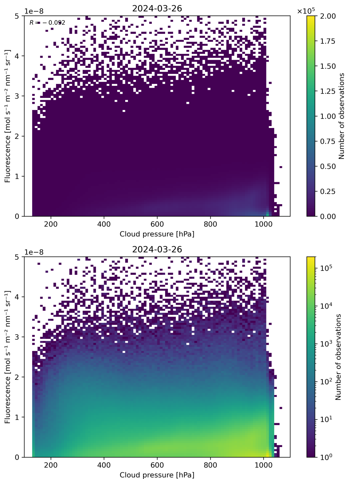
Figure 80: Scatter density plot of “Cloud pressure” against “Fluorescence” for 2024-03-25 to 2024-03-27.
