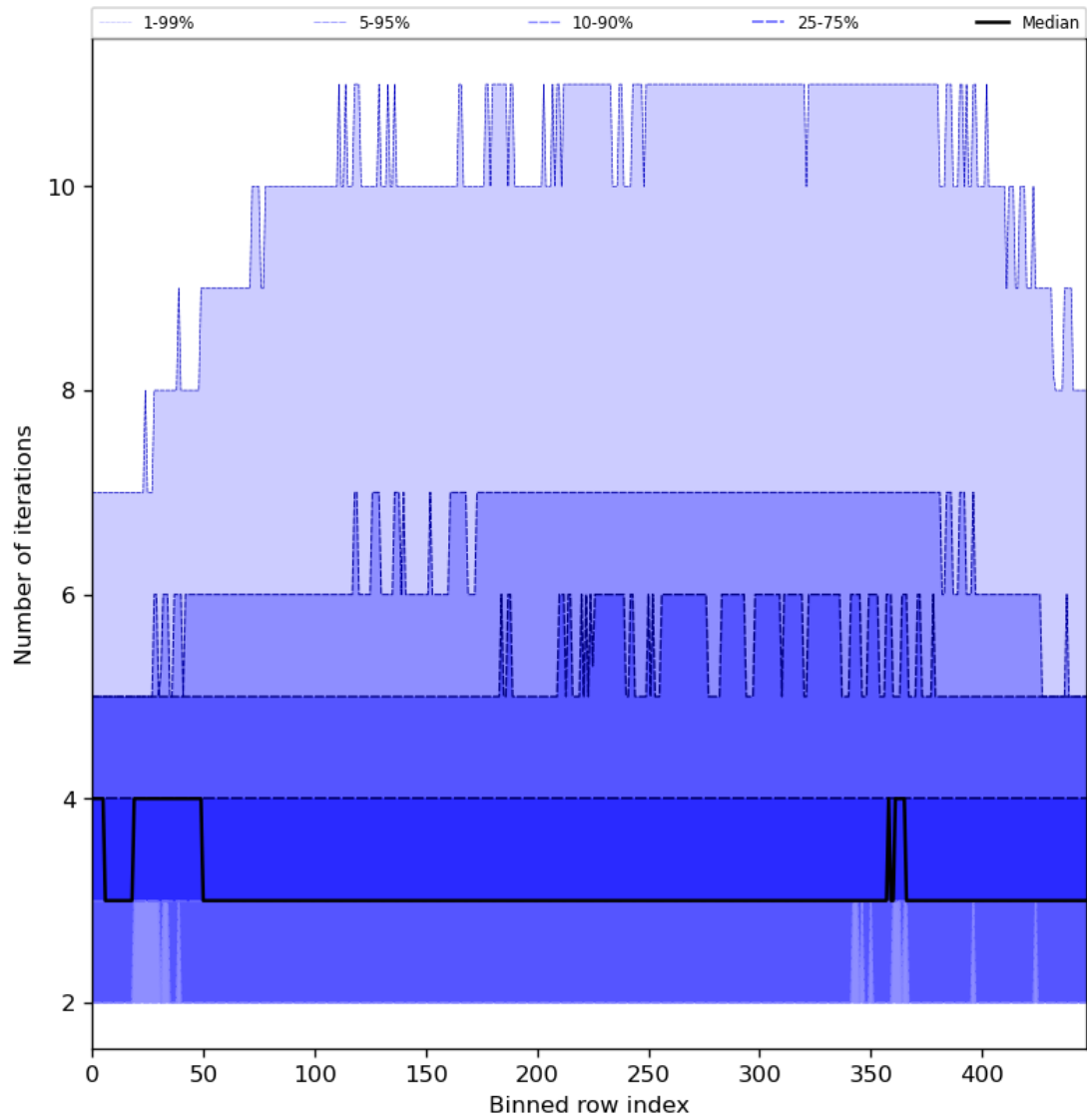
Figure 56: Along track statistics of “Number of iterations” for 2024-03-25 to 2024-03-27
