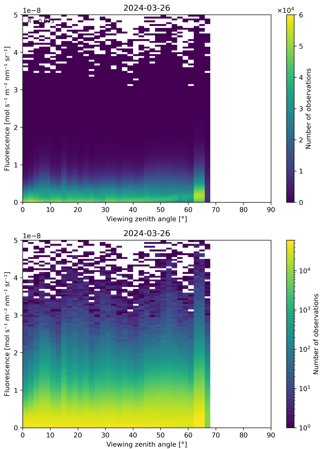
Figure 122: Scatter density plot of “Viewing zenith angle” against “Fluorescence” for 2024-03-25 to 2024-03-27.
