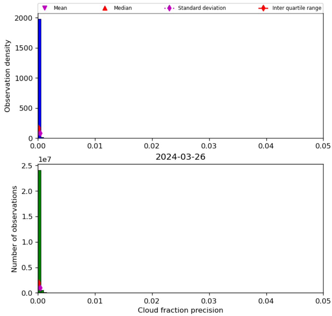
Figure 33: Histogram of “Cloud fraction precision” for 2024-03-25 to 2024-03-27
