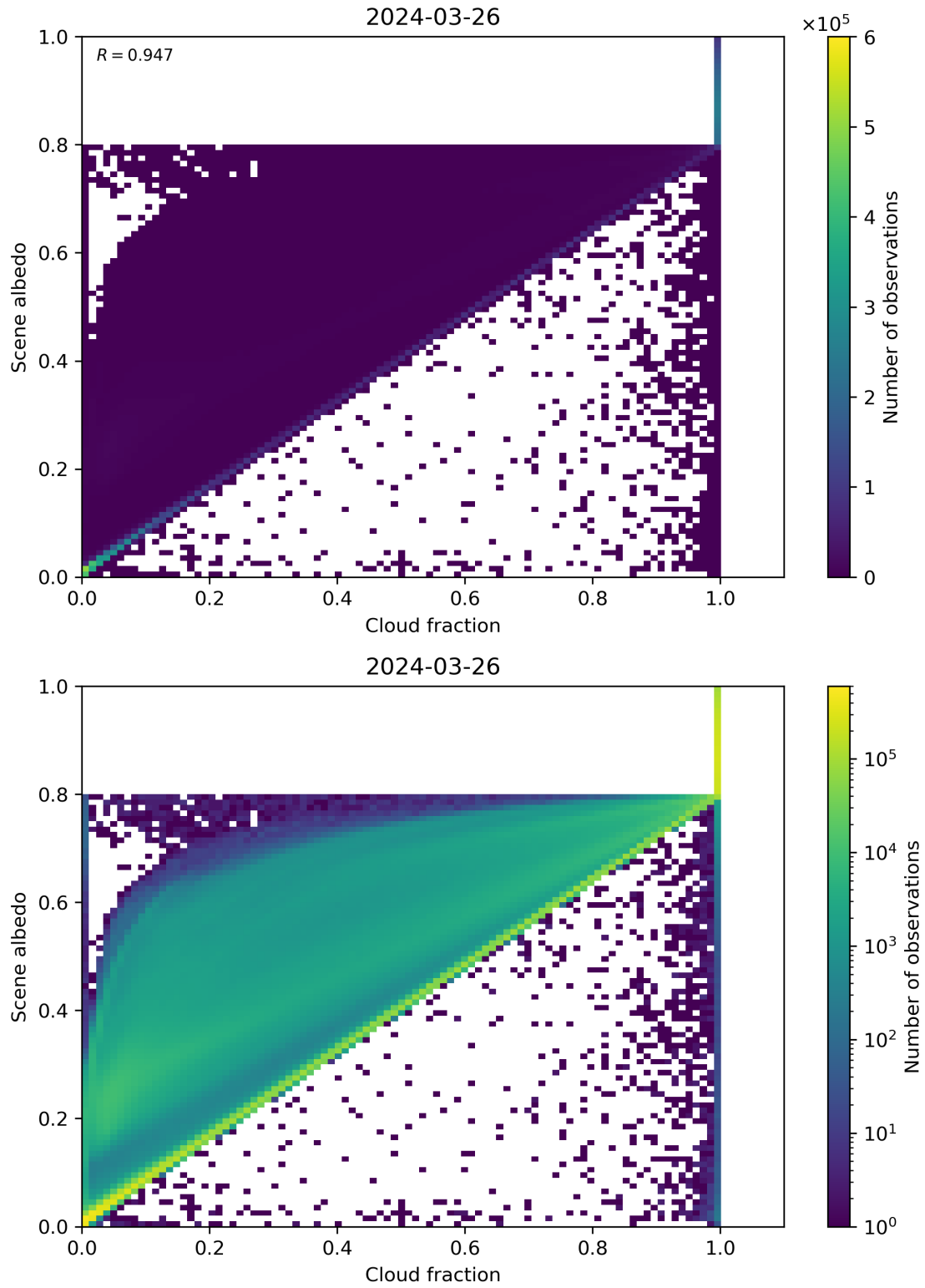
Figure 75: Scatter density plot of “Cloud fraction” against “Scene albedo” for 2024-03-25 to 2024-03-27.
