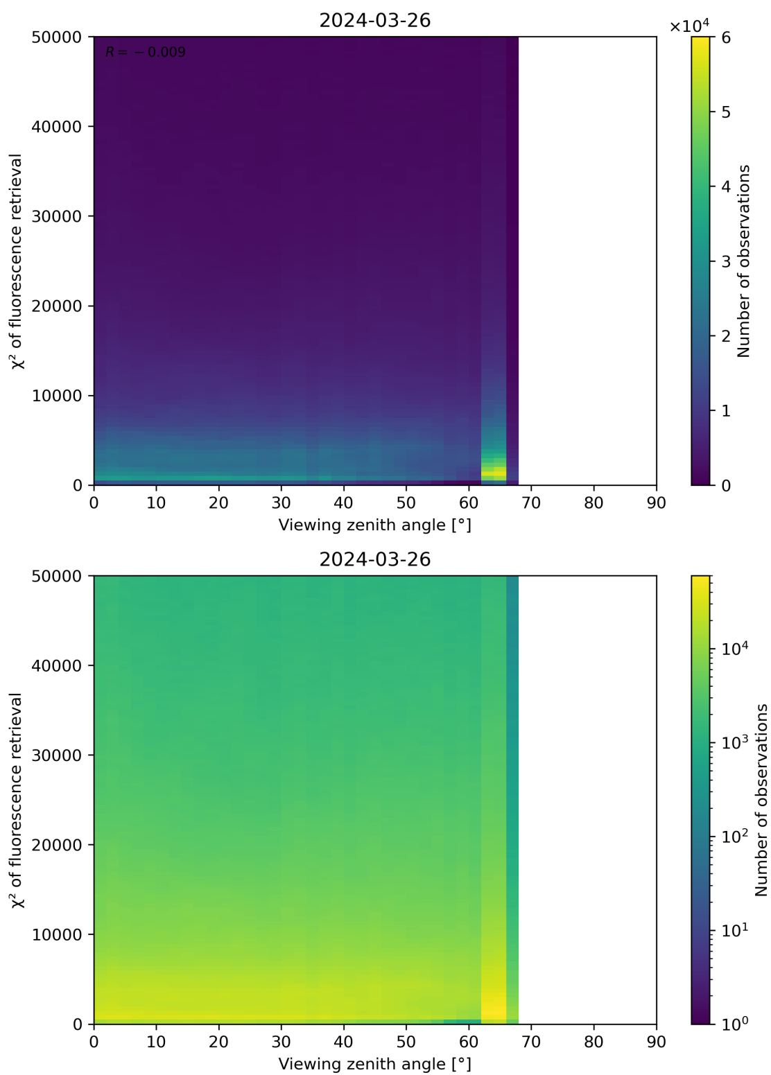
Figure 119: Scatter density plot of “Viewing zenith angle” against “ \chi^2 of fluorescence retrieval” for 2024-03-25 to 2024-03-27.
