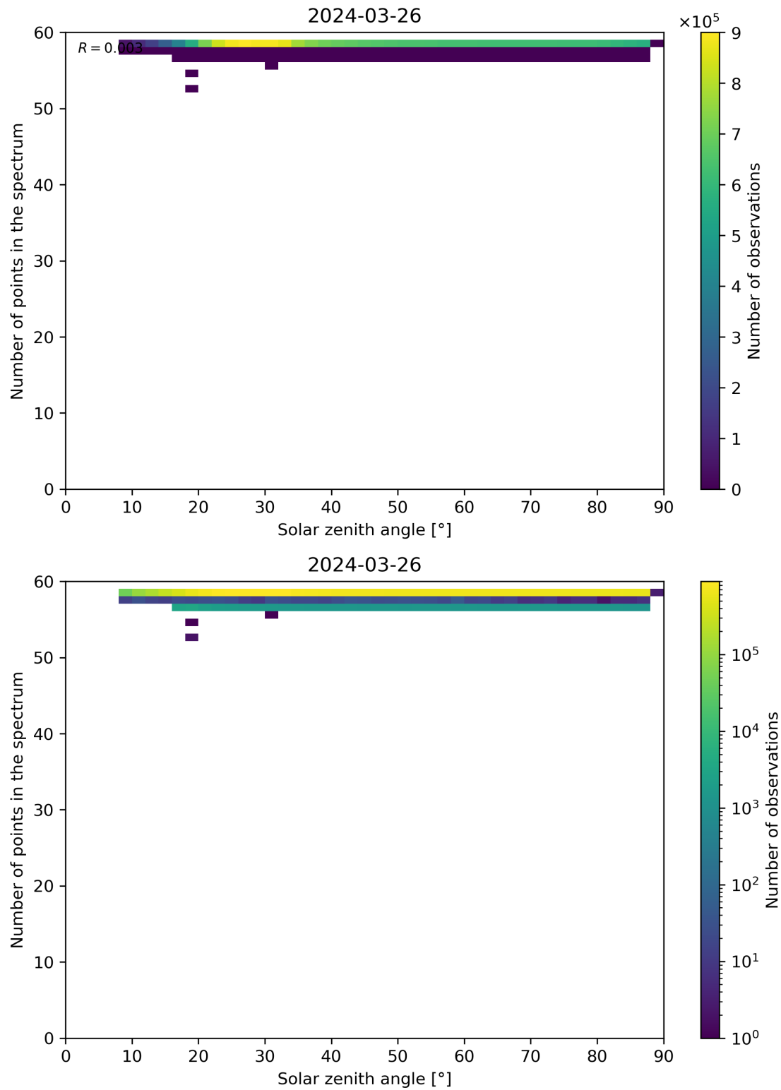
Figure 115: Scatter density plot of “Solar zenith angle” against “Number of points in the spectrum” for 2024-03-25 to 2024-03-27.
