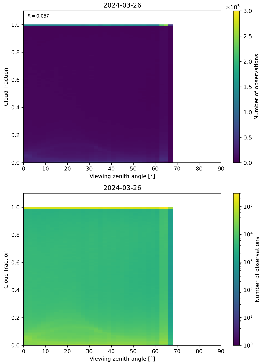
Figure 120: Scatter density plot of “Viewing zenith angle” against “Cloud fraction” for 2024-03-25 to 2024-03-27.
