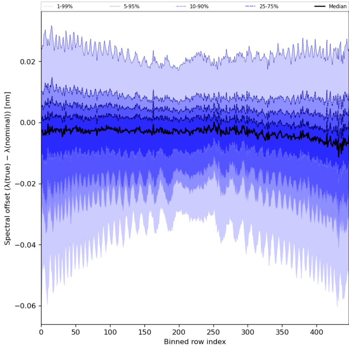
Figure 62: Along track statistics of “Spectral offset ( \lambda(\text{true}) - \lambda(\text{nominal}) )” for 2024-03-25 to 2024-03-27
