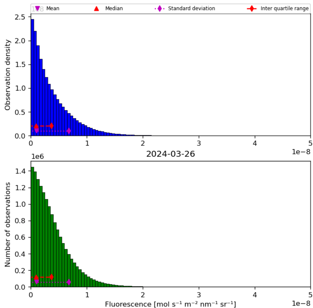
Figure 40: Histogram of “Fluorescence” for 2024-03-25 to 2024-03-27
