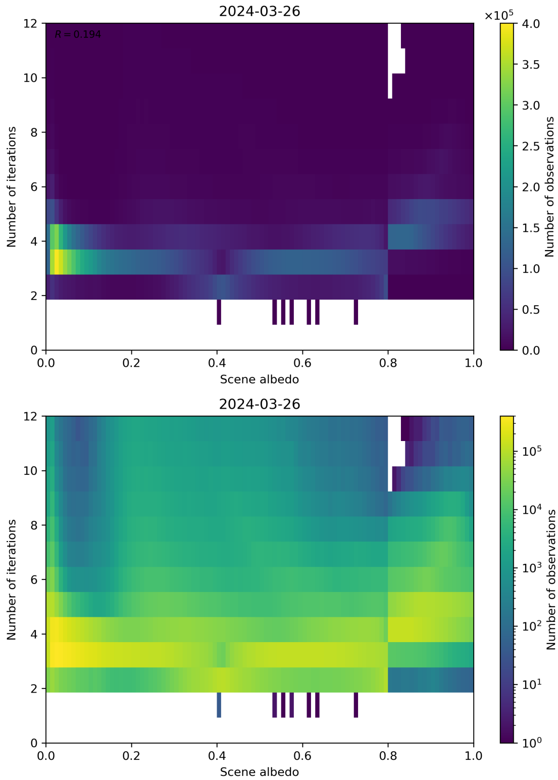
Figure 105: Scatter density plot of “Scene albedo” against “Number of iterations” for 2024-03-25 to 2024-03-27.
