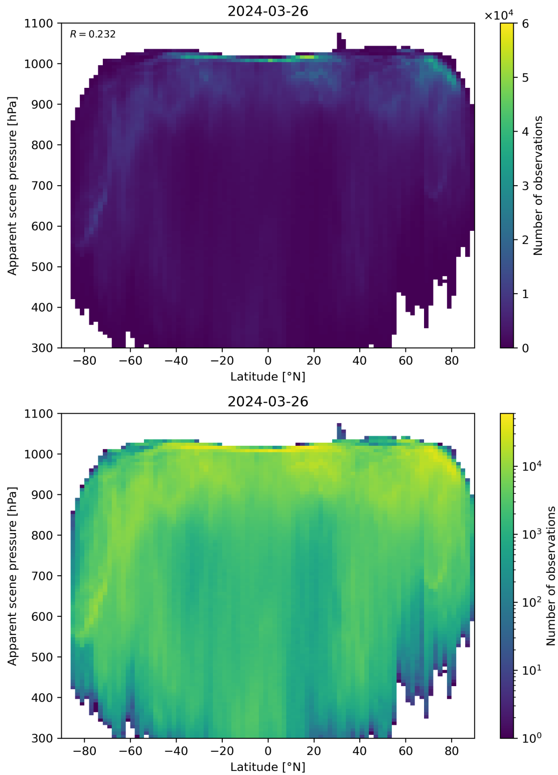
Figure 88: Scatter density plot of “Latitude” against “Apparent scene pressure” for 2024-03-25 to 2024-03-27.
