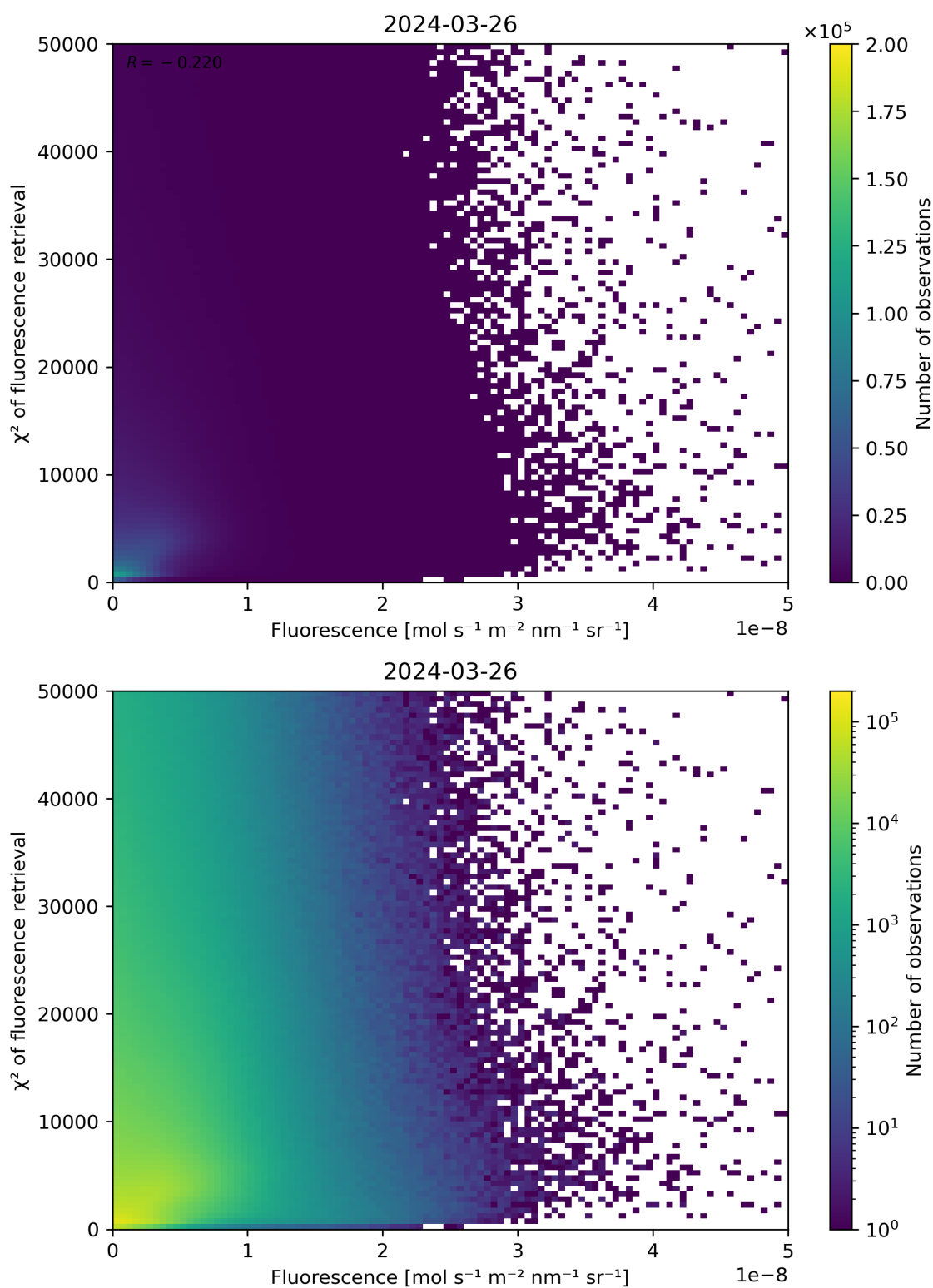
Figure 85: Scatter density plot of “Fluorescence” against “ \chi^2 of fluorescence retrieval” for 2024-03-25 to 2024-03-27.
