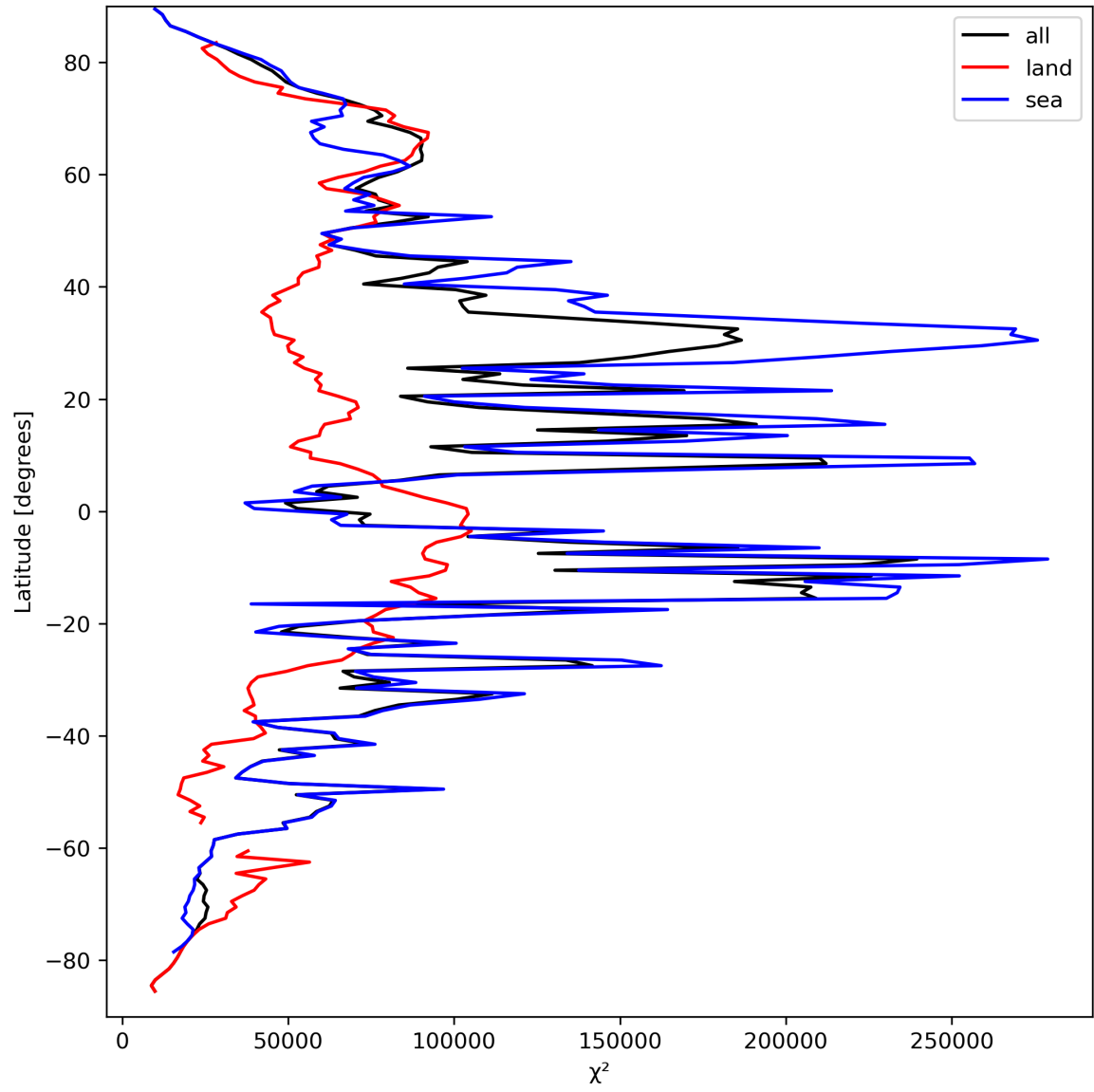
Figure 21: Zonal average of “ \chi^2 ” for 2024-03-25 to 2024-03-27.
