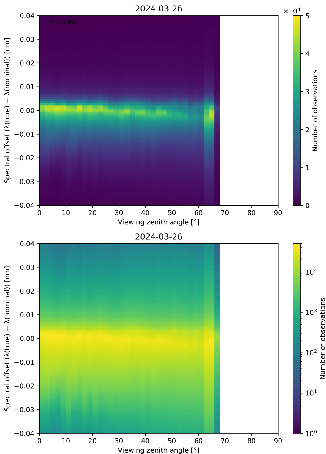
Figure 128: Scatter density plot of “Viewing zenith angle” against “Spectral offset ( \lambda(\text{true}) - \lambda(\text{nominal}) )” for 2024-03-25 to 2024-03-27.
