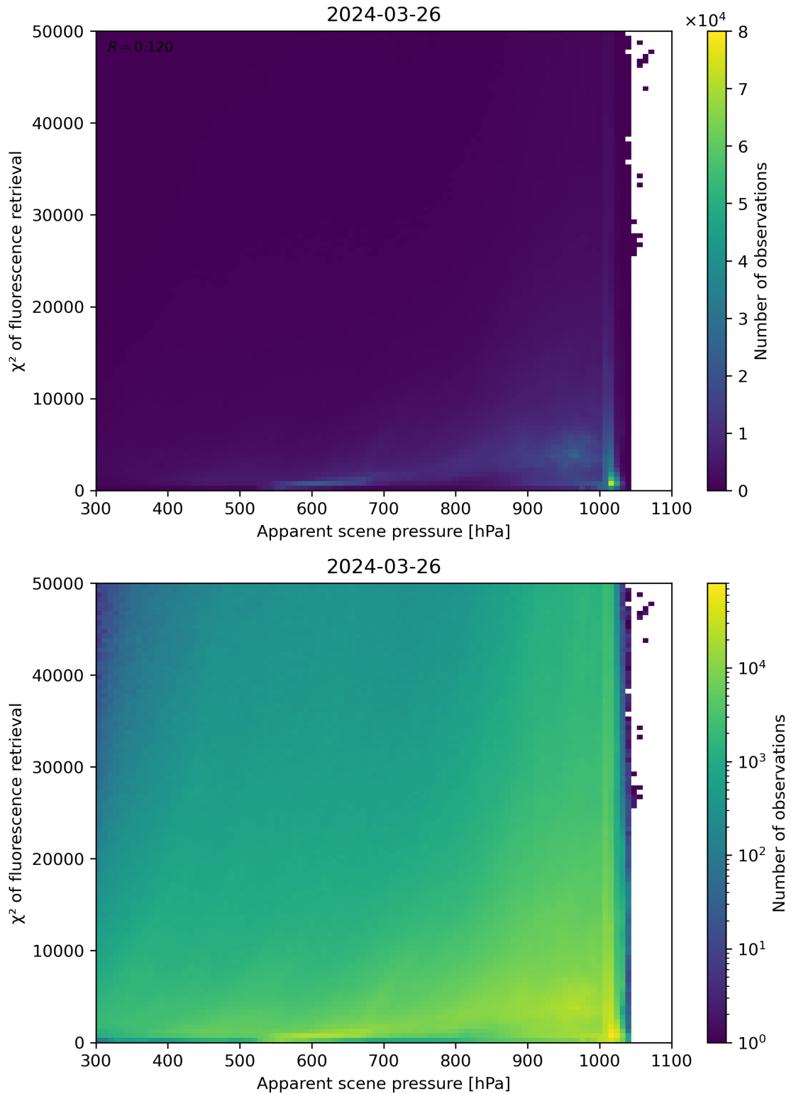
Figure 63: Scatter density plot of “Apparent scene pressure” against “ \chi^2 of fluorescence retrieval” for 2024-03-25 to 2024-03-27.
