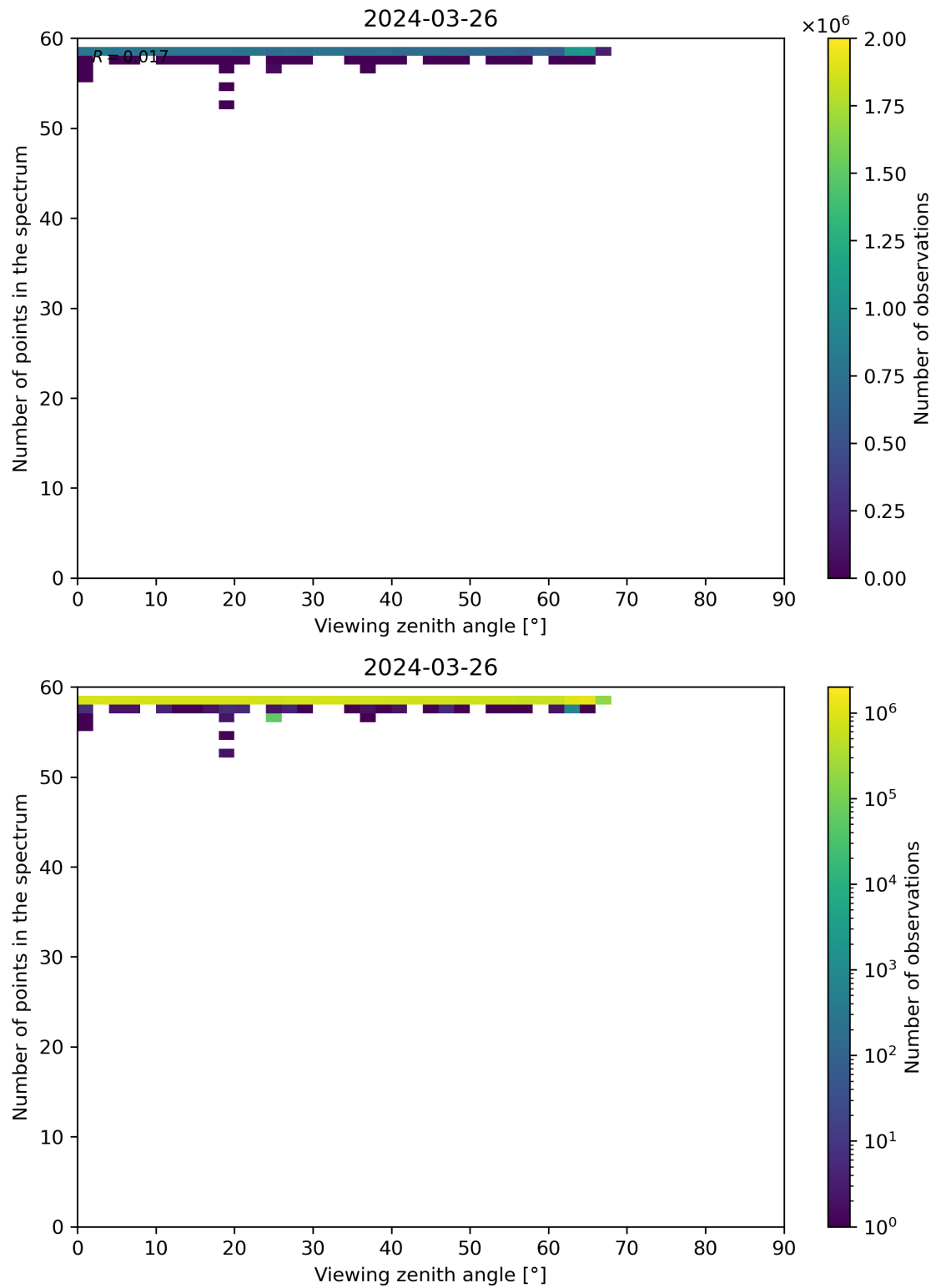
Figure 125: Scatter density plot of “Viewing zenith angle” against “Number of points in the spectrum” for 2024-03-25 to 2024-03-27.
