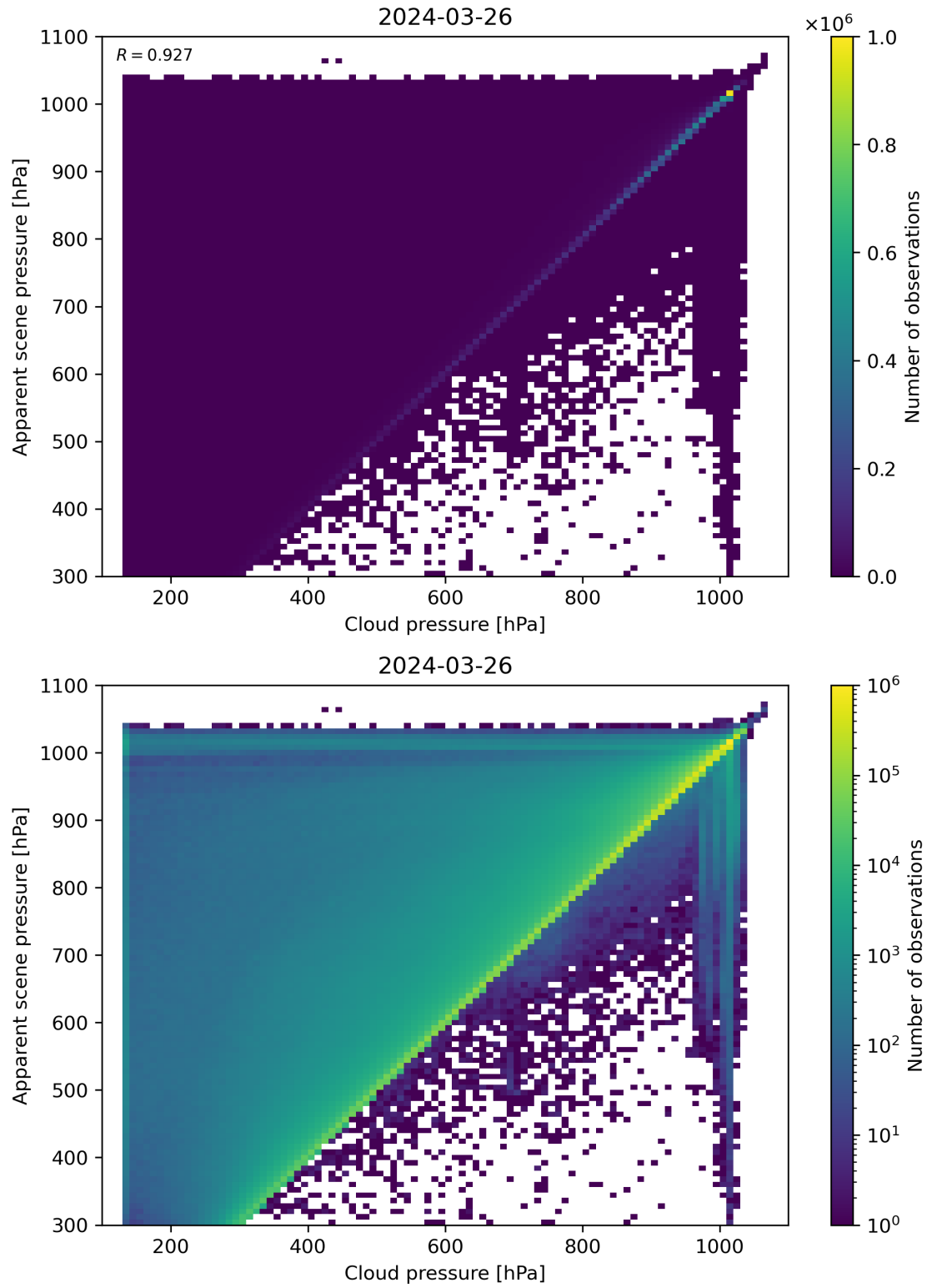
Figure 77: Scatter density plot of “Cloud pressure” against “Apparent scene pressure” for 2024-03-25 to 2024-03-27.
