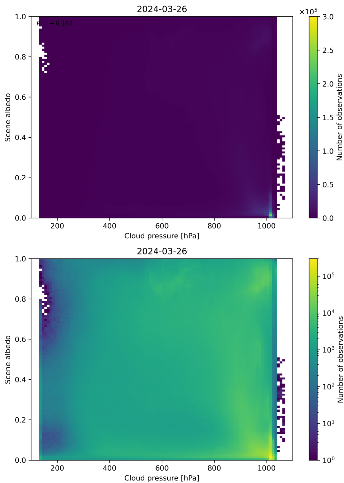
Figure 83: Scatter density plot of “Cloud pressure” against “Scene albedo” for 2024-03-25 to 2024-03-27.
