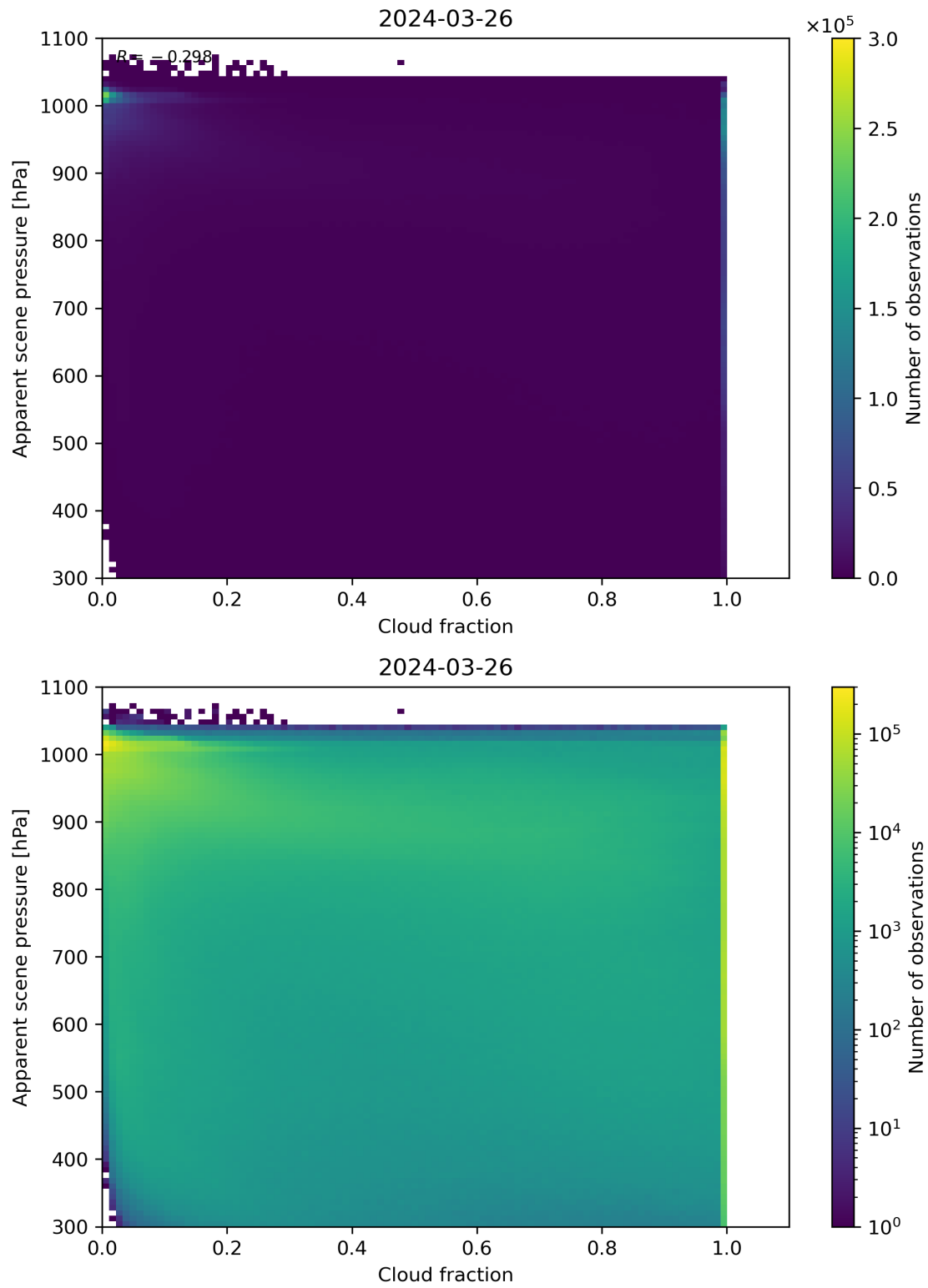
Figure 70: Scatter density plot of “Cloud fraction” against “Apparent scene pressure” for 2024-03-25 to 2024-03-27.
