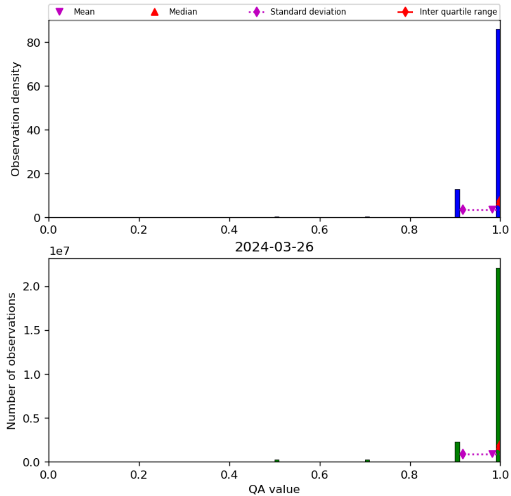
Figure 29: Histogram of “QA value” for 2024-03-25 to 2024-03-27
