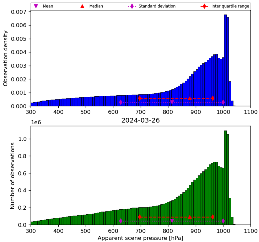
Figure 36: Histogram of “Apparent scene pressure” for 2024-03-25 to 2024-03-27
