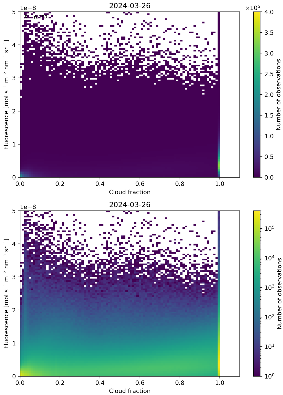
Figure 72: Scatter density plot of “Cloud fraction” against “Fluorescence” for 2024-03-25 to 2024-03-27.
