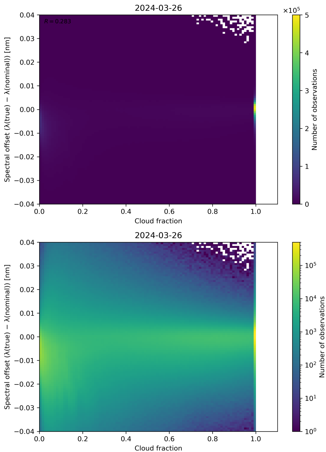
Figure 76: Scatter density plot of “Cloud fraction” against “Spectral offset ( \lambda(\text{true}) - \lambda(\text{nominal}) )” for 2024-03-25 to 2024-03-27.
