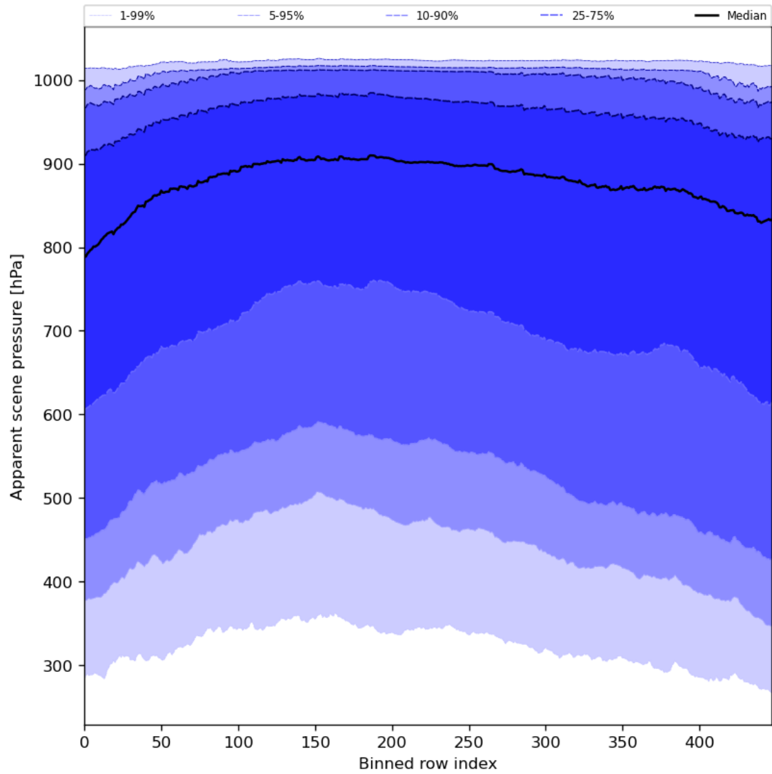
Figure 53: Along track statistics of “Apparent scene pressure” for 2024-03-25 to 2024-03-27
