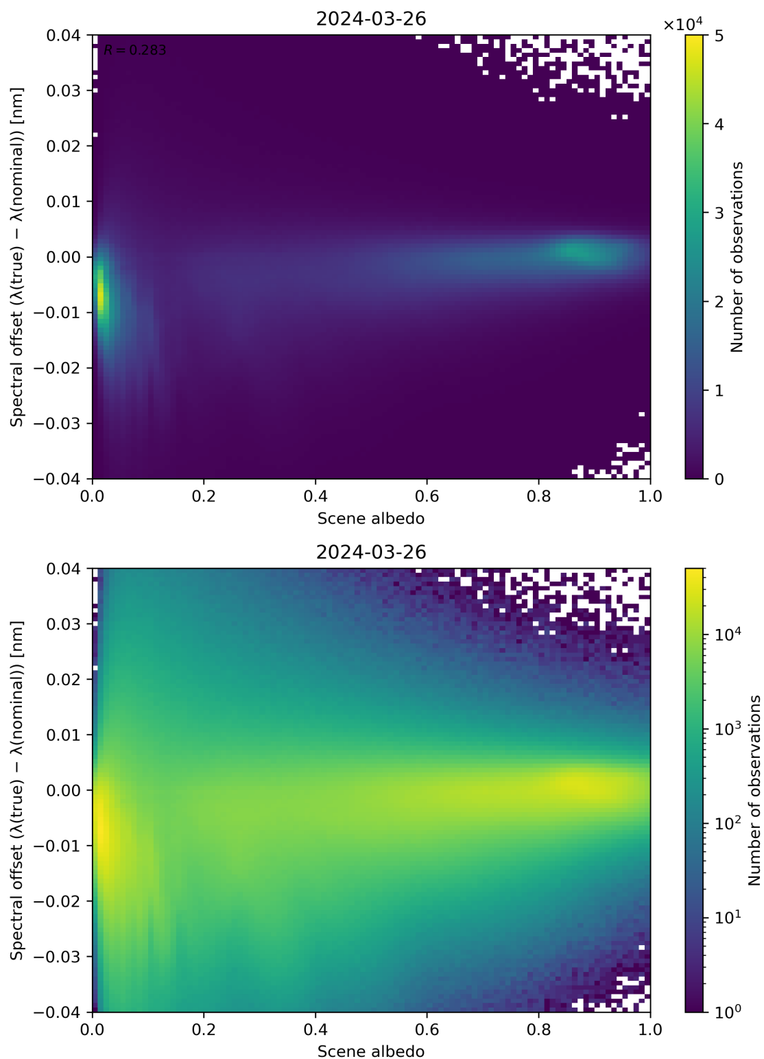
Figure 107: Scatter density plot of “Scene albedo” against “Spectral offset ( \lambda(\text{true}) - \lambda(\text{nominal}) )” for 2024-03-25 to 2024-03-27.
