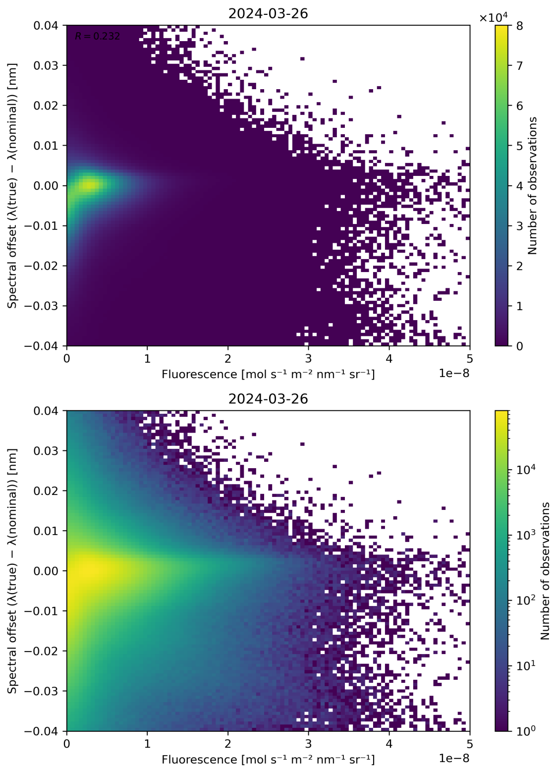
Figure 87: Scatter density plot of “Fluorescence” against “Spectral offset ( \lambda(\text{true}) - \lambda(\text{nominal}) )” for 2024-03-25 to 2024-03-27.
