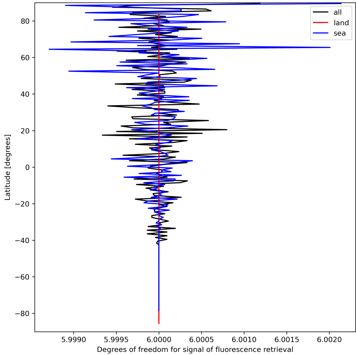
Figure 26: Zonal average of “Degrees of freedom for signal of fluorescence retrieval” for 2024-03-25 to 2024-03-27.
