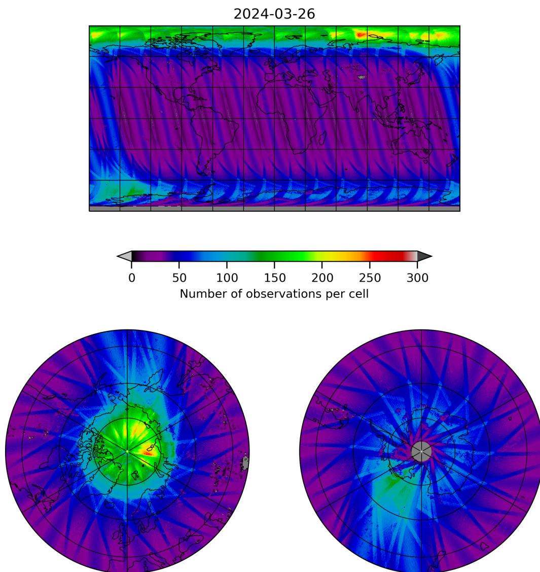
Figure 11: Map of the number of observations for 2024-03-25 to 2024-03-27
