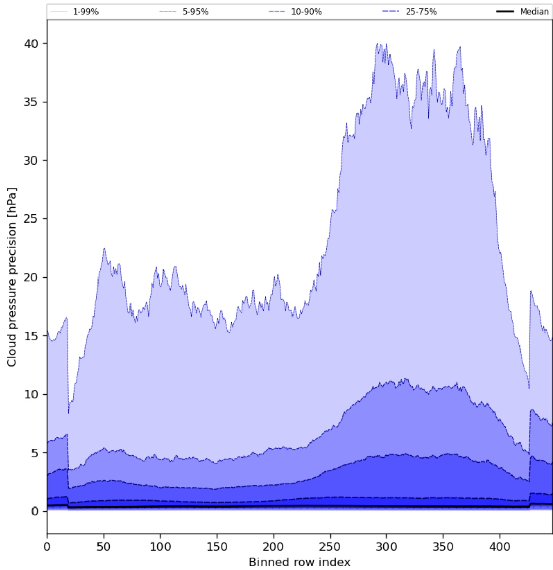
Figure 48: Along track statistics of “Cloud pressure precision” for 2024-03-25 to 2024-03-27
