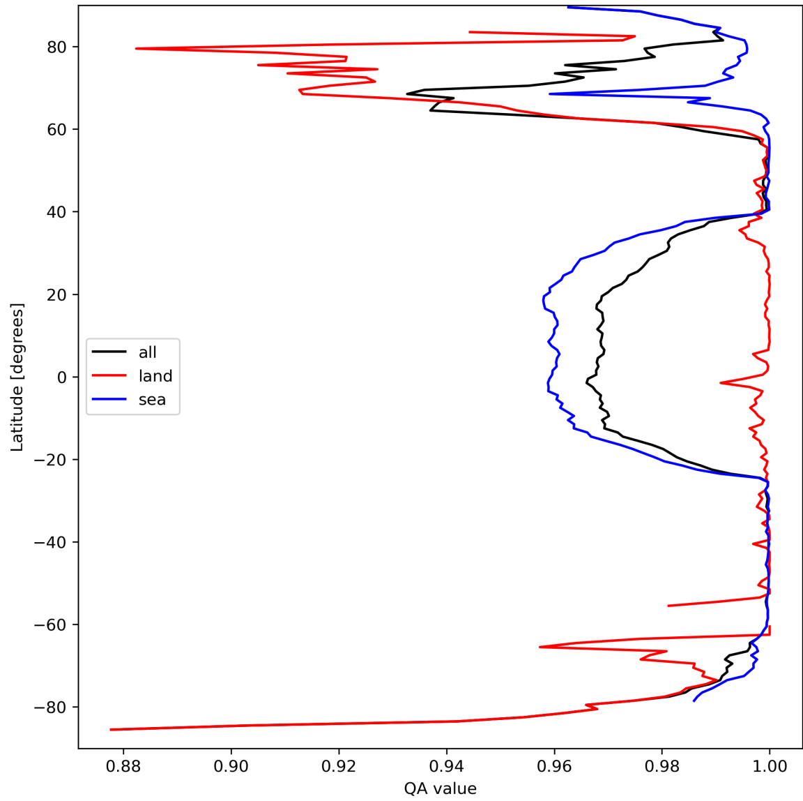
Figure 12: Zonal average of “QA value” for 2024-03-25 to 2024-03-27.
