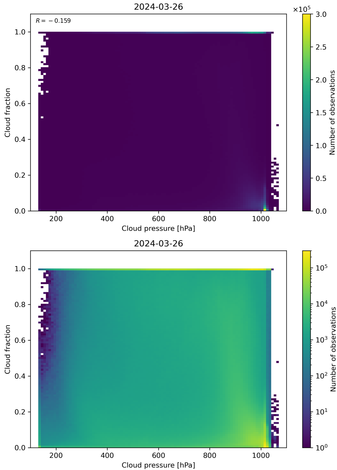
Figure 79: Scatter density plot of “Cloud pressure” against “Cloud fraction” for 2024-03-25 to 2024-03-27.
