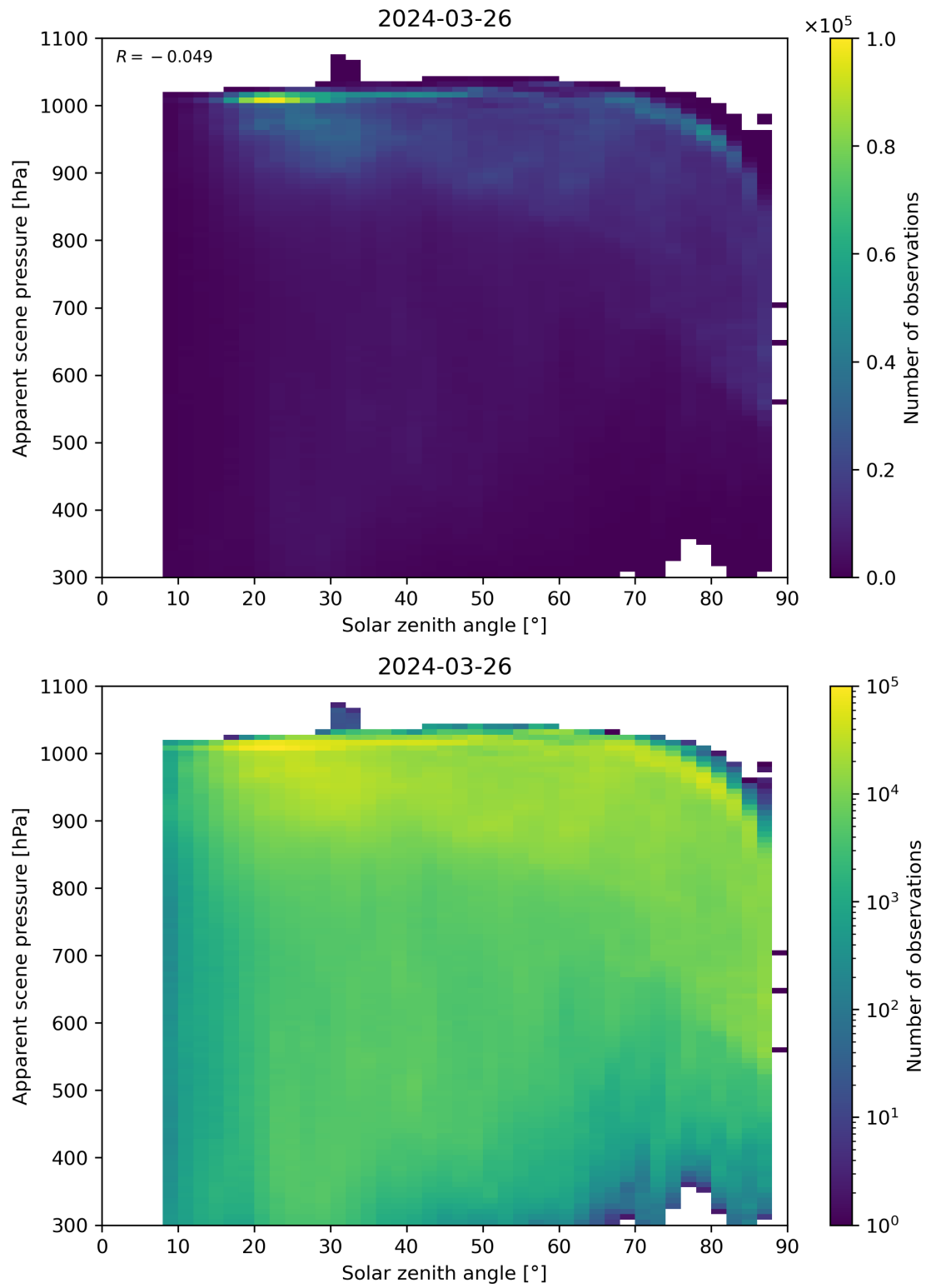
Figure 108: Scatter density plot of “Solar zenith angle” against “Apparent scene pressure” for 2024-03-25 to 2024-03-27.
