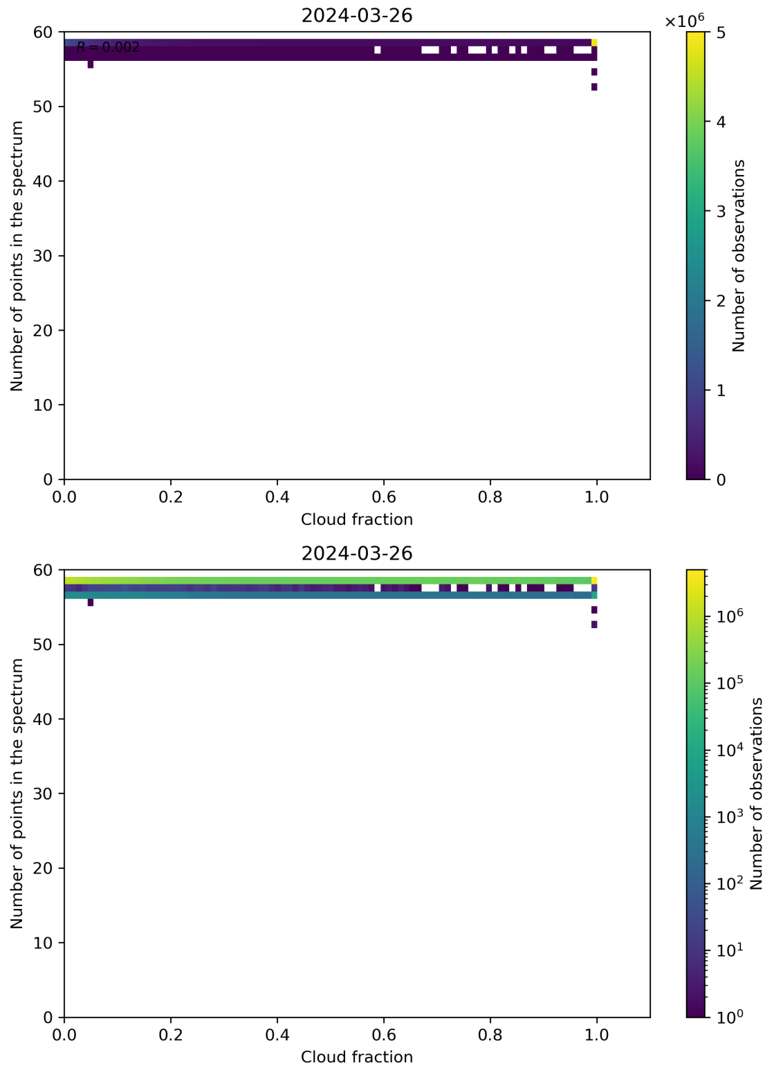
Figure 74: Scatter density plot of “Cloud fraction” against “Number of points in the spectrum” for 2024-03-25 to 2024-03-27.
