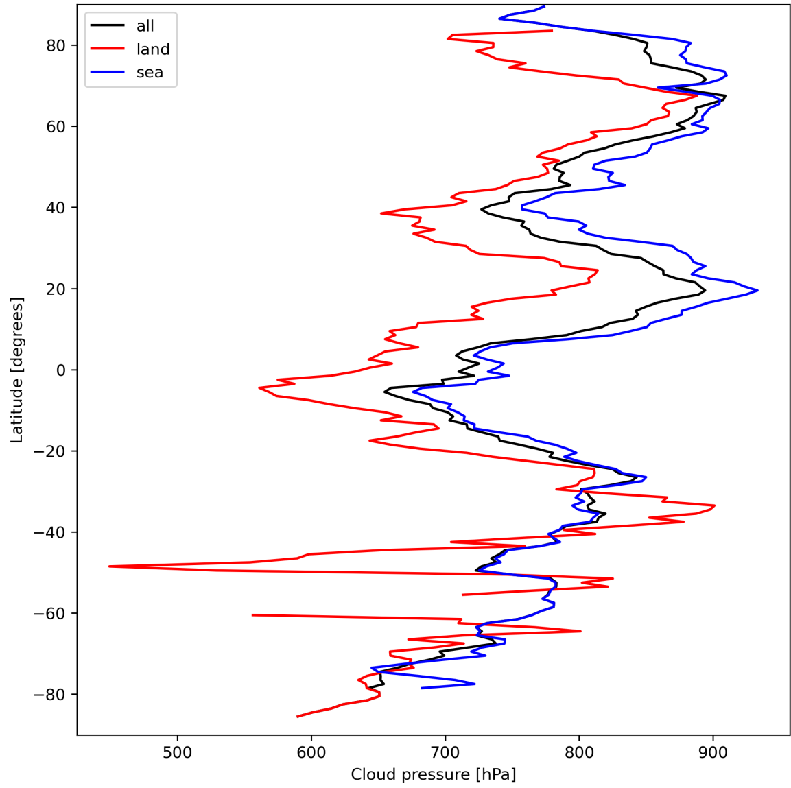
Figure 13: Zonal average of “Cloud pressure” for 2024-03-25 to 2024-03-27.
