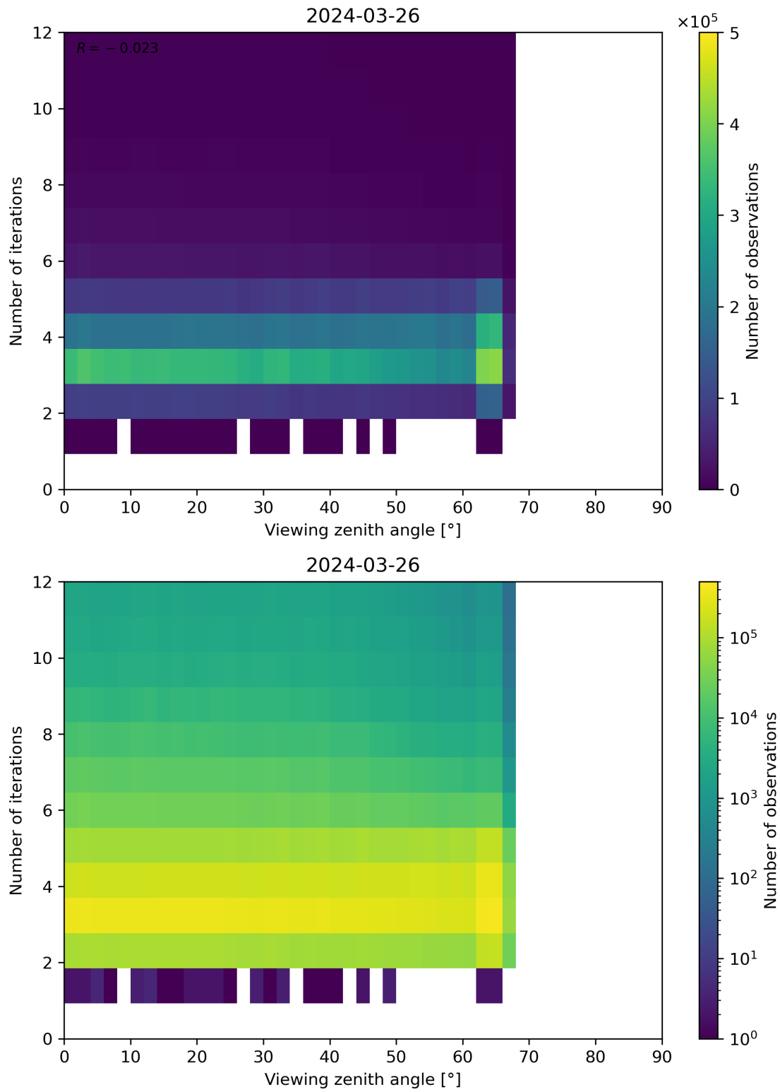
Figure 124: Scatter density plot of “Viewing zenith angle” against “Number of iterations” for 2024-03-25 to 2024-03-27.
