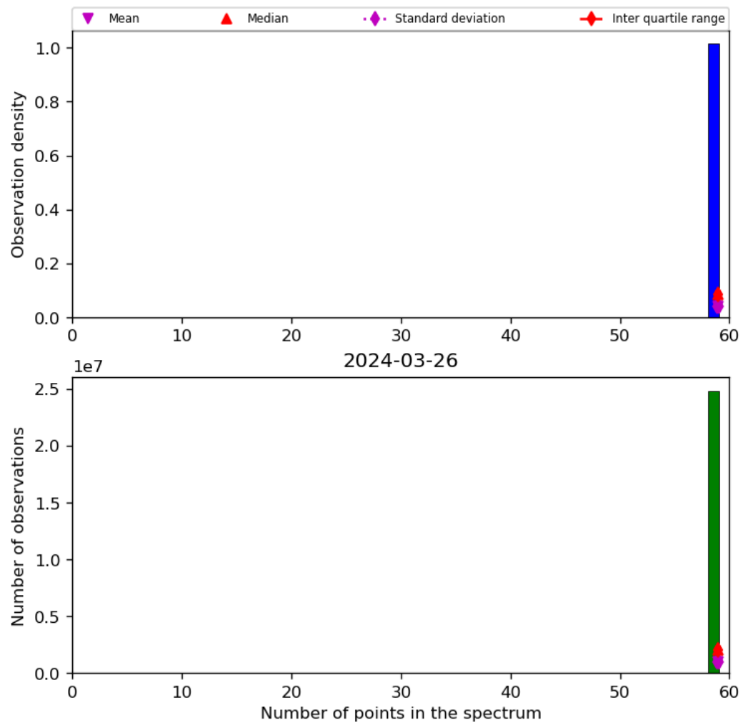
Figure 44: Histogram of “Number of points in the spectrum” for 2024-03-25 to 2024-03-27
