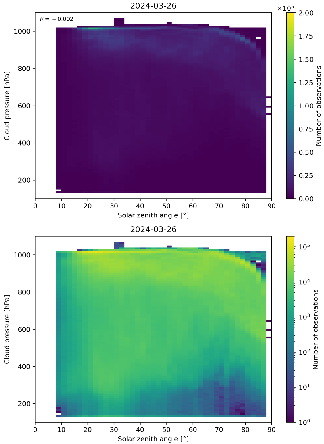
Figure 111: Scatter density plot of “Solar zenith angle” against “Cloud pressure” for 2024-03-25 to 2024-03-27.
