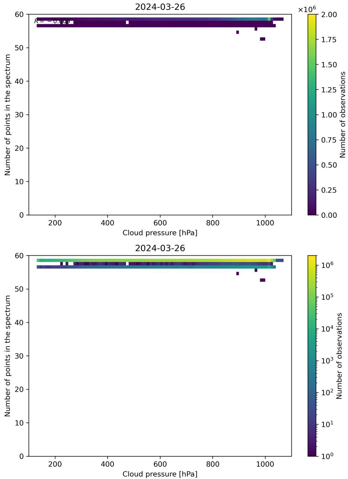
Figure 82: Scatter density plot of “Cloud pressure” against “Number of points in the spectrum” for 2024-03-25 to 2024-03-27.
