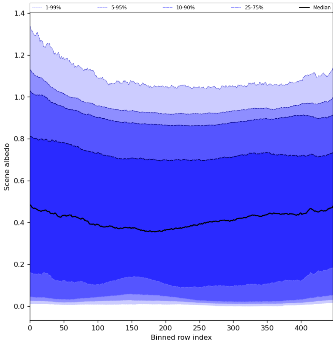
Figure 51: Along track statistics of “Scene albedo” for 2024-03-25 to 2024-03-27
