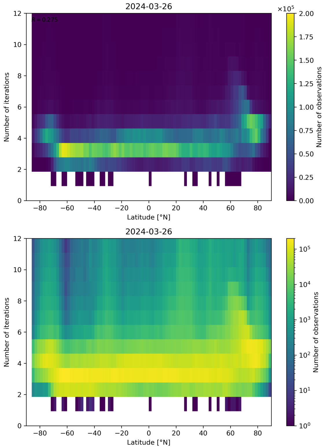
Figure 93: Scatter density plot of “Latitude” against “Number of iterations” for 2024-03-25 to 2024-03-27.
