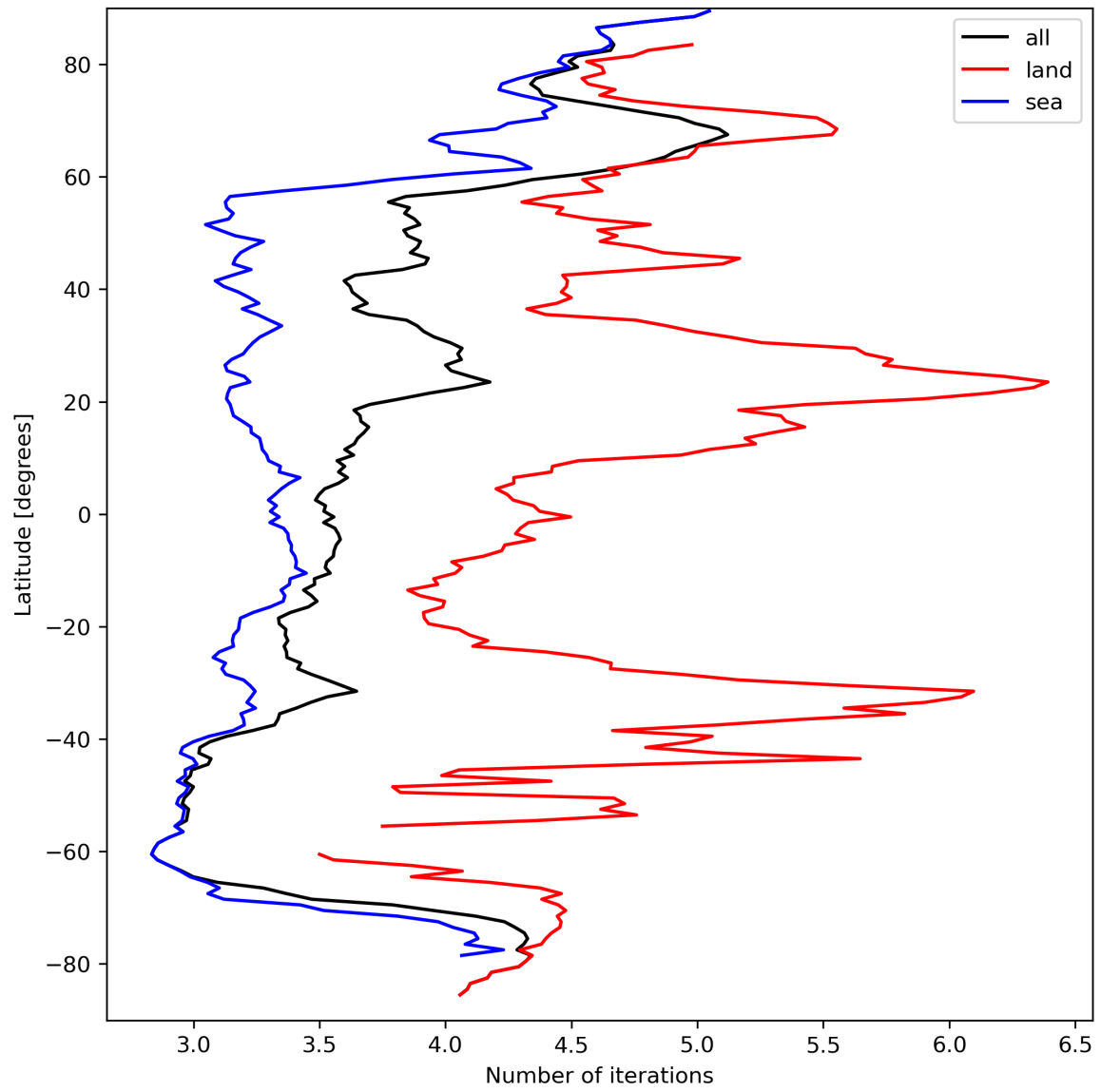
Figure 22: Zonal average of “Number of iterations” for 2024-03-25 to 2024-03-27.
