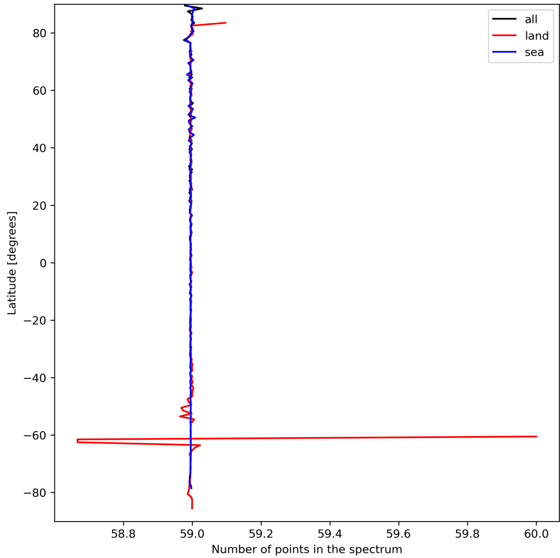
Figure 27: Zonal average of “Number of points in the spectrum” for 2024-03-25 to 2024-03-27.
