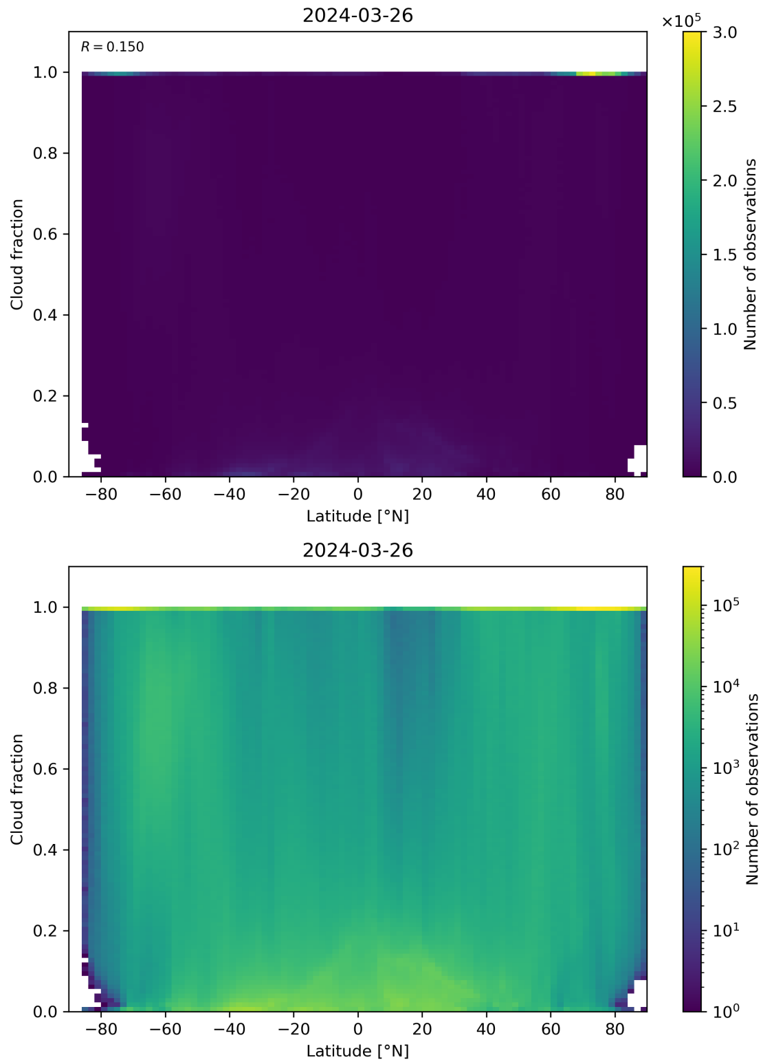
Figure 90: Scatter density plot of “Latitude” against “Cloud fraction” for 2024-03-25 to 2024-03-27.
