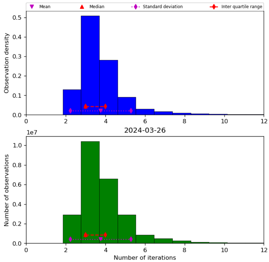
Figure 39: Histogram of “Number of iterations” for 2024-03-25 to 2024-03-27
