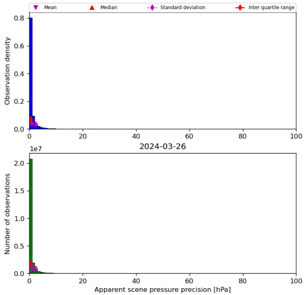
Figure 37: Histogram of “Apparent scene pressure precision” for 2024-03-25 to 2024-03-27
