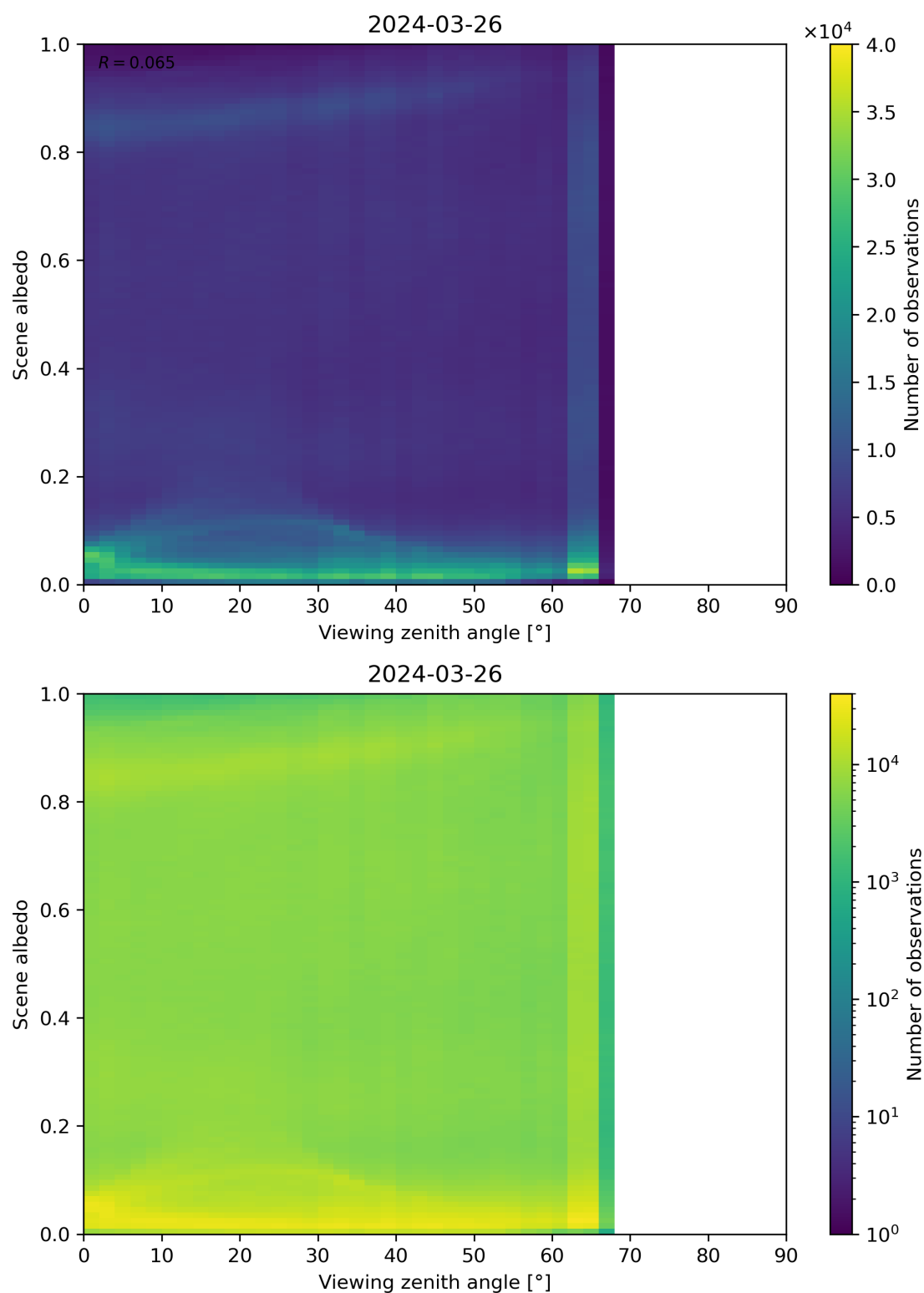
Figure 126: Scatter density plot of “Viewing zenith angle” against “Scene albedo” for 2024-03-25 to 2024-03-27.
