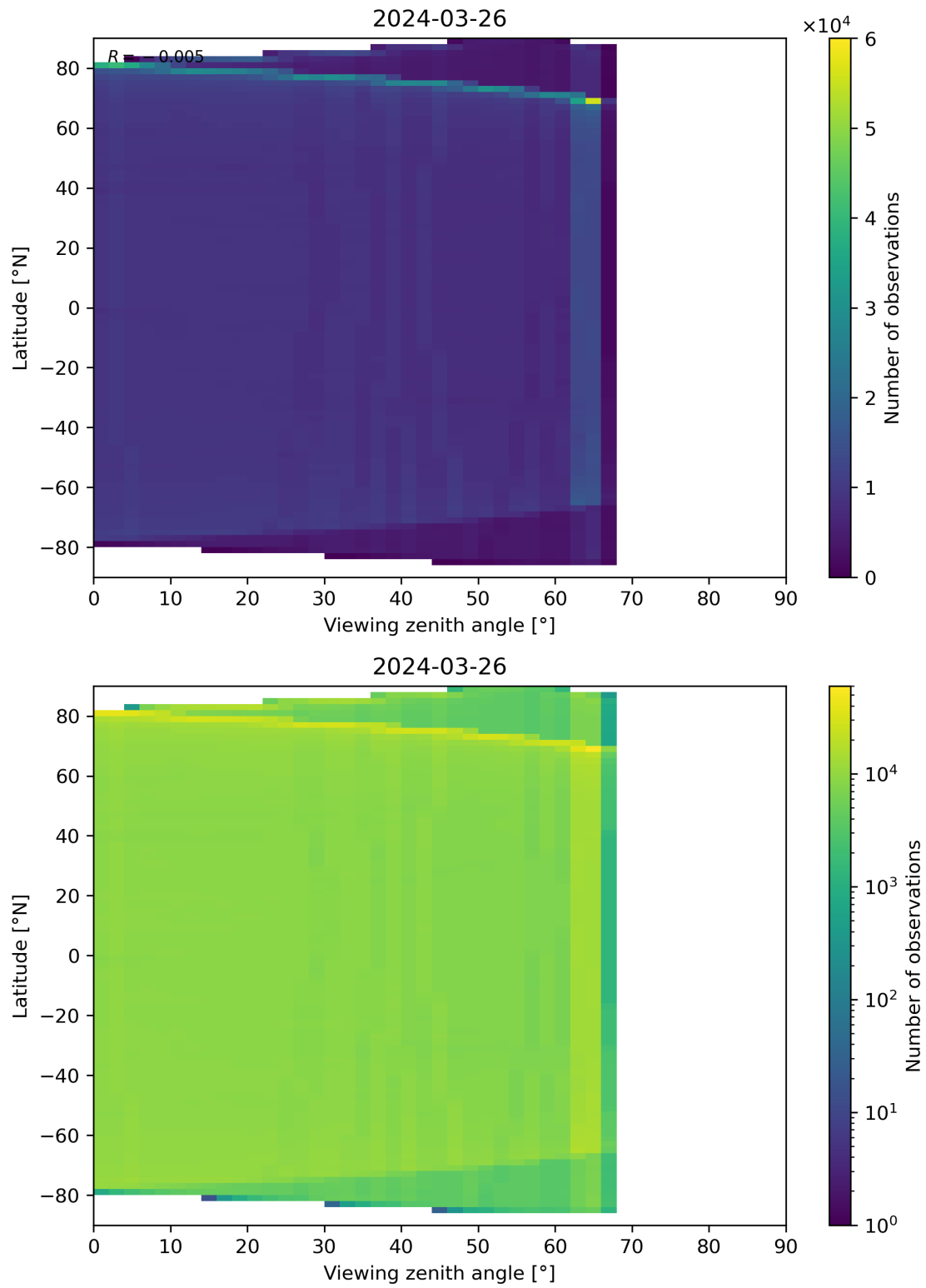
Figure 123: Scatter density plot of “Viewing zenith angle” against “Latitude” for 2024-03-25 to 2024-03-27.
