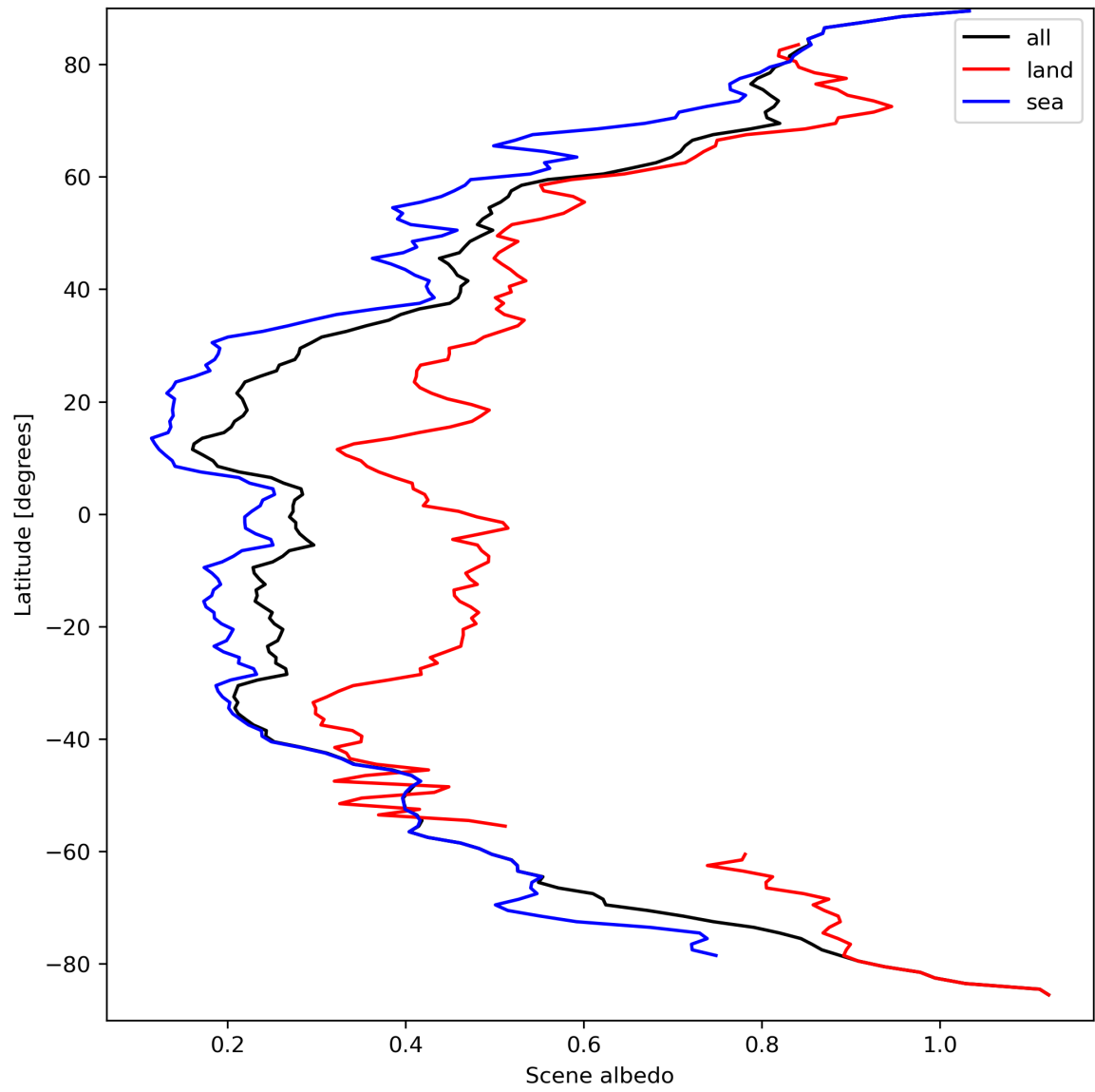
Figure 17: Zonal average of “Scene albedo” for 2024-03-25 to 2024-03-27.
