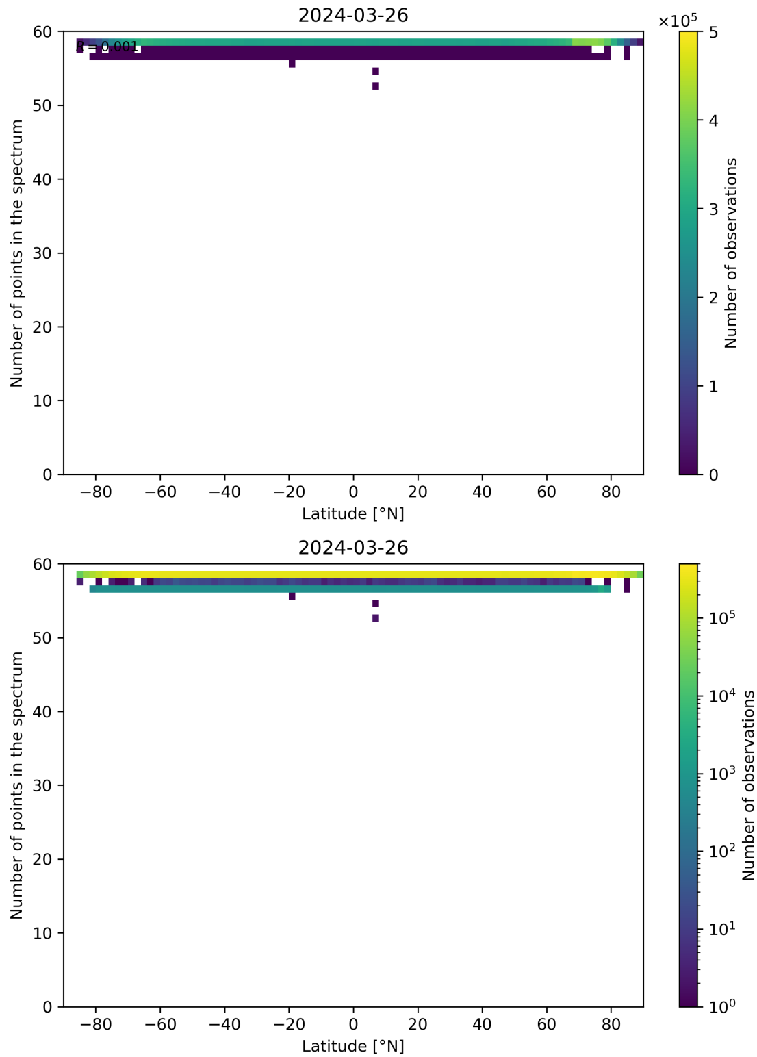
Figure 94: Scatter density plot of “Latitude” against “Number of points in the spectrum” for 2024-03-25 to 2024-03-27.
