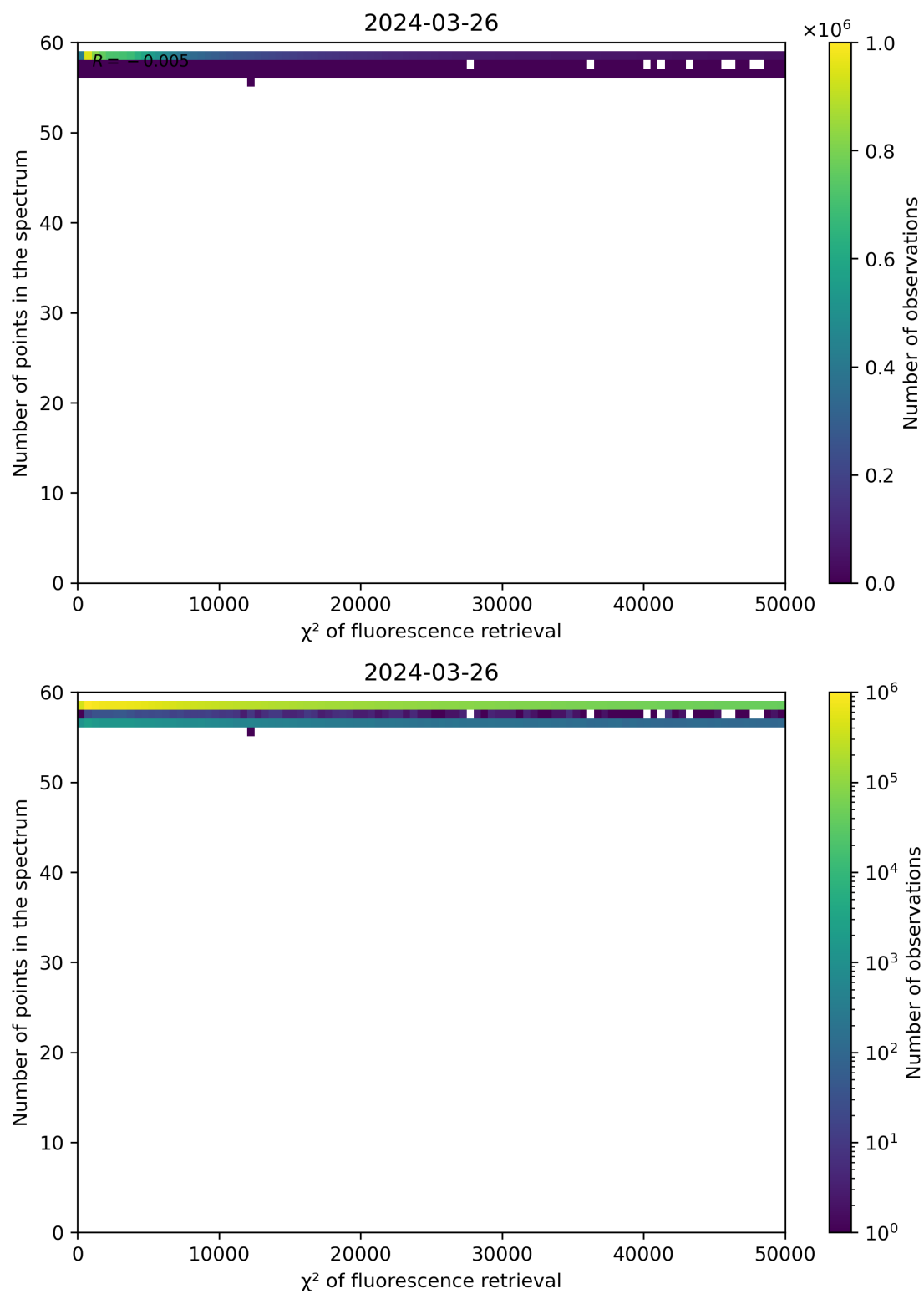
Figure 68: Scatter density plot of “ \chi^2 of fluorescence retrieval” against “Number of points in the spectrum” for 2024-03-25 to 2024-03-27.
