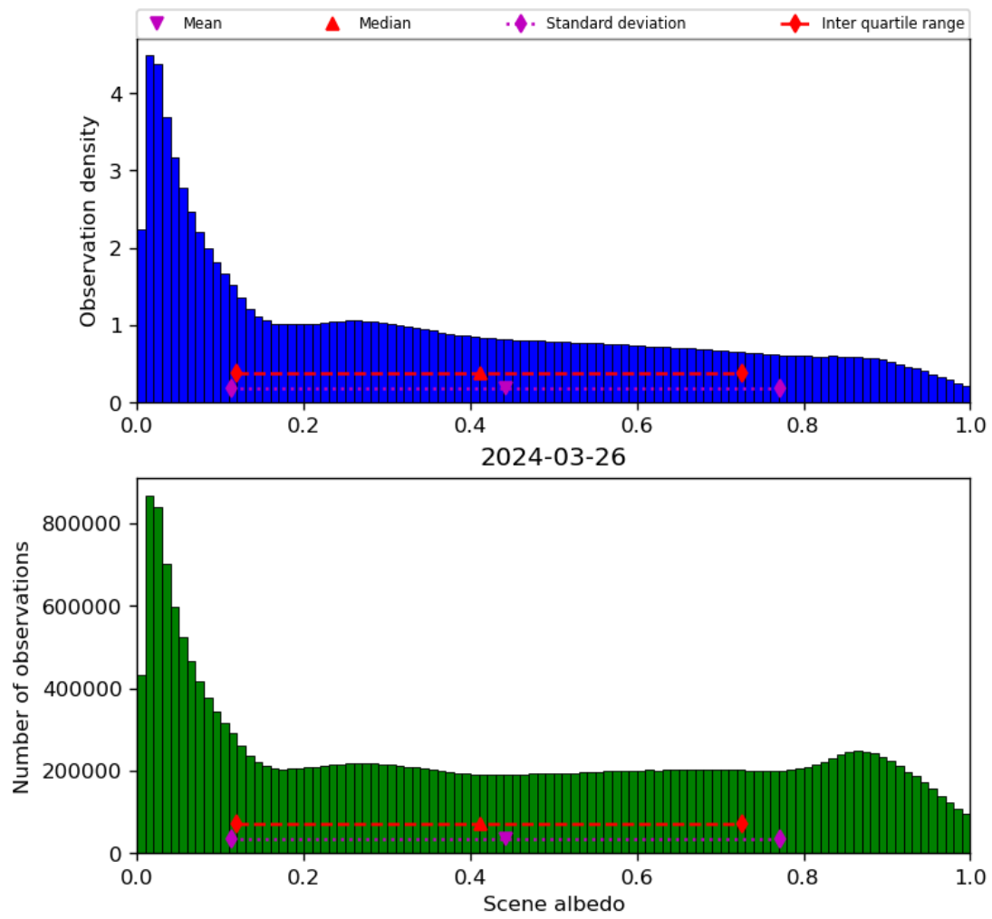
Figure 34: Histogram of “Scene albedo” for 2024-03-25 to 2024-03-27
