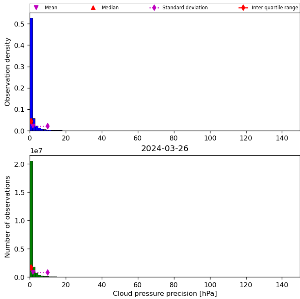
Figure 31: Histogram of “Cloud pressure precision” for 2024-03-25 to 2024-03-27
