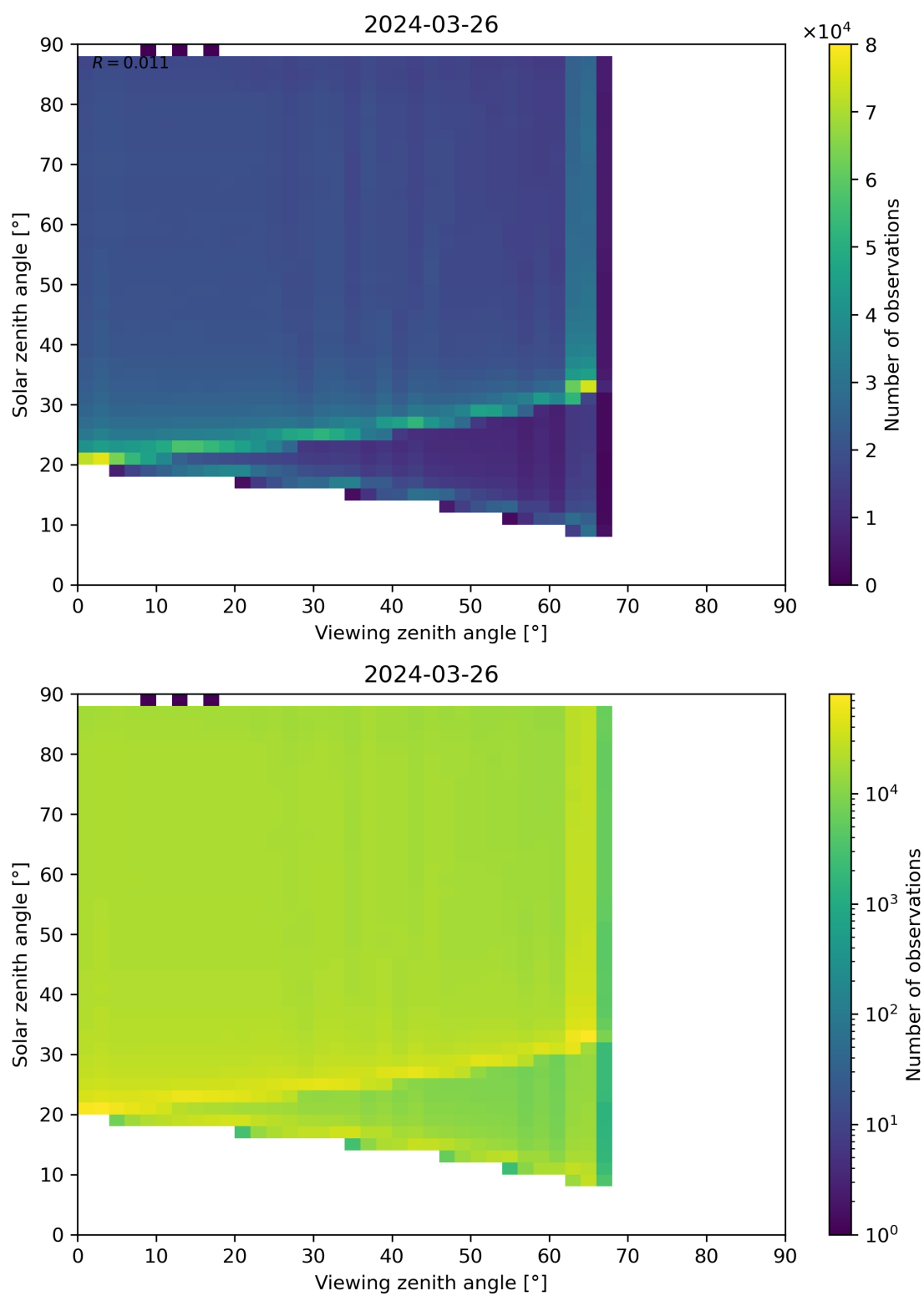
Figure 127: Scatter density plot of “Viewing zenith angle” against “Solar zenith angle” for 2024-03-25 to 2024-03-27.
