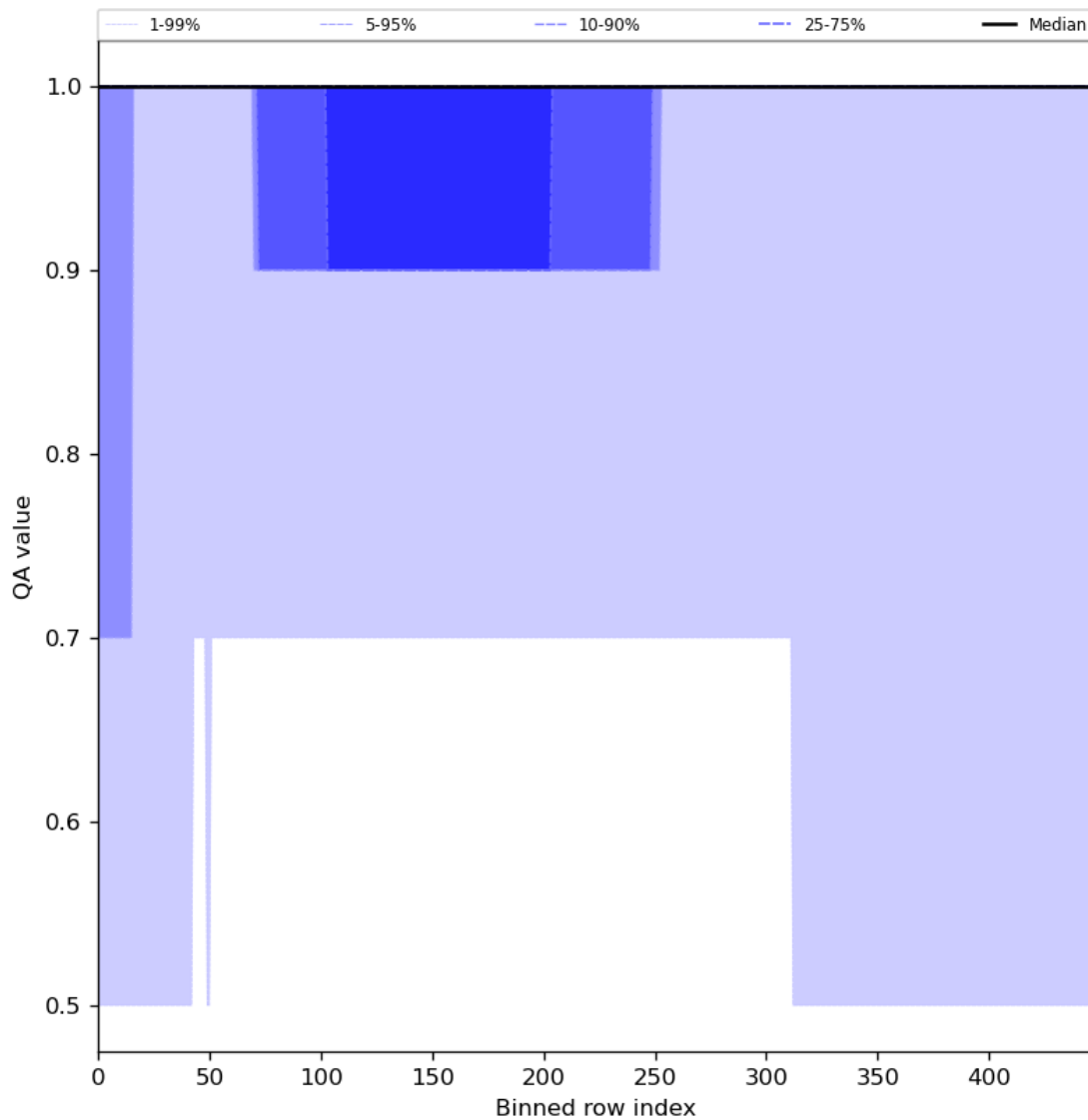
Figure 46: Along track statistics of “QA value” for 2024-03-25 to 2024-03-27
