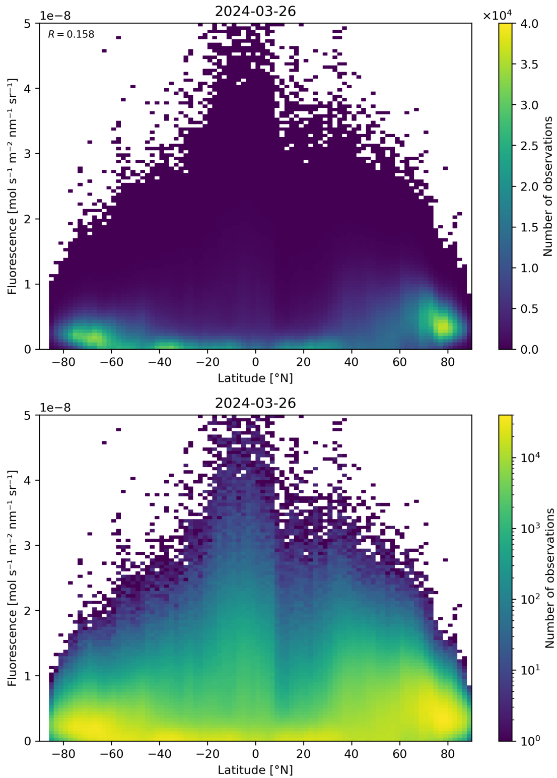
Figure 92: Scatter density plot of “Latitude” against “Fluorescence” for 2024-03-25 to 2024-03-27.
