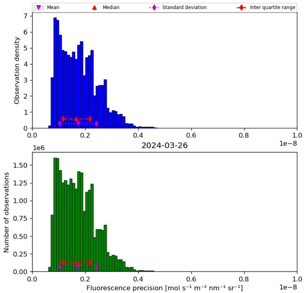
Figure 41: Histogram of “Fluorescence precision” for 2024-03-25 to 2024-03-27
