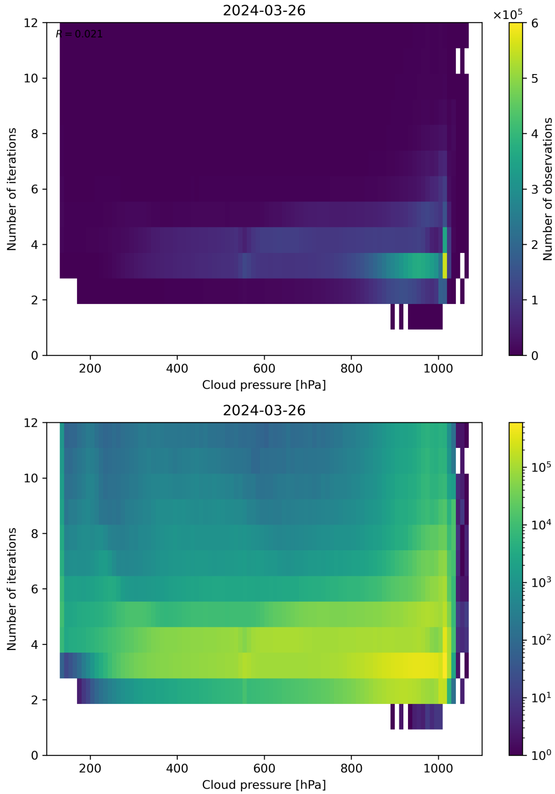
Figure 81: Scatter density plot of “Cloud pressure” against “Number of iterations” for 2024-03-25 to 2024-03-27.
