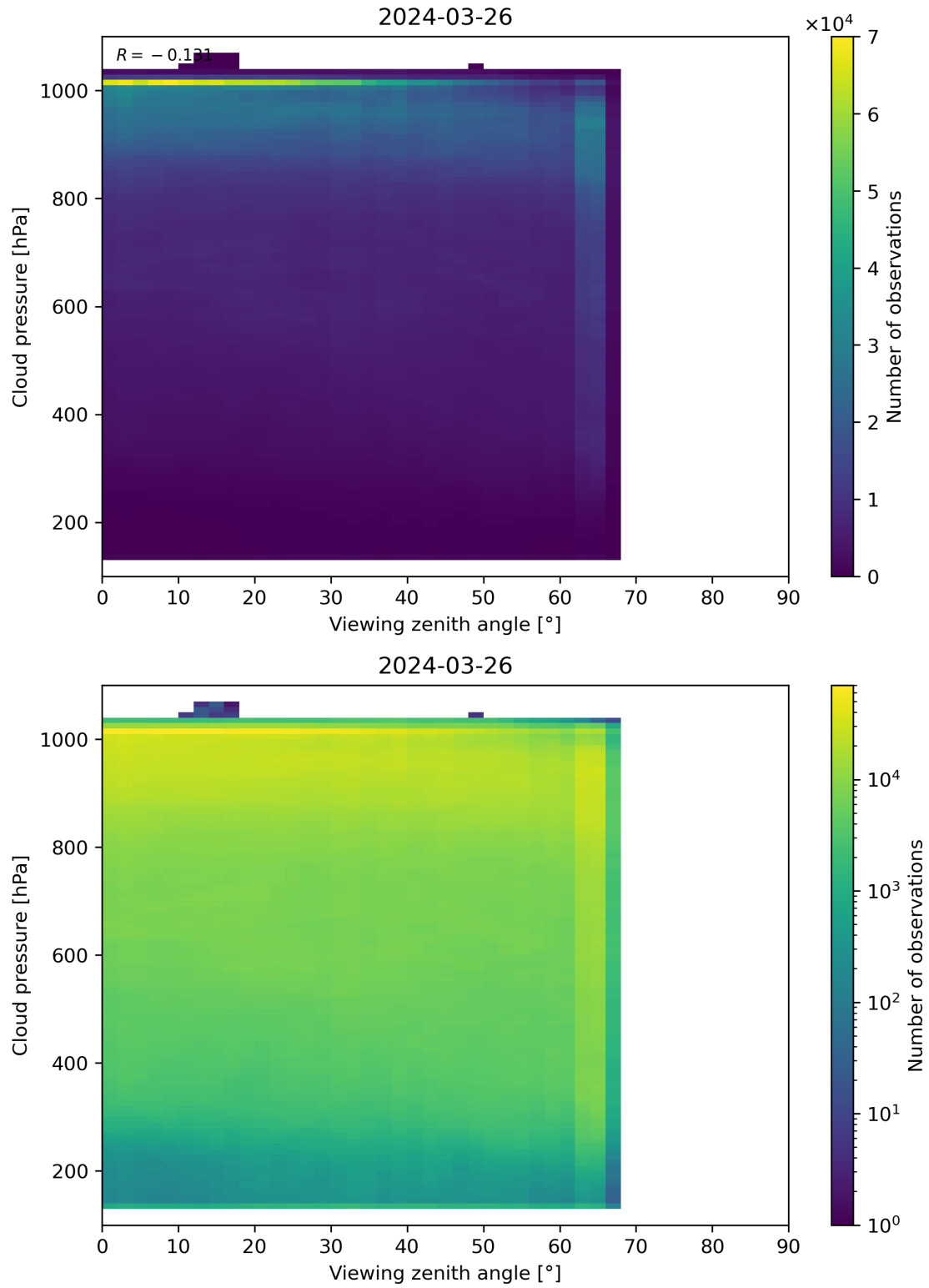
Figure 121: Scatter density plot of “Viewing zenith angle” against “Cloud pressure” for 2024-03-25 to 2024-03-27.
