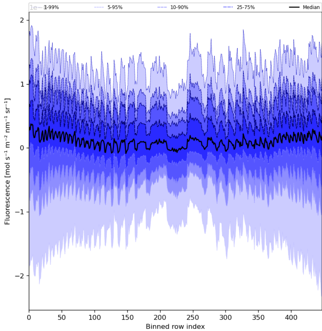
Figure 57: Along track statistics of “Fluorescence” for 2024-03-25 to 2024-03-27
