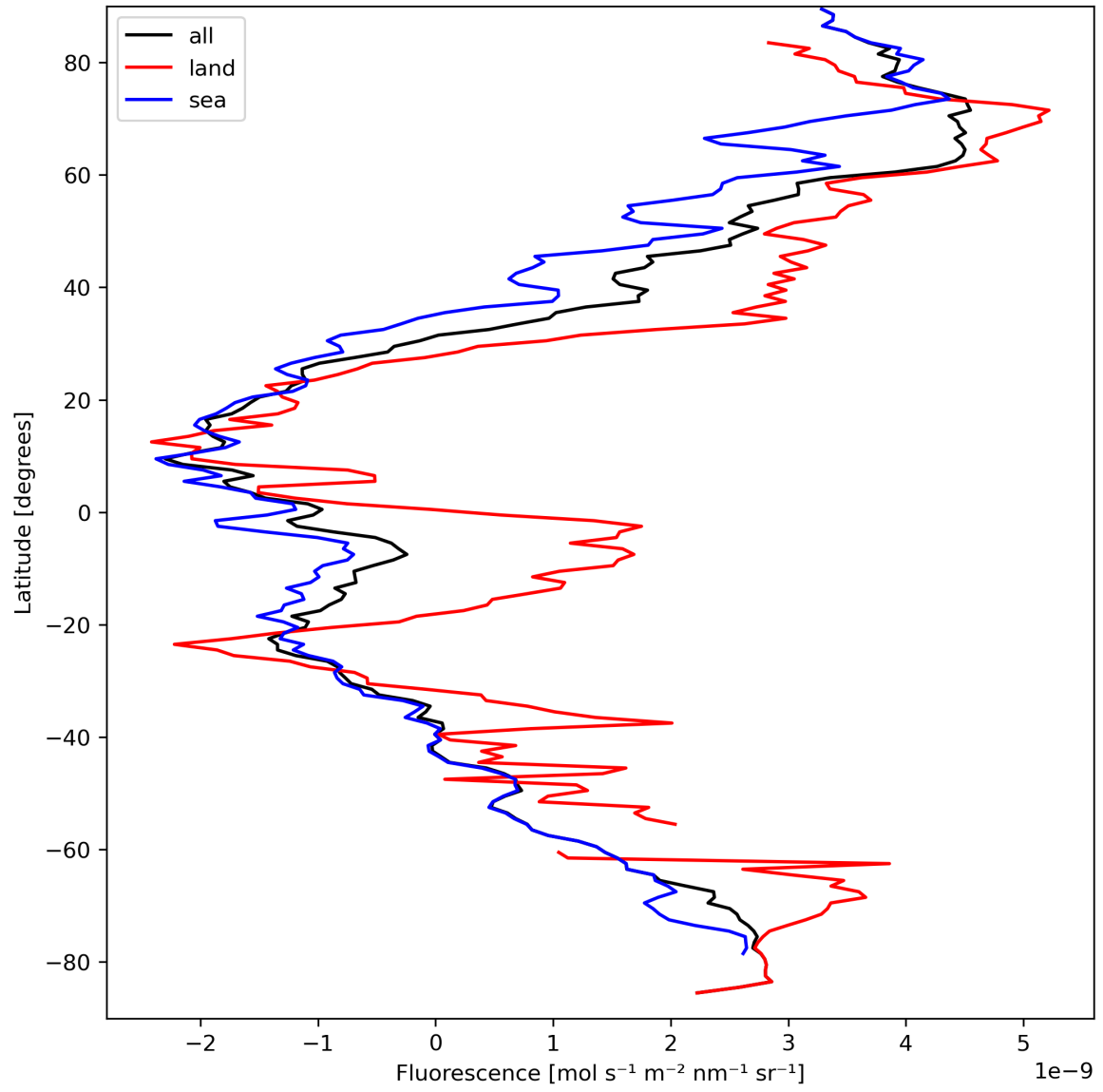
Figure 23: Zonal average of “Fluorescence” for 2024-03-25 to 2024-03-27.
