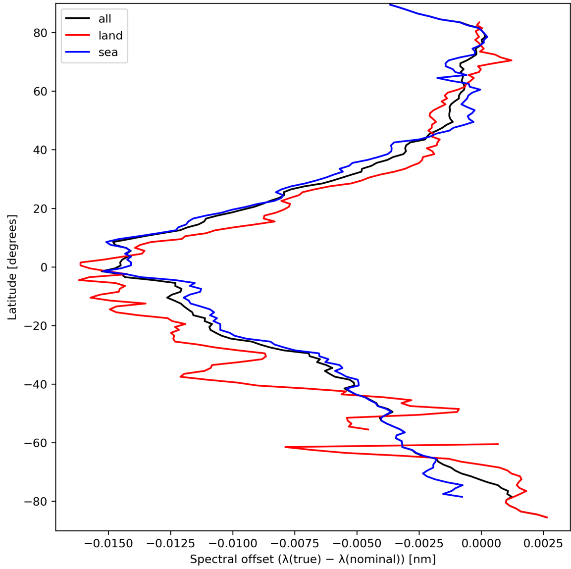
Figure 28: Zonal average of “Spectral offset ( \lambda(\text{true}) - \lambda(\text{nominal}) )” for 2024-03-25 to 2024-03-27.
