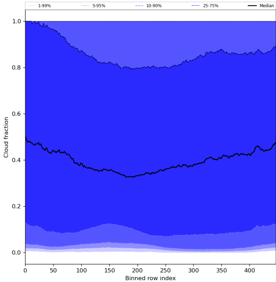
Figure 49: Along track statistics of “Cloud fraction” for 2024-03-25 to 2024-03-27
