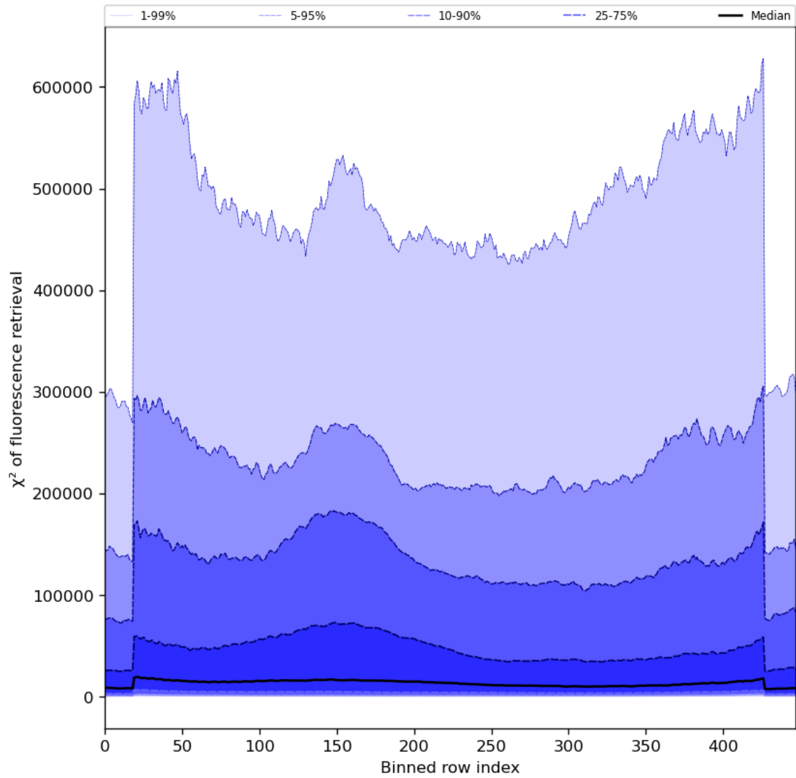
Figure 59: Along track statistics of “ \chi^2 of fluorescence retrieval” for 2024-03-25 to 2024-03-27
