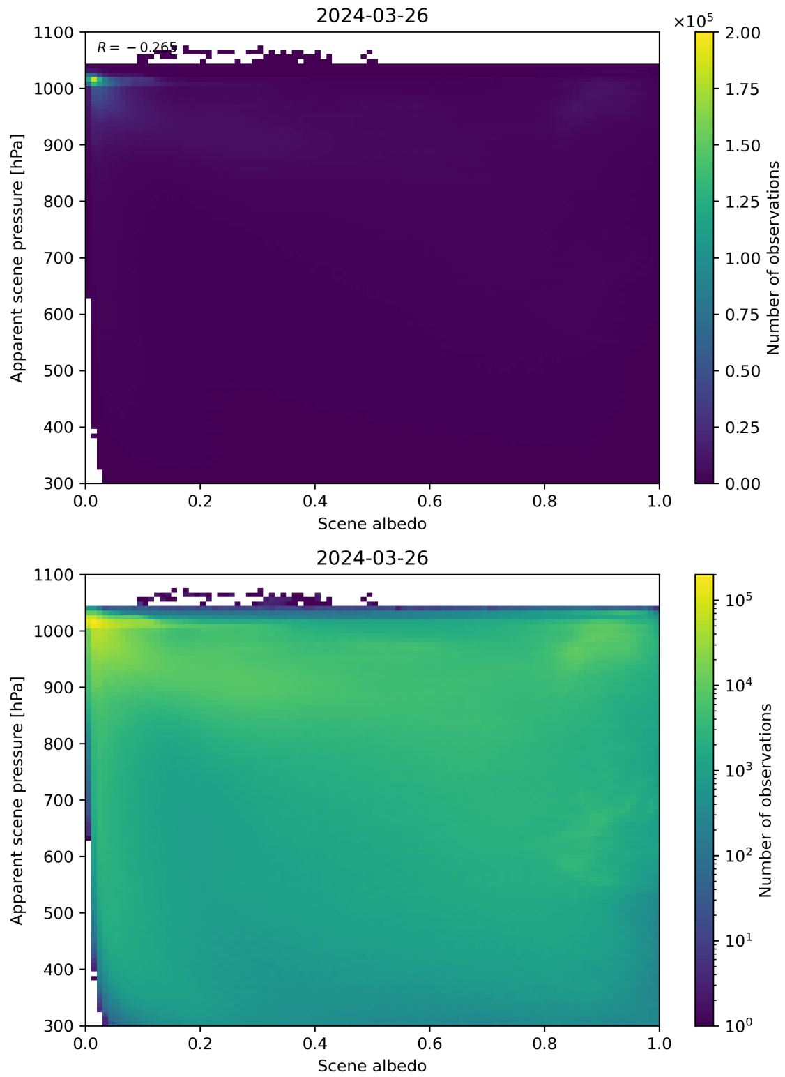
Figure 102: Scatter density plot of “Scene albedo” against “Apparent scene pressure” for 2024-03-25 to 2024-03-27.
