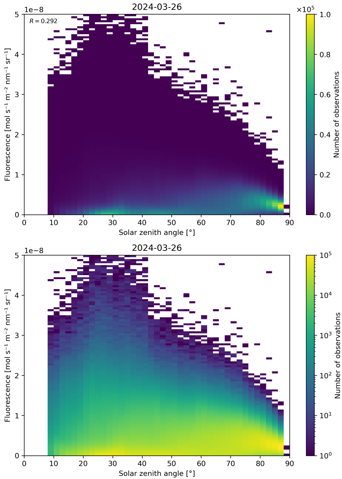
Figure 112: Scatter density plot of “Solar zenith angle” against “Fluorescence” for 2024-03-25 to 2024-03-27.
