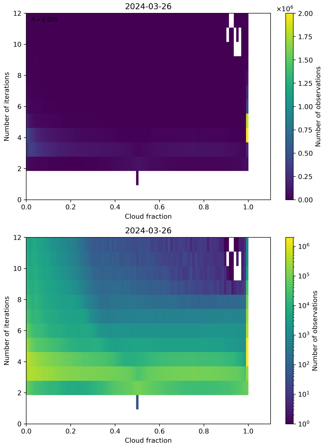
Figure 73: Scatter density plot of “Cloud fraction” against “Number of iterations” for 2024-03-25 to 2024-03-27.
