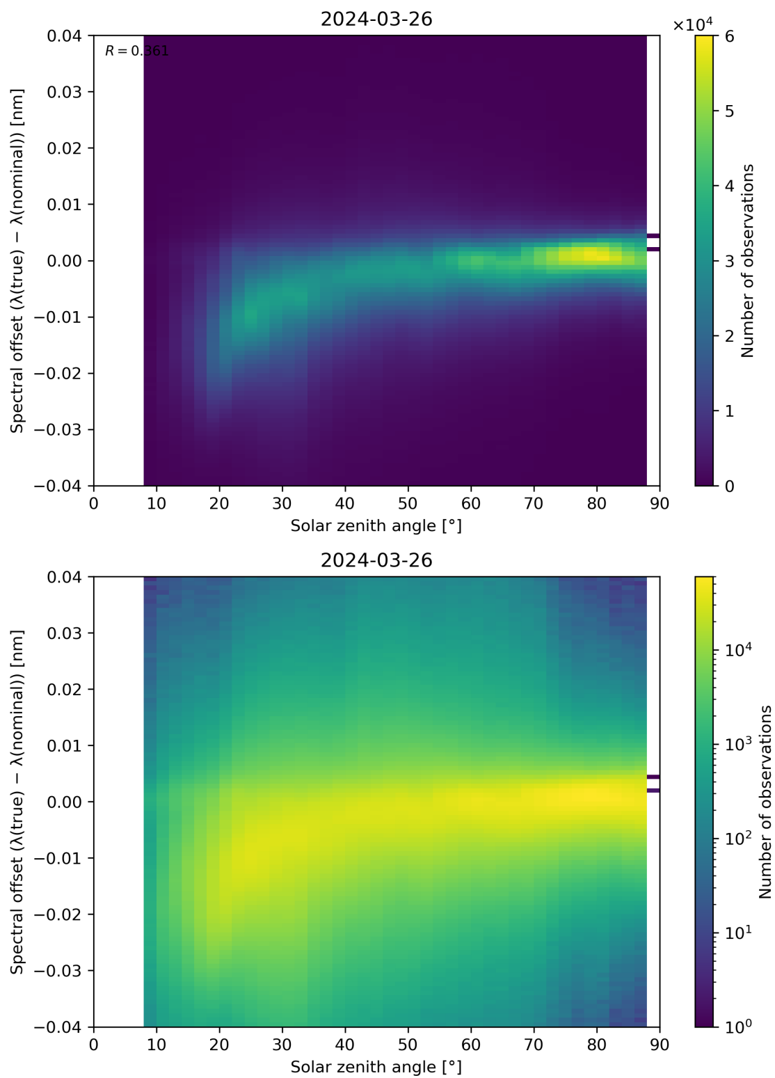
Figure 117: Scatter density plot of “Solar zenith angle” against “Spectral offset ( \lambda(\text{true}) - \lambda(\text{nominal}) )” for 2024-03-25 to 2024-03-27.
