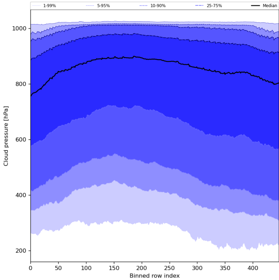
Figure 47: Along track statistics of “Cloud pressure” for 2024-03-25 to 2024-03-27
