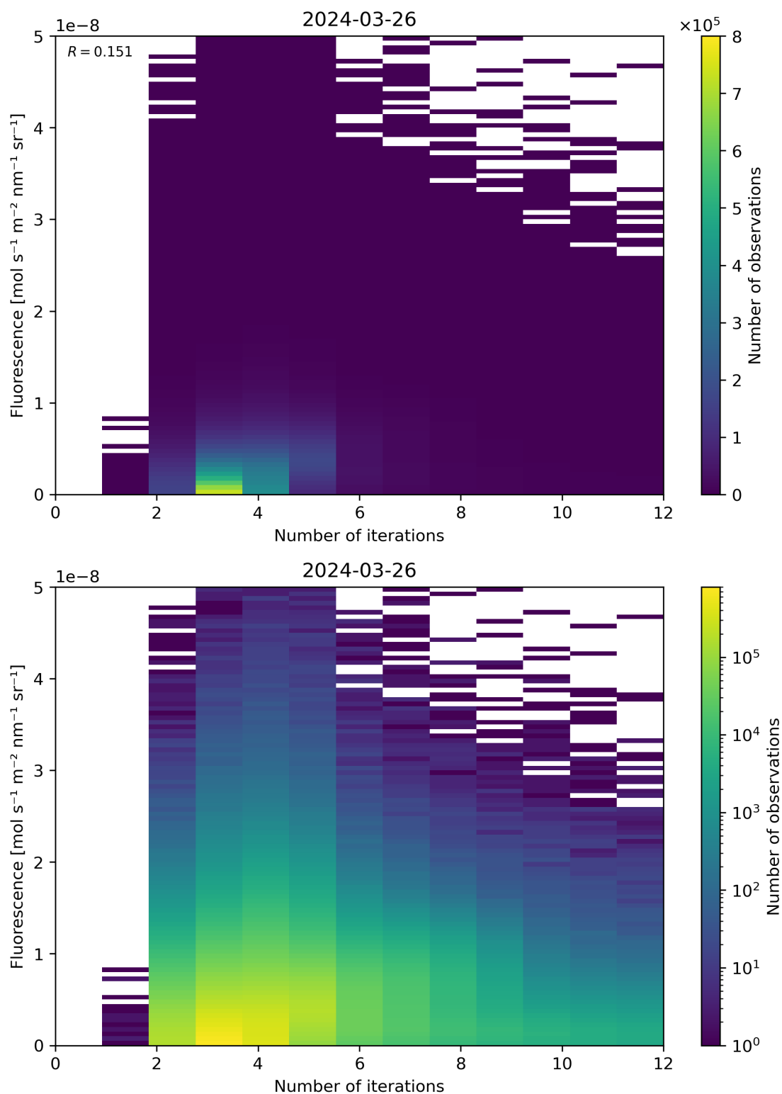
Figure 98: Scatter density plot of “Number of iterations” against “Fluorescence” for 2024-03-25 to 2024-03-27.
