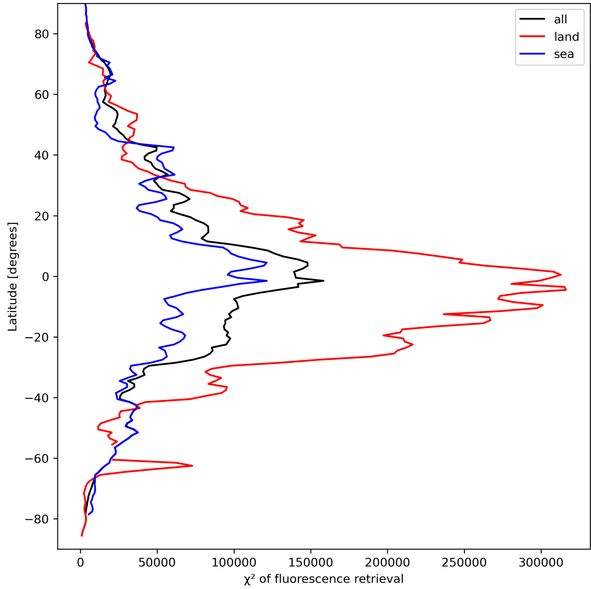
Figure 25: Zonal average of “ \chi^2 of fluorescence retrieval” for 2024-03-25 to 2024-03-27.
