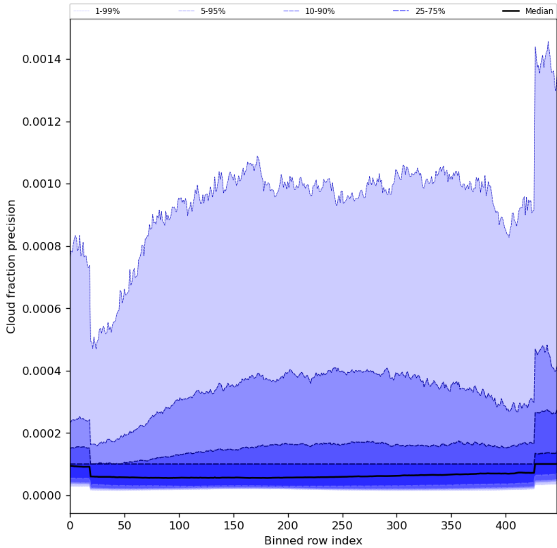
Figure 50: Along track statistics of “Cloud fraction precision” for 2024-03-25 to 2024-03-27
