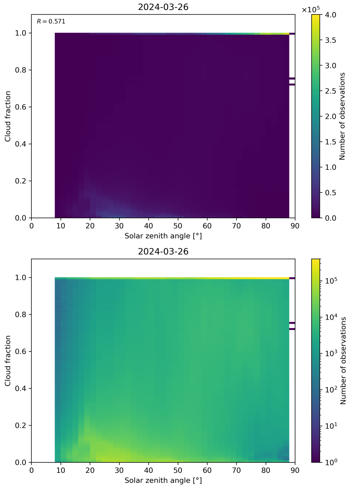
Figure 110: Scatter density plot of “Solar zenith angle” against “Cloud fraction” for 2024-03-25 to 2024-03-27.
