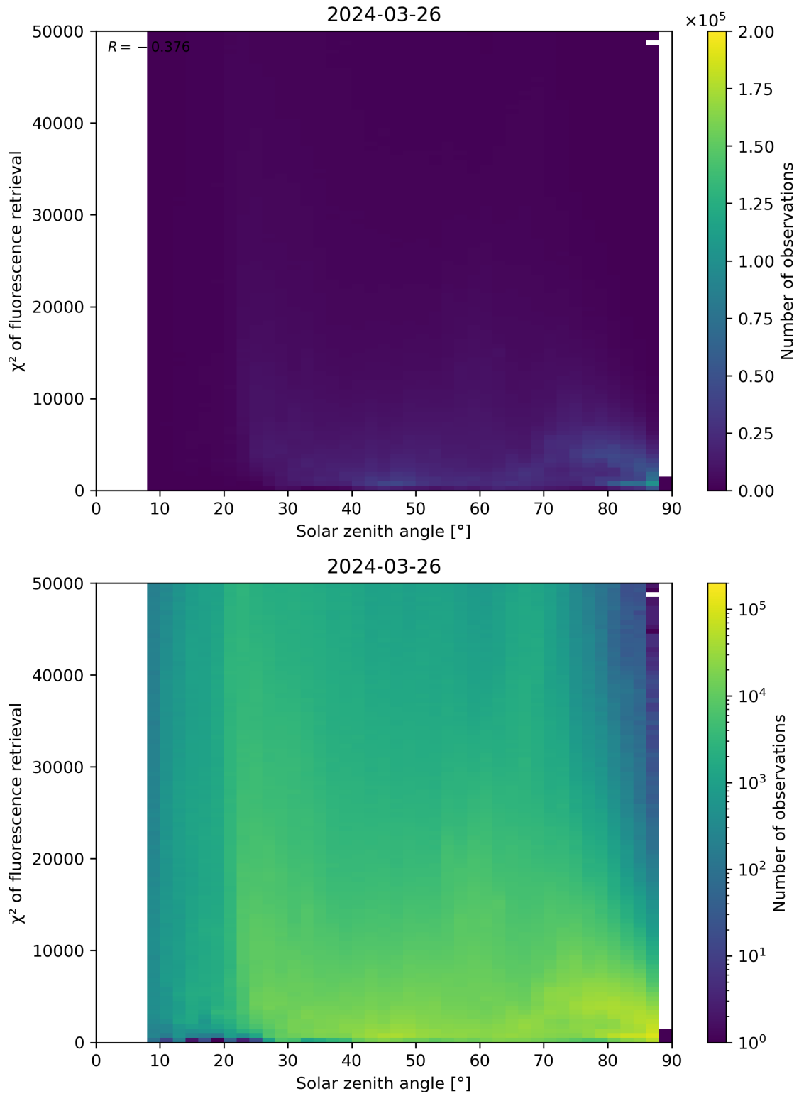
Figure 109: Scatter density plot of “Solar zenith angle” against “ \chi^2 of fluorescence retrieval” for 2024-03-25 to 2024-03-27.
