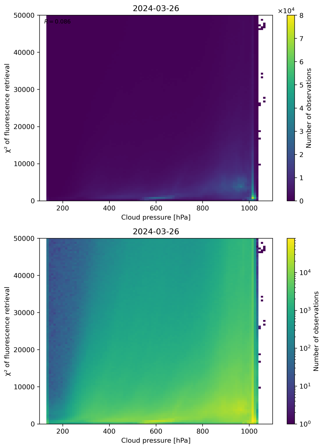
Figure 78: Scatter density plot of “Cloud pressure” against “ \chi^2 of fluorescence retrieval” for 2024-03-25 to 2024-03-27.
