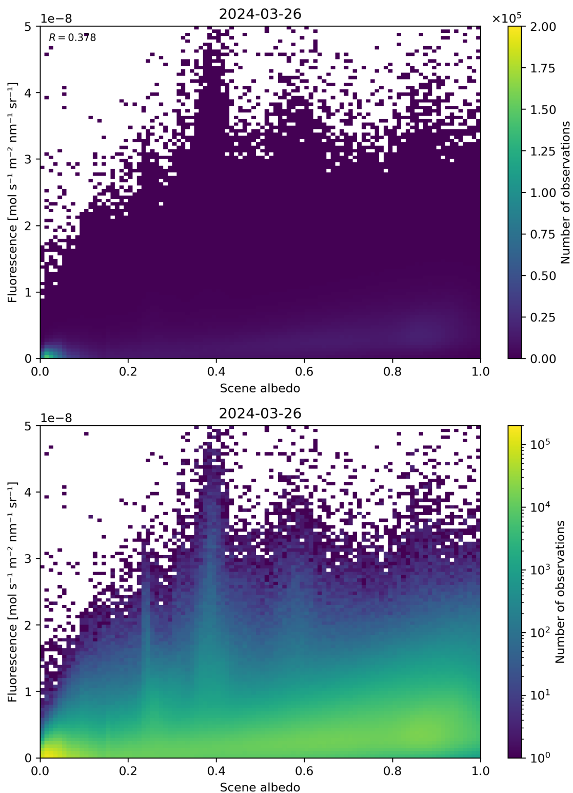
Figure 104: Scatter density plot of “Scene albedo” against “Fluorescence” for 2024-03-25 to 2024-03-27.
