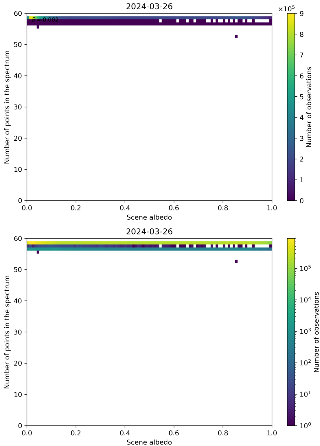
Figure 106: Scatter density plot of “Scene albedo” against “Number of points in the spectrum” for 2024-03-25 to 2024-03-27.
