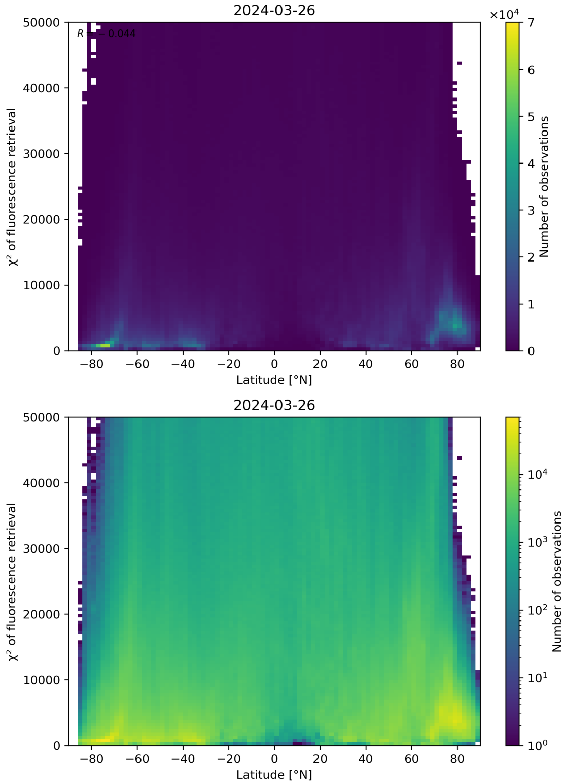
Figure 89: Scatter density plot of “Latitude” against “ \chi^2 of fluorescence retrieval” for 2024-03-25 to 2024-03-27.
