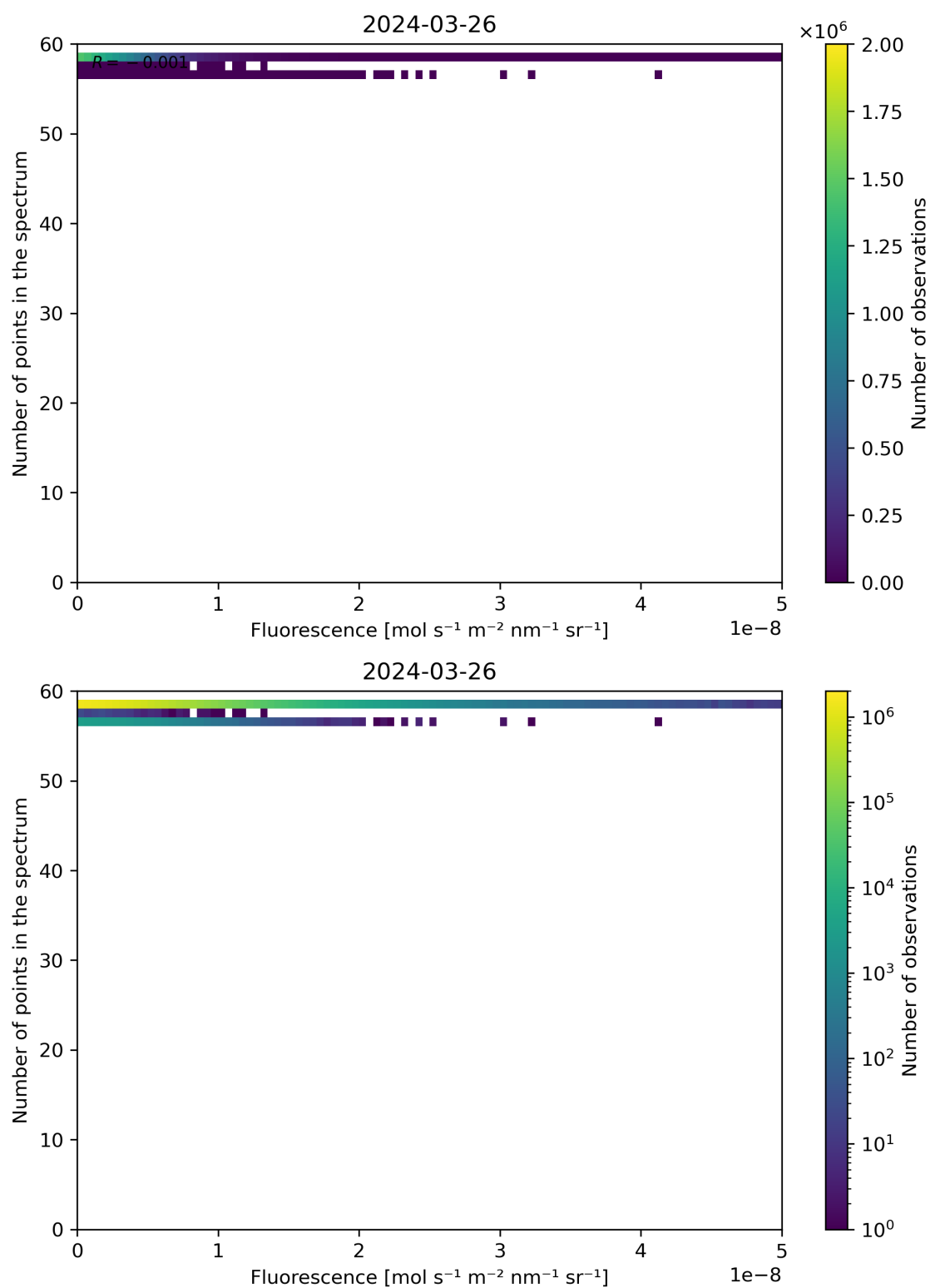
Figure 86: Scatter density plot of “Fluorescence” against “Number of points in the spectrum” for 2024-03-25 to 2024-03-27.
