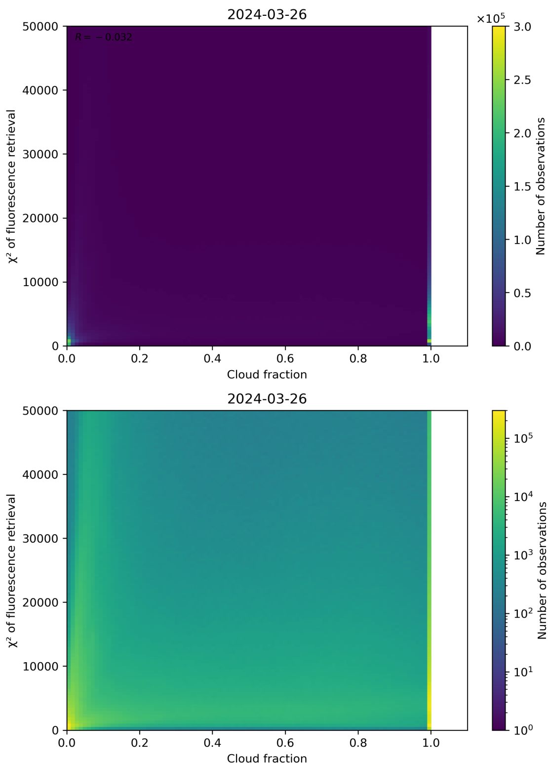
Figure 71: Scatter density plot of “Cloud fraction” against “ \chi^2 of fluorescence retrieval” for 2024-03-25 to 2024-03-27.
