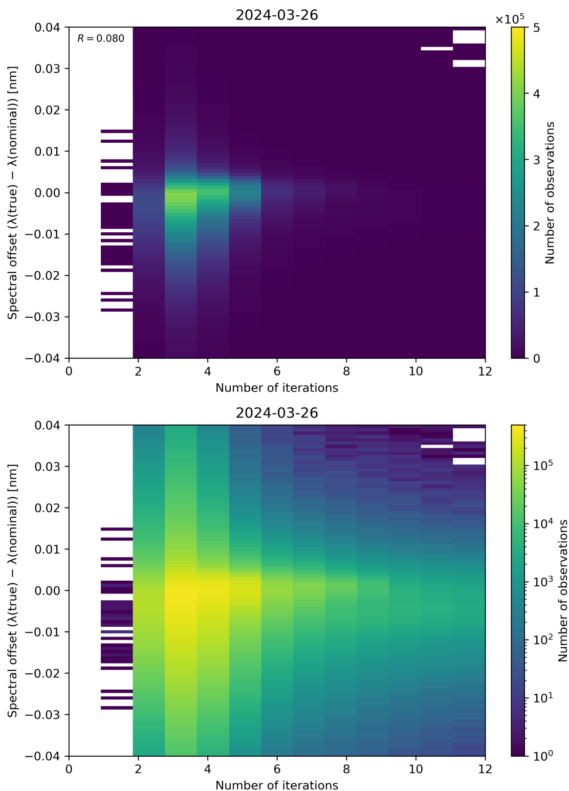
Figure 100: Scatter density plot of “Number of iterations” against “Spectral offset ( \lambda(\text{true}) - \lambda(\text{nominal}) )” for 2024-03-25 to 2024-03-27.
