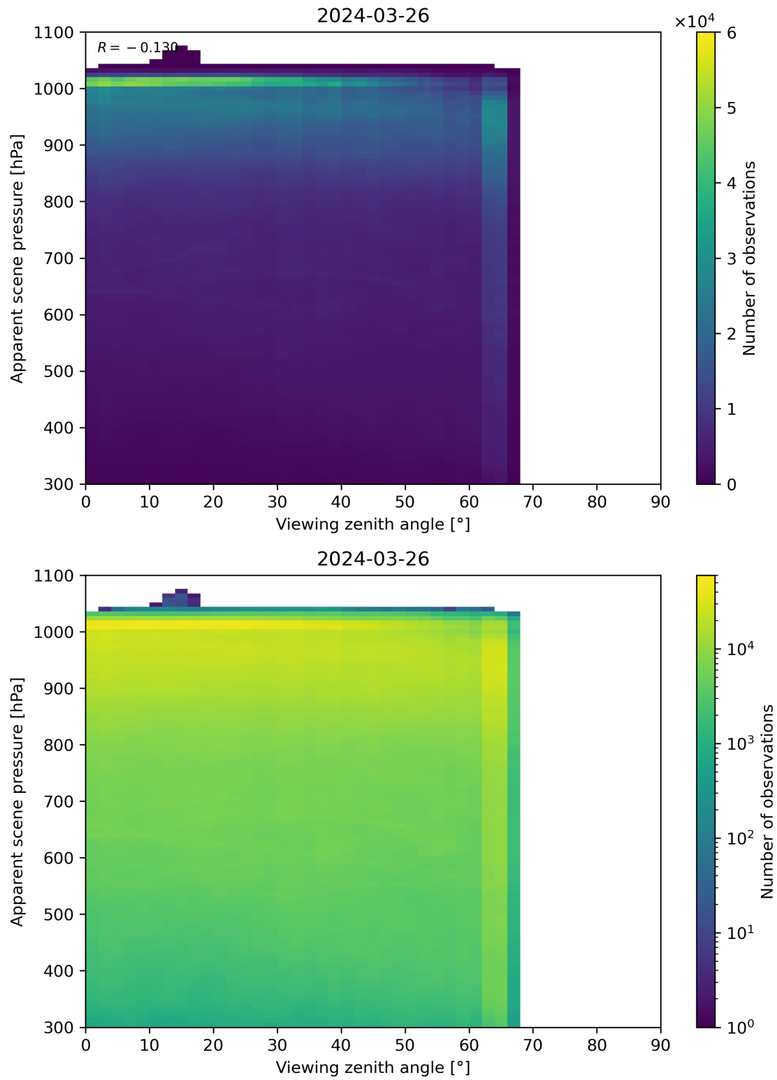
Figure 118: Scatter density plot of “Viewing zenith angle” against “Apparent scene pressure” for 2024-03-25 to 2024-03-27.
