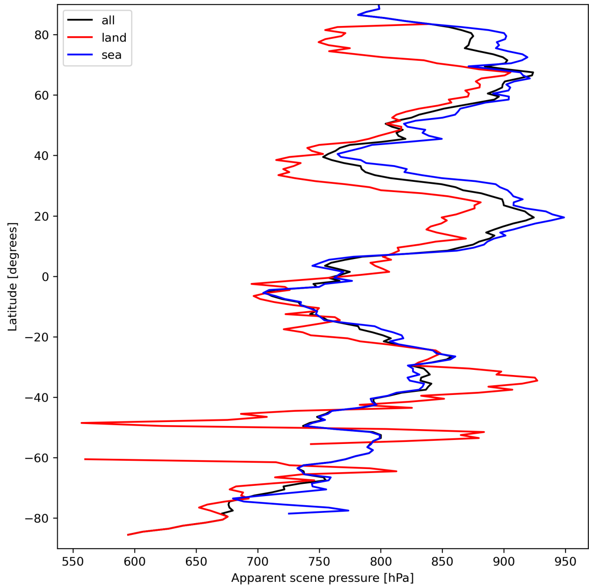
Figure 19: Zonal average of “Apparent scene pressure” for 2024-03-25 to 2024-03-27.
