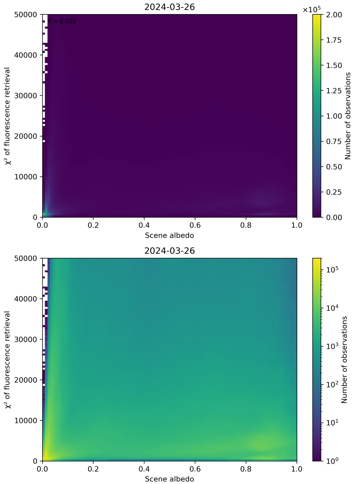
Figure 103: Scatter density plot of “Scene albedo” against “ \chi^2 of fluorescence retrieval” for 2024-03-25 to 2024-03-27.
