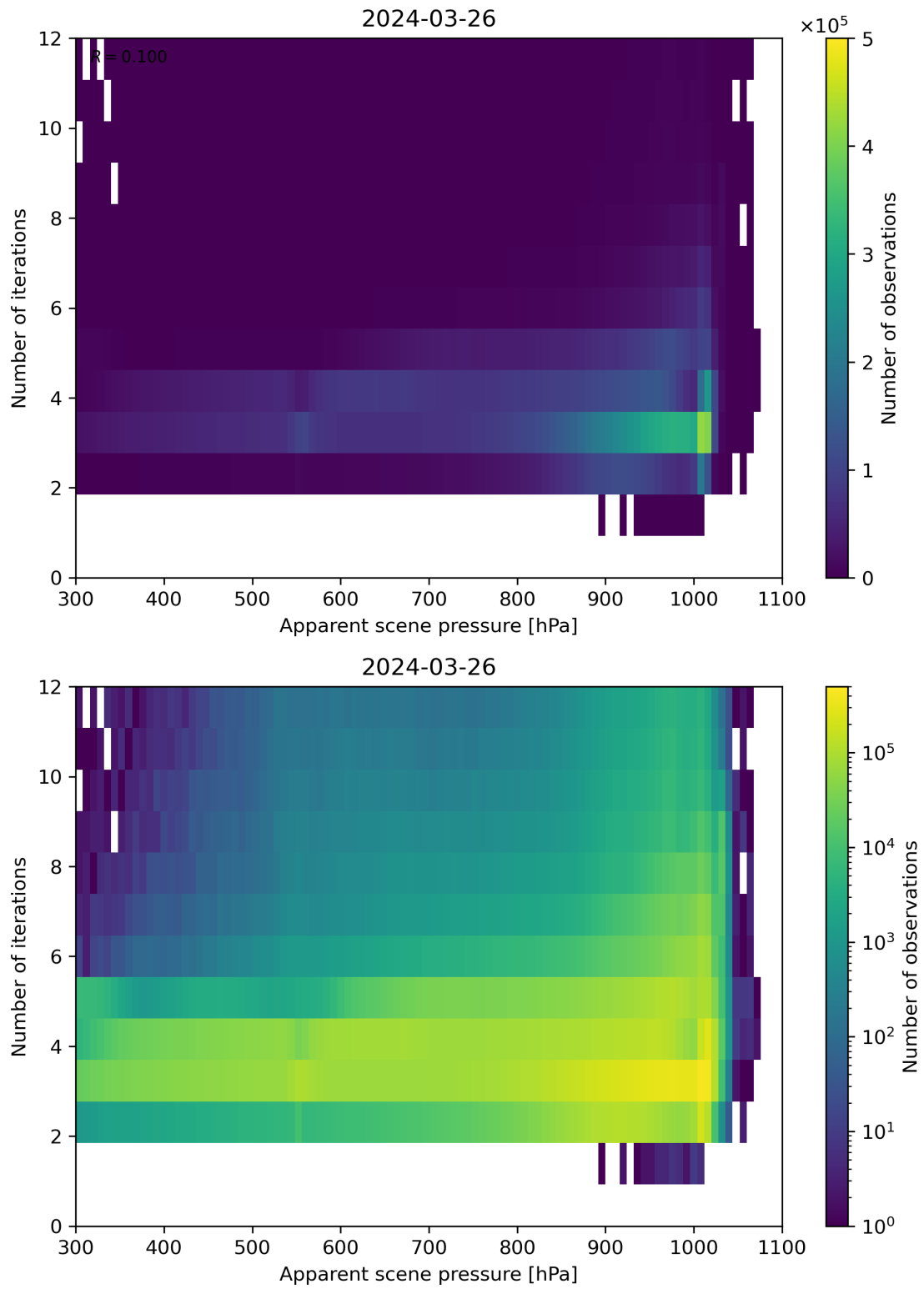
Figure 65: Scatter density plot of “Apparent scene pressure” against “Number of iterations” for 2024-03-25 to 2024-03-27.
