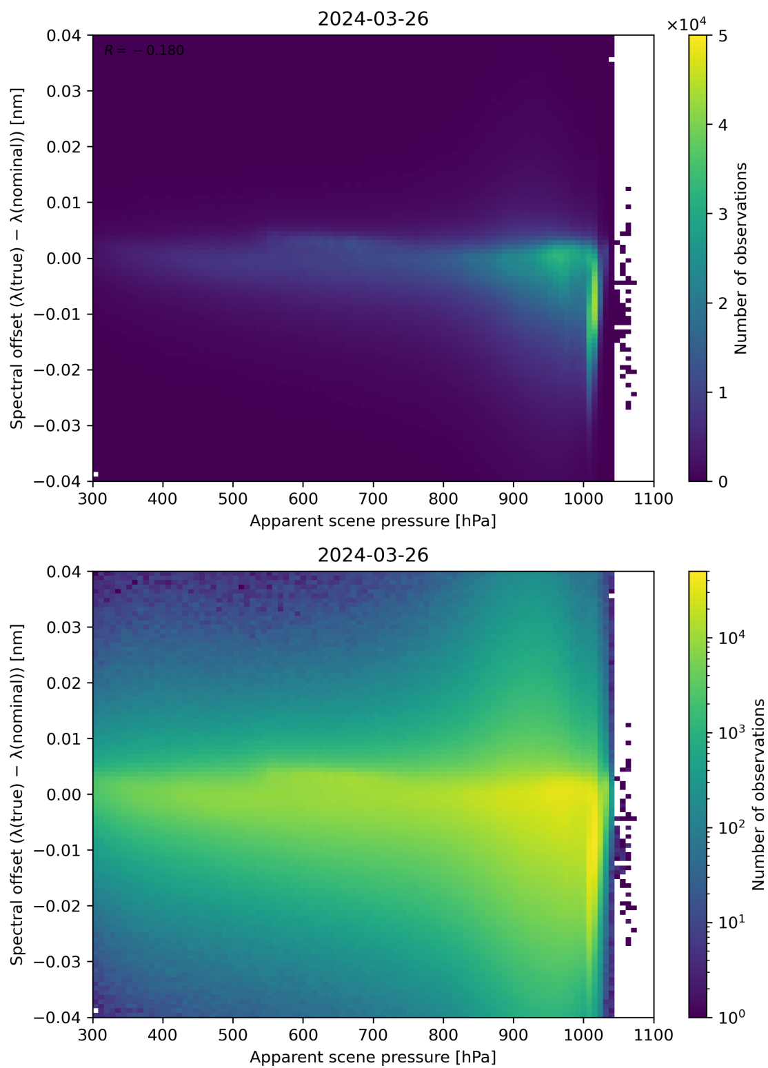
Figure 67: Scatter density plot of “Apparent scene pressure” against “Spectral offset ( \lambda(\text{true}) - \lambda(\text{nominal}) )” for 2024-03-25 to 2024-03-27.
