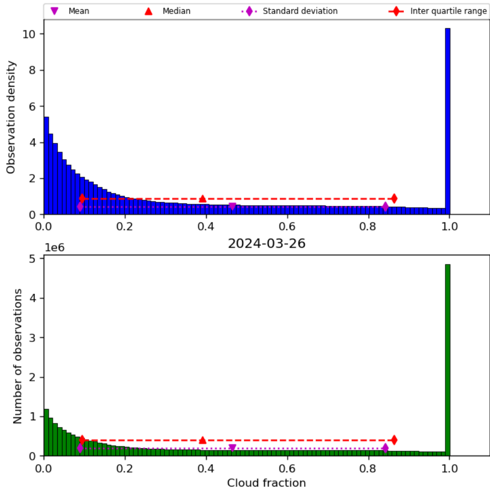
Figure 32: Histogram of “Cloud fraction” for 2024-03-25 to 2024-03-27
