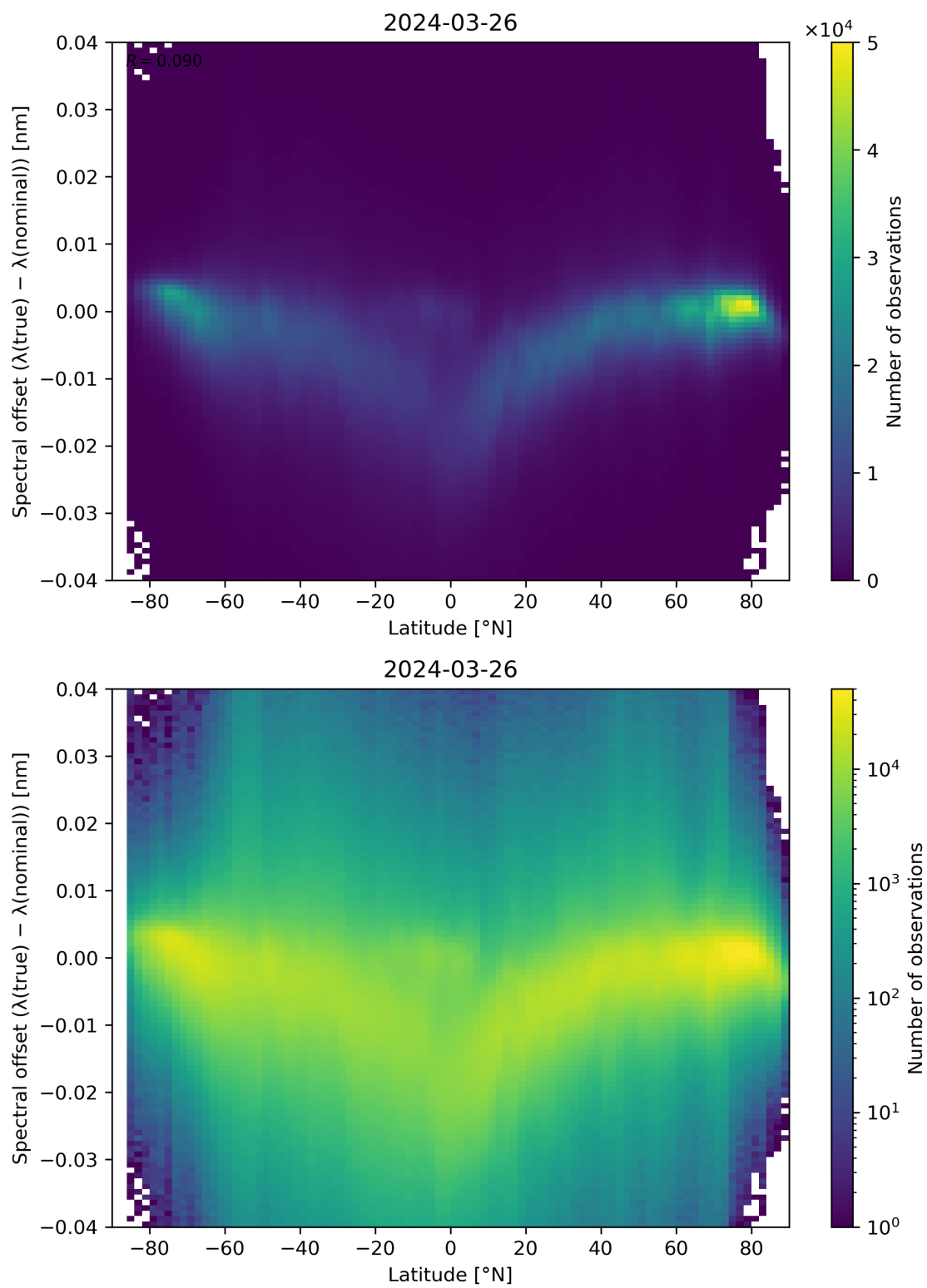
Figure 96: Scatter density plot of “Latitude” against “Spectral offset ( \lambda(\text{true}) - \lambda(\text{nominal}) )” for 2024-03-25 to 2024-03-27.
