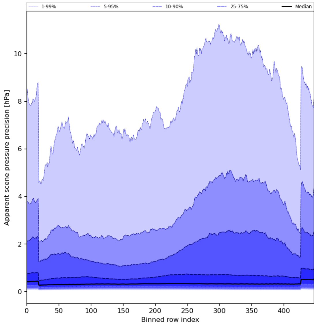
Figure 54: Along track statistics of “Apparent scene pressure precision” for 2024-03-25 to 2024-03-27
