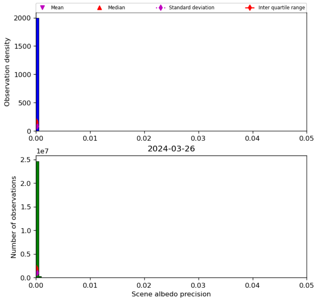
Figure 35: Histogram of “Scene albedo precision” for 2024-03-25 to 2024-03-27
