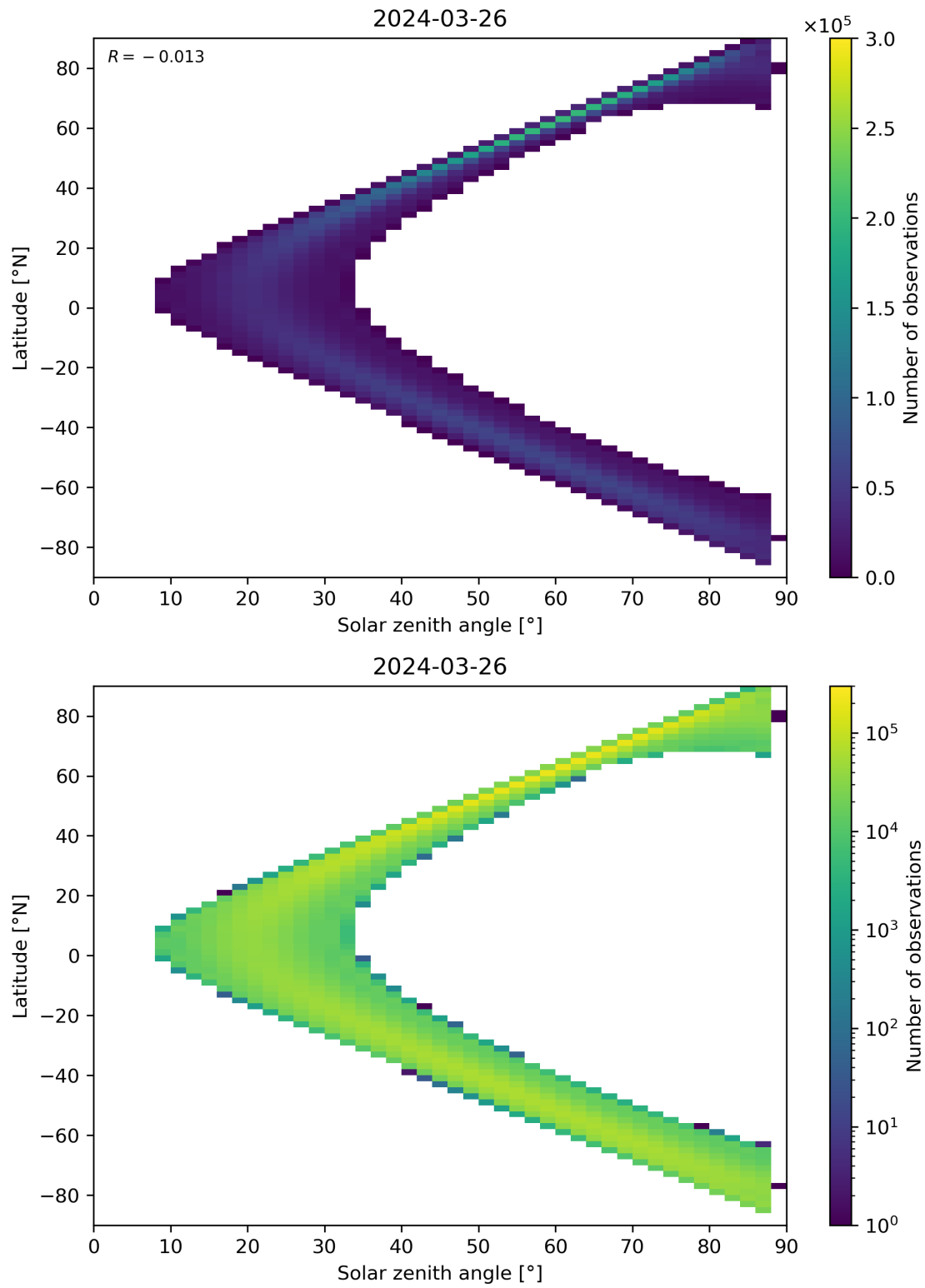
Figure 113: Scatter density plot of “Solar zenith angle” against “Latitude” for 2024-03-25 to 2024-03-27.
