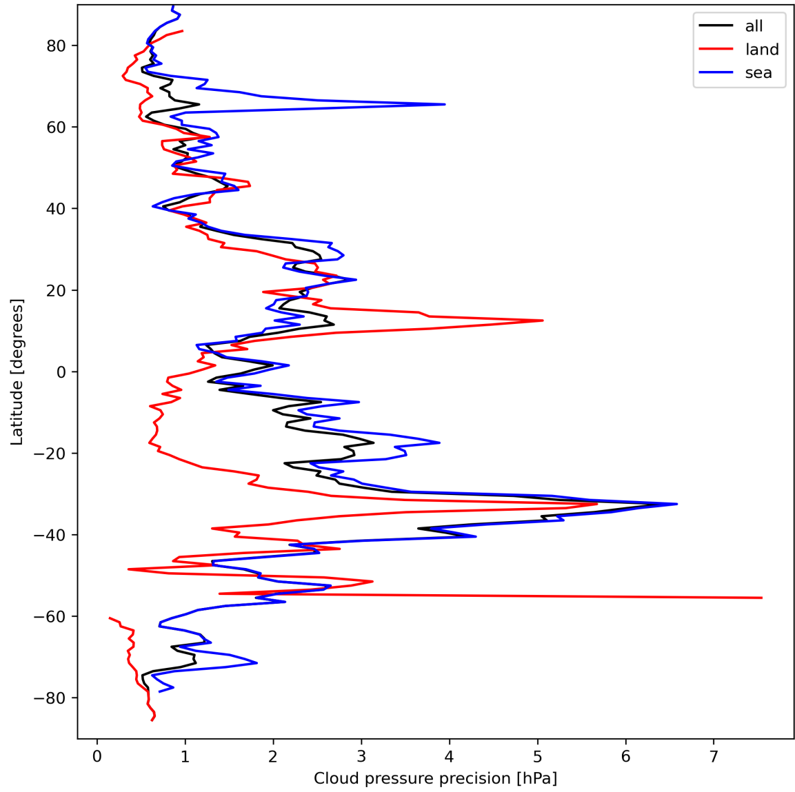
Figure 14: Zonal average of “Cloud pressure precision” for 2024-03-25 to 2024-03-27.
