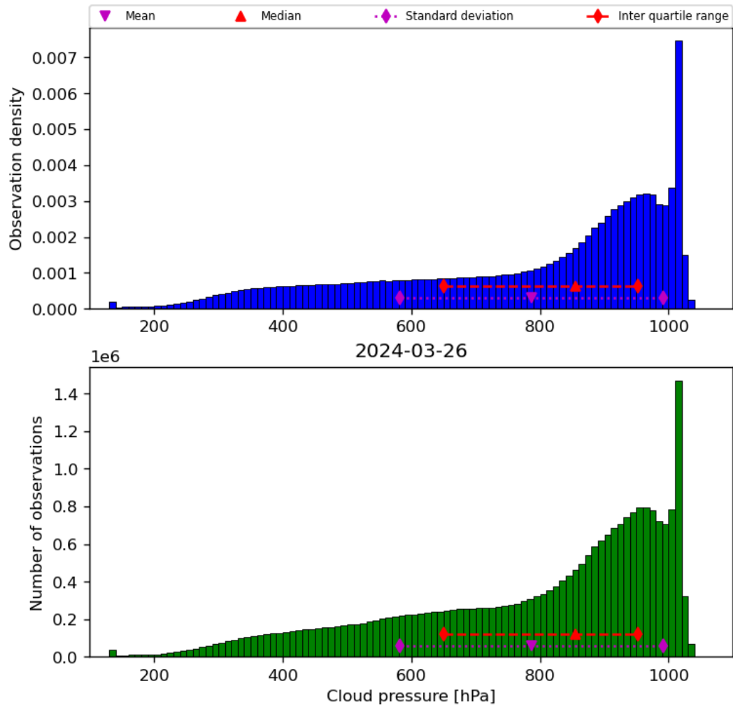
Figure 30: Histogram of “Cloud pressure” for 2024-03-25 to 2024-03-27
