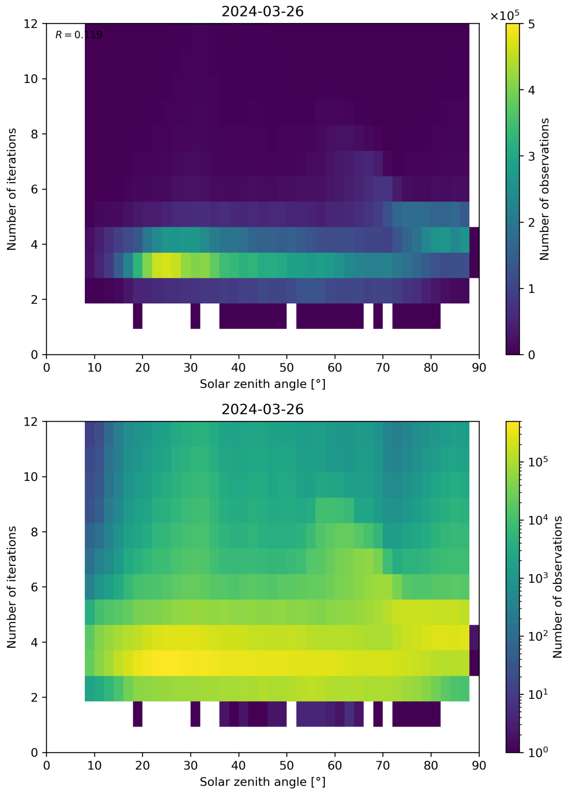
Figure 114: Scatter density plot of “Solar zenith angle” against “Number of iterations” for 2024-03-25 to 2024-03-27.
