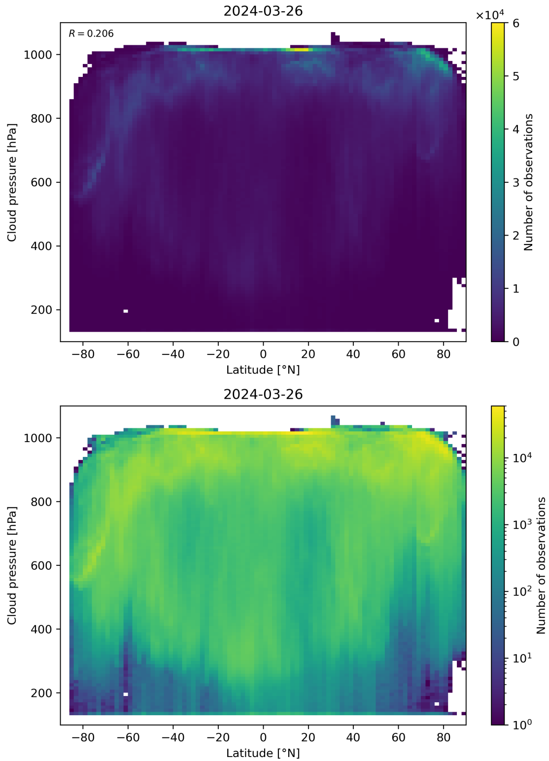
Figure 91: Scatter density plot of “Latitude” against “Cloud pressure” for 2024-03-25 to 2024-03-27.
