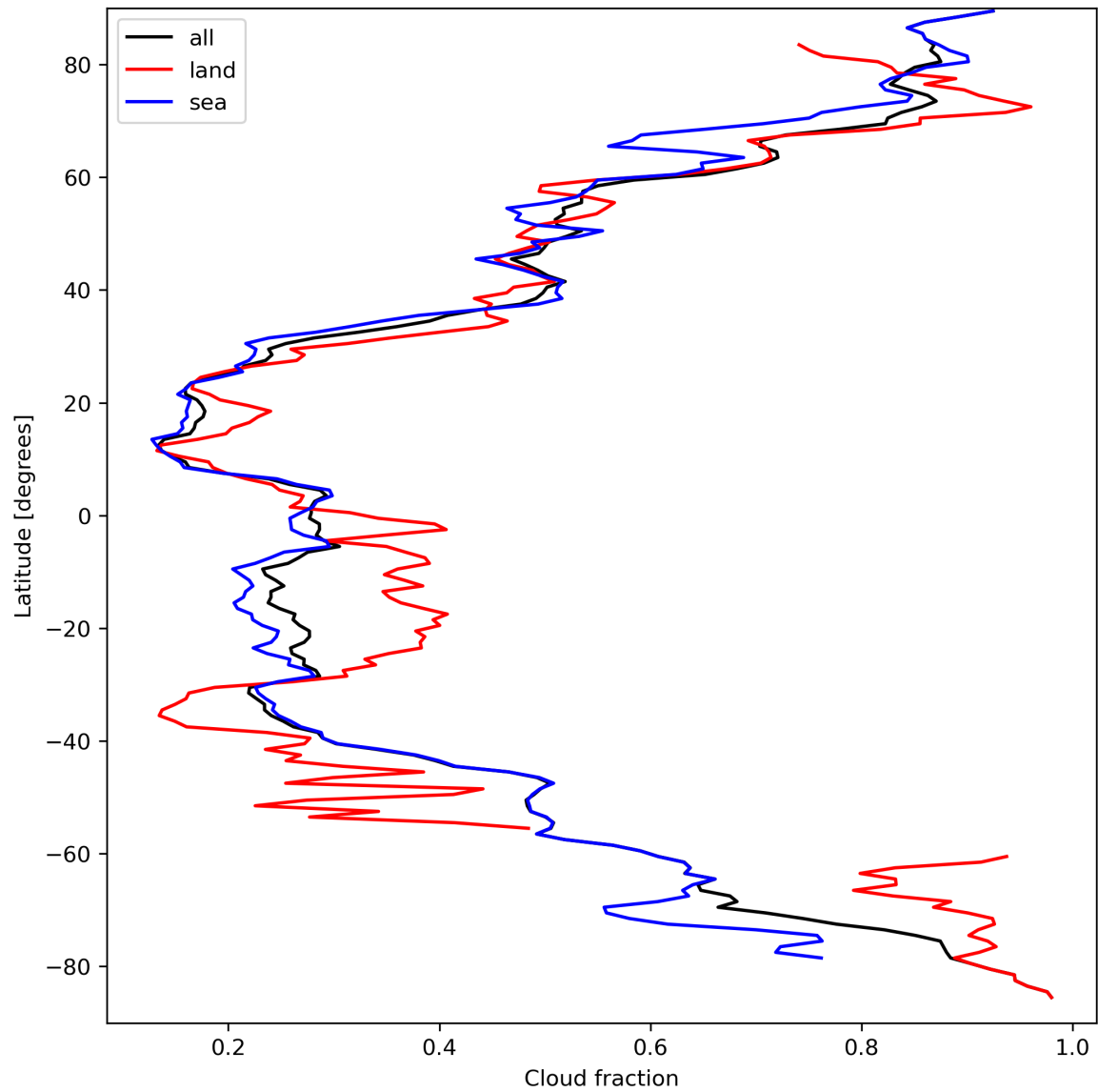
Figure 15: Zonal average of “Cloud fraction” for 2024-03-25 to 2024-03-27.
