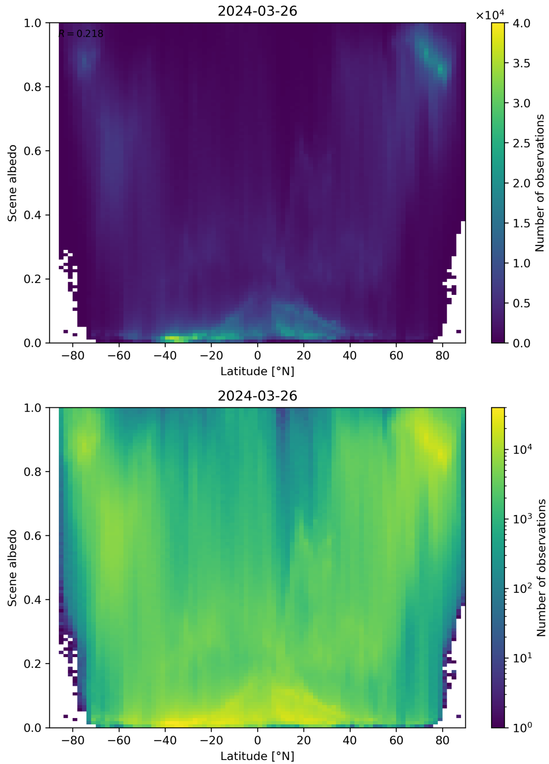
Figure 95: Scatter density plot of “Latitude” against “Scene albedo” for 2024-03-25 to 2024-03-27.
