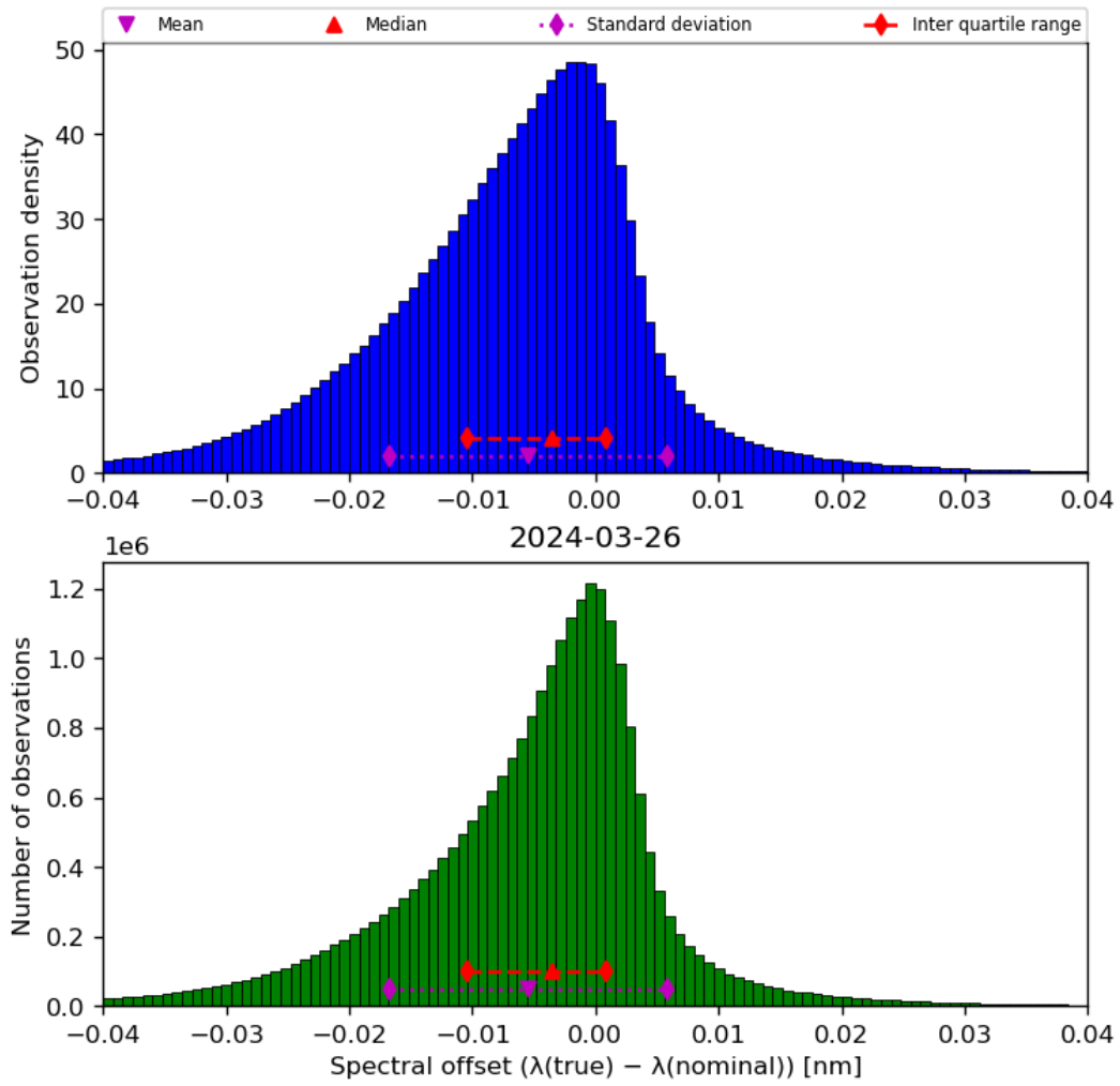
Figure 45: Histogram of “Spectral offset ( \lambda(\text{true}) - \lambda(\text{nominal}) )” for 2024-03-25 to 2024-03-27
