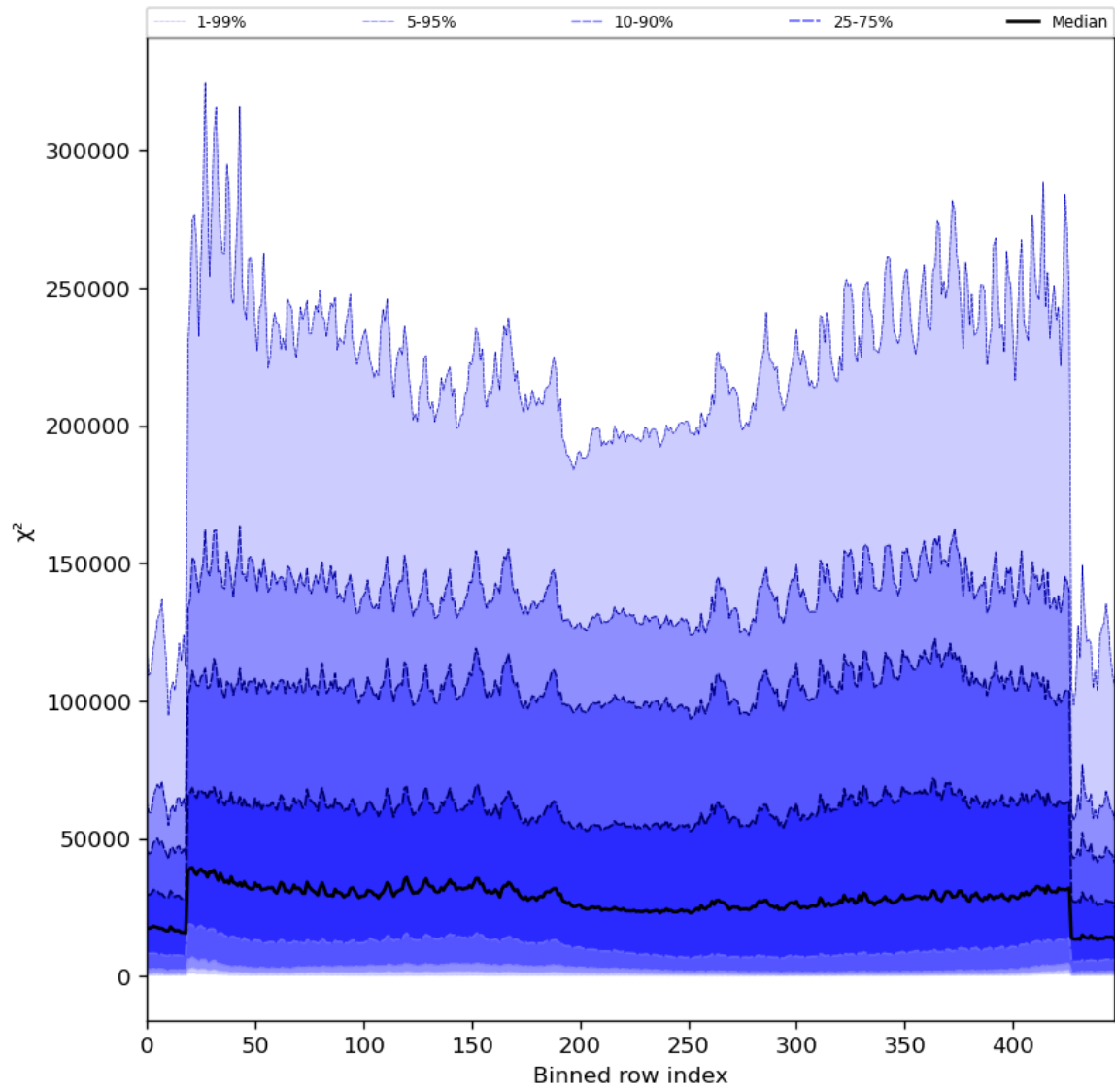
Figure 55: Along track statistics of “ \chi^2 ” for 2024-03-25 to 2024-03-27
