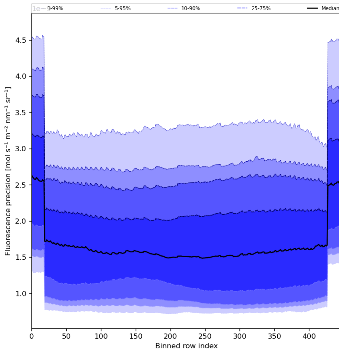
Figure 58: Along track statistics of “Fluorescence precision” for 2024-03-25 to 2024-03-27
