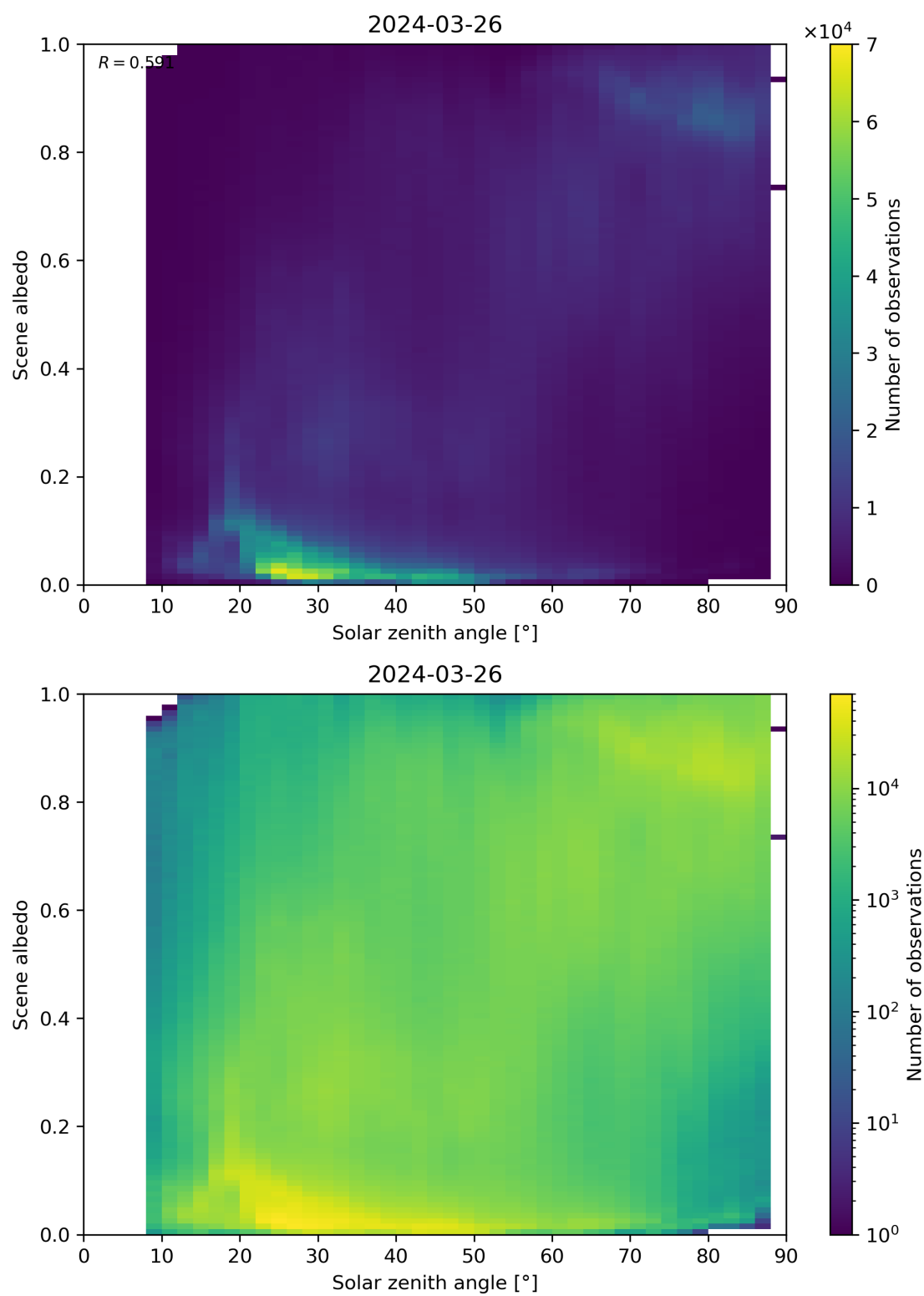
Figure 116: Scatter density plot of “Solar zenith angle” against “Scene albedo” for 2024-03-25 to 2024-03-27.
