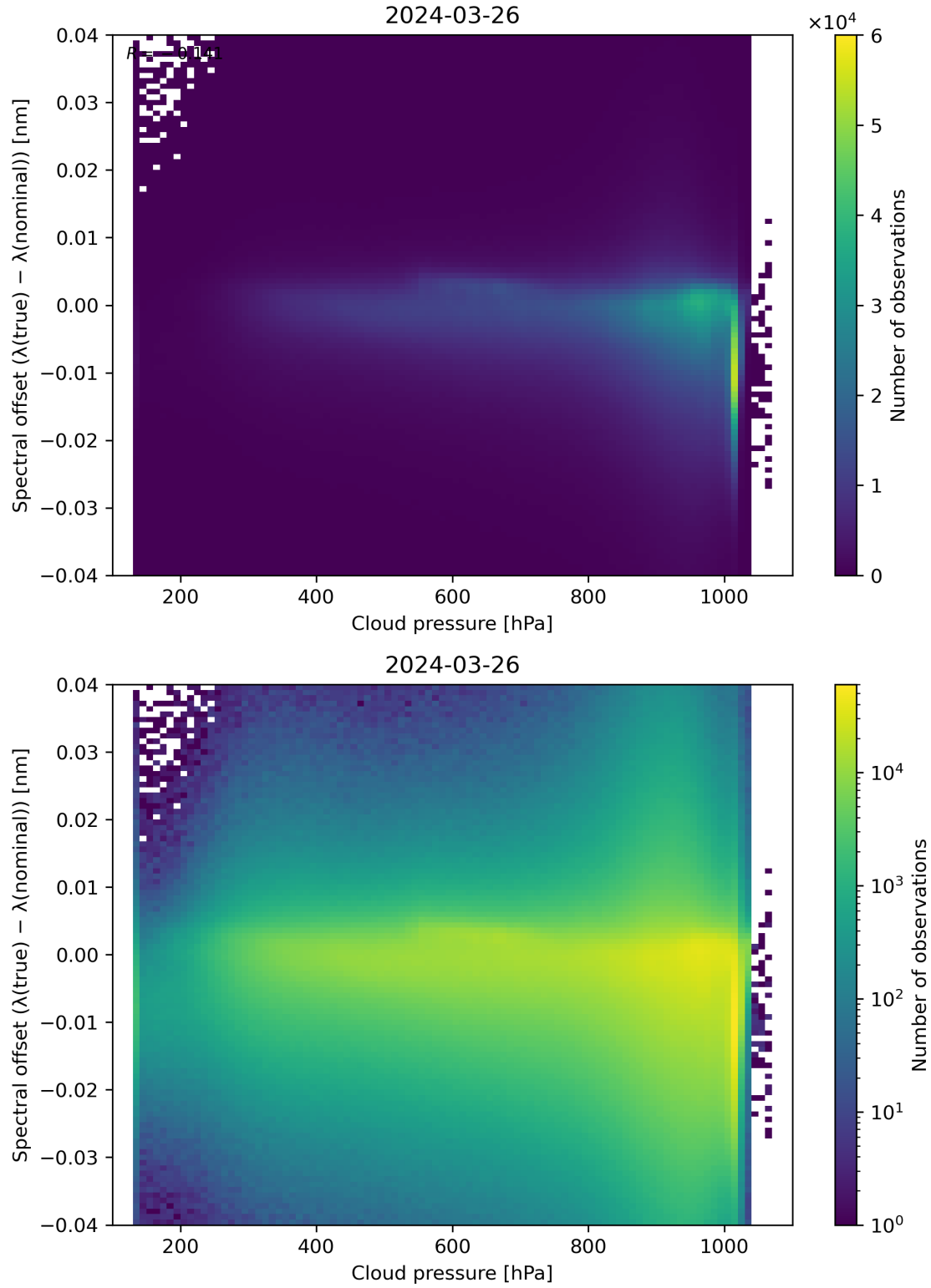
Figure 84: Scatter density plot of “Cloud pressure” against “Spectral offset ( \lambda(\text{true}) - \lambda(\text{nominal}) )” for 2024-03-25 to 2024-03-27.
