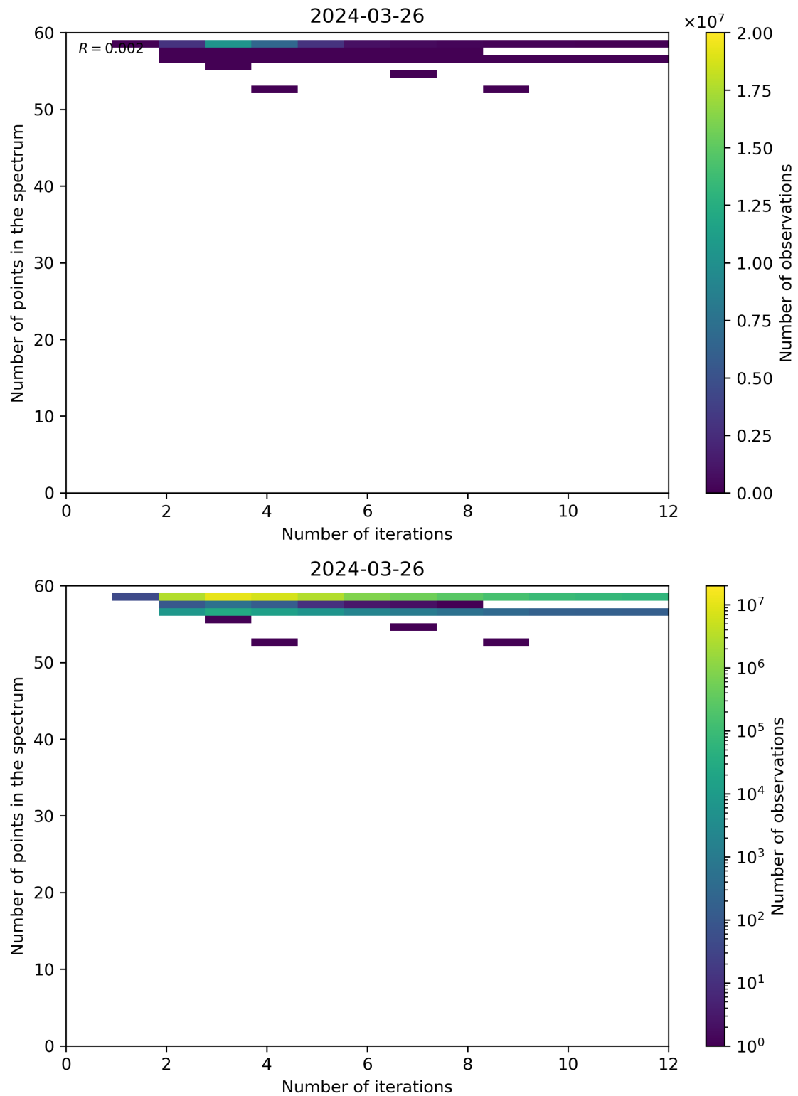
Figure 99: Scatter density plot of “Number of iterations” against “Number of points in the spectrum” for 2024-03-25 to 2024-03-27.
