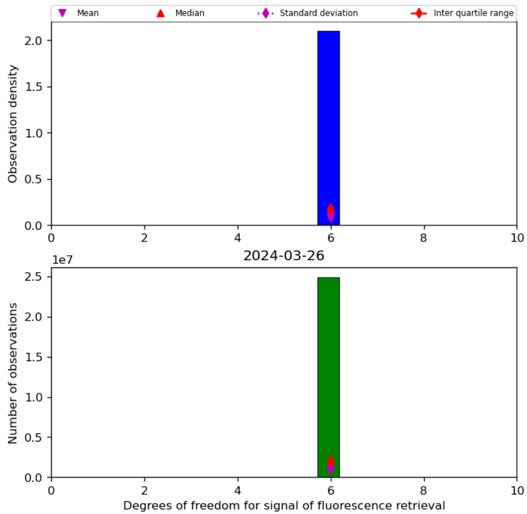
Figure 43: Histogram of “Degrees of freedom for signal of fluorescence retrieval” for 2024-03-25 to 2024-03-27
