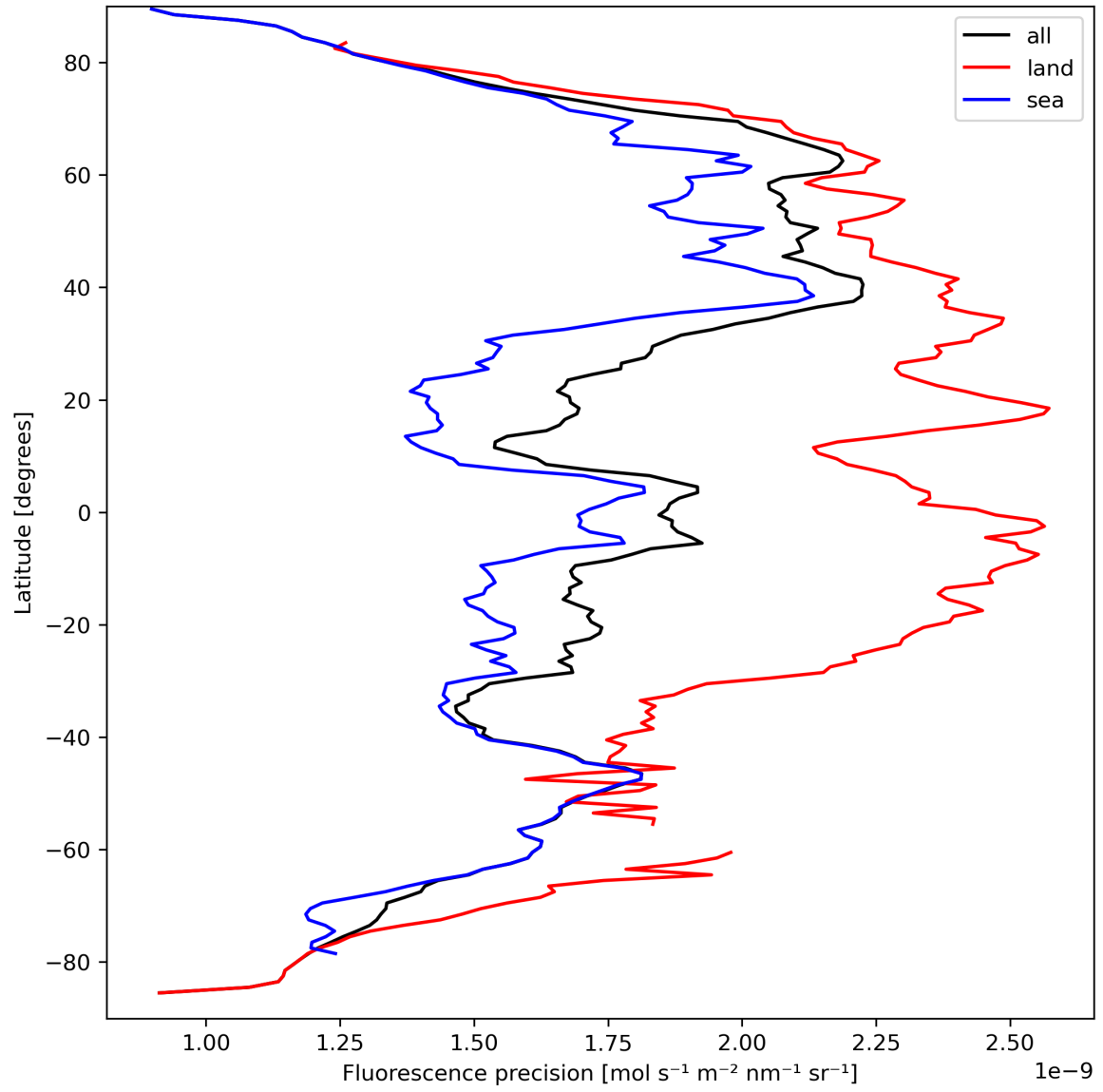
Figure 24: Zonal average of “Fluorescence precision” for 2024-03-25 to 2024-03-27.
