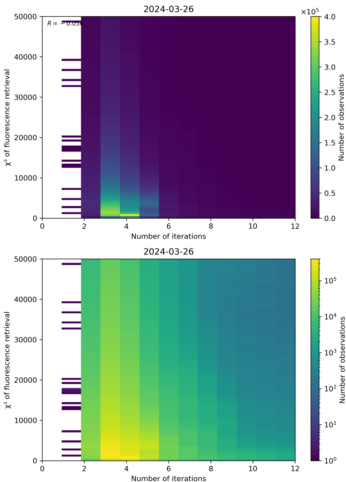
Figure 97: Scatter density plot of “Number of iterations” against “ \chi^2 of fluorescence retrieval” for 2024-03-25 to 2024-03-27.
