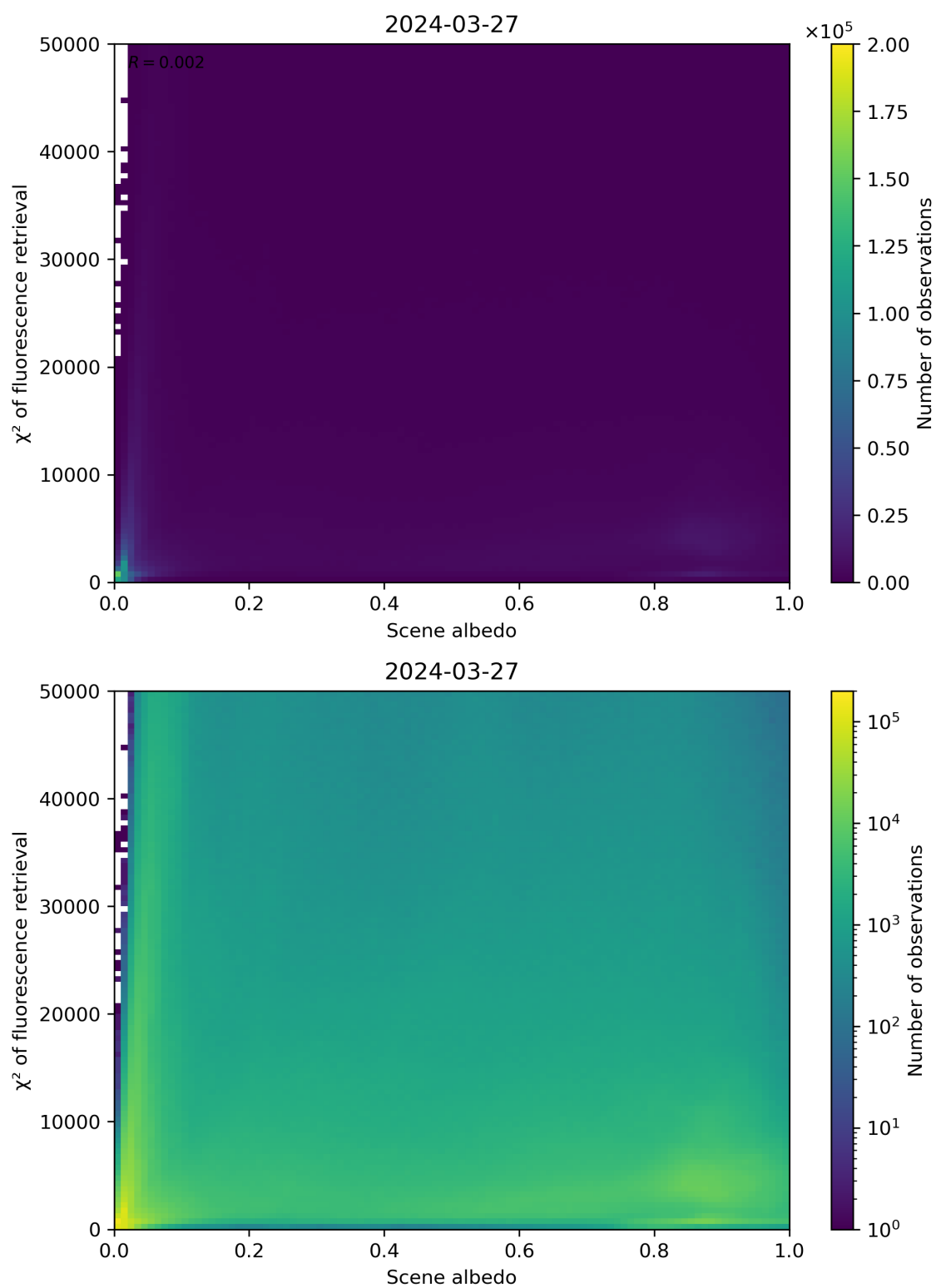
Figure 103: Scatter density plot of “Scene albedo” against “ \chi^2 of fluorescence retrieval” for 2024-03-26 to 2024-03-28.
