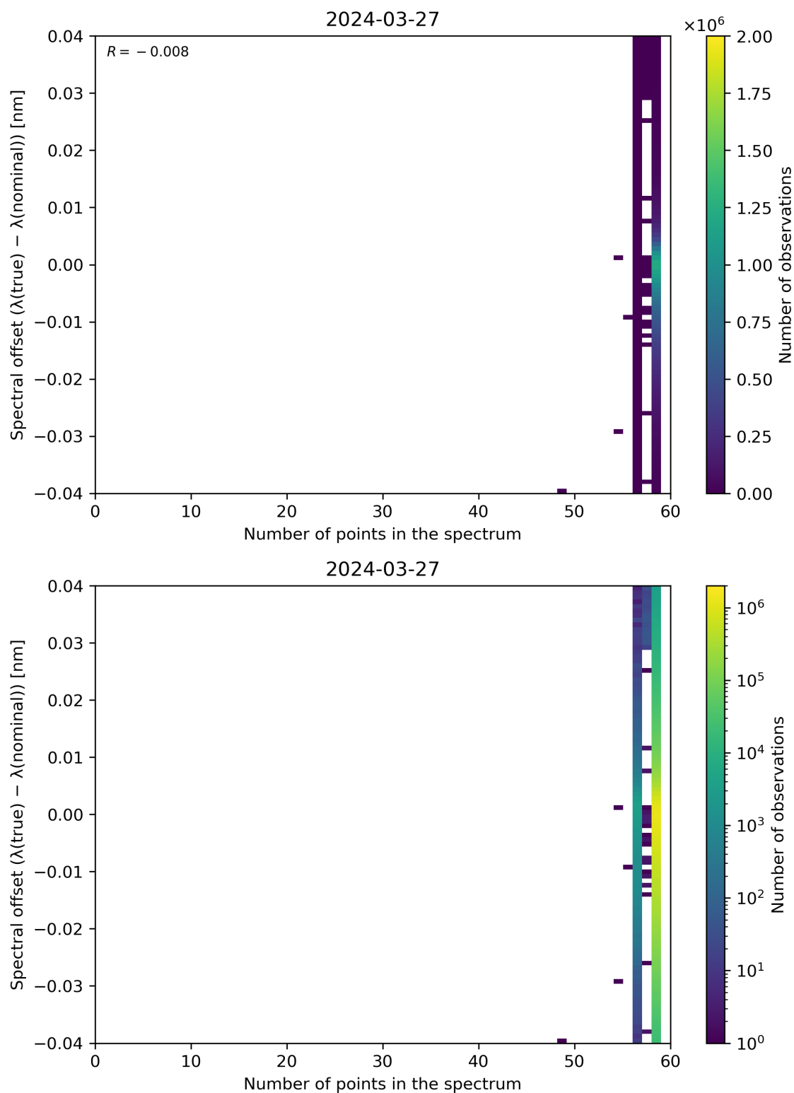
Figure 101: Scatter density plot of “Number of points in the spectrum” against “Spectral offset ( \lambda(\text{true}) - \lambda(\text{nominal}) )” for 2024-03-26 to 2024-03-28.
