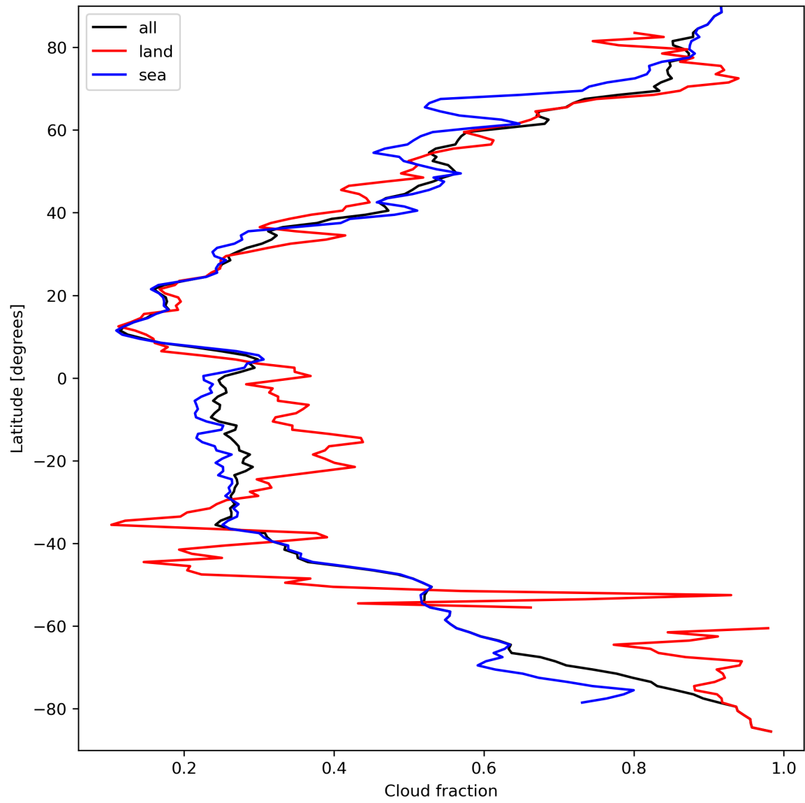
Figure 15: Zonal average of “Cloud fraction” for 2024-03-26 to 2024-03-28.
