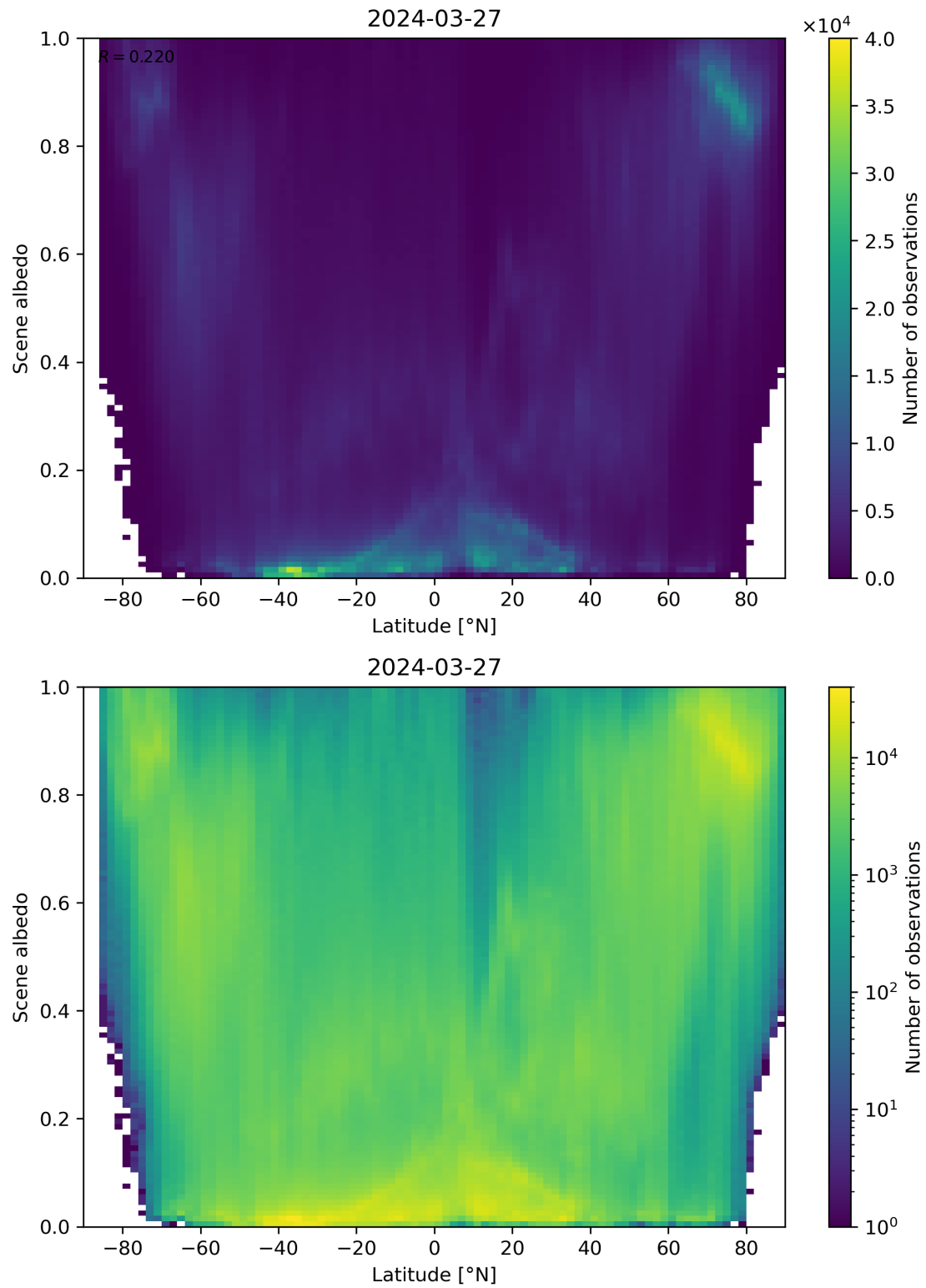
Figure 95: Scatter density plot of “Latitude” against “Scene albedo” for 2024-03-26 to 2024-03-28.
