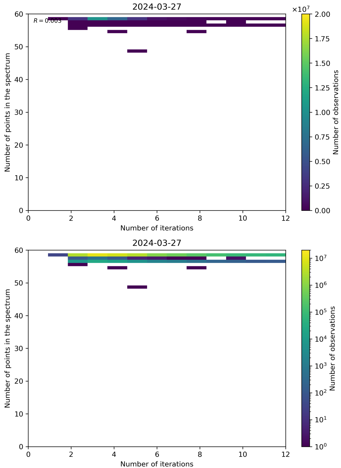
Figure 99: Scatter density plot of “Number of iterations” against “Number of points in the spectrum” for 2024-03-26 to 2024-03-28.
