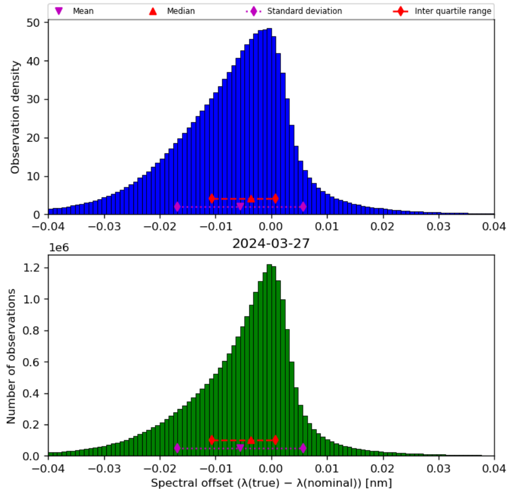
Figure 45: Histogram of “Spectral offset ( \lambda(\text{true}) - \lambda(\text{nominal}) )” for 2024-03-26 to 2024-03-28
