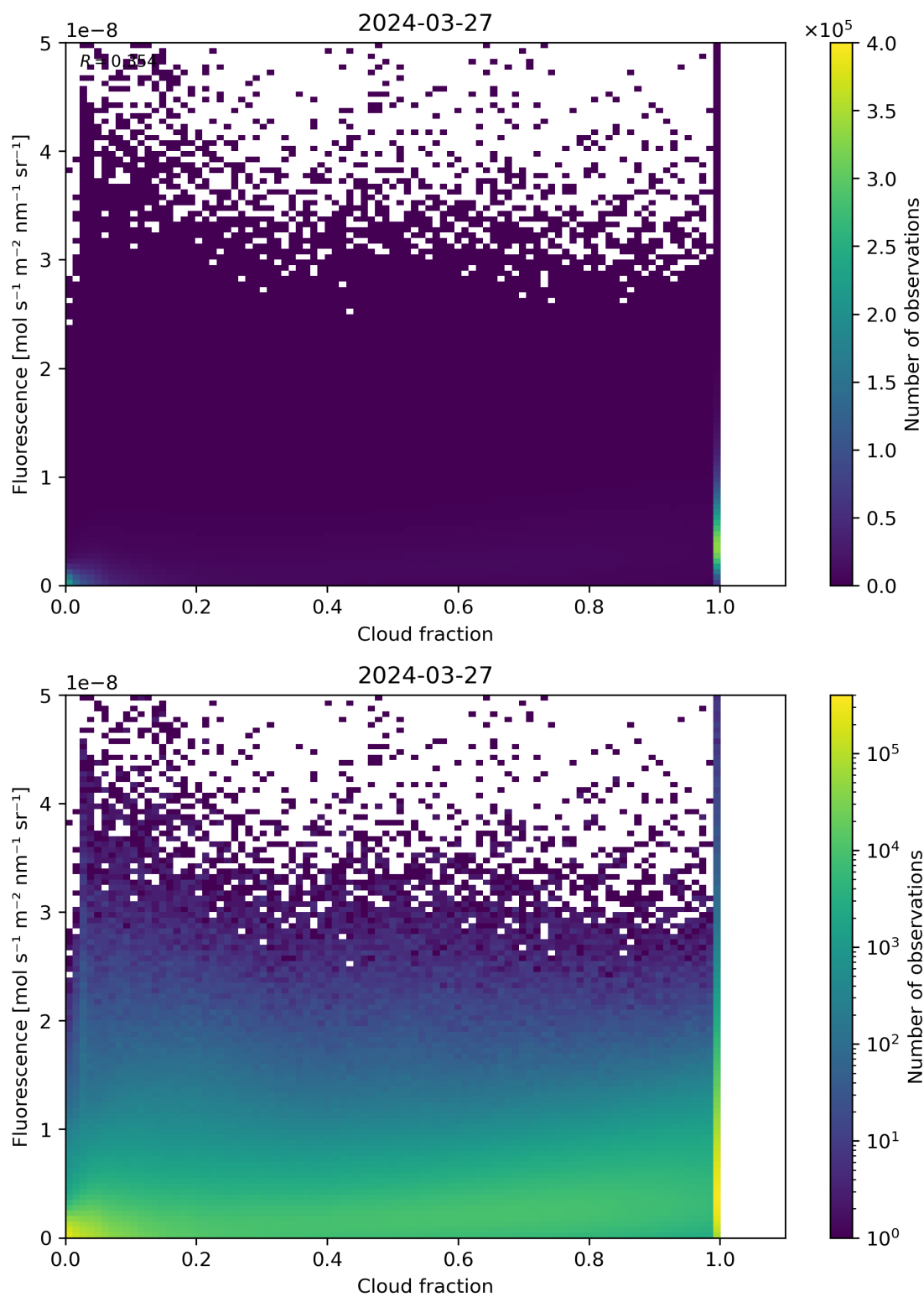
Figure 72: Scatter density plot of “Cloud fraction” against “Fluorescence” for 2024-03-26 to 2024-03-28.
