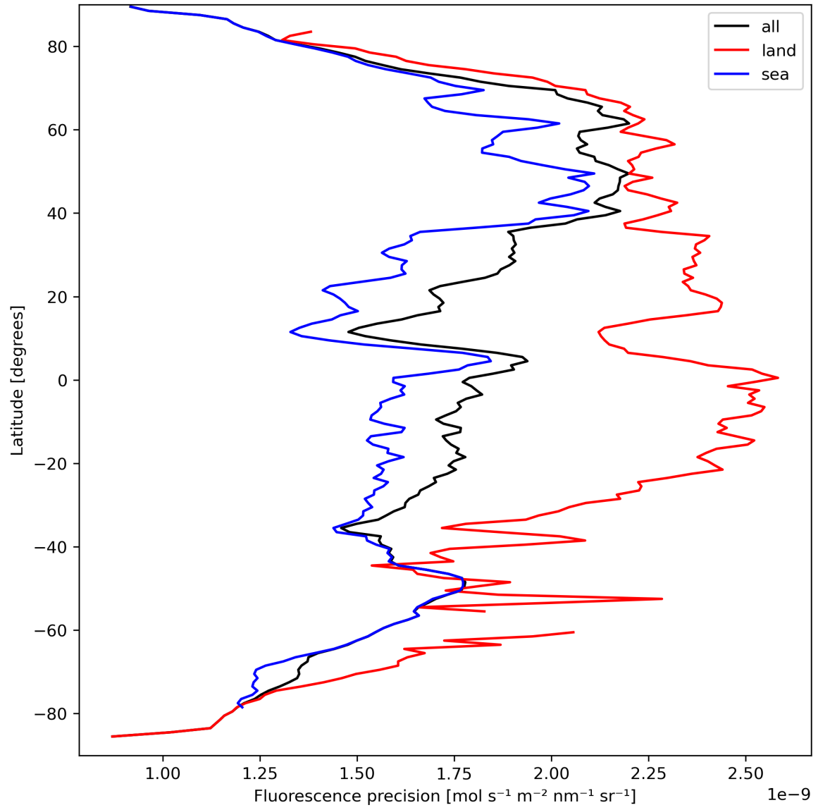
Figure 24: Zonal average of “Fluorescence precision” for 2024-03-26 to 2024-03-28.
