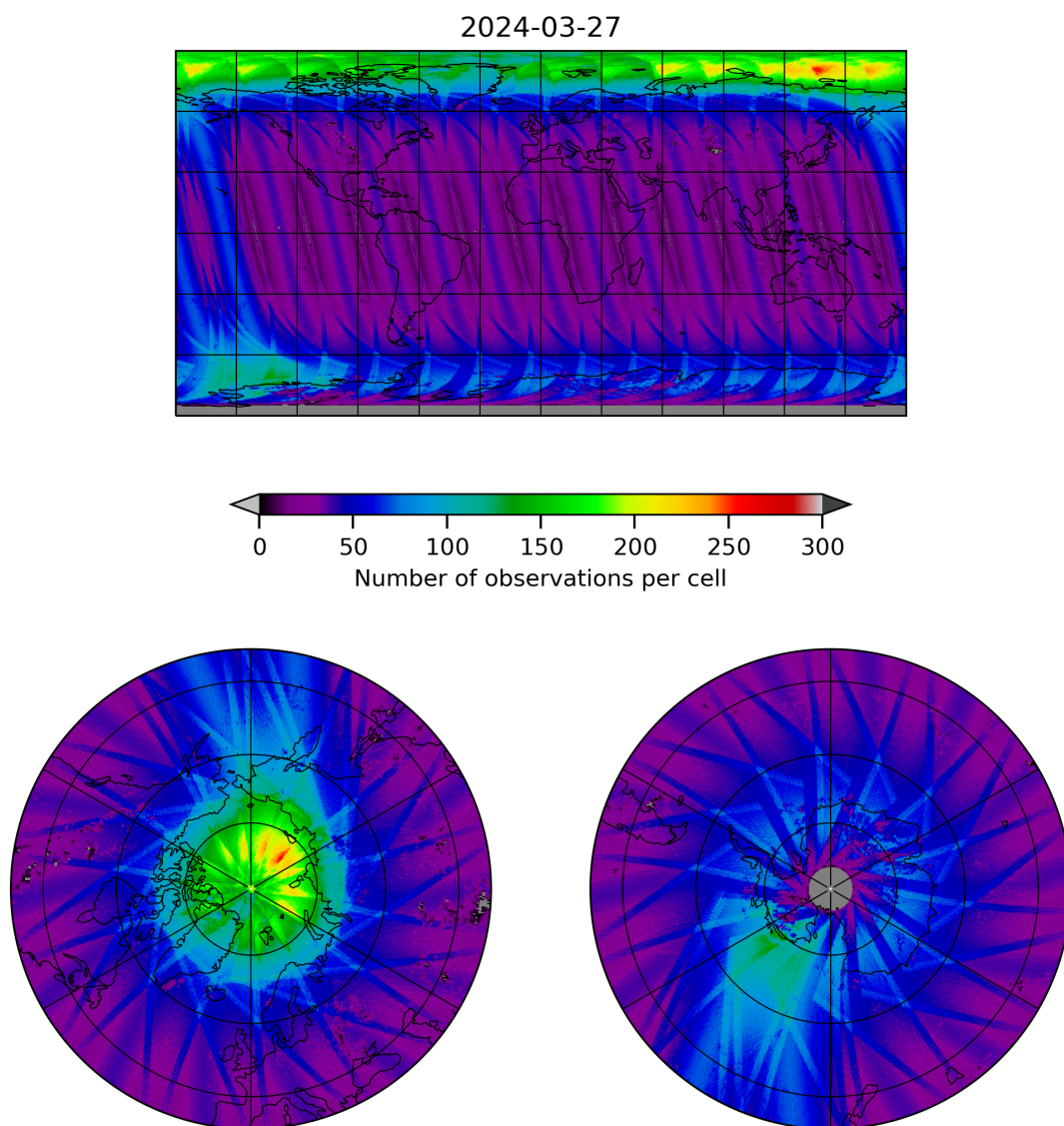
Figure 11: Map of the number of observations for 2024-03-26 to 2024-03-28
