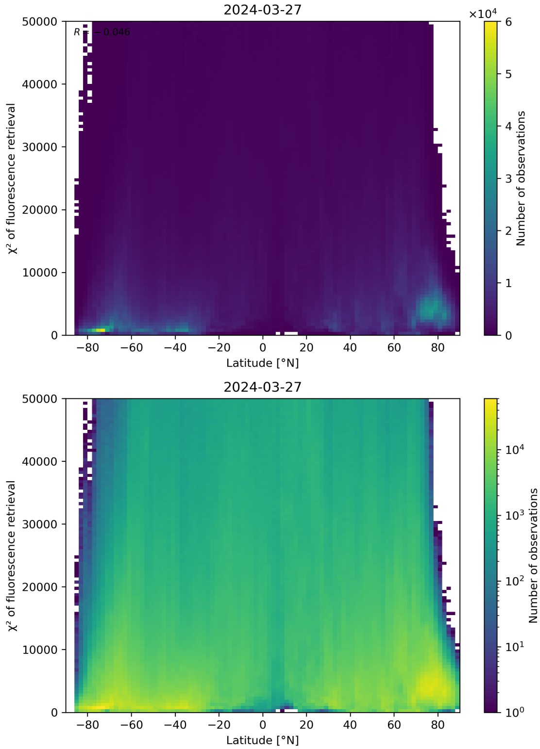
Figure 89: Scatter density plot of “Latitude” against “ \chi^2 of fluorescence retrieval” for 2024-03-26 to 2024-03-28.
