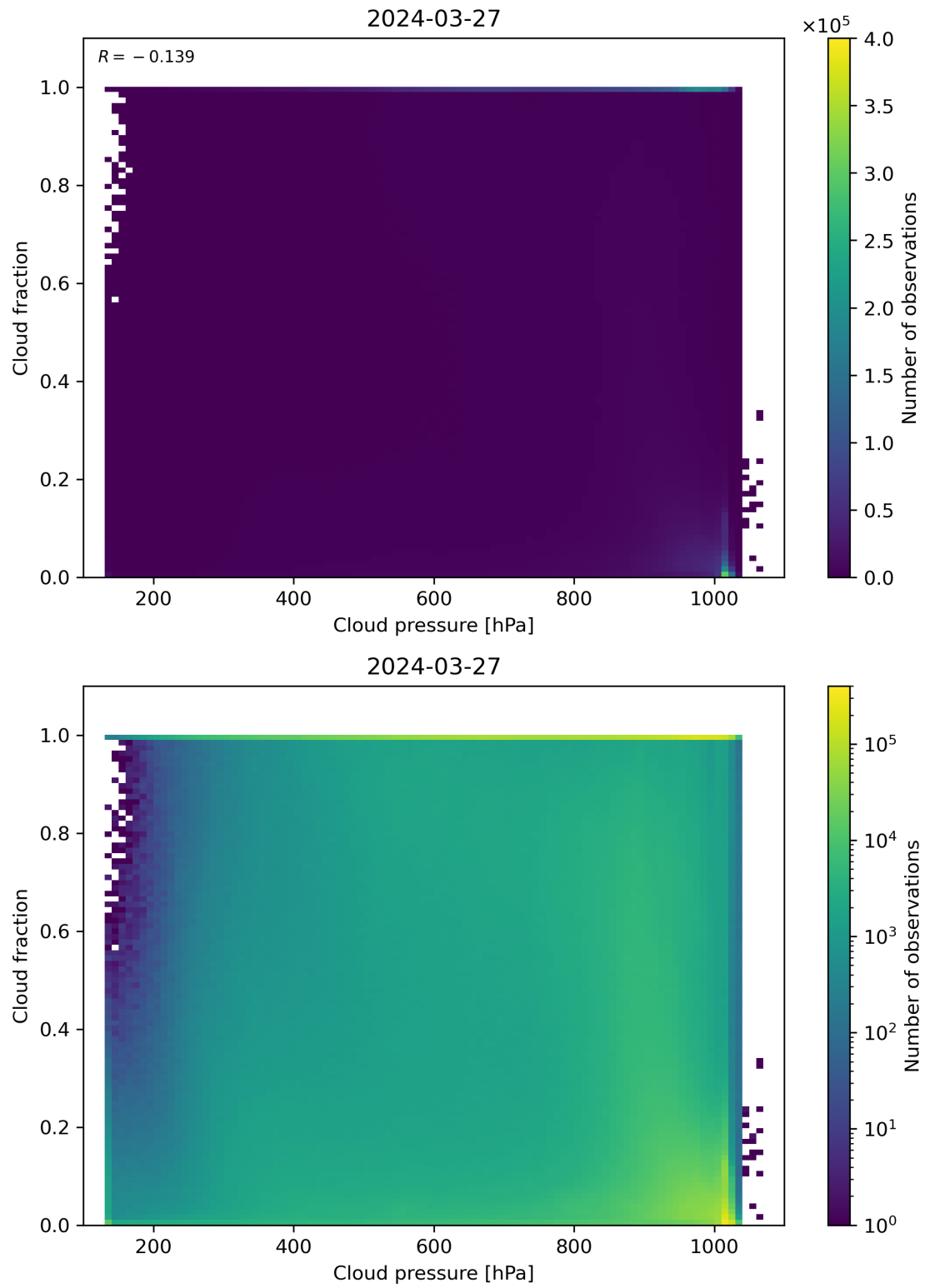
Figure 79: Scatter density plot of “Cloud pressure” against “Cloud fraction” for 2024-03-26 to 2024-03-28.
