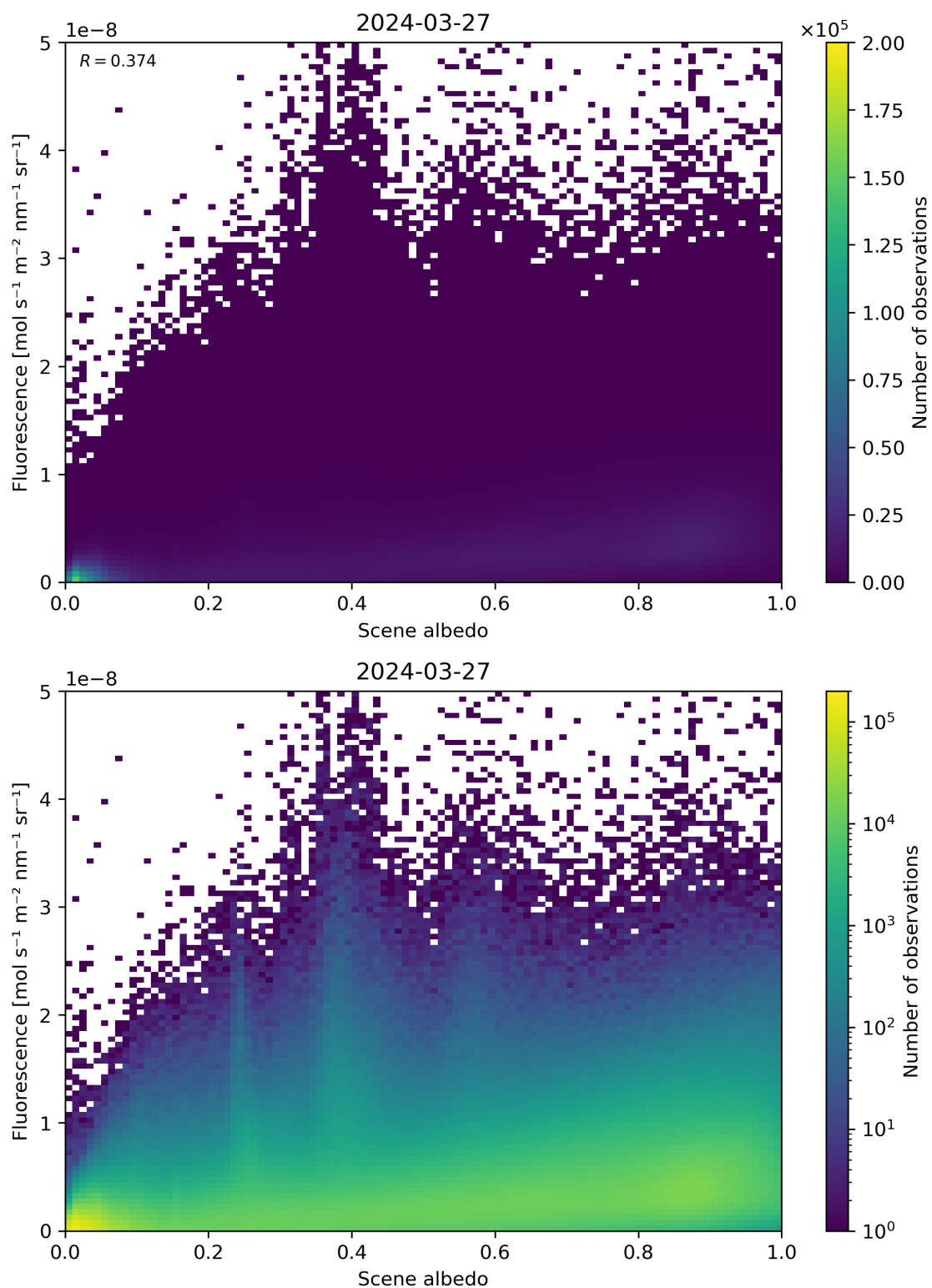
Figure 104: Scatter density plot of “Scene albedo” against “Fluorescence” for 2024-03-26 to 2024-03-28.
