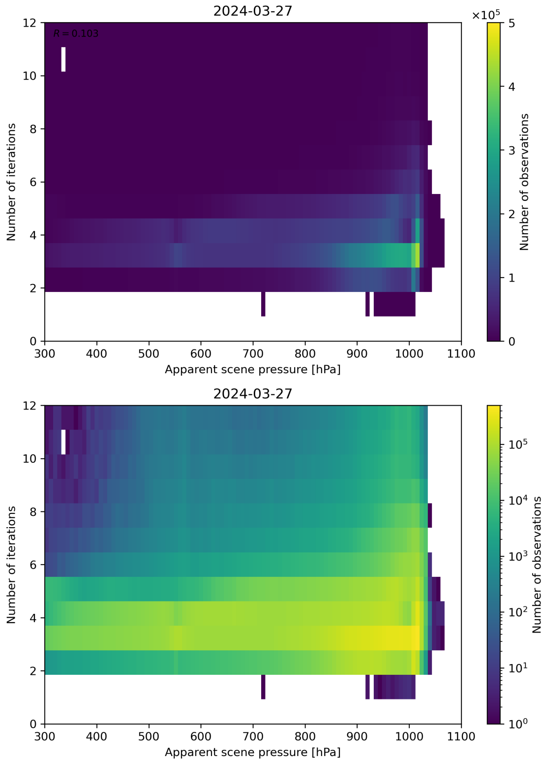
Figure 65: Scatter density plot of “Apparent scene pressure” against “Number of iterations” for 2024-03-26 to 2024-03-28.
