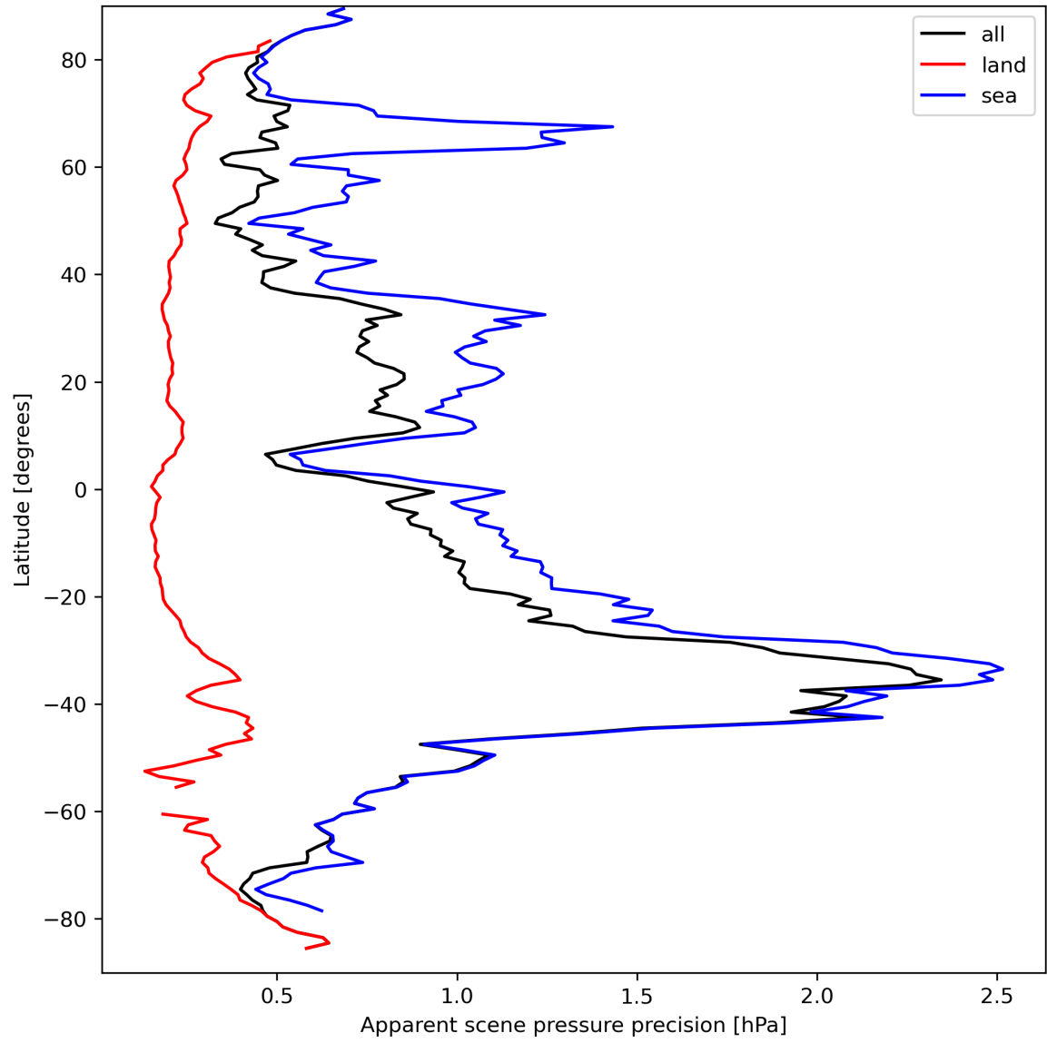
Figure 20: Zonal average of “Apparent scene pressure precision” for 2024-03-26 to 2024-03-28.
