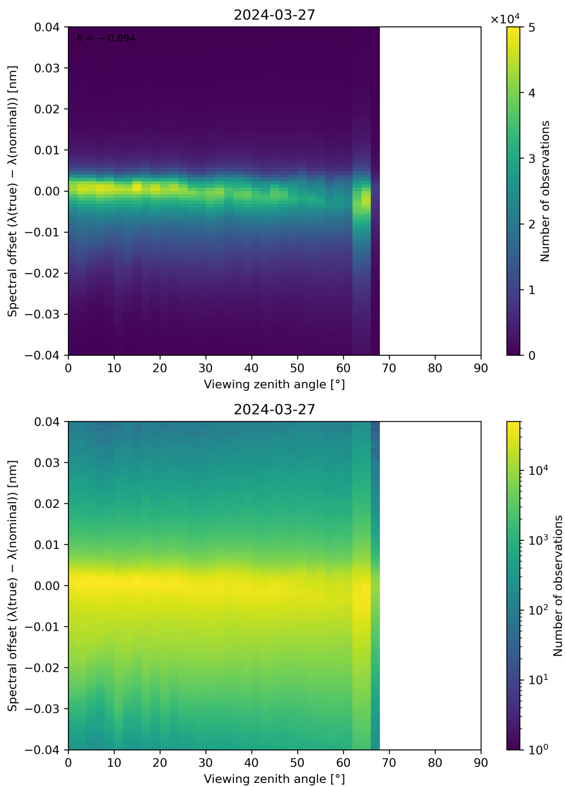
Figure 128: Scatter density plot of “Viewing zenith angle” against “Spectral offset ( \lambda(\text{true}) - \lambda(\text{nominal}) )” for 2024-03-26 to 2024-03-28.
