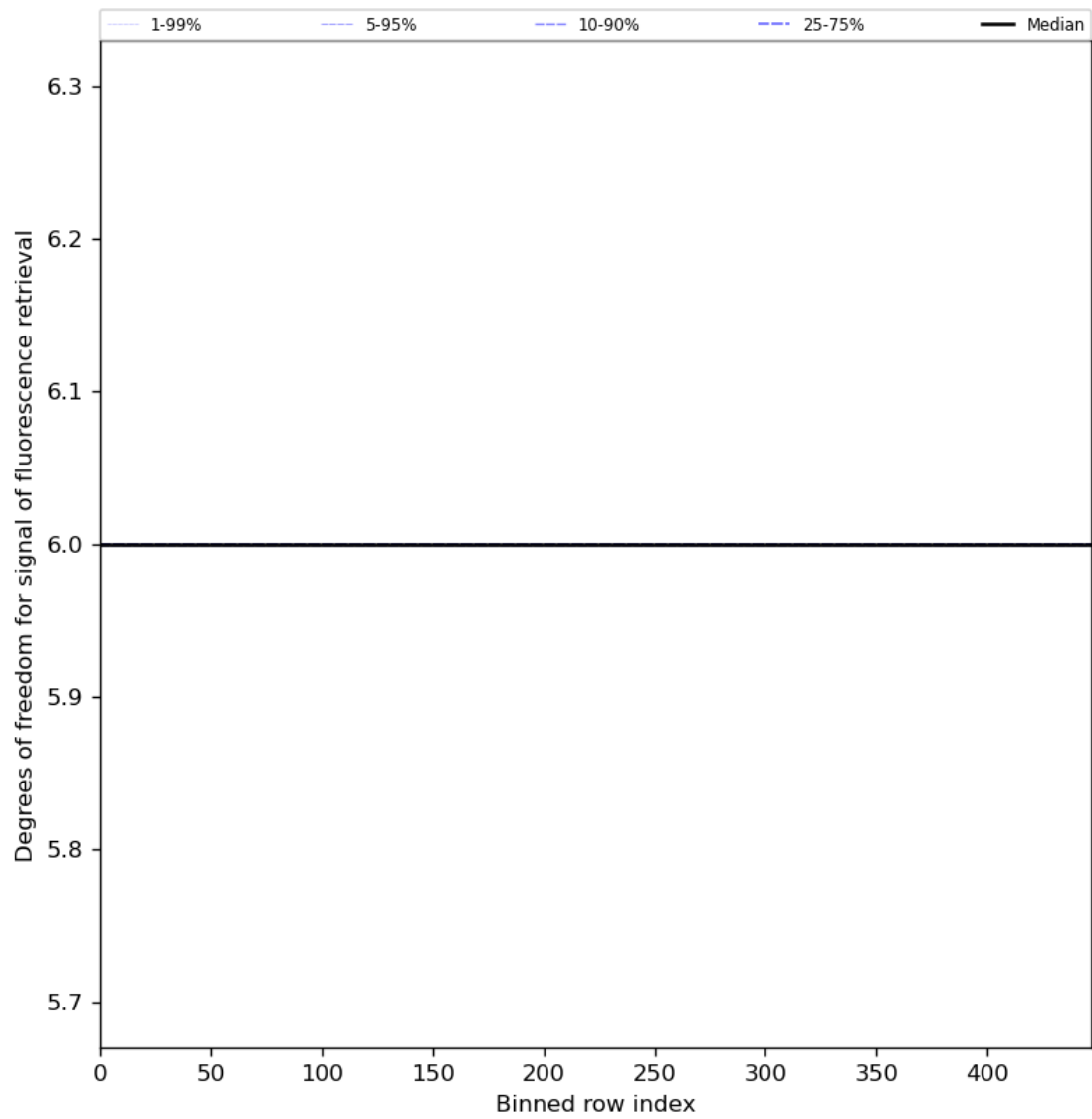
Figure 60: Along track statistics of “Degrees of freedom for signal of fluorescence retrieval” for 2024-03-26 to 2024-03-28
