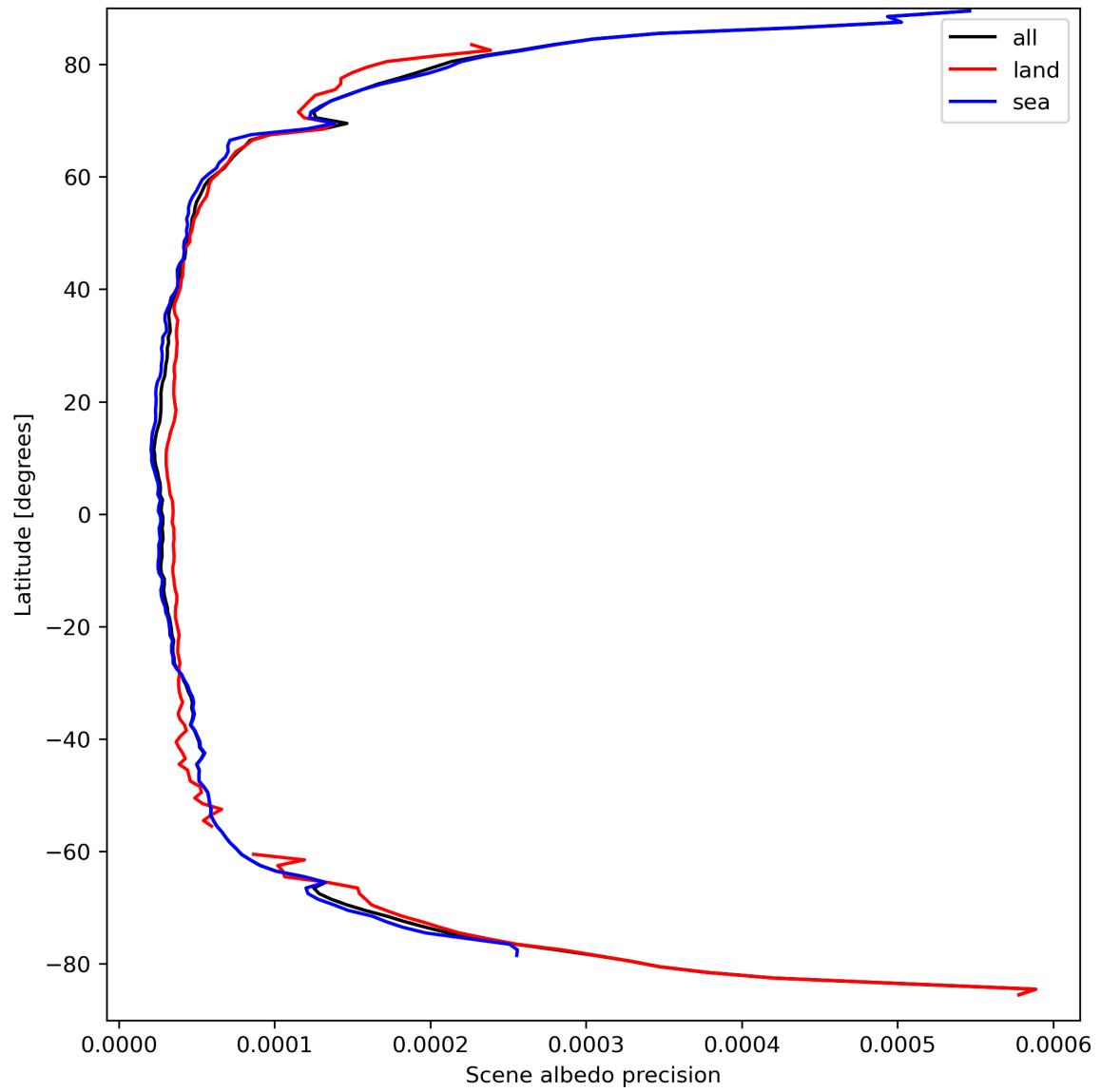
Figure 18: Zonal average of “Scene albedo precision” for 2024-03-26 to 2024-03-28.
