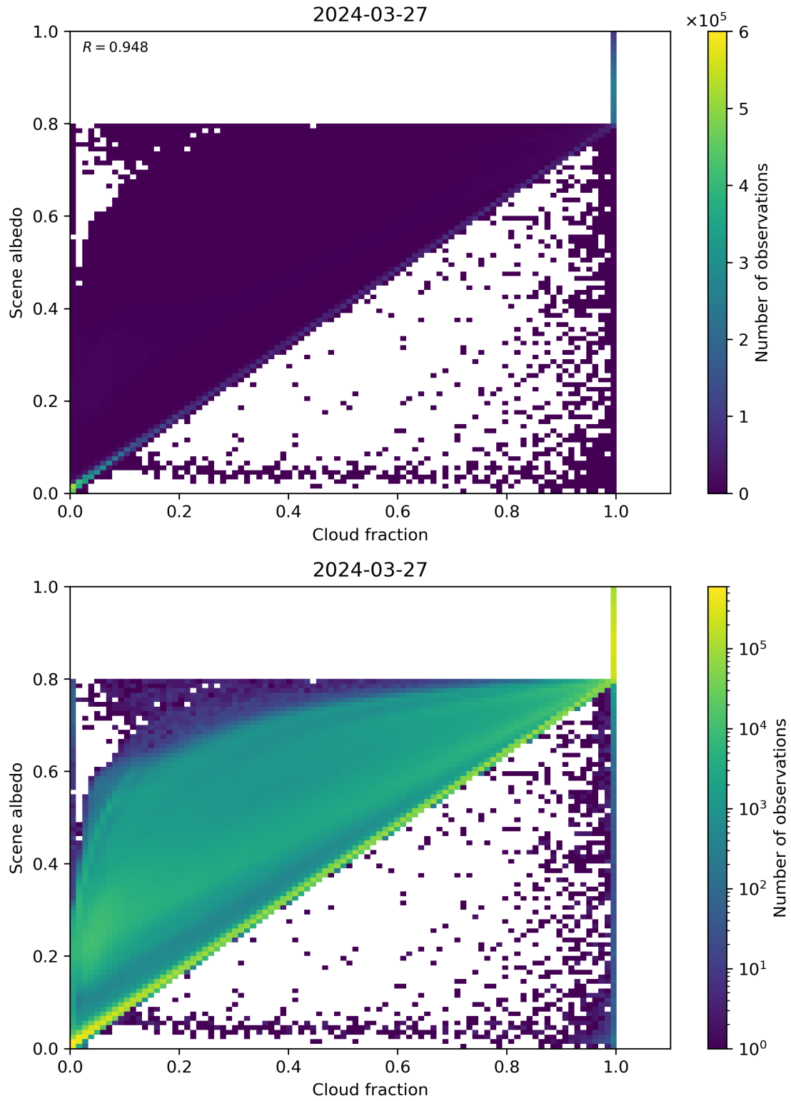
Figure 75: Scatter density plot of “Cloud fraction” against “Scene albedo” for 2024-03-26 to 2024-03-28.
