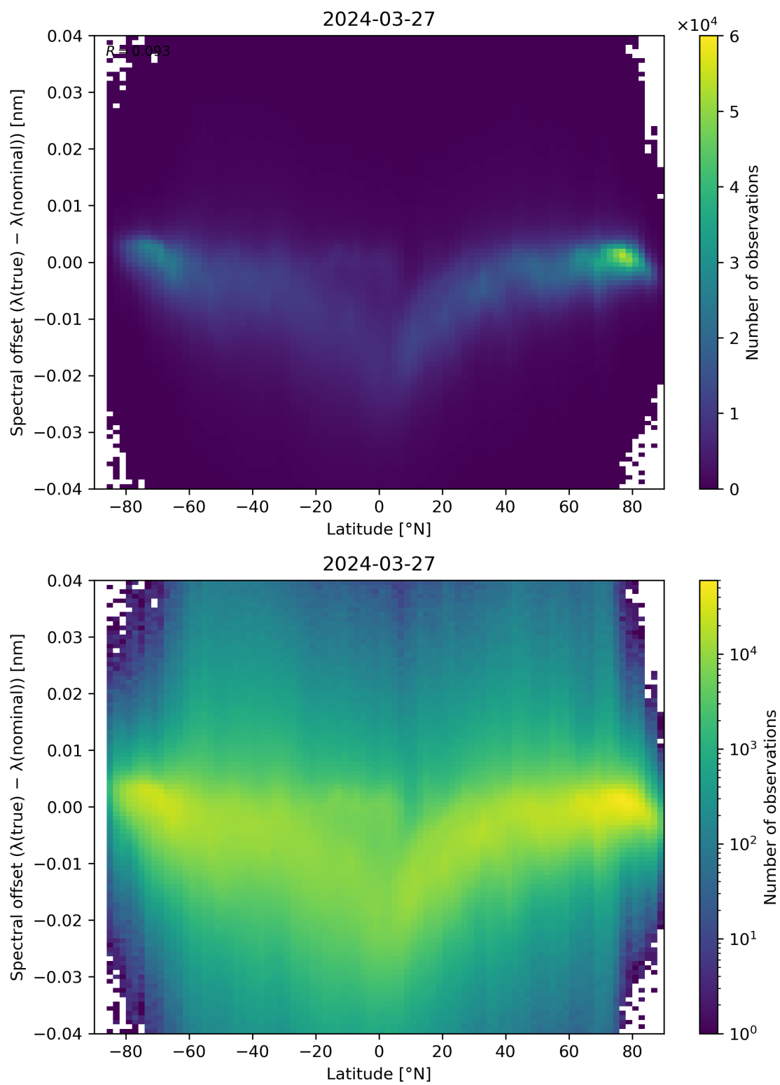
Figure 96: Scatter density plot of “Latitude” against “Spectral offset ( \lambda(\text{true}) - \lambda(\text{nominal}) )” for 2024-03-26 to 2024-03-28.
