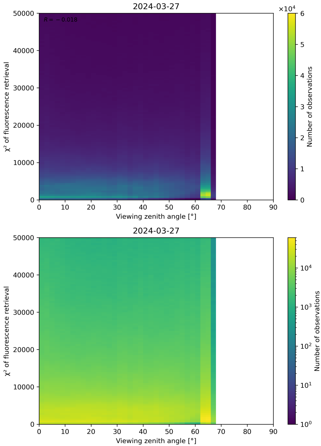
Figure 119: Scatter density plot of “Viewing zenith angle” against “ \chi^2 of fluorescence retrieval” for 2024-03-26 to 2024-03-28.
