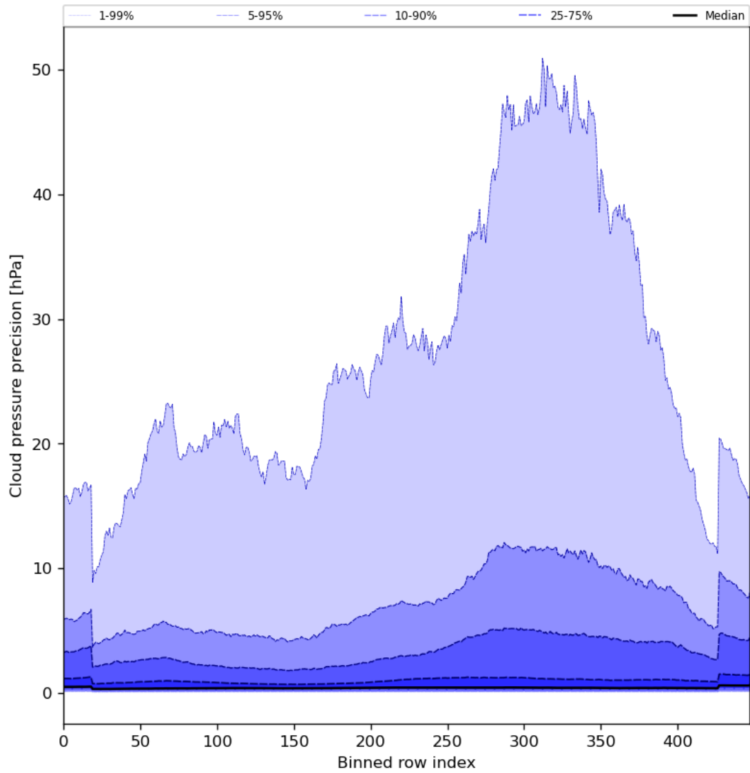
Figure 48: Along track statistics of “Cloud pressure precision” for 2024-03-26 to 2024-03-28
