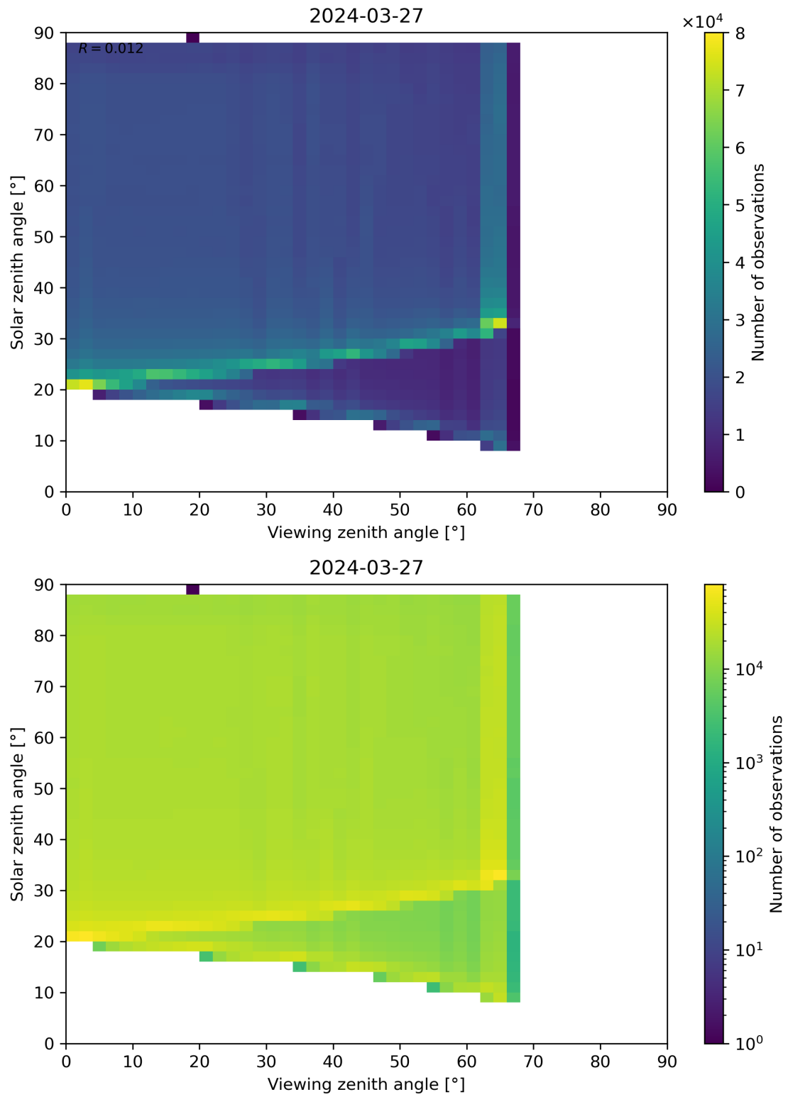
Figure 127: Scatter density plot of “Viewing zenith angle” against “Solar zenith angle” for 2024-03-26 to 2024-03-28.
