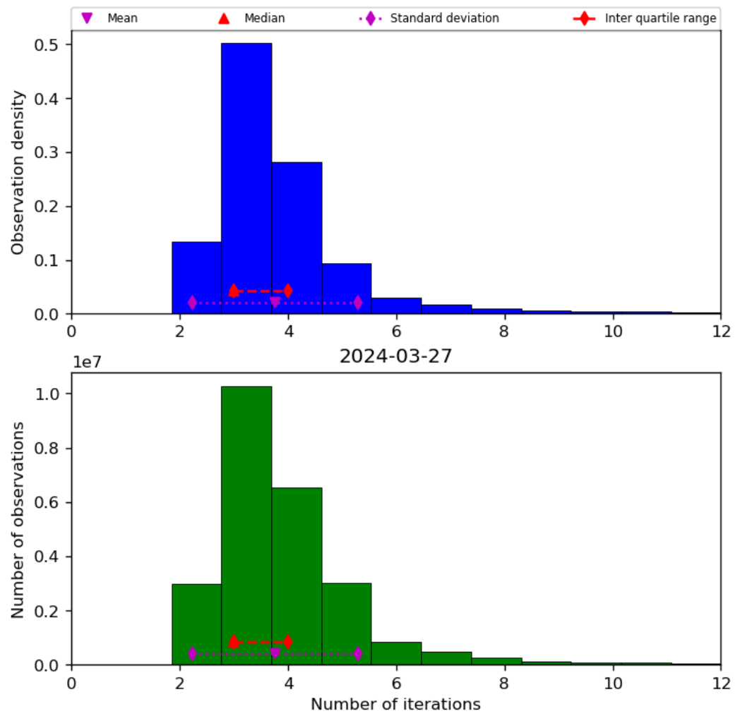
Figure 39: Histogram of “Number of iterations” for 2024-03-26 to 2024-03-28
