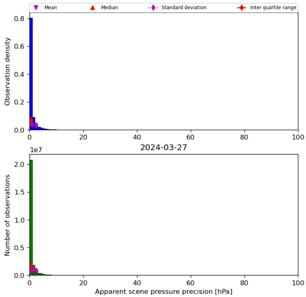
Figure 37: Histogram of “Apparent scene pressure precision” for 2024-03-26 to 2024-03-28
