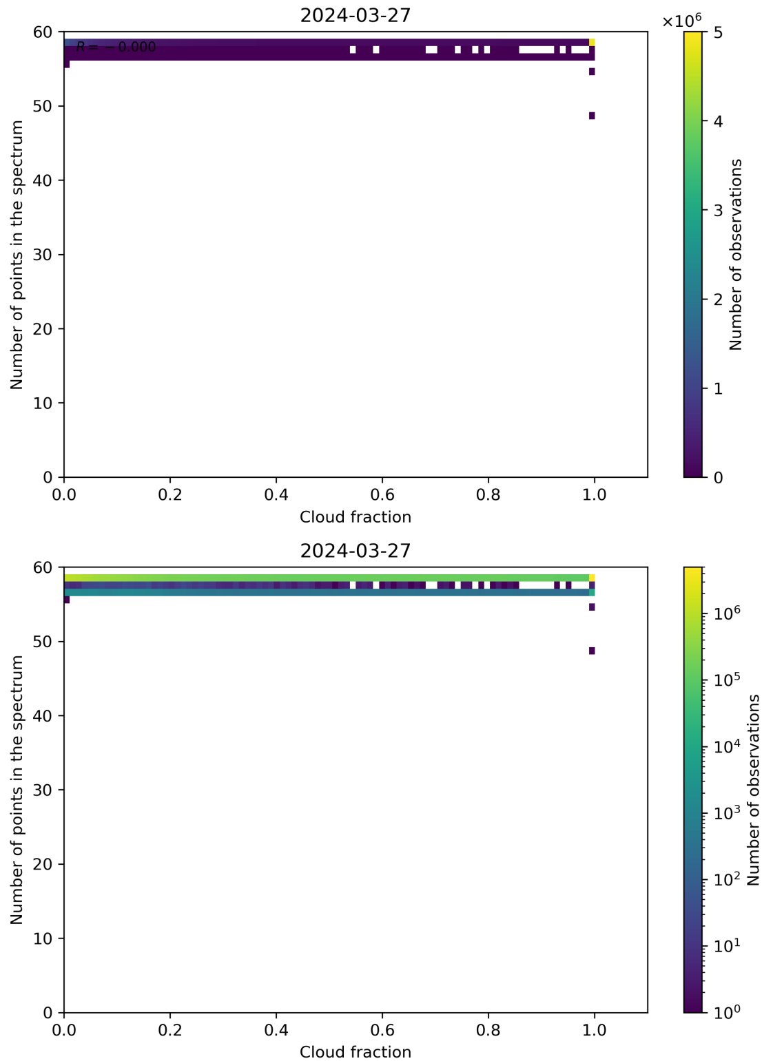
Figure 74: Scatter density plot of “Cloud fraction” against “Number of points in the spectrum” for 2024-03-26 to 2024-03-28.
