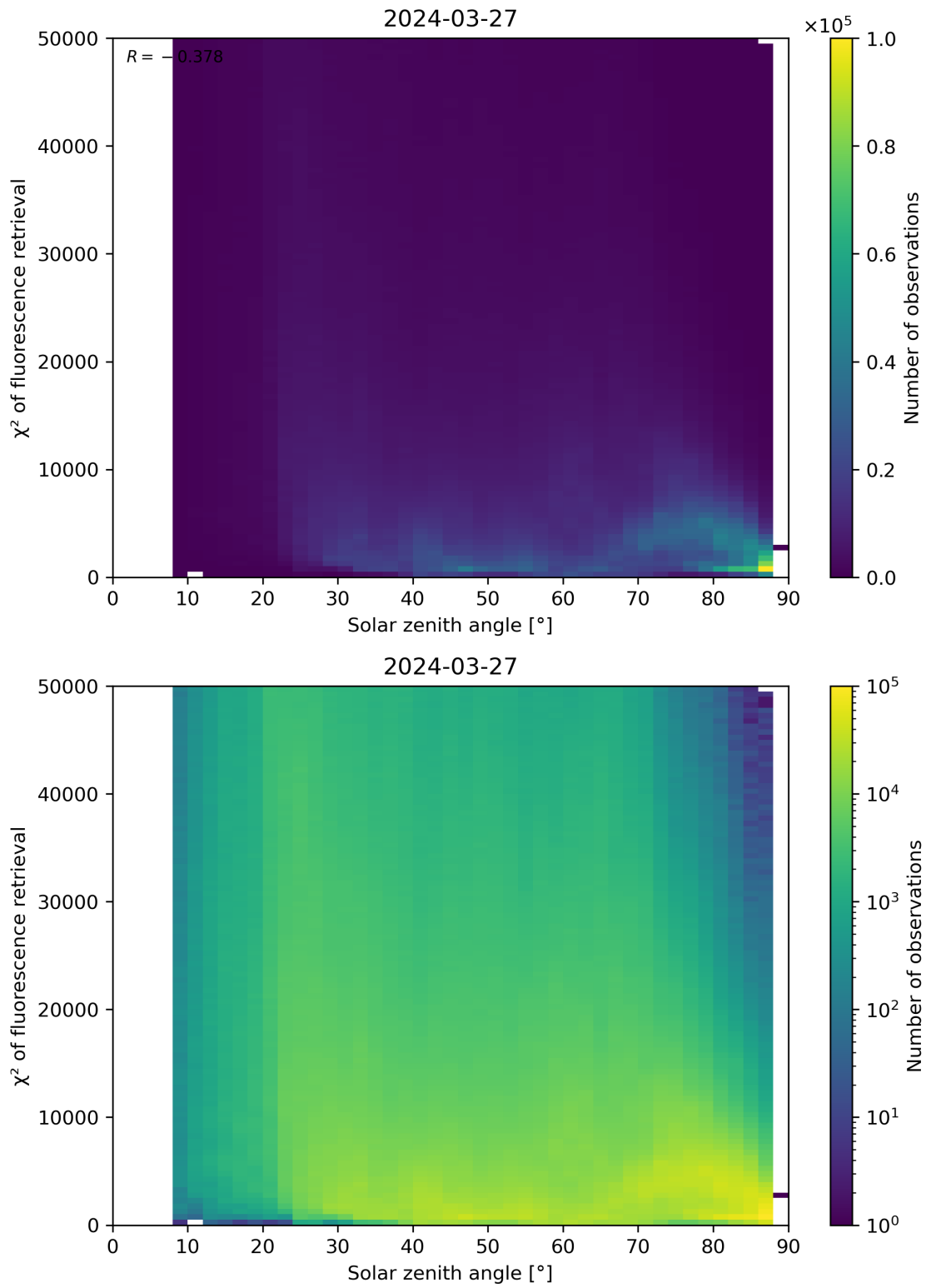
Figure 109: Scatter density plot of “Solar zenith angle” against “ \chi^2 of fluorescence retrieval” for 2024-03-26 to 2024-03-28.
