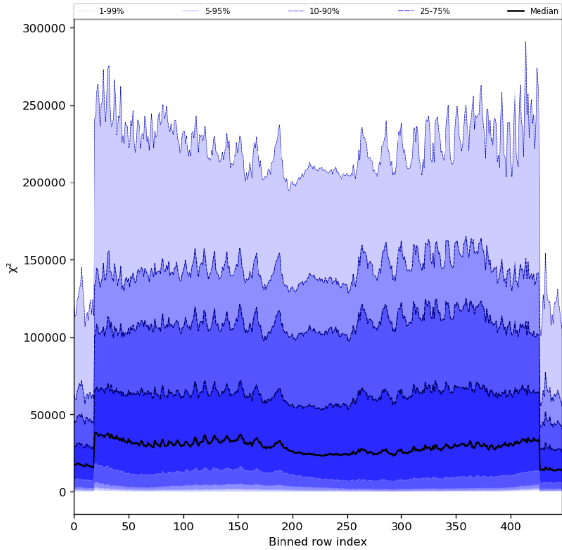
Figure 55: Along track statistics of “ \chi^2 ” for 2024-03-26 to 2024-03-28
