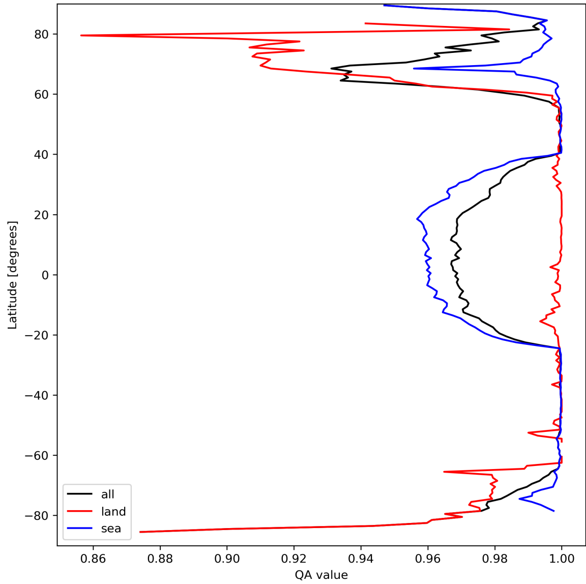
Figure 12: Zonal average of “QA value” for 2024-03-26 to 2024-03-28.
