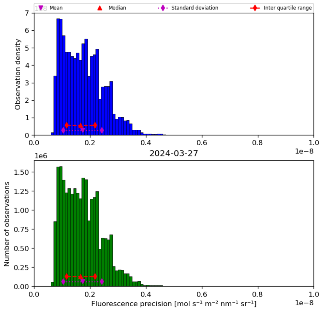
Figure 41: Histogram of “Fluorescence precision” for 2024-03-26 to 2024-03-28
