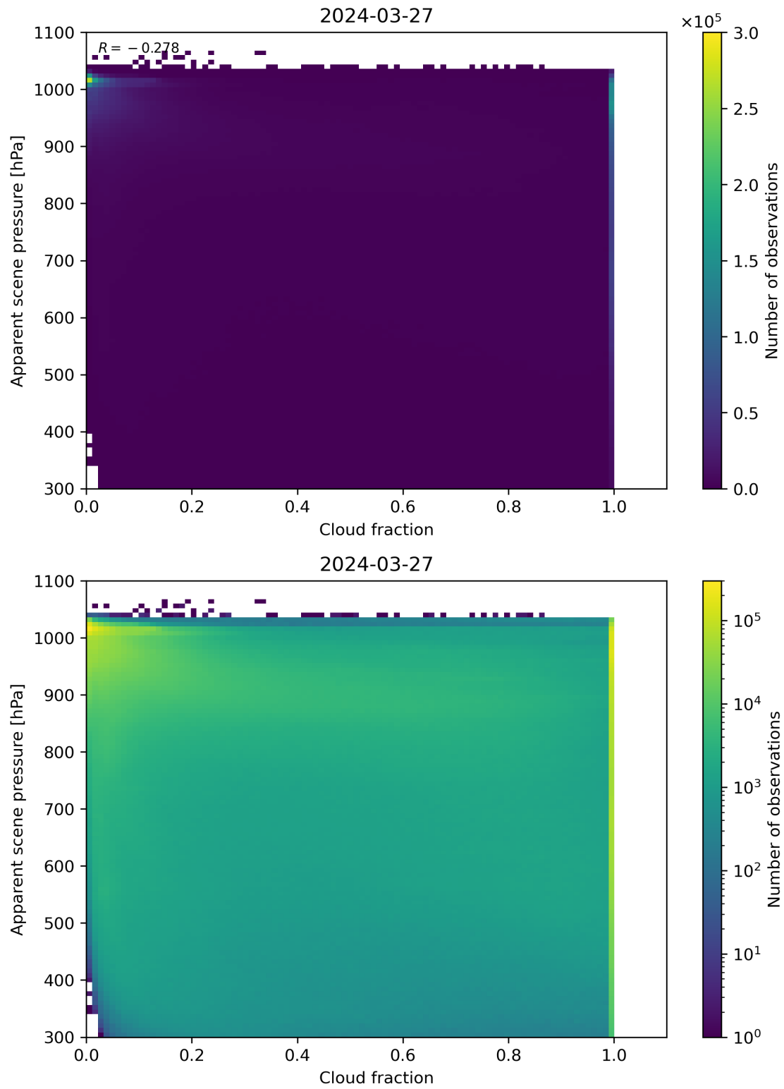
Figure 70: Scatter density plot of “Cloud fraction” against “Apparent scene pressure” for 2024-03-26 to 2024-03-28.
