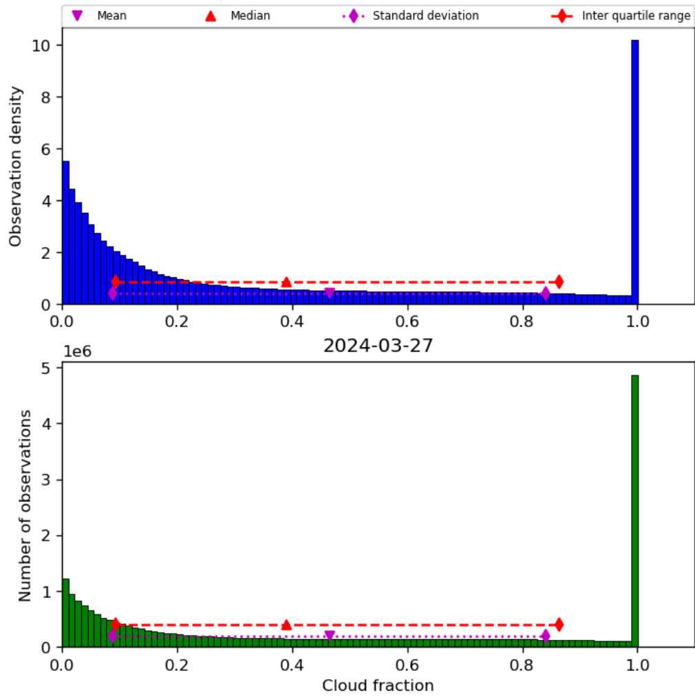
Figure 32: Histogram of “Cloud fraction” for 2024-03-26 to 2024-03-28
