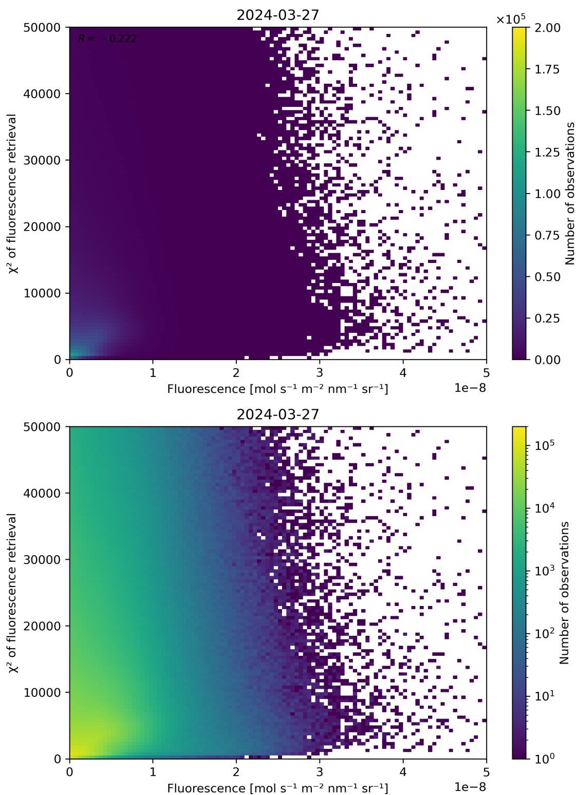
Figure 85: Scatter density plot of “Fluorescence” against “ \chi^2 of fluorescence retrieval” for 2024-03-26 to 2024-03-28.
