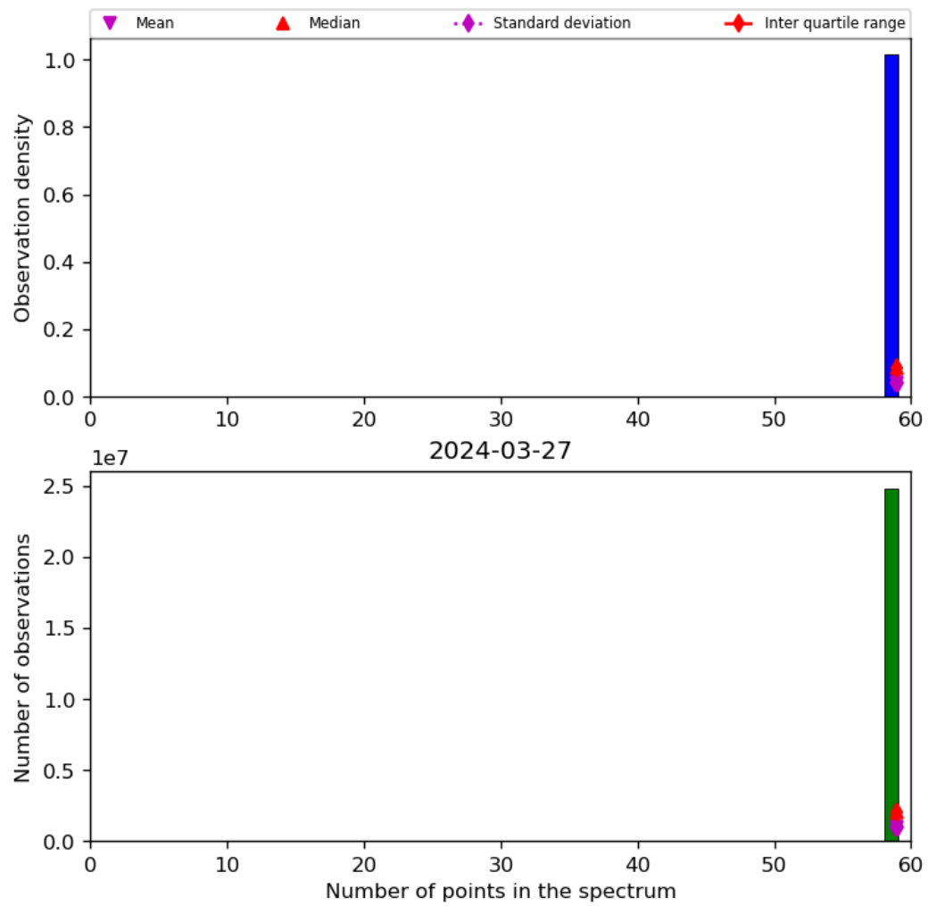
Figure 44: Histogram of “Number of points in the spectrum” for 2024-03-26 to 2024-03-28
