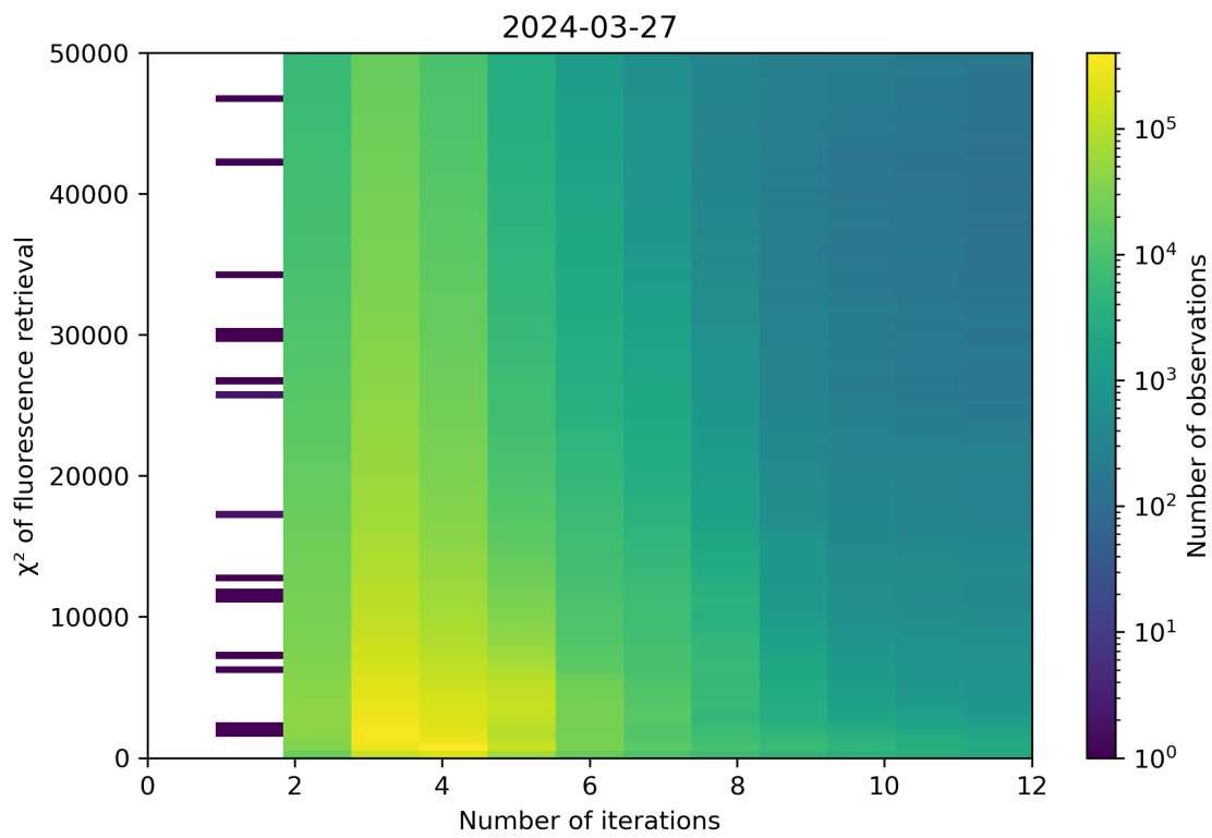
Figure 97: Scatter density plot of “Number of iterations” against “ \chi^2 of fluorescence retrieval” for 2024-03-26 to 2024-03-28.
