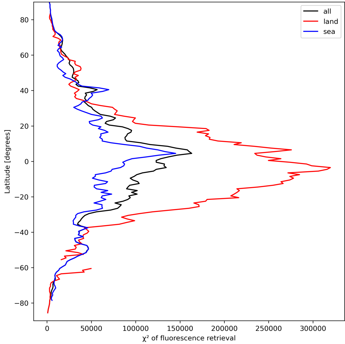
Figure 25: Zonal average of “ \chi^2 of fluorescence retrieval” for 2024-03-26 to 2024-03-28.
