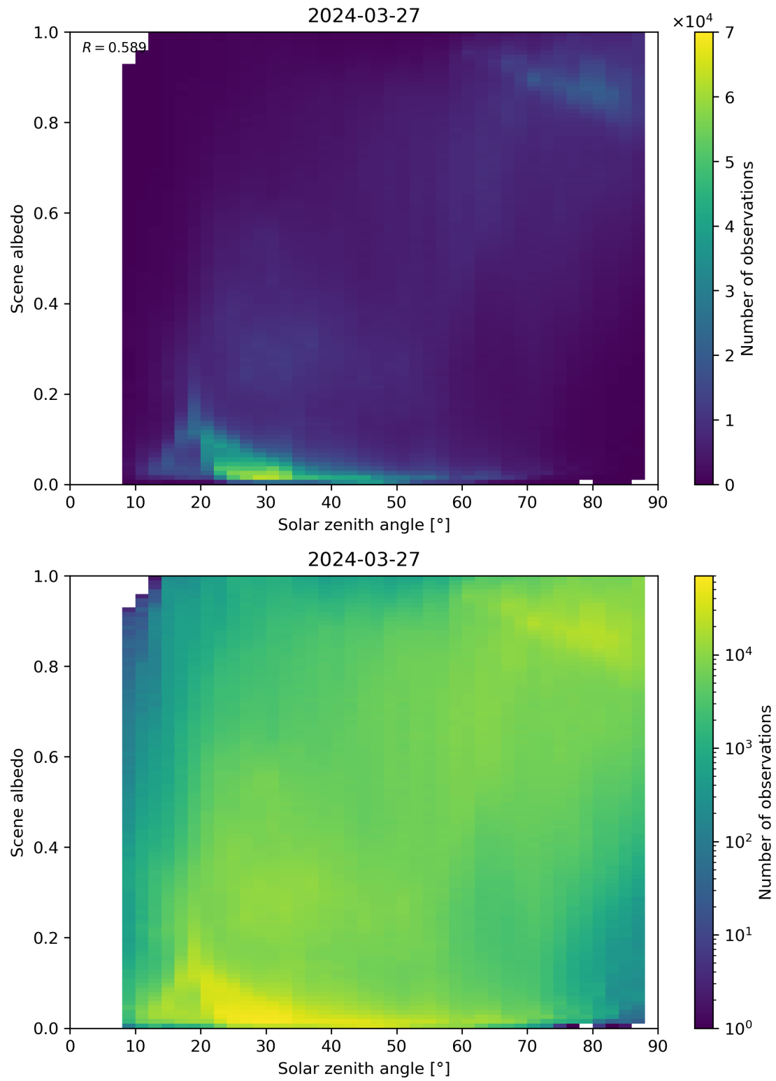
Figure 116: Scatter density plot of “Solar zenith angle” against “Scene albedo” for 2024-03-26 to 2024-03-28.
