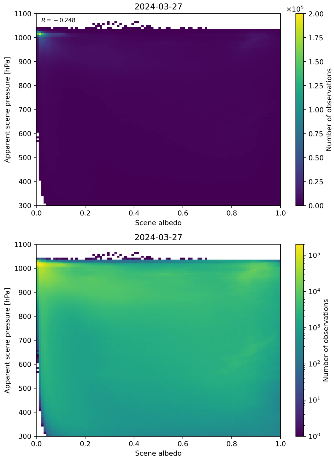
Figure 102: Scatter density plot of “Scene albedo” against “Apparent scene pressure” for 2024-03-26 to 2024-03-28.
