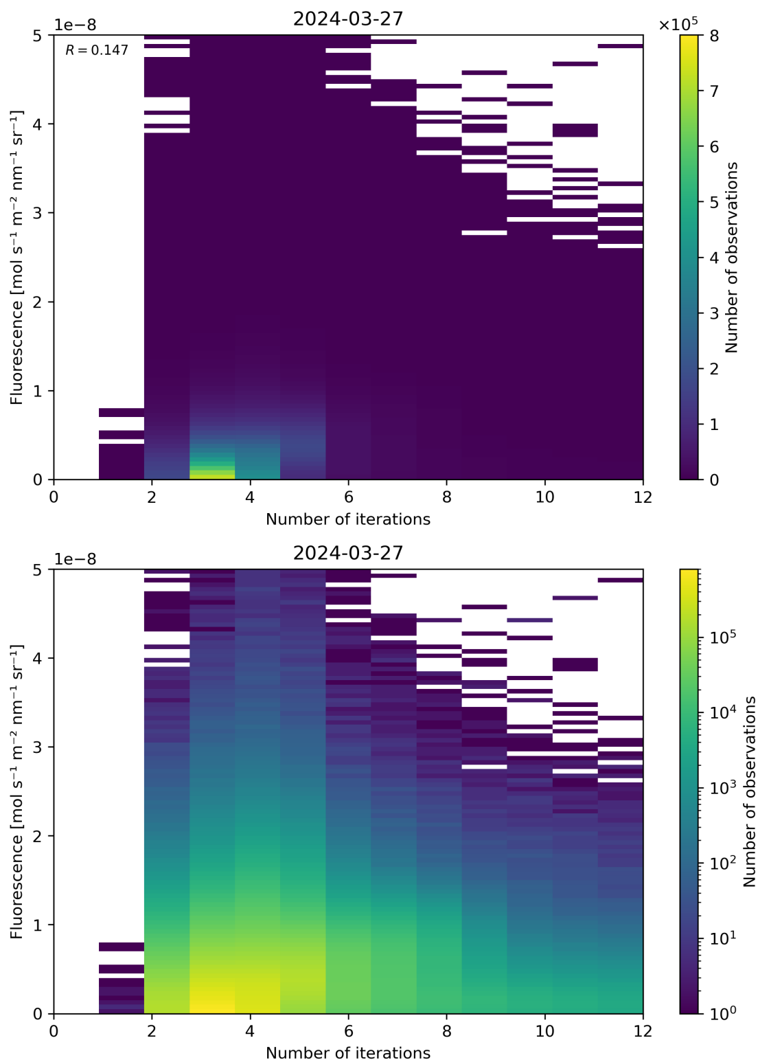
Figure 98: Scatter density plot of “Number of iterations” against “Fluorescence” for 2024-03-26 to 2024-03-28.
