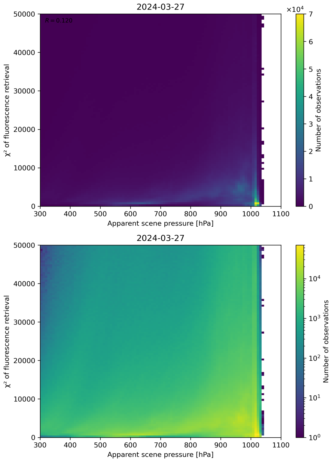
Figure 63: Scatter density plot of “Apparent scene pressure” against “ \chi^2 of fluorescence retrieval” for 2024-03-26 to 2024-03-28.
