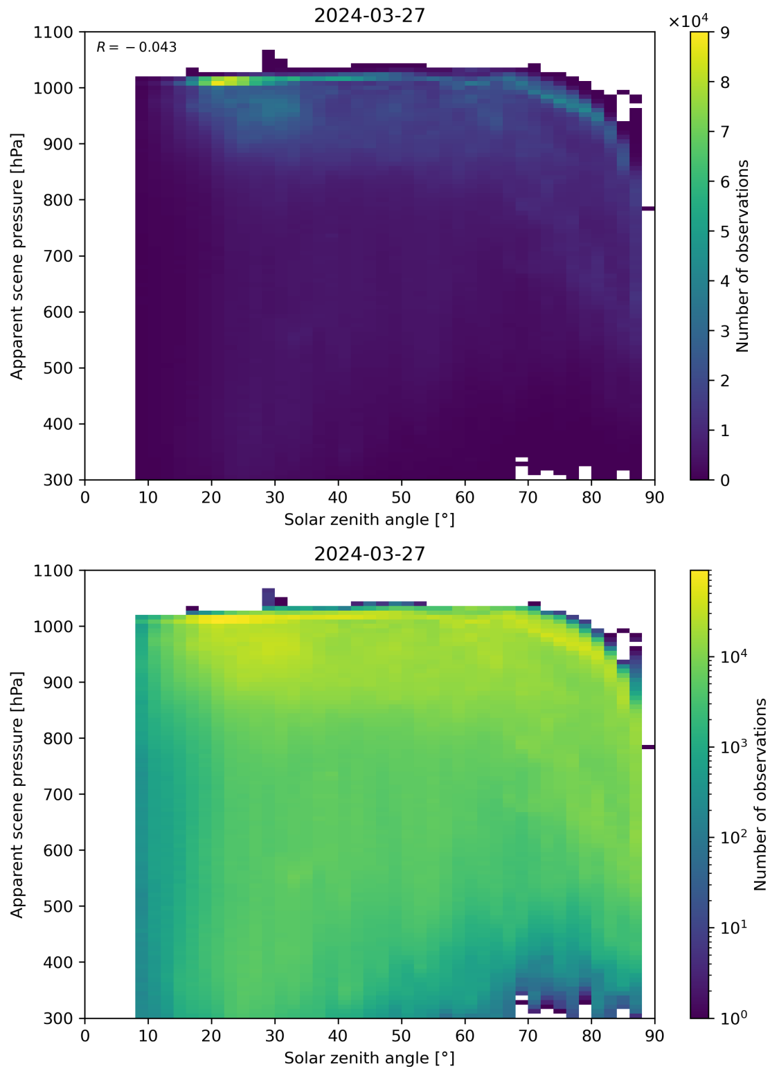
Figure 108: Scatter density plot of “Solar zenith angle” against “Apparent scene pressure” for 2024-03-26 to 2024-03-28.
