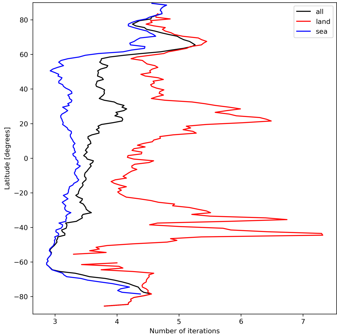
Figure 22: Zonal average of “Number of iterations” for 2024-03-26 to 2024-03-28.
