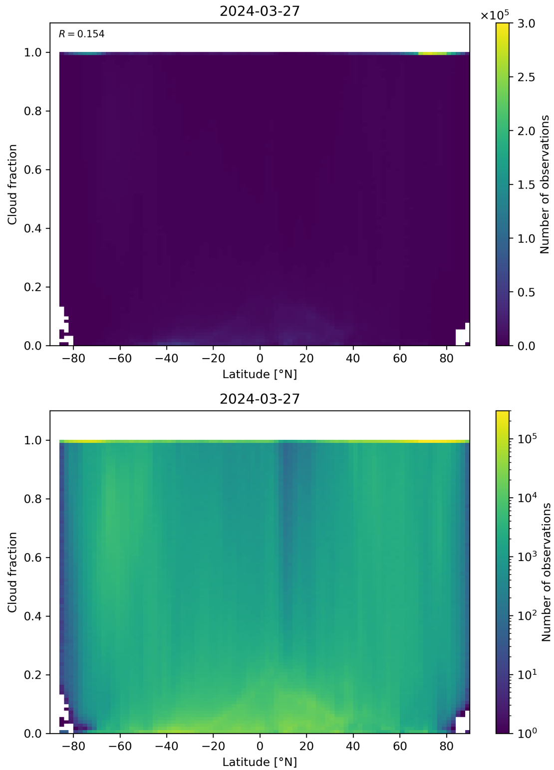
Figure 90: Scatter density plot of “Latitude” against “Cloud fraction” for 2024-03-26 to 2024-03-28.
