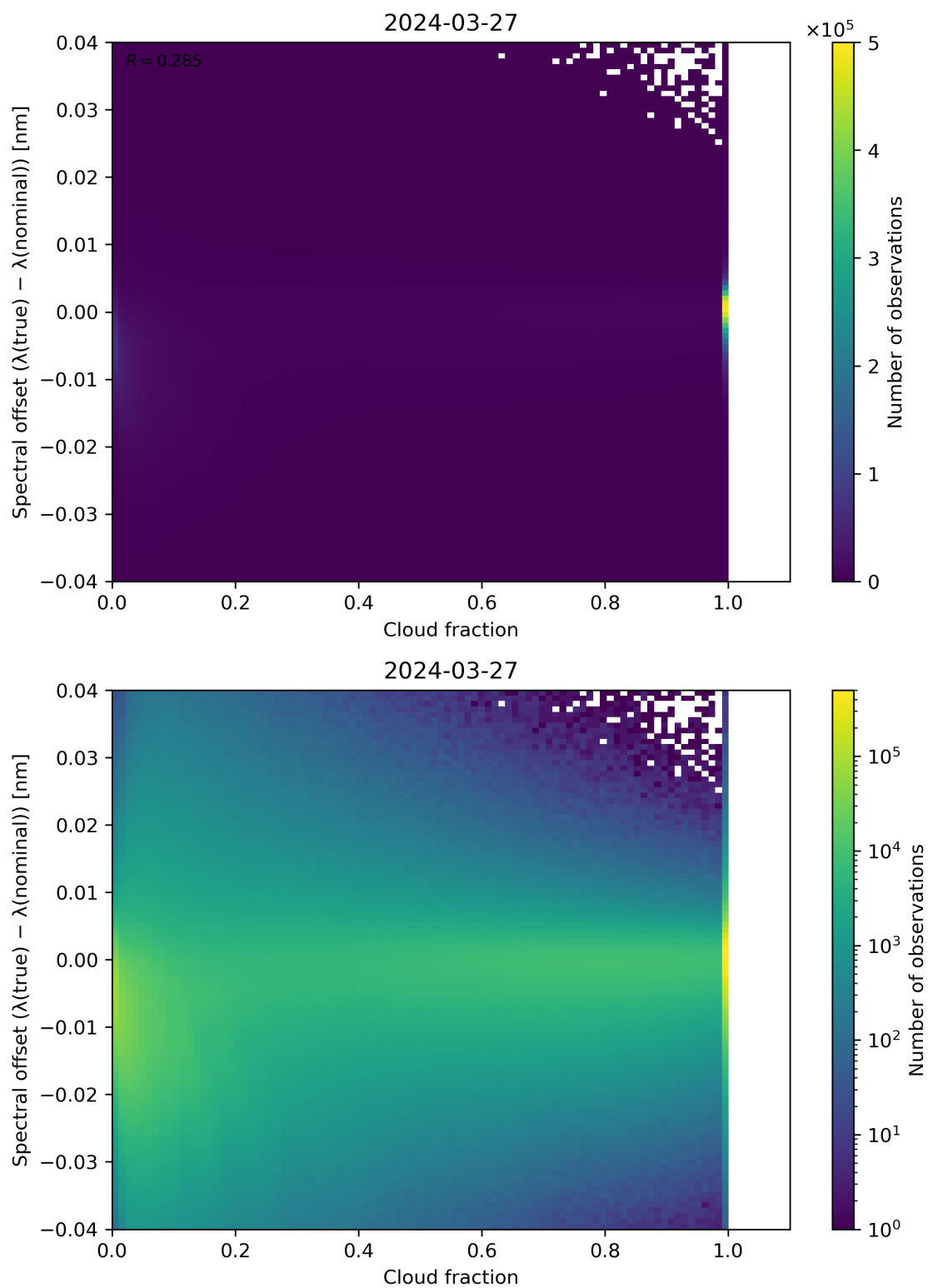
Figure 76: Scatter density plot of “Cloud fraction” against “Spectral offset ( \lambda(\text{true}) - \lambda(\text{nominal}) )” for 2024-03-26 to 2024-03-28.
