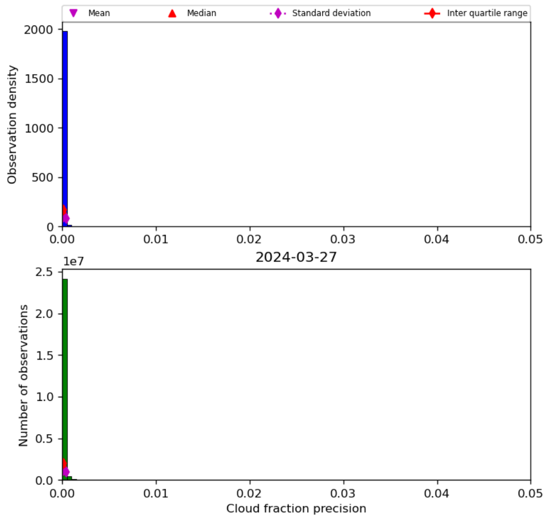
Figure 33: Histogram of “Cloud fraction precision” for 2024-03-26 to 2024-03-28
