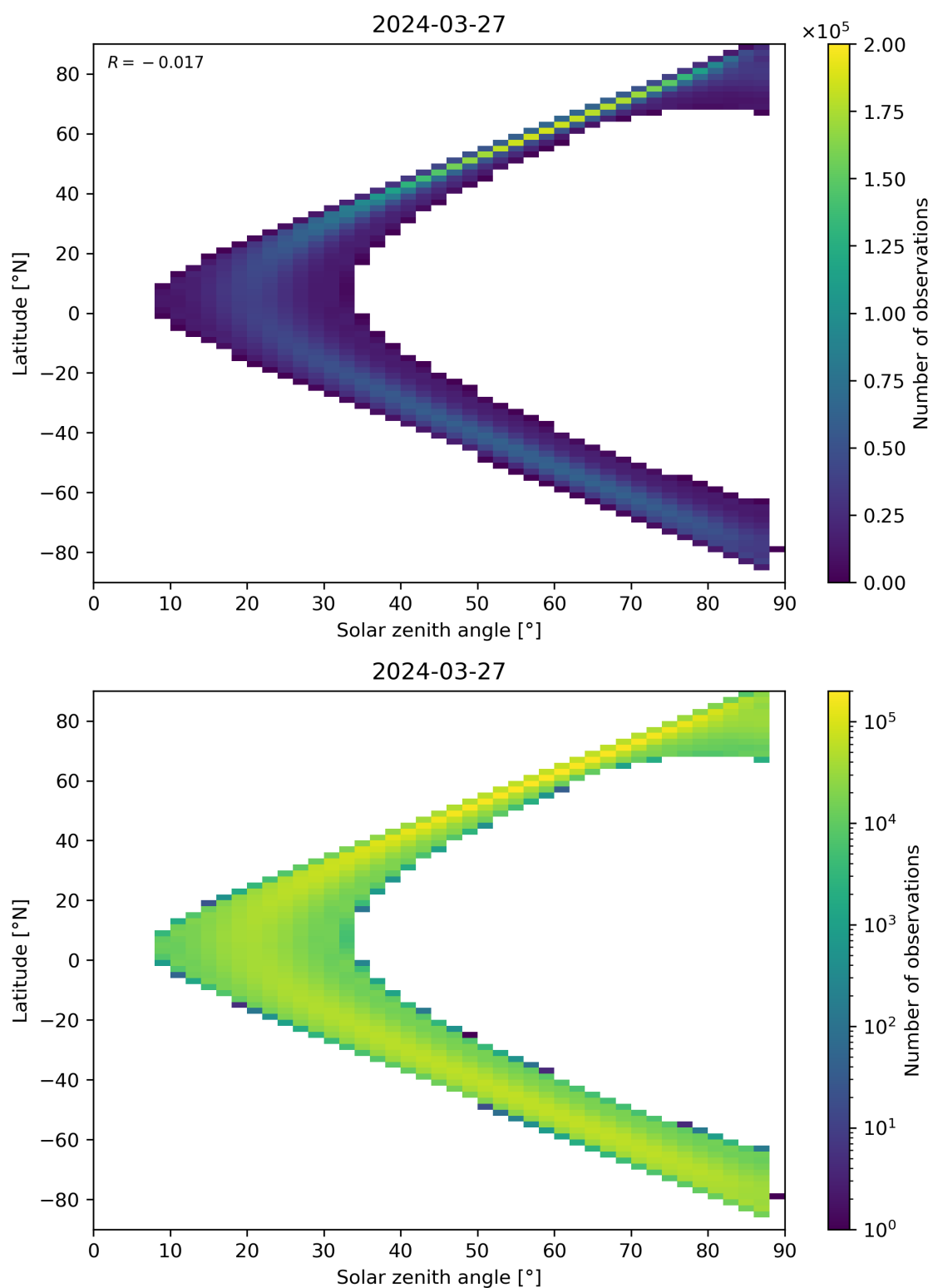
Figure 113: Scatter density plot of “Solar zenith angle” against “Latitude” for 2024-03-26 to 2024-03-28.
