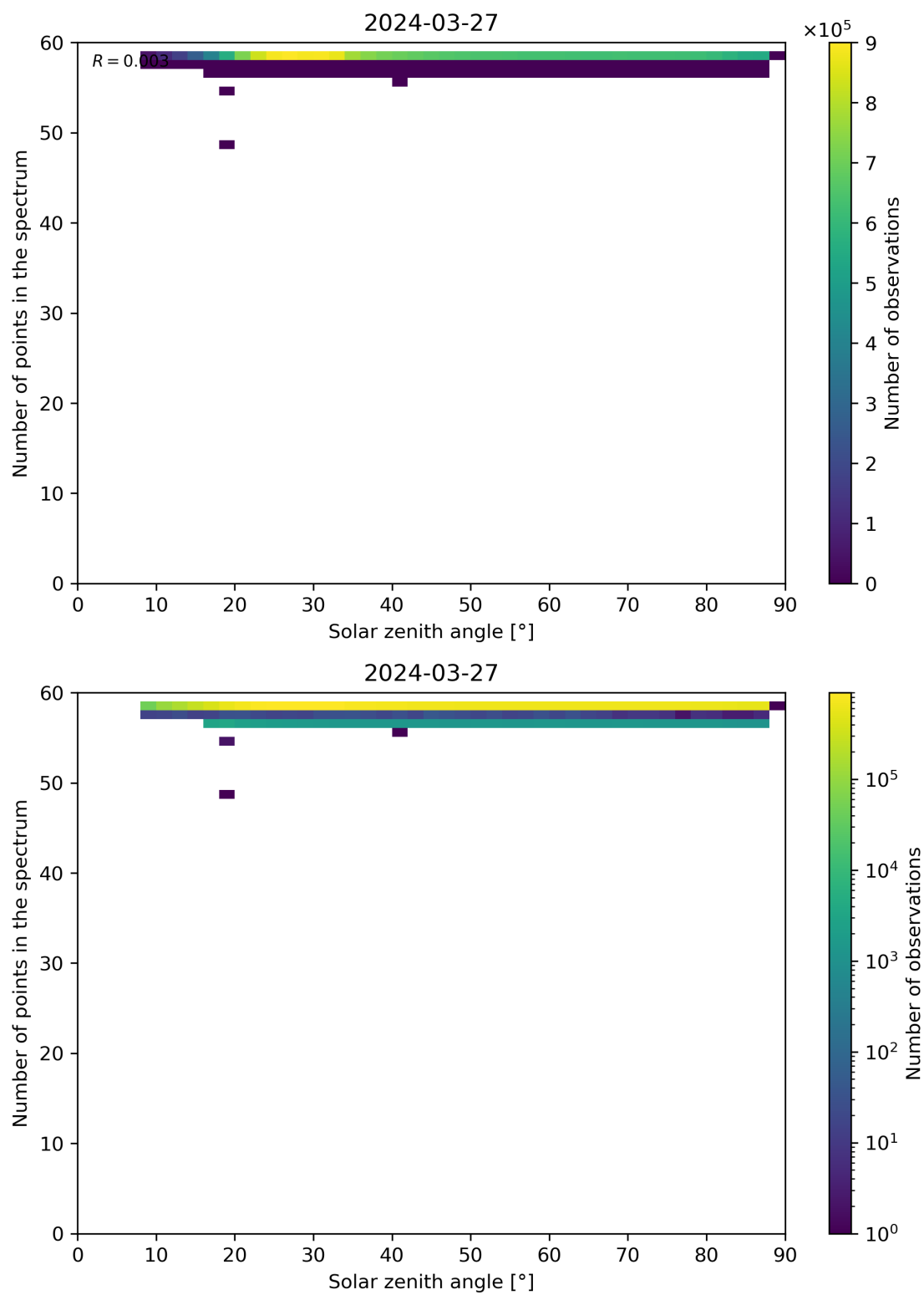
Figure 115: Scatter density plot of “Solar zenith angle” against “Number of points in the spectrum” for 2024-03-26 to 2024-03-28.
