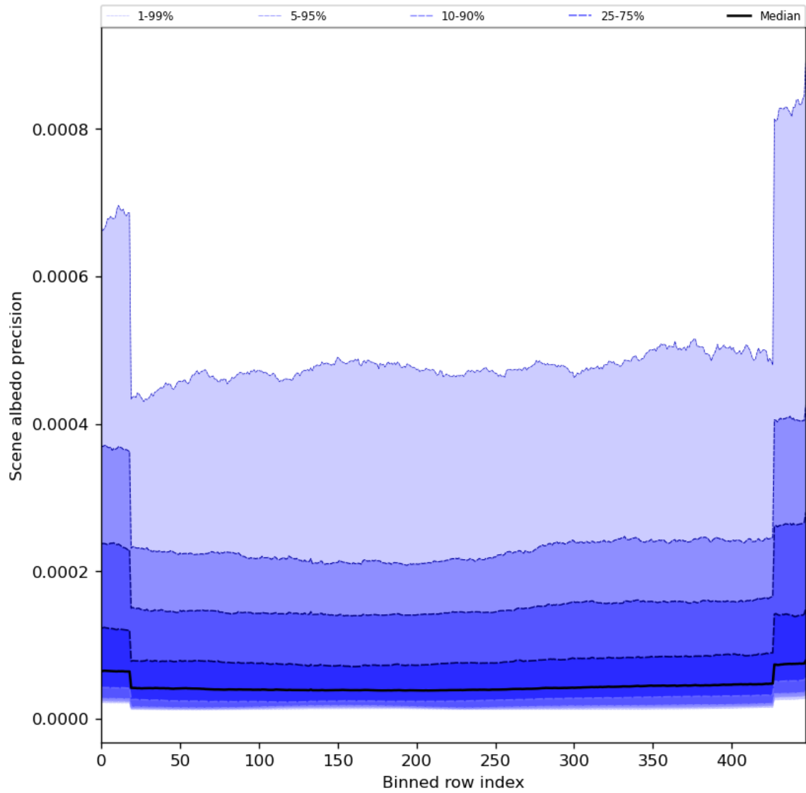
Figure 52: Along track statistics of “Scene albedo precision” for 2024-03-26 to 2024-03-28
