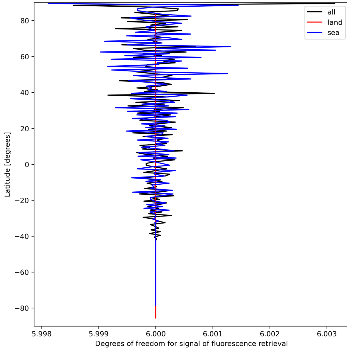
Figure 26: Zonal average of “Degrees of freedom for signal of fluorescence retrieval” for 2024-03-26 to 2024-03-28.
