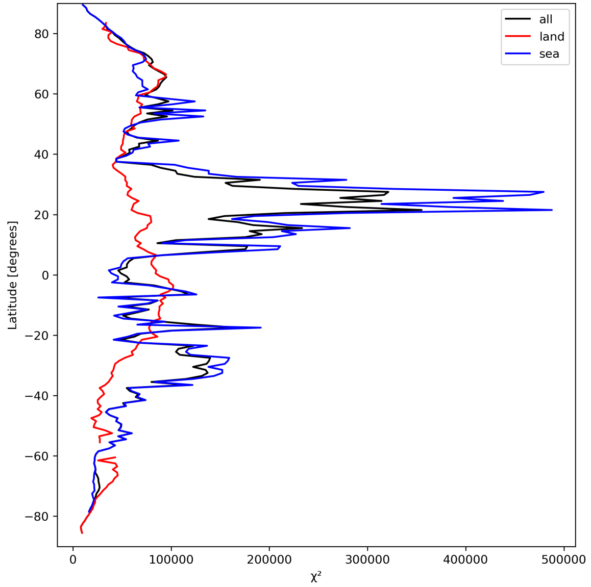
Figure 21: Zonal average of “ \chi^2 ” for 2024-03-26 to 2024-03-28.
