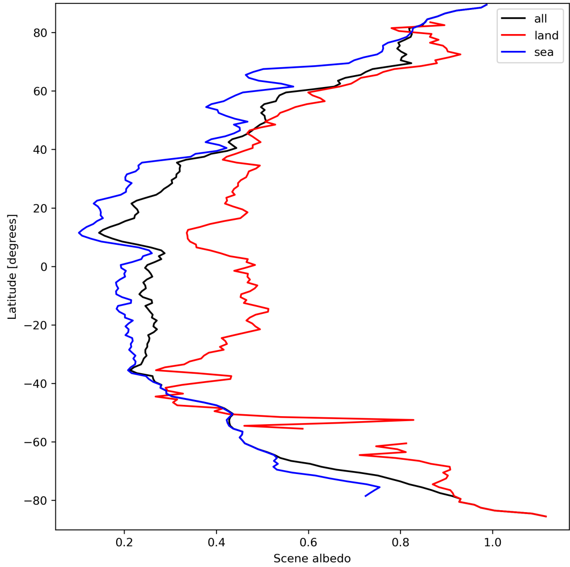
Figure 17: Zonal average of “Scene albedo” for 2024-03-26 to 2024-03-28.
