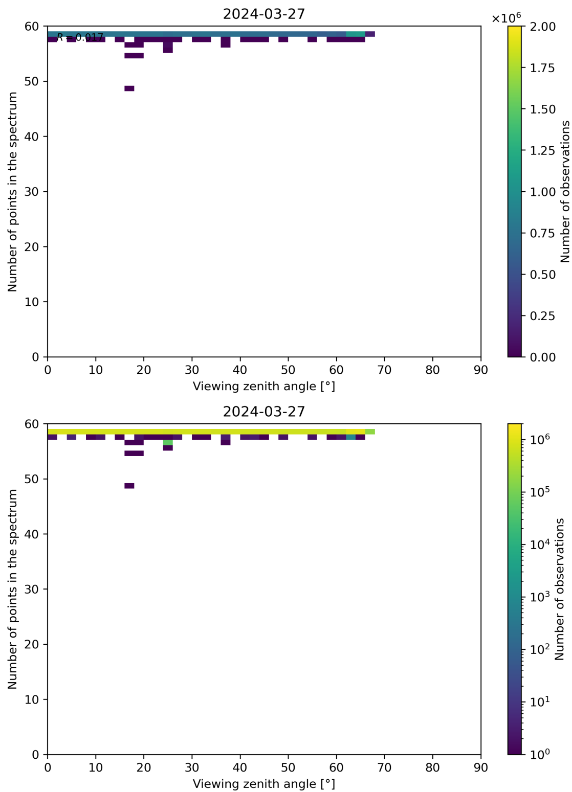
Figure 125: Scatter density plot of “Viewing zenith angle” against “Number of points in the spectrum” for 2024-03-26 to 2024-03-28.
