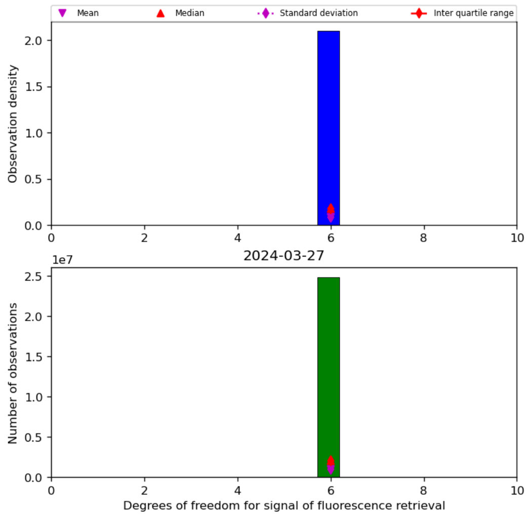
Figure 43: Histogram of “Degrees of freedom for signal of fluorescence retrieval” for 2024-03-26 to 2024-03-28
