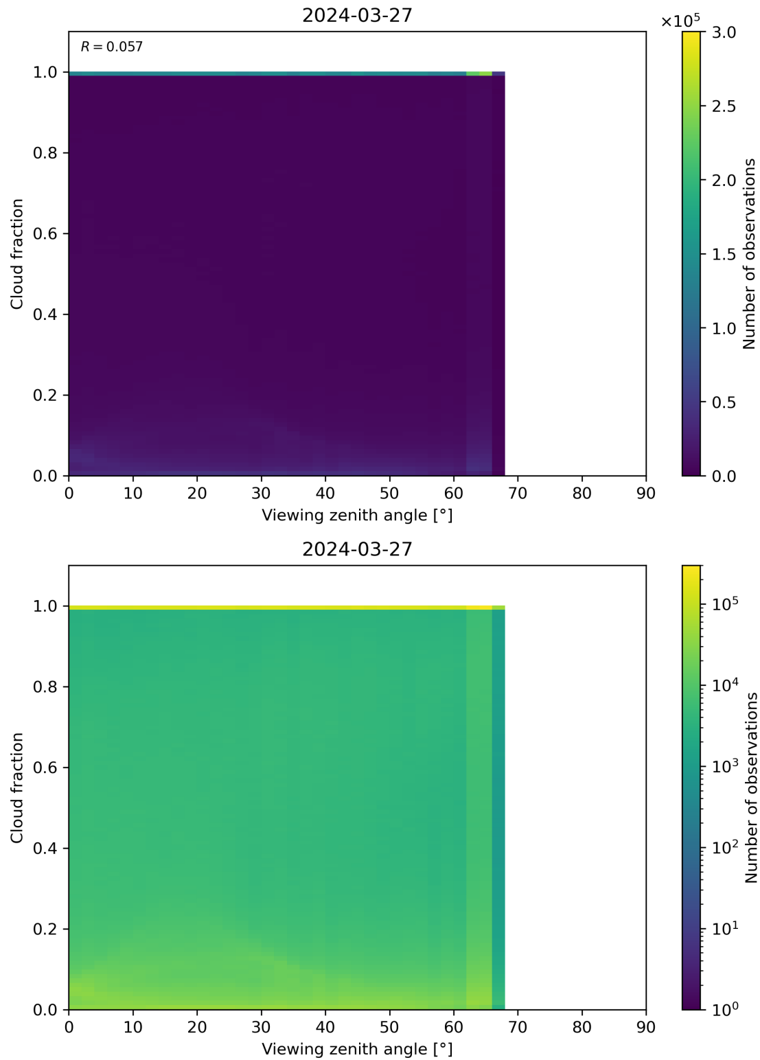
Figure 120: Scatter density plot of “Viewing zenith angle” against “Cloud fraction” for 2024-03-26 to 2024-03-28.
