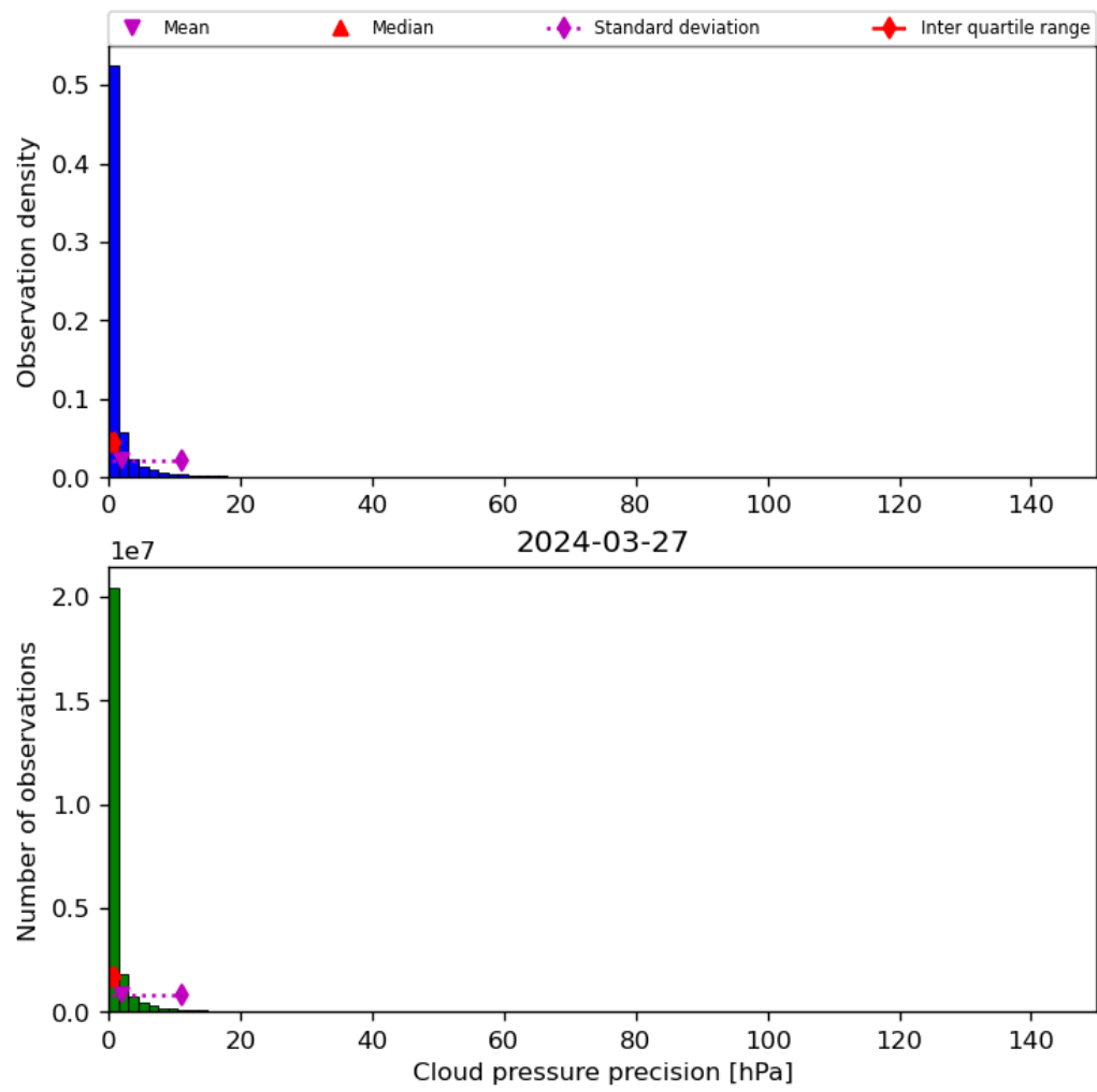
Figure 31: Histogram of “Cloud pressure precision” for 2024-03-26 to 2024-03-28
