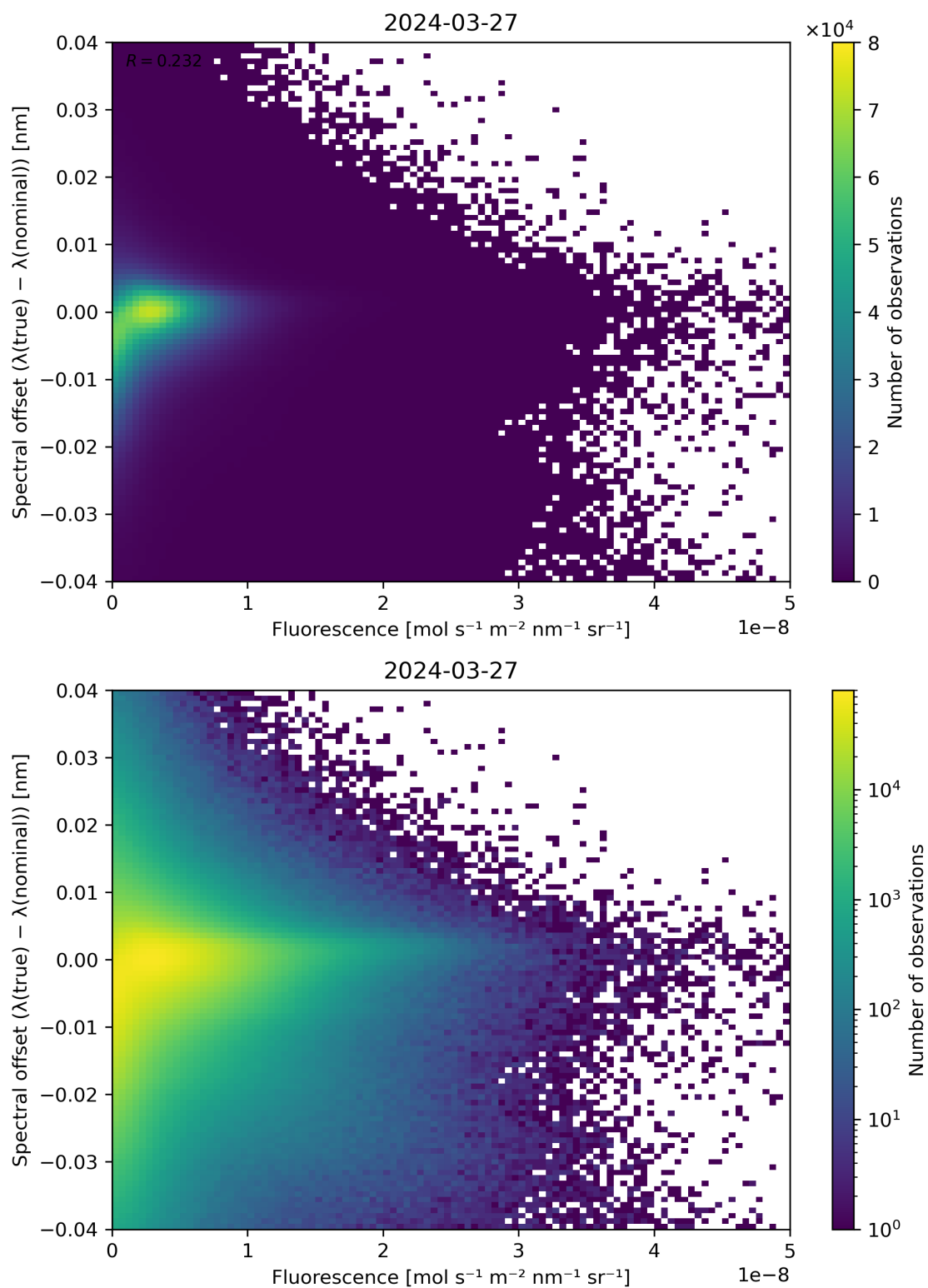
Figure 87: Scatter density plot of “Fluorescence” against “Spectral offset ( \lambda(\text{true}) - \lambda(\text{nominal}) )” for 2024-03-26 to 2024-03-28.
