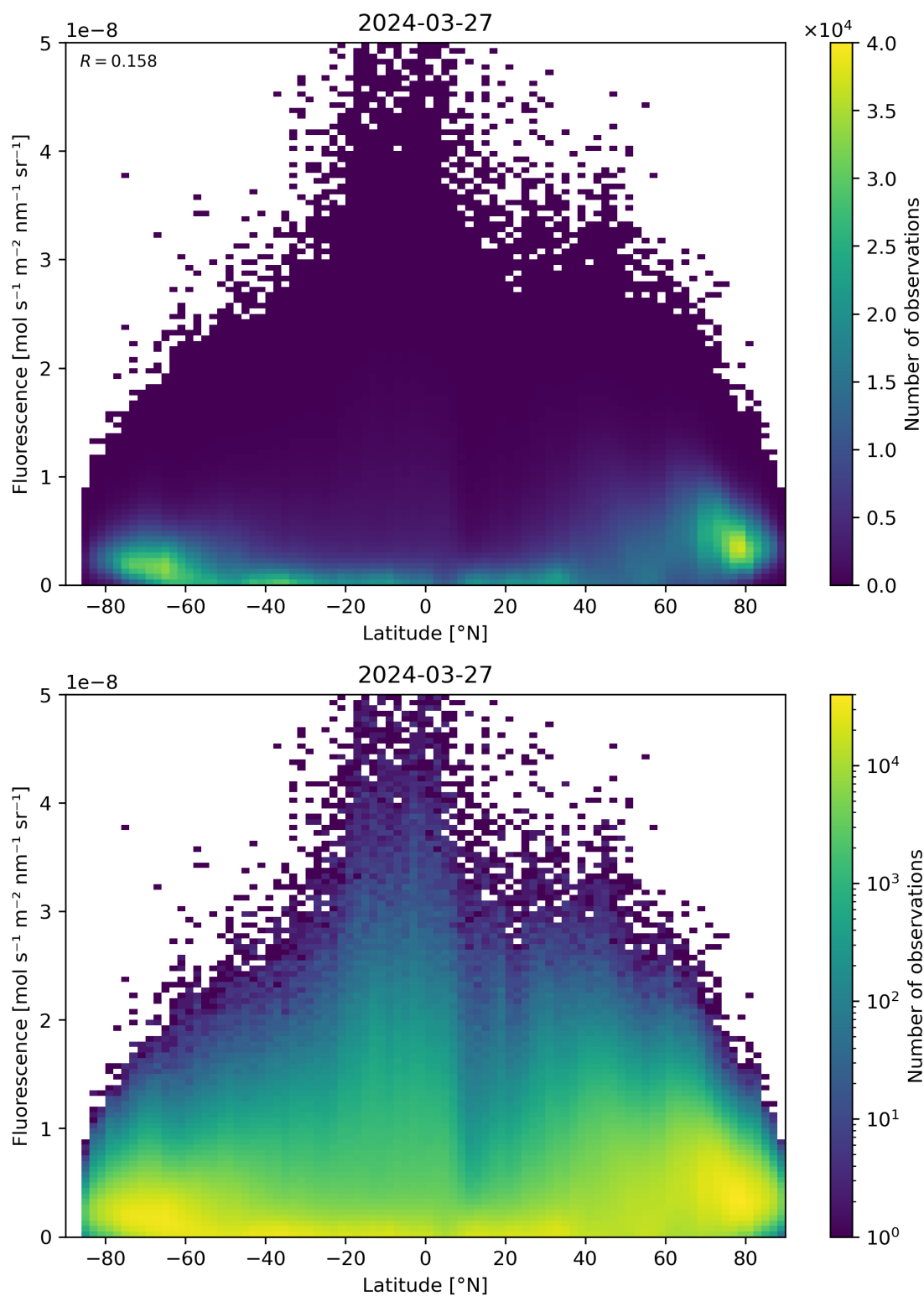
Figure 92: Scatter density plot of “Latitude” against “Fluorescence” for 2024-03-26 to 2024-03-28.
