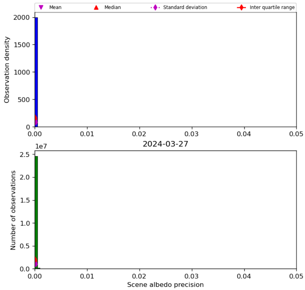
Figure 35: Histogram of “Scene albedo precision” for 2024-03-26 to 2024-03-28
