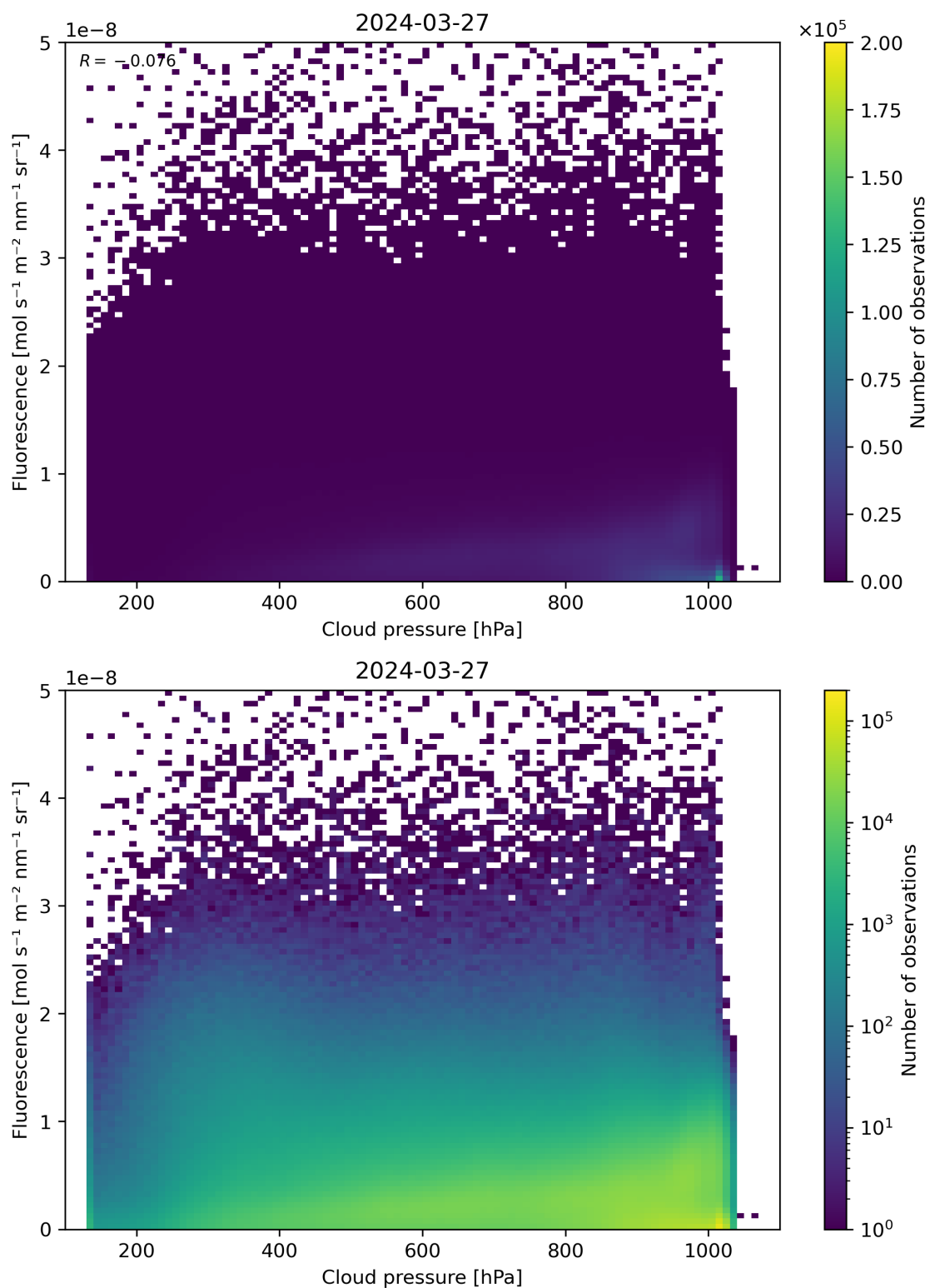
Figure 80: Scatter density plot of “Cloud pressure” against “Fluorescence” for 2024-03-26 to 2024-03-28.
