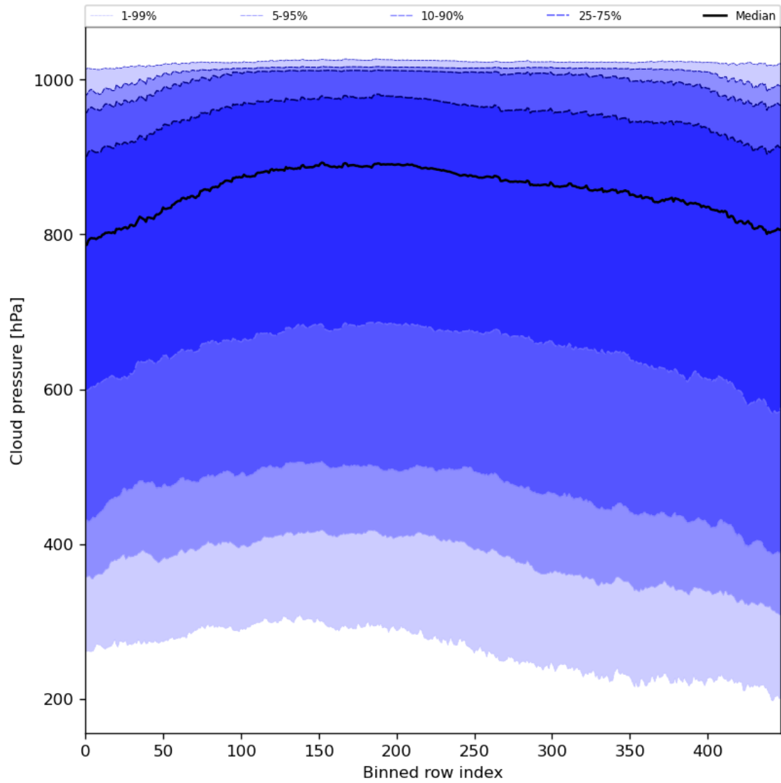
Figure 47: Along track statistics of “Cloud pressure” for 2024-03-26 to 2024-03-28
