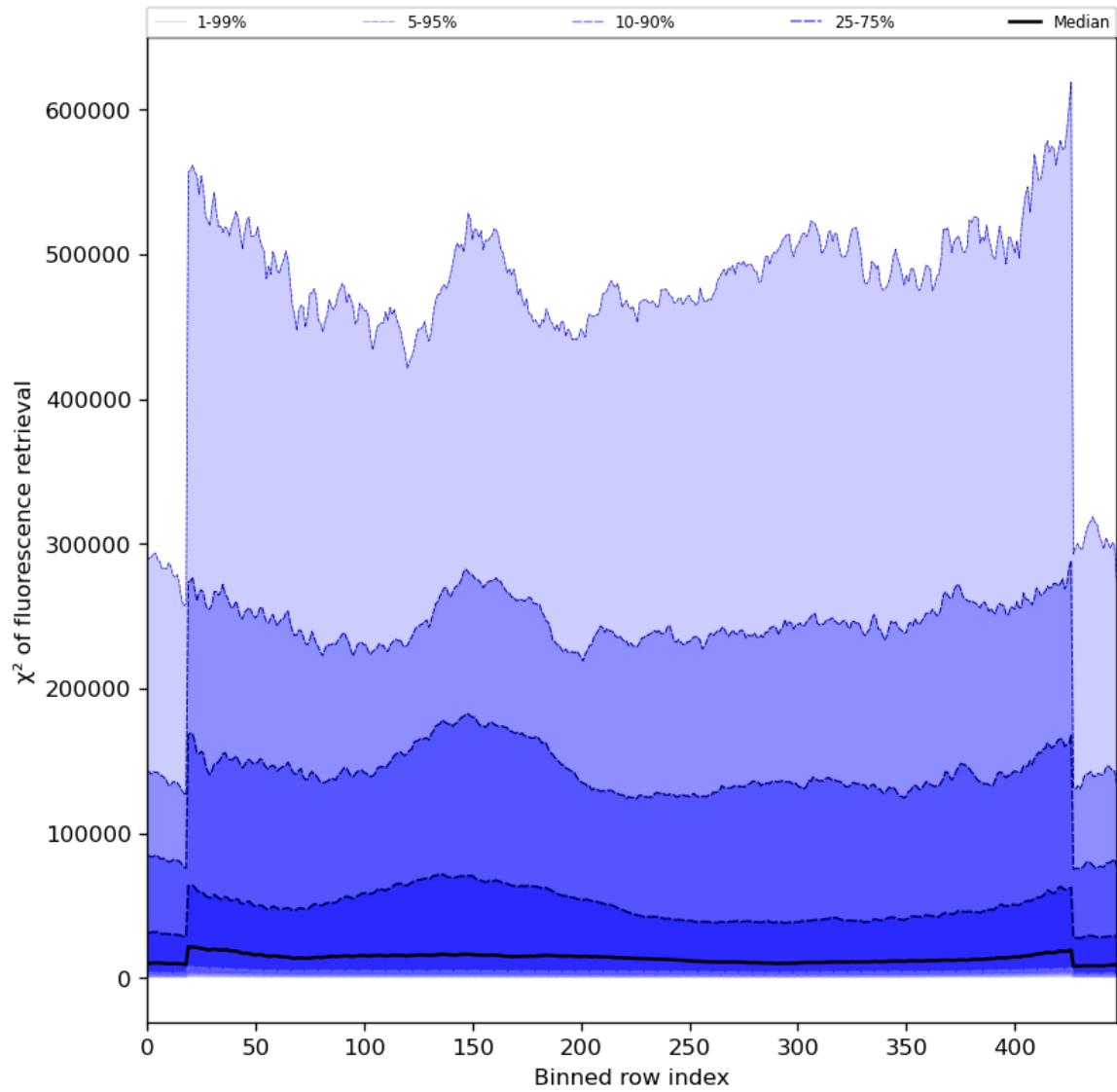
Figure 59: Along track statistics of “ \chi^2 of fluorescence retrieval” for 2024-03-26 to 2024-03-28
