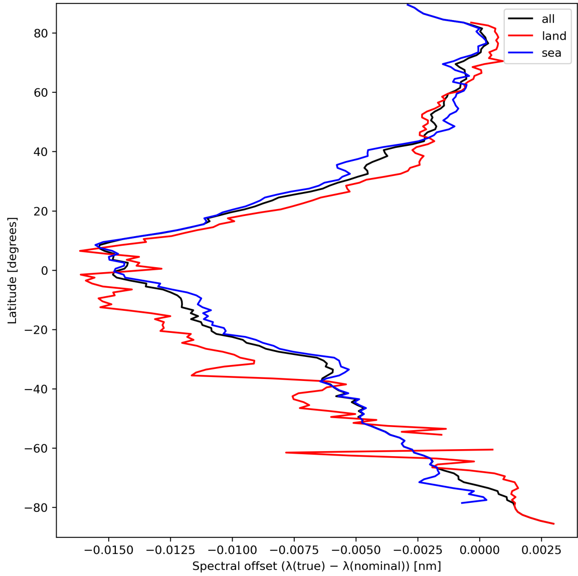
Figure 28: Zonal average of “Spectral offset ( \lambda(\text{true}) - \lambda(\text{nominal}) )” for 2024-03-26 to 2024-03-28.
