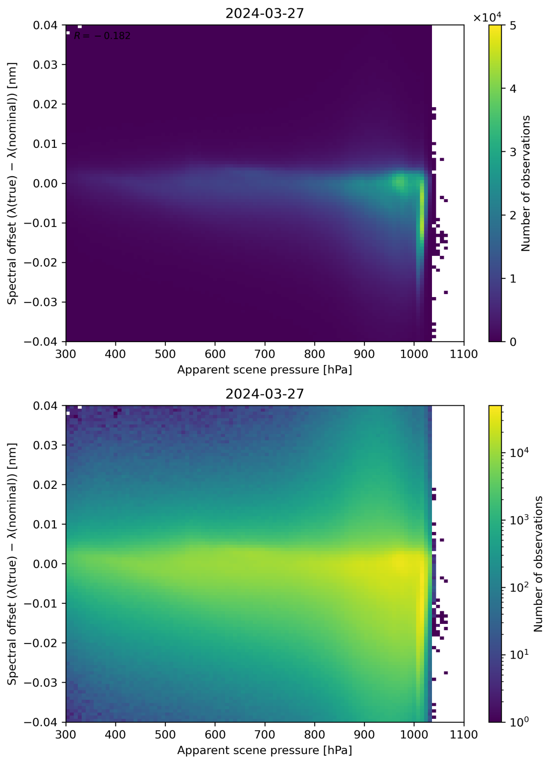
Figure 67: Scatter density plot of “Apparent scene pressure” against “Spectral offset ( \lambda(\text{true}) - \lambda(\text{nominal}) )” for 2024-03-26 to 2024-03-28.
