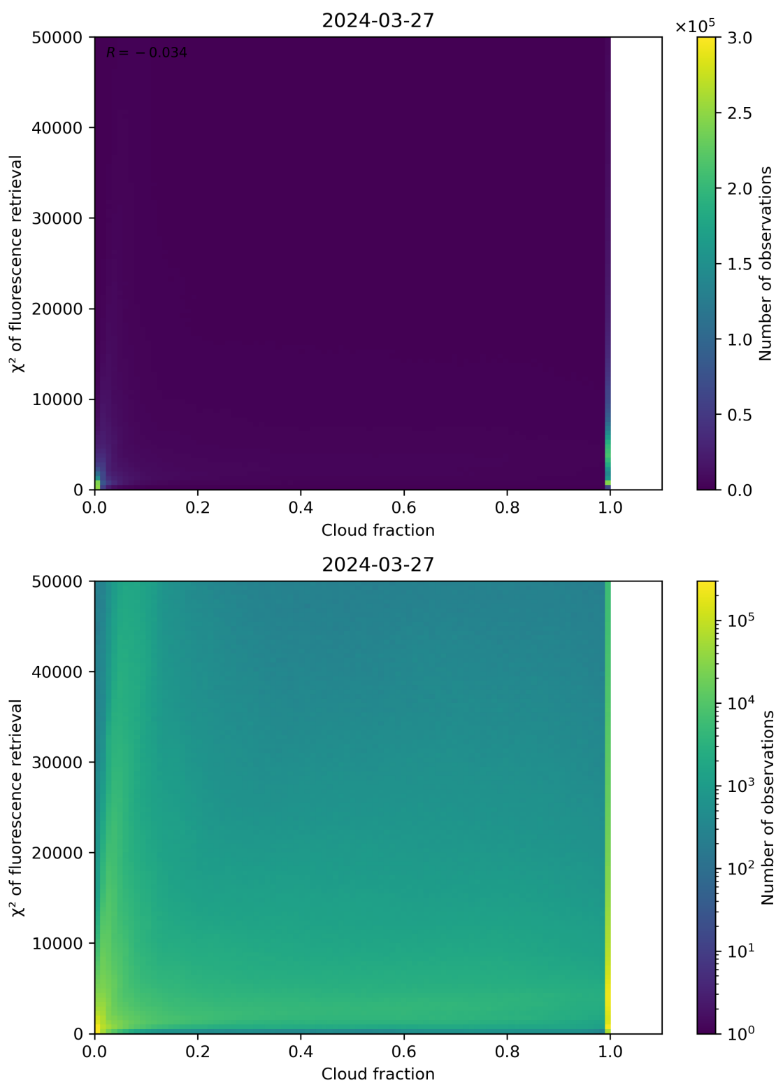
Figure 71: Scatter density plot of “Cloud fraction” against “ \chi^2 of fluorescence retrieval” for 2024-03-26 to 2024-03-28.
