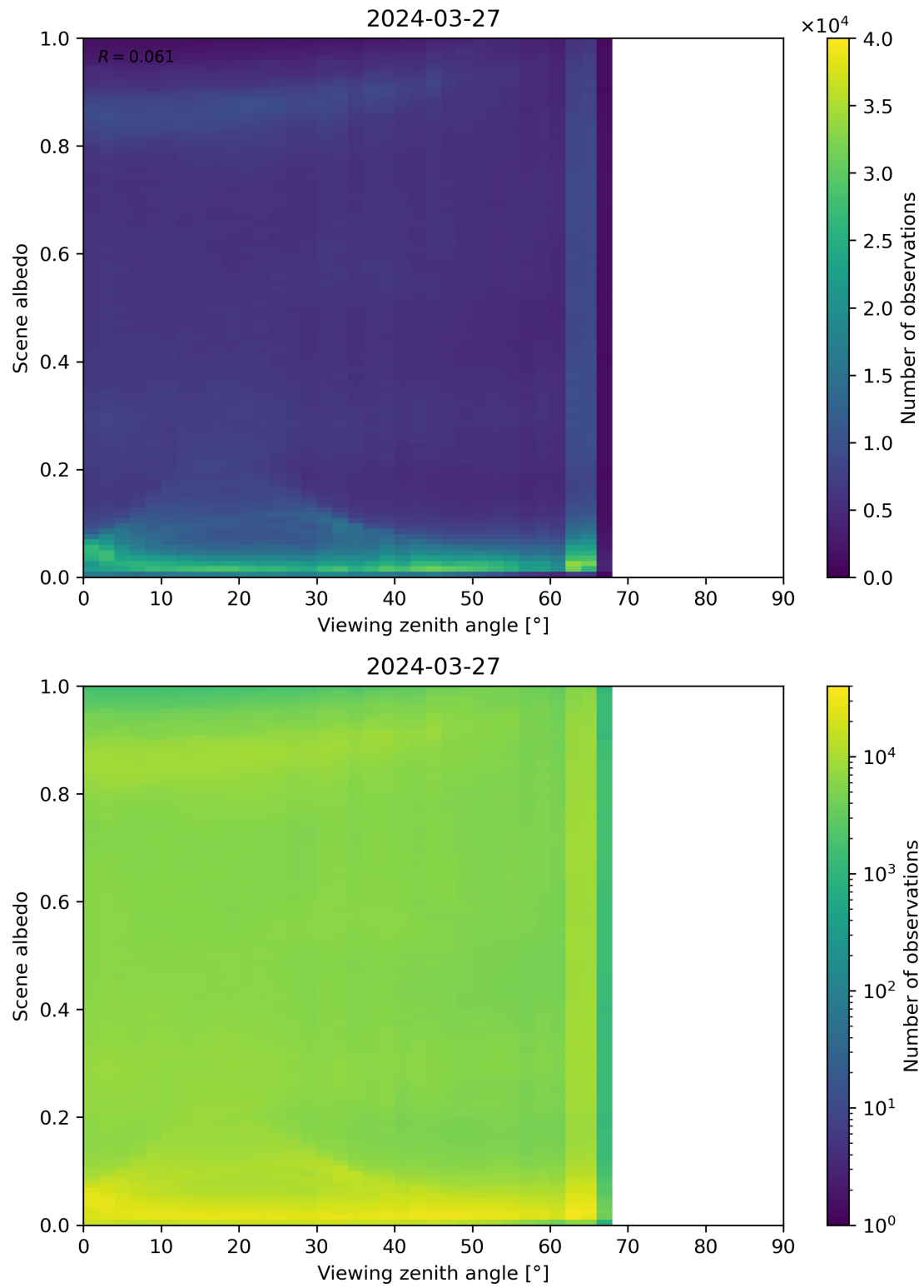
Figure 126: Scatter density plot of “Viewing zenith angle” against “Scene albedo” for 2024-03-26 to 2024-03-28.
