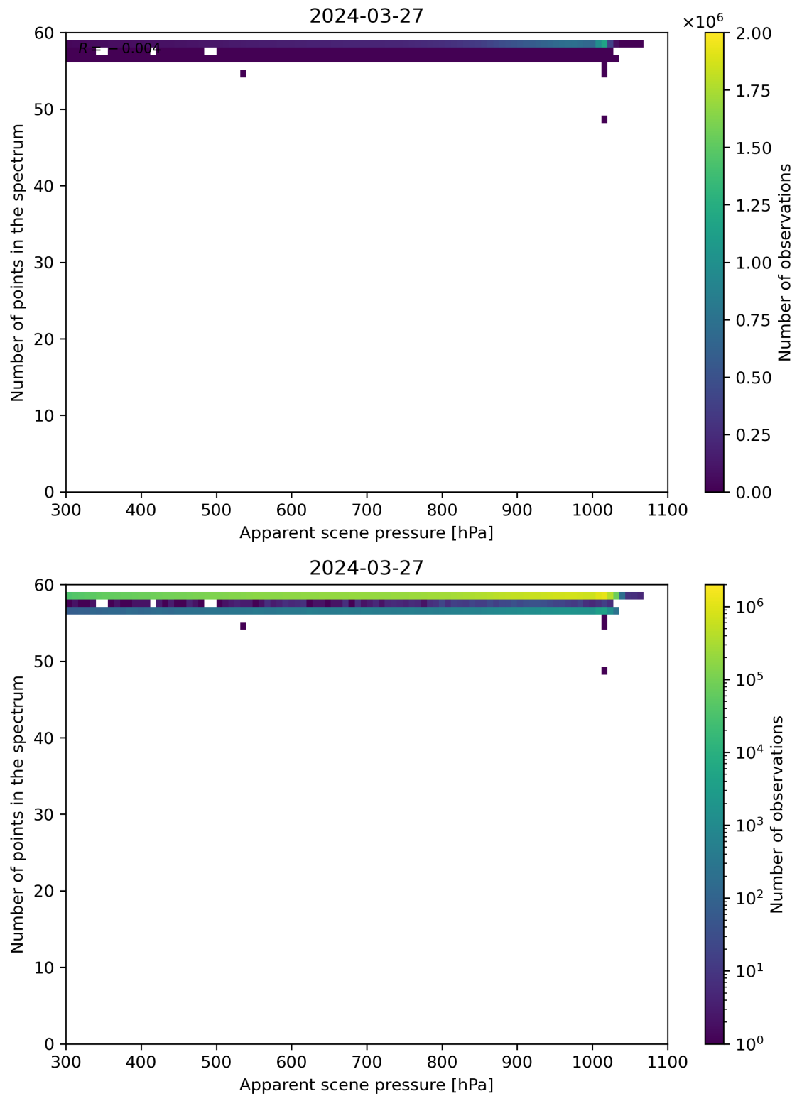
Figure 66: Scatter density plot of “Apparent scene pressure” against “Number of points in the spectrum” for 2024-03-26 to 2024-03-28.
