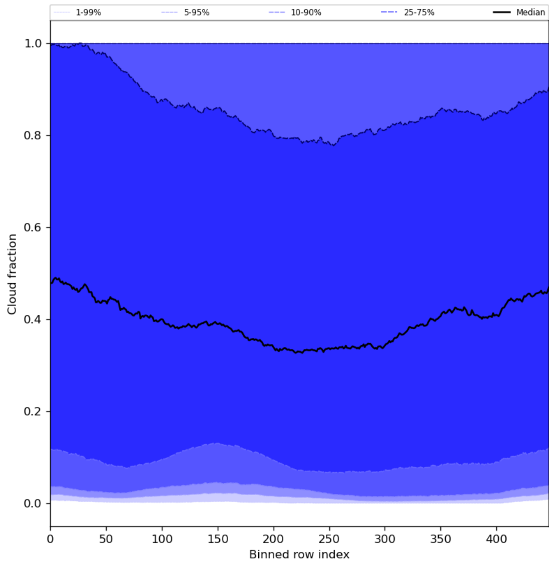
Figure 49: Along track statistics of “Cloud fraction” for 2024-03-26 to 2024-03-28
