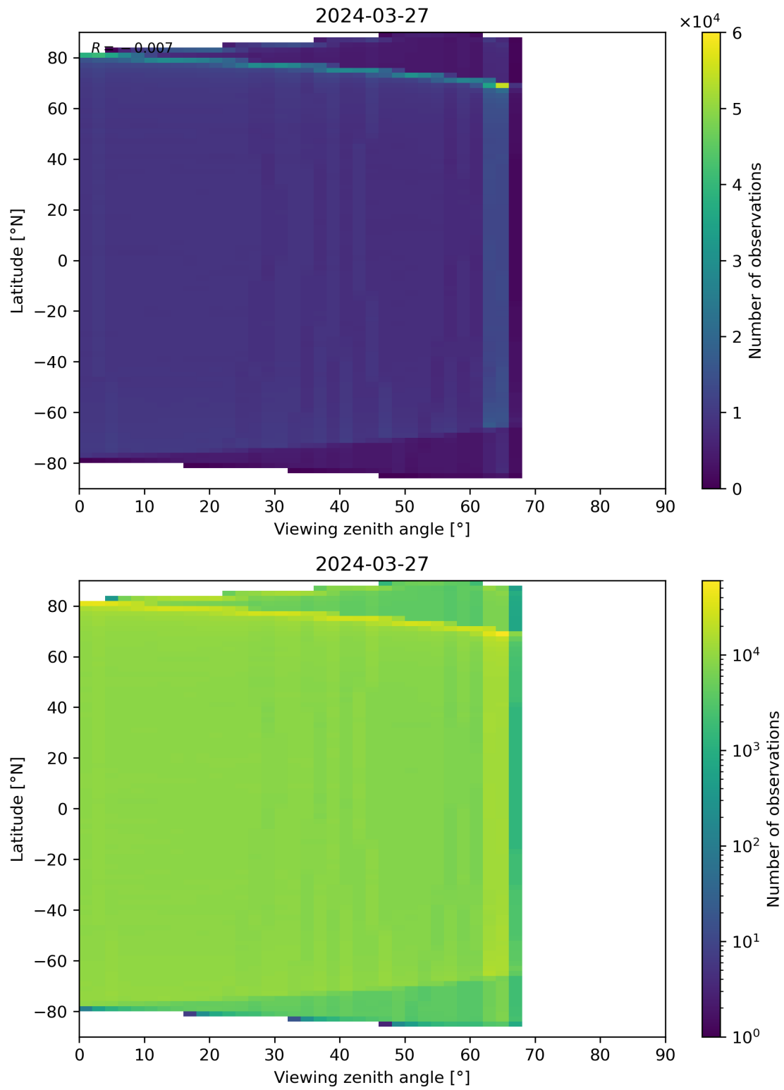
Figure 123: Scatter density plot of “Viewing zenith angle” against “Latitude” for 2024-03-26 to 2024-03-28.
