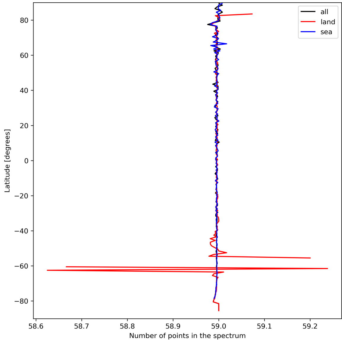
Figure 27: Zonal average of “Number of points in the spectrum” for 2024-03-26 to 2024-03-28.
