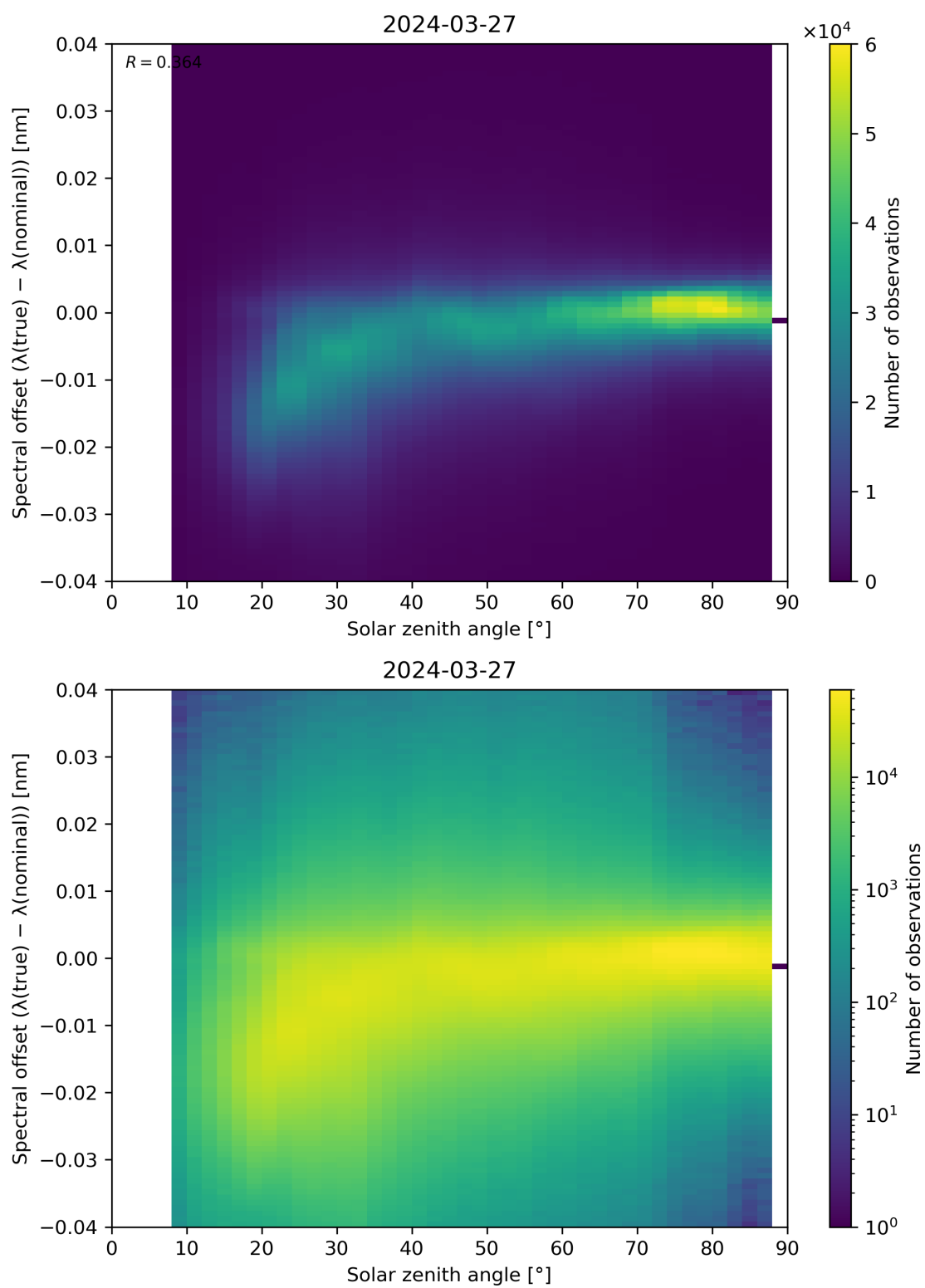
Figure 117: Scatter density plot of “Solar zenith angle” against “Spectral offset ( \lambda(\text{true}) - \lambda(\text{nominal}) )” for 2024-03-26 to 2024-03-28.
