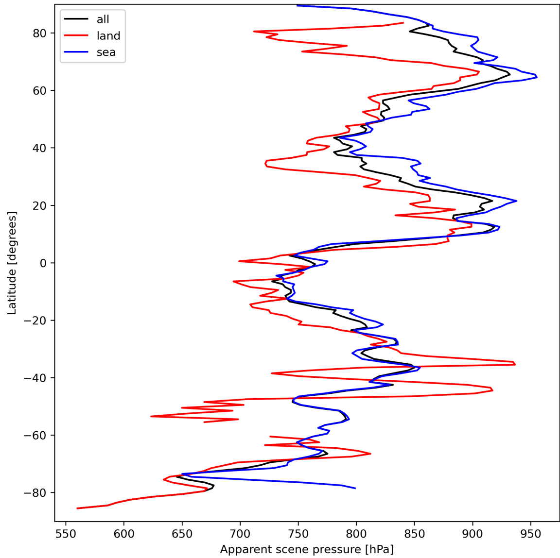
Figure 19: Zonal average of “Apparent scene pressure” for 2024-03-26 to 2024-03-28.
