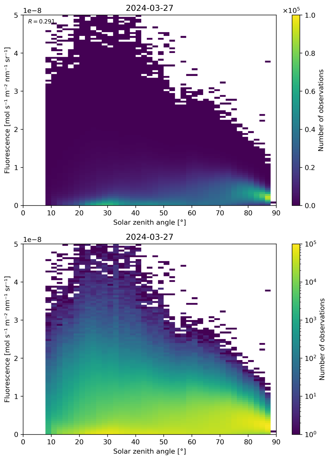
Figure 112: Scatter density plot of “Solar zenith angle” against “Fluorescence” for 2024-03-26 to 2024-03-28.
