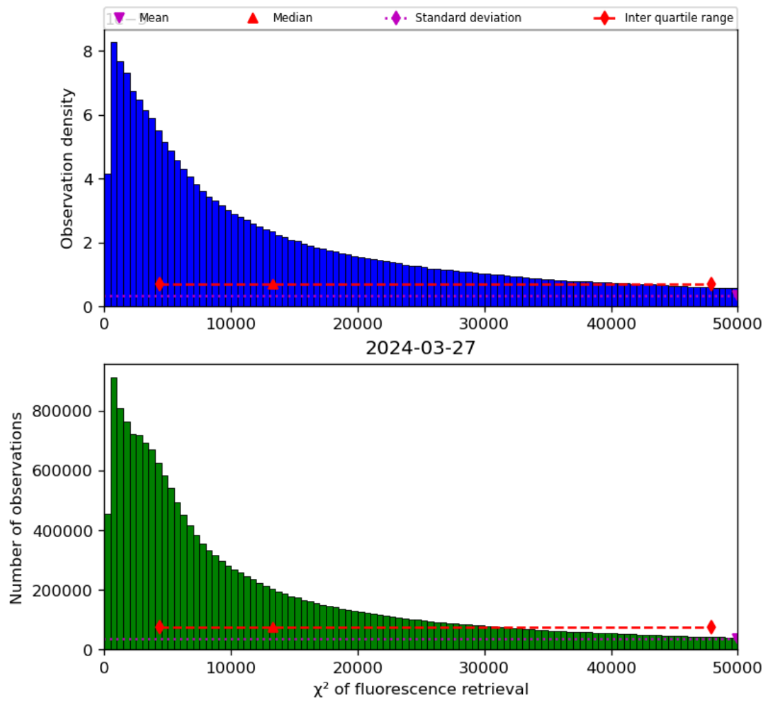
Figure 42: Histogram of “ \chi^2 of fluorescence retrieval” for 2024-03-26 to 2024-03-28
