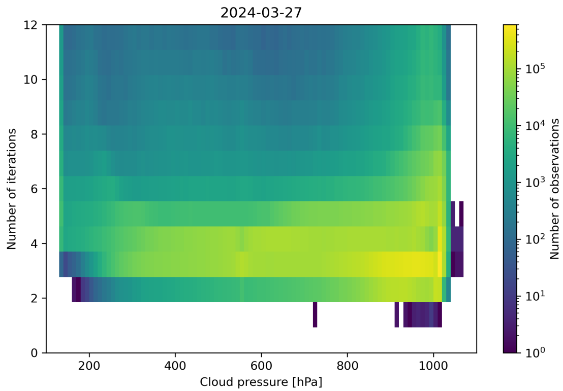
Figure 81: Scatter density plot of “Cloud pressure” against “Number of iterations” for 2024-03-26 to 2024-03-28.
