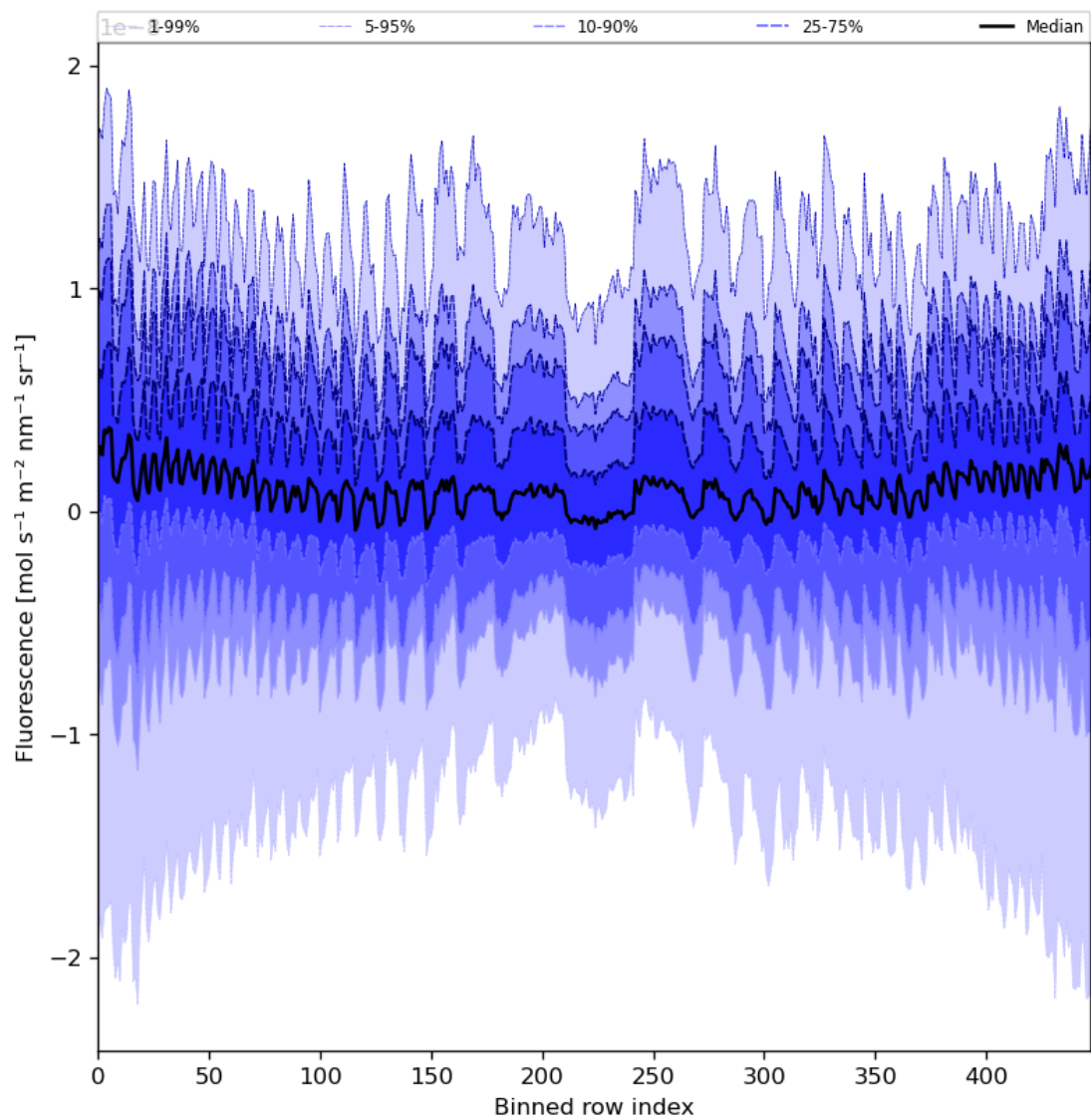
Figure 57: Along track statistics of “Fluorescence” for 2024-03-26 to 2024-03-28
