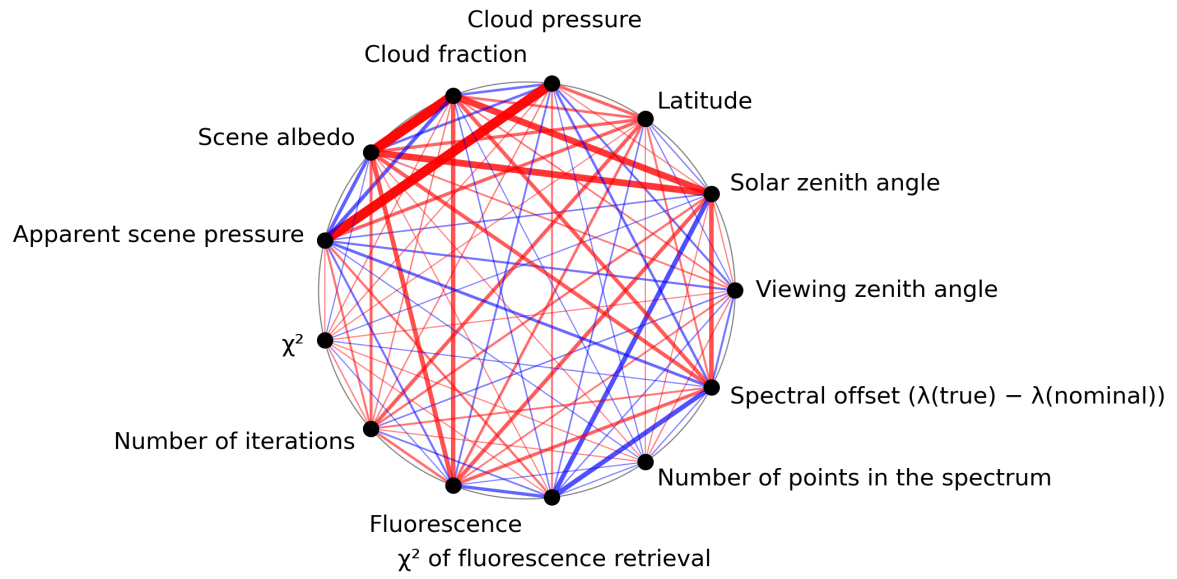
Figure 1: Map of correlation graph for 2024-03-26 to 2024-03-28.
