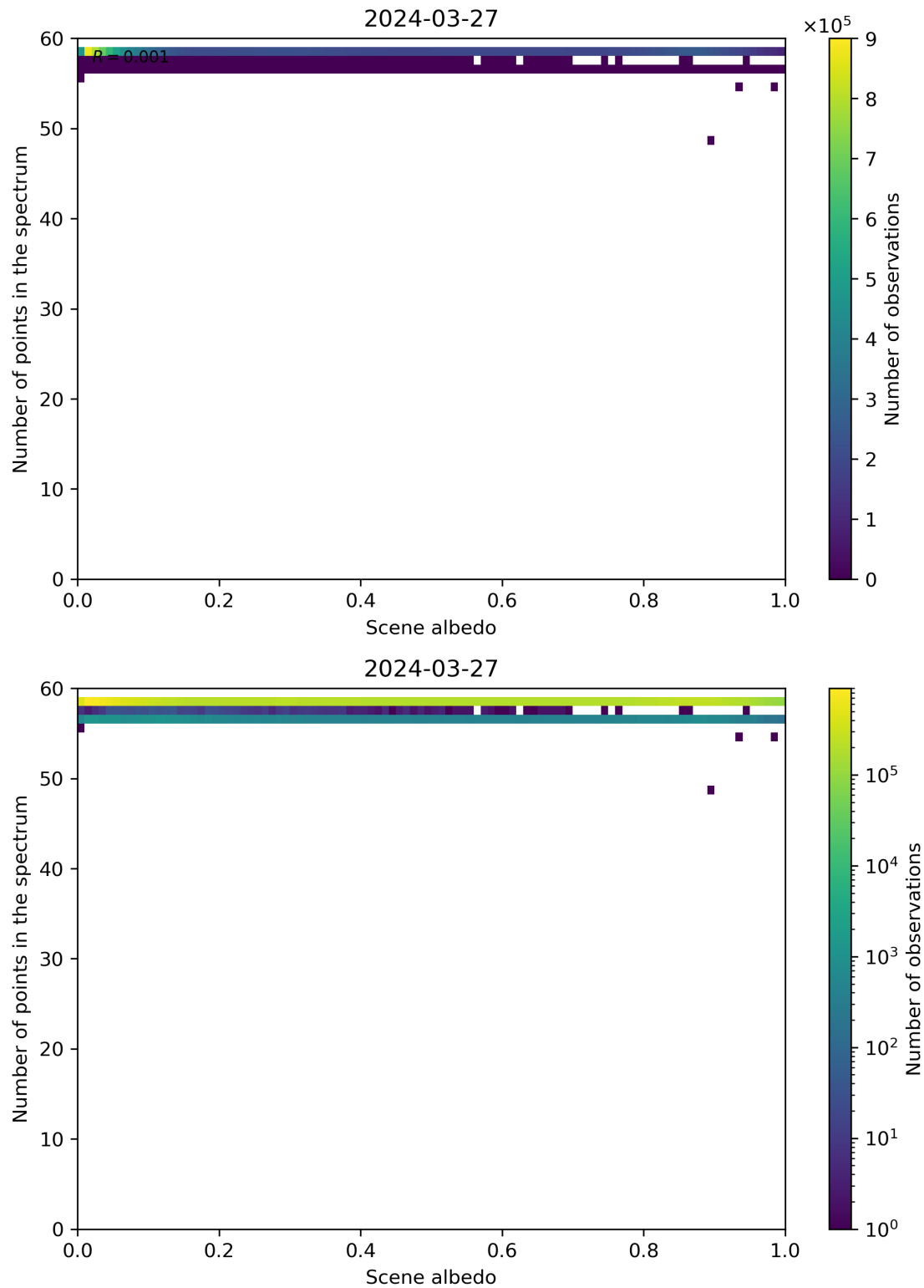
Figure 106: Scatter density plot of “Scene albedo” against “Number of points in the spectrum” for 2024-03-26 to 2024-03-28.
