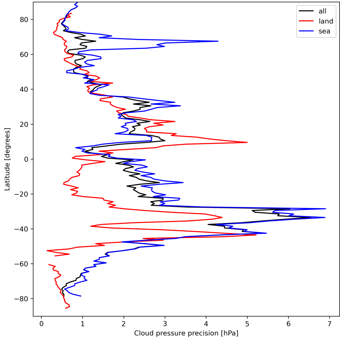
Figure 14: Zonal average of “Cloud pressure precision” for 2024-03-26 to 2024-03-28.
