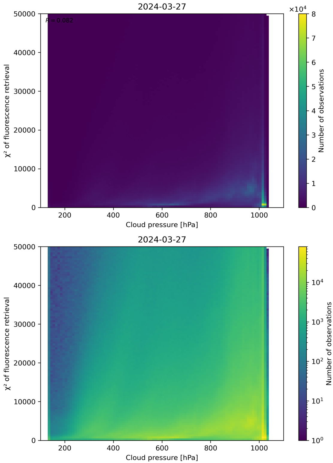
Figure 78: Scatter density plot of “Cloud pressure” against “ \chi^2 of fluorescence retrieval” for 2024-03-26 to 2024-03-28.
