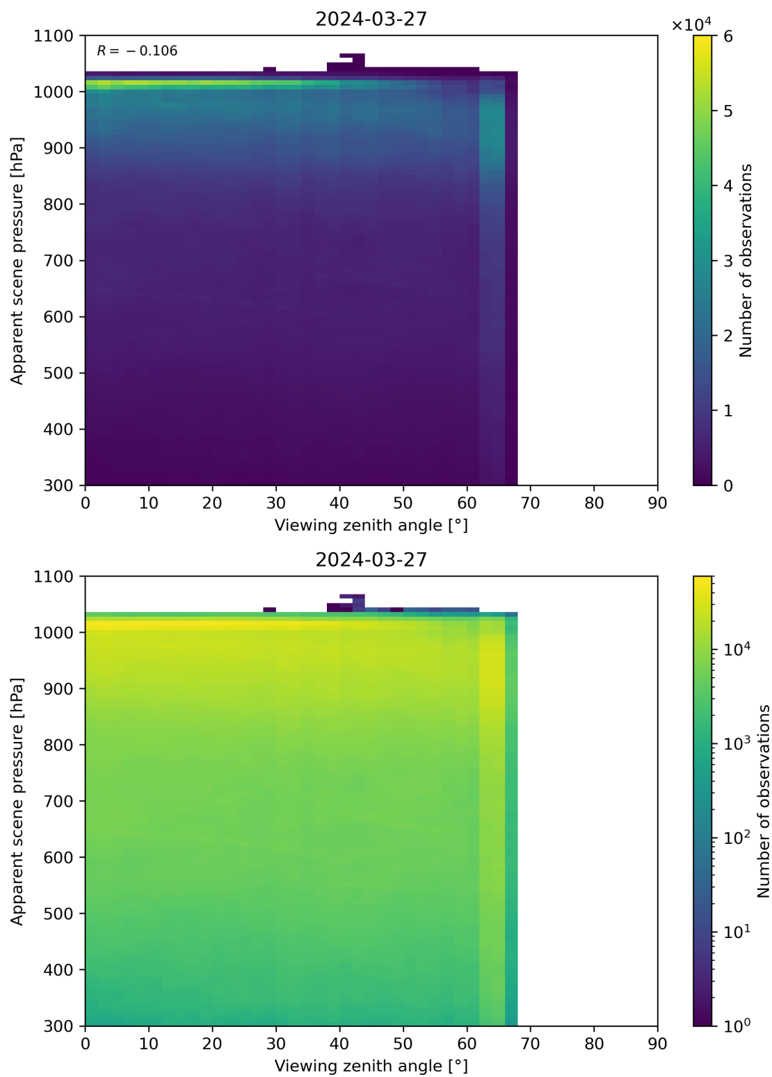
Figure 118: Scatter density plot of “Viewing zenith angle” against “Apparent scene pressure” for 2024-03-26 to 2024-03-28.
