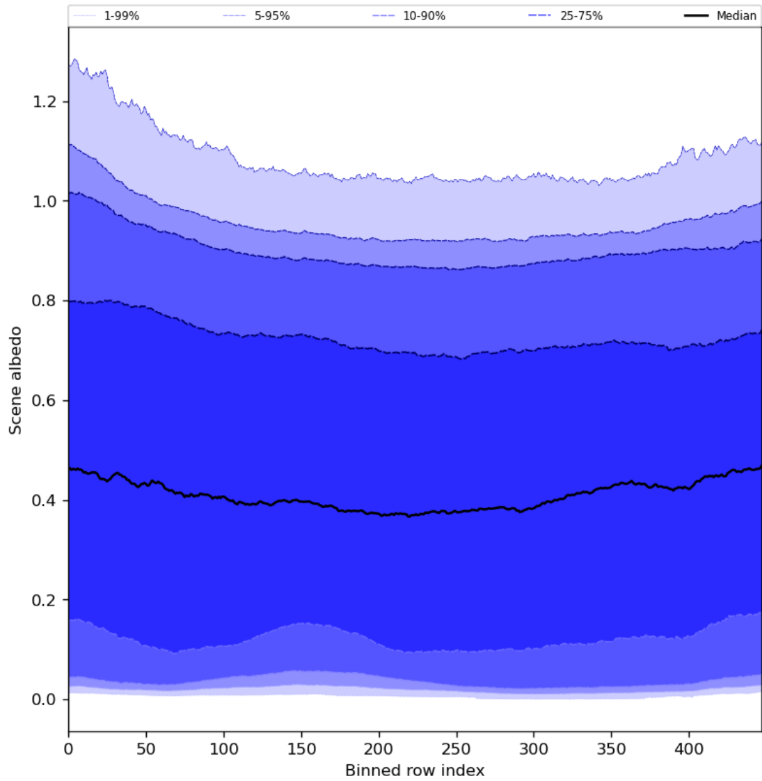
Figure 51: Along track statistics of “Scene albedo” for 2024-03-26 to 2024-03-28
