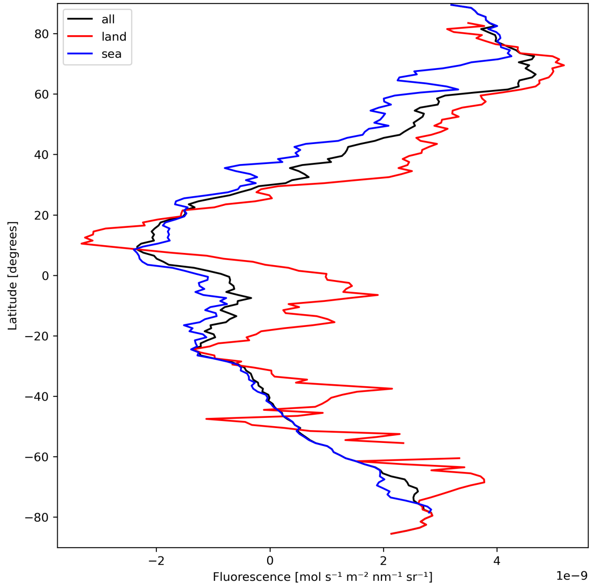
Figure 23: Zonal average of “Fluorescence” for 2024-03-26 to 2024-03-28.
