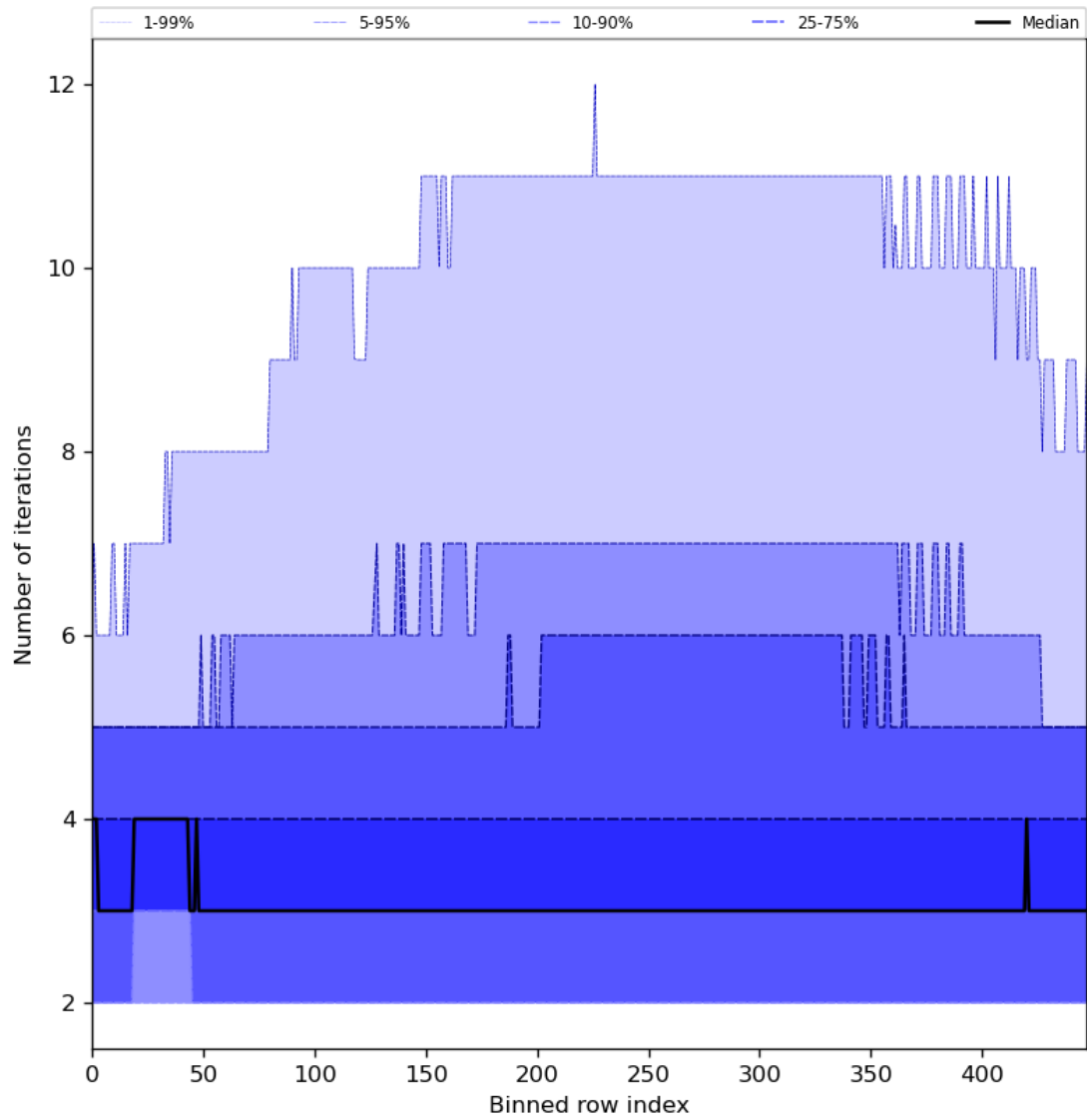
Figure 56: Along track statistics of “Number of iterations” for 2024-03-26 to 2024-03-28
