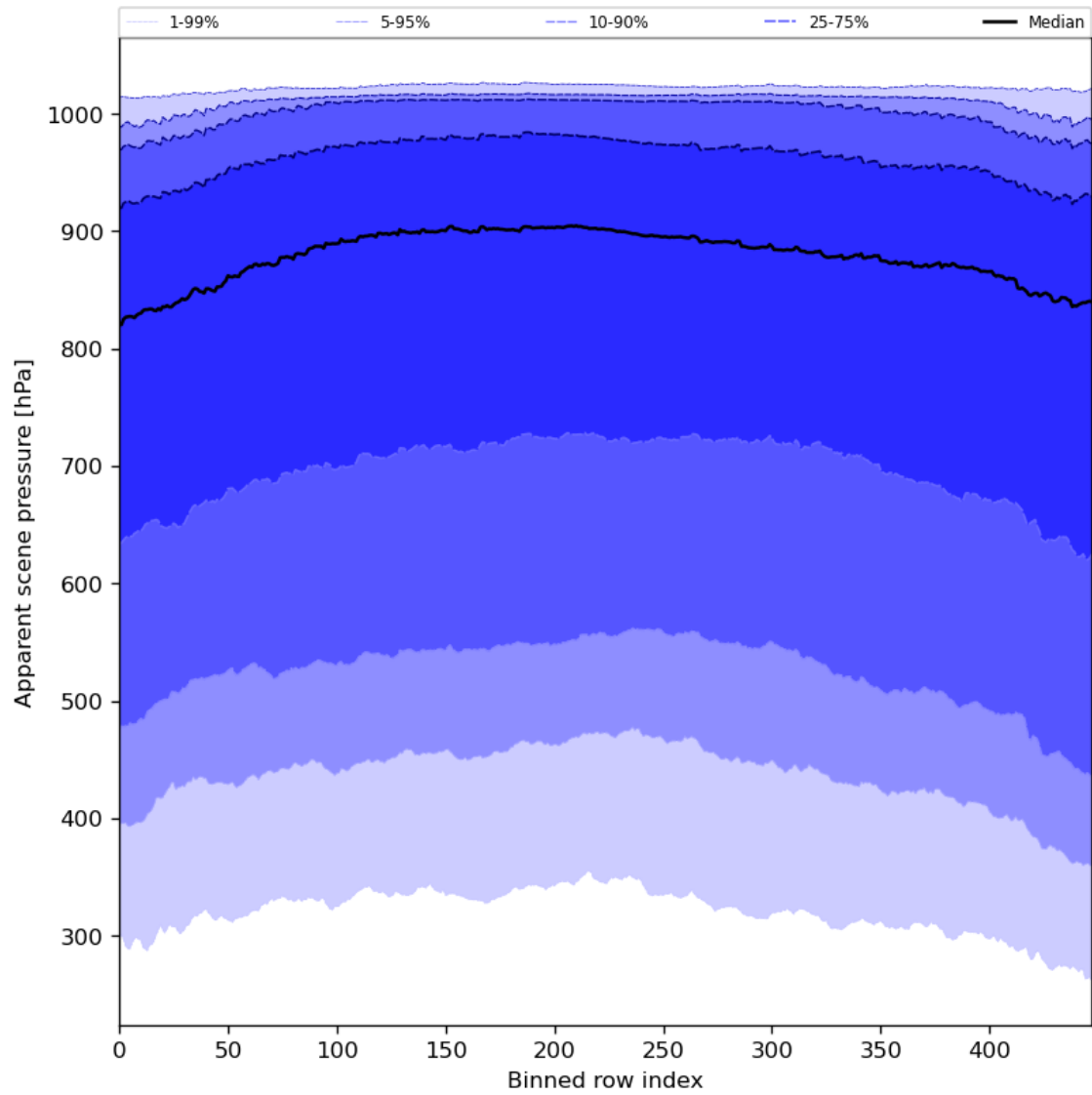
Figure 53: Along track statistics of “Apparent scene pressure” for 2024-03-26 to 2024-03-28
