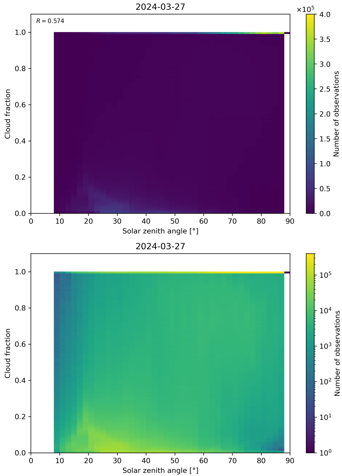
Figure 110: Scatter density plot of “Solar zenith angle” against “Cloud fraction” for 2024-03-26 to 2024-03-28.
