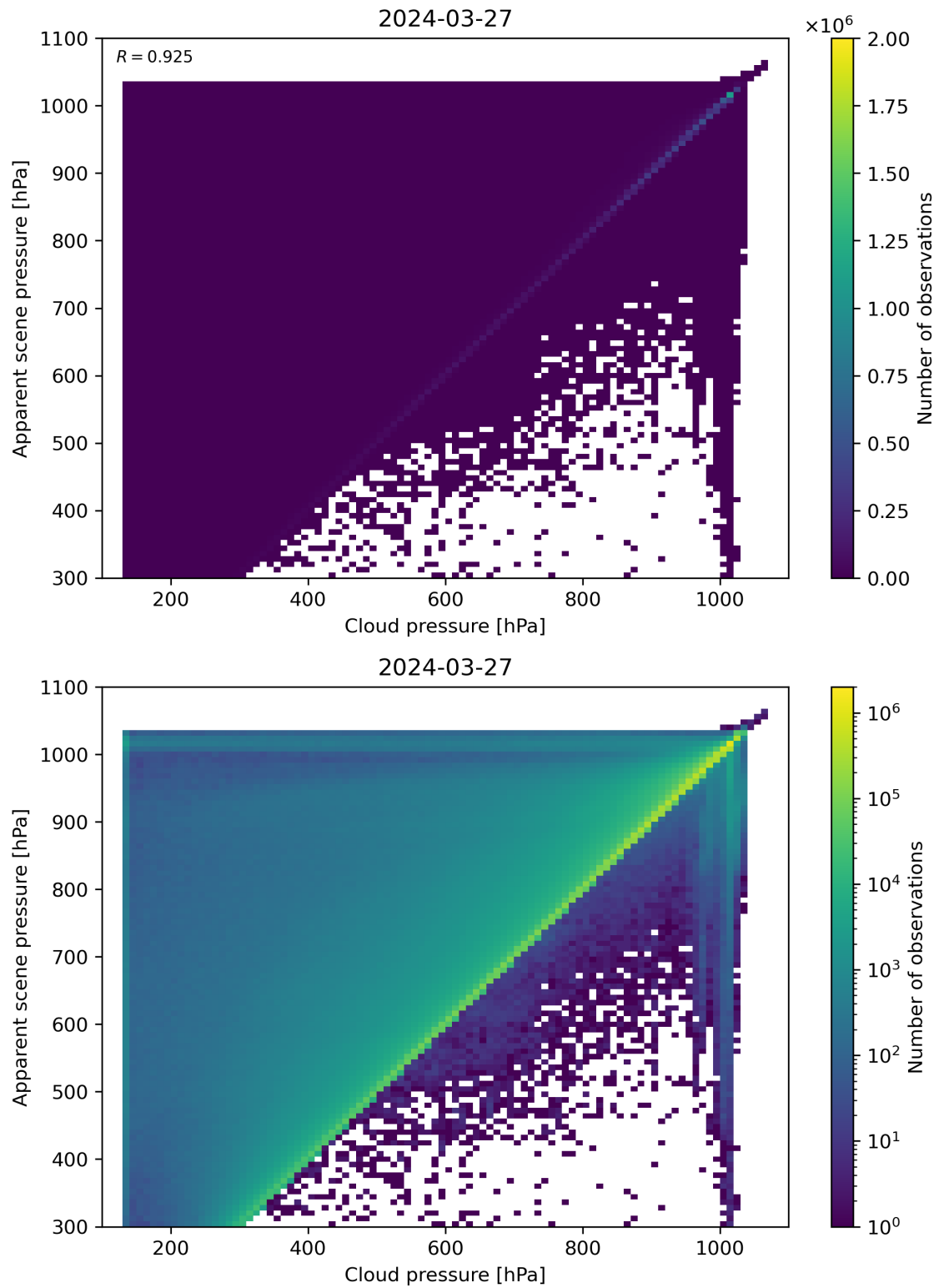
Figure 77: Scatter density plot of “Cloud pressure” against “Apparent scene pressure” for 2024-03-26 to 2024-03-28.
