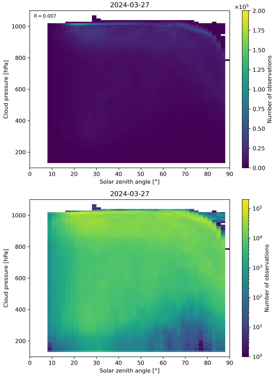
Figure 111: Scatter density plot of “Solar zenith angle” against “Cloud pressure” for 2024-03-26 to 2024-03-28.
