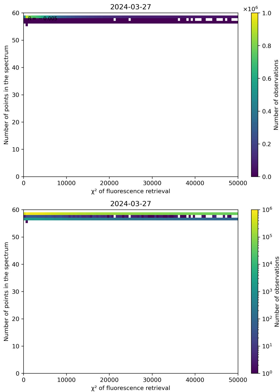
Figure 68: Scatter density plot of “ \chi^2 of fluorescence retrieval” against “Number of points in the spectrum” for 2024-03-26 to 2024-03-28.
