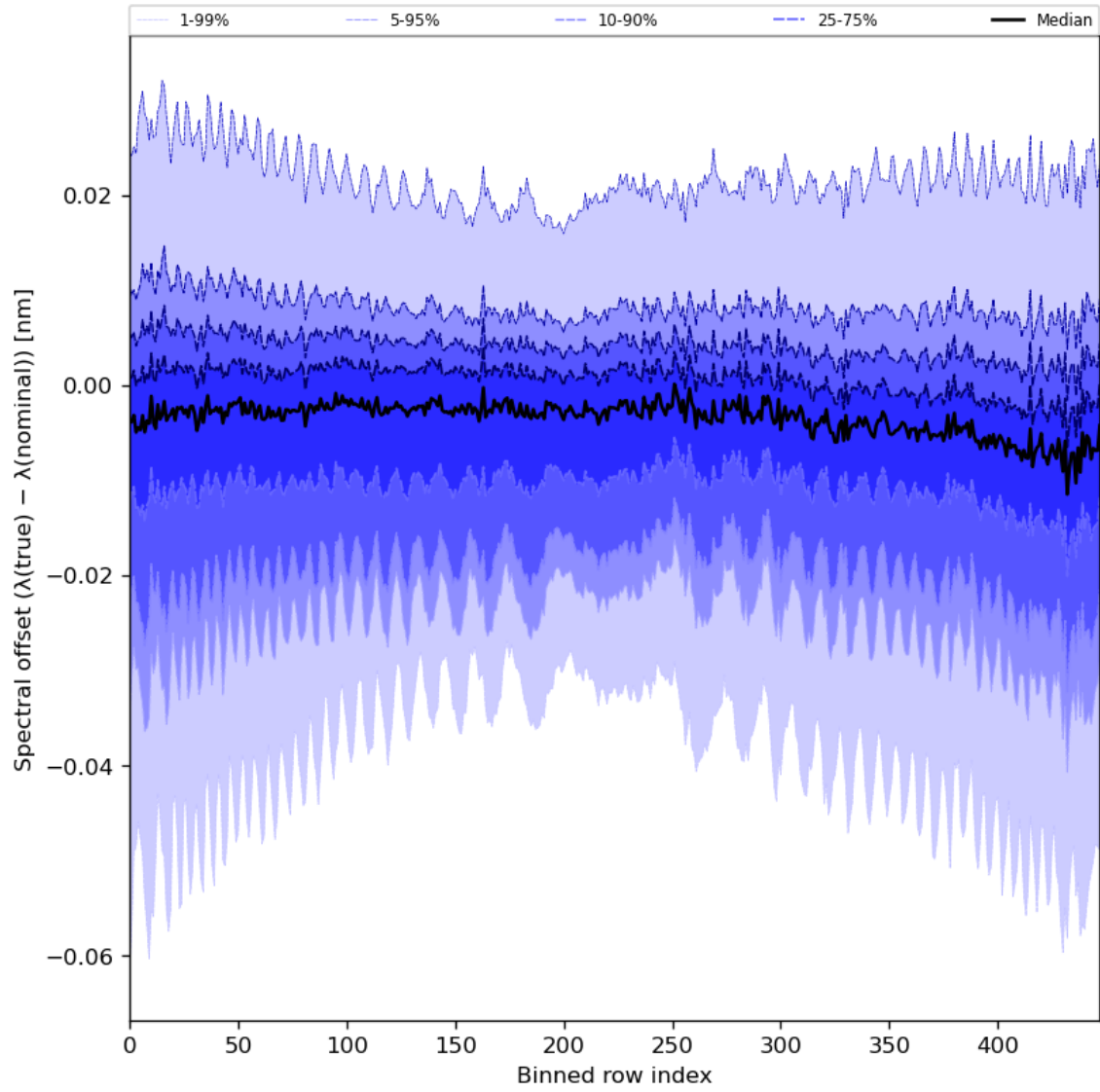
Figure 62: Along track statistics of “Spectral offset ( \lambda(\text{true}) - \lambda(\text{nominal}) )” for 2024-03-26 to 2024-03-28
