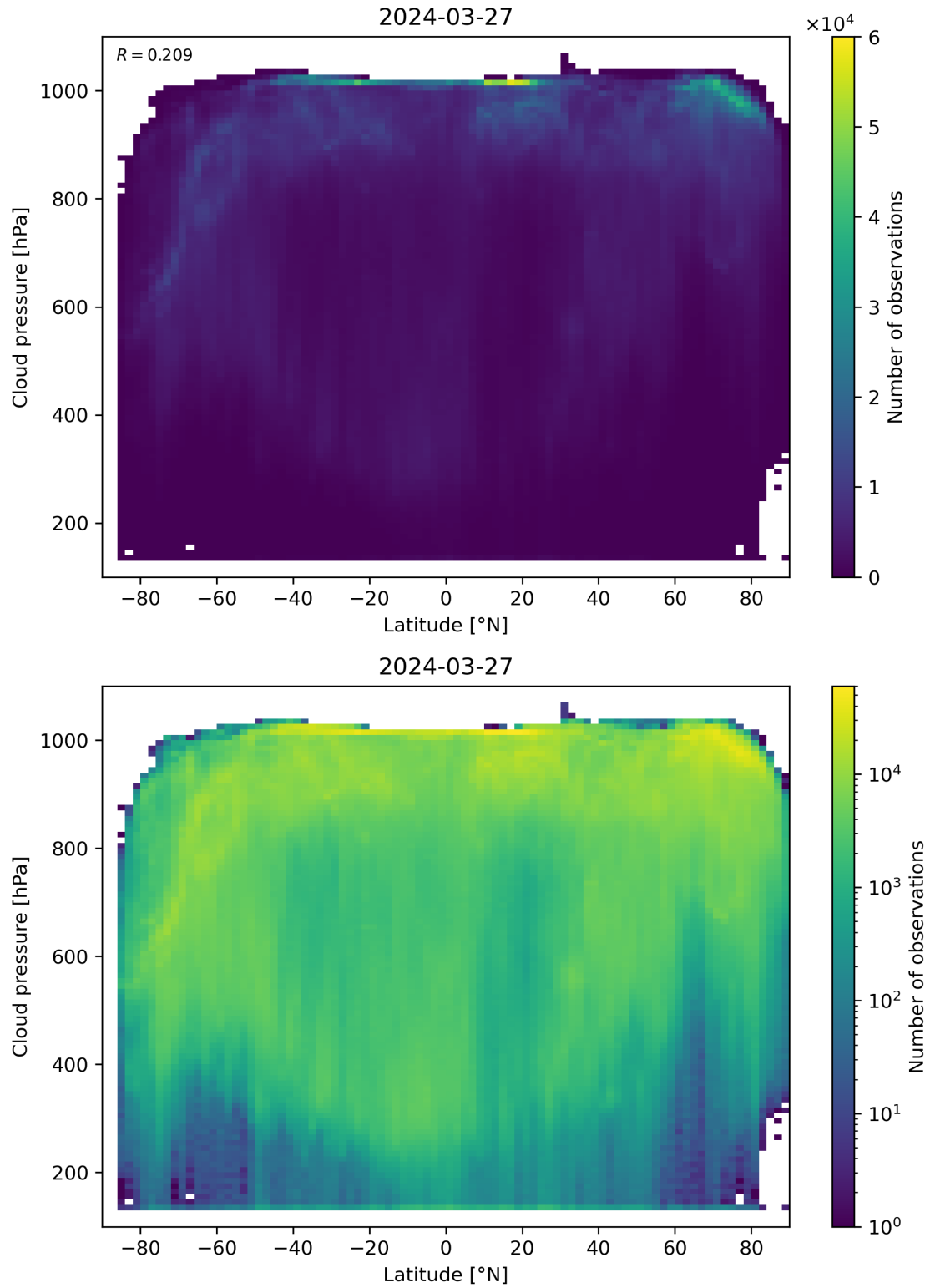
Figure 91: Scatter density plot of “Latitude” against “Cloud pressure” for 2024-03-26 to 2024-03-28.
