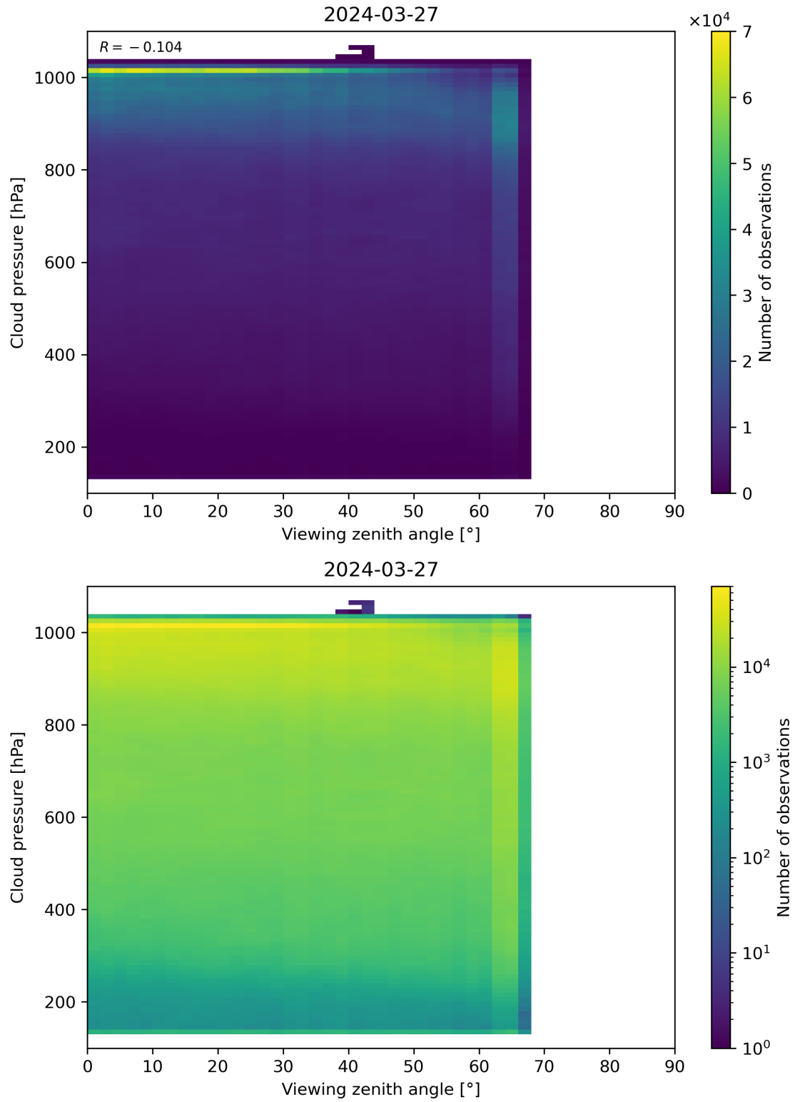
Figure 121: Scatter density plot of “Viewing zenith angle” against “Cloud pressure” for 2024-03-26 to 2024-03-28.
