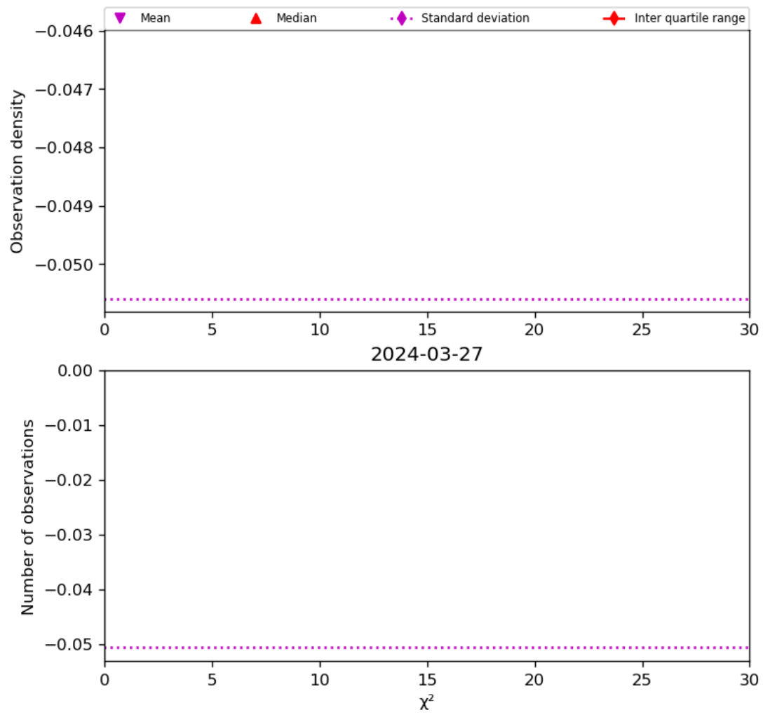
Figure 38: Histogram of “ \chi^2 ” for 2024-03-26 to 2024-03-28
