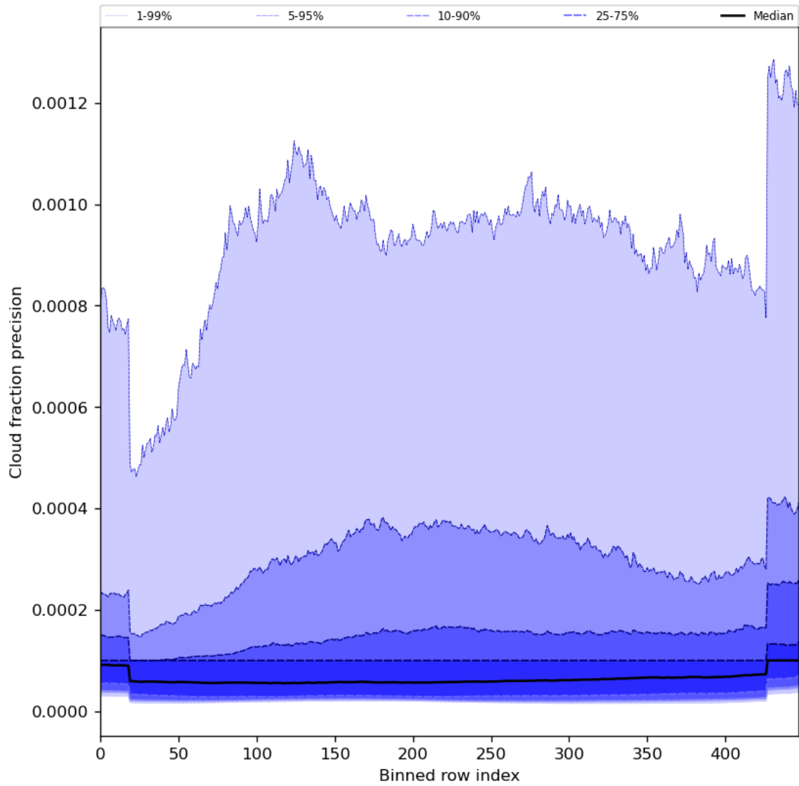
Figure 50: Along track statistics of “Cloud fraction precision” for 2024-03-26 to 2024-03-28
