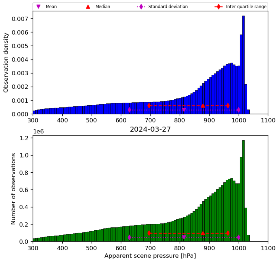
Figure 36: Histogram of “Apparent scene pressure” for 2024-03-26 to 2024-03-28
