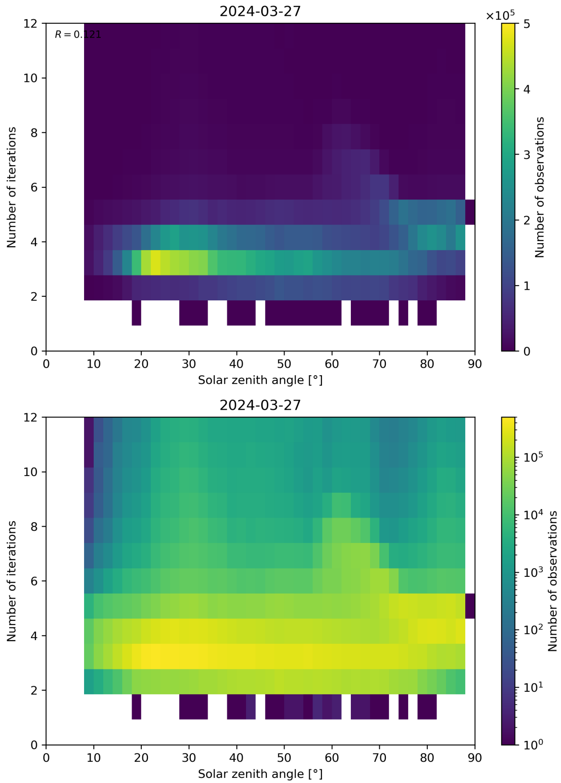
Figure 114: Scatter density plot of “Solar zenith angle” against “Number of iterations” for 2024-03-26 to 2024-03-28.
