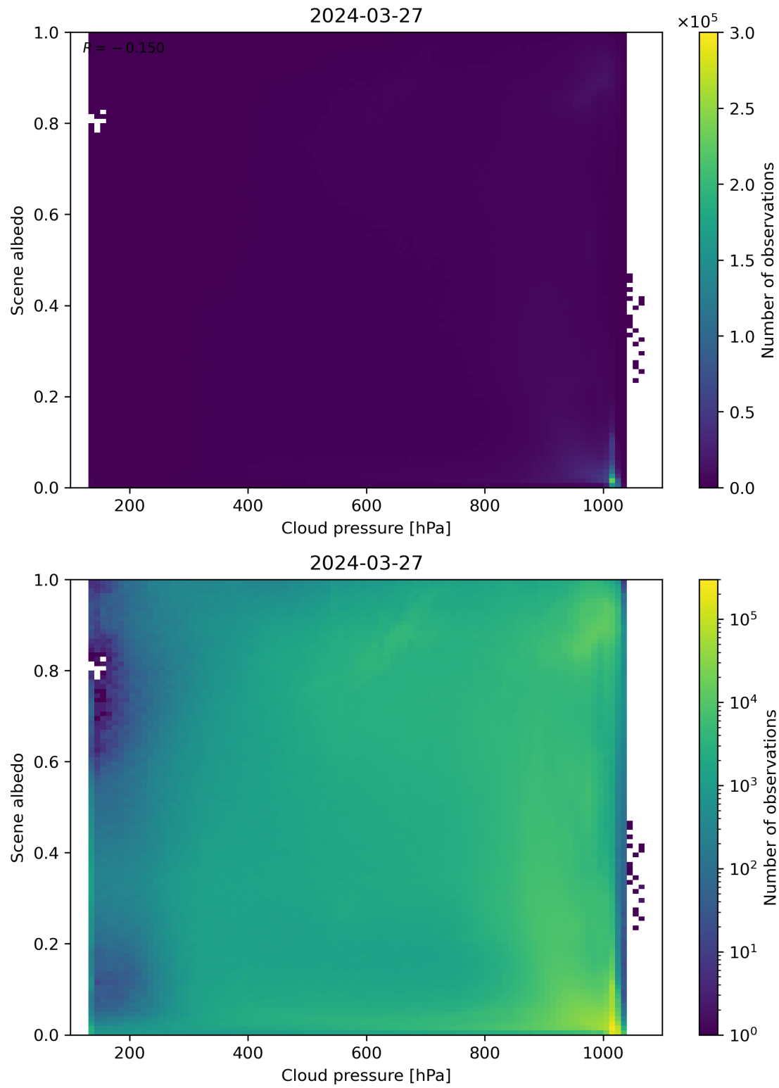
Figure 83: Scatter density plot of “Cloud pressure” against “Scene albedo” for 2024-03-26 to 2024-03-28.
