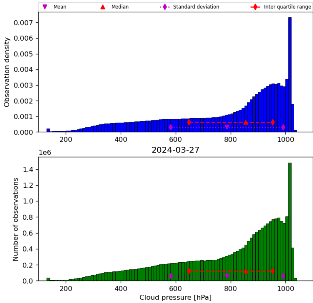
Figure 30: Histogram of “Cloud pressure” for 2024-03-26 to 2024-03-28
