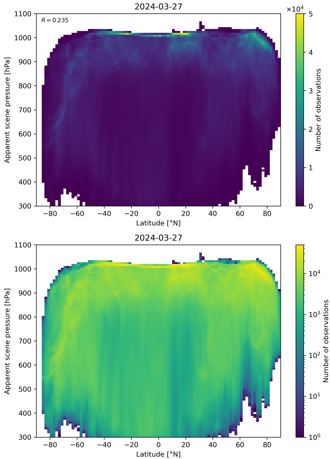
Figure 88: Scatter density plot of “Latitude” against “Apparent scene pressure” for 2024-03-26 to 2024-03-28.
