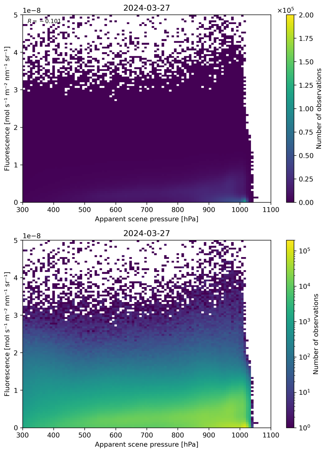
Figure 64: Scatter density plot of “Apparent scene pressure” against “Fluorescence” for 2024-03-26 to 2024-03-28.
