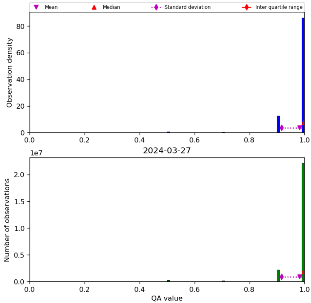
Figure 29: Histogram of “QA value” for 2024-03-26 to 2024-03-28
