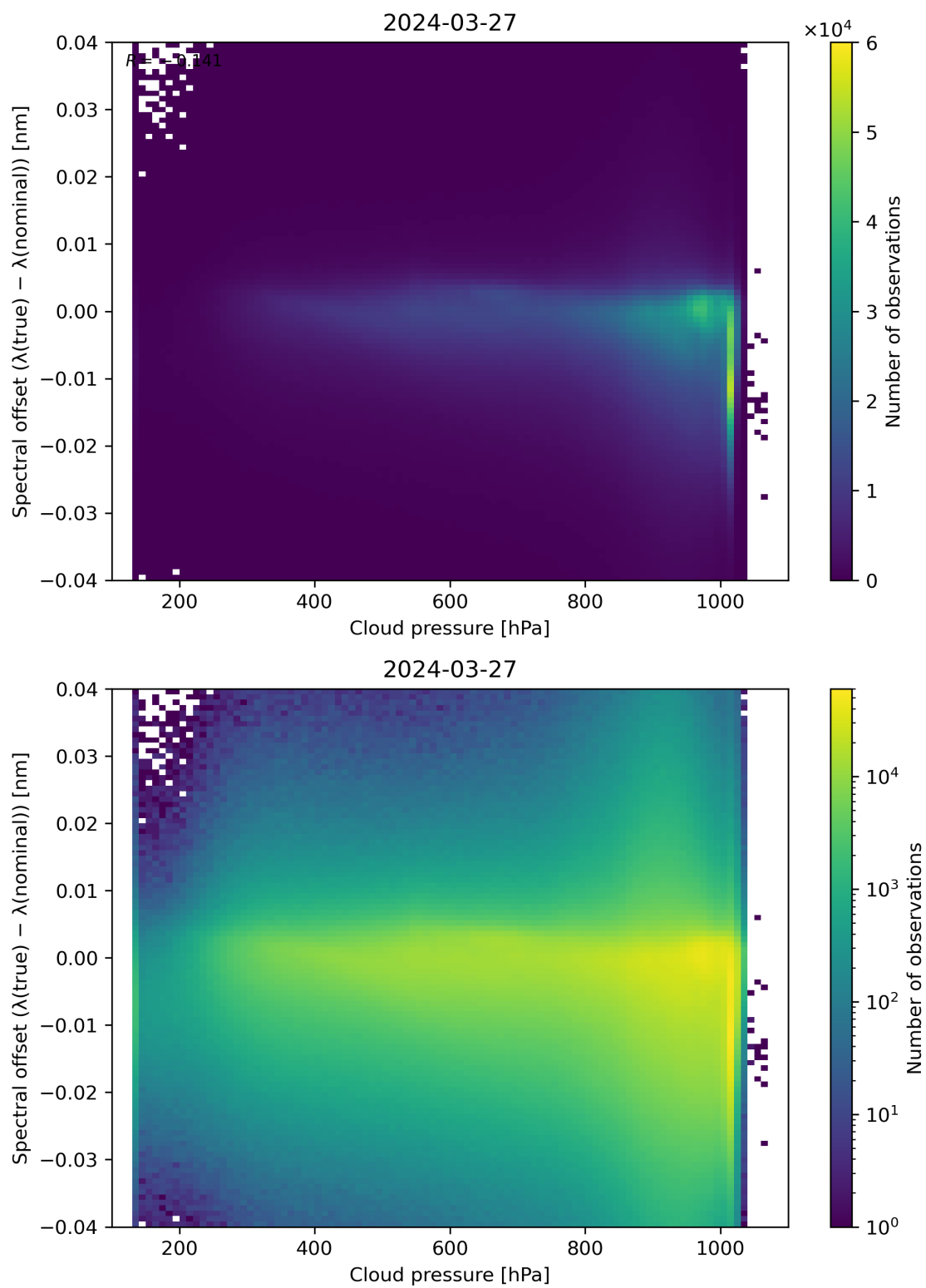
Figure 84: Scatter density plot of “Cloud pressure” against “Spectral offset ( \lambda(\text{true}) - \lambda(\text{nominal}) )” for 2024-03-26 to 2024-03-28.
