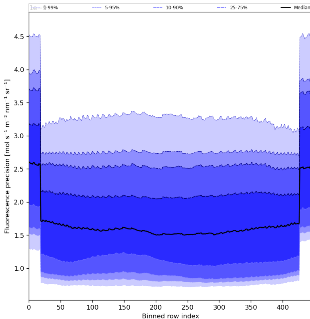
Figure 58: Along track statistics of “Fluorescence precision” for 2024-03-26 to 2024-03-28
