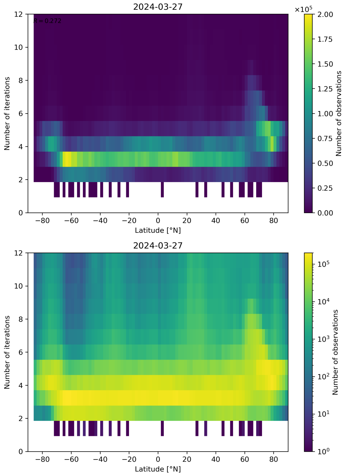
Figure 93: Scatter density plot of “Latitude” against “Number of iterations” for 2024-03-26 to 2024-03-28.
