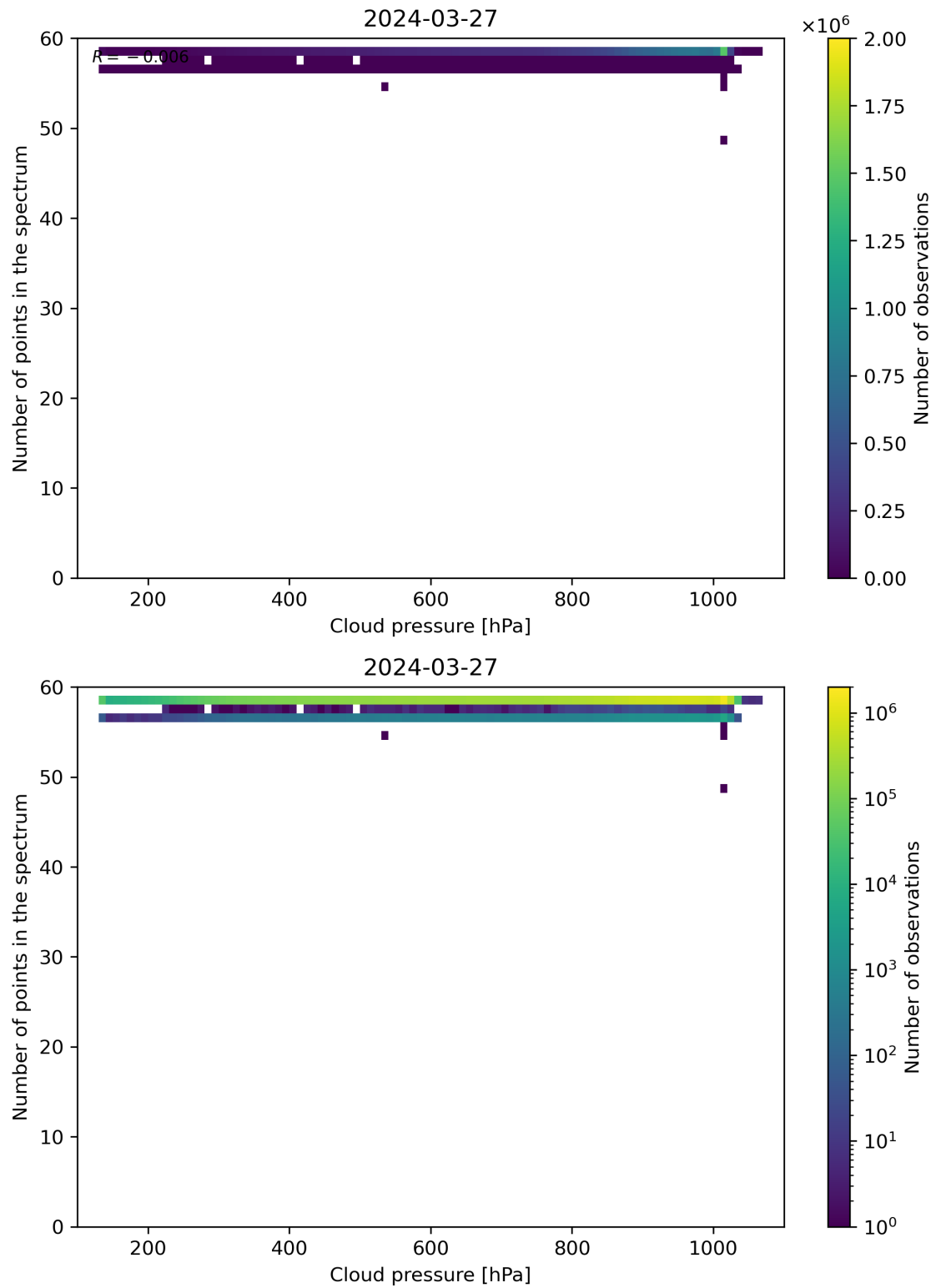
Figure 82: Scatter density plot of “Cloud pressure” against “Number of points in the spectrum” for 2024-03-26 to 2024-03-28.
