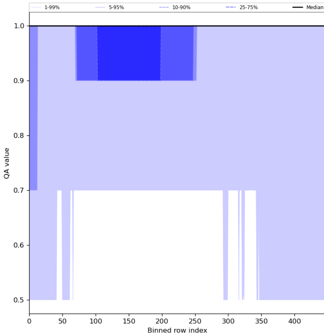
Figure 46: Along track statistics of “QA value” for 2024-03-26 to 2024-03-28
