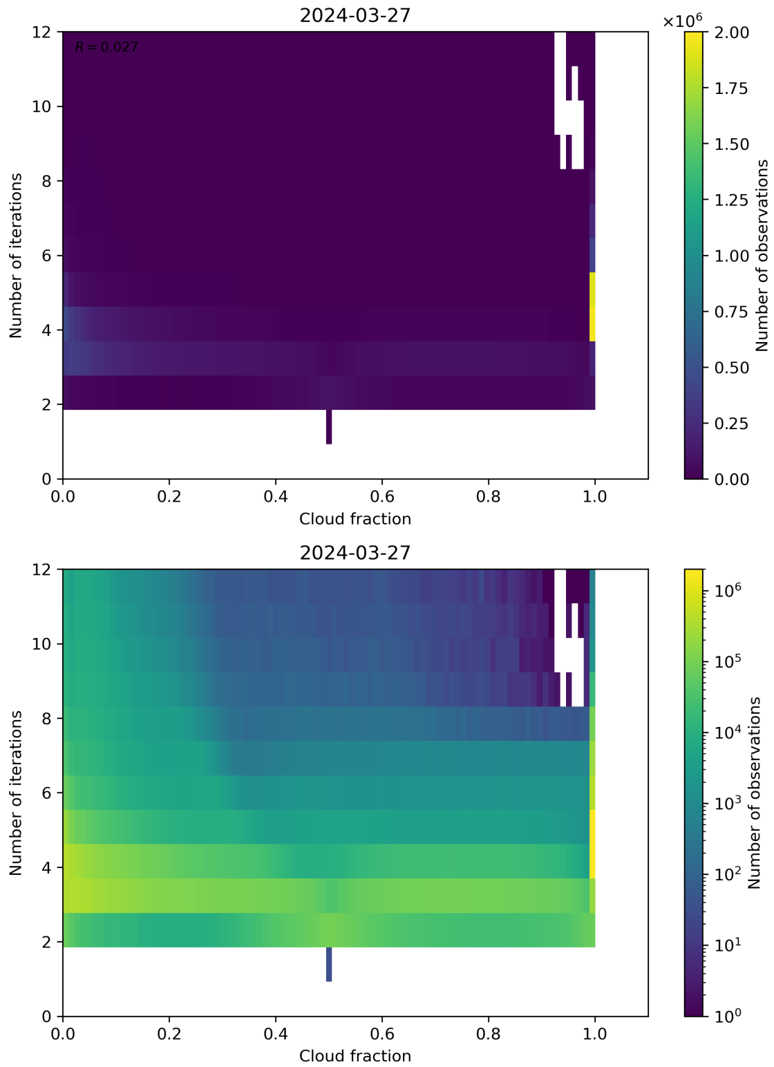
Figure 73: Scatter density plot of “Cloud fraction” against “Number of iterations” for 2024-03-26 to 2024-03-28.
