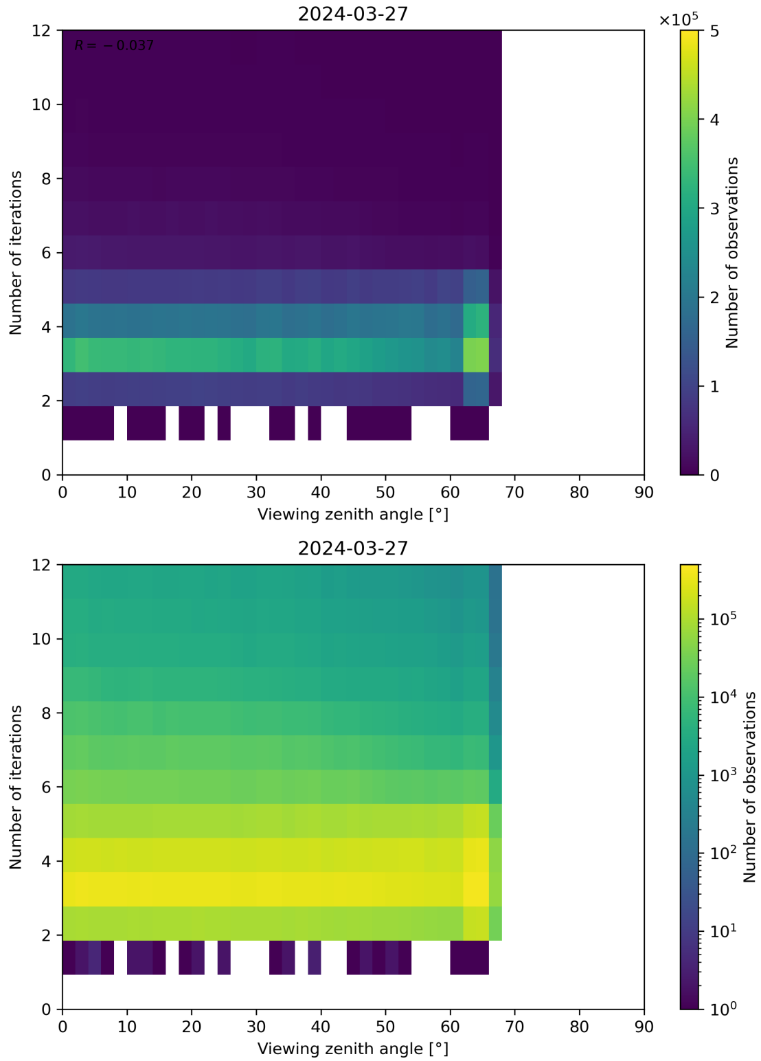
Figure 124: Scatter density plot of “Viewing zenith angle” against “Number of iterations” for 2024-03-26 to 2024-03-28.
