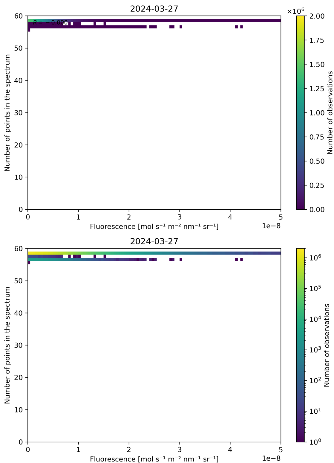
Figure 86: Scatter density plot of “Fluorescence” against “Number of points in the spectrum” for 2024-03-26 to 2024-03-28.
