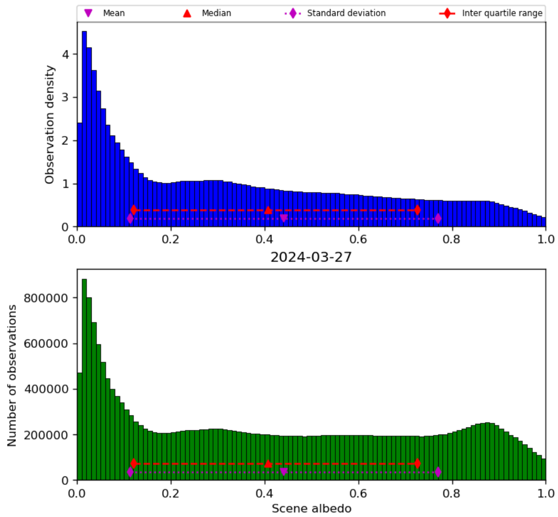
Figure 34: Histogram of “Scene albedo” for 2024-03-26 to 2024-03-28
