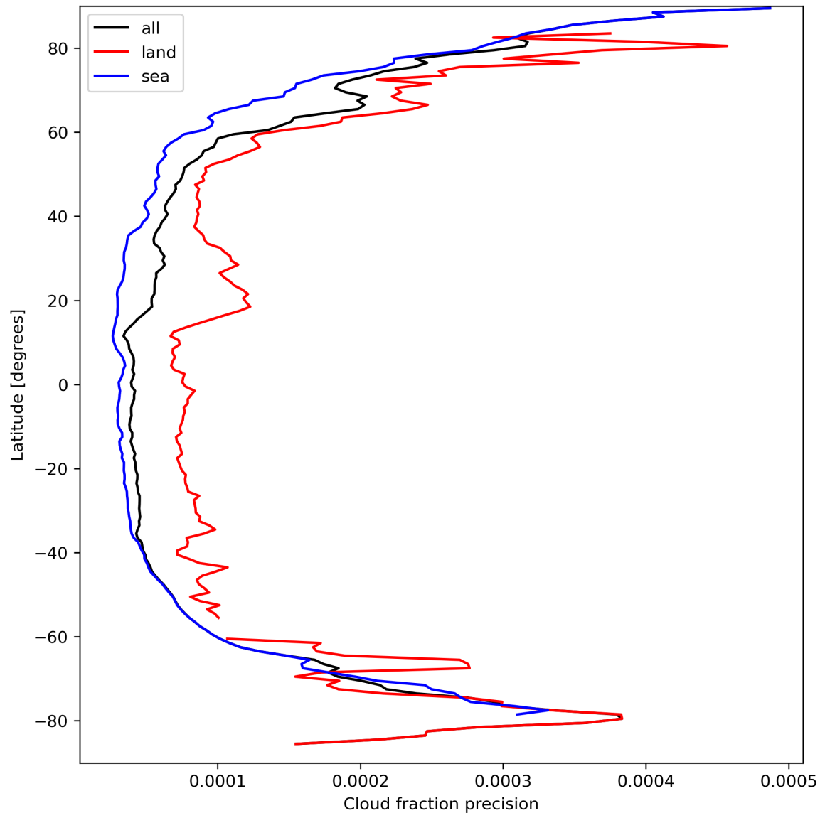
Figure 16: Zonal average of “Cloud fraction precision” for 2024-03-26 to 2024-03-28.
