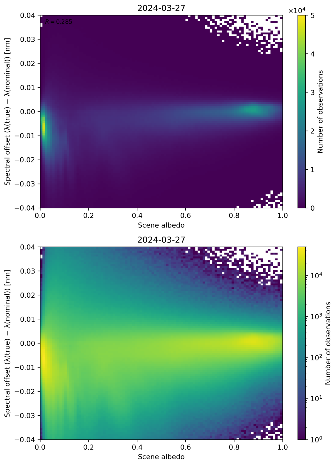
Figure 107: Scatter density plot of “Scene albedo” against “Spectral offset ( \lambda(\text{true}) - \lambda(\text{nominal}) )” for 2024-03-26 to 2024-03-28.
