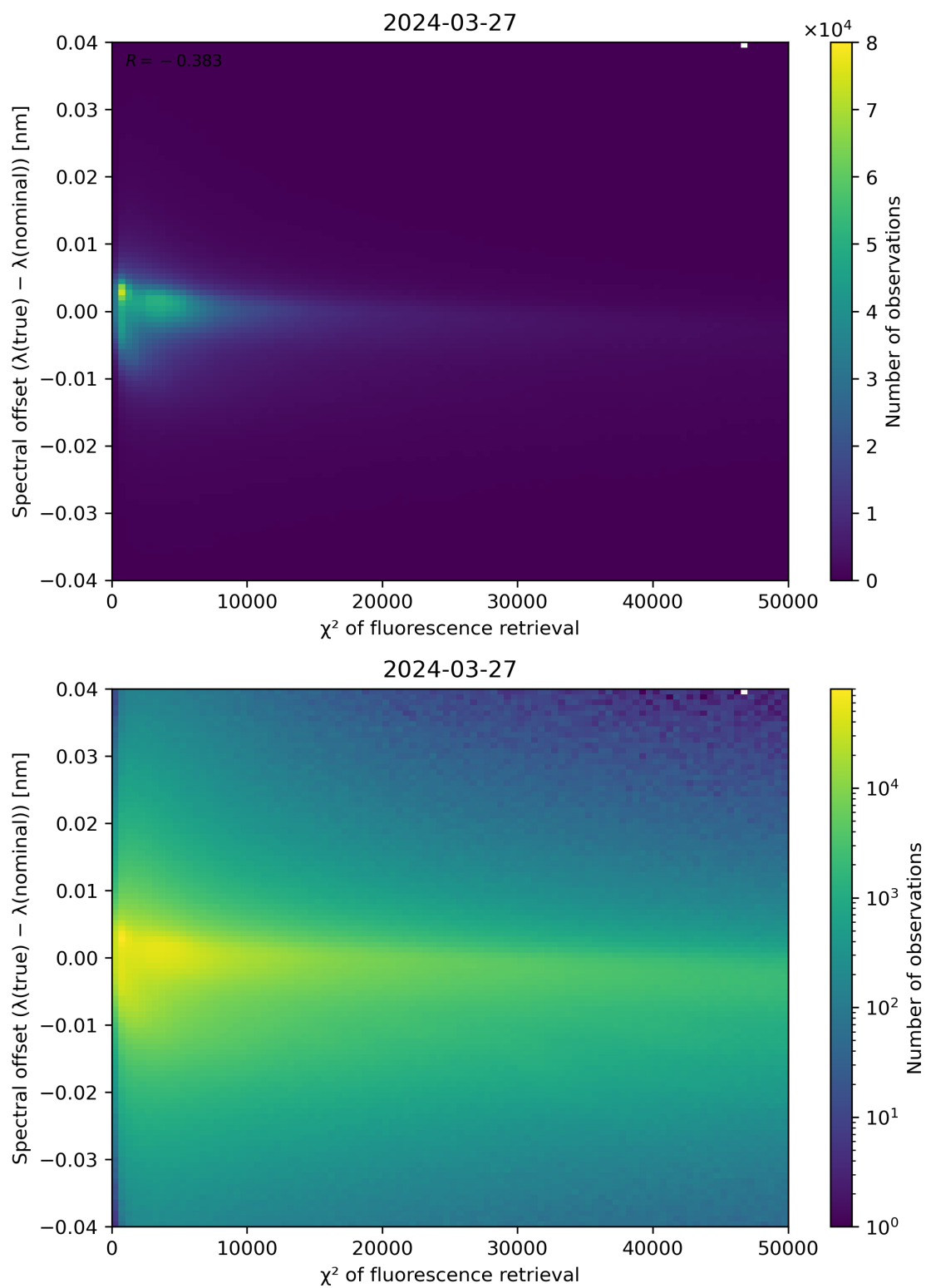
Figure 69: Scatter density plot of " \chi^2 of fluorescence retrieval" against "Spectral offset ( \lambda(\text{true}) - \lambda(\text{nominal})) " for 2024-03-26 to 2024-03-28.
