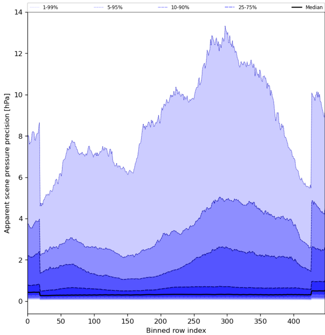
Figure 54: Along track statistics of “Apparent scene pressure precision” for 2024-03-26 to 2024-03-28
