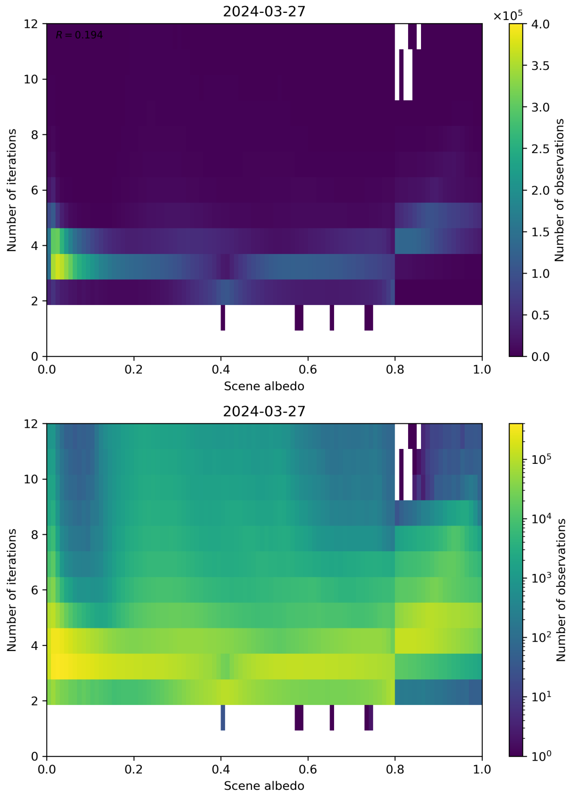
Figure 105: Scatter density plot of “Scene albedo” against “Number of iterations” for 2024-03-26 to 2024-03-28.
