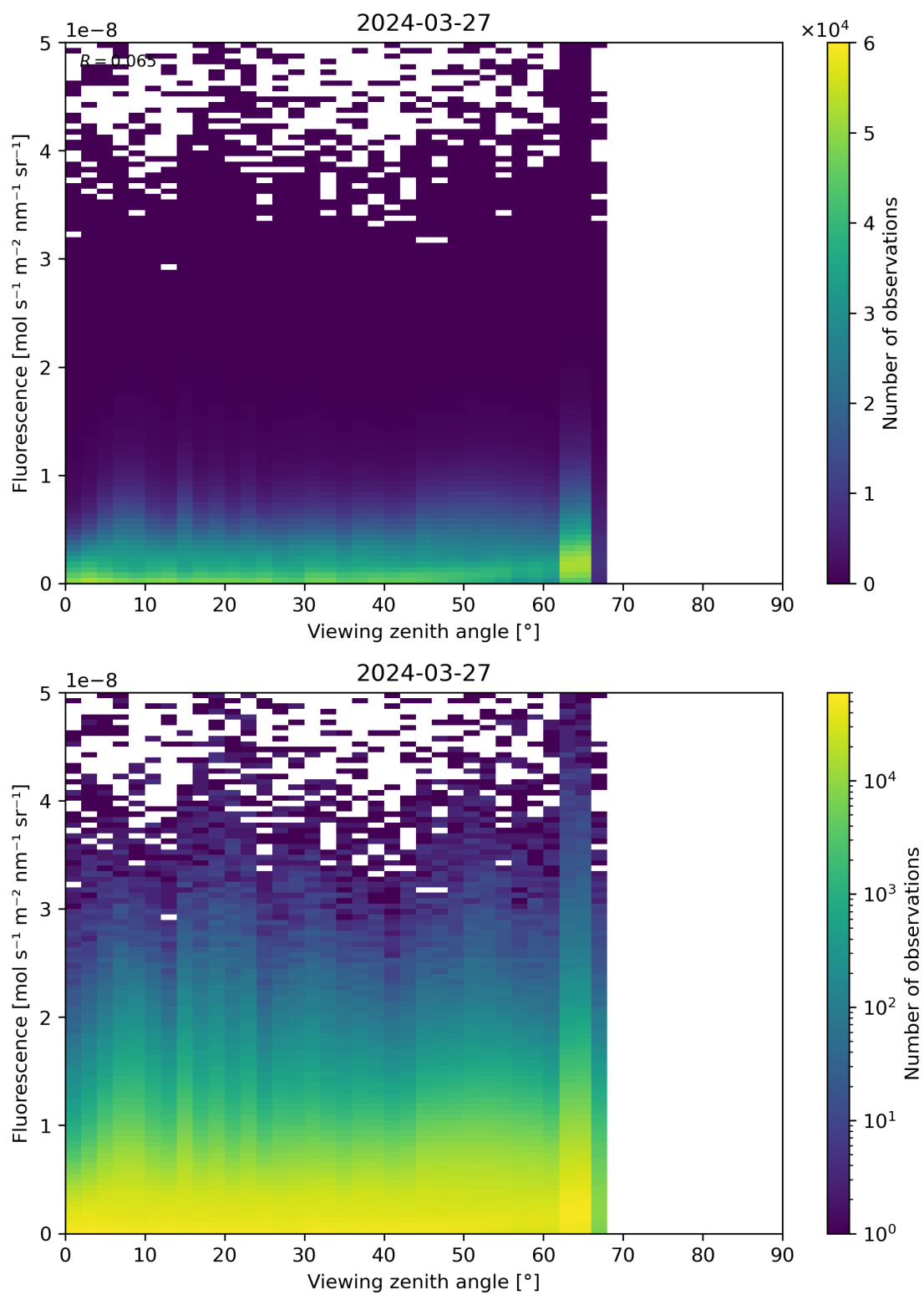
Figure 122: Scatter density plot of “Viewing zenith angle” against “Fluorescence” for 2024-03-26 to 2024-03-28.
