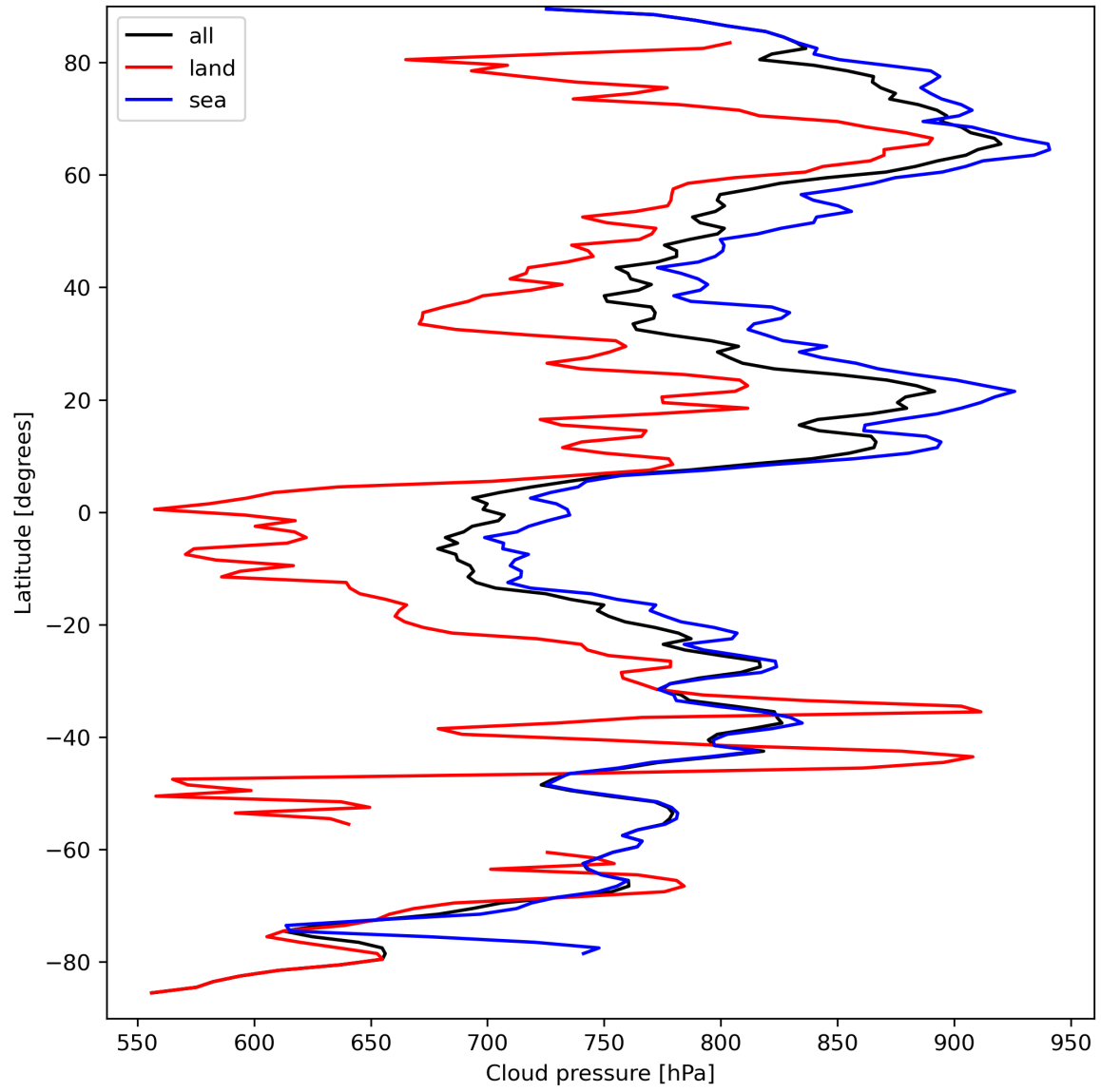
Figure 13: Zonal average of “Cloud pressure” for 2024-03-26 to 2024-03-28.
