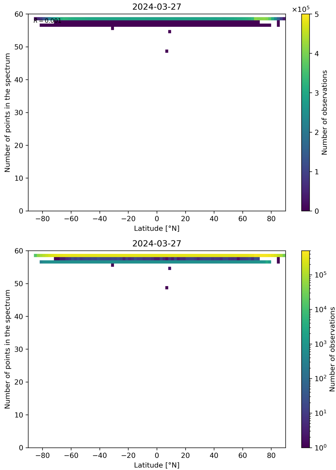
Figure 94: Scatter density plot of “Latitude” against “Number of points in the spectrum” for 2024-03-26 to 2024-03-28.
