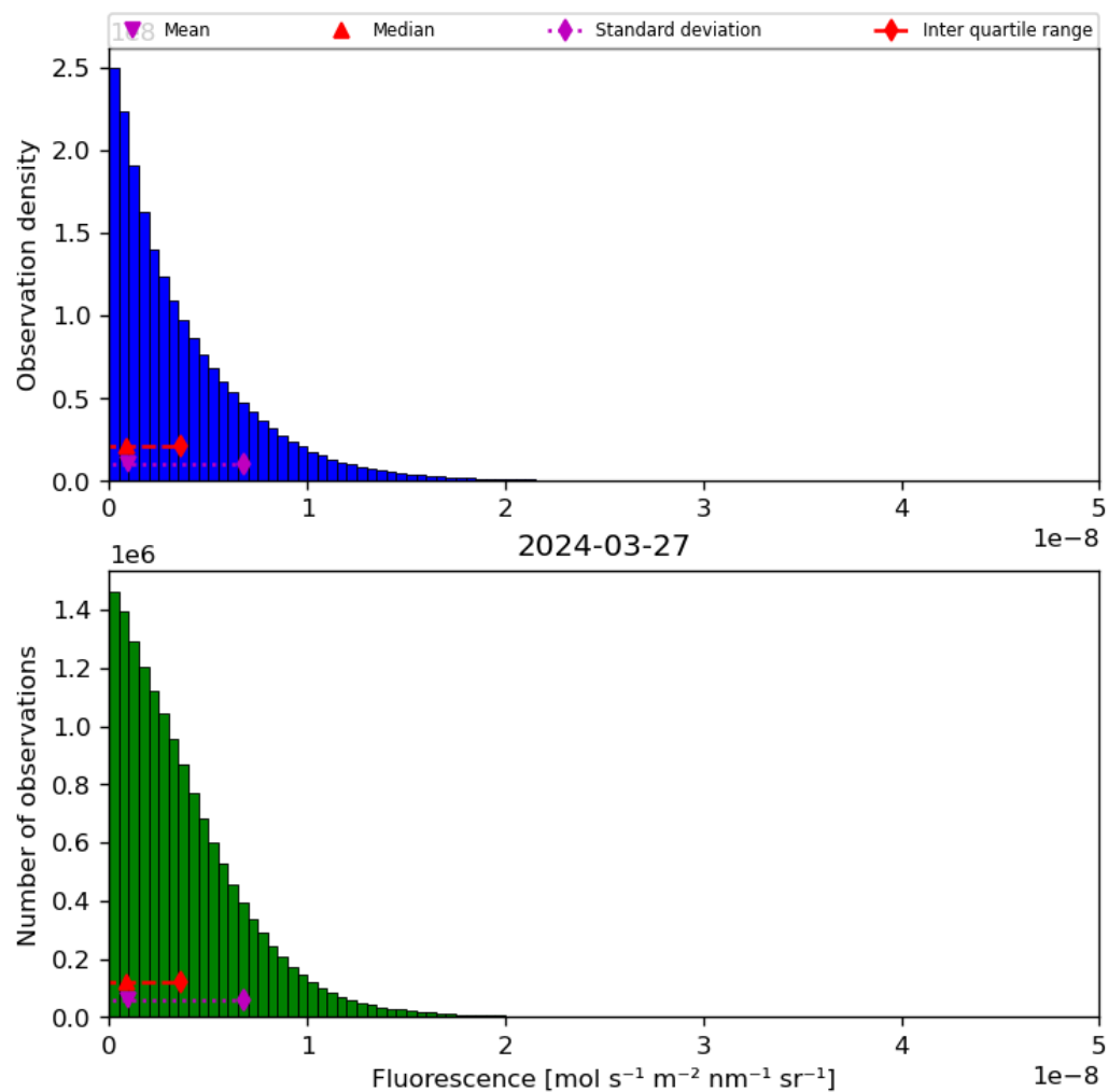
Figure 40: Histogram of “Fluorescence” for 2024-03-26 to 2024-03-28
