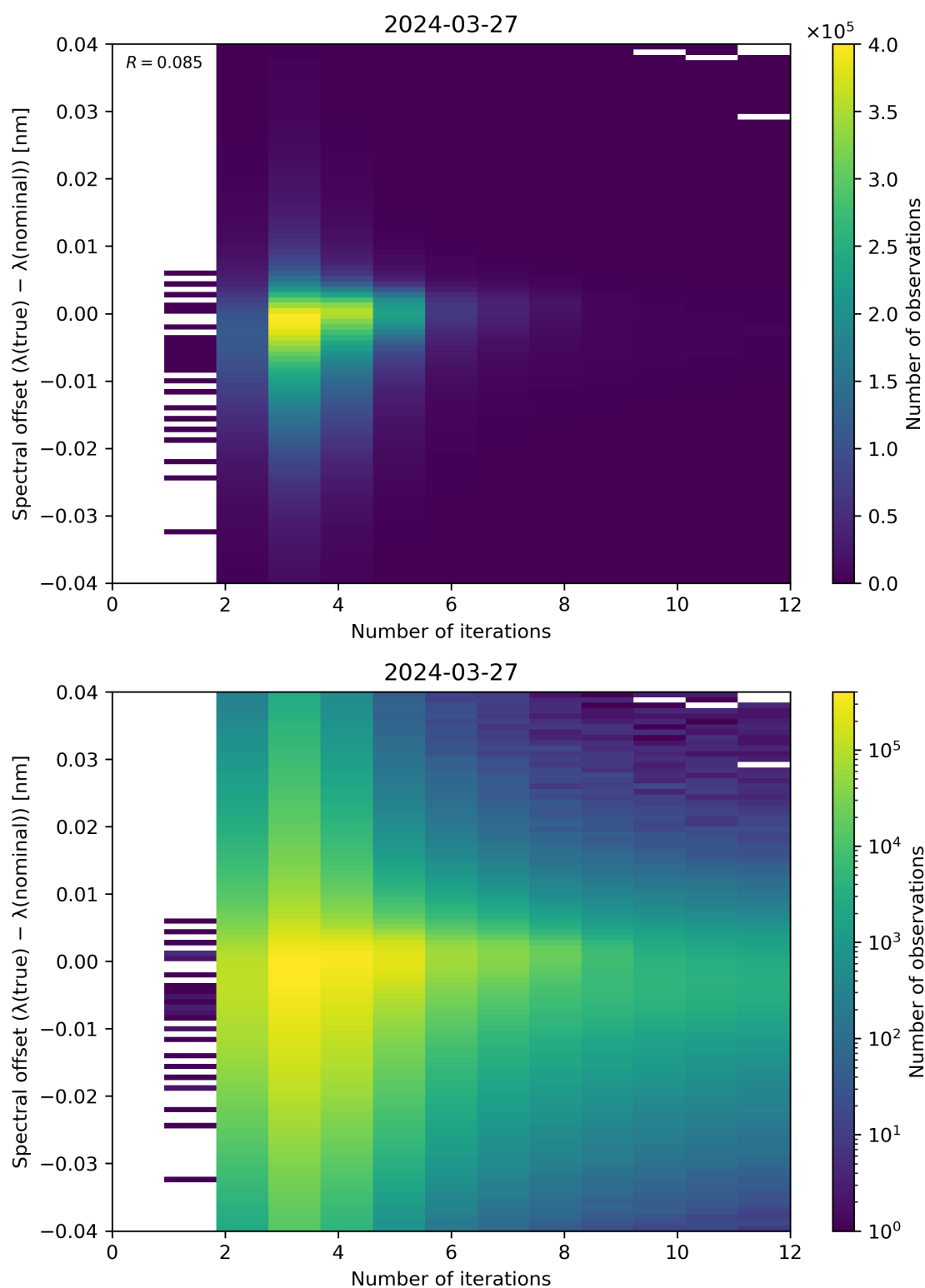
Figure 100: Scatter density plot of “Number of iterations” against “Spectral offset ( \lambda(\text{true}) - \lambda(\text{nominal}) )” for 2024-03-26 to 2024-03-28.
