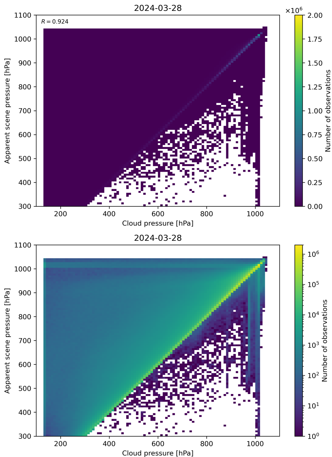
Figure 77: Scatter density plot of “Cloud pressure” against “Apparent scene pressure” for 2024-03-27 to 2024-03-29.
