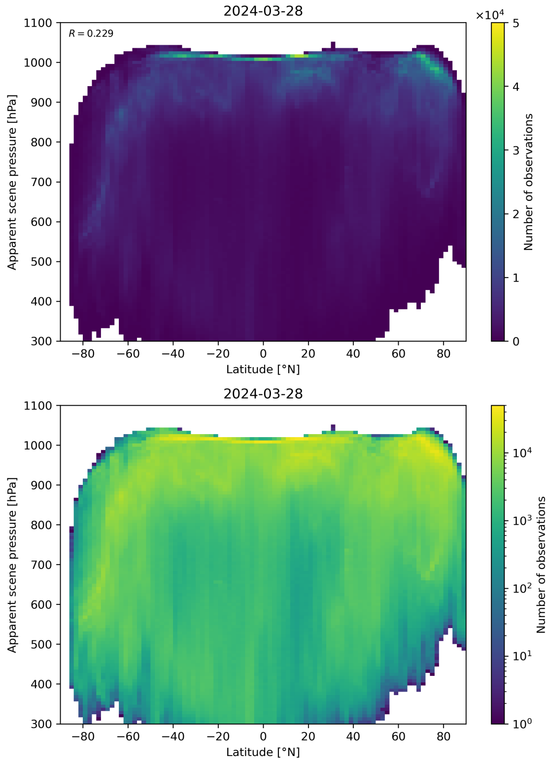
Figure 88: Scatter density plot of “Latitude” against “Apparent scene pressure” for 2024-03-27 to 2024-03-29.
