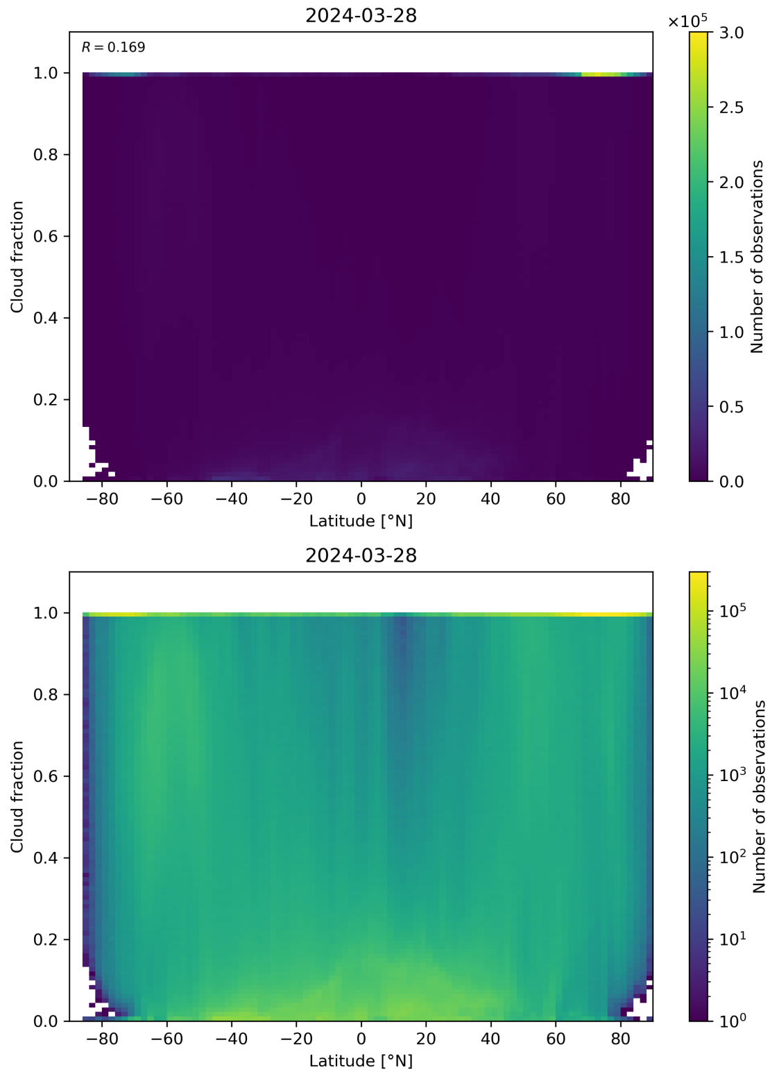
Figure 90: Scatter density plot of “Latitude” against “Cloud fraction” for 2024-03-27 to 2024-03-29.
