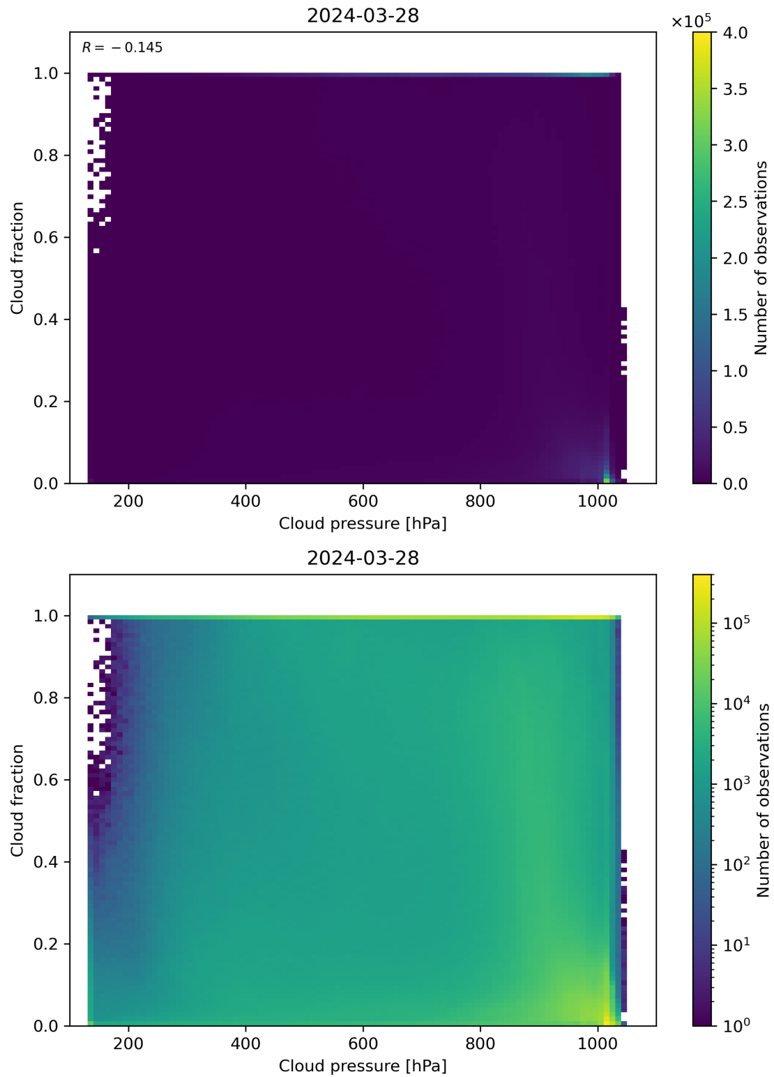
Figure 79: Scatter density plot of “Cloud pressure” against “Cloud fraction” for 2024-03-27 to 2024-03-29.
