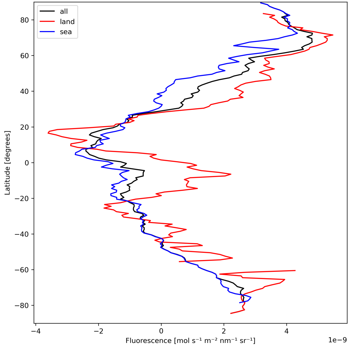
Figure 23: Zonal average of “Fluorescence” for 2024-03-27 to 2024-03-29.
