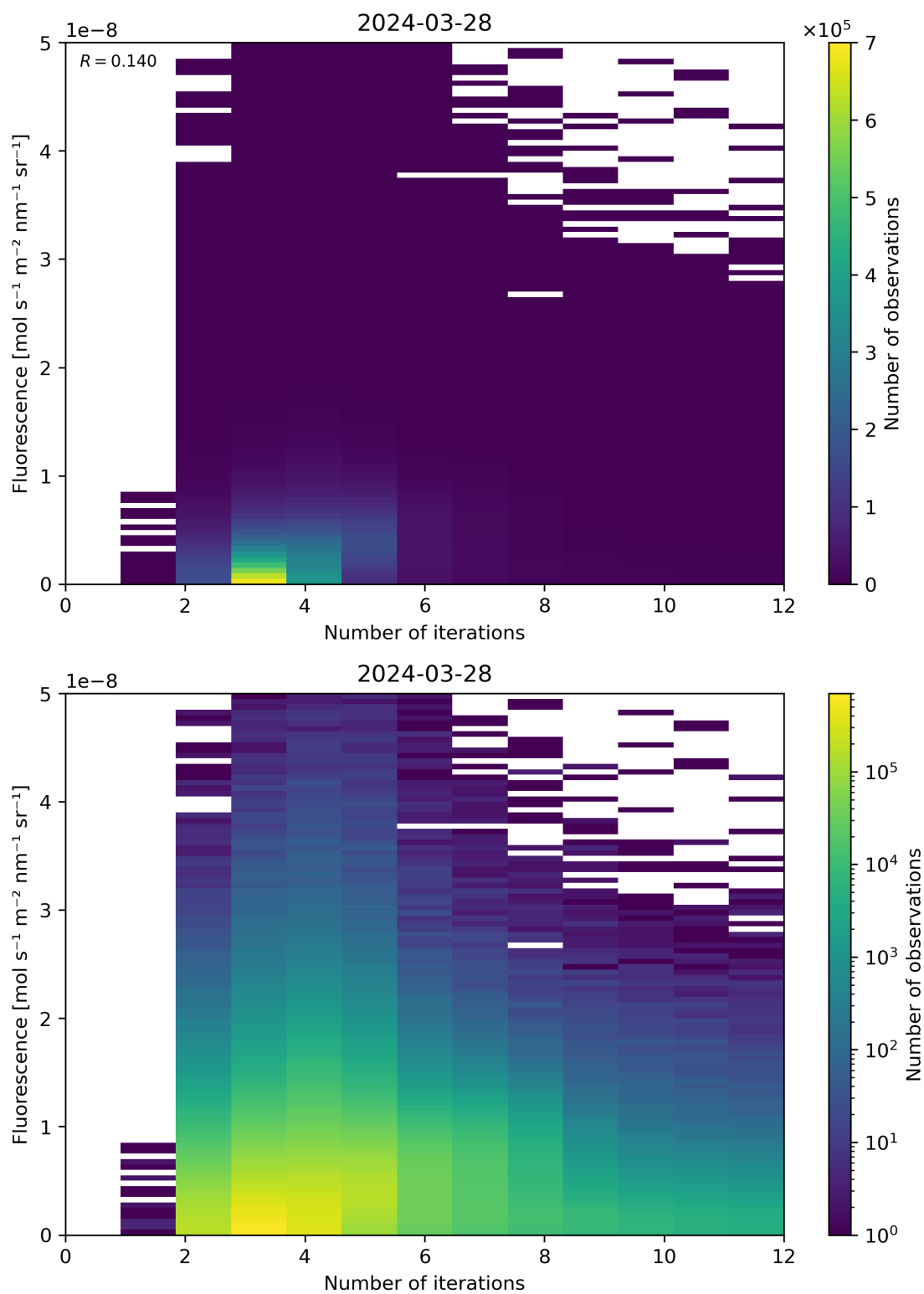
Figure 98: Scatter density plot of “Number of iterations” against “Fluorescence” for 2024-03-27 to 2024-03-29.
