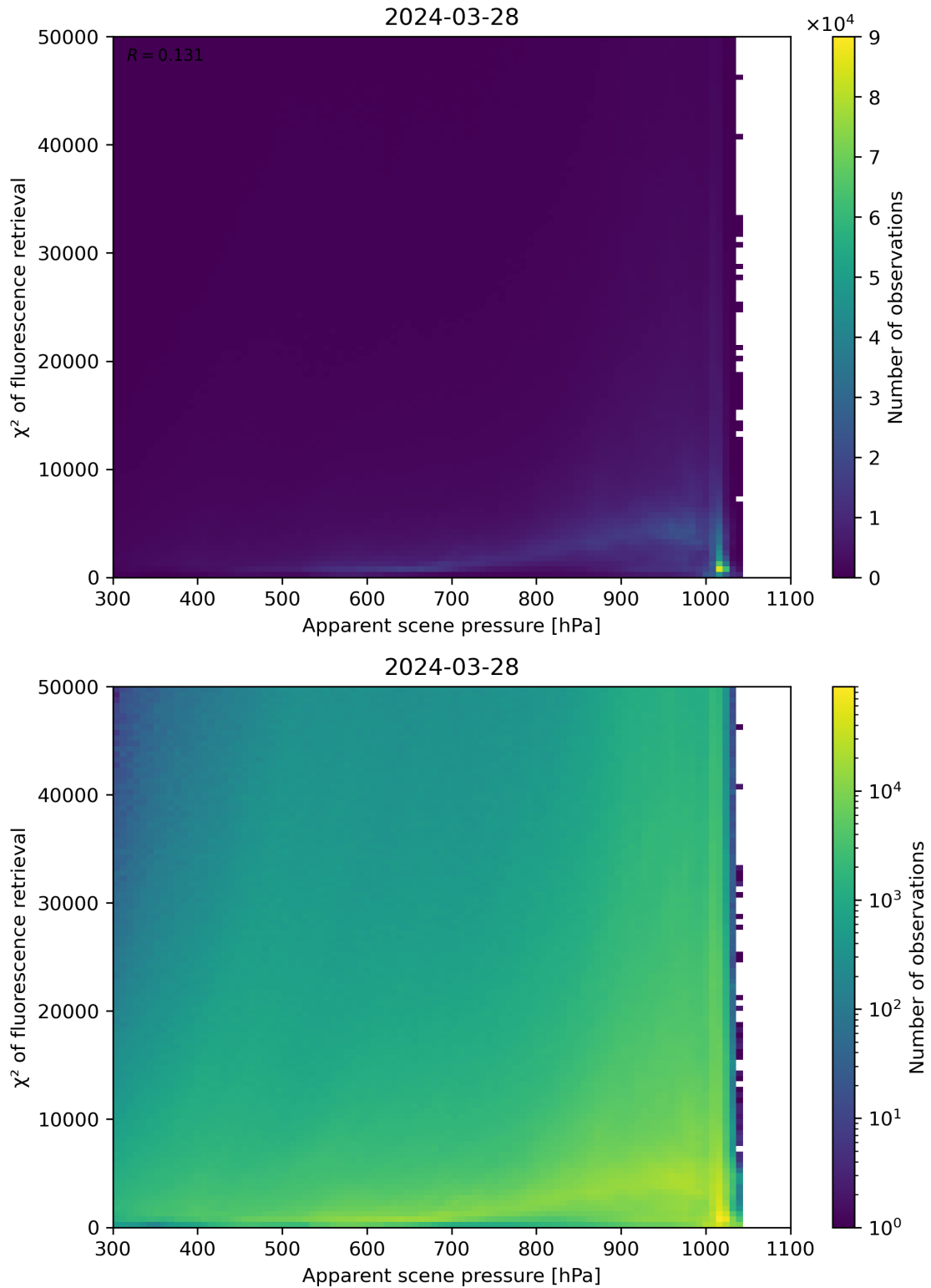
Figure 63: Scatter density plot of “Apparent scene pressure” against “ \chi^2 of fluorescence retrieval” for 2024-03-27 to 2024-03-29.
