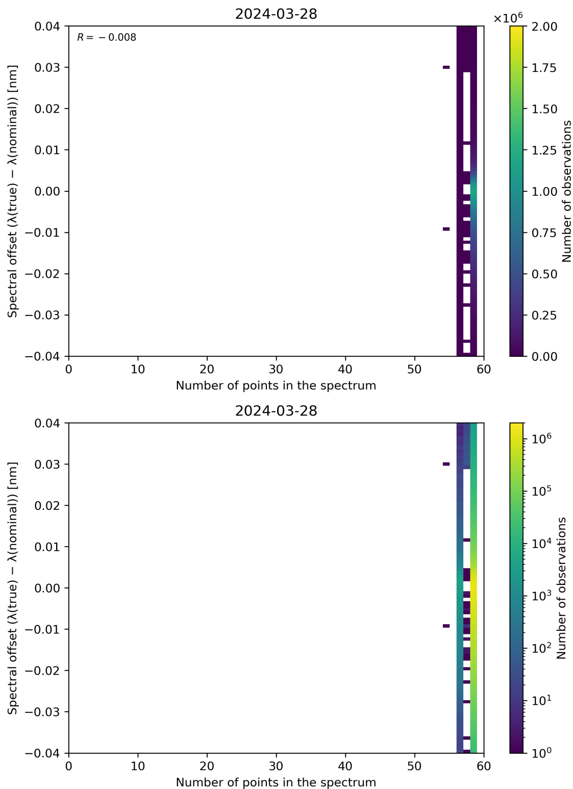
Figure 101: Scatter density plot of “Number of points in the spectrum” against “Spectral offset ( \lambda(\text{true}) - \lambda(\text{nominal}) )” for 2024-03-27 to 2024-03-29.
