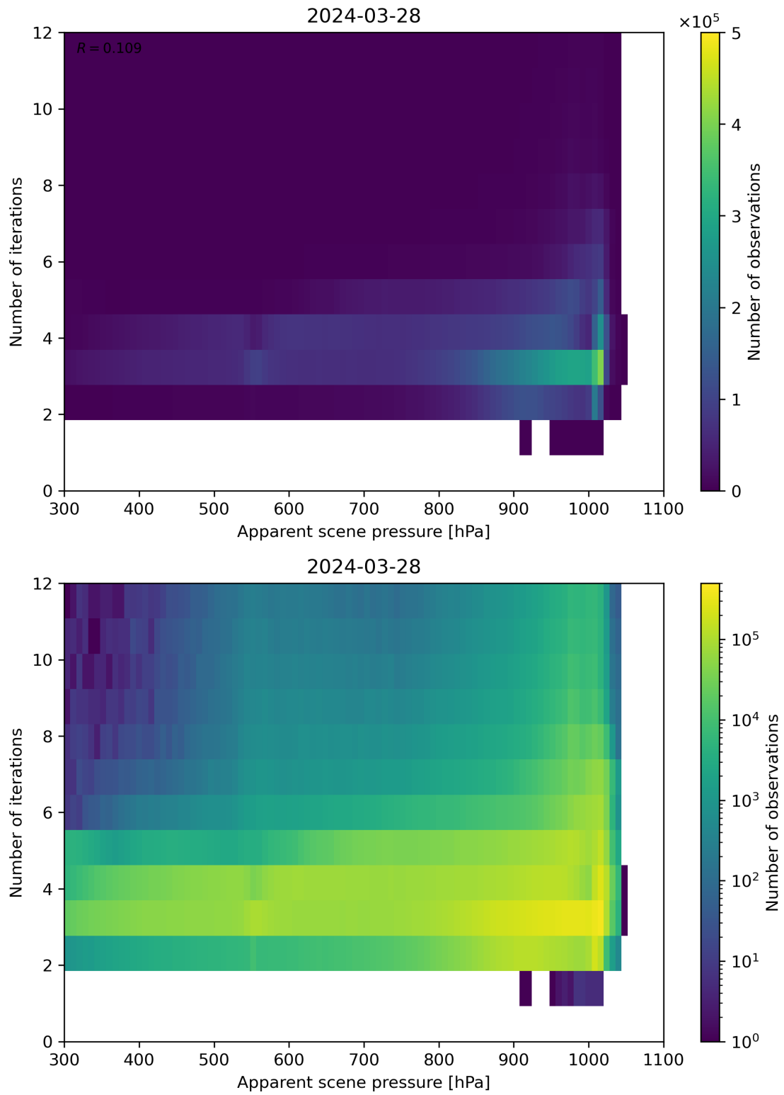
Figure 65: Scatter density plot of “Apparent scene pressure” against “Number of iterations” for 2024-03-27 to 2024-03-29.
