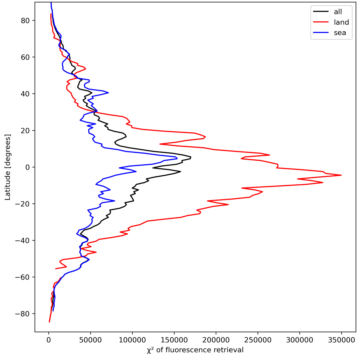
Figure 25: Zonal average of “ \chi^2 of fluorescence retrieval” for 2024-03-27 to 2024-03-29.
