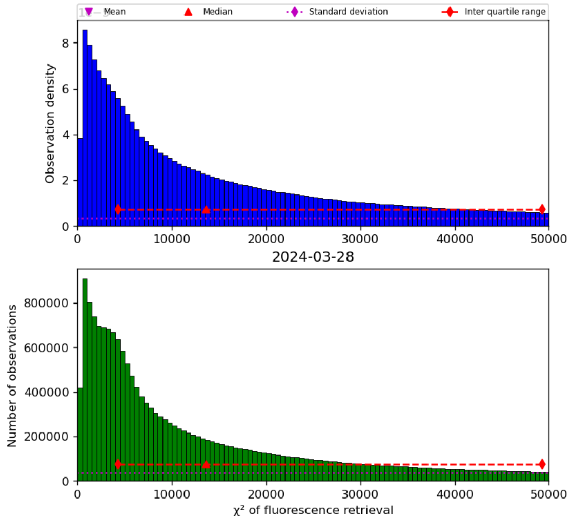
Figure 42: Histogram of “ \chi^2 of fluorescence retrieval” for 2024-03-27 to 2024-03-29
