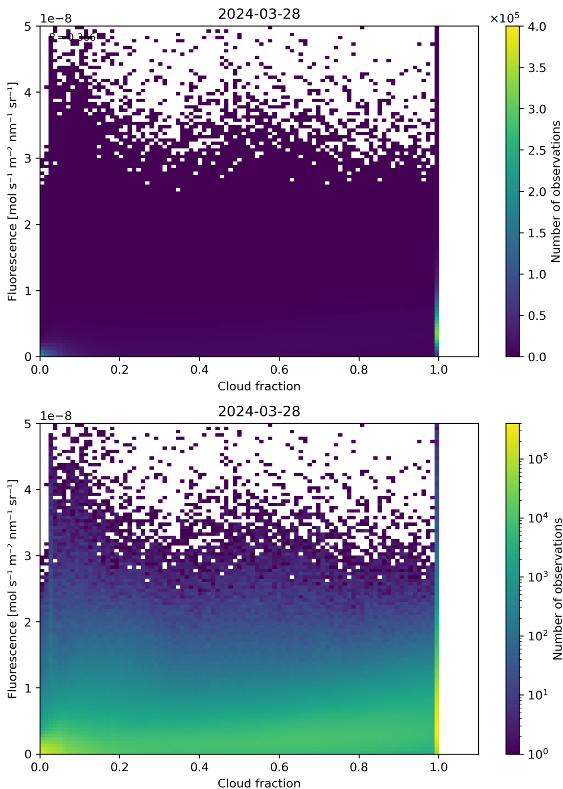
Figure 72: Scatter density plot of “Cloud fraction” against “Fluorescence” for 2024-03-27 to 2024-03-29.
