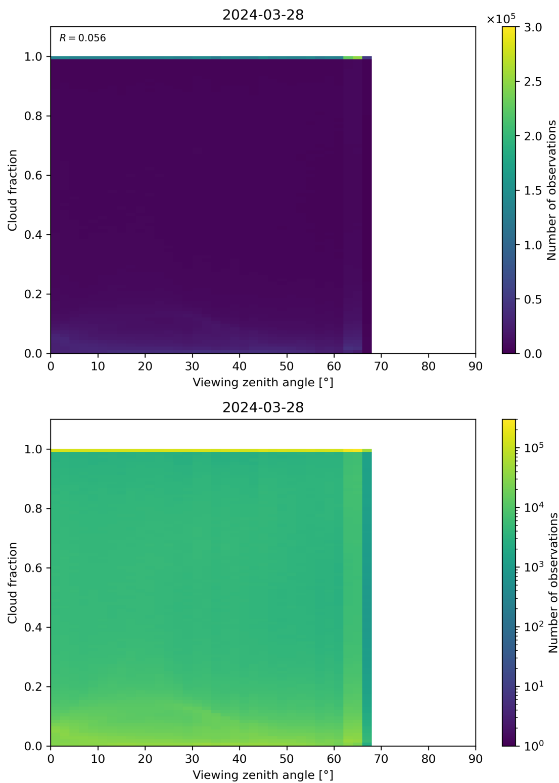
Figure 120: Scatter density plot of “Viewing zenith angle” against “Cloud fraction” for 2024-03-27 to 2024-03-29.
