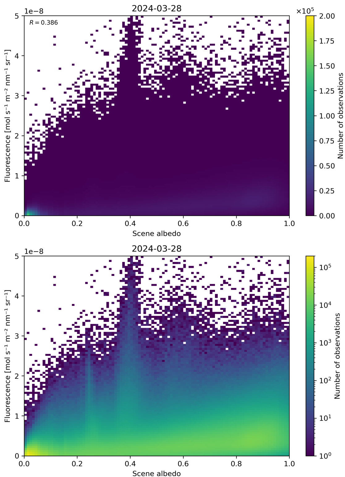
Figure 104: Scatter density plot of “Scene albedo” against “Fluorescence” for 2024-03-27 to 2024-03-29.
