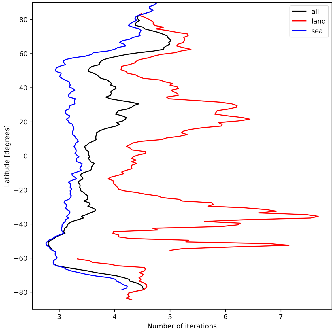
Figure 22: Zonal average of “Number of iterations” for 2024-03-27 to 2024-03-29.
