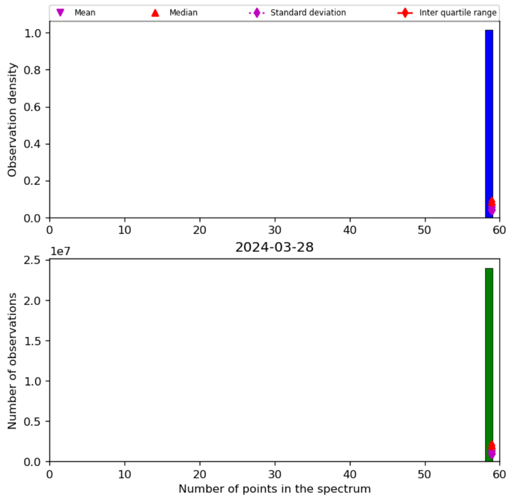
Figure 44: Histogram of “Number of points in the spectrum” for 2024-03-27 to 2024-03-29
