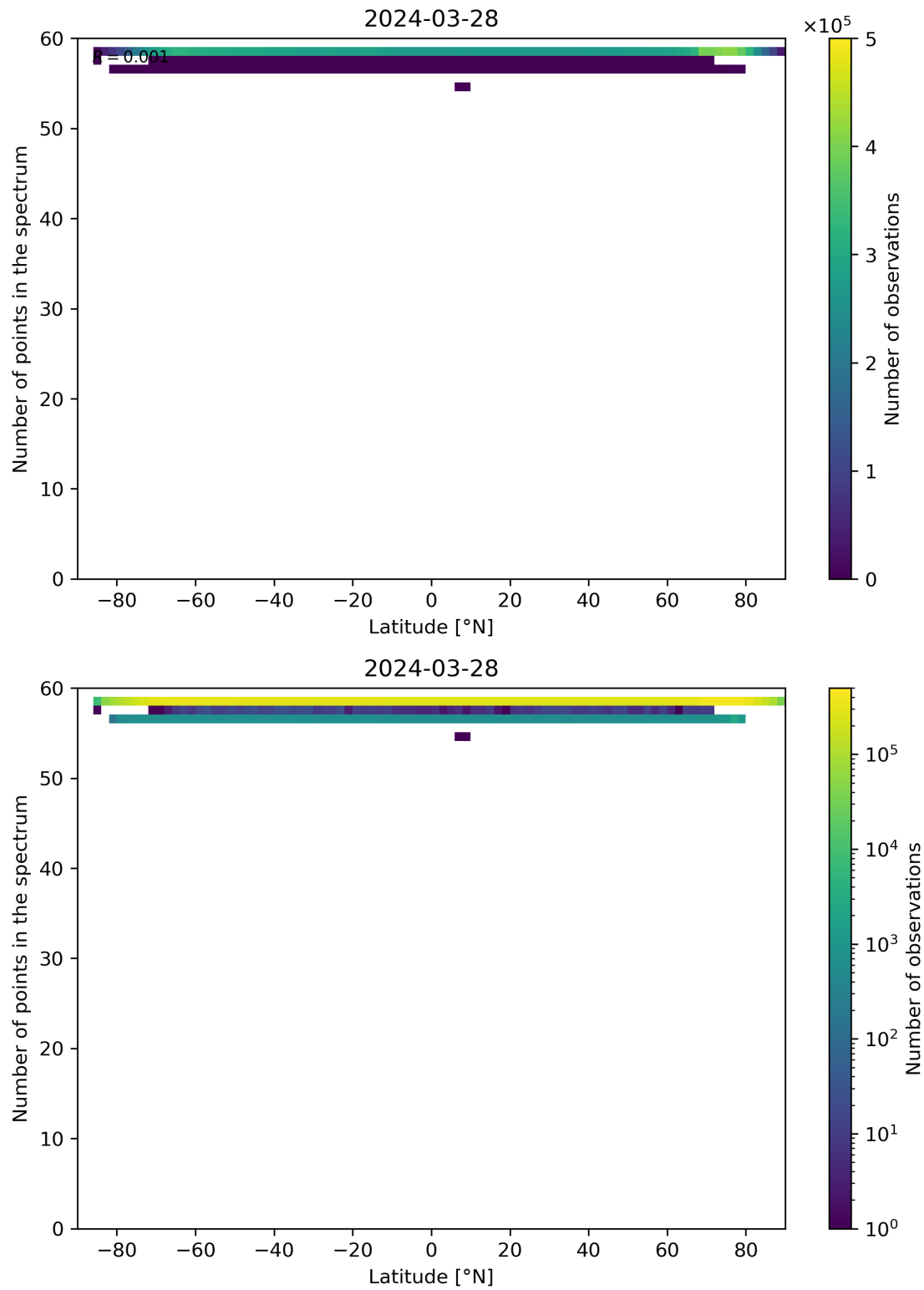
Figure 94: Scatter density plot of “Latitude” against “Number of points in the spectrum” for 2024-03-27 to 2024-03-29.
