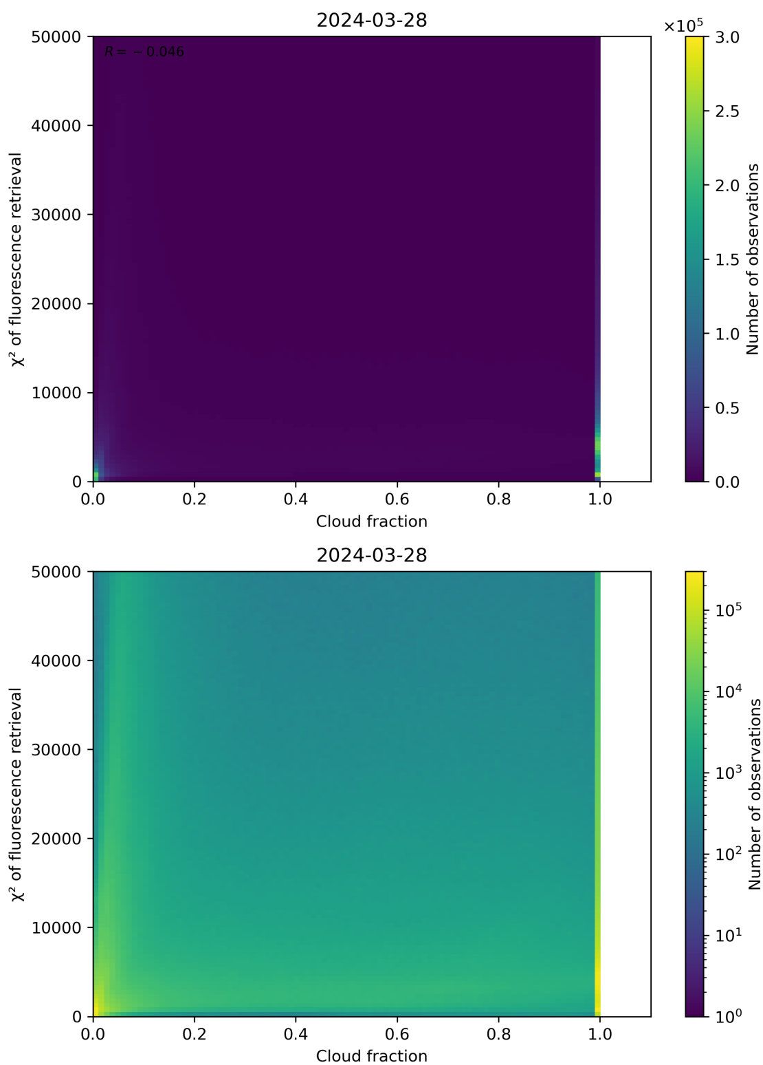
Figure 71: Scatter density plot of “Cloud fraction” against “ \chi^2 of fluorescence retrieval” for 2024-03-27 to 2024-03-29.
