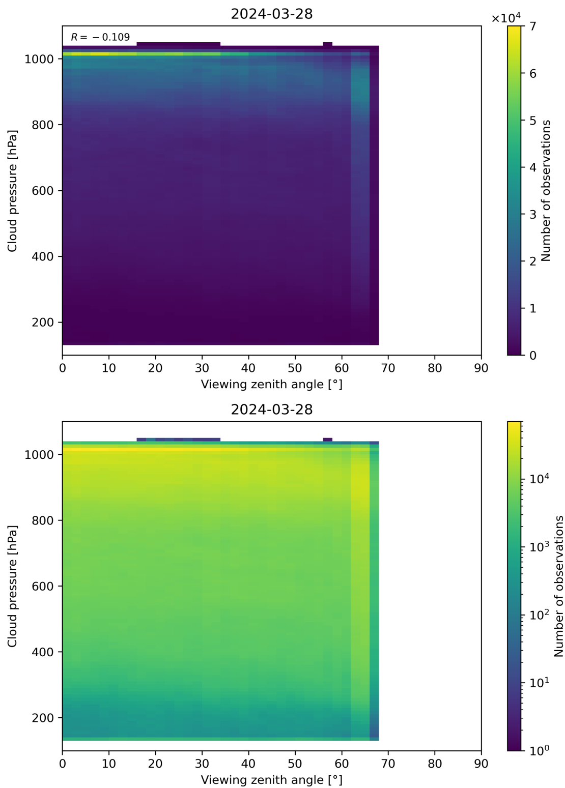
Figure 121: Scatter density plot of “Viewing zenith angle” against “Cloud pressure” for 2024-03-27 to 2024-03-29.
