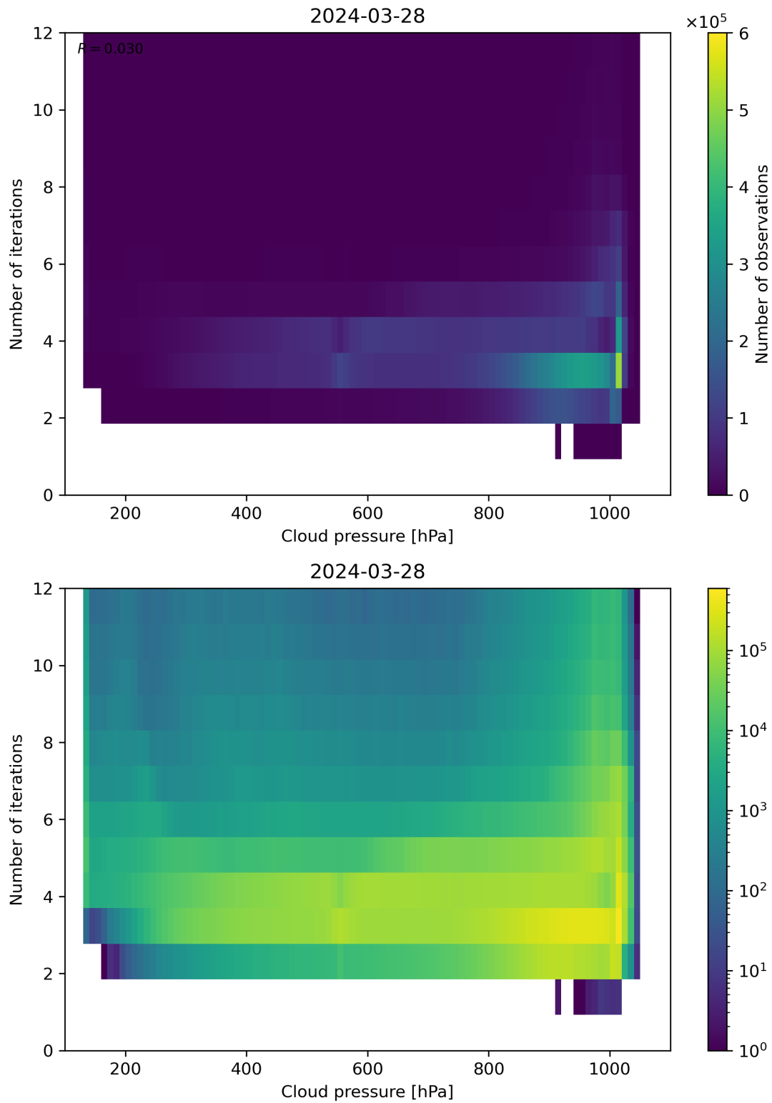
Figure 81: Scatter density plot of “Cloud pressure” against “Number of iterations” for 2024-03-27 to 2024-03-29.
