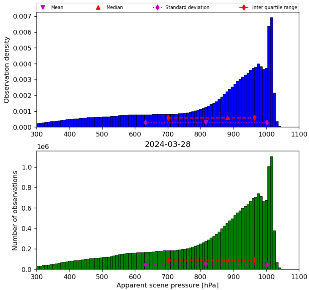
Figure 36: Histogram of “Apparent scene pressure” for 2024-03-27 to 2024-03-29
