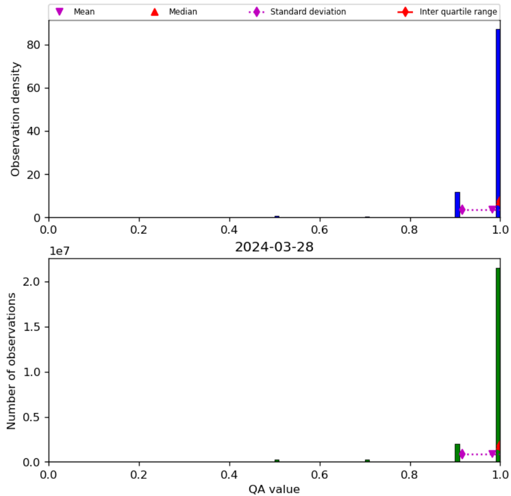
Figure 29: Histogram of “QA value” for 2024-03-27 to 2024-03-29
