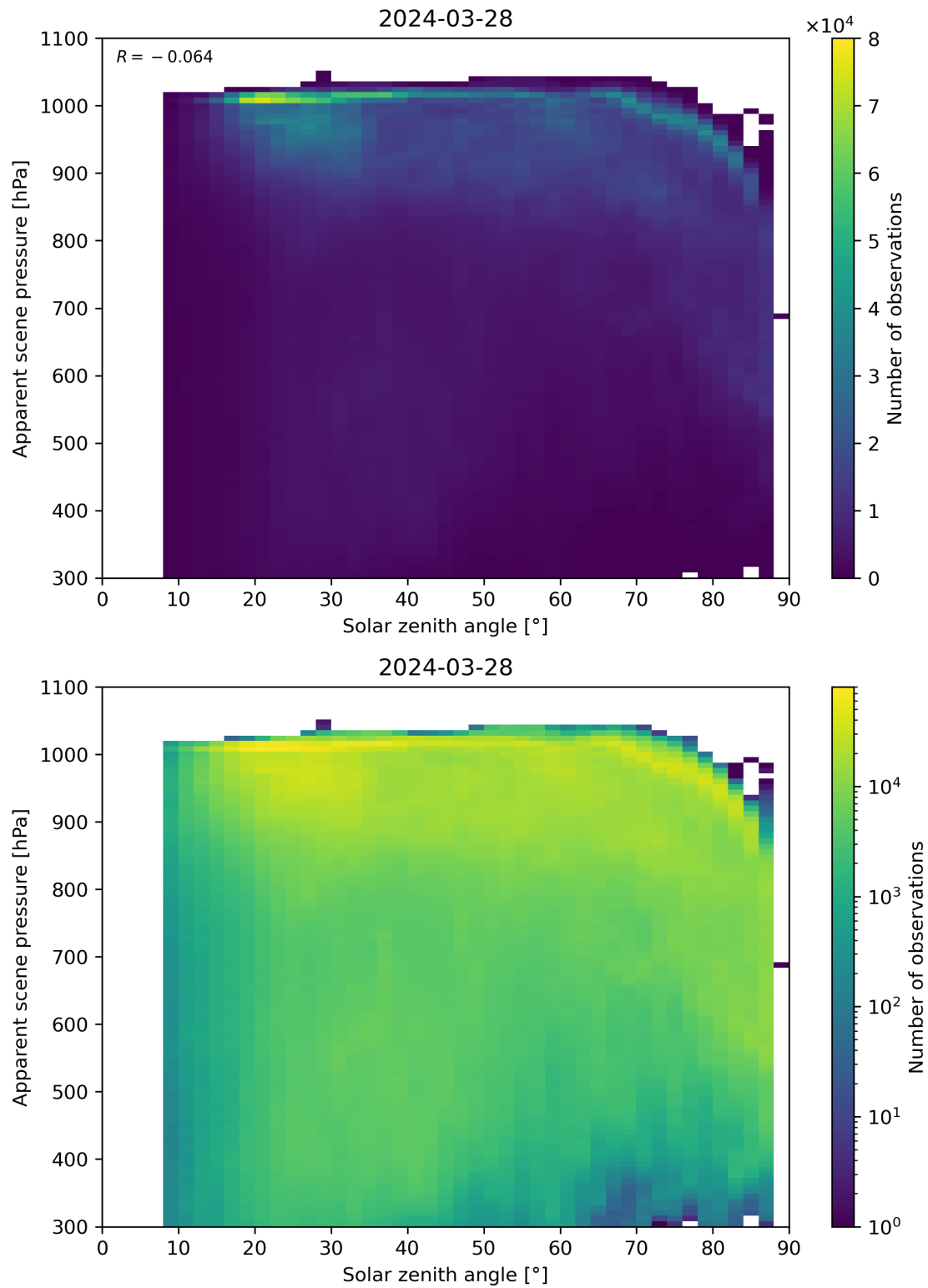
Figure 108: Scatter density plot of “Solar zenith angle” against “Apparent scene pressure” for 2024-03-27 to 2024-03-29.
