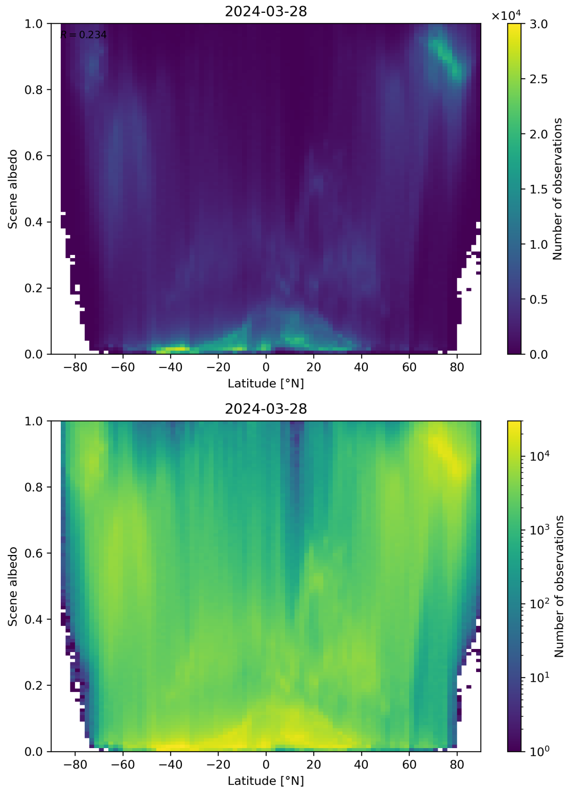
Figure 95: Scatter density plot of “Latitude” against “Scene albedo” for 2024-03-27 to 2024-03-29.
