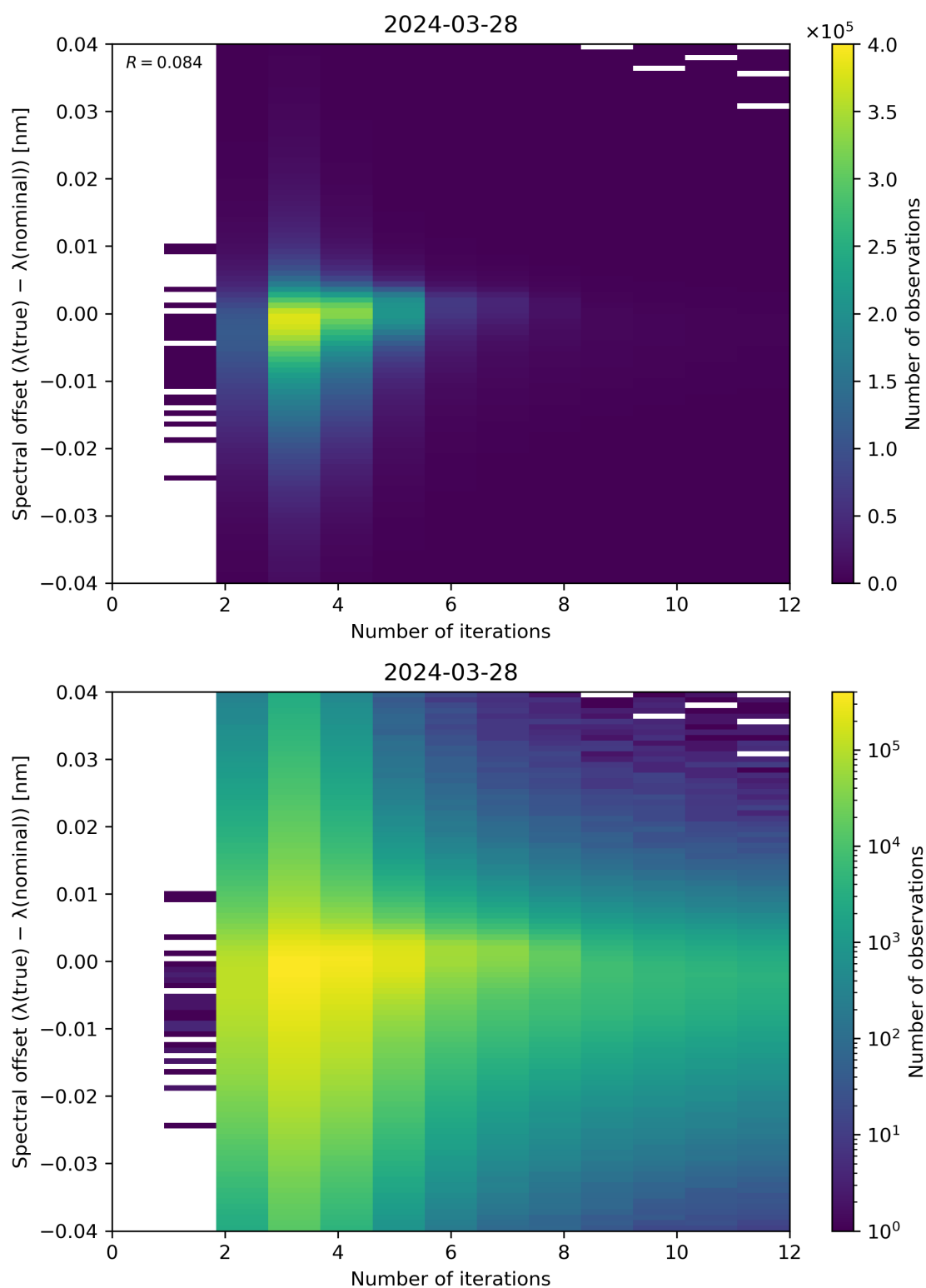
Figure 100: Scatter density plot of “Number of iterations” against “Spectral offset ( \lambda(\text{true}) - \lambda(\text{nominal}) )” for 2024-03-27 to 2024-03-29.
