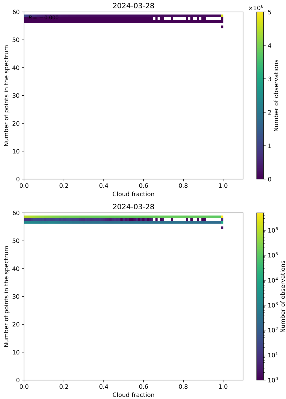
Figure 74: Scatter density plot of “Cloud fraction” against “Number of points in the spectrum” for 2024-03-27 to 2024-03-29.
