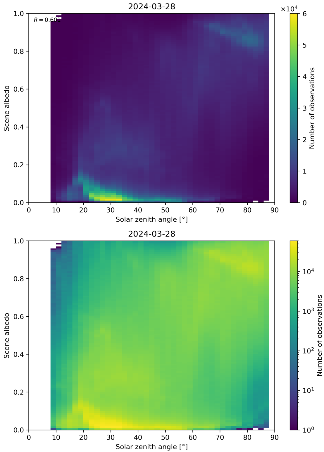
Figure 116: Scatter density plot of “Solar zenith angle” against “Scene albedo” for 2024-03-27 to 2024-03-29.
