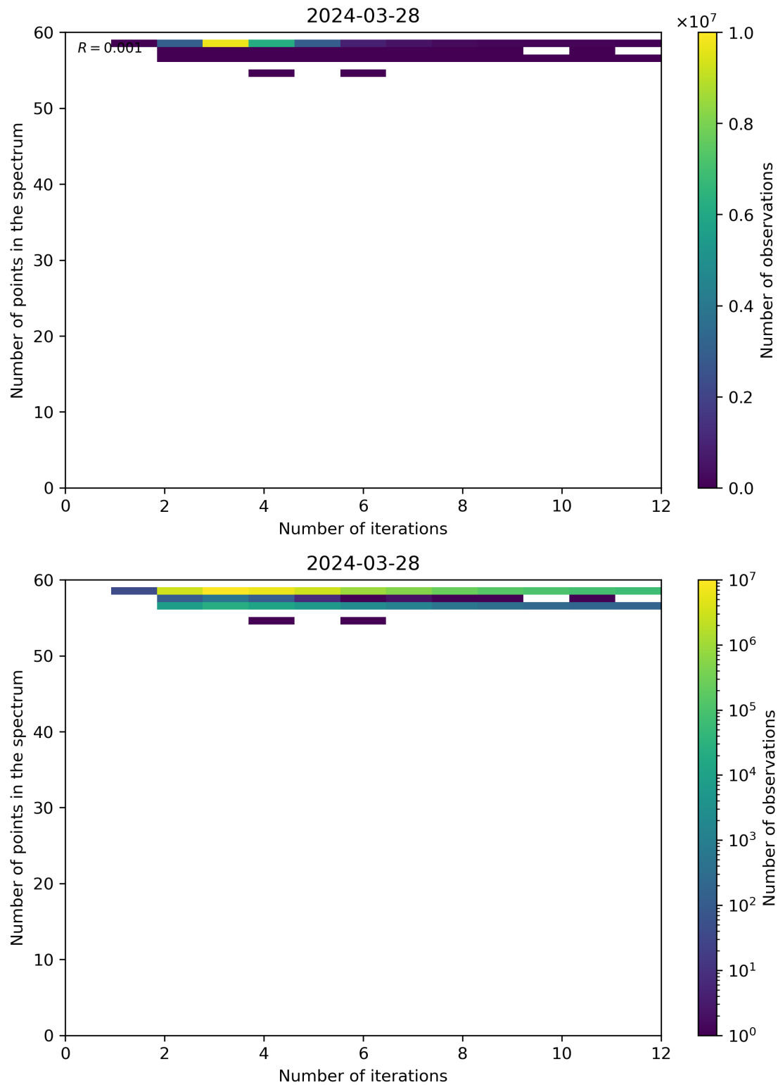
Figure 99: Scatter density plot of “Number of iterations” against “Number of points in the spectrum” for 2024-03-27 to 2024-03-29.
