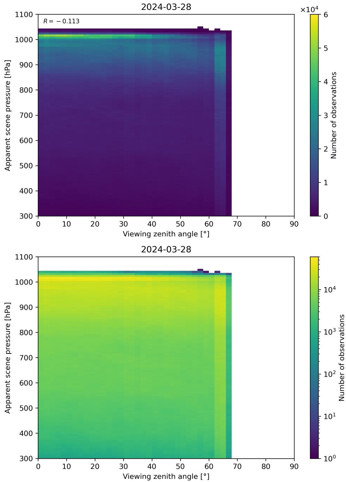
Figure 118: Scatter density plot of “Viewing zenith angle” against “Apparent scene pressure” for 2024-03-27 to 2024-03-29.
