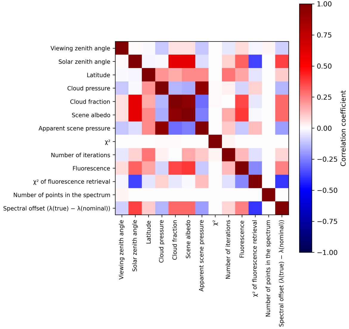
Figure 2: Map of correlation matrix for 2024-03-27 to 2024-03-29.
