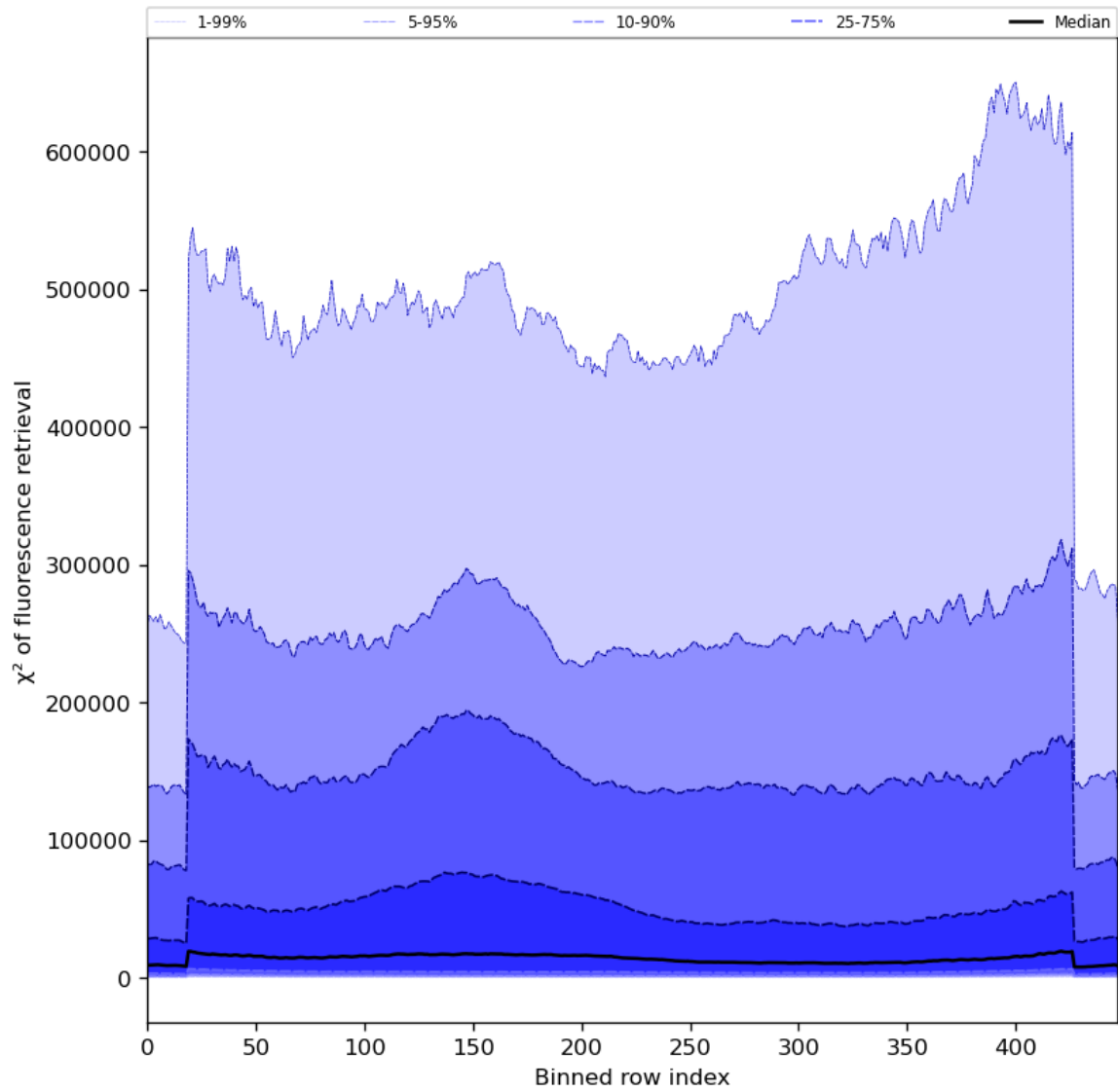
Figure 59: Along track statistics of “ \chi^2 of fluorescence retrieval” for 2024-03-27 to 2024-03-29
