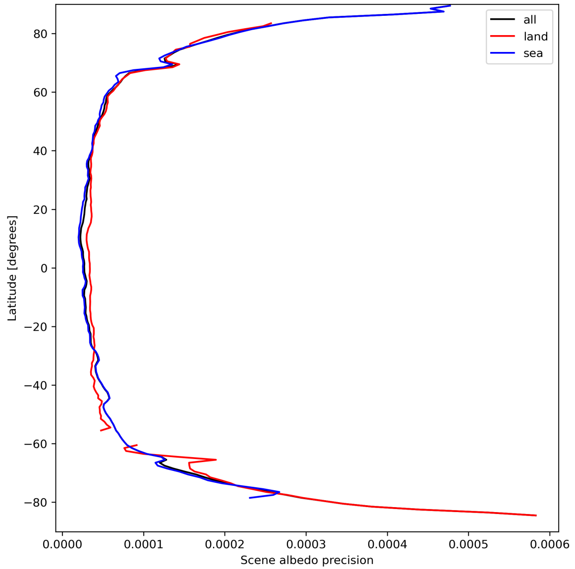
Figure 18: Zonal average of “Scene albedo precision” for 2024-03-27 to 2024-03-29.
