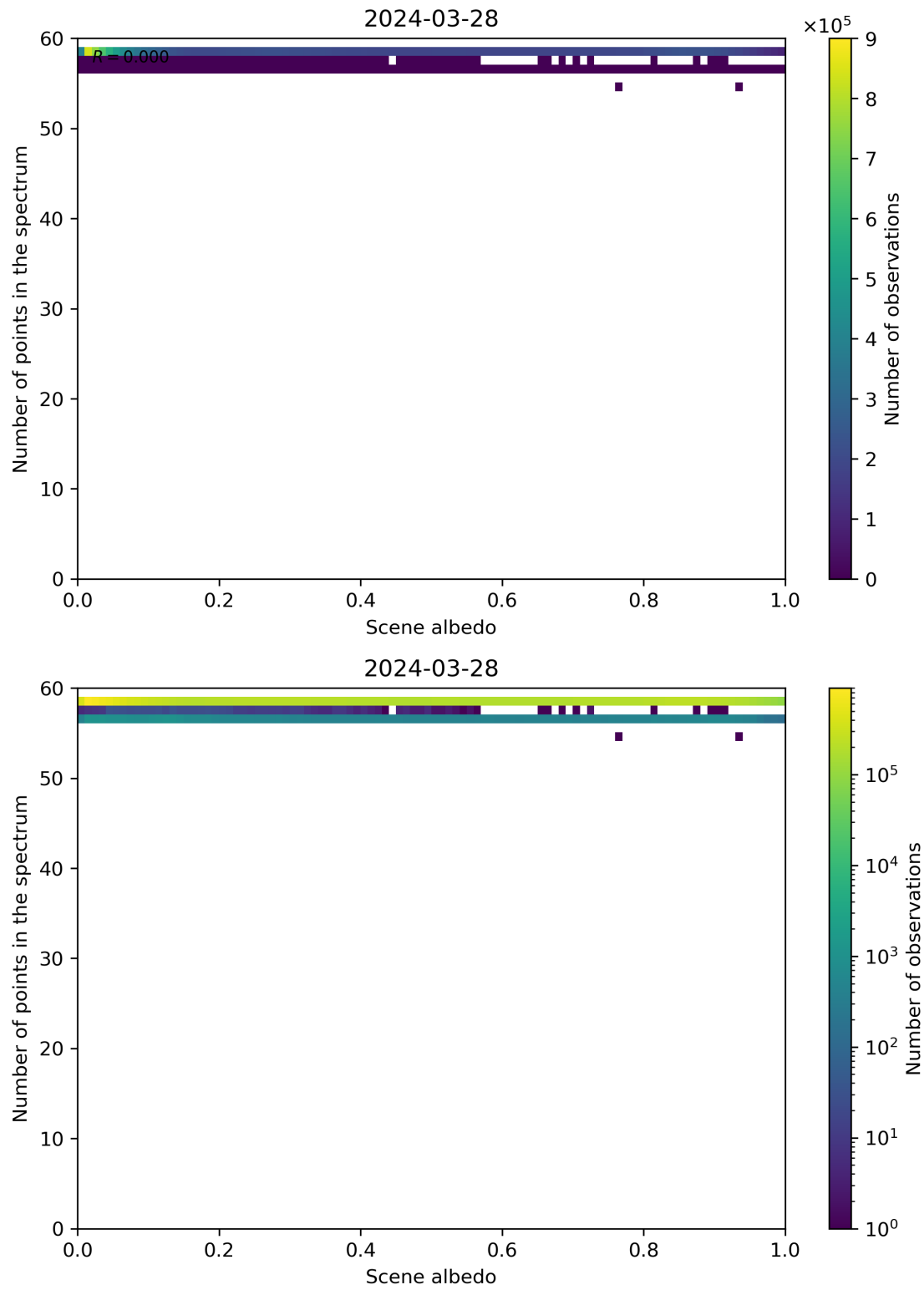
Figure 106: Scatter density plot of “Scene albedo” against “Number of points in the spectrum” for 2024-03-27 to 2024-03-29.
