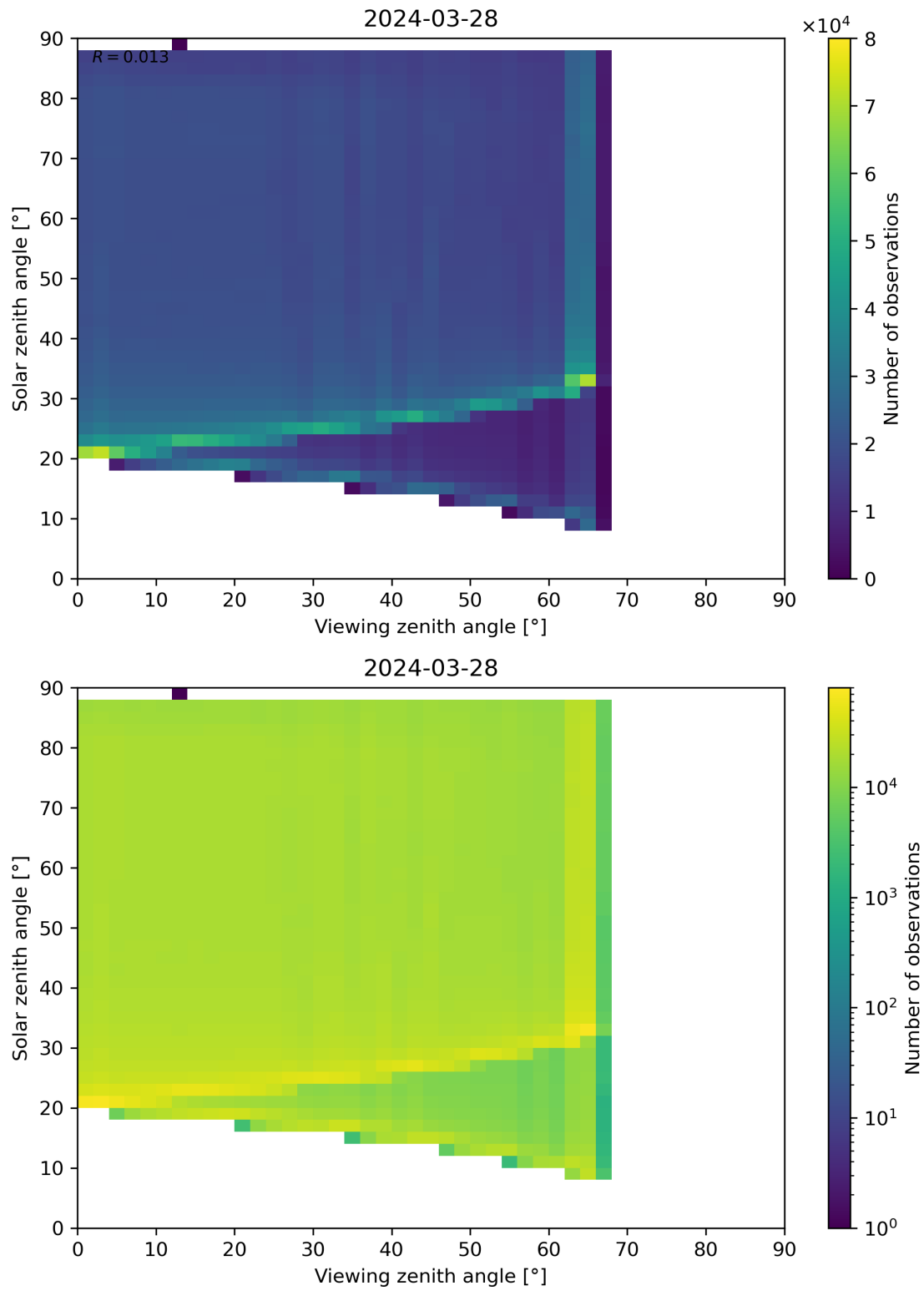
Figure 127: Scatter density plot of “Viewing zenith angle” against “Solar zenith angle” for 2024-03-27 to 2024-03-29.
