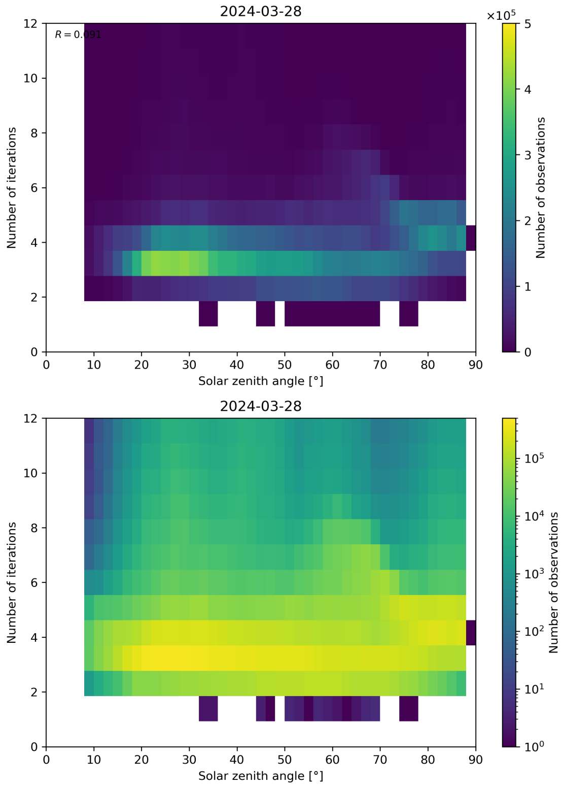
Figure 114: Scatter density plot of “Solar zenith angle” against “Number of iterations” for 2024-03-27 to 2024-03-29.
