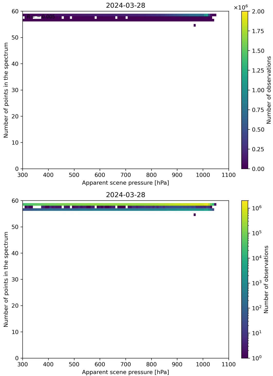
Figure 66: Scatter density plot of “Apparent scene pressure” against “Number of points in the spectrum” for 2024-03-27 to 2024-03-29.
