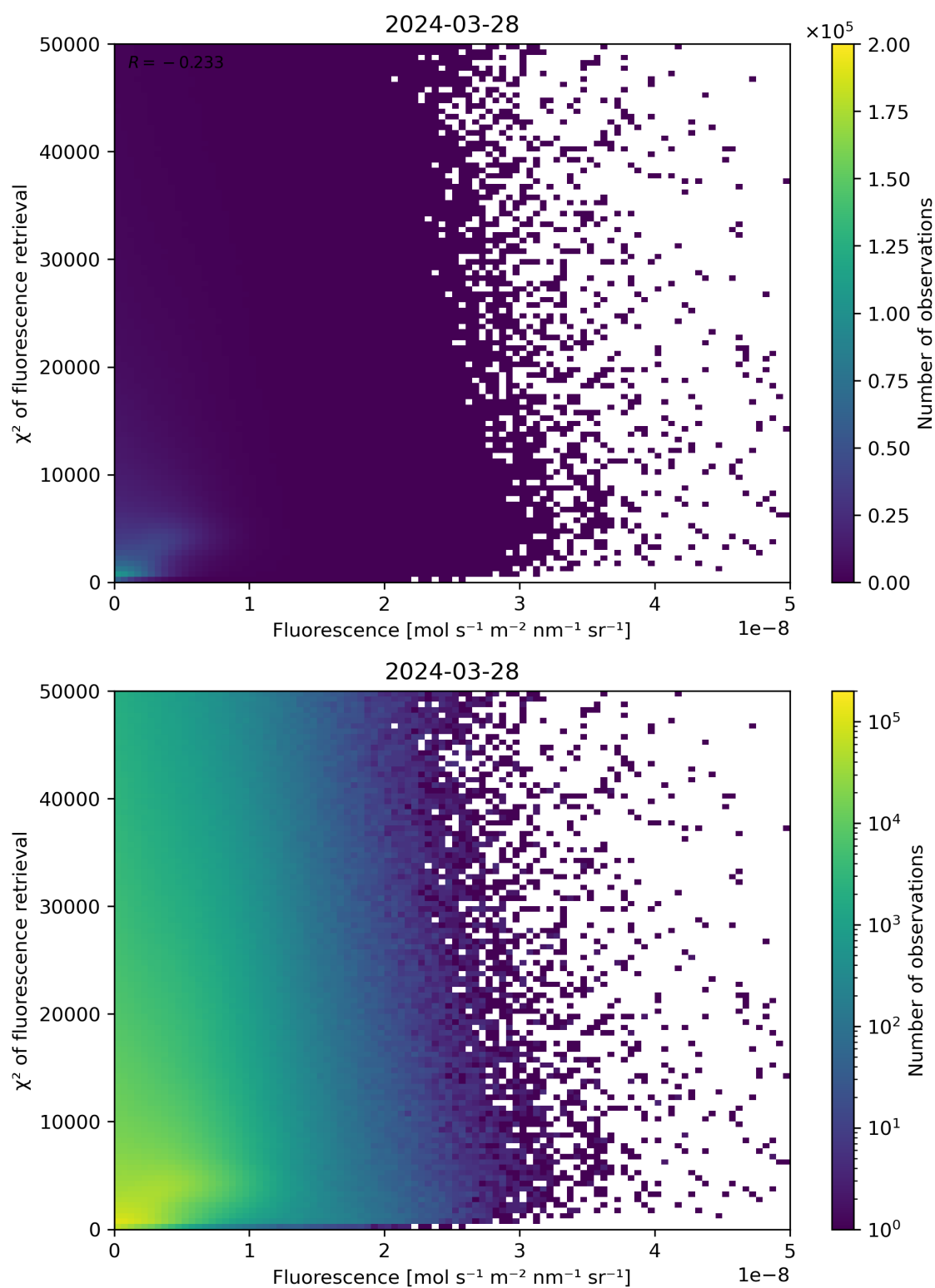
Figure 85: Scatter density plot of “Fluorescence” against “ \chi^2 of fluorescence retrieval” for 2024-03-27 to 2024-03-29.
