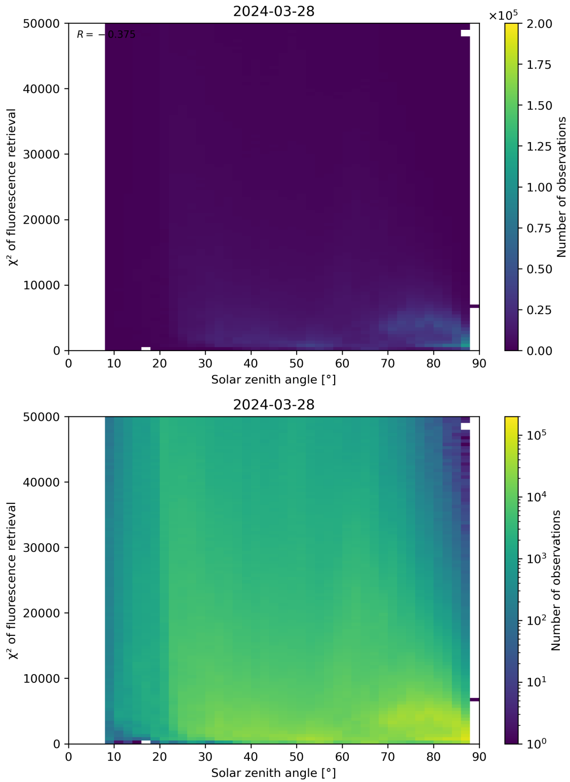
Figure 109: Scatter density plot of “Solar zenith angle” against “ \chi^2 of fluorescence retrieval” for 2024-03-27 to 2024-03-29.
