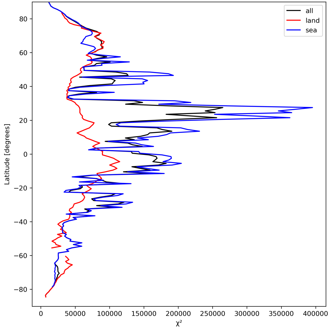
Figure 21: Zonal average of “ \chi^2 ” for 2024-03-27 to 2024-03-29.
