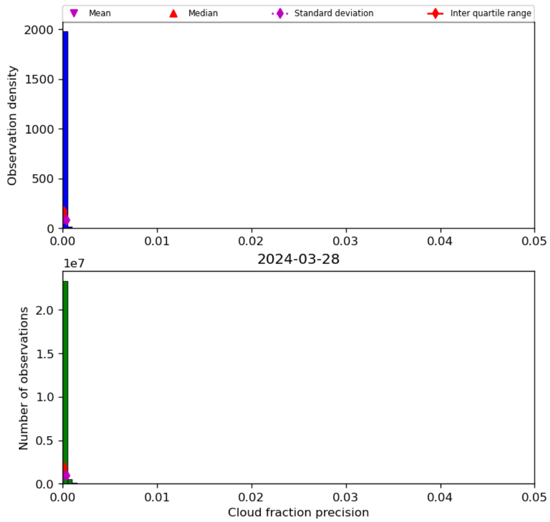
Figure 33: Histogram of “Cloud fraction precision” for 2024-03-27 to 2024-03-29
