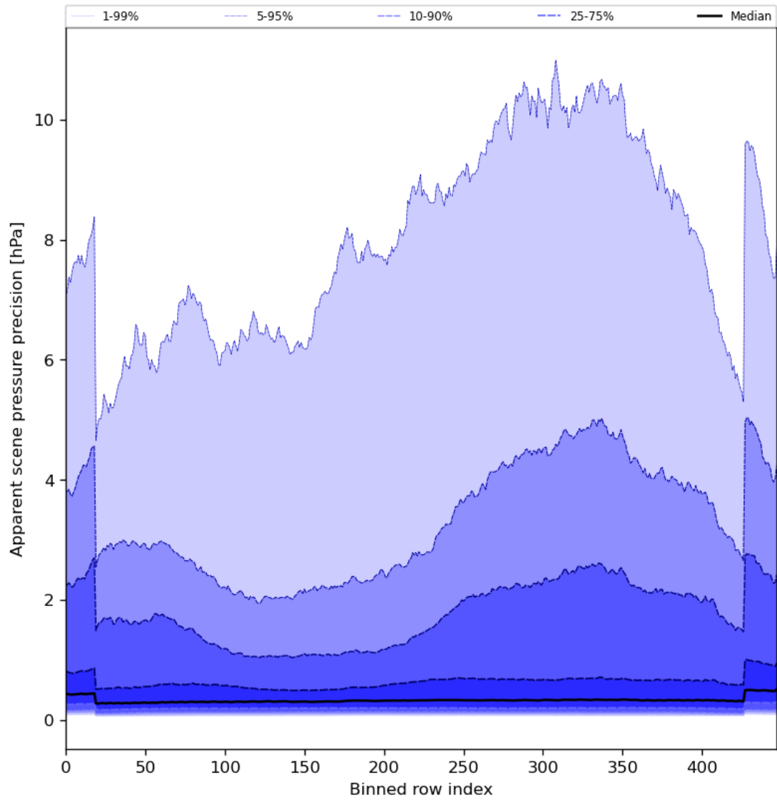
Figure 54: Along track statistics of “Apparent scene pressure precision” for 2024-03-27 to 2024-03-29
