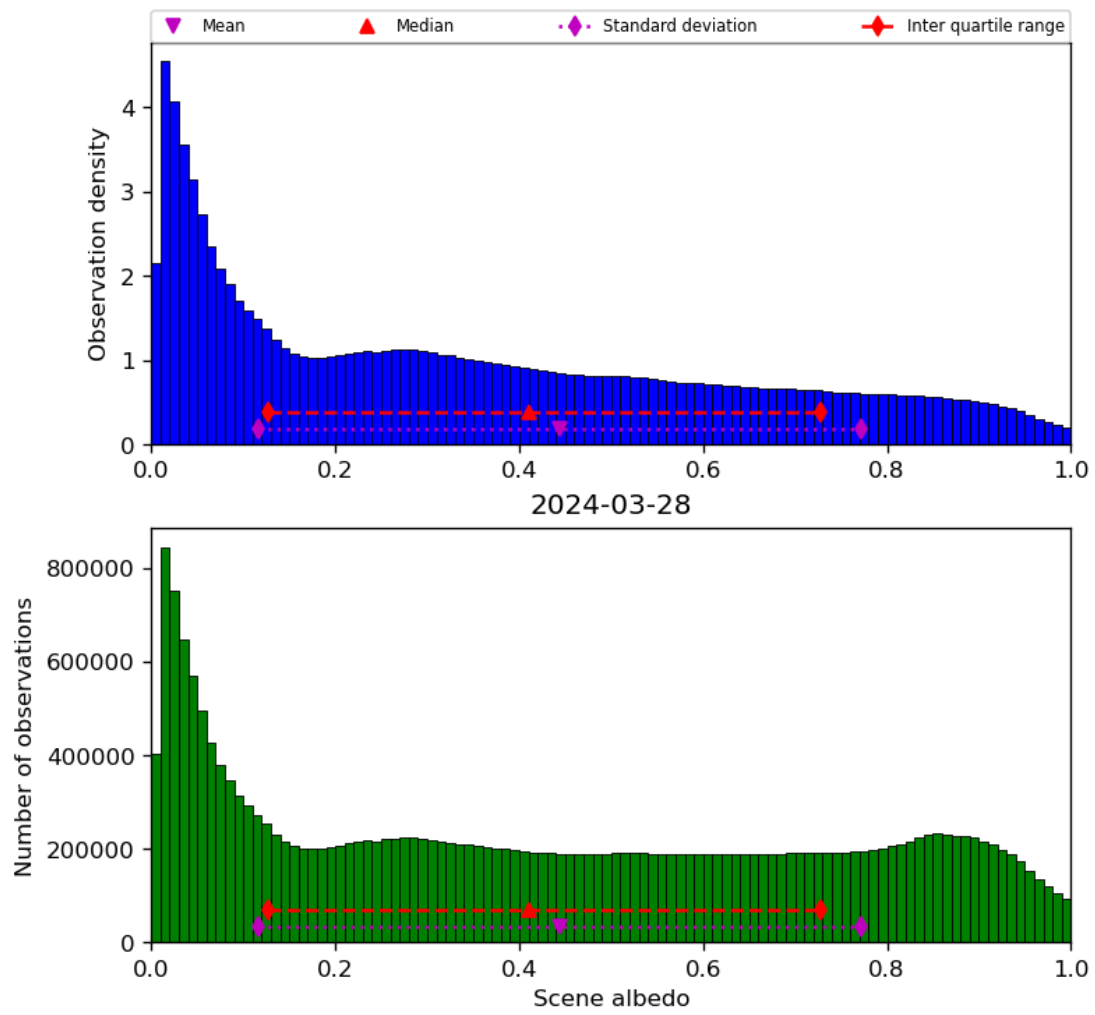
Figure 34: Histogram of “Scene albedo” for 2024-03-27 to 2024-03-29
