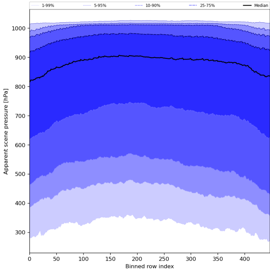
Figure 53: Along track statistics of “Apparent scene pressure” for 2024-03-27 to 2024-03-29
