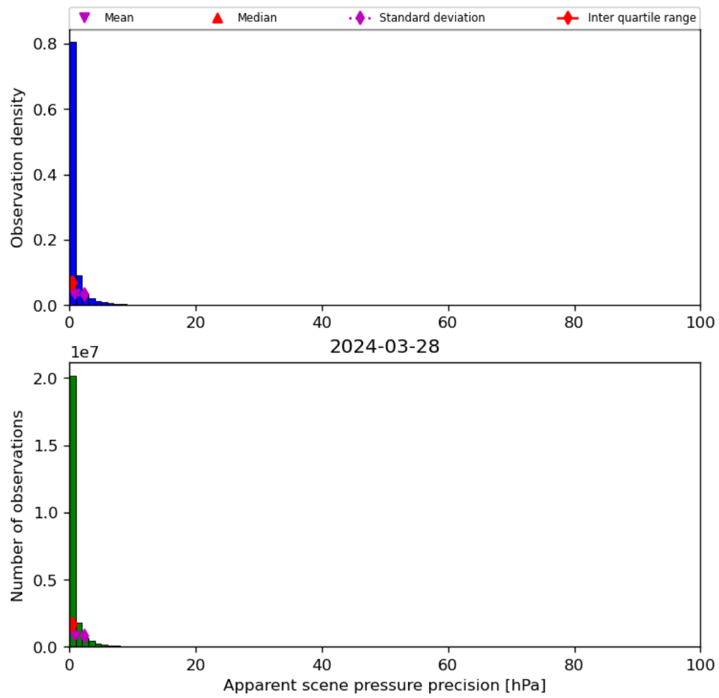
Figure 37: Histogram of “Apparent scene pressure precision” for 2024-03-27 to 2024-03-29
