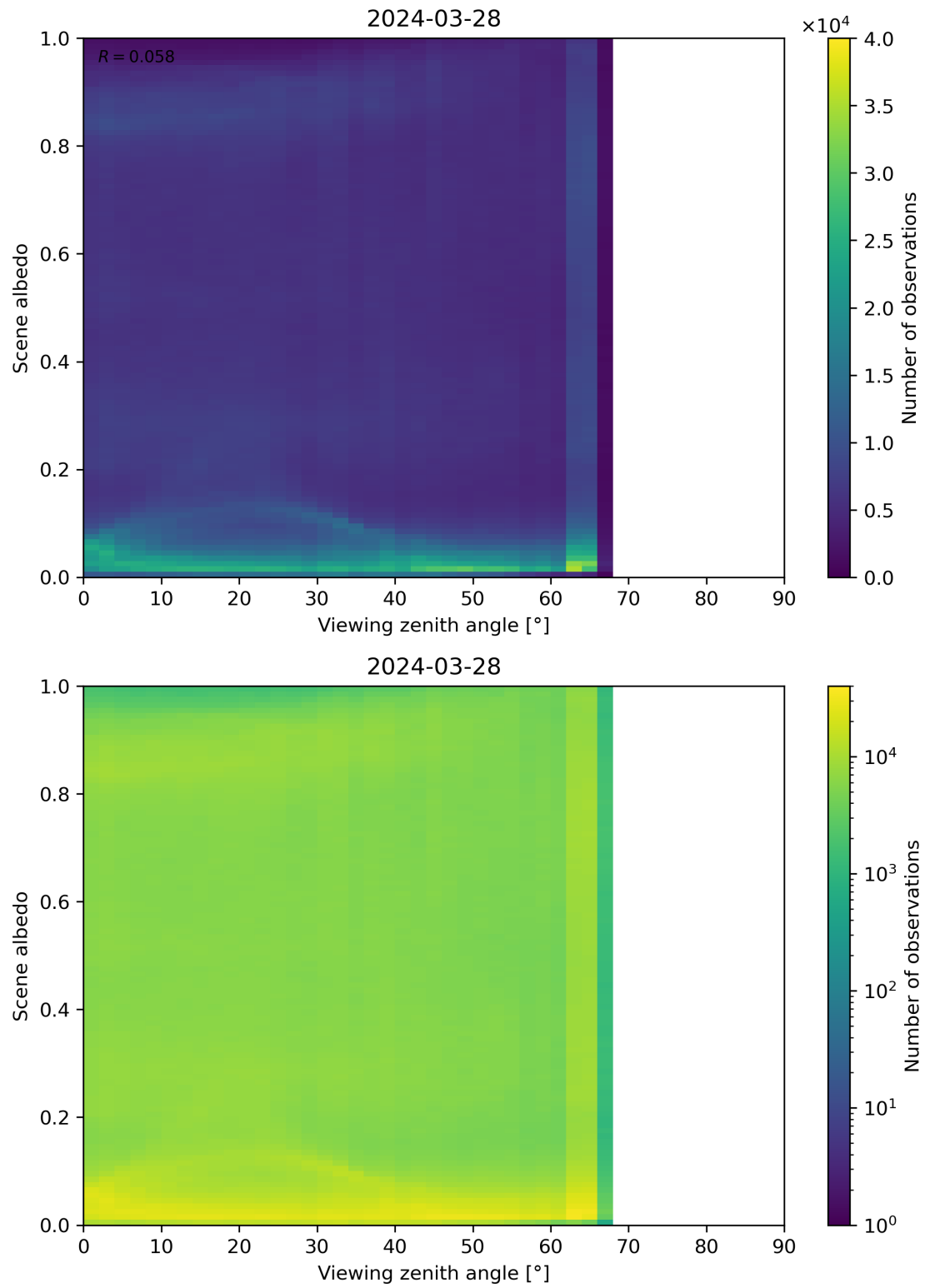
Figure 126: Scatter density plot of “Viewing zenith angle” against “Scene albedo” for 2024-03-27 to 2024-03-29.
