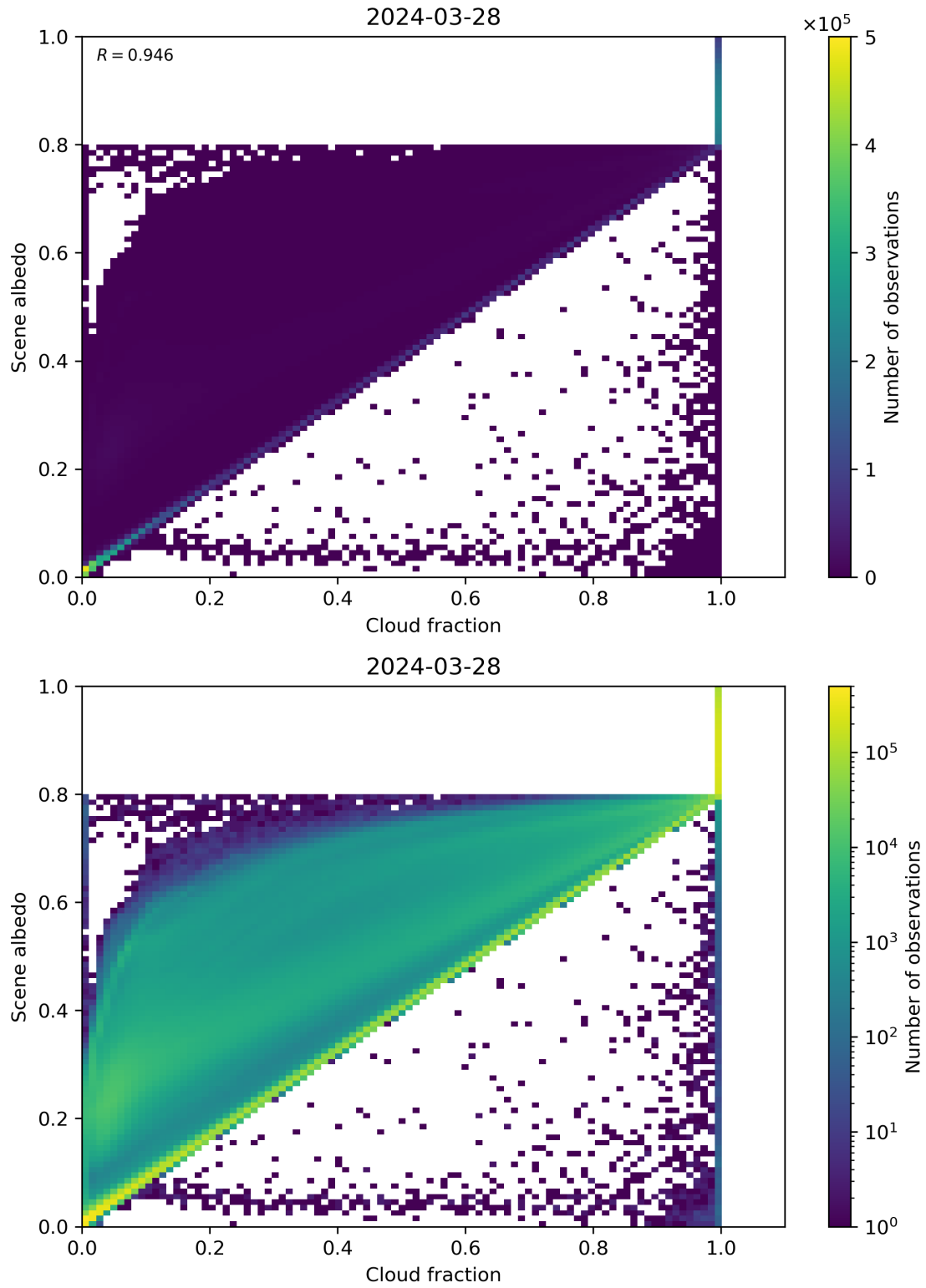
Figure 75: Scatter density plot of “Cloud fraction” against “Scene albedo” for 2024-03-27 to 2024-03-29.
