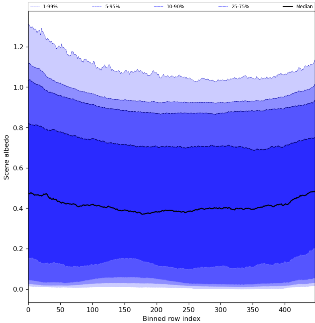
Figure 51: Along track statistics of “Scene albedo” for 2024-03-27 to 2024-03-29
