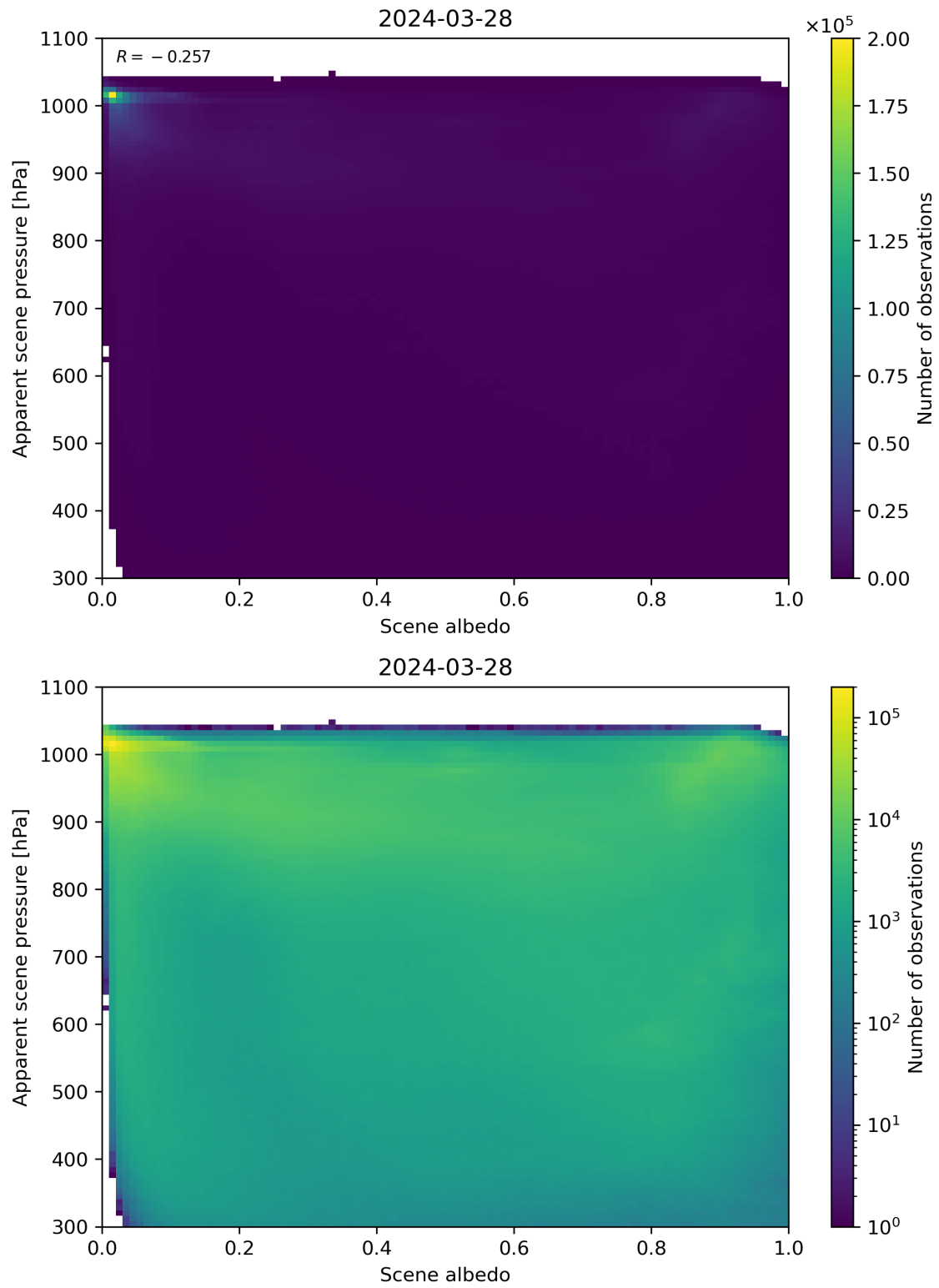
Figure 102: Scatter density plot of “Scene albedo” against “Apparent scene pressure” for 2024-03-27 to 2024-03-29.
