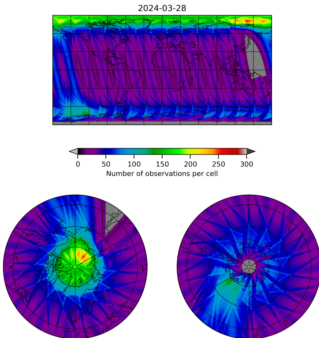
Figure 11: Map of the number of observations for 2024-03-27 to 2024-03-29
