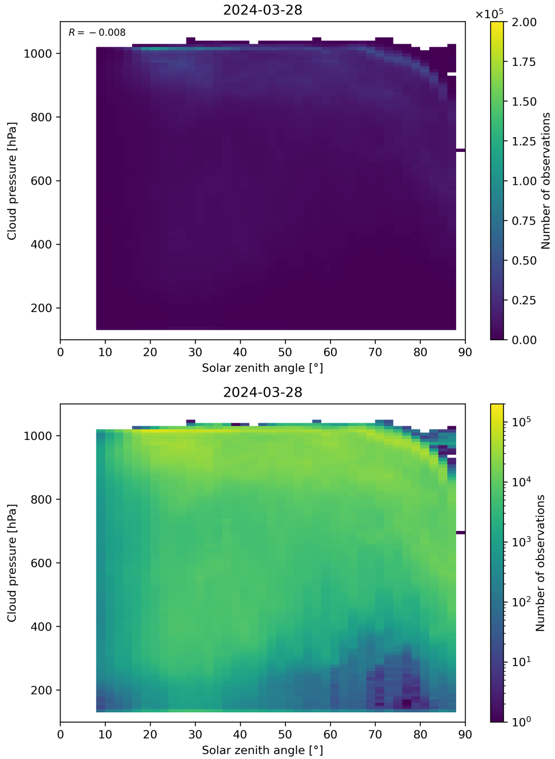
Figure 111: Scatter density plot of “Solar zenith angle” against “Cloud pressure” for 2024-03-27 to 2024-03-29.
