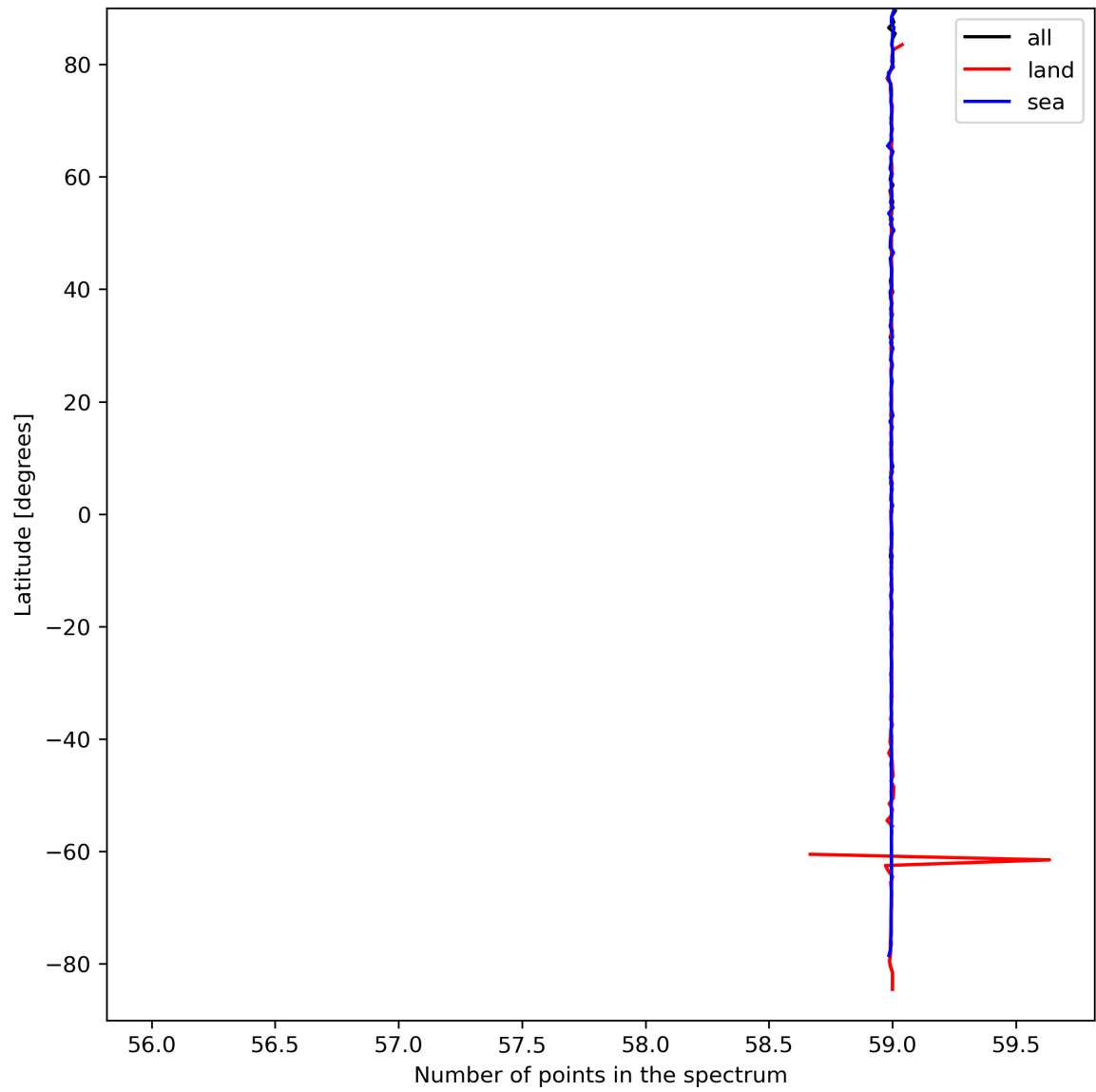
Figure 27: Zonal average of “Number of points in the spectrum” for 2024-03-27 to 2024-03-29.
