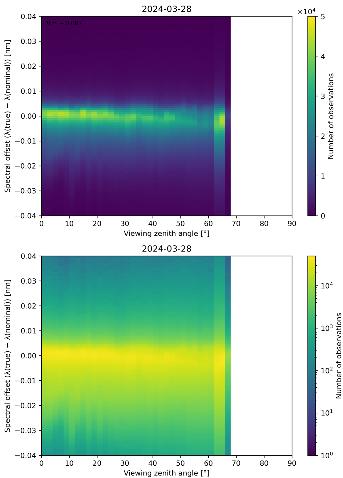
Figure 128: Scatter density plot of “Viewing zenith angle” against “Spectral offset ( \lambda(\text{true}) - \lambda(\text{nominal}) )” for 2024-03-27 to 2024-03-29.
