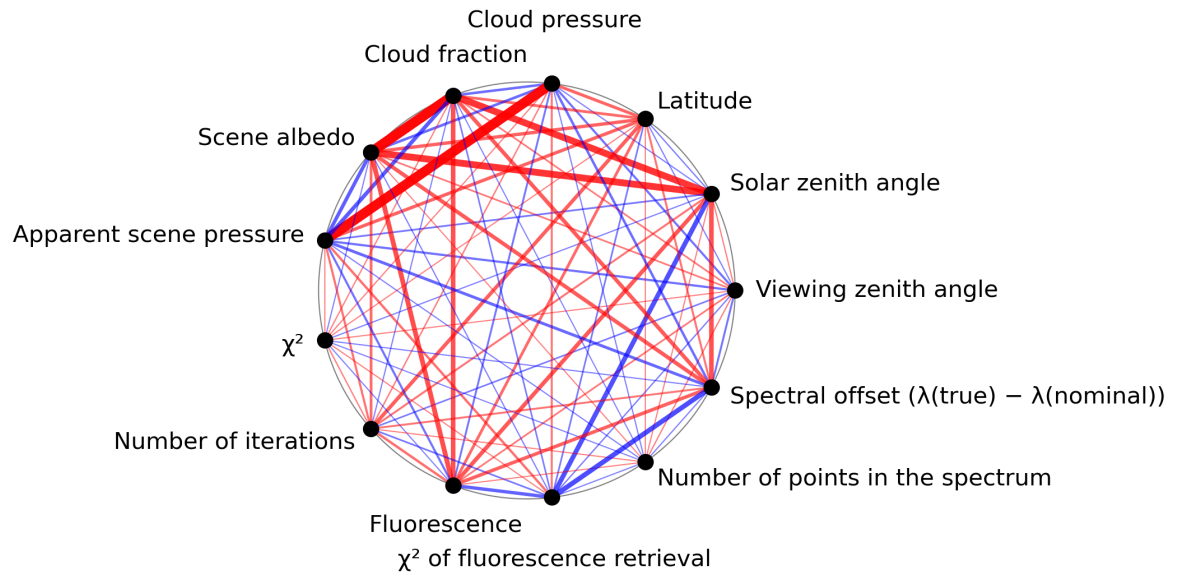
Figure 1: Map of correlation graph for 2024-03-27 to 2024-03-29.
