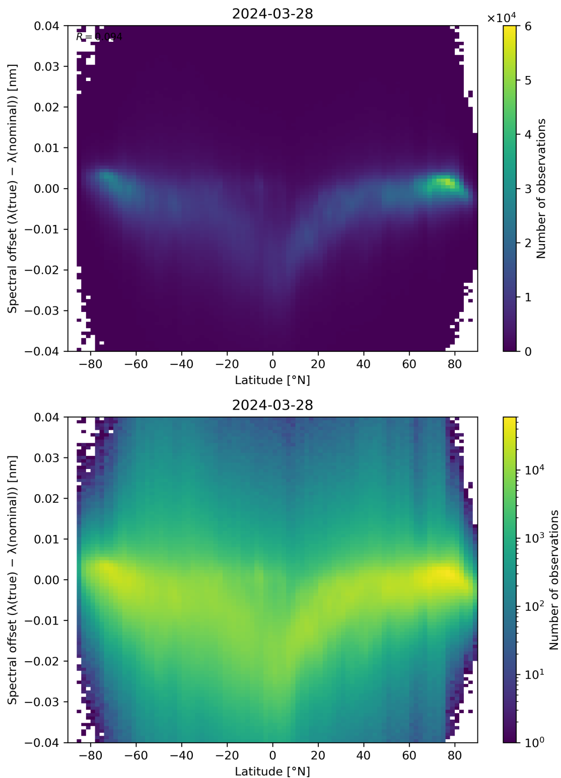
Figure 96: Scatter density plot of “Latitude” against “Spectral offset ( \lambda(\text{true}) - \lambda(\text{nominal}) )” for 2024-03-27 to 2024-03-29.
