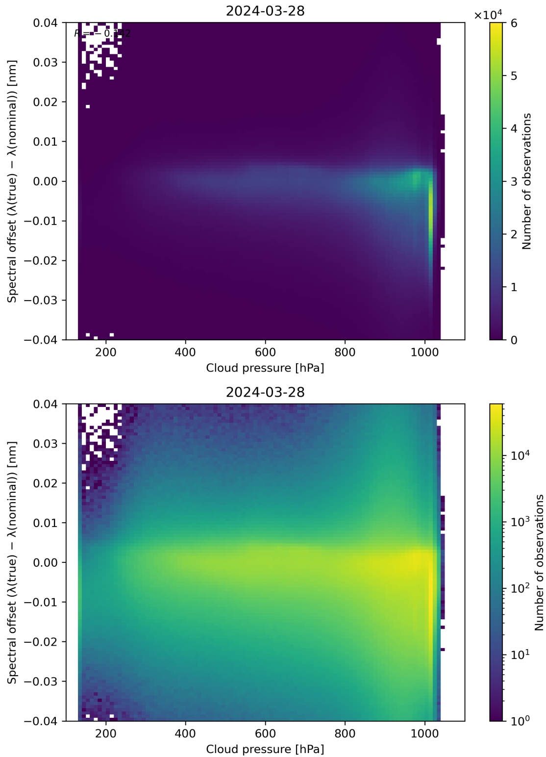
Figure 84: Scatter density plot of “Cloud pressure” against “Spectral offset ( \lambda(\text{true}) - \lambda(\text{nominal}) )” for 2024-03-27 to 2024-03-29.
