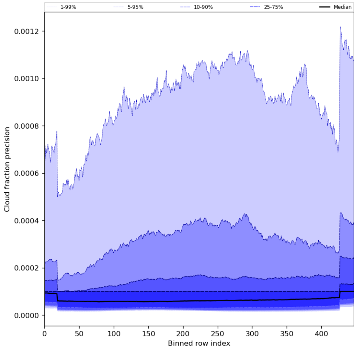
Figure 50: Along track statistics of “Cloud fraction precision” for 2024-03-27 to 2024-03-29
