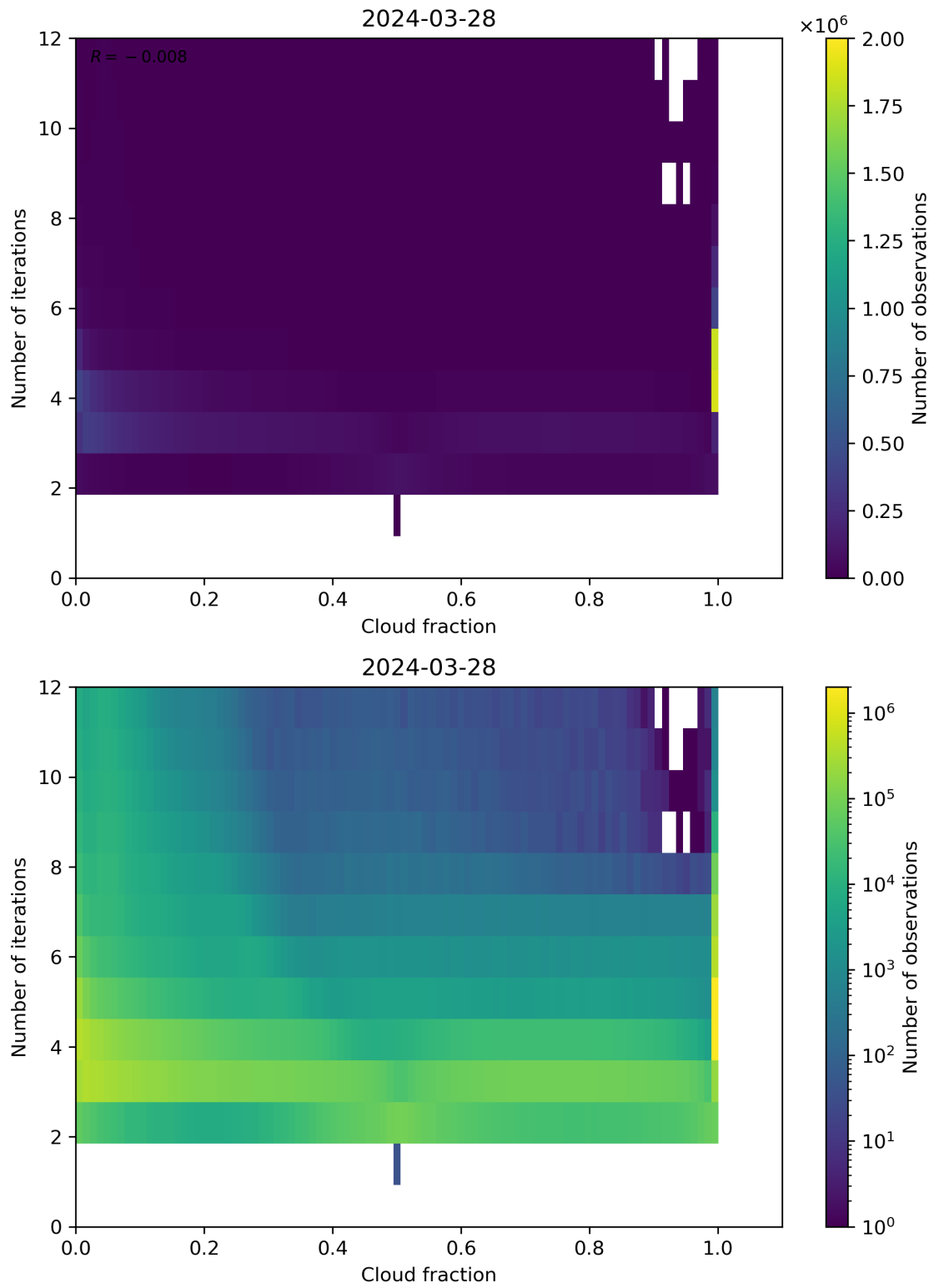
Figure 73: Scatter density plot of “Cloud fraction” against “Number of iterations” for 2024-03-27 to 2024-03-29.
