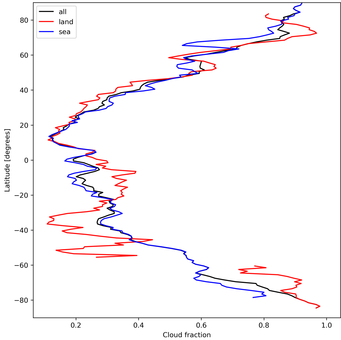
Figure 15: Zonal average of “Cloud fraction” for 2024-03-27 to 2024-03-29.
