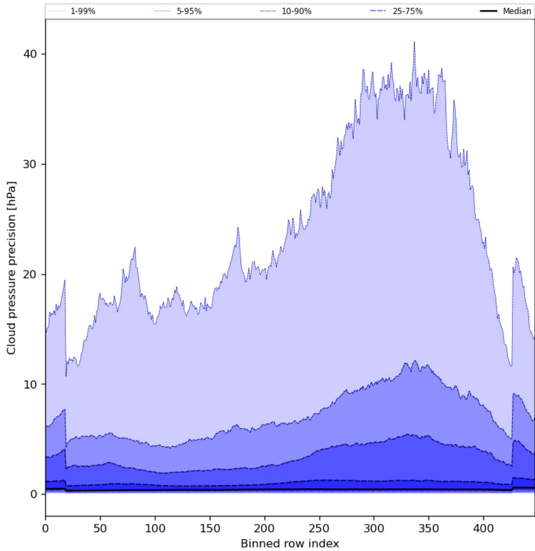
Figure 48: Along track statistics of “Cloud pressure precision” for 2024-03-27 to 2024-03-29
