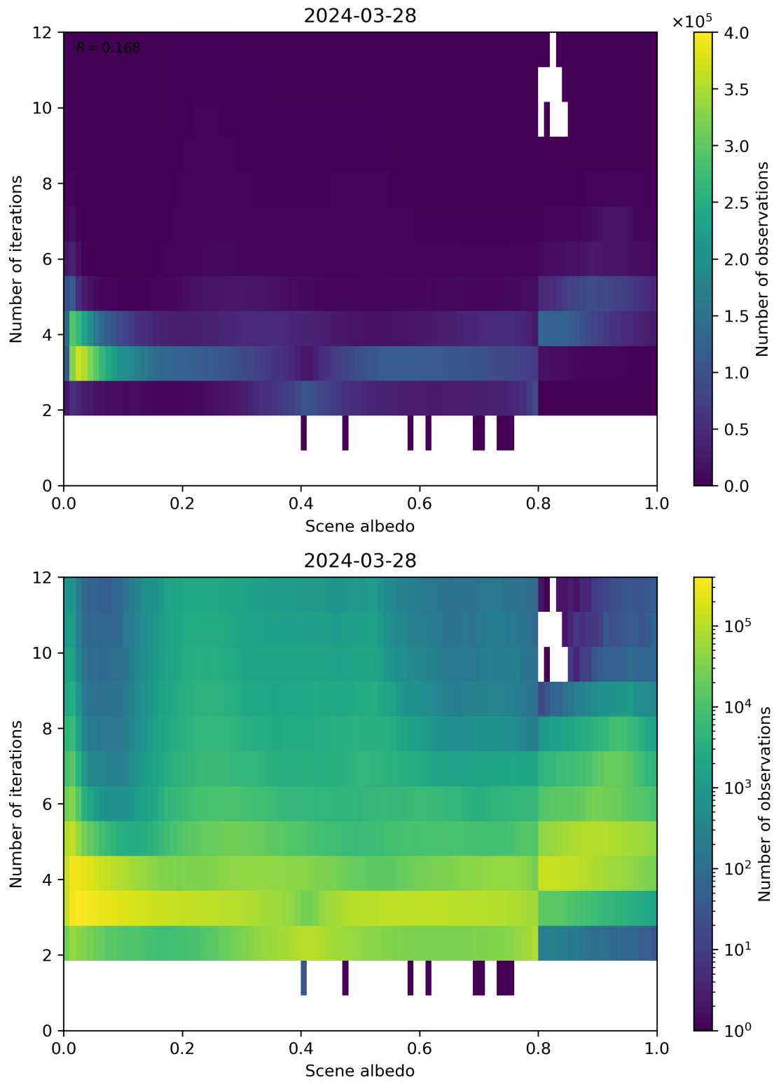
Figure 105: Scatter density plot of “Scene albedo” against “Number of iterations” for 2024-03-27 to 2024-03-29.
