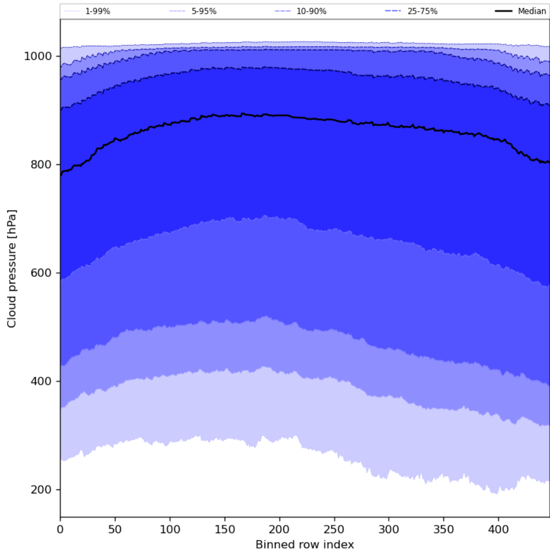
Figure 47: Along track statistics of “Cloud pressure” for 2024-03-27 to 2024-03-29
