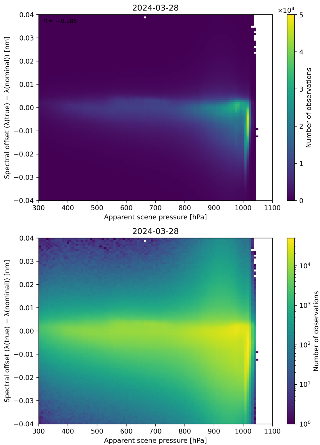
Figure 67: Scatter density plot of “Apparent scene pressure” against “Spectral offset ( \lambda(\text{true}) - \lambda(\text{nominal}) )” for 2024-03-27 to 2024-03-29.
