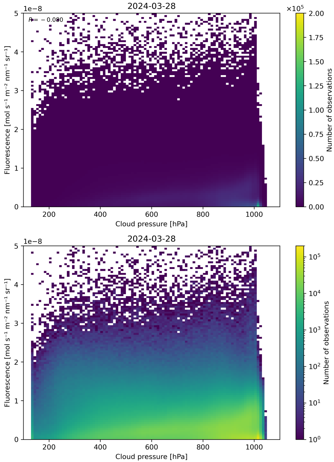
Figure 80: Scatter density plot of “Cloud pressure” against “Fluorescence” for 2024-03-27 to 2024-03-29.
