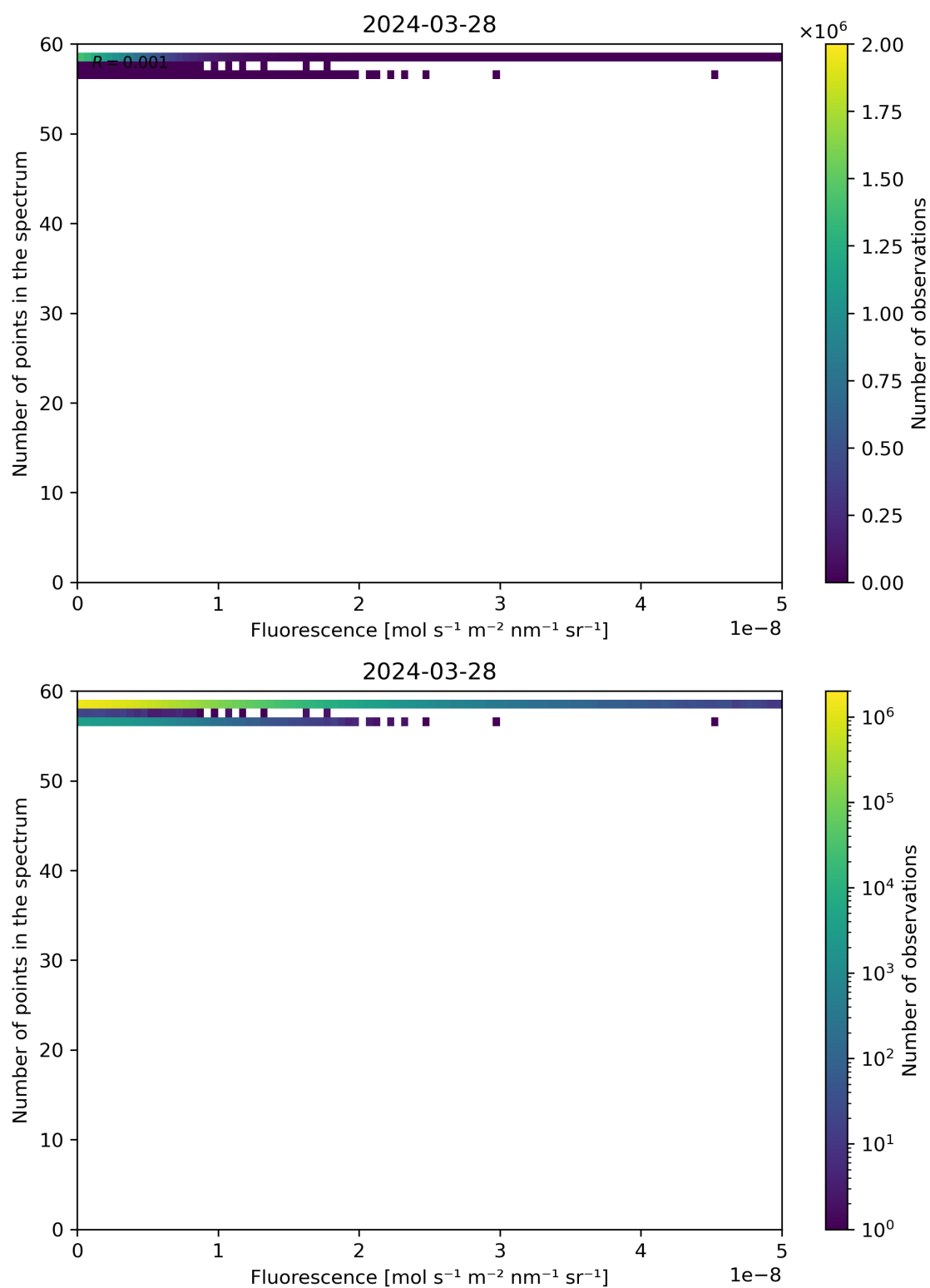
Figure 86: Scatter density plot of “Fluorescence” against “Number of points in the spectrum” for 2024-03-27 to 2024-03-29.
