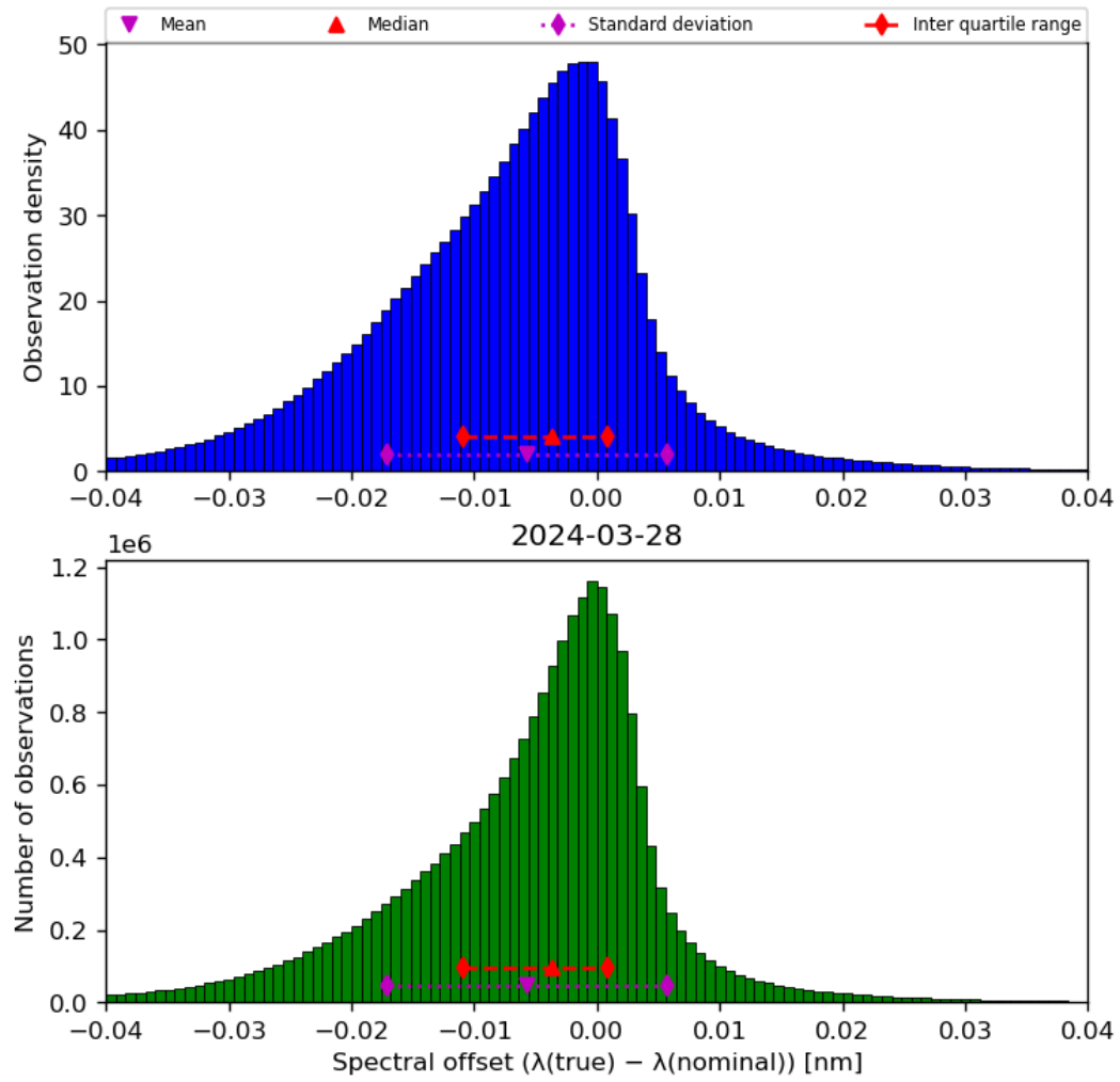
Figure 45: Histogram of “Spectral offset ( \lambda(\text{true}) - \lambda(\text{nominal}) )” for 2024-03-27 to 2024-03-29
