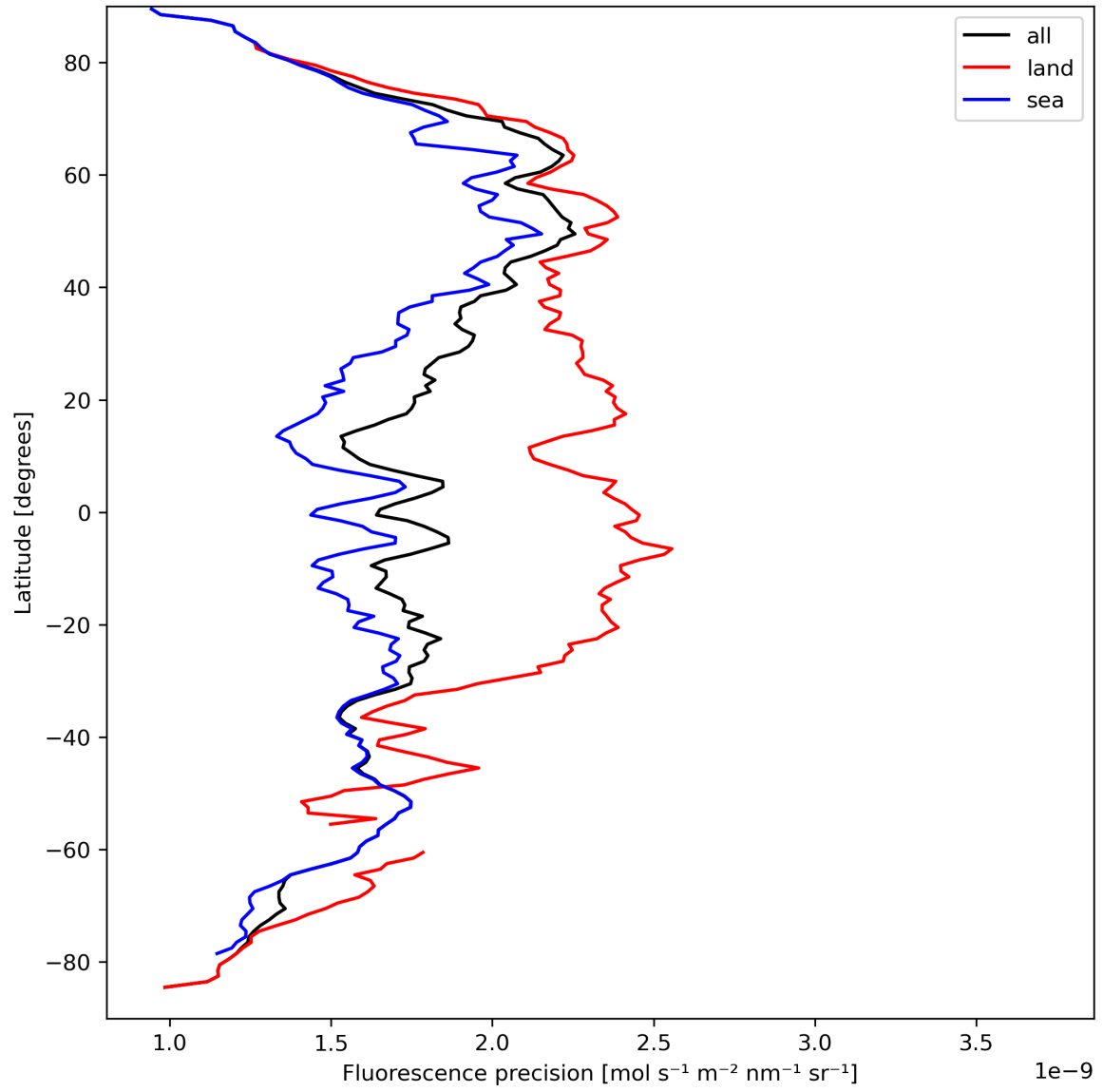
Figure 24: Zonal average of “Fluorescence precision” for 2024-03-27 to 2024-03-29.
