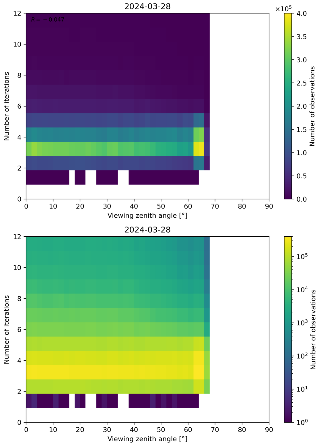
Figure 124: Scatter density plot of “Viewing zenith angle” against “Number of iterations” for 2024-03-27 to 2024-03-29.
