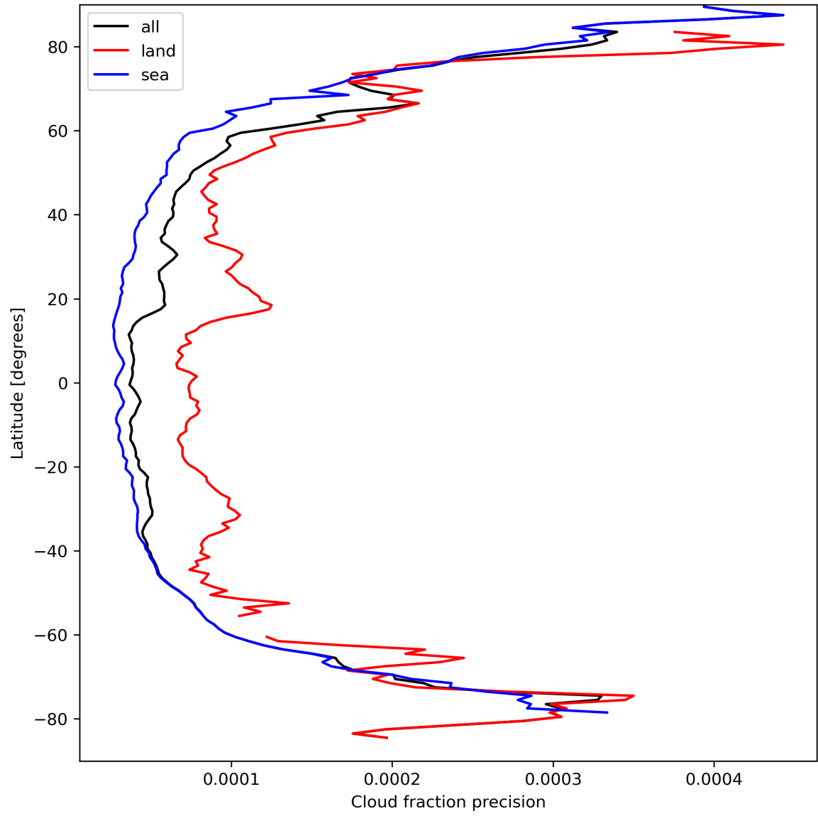
Figure 16: Zonal average of “Cloud fraction precision” for 2024-03-27 to 2024-03-29.
