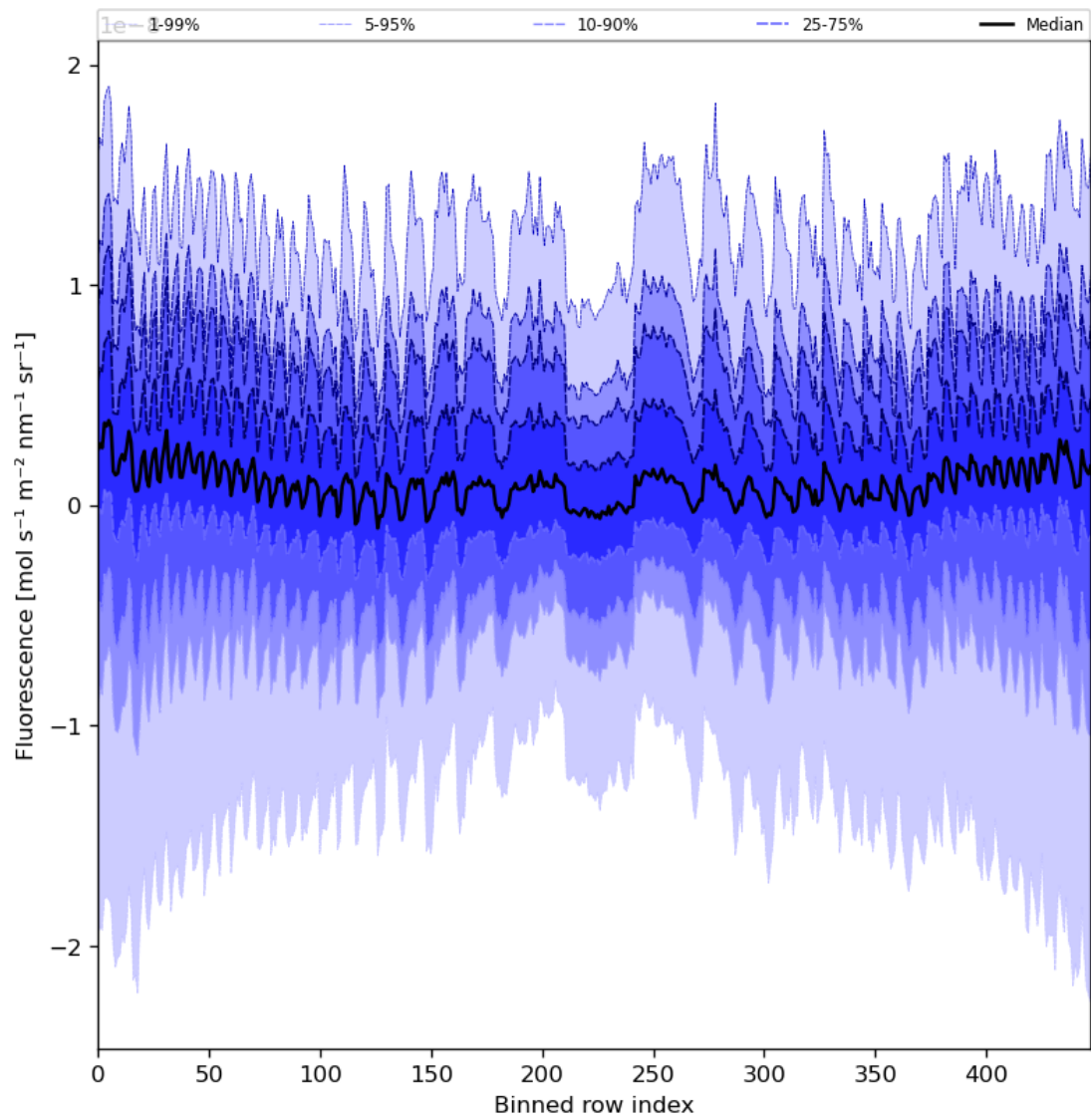
Figure 57: Along track statistics of “Fluorescence” for 2024-03-27 to 2024-03-29
