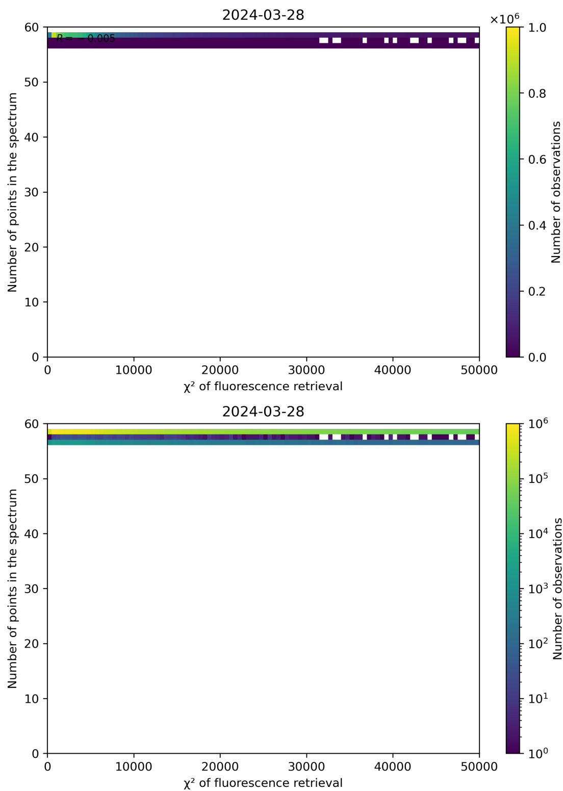
Figure 68: Scatter density plot of “ \chi^2 of fluorescence retrieval” against “Number of points in the spectrum” for 2024-03-27 to 2024-03-29.
