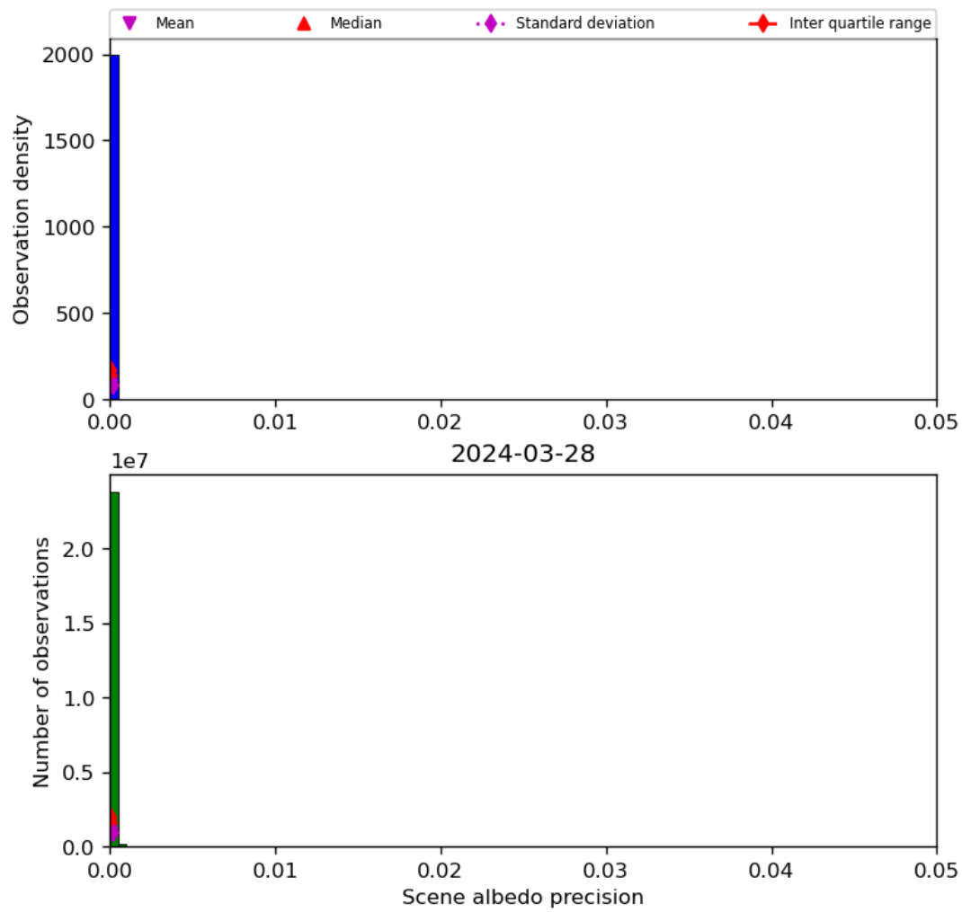
Figure 35: Histogram of “Scene albedo precision” for 2024-03-27 to 2024-03-29
