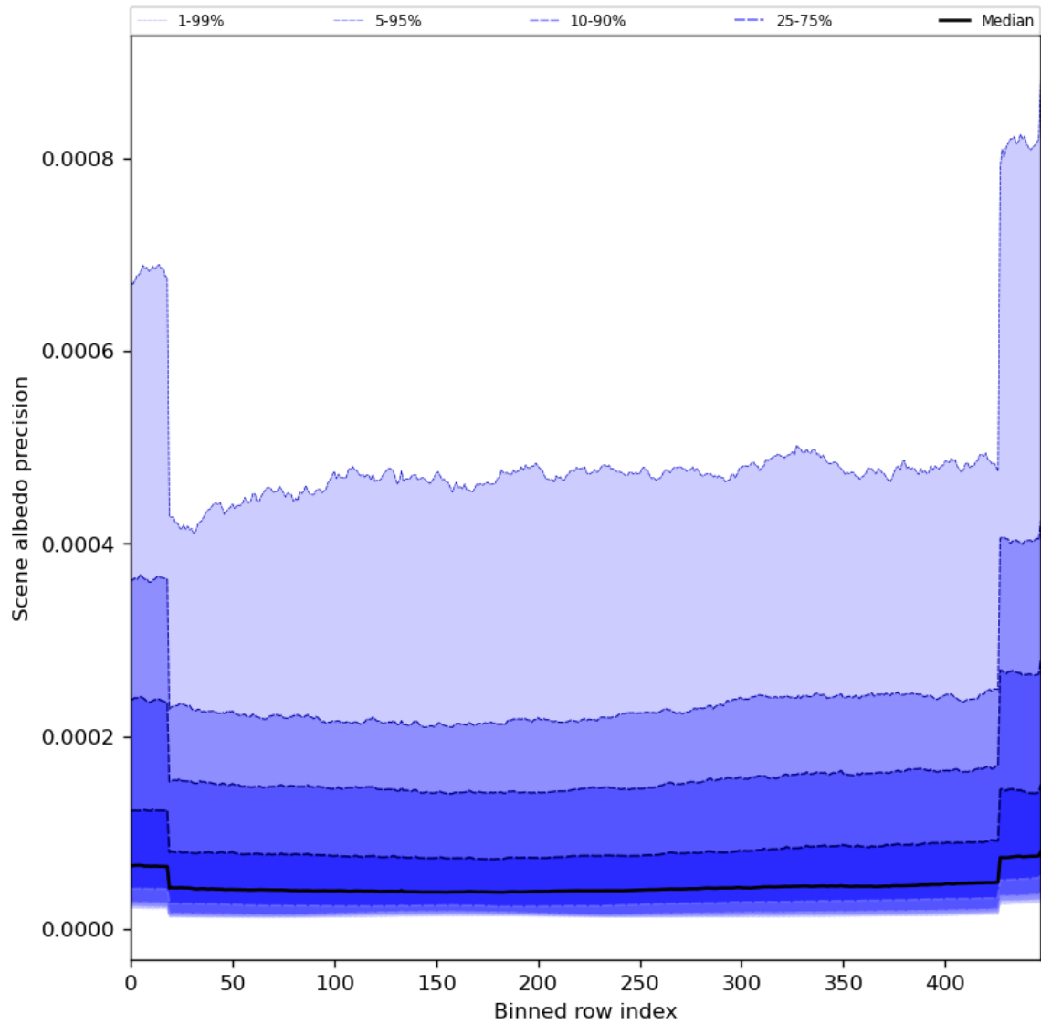
Figure 52: Along track statistics of “Scene albedo precision” for 2024-03-27 to 2024-03-29
