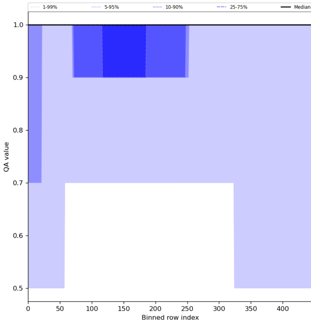
Figure 46: Along track statistics of “QA value” for 2024-03-27 to 2024-03-29
