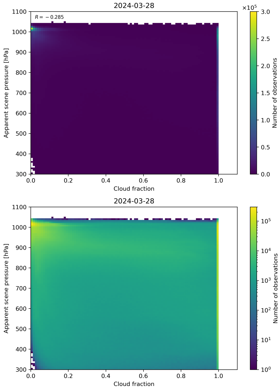
Figure 70: Scatter density plot of “Cloud fraction” against “Apparent scene pressure” for 2024-03-27 to 2024-03-29.
