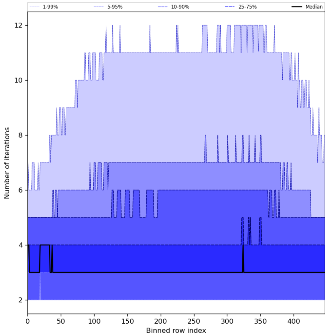
Figure 56: Along track statistics of “Number of iterations” for 2024-03-27 to 2024-03-29
