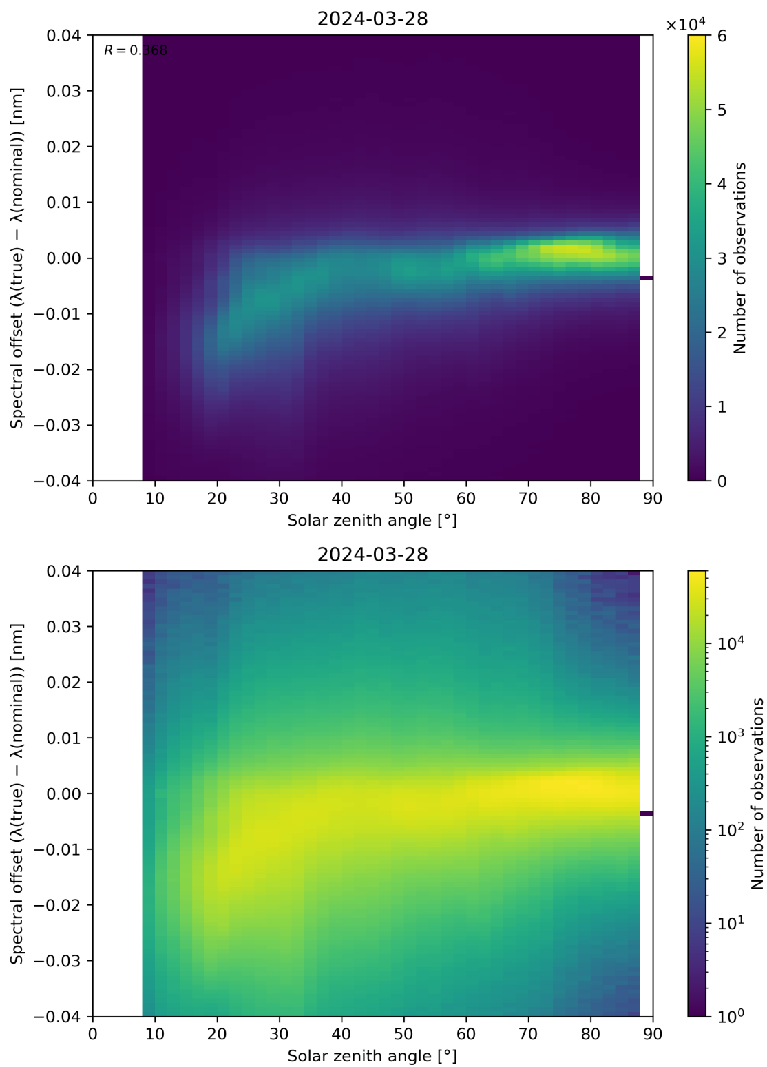
Figure 117: Scatter density plot of “Solar zenith angle” against “Spectral offset ( \lambda(\text{true}) - \lambda(\text{nominal}) )” for 2024-03-27 to 2024-03-29.
