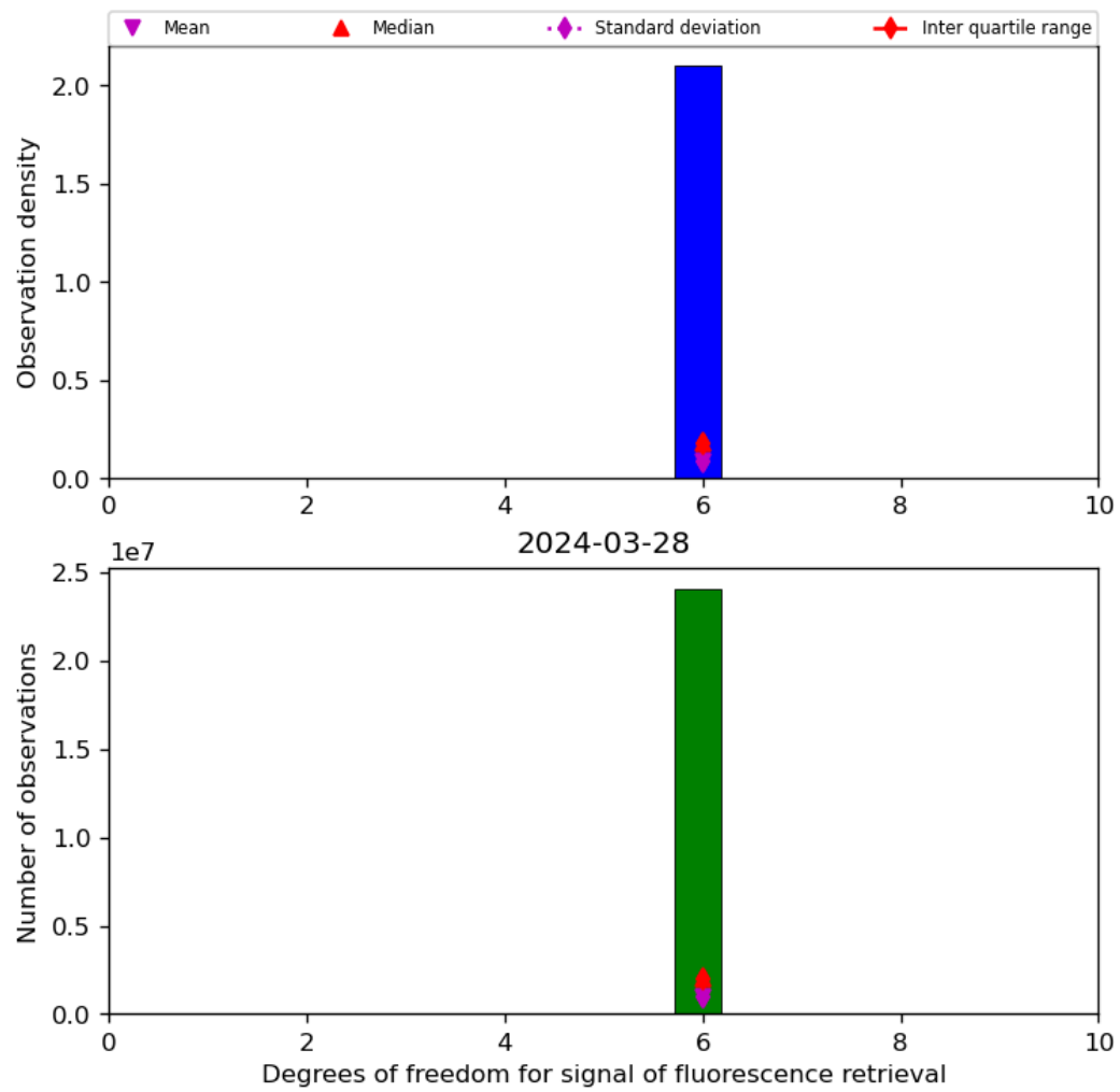
Figure 43: Histogram of “Degrees of freedom for signal of fluorescence retrieval” for 2024-03-27 to 2024-03-29
