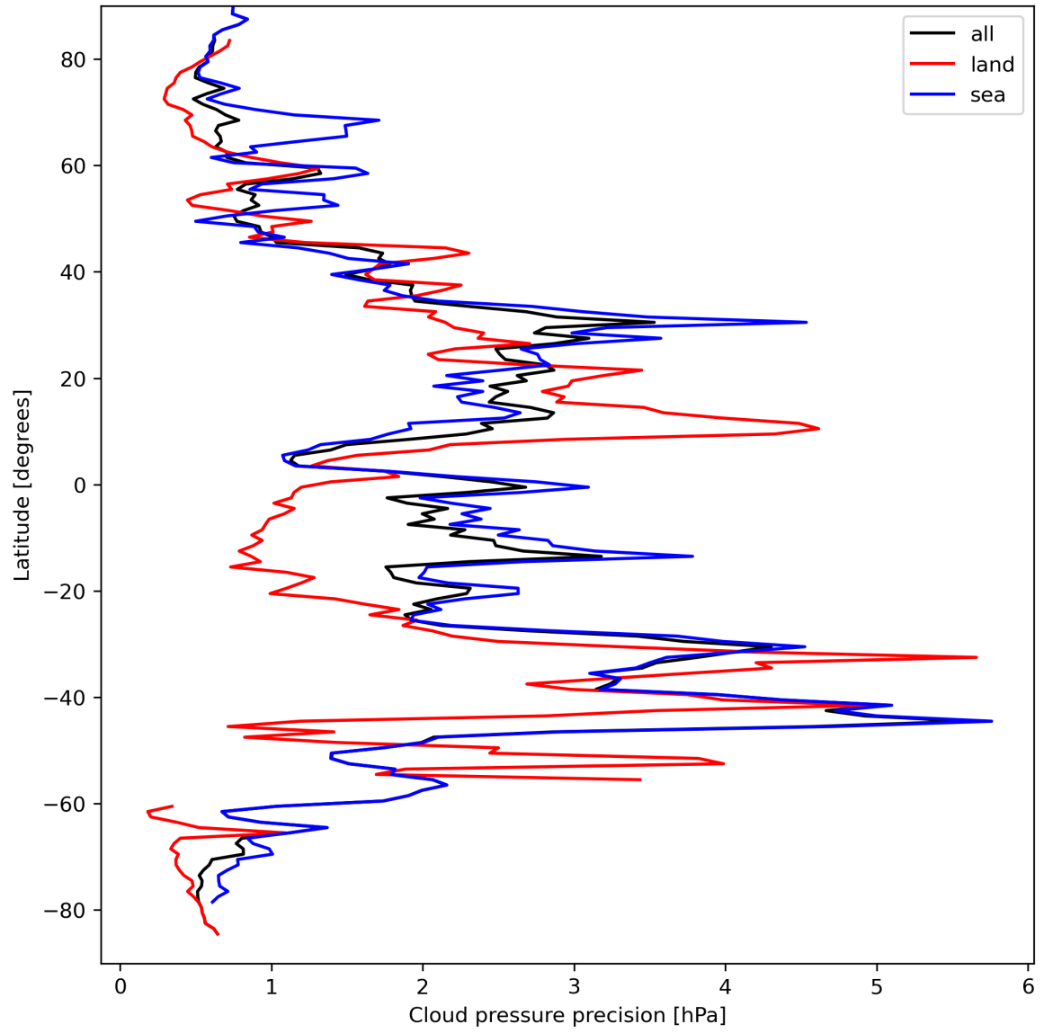
Figure 14: Zonal average of “Cloud pressure precision” for 2024-03-27 to 2024-03-29.
