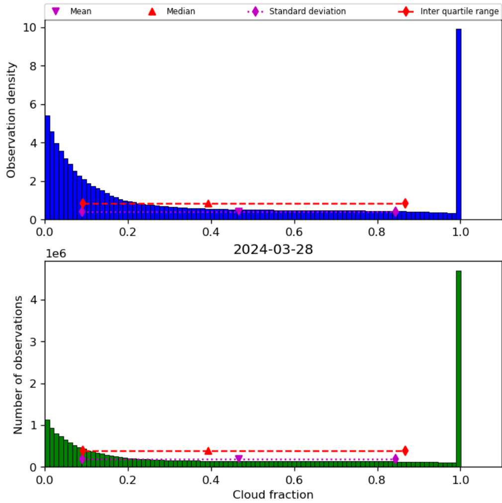
Figure 32: Histogram of “Cloud fraction” for 2024-03-27 to 2024-03-29
