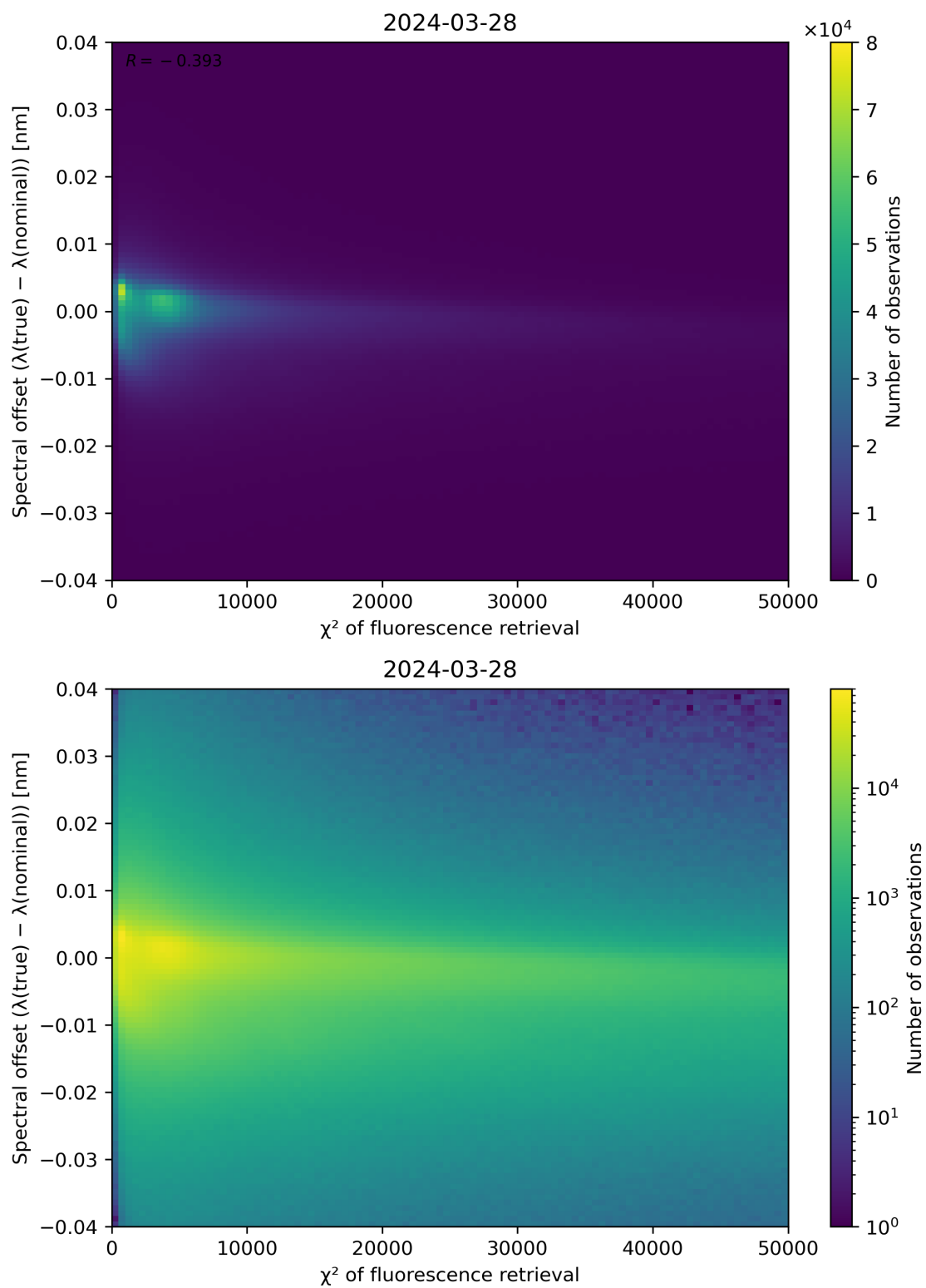
Figure 69: Scatter density plot of " \chi^2 of fluorescence retrieval" against "Spectral offset ( \lambda(\text{true}) - \lambda(\text{nominal})) " for 2024-03-27 to 2024-03-29.
