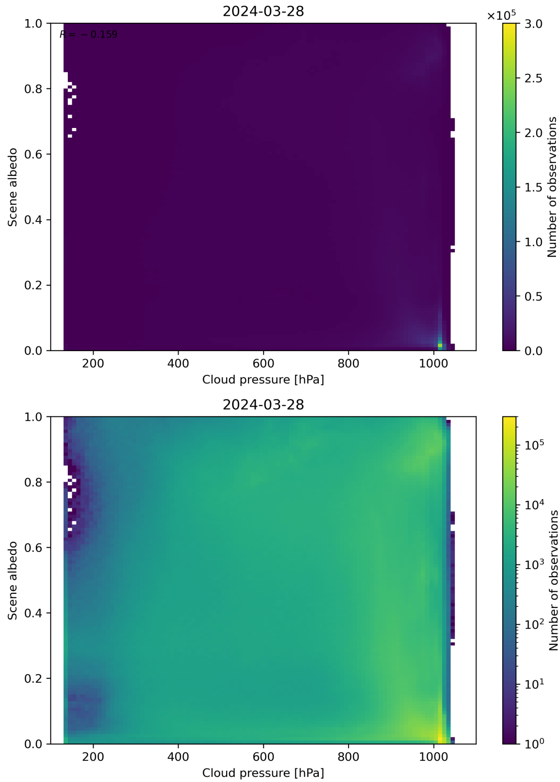
Figure 83: Scatter density plot of “Cloud pressure” against “Scene albedo” for 2024-03-27 to 2024-03-29.
