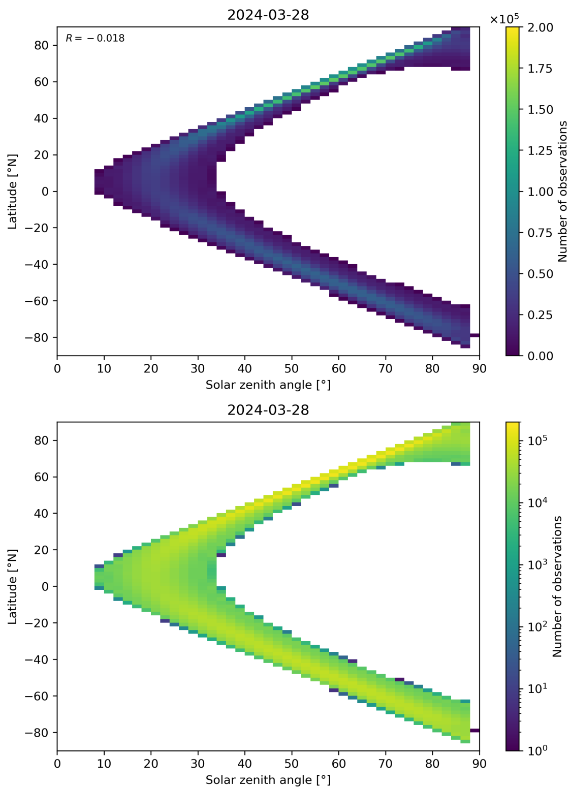
Figure 113: Scatter density plot of “Solar zenith angle” against “Latitude” for 2024-03-27 to 2024-03-29.
