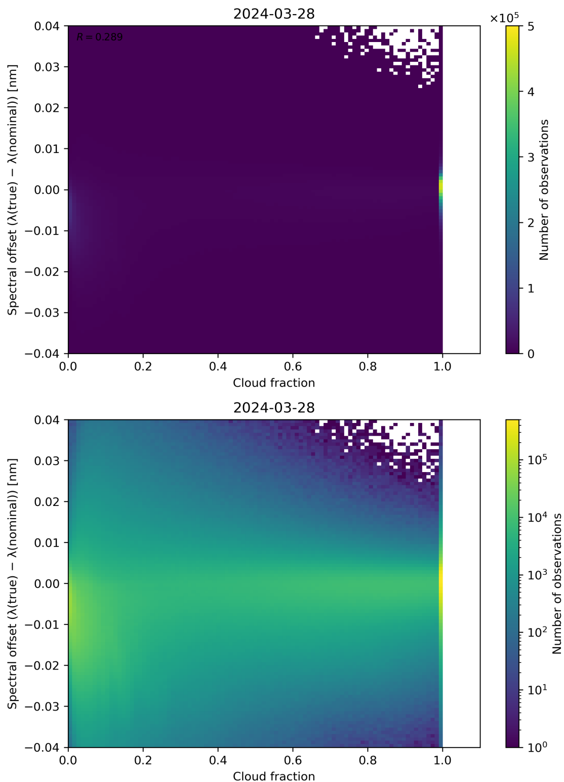
Figure 76: Scatter density plot of “Cloud fraction” against “Spectral offset ( \lambda(\text{true}) - \lambda(\text{nominal}) )” for 2024-03-27 to 2024-03-29.
