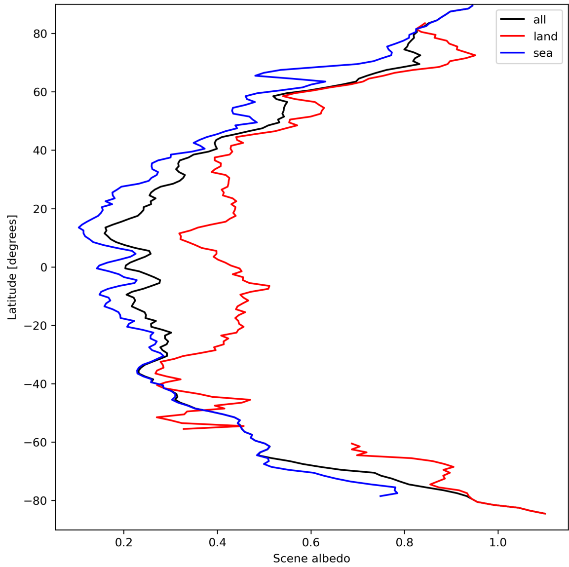
Figure 17: Zonal average of “Scene albedo” for 2024-03-27 to 2024-03-29.
