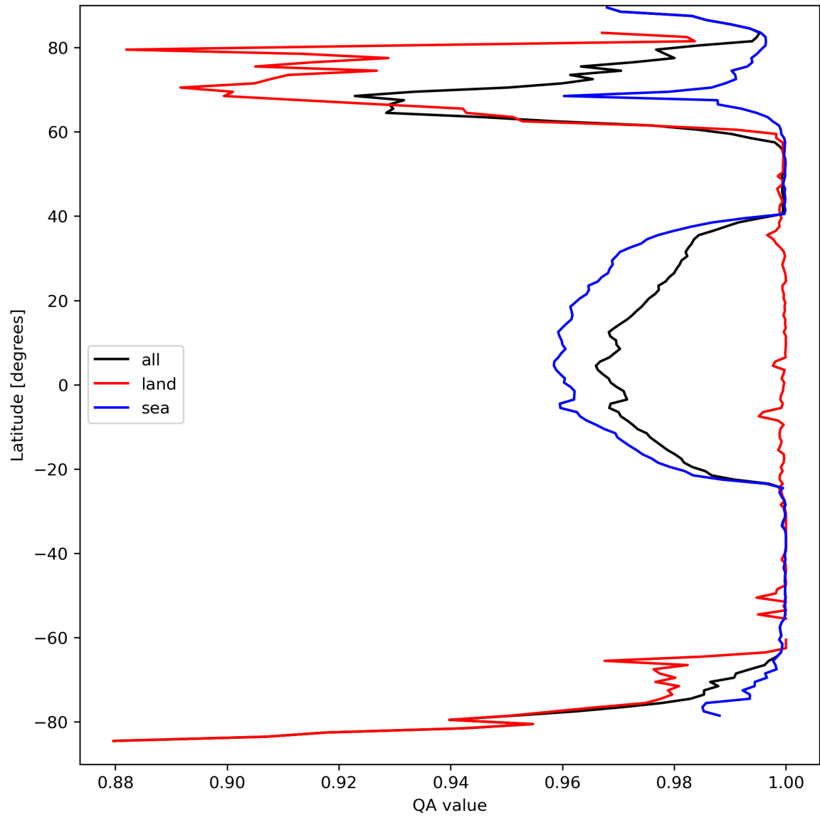
Figure 12: Zonal average of “QA value” for 2024-03-27 to 2024-03-29.
