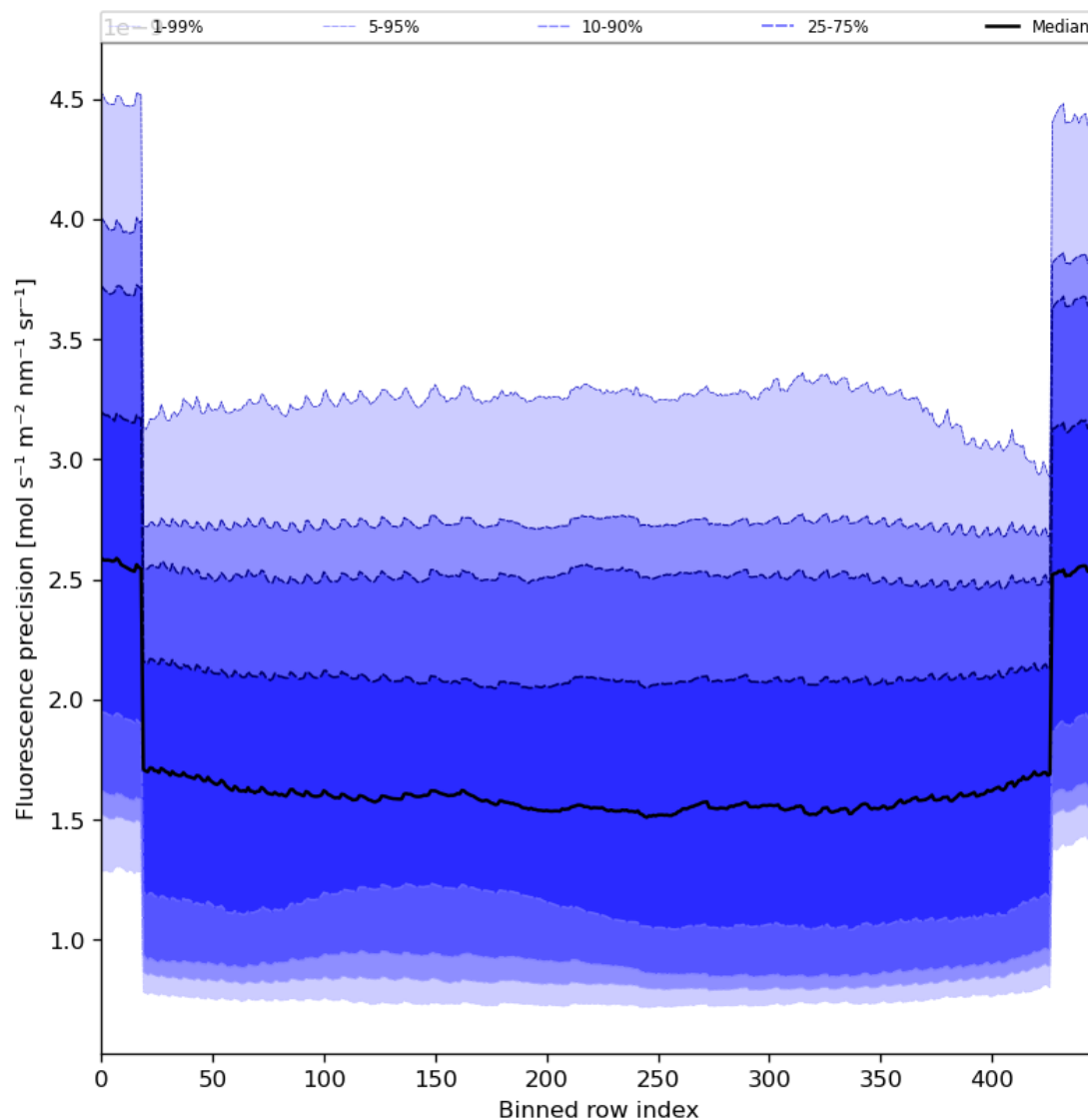
Figure 58: Along track statistics of “Fluorescence precision” for 2024-03-27 to 2024-03-29
