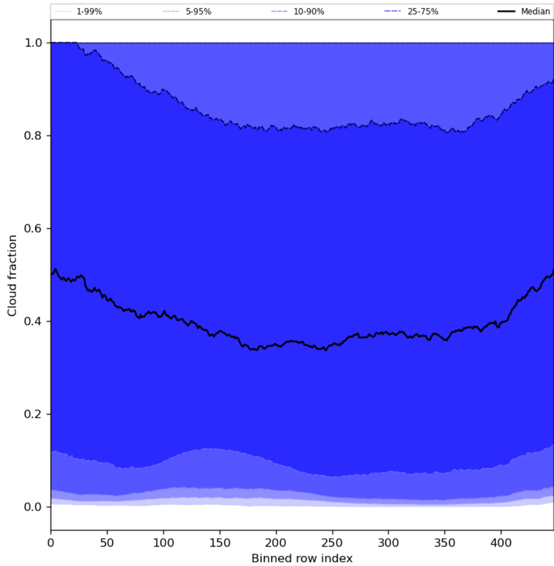
Figure 49: Along track statistics of “Cloud fraction” for 2024-03-27 to 2024-03-29
