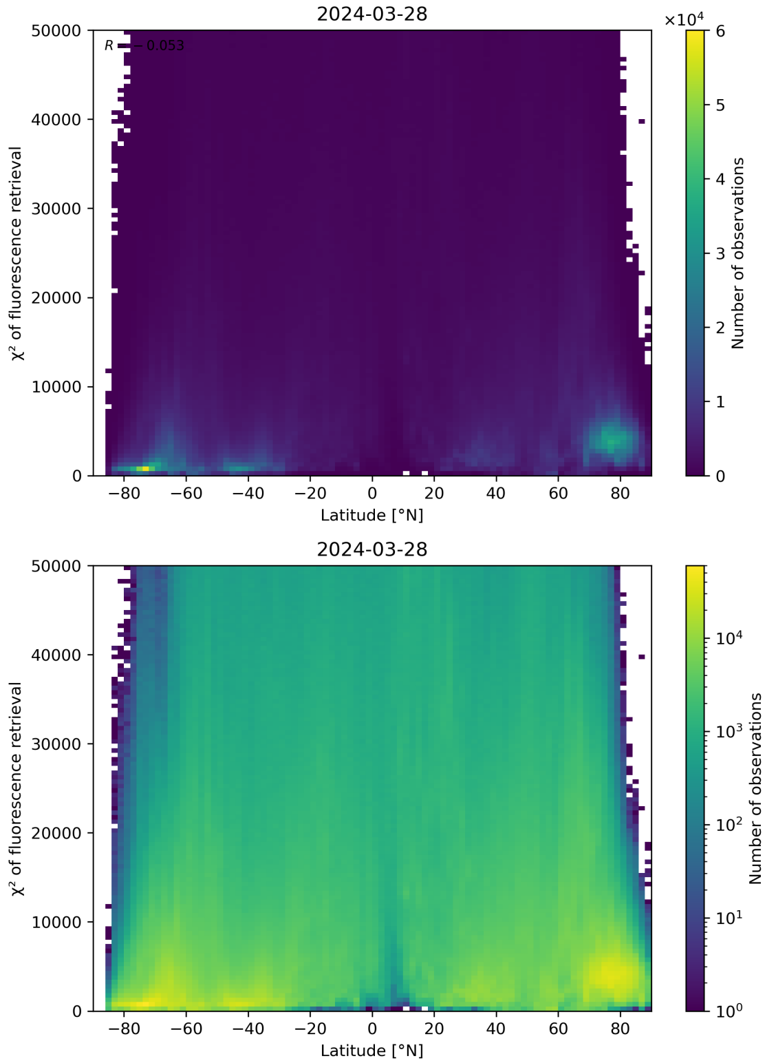
Figure 89: Scatter density plot of “Latitude” against “ \chi^2 of fluorescence retrieval” for 2024-03-27 to 2024-03-29.
