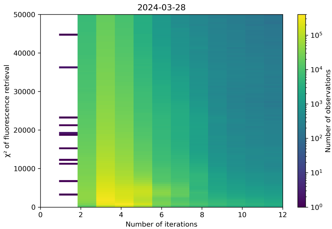
Figure 97: Scatter density plot of “Number of iterations” against “ \chi^2 of fluorescence retrieval” for 2024-03-27 to 2024-03-29.
