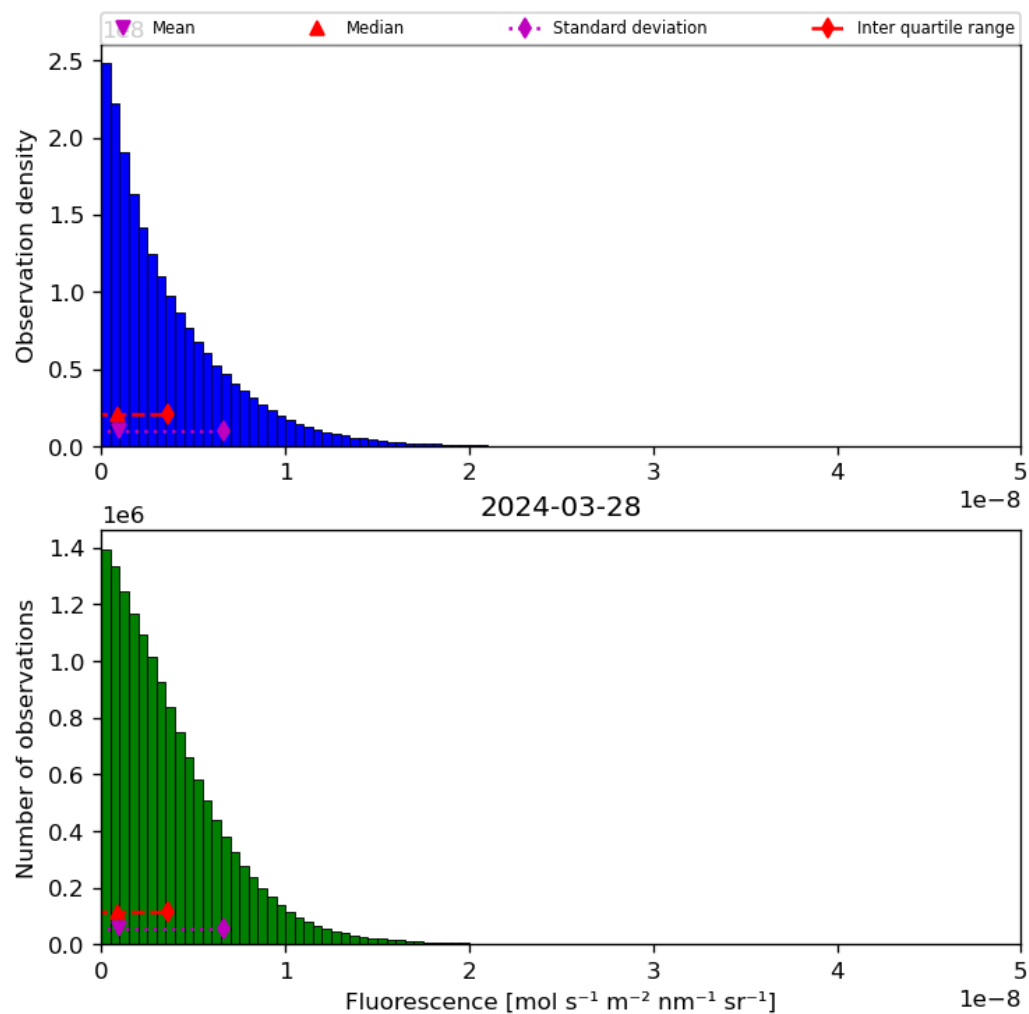
Figure 40: Histogram of “Fluorescence” for 2024-03-27 to 2024-03-29
