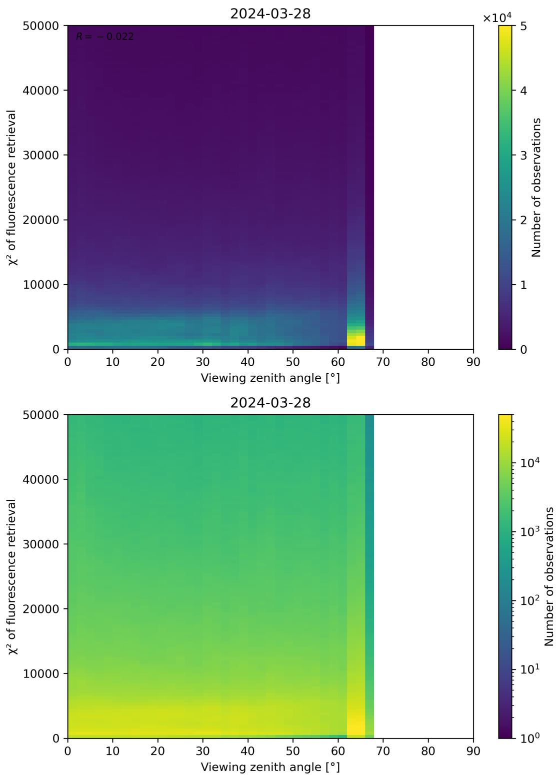
Figure 119: Scatter density plot of “Viewing zenith angle” against “ \chi^2 of fluorescence retrieval” for 2024-03-27 to 2024-03-29.
