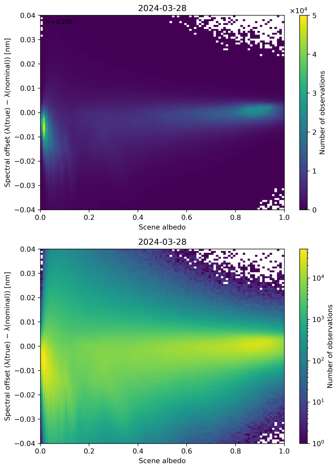
Figure 107: Scatter density plot of “Scene albedo” against “Spectral offset ( \lambda(\text{true}) - \lambda(\text{nominal}) )” for 2024-03-27 to 2024-03-29.
