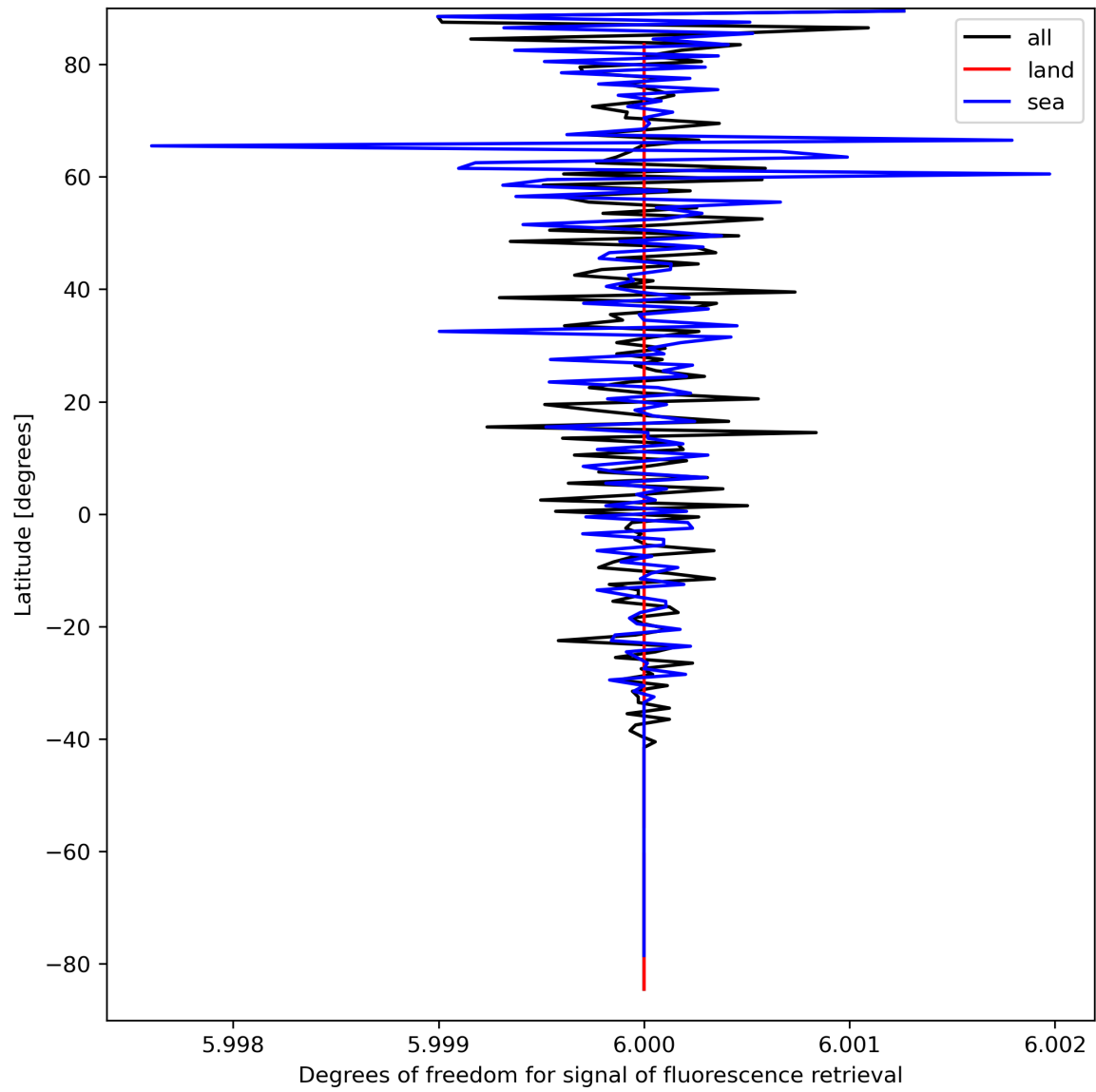
Figure 26: Zonal average of “Degrees of freedom for signal of fluorescence retrieval” for 2024-03-27 to 2024-03-29.
