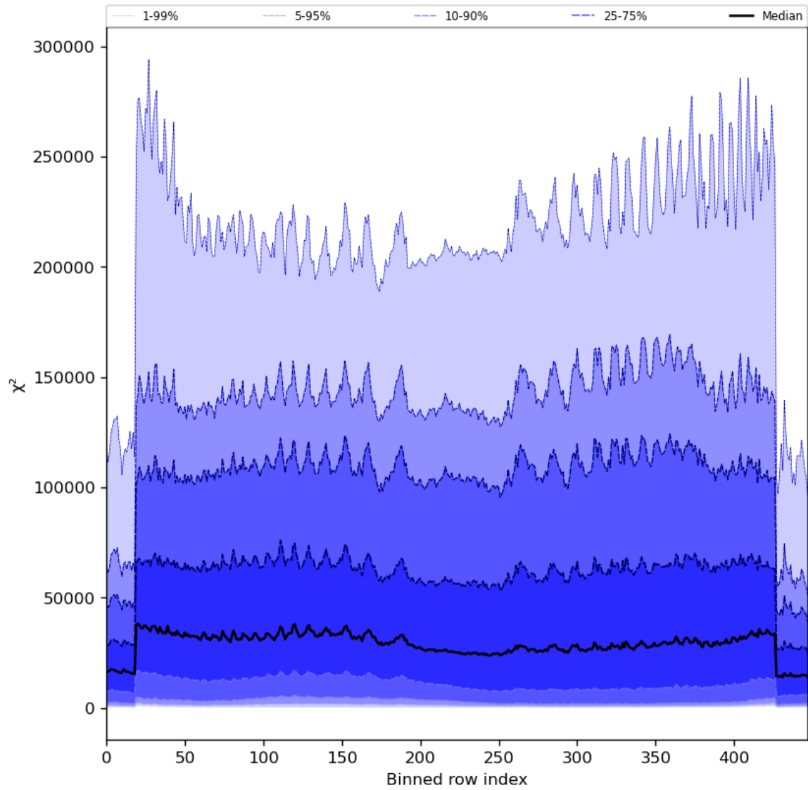
Figure 55: Along track statistics of “ \chi^2 ” for 2024-03-27 to 2024-03-29
