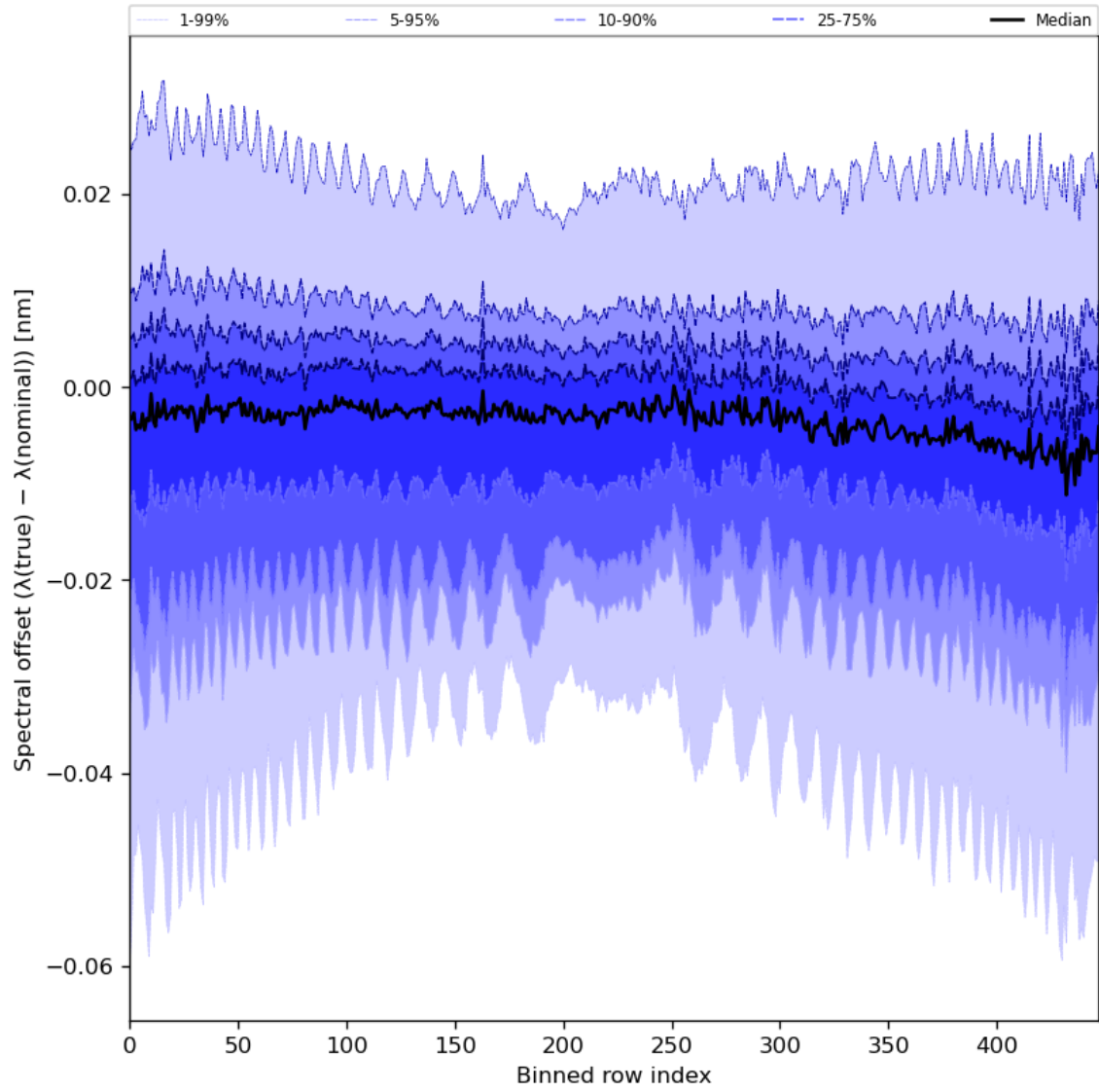
Figure 62: Along track statistics of “Spectral offset ( \lambda(\text{true}) - \lambda(\text{nominal}) )” for 2024-03-27 to 2024-03-29
