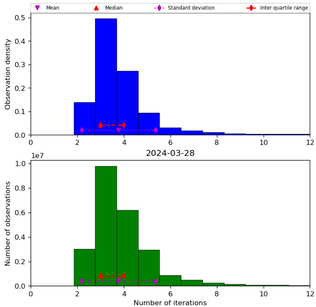
Figure 39: Histogram of “Number of iterations” for 2024-03-27 to 2024-03-29
