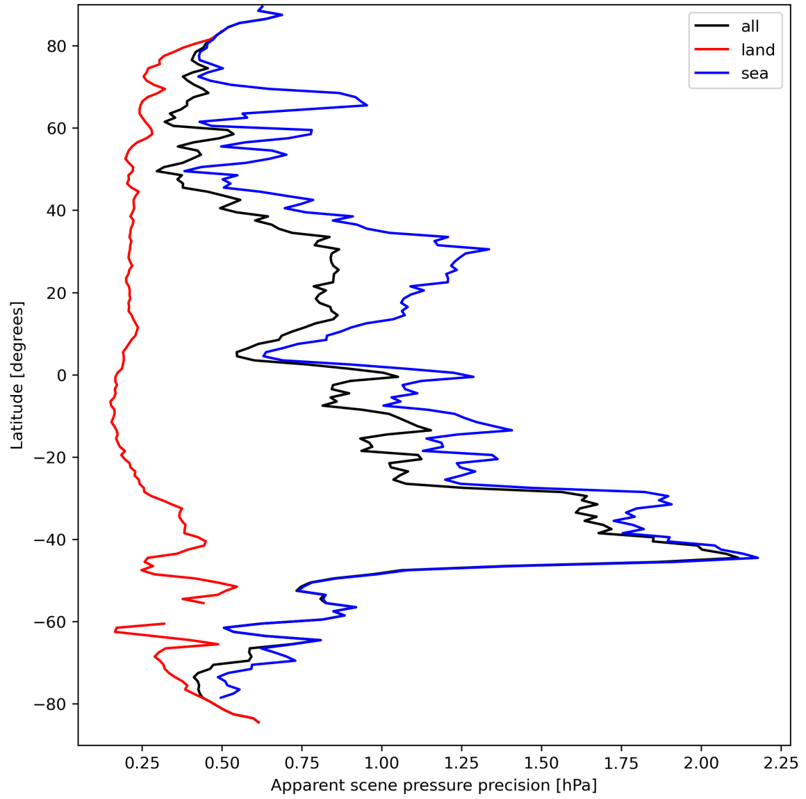
Figure 20: Zonal average of “Apparent scene pressure precision” for 2024-03-27 to 2024-03-29.
