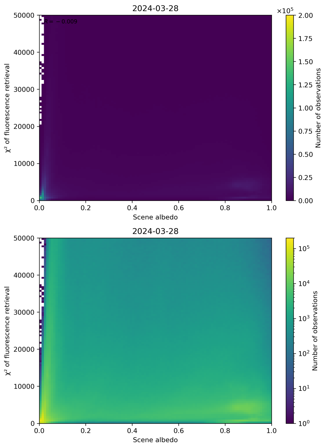
Figure 103: Scatter density plot of “Scene albedo” against “ \chi^2 of fluorescence retrieval” for 2024-03-27 to 2024-03-29.
