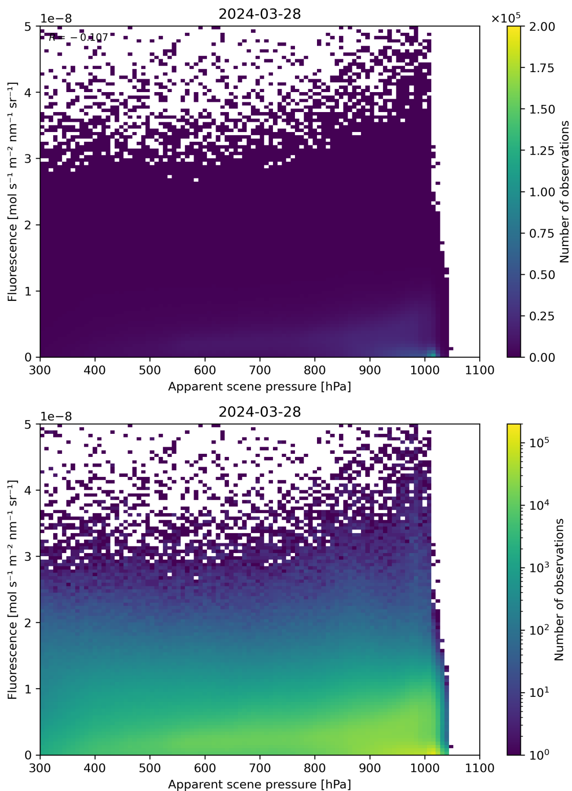
Figure 64: Scatter density plot of “Apparent scene pressure” against “Fluorescence” for 2024-03-27 to 2024-03-29.
