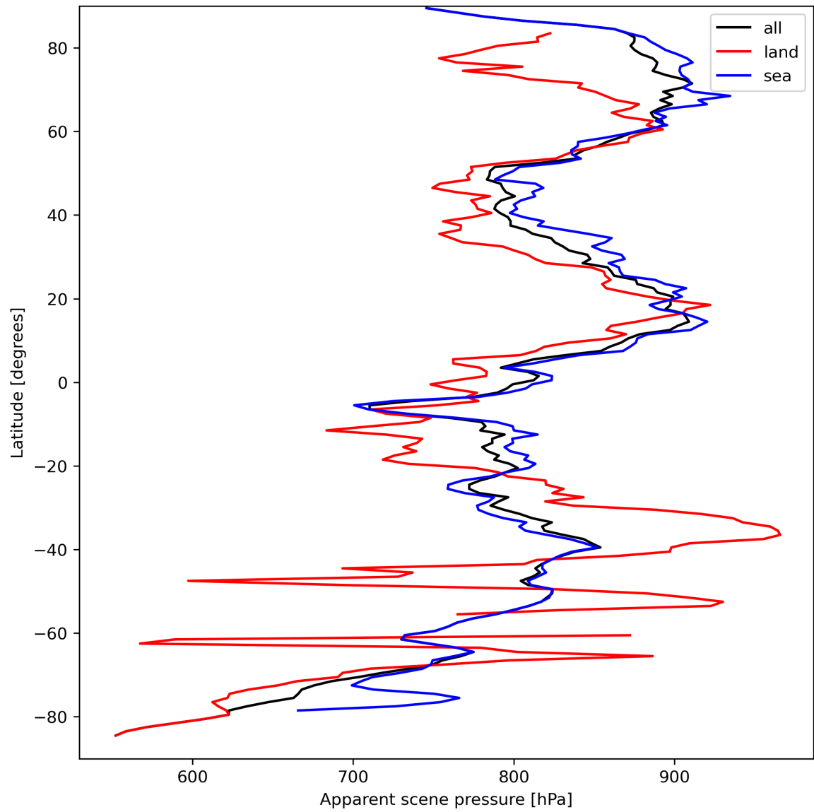
Figure 19: Zonal average of “Apparent scene pressure” for 2024-03-27 to 2024-03-29.
