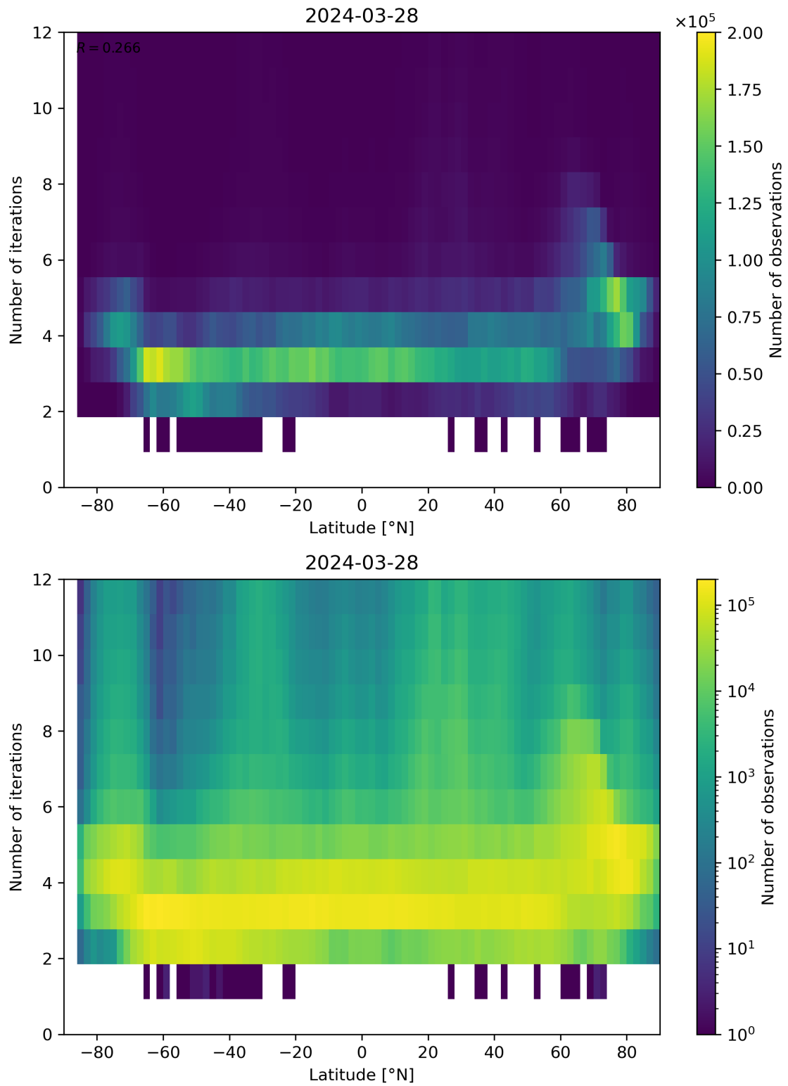
Figure 93: Scatter density plot of “Latitude” against “Number of iterations” for 2024-03-27 to 2024-03-29.
