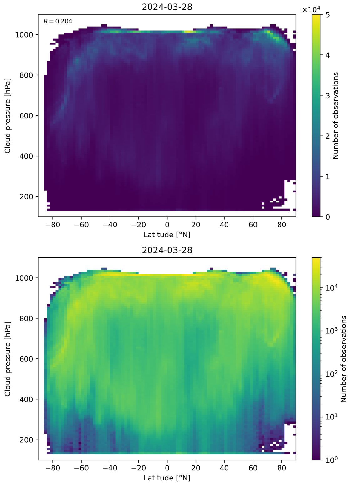
Figure 91: Scatter density plot of “Latitude” against “Cloud pressure” for 2024-03-27 to 2024-03-29.
