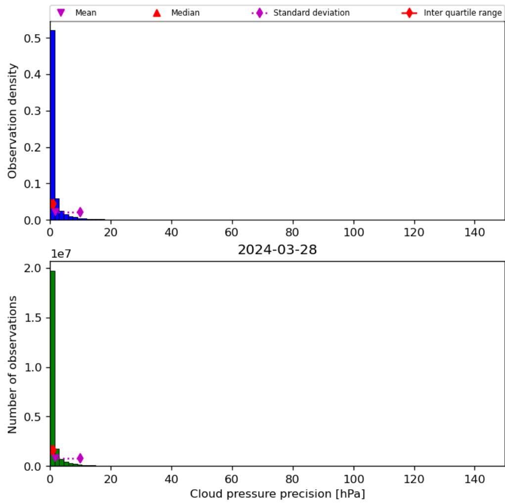
Figure 31: Histogram of “Cloud pressure precision” for 2024-03-27 to 2024-03-29
