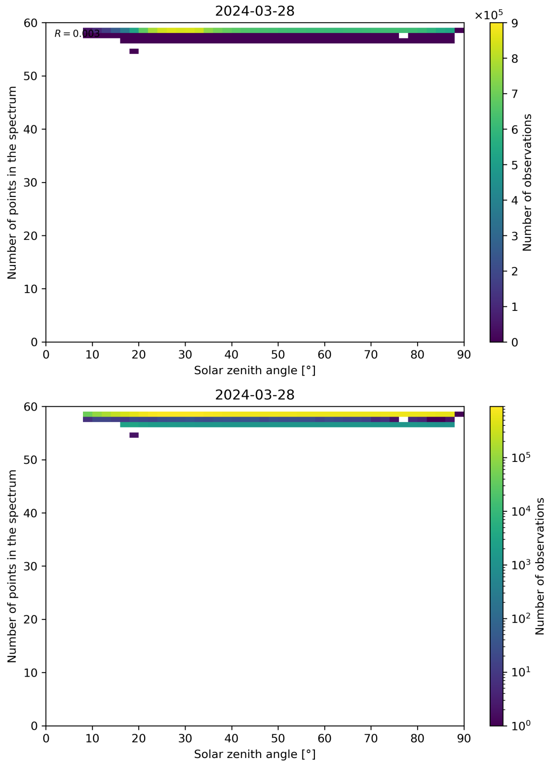
Figure 115: Scatter density plot of “Solar zenith angle” against “Number of points in the spectrum” for 2024-03-27 to 2024-03-29.
