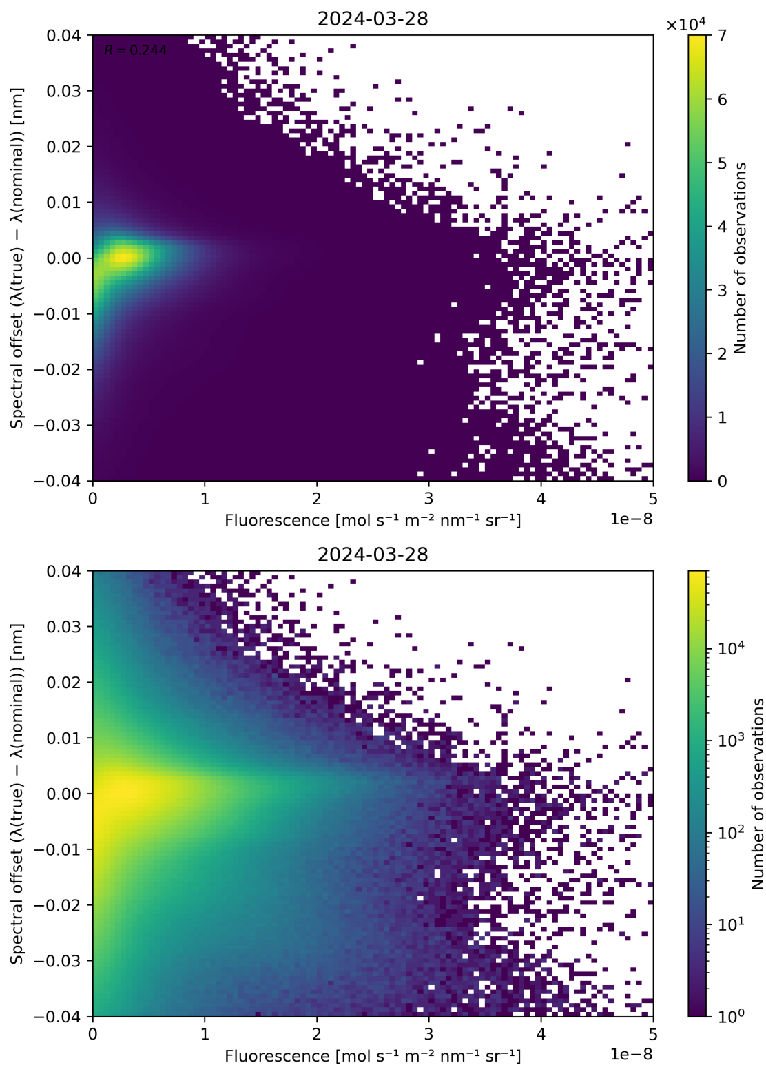
Figure 87: Scatter density plot of “Fluorescence” against “Spectral offset ( \lambda(\text{true}) - \lambda(\text{nominal}) )” for 2024-03-27 to 2024-03-29.
