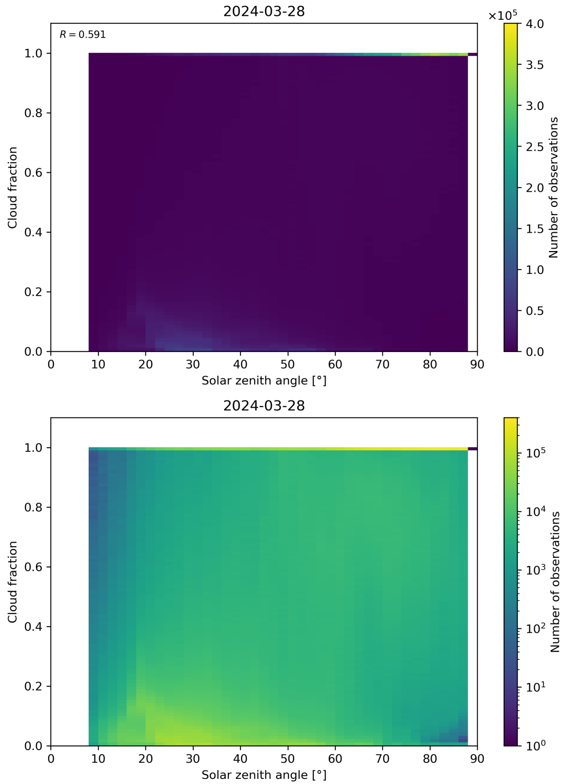
Figure 110: Scatter density plot of “Solar zenith angle” against “Cloud fraction” for 2024-03-27 to 2024-03-29.
