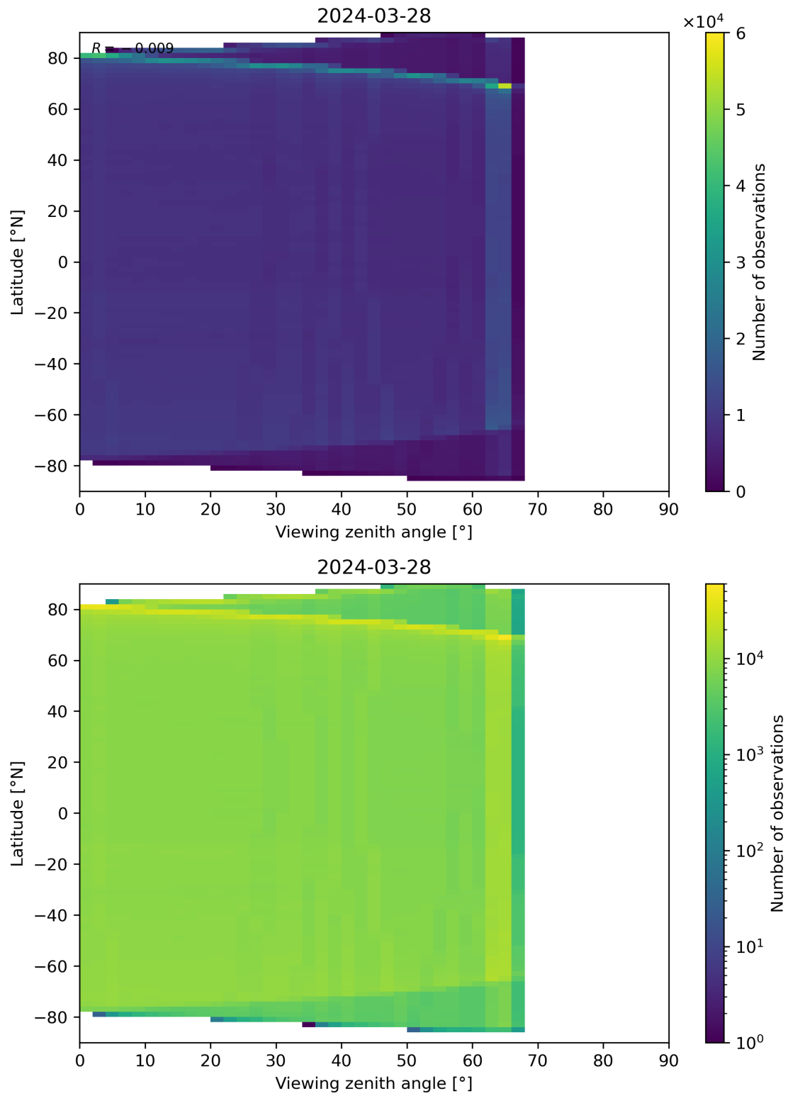
Figure 123: Scatter density plot of “Viewing zenith angle” against “Latitude” for 2024-03-27 to 2024-03-29.
