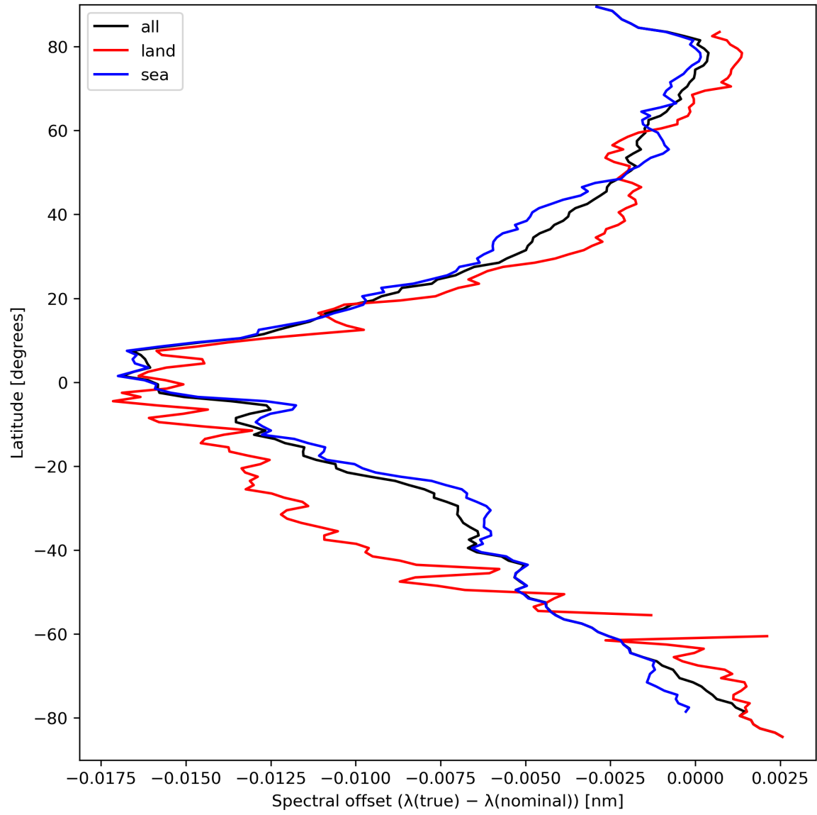
Figure 28: Zonal average of “Spectral offset ( \lambda(\text{true}) - \lambda(\text{nominal}) )” for 2024-03-27 to 2024-03-29.
