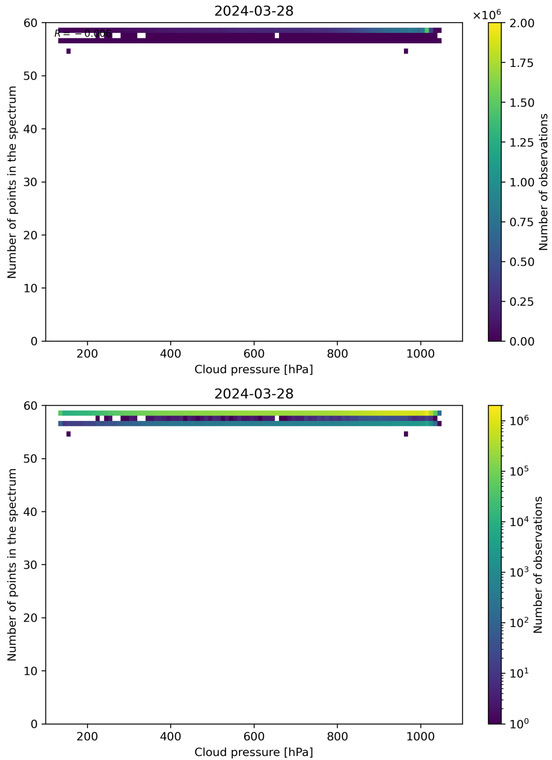
Figure 82: Scatter density plot of “Cloud pressure” against “Number of points in the spectrum” for 2024-03-27 to 2024-03-29.
