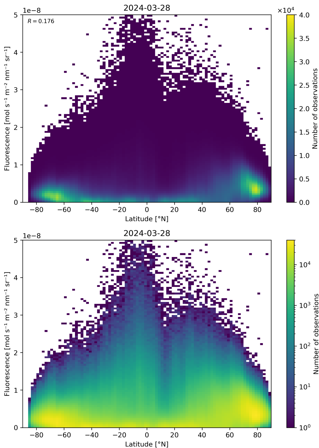
Figure 92: Scatter density plot of “Latitude” against “Fluorescence” for 2024-03-27 to 2024-03-29.
