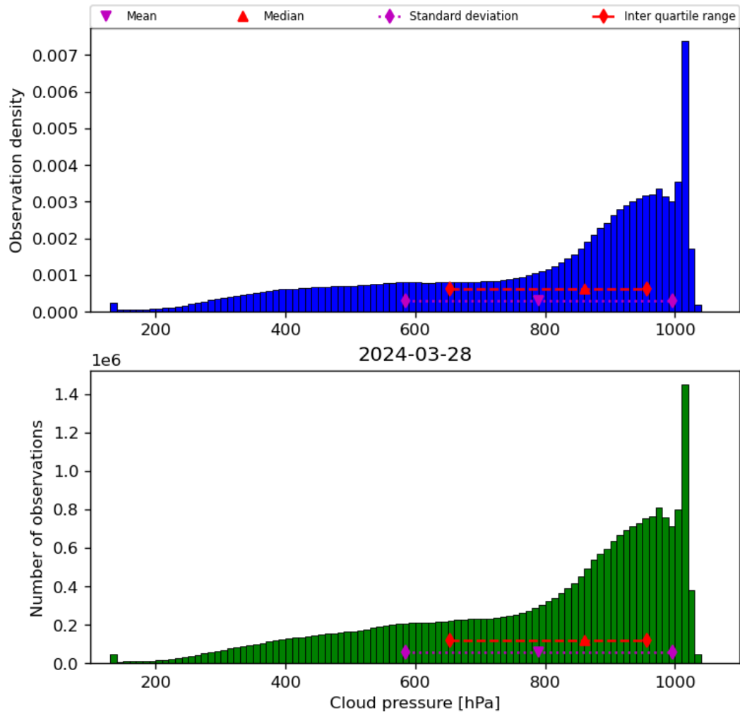
Figure 30: Histogram of “Cloud pressure” for 2024-03-27 to 2024-03-29
