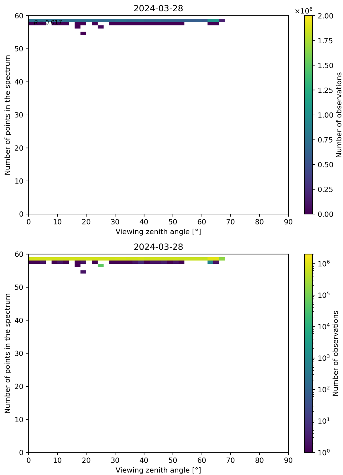
Figure 125: Scatter density plot of “Viewing zenith angle” against “Number of points in the spectrum” for 2024-03-27 to 2024-03-29.
