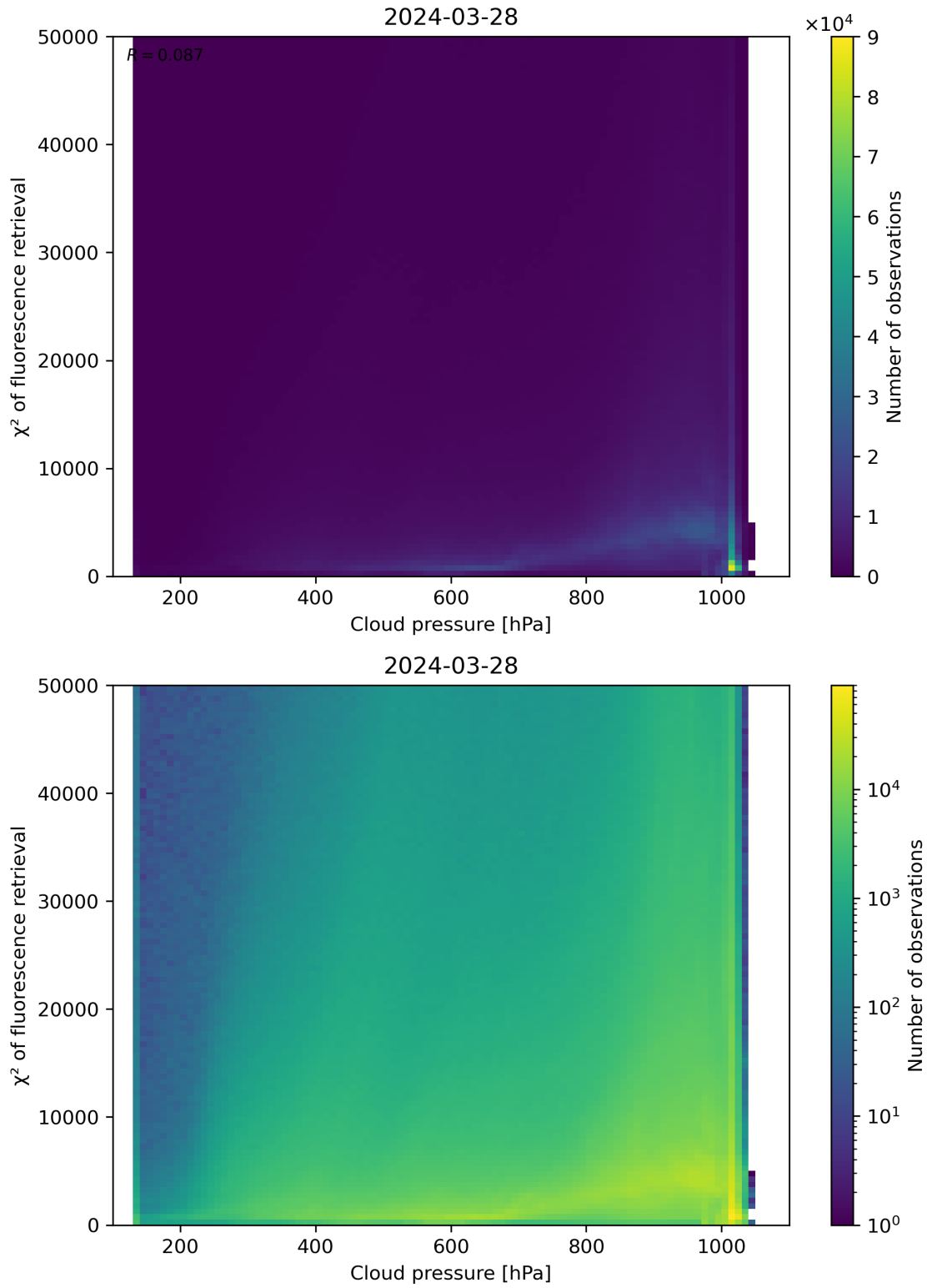
Figure 78: Scatter density plot of “Cloud pressure” against “ \chi^2 of fluorescence retrieval” for 2024-03-27 to 2024-03-29.
