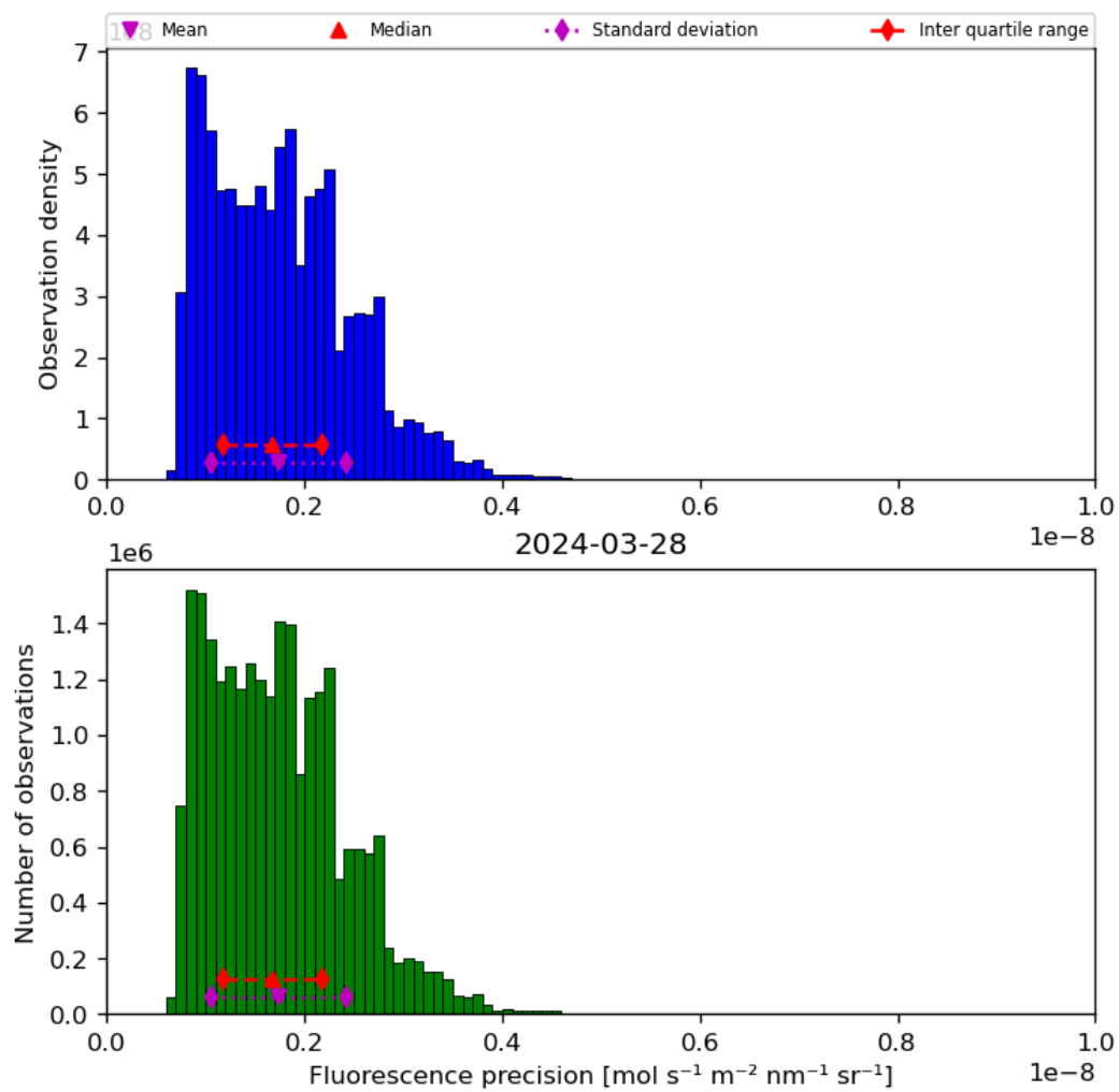
Figure 41: Histogram of “Fluorescence precision” for 2024-03-27 to 2024-03-29
