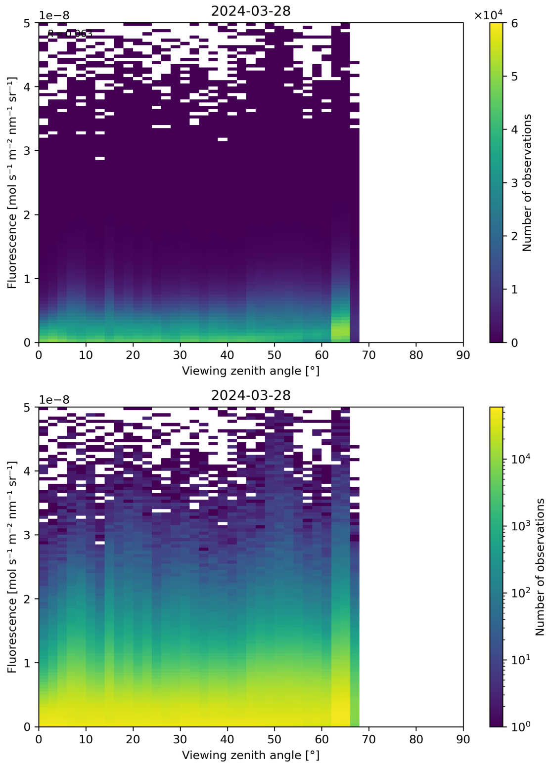
Figure 122: Scatter density plot of “Viewing zenith angle” against “Fluorescence” for 2024-03-27 to 2024-03-29.
