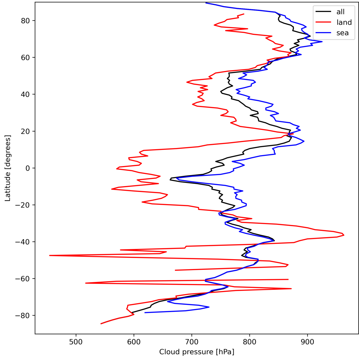
Figure 13: Zonal average of “Cloud pressure” for 2024-03-27 to 2024-03-29.
