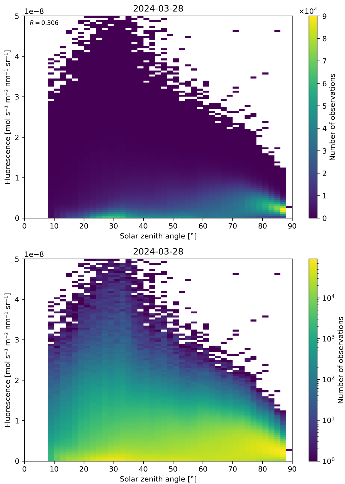
Figure 112: Scatter density plot of “Solar zenith angle” against “Fluorescence” for 2024-03-27 to 2024-03-29.
