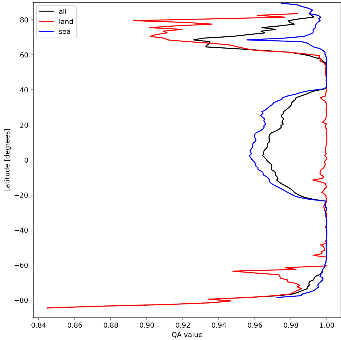
Figure 12: Zonal average of “QA value” for 2024-03-28 to 2024-03-30.
