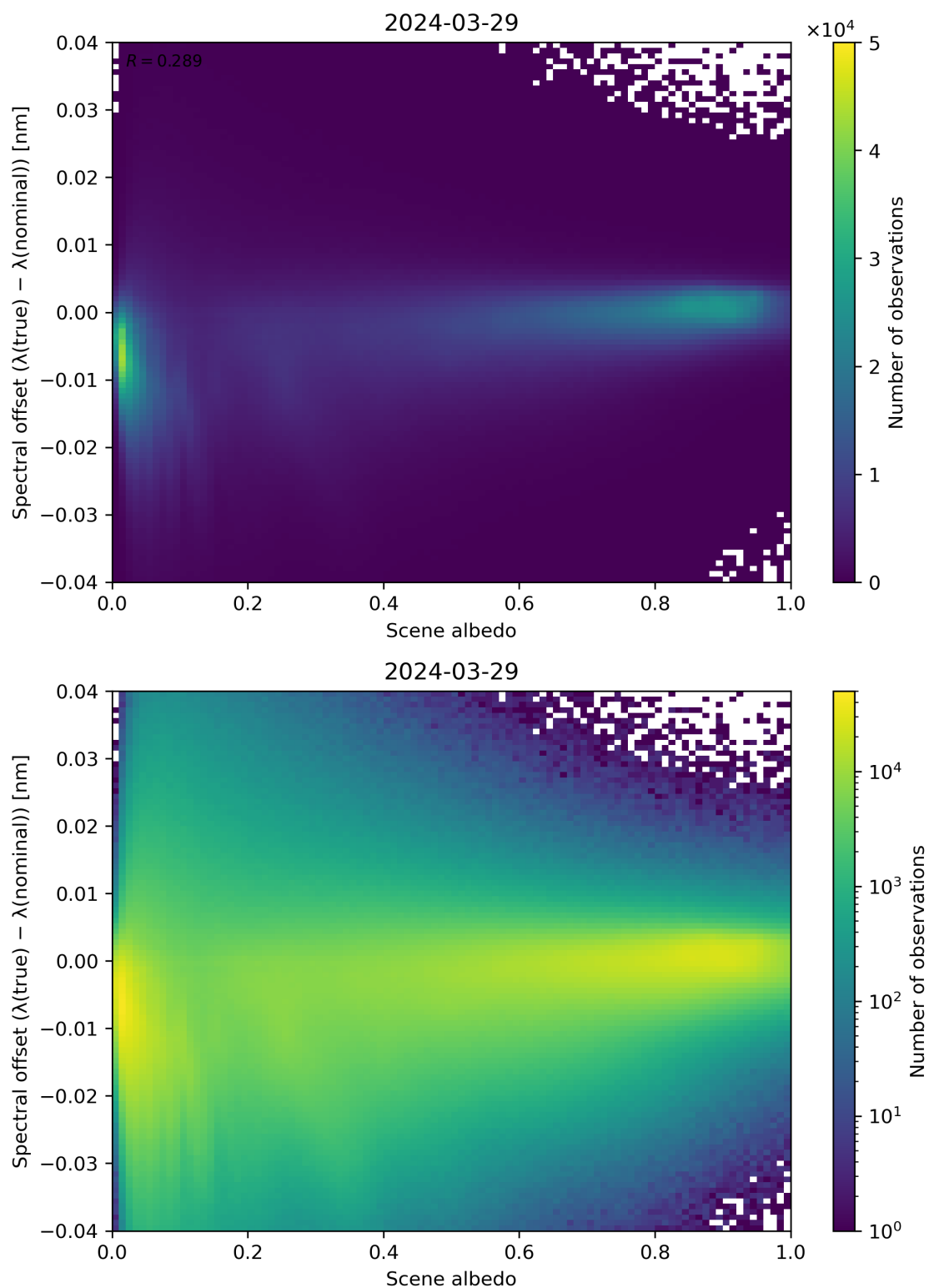
Figure 107: Scatter density plot of “Scene albedo” against “Spectral offset ( \lambda(\text{true}) - \lambda(\text{nominal}) )” for 2024-03-28 to 2024-03-30.
