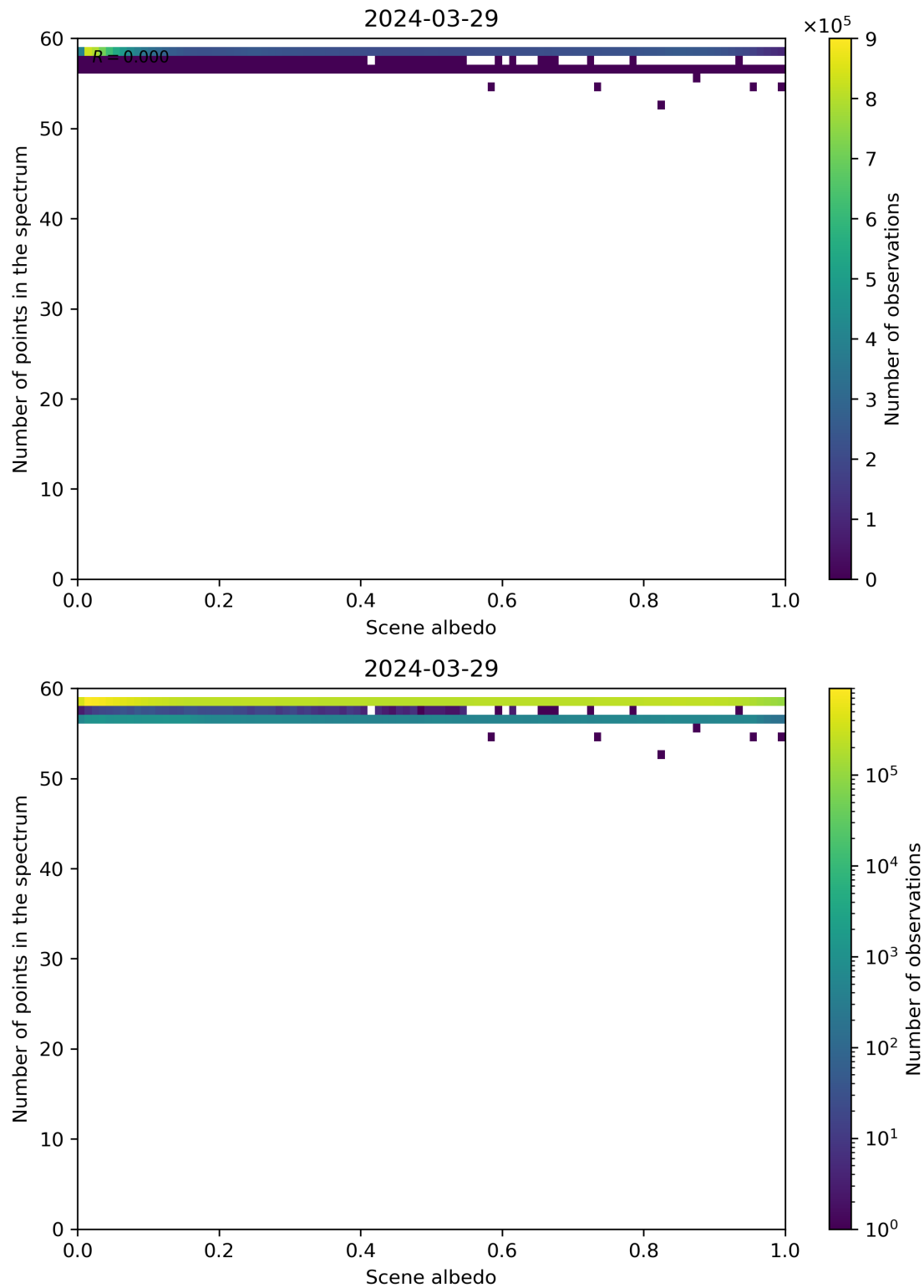
Figure 106: Scatter density plot of “Scene albedo” against “Number of points in the spectrum” for 2024-03-28 to 2024-03-30.
