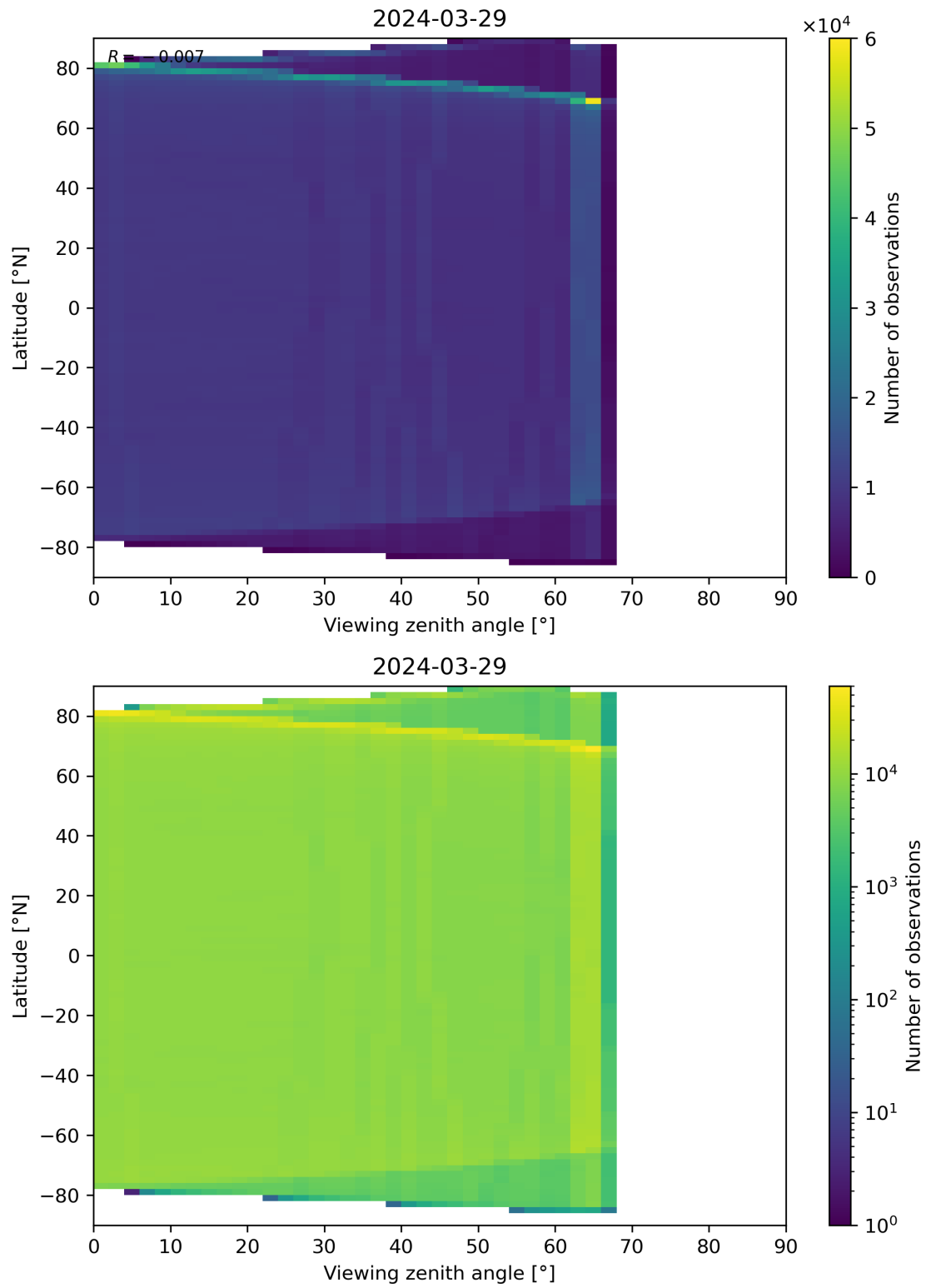
Figure 123: Scatter density plot of “Viewing zenith angle” against “Latitude” for 2024-03-28 to 2024-03-30.
