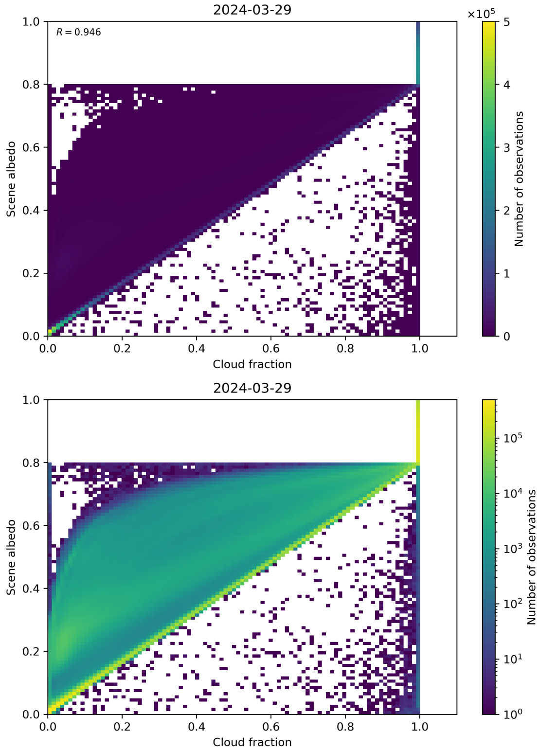
Figure 75: Scatter density plot of “Cloud fraction” against “Scene albedo” for 2024-03-28 to 2024-03-30.
