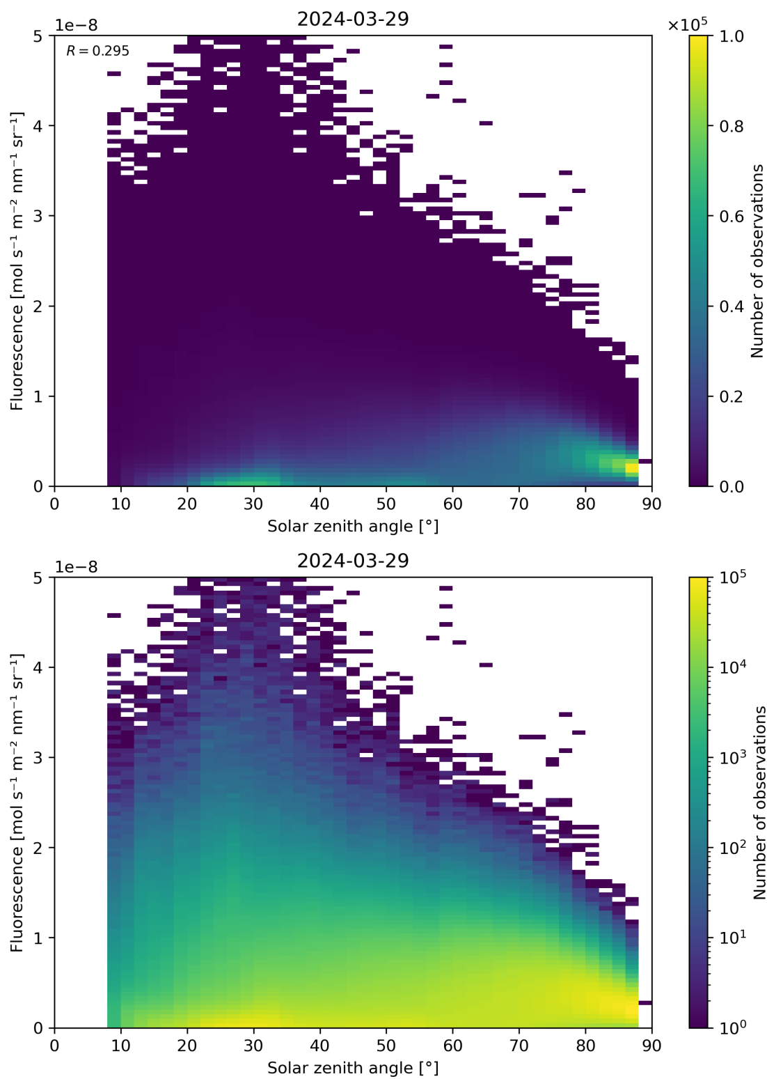
Figure 112: Scatter density plot of “Solar zenith angle” against “Fluorescence” for 2024-03-28 to 2024-03-30.
