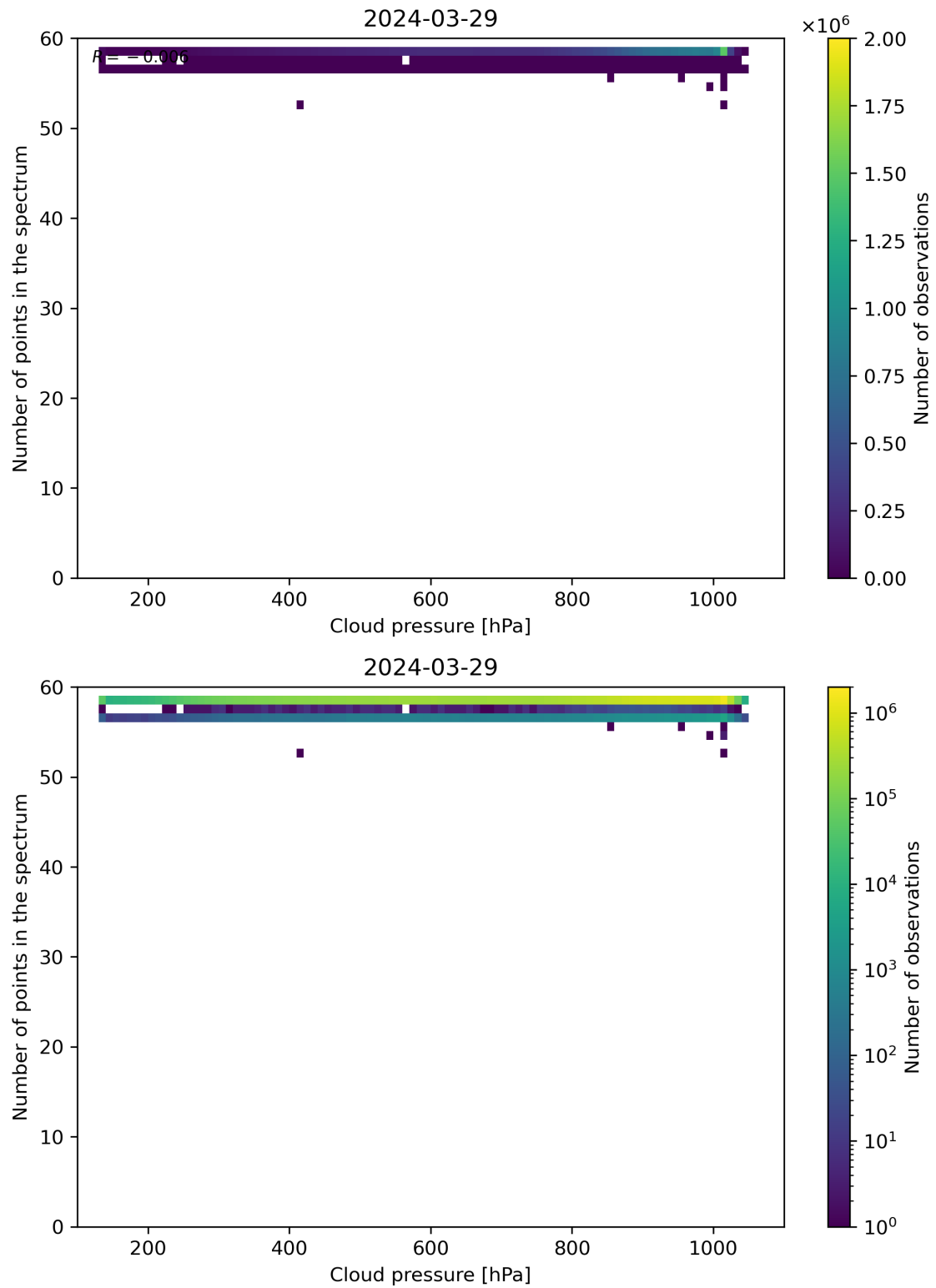
Figure 82: Scatter density plot of “Cloud pressure” against “Number of points in the spectrum” for 2024-03-28 to 2024-03-30.
