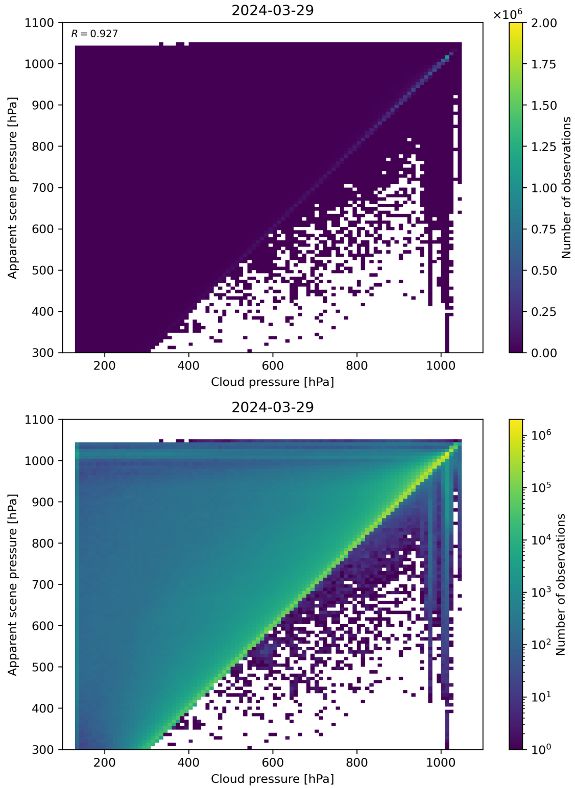
Figure 77: Scatter density plot of “Cloud pressure” against “Apparent scene pressure” for 2024-03-28 to 2024-03-30.
