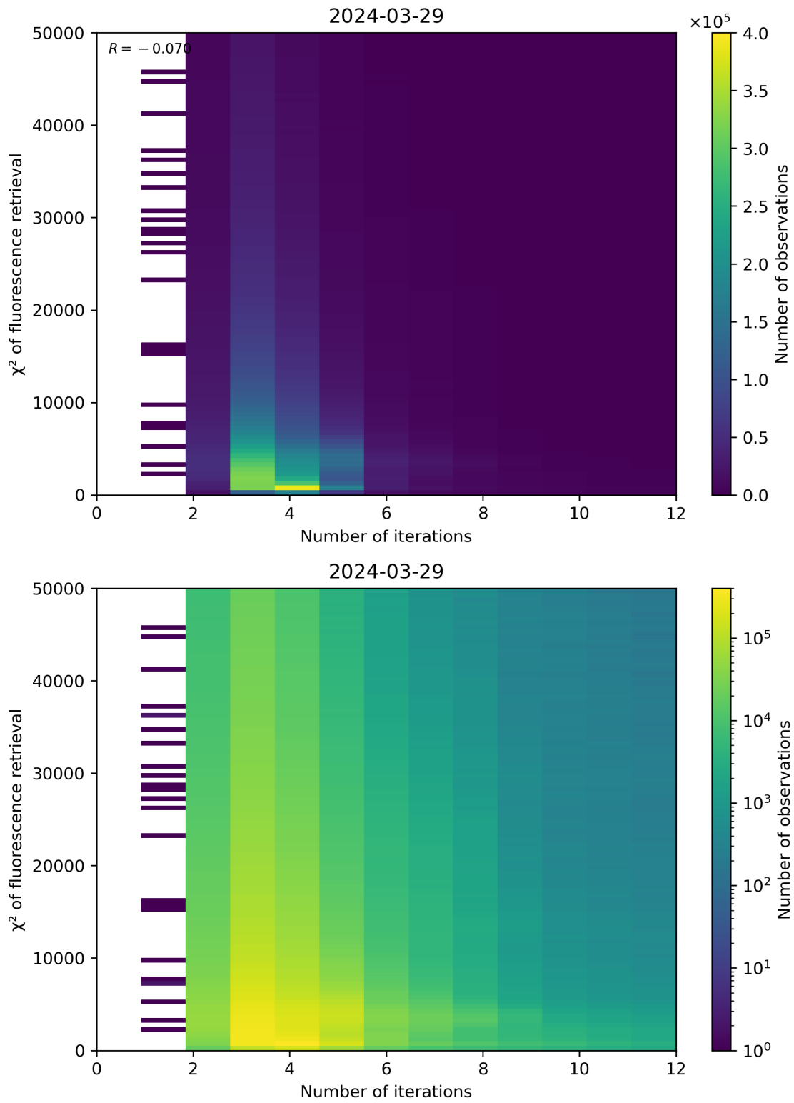
Figure 97: Scatter density plot of “Number of iterations” against “ \chi^2 of fluorescence retrieval” for 2024-03-28 to 2024-03-30.
