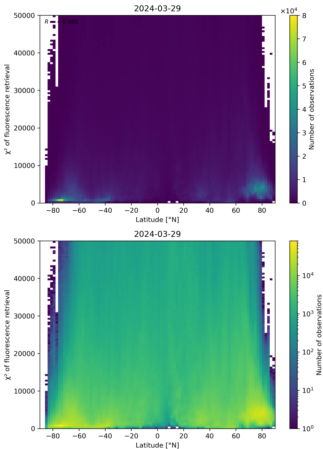
Figure 89: Scatter density plot of “Latitude” against “ \chi^2 of fluorescence retrieval” for 2024-03-28 to 2024-03-30.
