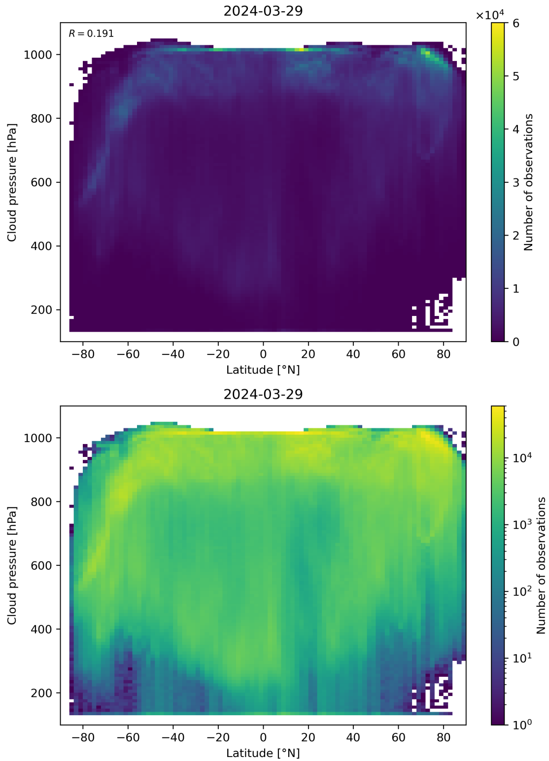
Figure 91: Scatter density plot of “Latitude” against “Cloud pressure” for 2024-03-28 to 2024-03-30.
