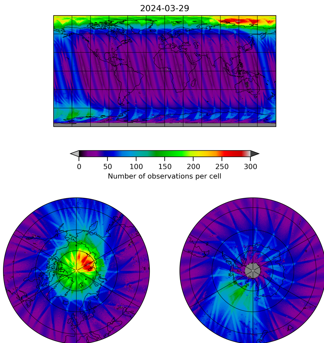
Figure 11: Map of the number of observations for 2024-03-28 to 2024-03-30
