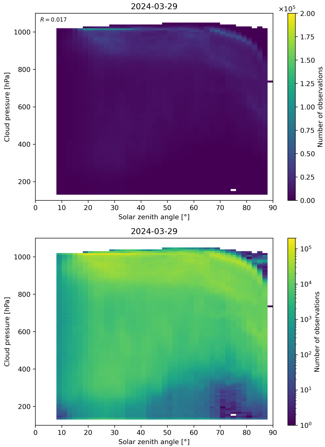
Figure 111: Scatter density plot of “Solar zenith angle” against “Cloud pressure” for 2024-03-28 to 2024-03-30.
