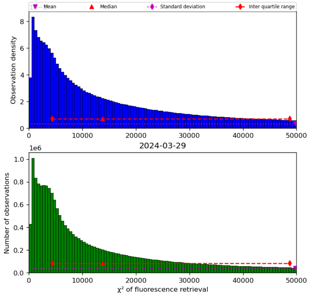
Figure 42: Histogram of “ \chi^2 of fluorescence retrieval” for 2024-03-28 to 2024-03-30
