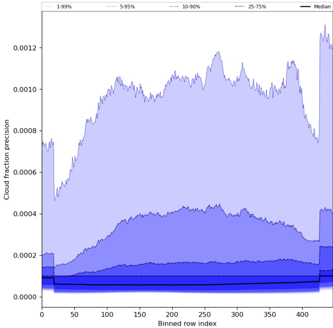
Figure 50: Along track statistics of “Cloud fraction precision” for 2024-03-28 to 2024-03-30
