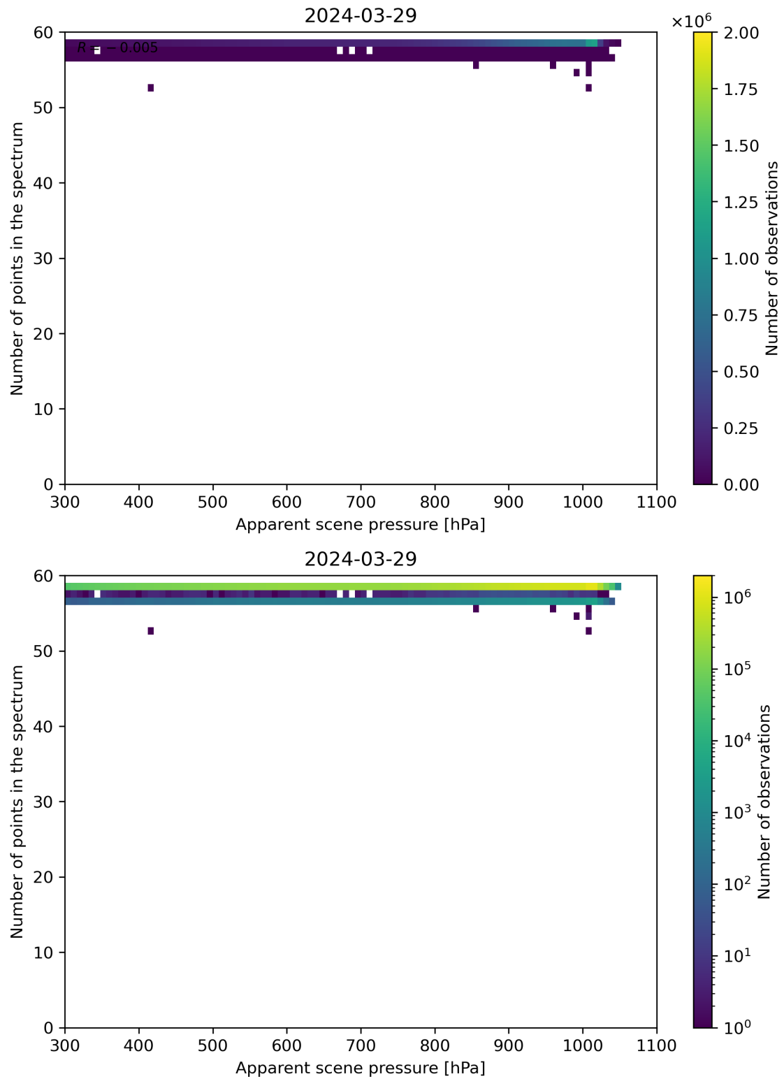
Figure 66: Scatter density plot of “Apparent scene pressure” against “Number of points in the spectrum” for 2024-03-28 to 2024-03-30.
