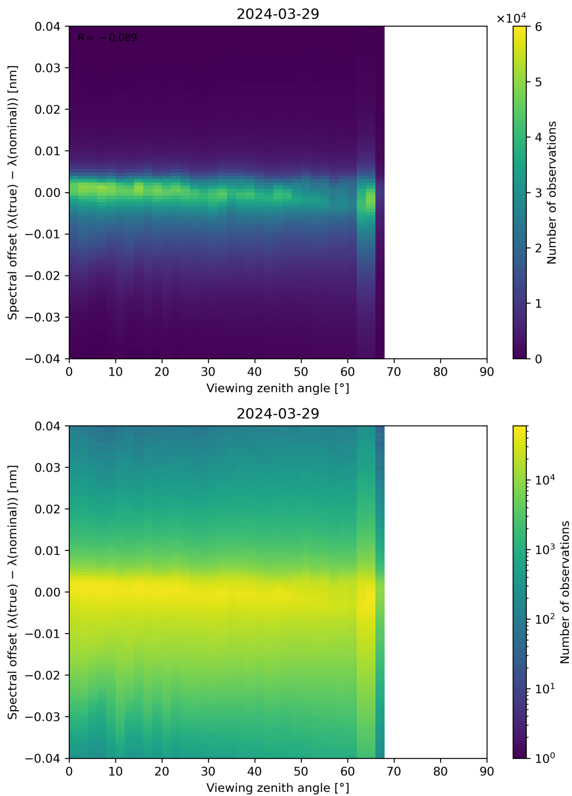
Figure 128: Scatter density plot of “Viewing zenith angle” against “Spectral offset ( \lambda(\text{true}) - \lambda(\text{nominal}) )” for 2024-03-28 to 2024-03-30.
