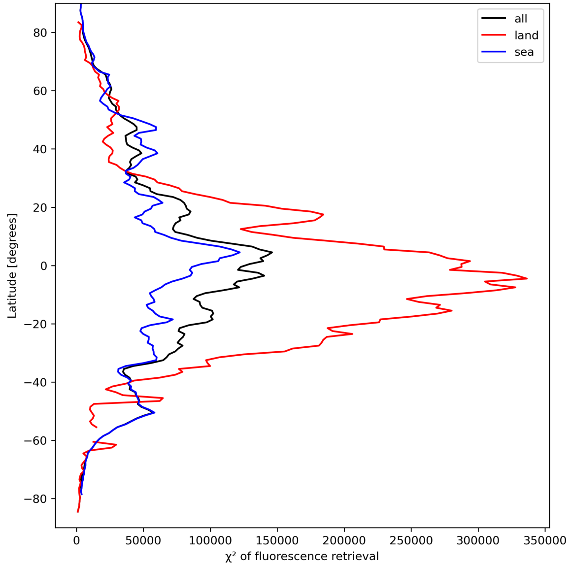
Figure 25: Zonal average of “ \chi^2 of fluorescence retrieval” for 2024-03-28 to 2024-03-30.
