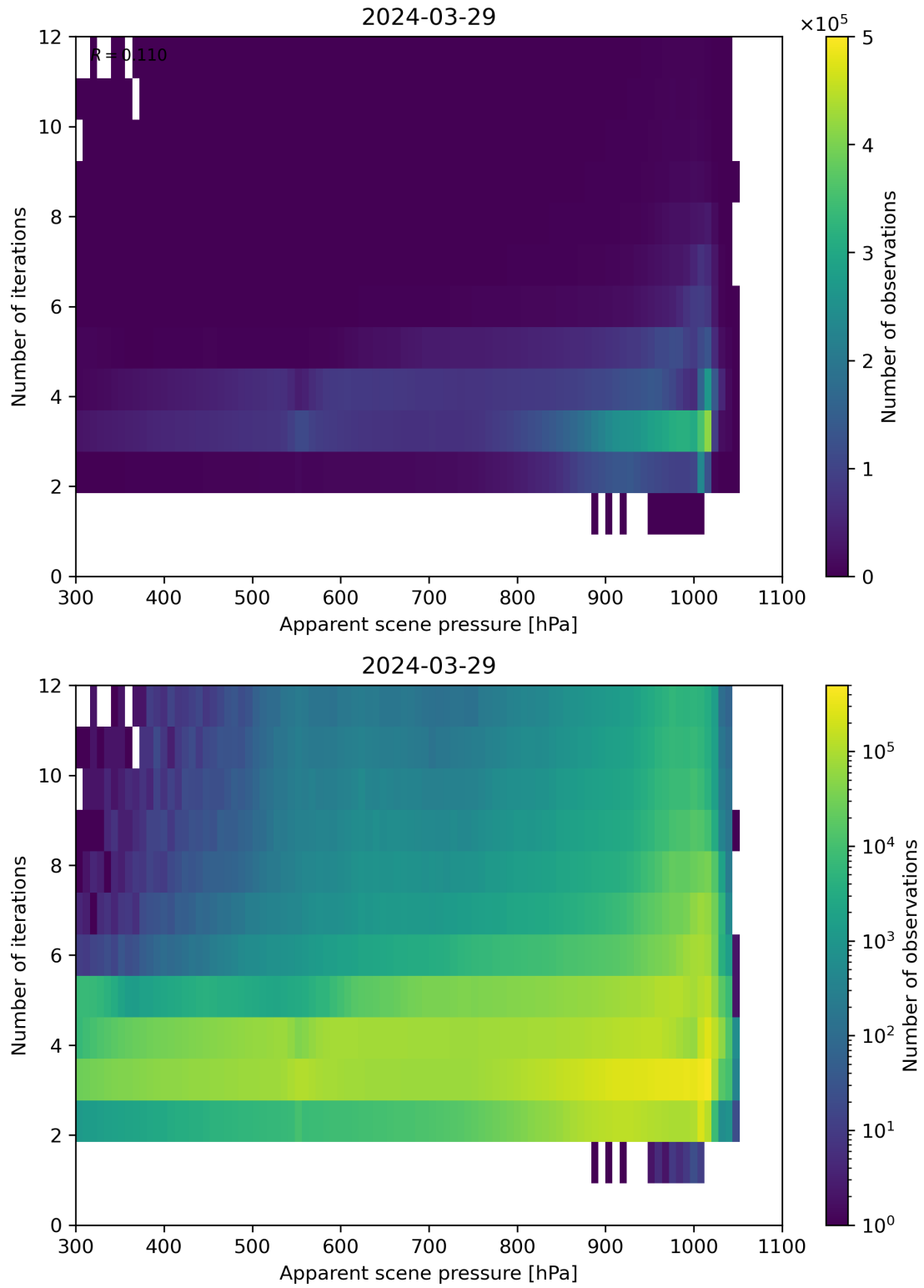
Figure 65: Scatter density plot of “Apparent scene pressure” against “Number of iterations” for 2024-03-28 to 2024-03-30.
