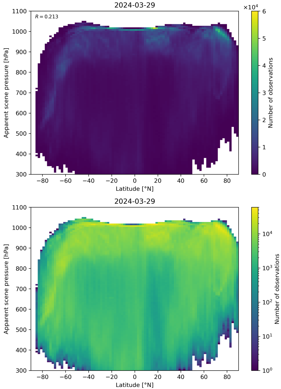
Figure 88: Scatter density plot of “Latitude” against “Apparent scene pressure” for 2024-03-28 to 2024-03-30.
