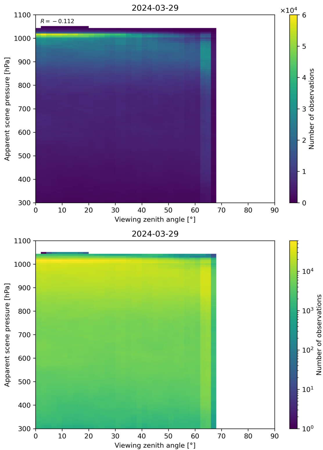
Figure 118: Scatter density plot of “Viewing zenith angle” against “Apparent scene pressure” for 2024-03-28 to 2024-03-30.
