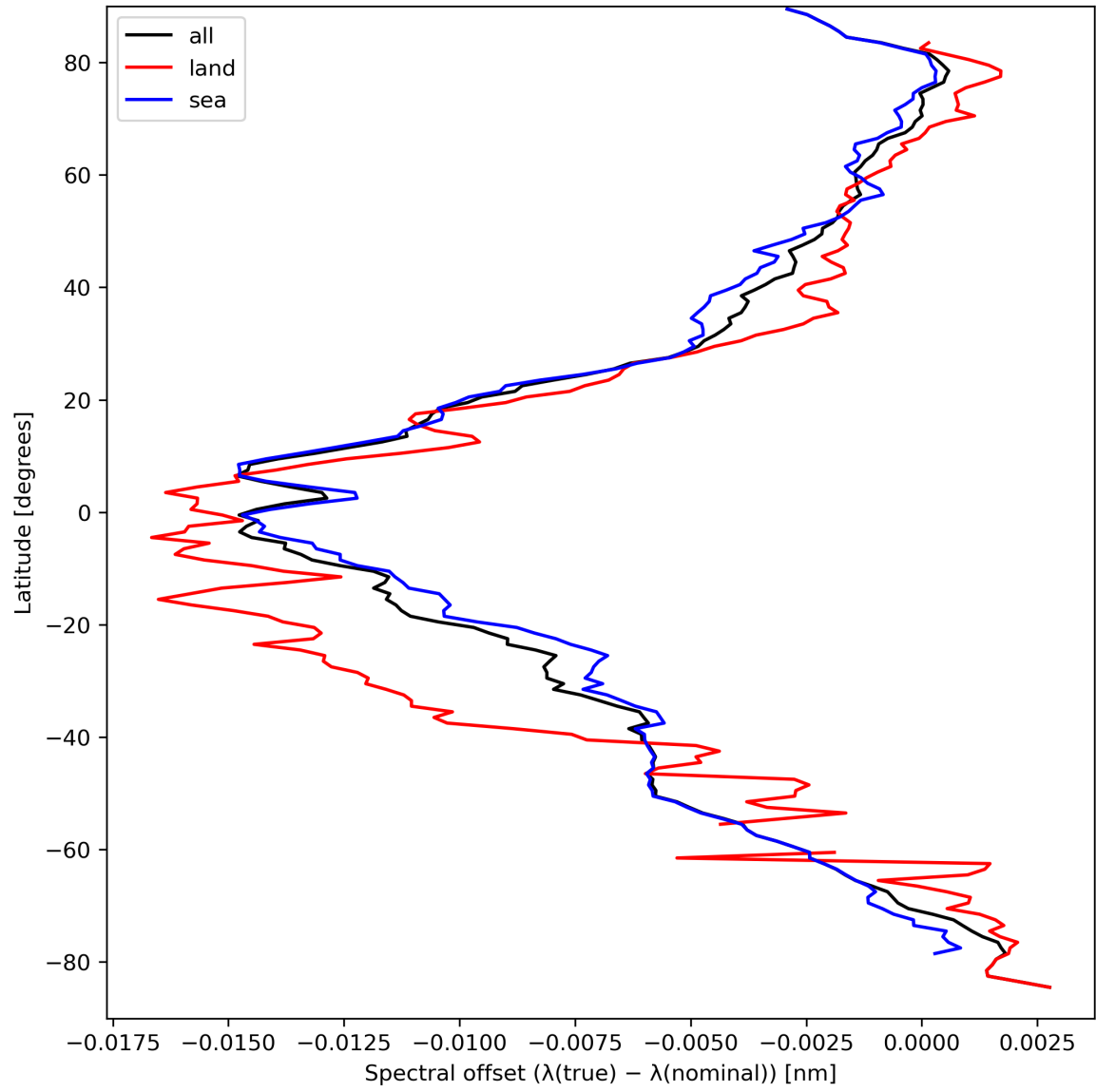
Figure 28: Zonal average of “Spectral offset ( \lambda(\text{true}) - \lambda(\text{nominal}) )” for 2024-03-28 to 2024-03-30.
