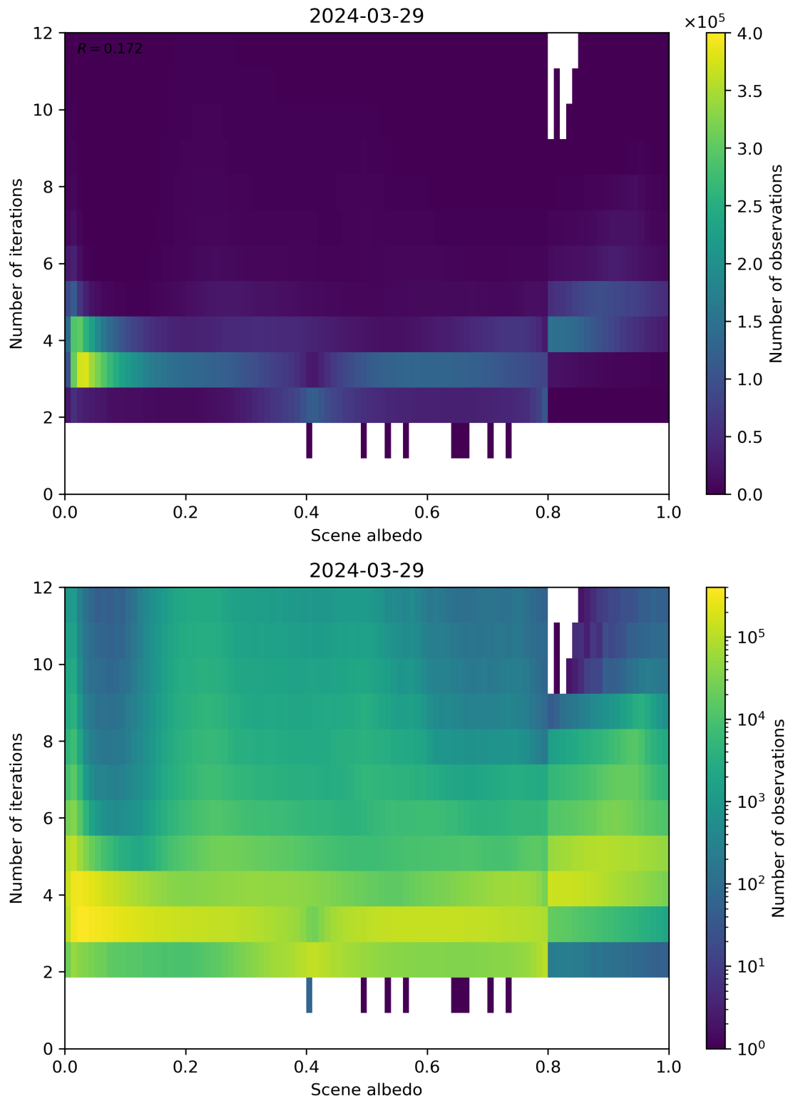
Figure 105: Scatter density plot of “Scene albedo” against “Number of iterations” for 2024-03-28 to 2024-03-30.
