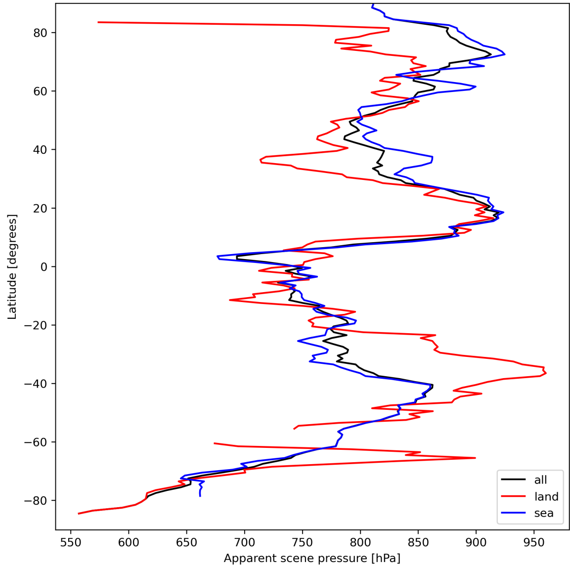
Figure 19: Zonal average of “Apparent scene pressure” for 2024-03-28 to 2024-03-30.
