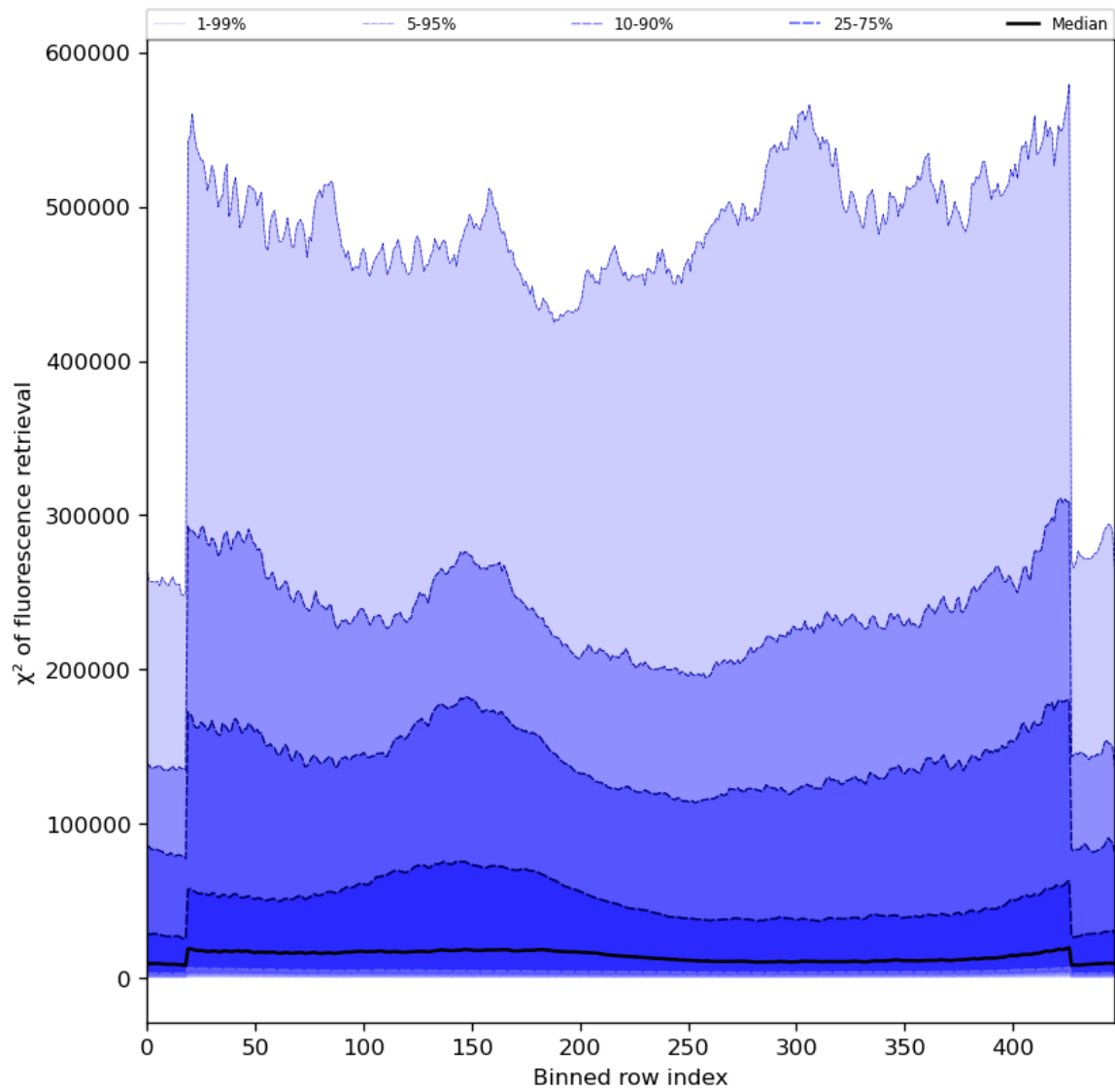
Figure 59: Along track statistics of “ \chi^2 of fluorescence retrieval” for 2024-03-28 to 2024-03-30
