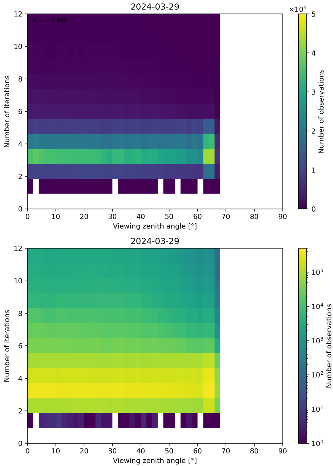
Figure 124: Scatter density plot of “Viewing zenith angle” against “Number of iterations” for 2024-03-28 to 2024-03-30.
