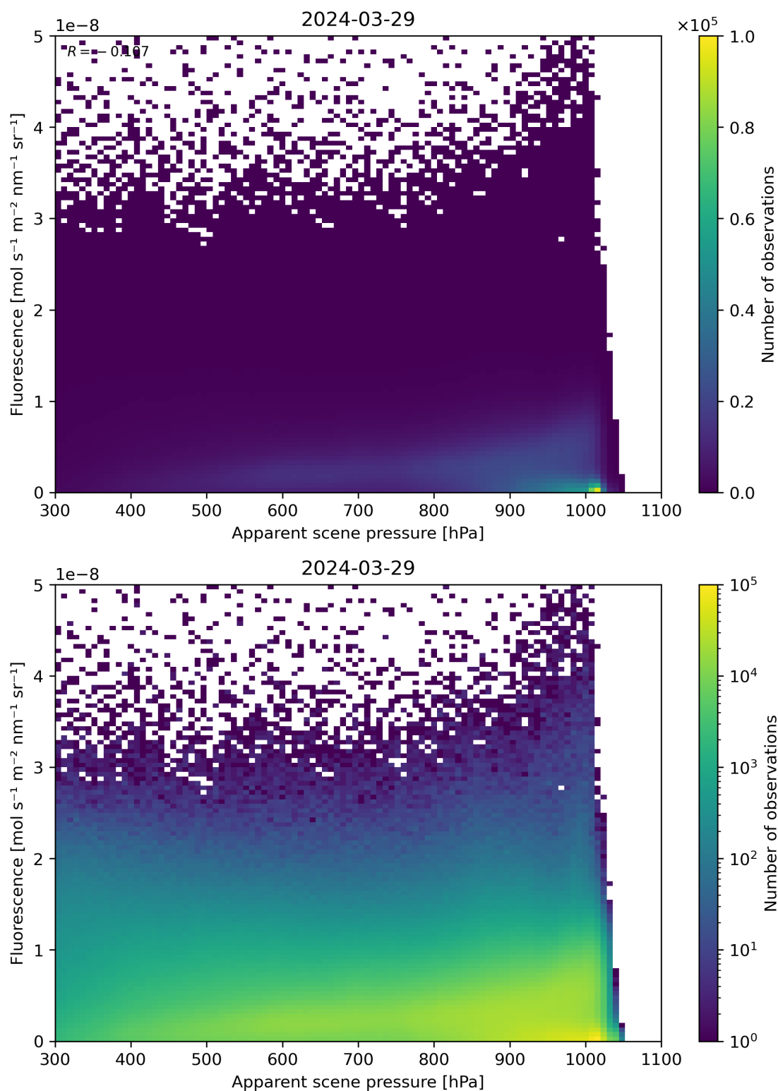
Figure 64: Scatter density plot of “Apparent scene pressure” against “Fluorescence” for 2024-03-28 to 2024-03-30.
