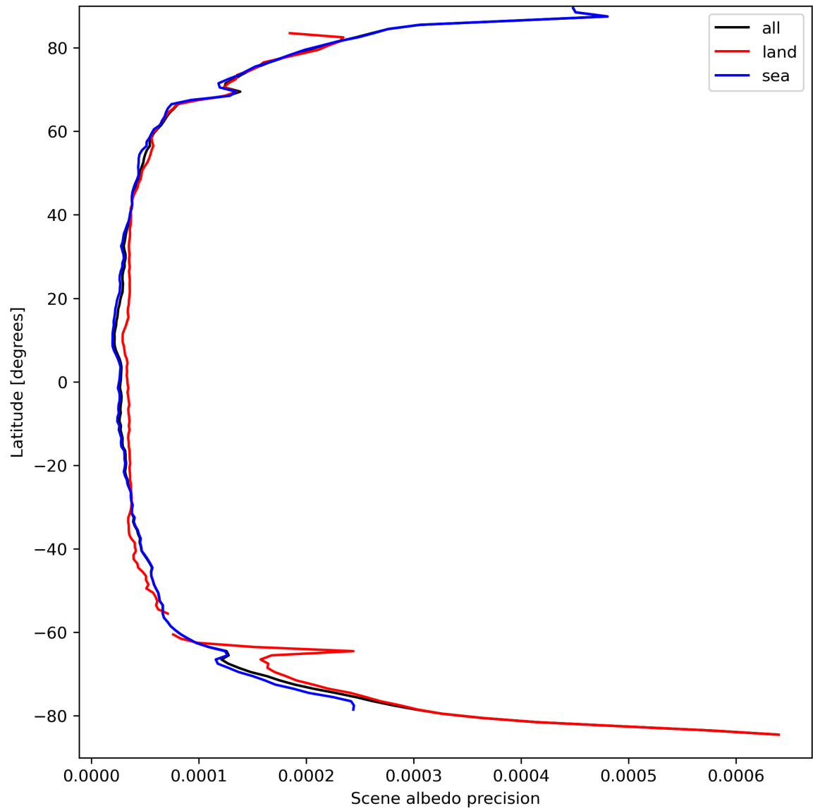
Figure 18: Zonal average of “Scene albedo precision” for 2024-03-28 to 2024-03-30.
