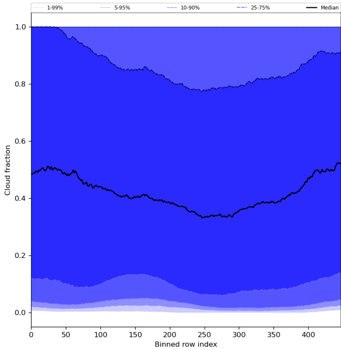
Figure 49: Along track statistics of “Cloud fraction” for 2024-03-28 to 2024-03-30
