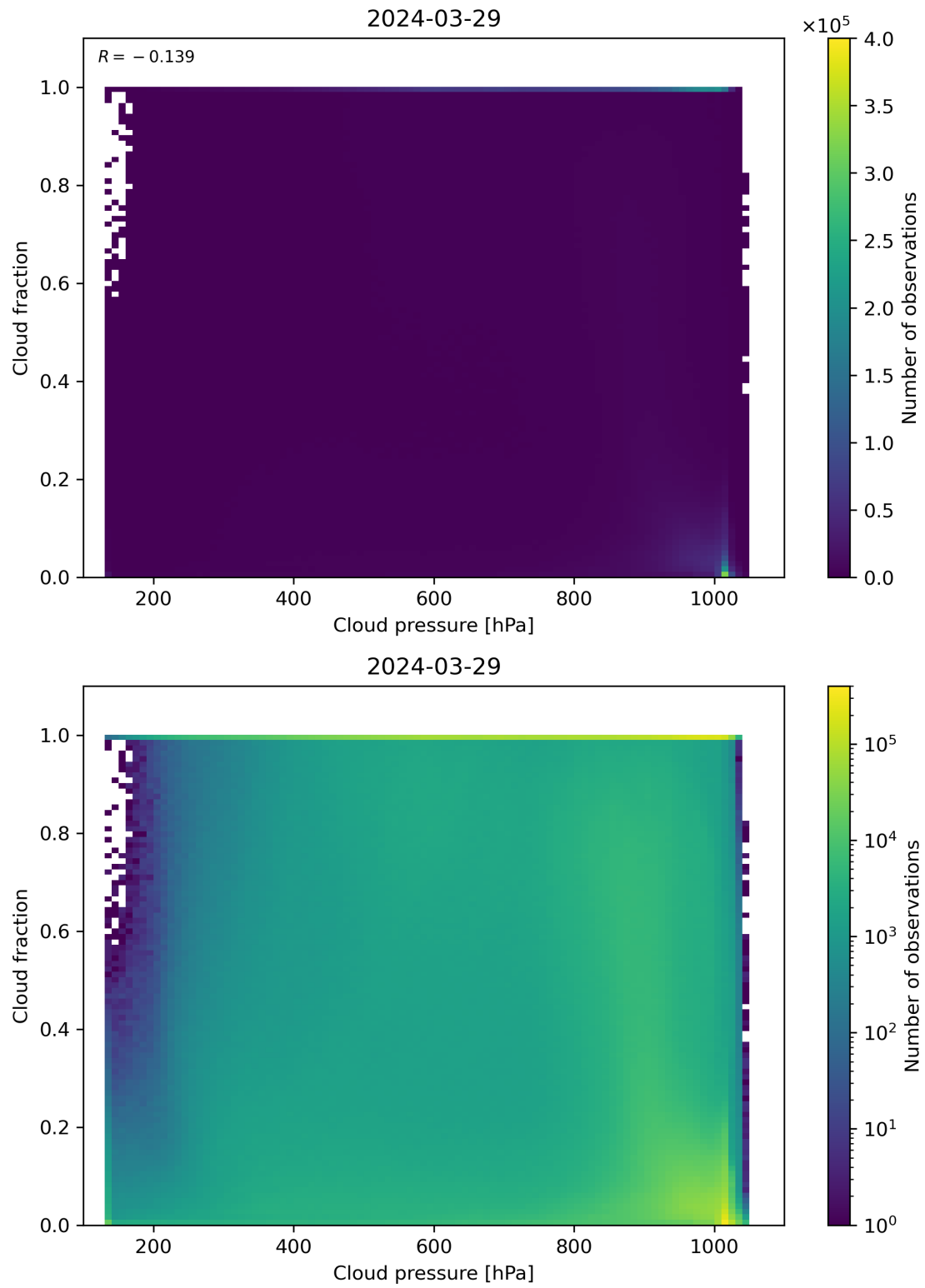
Figure 79: Scatter density plot of “Cloud pressure” against “Cloud fraction” for 2024-03-28 to 2024-03-30.
