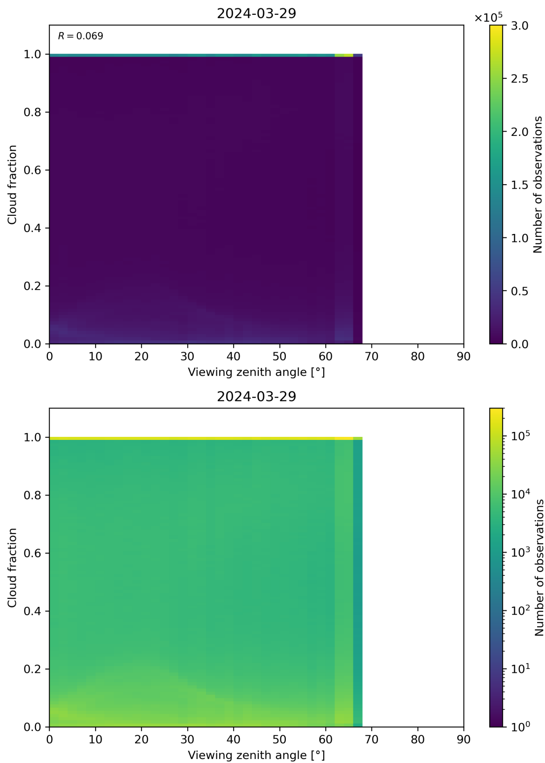
Figure 120: Scatter density plot of “Viewing zenith angle” against “Cloud fraction” for 2024-03-28 to 2024-03-30.
