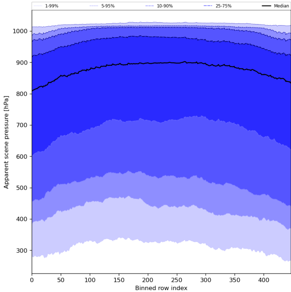
Figure 53: Along track statistics of “Apparent scene pressure” for 2024-03-28 to 2024-03-30
