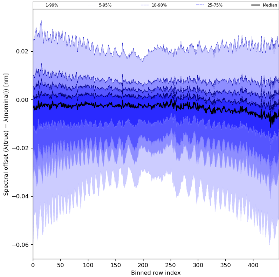
Figure 62: Along track statistics of “Spectral offset ( \lambda(\text{true}) - \lambda(\text{nominal}) )” for 2024-03-28 to 2024-03-30
