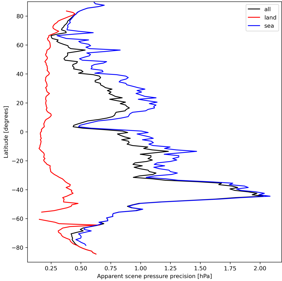
Figure 20: Zonal average of “Apparent scene pressure precision” for 2024-03-28 to 2024-03-30.
