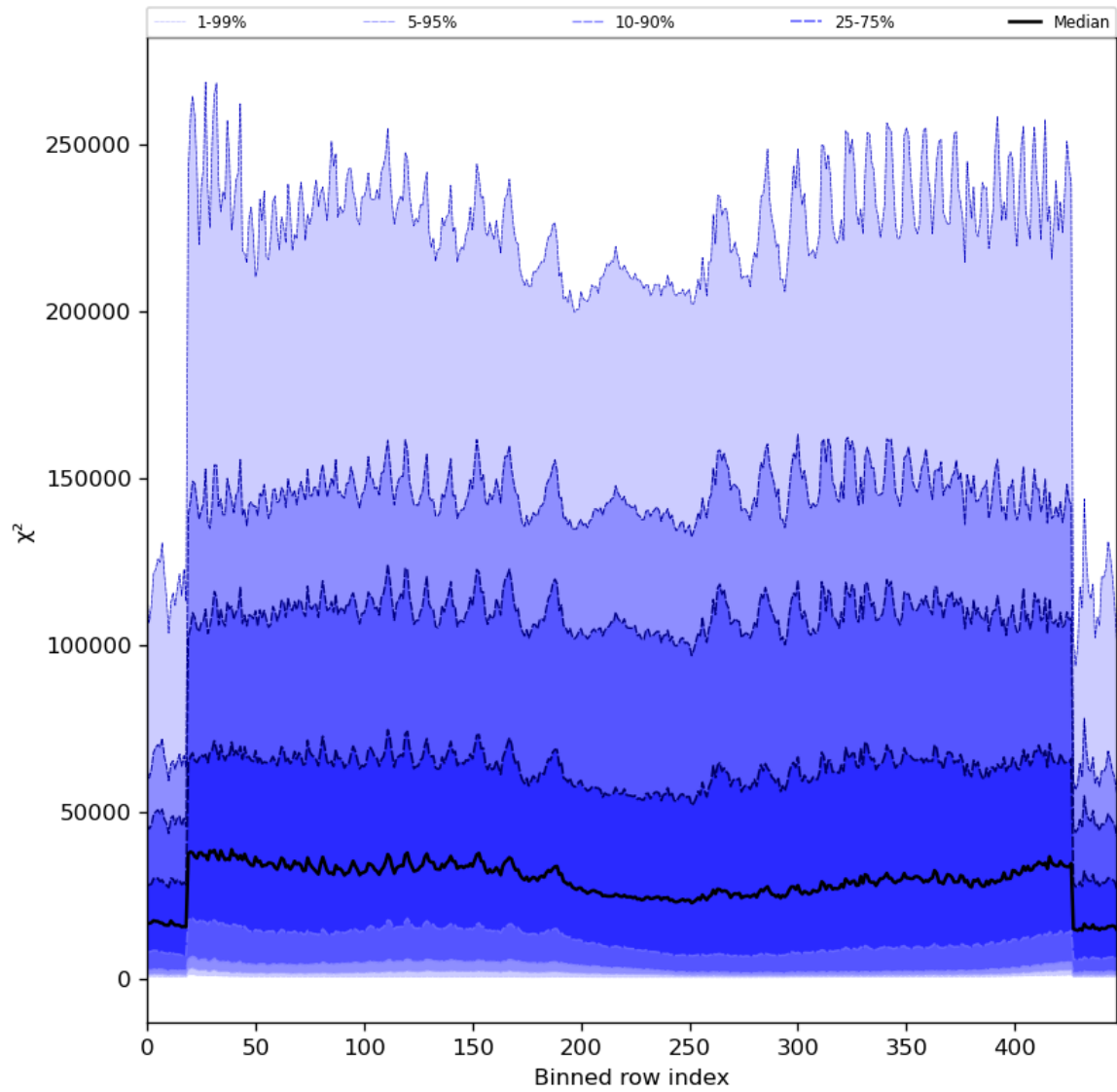
Figure 55: Along track statistics of “ \chi^2 ” for 2024-03-28 to 2024-03-30
