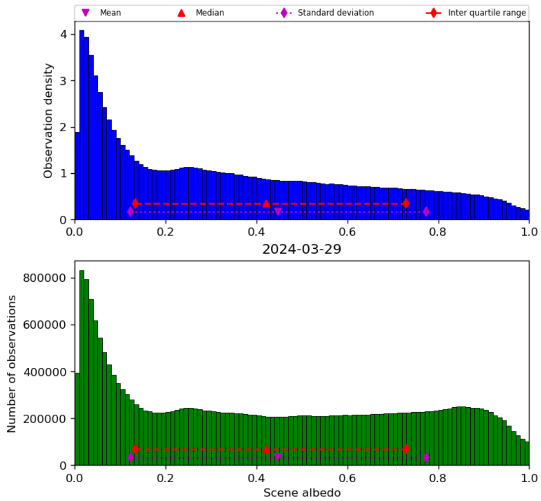
Figure 34: Histogram of “Scene albedo” for 2024-03-28 to 2024-03-30
