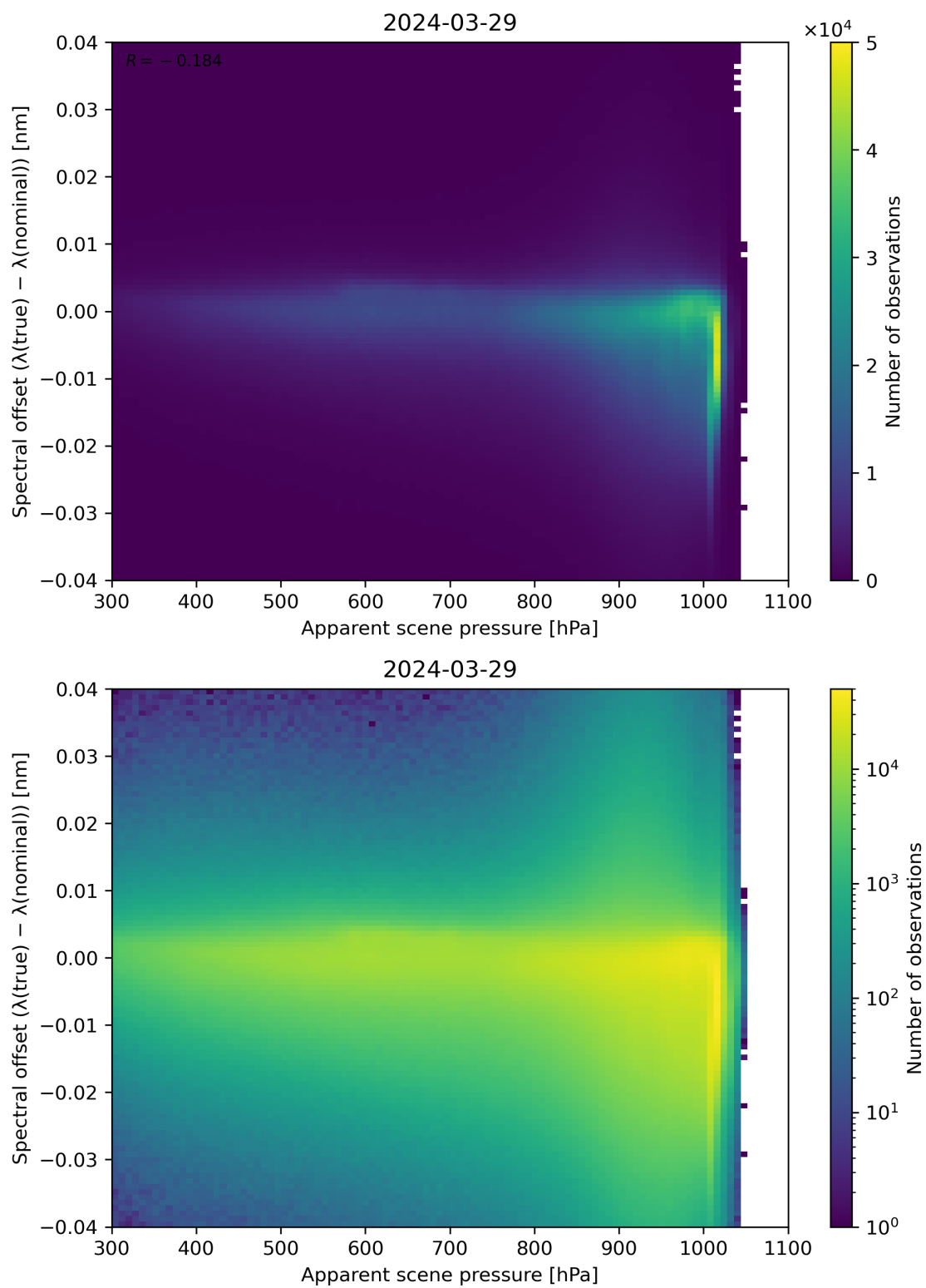
Figure 67: Scatter density plot of “Apparent scene pressure” against “Spectral offset ( \lambda(\text{true}) - \lambda(\text{nominal}) )” for 2024-03-28 to 2024-03-30.
