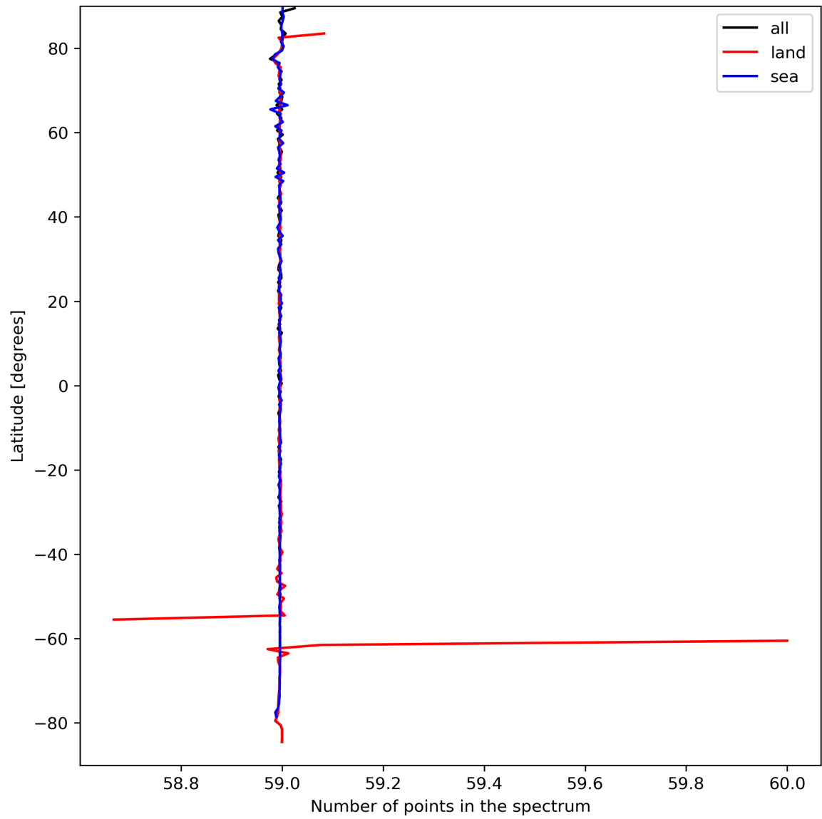
Figure 27: Zonal average of “Number of points in the spectrum” for 2024-03-28 to 2024-03-30.
