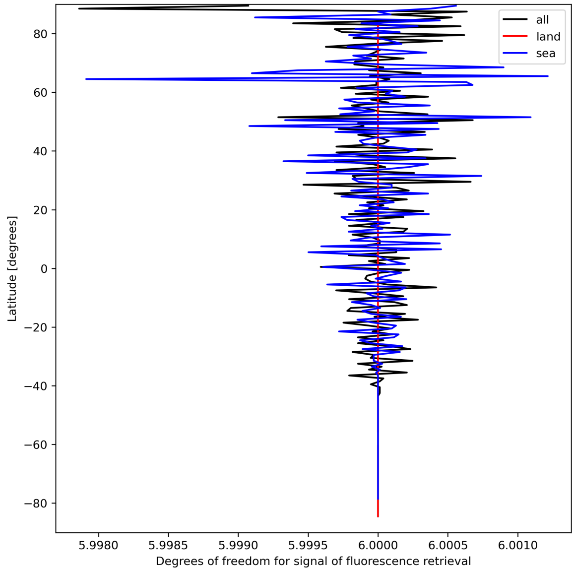
Figure 26: Zonal average of “Degrees of freedom for signal of fluorescence retrieval” for 2024-03-28 to 2024-03-30.
