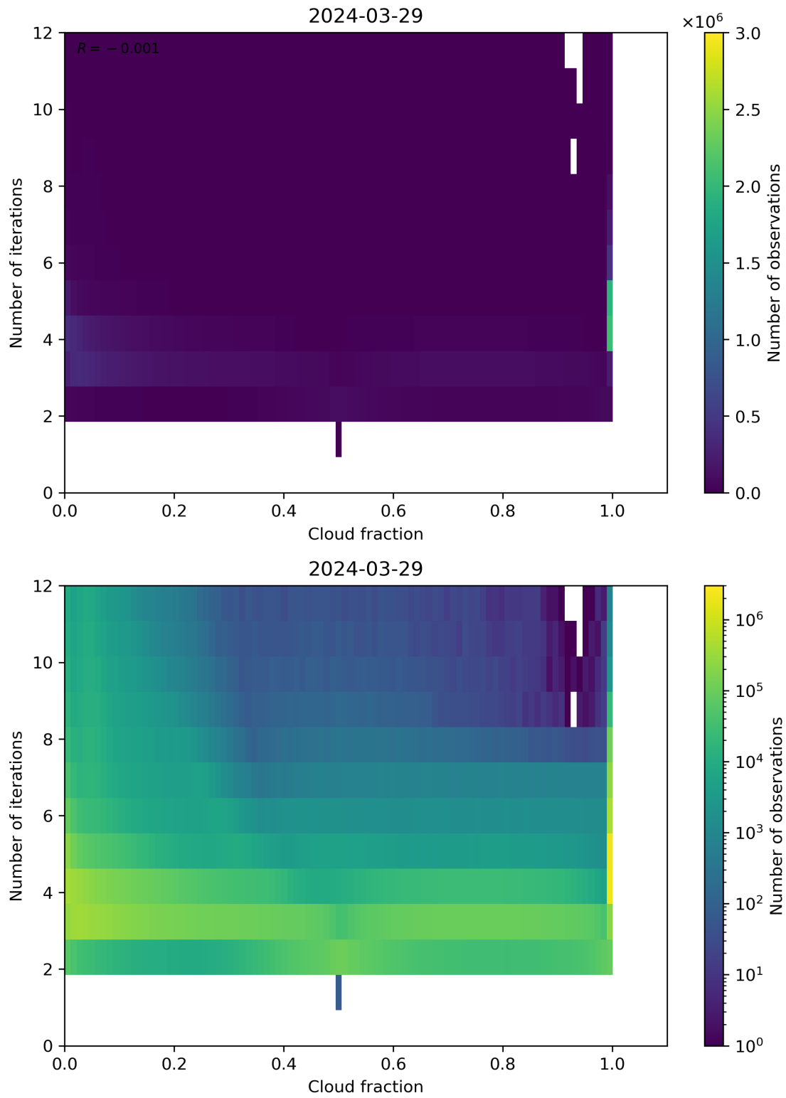
Figure 73: Scatter density plot of “Cloud fraction” against “Number of iterations” for 2024-03-28 to 2024-03-30.
