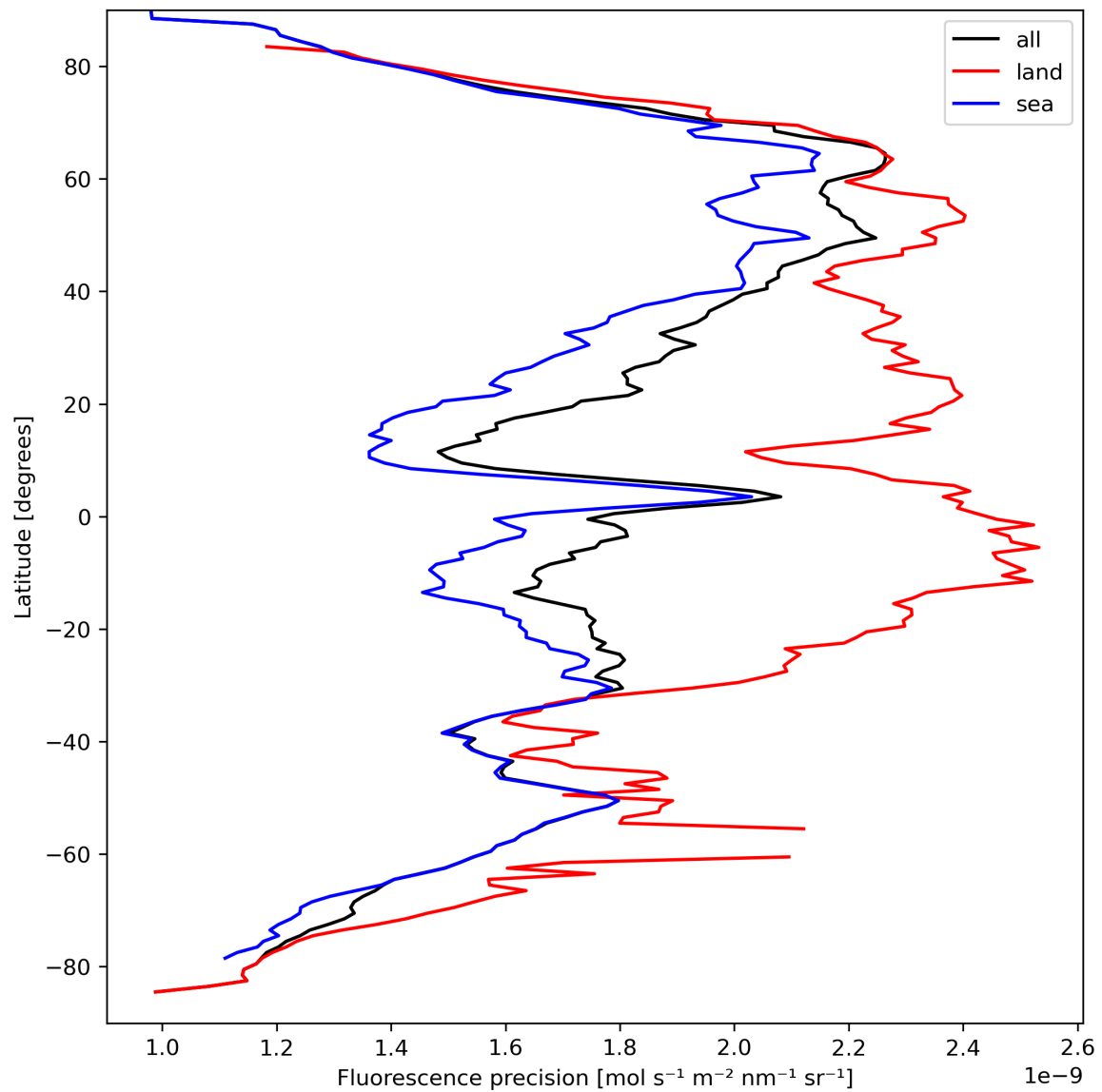
Figure 24: Zonal average of “Fluorescence precision” for 2024-03-28 to 2024-03-30.
