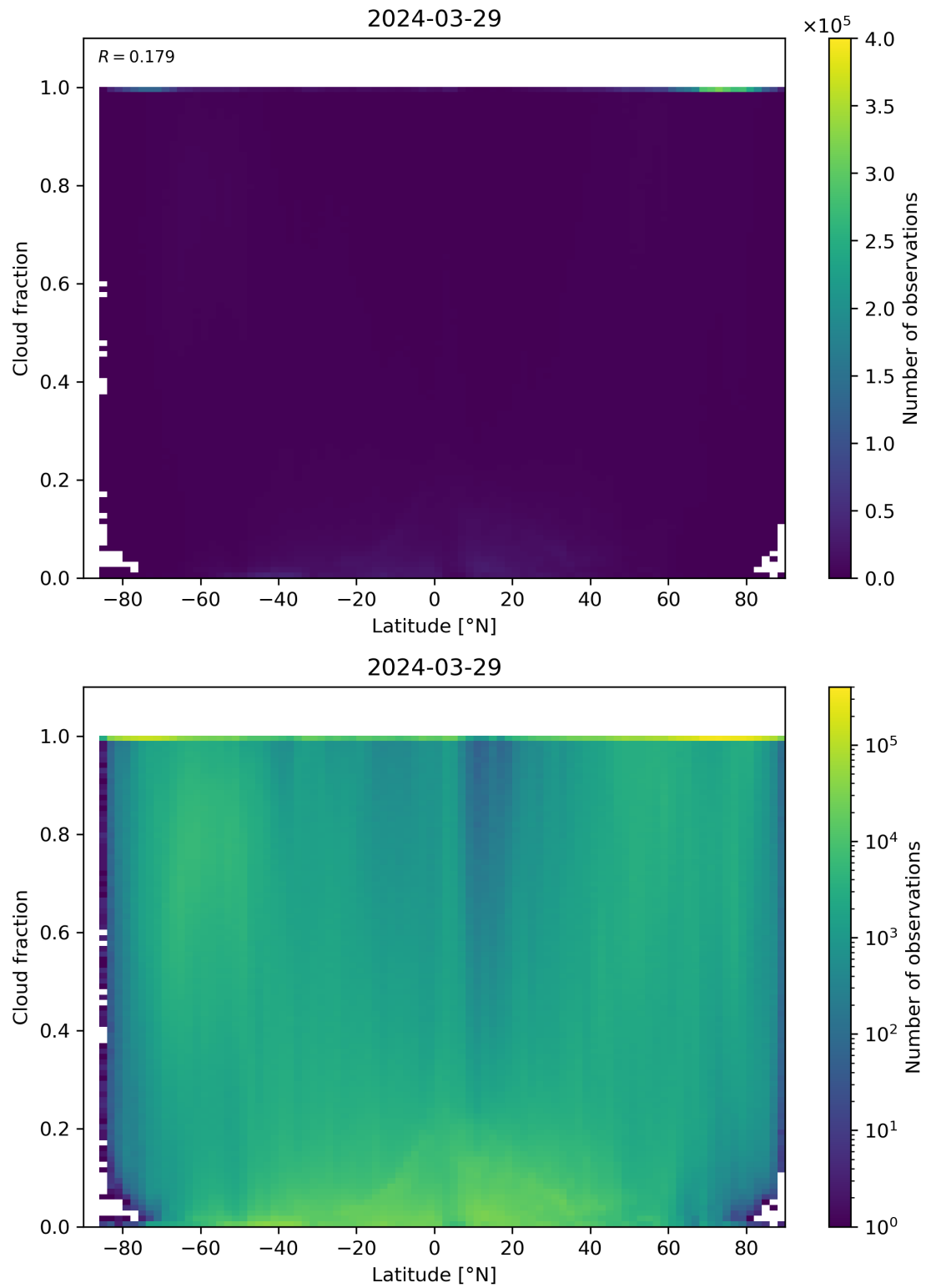
Figure 90: Scatter density plot of “Latitude” against “Cloud fraction” for 2024-03-28 to 2024-03-30.
