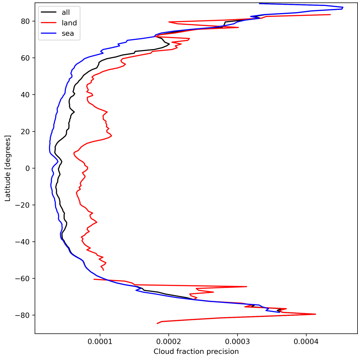
Figure 16: Zonal average of “Cloud fraction precision” for 2024-03-28 to 2024-03-30.
