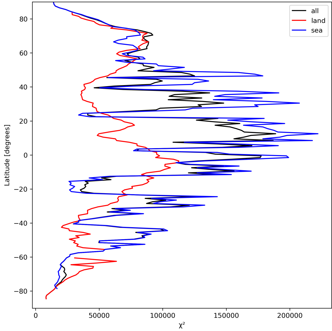
Figure 21: Zonal average of “ \chi^2 ” for 2024-03-28 to 2024-03-30.
