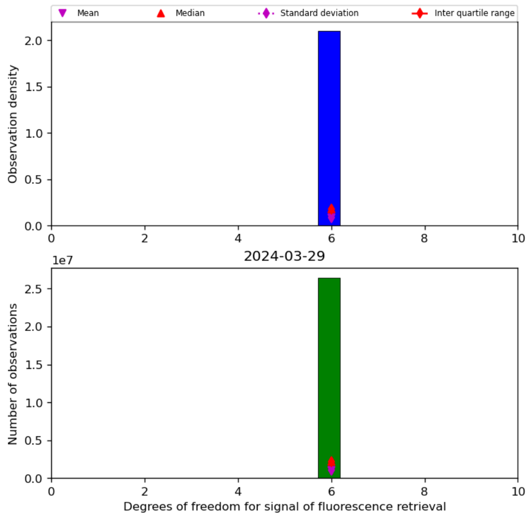
Figure 43: Histogram of “Degrees of freedom for signal of fluorescence retrieval” for 2024-03-28 to 2024-03-30
