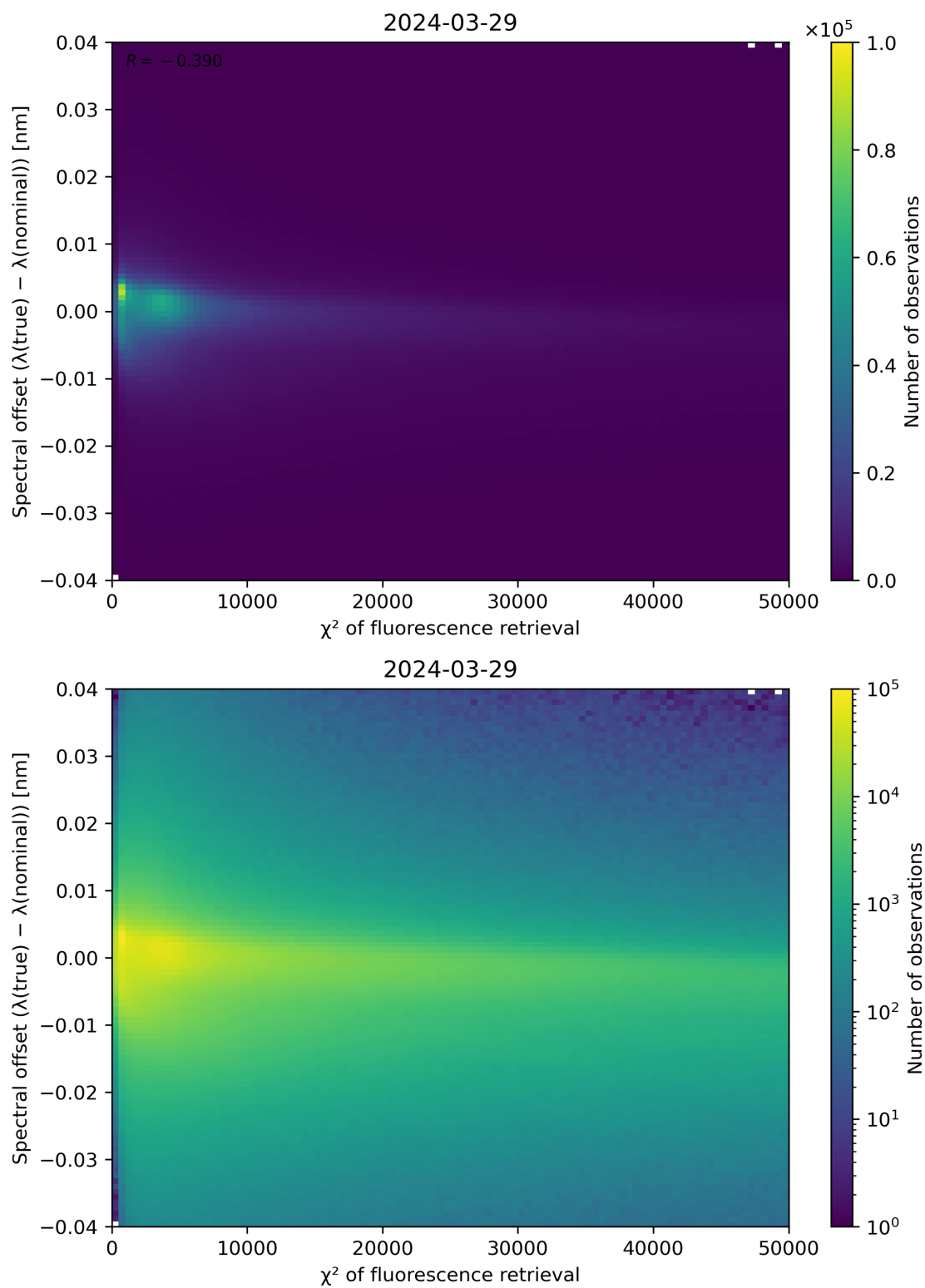
Figure 69: Scatter density plot of " \chi^2 of fluorescence retrieval" against "Spectral offset ( \lambda(\text{true}) - \lambda(\text{nominal})) " for 2024-03-28 to 2024-03-30.
