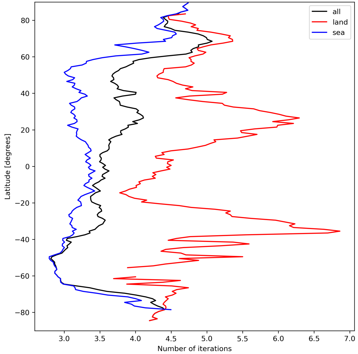
Figure 22: Zonal average of “Number of iterations” for 2024-03-28 to 2024-03-30.
