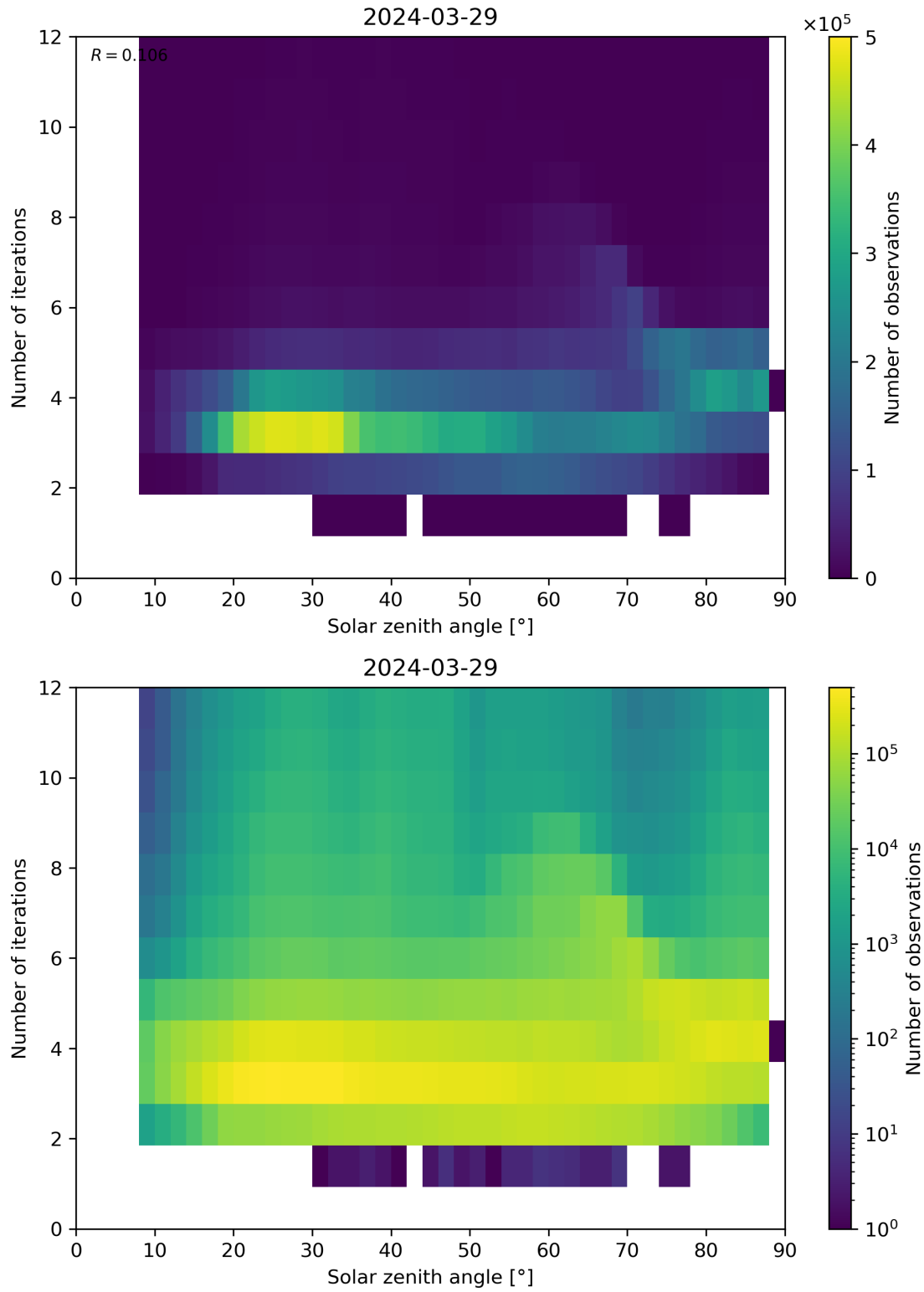
Figure 114: Scatter density plot of “Solar zenith angle” against “Number of iterations” for 2024-03-28 to 2024-03-30.
