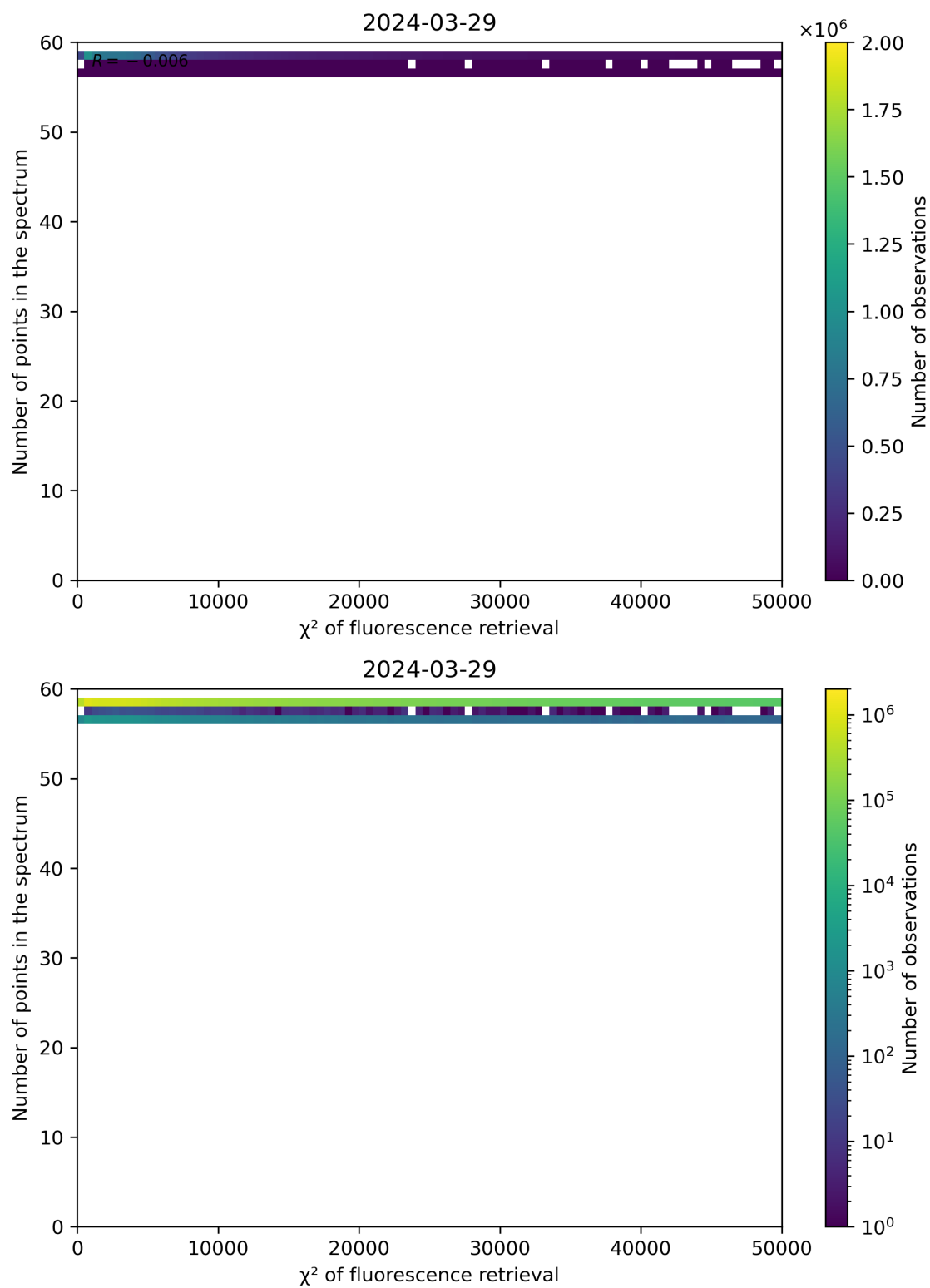
Figure 68: Scatter density plot of “ \chi^2 of fluorescence retrieval” against “Number of points in the spectrum” for 2024-03-28 to 2024-03-30.
