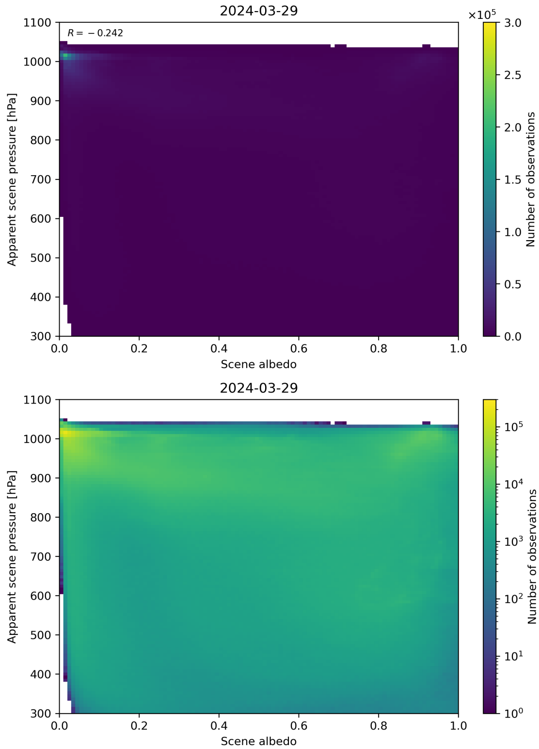
Figure 102: Scatter density plot of “Scene albedo” against “Apparent scene pressure” for 2024-03-28 to 2024-03-30.
