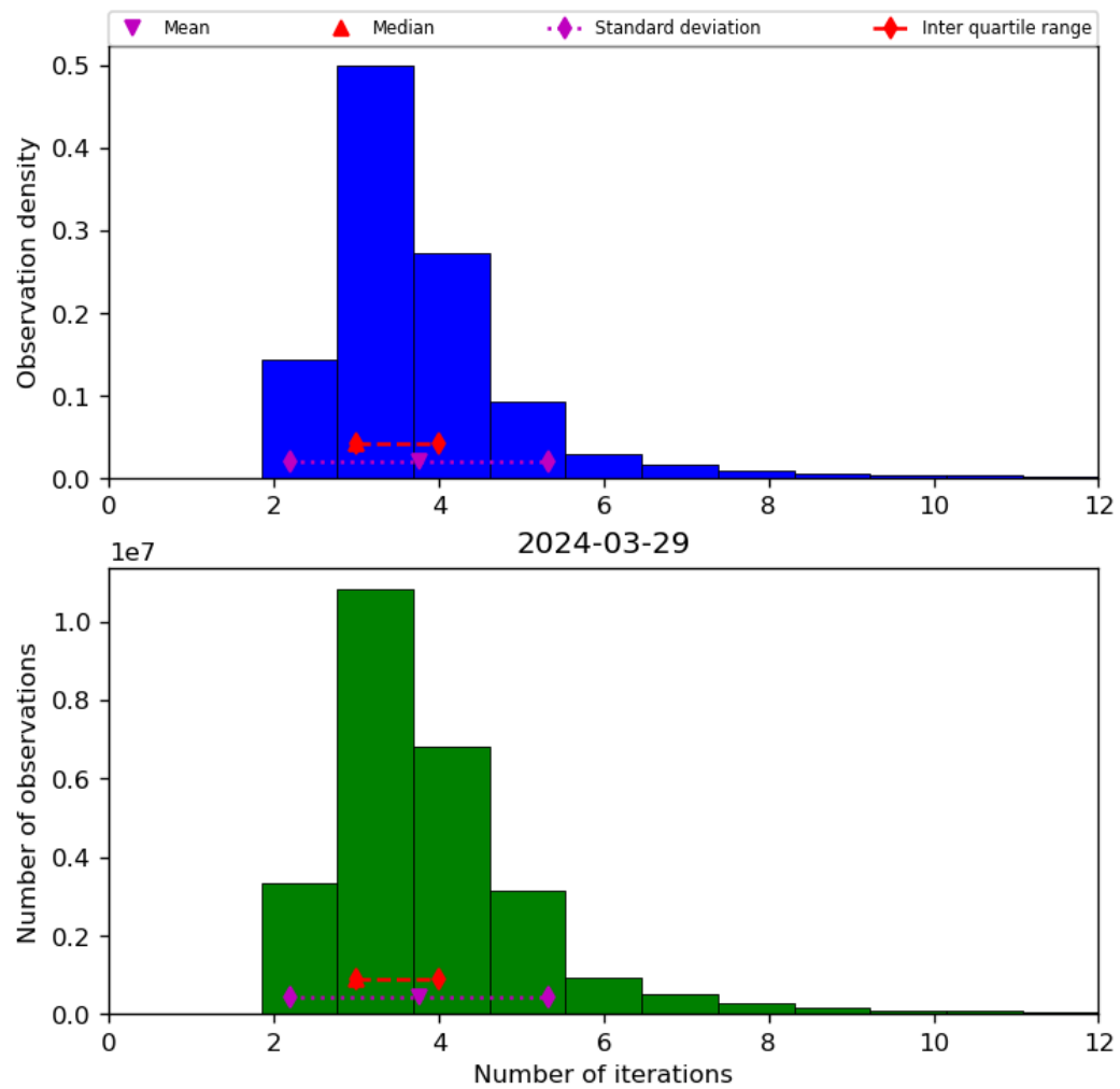
Figure 39: Histogram of “Number of iterations” for 2024-03-28 to 2024-03-30
