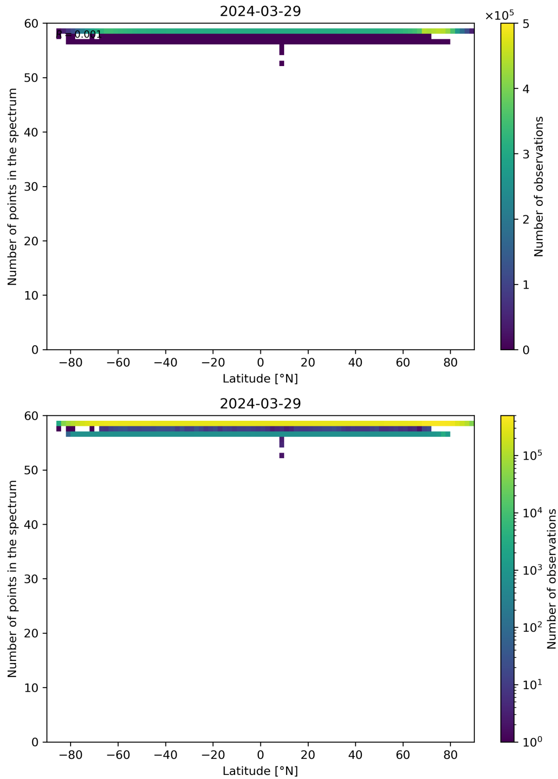
Figure 94: Scatter density plot of “Latitude” against “Number of points in the spectrum” for 2024-03-28 to 2024-03-30.
