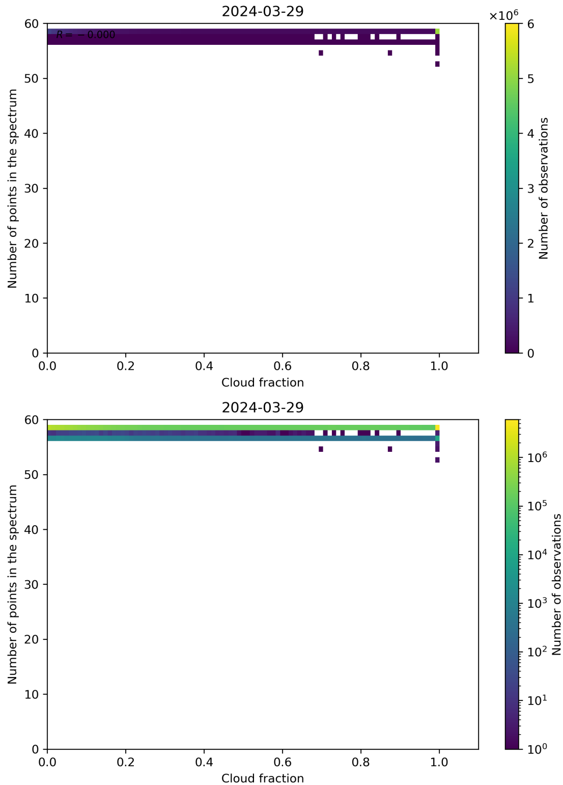
Figure 74: Scatter density plot of “Cloud fraction” against “Number of points in the spectrum” for 2024-03-28 to 2024-03-30.
