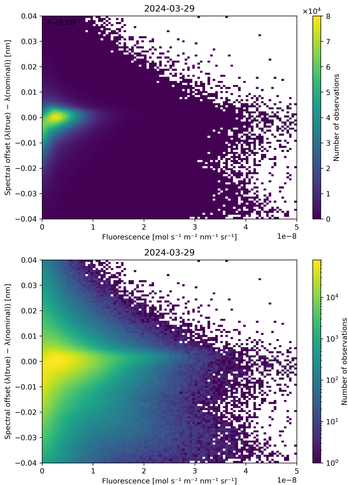
Figure 87: Scatter density plot of “Fluorescence” against “Spectral offset ( \lambda(\text{true}) - \lambda(\text{nominal}) )” for 2024-03-28 to 2024-03-30.
