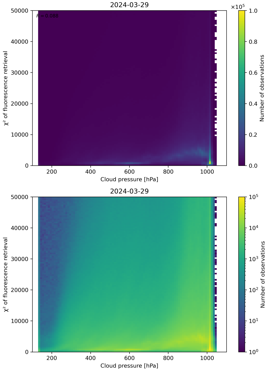
Figure 78: Scatter density plot of “Cloud pressure” against “ \chi^2 of fluorescence retrieval” for 2024-03-28 to 2024-03-30.
