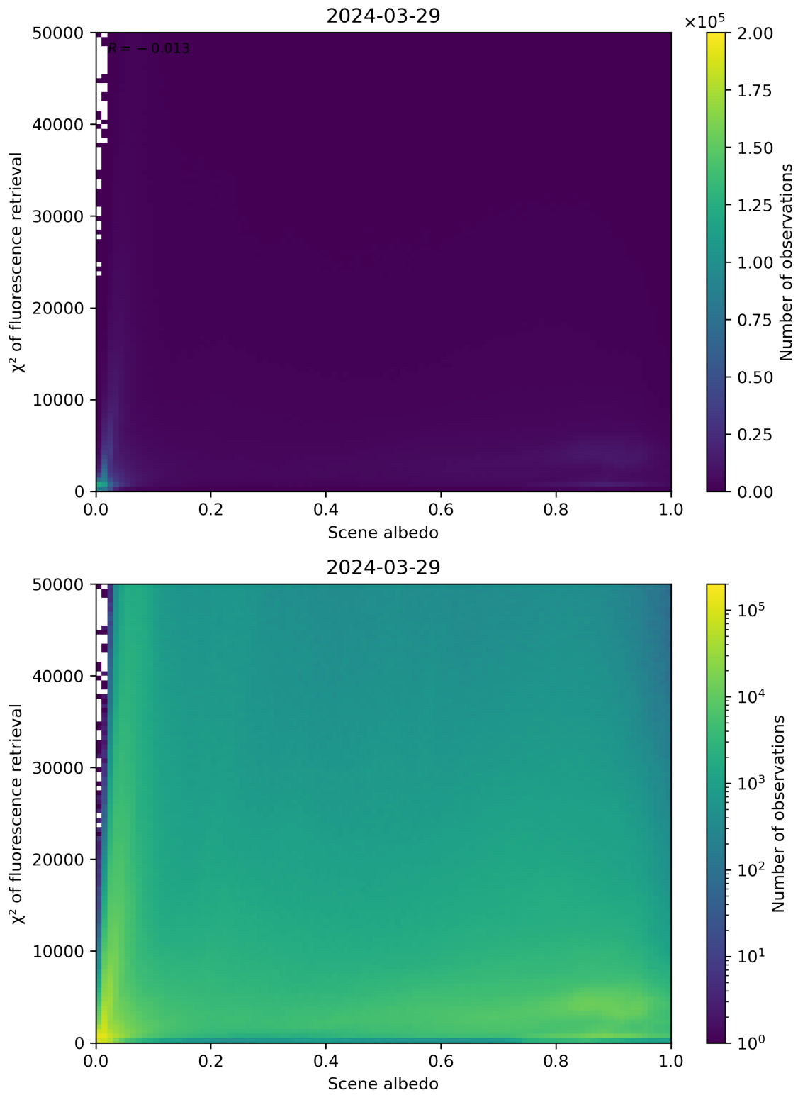
Figure 103: Scatter density plot of “Scene albedo” against “ \chi^2 of fluorescence retrieval” for 2024-03-28 to 2024-03-30.
