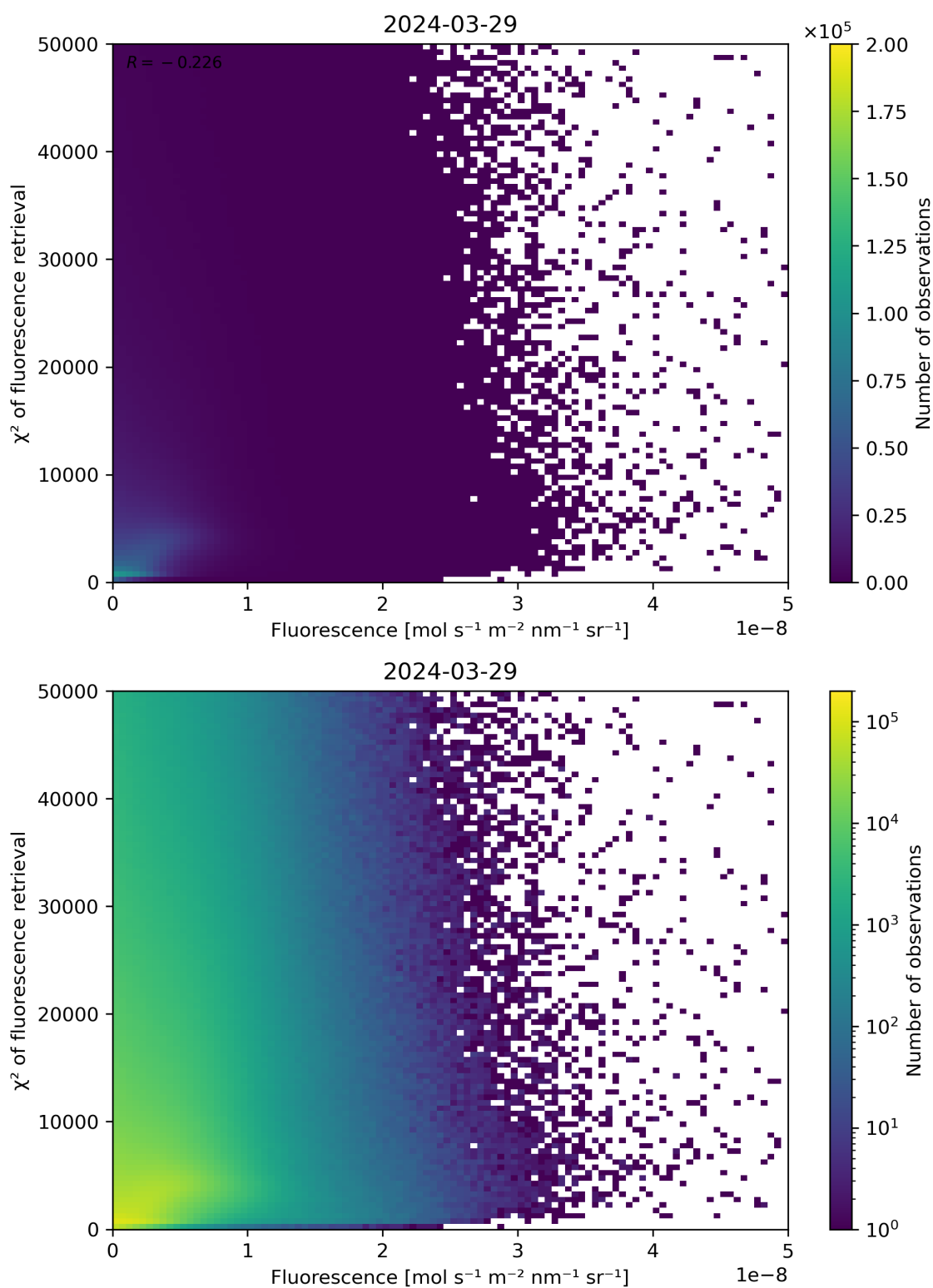
Figure 85: Scatter density plot of “Fluorescence” against “ \chi^2 of fluorescence retrieval” for 2024-03-28 to 2024-03-30.
