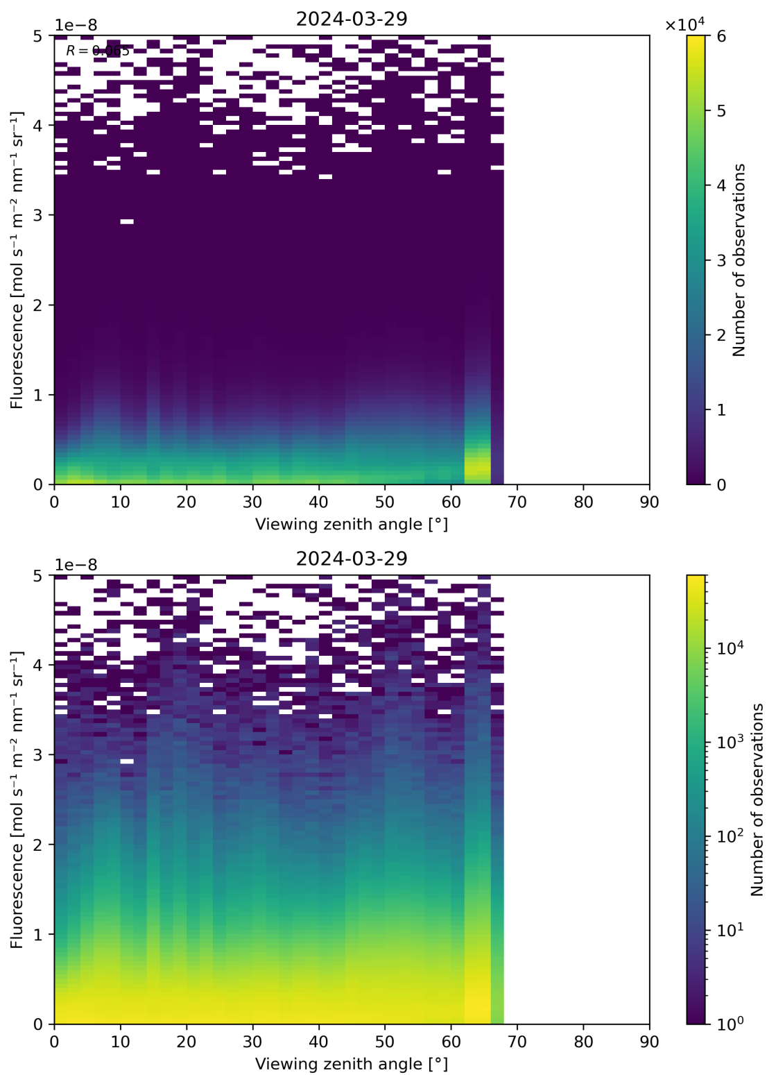
Figure 122: Scatter density plot of “Viewing zenith angle” against “Fluorescence” for 2024-03-28 to 2024-03-30.
