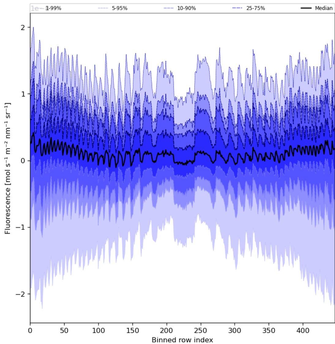
Figure 57: Along track statistics of “Fluorescence” for 2024-03-28 to 2024-03-30
