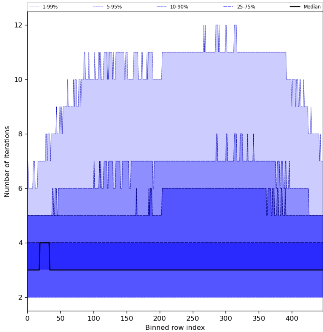
Figure 56: Along track statistics of “Number of iterations” for 2024-03-28 to 2024-03-30
