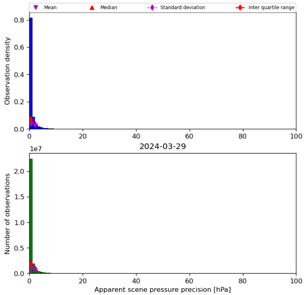
Figure 37: Histogram of “Apparent scene pressure precision” for 2024-03-28 to 2024-03-30
