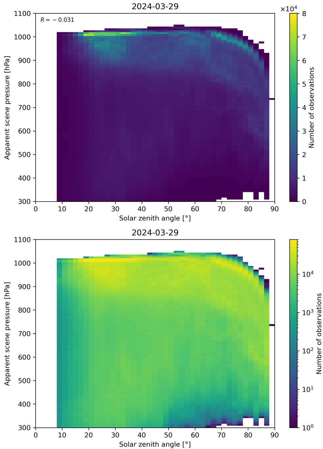
Figure 108: Scatter density plot of “Solar zenith angle” against “Apparent scene pressure” for 2024-03-28 to 2024-03-30.
