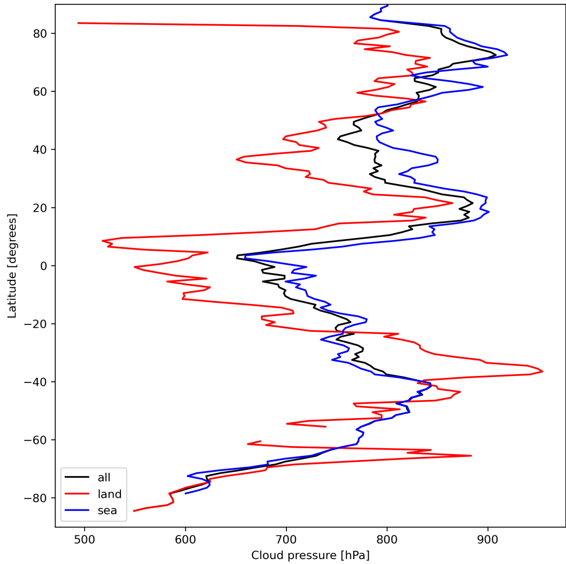
Figure 13: Zonal average of “Cloud pressure” for 2024-03-28 to 2024-03-30.
