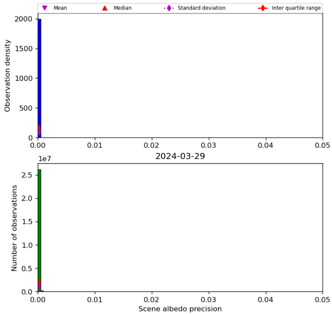
Figure 35: Histogram of “Scene albedo precision” for 2024-03-28 to 2024-03-30
