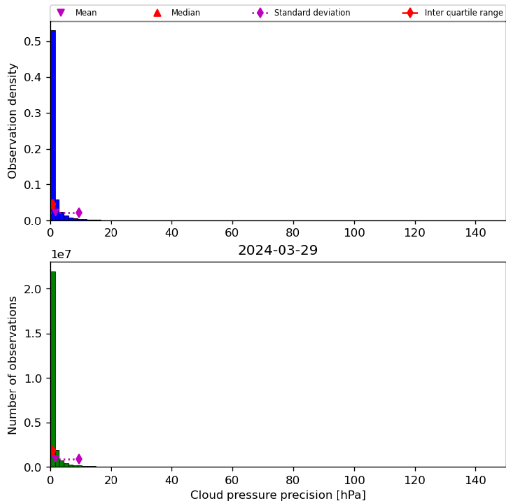
Figure 31: Histogram of “Cloud pressure precision” for 2024-03-28 to 2024-03-30
