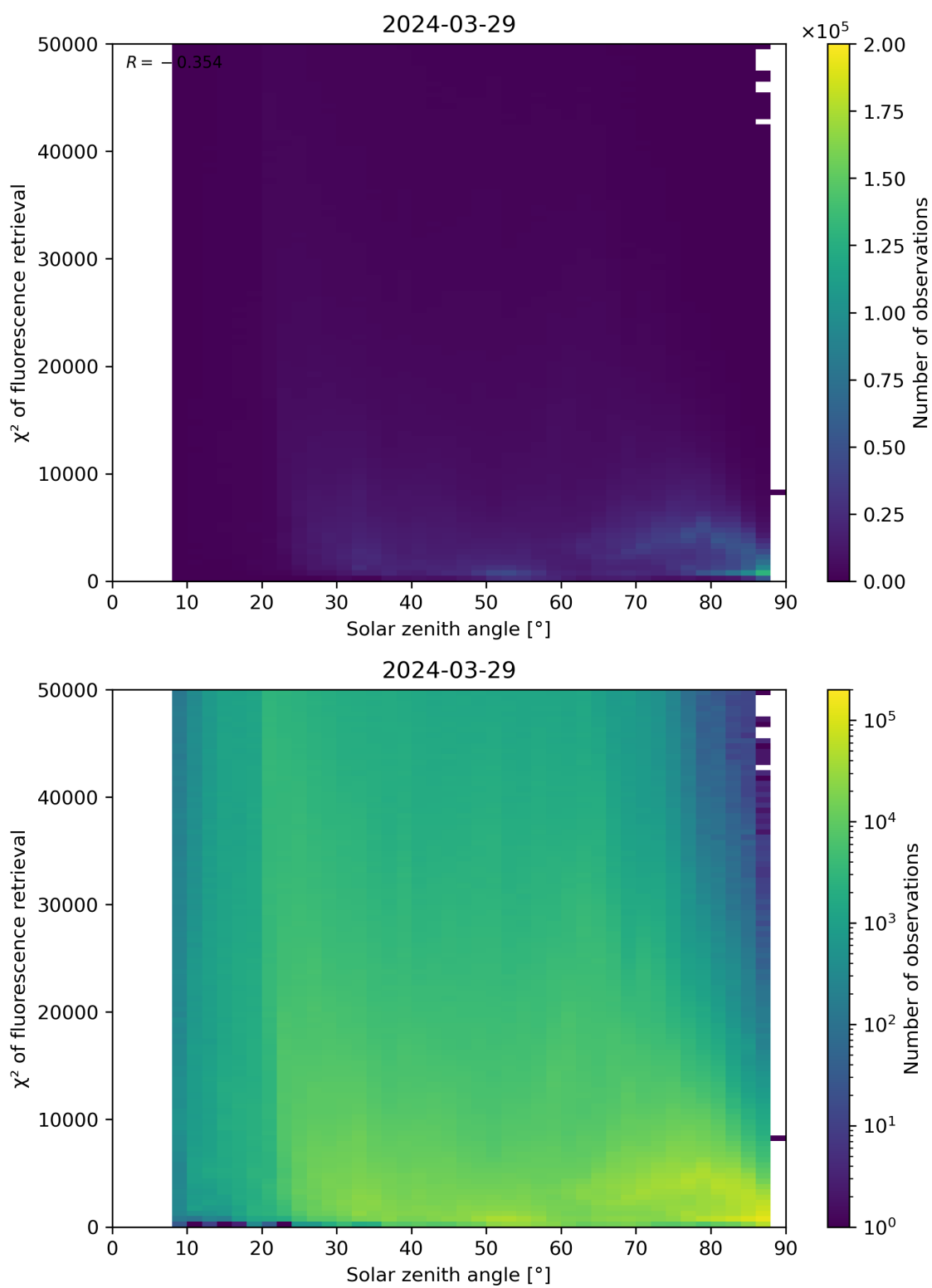
Figure 109: Scatter density plot of “Solar zenith angle” against “ \chi^2 of fluorescence retrieval” for 2024-03-28 to 2024-03-30.
