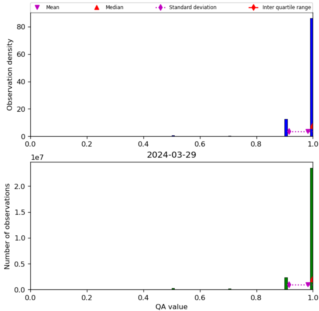
Figure 29: Histogram of “QA value” for 2024-03-28 to 2024-03-30
