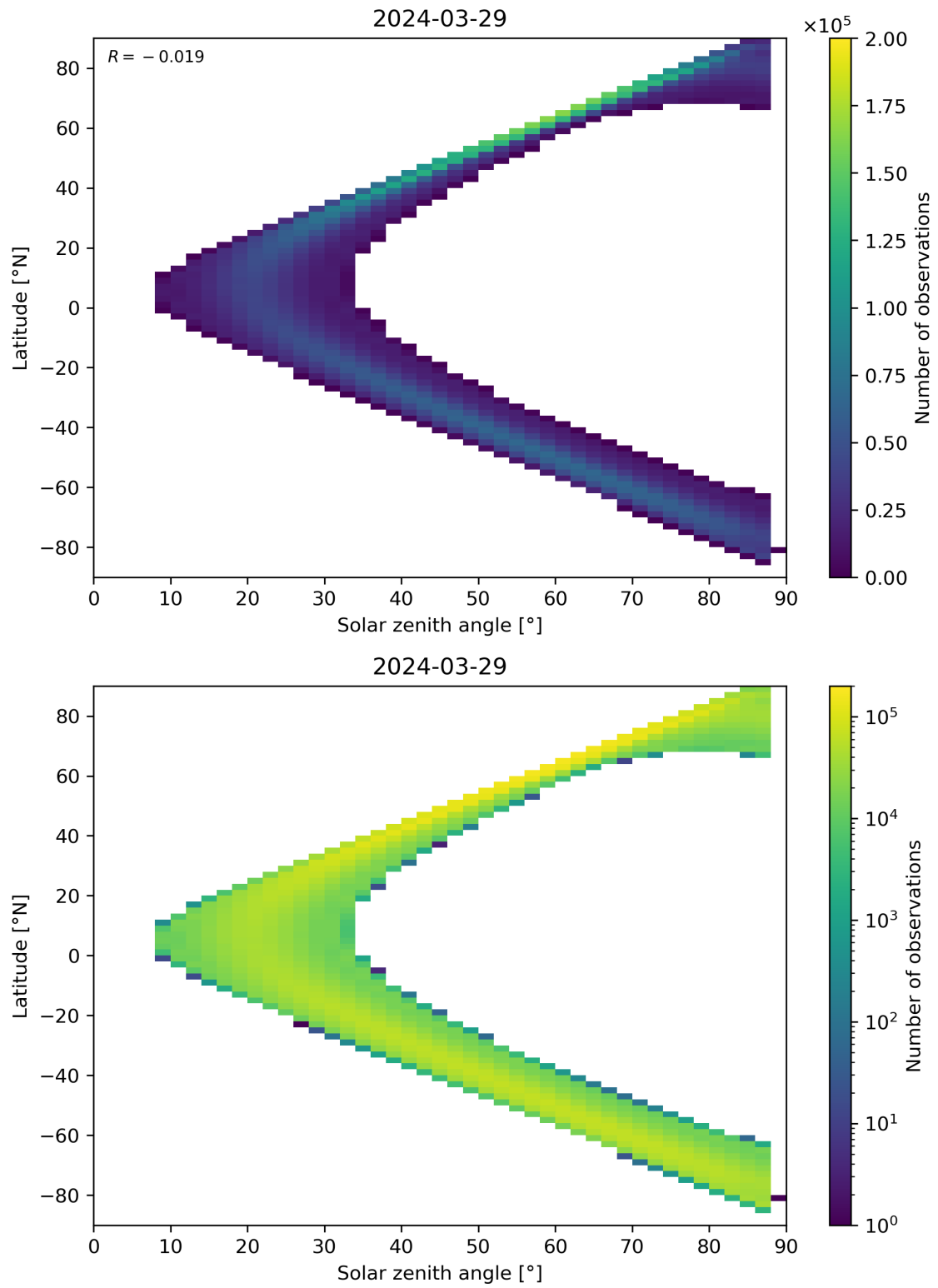
Figure 113: Scatter density plot of “Solar zenith angle” against “Latitude” for 2024-03-28 to 2024-03-30.
