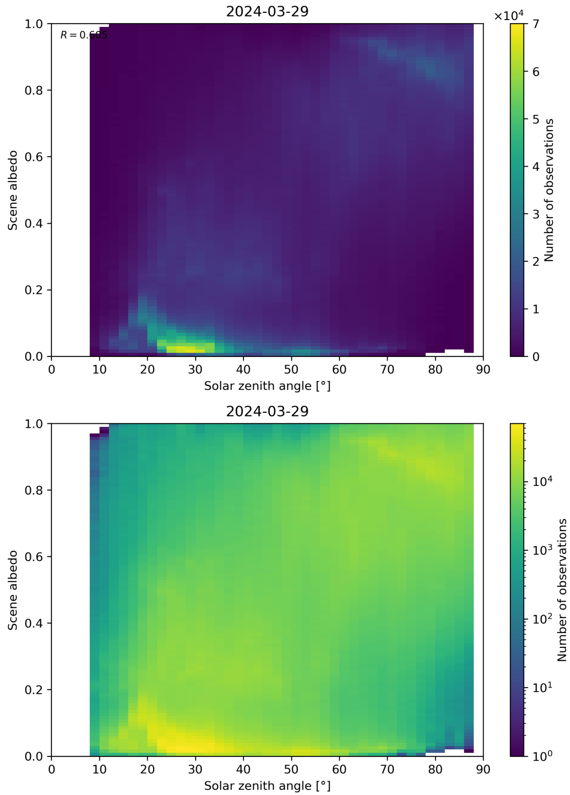
Figure 116: Scatter density plot of “Solar zenith angle” against “Scene albedo” for 2024-03-28 to 2024-03-30.
