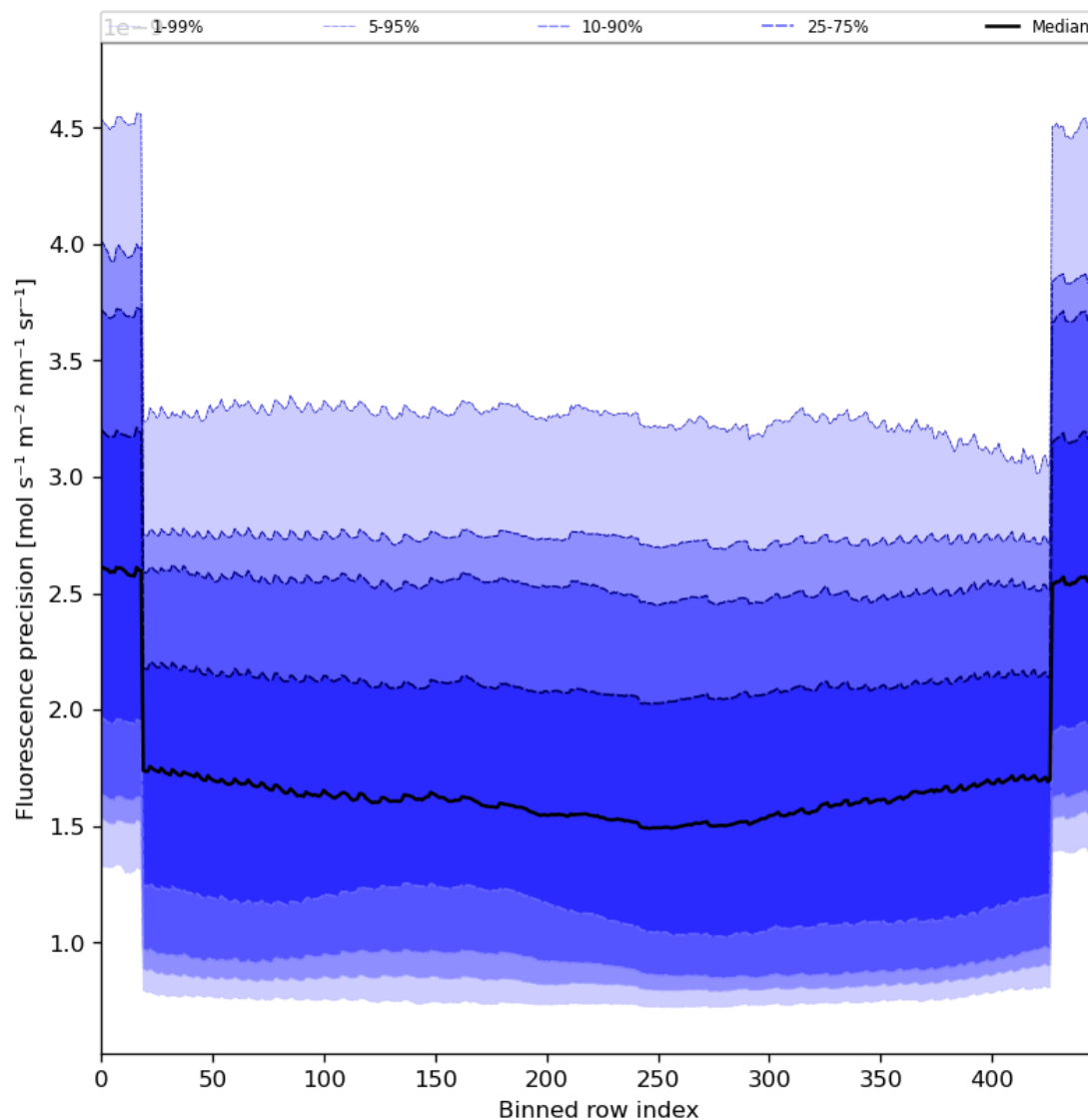
Figure 58: Along track statistics of “Fluorescence precision” for 2024-03-28 to 2024-03-30
