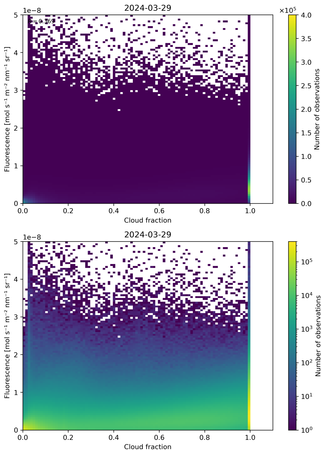
Figure 72: Scatter density plot of “Cloud fraction” against “Fluorescence” for 2024-03-28 to 2024-03-30.
