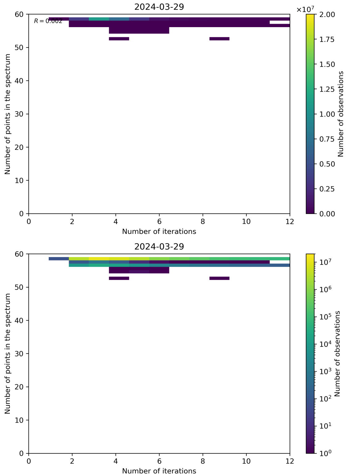
Figure 99: Scatter density plot of “Number of iterations” against “Number of points in the spectrum” for 2024-03-28 to 2024-03-30.
