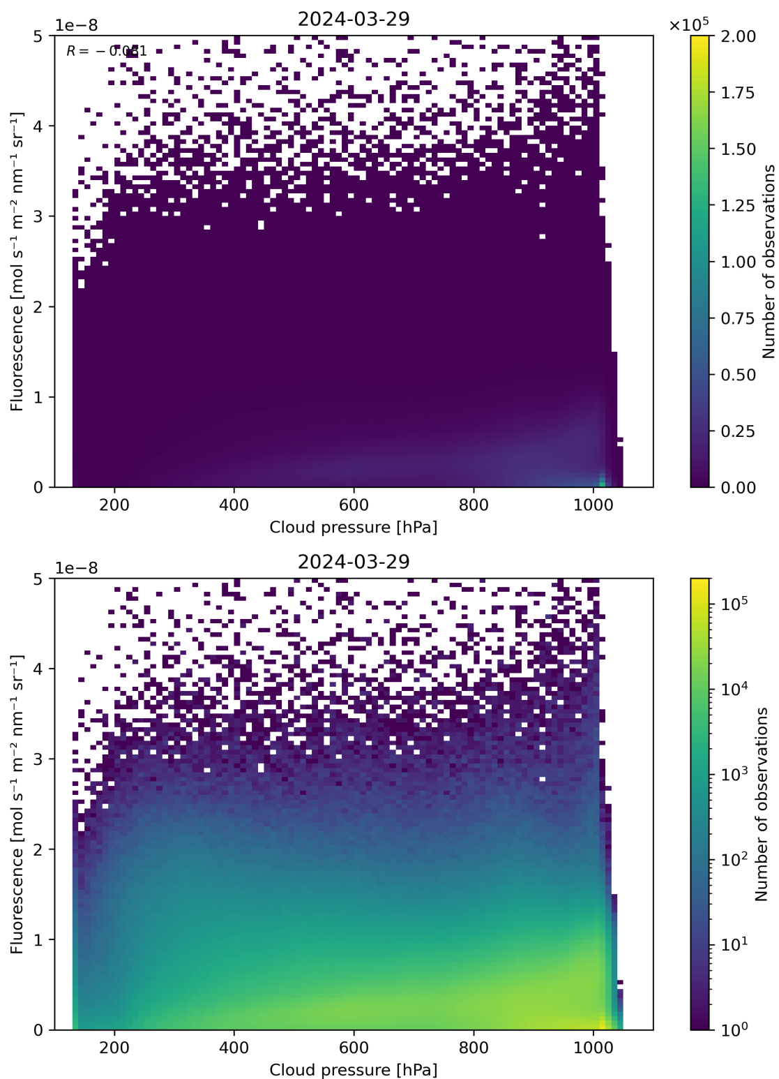
Figure 80: Scatter density plot of “Cloud pressure” against “Fluorescence” for 2024-03-28 to 2024-03-30.
