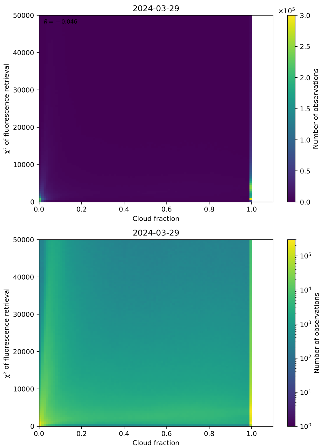
Figure 71: Scatter density plot of “Cloud fraction” against “ \chi^2 of fluorescence retrieval” for 2024-03-28 to 2024-03-30.
