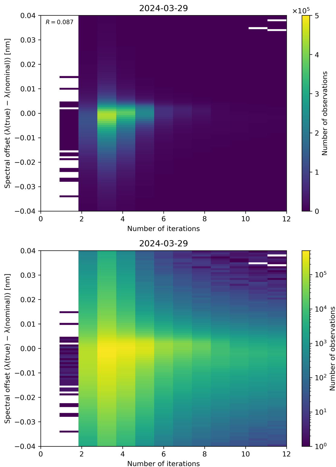
Figure 100: Scatter density plot of “Number of iterations” against “Spectral offset ( \lambda(\text{true}) - \lambda(\text{nominal}) )” for 2024-03-28 to 2024-03-30.
