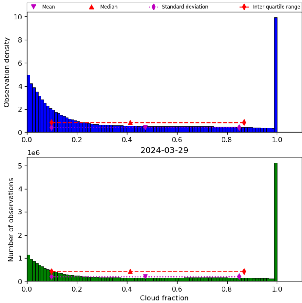
Figure 32: Histogram of “Cloud fraction” for 2024-03-28 to 2024-03-30
