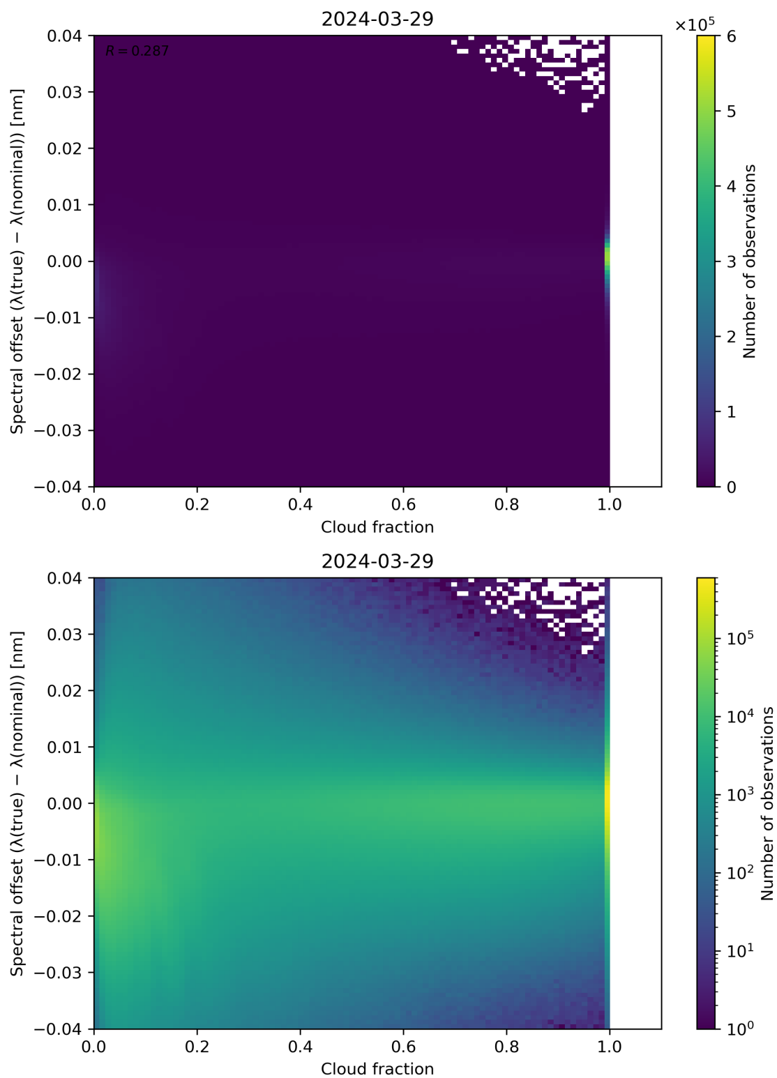
Figure 76: Scatter density plot of “Cloud fraction” against “Spectral offset ( \lambda(\text{true}) - \lambda(\text{nominal}) )” for 2024-03-28 to 2024-03-30.
