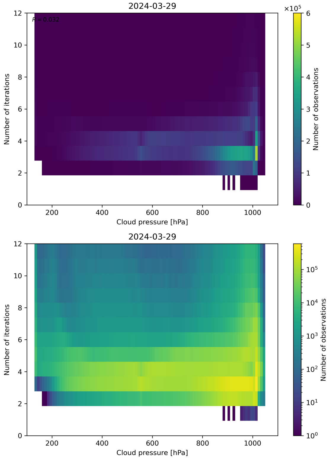
Figure 81: Scatter density plot of “Cloud pressure” against “Number of iterations” for 2024-03-28 to 2024-03-30.
