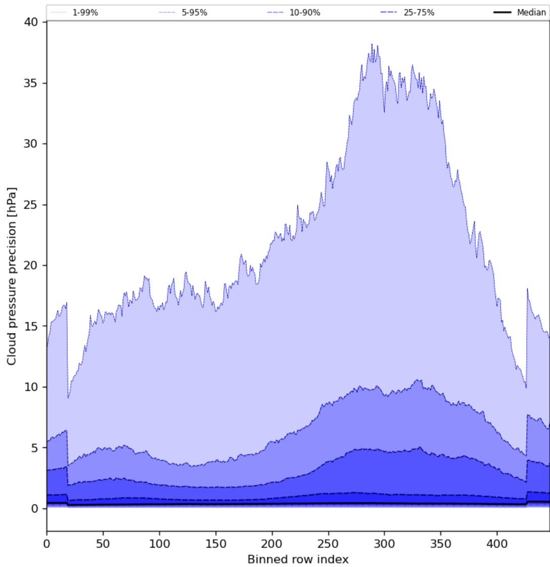
Figure 48: Along track statistics of “Cloud pressure precision” for 2024-03-28 to 2024-03-30
