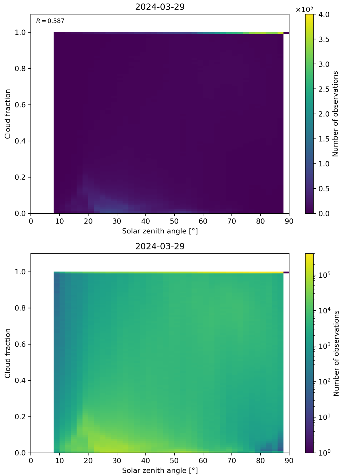
Figure 110: Scatter density plot of “Solar zenith angle” against “Cloud fraction” for 2024-03-28 to 2024-03-30.
