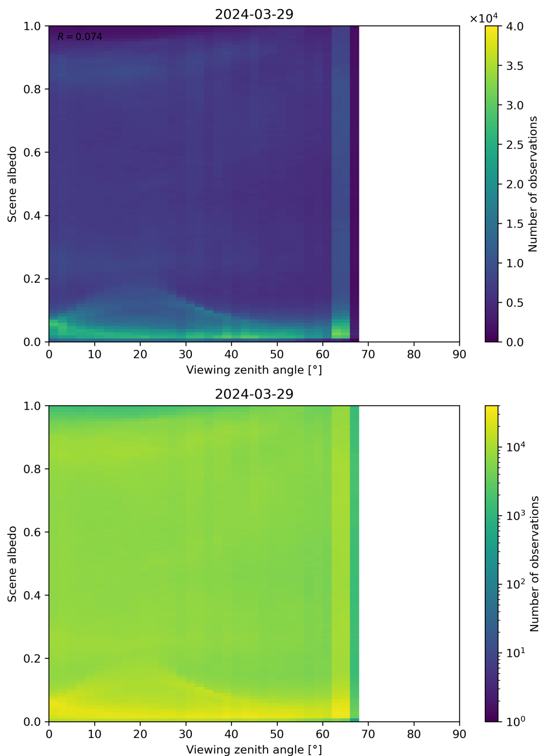
Figure 126: Scatter density plot of “Viewing zenith angle” against “Scene albedo” for 2024-03-28 to 2024-03-30.
