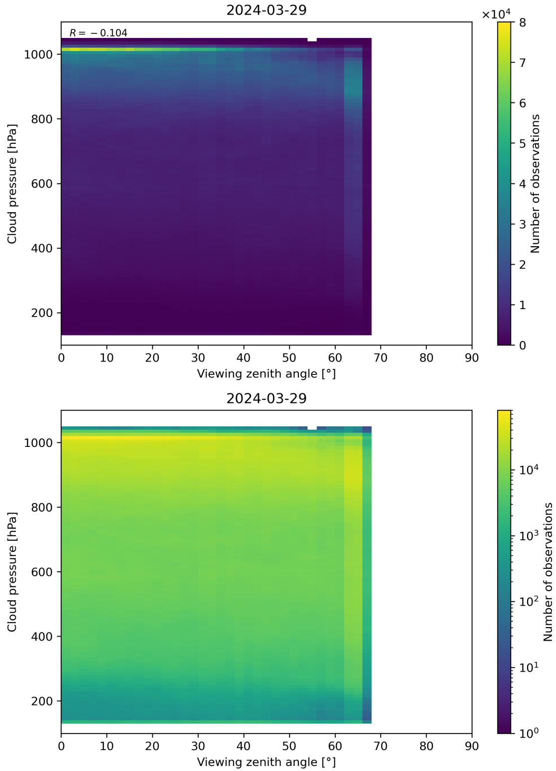
Figure 121: Scatter density plot of “Viewing zenith angle” against “Cloud pressure” for 2024-03-28 to 2024-03-30.
