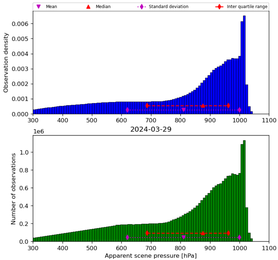
Figure 36: Histogram of “Apparent scene pressure” for 2024-03-28 to 2024-03-30
