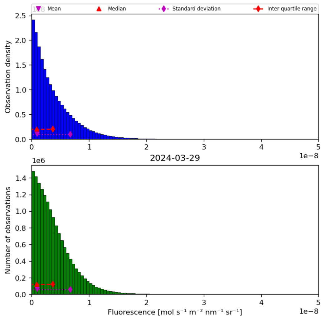
Figure 40: Histogram of “Fluorescence” for 2024-03-28 to 2024-03-30
