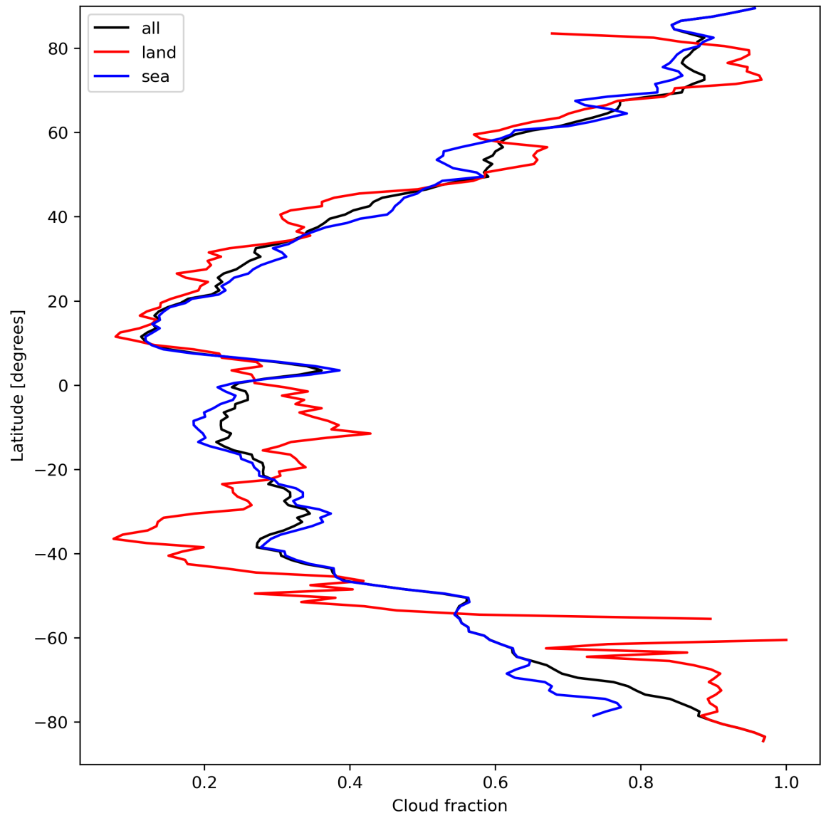
Figure 15: Zonal average of “Cloud fraction” for 2024-03-28 to 2024-03-30.
