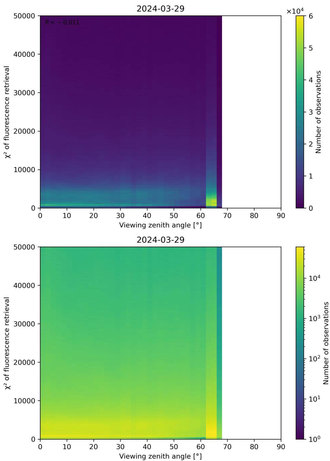
Figure 119: Scatter density plot of “Viewing zenith angle” against “ \chi^2 of fluorescence retrieval” for 2024-03-28 to 2024-03-30.
