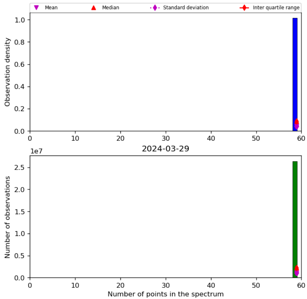
Figure 44: Histogram of “Number of points in the spectrum” for 2024-03-28 to 2024-03-30
