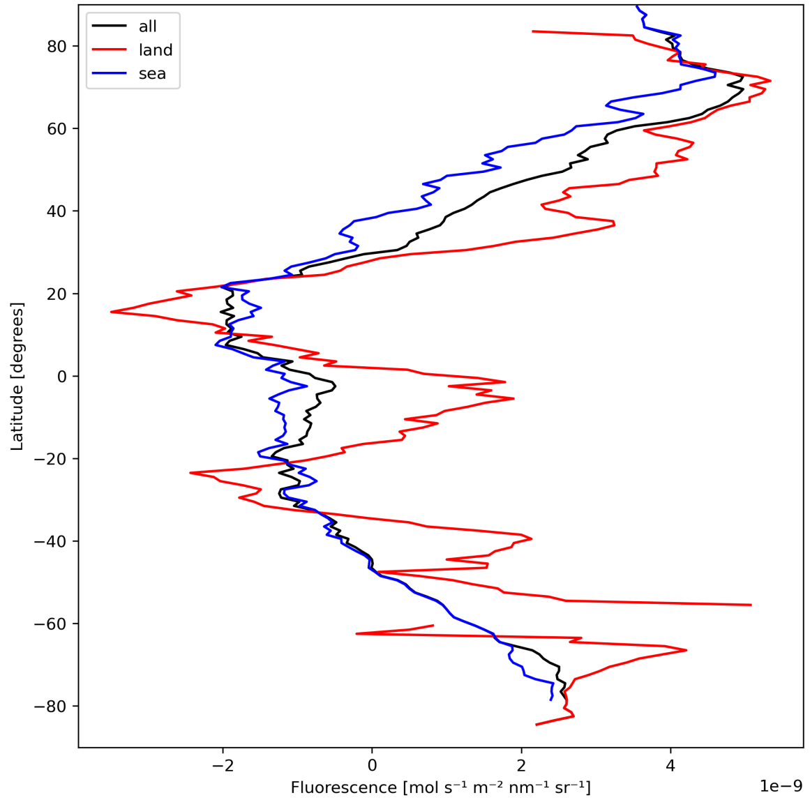
Figure 23: Zonal average of “Fluorescence” for 2024-03-28 to 2024-03-30.
