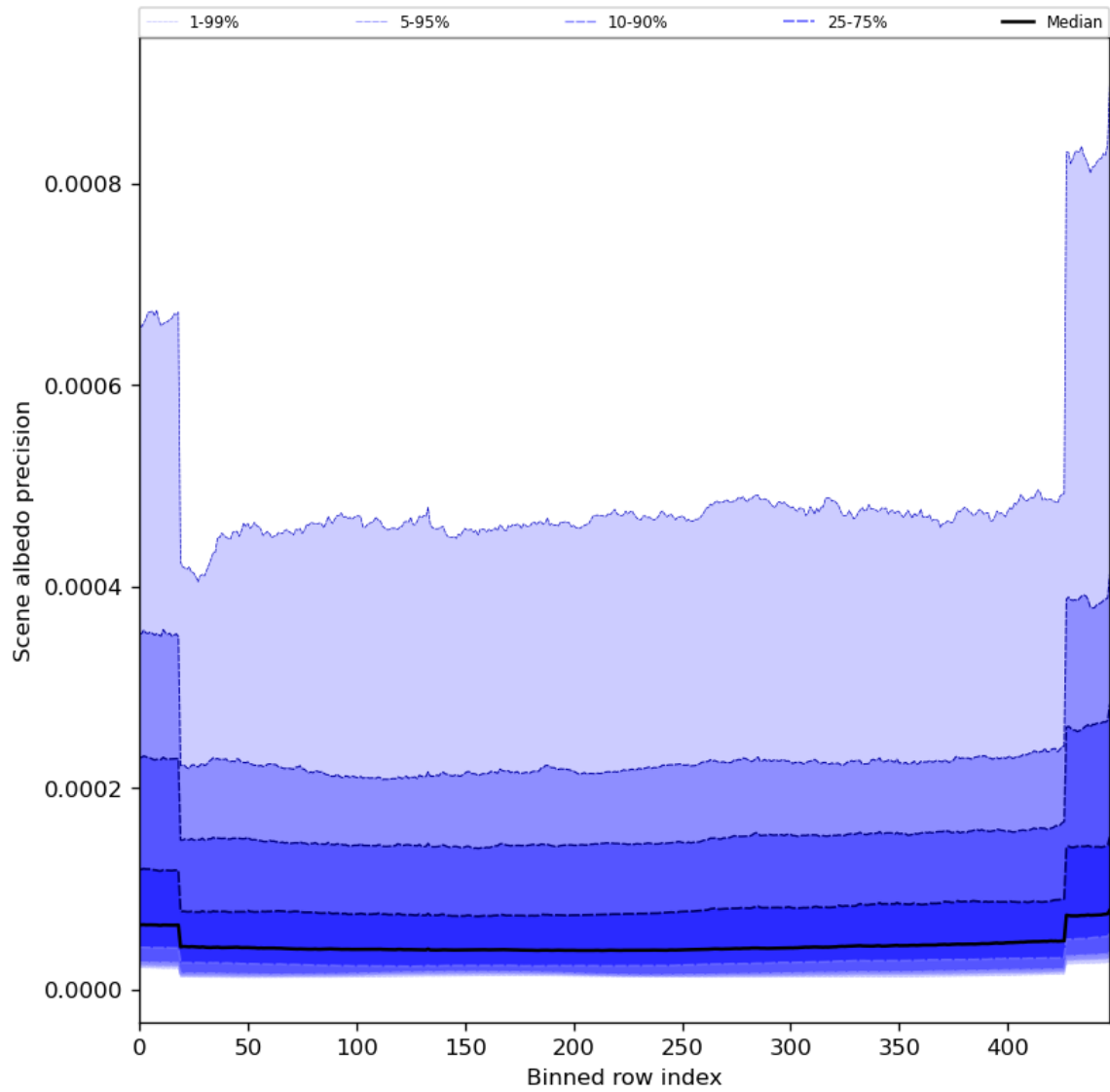
Figure 52: Along track statistics of “Scene albedo precision” for 2024-03-28 to 2024-03-30
