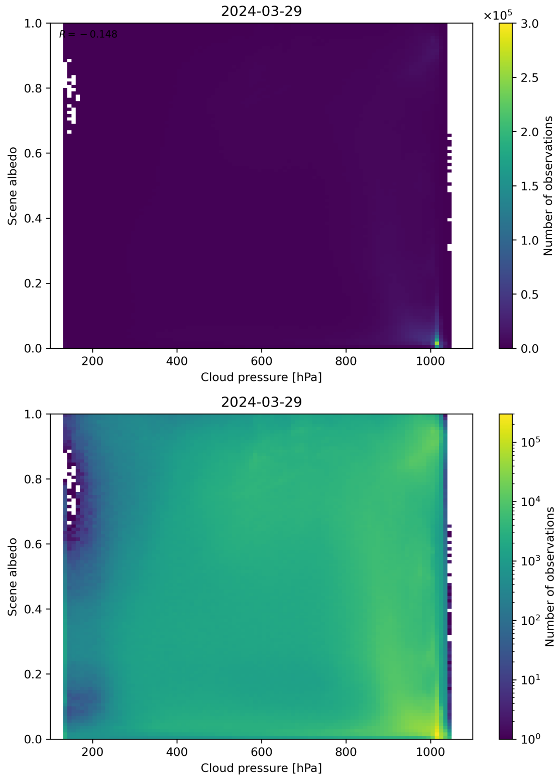
Figure 83: Scatter density plot of “Cloud pressure” against “Scene albedo” for 2024-03-28 to 2024-03-30.
