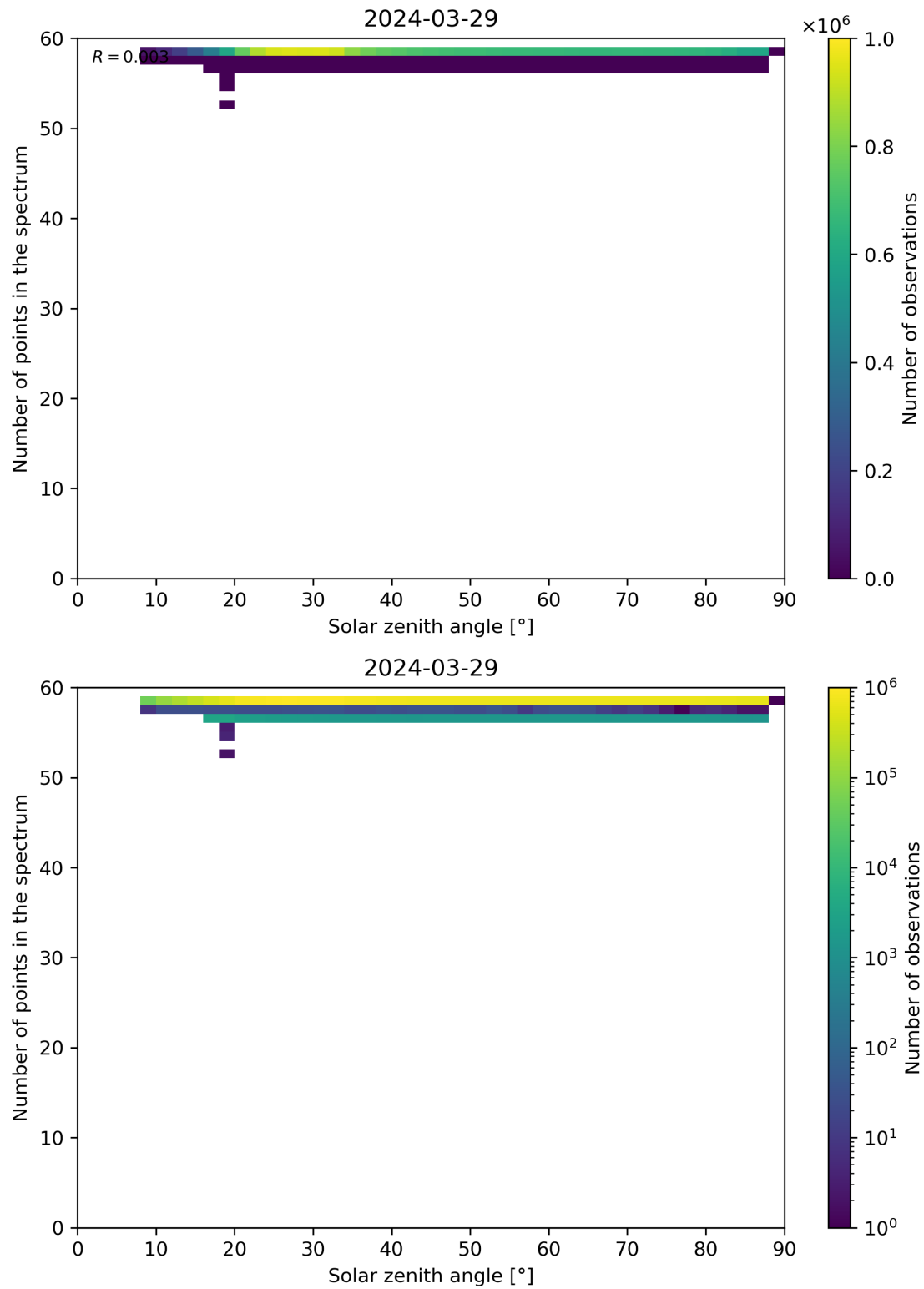
Figure 115: Scatter density plot of “Solar zenith angle” against “Number of points in the spectrum” for 2024-03-28 to 2024-03-30.
