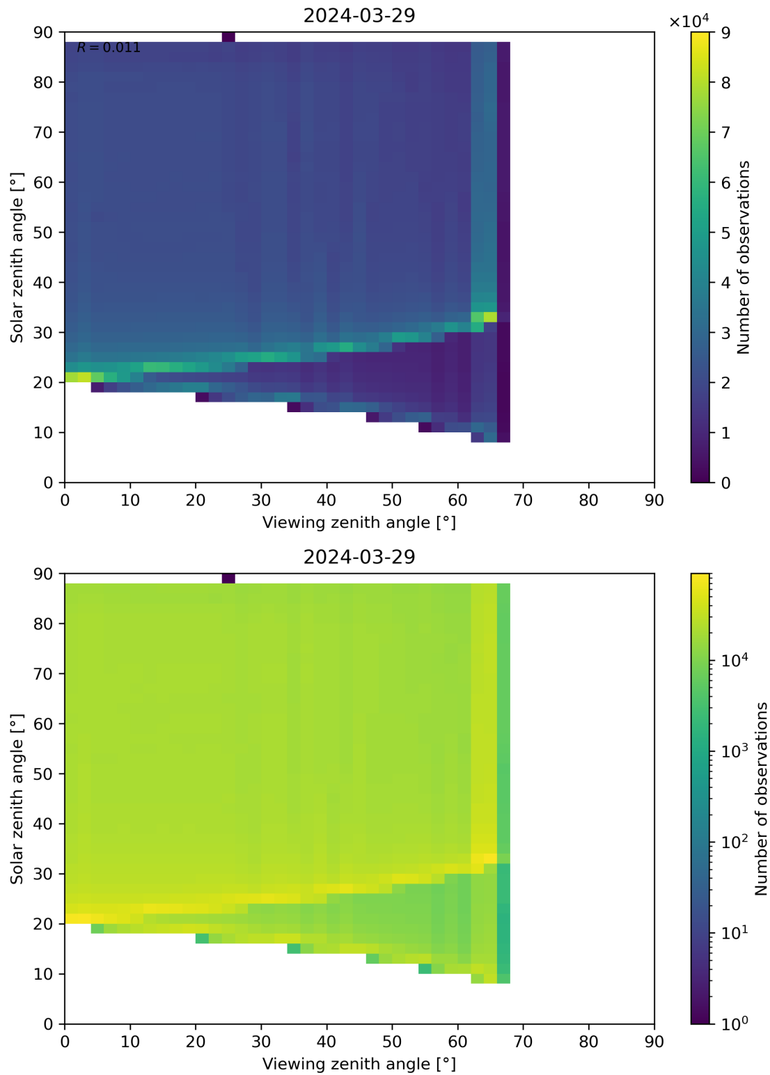
Figure 127: Scatter density plot of “Viewing zenith angle” against “Solar zenith angle” for 2024-03-28 to 2024-03-30.
