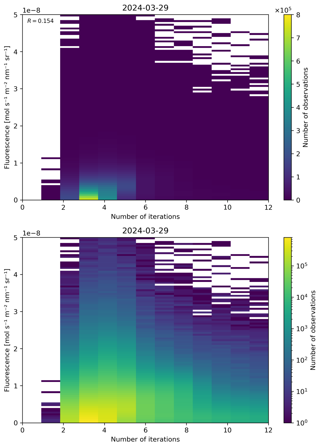
Figure 98: Scatter density plot of “Number of iterations” against “Fluorescence” for 2024-03-28 to 2024-03-30.
