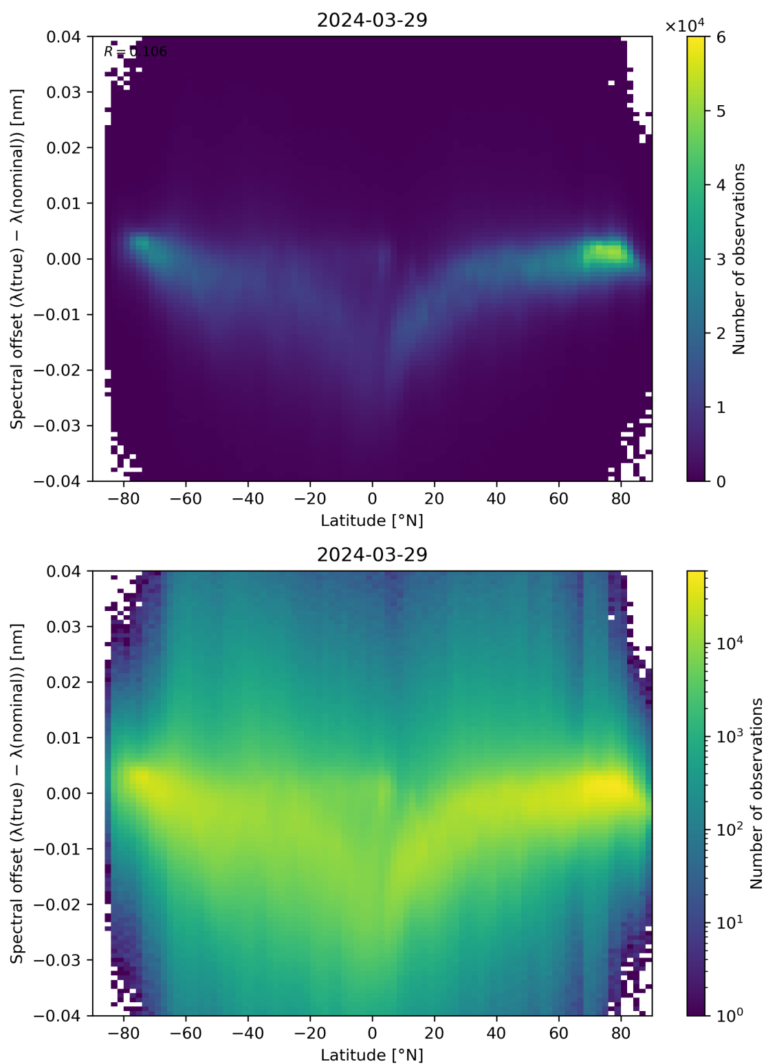
Figure 96: Scatter density plot of “Latitude” against “Spectral offset ( \lambda(\text{true}) - \lambda(\text{nominal}) )” for 2024-03-28 to 2024-03-30.
