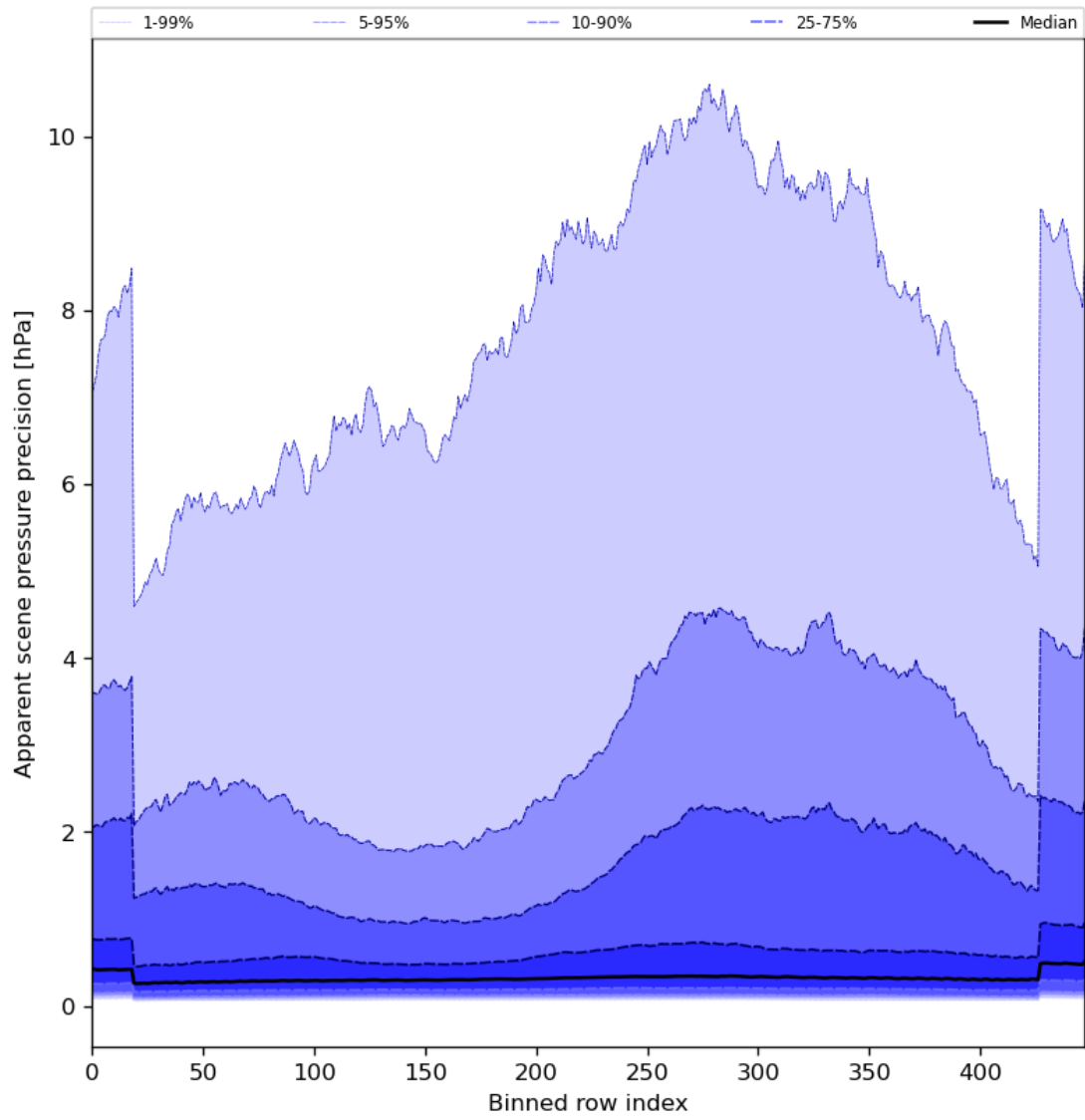
Figure 54: Along track statistics of “Apparent scene pressure precision” for 2024-03-28 to 2024-03-30
