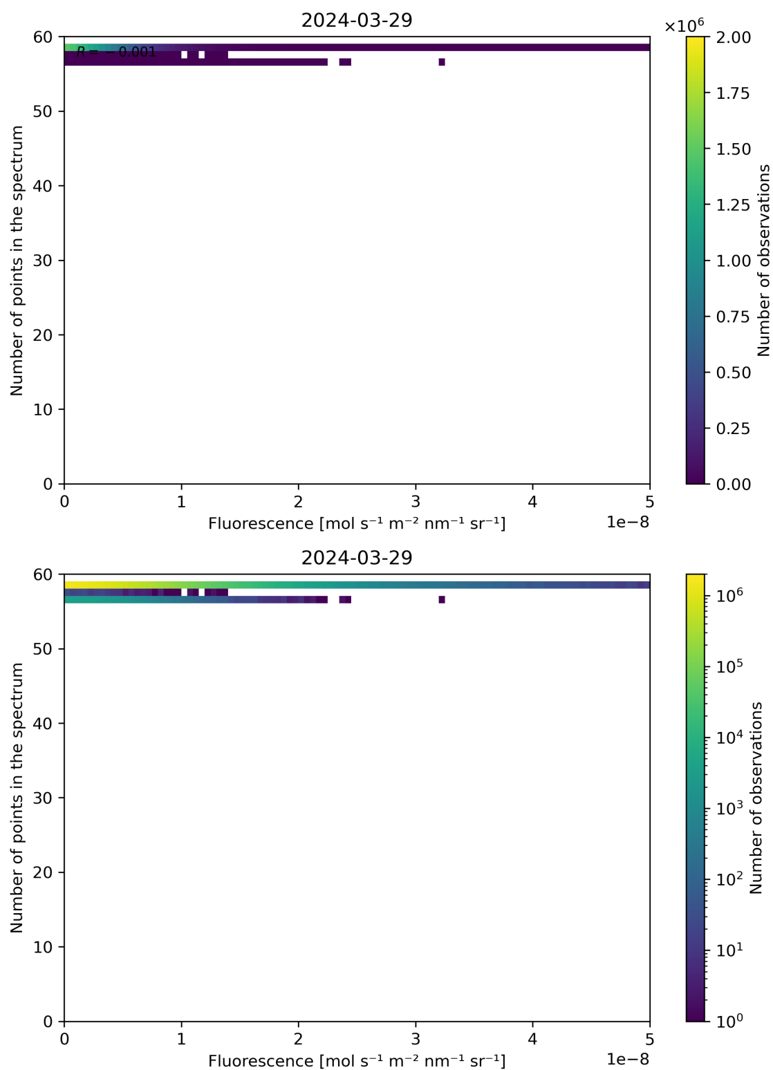
Figure 86: Scatter density plot of “Fluorescence” against “Number of points in the spectrum” for 2024-03-28 to 2024-03-30.
