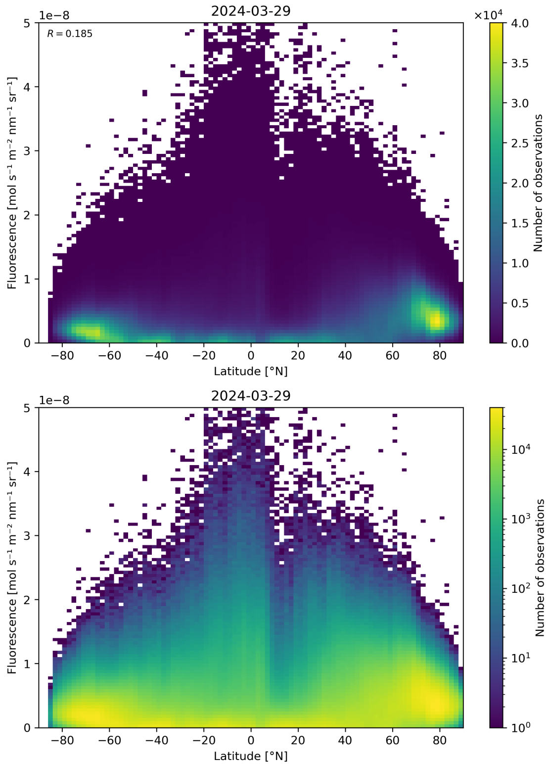
Figure 92: Scatter density plot of “Latitude” against “Fluorescence” for 2024-03-28 to 2024-03-30.
