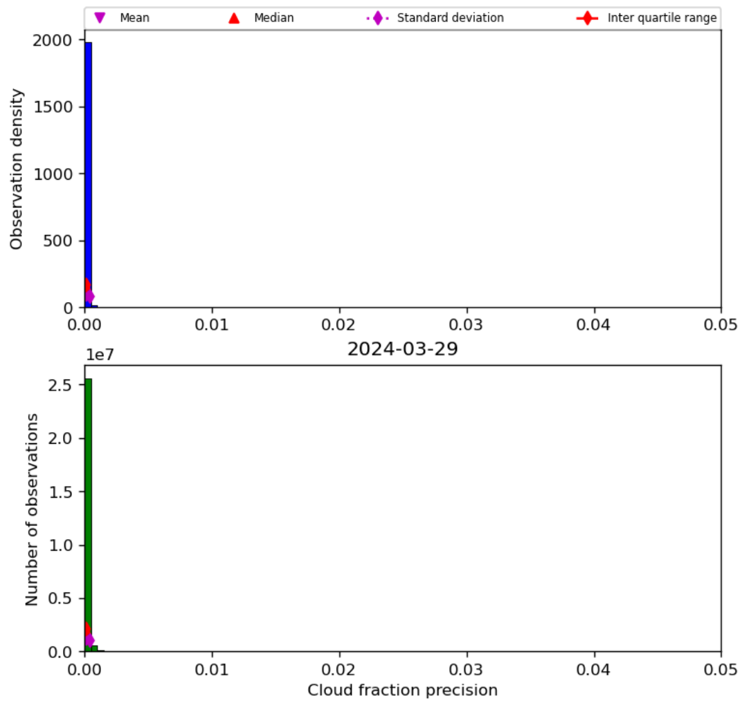
Figure 33: Histogram of “Cloud fraction precision” for 2024-03-28 to 2024-03-30
