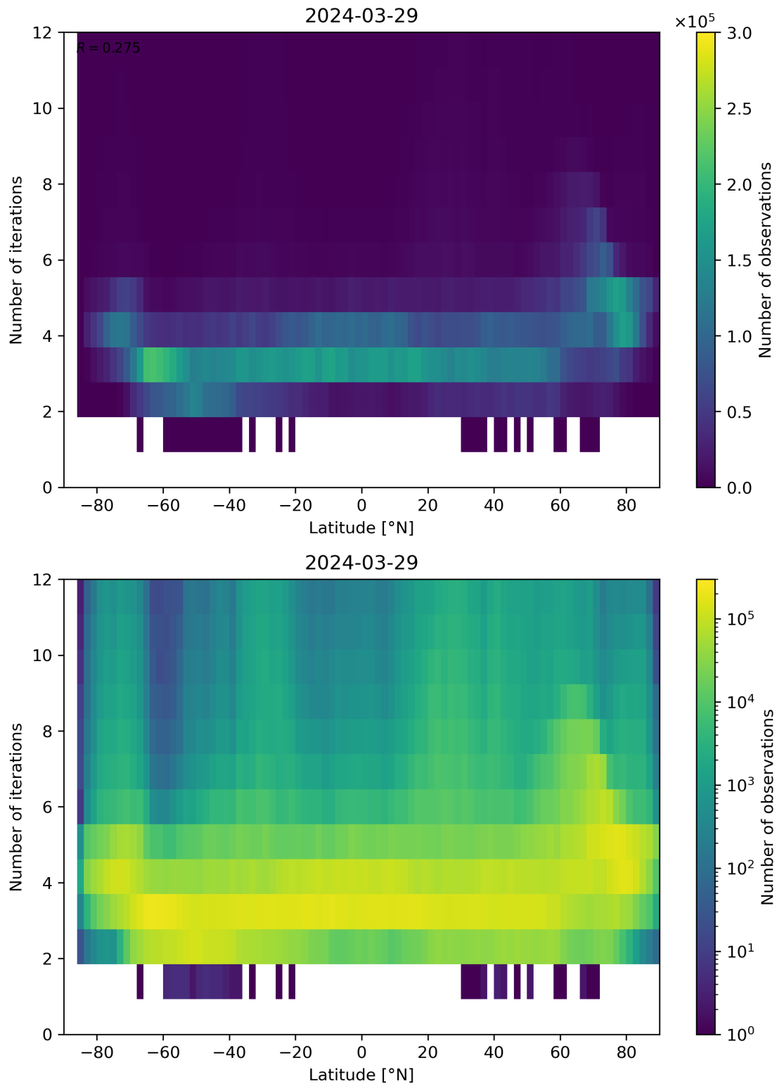
Figure 93: Scatter density plot of “Latitude” against “Number of iterations” for 2024-03-28 to 2024-03-30.
