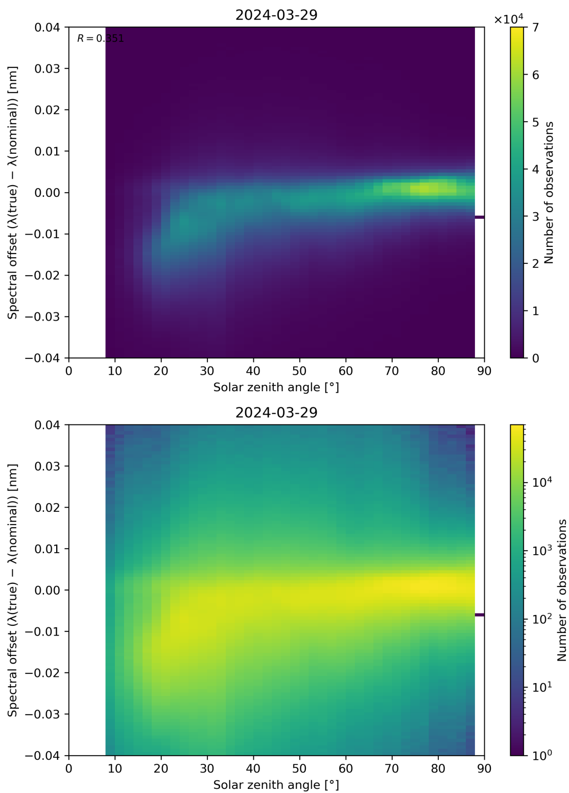
Figure 117: Scatter density plot of “Solar zenith angle” against “Spectral offset ( \lambda(\text{true}) - \lambda(\text{nominal}) )” for 2024-03-28 to 2024-03-30.
