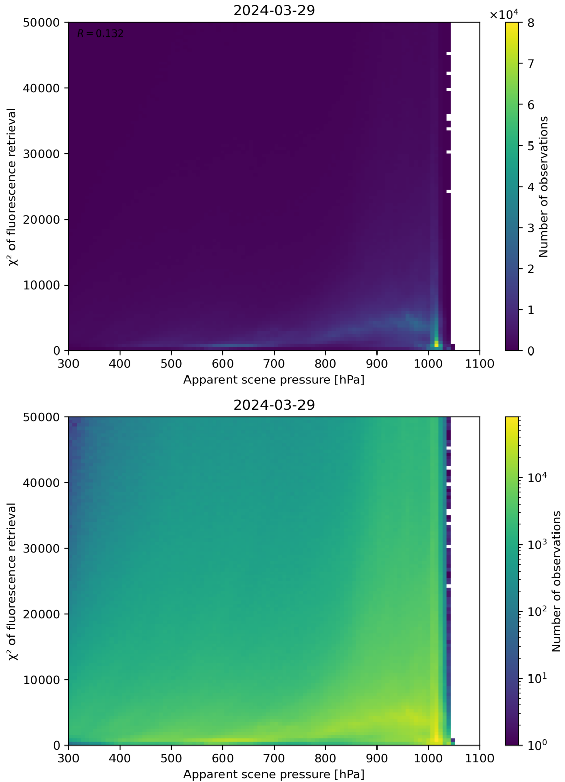
Figure 63: Scatter density plot of “Apparent scene pressure” against “ \chi^2 of fluorescence retrieval” for 2024-03-28 to 2024-03-30.
