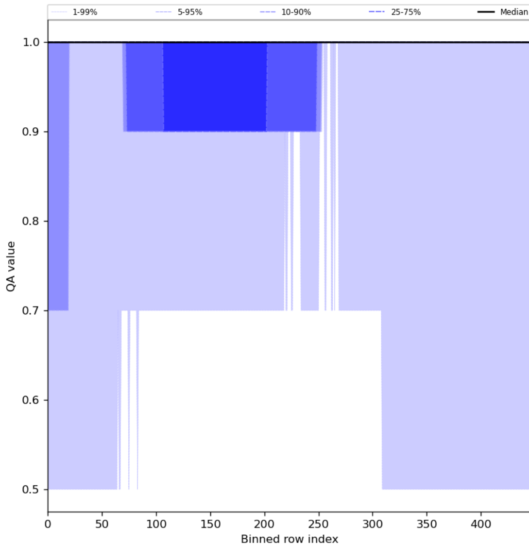
Figure 46: Along track statistics of “QA value” for 2024-03-28 to 2024-03-30
