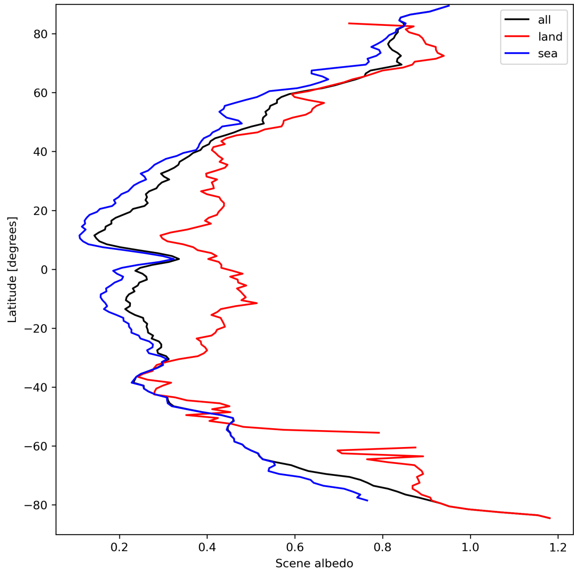
Figure 17: Zonal average of “Scene albedo” for 2024-03-28 to 2024-03-30.
