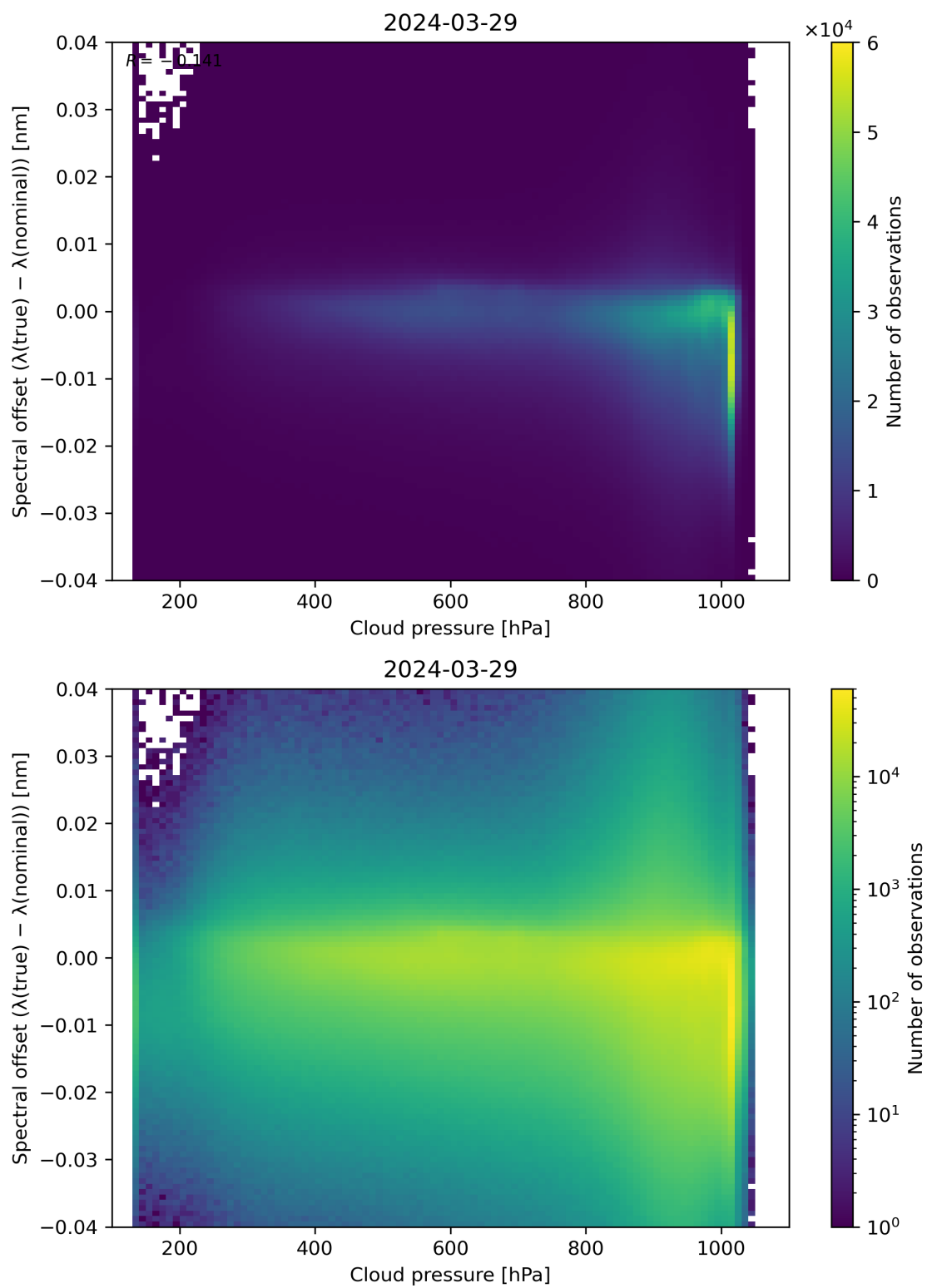
Figure 84: Scatter density plot of “Cloud pressure” against “Spectral offset ( \lambda(\text{true}) - \lambda(\text{nominal}) )” for 2024-03-28 to 2024-03-30.
