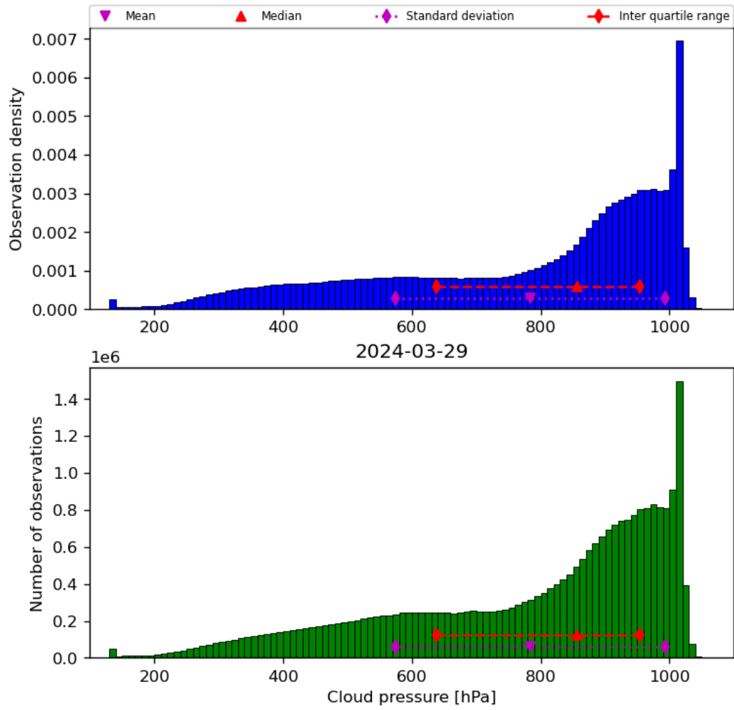
Figure 30: Histogram of “Cloud pressure” for 2024-03-28 to 2024-03-30
