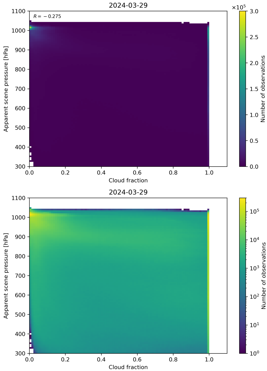
Figure 70: Scatter density plot of “Cloud fraction” against “Apparent scene pressure” for 2024-03-28 to 2024-03-30.
