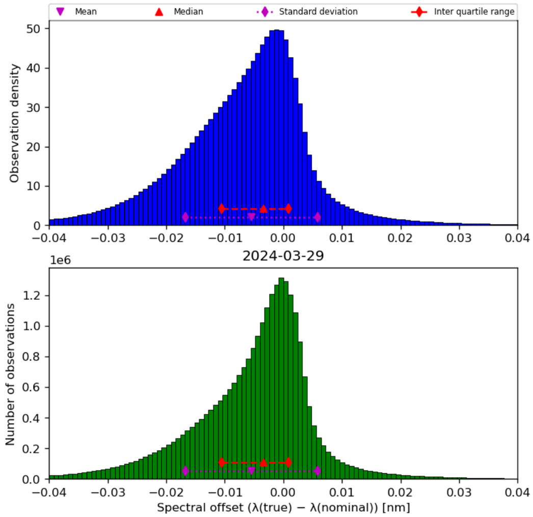
Figure 45: Histogram of “Spectral offset ( \lambda(\text{true}) - \lambda(\text{nominal}) )” for 2024-03-28 to 2024-03-30
