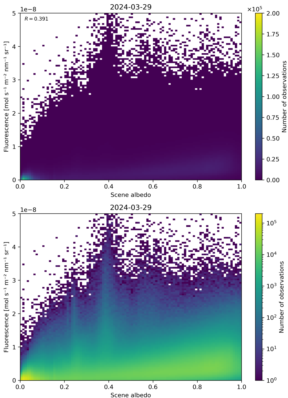
Figure 104: Scatter density plot of “Scene albedo” against “Fluorescence” for 2024-03-28 to 2024-03-30.
