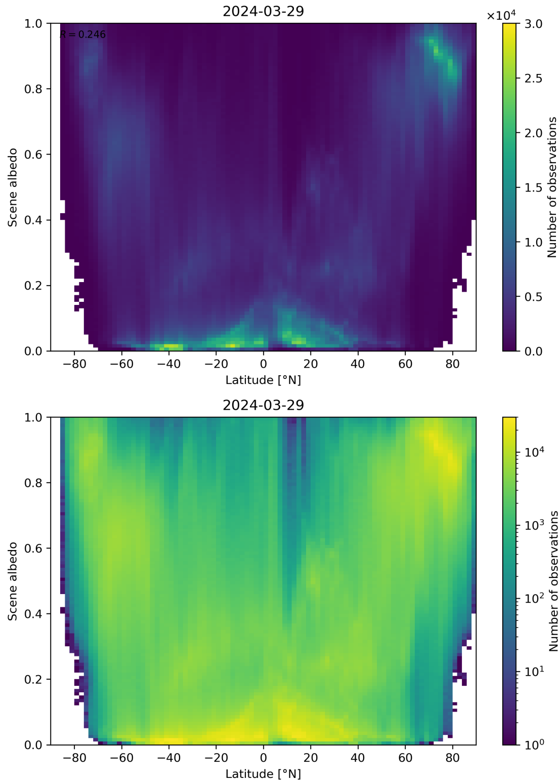
Figure 95: Scatter density plot of “Latitude” against “Scene albedo” for 2024-03-28 to 2024-03-30.
