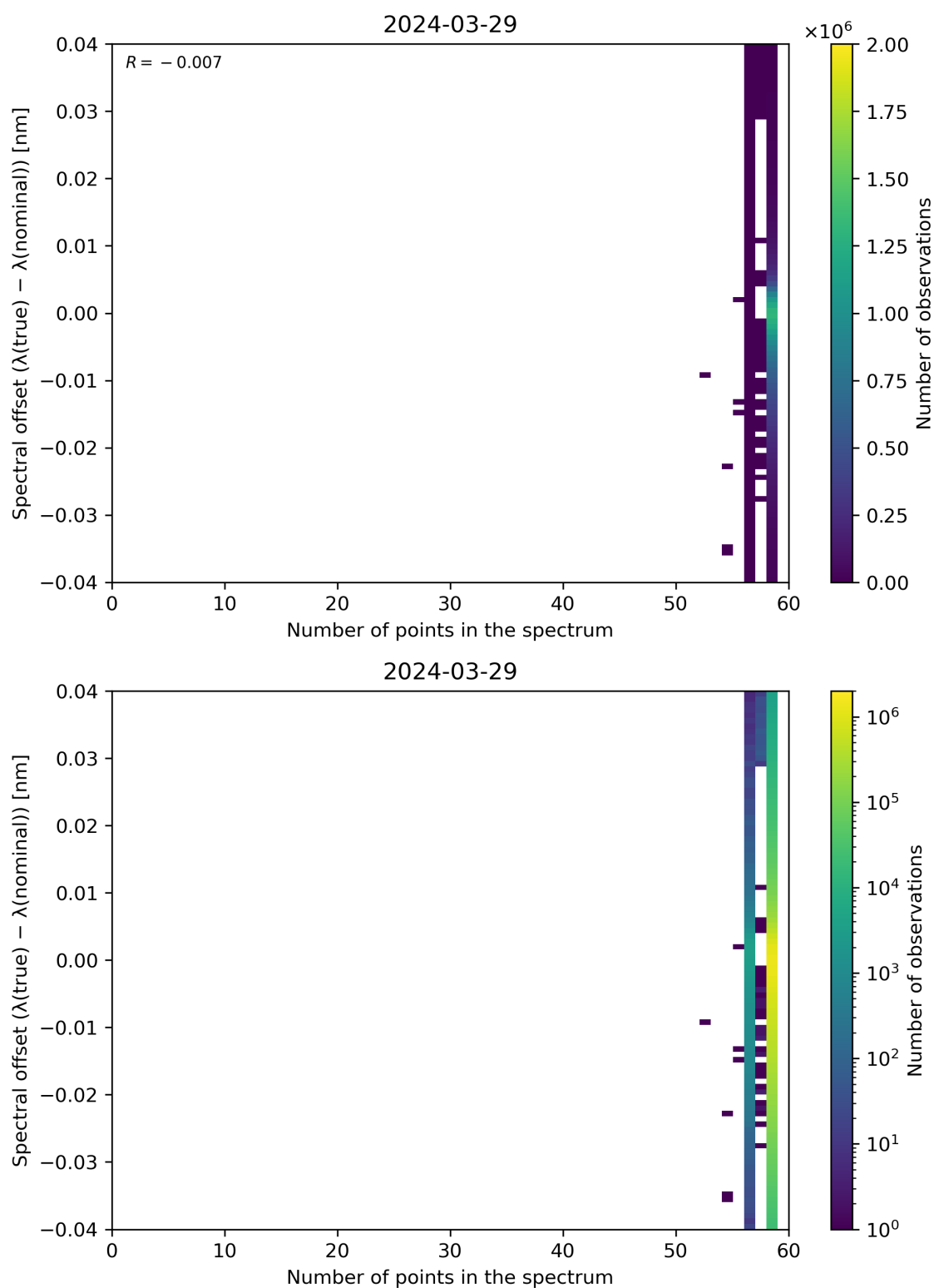
Figure 101: Scatter density plot of “Number of points in the spectrum” against “Spectral offset ( \lambda(\text{true}) - \lambda(\text{nominal}) )” for 2024-03-28 to 2024-03-30.
