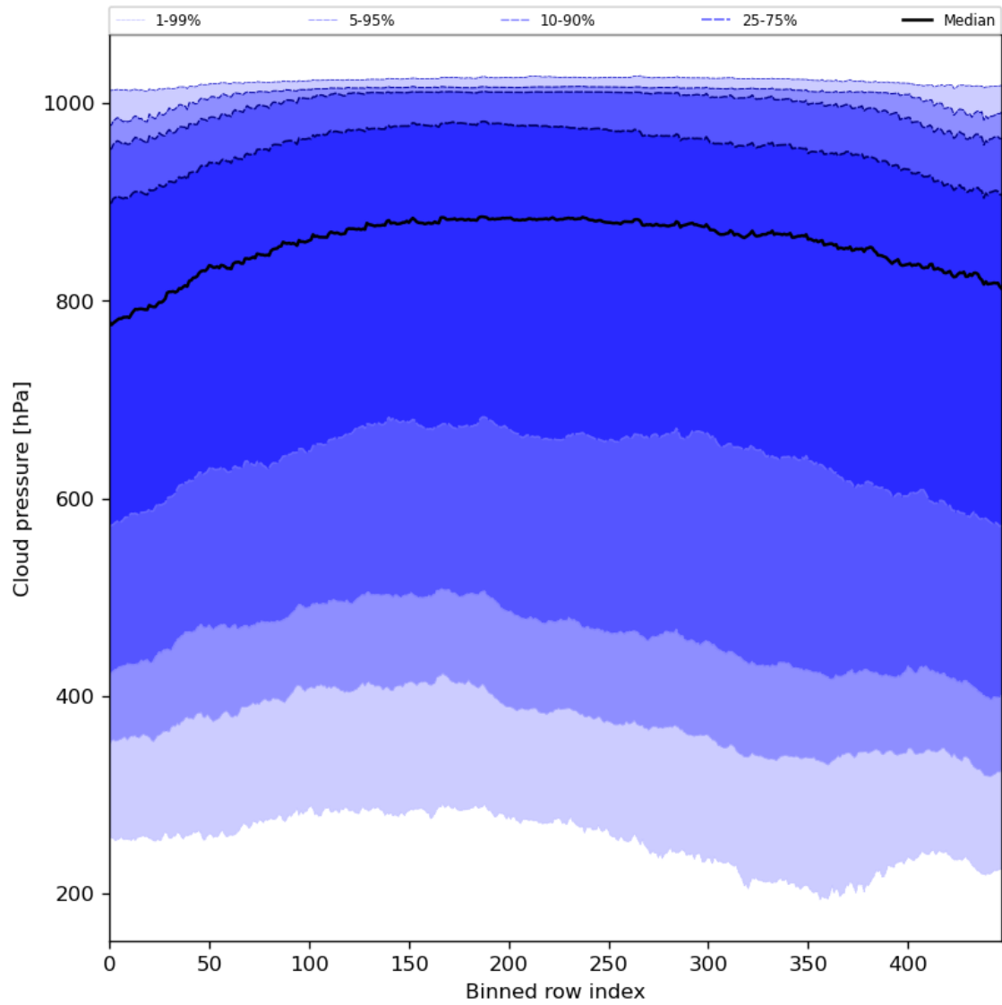
Figure 47: Along track statistics of “Cloud pressure” for 2024-03-28 to 2024-03-30
