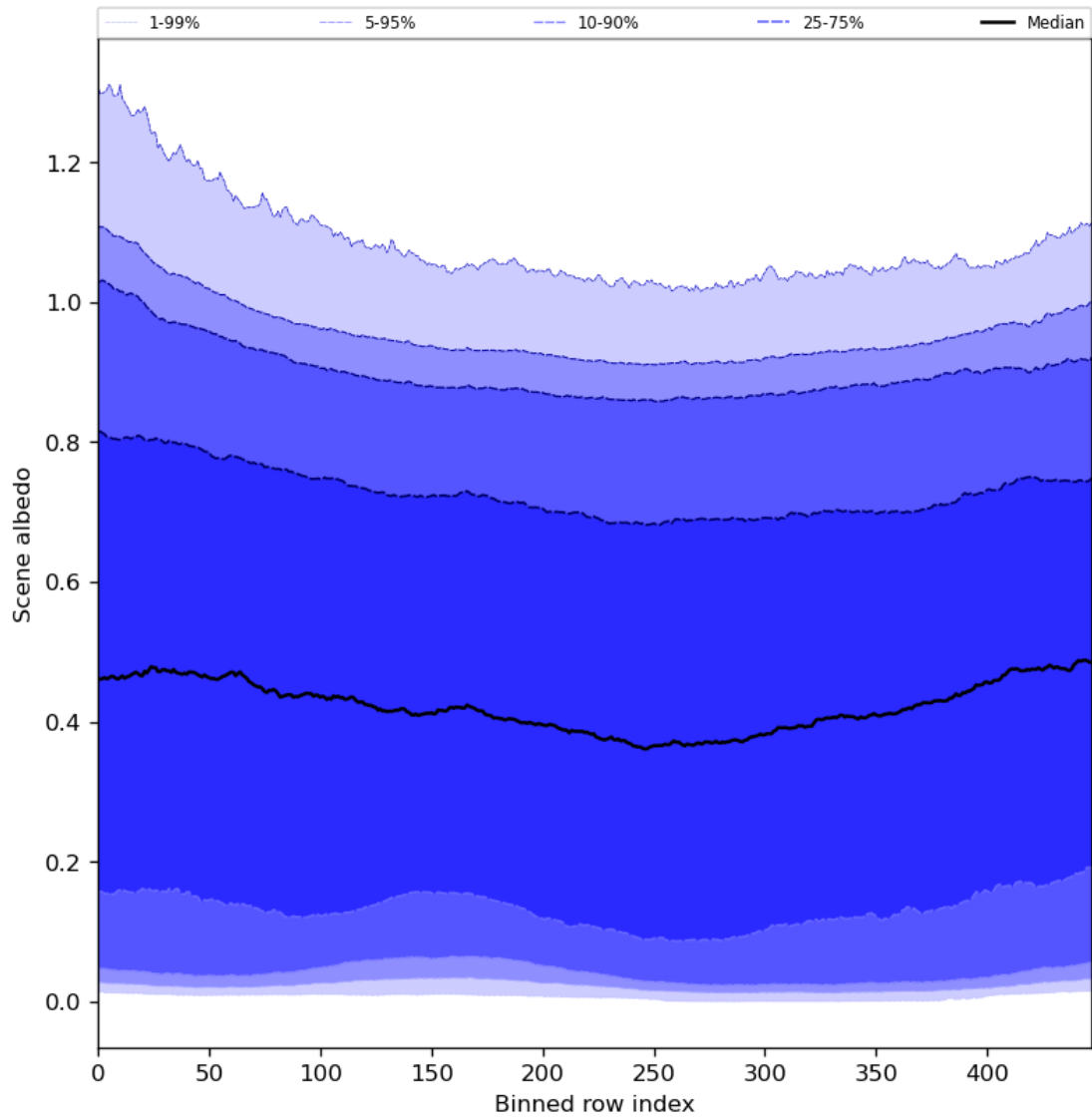
Figure 51: Along track statistics of “Scene albedo” for 2024-03-28 to 2024-03-30
