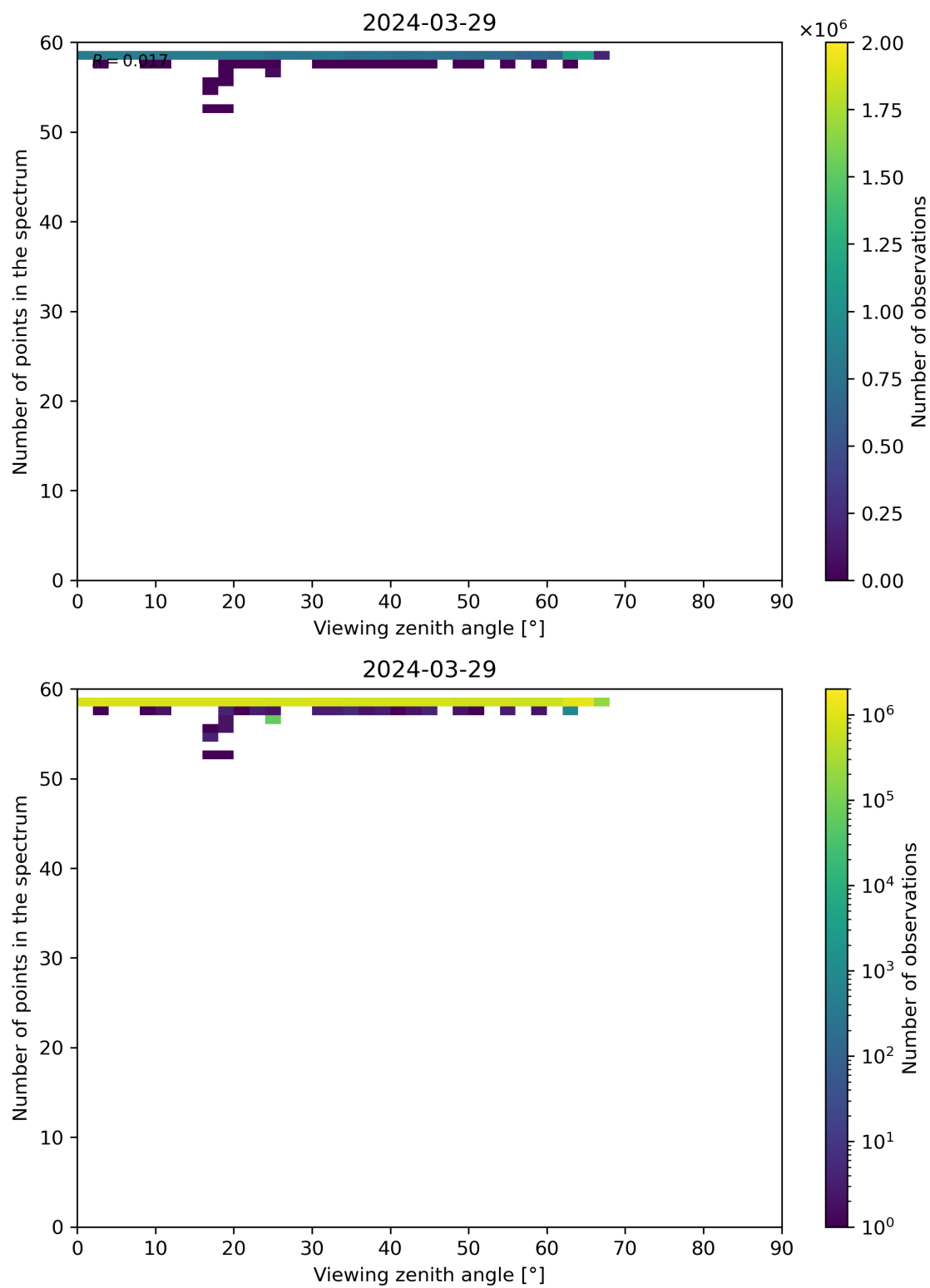
Figure 125: Scatter density plot of “Viewing zenith angle” against “Number of points in the spectrum” for 2024-03-28 to 2024-03-30.
