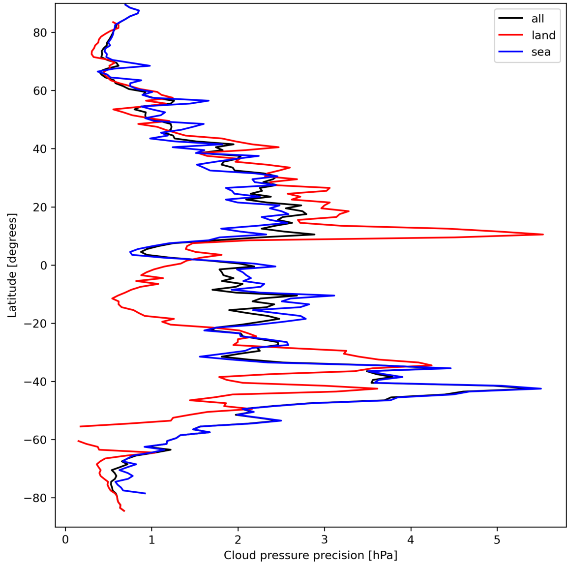
Figure 14: Zonal average of “Cloud pressure precision” for 2024-03-28 to 2024-03-30.
