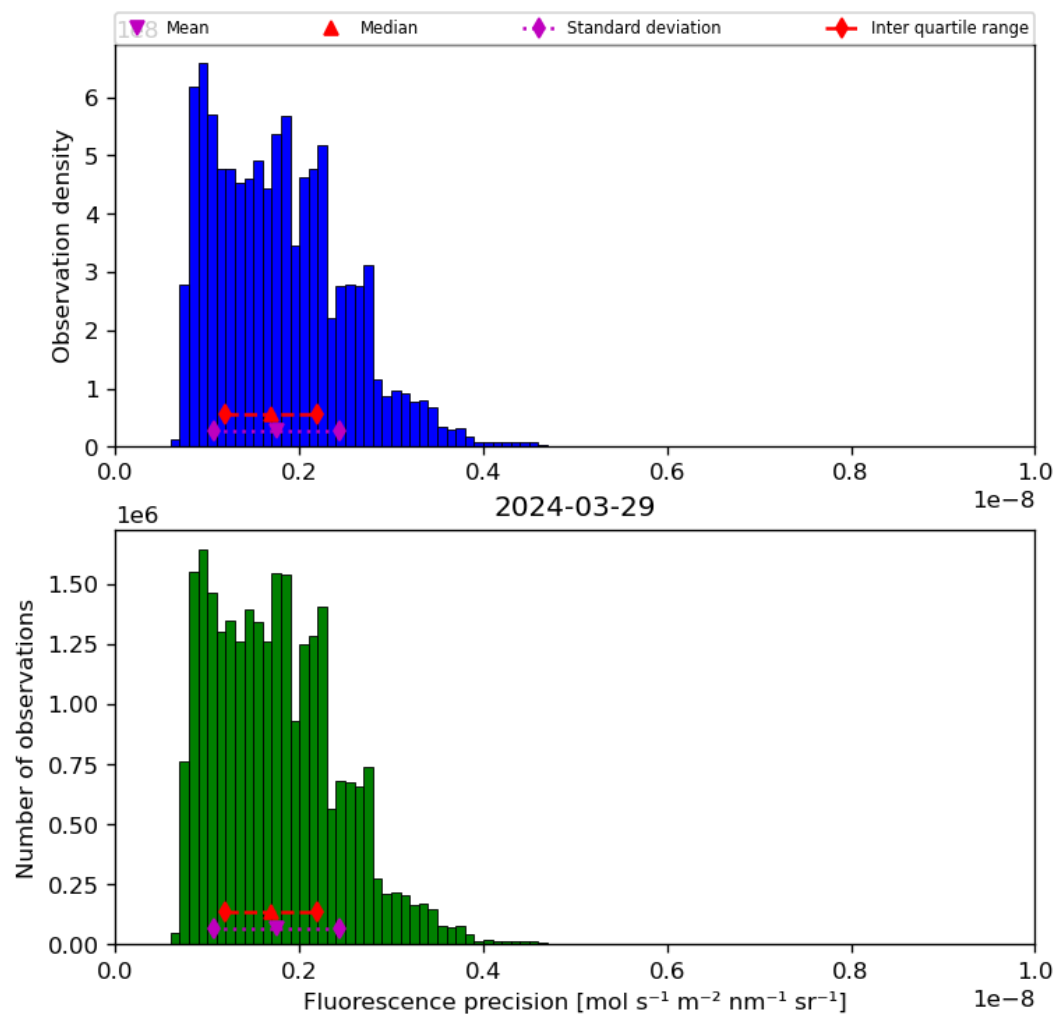
Figure 41: Histogram of “Fluorescence precision” for 2024-03-28 to 2024-03-30
