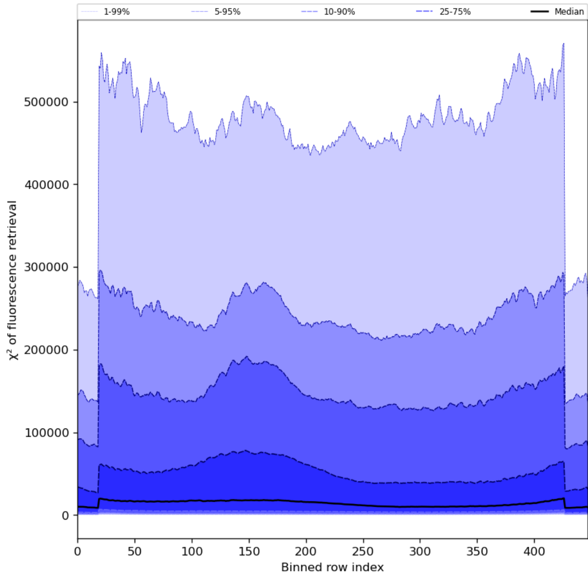
Figure 59: Along track statistics of “ \chi^2 of fluorescence retrieval” for 2024-03-30 to 2024-03-31
