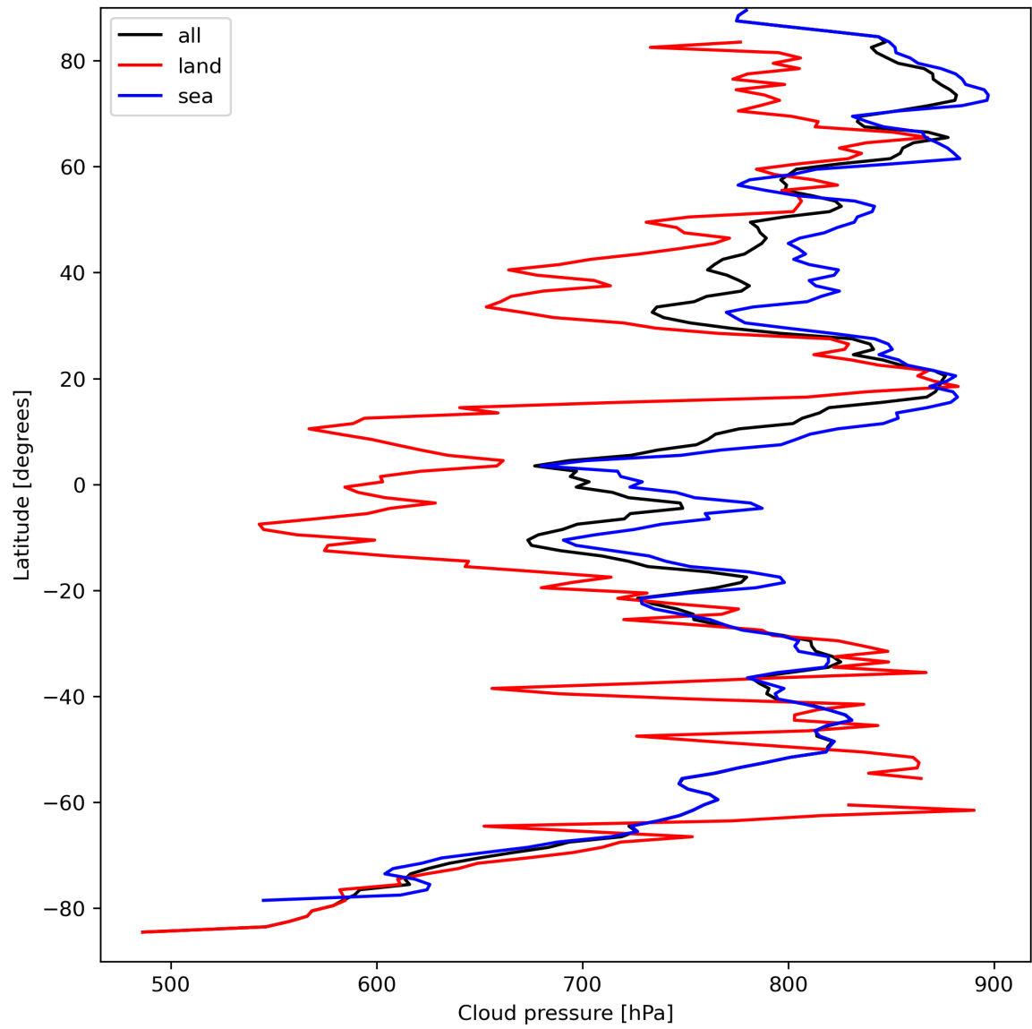
Figure 13: Zonal average of “Cloud pressure” for 2024-03-30 to 2024-03-31.
