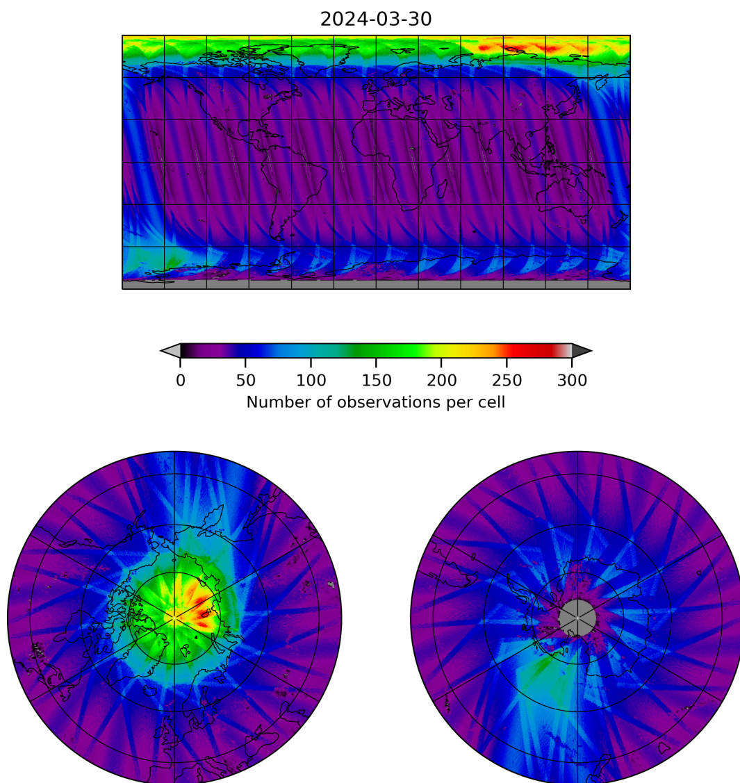
Figure 11: Map of the number of observations for 2024-03-30 to 2024-03-31
