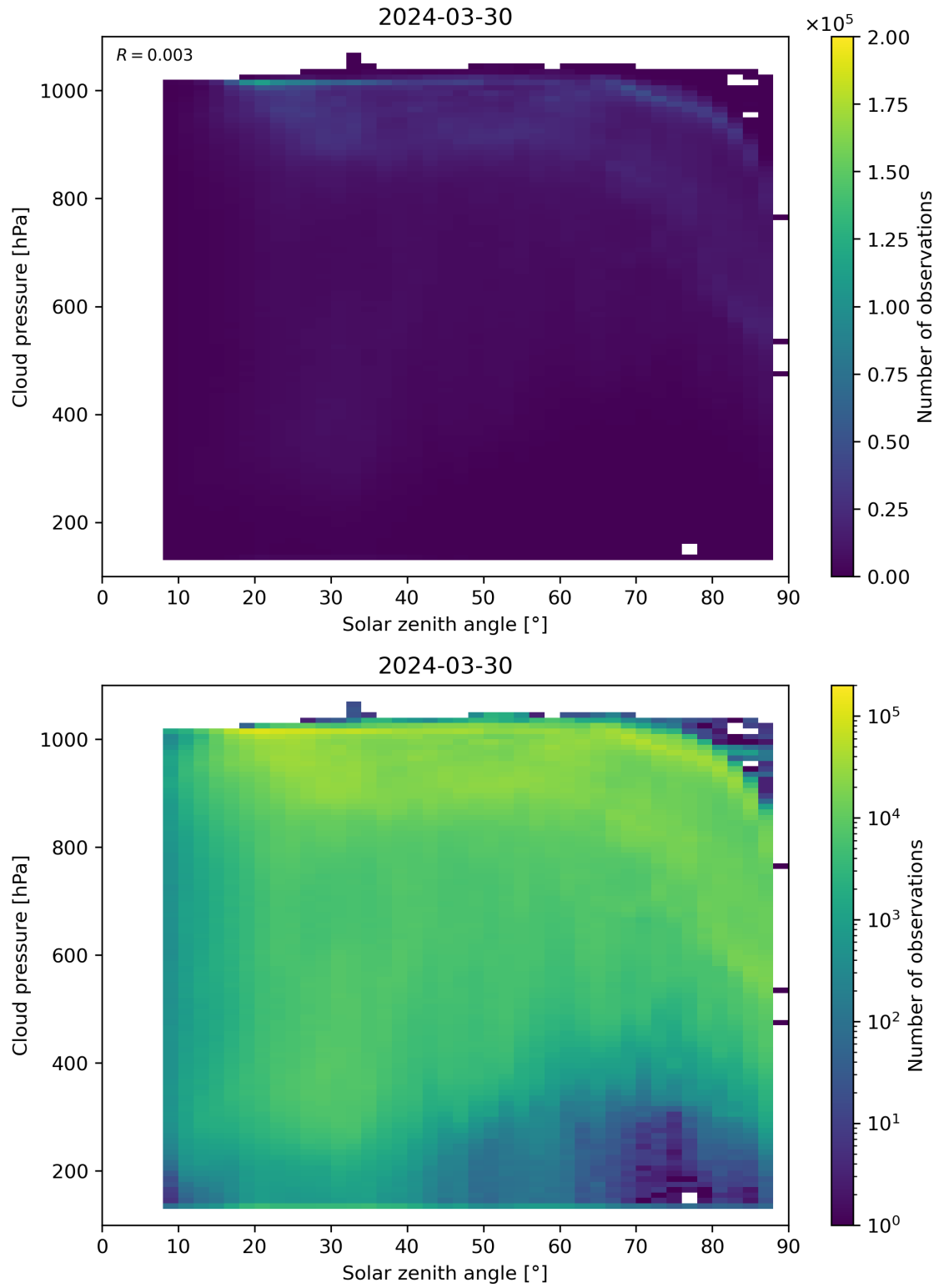
Figure 111: Scatter density plot of “Solar zenith angle” against “Cloud pressure” for 2024-03-30 to 2024-03-31.
