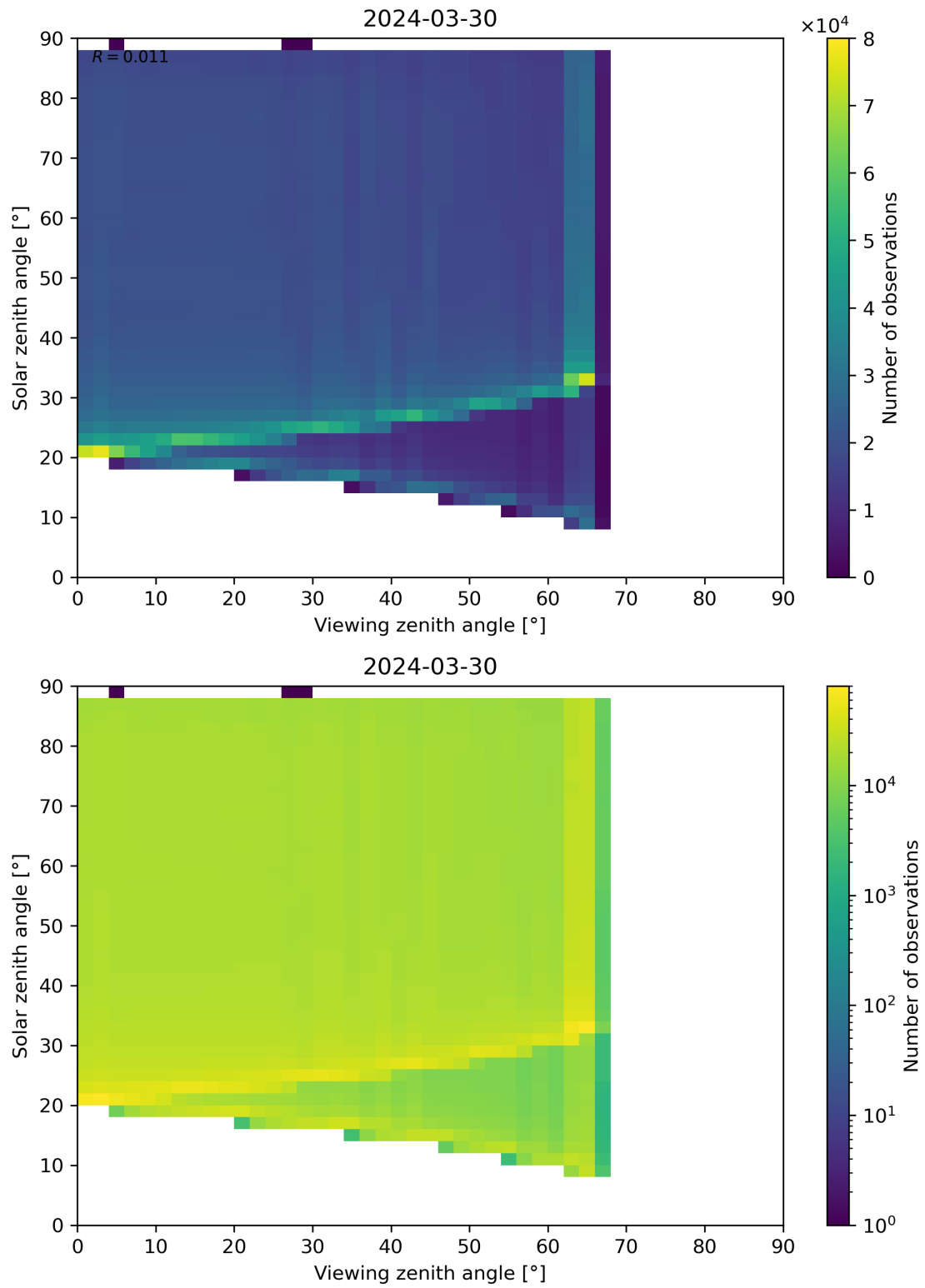
Figure 127: Scatter density plot of “Viewing zenith angle” against “Solar zenith angle” for 2024-03-30 to 2024-03-31.
