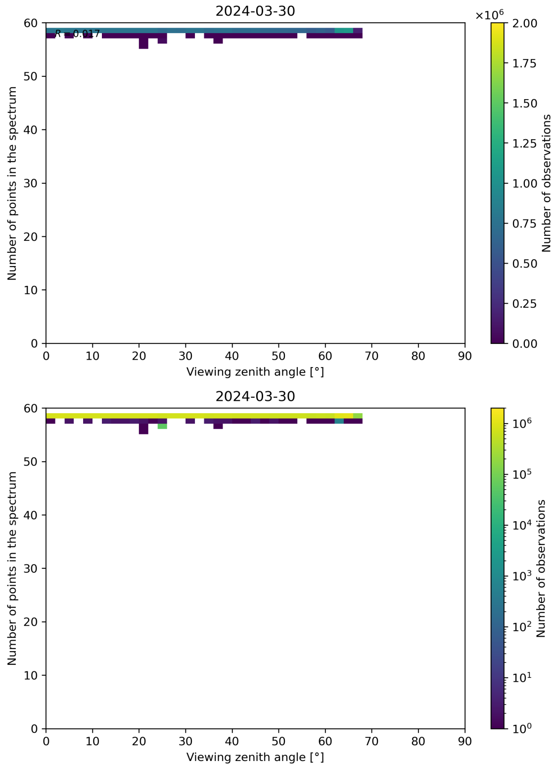
Figure 125: Scatter density plot of “Viewing zenith angle” against “Number of points in the spectrum” for 2024-03-30 to 2024-03-31.
