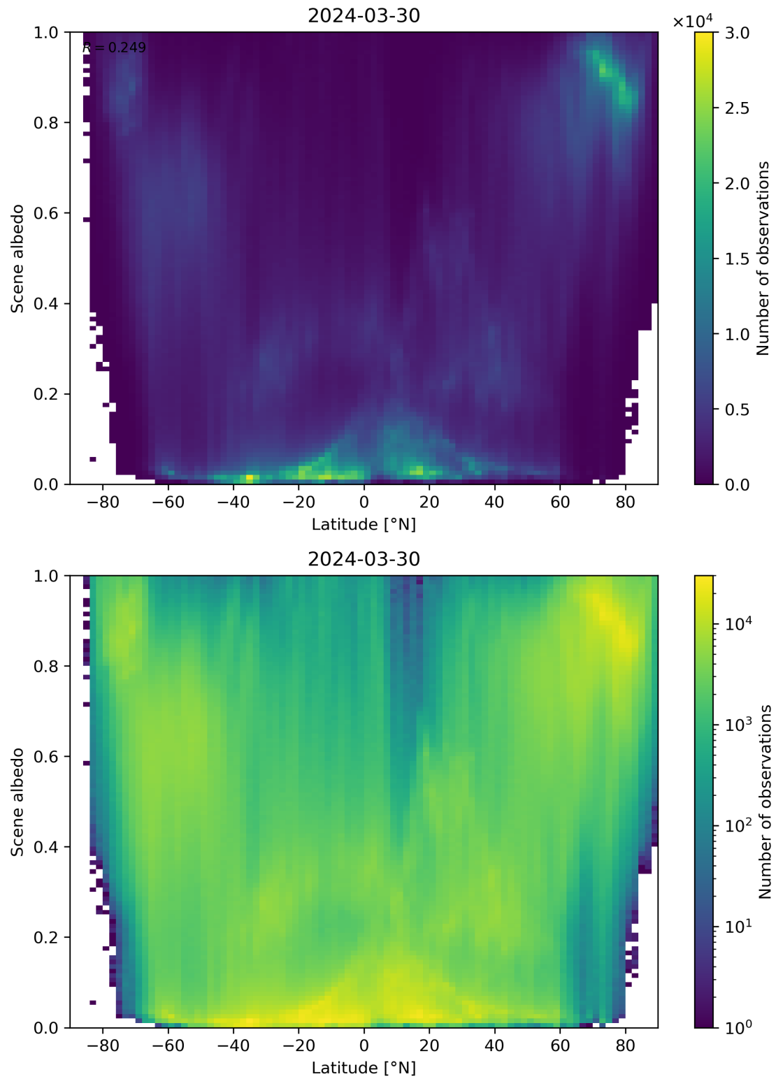
Figure 95: Scatter density plot of “Latitude” against “Scene albedo” for 2024-03-30 to 2024-03-31.
