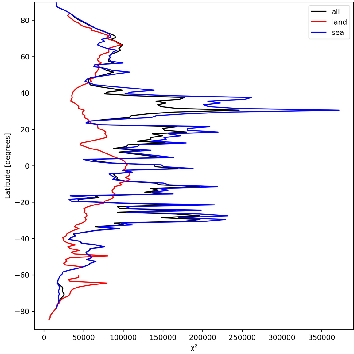
Figure 21: Zonal average of “ \chi^2 ” for 2024-03-30 to 2024-03-31.
