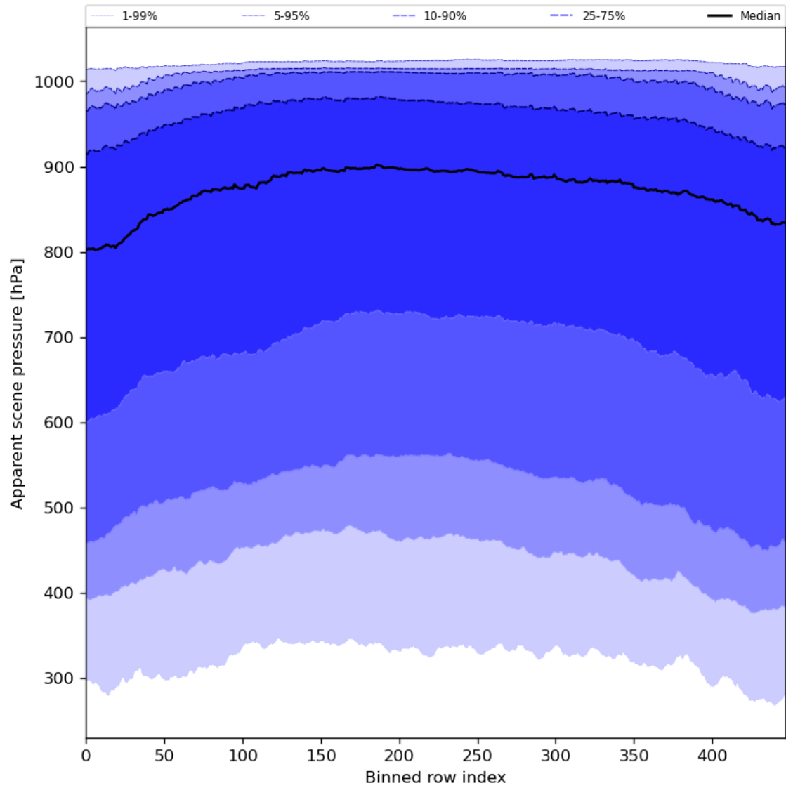
Figure 53: Along track statistics of “Apparent scene pressure” for 2024-03-30 to 2024-03-31
