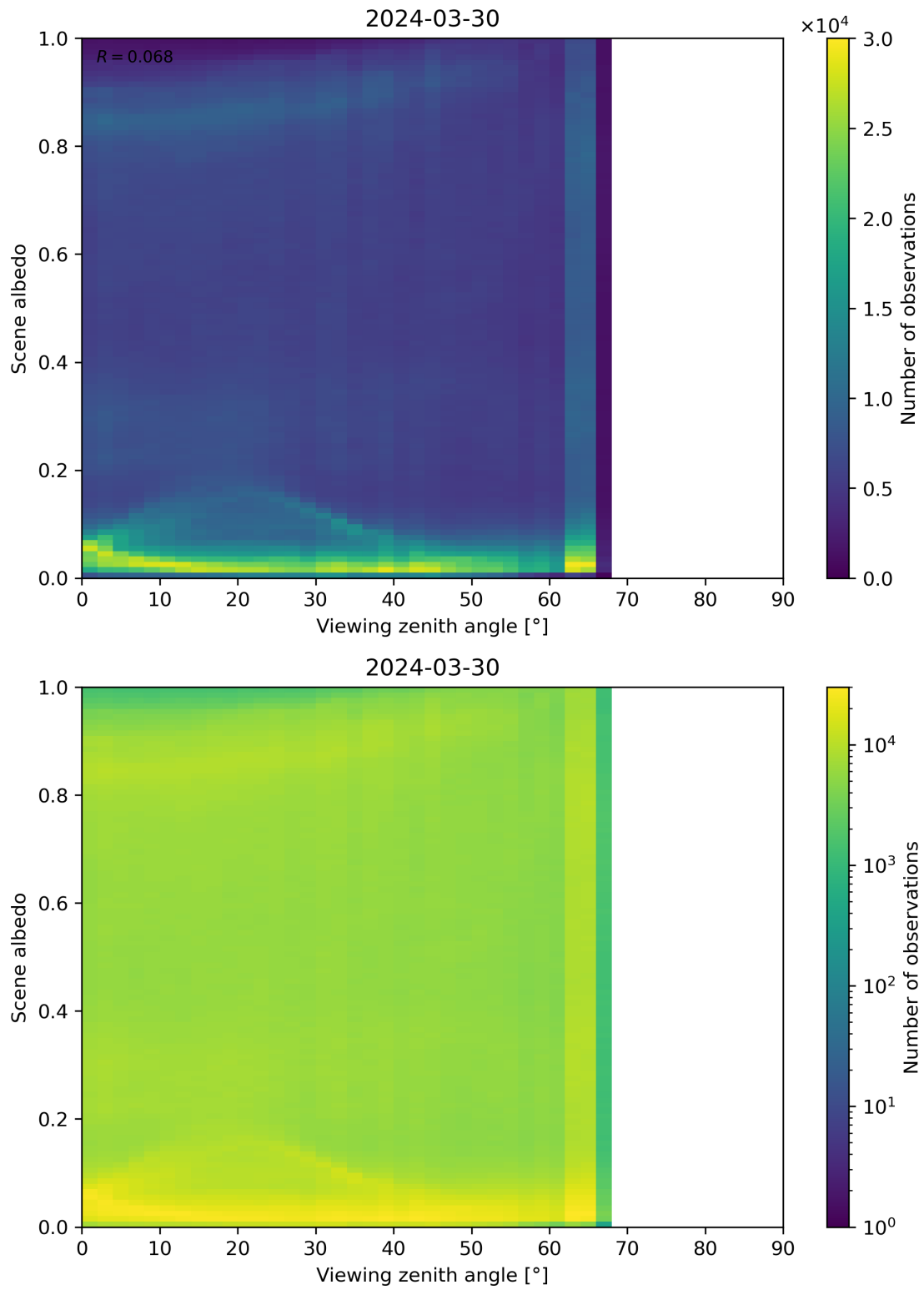
Figure 126: Scatter density plot of “Viewing zenith angle” against “Scene albedo” for 2024-03-30 to 2024-03-31.
