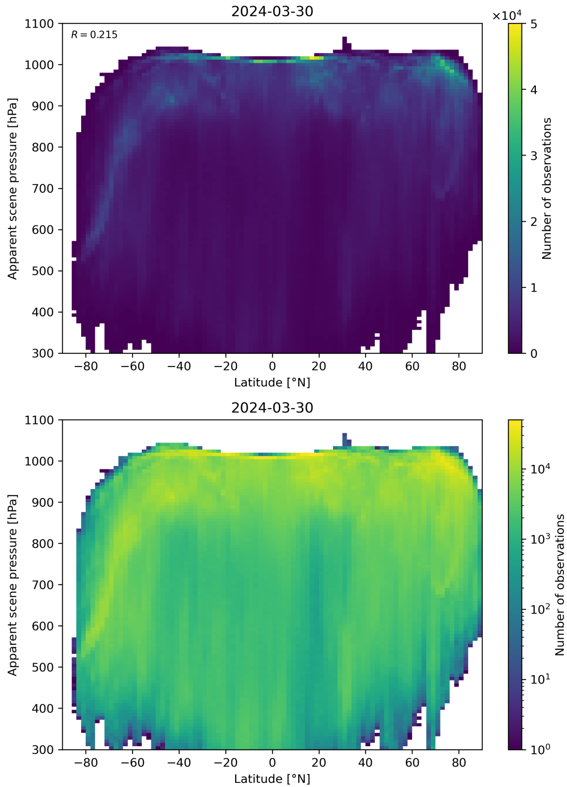
Figure 88: Scatter density plot of “Latitude” against “Apparent scene pressure” for 2024-03-30 to 2024-03-31.
