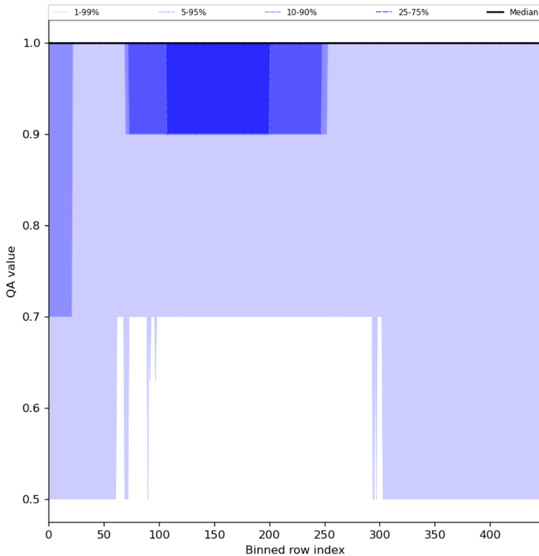
Figure 46: Along track statistics of “QA value” for 2024-03-30 to 2024-03-31
