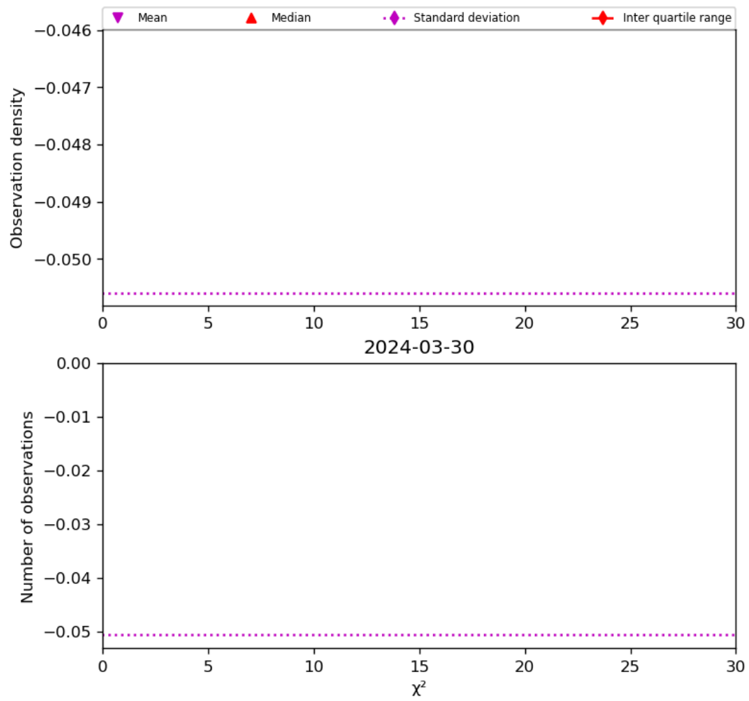
Figure 38: Histogram of “ \chi^2 ” for 2024-03-30 to 2024-03-31
