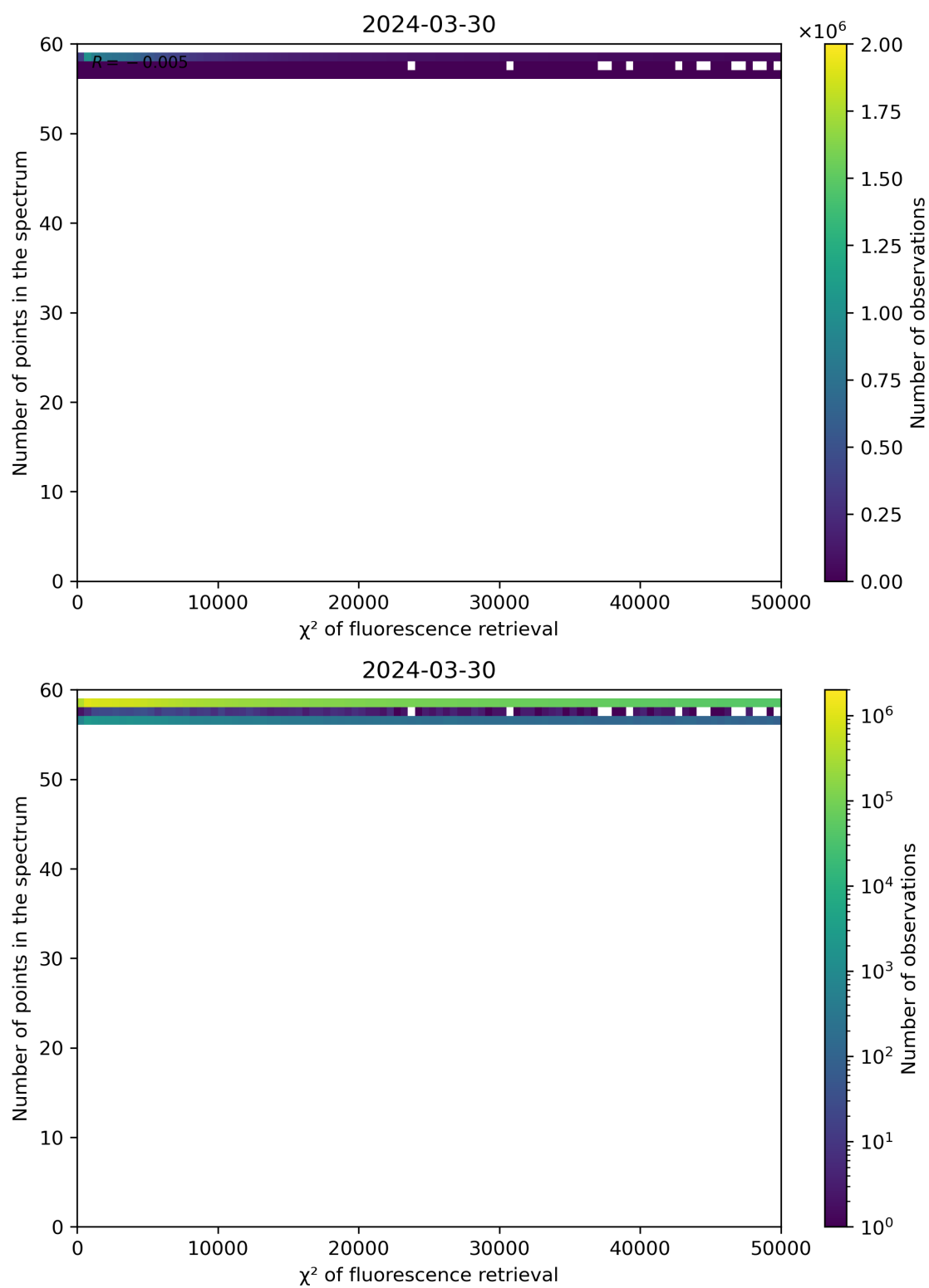
Figure 68: Scatter density plot of “ \chi^2 of fluorescence retrieval” against “Number of points in the spectrum” for 2024-03-30 to 2024-03-31.
