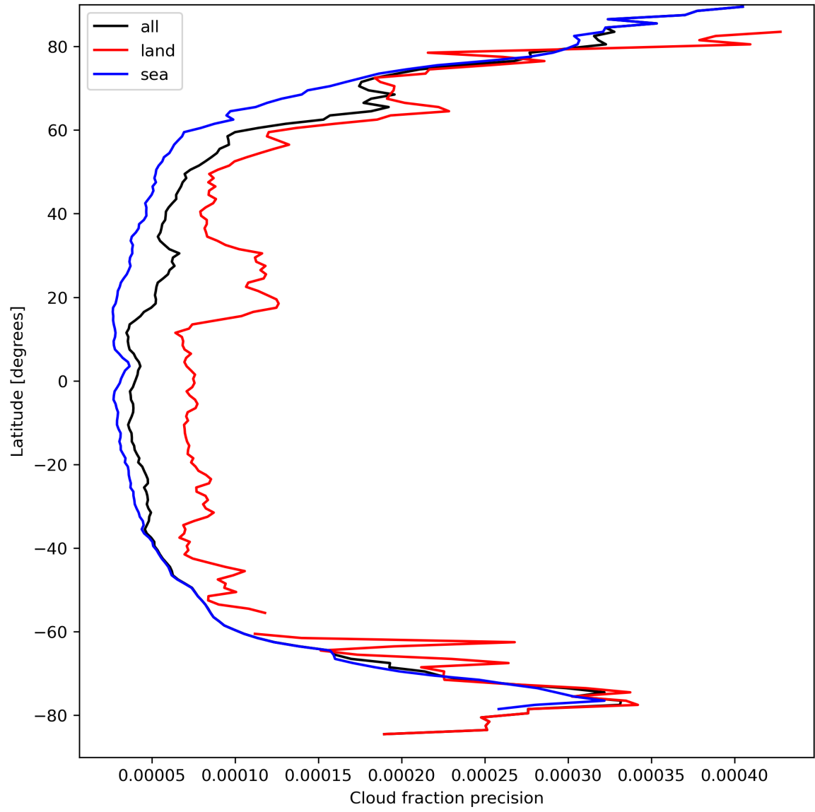
Figure 16: Zonal average of “Cloud fraction precision” for 2024-03-30 to 2024-03-31.
