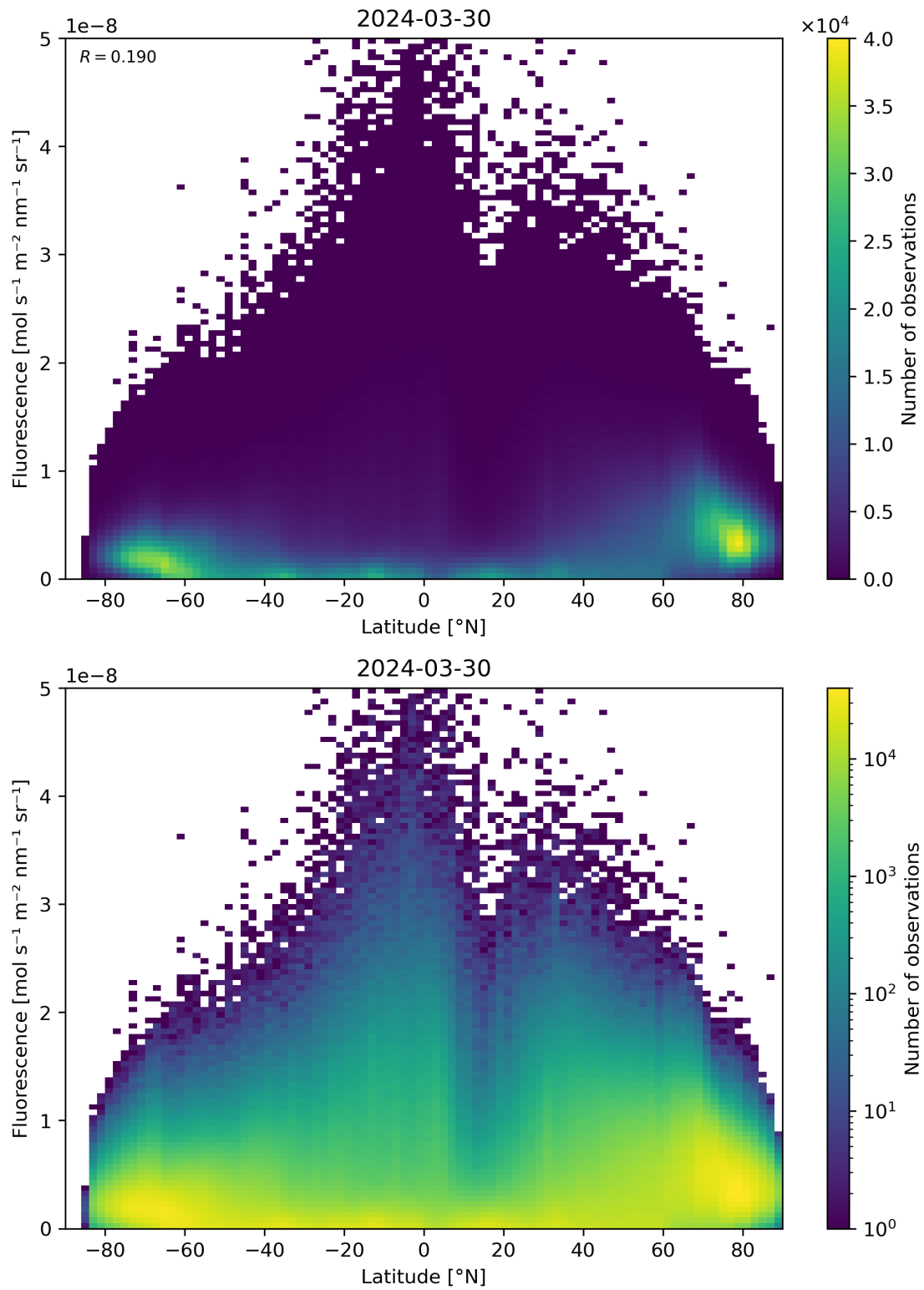
Figure 92: Scatter density plot of “Latitude” against “Fluorescence” for 2024-03-30 to 2024-03-31.
