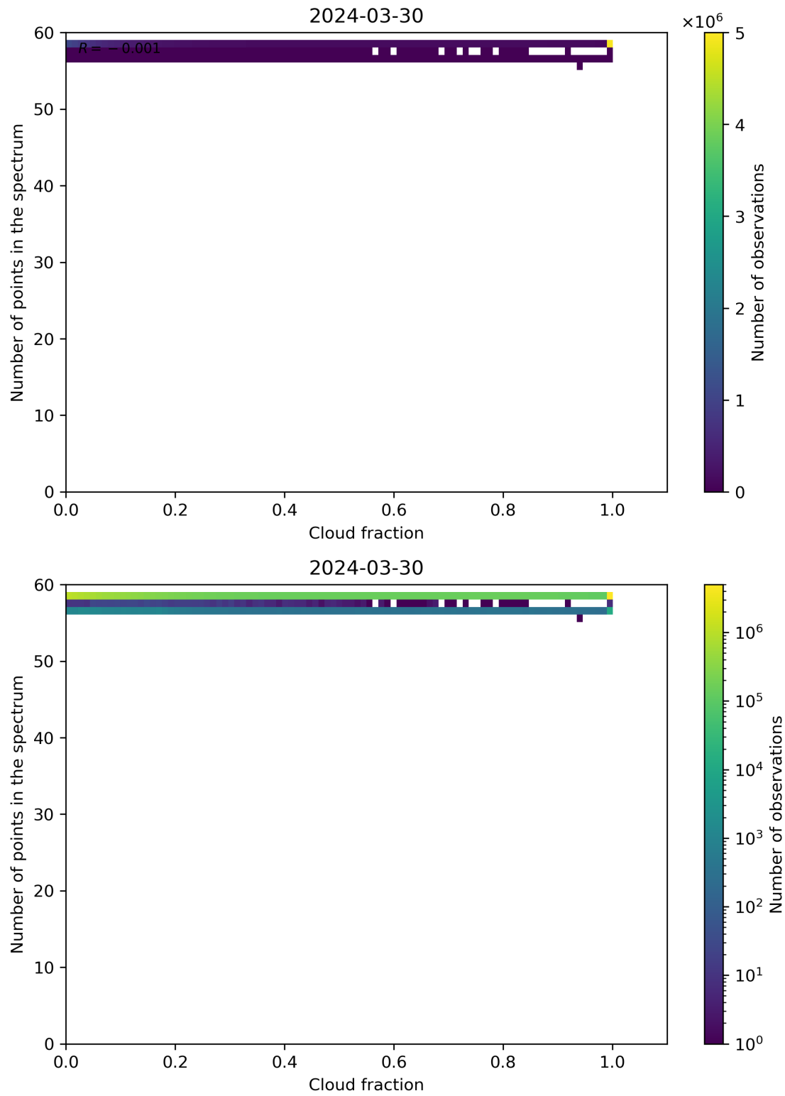
Figure 74: Scatter density plot of “Cloud fraction” against “Number of points in the spectrum” for 2024-03-30 to 2024-03-31.
