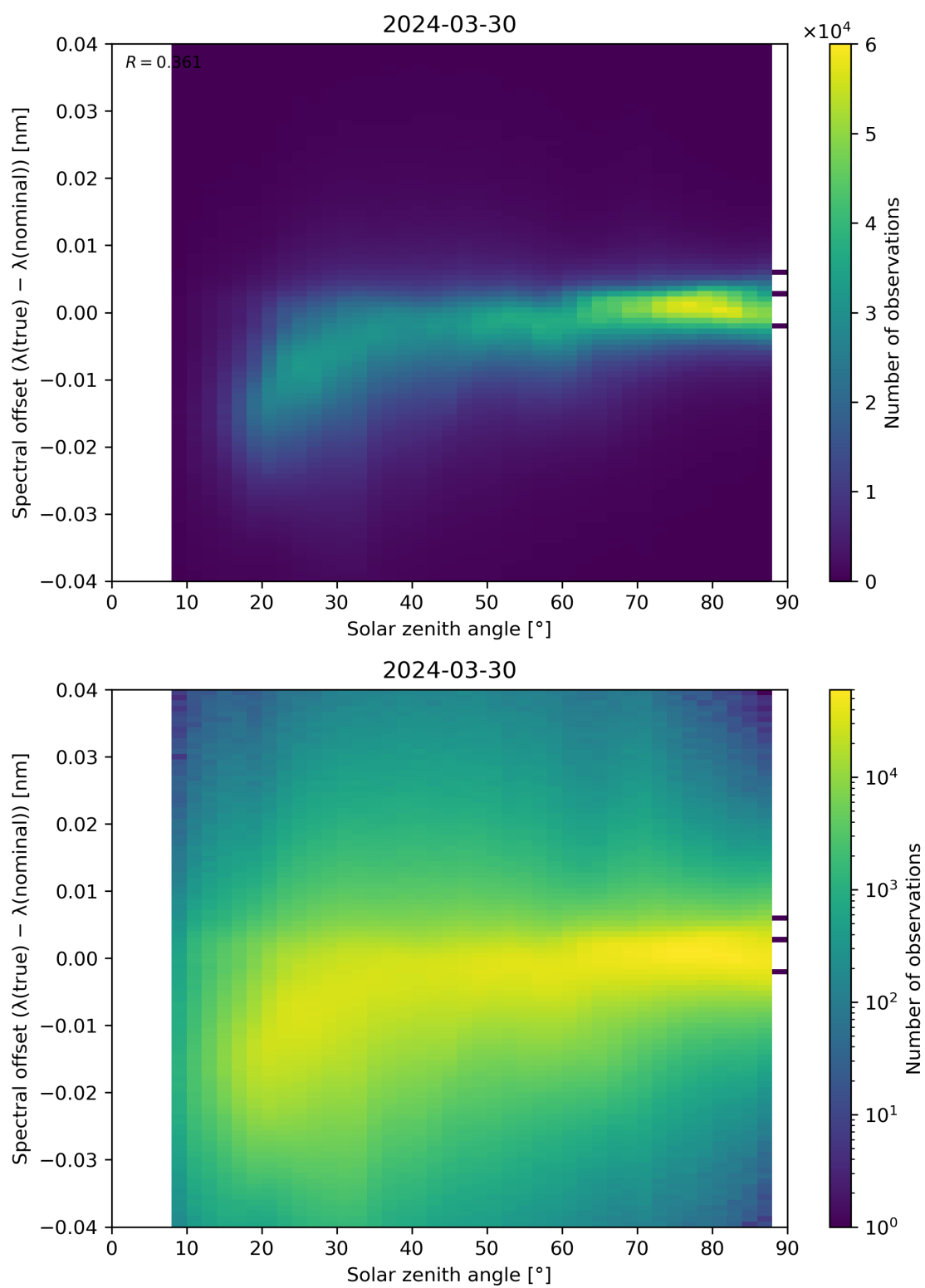
Figure 117: Scatter density plot of “Solar zenith angle” against “Spectral offset ( \lambda(\text{true}) - \lambda(\text{nominal}) )” for 2024-03-30 to 2024-03-31.
