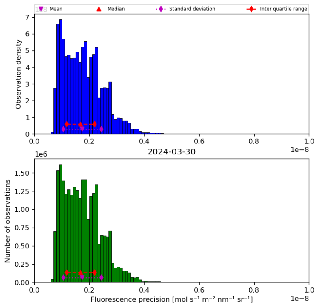
Figure 41: Histogram of “Fluorescence precision” for 2024-03-30 to 2024-03-31
