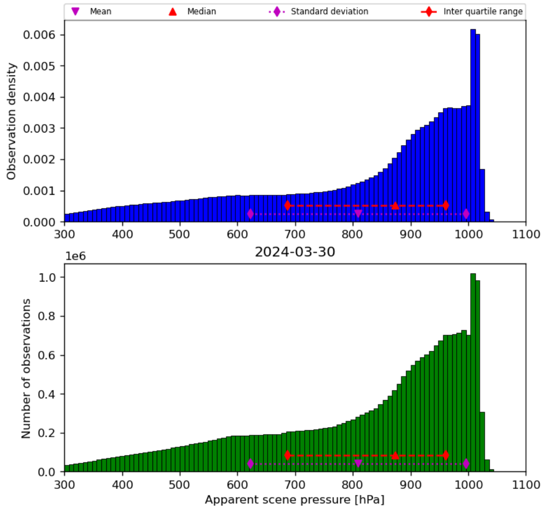
Figure 36: Histogram of “Apparent scene pressure” for 2024-03-30 to 2024-03-31
