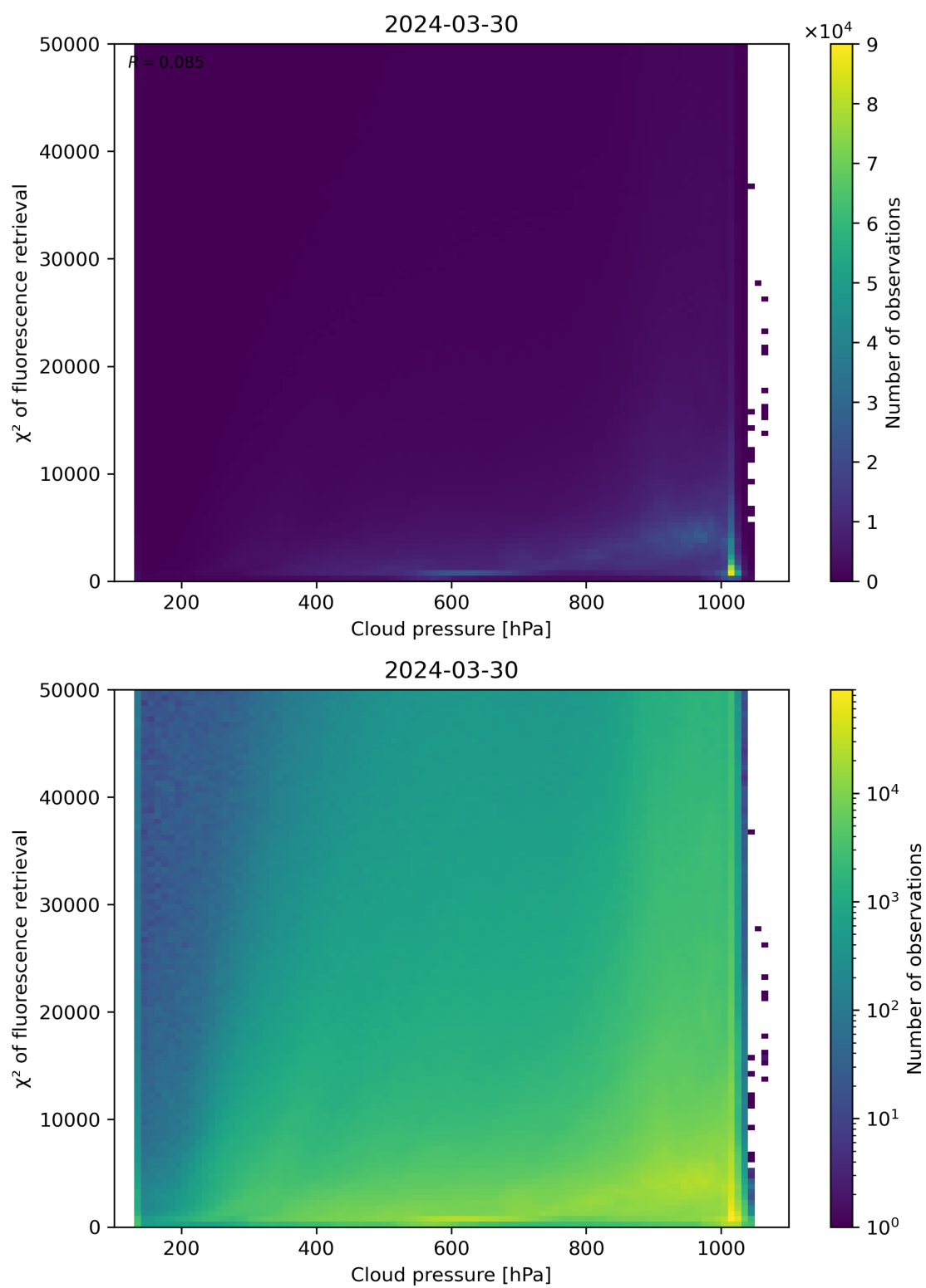
Figure 78: Scatter density plot of “Cloud pressure” against “ \chi^2 of fluorescence retrieval” for 2024-03-30 to 2024-03-31.
