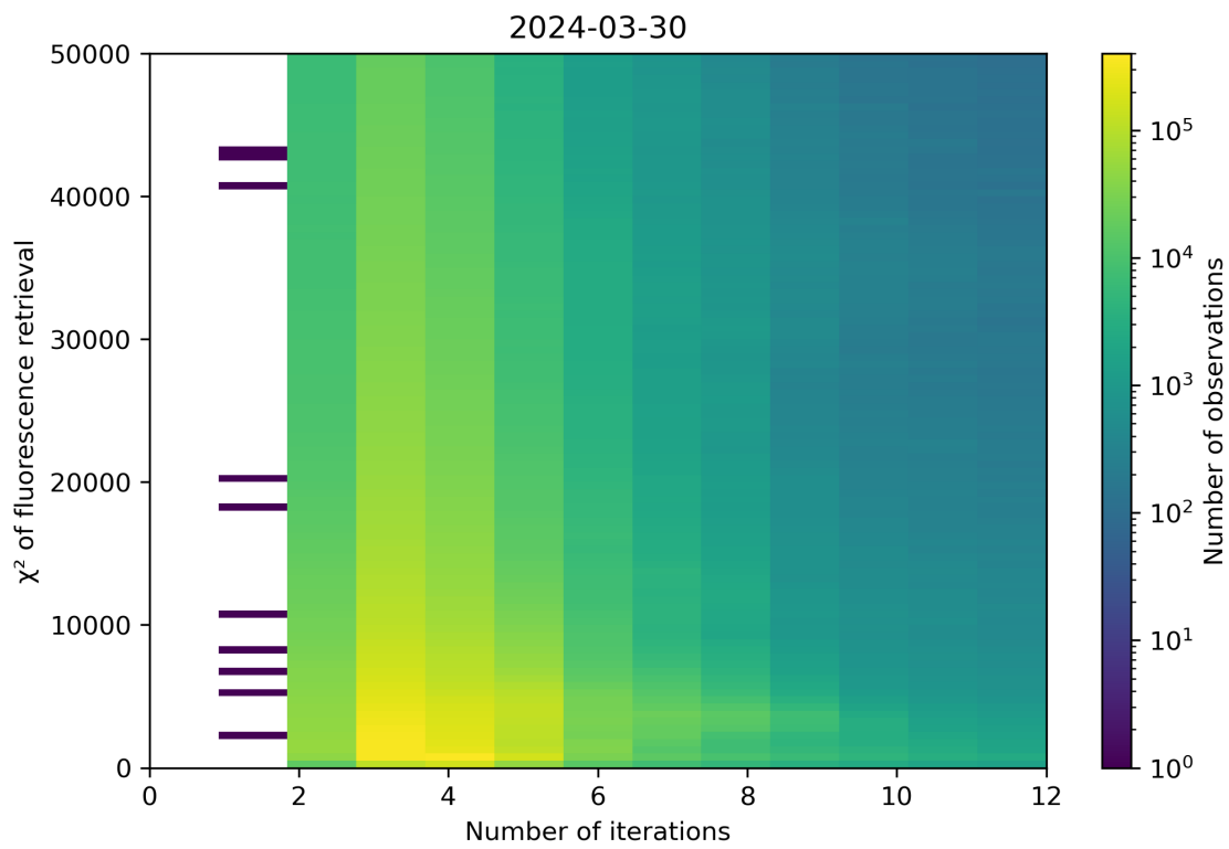
Figure 97: Scatter density plot of “Number of iterations” against “ \chi^2 of fluorescence retrieval” for 2024-03-30 to 2024-03-31.
