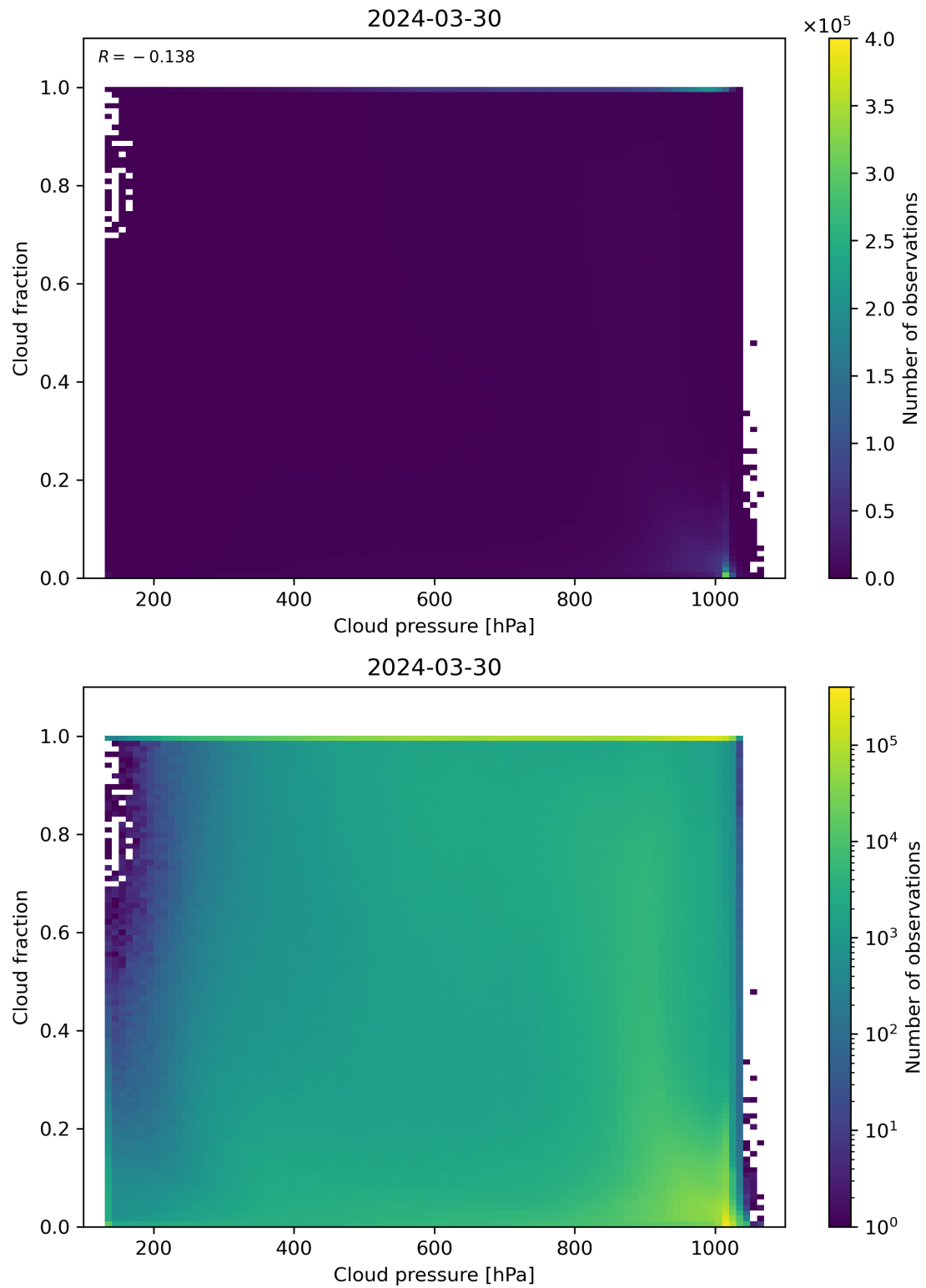
Figure 79: Scatter density plot of “Cloud pressure” against “Cloud fraction” for 2024-03-30 to 2024-03-31.
