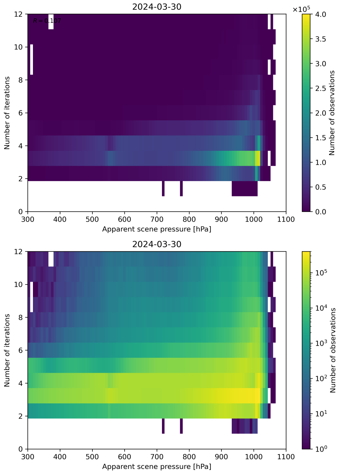
Figure 65: Scatter density plot of “Apparent scene pressure” against “Number of iterations” for 2024-03-30 to 2024-03-31.
