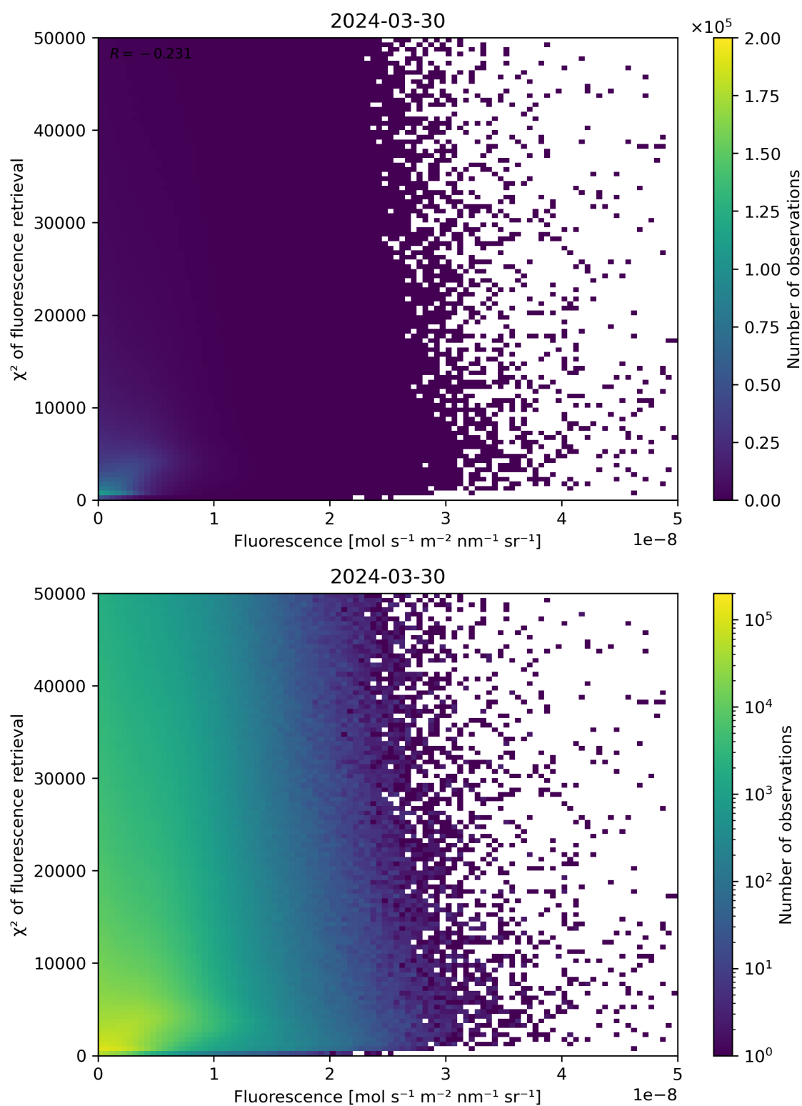
Figure 85: Scatter density plot of “Fluorescence” against “ \chi^2 of fluorescence retrieval” for 2024-03-30 to 2024-03-31.
