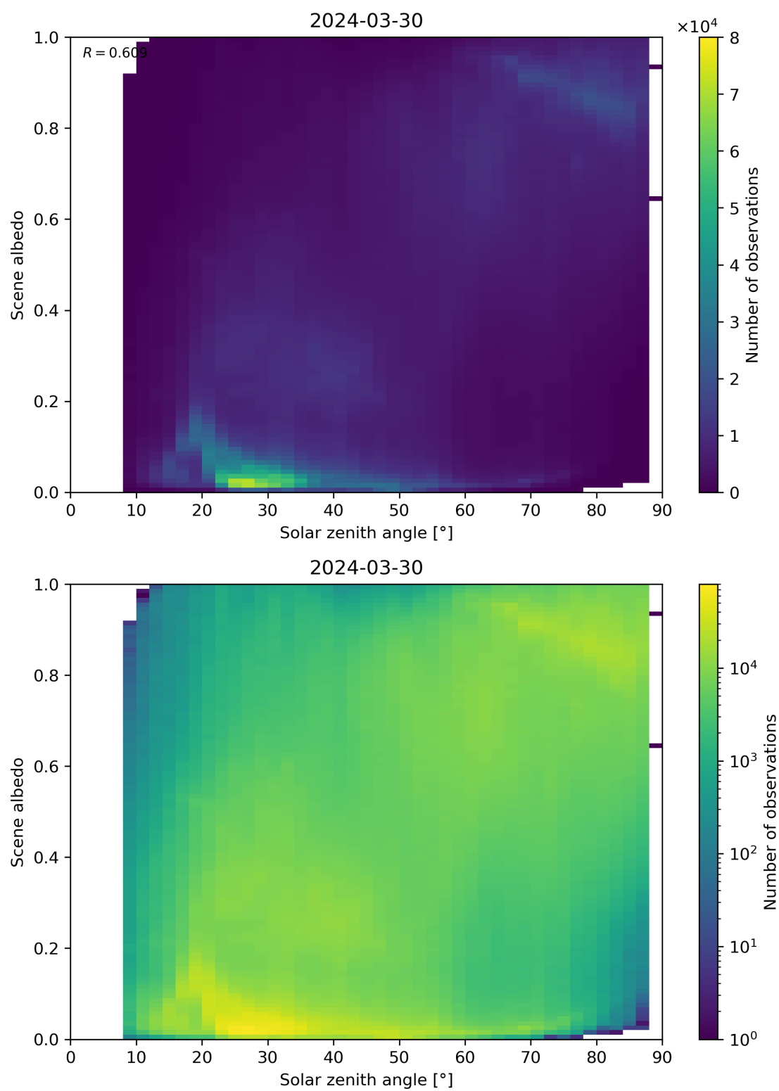
Figure 116: Scatter density plot of “Solar zenith angle” against “Scene albedo” for 2024-03-30 to 2024-03-31.
