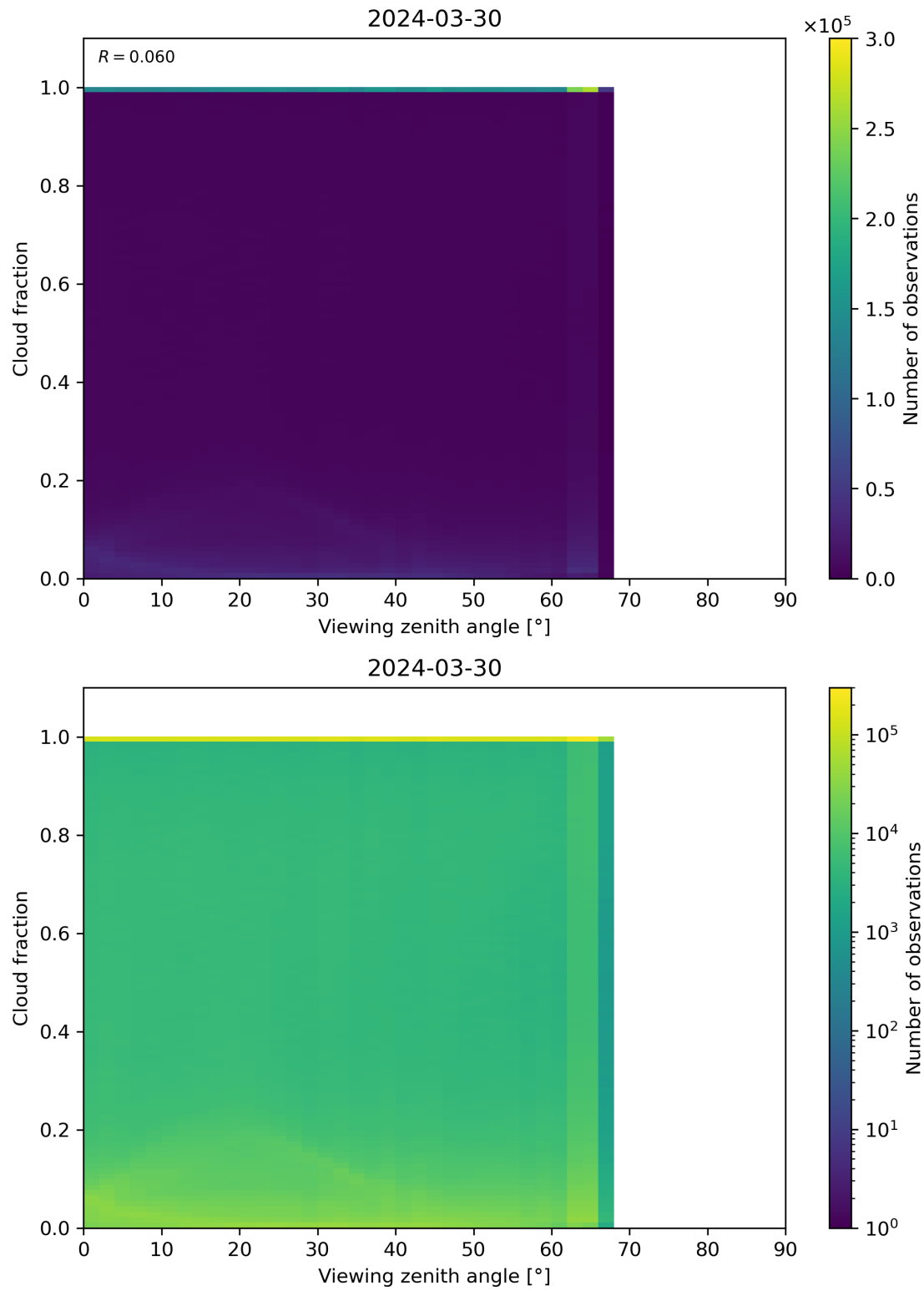
Figure 120: Scatter density plot of “Viewing zenith angle” against “Cloud fraction” for 2024-03-30 to 2024-03-31.
