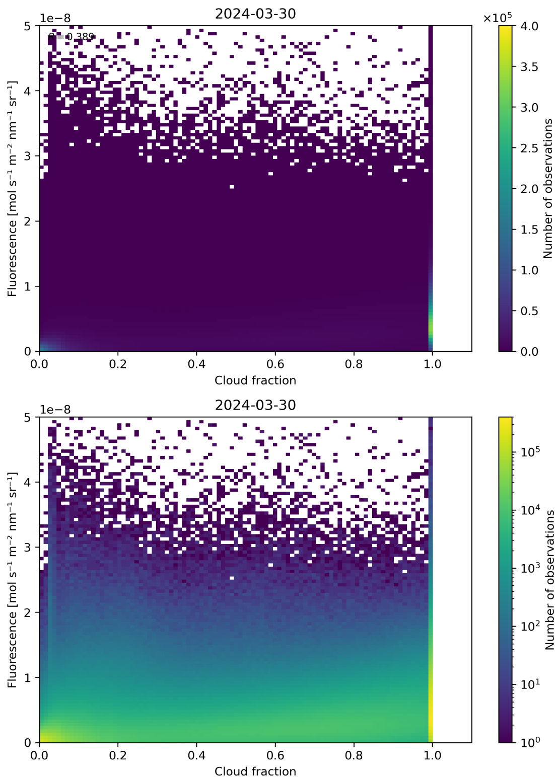
Figure 72: Scatter density plot of “Cloud fraction” against “Fluorescence” for 2024-03-30 to 2024-03-31.
