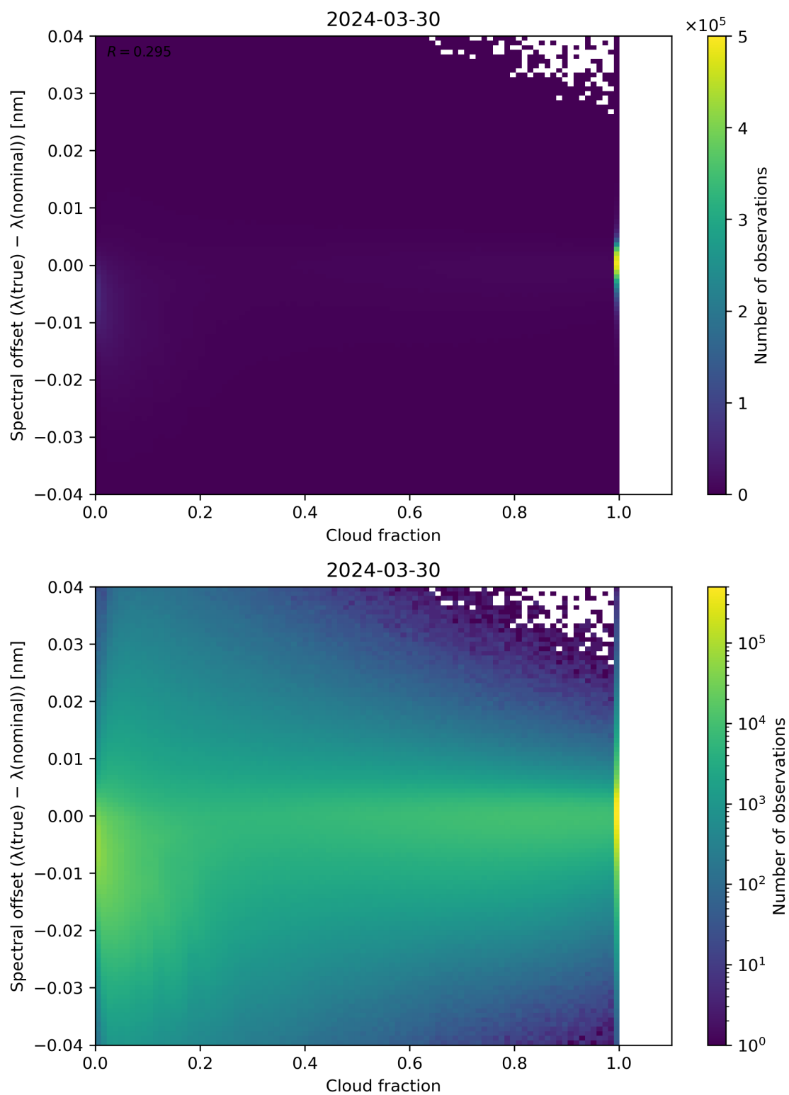
Figure 76: Scatter density plot of “Cloud fraction” against “Spectral offset ( \lambda(\text{true}) - \lambda(\text{nominal}) )” for 2024-03-30 to 2024-03-31.
