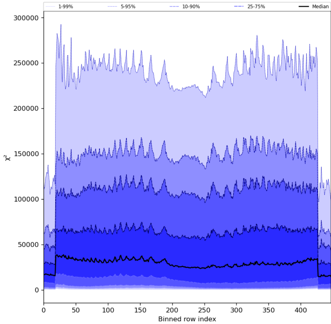
Figure 55: Along track statistics of " \chi^2 " for 2024-03-30 to 2024-03-31
