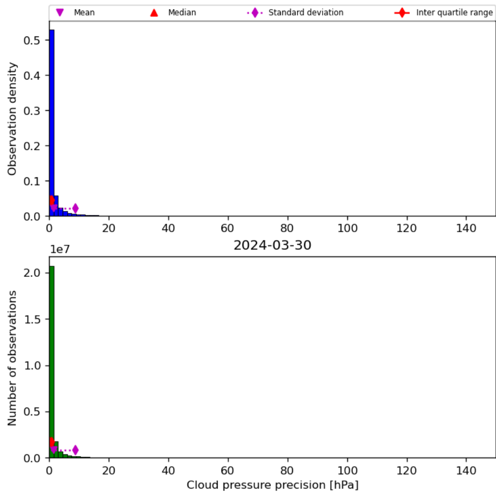
Figure 31: Histogram of “Cloud pressure precision” for 2024-03-30 to 2024-03-31
