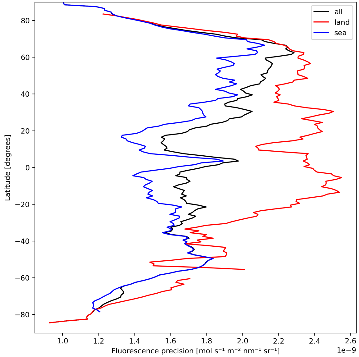
Figure 24: Zonal average of “Fluorescence precision” for 2024-03-30 to 2024-03-31.
