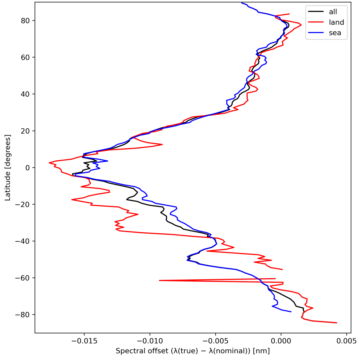
Figure 28: Zonal average of “Spectral offset ( \lambda(\text{true}) - \lambda(\text{nominal}) )” for 2024-03-30 to 2024-03-31.
