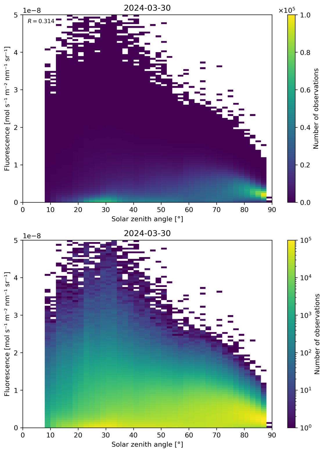
Figure 112: Scatter density plot of “Solar zenith angle” against “Fluorescence” for 2024-03-30 to 2024-03-31.
