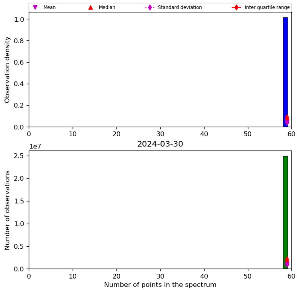
Figure 44: Histogram of “Number of points in the spectrum” for 2024-03-30 to 2024-03-31
