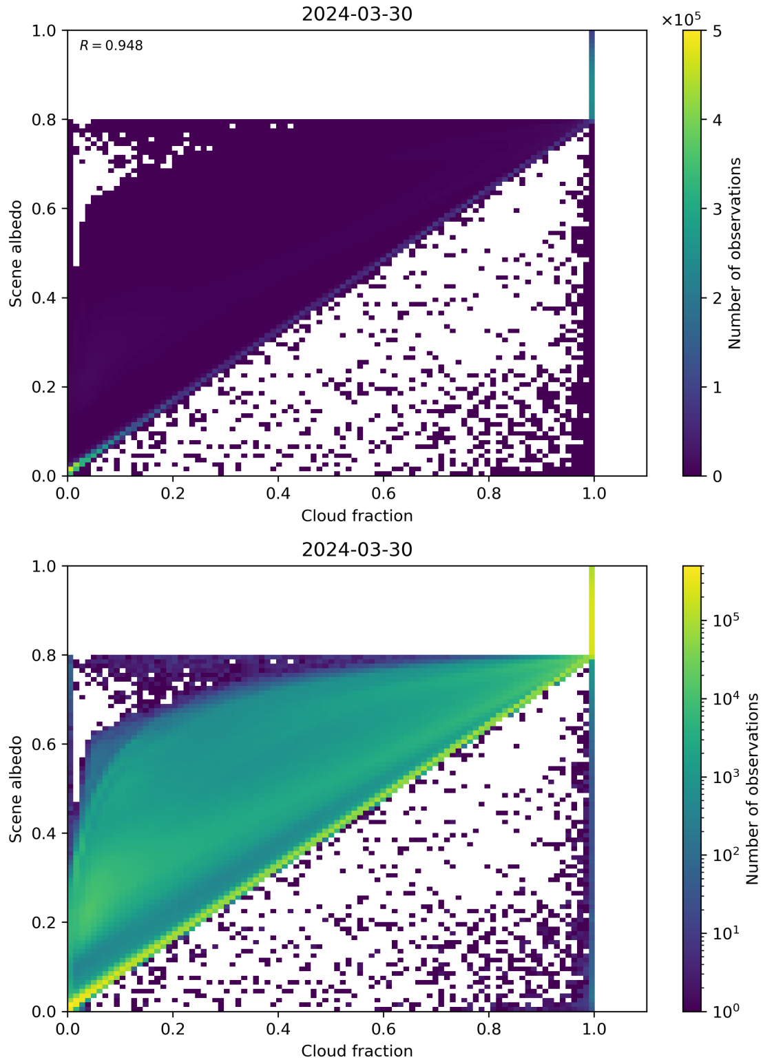
Figure 75: Scatter density plot of “Cloud fraction” against “Scene albedo” for 2024-03-30 to 2024-03-31.
