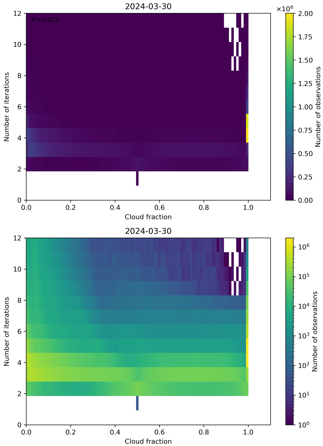
Figure 73: Scatter density plot of “Cloud fraction” against “Number of iterations” for 2024-03-30 to 2024-03-31.
