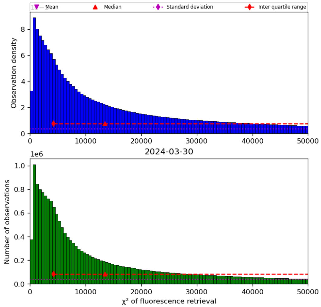
Figure 42: Histogram of “ \chi^2 of fluorescence retrieval” for 2024-03-30 to 2024-03-31
