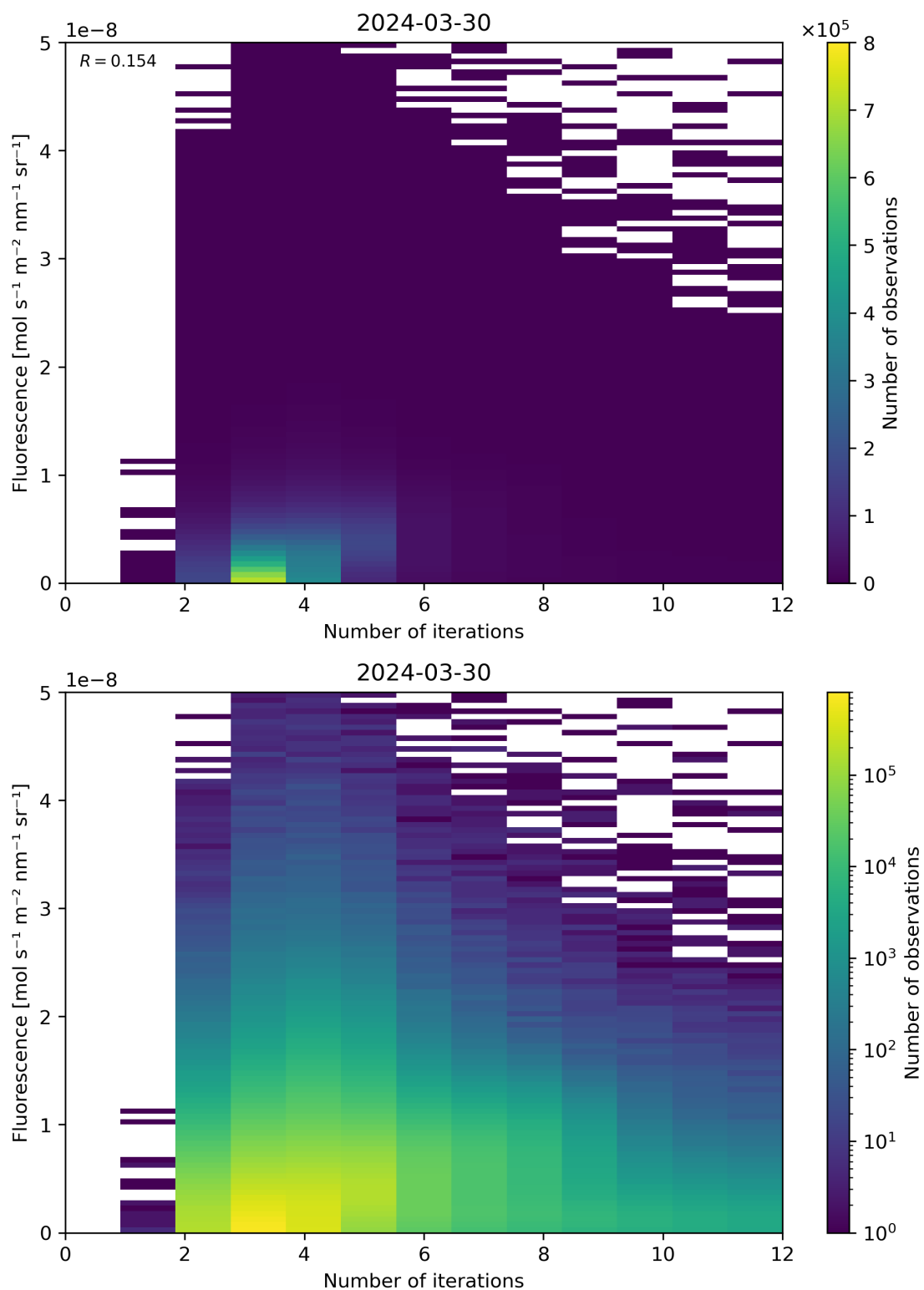
Figure 98: Scatter density plot of “Number of iterations” against “Fluorescence” for 2024-03-30 to 2024-03-31.
