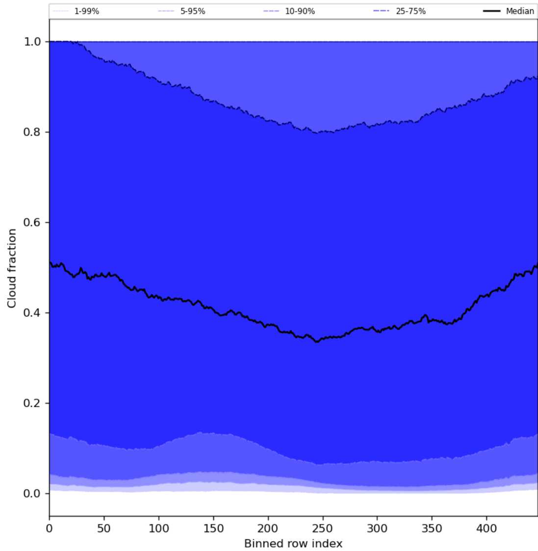
Figure 49: Along track statistics of “Cloud fraction” for 2024-03-30 to 2024-03-31
