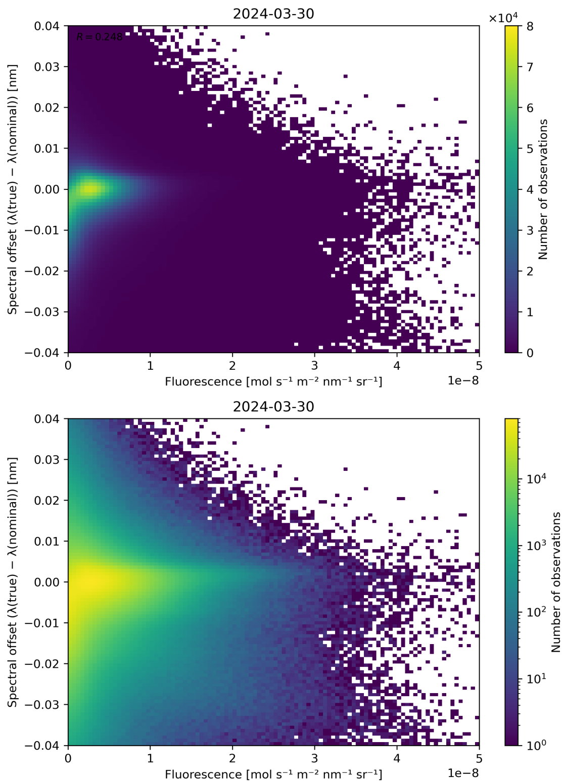
Figure 87: Scatter density plot of “Fluorescence” against “Spectral offset ( \lambda(\text{true}) - \lambda(\text{nominal}) )” for 2024-03-30 to 2024-03-31.
