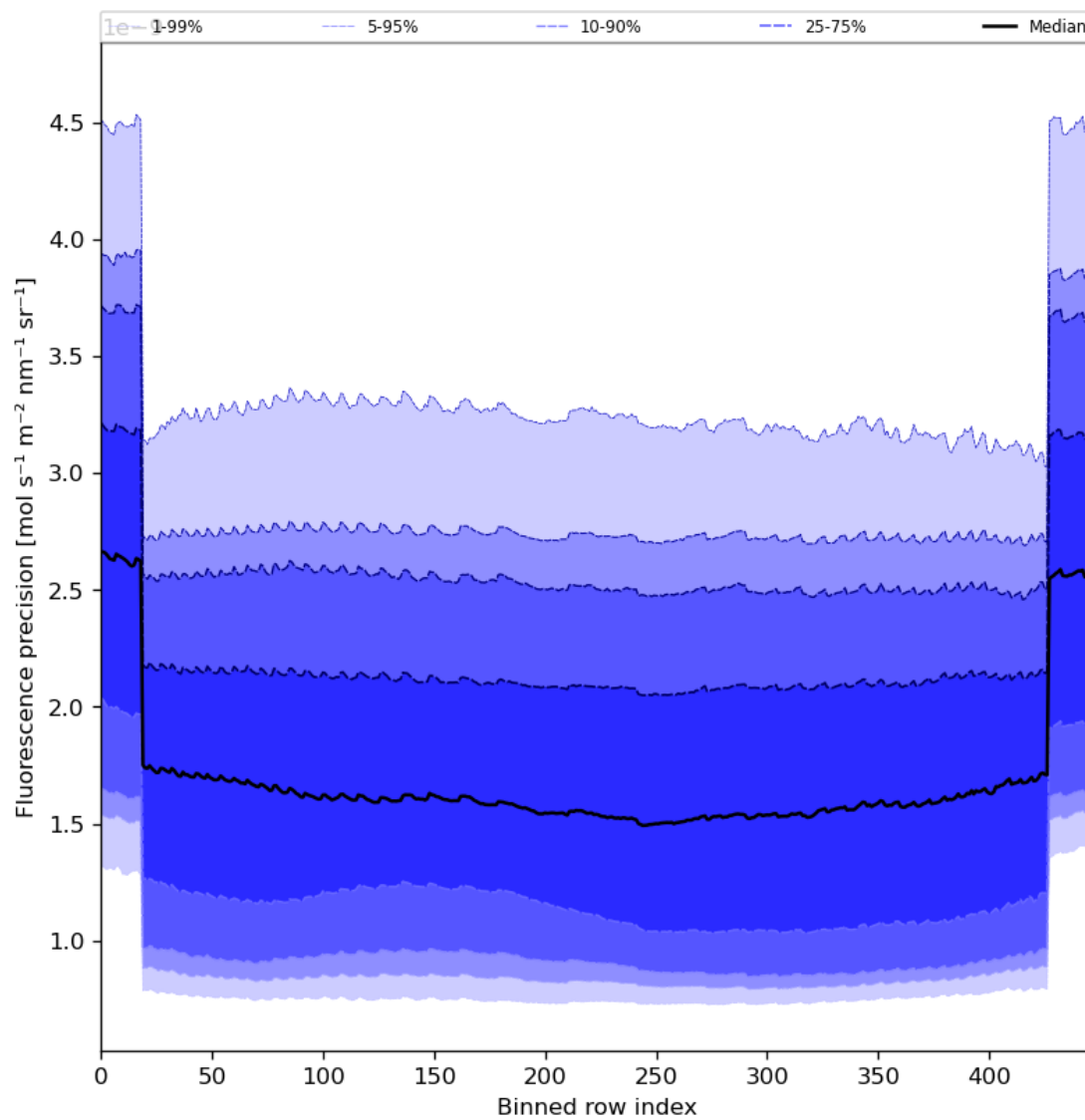
Figure 58: Along track statistics of “Fluorescence precision” for 2024-03-30 to 2024-03-31
