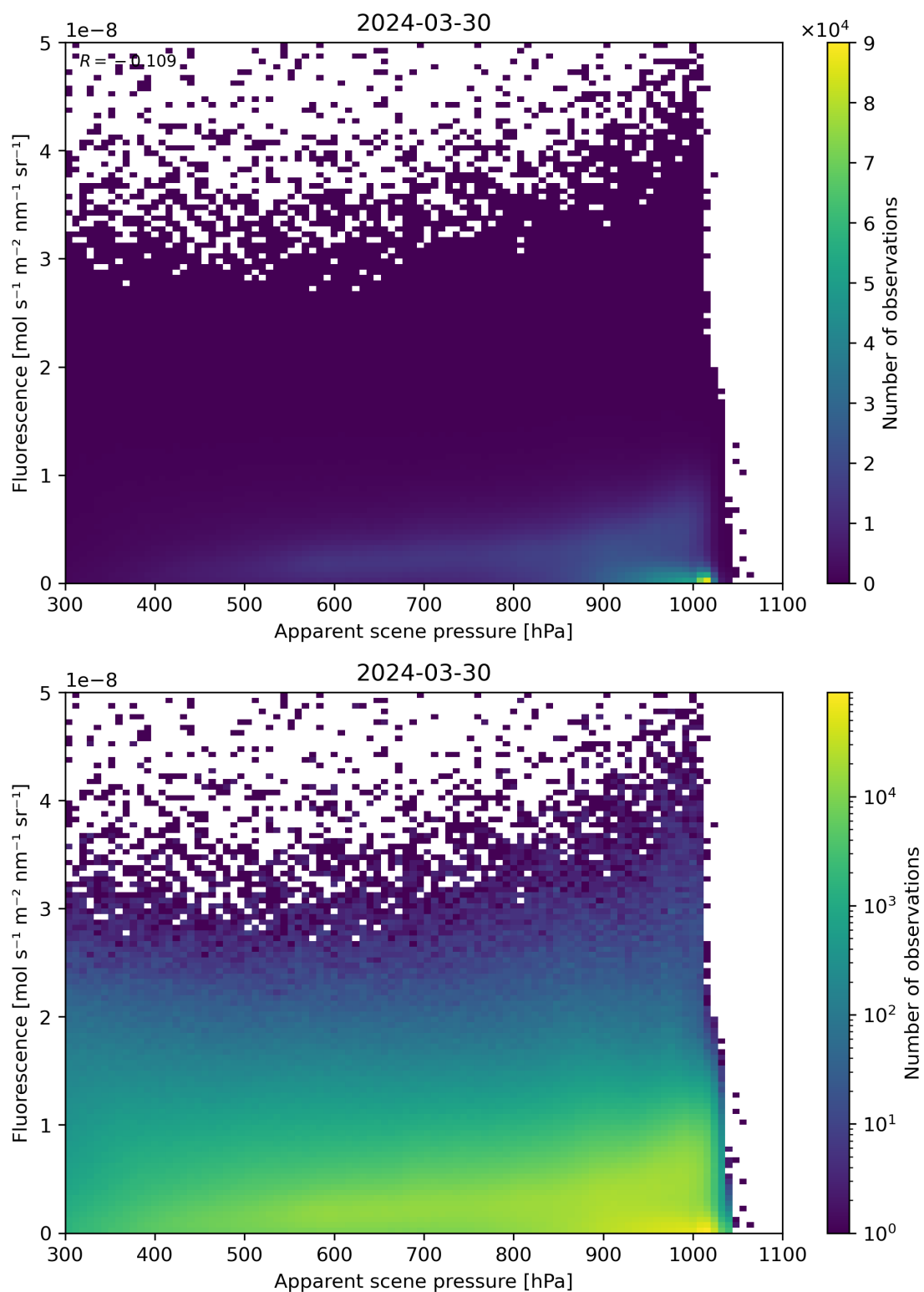
Figure 64: Scatter density plot of “Apparent scene pressure” against “Fluorescence” for 2024-03-30 to 2024-03-31.
