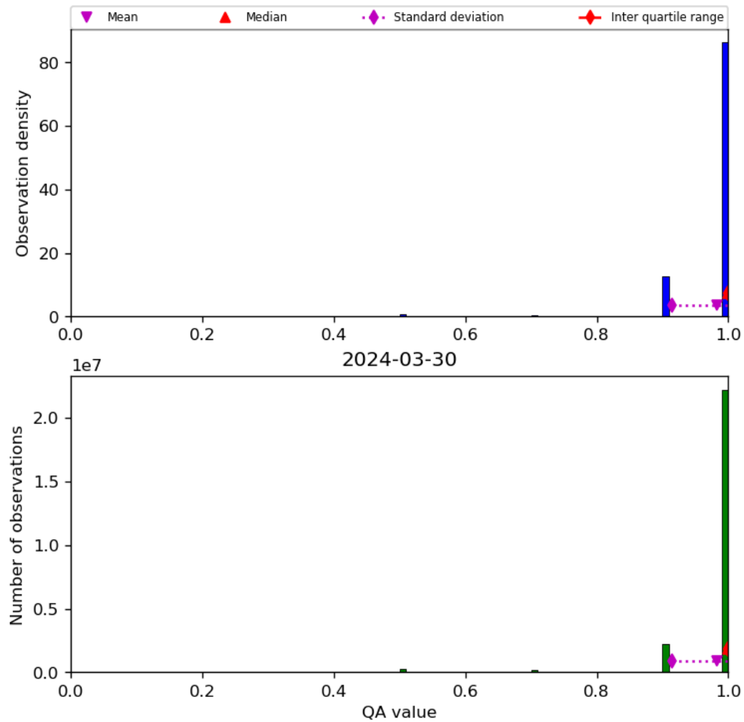
Figure 29: Histogram of “QA value” for 2024-03-30 to 2024-03-31
