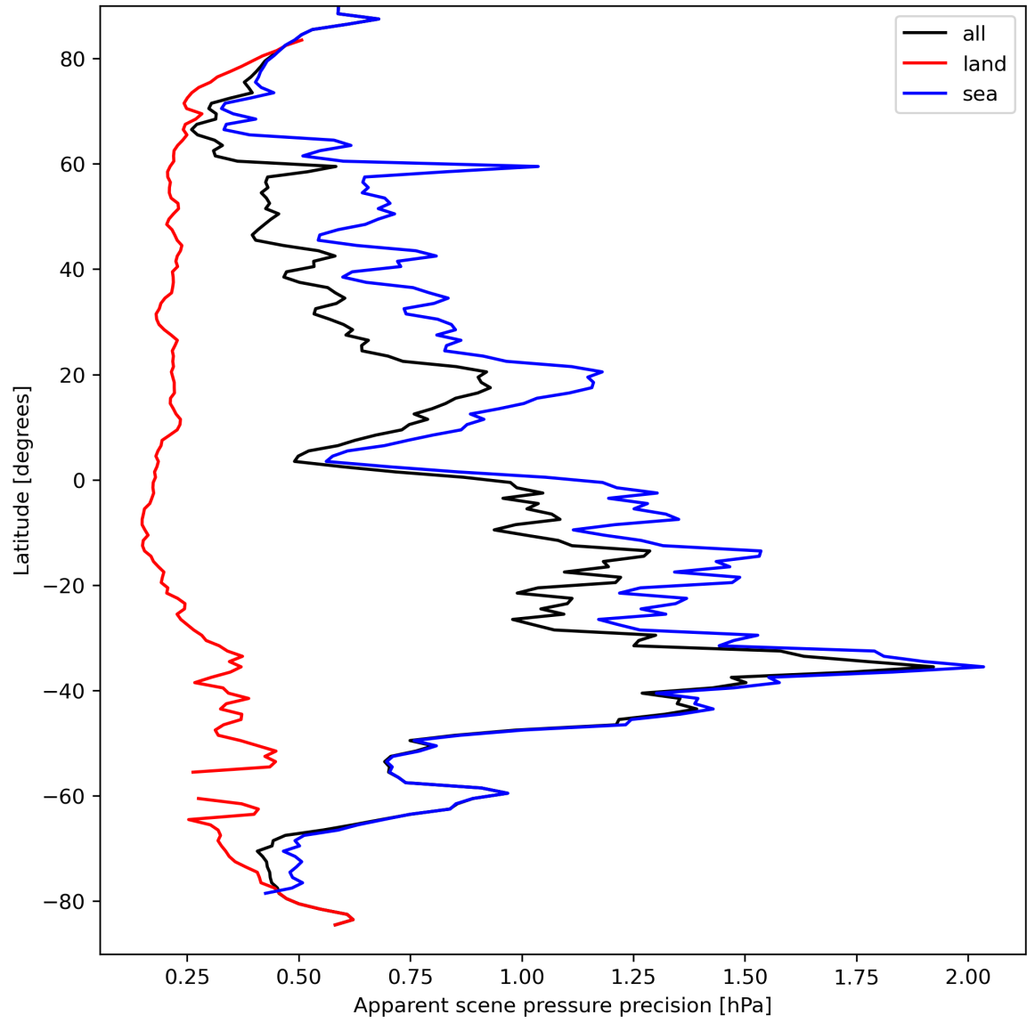
Figure 20: Zonal average of “Apparent scene pressure precision” for 2024-03-30 to 2024-03-31.
