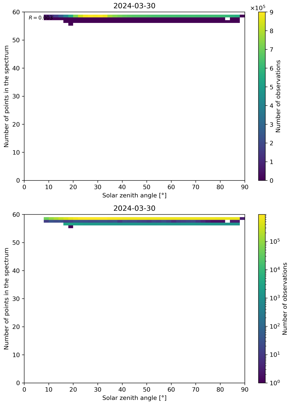
Figure 115: Scatter density plot of “Solar zenith angle” against “Number of points in the spectrum” for 2024-03-30 to 2024-03-31.
