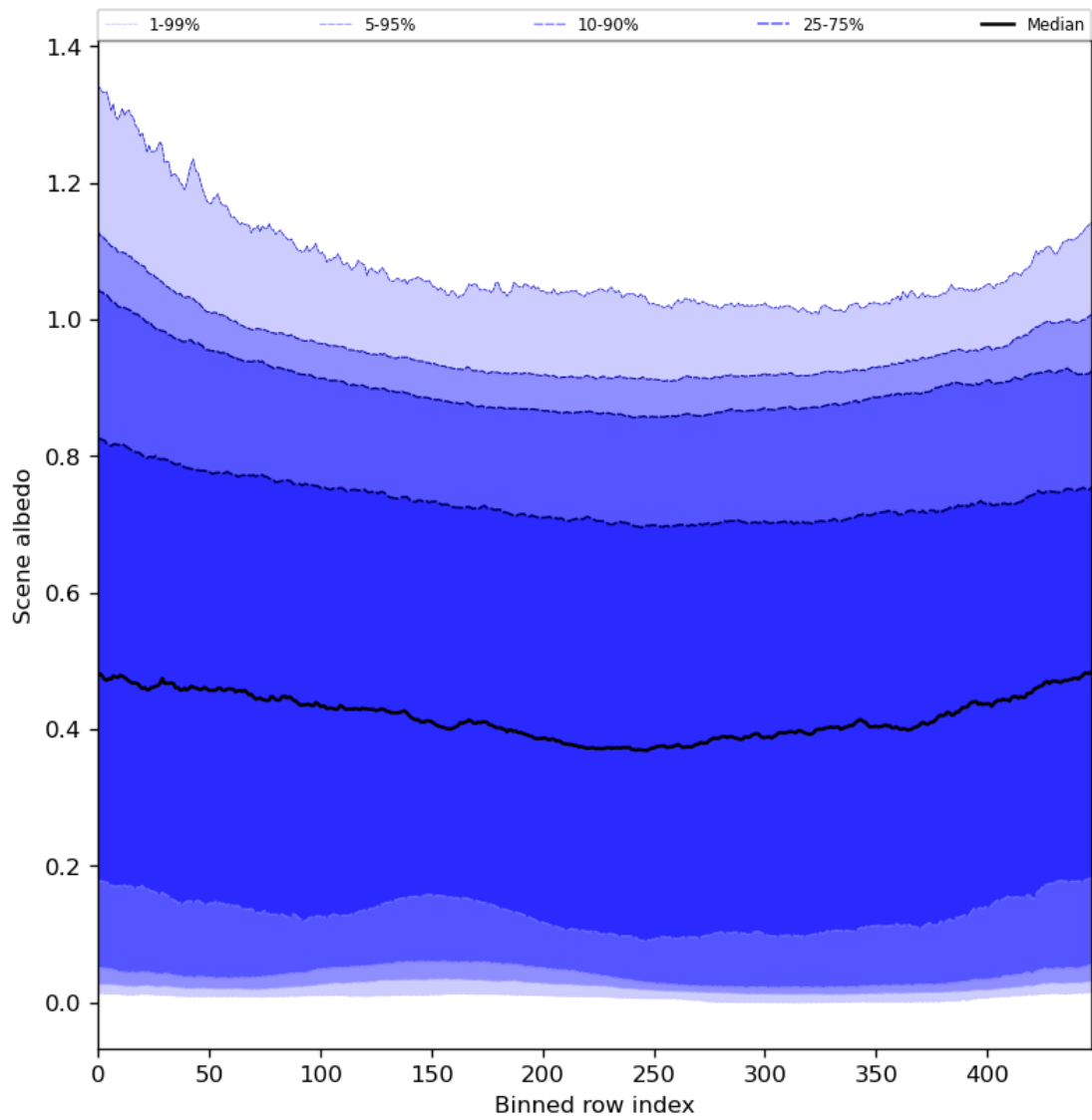
Figure 51: Along track statistics of “Scene albedo” for 2024-03-30 to 2024-03-31
