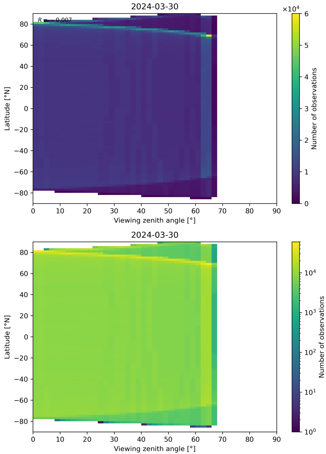
Figure 123: Scatter density plot of “Viewing zenith angle” against “Latitude” for 2024-03-30 to 2024-03-31.
