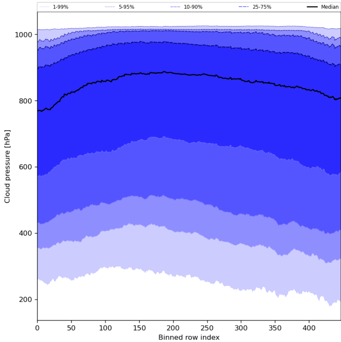
Figure 47: Along track statistics of “Cloud pressure” for 2024-03-30 to 2024-03-31
