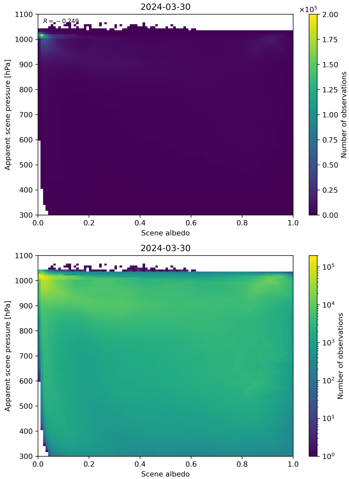
Figure 102: Scatter density plot of “Scene albedo” against “Apparent scene pressure” for 2024-03-30 to 2024-03-31.
