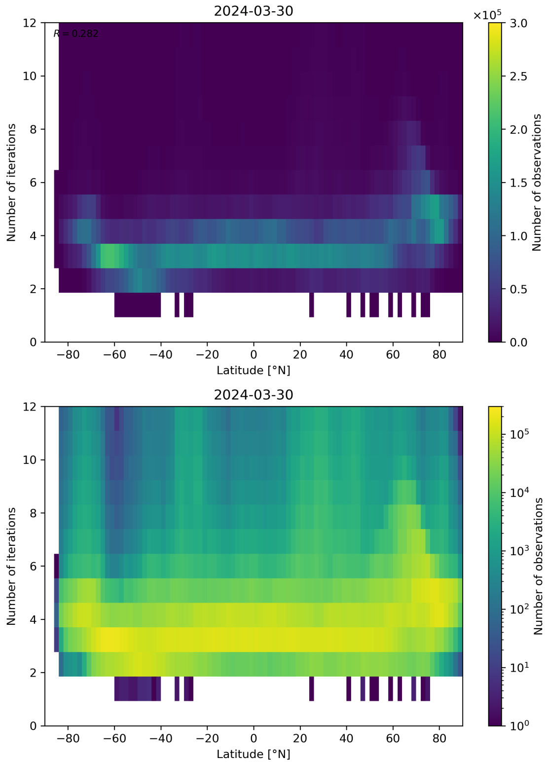
Figure 93: Scatter density plot of “Latitude” against “Number of iterations” for 2024-03-30 to 2024-03-31.
