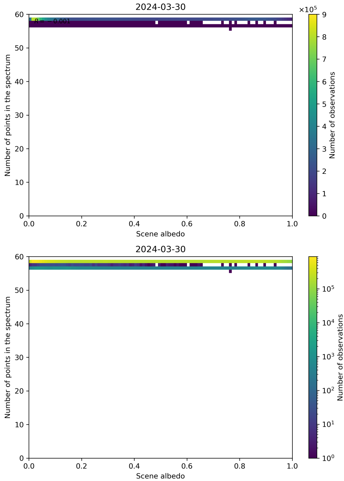
Figure 106: Scatter density plot of “Scene albedo” against “Number of points in the spectrum” for 2024-03-30 to 2024-03-31.
