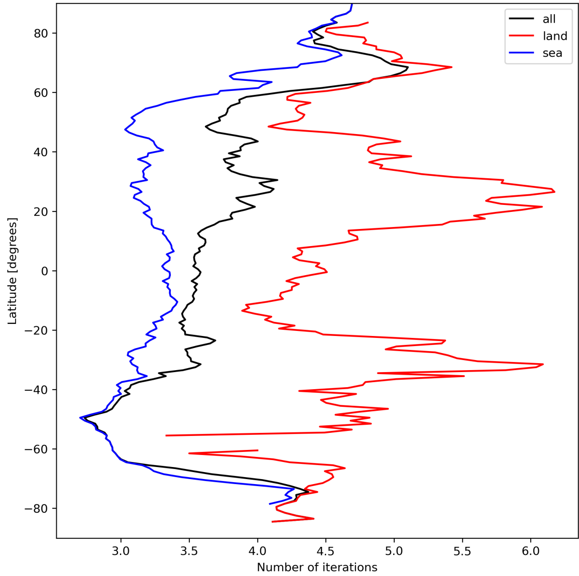
Figure 22: Zonal average of “Number of iterations” for 2024-03-30 to 2024-03-31.
