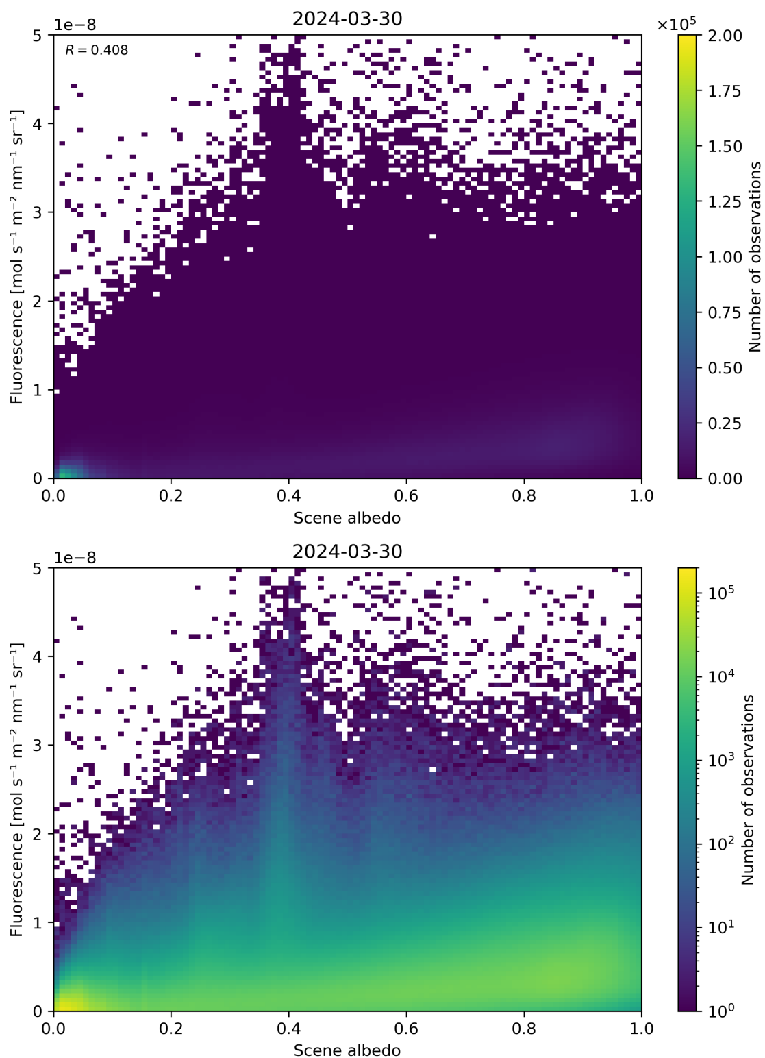
Figure 104: Scatter density plot of “Scene albedo” against “Fluorescence” for 2024-03-30 to 2024-03-31.
