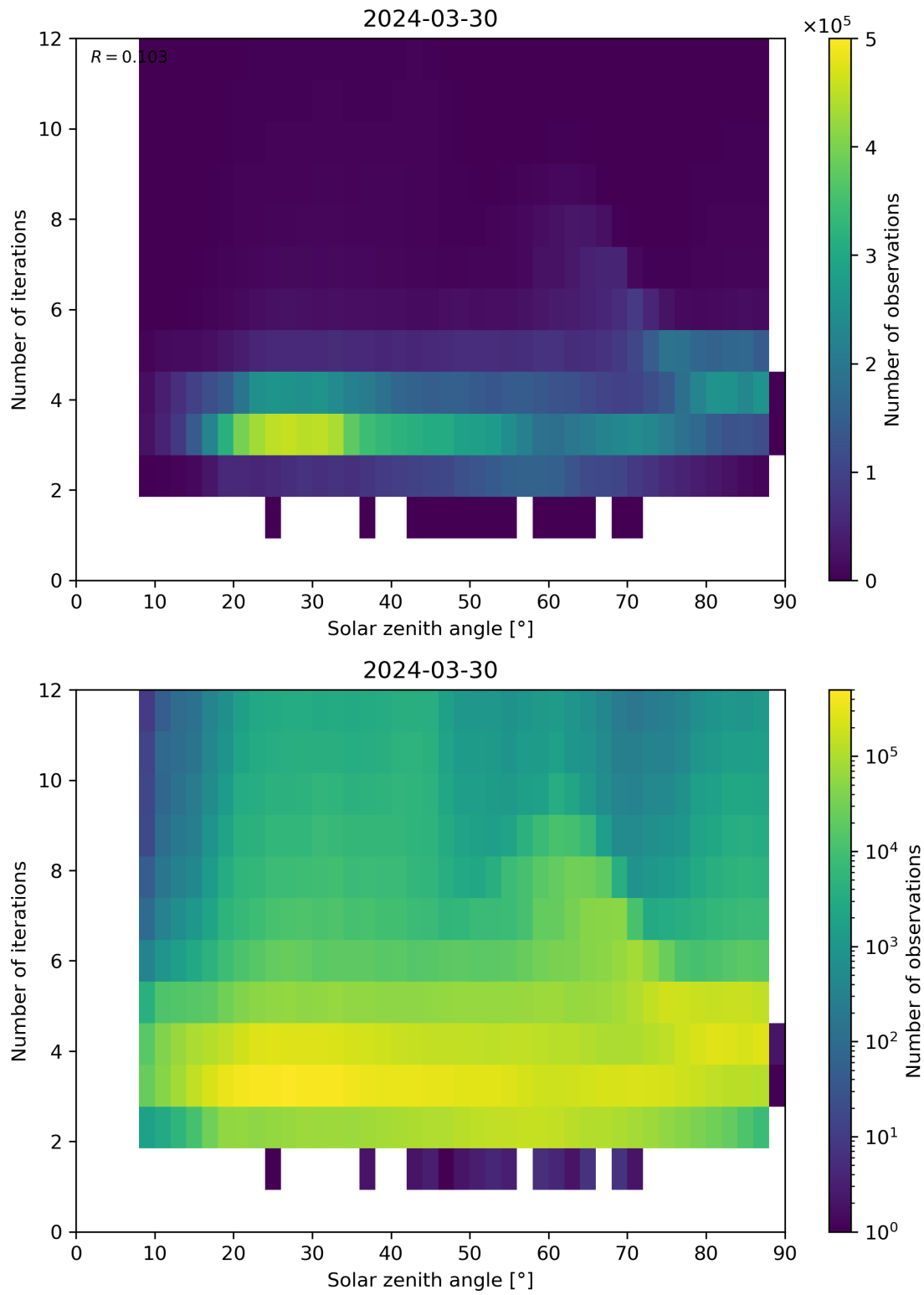
Figure 114: Scatter density plot of “Solar zenith angle” against “Number of iterations” for 2024-03-30 to 2024-03-31.
