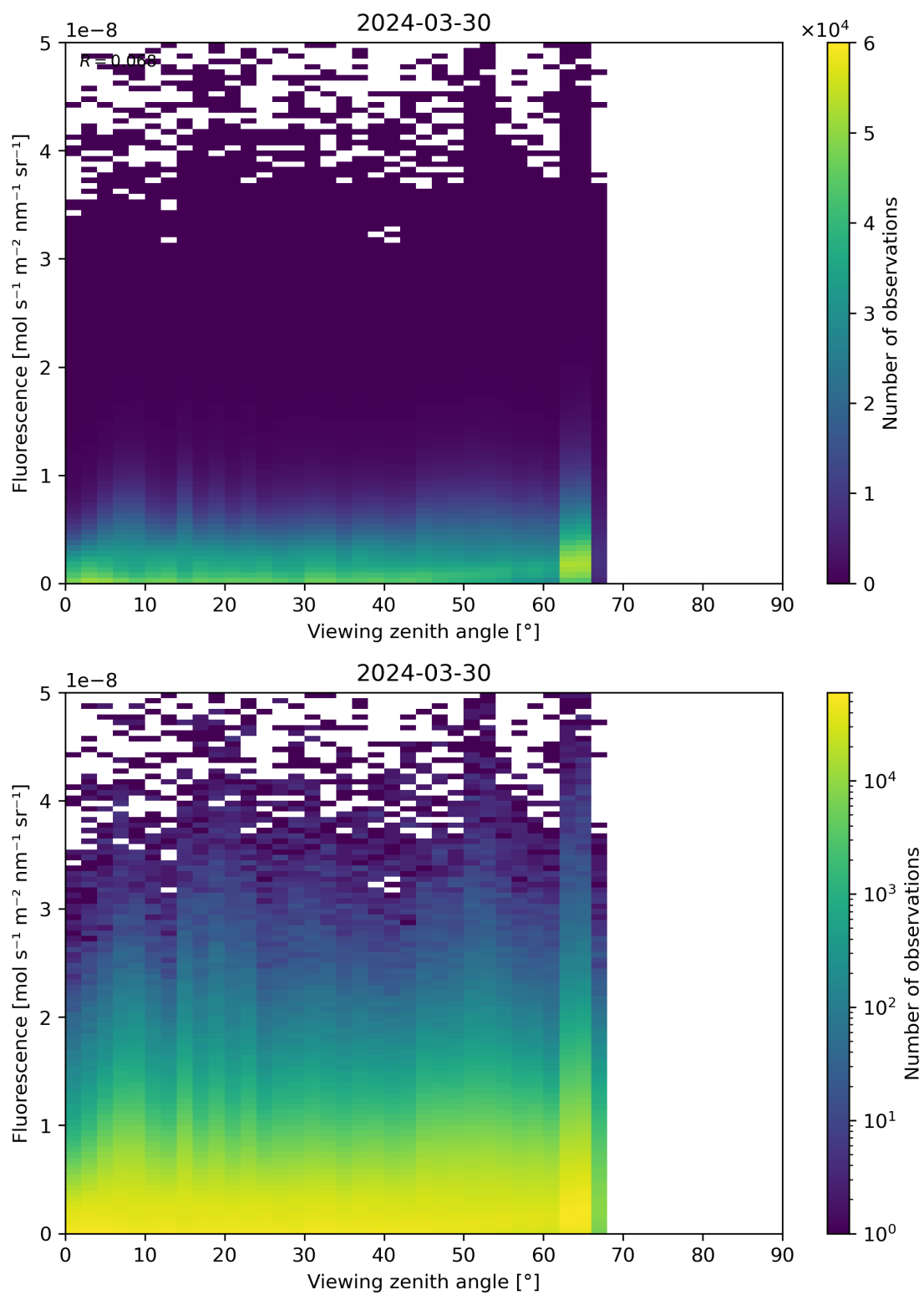
Figure 122: Scatter density plot of “Viewing zenith angle” against “Fluorescence” for 2024-03-30 to 2024-03-31.
