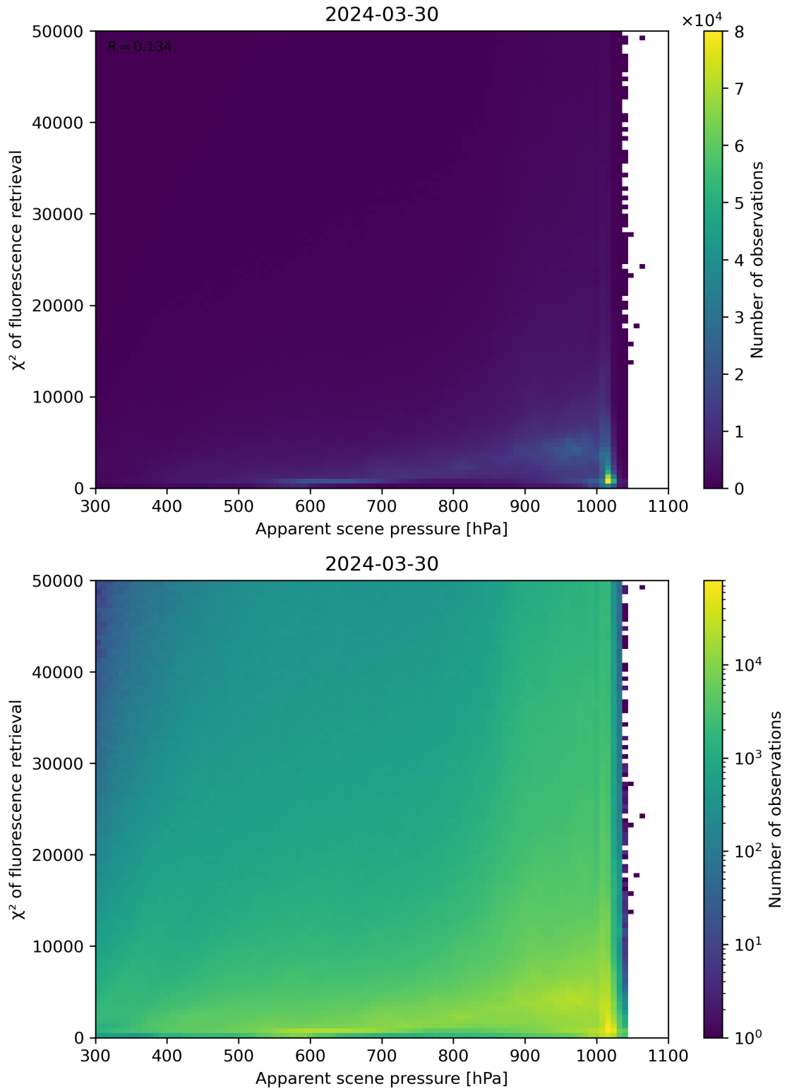
Figure 63: Scatter density plot of “Apparent scene pressure” against “ \chi^2 of fluorescence retrieval” for 2024-03-30 to 2024-03-31.
