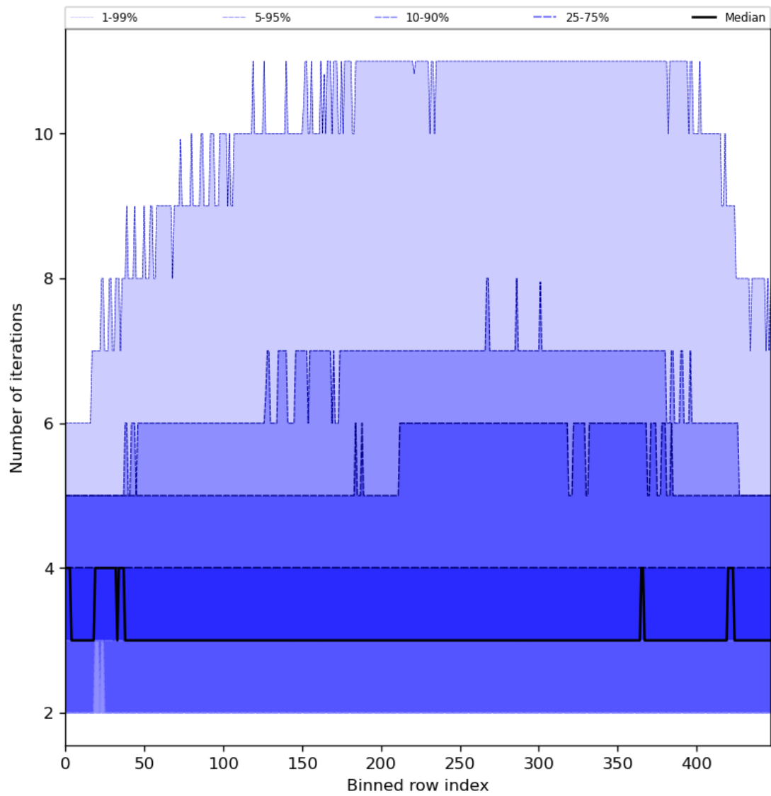
Figure 56: Along track statistics of “Number of iterations” for 2024-03-30 to 2024-03-31
