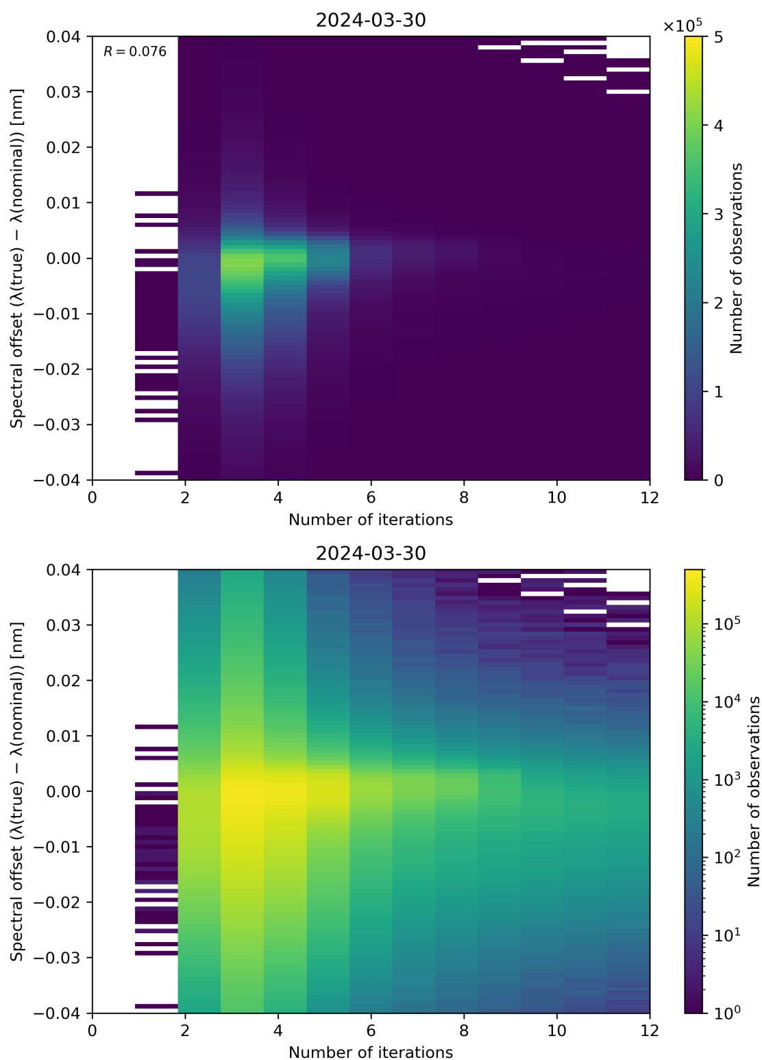
Figure 100: Scatter density plot of “Number of iterations” against “Spectral offset ( \lambda(\text{true}) - \lambda(\text{nominal}) )” for 2024-03-30 to 2024-03-31.
