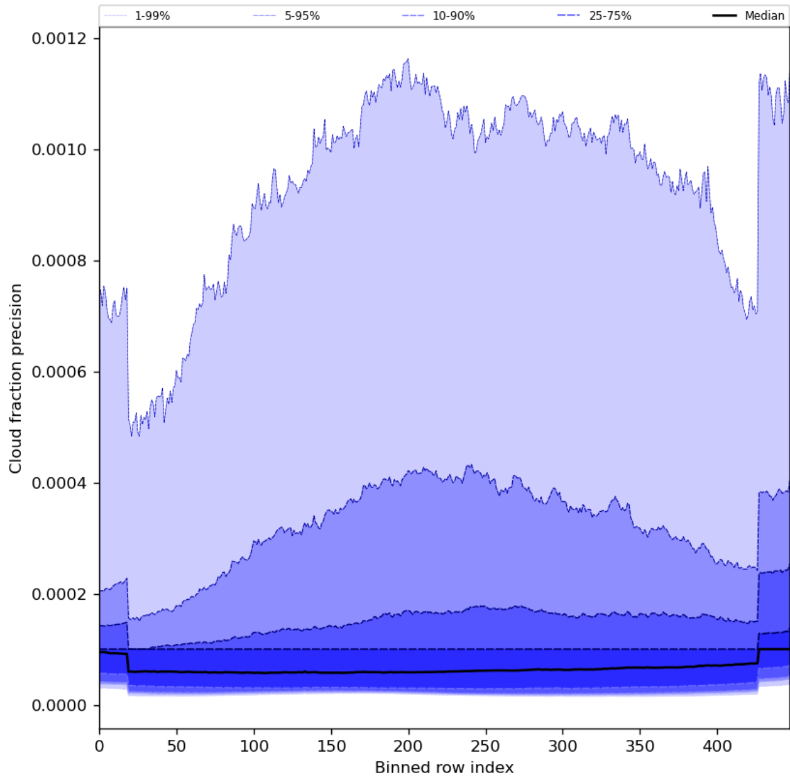
Figure 50: Along track statistics of “Cloud fraction precision” for 2024-03-30 to 2024-03-31
