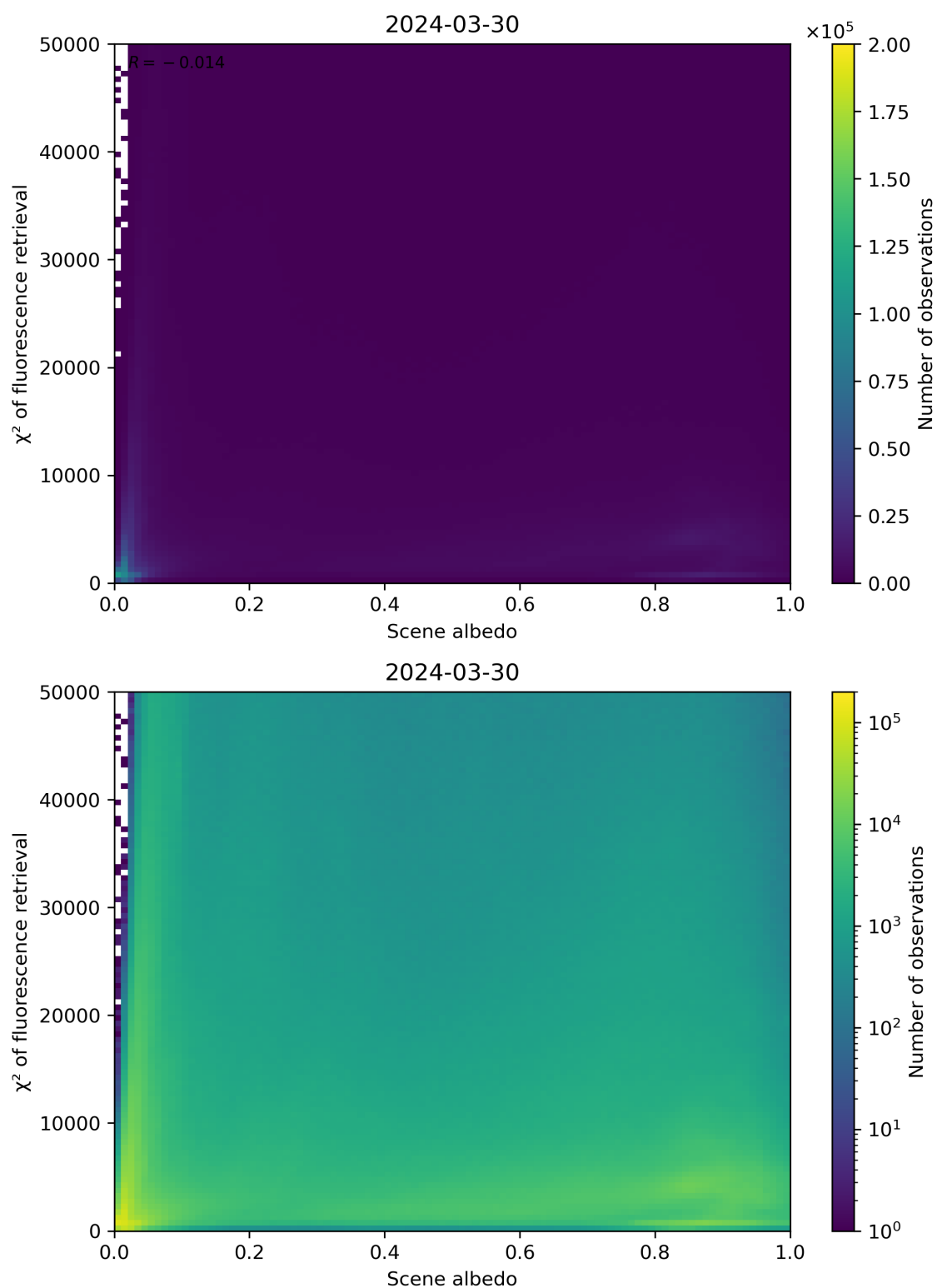
Figure 103: Scatter density plot of “Scene albedo” against “ \chi^2 of fluorescence retrieval” for 2024-03-30 to 2024-03-31.
