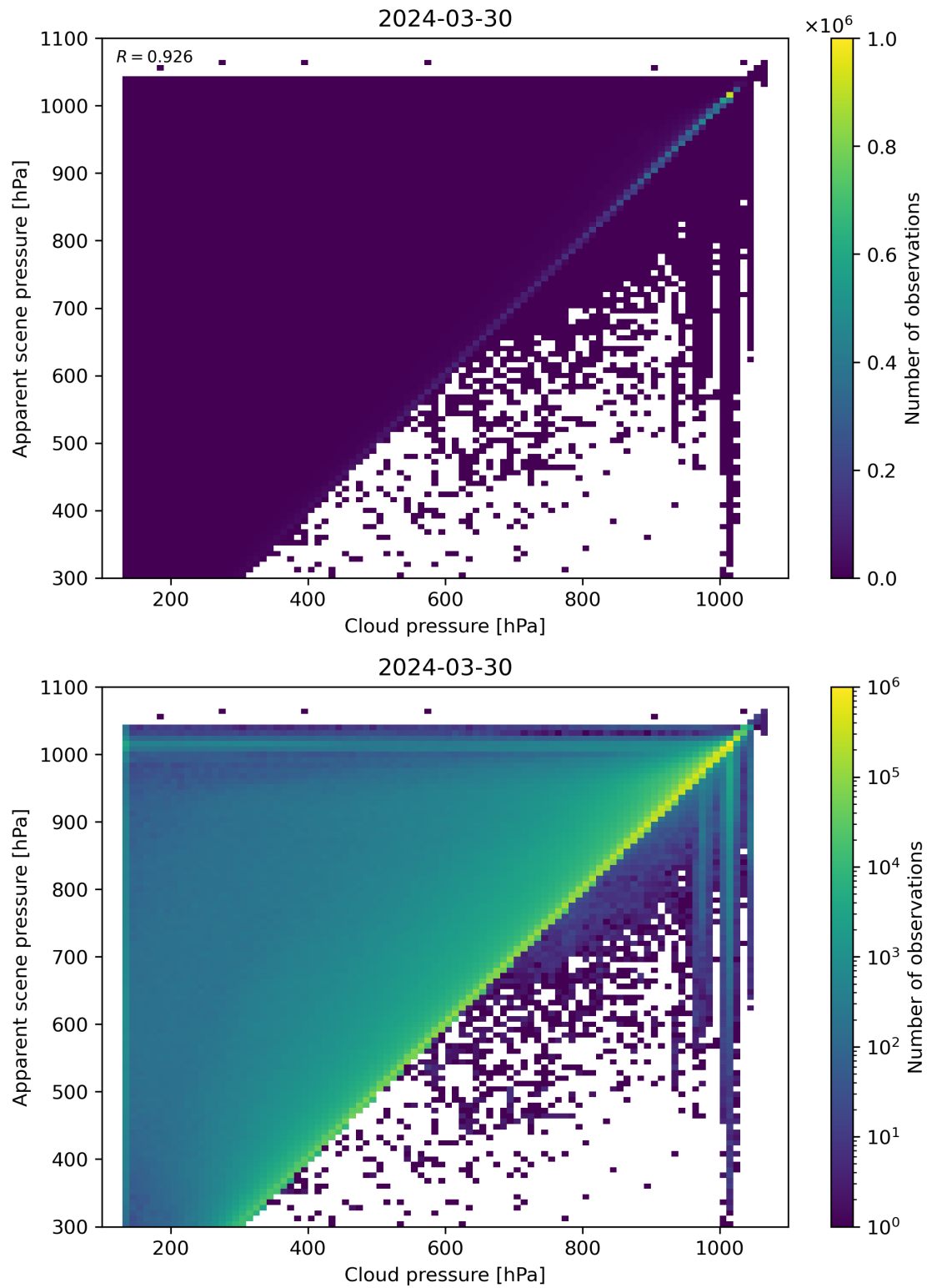
Figure 77: Scatter density plot of “Cloud pressure” against “Apparent scene pressure” for 2024-03-30 to 2024-03-31.
