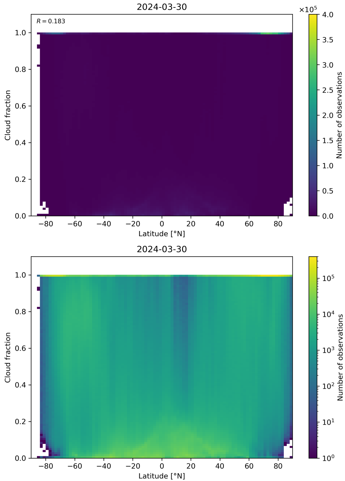
Figure 90: Scatter density plot of “Latitude” against “Cloud fraction” for 2024-03-30 to 2024-03-31.
