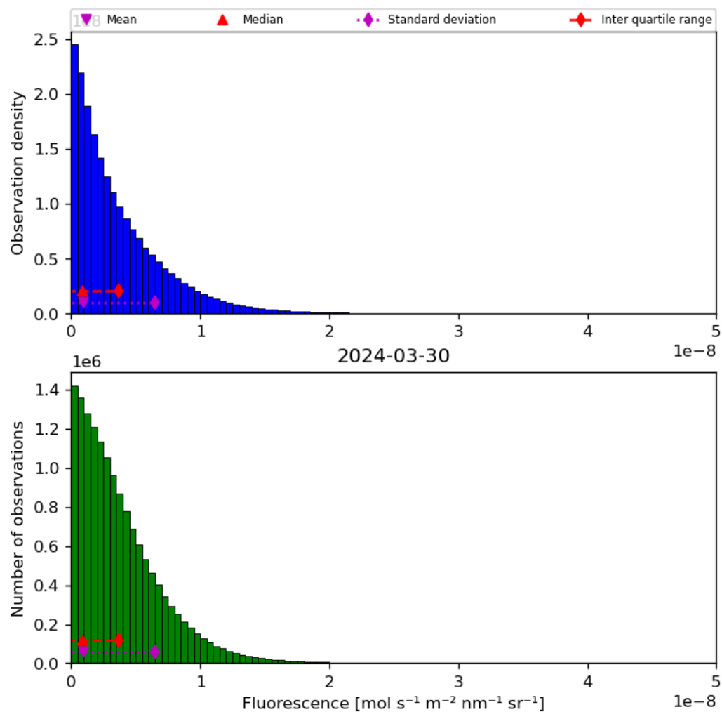
Figure 40: Histogram of “Fluorescence” for 2024-03-30 to 2024-03-31
