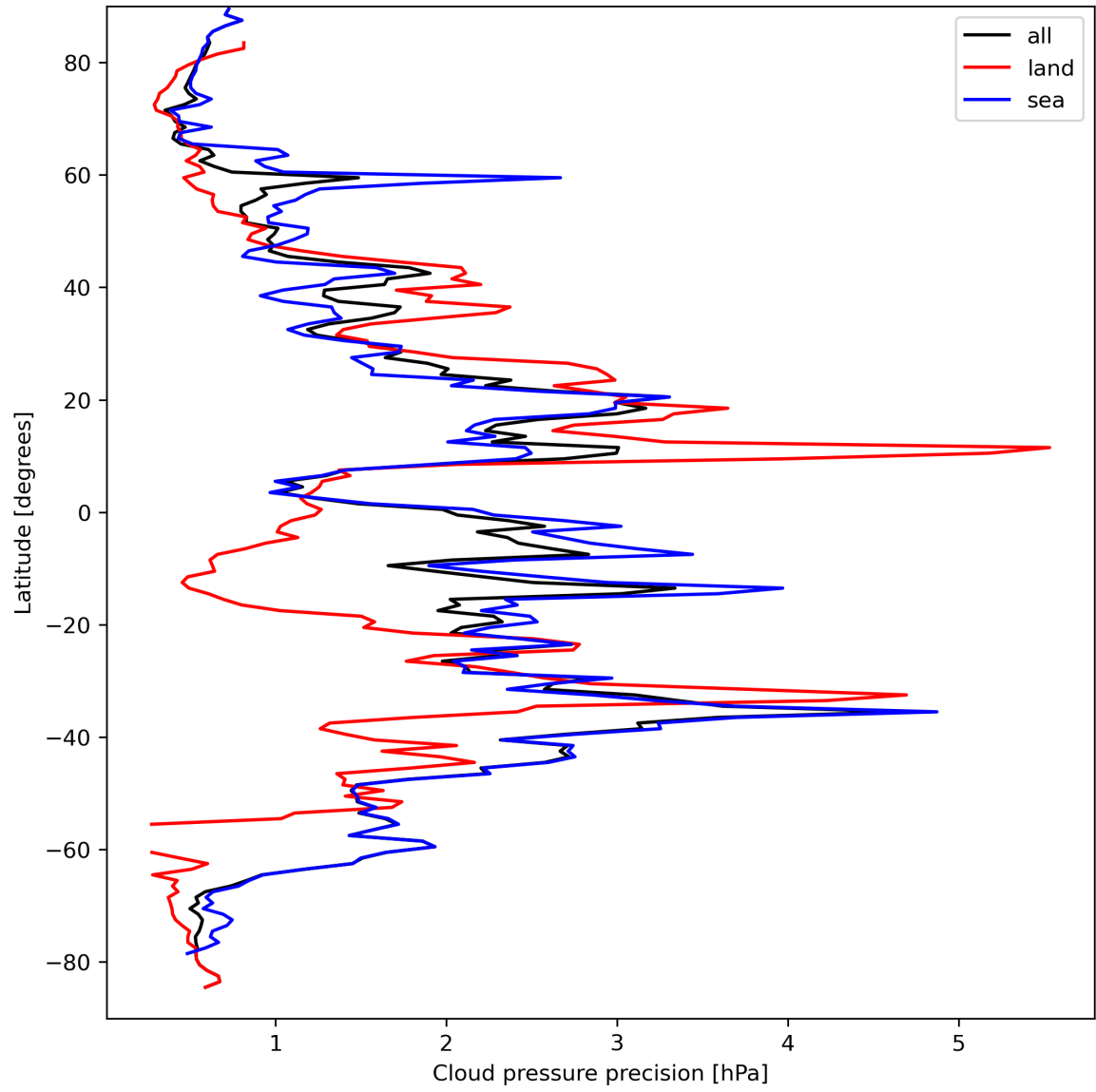
Figure 14: Zonal average of “Cloud pressure precision” for 2024-03-30 to 2024-03-31.
