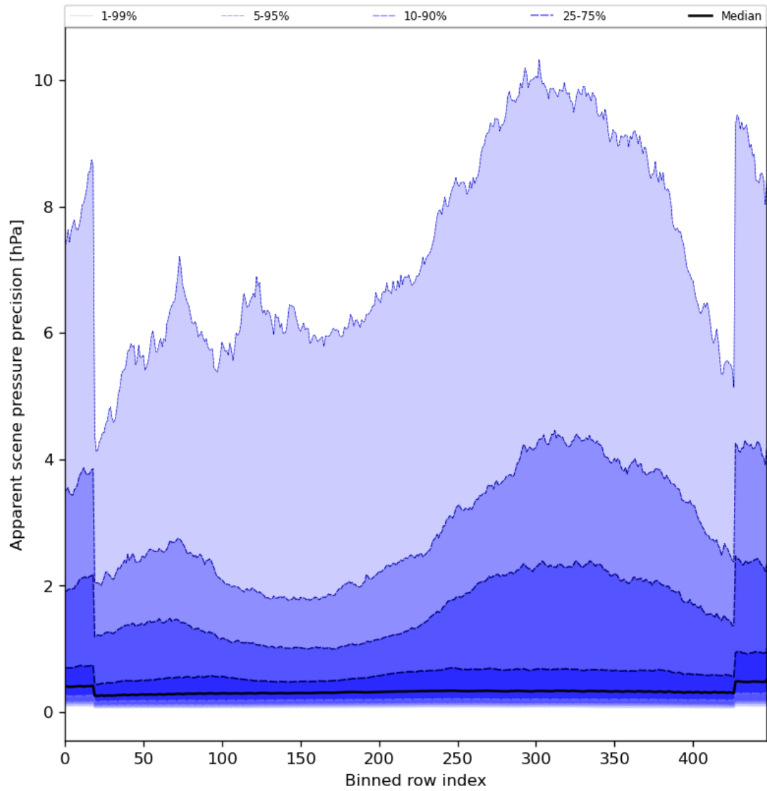
Figure 54: Along track statistics of “Apparent scene pressure precision” for 2024-03-30 to 2024-03-31
