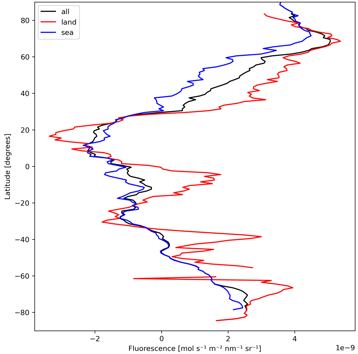
Figure 23: Zonal average of “Fluorescence” for 2024-03-30 to 2024-03-31.
