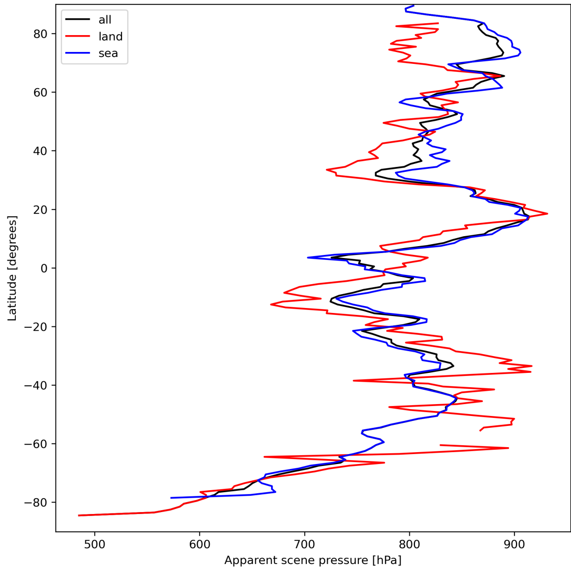
Figure 19: Zonal average of “Apparent scene pressure” for 2024-03-30 to 2024-03-31.
