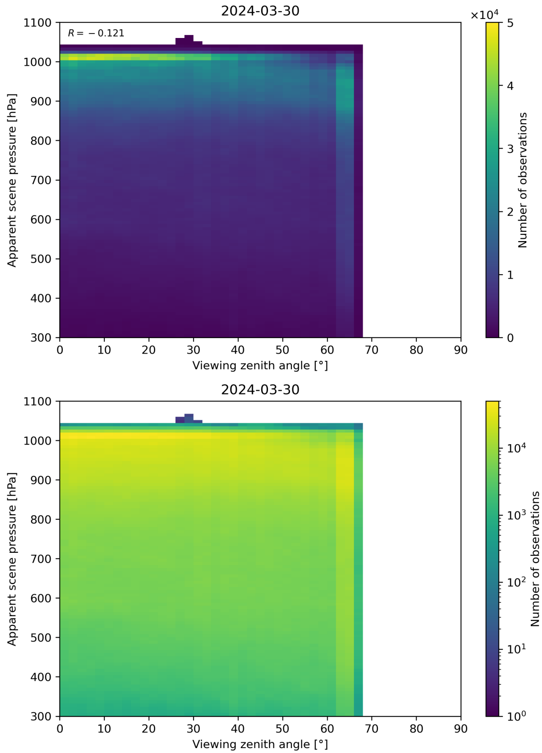
Figure 118: Scatter density plot of “Viewing zenith angle” against “Apparent scene pressure” for 2024-03-30 to 2024-03-31.
