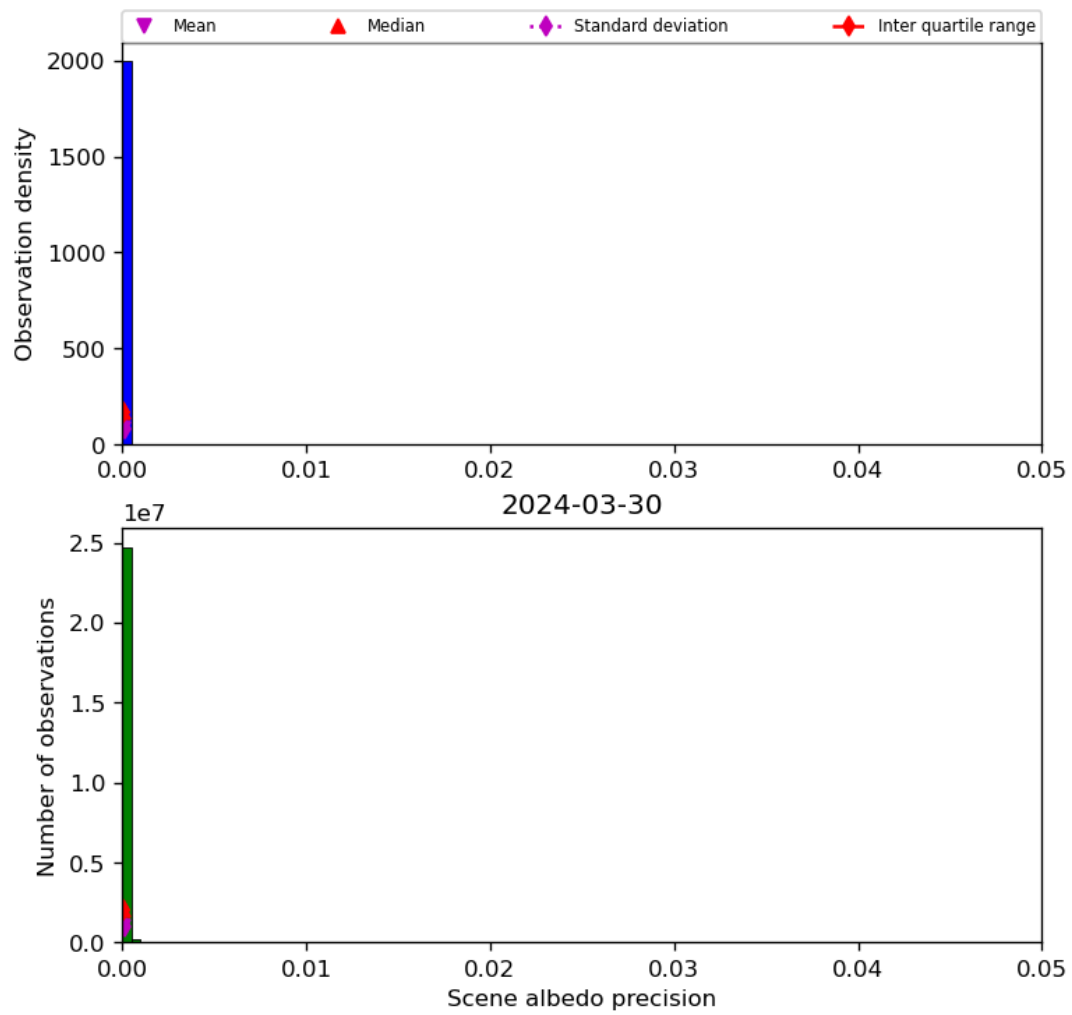
Figure 35: Histogram of “Scene albedo precision” for 2024-03-30 to 2024-03-31
