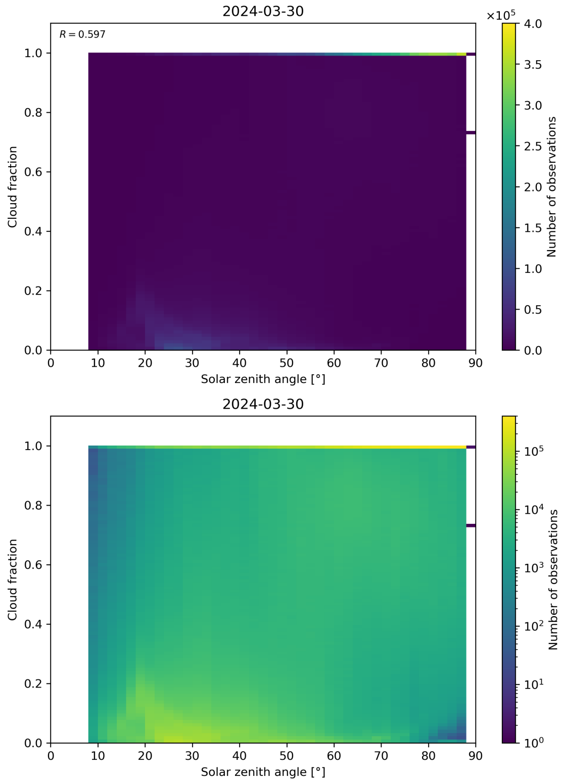
Figure 110: Scatter density plot of “Solar zenith angle” against “Cloud fraction” for 2024-03-30 to 2024-03-31.
