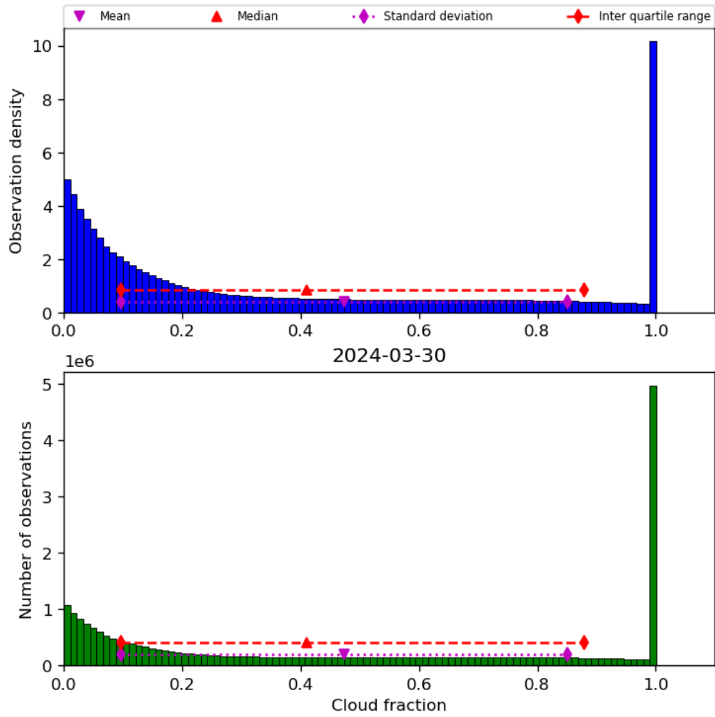
Figure 32: Histogram of “Cloud fraction” for 2024-03-30 to 2024-03-31
