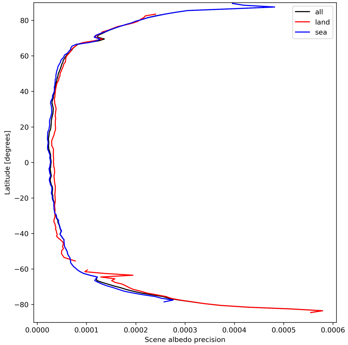
Figure 18: Zonal average of “Scene albedo precision” for 2024-03-30 to 2024-03-31.
