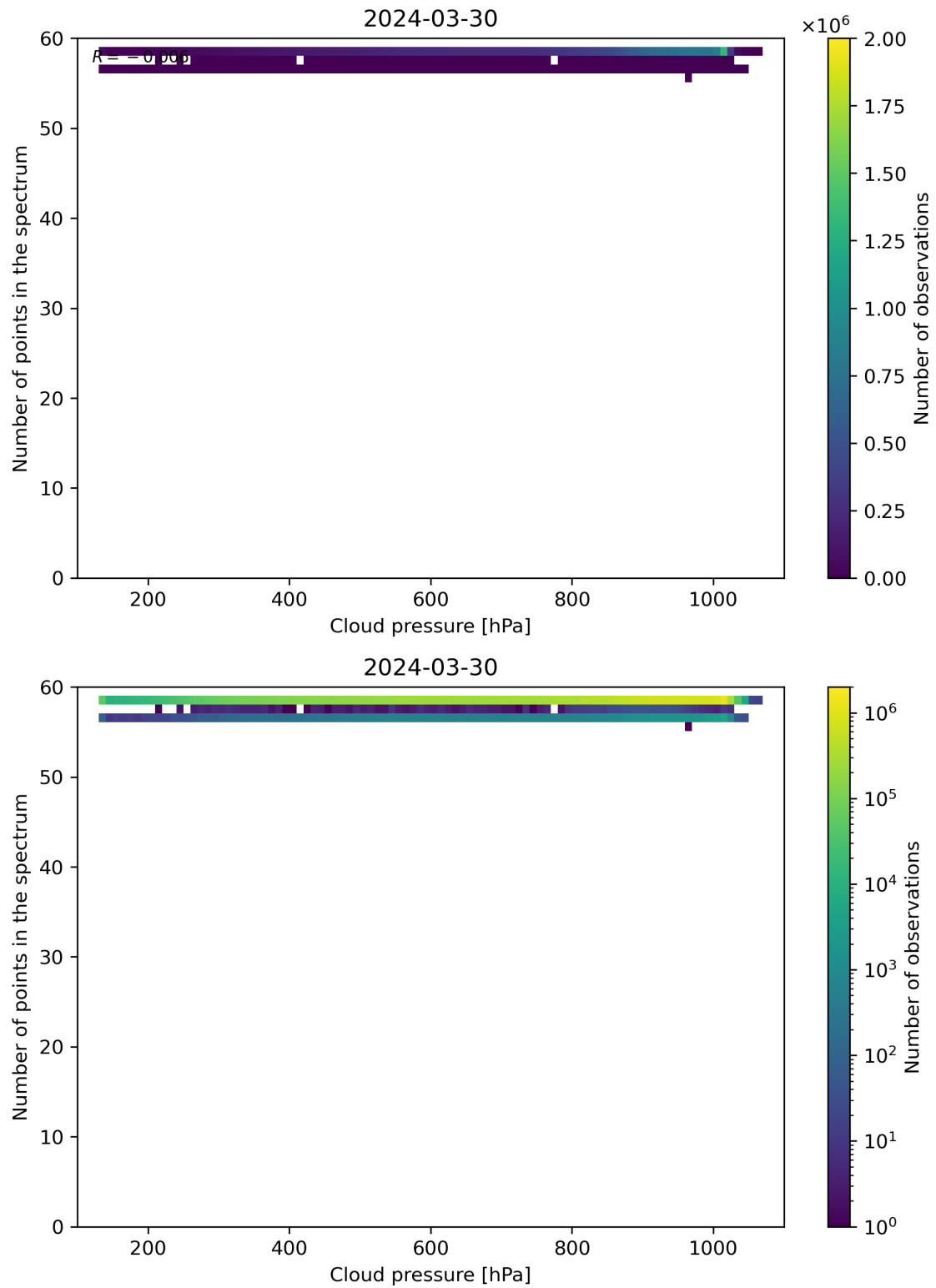
Figure 82: Scatter density plot of “Cloud pressure” against “Number of points in the spectrum” for 2024-03-30 to 2024-03-31.
