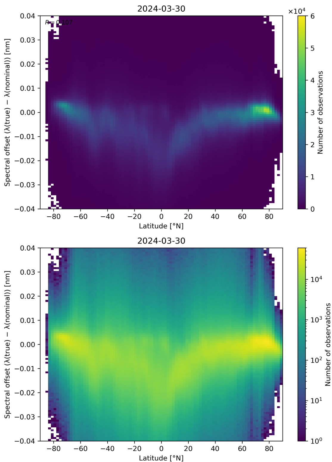
Figure 96: Scatter density plot of “Latitude” against “Spectral offset ( \lambda(\text{true}) - \lambda(\text{nominal}) )” for 2024-03-30 to 2024-03-31.
