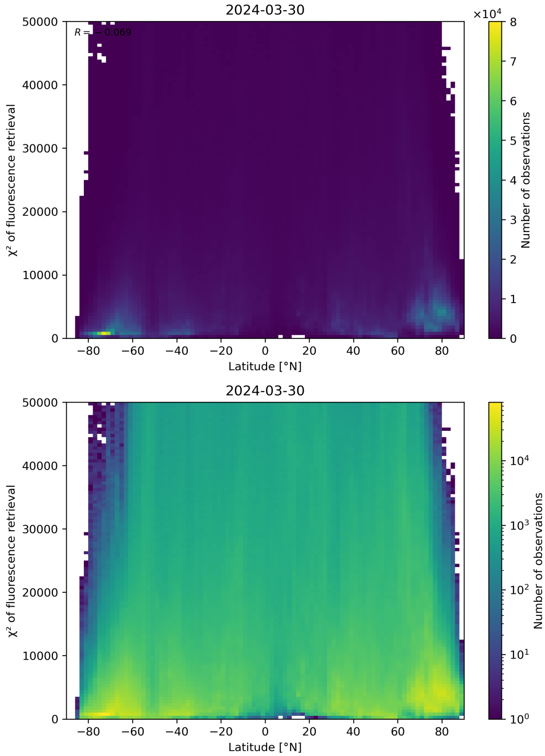
Figure 89: Scatter density plot of “Latitude” against “ \chi^2 of fluorescence retrieval” for 2024-03-30 to 2024-03-31.
