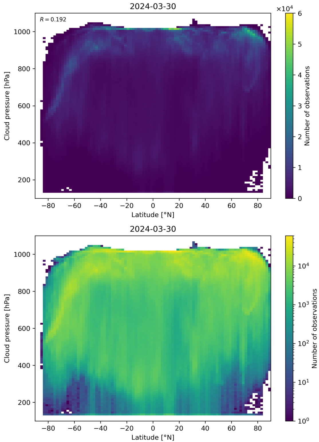
Figure 91: Scatter density plot of “Latitude” against “Cloud pressure” for 2024-03-30 to 2024-03-31.
