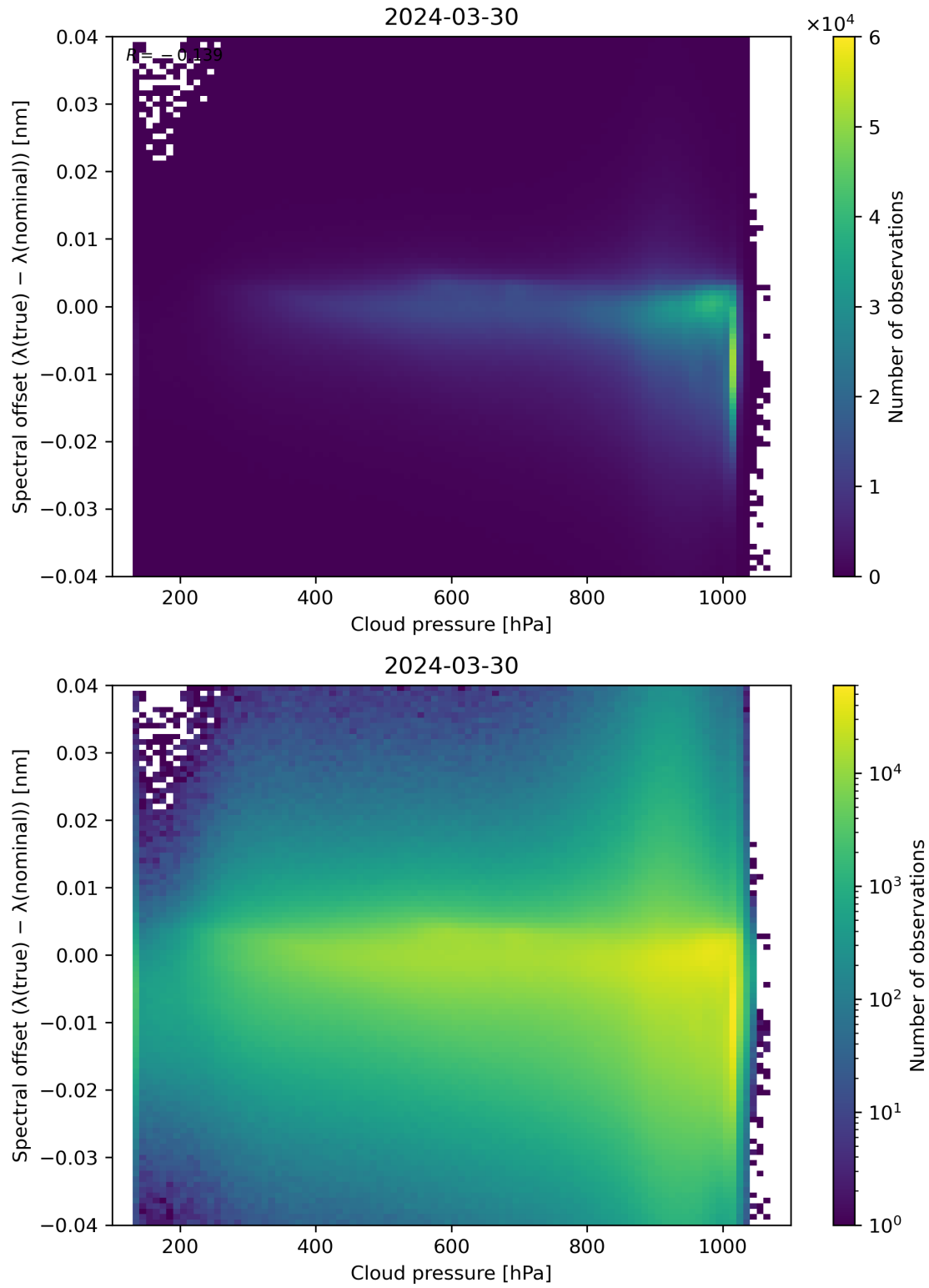
Figure 84: Scatter density plot of “Cloud pressure” against “Spectral offset ( \lambda(\text{true}) - \lambda(\text{nominal}) )” for 2024-03-30 to 2024-03-31.
