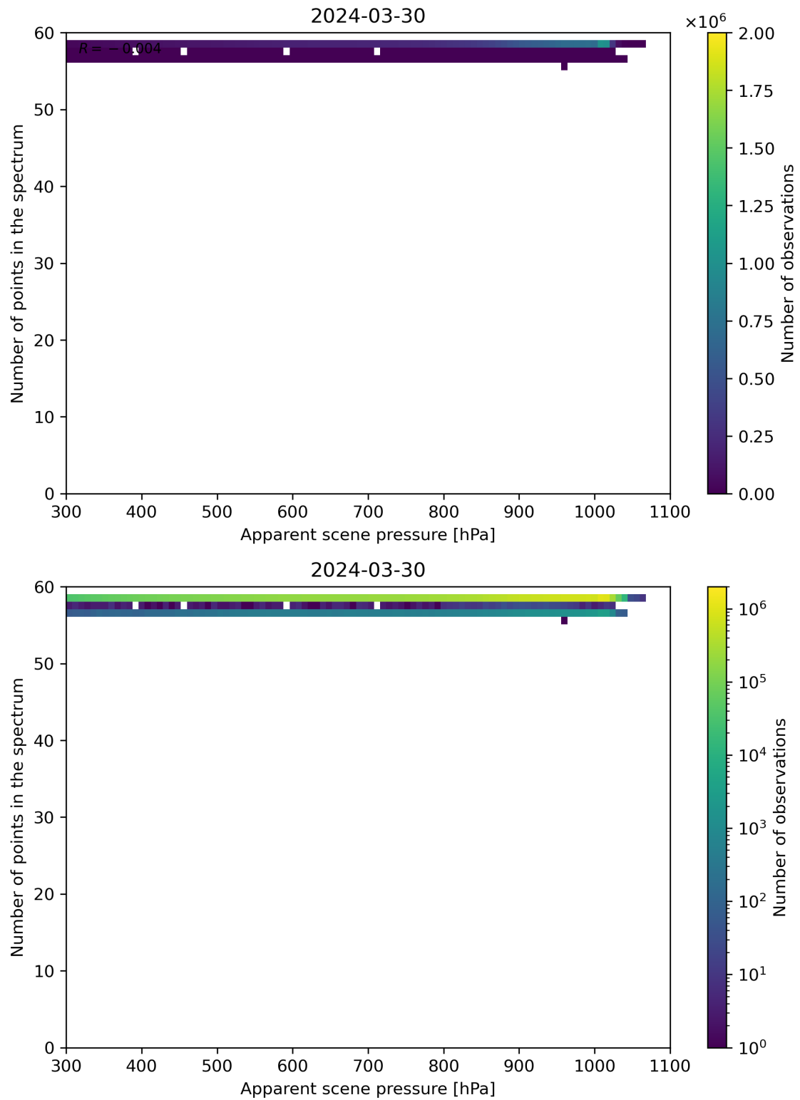
Figure 66: Scatter density plot of “Apparent scene pressure” against “Number of points in the spectrum” for 2024-03-30 to 2024-03-31.
