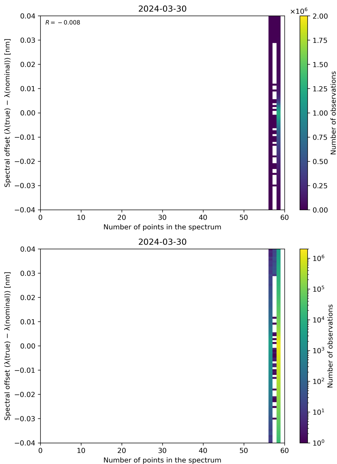
Figure 101: Scatter density plot of “Number of points in the spectrum” against “Spectral offset ( \lambda(\text{true}) - \lambda(\text{nominal}) )” for 2024-03-30 to 2024-03-31.
