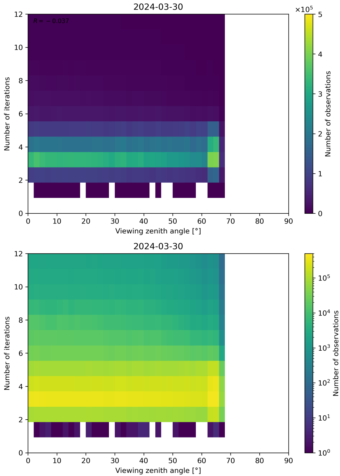
Figure 124: Scatter density plot of “Viewing zenith angle” against “Number of iterations” for 2024-03-30 to 2024-03-31.
