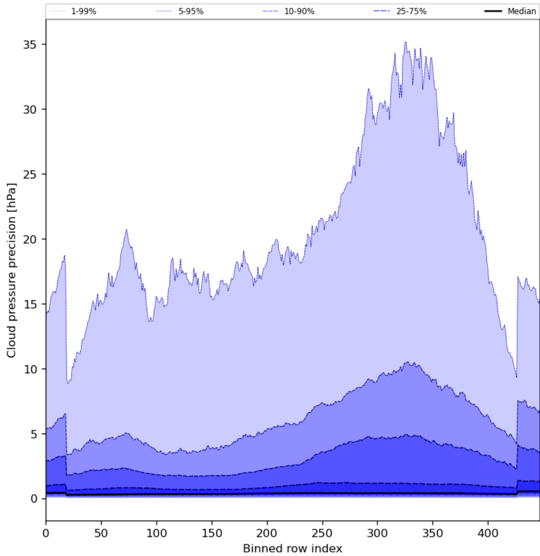
Figure 48: Along track statistics of “Cloud pressure precision” for 2024-03-30 to 2024-03-31
