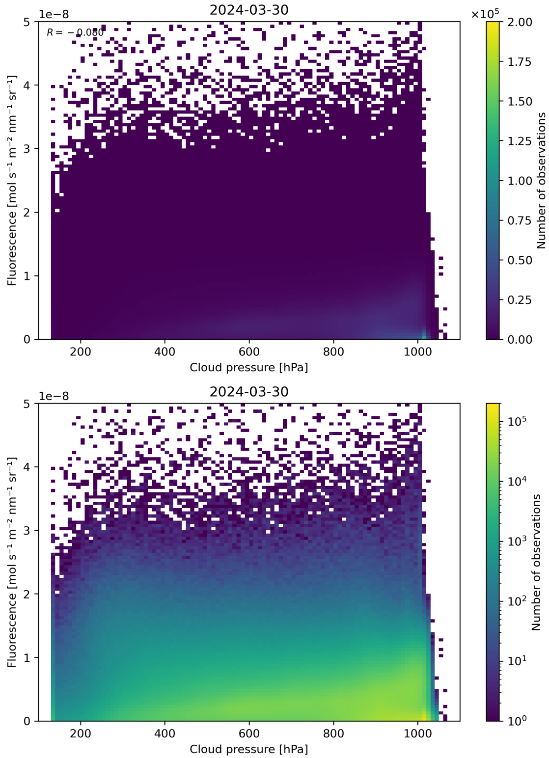
Figure 80: Scatter density plot of “Cloud pressure” against “Fluorescence” for 2024-03-30 to 2024-03-31.
