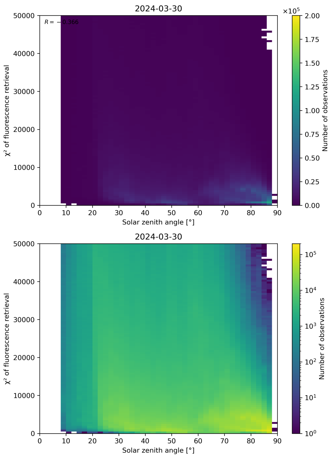
Figure 109: Scatter density plot of “Solar zenith angle” against “ \chi^2 of fluorescence retrieval” for 2024-03-30 to 2024-03-31.
