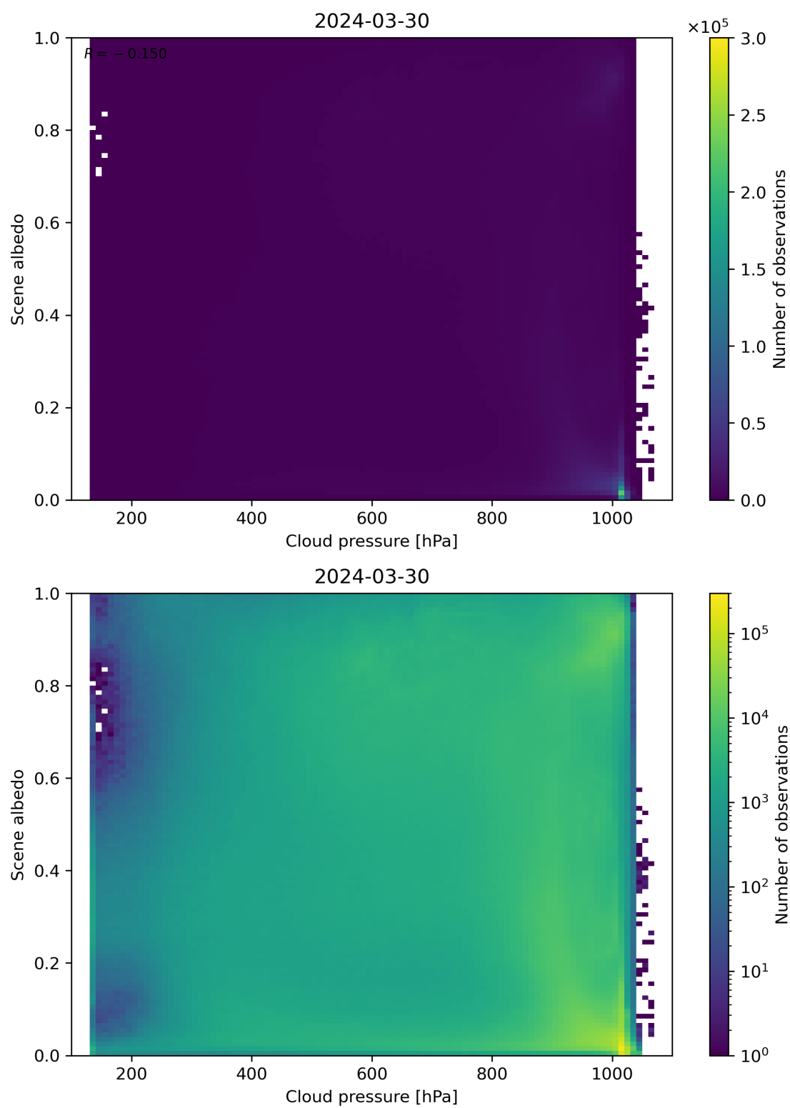
Figure 83: Scatter density plot of “Cloud pressure” against “Scene albedo” for 2024-03-30 to 2024-03-31.
