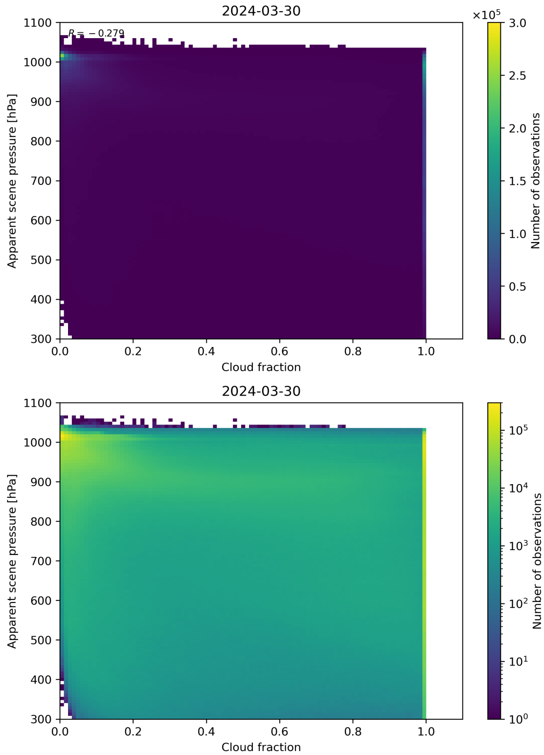
Figure 70: Scatter density plot of “Cloud fraction” against “Apparent scene pressure” for 2024-03-30 to 2024-03-31.
