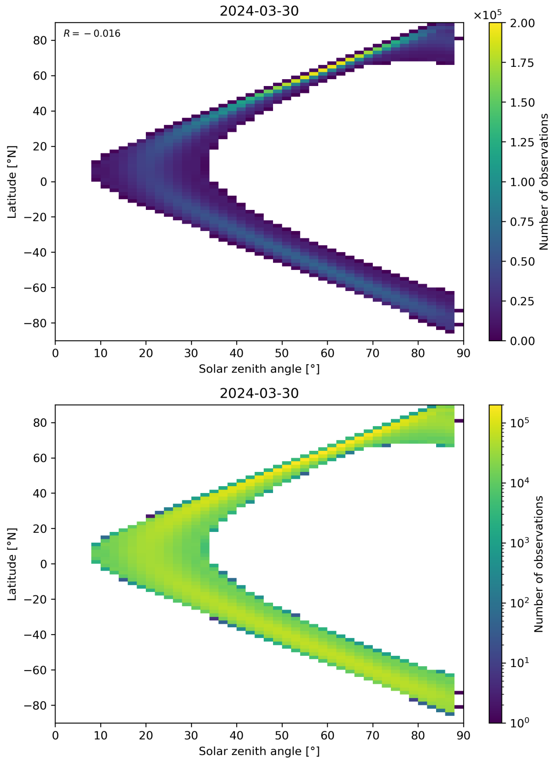
Figure 113: Scatter density plot of “Solar zenith angle” against “Latitude” for 2024-03-30 to 2024-03-31.
