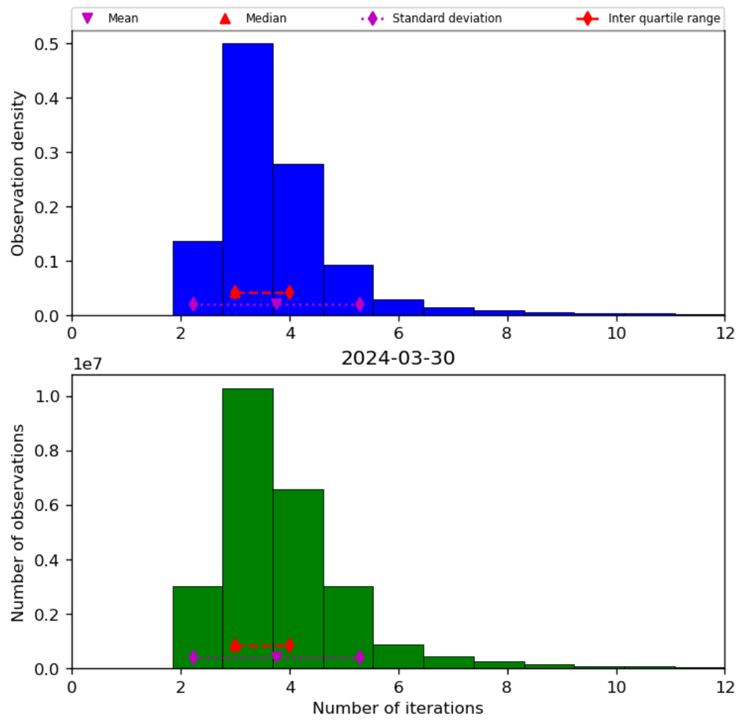
Figure 39: Histogram of “Number of iterations” for 2024-03-30 to 2024-03-31
