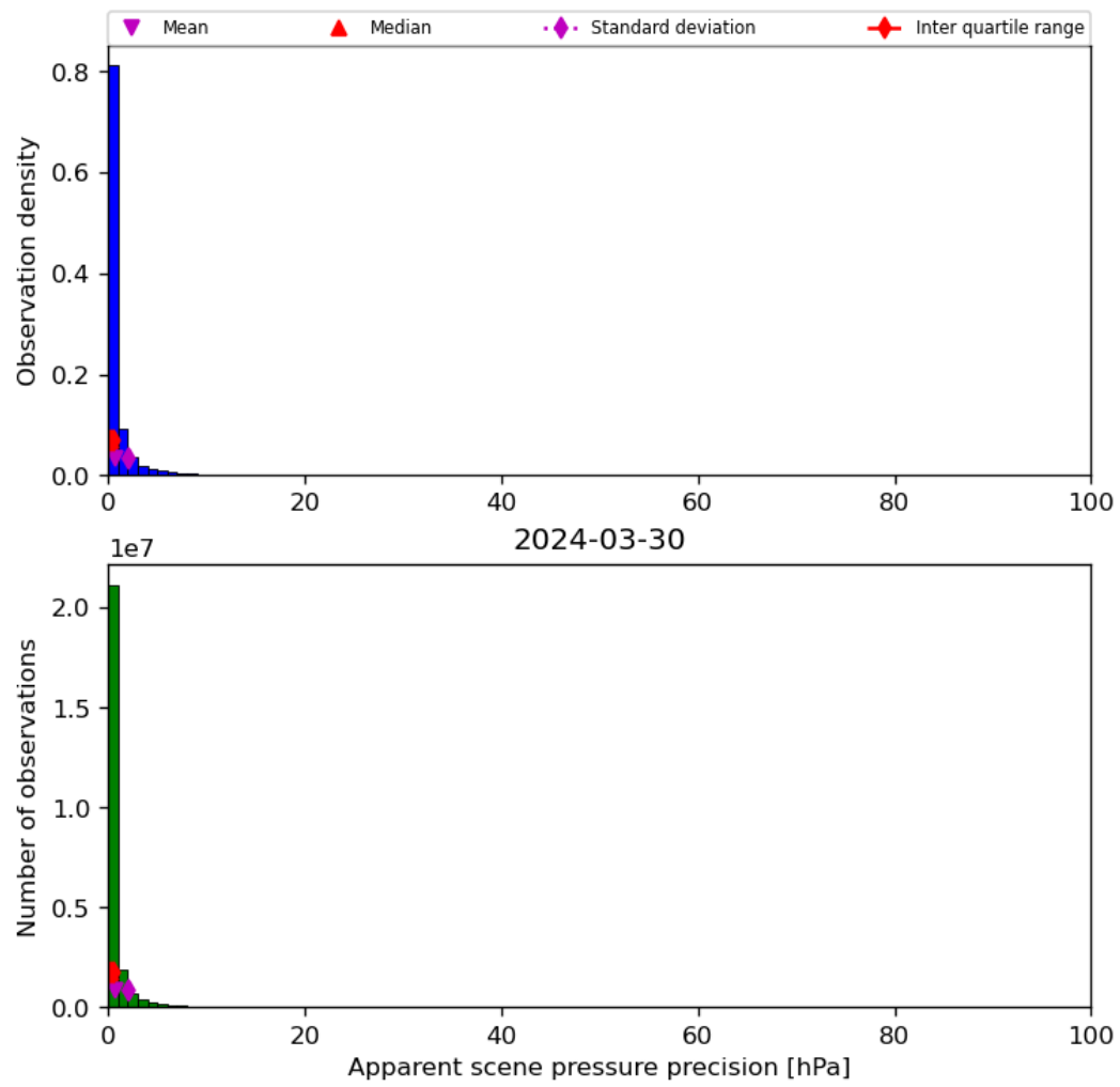
Figure 37: Histogram of “Apparent scene pressure precision” for 2024-03-30 to 2024-03-31
