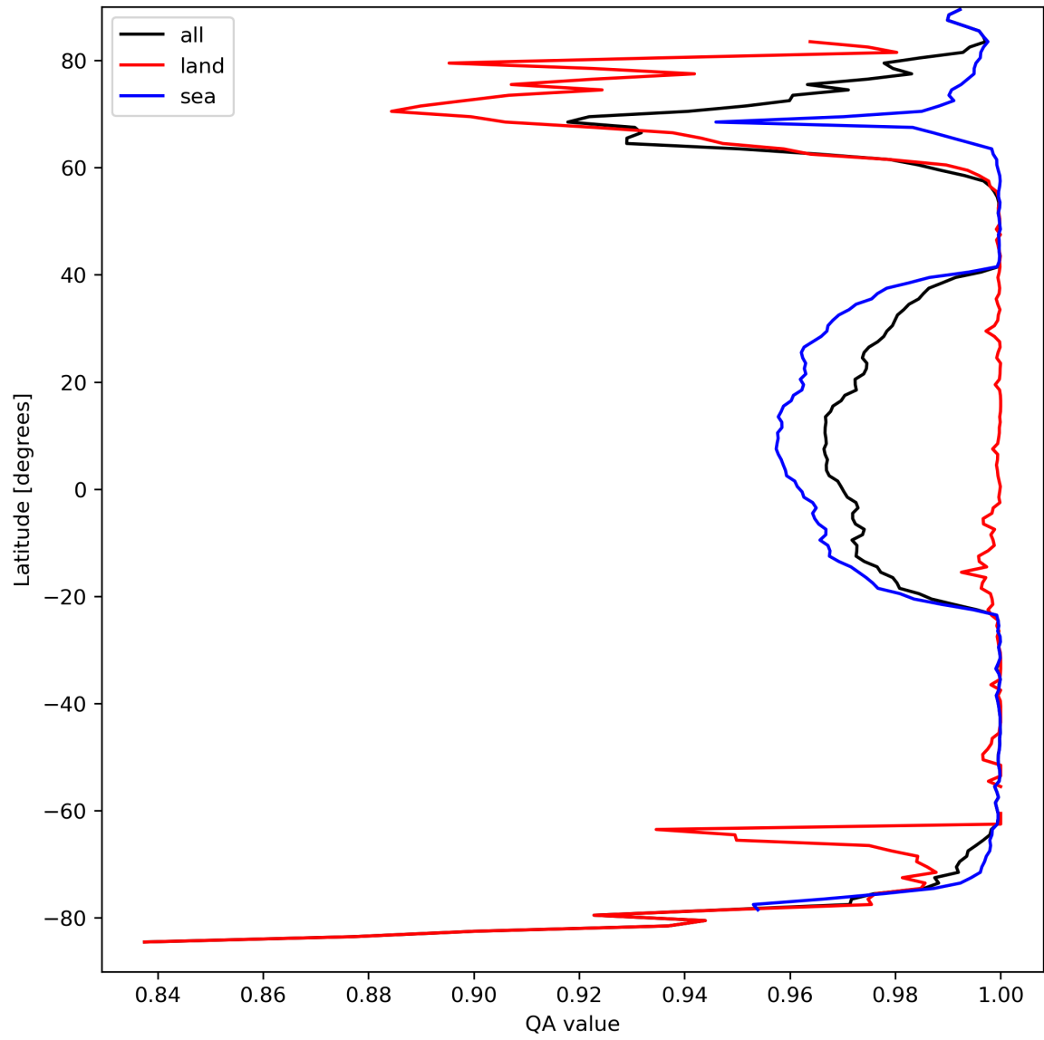
Figure 12: Zonal average of "QA value" for 2024-03-30 to 2024-03-31.
