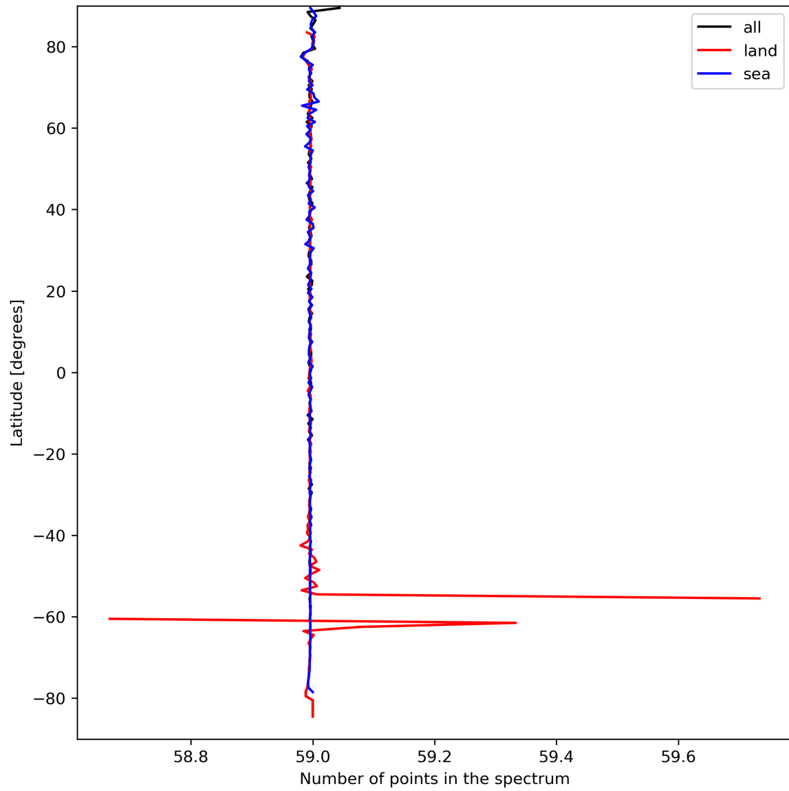
Figure 27: Zonal average of “Number of points in the spectrum” for 2024-03-30 to 2024-03-31.
