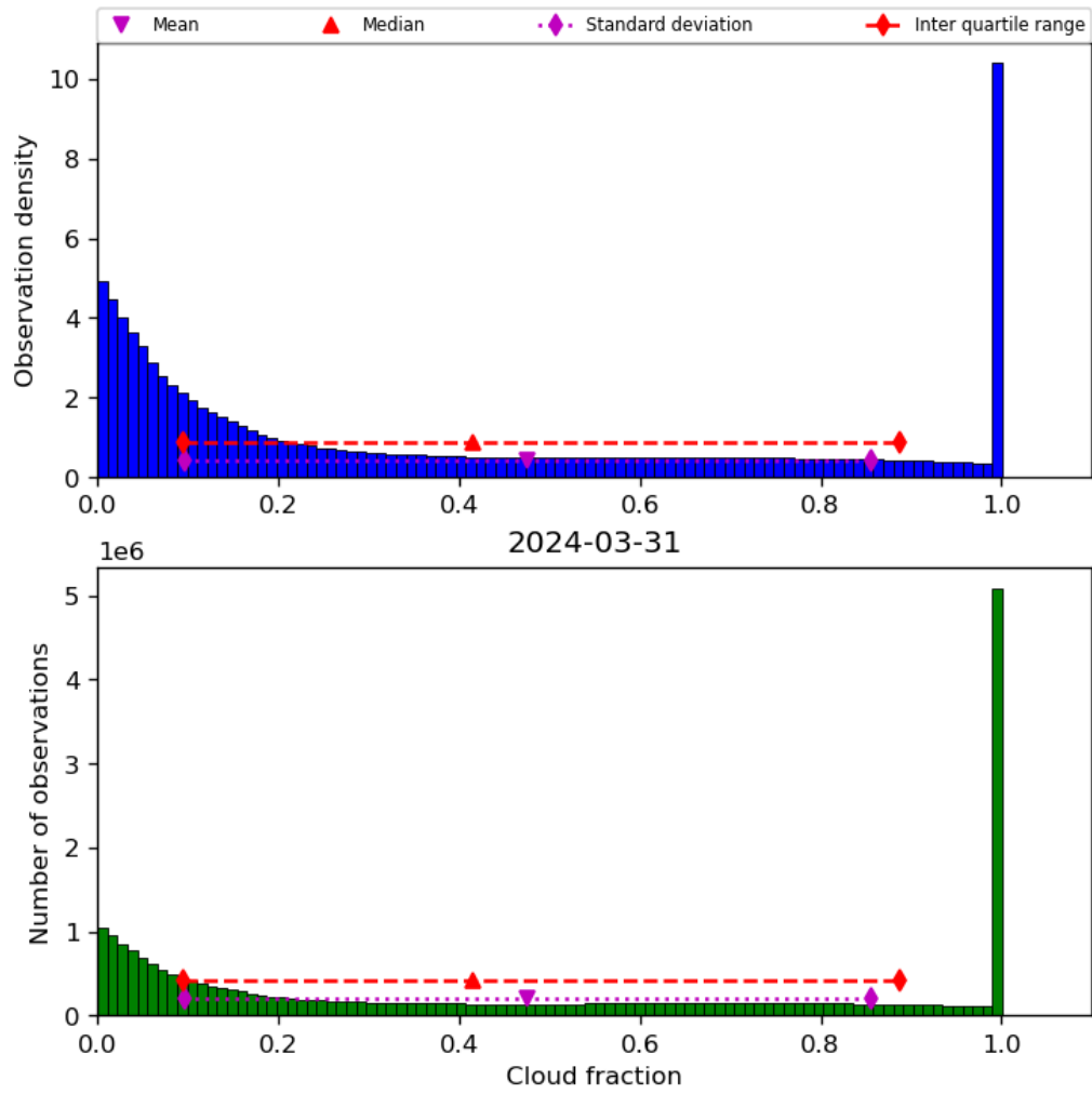
Figure 32: Histogram of “Cloud fraction” for 2024-03-31 to 2024-04-01
