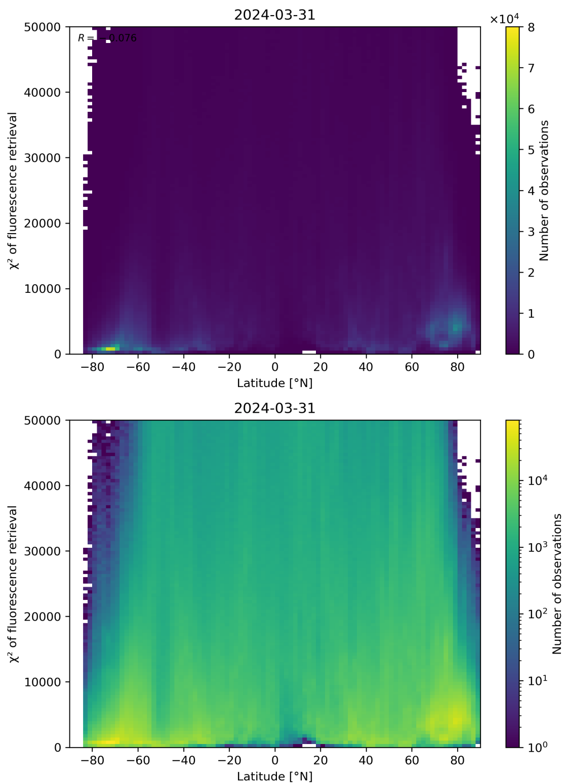
Figure 89: Scatter density plot of “Latitude” against “ \chi^2 of fluorescence retrieval” for 2024-03-31 to 2024-04-01.
