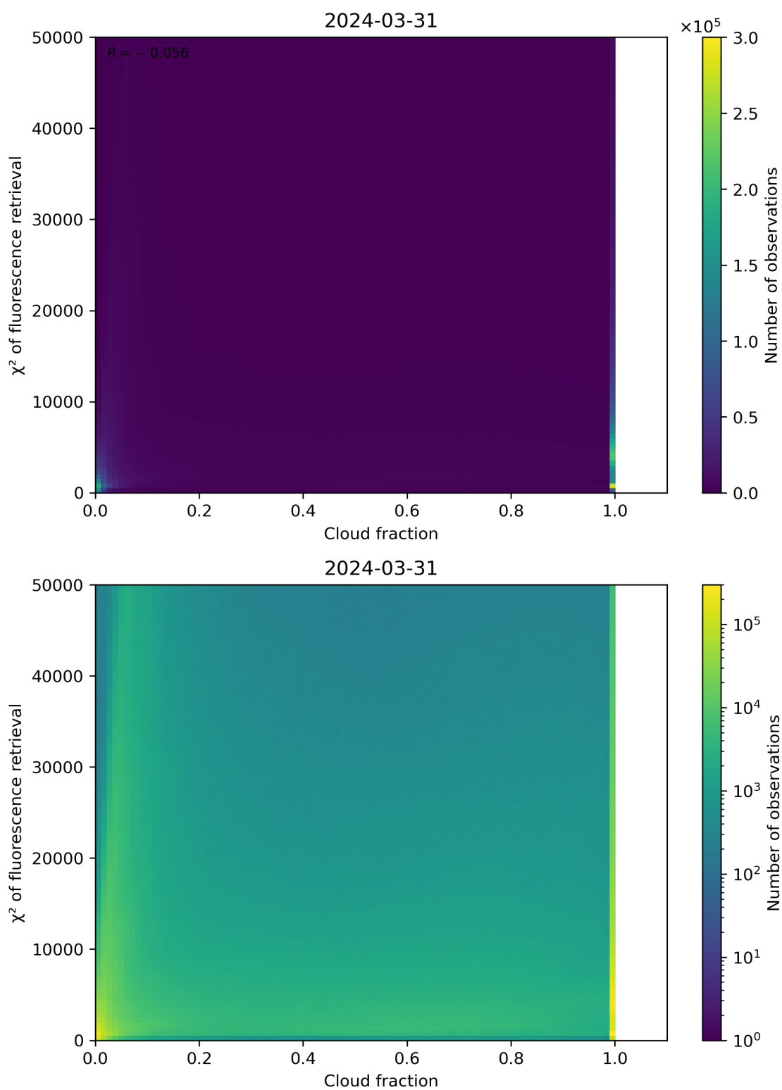
Figure 71: Scatter density plot of “Cloud fraction” against “ \chi^2 of fluorescence retrieval” for 2024-03-31 to 2024-04-01.
