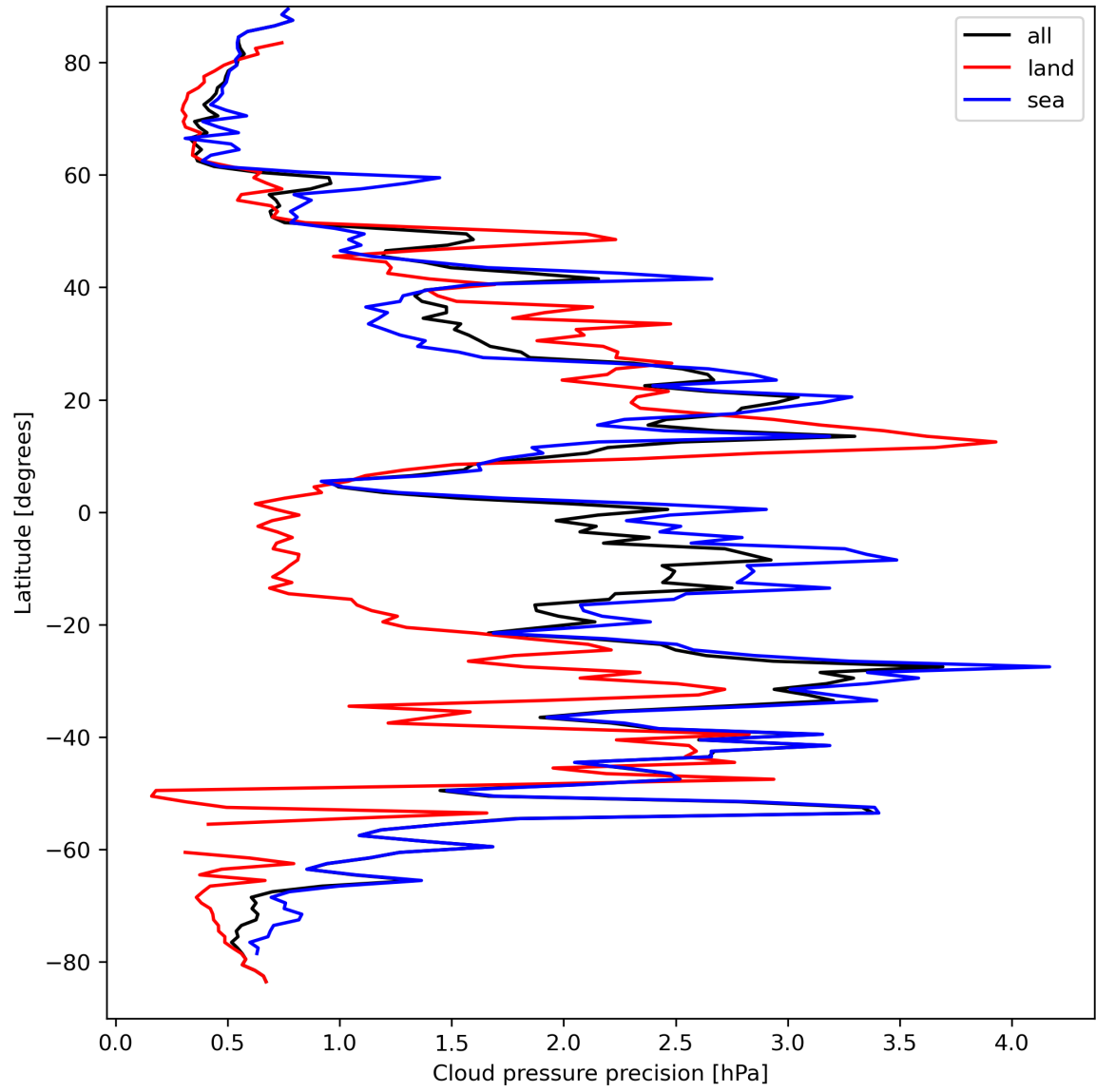
Figure 14: Zonal average of “Cloud pressure precision” for 2024-03-31 to 2024-04-01.
