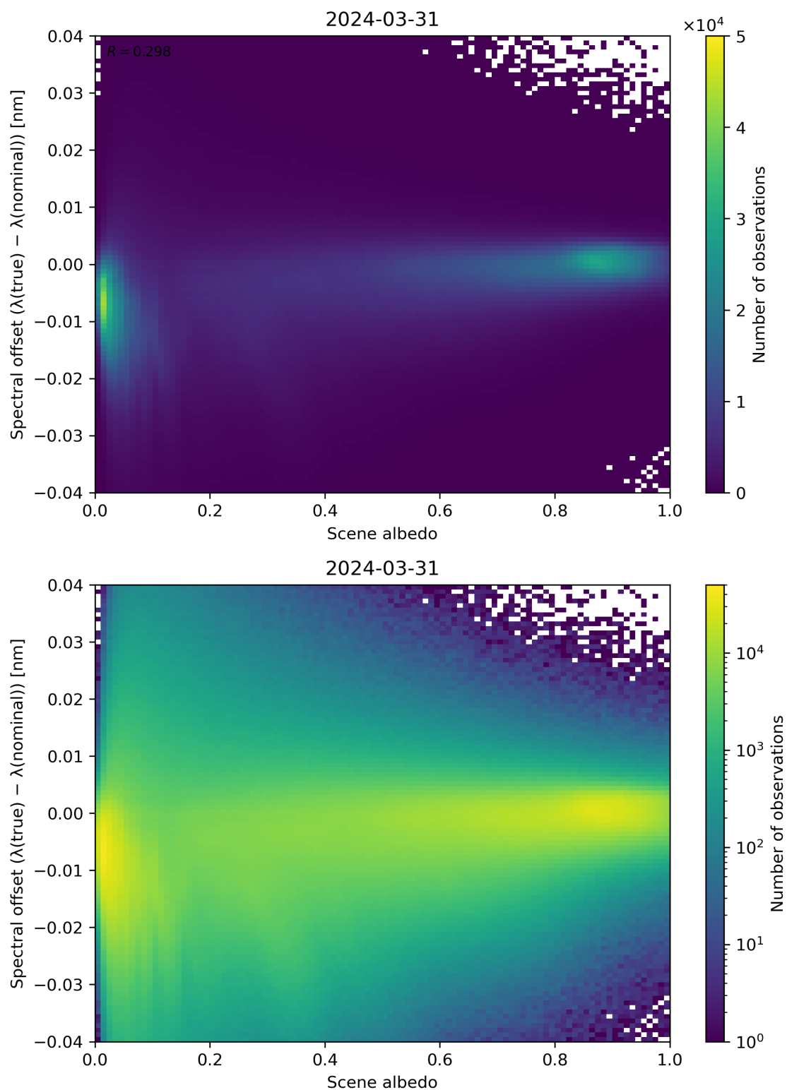
Figure 107: Scatter density plot of “Scene albedo” against “Spectral offset ( \lambda(\text{true}) - \lambda(\text{nominal}) )” for 2024-03-31 to 2024-04-01.
