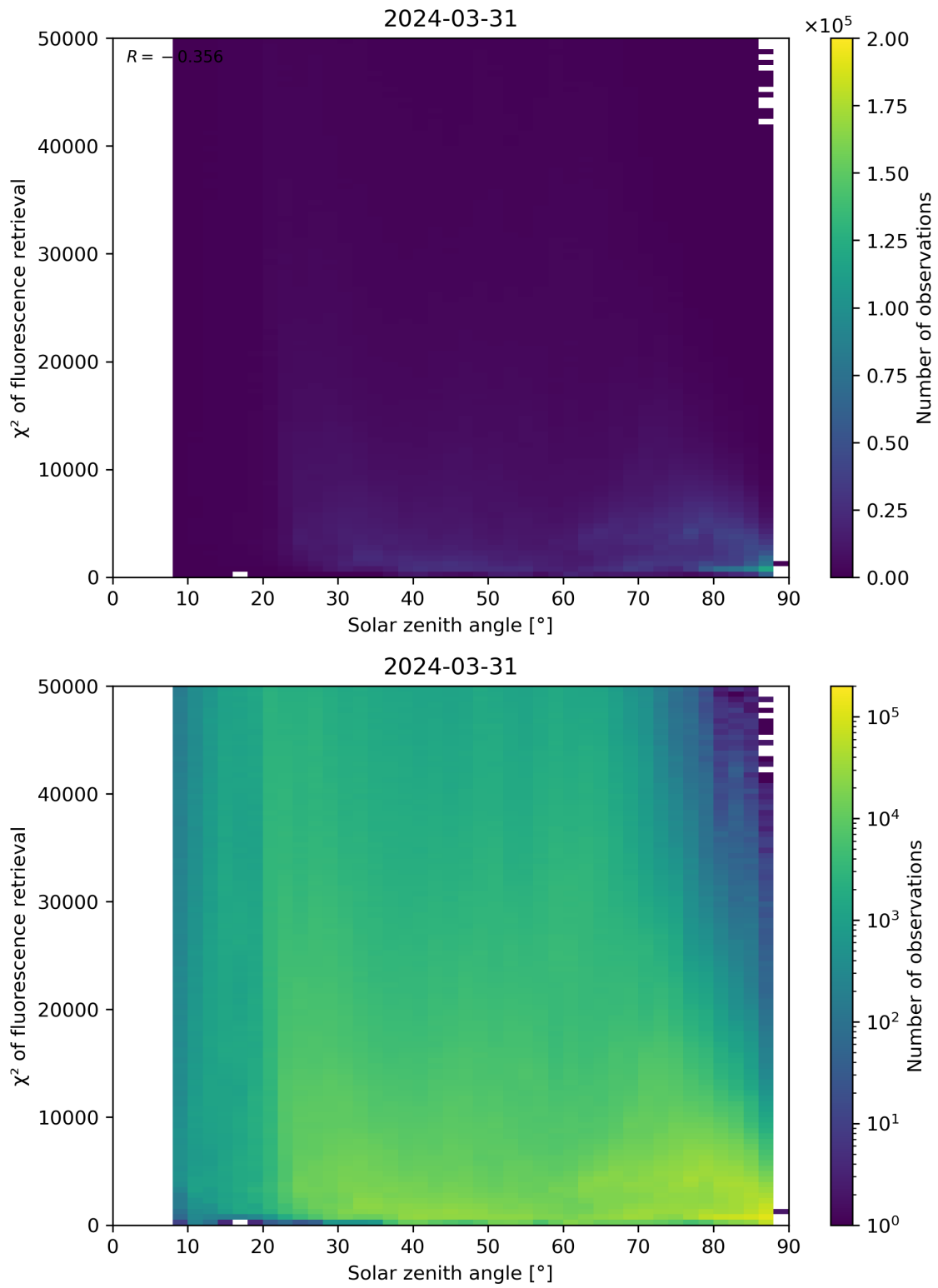
Figure 109: Scatter density plot of “Solar zenith angle” against “ \chi^2 of fluorescence retrieval” for 2024-03-31 to 2024-04-01.
