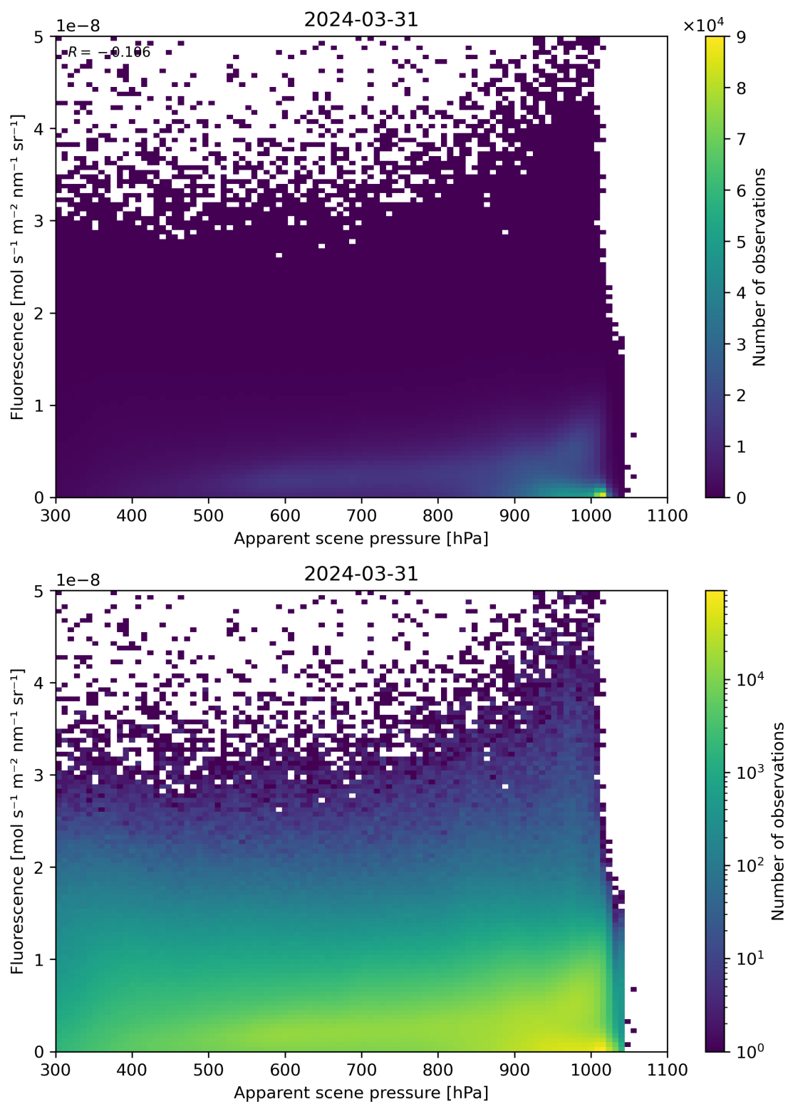
Figure 64: Scatter density plot of “Apparent scene pressure” against “Fluorescence” for 2024-03-31 to 2024-04-01.
