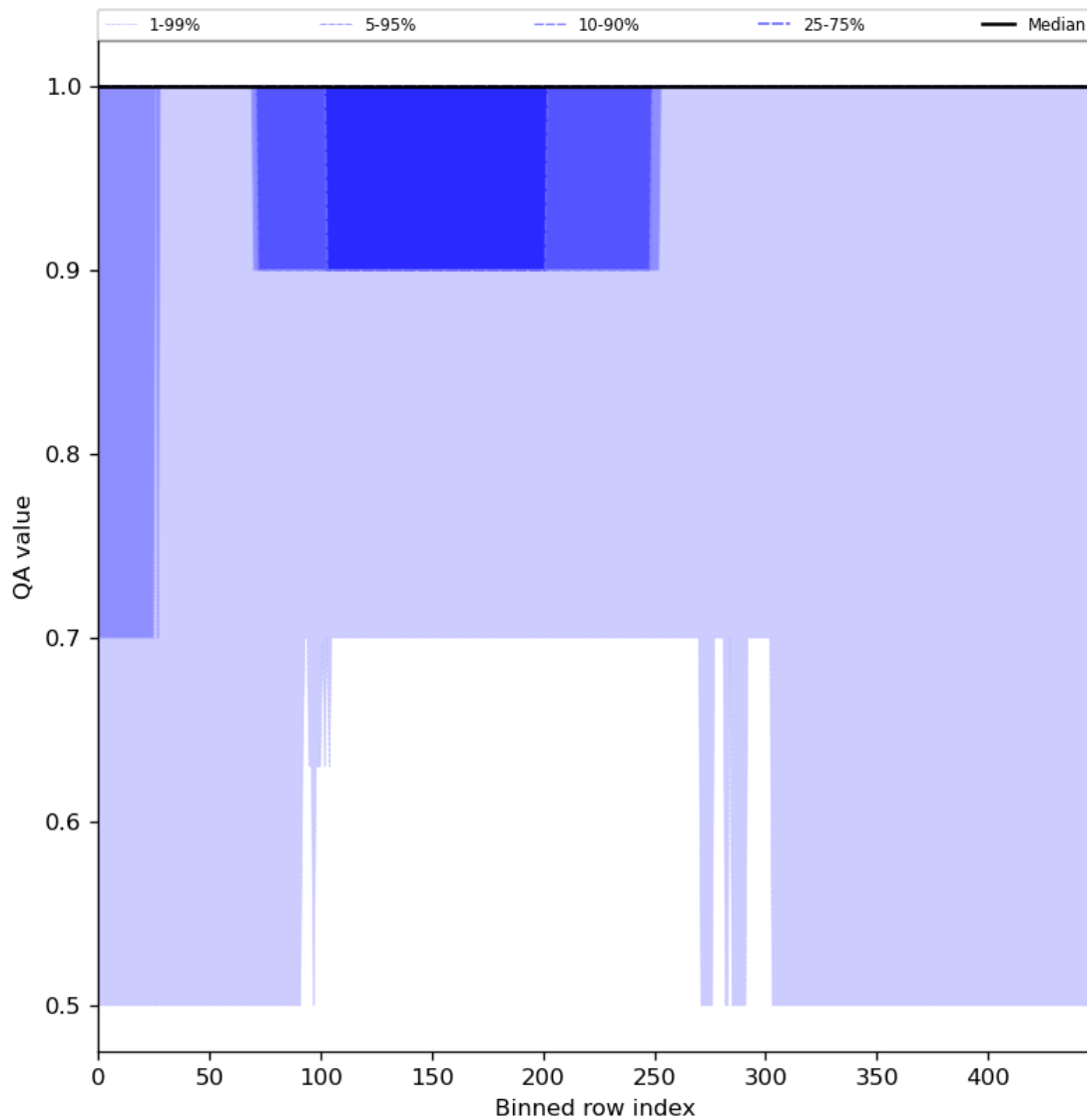
Figure 46: Along track statistics of “QA value” for 2024-03-31 to 2024-04-01
