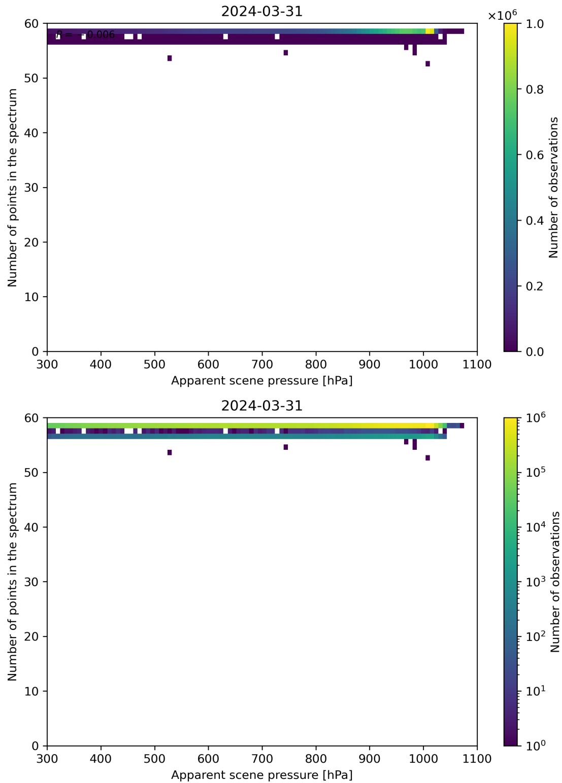
Figure 66: Scatter density plot of “Apparent scene pressure” against “Number of points in the spectrum” for 2024-03-31 to 2024-04-01.
