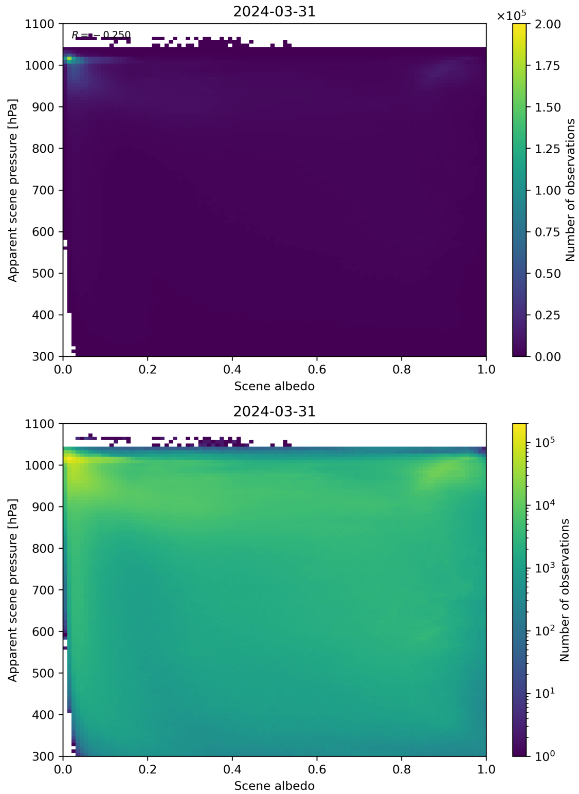
Figure 102: Scatter density plot of “Scene albedo” against “Apparent scene pressure” for 2024-03-31 to 2024-04-01.
