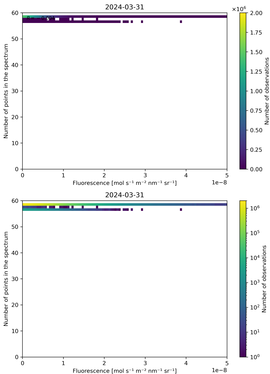
Figure 86: Scatter density plot of “Fluorescence” against “Number of points in the spectrum” for 2024-03-31 to 2024-04-01.
