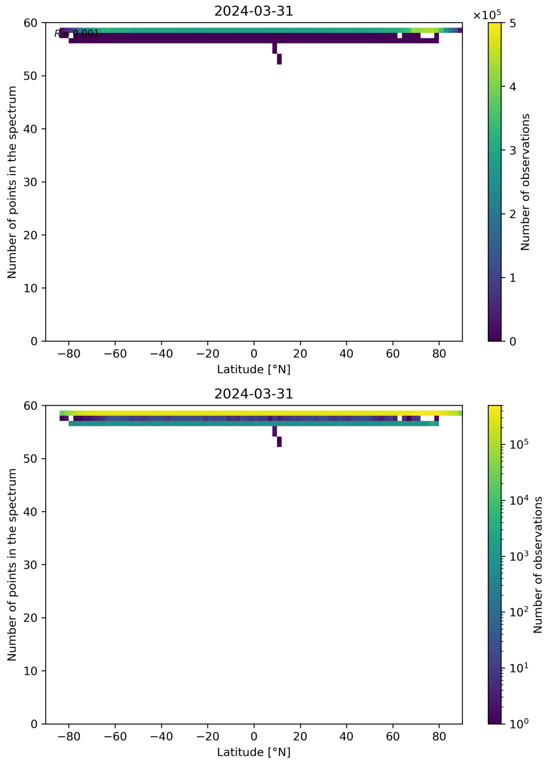
Figure 94: Scatter density plot of “Latitude” against “Number of points in the spectrum” for 2024-03-31 to 2024-04-01.
