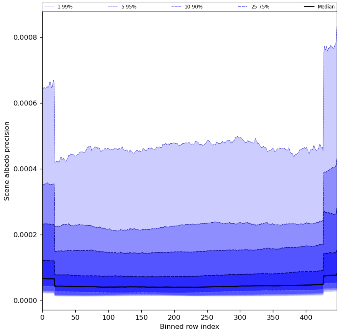
Figure 52: Along track statistics of “Scene albedo precision” for 2024-03-31 to 2024-04-01
