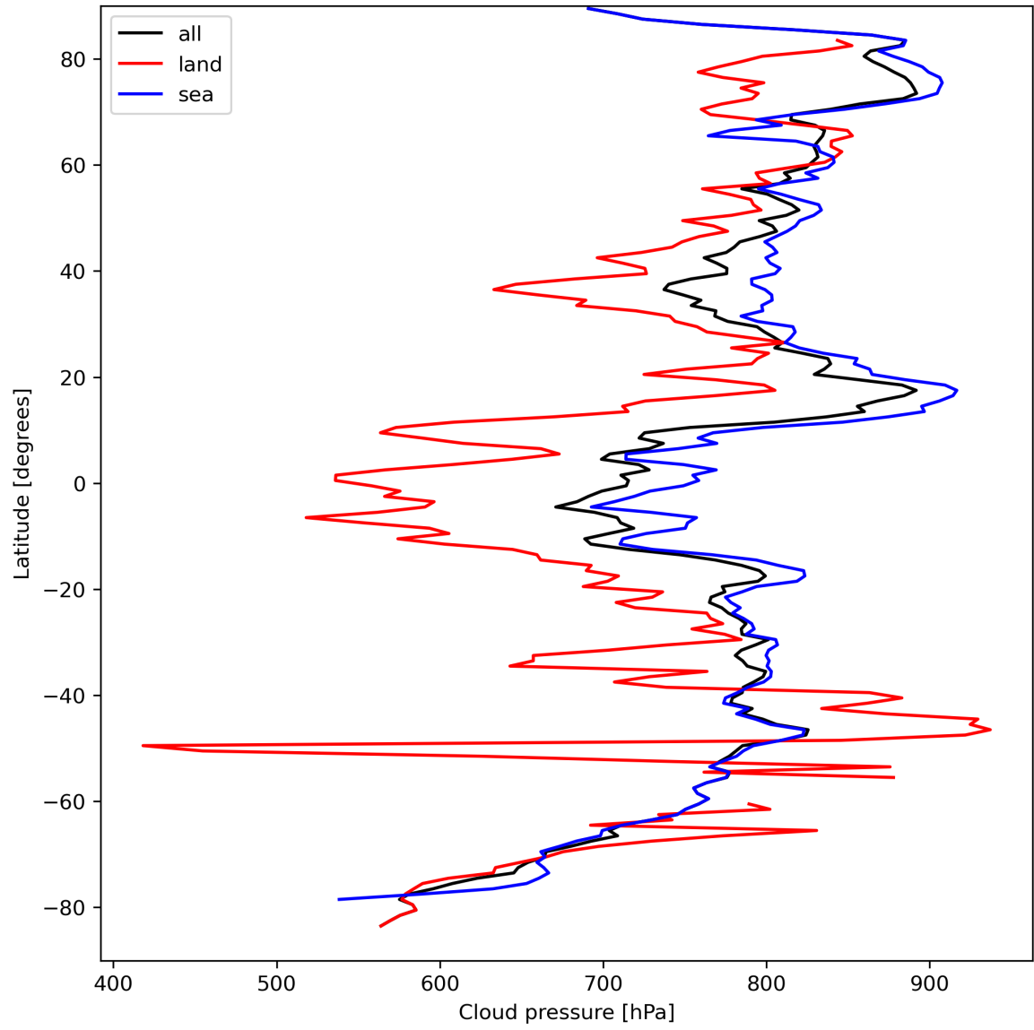
Figure 13: Zonal average of “Cloud pressure” for 2024-03-31 to 2024-04-01.
