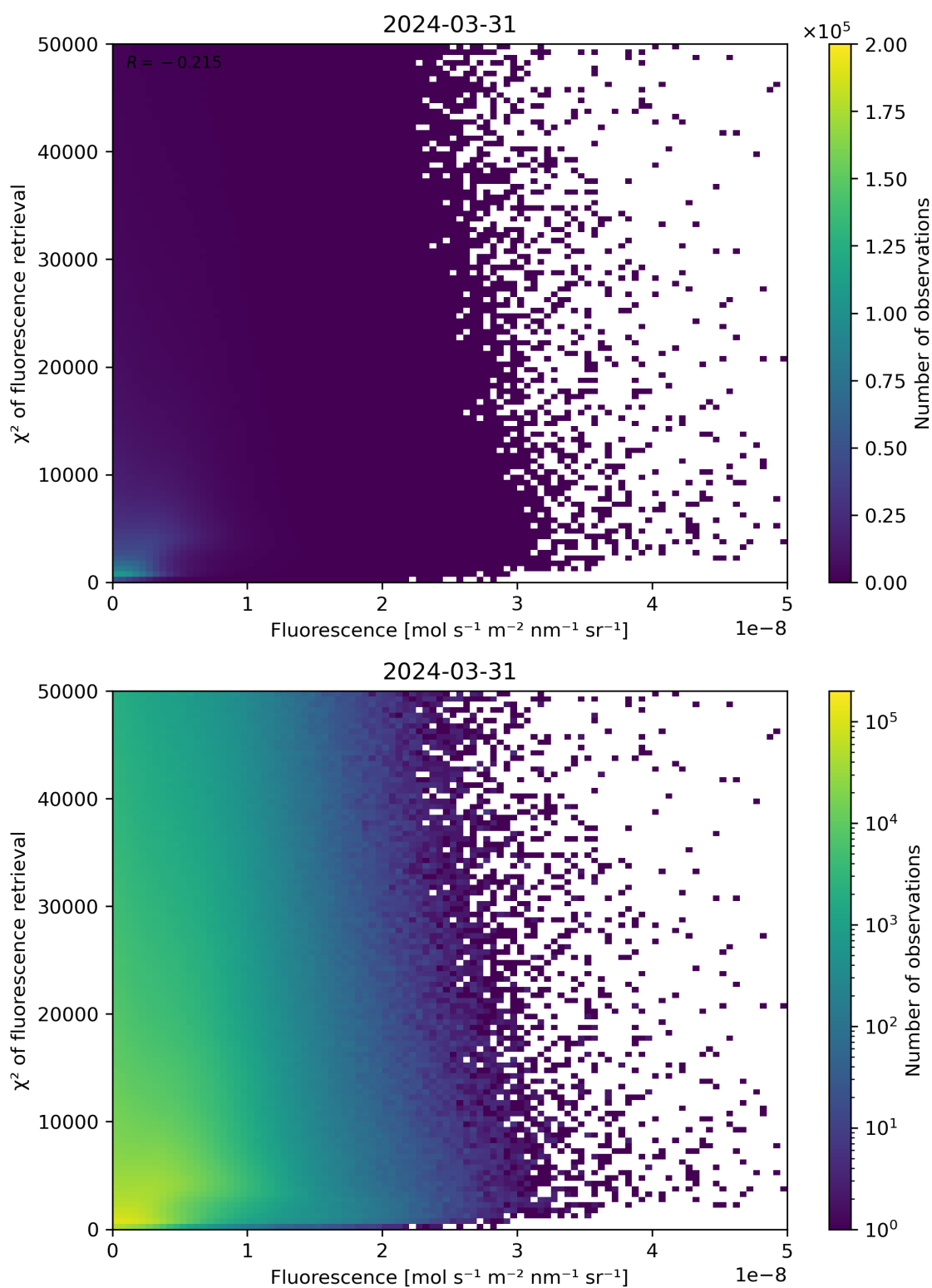
Figure 85: Scatter density plot of “Fluorescence” against “ \chi^2 of fluorescence retrieval” for 2024-03-31 to 2024-04-01.
