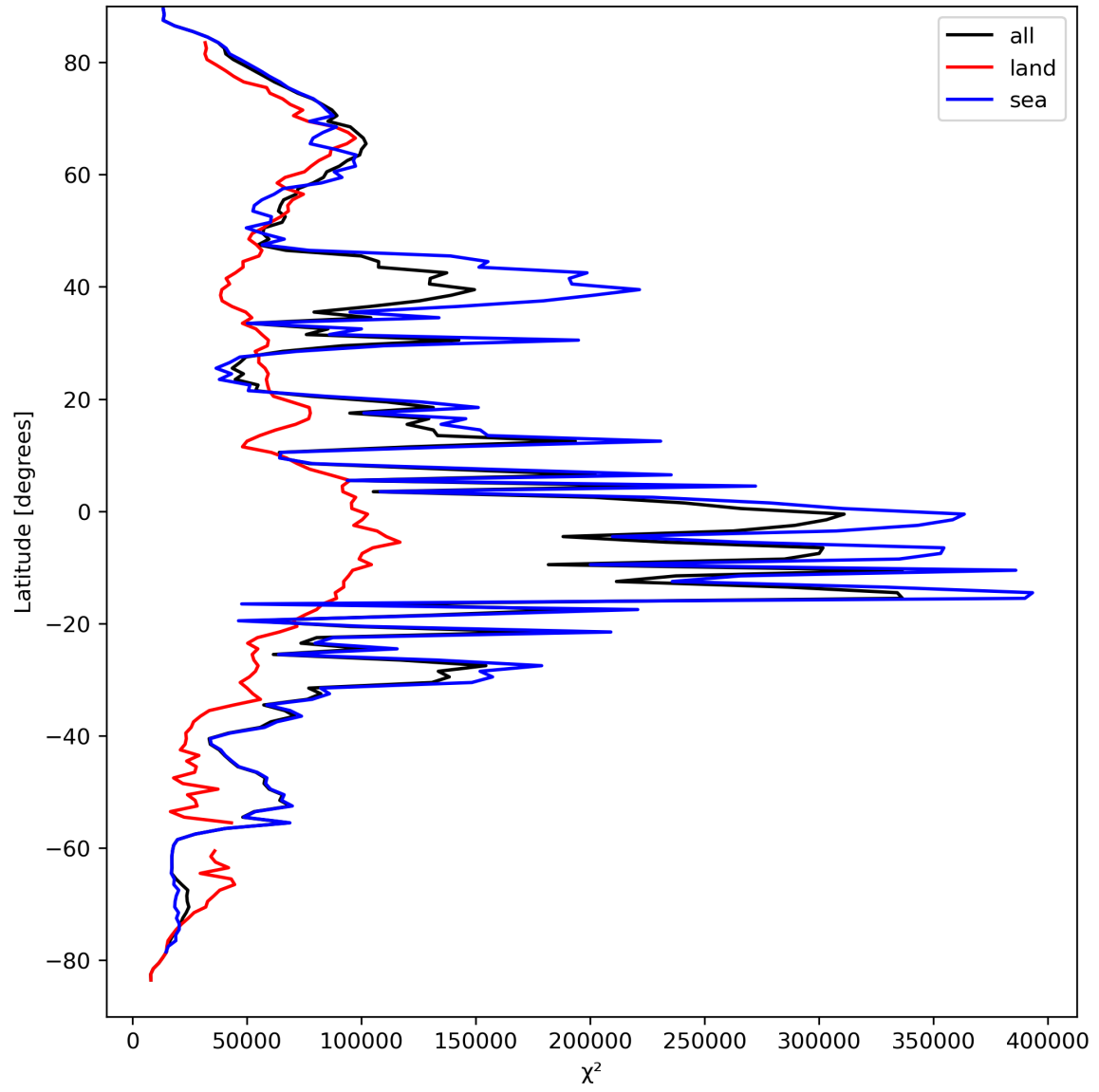
Figure 21: Zonal average of “ \chi^2 ” for 2024-03-31 to 2024-04-01.
