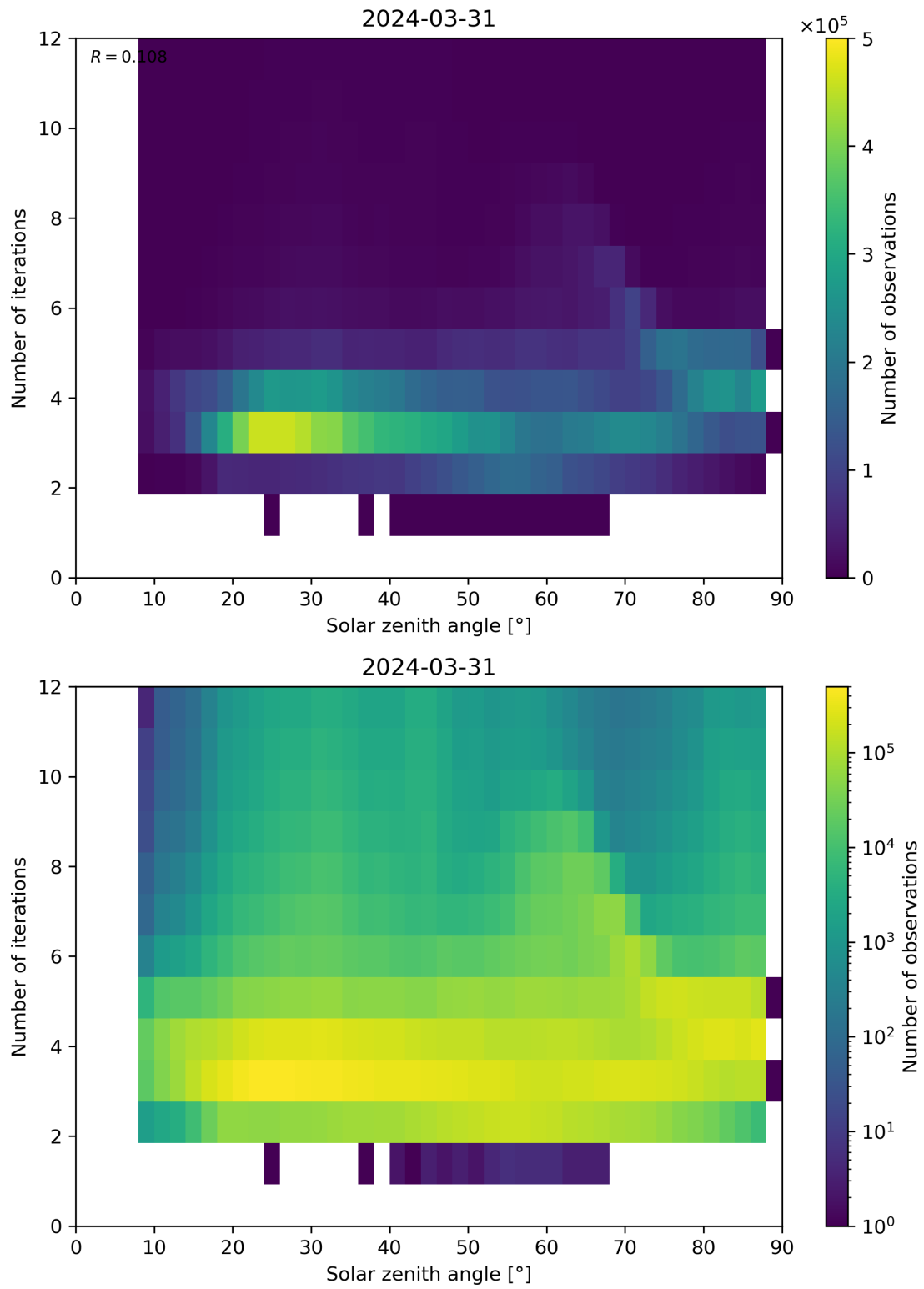
Figure 114: Scatter density plot of “Solar zenith angle” against “Number of iterations” for 2024-03-31 to 2024-04-01.
