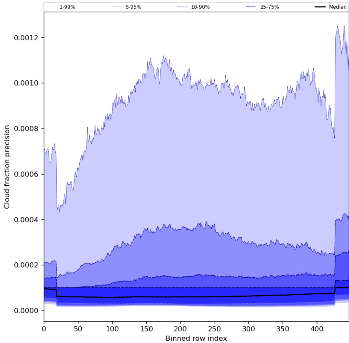
Figure 50: Along track statistics of “Cloud fraction precision” for 2024-03-31 to 2024-04-01
