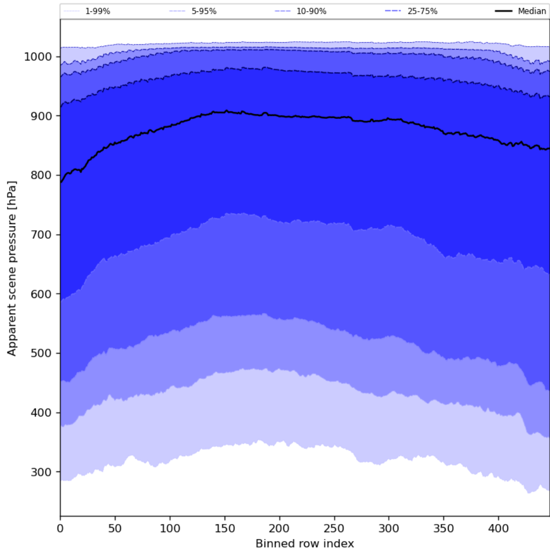
Figure 53: Along track statistics of “Apparent scene pressure” for 2024-03-31 to 2024-04-01
