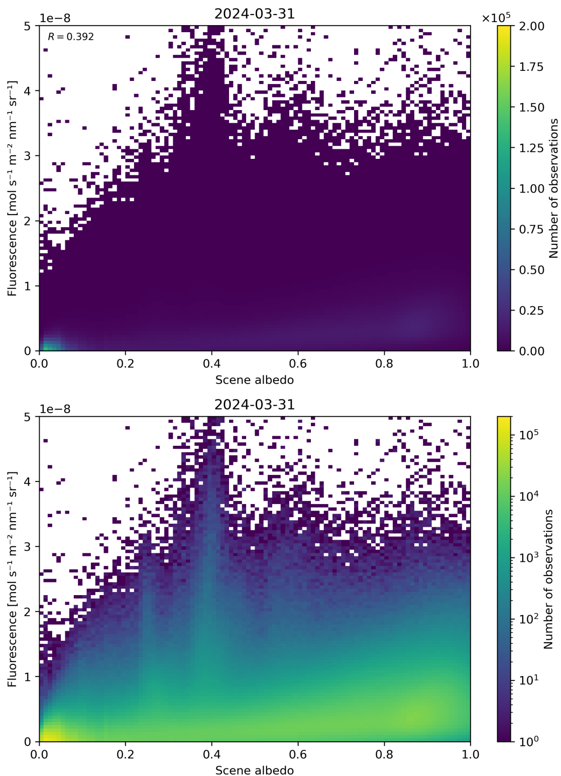
Figure 104: Scatter density plot of “Scene albedo” against “Fluorescence” for 2024-03-31 to 2024-04-01.
