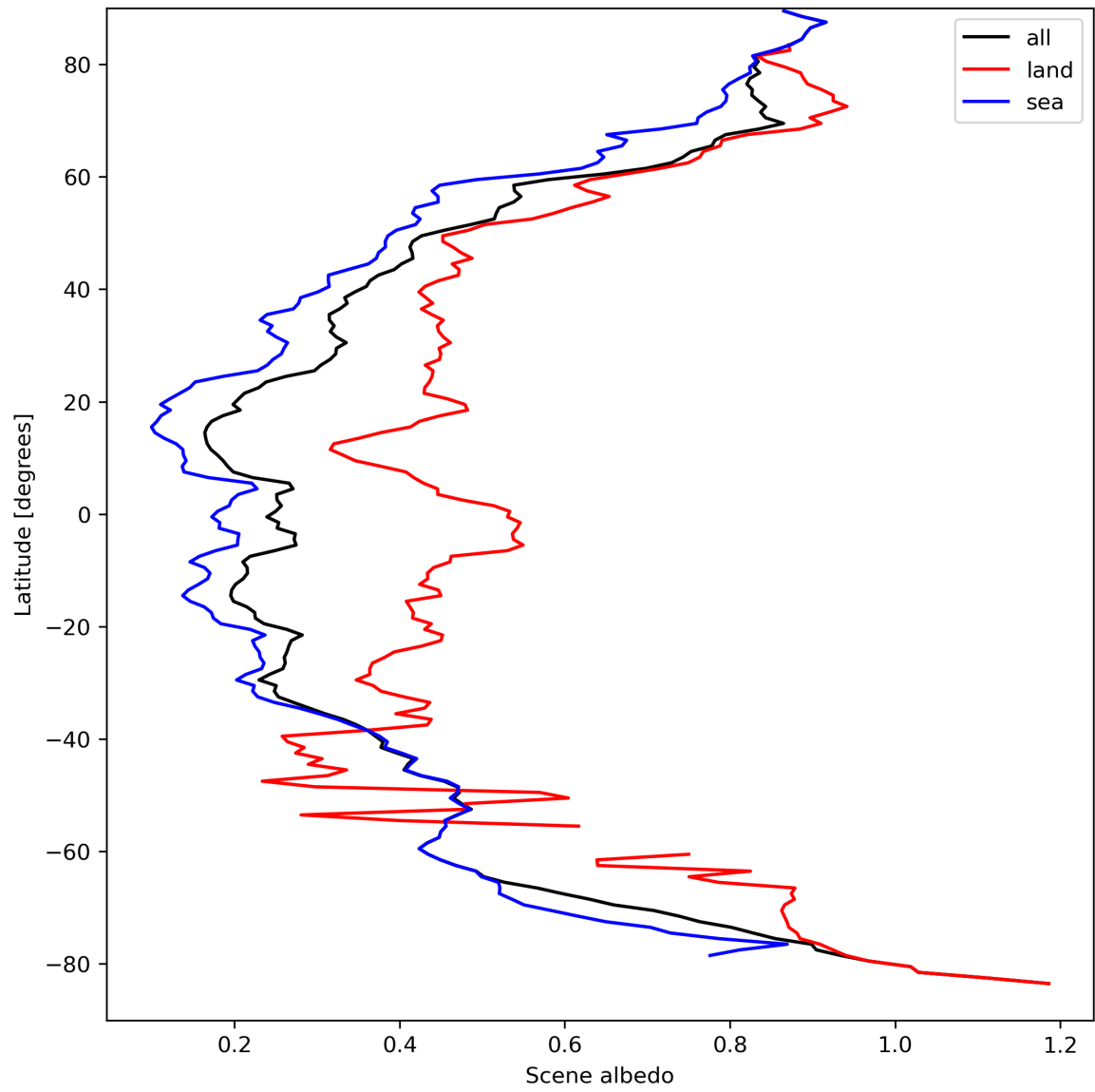
Figure 17: Zonal average of “Scene albedo” for 2024-03-31 to 2024-04-01.
