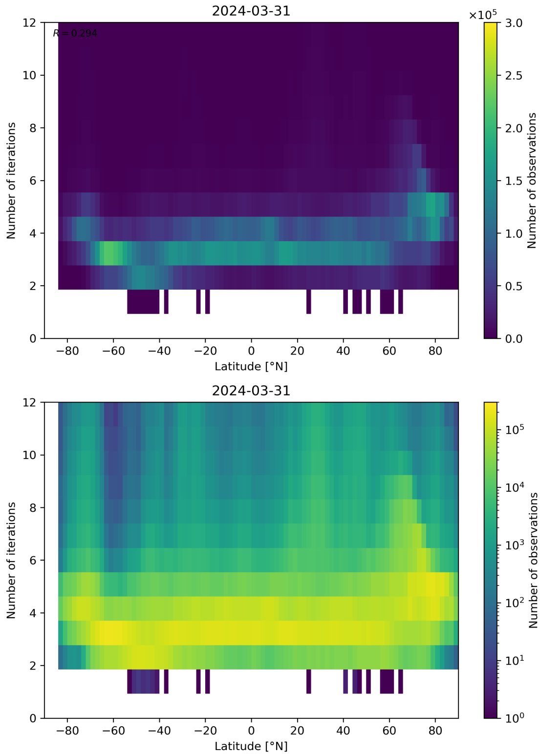
Figure 93: Scatter density plot of “Latitude” against “Number of iterations” for 2024-03-31 to 2024-04-01.
