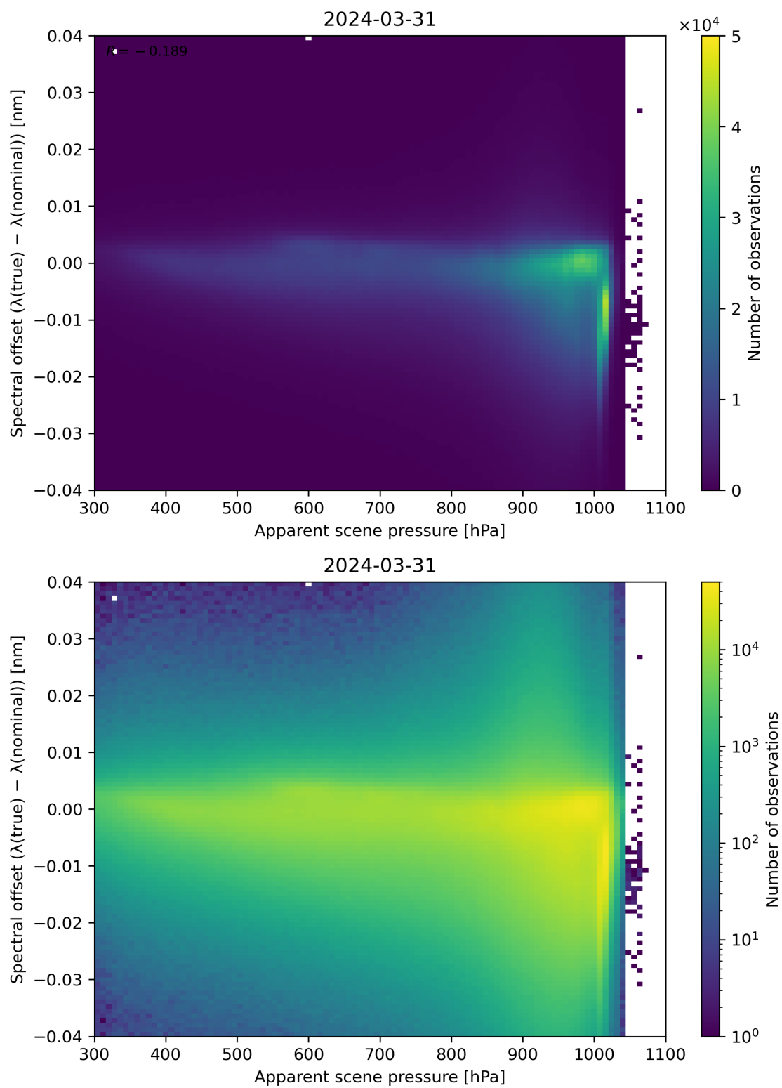
Figure 67: Scatter density plot of “Apparent scene pressure” against “Spectral offset ( \lambda(\text{true}) - \lambda(\text{nominal}) )” for 2024-03-31 to 2024-04-01.
