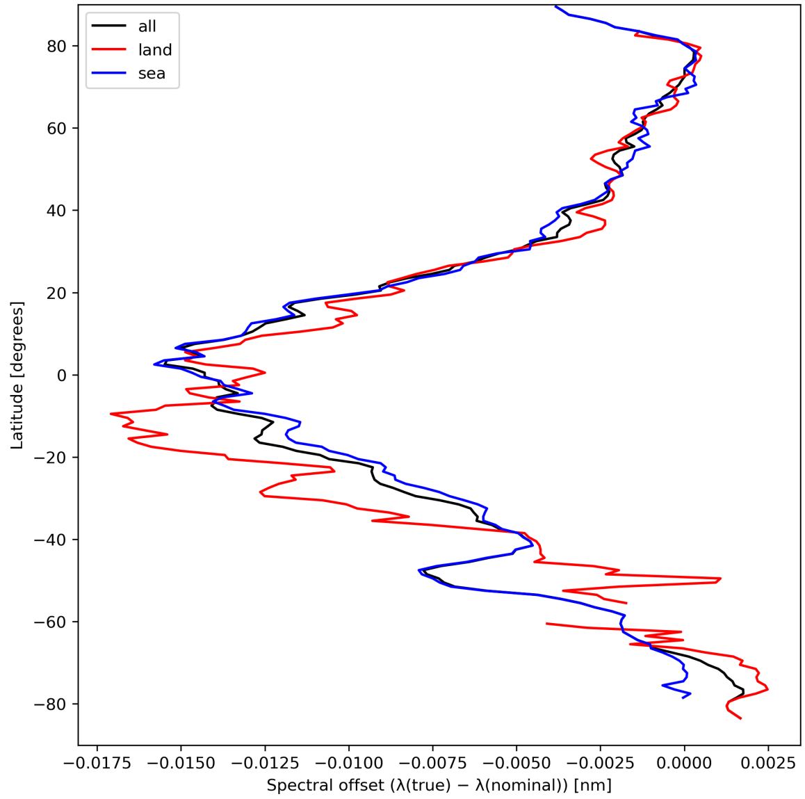
Figure 28: Zonal average of “Spectral offset ( \lambda(\text{true}) - \lambda(\text{nominal}) )” for 2024-03-31 to 2024-04-01.
