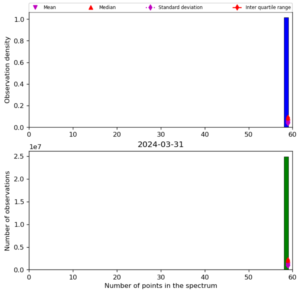
Figure 44: Histogram of “Number of points in the spectrum” for 2024-03-31 to 2024-04-01
