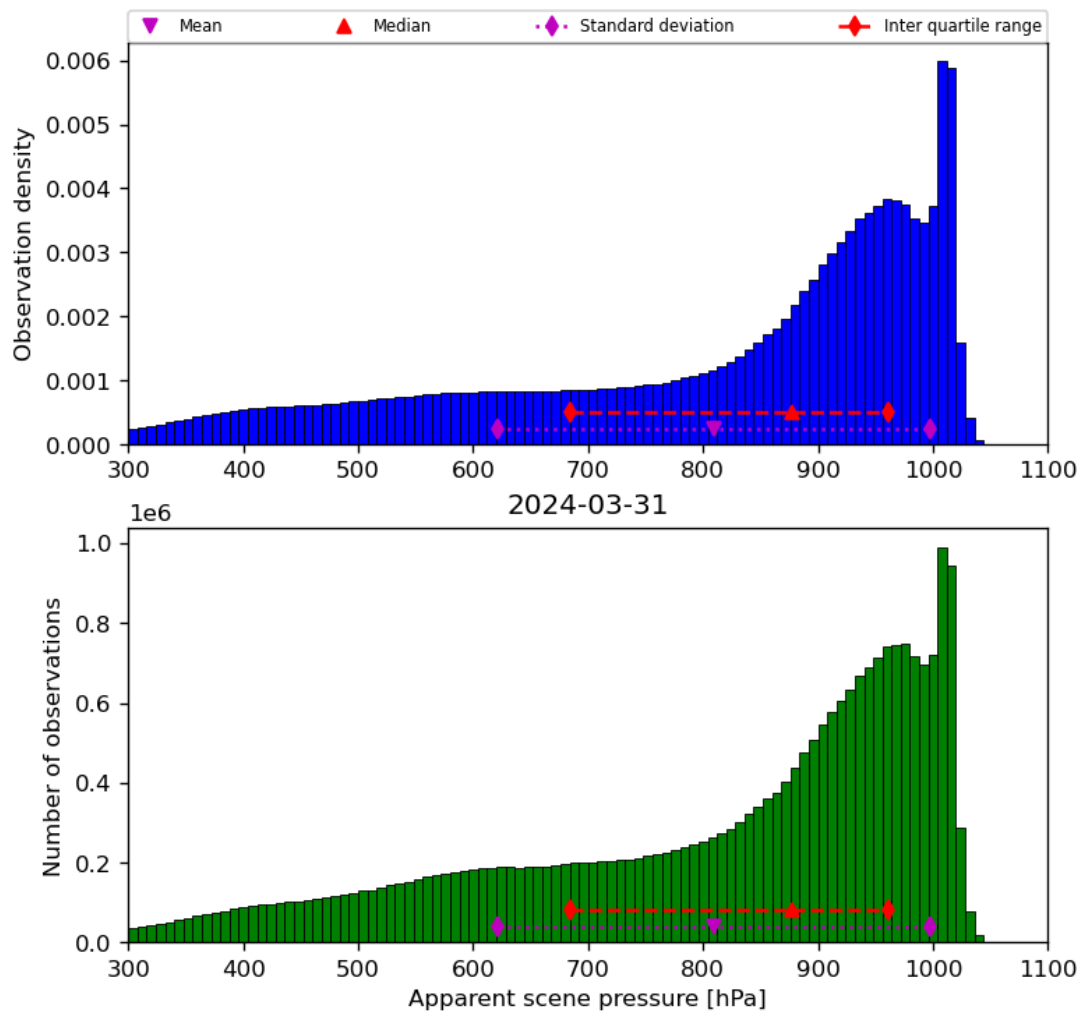
Figure 36: Histogram of “Apparent scene pressure” for 2024-03-31 to 2024-04-01
