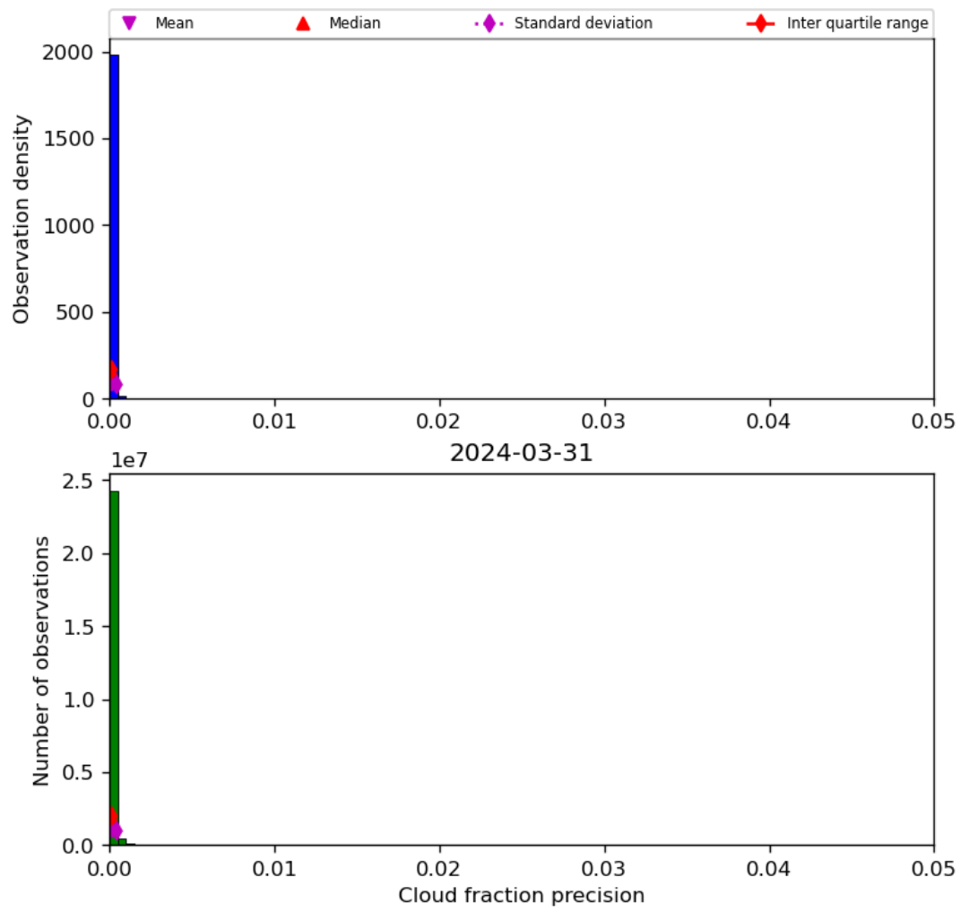
Figure 33: Histogram of “Cloud fraction precision” for 2024-03-31 to 2024-04-01
