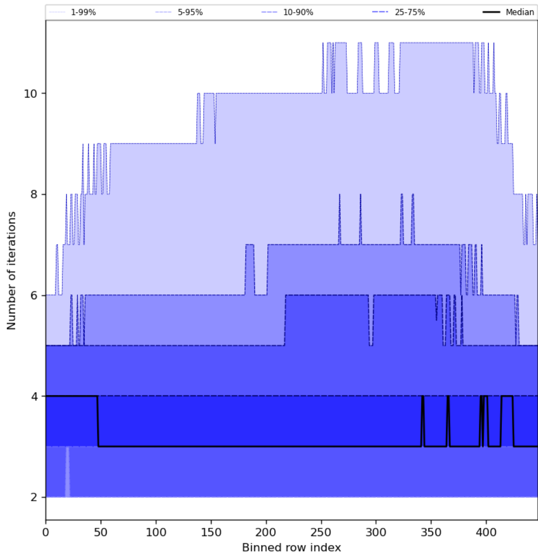
Figure 56: Along track statistics of “Number of iterations” for 2024-03-31 to 2024-04-01
