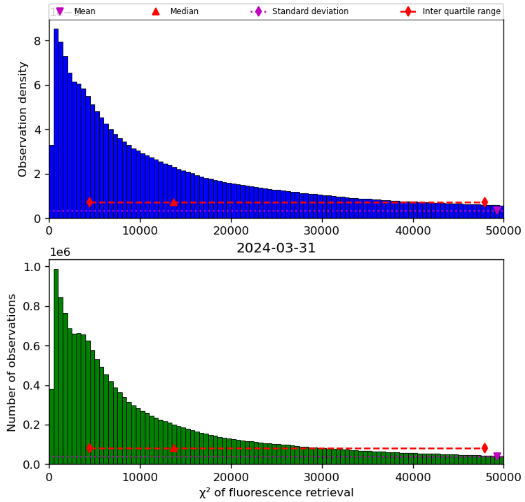
Figure 42: Histogram of “ \chi^2 of fluorescence retrieval” for 2024-03-31 to 2024-04-01
