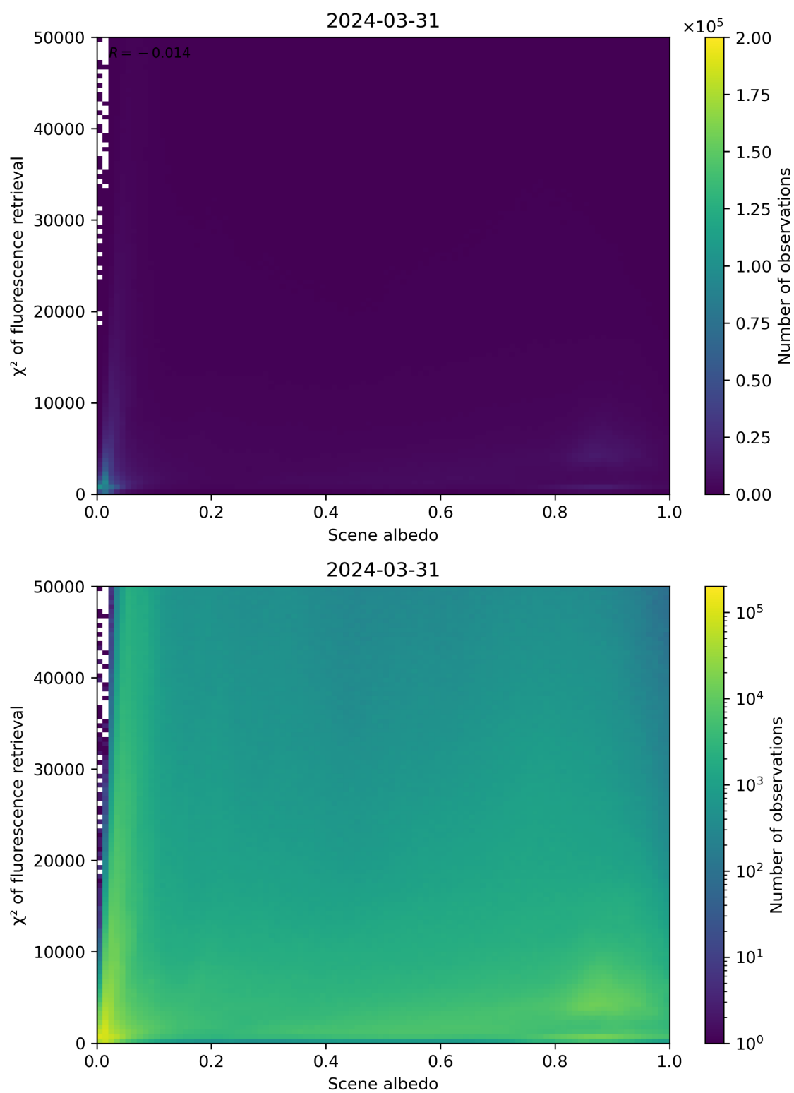
Figure 103: Scatter density plot of “Scene albedo” against “ \chi^2 of fluorescence retrieval” for 2024-03-31 to 2024-04-01.
