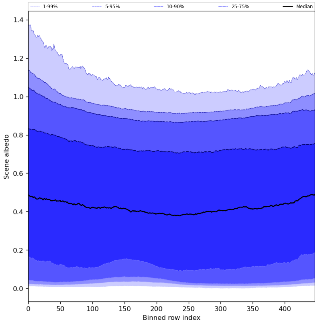
Figure 51: Along track statistics of “Scene albedo” for 2024-03-31 to 2024-04-01
