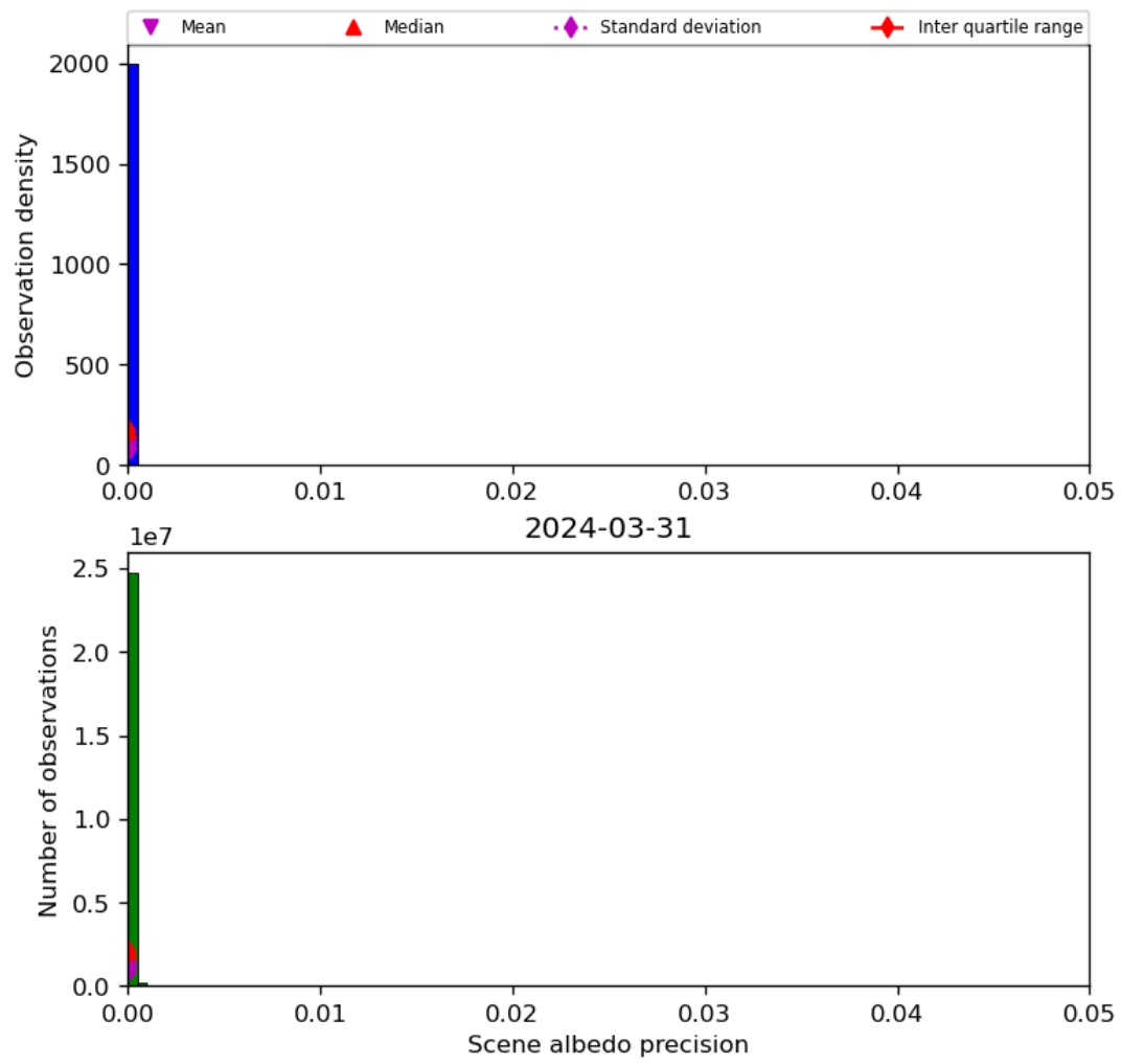
Figure 35: Histogram of “Scene albedo precision” for 2024-03-31 to 2024-04-01
