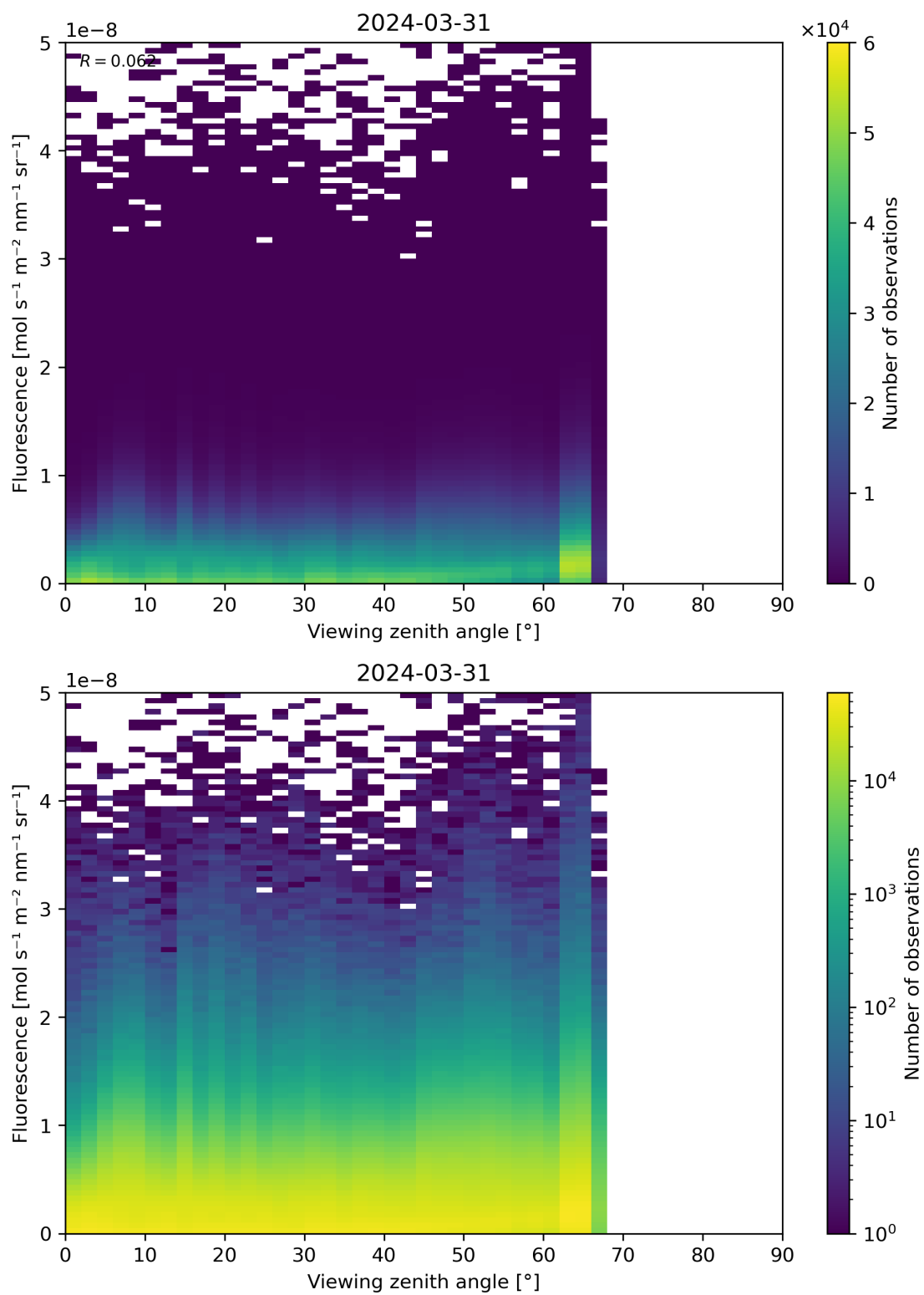
Figure 122: Scatter density plot of “Viewing zenith angle” against “Fluorescence” for 2024-03-31 to 2024-04-01.
