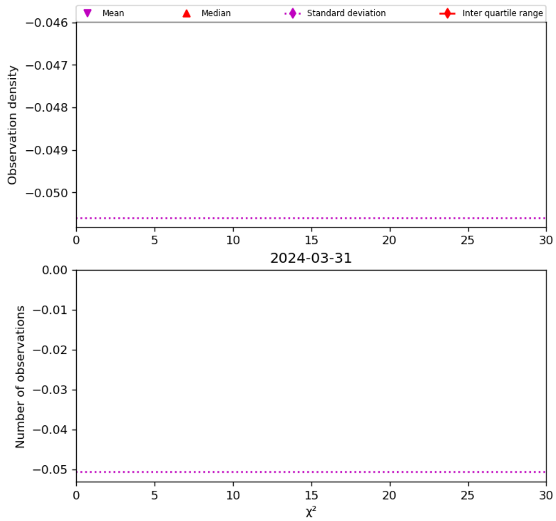
Figure 38: Histogram of “ \chi^2 ” for 2024-03-31 to 2024-04-01
