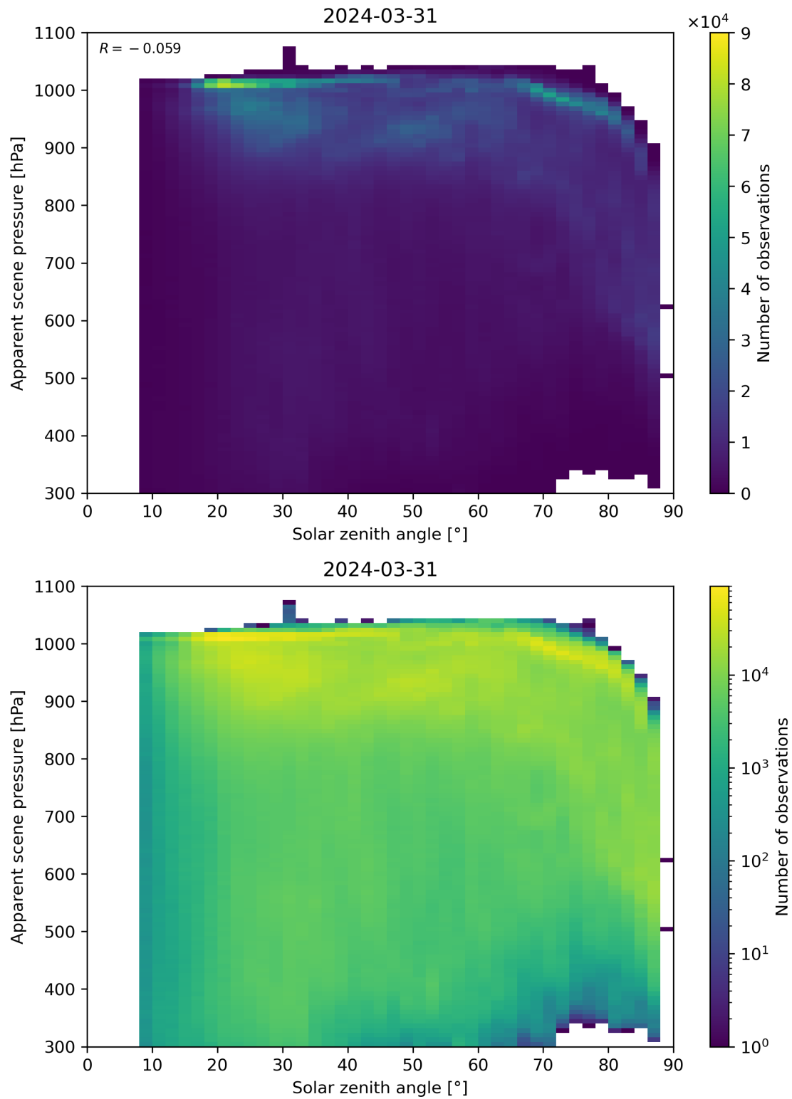
Figure 108: Scatter density plot of “Solar zenith angle” against “Apparent scene pressure” for 2024-03-31 to 2024-04-01.
