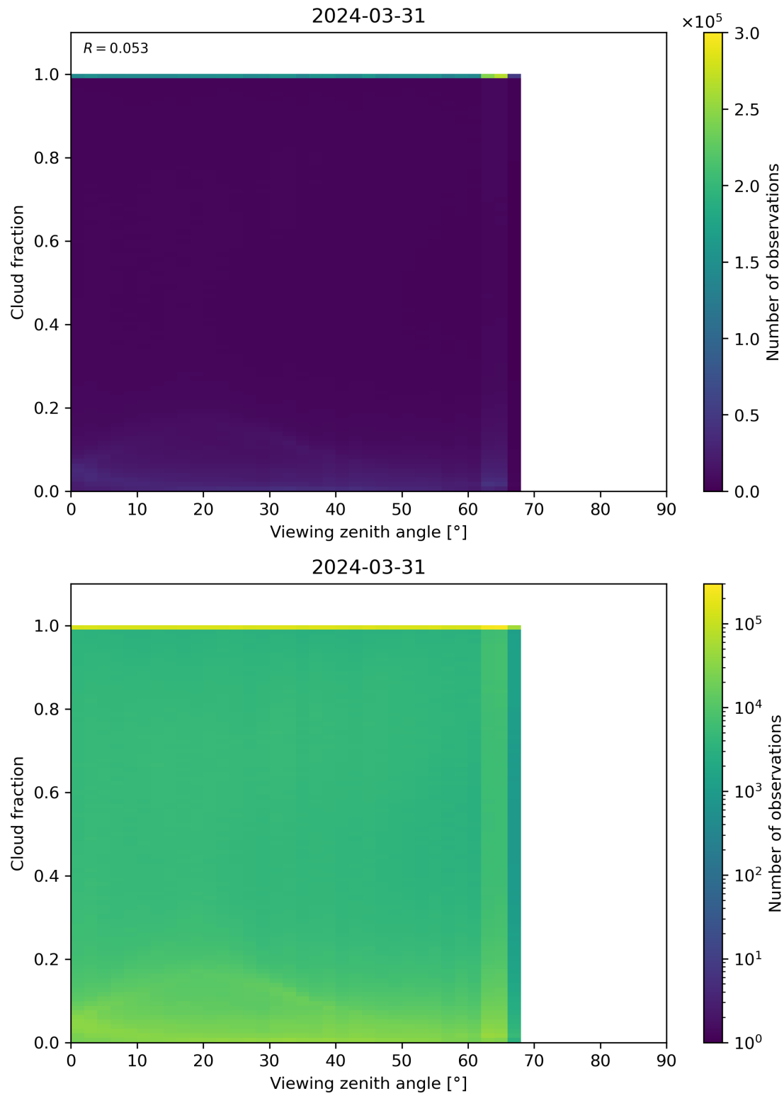
Figure 120: Scatter density plot of “Viewing zenith angle” against “Cloud fraction” for 2024-03-31 to 2024-04-01.
