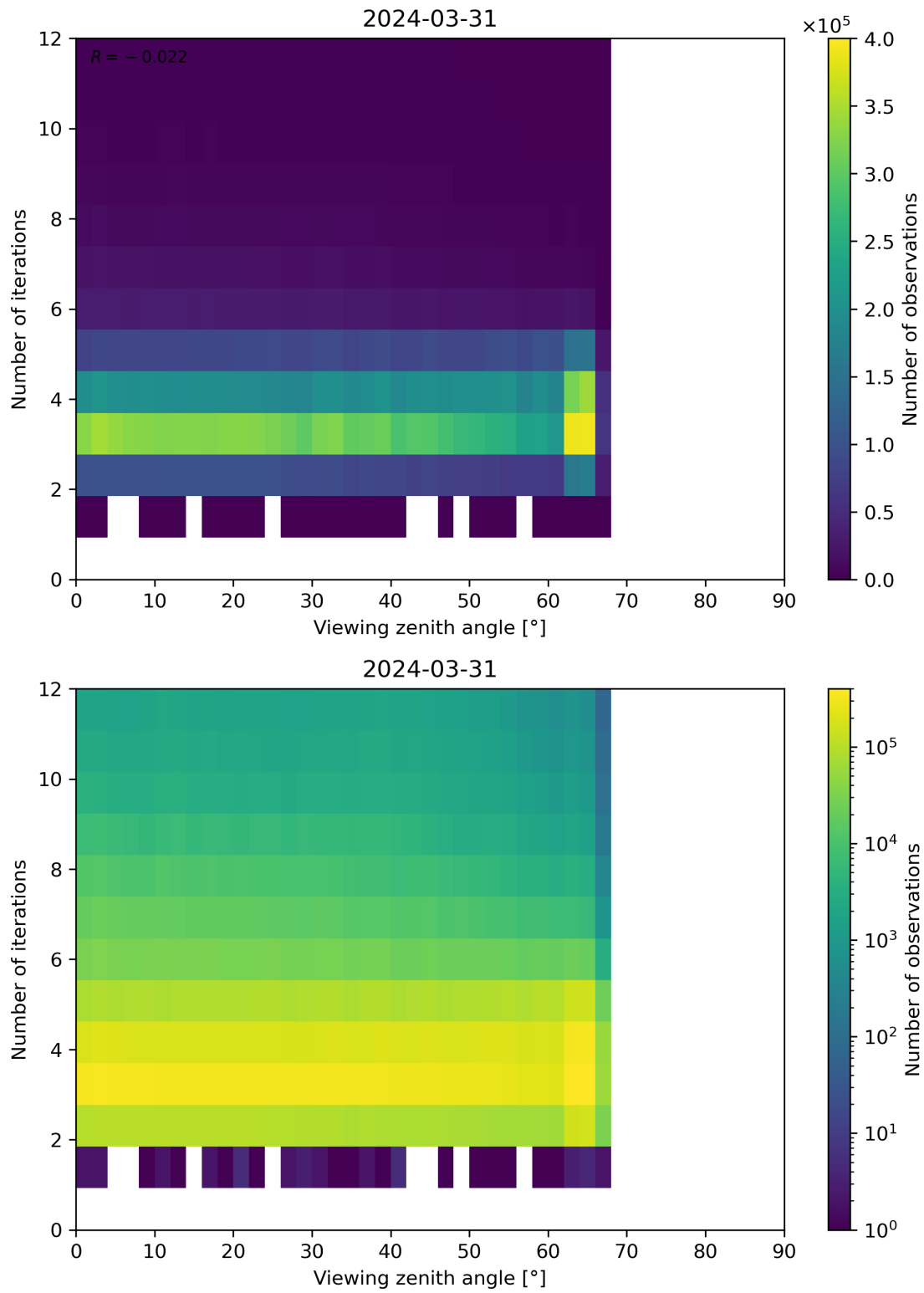
Figure 124: Scatter density plot of “Viewing zenith angle” against “Number of iterations” for 2024-03-31 to 2024-04-01.
