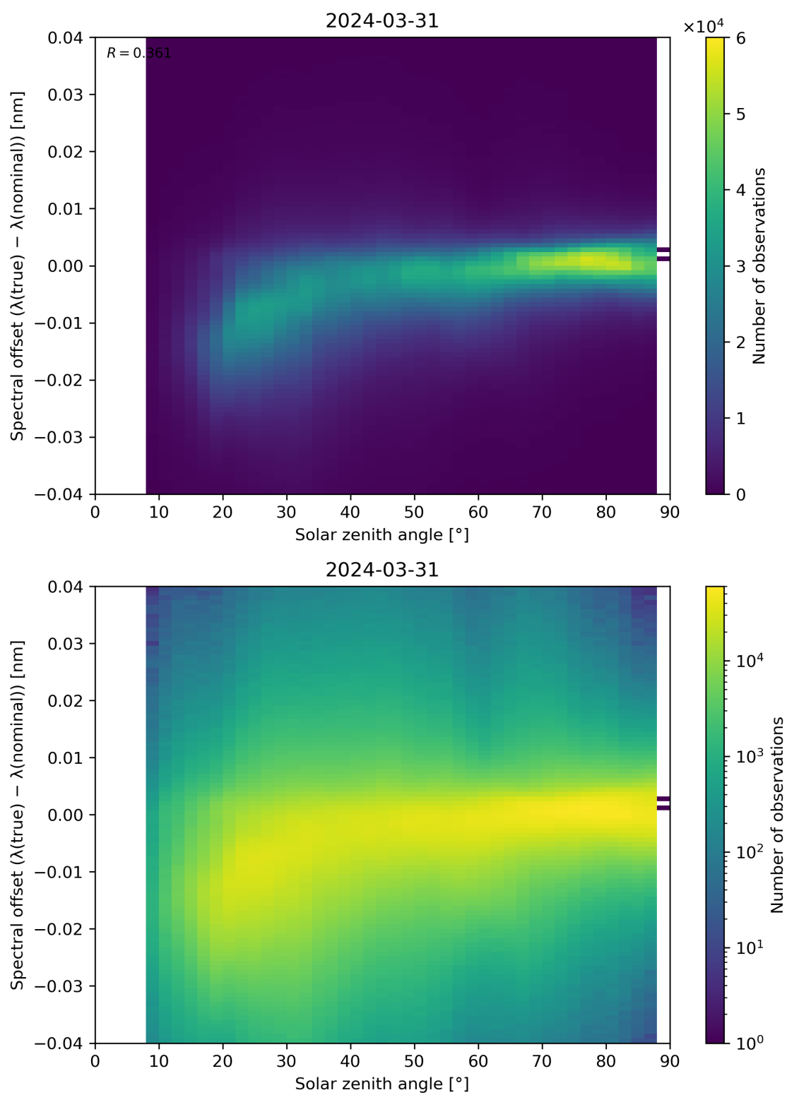
Figure 117: Scatter density plot of “Solar zenith angle” against “Spectral offset ( \lambda(\text{true}) - \lambda(\text{nominal}) )” for 2024-03-31 to 2024-04-01.
