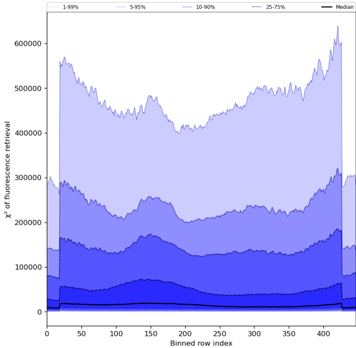
Figure 59: Along track statistics of “ \chi^2 of fluorescence retrieval” for 2024-03-31 to 2024-04-01
