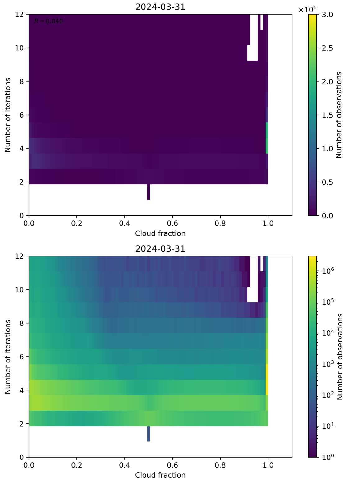
Figure 73: Scatter density plot of “Cloud fraction” against “Number of iterations” for 2024-03-31 to 2024-04-01.
