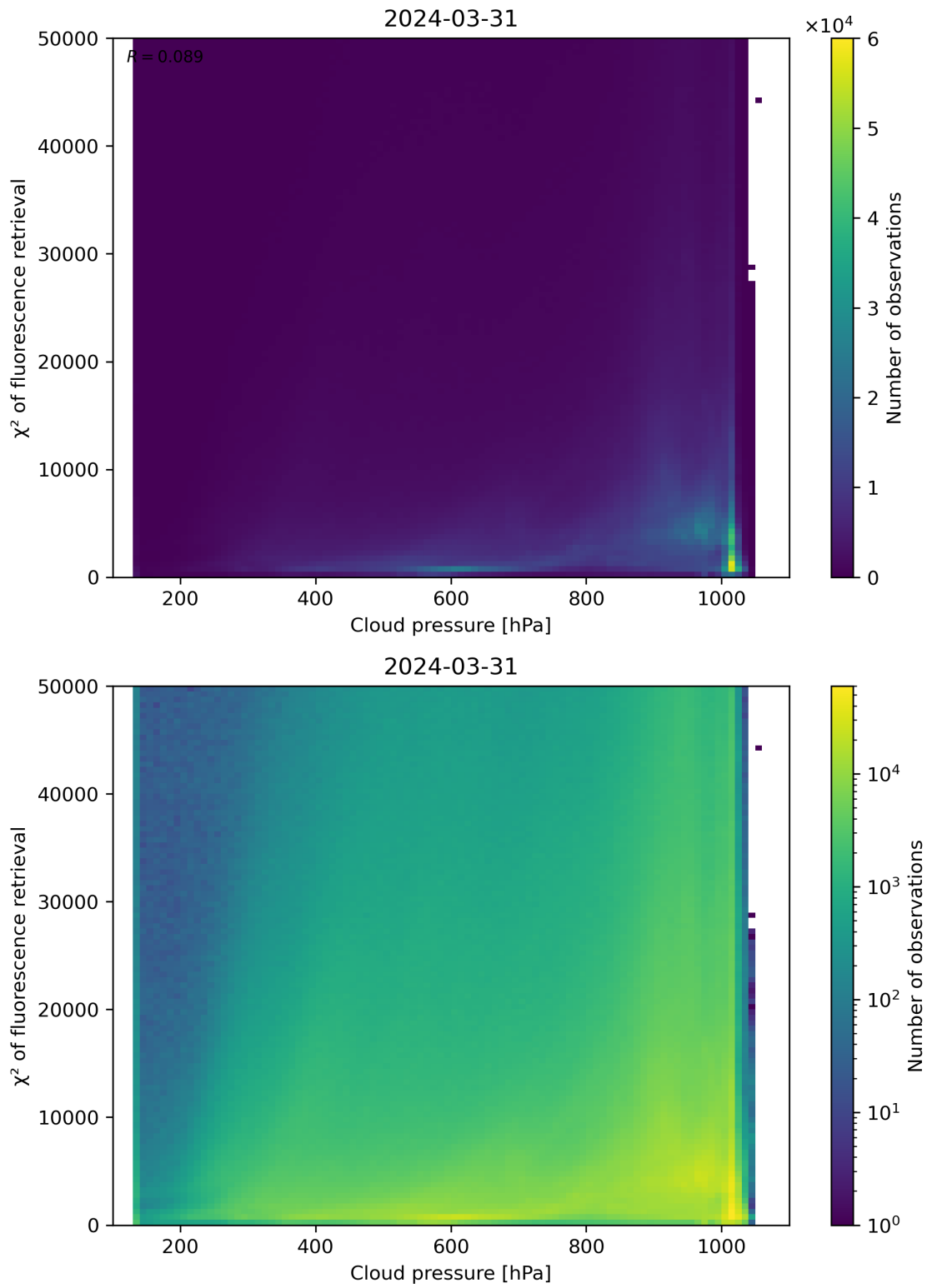
Figure 78: Scatter density plot of “Cloud pressure” against “ \chi^2 of fluorescence retrieval” for 2024-03-31 to 2024-04-01.
