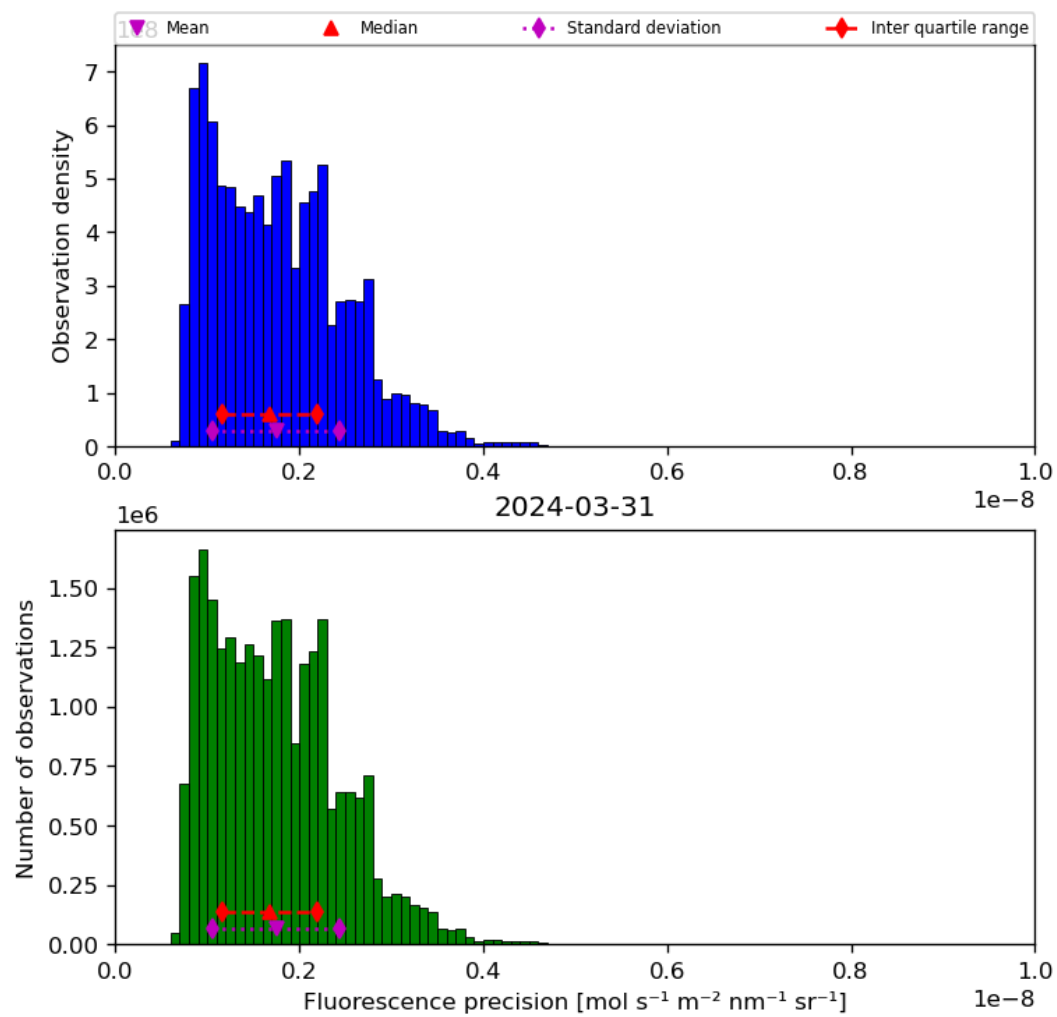
Figure 41: Histogram of “Fluorescence precision” for 2024-03-31 to 2024-04-01
