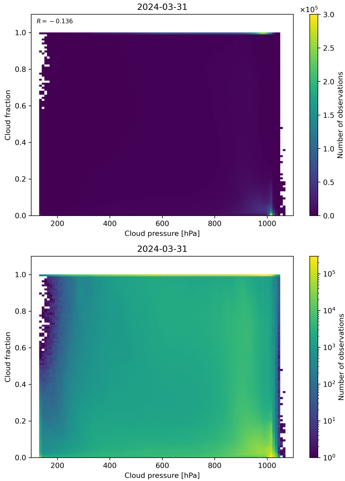
Figure 79: Scatter density plot of “Cloud pressure” against “Cloud fraction” for 2024-03-31 to 2024-04-01.
