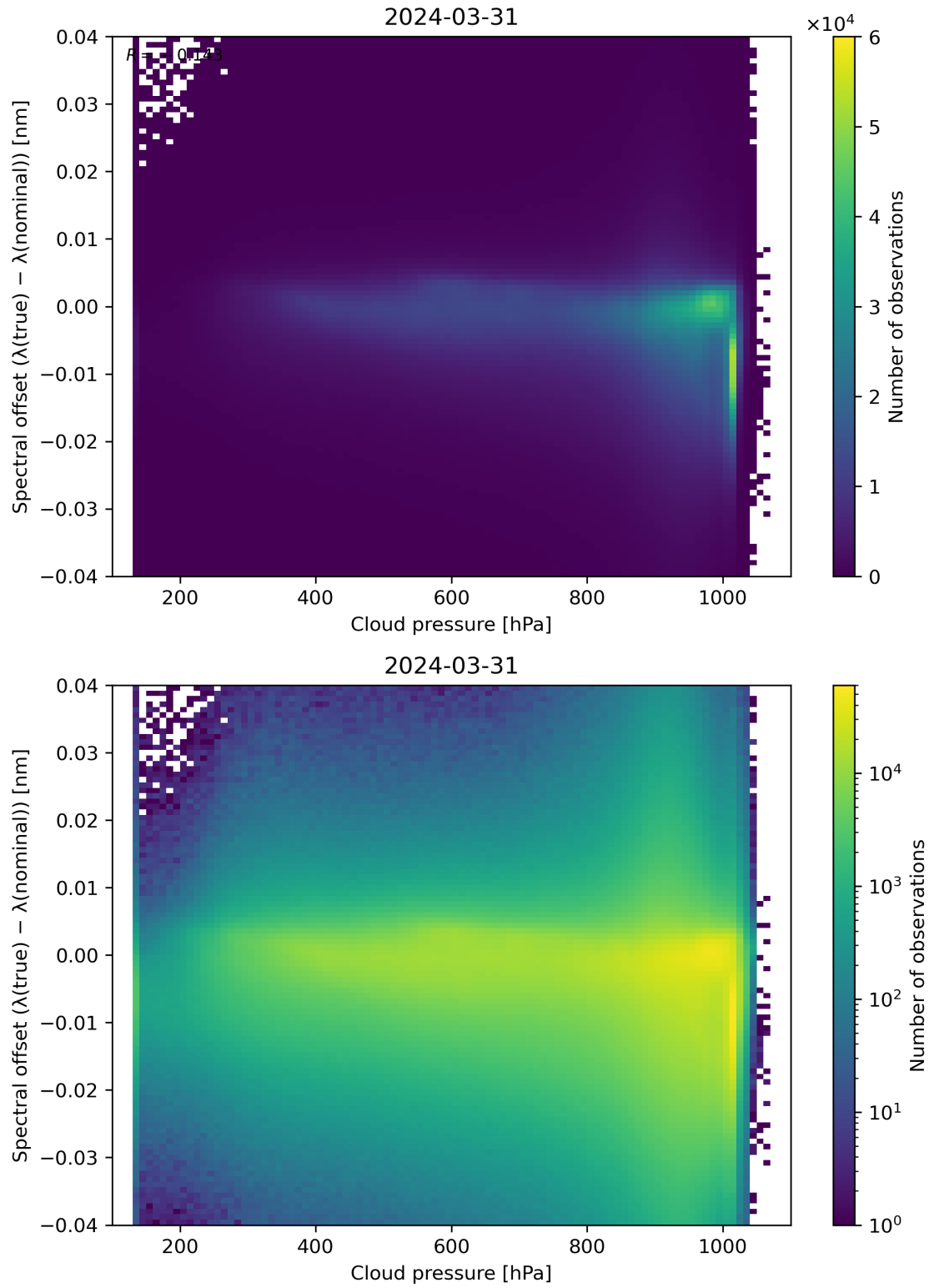
Figure 84: Scatter density plot of “Cloud pressure” against “Spectral offset ( \lambda(\text{true}) - \lambda(\text{nominal}) )” for 2024-03-31 to 2024-04-01.
