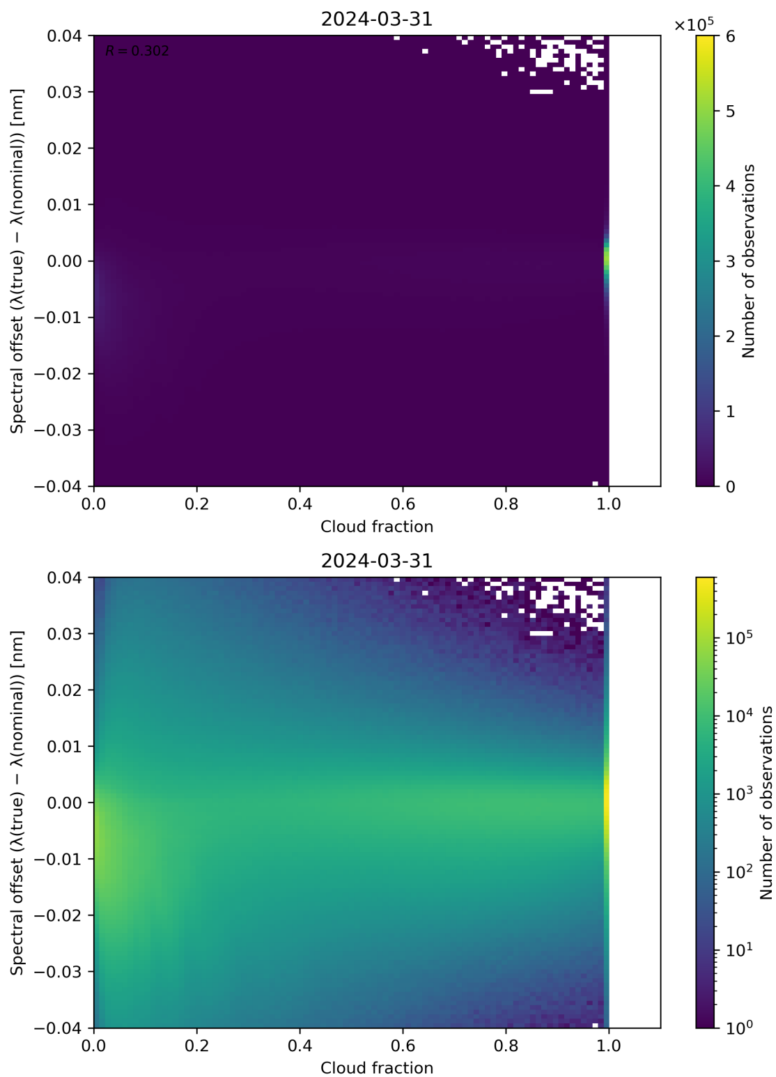
Figure 76: Scatter density plot of “Cloud fraction” against “Spectral offset ( \lambda(\text{true}) - \lambda(\text{nominal}) )” for 2024-03-31 to 2024-04-01.
