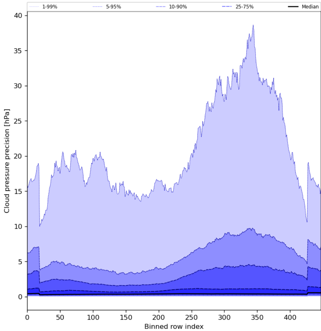
Figure 48: Along track statistics of “Cloud pressure precision” for 2024-03-31 to 2024-04-01
