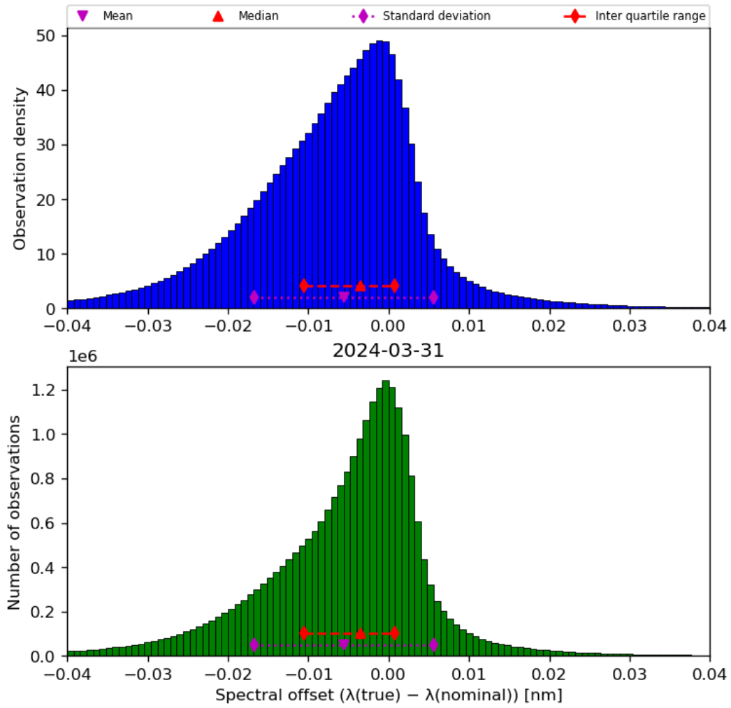
Figure 45: Histogram of “Spectral offset ( \lambda(\text{true}) - \lambda(\text{nominal}) )” for 2024-03-31 to 2024-04-01
