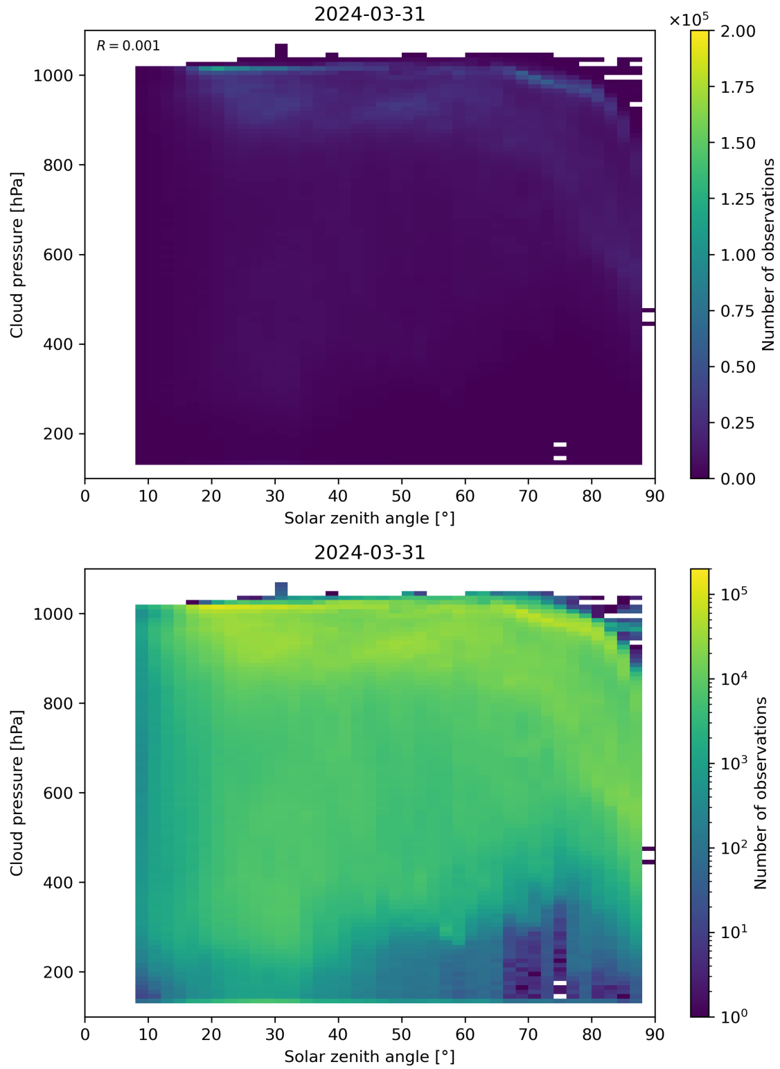
Figure 111: Scatter density plot of “Solar zenith angle” against “Cloud pressure” for 2024-03-31 to 2024-04-01.
