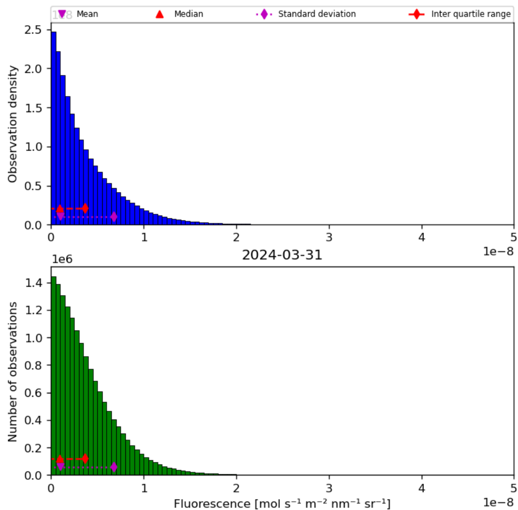
Figure 40: Histogram of “Fluorescence” for 2024-03-31 to 2024-04-01
