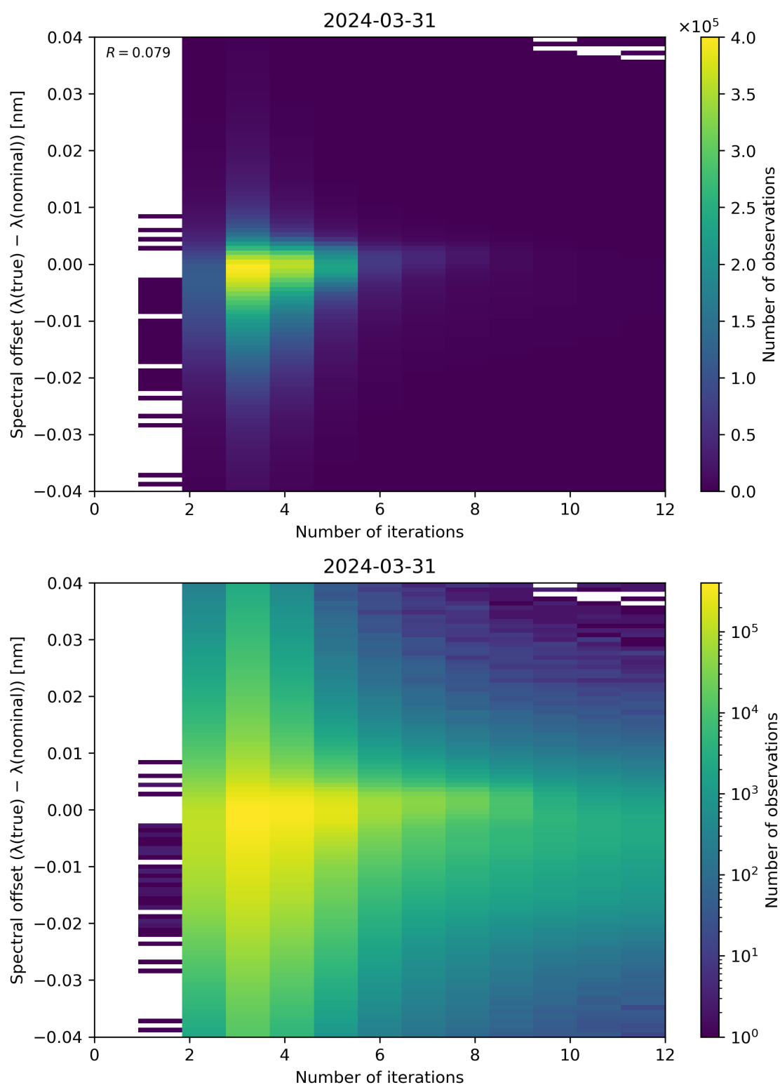
Figure 100: Scatter density plot of “Number of iterations” against “Spectral offset ( \lambda(\text{true}) - \lambda(\text{nominal}) )” for 2024-03-31 to 2024-04-01.
