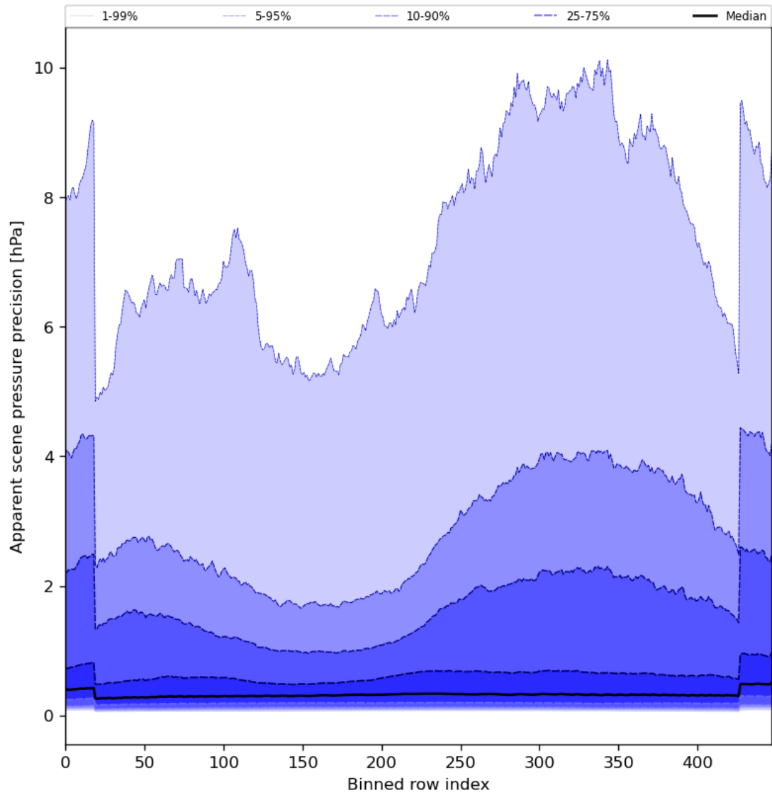
Figure 54: Along track statistics of “Apparent scene pressure precision” for 2024-03-31 to 2024-04-01
