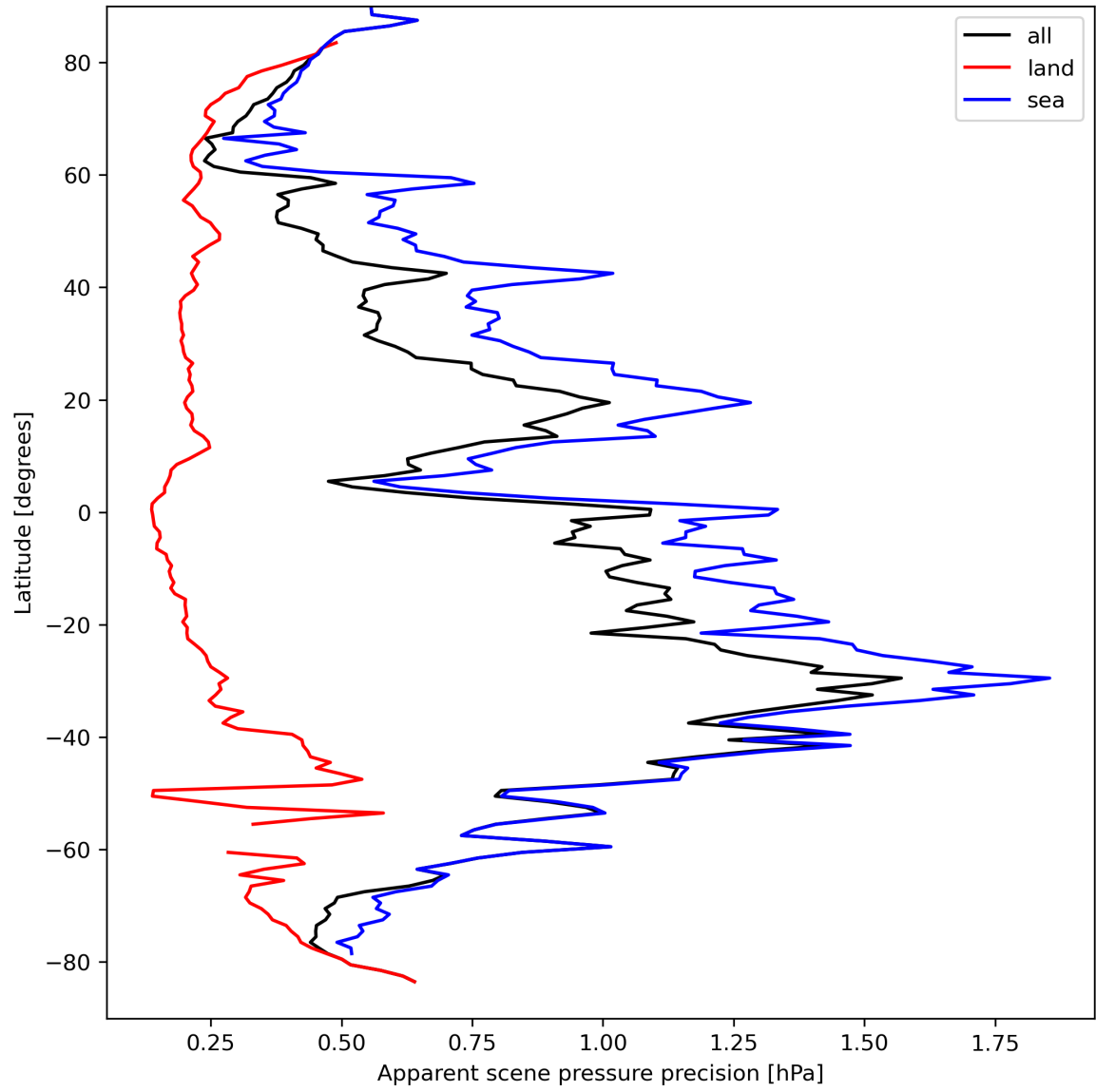
Figure 20: Zonal average of “Apparent scene pressure precision” for 2024-03-31 to 2024-04-01.
