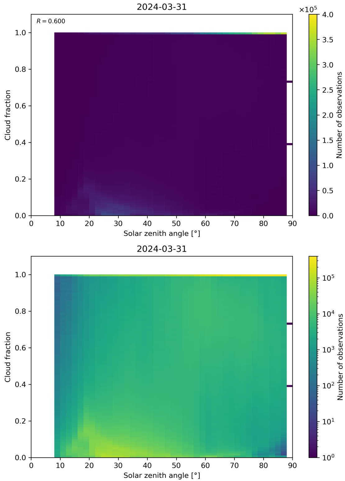
Figure 110: Scatter density plot of “Solar zenith angle” against “Cloud fraction” for 2024-03-31 to 2024-04-01.
