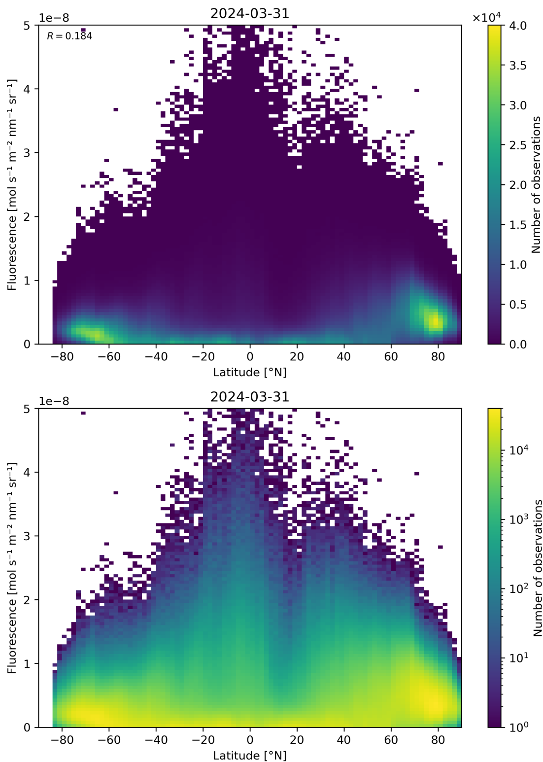
Figure 92: Scatter density plot of “Latitude” against “Fluorescence” for 2024-03-31 to 2024-04-01.
