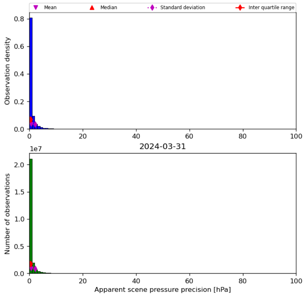
Figure 37: Histogram of “Apparent scene pressure precision” for 2024-03-31 to 2024-04-01
