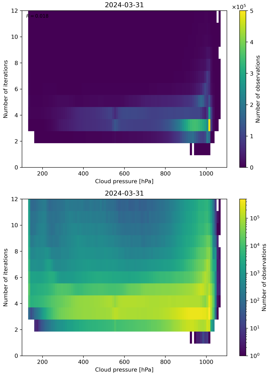
Figure 81: Scatter density plot of “Cloud pressure” against “Number of iterations” for 2024-03-31 to 2024-04-01.
