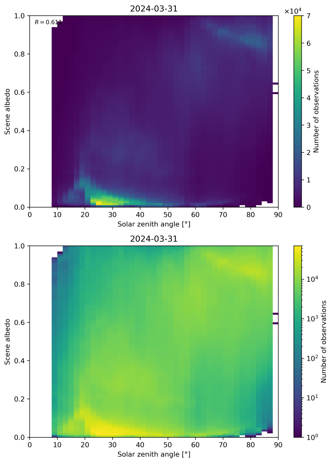
Figure 116: Scatter density plot of “Solar zenith angle” against “Scene albedo” for 2024-03-31 to 2024-04-01.
