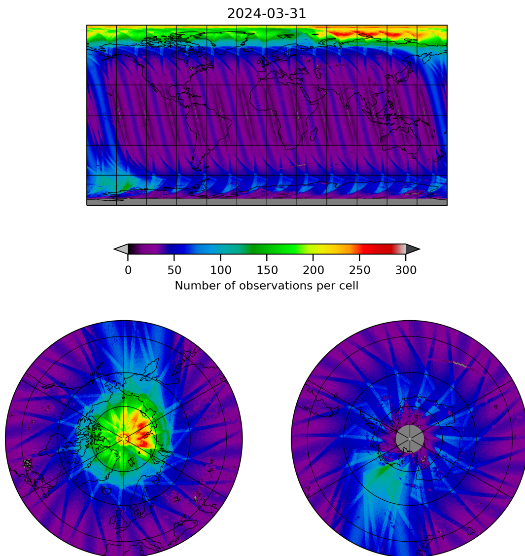
Figure 11: Map of the number of observations for 2024-03-31 to 2024-04-01
