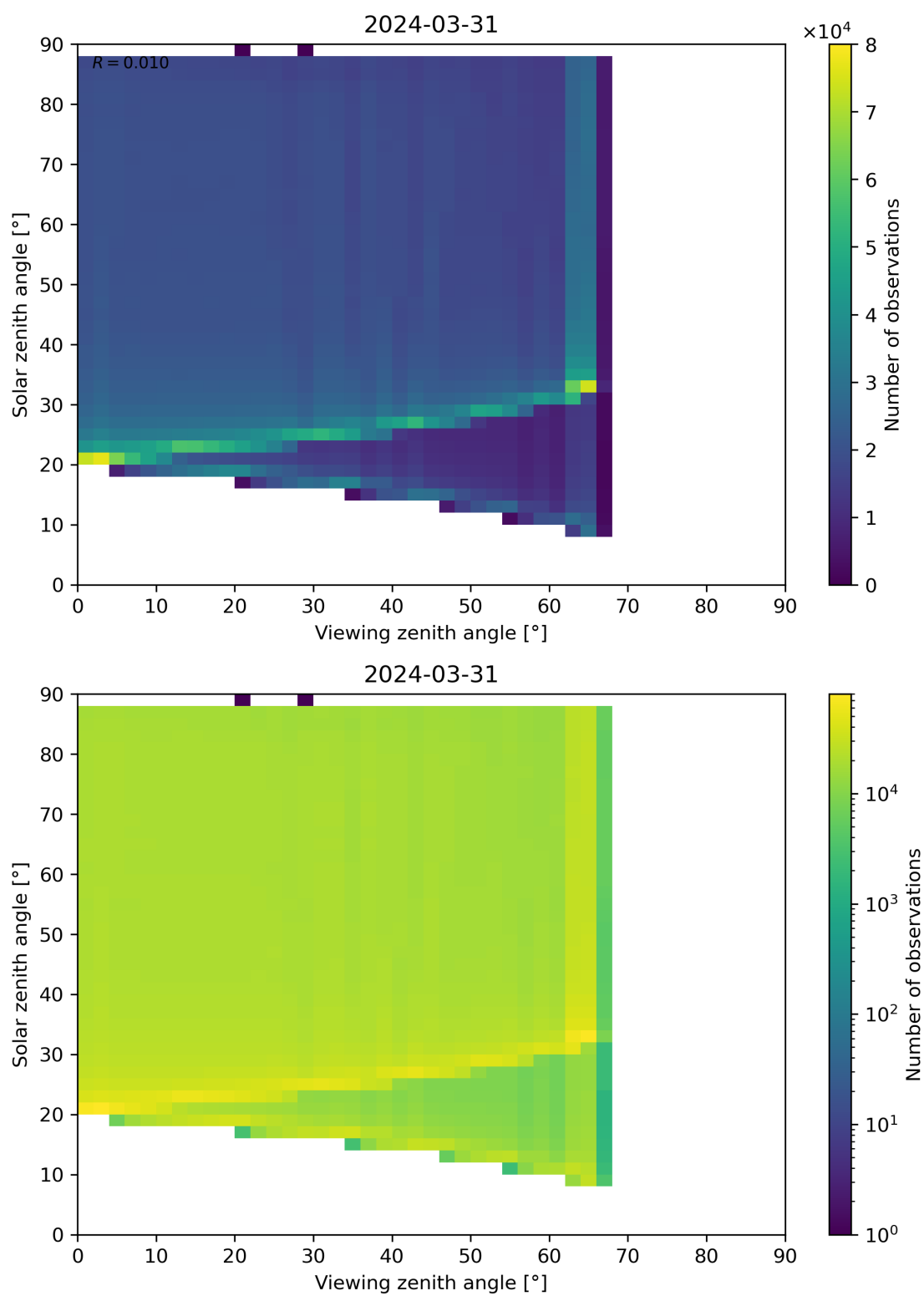
Figure 127: Scatter density plot of “Viewing zenith angle” against “Solar zenith angle” for 2024-03-31 to 2024-04-01.
