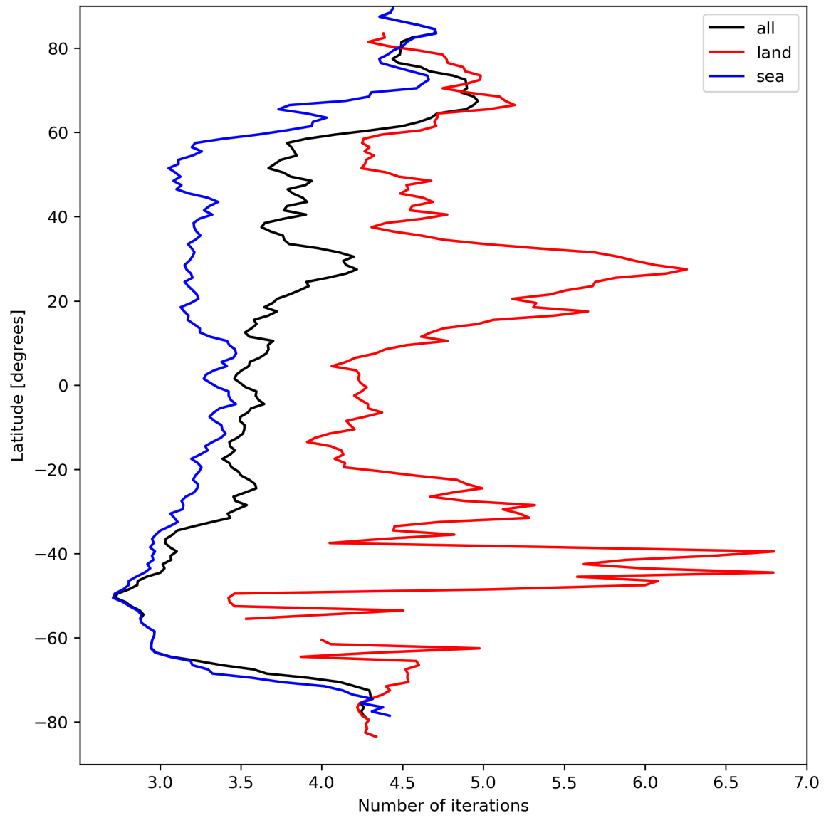
Figure 22: Zonal average of “Number of iterations” for 2024-03-31 to 2024-04-01.
