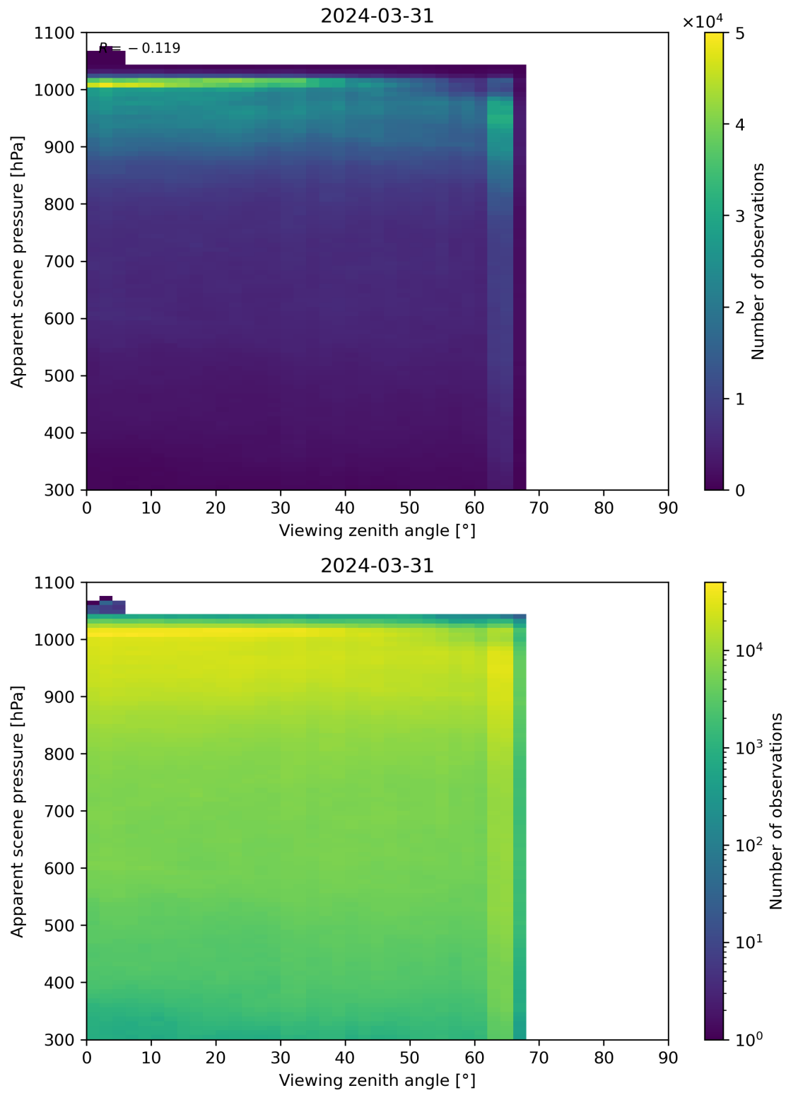
Figure 118: Scatter density plot of “Viewing zenith angle” against “Apparent scene pressure” for 2024-03-31 to 2024-04-01.
