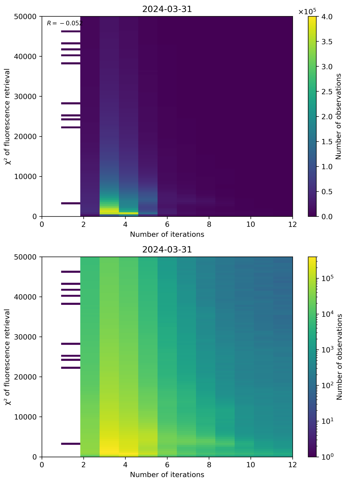
Figure 97: Scatter density plot of “Number of iterations” against “ \chi^2 of fluorescence retrieval” for 2024-03-31 to 2024-04-01.
