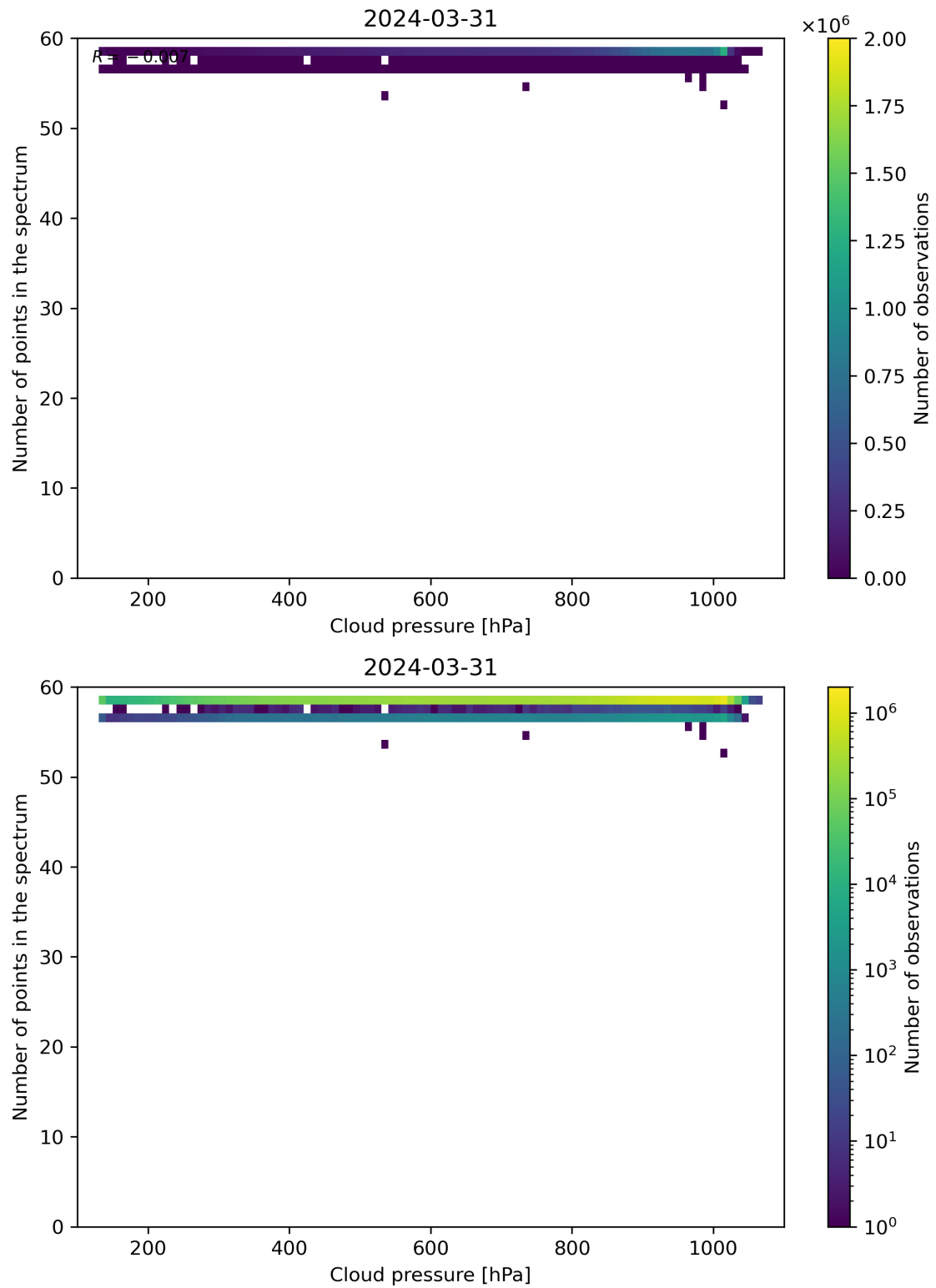
Figure 82: Scatter density plot of “Cloud pressure” against “Number of points in the spectrum” for 2024-03-31 to 2024-04-01.
