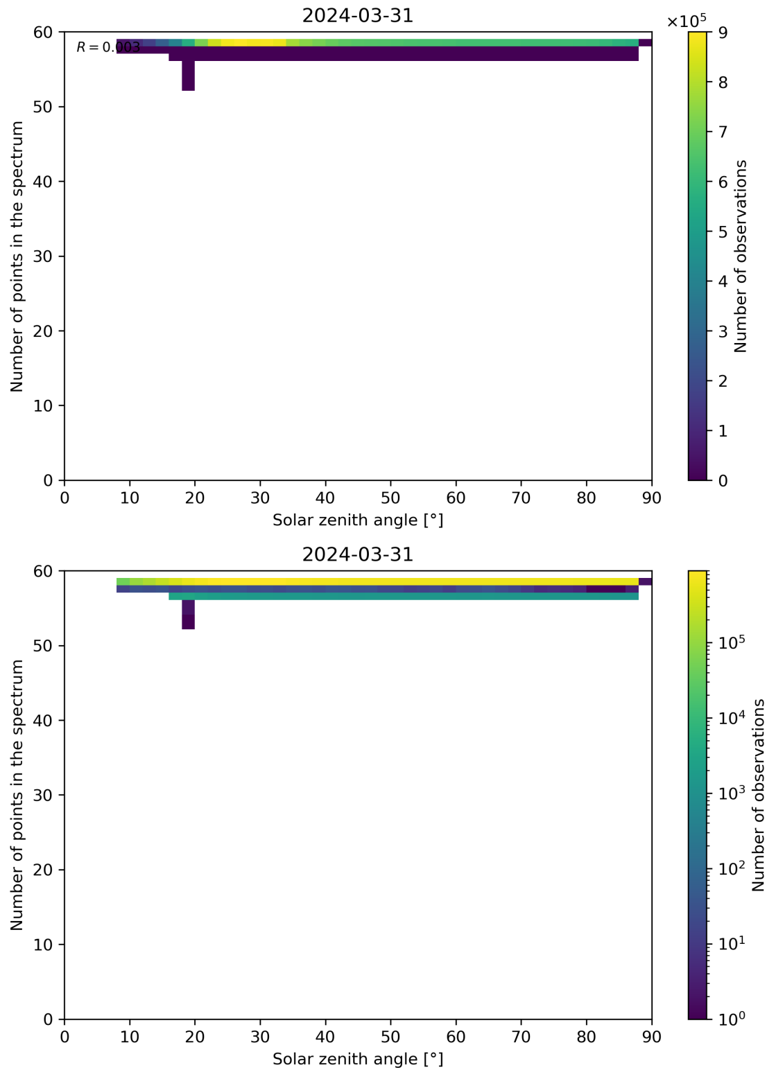
Figure 115: Scatter density plot of “Solar zenith angle” against “Number of points in the spectrum” for 2024-03-31 to 2024-04-01.
