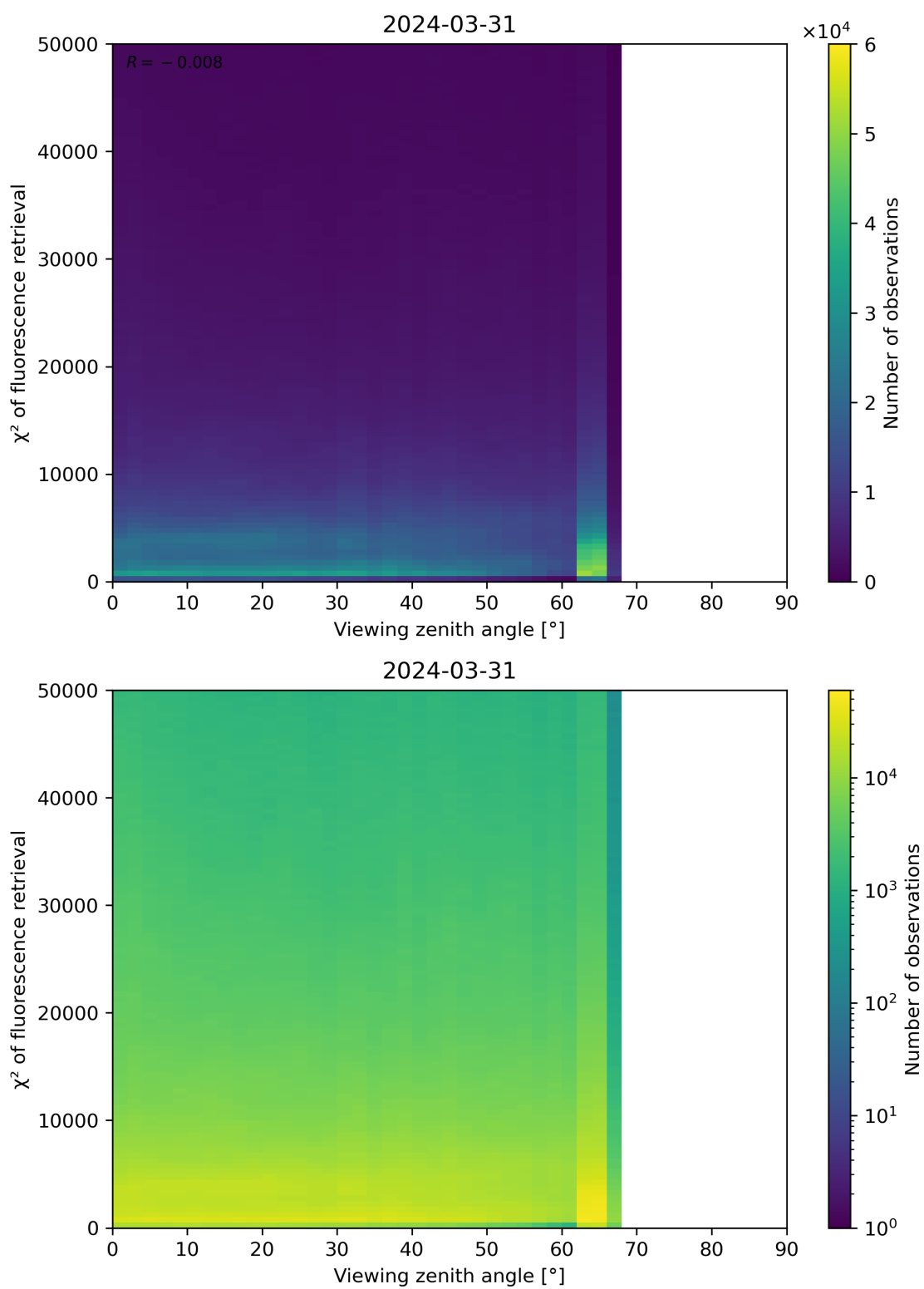
Figure 119: Scatter density plot of “Viewing zenith angle” against “ \chi^2 of fluorescence retrieval” for 2024-03-31 to 2024-04-01.
