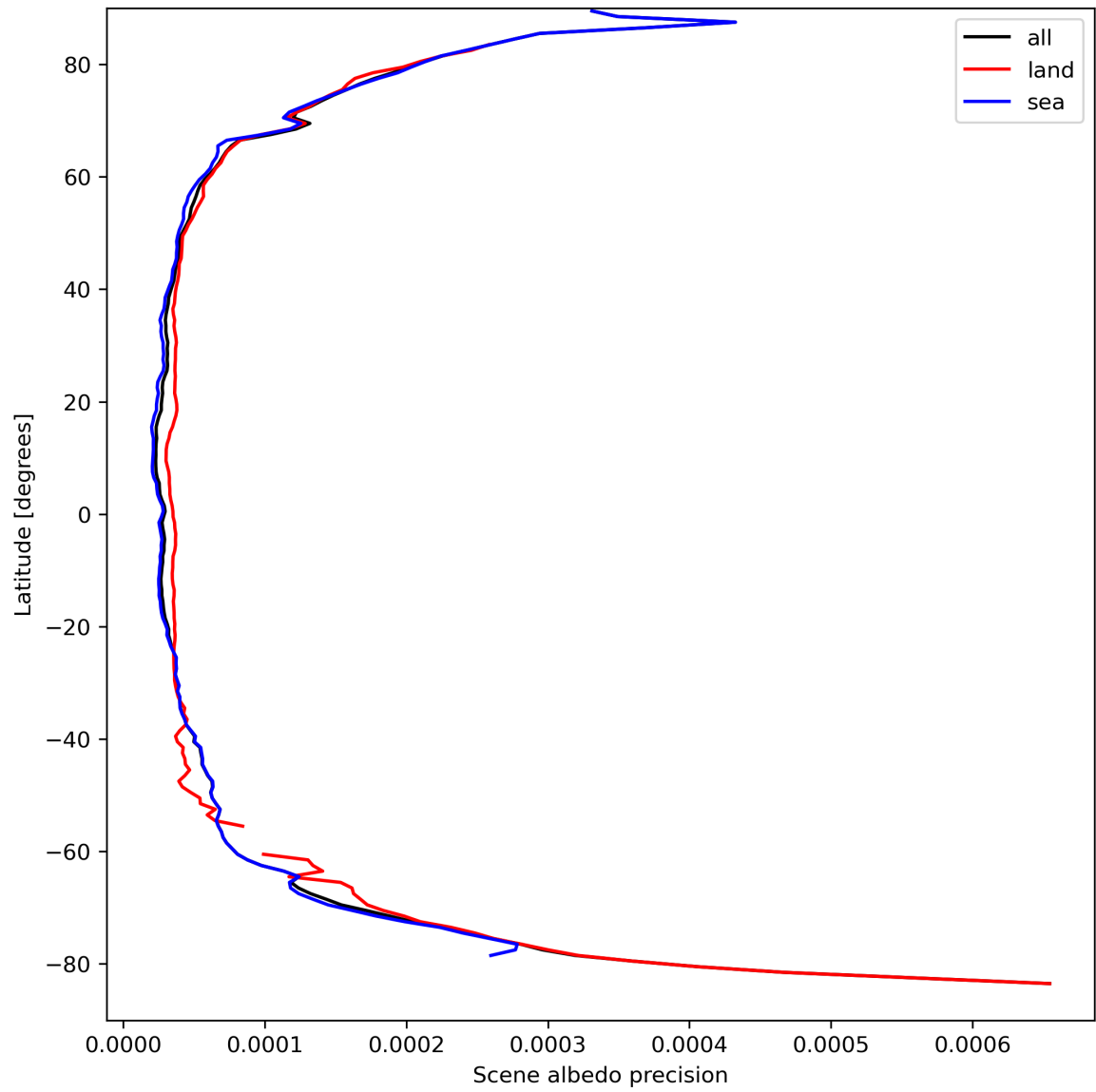
Figure 18: Zonal average of “Scene albedo precision” for 2024-03-31 to 2024-04-01.
