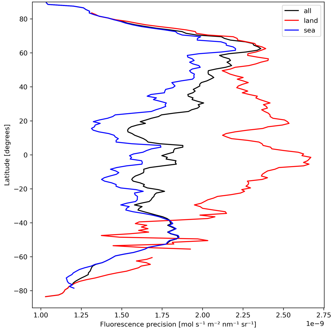
Figure 24: Zonal average of “Fluorescence precision” for 2024-03-31 to 2024-04-01.
