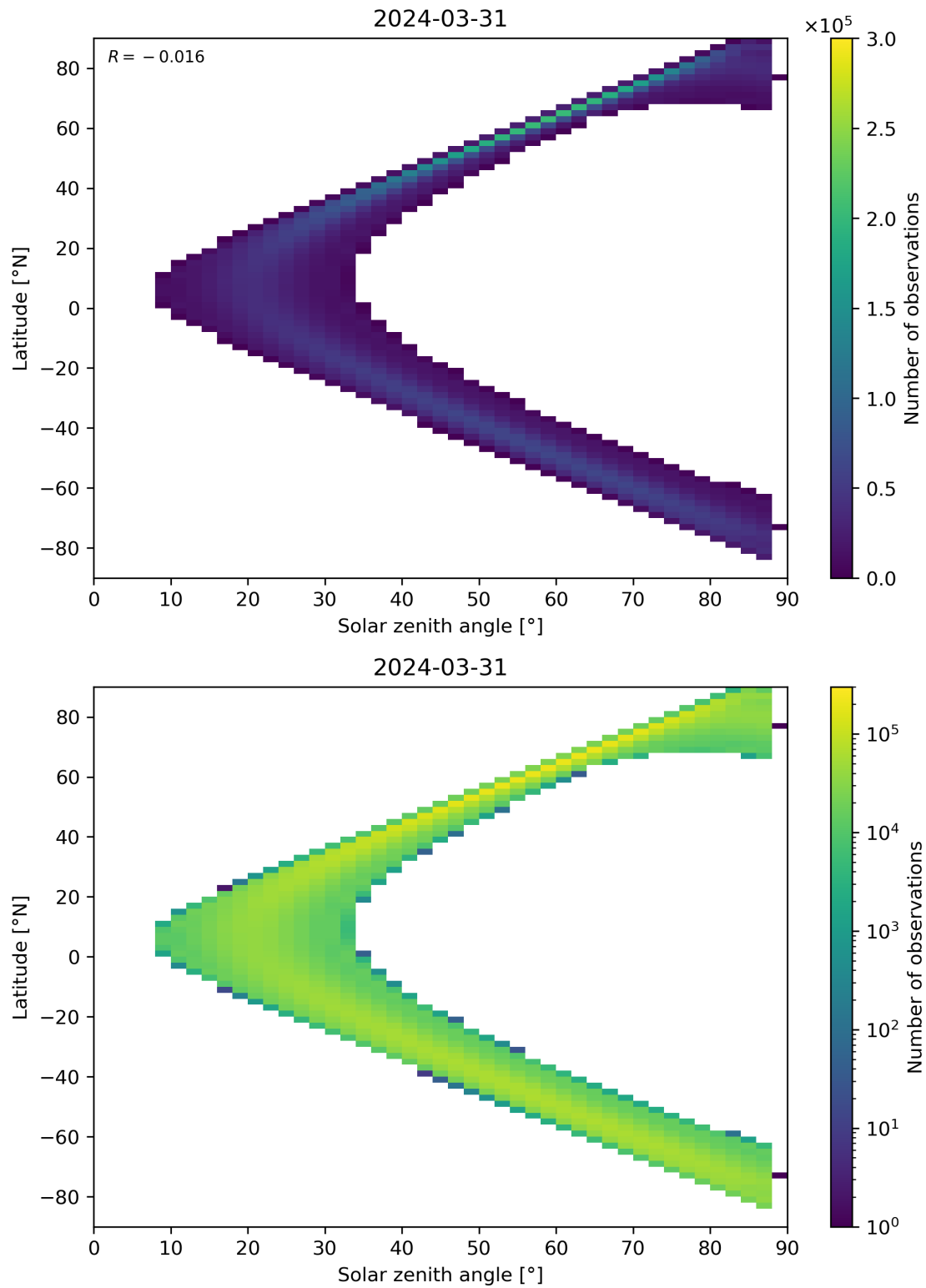
Figure 113: Scatter density plot of “Solar zenith angle” against “Latitude” for 2024-03-31 to 2024-04-01.
