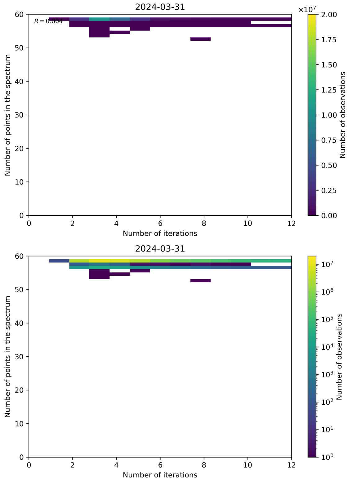
Figure 99: Scatter density plot of “Number of iterations” against “Number of points in the spectrum” for 2024-03-31 to 2024-04-01.
