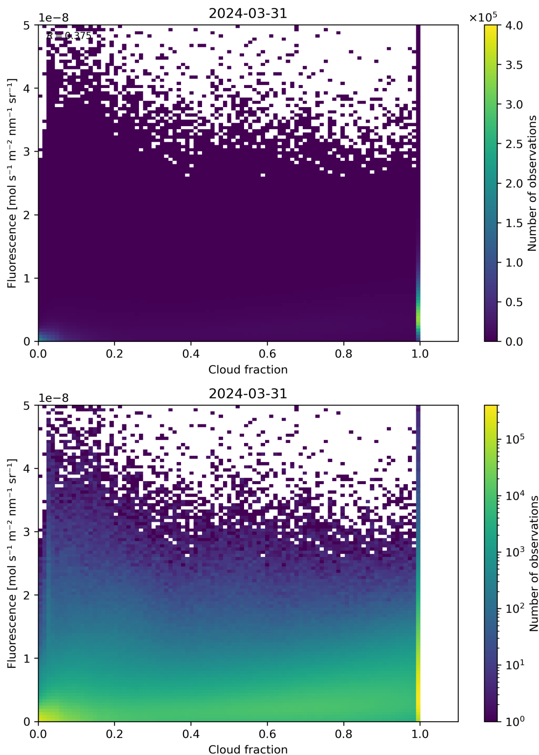
Figure 72: Scatter density plot of “Cloud fraction” against “Fluorescence” for 2024-03-31 to 2024-04-01.
