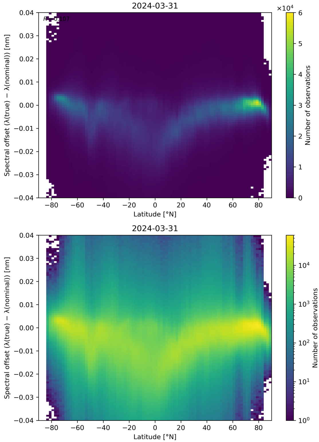
Figure 96: Scatter density plot of “Latitude” against “Spectral offset ( \lambda(\text{true}) - \lambda(\text{nominal}) )” for 2024-03-31 to 2024-04-01.
