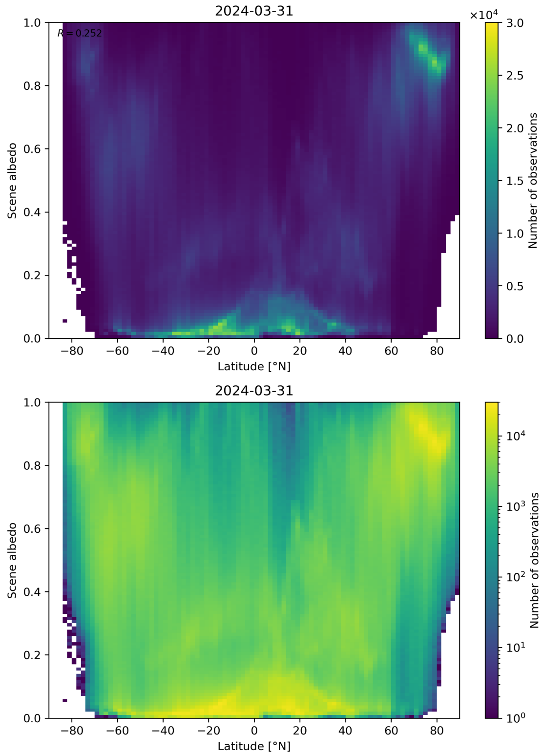
Figure 95: Scatter density plot of “Latitude” against “Scene albedo” for 2024-03-31 to 2024-04-01.
