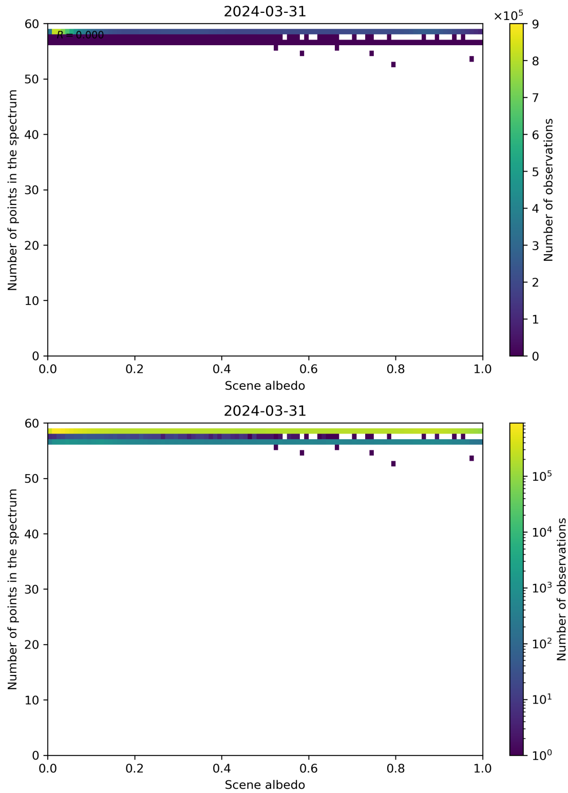
Figure 106: Scatter density plot of “Scene albedo” against “Number of points in the spectrum” for 2024-03-31 to 2024-04-01.
