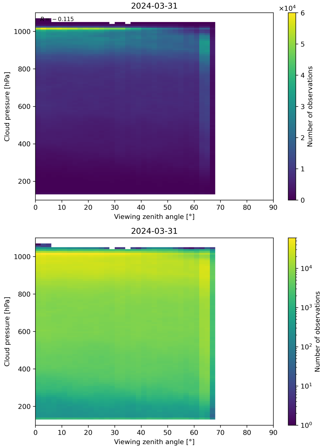
Figure 121: Scatter density plot of “Viewing zenith angle” against “Cloud pressure” for 2024-03-31 to 2024-04-01.
