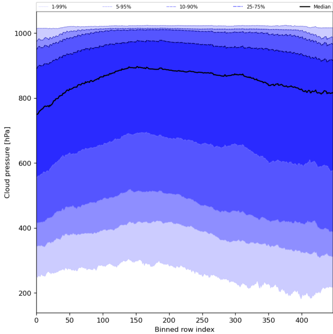
Figure 47: Along track statistics of “Cloud pressure” for 2024-03-31 to 2024-04-01
