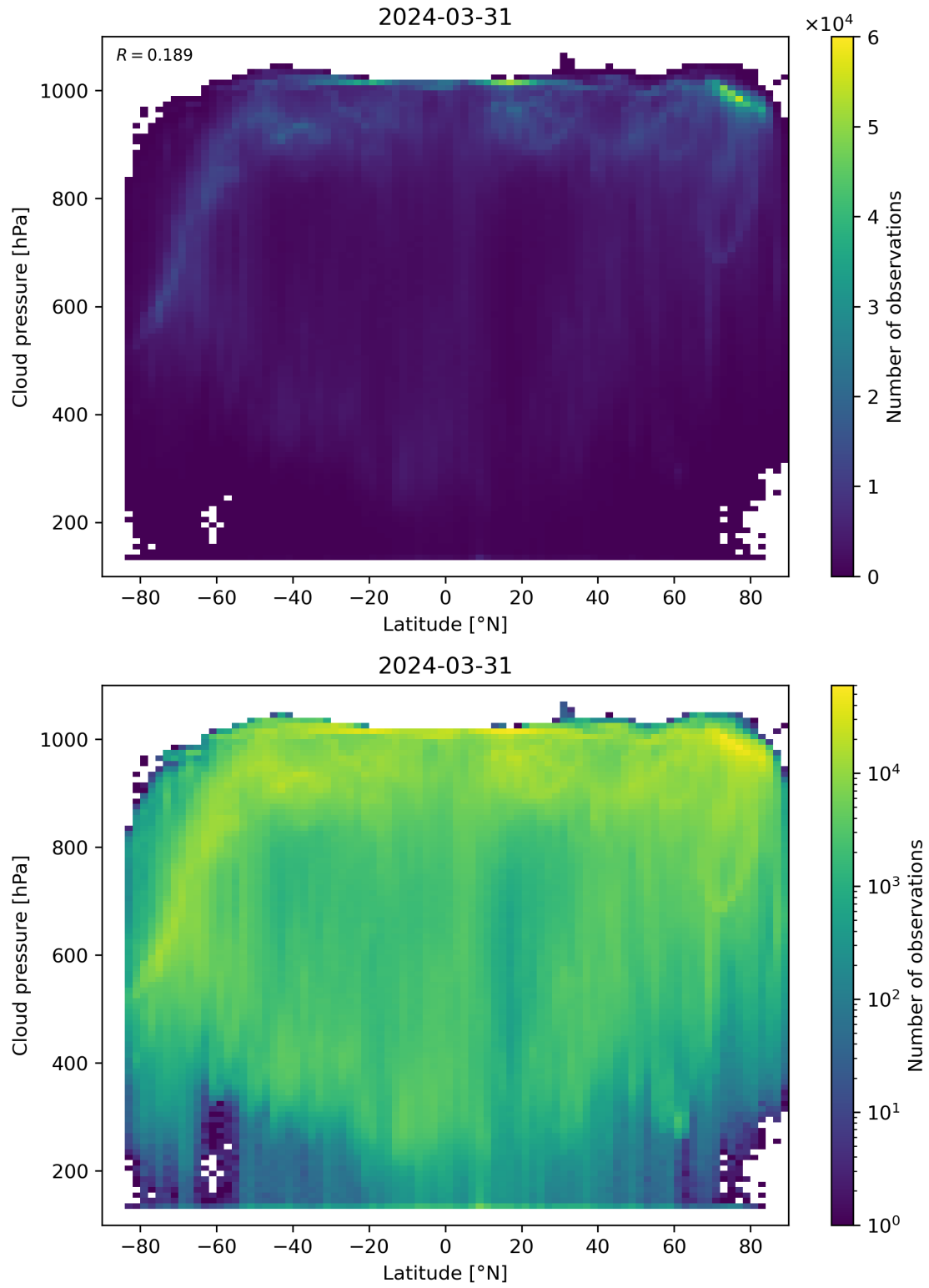
Figure 91: Scatter density plot of “Latitude” against “Cloud pressure” for 2024-03-31 to 2024-04-01.
