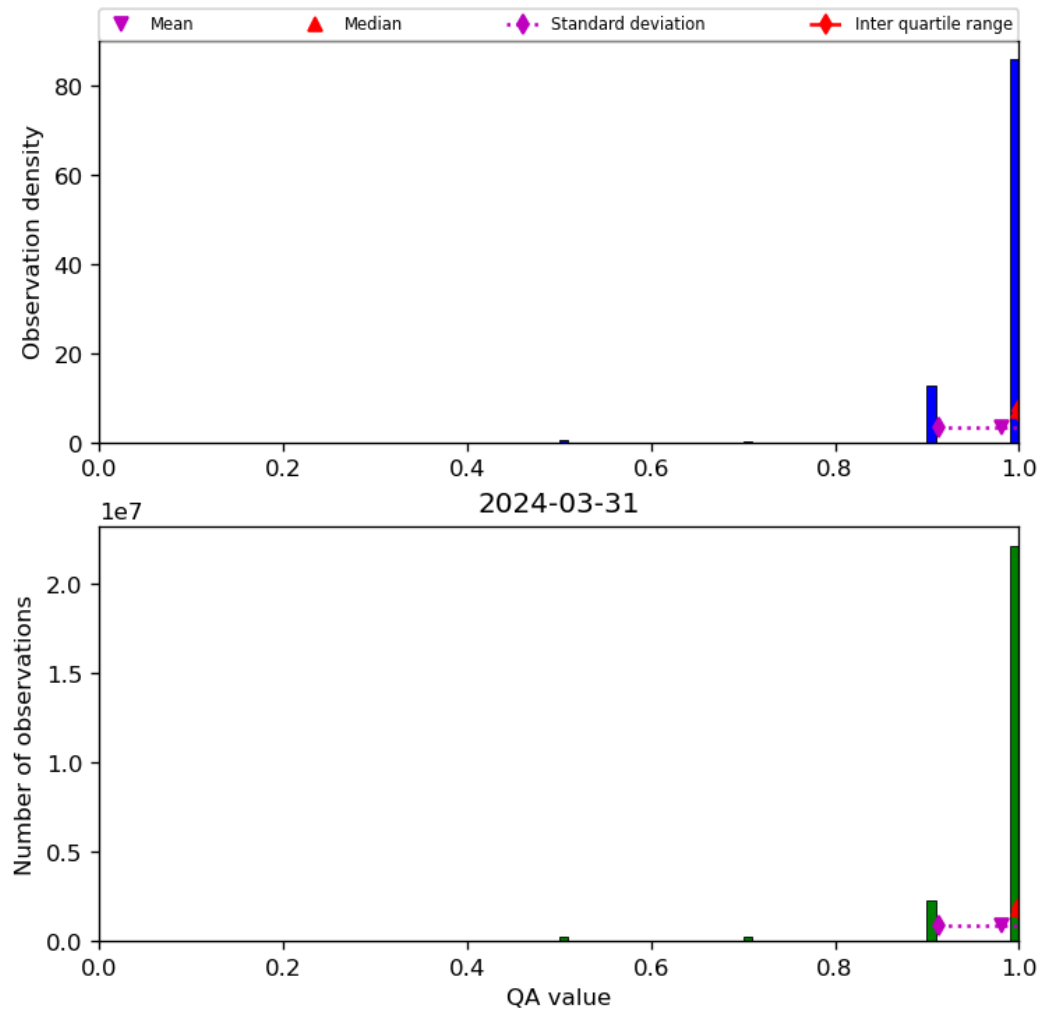
Figure 29: Histogram of “QA value” for 2024-03-31 to 2024-04-01
