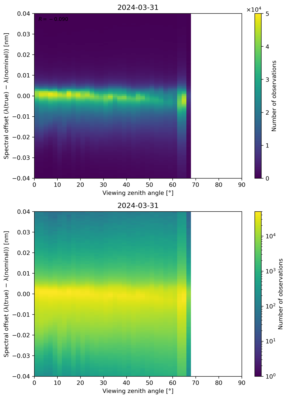
Figure 128: Scatter density plot of “Viewing zenith angle” against “Spectral offset ( \lambda(\text{true}) - \lambda(\text{nominal}) )” for 2024-03-31 to 2024-04-01.
