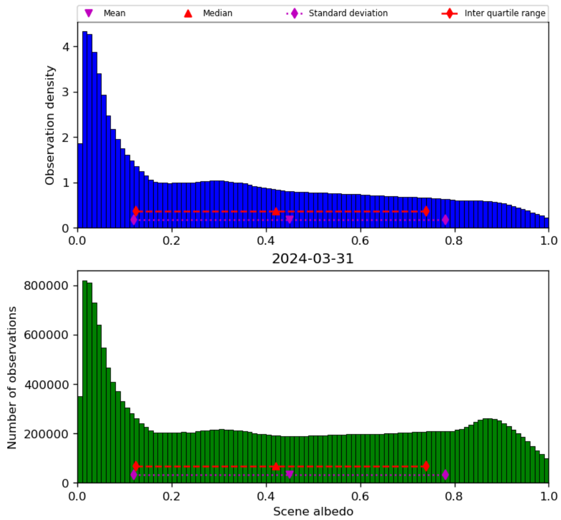
Figure 34: Histogram of “Scene albedo” for 2024-03-31 to 2024-04-01
