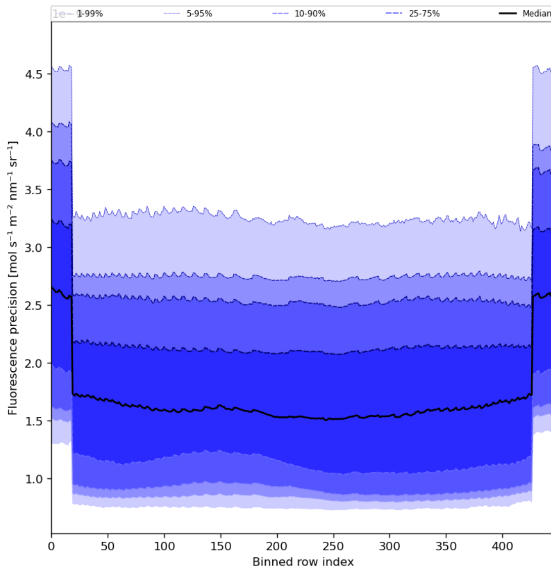
Figure 58: Along track statistics of “Fluorescence precision” for 2024-03-31 to 2024-04-01
