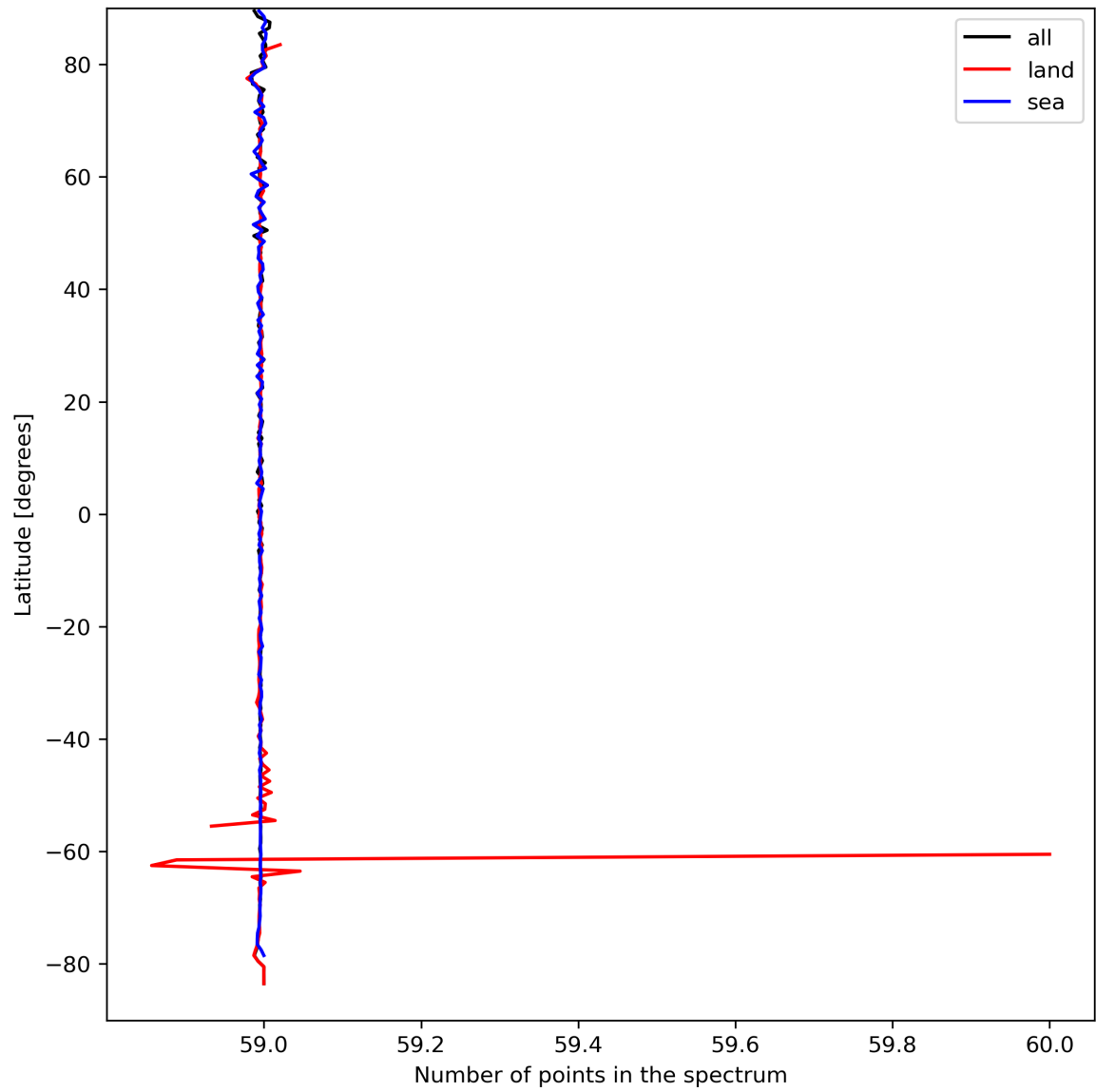
Figure 27: Zonal average of “Number of points in the spectrum” for 2024-03-31 to 2024-04-01.
