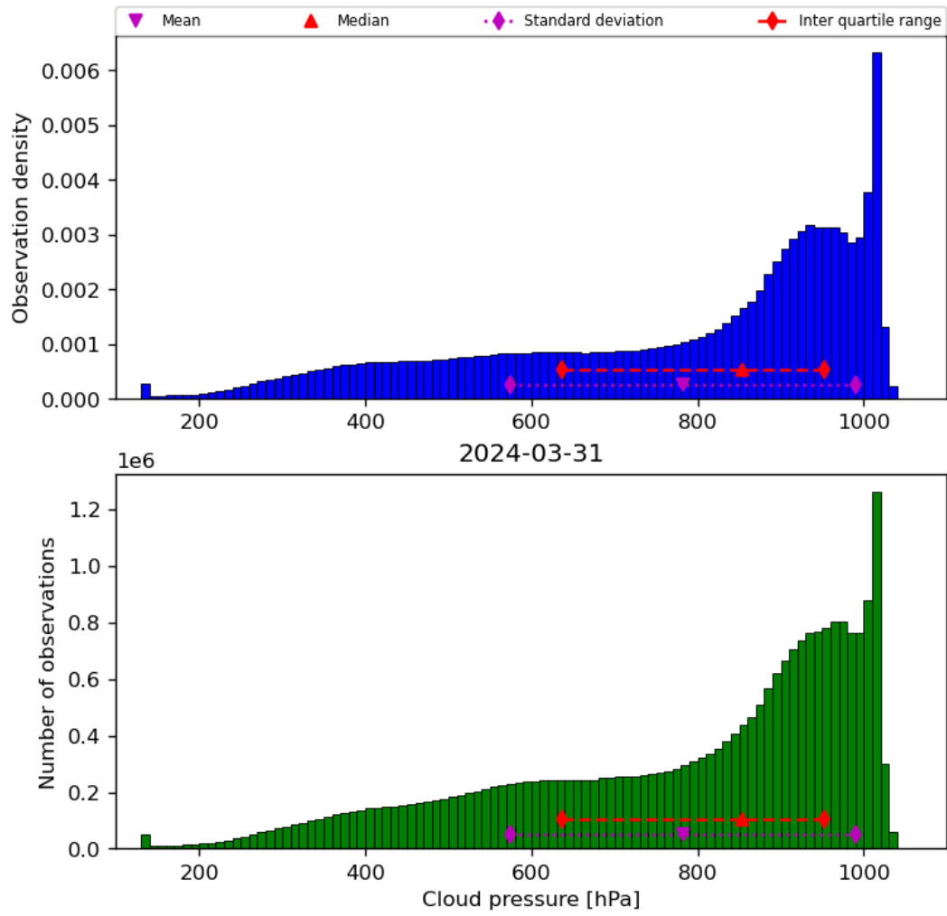
Figure 30: Histogram of “Cloud pressure” for 2024-03-31 to 2024-04-01
