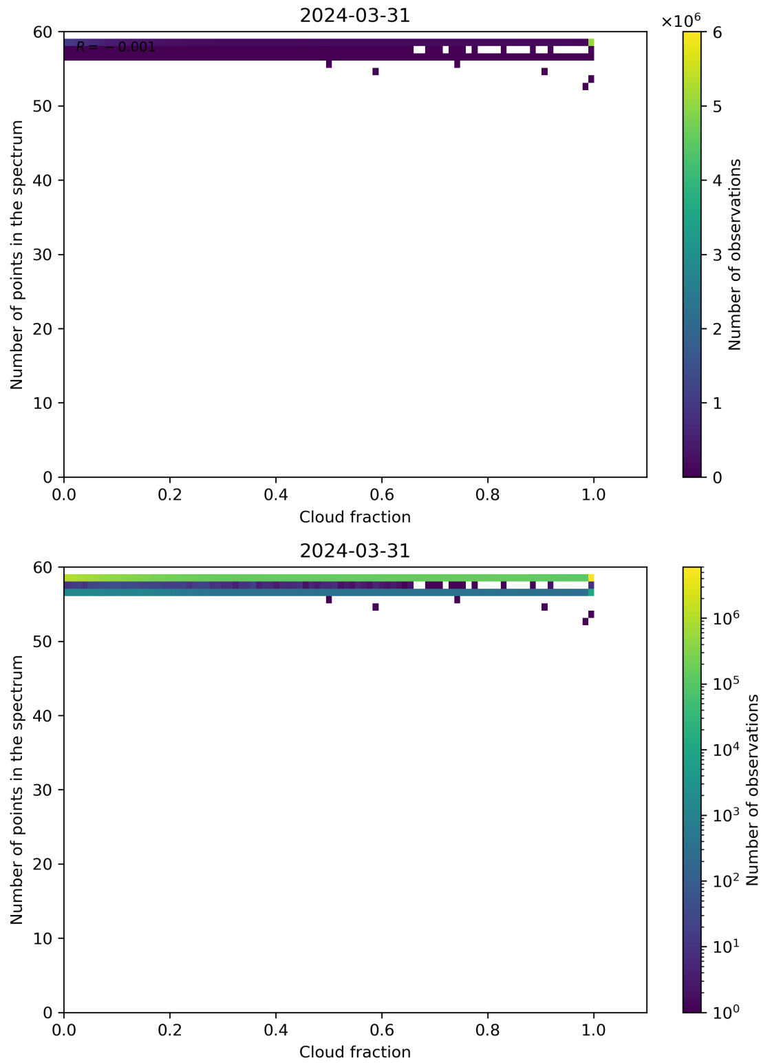
Figure 74: Scatter density plot of “Cloud fraction” against “Number of points in the spectrum” for 2024-03-31 to 2024-04-01.
