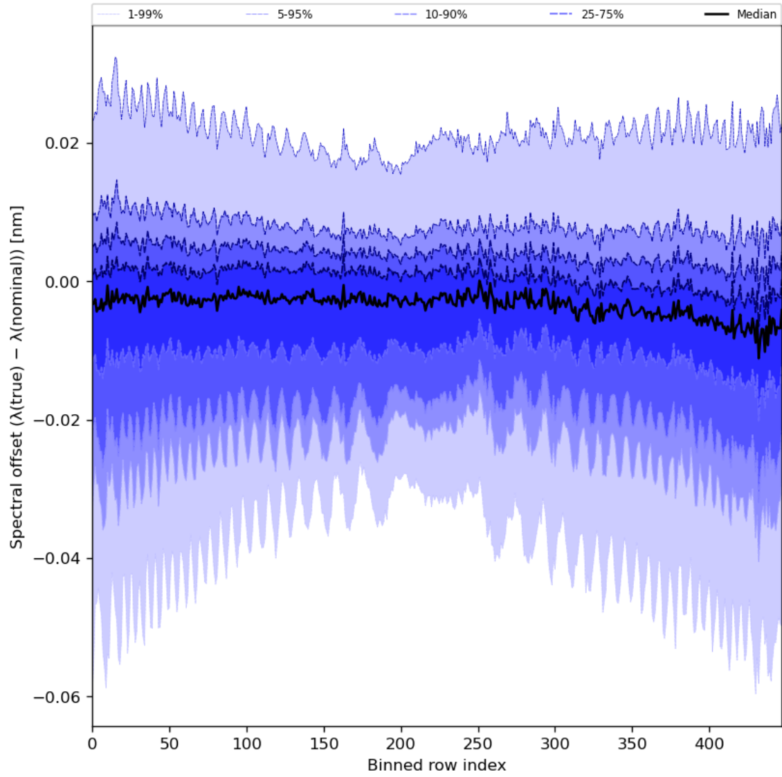
Figure 62: Along track statistics of “Spectral offset ( \lambda(\text{true}) - \lambda(\text{nominal}) )” for 2024-03-31 to 2024-04-01
