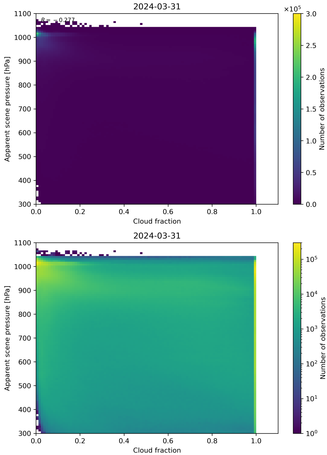
Figure 70: Scatter density plot of “Cloud fraction” against “Apparent scene pressure” for 2024-03-31 to 2024-04-01.
