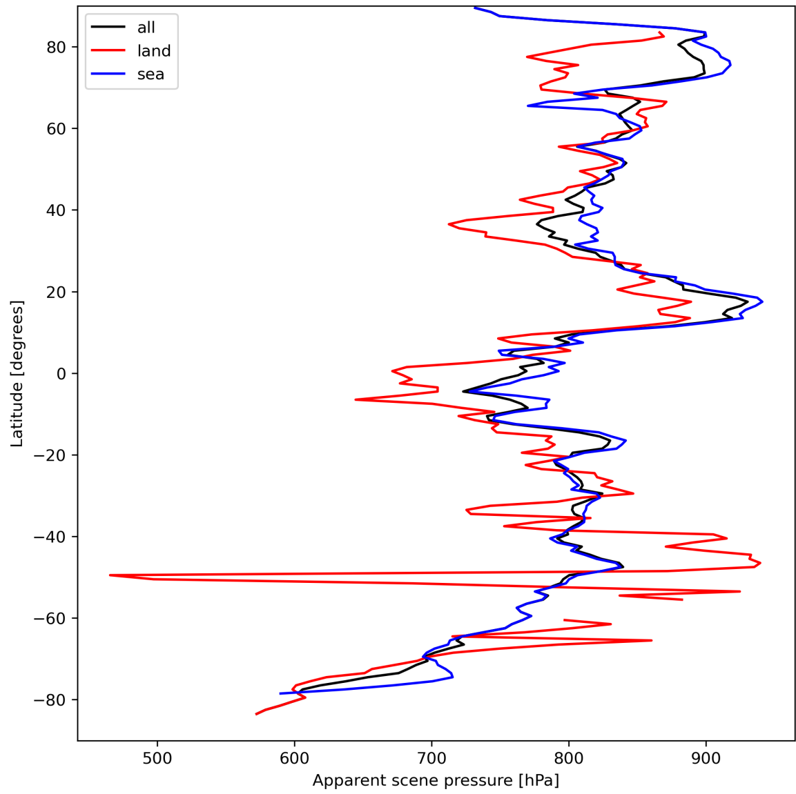
Figure 19: Zonal average of “Apparent scene pressure” for 2024-03-31 to 2024-04-01.
