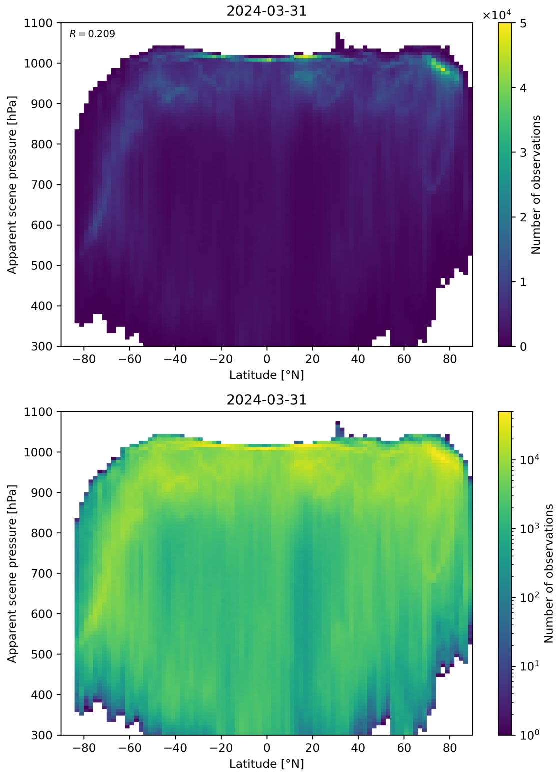
Figure 88: Scatter density plot of “Latitude” against “Apparent scene pressure” for 2024-03-31 to 2024-04-01.
