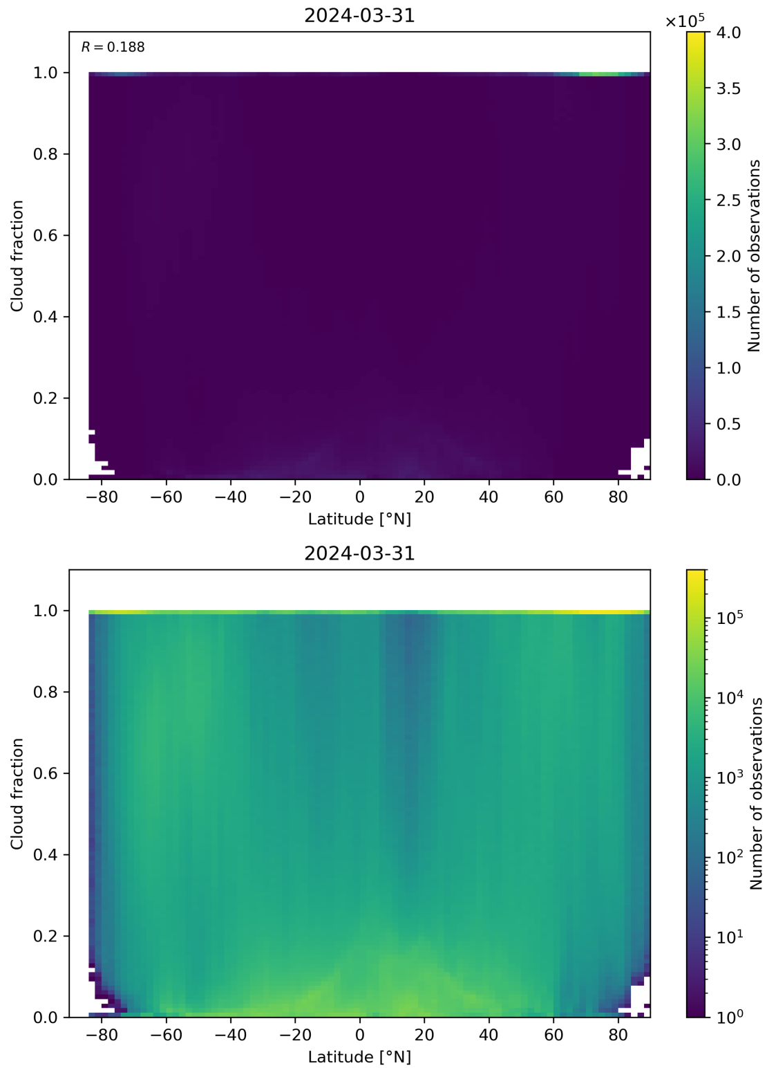
Figure 90: Scatter density plot of “Latitude” against “Cloud fraction” for 2024-03-31 to 2024-04-01.
