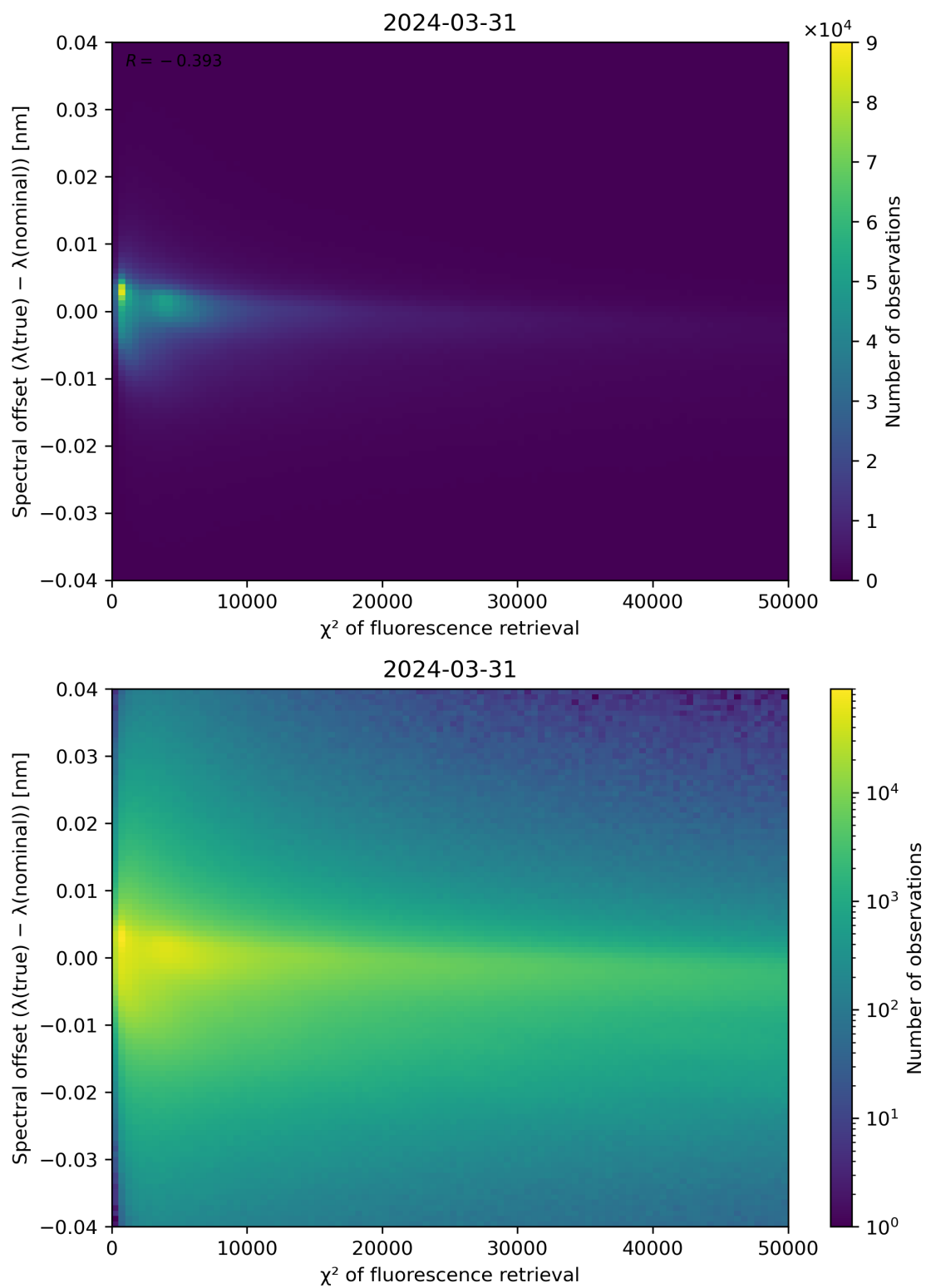
Figure 69: Scatter density plot of " \chi^2 of fluorescence retrieval" against "Spectral offset ( \lambda(\text{true}) - \lambda(\text{nominal}) )" for 2024-03-31 to 2024-04-01.
