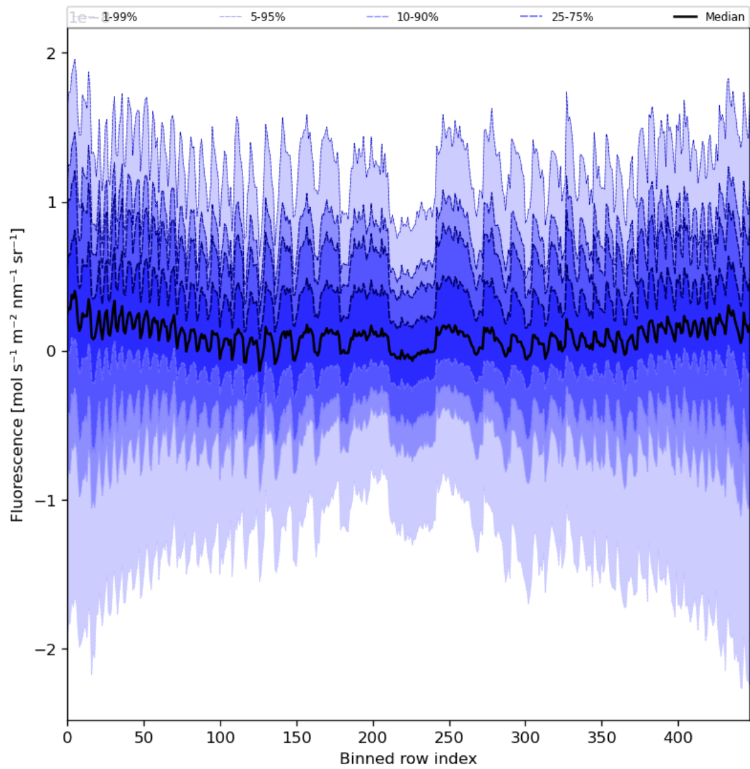
Figure 57: Along track statistics of “Fluorescence” for 2024-03-31 to 2024-04-01
