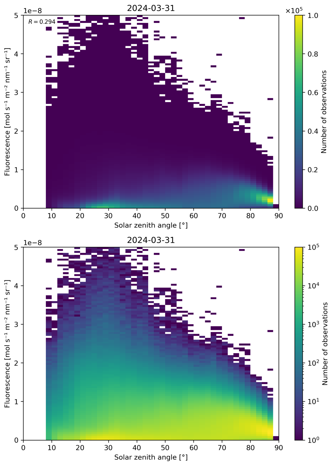
Figure 112: Scatter density plot of “Solar zenith angle” against “Fluorescence” for 2024-03-31 to 2024-04-01.
