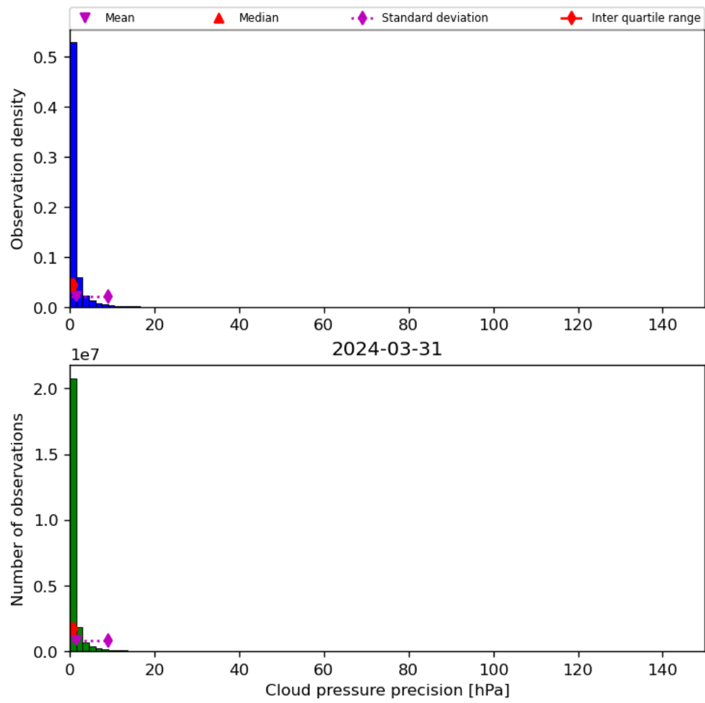
Figure 31: Histogram of “Cloud pressure precision” for 2024-03-31 to 2024-04-01
