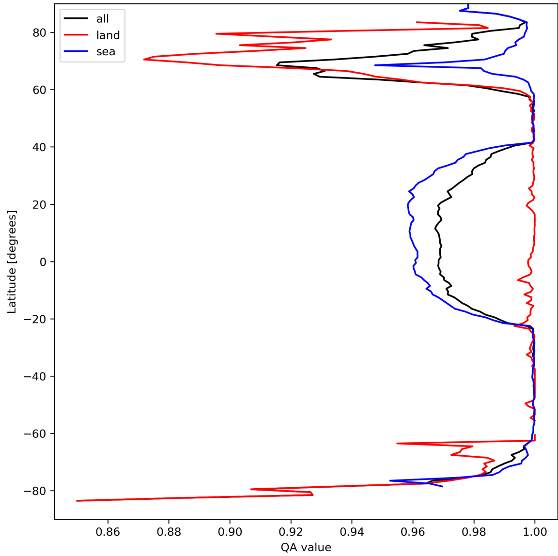
Figure 12: Zonal average of “QA value” for 2024-03-31 to 2024-04-01.
