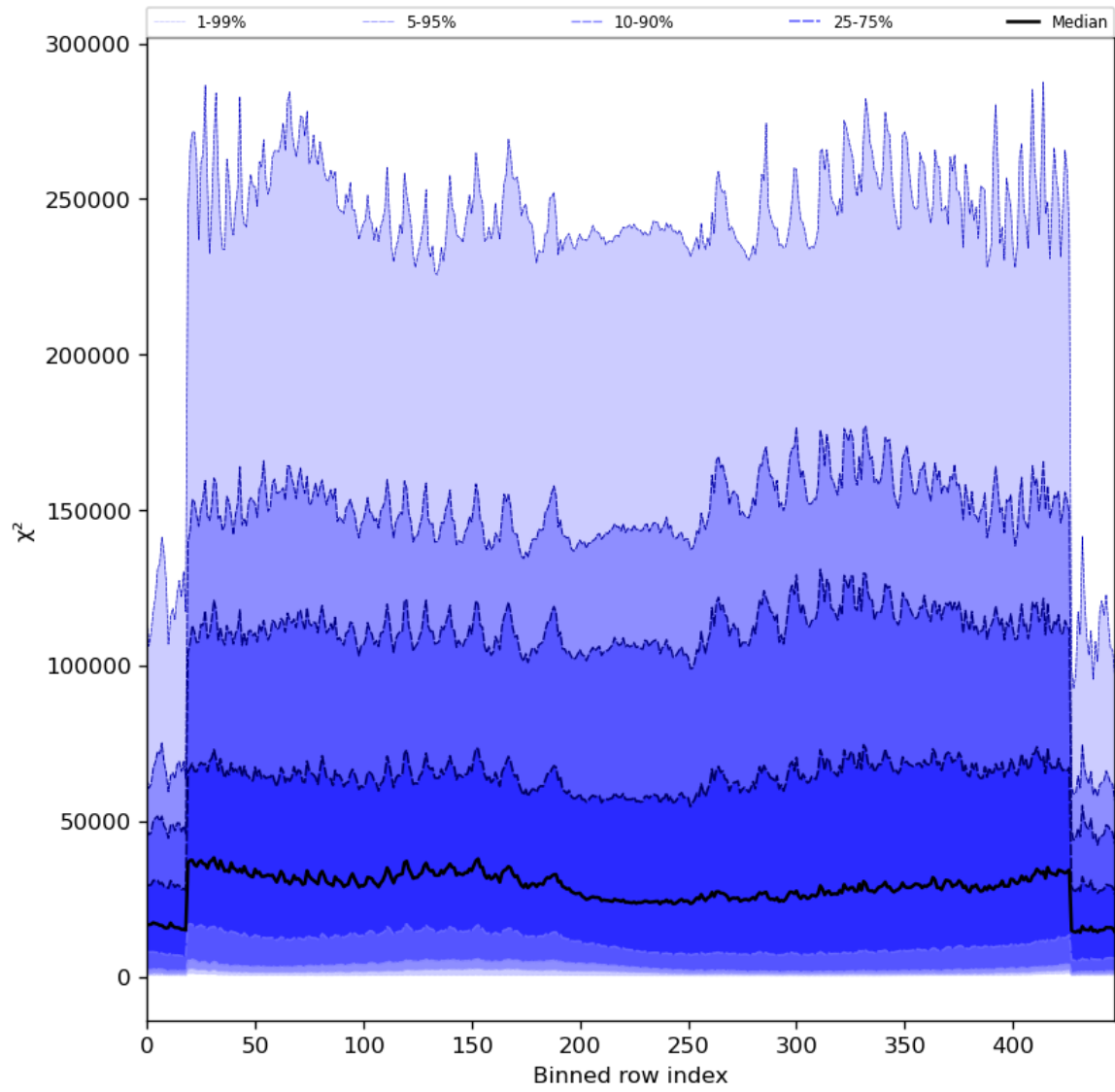
Figure 55: Along track statistics of “ \chi^2 ” for 2024-03-31 to 2024-04-01
