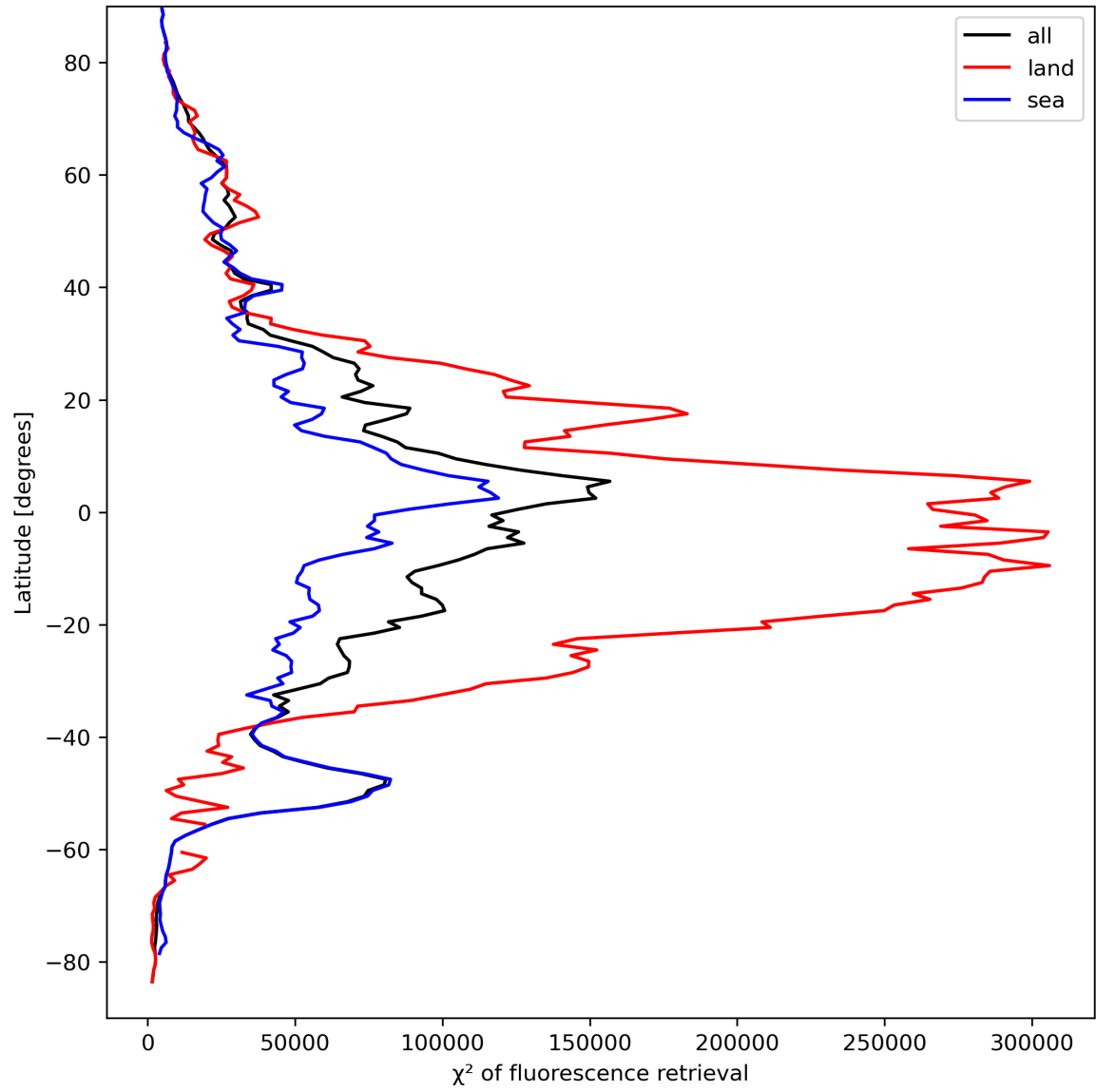
Figure 25: Zonal average of “ \chi^2 of fluorescence retrieval” for 2024-03-31 to 2024-04-01.
