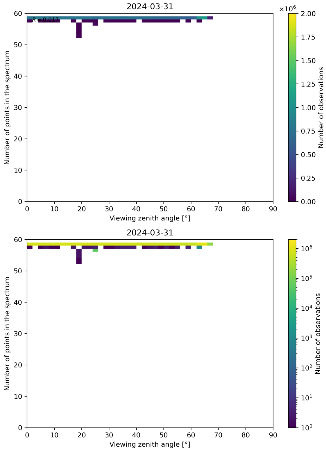
Figure 125: Scatter density plot of “Viewing zenith angle” against “Number of points in the spectrum” for 2024-03-31 to 2024-04-01.
