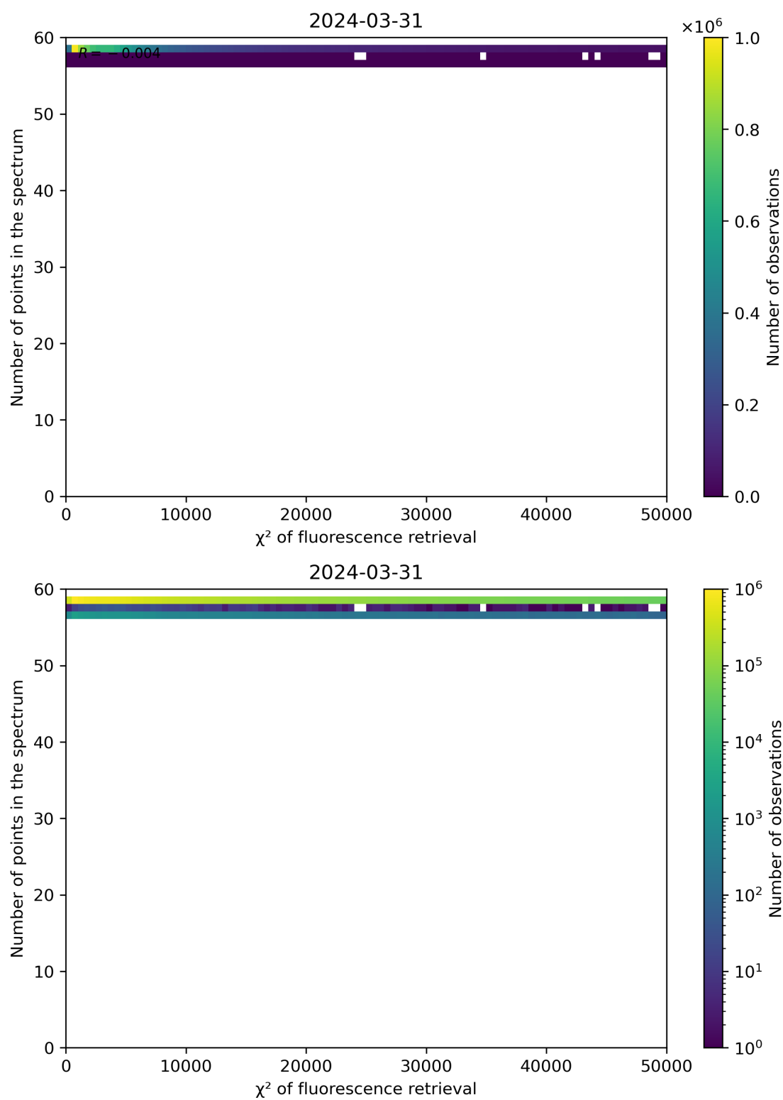
Figure 68: Scatter density plot of “ \chi^2 of fluorescence retrieval” against “Number of points in the spectrum” for 2024-03-31 to 2024-04-01.
