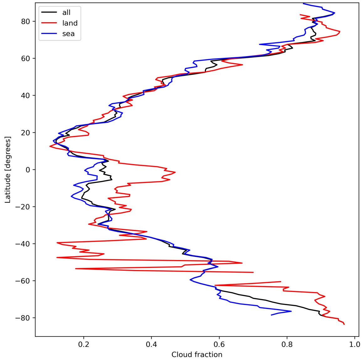
Figure 15: Zonal average of “Cloud fraction” for 2024-03-31 to 2024-04-01.
