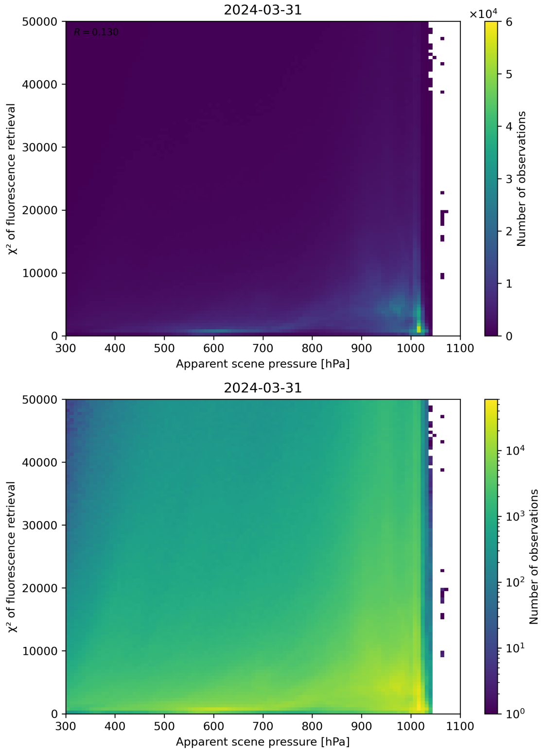
Figure 63: Scatter density plot of “Apparent scene pressure” against “ \chi^2 of fluorescence retrieval” for 2024-03-31 to 2024-04-01.
