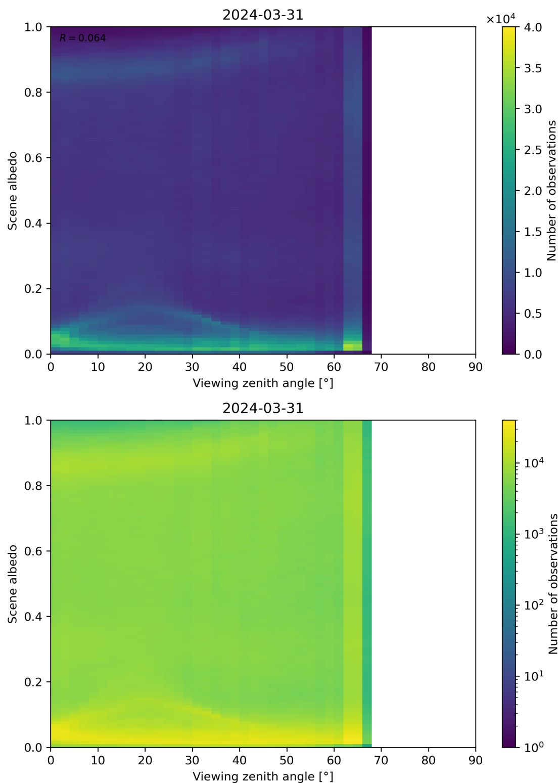
Figure 126: Scatter density plot of “Viewing zenith angle” against “Scene albedo” for 2024-03-31 to 2024-04-01.
