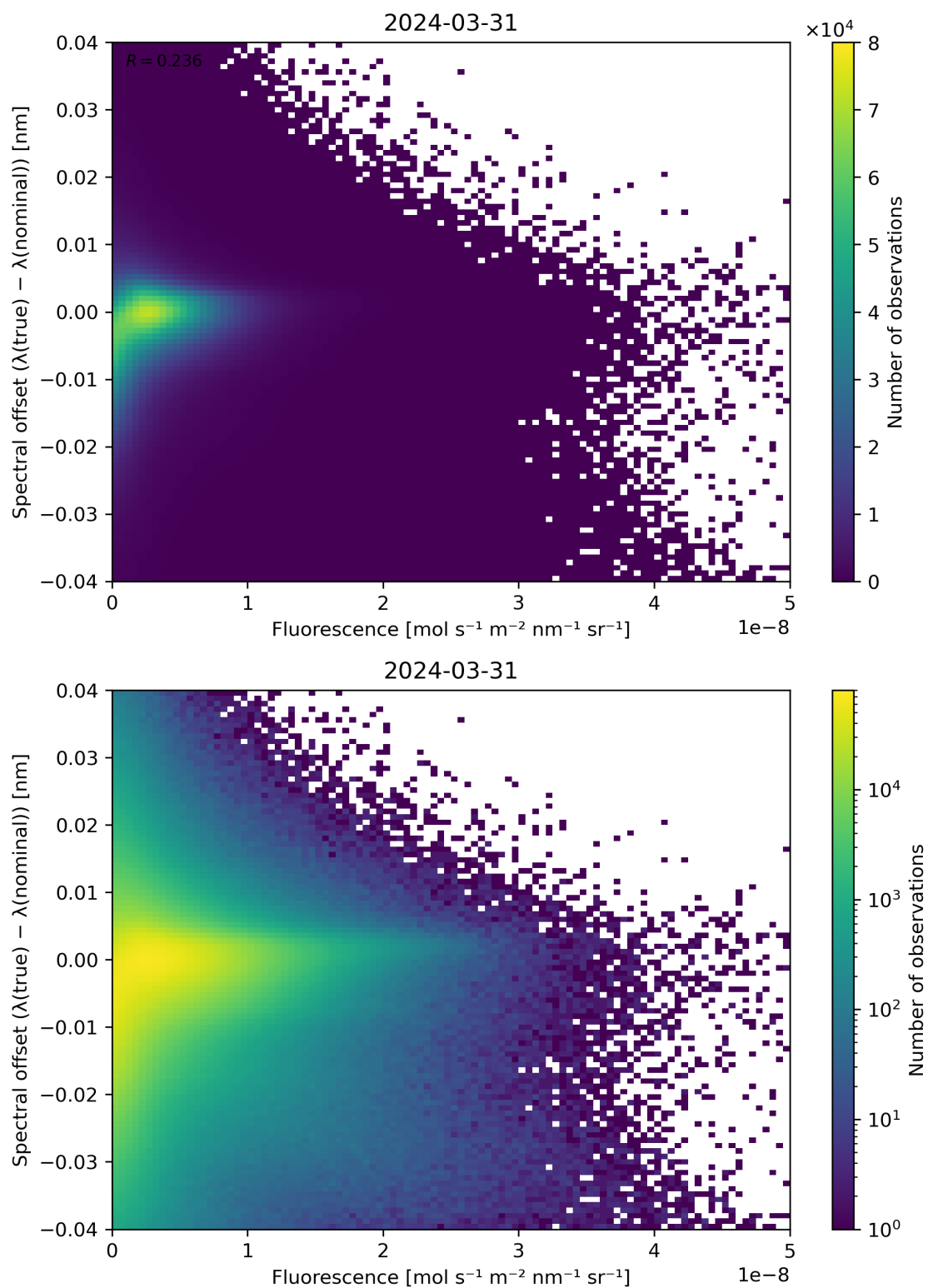
Figure 87: Scatter density plot of “Fluorescence” against “Spectral offset ( \lambda(\text{true}) - \lambda(\text{nominal}) )” for 2024-03-31 to 2024-04-01.
