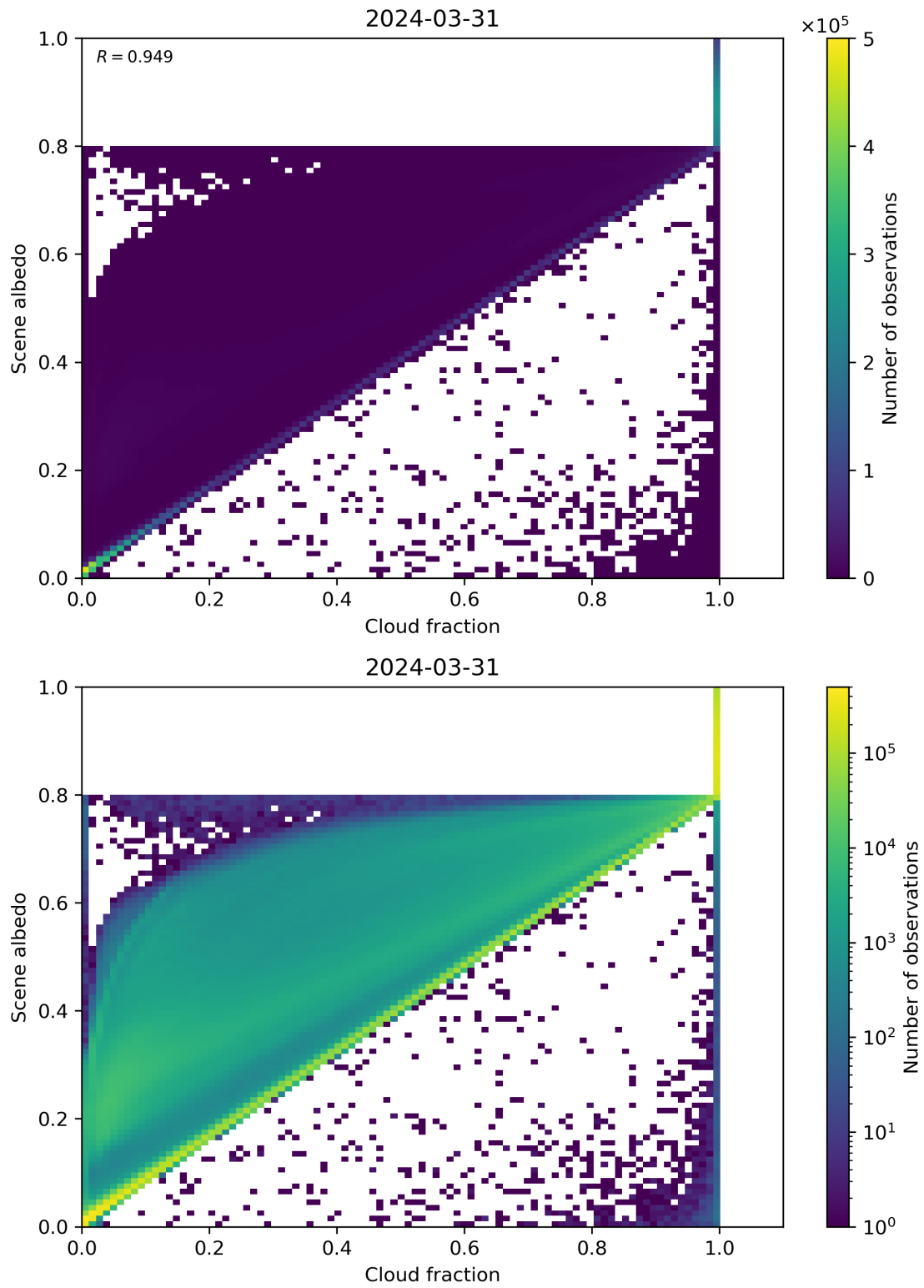
Figure 75: Scatter density plot of “Cloud fraction” against “Scene albedo” for 2024-03-31 to 2024-04-01.
