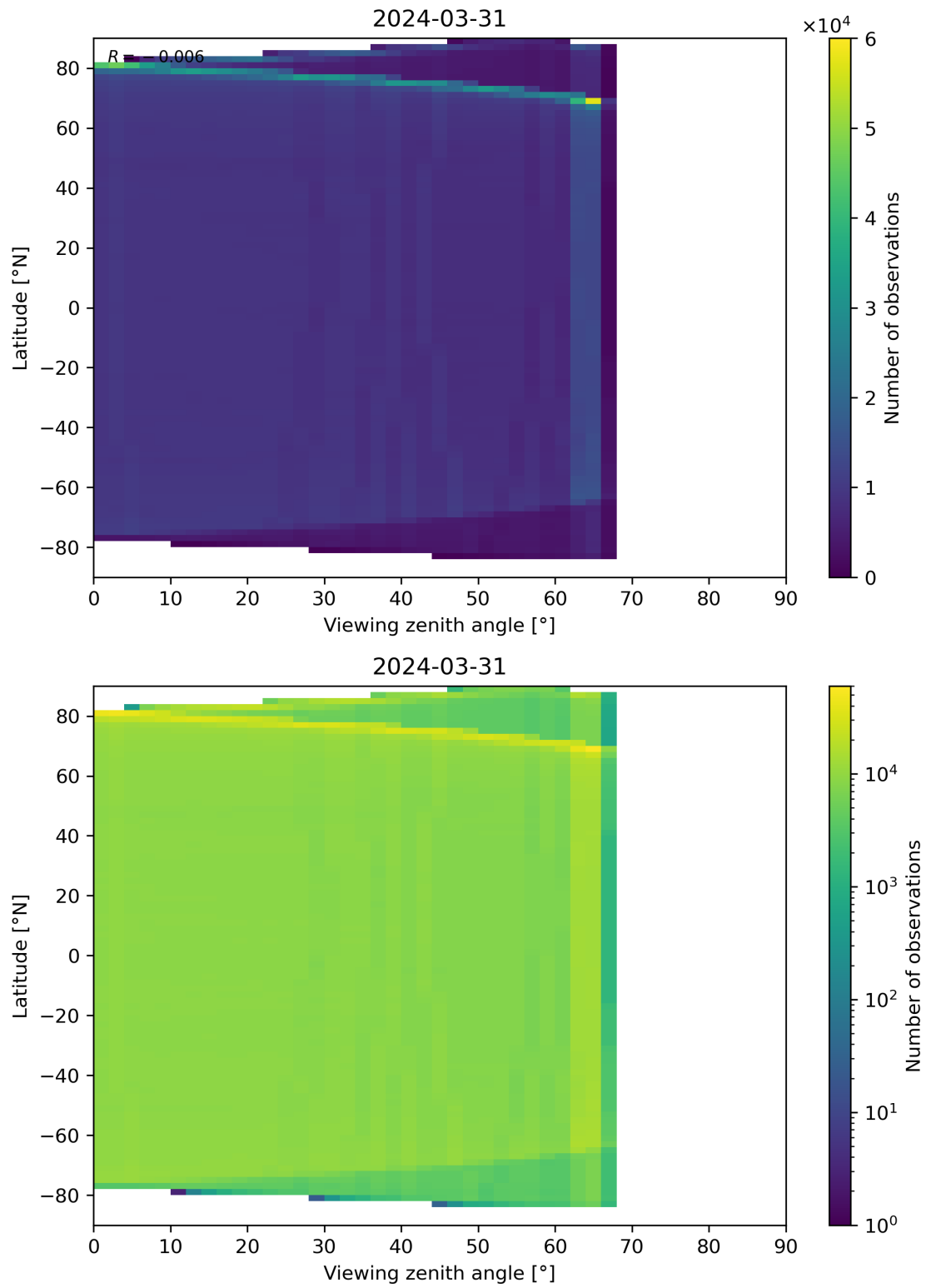
Figure 123: Scatter density plot of “Viewing zenith angle” against “Latitude” for 2024-03-31 to 2024-04-01.
