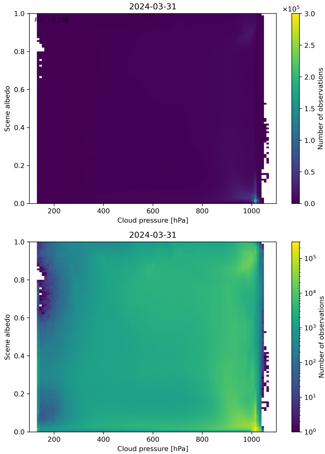
Figure 83: Scatter density plot of “Cloud pressure” against “Scene albedo” for 2024-03-31 to 2024-04-01.
