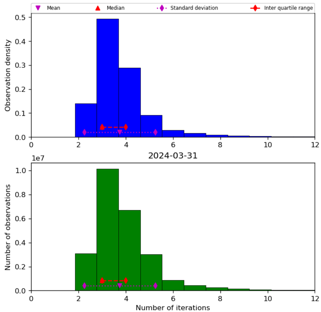
Figure 39: Histogram of “Number of iterations” for 2024-03-31 to 2024-04-01
