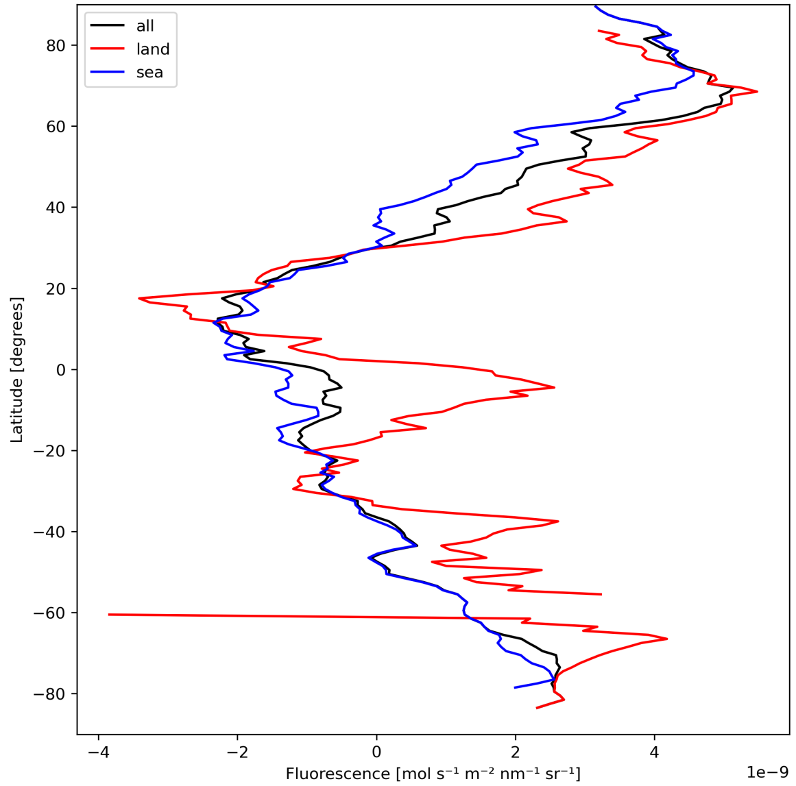
Figure 23: Zonal average of “Fluorescence” for 2024-03-31 to 2024-04-01.
