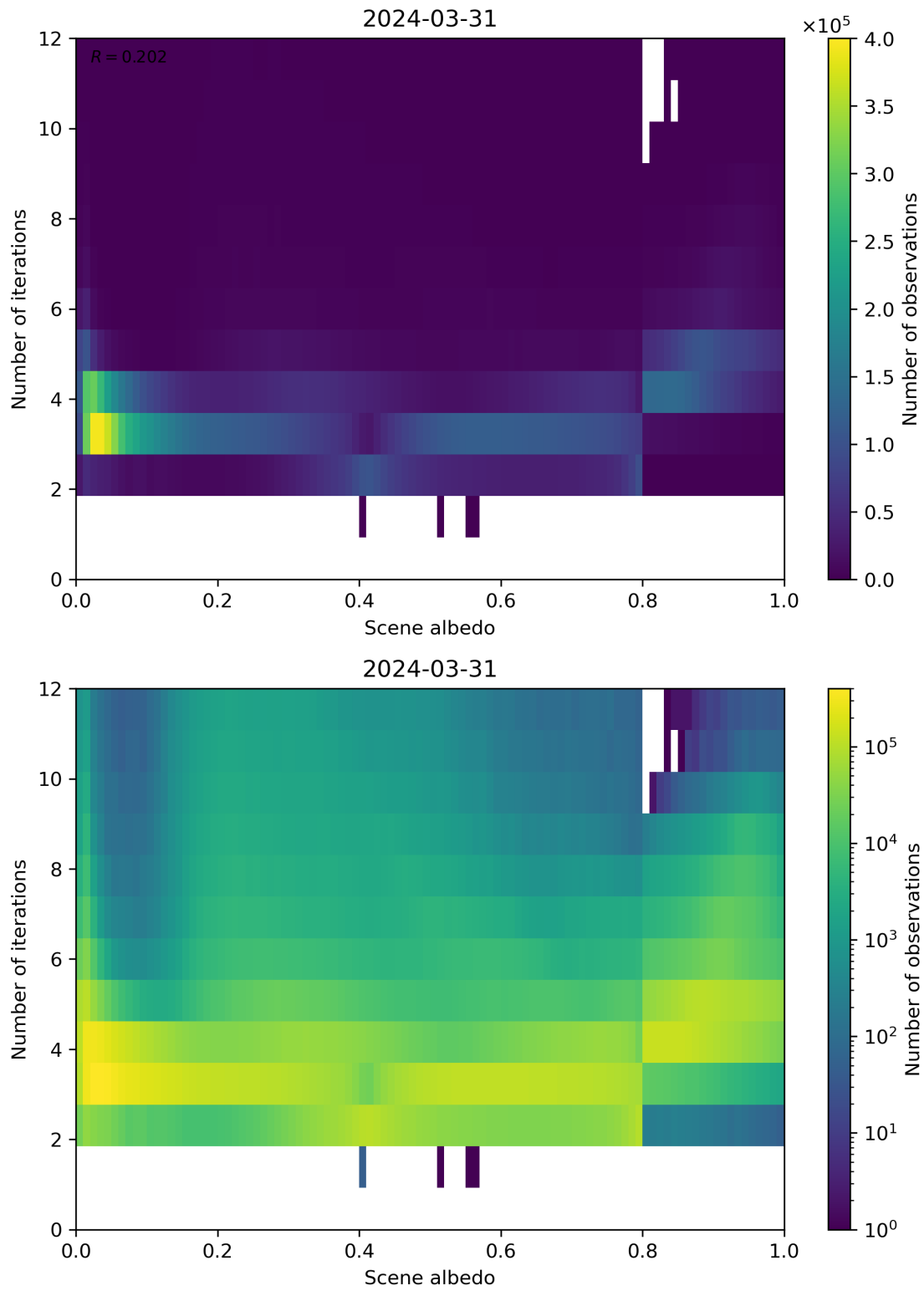
Figure 105: Scatter density plot of “Scene albedo” against “Number of iterations” for 2024-03-31 to 2024-04-01.
