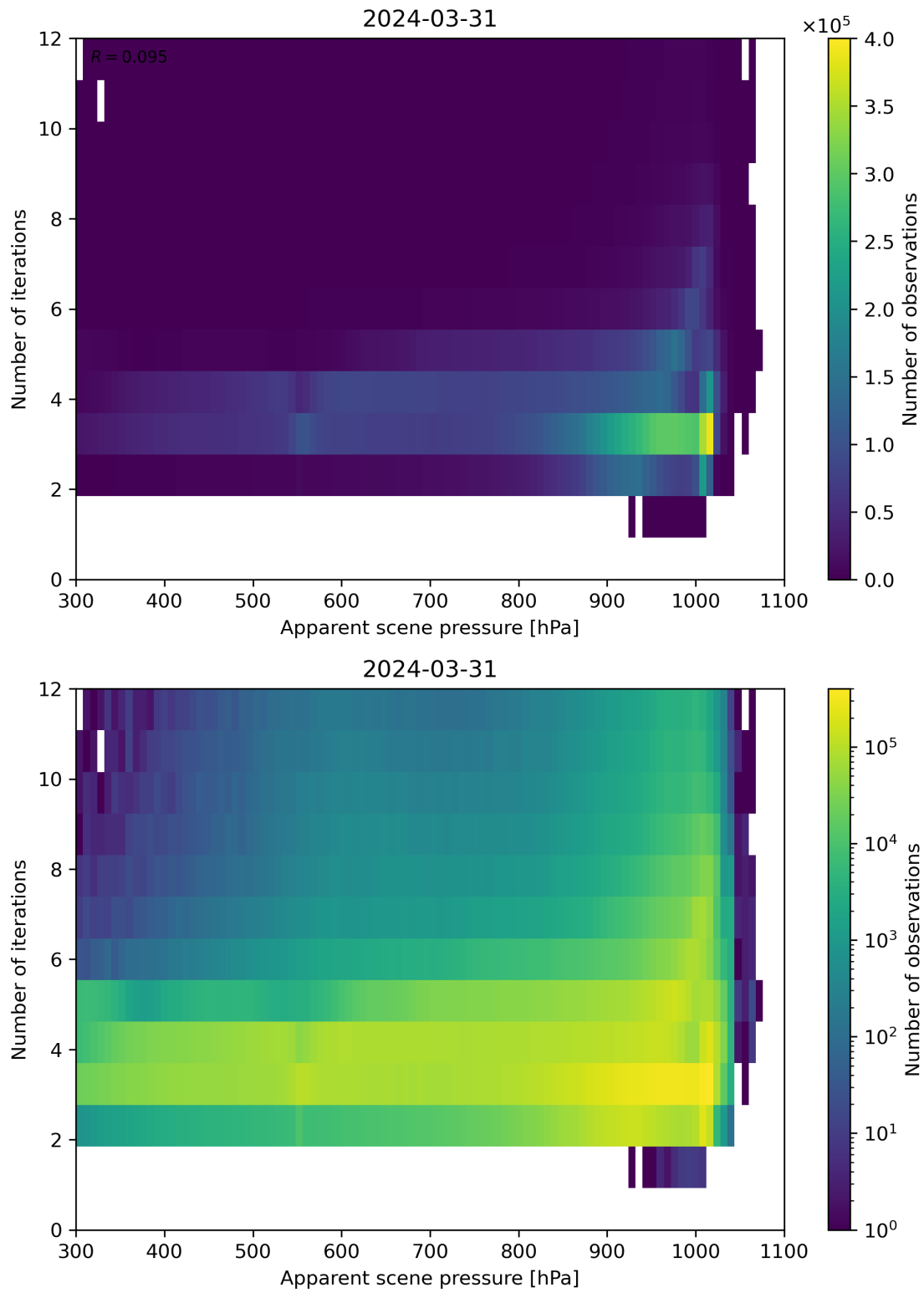
Figure 65: Scatter density plot of “Apparent scene pressure” against “Number of iterations” for 2024-03-31 to 2024-04-01.
