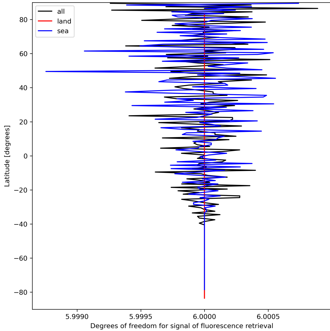
Figure 26: Zonal average of “Degrees of freedom for signal of fluorescence retrieval” for 2024-03-31 to 2024-04-01.
