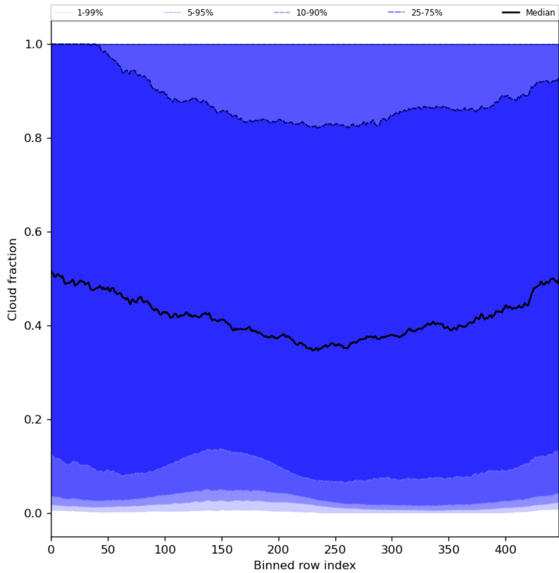
Figure 49: Along track statistics of “Cloud fraction” for 2024-03-31 to 2024-04-01
