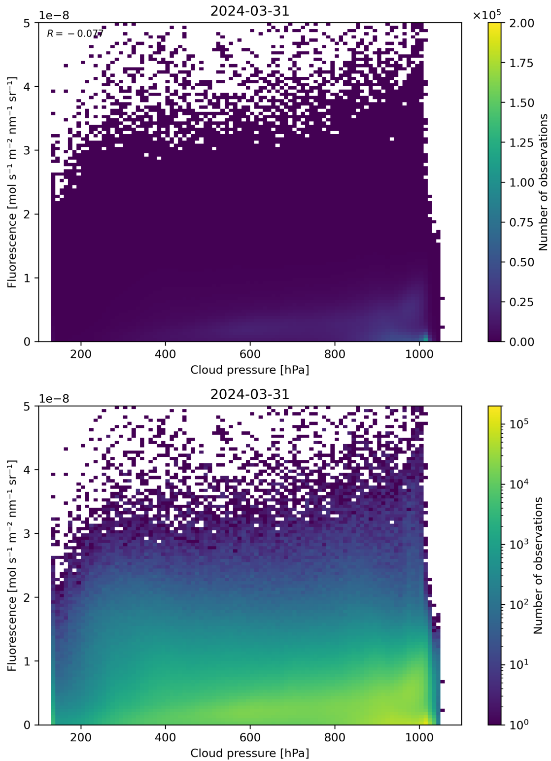
Figure 80: Scatter density plot of “Cloud pressure” against “Fluorescence” for 2024-03-31 to 2024-04-01.
