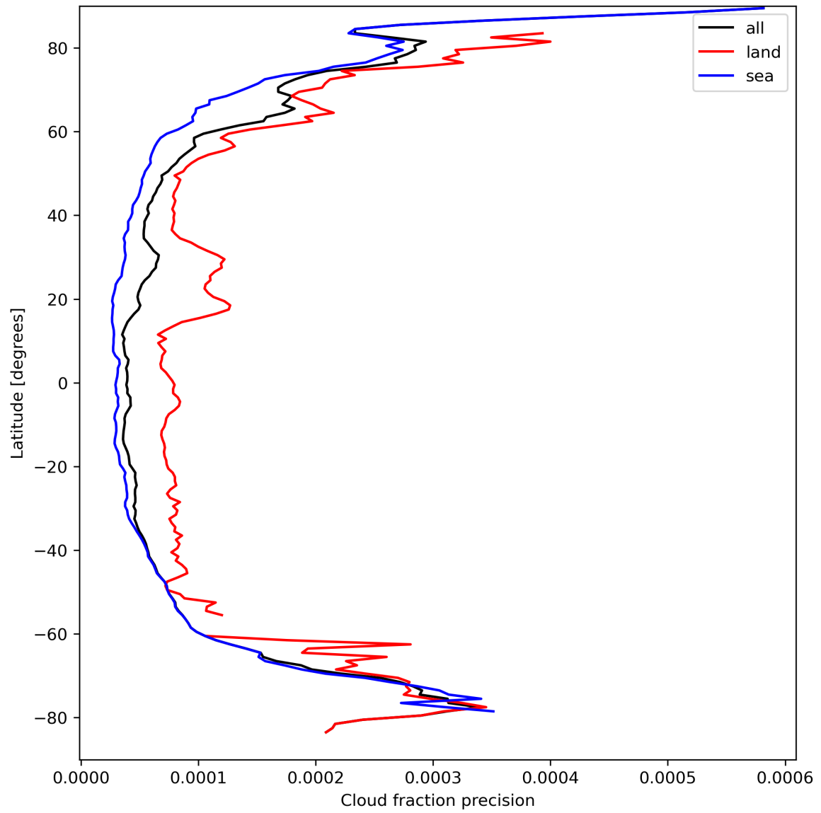
Figure 16: Zonal average of “Cloud fraction precision” for 2024-03-31 to 2024-04-01.
