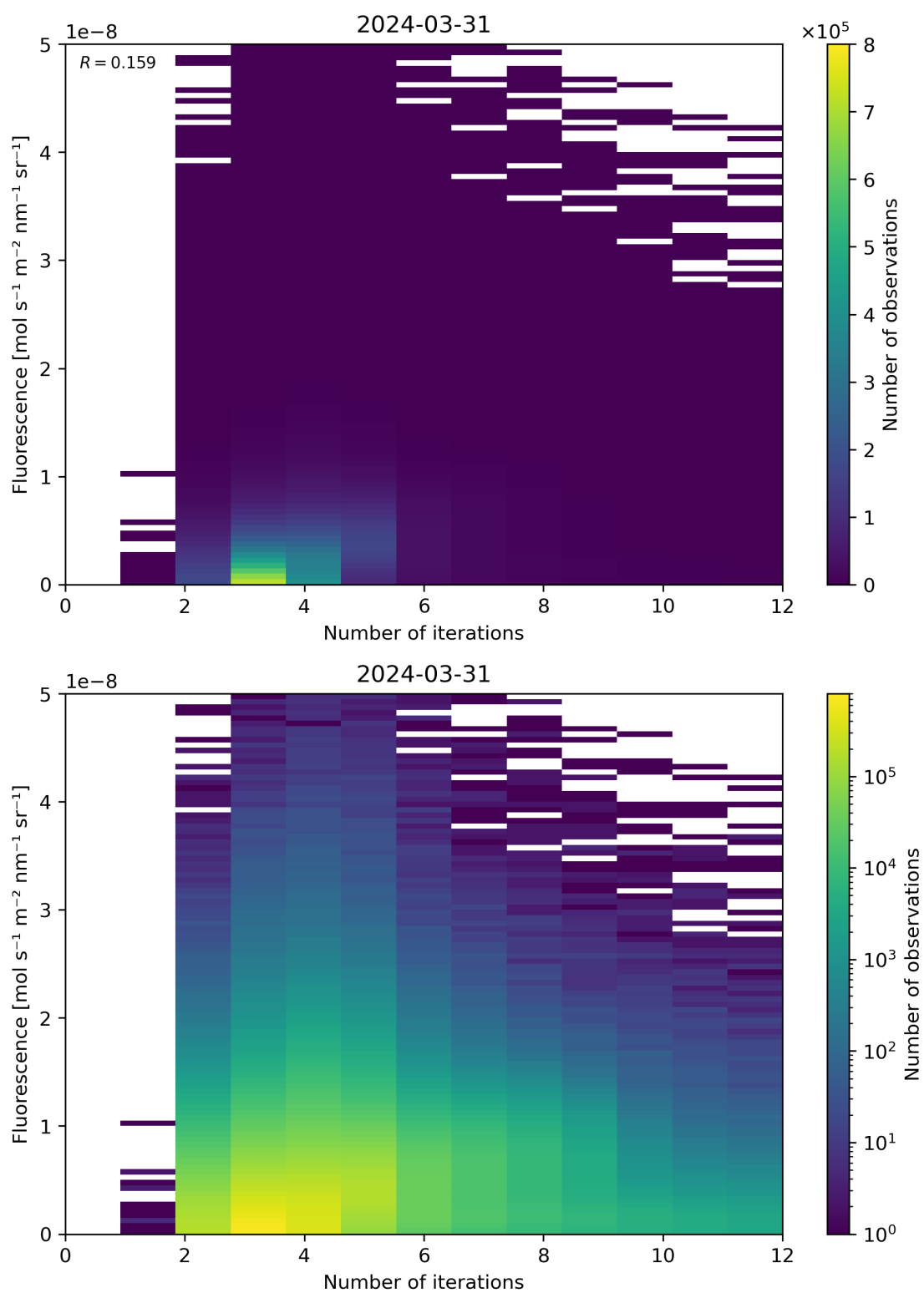
Figure 98: Scatter density plot of “Number of iterations” against “Fluorescence” for 2024-03-31 to 2024-04-01.
