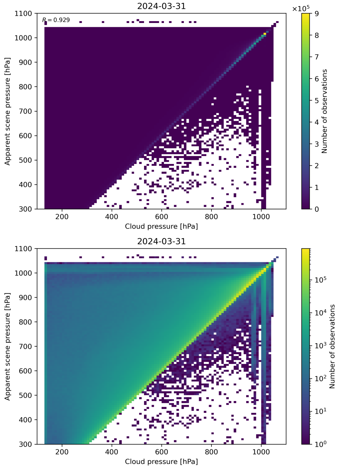
Figure 77: Scatter density plot of “Cloud pressure” against “Apparent scene pressure” for 2024-03-31 to 2024-04-01.
