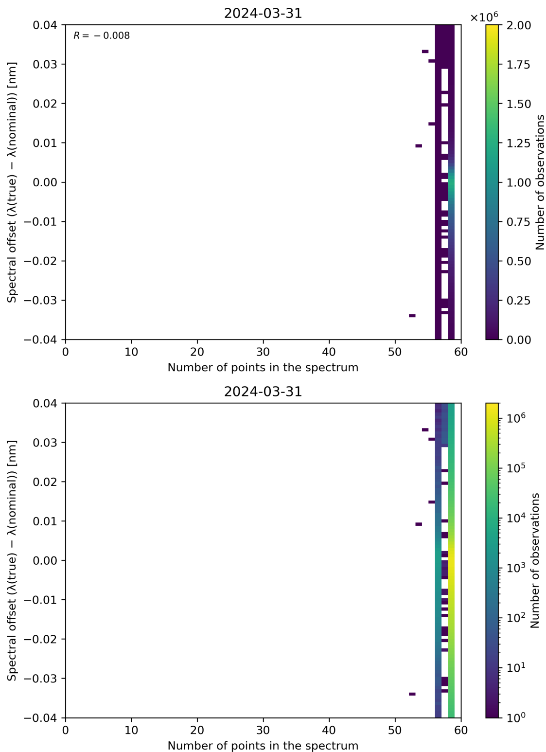
Figure 101: Scatter density plot of “Number of points in the spectrum” against “Spectral offset ( \lambda(\text{true}) - \lambda(\text{nominal}) )” for 2024-03-31 to 2024-04-01.
