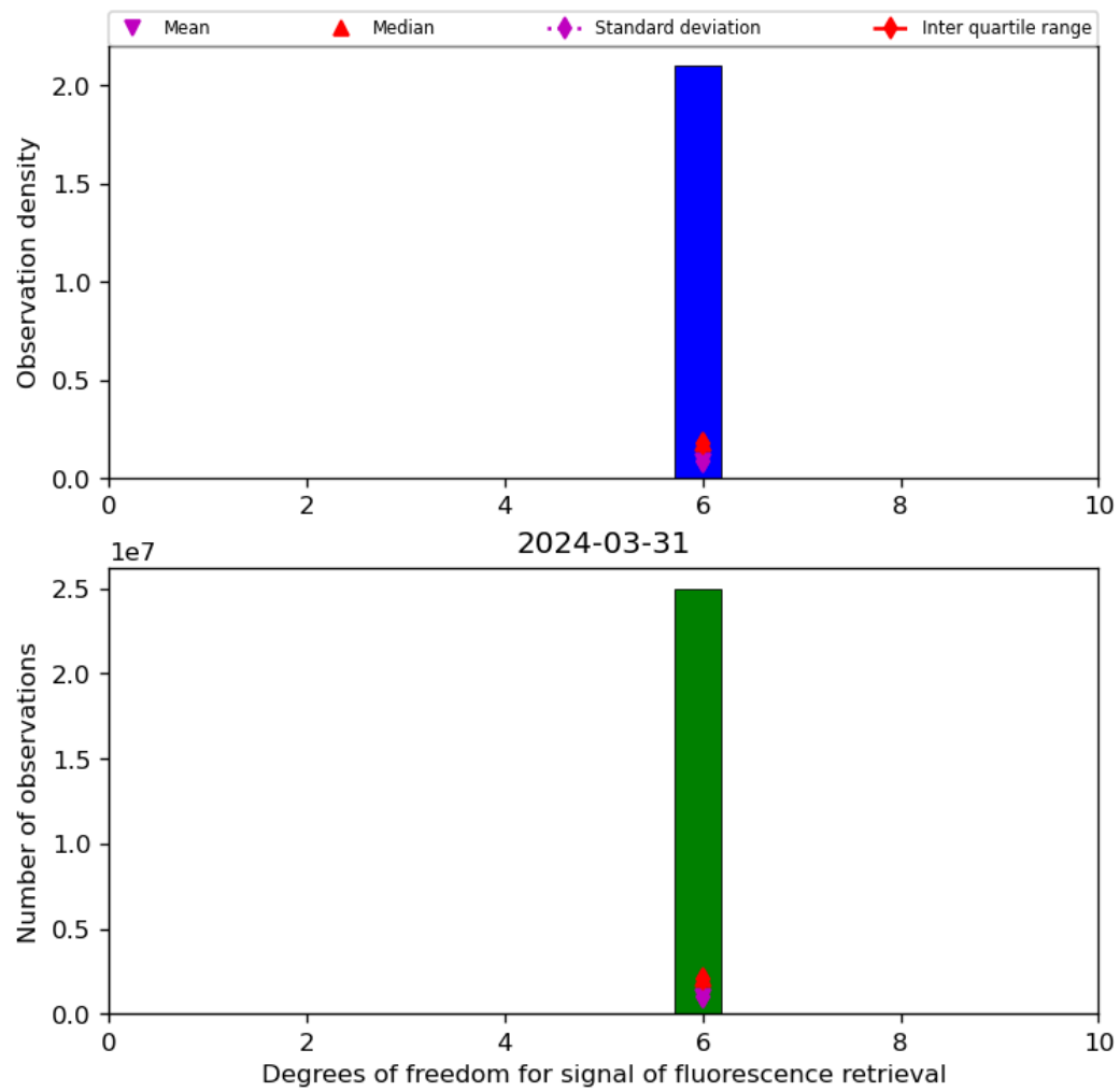
Figure 43: Histogram of “Degrees of freedom for signal of fluorescence retrieval” for 2024-03-31 to 2024-04-01
