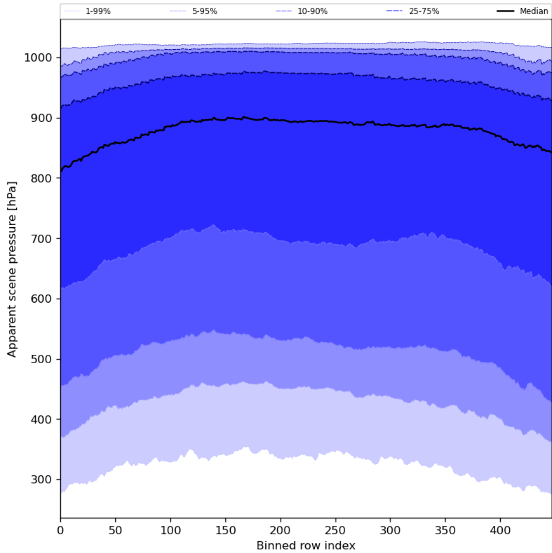
Figure 53: Along track statistics of “Apparent scene pressure” for 2024-03-31 to 2024-04-02
