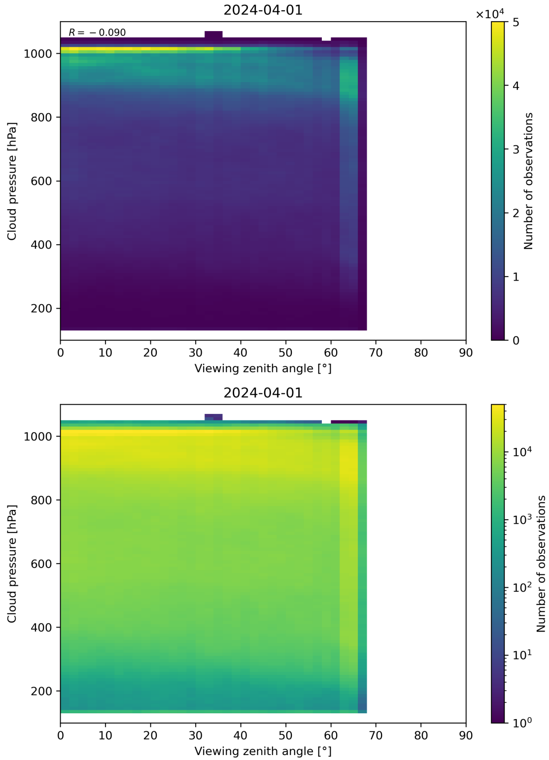
Figure 121: Scatter density plot of “Viewing zenith angle” against “Cloud pressure” for 2024-03-31 to 2024-04-02.
