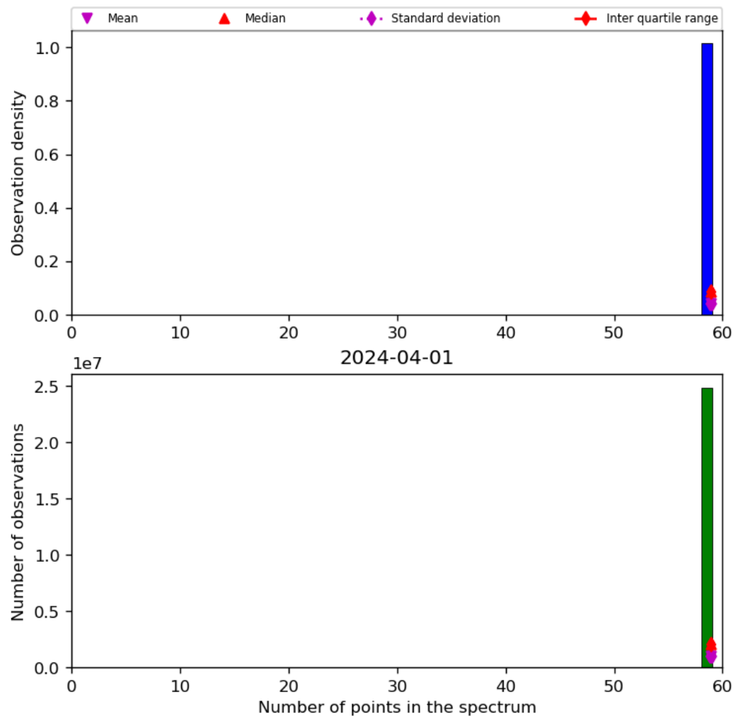
Figure 44: Histogram of “Number of points in the spectrum” for 2024-03-31 to 2024-04-02
