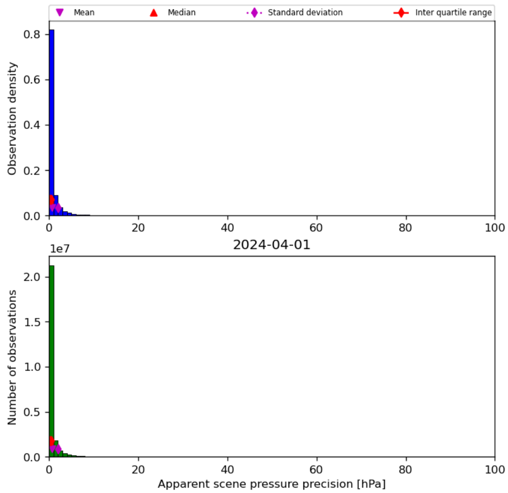
Figure 37: Histogram of “Apparent scene pressure precision” for 2024-03-31 to 2024-04-02
