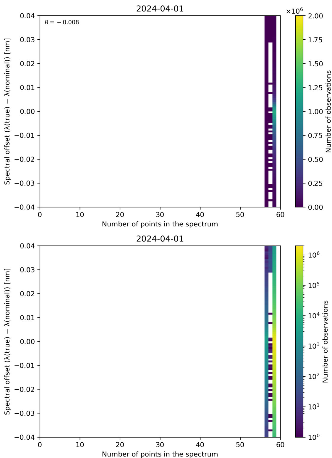
Figure 101: Scatter density plot of “Number of points in the spectrum” against “Spectral offset ( \lambda(\text{true}) - \lambda(\text{nominal}) )” for 2024-03-31 to 2024-04-02.
