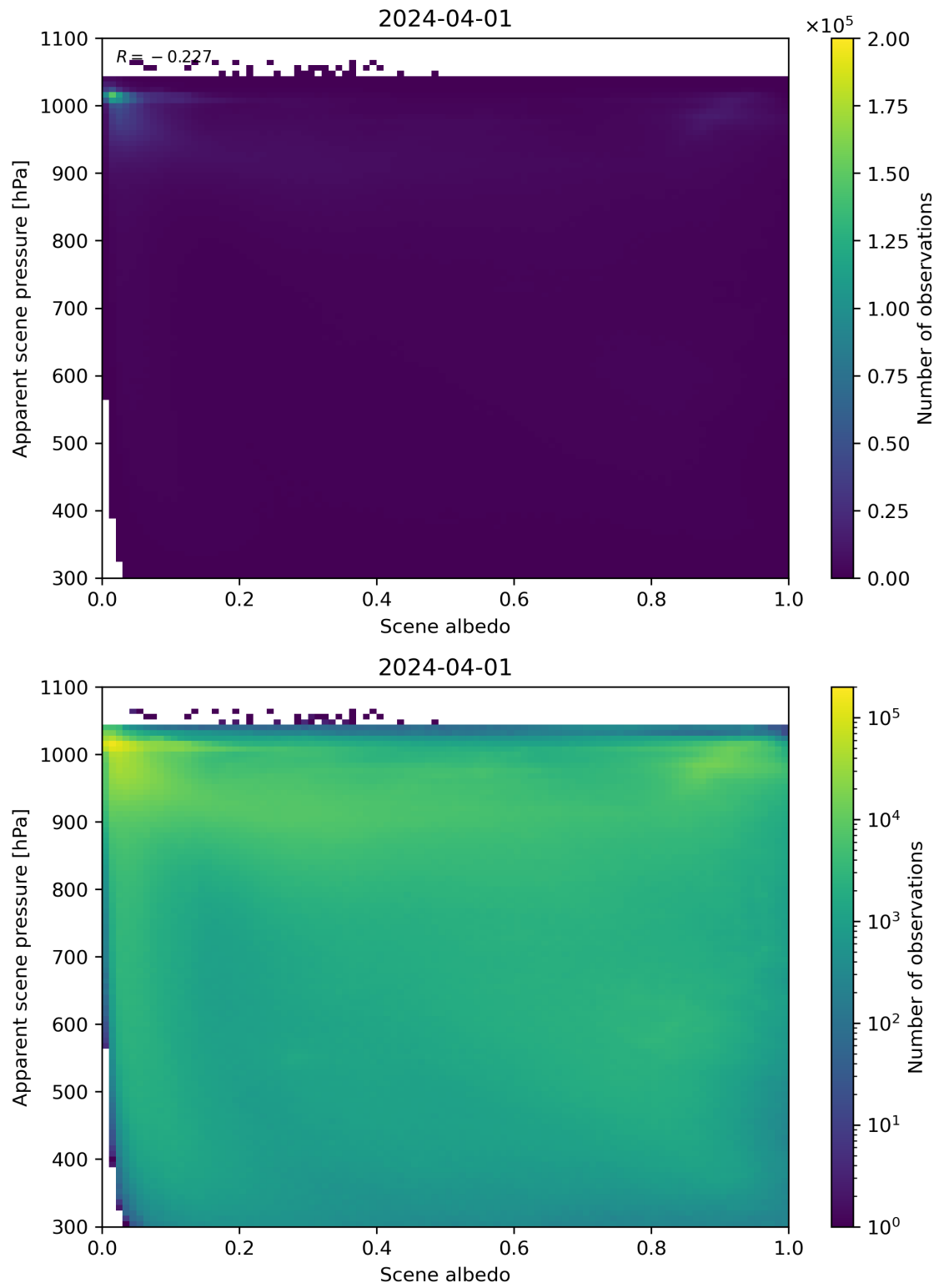
Figure 102: Scatter density plot of “Scene albedo” against “Apparent scene pressure” for 2024-03-31 to 2024-04-02.
