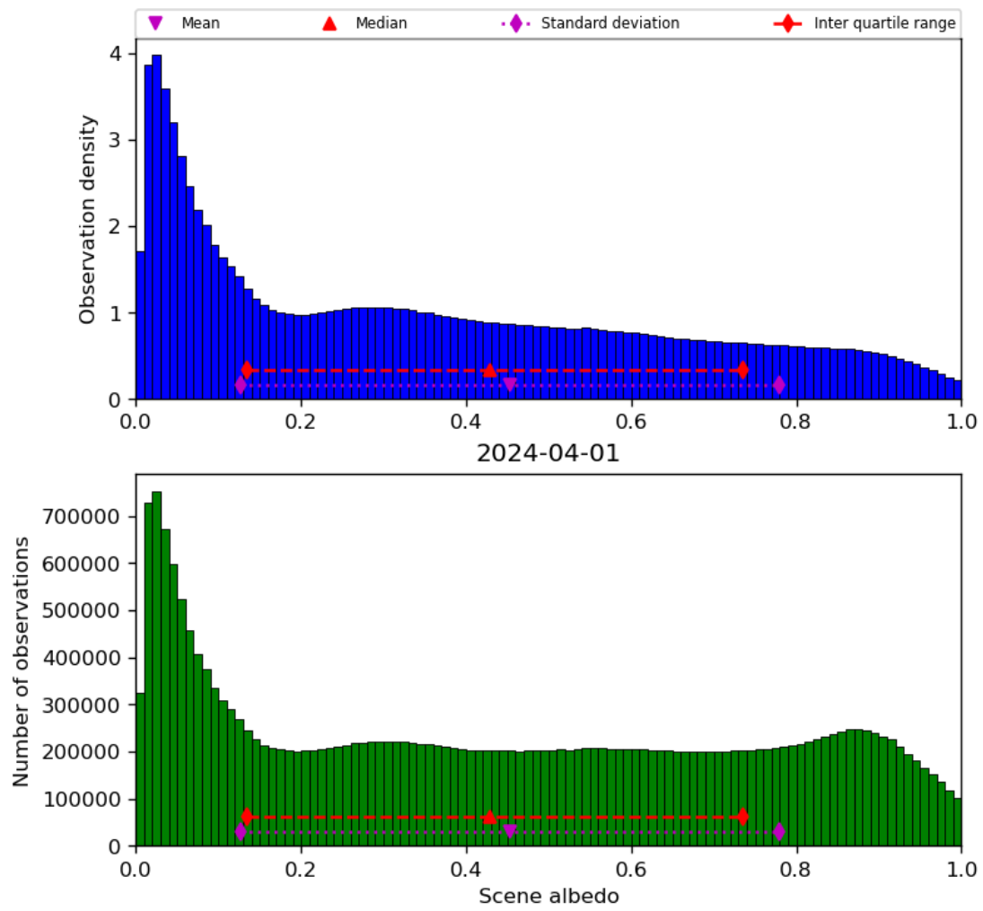
Figure 34: Histogram of “Scene albedo” for 2024-03-31 to 2024-04-02
