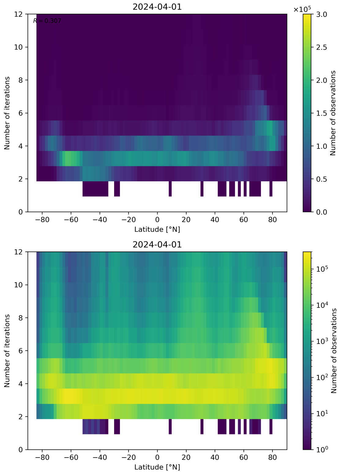
Figure 93: Scatter density plot of “Latitude” against “Number of iterations” for 2024-03-31 to 2024-04-02.
