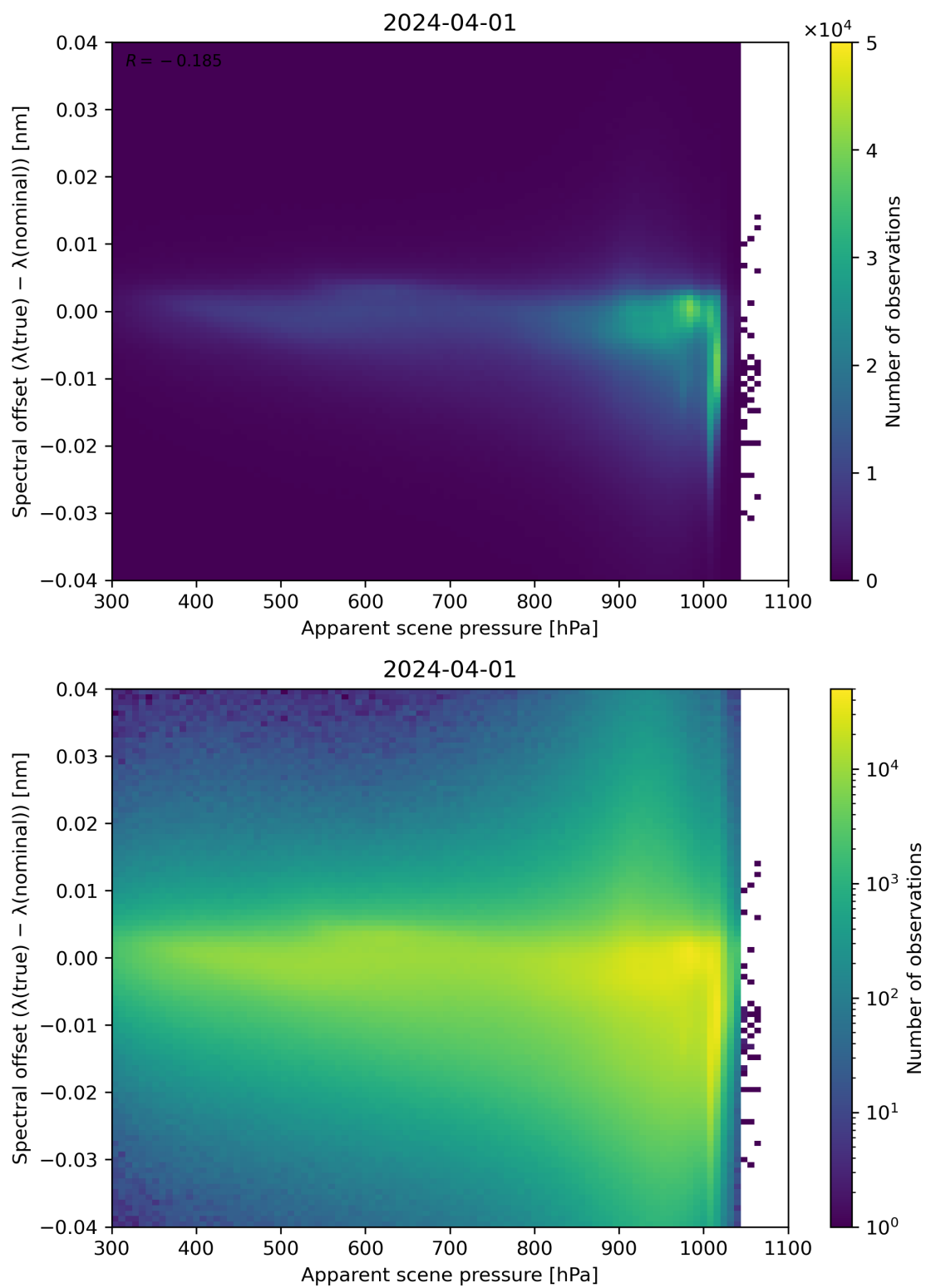
Figure 67: Scatter density plot of “Apparent scene pressure” against “Spectral offset ( \lambda(\text{true}) - \lambda(\text{nominal}) )” for 2024-03-31 to 2024-04-02.
