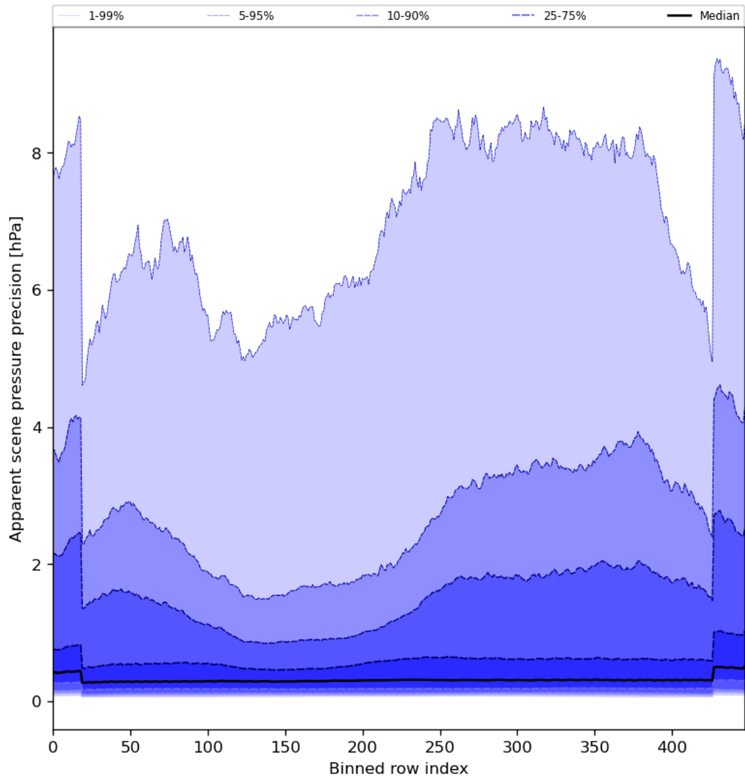
Figure 54: Along track statistics of “Apparent scene pressure precision” for 2024-03-31 to 2024-04-02
