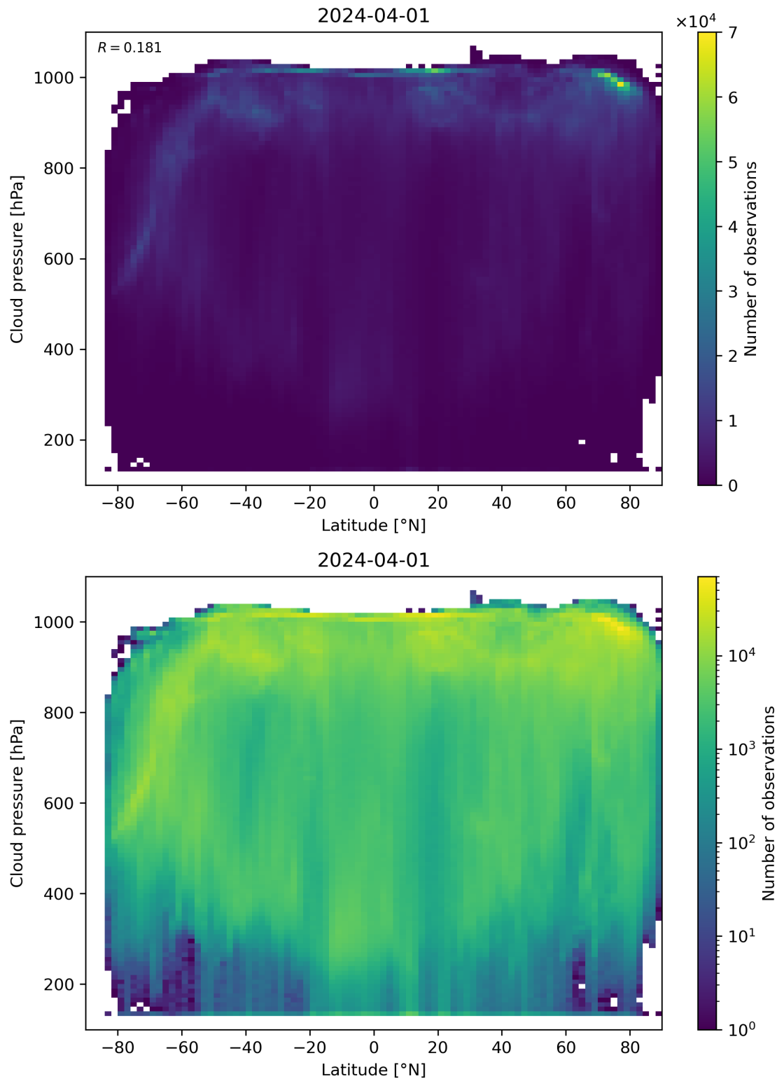
Figure 91: Scatter density plot of “Latitude” against “Cloud pressure” for 2024-03-31 to 2024-04-02.
