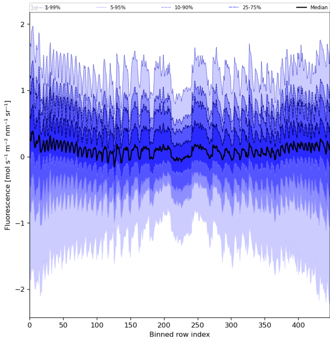
Figure 57: Along track statistics of “Fluorescence” for 2024-03-31 to 2024-04-02
