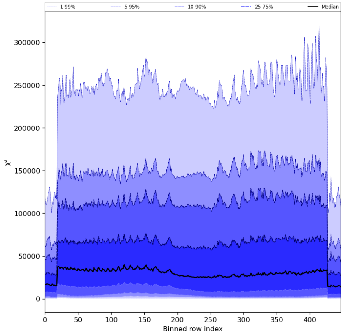
Figure 55: Along track statistics of “ \chi^2 ” for 2024-03-31 to 2024-04-02
