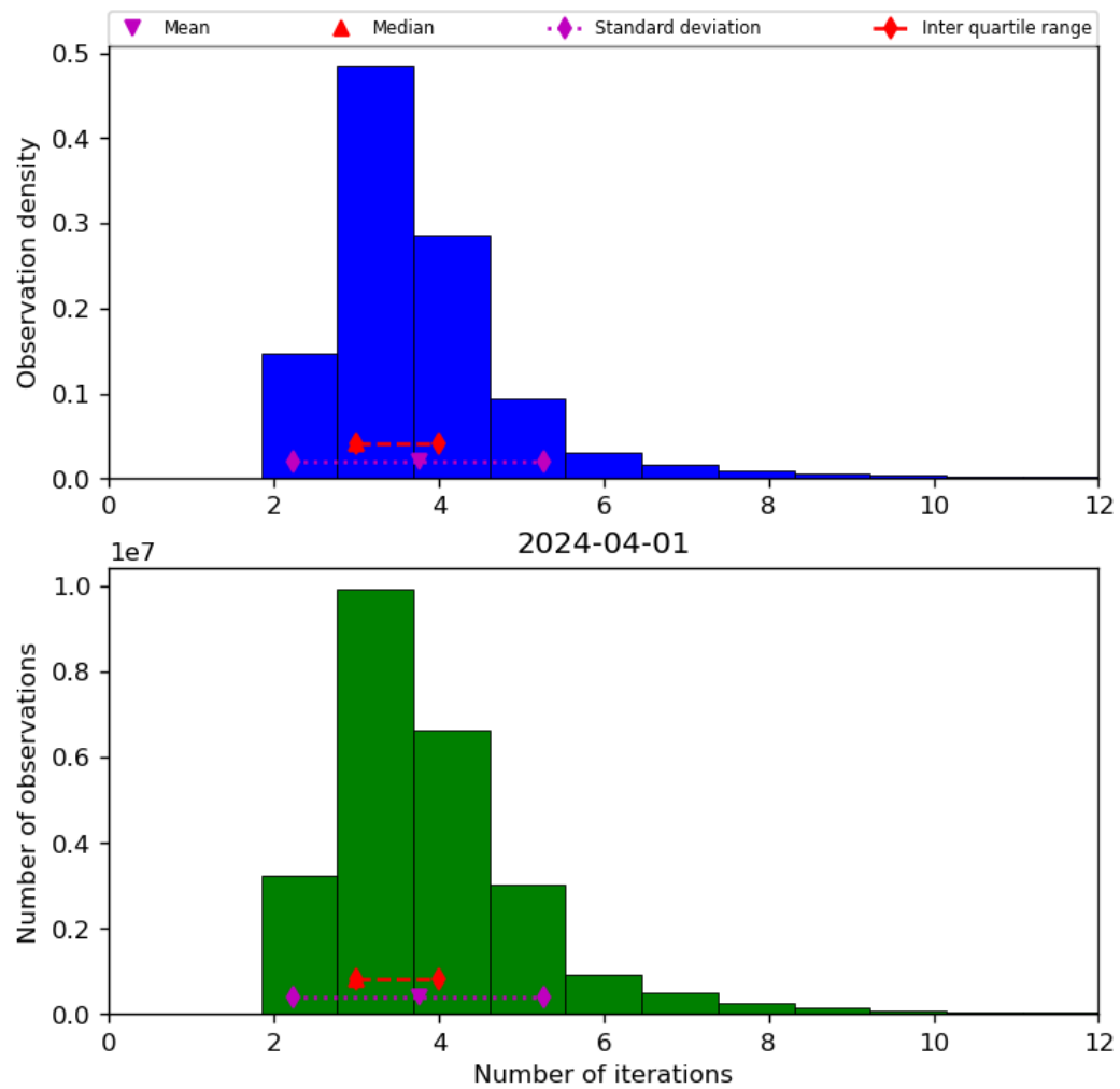
Figure 39: Histogram of “Number of iterations” for 2024-03-31 to 2024-04-02
