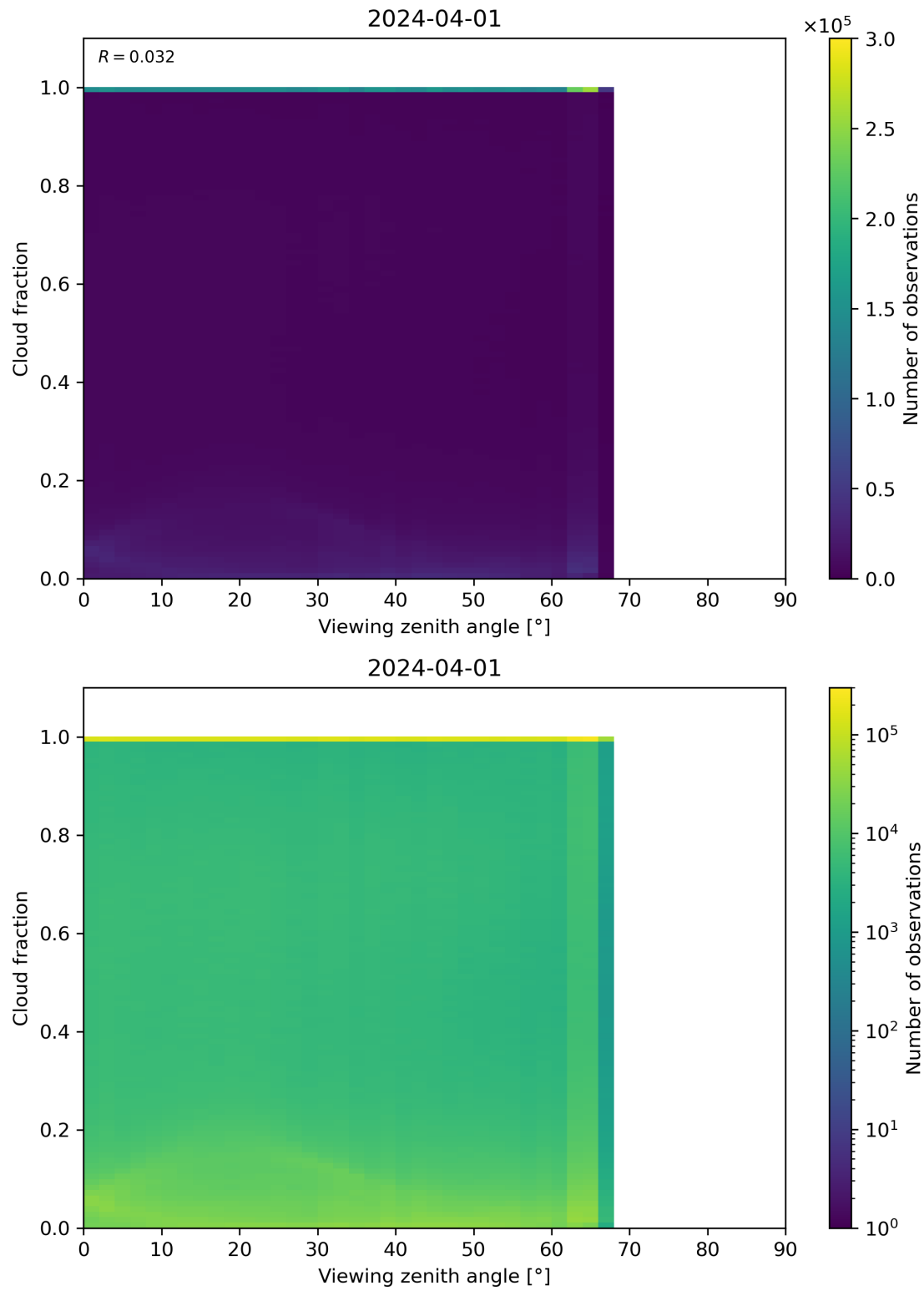
Figure 120: Scatter density plot of “Viewing zenith angle” against “Cloud fraction” for 2024-03-31 to 2024-04-02.
