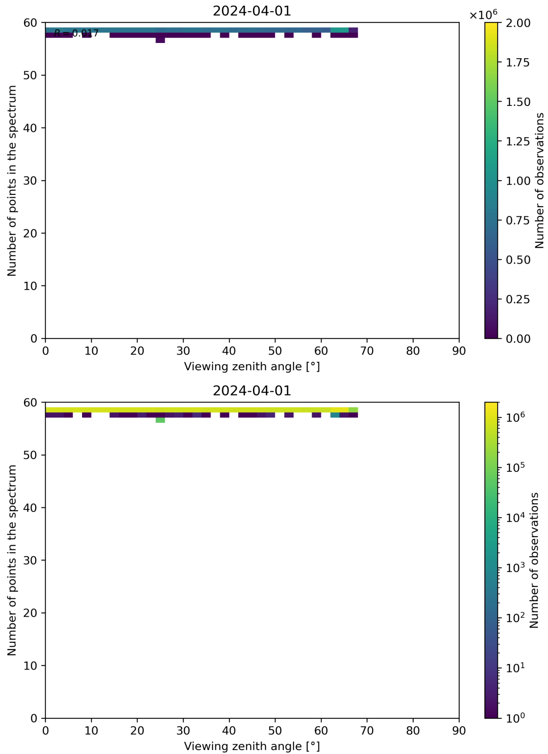
Figure 125: Scatter density plot of “Viewing zenith angle” against “Number of points in the spectrum” for 2024-03-31 to 2024-04-02.
