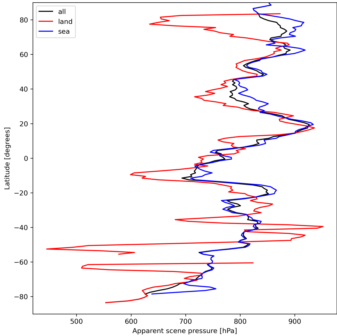
Figure 19: Zonal average of “Apparent scene pressure” for 2024-03-31 to 2024-04-02.
