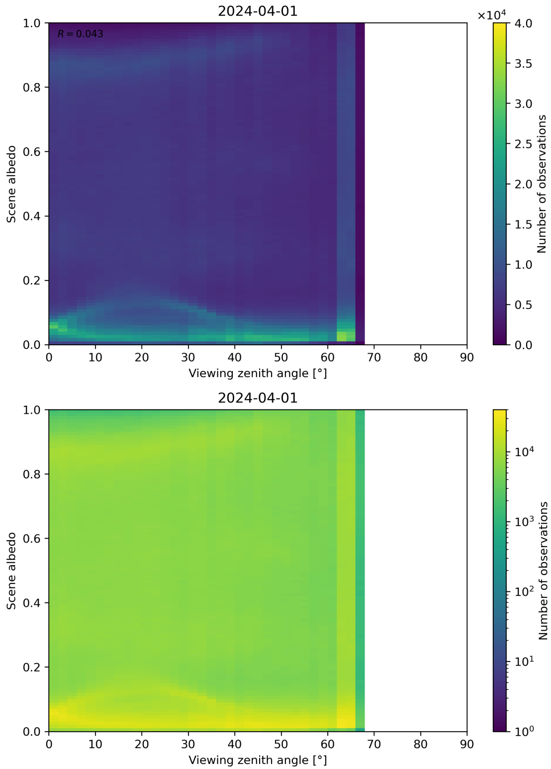
Figure 126: Scatter density plot of “Viewing zenith angle” against “Scene albedo” for 2024-03-31 to 2024-04-02.
