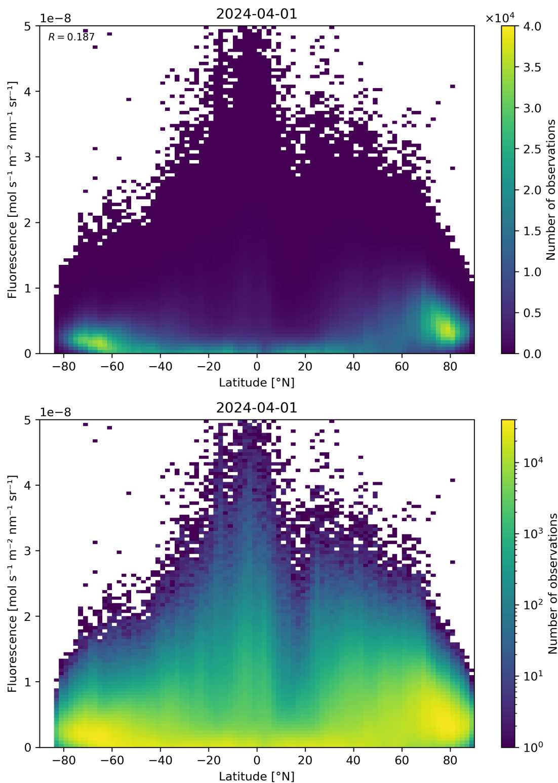
Figure 92: Scatter density plot of “Latitude” against “Fluorescence” for 2024-03-31 to 2024-04-02.
