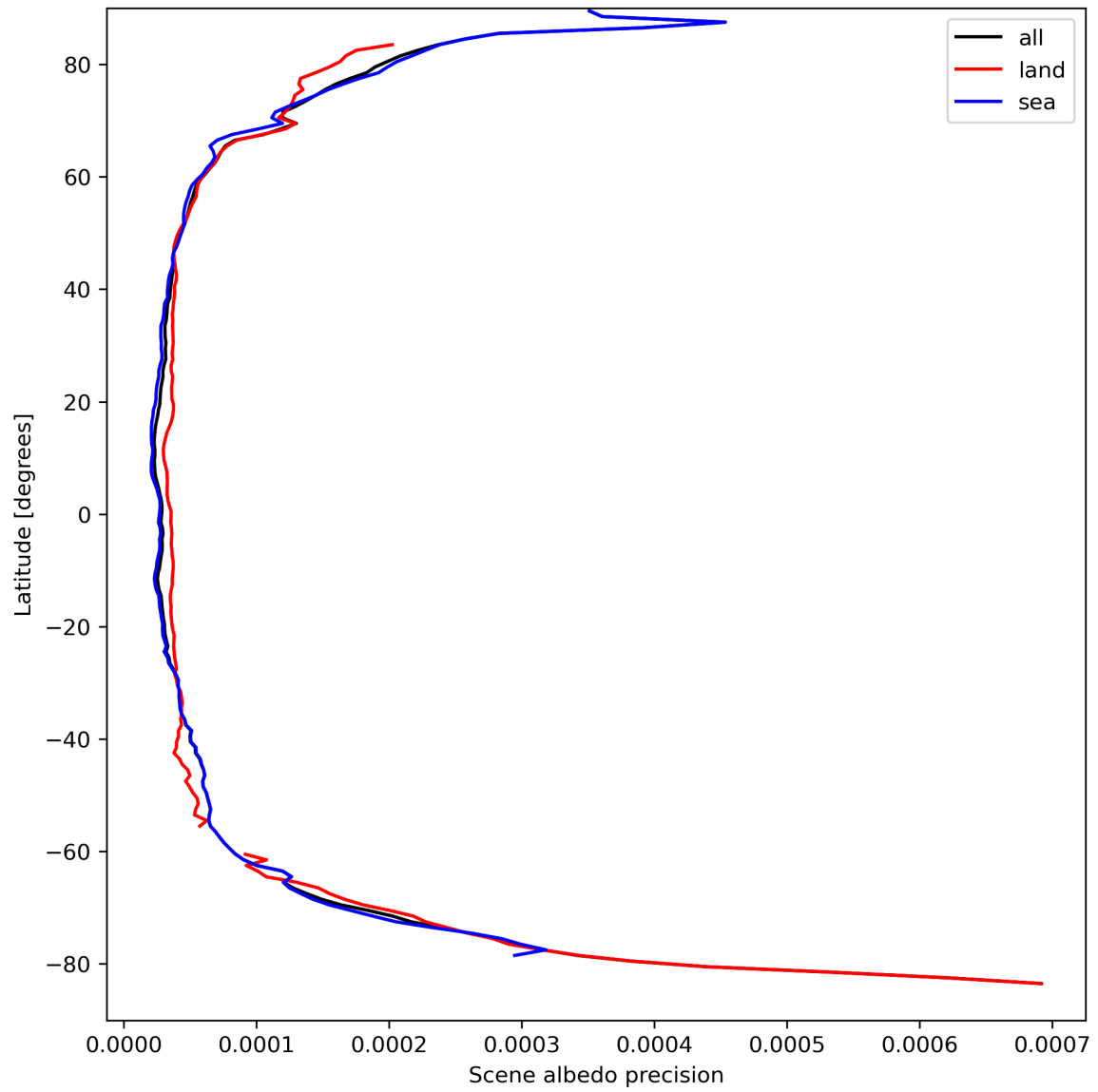
Figure 18: Zonal average of “Scene albedo precision” for 2024-03-31 to 2024-04-02.
