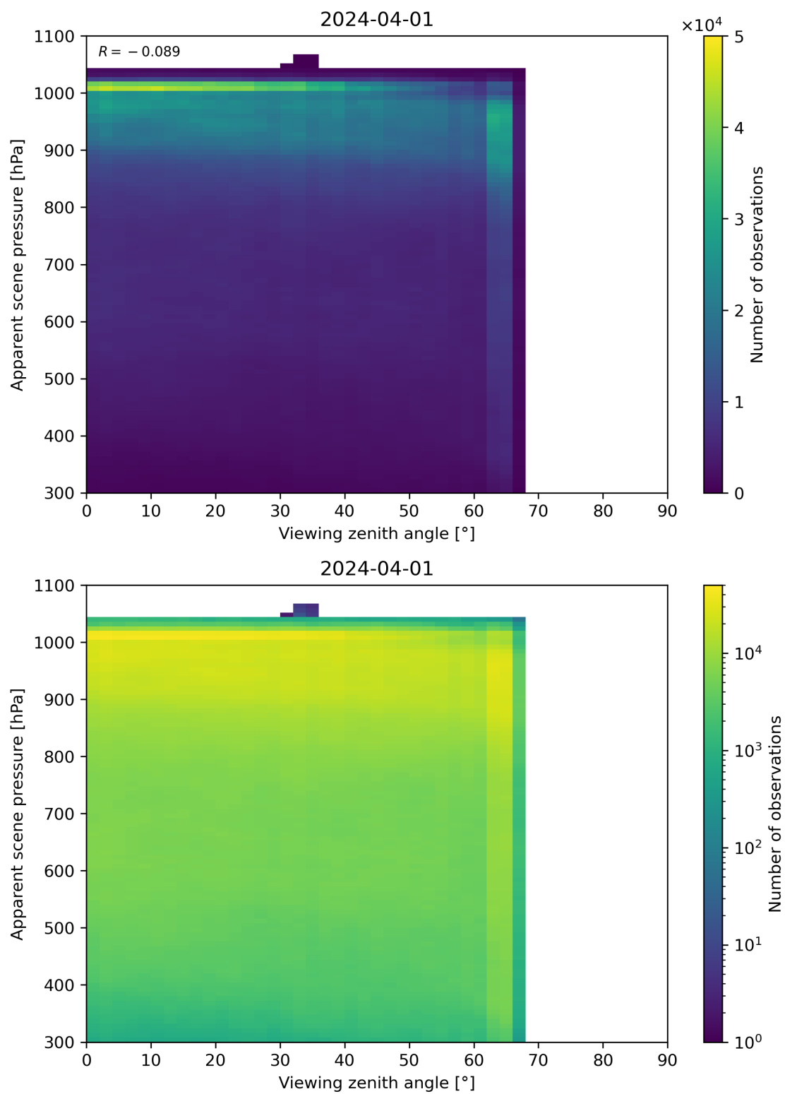
Figure 118: Scatter density plot of “Viewing zenith angle” against “Apparent scene pressure” for 2024-03-31 to 2024-04-02.
