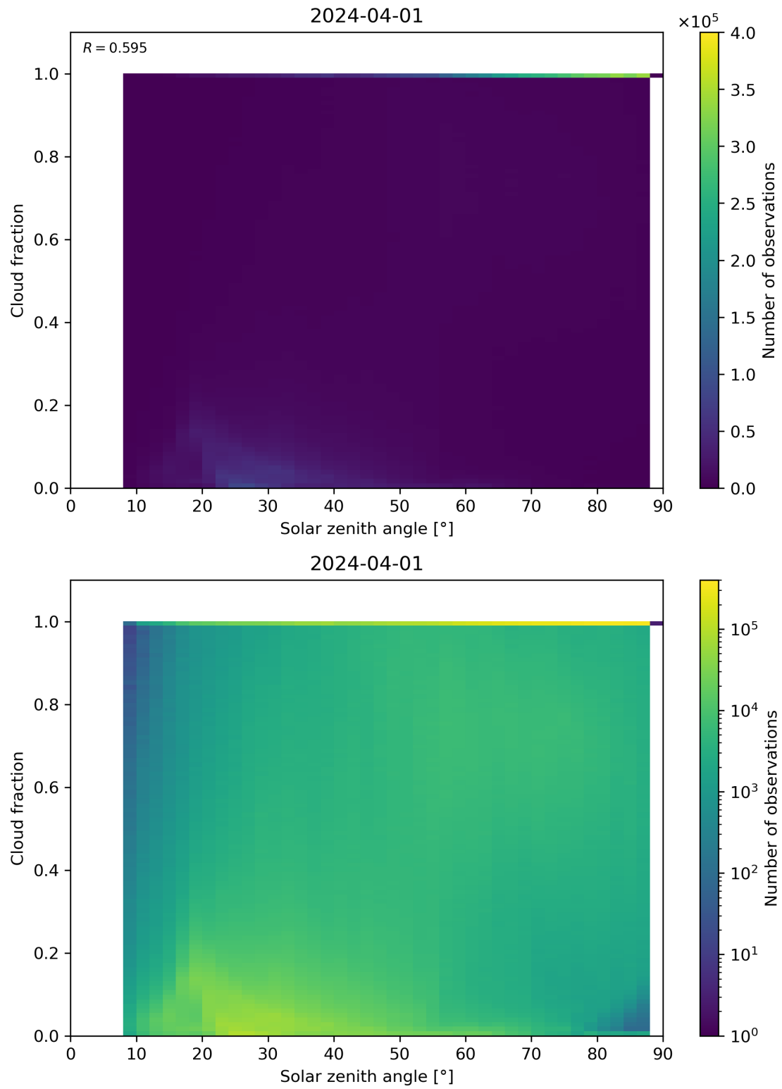
Figure 110: Scatter density plot of “Solar zenith angle” against “Cloud fraction” for 2024-03-31 to 2024-04-02.
