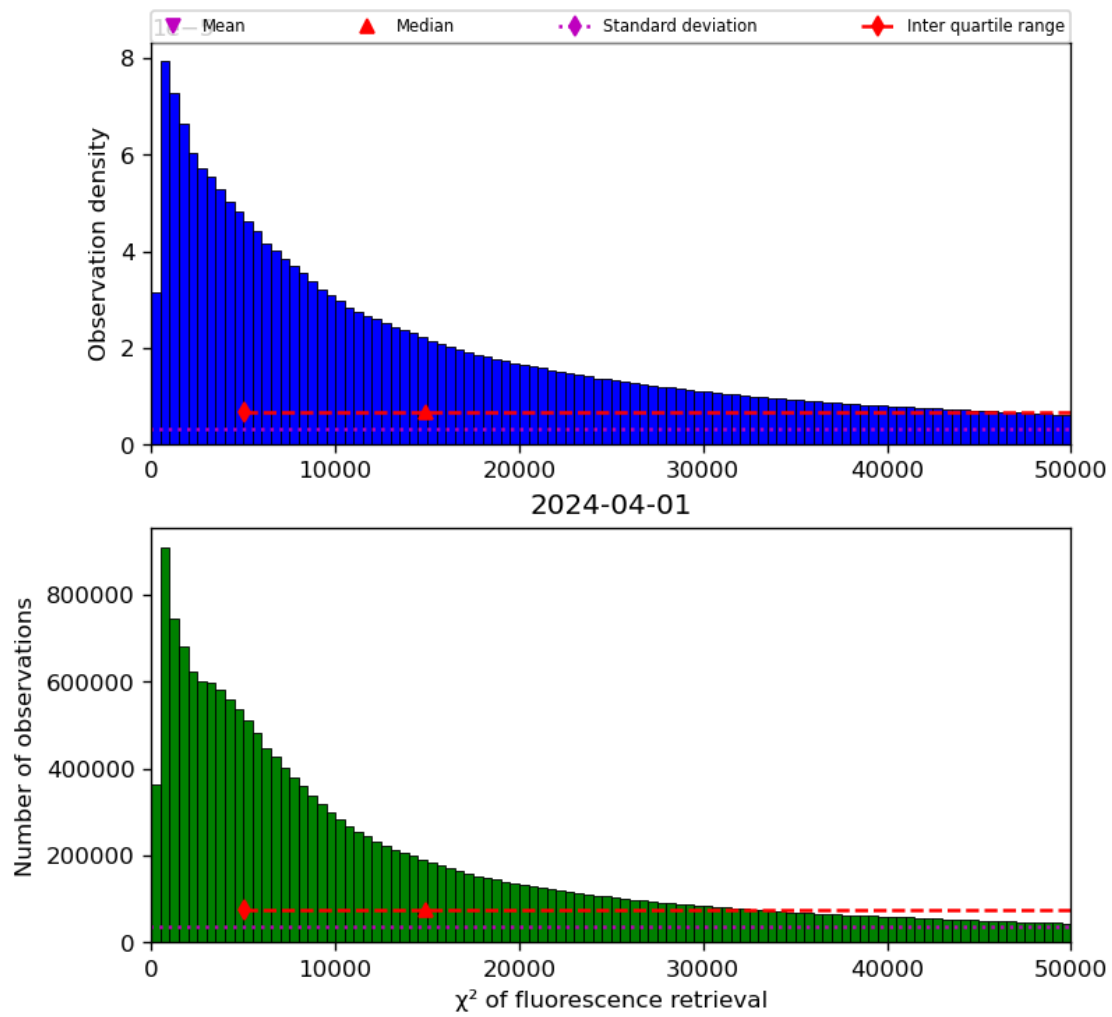
Figure 42: Histogram of “ \chi^2 of fluorescence retrieval” for 2024-03-31 to 2024-04-02
