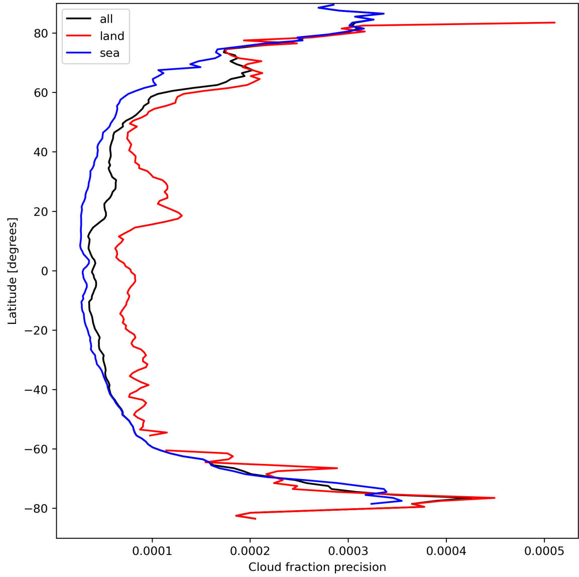
Figure 16: Zonal average of “Cloud fraction precision” for 2024-03-31 to 2024-04-02.
