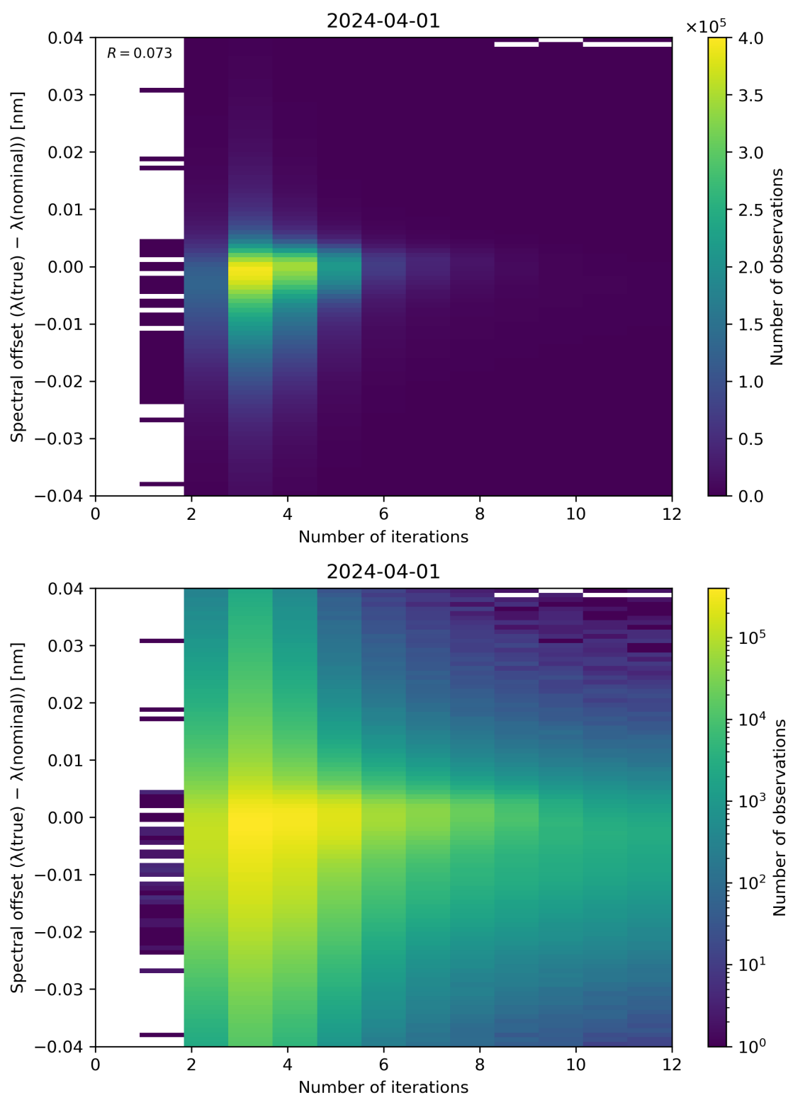
Figure 100: Scatter density plot of “Number of iterations” against “Spectral offset ( \lambda(\text{true}) - \lambda(\text{nominal}) )” for 2024-03-31 to 2024-04-02.
