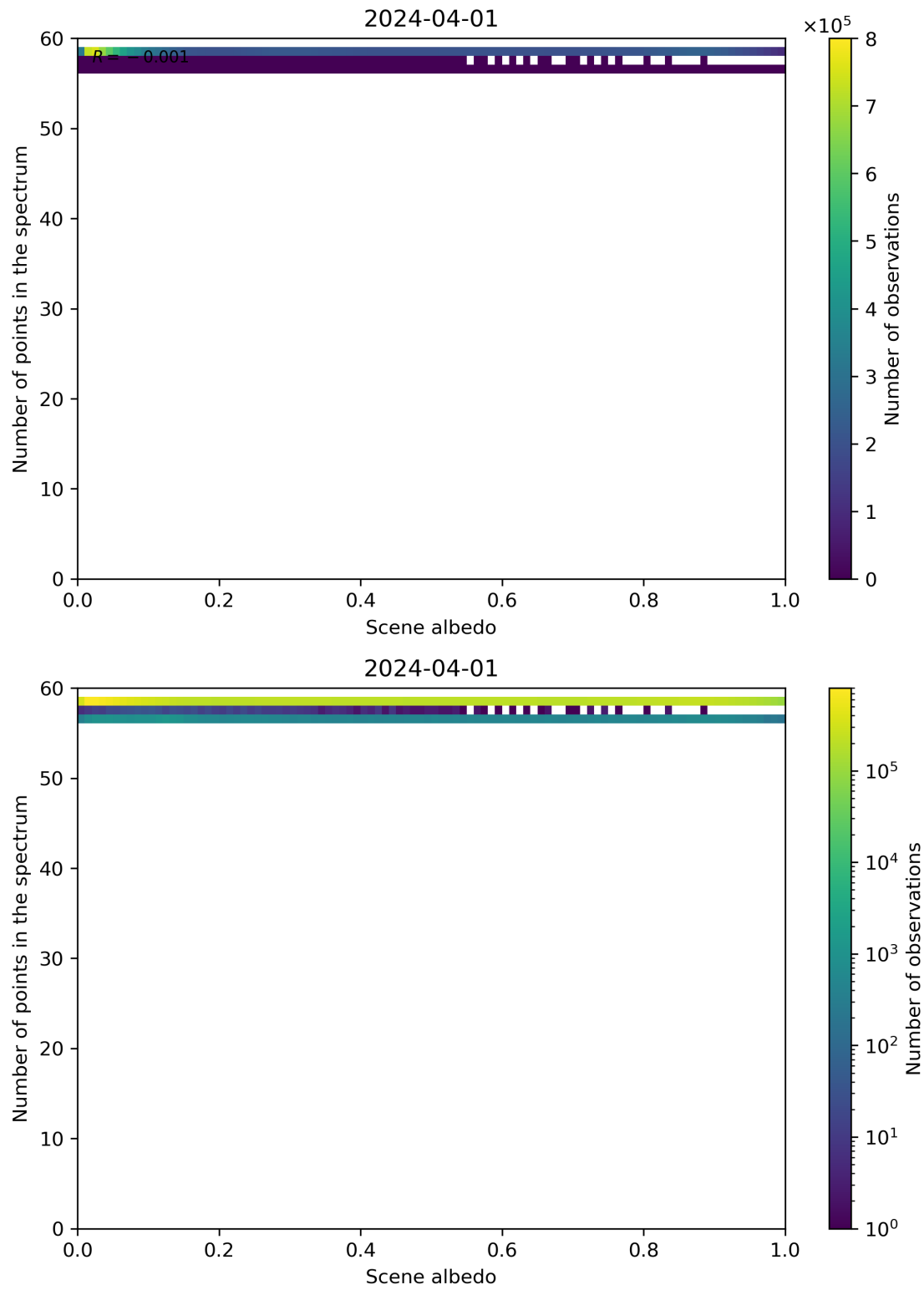
Figure 106: Scatter density plot of “Scene albedo” against “Number of points in the spectrum” for 2024-03-31 to 2024-04-02.
