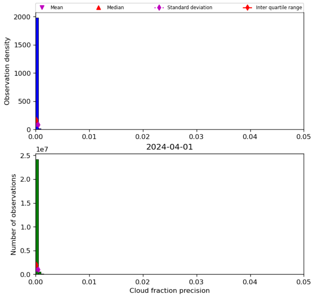
Figure 33: Histogram of “Cloud fraction precision” for 2024-03-31 to 2024-04-02
