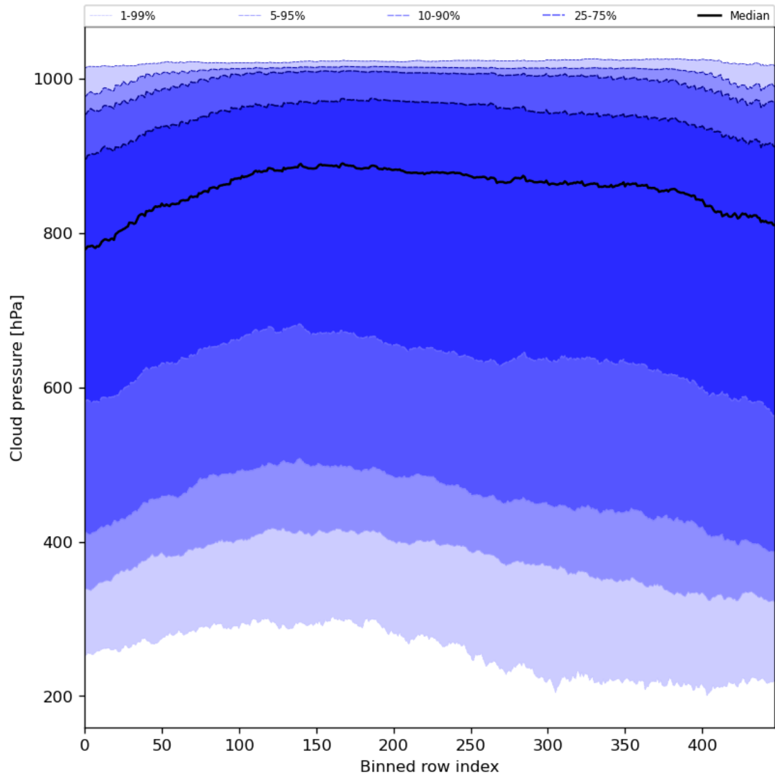
Figure 47: Along track statistics of “Cloud pressure” for 2024-03-31 to 2024-04-02
