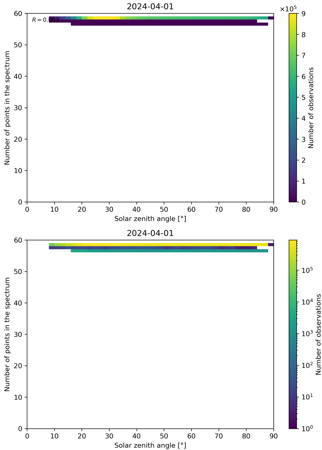
Figure 115: Scatter density plot of “Solar zenith angle” against “Number of points in the spectrum” for 2024-03-31 to 2024-04-02.
