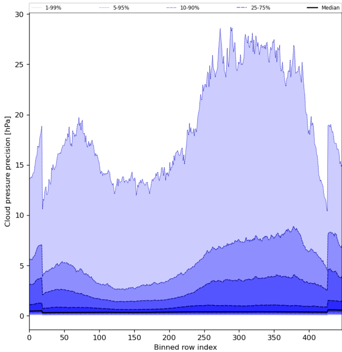
Figure 48: Along track statistics of “Cloud pressure precision” for 2024-03-31 to 2024-04-02
