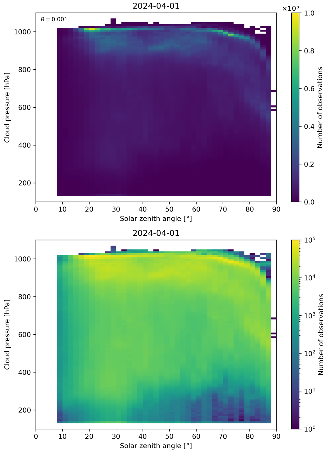
Figure 111: Scatter density plot of “Solar zenith angle” against “Cloud pressure” for 2024-03-31 to 2024-04-02.
