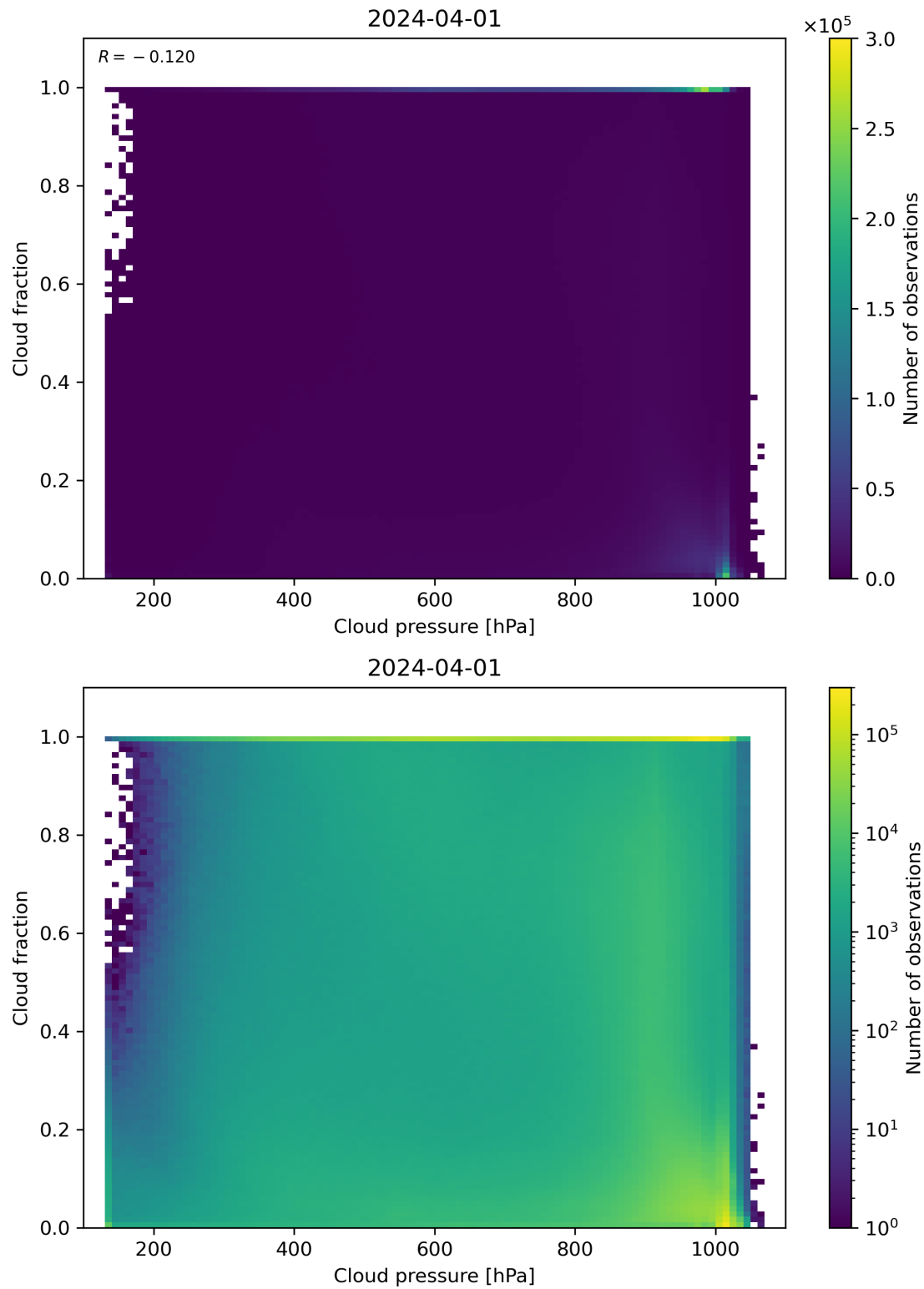
Figure 79: Scatter density plot of “Cloud pressure” against “Cloud fraction” for 2024-03-31 to 2024-04-02.
