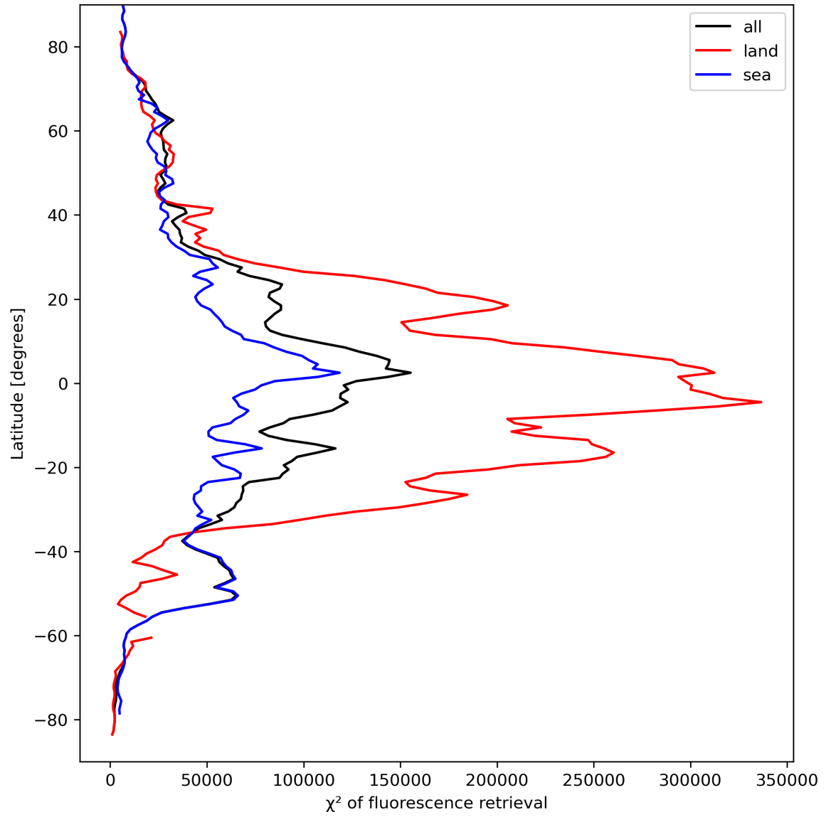
Figure 25: Zonal average of “ \chi^2 of fluorescence retrieval” for 2024-03-31 to 2024-04-02.
