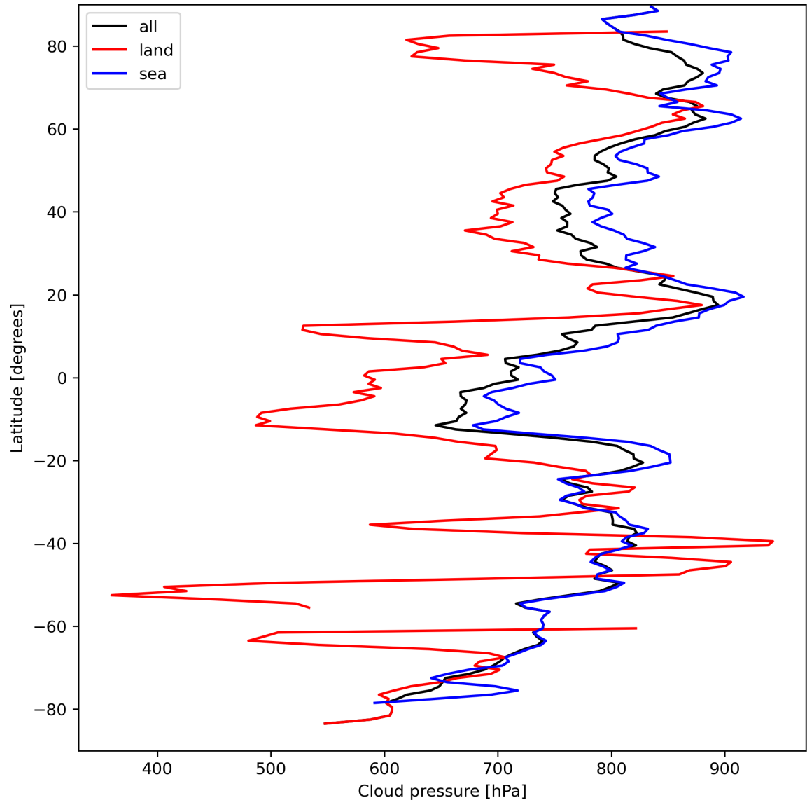
Figure 13: Zonal average of “Cloud pressure” for 2024-03-31 to 2024-04-02.
