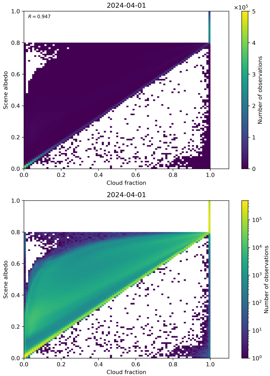
Figure 75: Scatter density plot of “Cloud fraction” against “Scene albedo” for 2024-03-31 to 2024-04-02.
