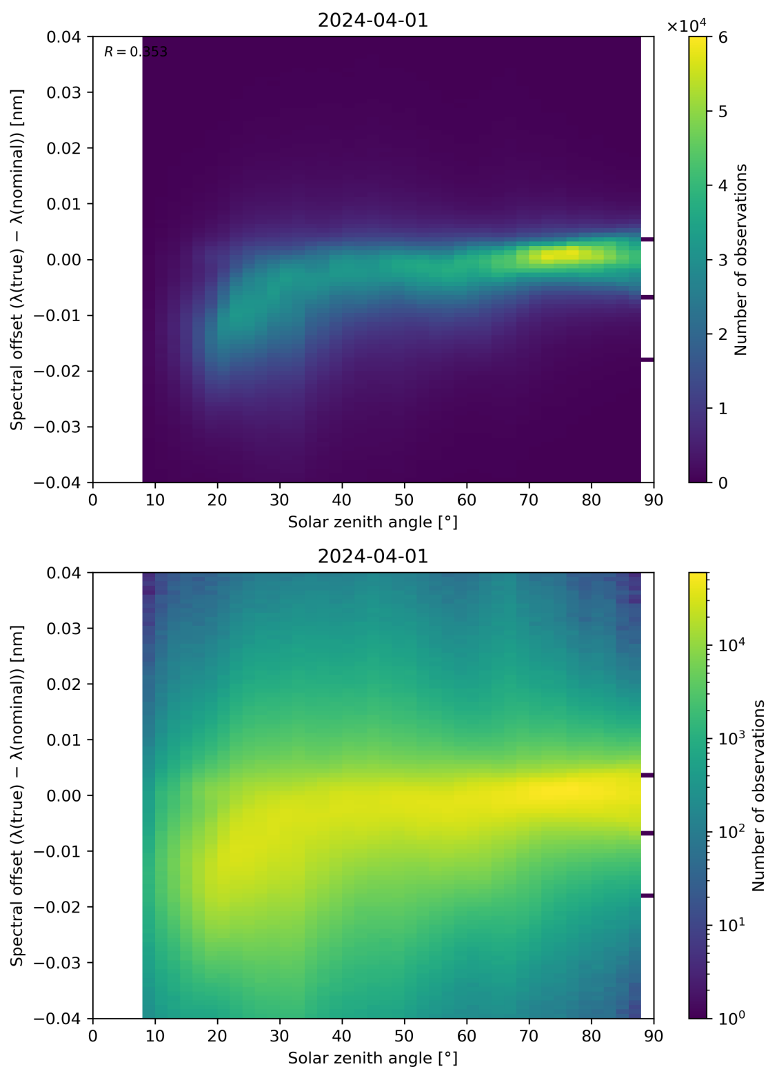
Figure 117: Scatter density plot of “Solar zenith angle” against “Spectral offset ( \lambda(\text{true}) - \lambda(\text{nominal}) )” for 2024-03-31 to 2024-04-02.
