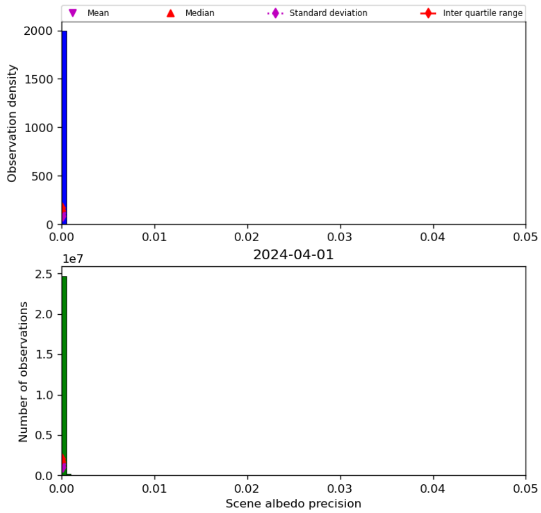
Figure 35: Histogram of “Scene albedo precision” for 2024-03-31 to 2024-04-02
