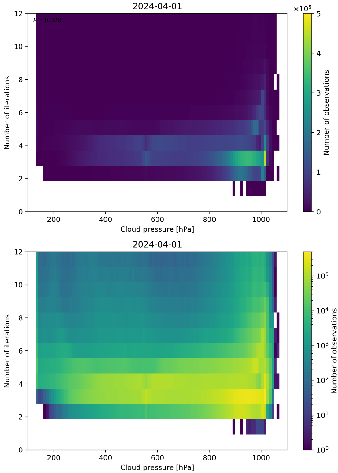
Figure 81: Scatter density plot of “Cloud pressure” against “Number of iterations” for 2024-03-31 to 2024-04-02.
