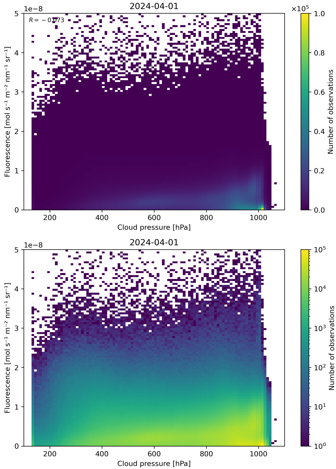
Figure 80: Scatter density plot of “Cloud pressure” against “Fluorescence” for 2024-03-31 to 2024-04-02.
