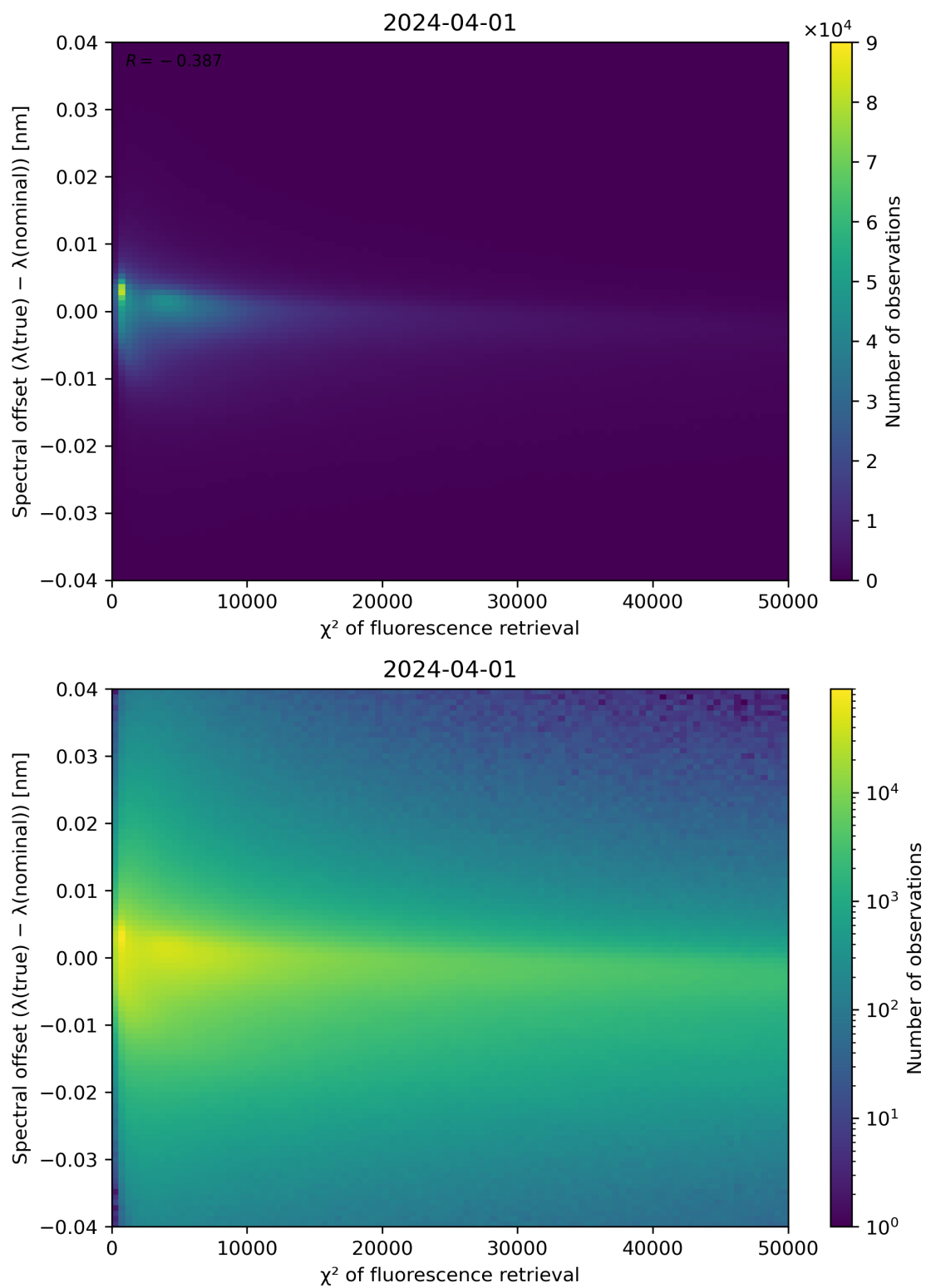
Figure 69: Scatter density plot of " \chi^2 of fluorescence retrieval" against "Spectral offset ( \lambda(\text{true}) - \lambda(\text{nominal}) )" for 2024-03-31 to 2024-04-02.
