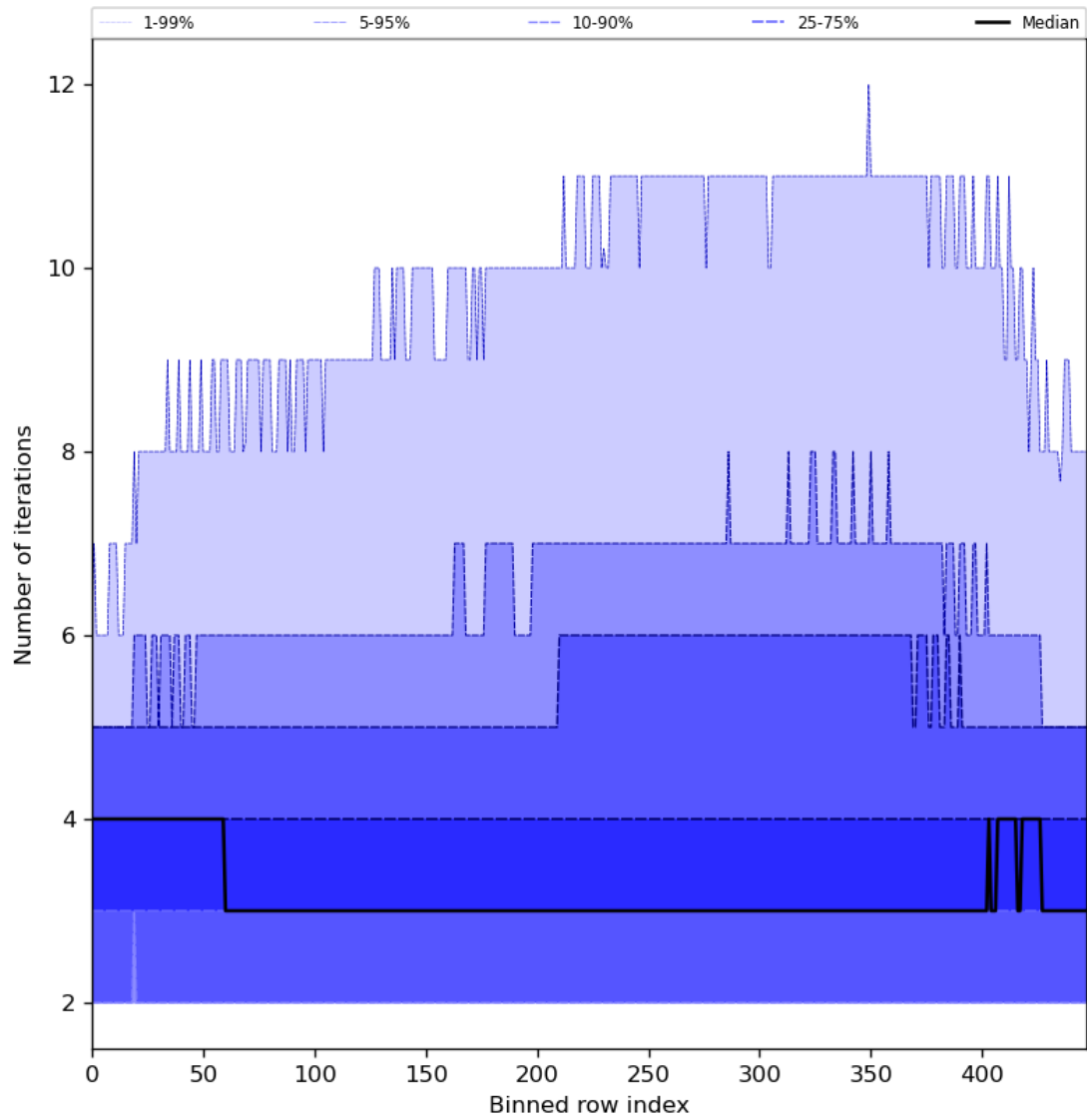
Figure 56: Along track statistics of “Number of iterations” for 2024-03-31 to 2024-04-02
