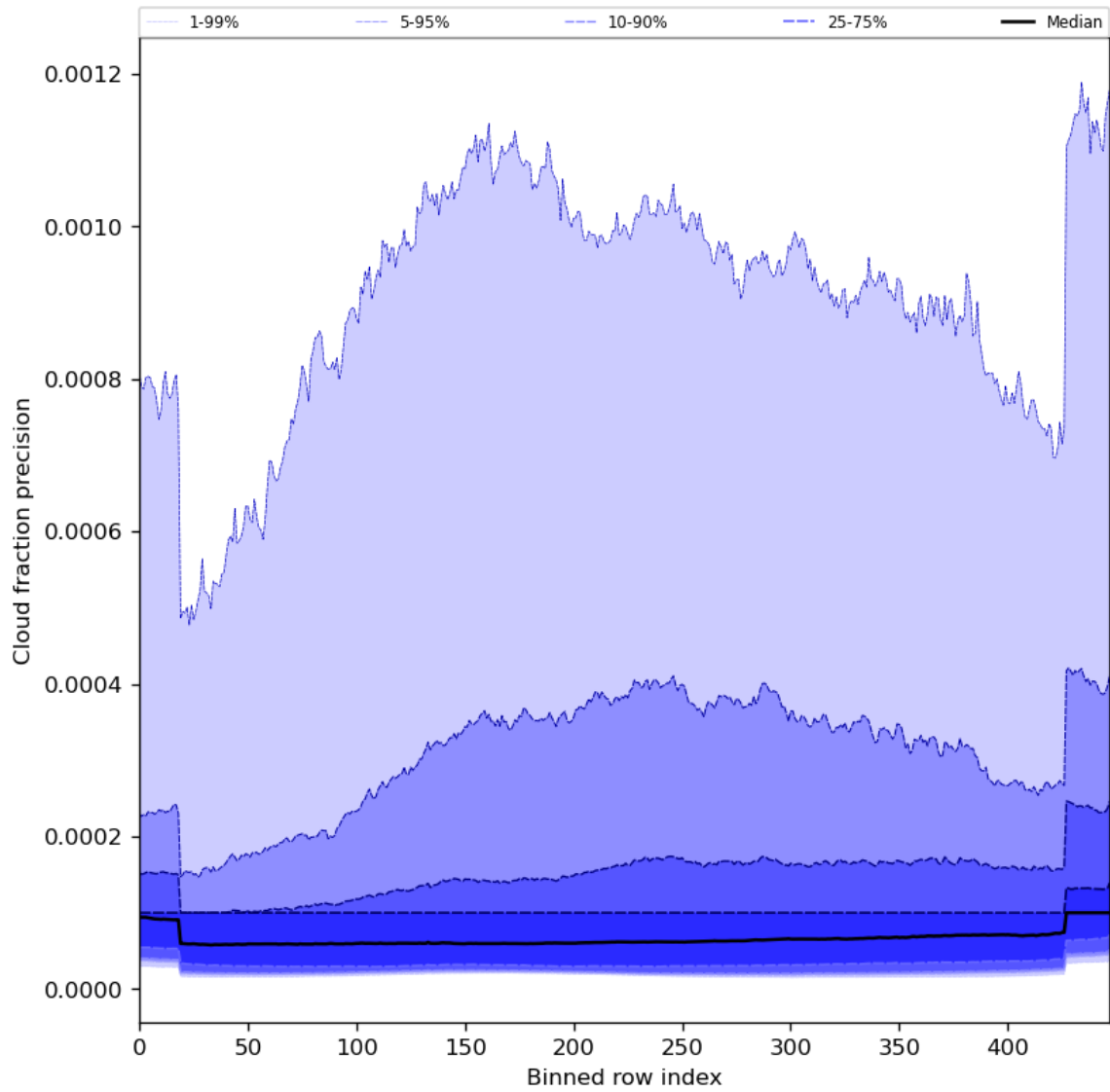
Figure 50: Along track statistics of “Cloud fraction precision” for 2024-03-31 to 2024-04-02
