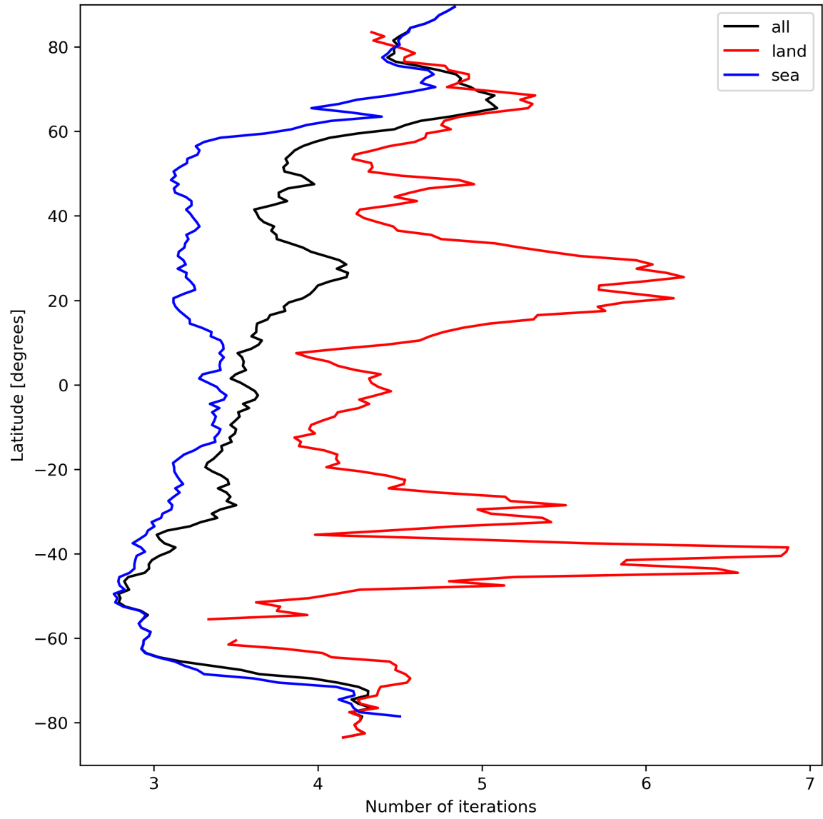
Figure 22: Zonal average of “Number of iterations” for 2024-03-31 to 2024-04-02.
