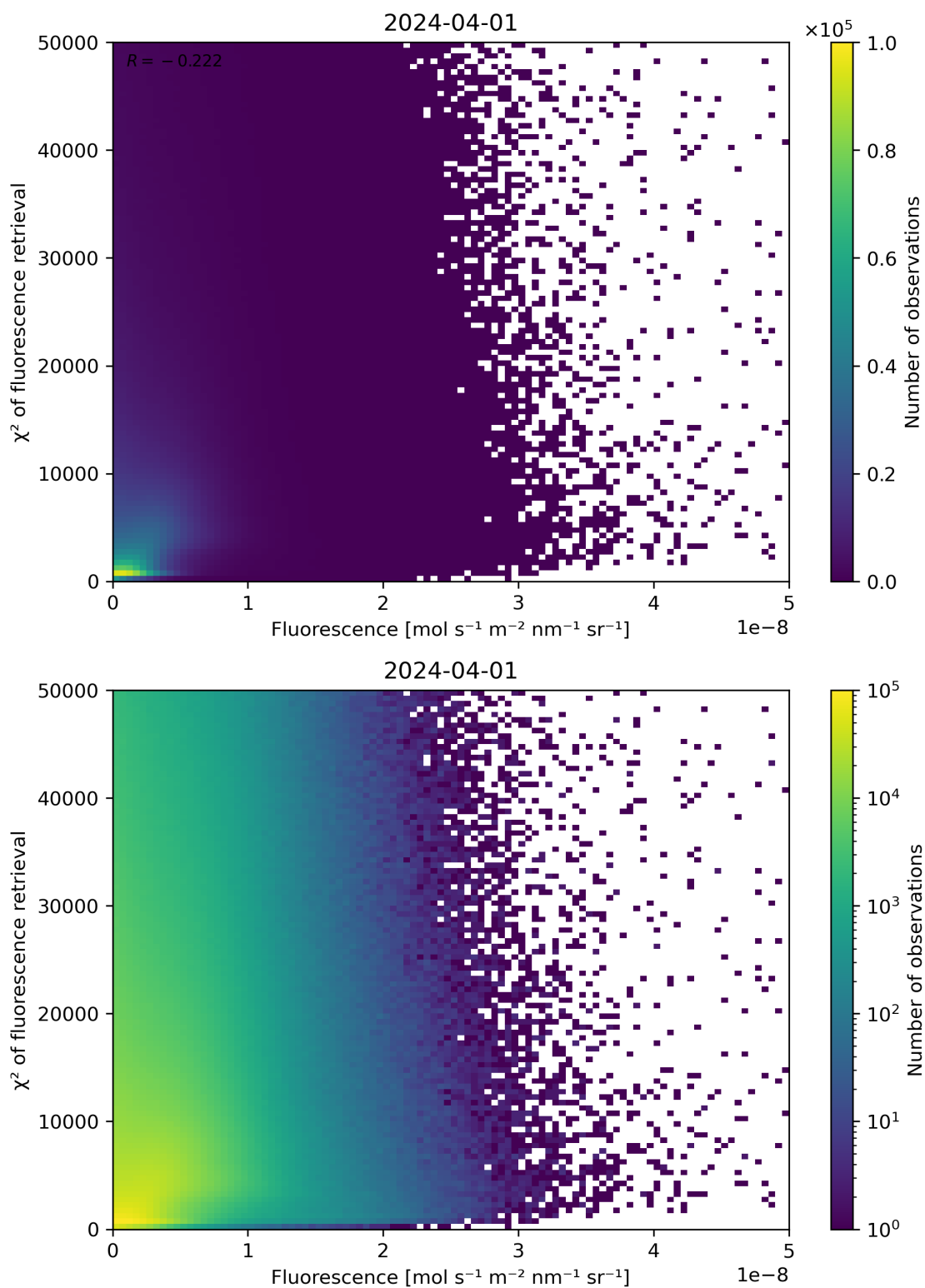
Figure 85: Scatter density plot of “Fluorescence” against “ \chi^2 of fluorescence retrieval” for 2024-03-31 to 2024-04-02.
