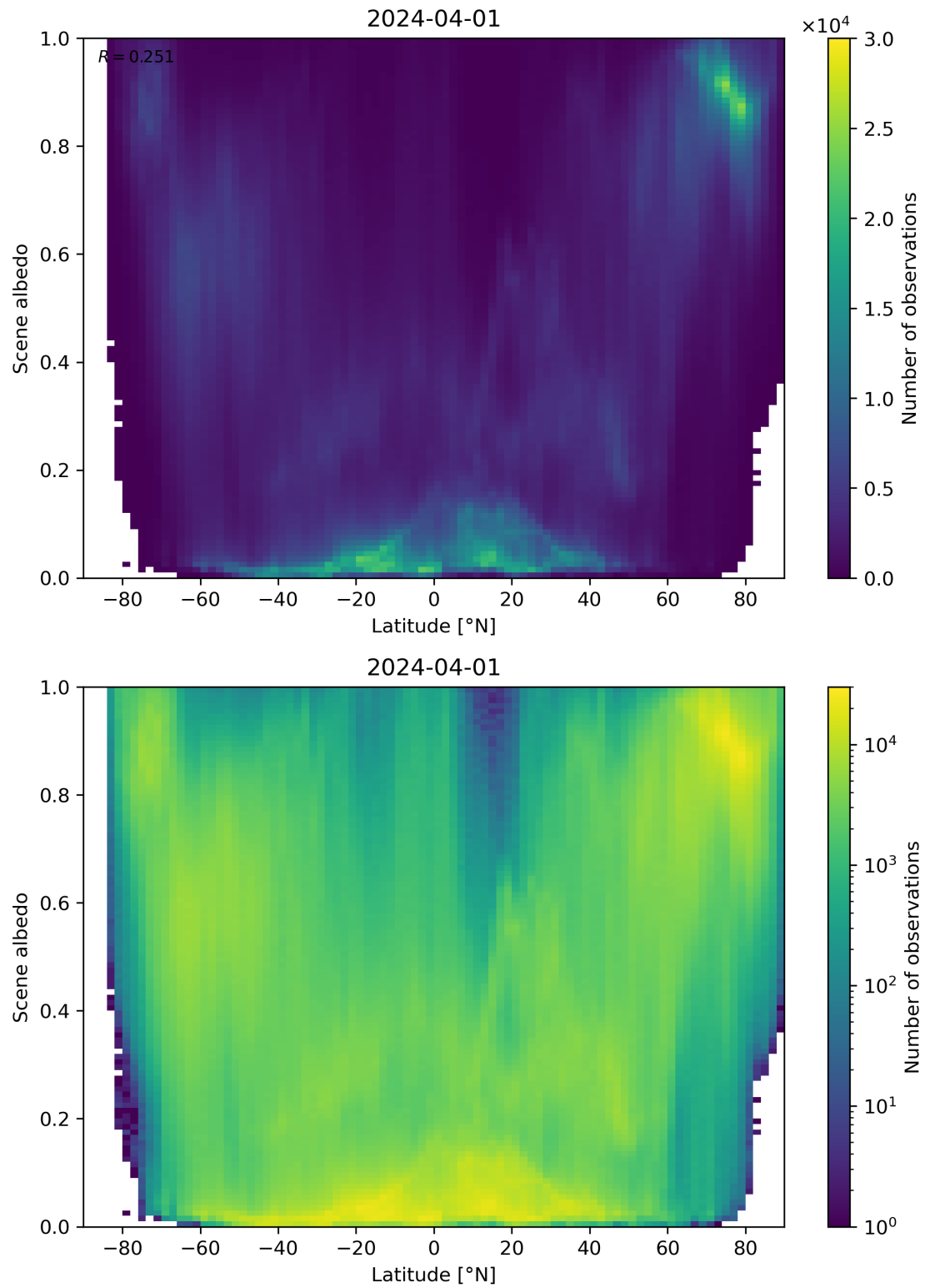
Figure 95: Scatter density plot of “Latitude” against “Scene albedo” for 2024-03-31 to 2024-04-02.
