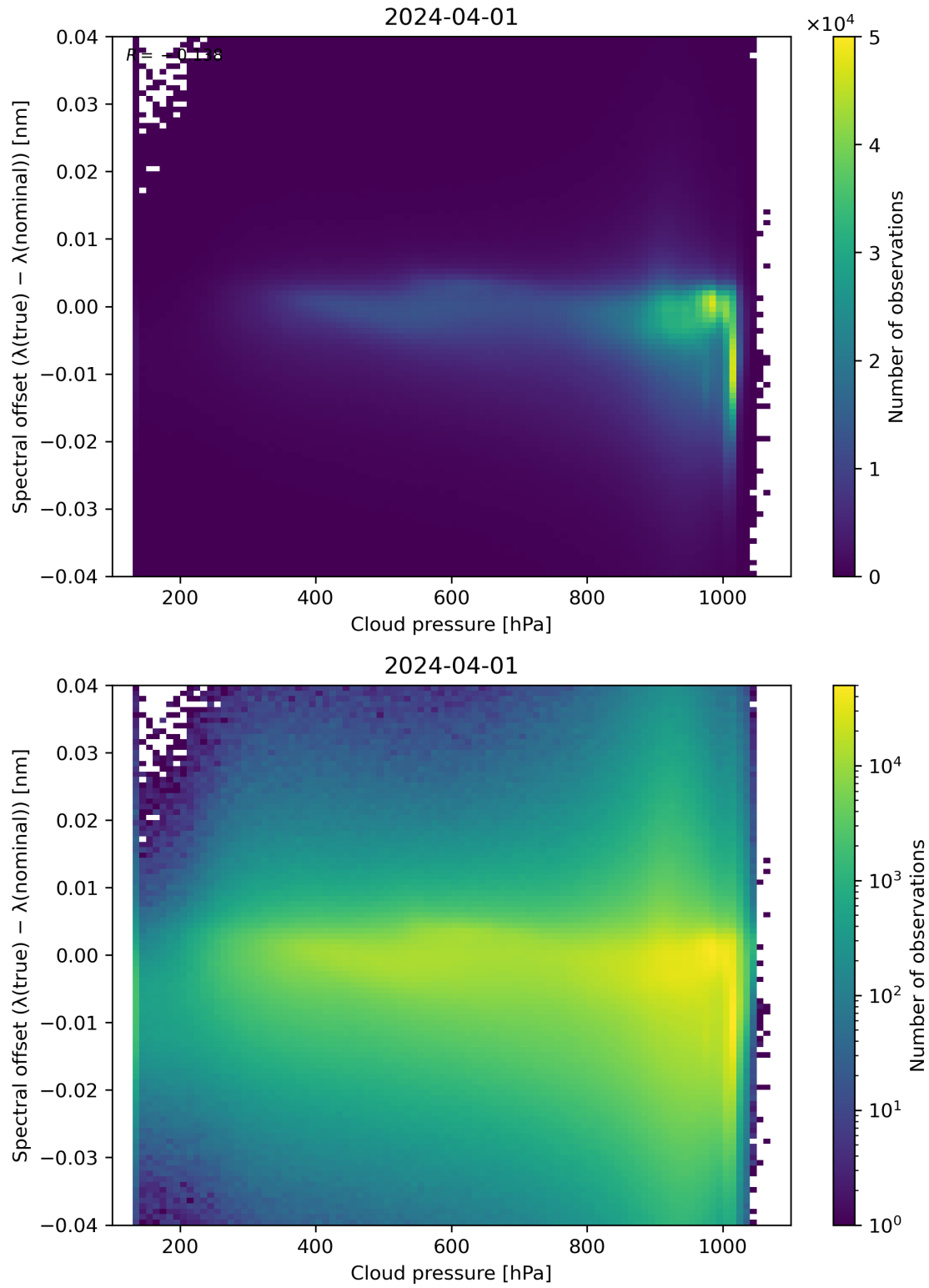
Figure 84: Scatter density plot of “Cloud pressure” against “Spectral offset ( \lambda(\text{true}) - \lambda(\text{nominal}) )” for 2024-03-31 to 2024-04-02.
