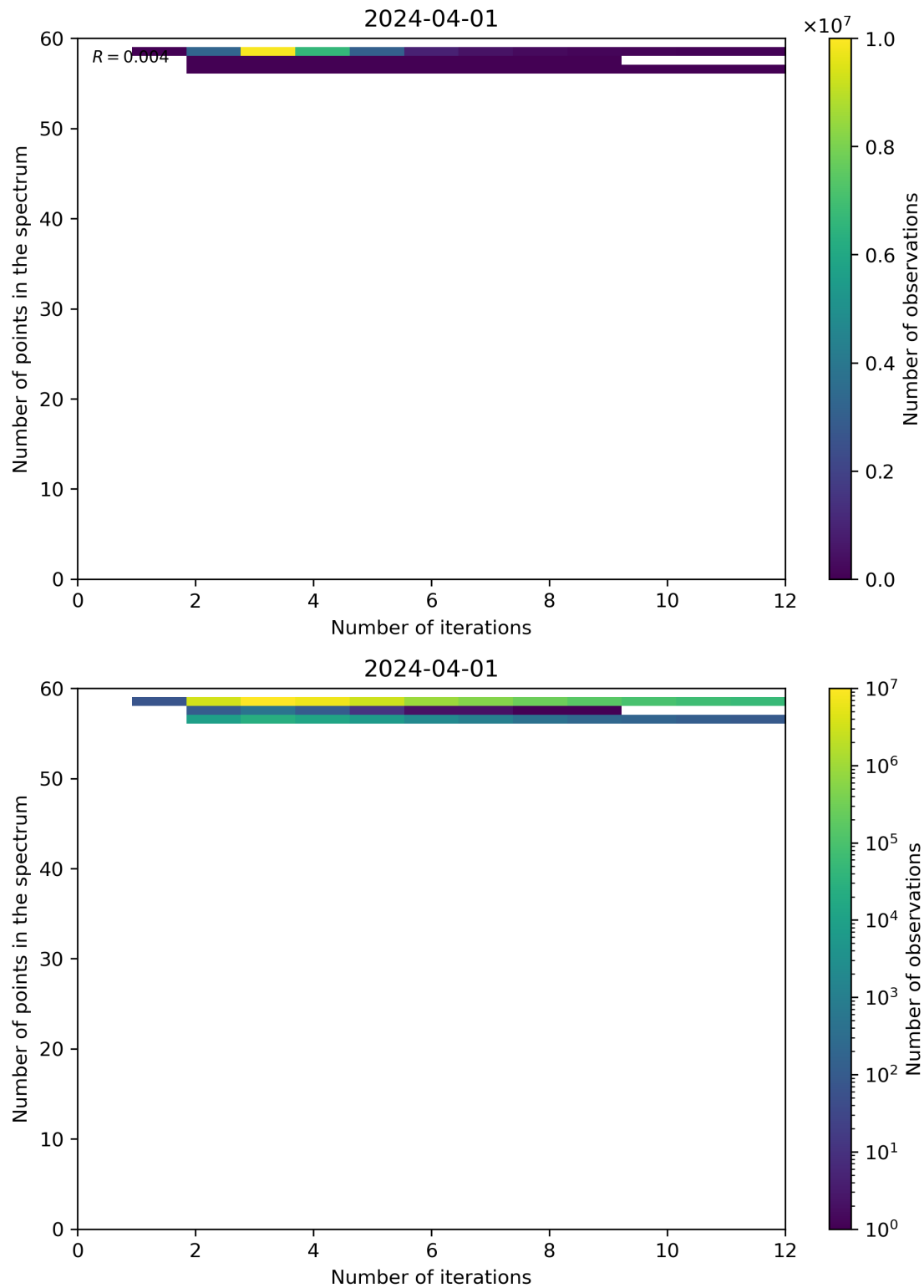
Figure 99: Scatter density plot of “Number of iterations” against “Number of points in the spectrum” for 2024-03-31 to 2024-04-02.
