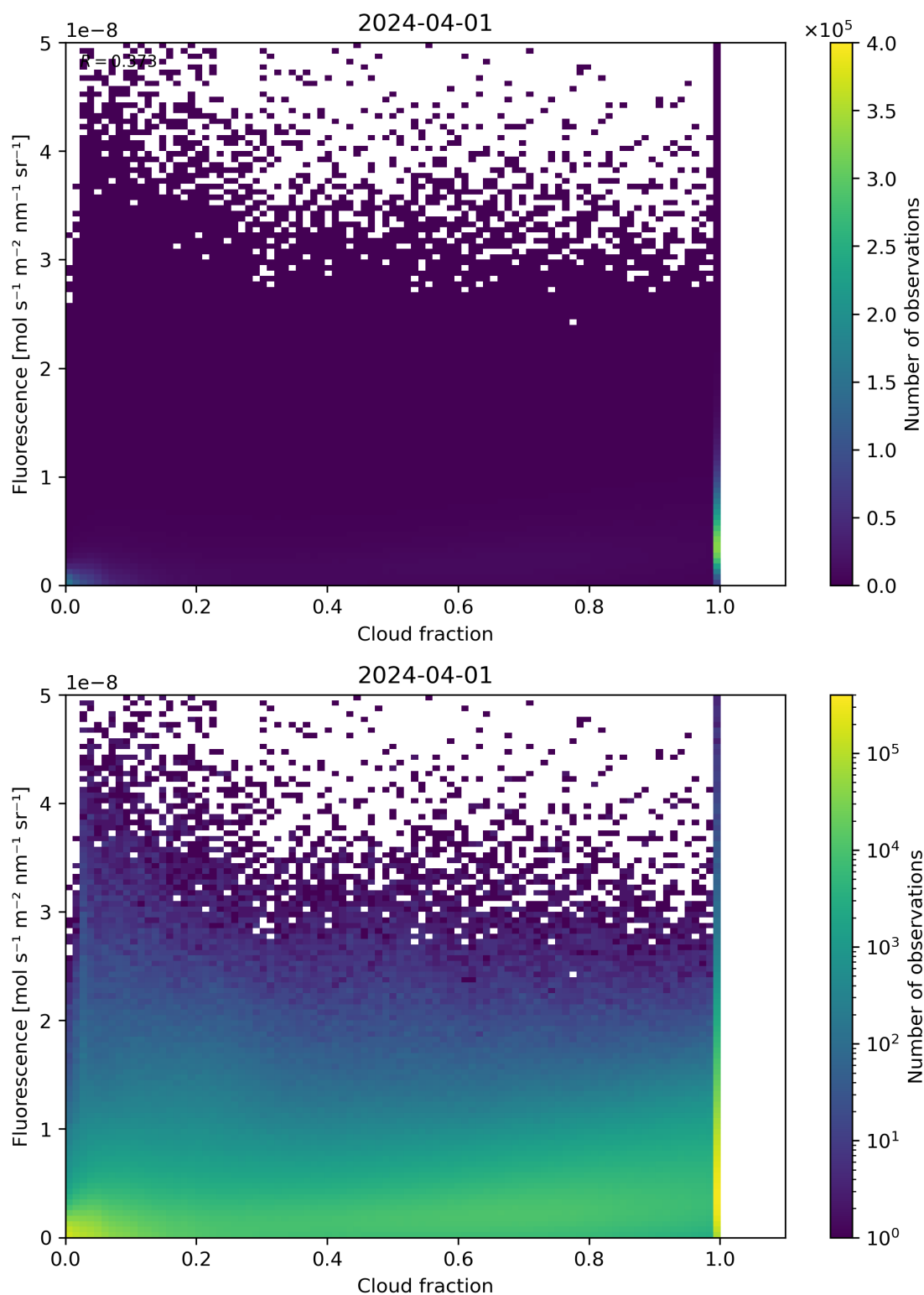
Figure 72: Scatter density plot of “Cloud fraction” against “Fluorescence” for 2024-03-31 to 2024-04-02.
