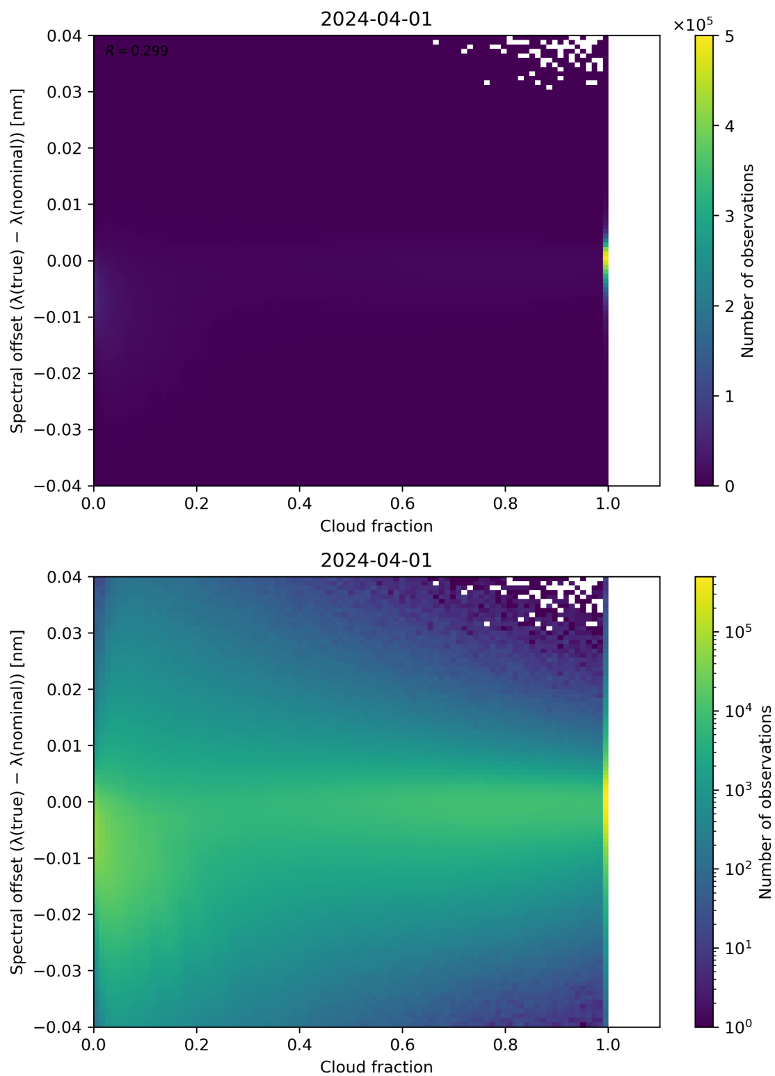
Figure 76: Scatter density plot of “Cloud fraction” against “Spectral offset ( \lambda(\text{true}) - \lambda(\text{nominal}) )” for 2024-03-31 to 2024-04-02.
