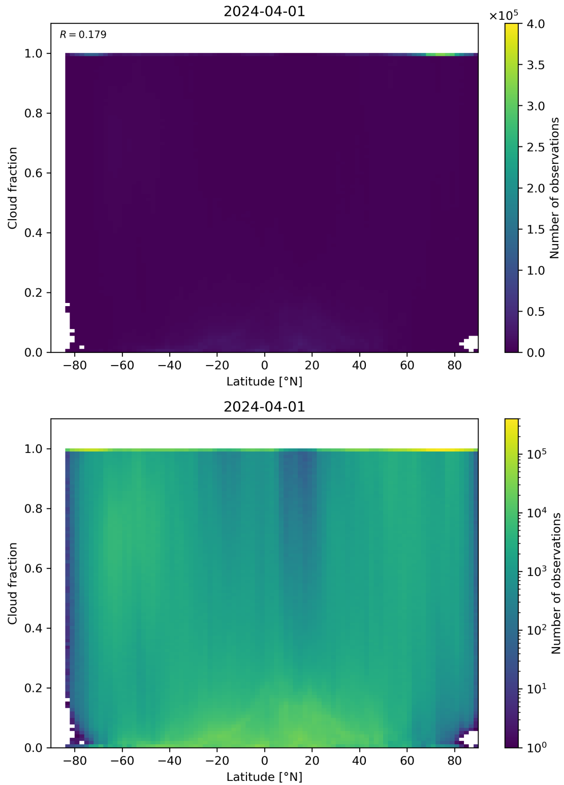
Figure 90: Scatter density plot of “Latitude” against “Cloud fraction” for 2024-03-31 to 2024-04-02.
