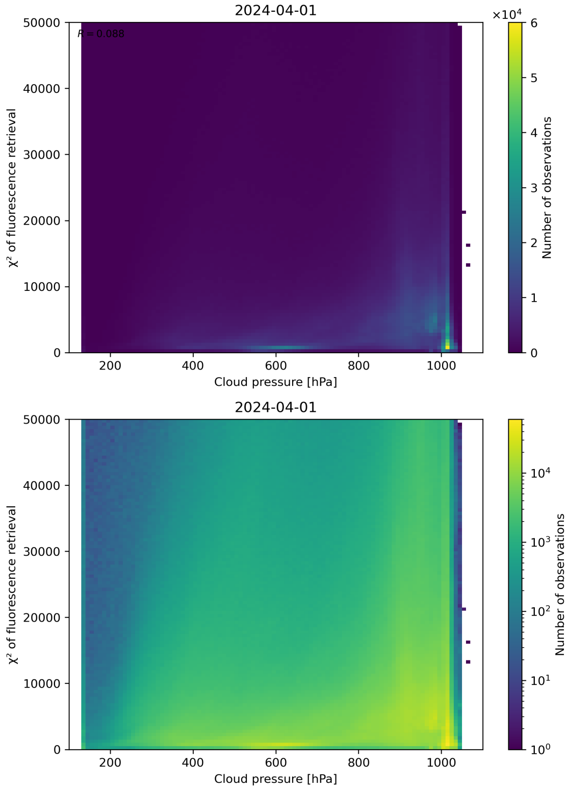
Figure 78: Scatter density plot of “Cloud pressure” against “ \chi^2 of fluorescence retrieval” for 2024-03-31 to 2024-04-02.
