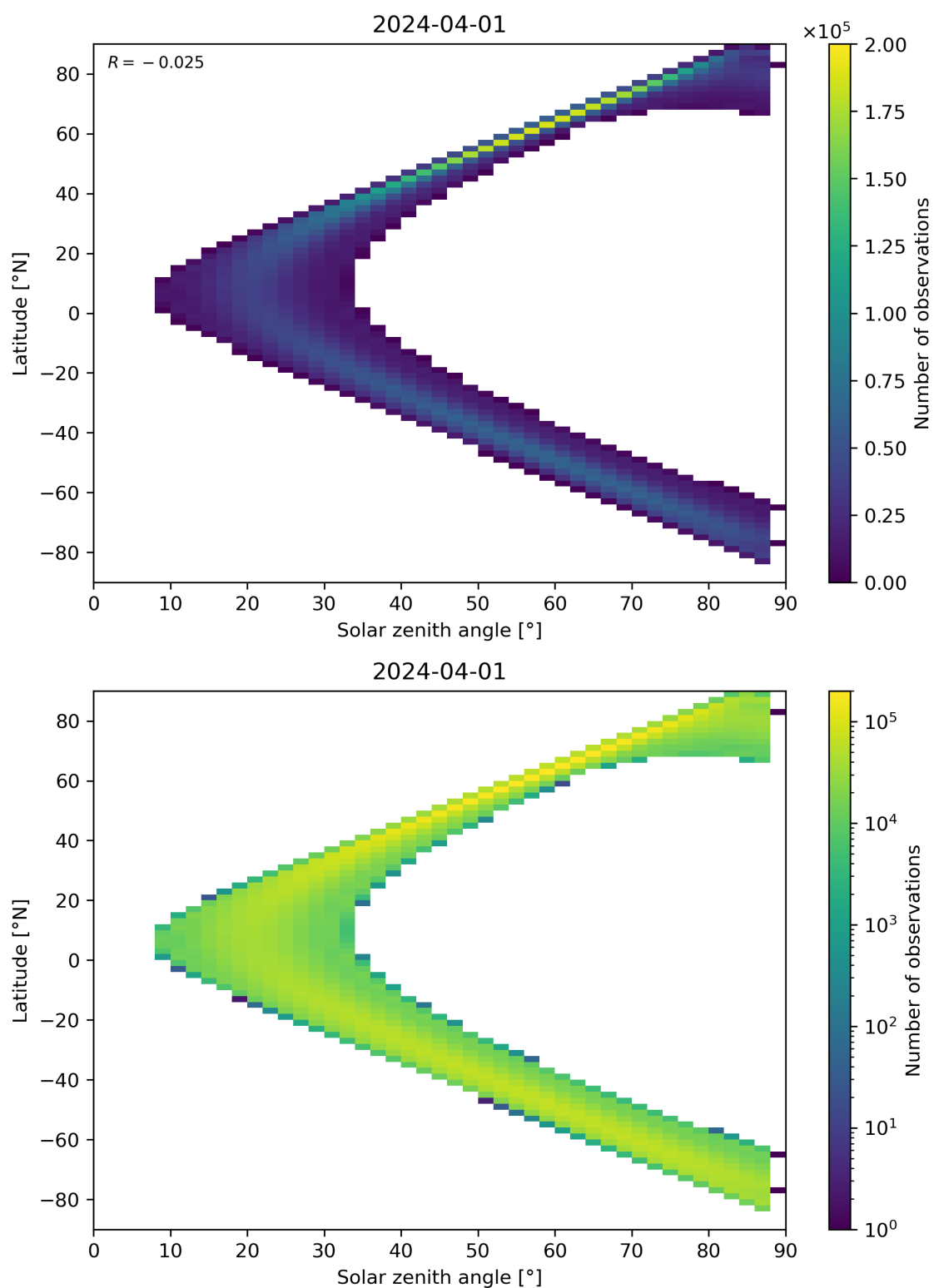
Figure 113: Scatter density plot of “Solar zenith angle” against “Latitude” for 2024-03-31 to 2024-04-02.
