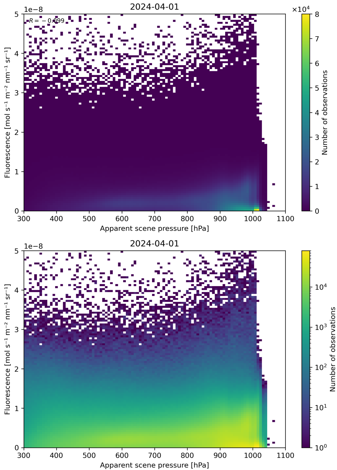
Figure 64: Scatter density plot of “Apparent scene pressure” against “Fluorescence” for 2024-03-31 to 2024-04-02.
