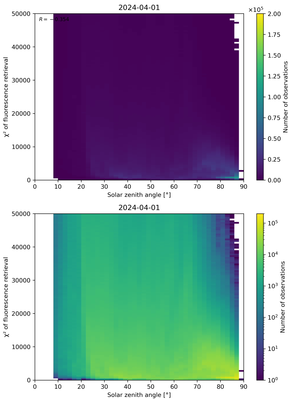
Figure 109: Scatter density plot of “Solar zenith angle” against “ \chi^2 of fluorescence retrieval” for 2024-03-31 to 2024-04-02.
