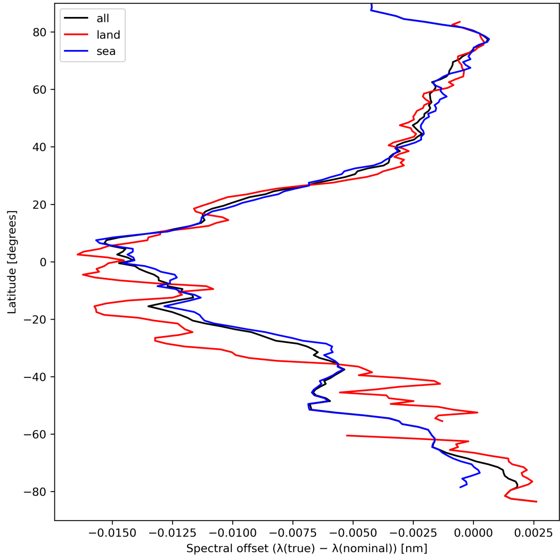
Figure 28: Zonal average of “Spectral offset ( \lambda(\text{true}) - \lambda(\text{nominal}) )” for 2024-03-31 to 2024-04-02.
