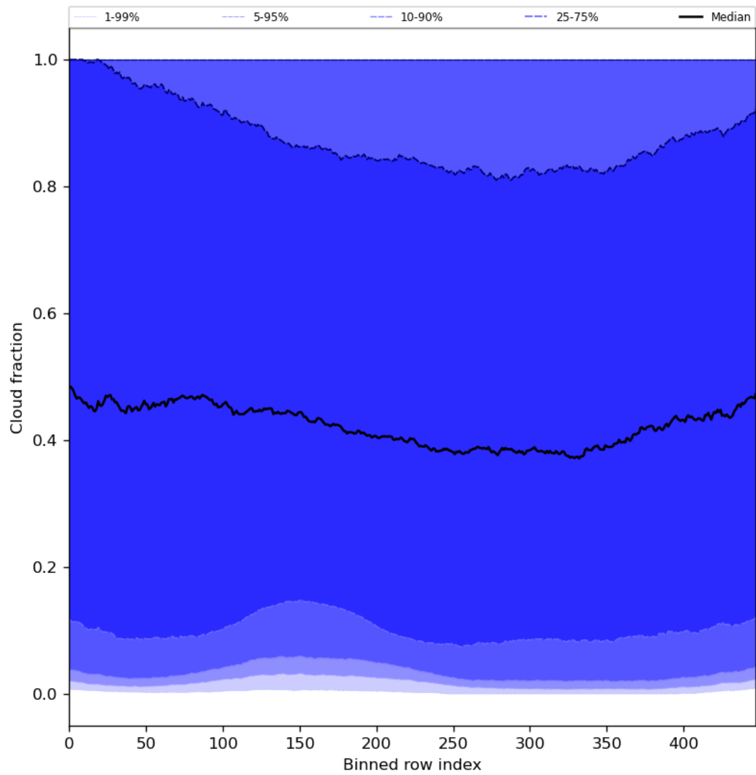
Figure 49: Along track statistics of “Cloud fraction” for 2024-03-31 to 2024-04-02
