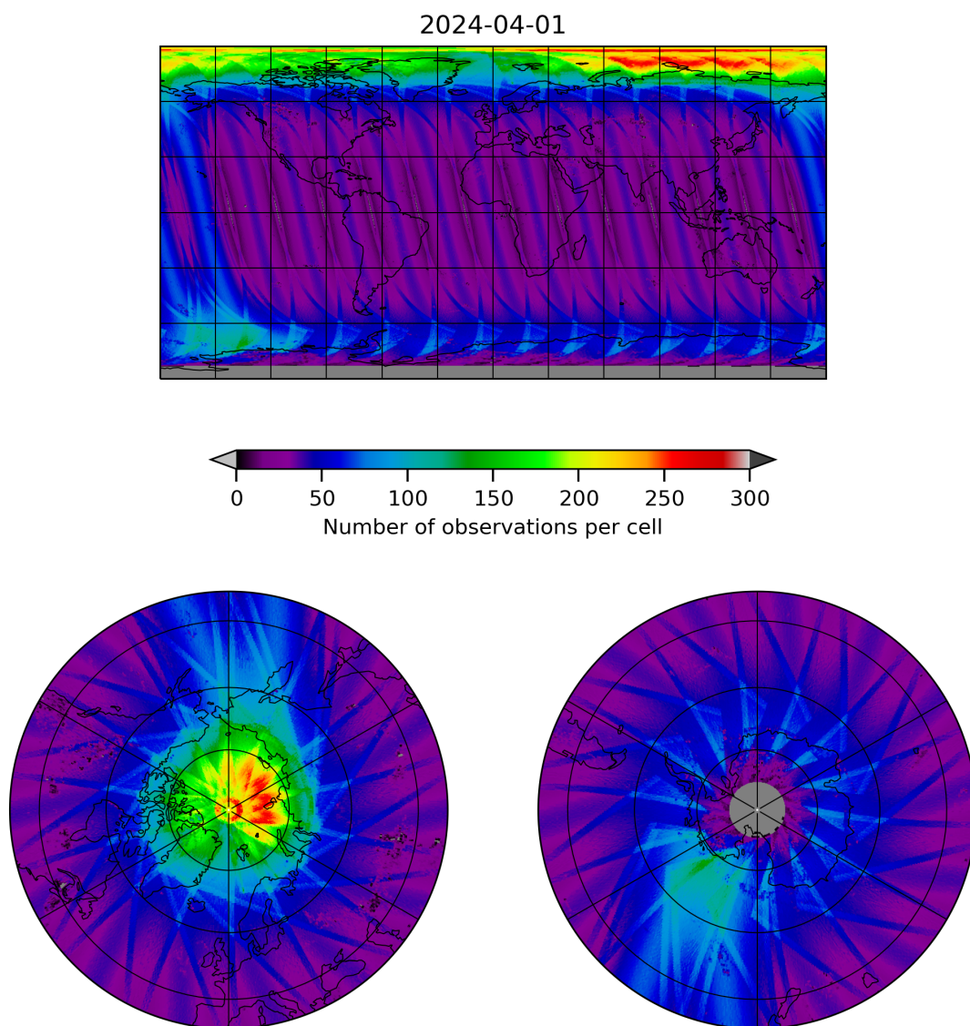
Figure 11: Map of the number of observations for 2024-03-31 to 2024-04-02
