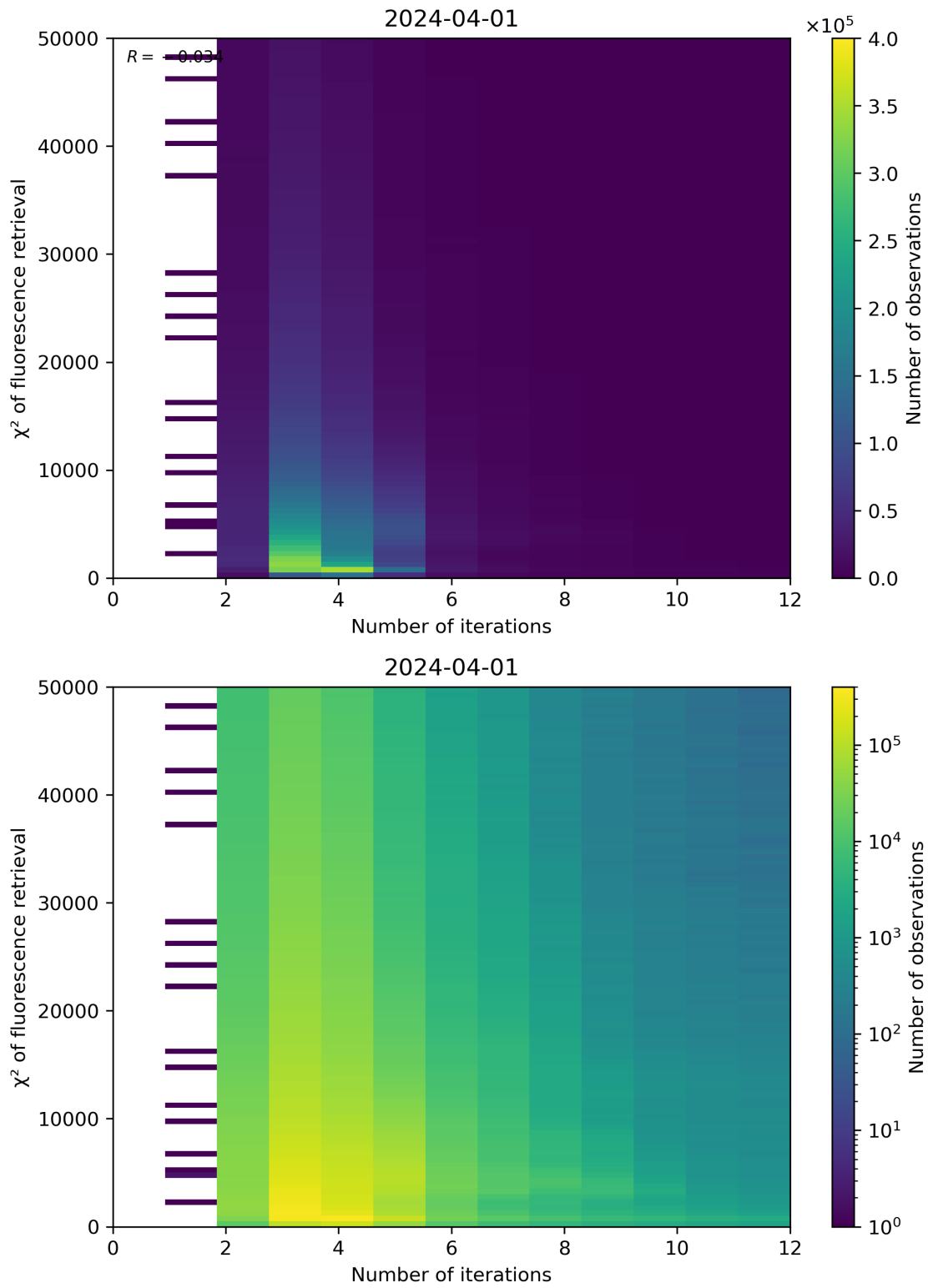
Figure 97: Scatter density plot of “Number of iterations” against “ \chi^2 of fluorescence retrieval” for 2024-03-31 to 2024-04-02.
