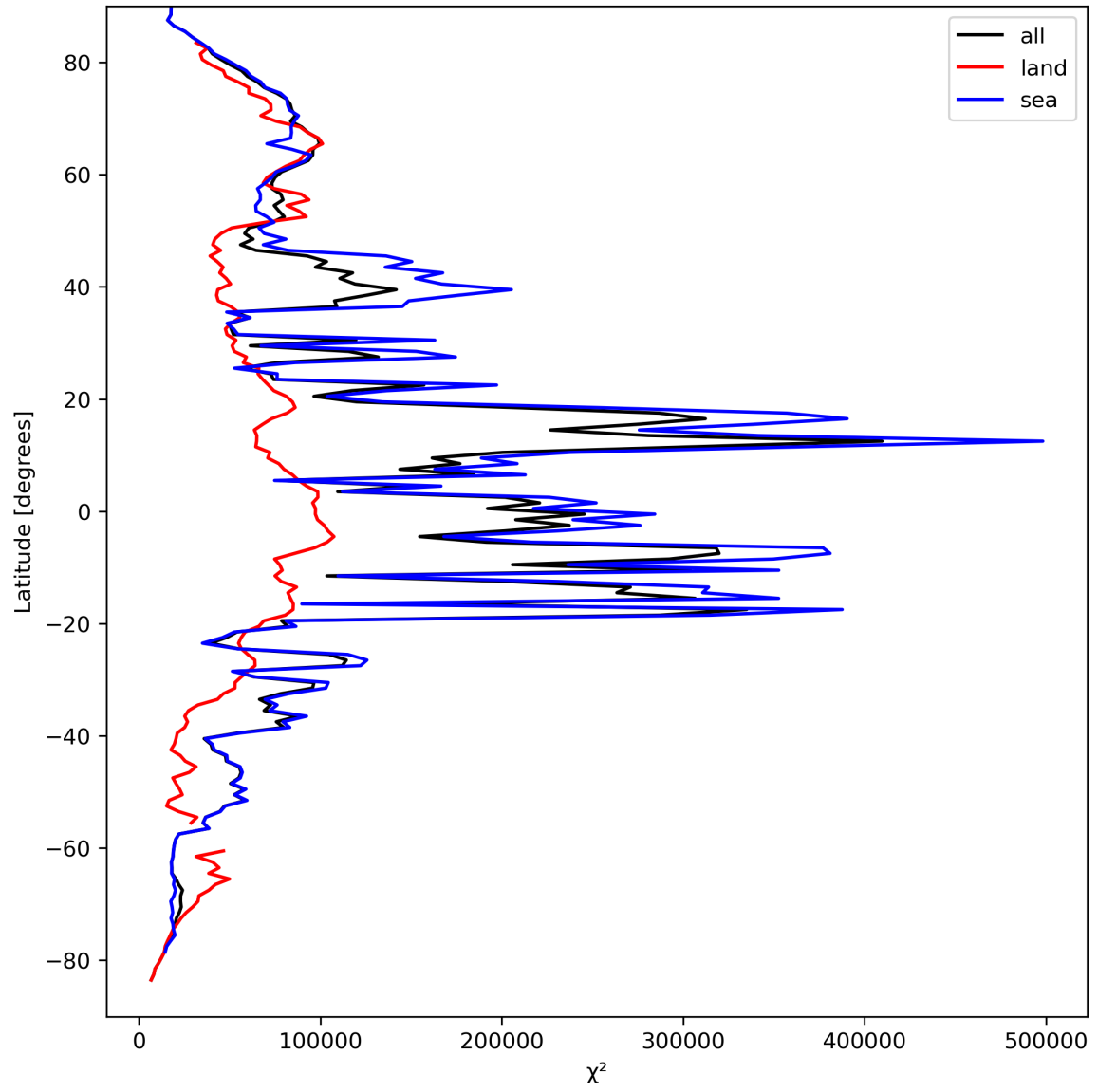
Figure 21: Zonal average of “ \chi^2 ” for 2024-03-31 to 2024-04-02.
