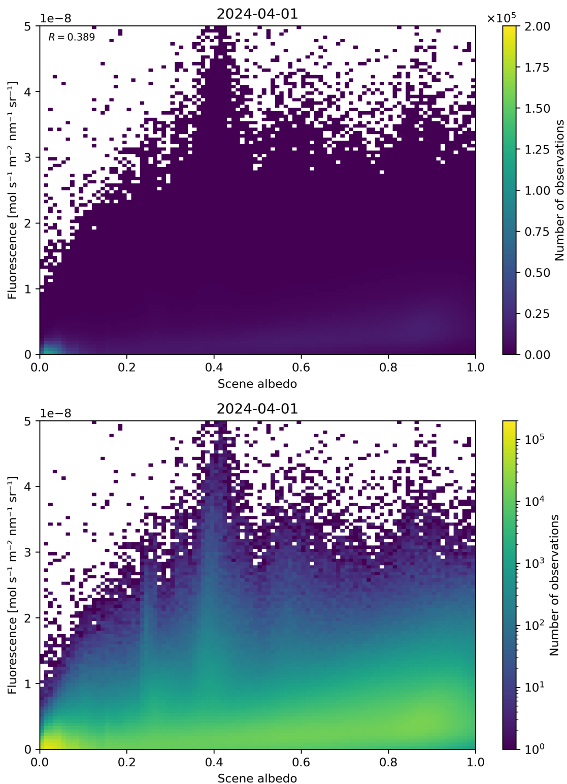
Figure 104: Scatter density plot of “Scene albedo” against “Fluorescence” for 2024-03-31 to 2024-04-02.
