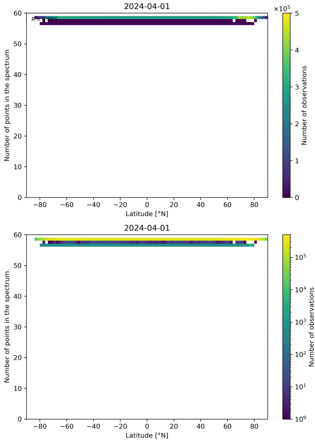
Figure 94: Scatter density plot of “Latitude” against “Number of points in the spectrum” for 2024-03-31 to 2024-04-02.
