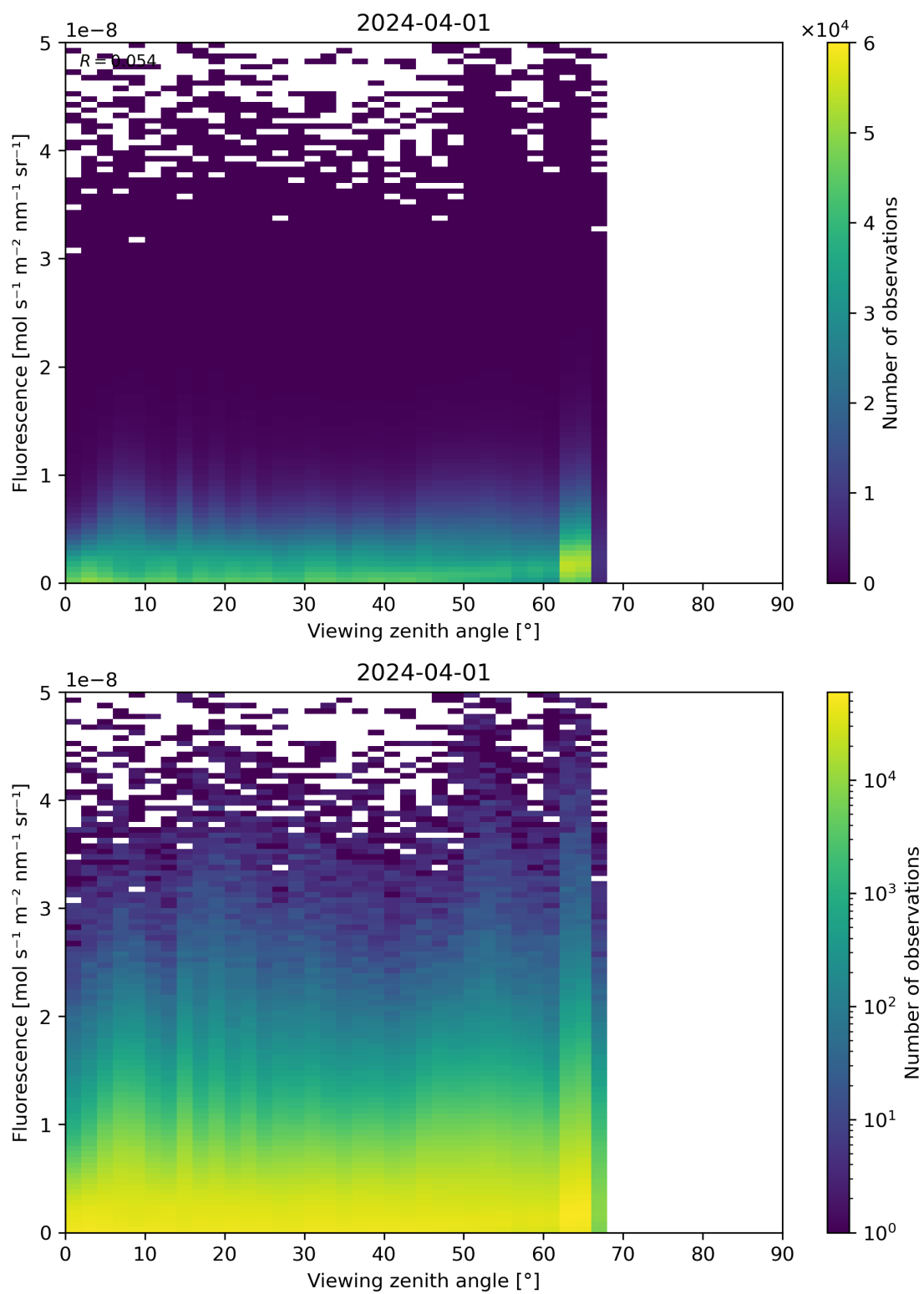
Figure 122: Scatter density plot of “Viewing zenith angle” against “Fluorescence” for 2024-03-31 to 2024-04-02.
