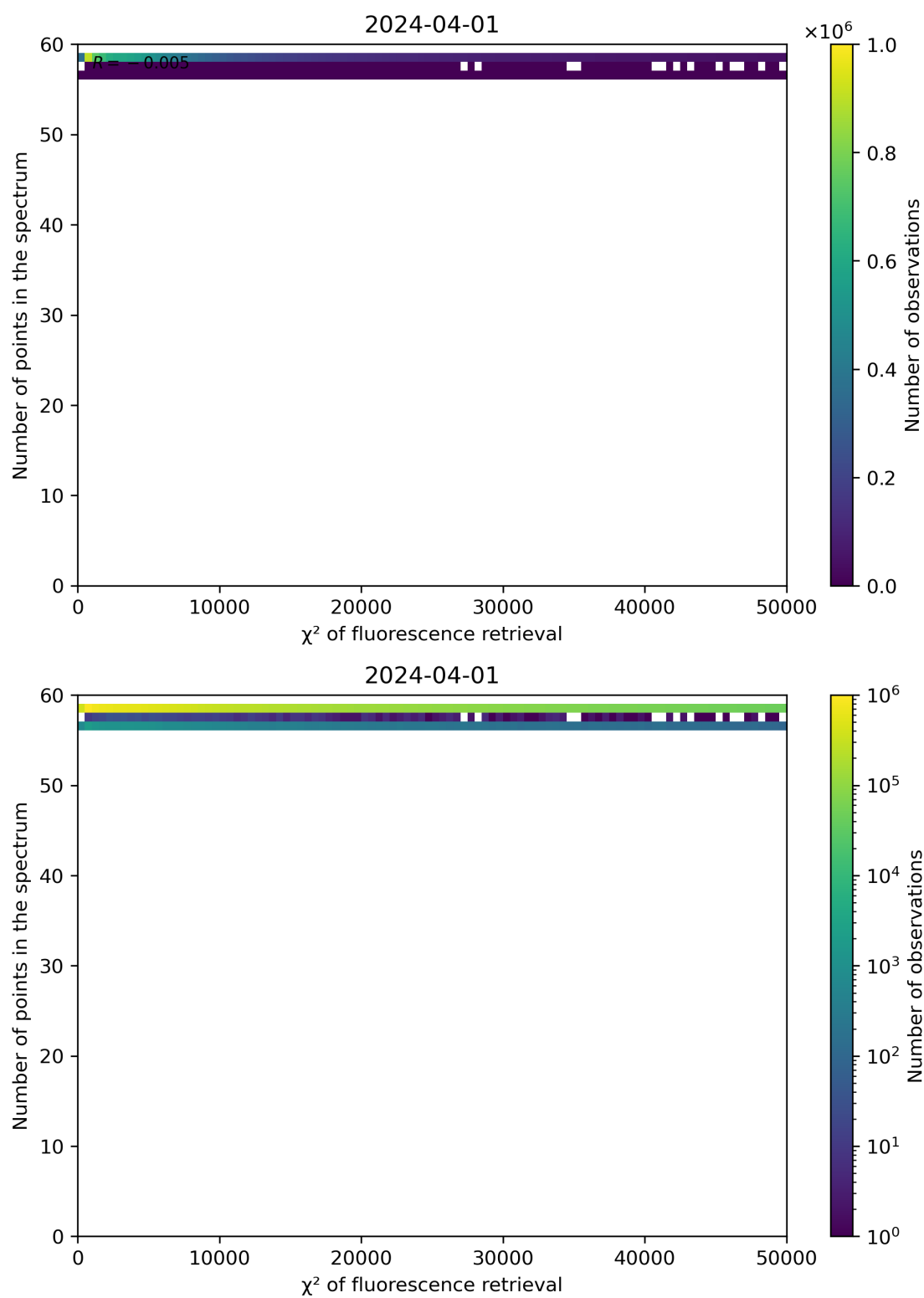
Figure 68: Scatter density plot of “ \chi^2 of fluorescence retrieval” against “Number of points in the spectrum” for 2024-03-31 to 2024-04-02.
