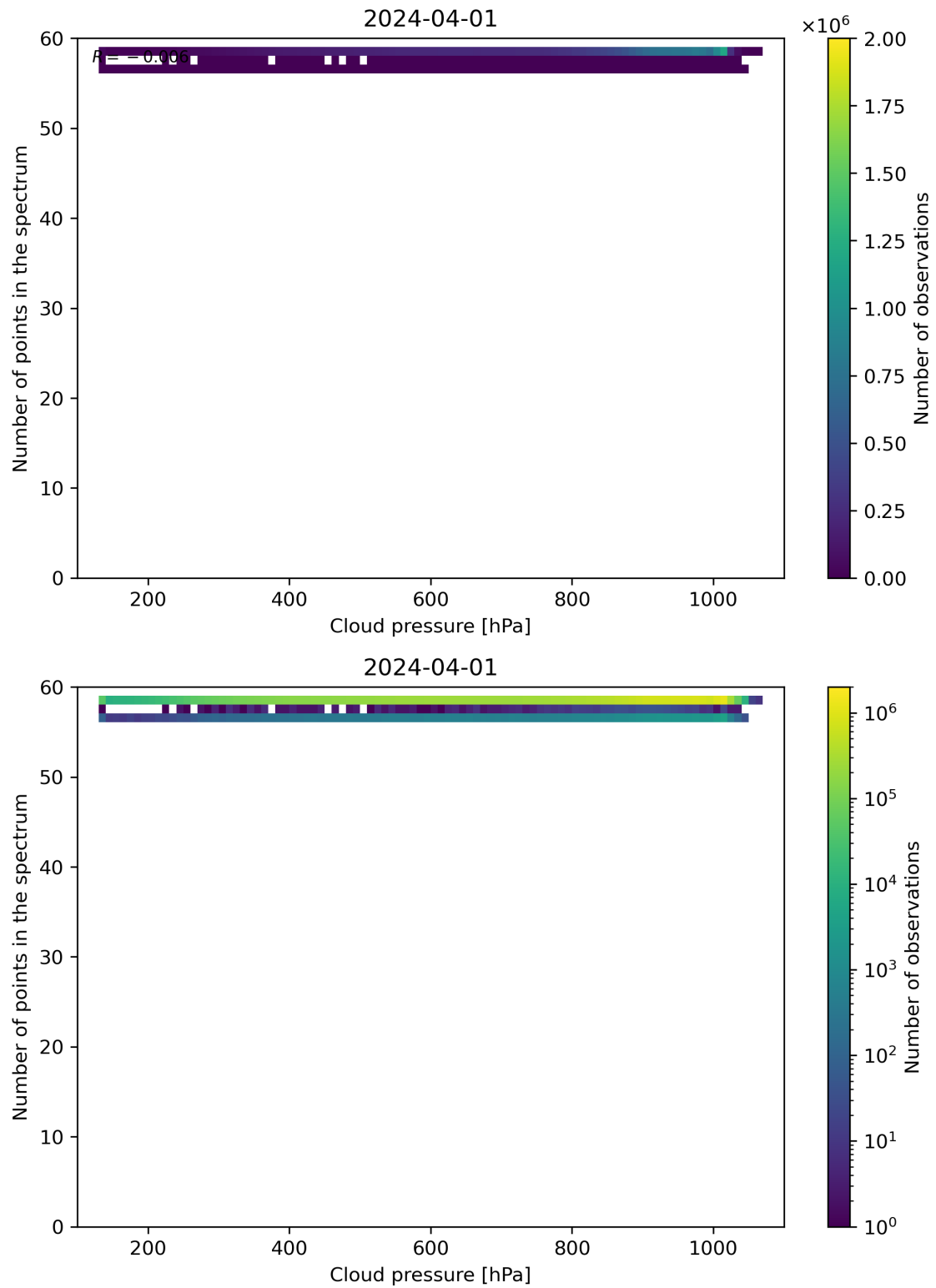
Figure 82: Scatter density plot of “Cloud pressure” against “Number of points in the spectrum” for 2024-03-31 to 2024-04-02.
