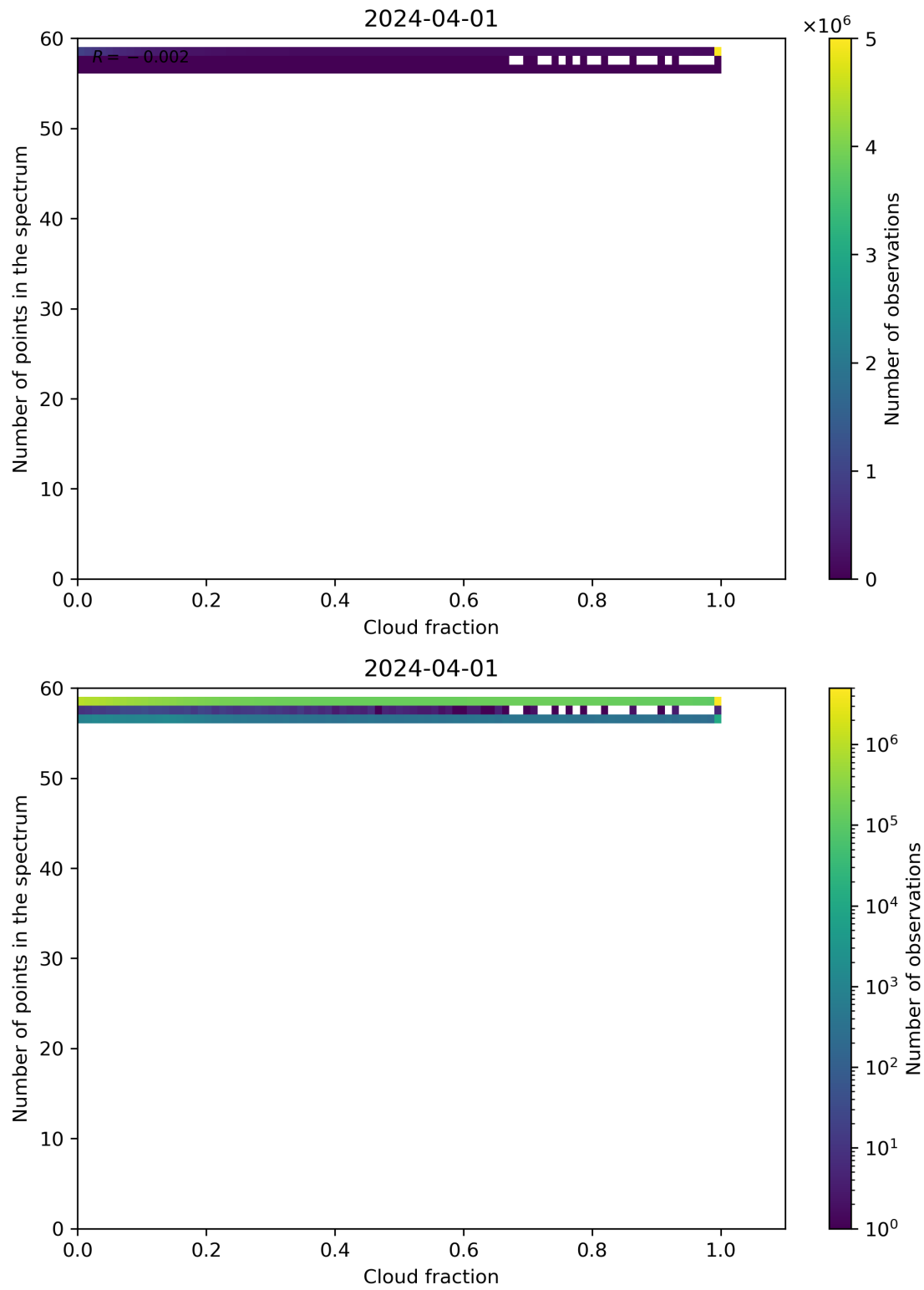
Figure 74: Scatter density plot of “Cloud fraction” against “Number of points in the spectrum” for 2024-03-31 to 2024-04-02.
