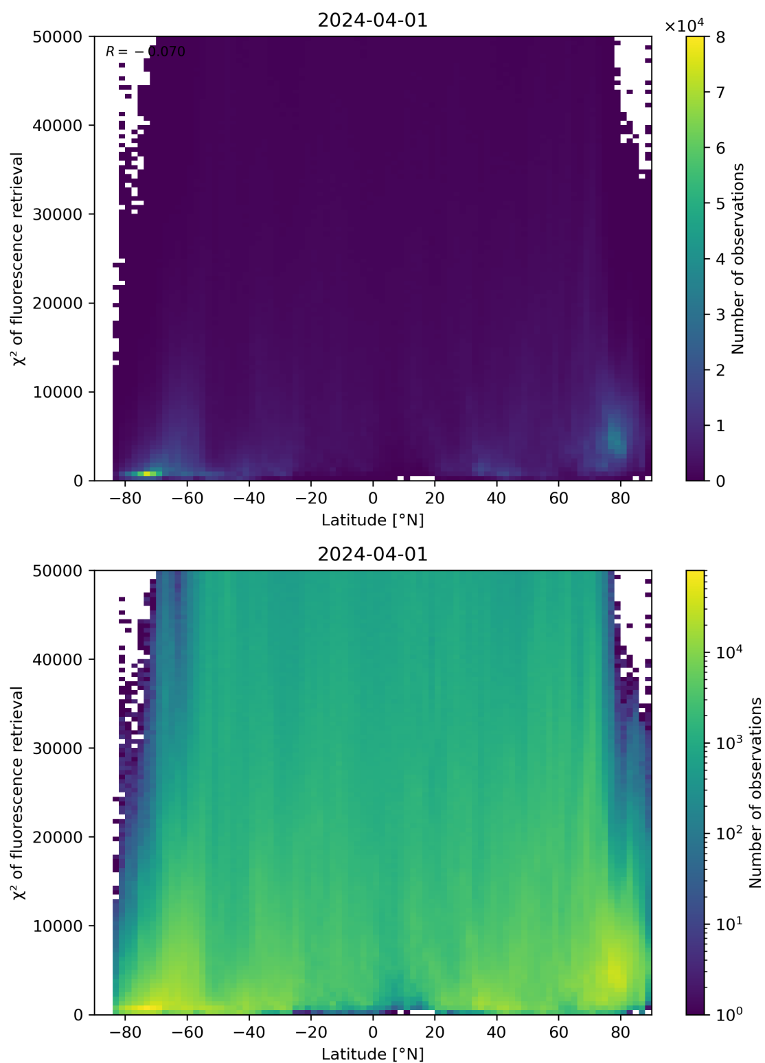
Figure 89: Scatter density plot of “Latitude” against “ \chi^2 of fluorescence retrieval” for 2024-03-31 to 2024-04-02.
