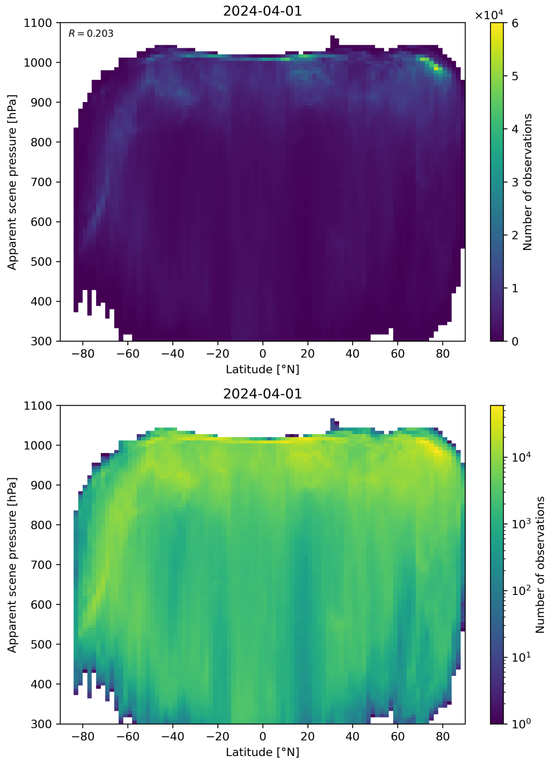
Figure 88: Scatter density plot of “Latitude” against “Apparent scene pressure” for 2024-03-31 to 2024-04-02.
