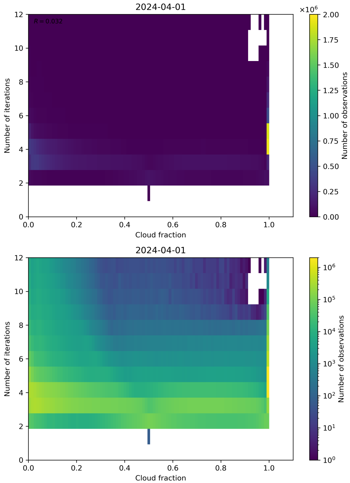
Figure 73: Scatter density plot of “Cloud fraction” against “Number of iterations” for 2024-03-31 to 2024-04-02.
