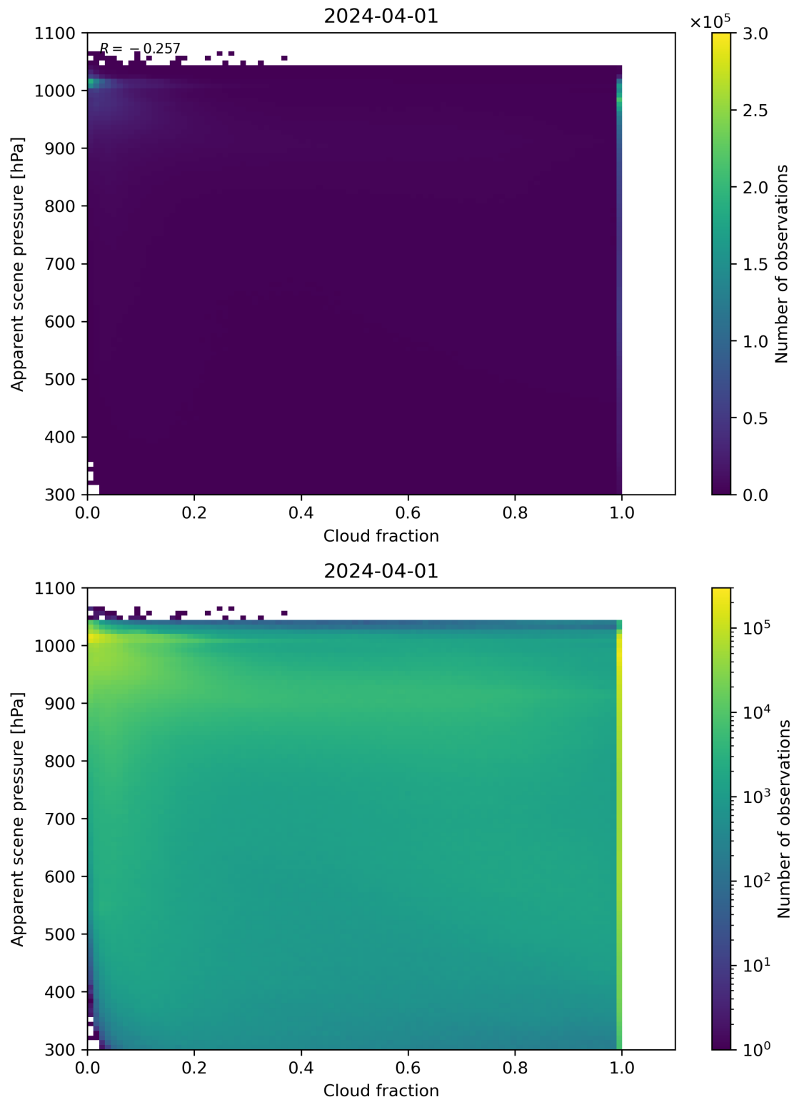
Figure 70: Scatter density plot of “Cloud fraction” against “Apparent scene pressure” for 2024-03-31 to 2024-04-02.
