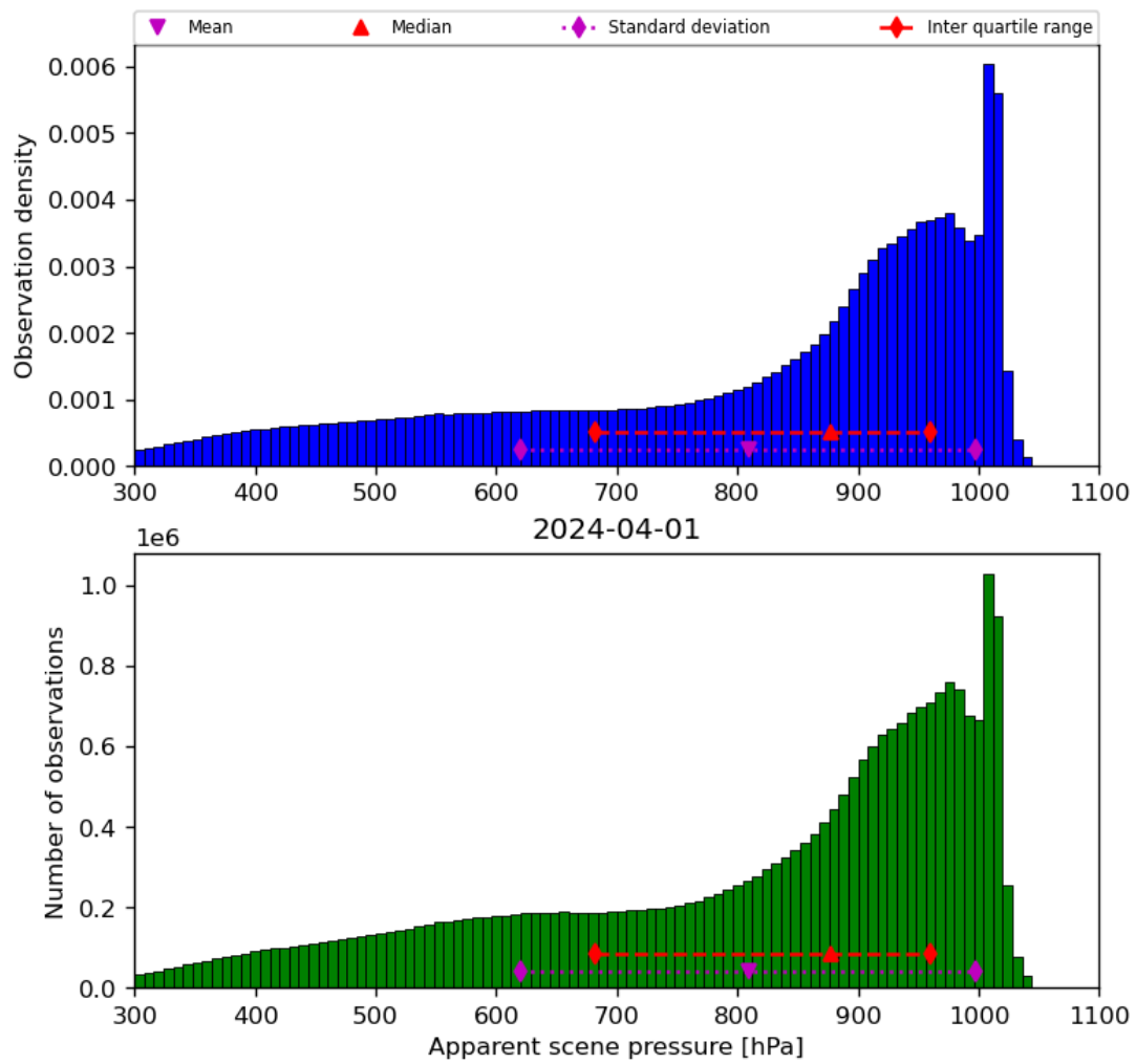
Figure 36: Histogram of “Apparent scene pressure” for 2024-03-31 to 2024-04-02
