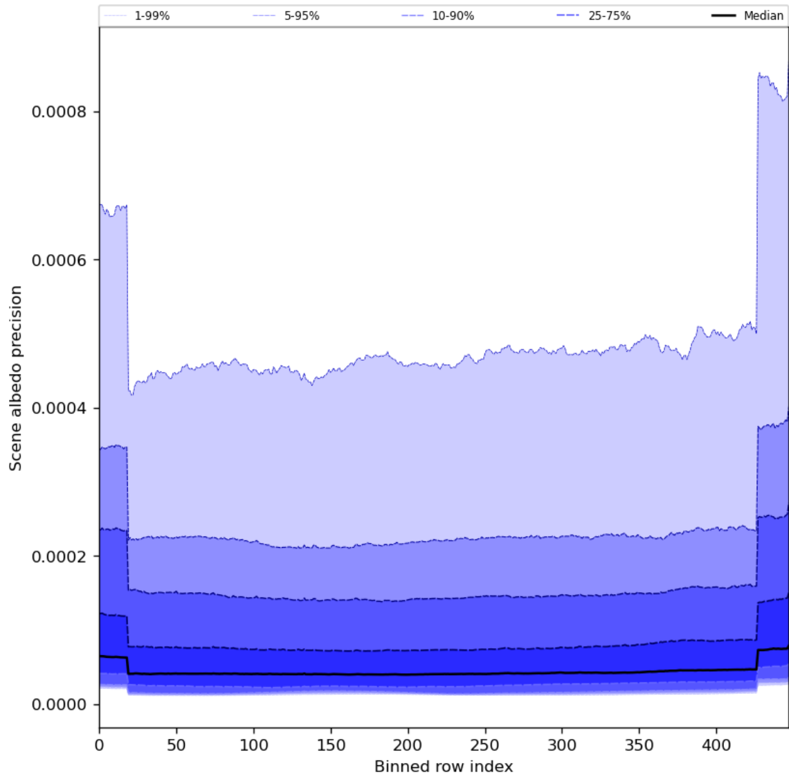
Figure 52: Along track statistics of “Scene albedo precision” for 2024-03-31 to 2024-04-02
