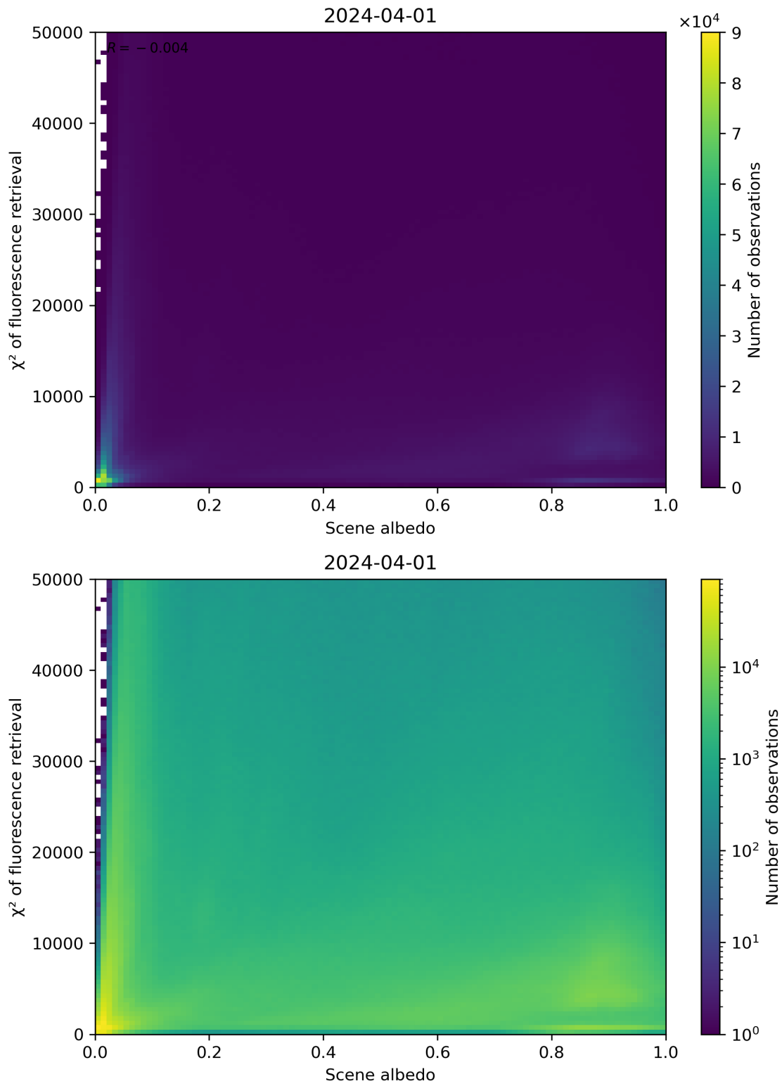
Figure 103: Scatter density plot of “Scene albedo” against “ \chi^2 of fluorescence retrieval” for 2024-03-31 to 2024-04-02.
