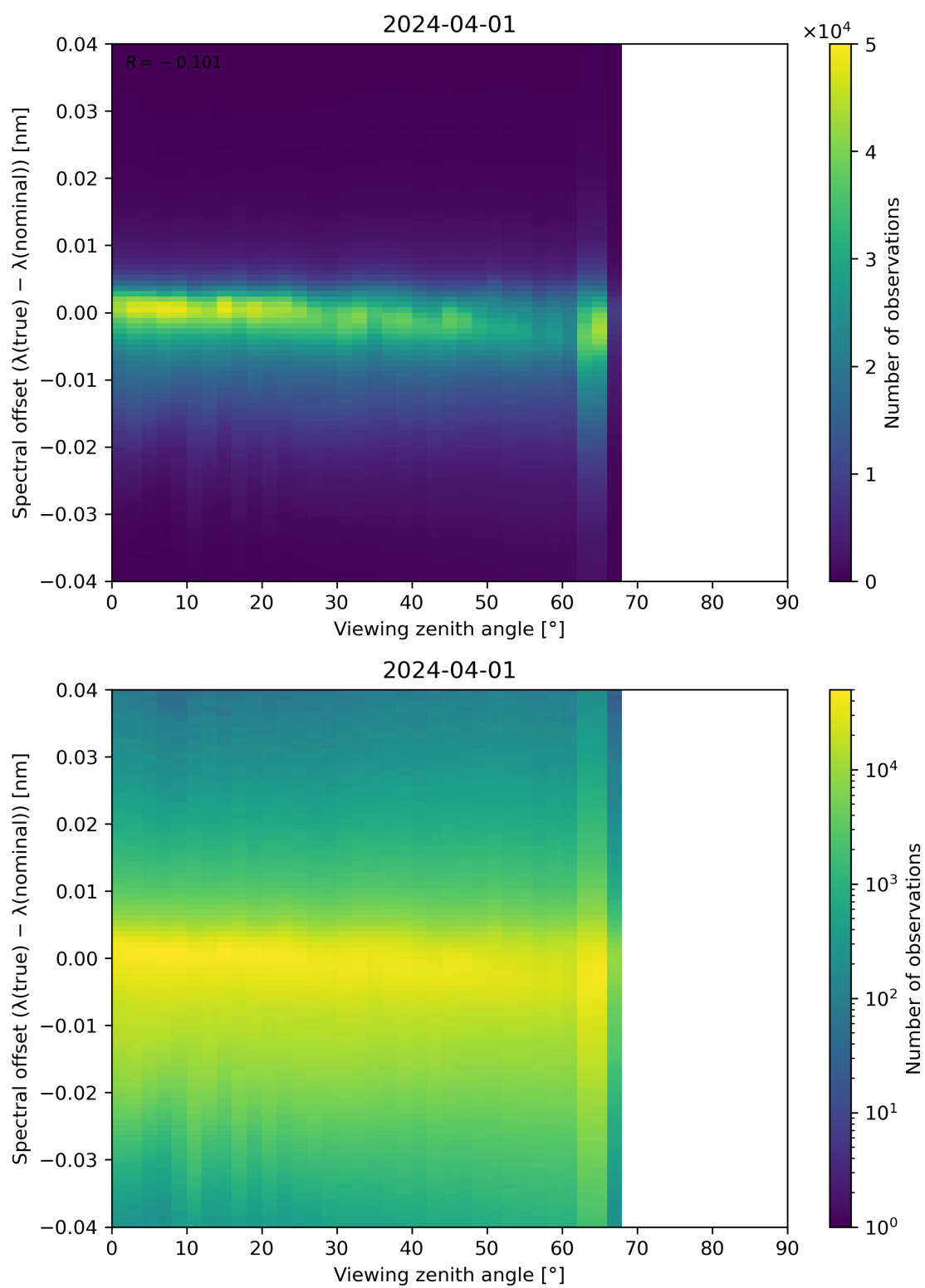
Figure 128: Scatter density plot of “Viewing zenith angle” against “Spectral offset ( \lambda(\text{true}) - \lambda(\text{nominal}) )” for 2024-03-31 to 2024-04-02.
