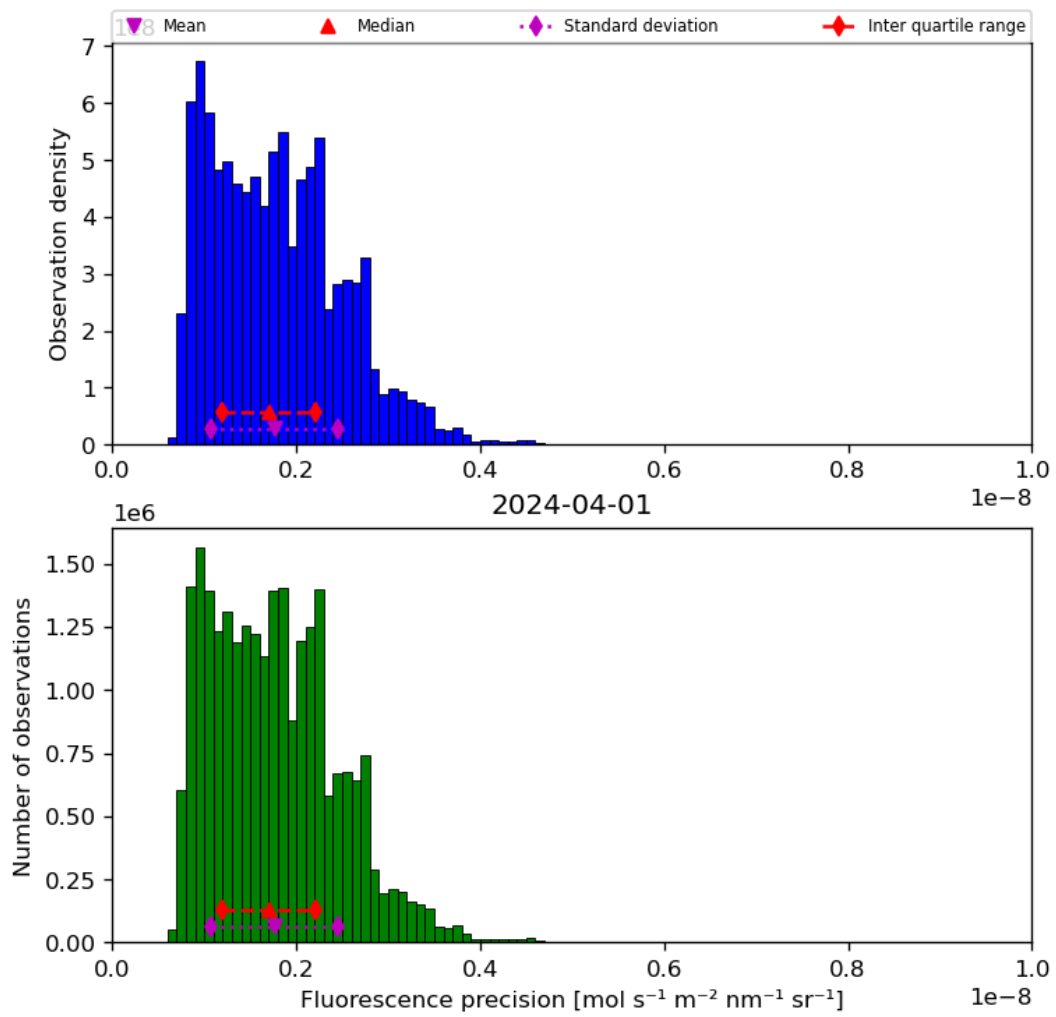
Figure 41: Histogram of “Fluorescence precision” for 2024-03-31 to 2024-04-02
