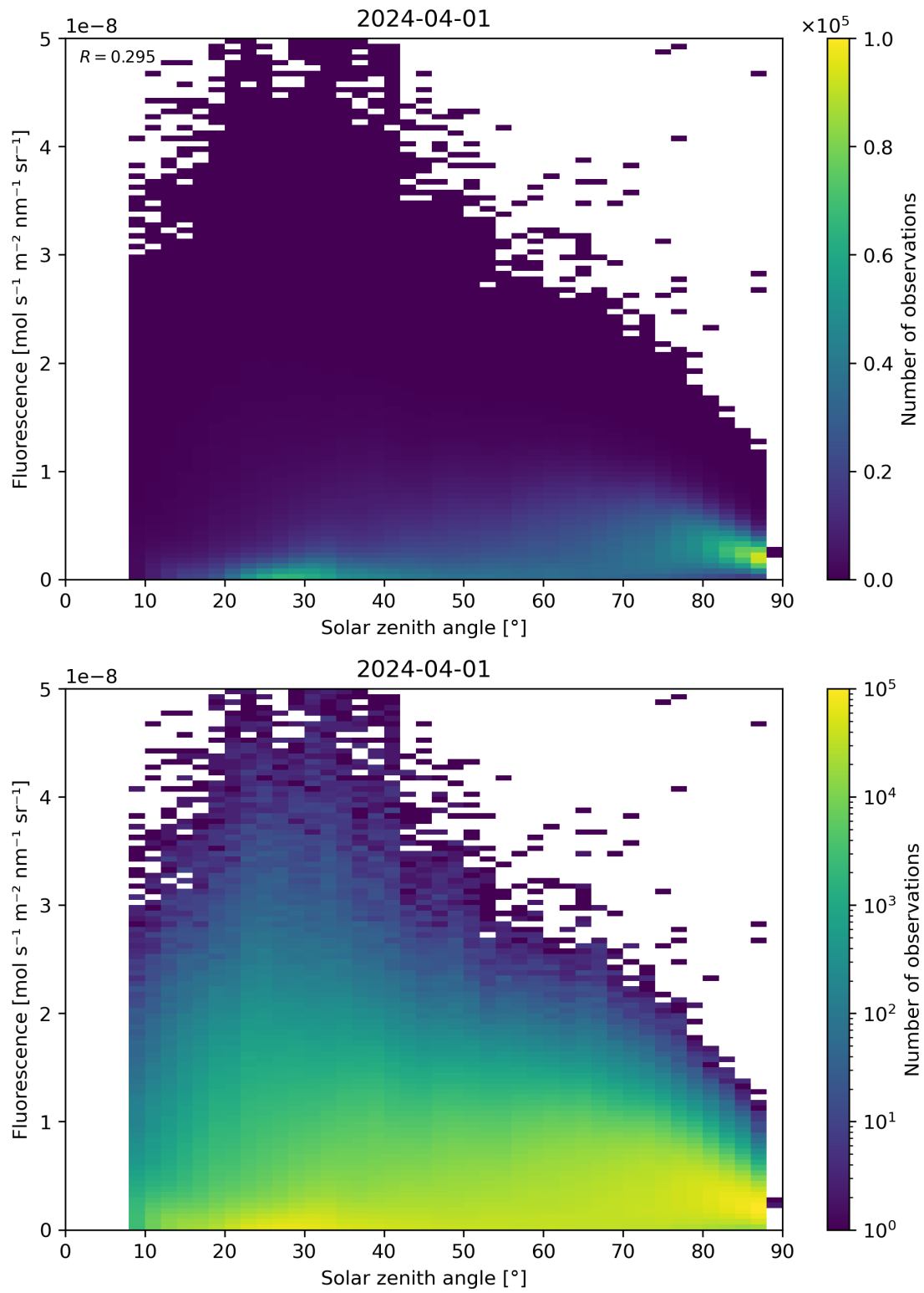
Figure 112: Scatter density plot of “Solar zenith angle” against “Fluorescence” for 2024-03-31 to 2024-04-02.
