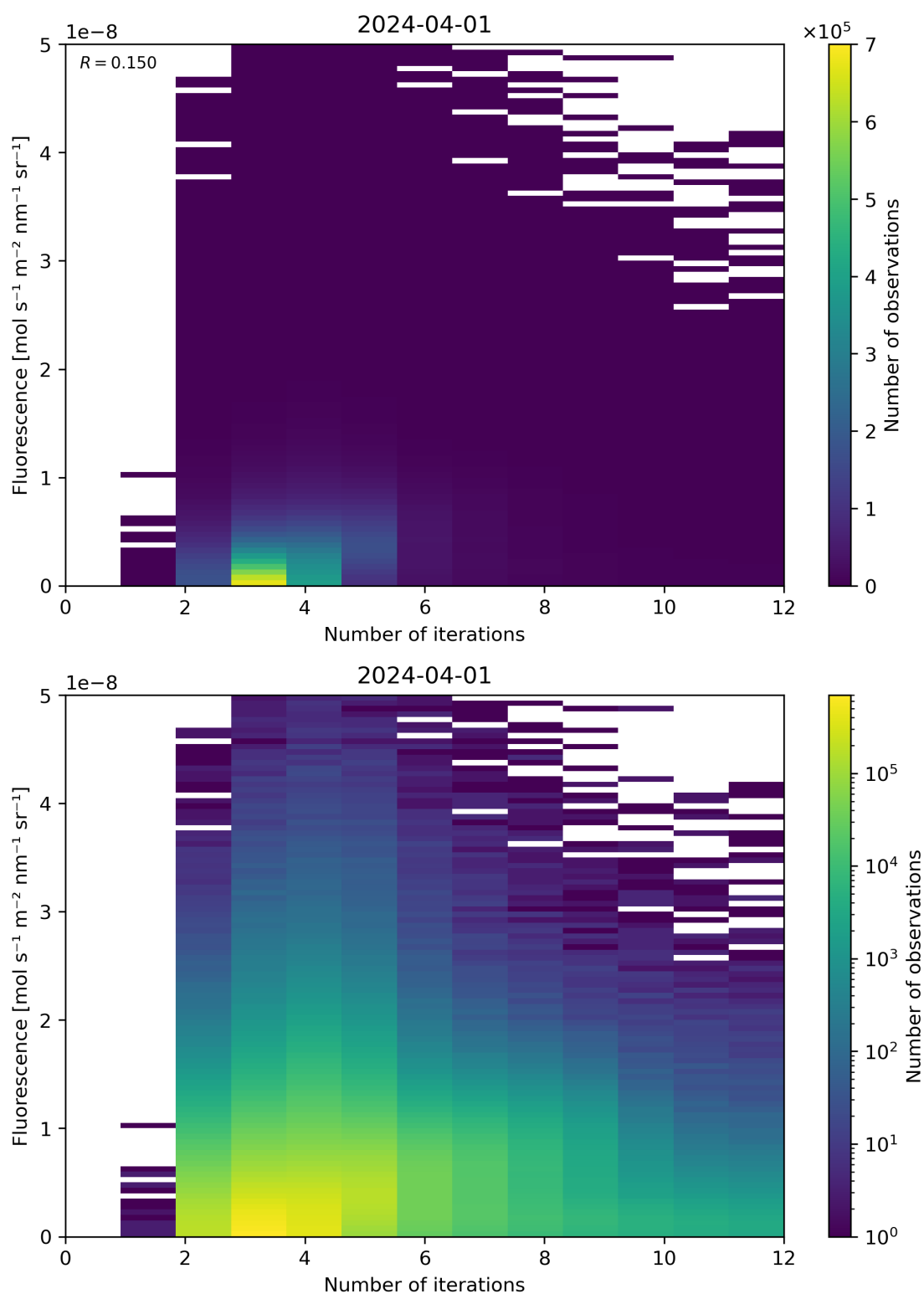
Figure 98: Scatter density plot of “Number of iterations” against “Fluorescence” for 2024-03-31 to 2024-04-02.
