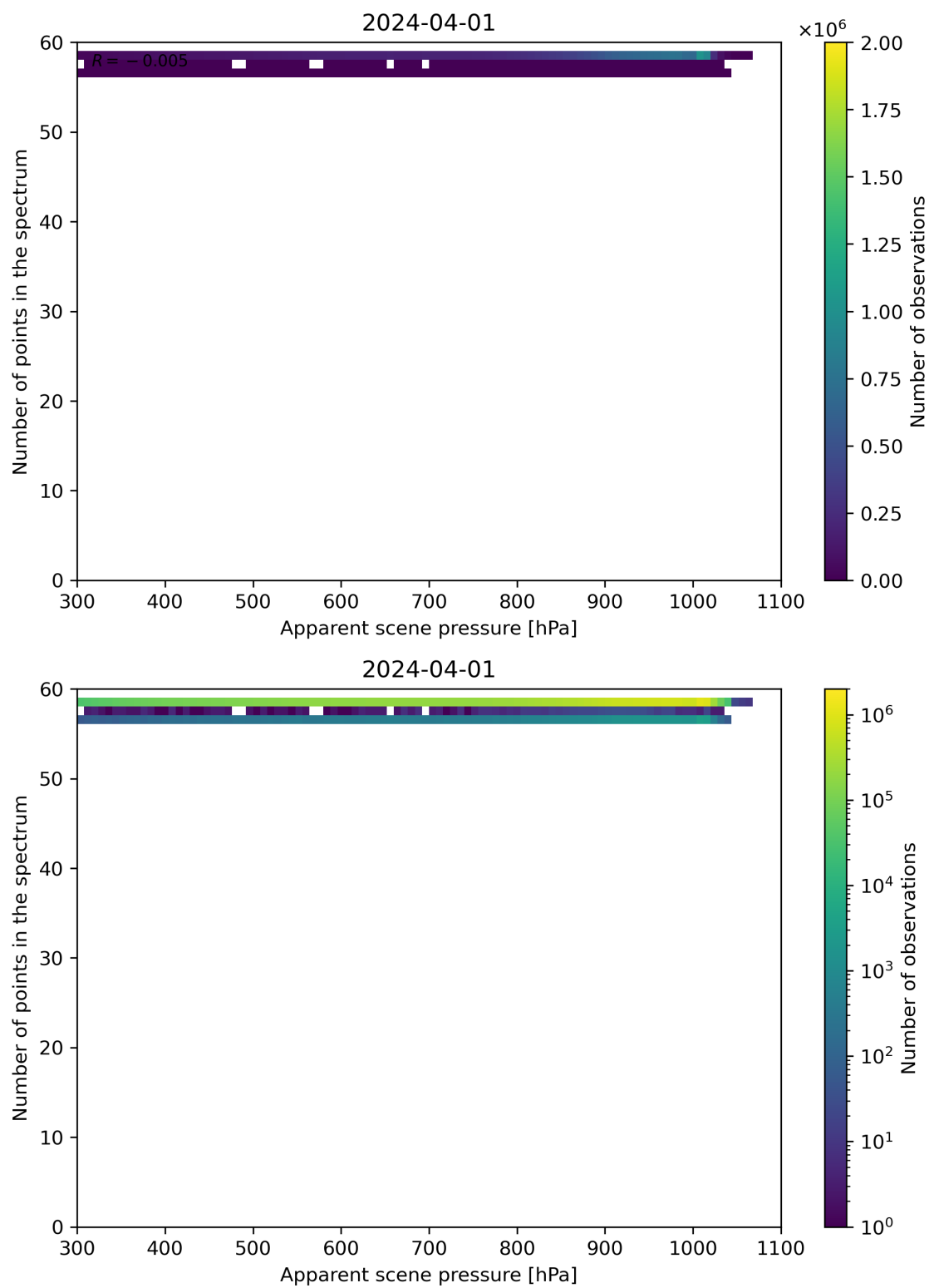
Figure 66: Scatter density plot of “Apparent scene pressure” against “Number of points in the spectrum” for 2024-03-31 to 2024-04-02.
