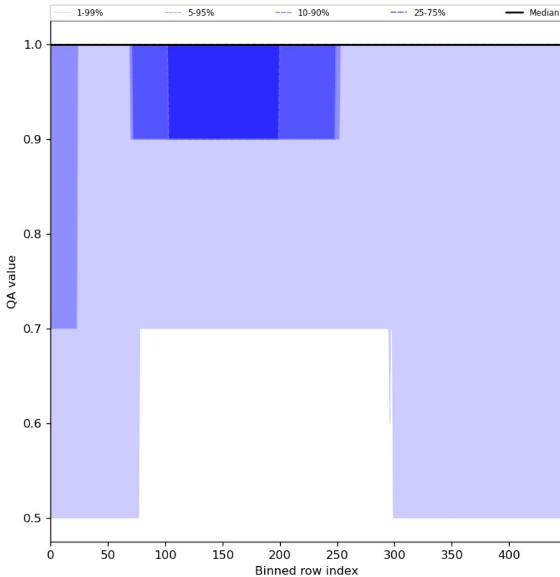
Figure 46: Along track statistics of “QA value” for 2024-03-31 to 2024-04-02
