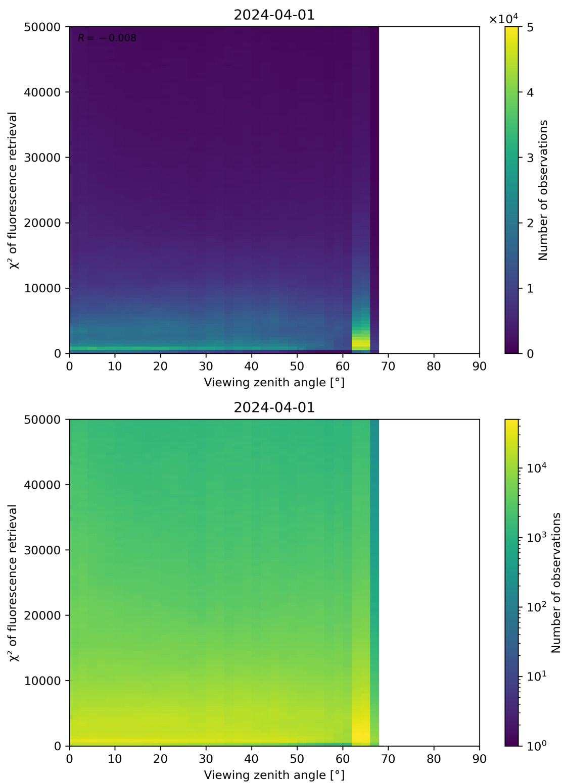
Figure 119: Scatter density plot of “Viewing zenith angle” against “ \chi^2 of fluorescence retrieval” for 2024-03-31 to 2024-04-02.
