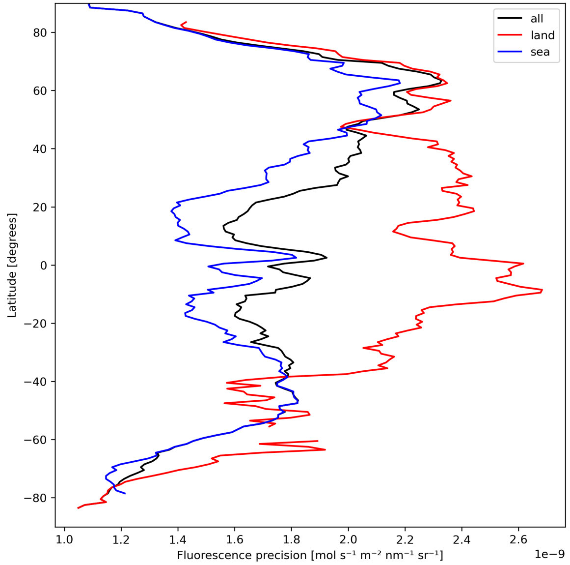
Figure 24: Zonal average of “Fluorescence precision” for 2024-03-31 to 2024-04-02.
