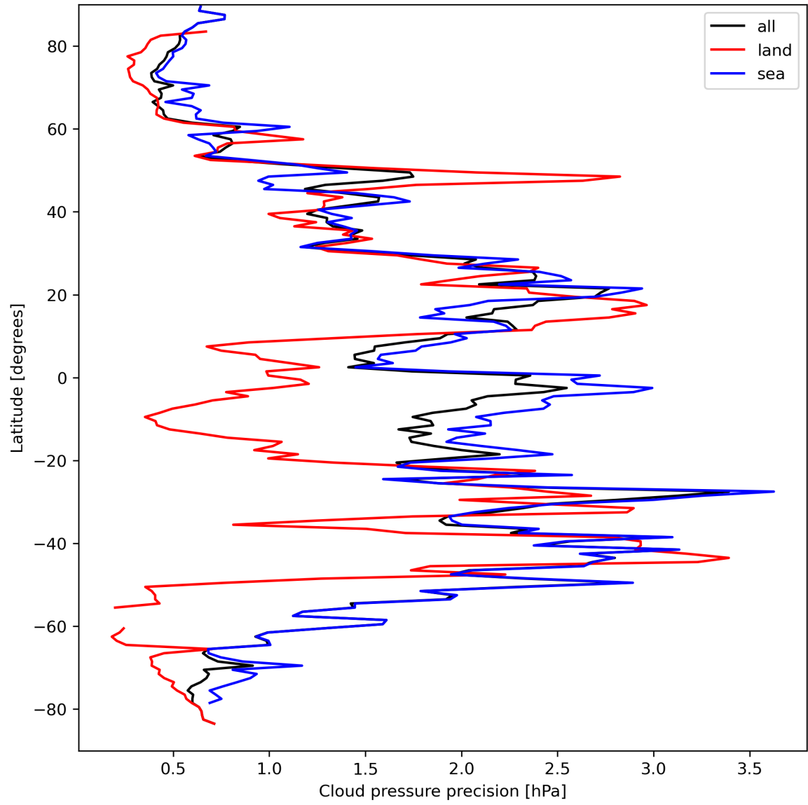
Figure 14: Zonal average of “Cloud pressure precision” for 2024-03-31 to 2024-04-02.
