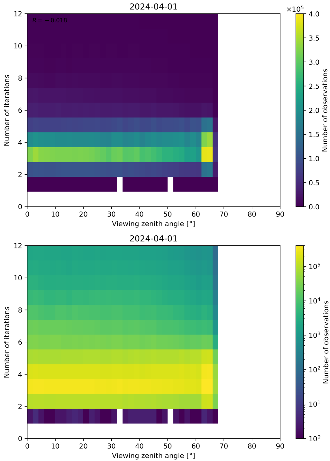
Figure 124: Scatter density plot of “Viewing zenith angle” against “Number of iterations” for 2024-03-31 to 2024-04-02.
