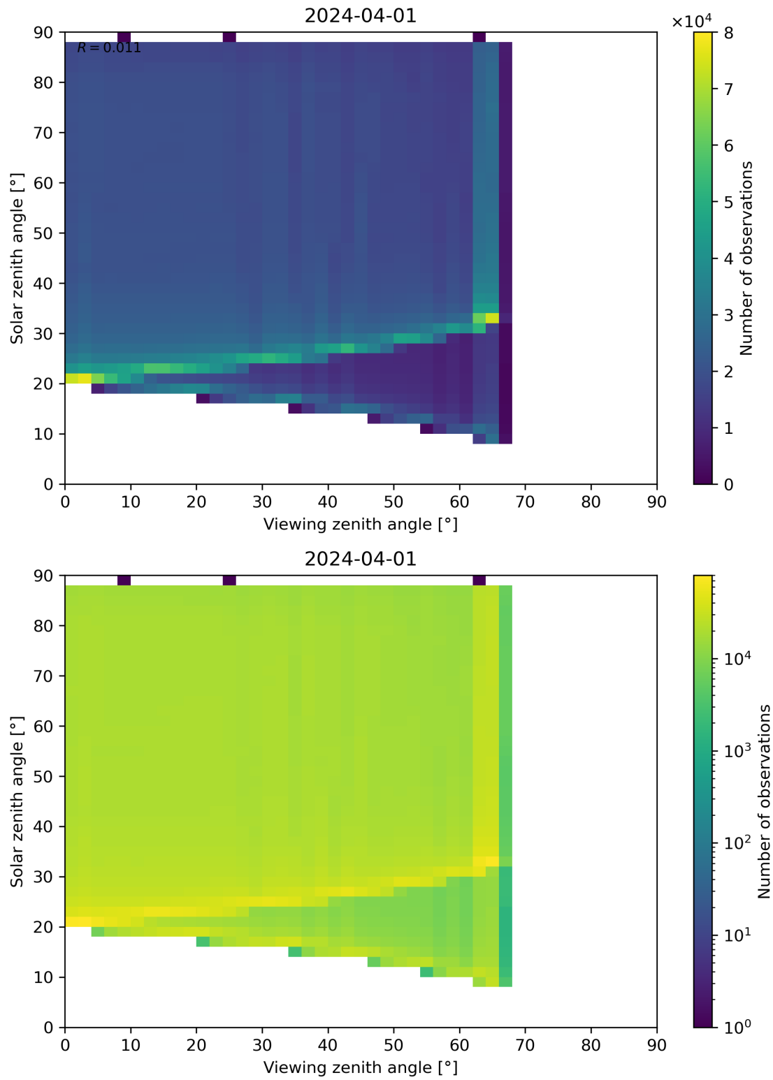
Figure 127: Scatter density plot of “Viewing zenith angle” against “Solar zenith angle” for 2024-03-31 to 2024-04-02.
