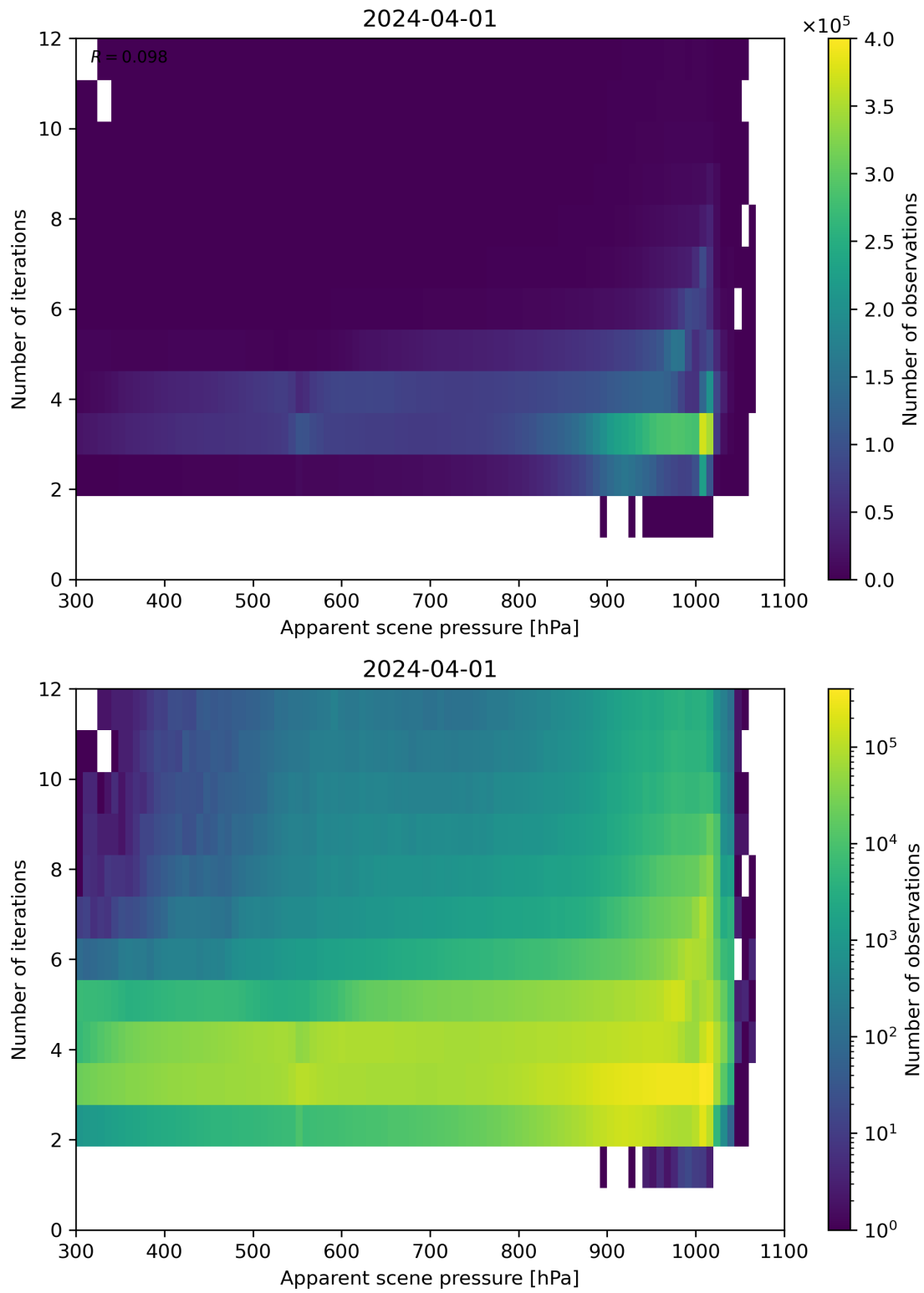
Figure 65: Scatter density plot of “Apparent scene pressure” against “Number of iterations” for 2024-03-31 to 2024-04-02.
