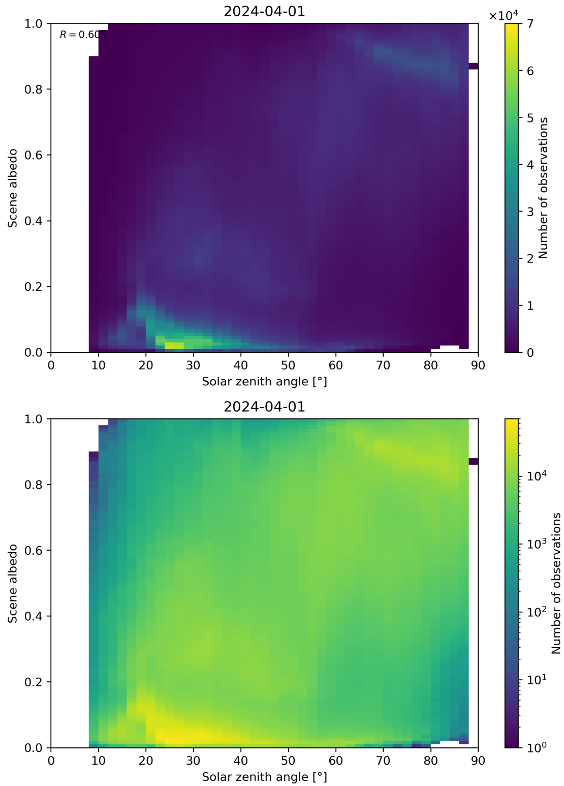
Figure 116: Scatter density plot of “Solar zenith angle” against “Scene albedo” for 2024-03-31 to 2024-04-02.
