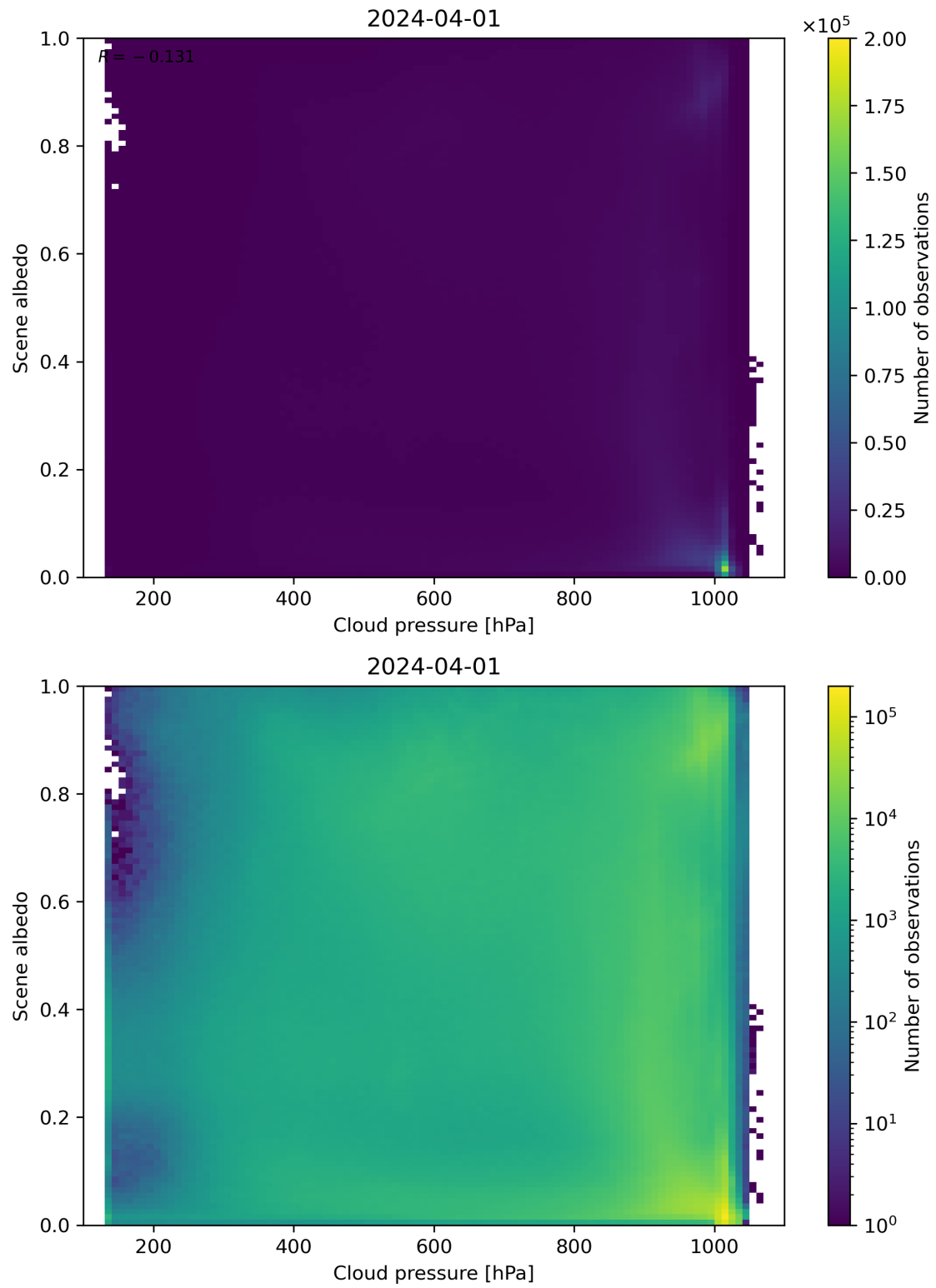
Figure 83: Scatter density plot of “Cloud pressure” against “Scene albedo” for 2024-03-31 to 2024-04-02.
