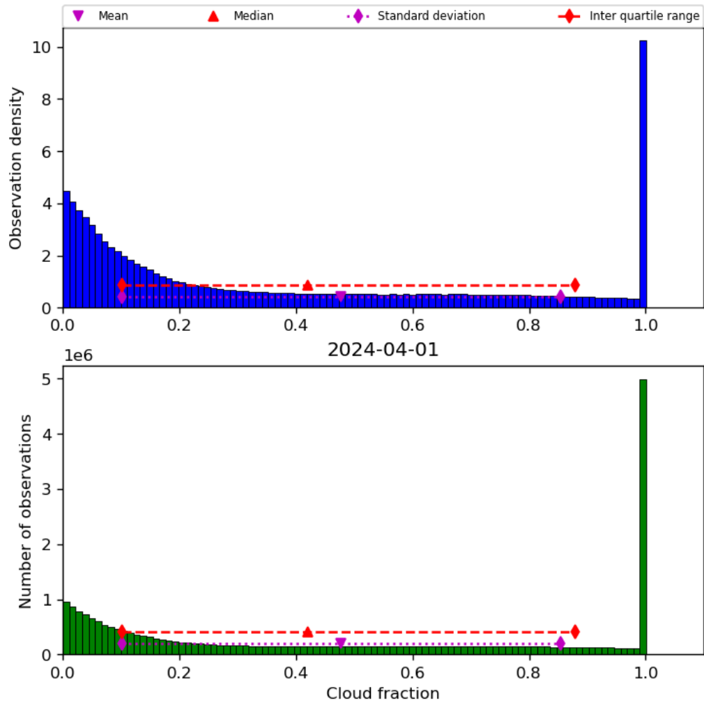
Figure 32: Histogram of “Cloud fraction” for 2024-03-31 to 2024-04-02
