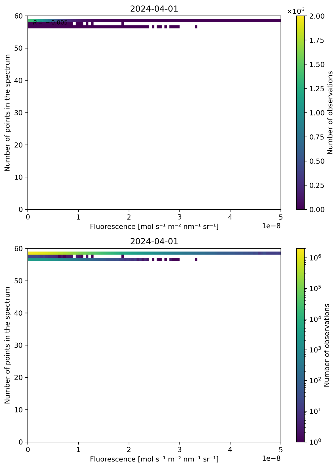
Figure 86: Scatter density plot of “Fluorescence” against “Number of points in the spectrum” for 2024-03-31 to 2024-04-02.
