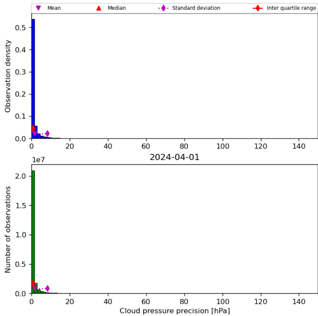
Figure 31: Histogram of “Cloud pressure precision” for 2024-03-31 to 2024-04-02
