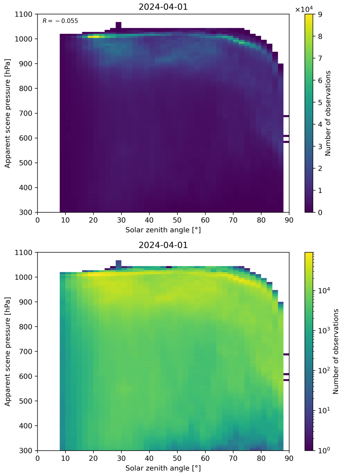
Figure 108: Scatter density plot of “Solar zenith angle” against “Apparent scene pressure” for 2024-03-31 to 2024-04-02.
