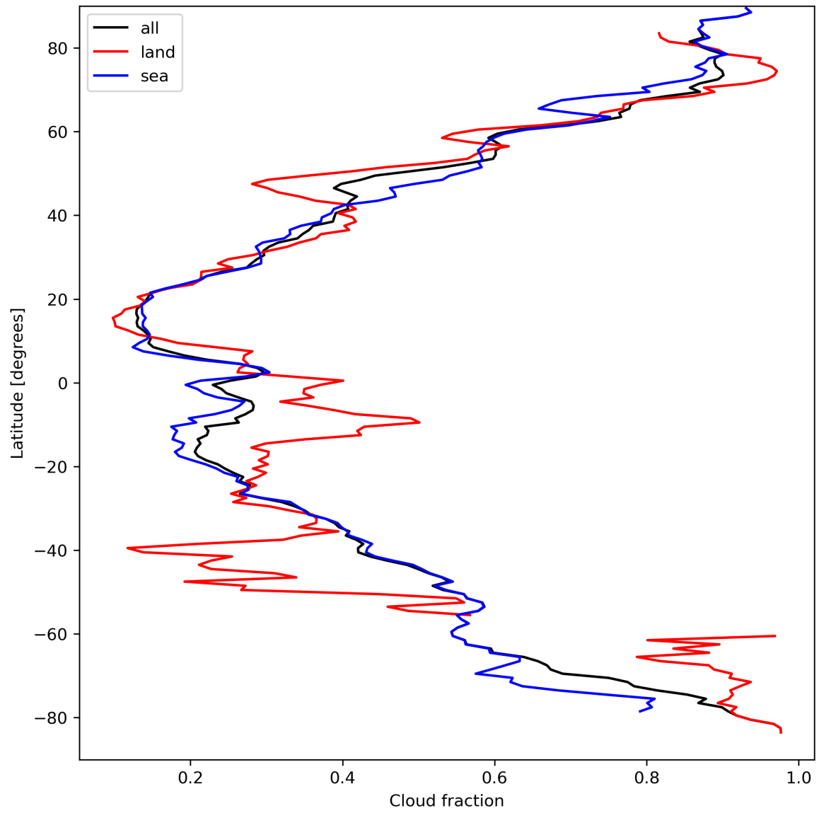
Figure 15: Zonal average of “Cloud fraction” for 2024-03-31 to 2024-04-02.
