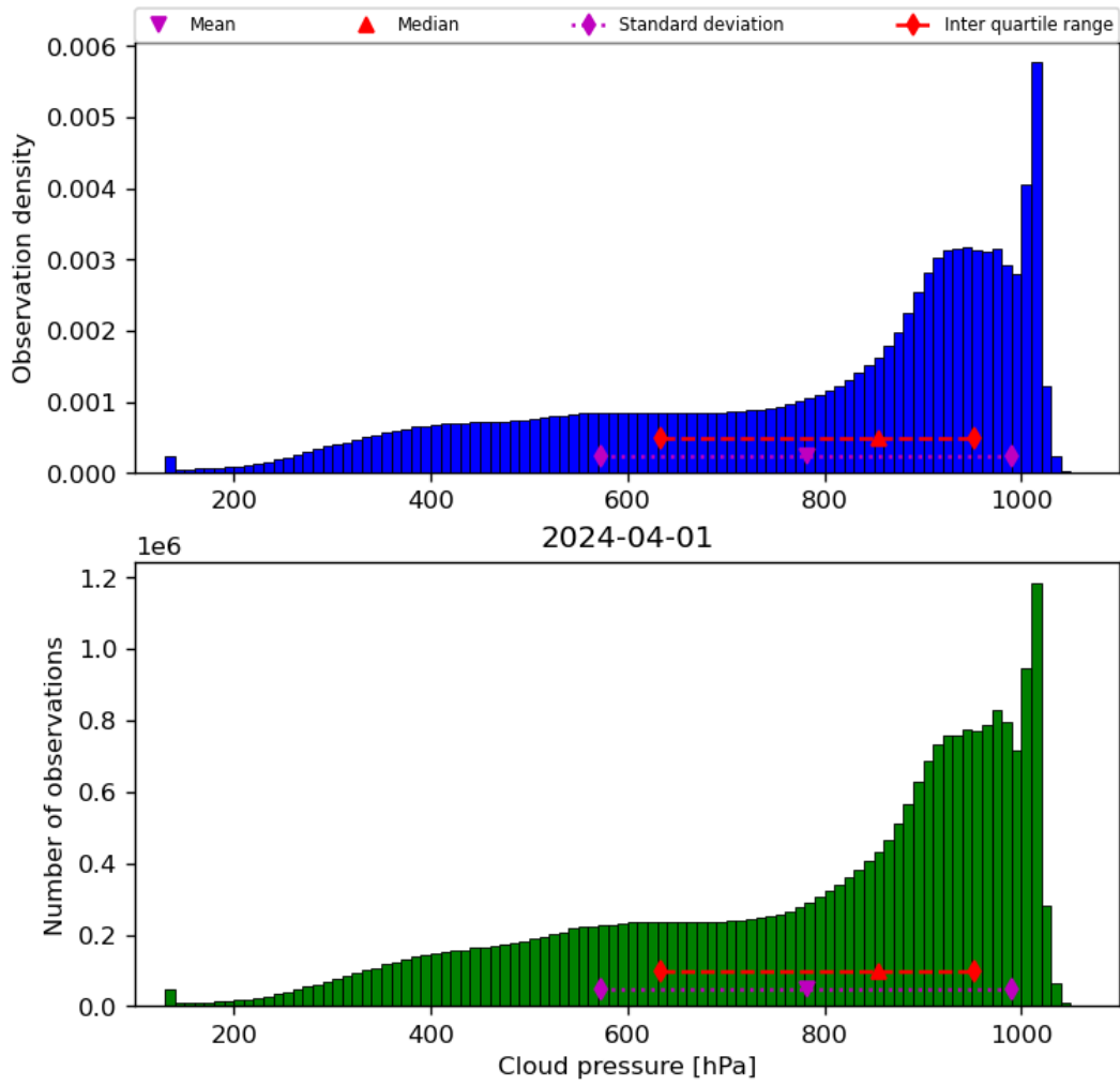
Figure 30: Histogram of “Cloud pressure” for 2024-03-31 to 2024-04-02
