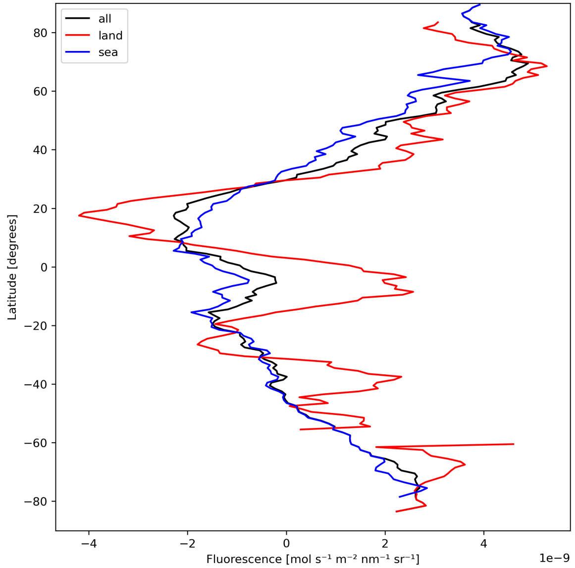
Figure 23: Zonal average of “Fluorescence” for 2024-03-31 to 2024-04-02.
