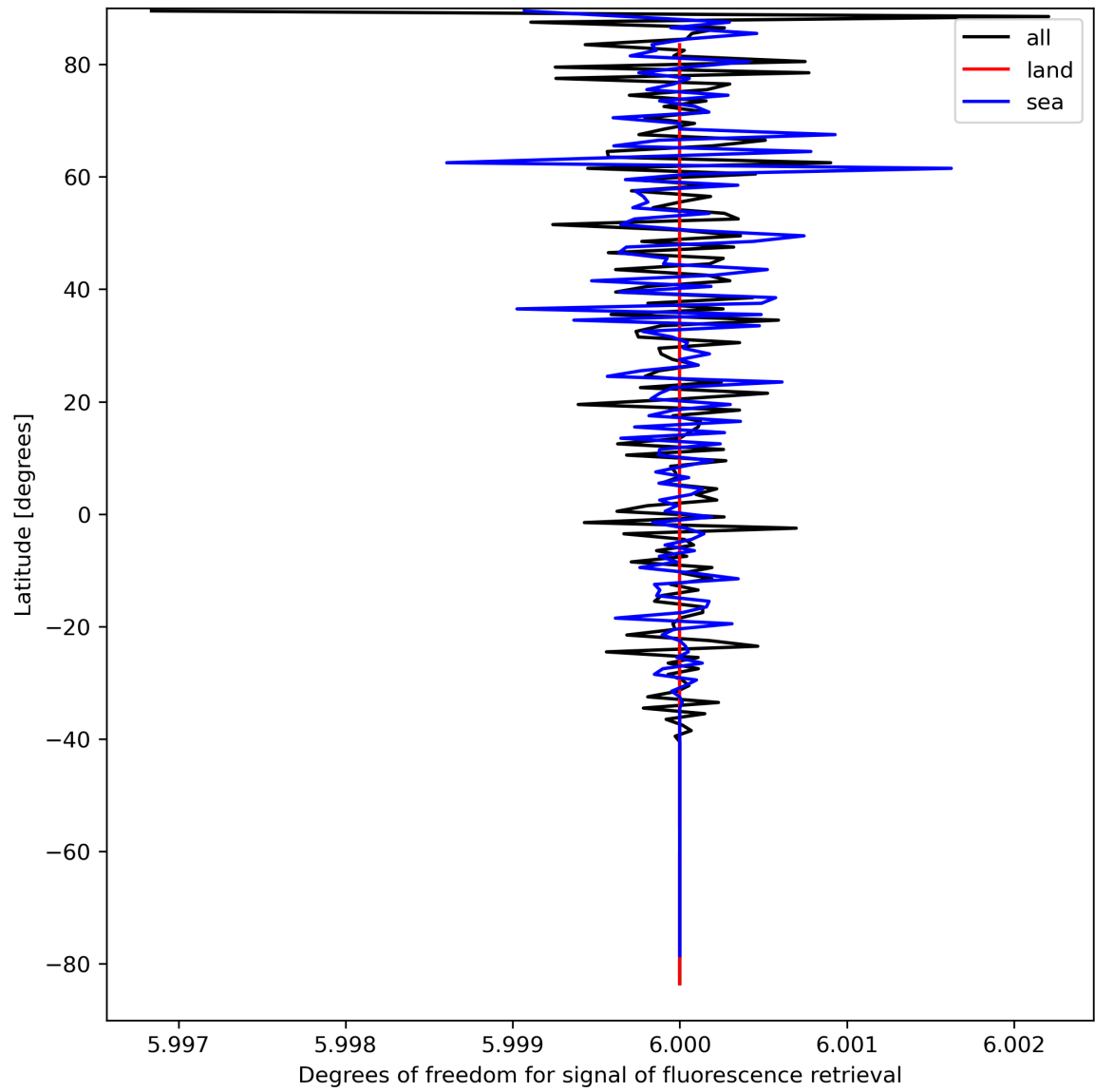
Figure 26: Zonal average of “Degrees of freedom for signal of fluorescence retrieval” for 2024-03-31 to 2024-04-02.
