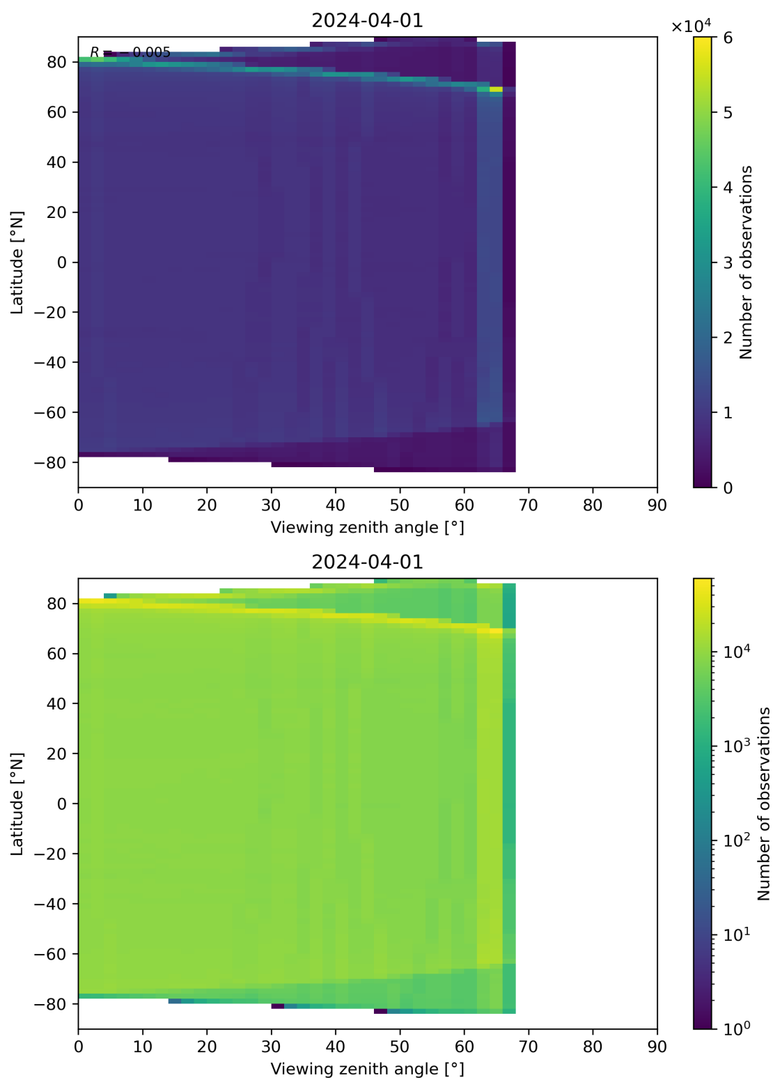
Figure 123: Scatter density plot of “Viewing zenith angle” against “Latitude” for 2024-03-31 to 2024-04-02.
