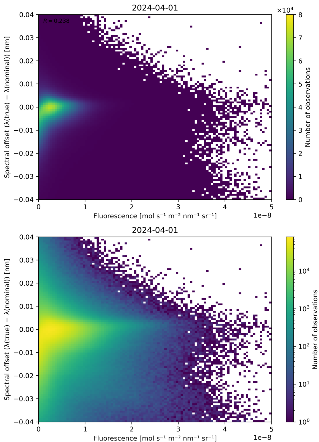
Figure 87: Scatter density plot of “Fluorescence” against “Spectral offset ( \lambda(\text{true}) - \lambda(\text{nominal}) )” for 2024-03-31 to 2024-04-02.
