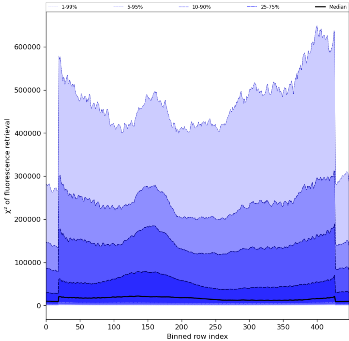
Figure 59: Along track statistics of “ \chi^2 of fluorescence retrieval” for 2024-03-31 to 2024-04-02
