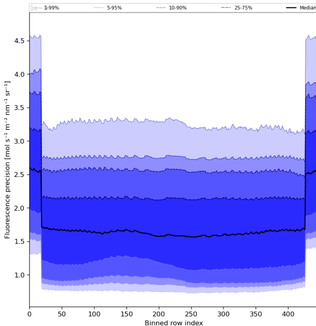
Figure 58: Along track statistics of “Fluorescence precision” for 2024-03-31 to 2024-04-02
