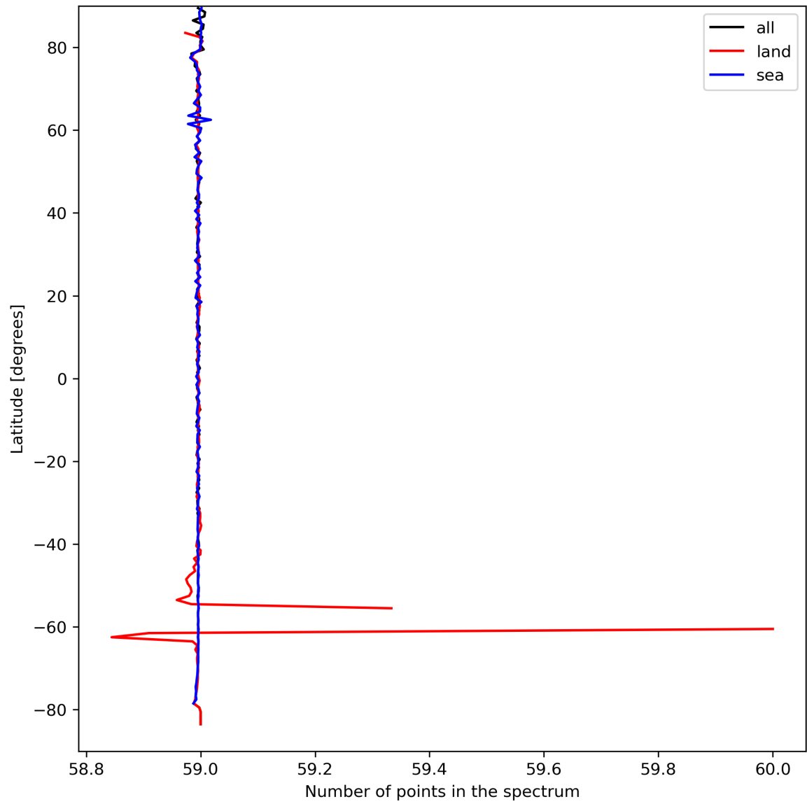
Figure 27: Zonal average of “Number of points in the spectrum” for 2024-03-31 to 2024-04-02.
