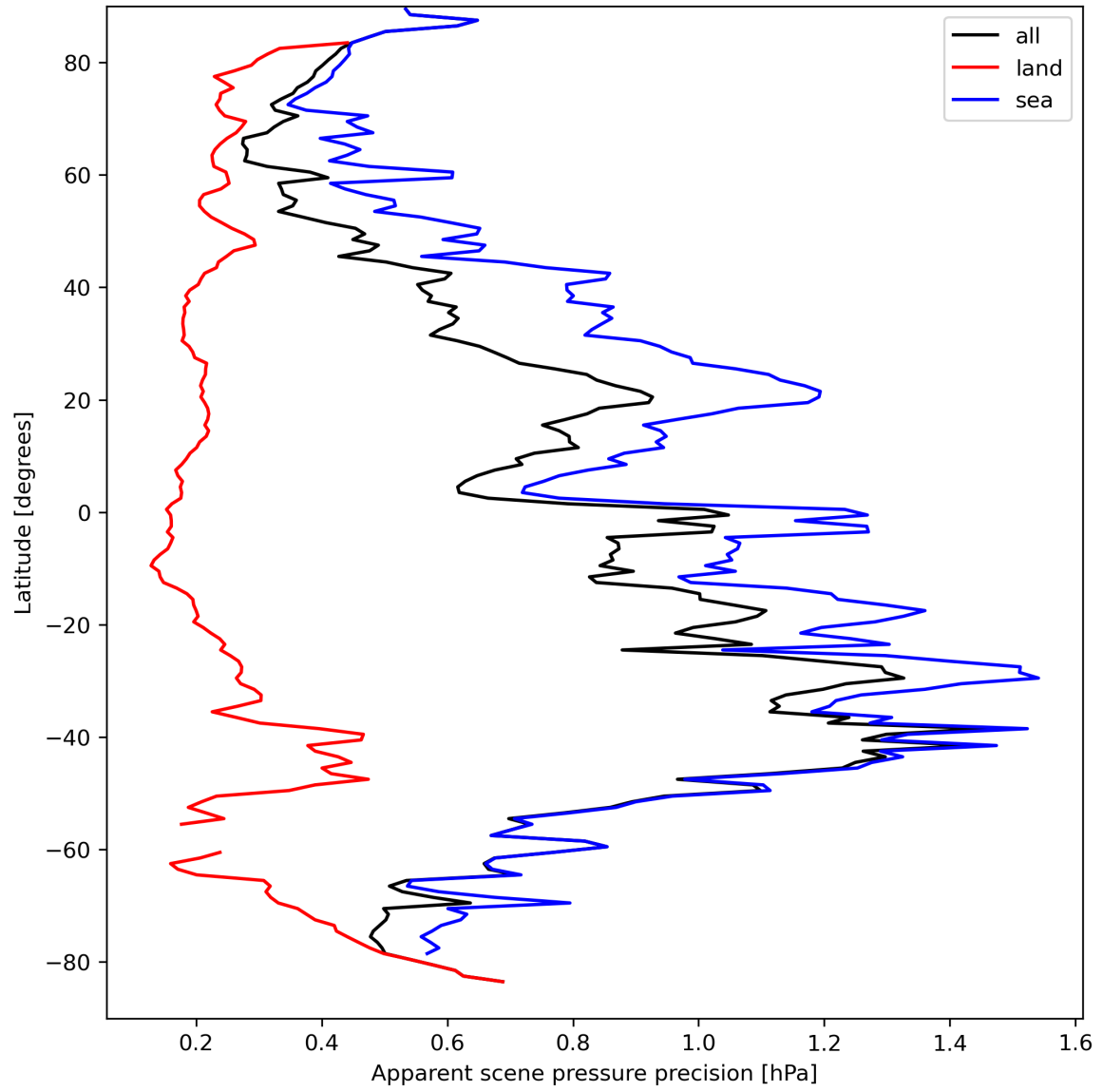
Figure 20: Zonal average of “Apparent scene pressure precision” for 2024-03-31 to 2024-04-02.
