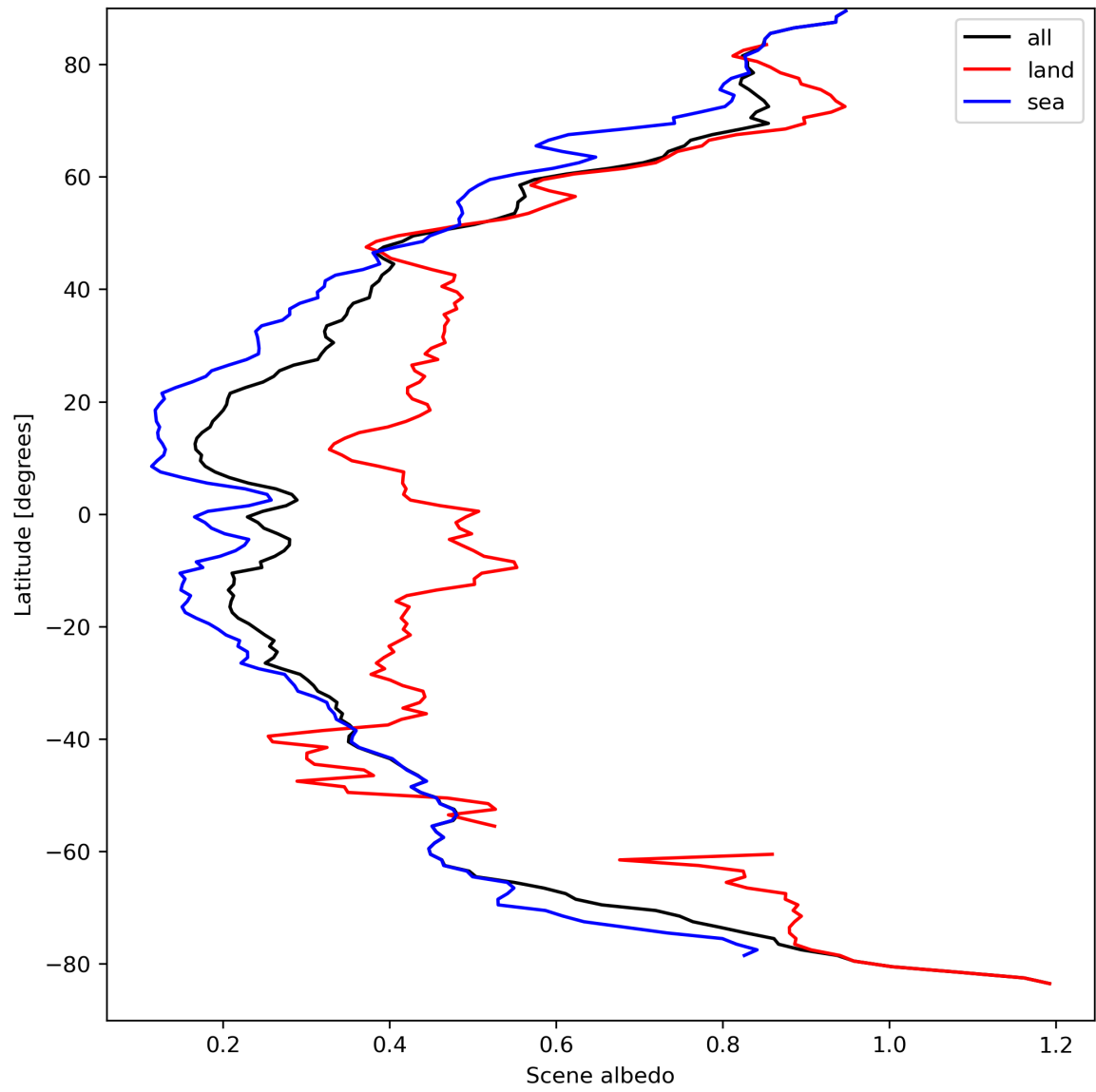
Figure 17: Zonal average of “Scene albedo” for 2024-03-31 to 2024-04-02.
