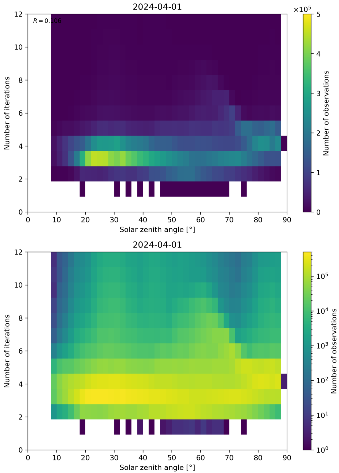
Figure 114: Scatter density plot of “Solar zenith angle” against “Number of iterations” for 2024-03-31 to 2024-04-02.
