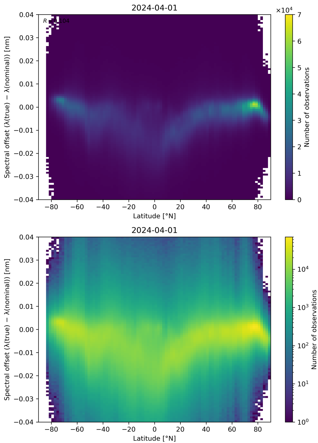
Figure 96: Scatter density plot of “Latitude” against “Spectral offset ( \lambda(\text{true}) - \lambda(\text{nominal}) )” for 2024-03-31 to 2024-04-02.
