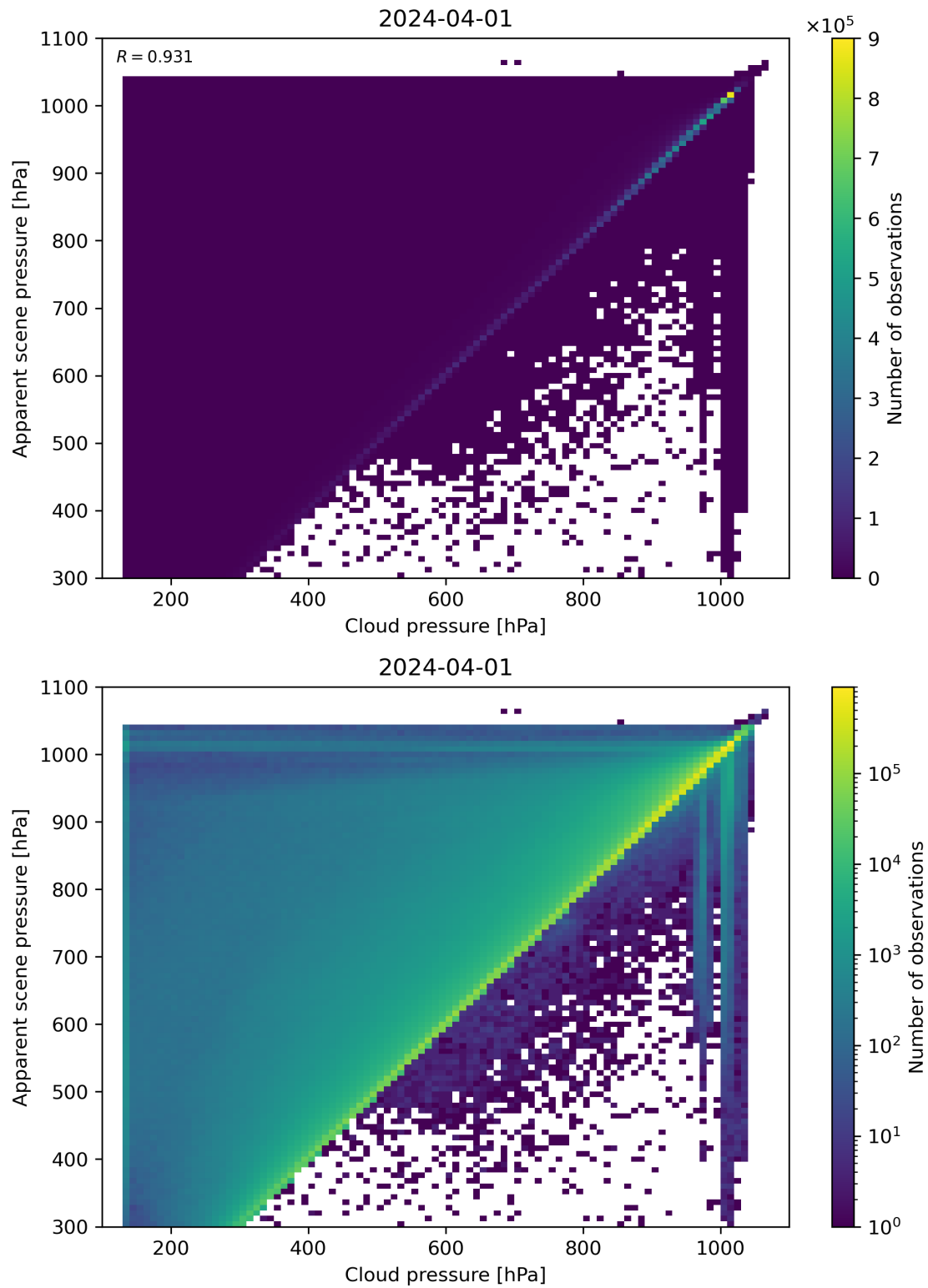
Figure 77: Scatter density plot of “Cloud pressure” against “Apparent scene pressure” for 2024-03-31 to 2024-04-02.
