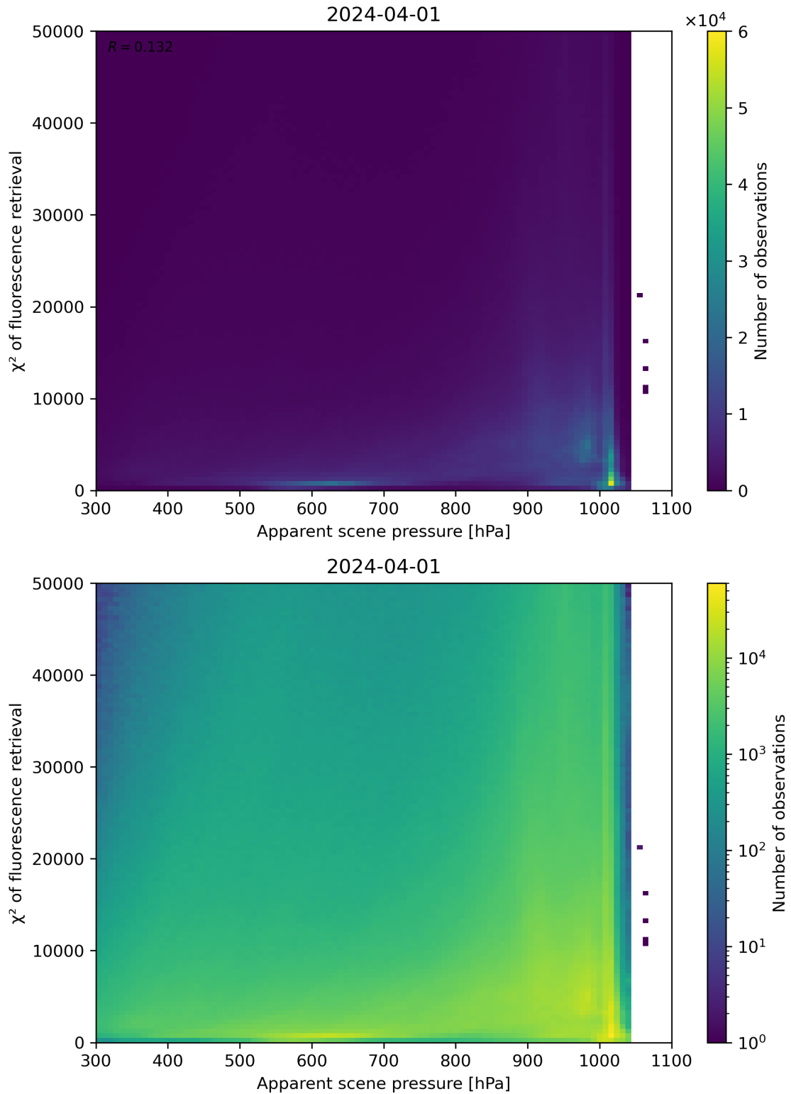
Figure 63: Scatter density plot of “Apparent scene pressure” against “ \chi^2 of fluorescence retrieval” for 2024-03-31 to 2024-04-02.
