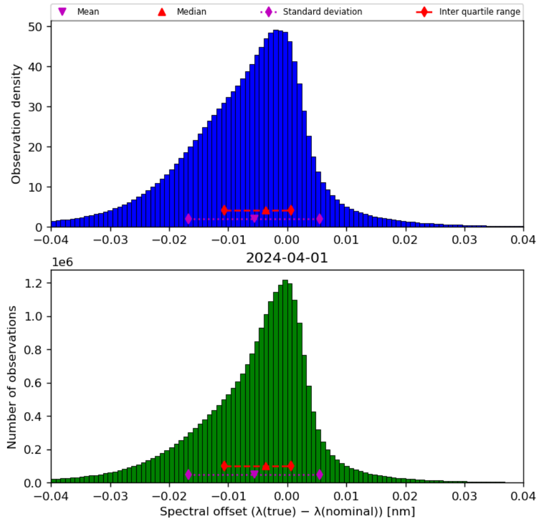
Figure 45: Histogram of “Spectral offset ( \lambda(\text{true}) - \lambda(\text{nominal}) )” for 2024-03-31 to 2024-04-02
