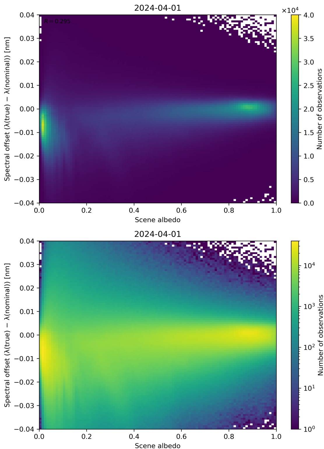
Figure 107: Scatter density plot of “Scene albedo” against “Spectral offset ( \lambda(\text{true}) - \lambda(\text{nominal}) )” for 2024-03-31 to 2024-04-02.
