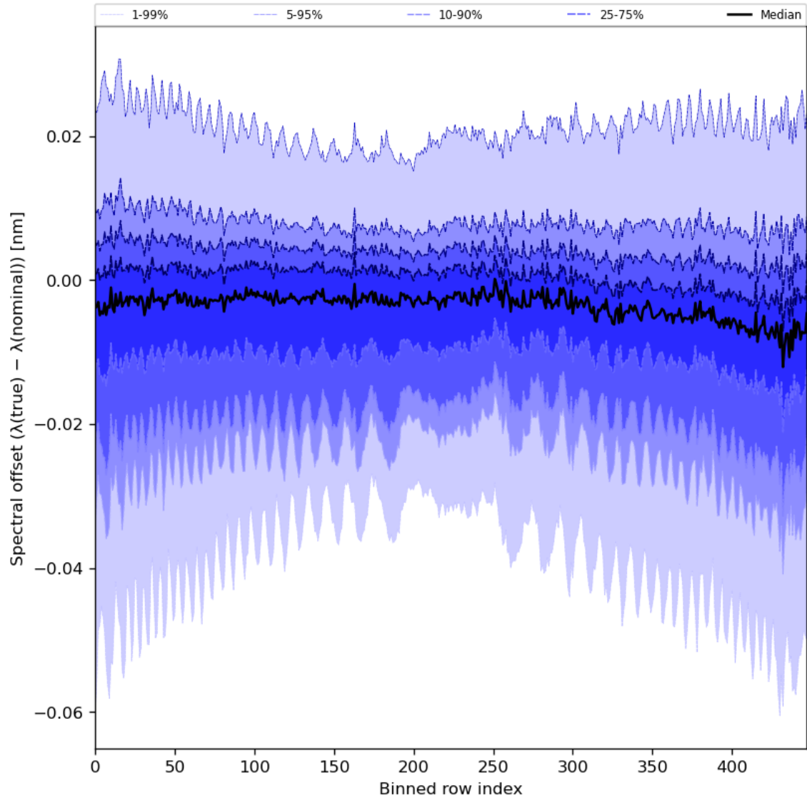
Figure 62: Along track statistics of “Spectral offset ( \lambda(\text{true}) - \lambda(\text{nominal}) )” for 2024-03-31 to 2024-04-02
