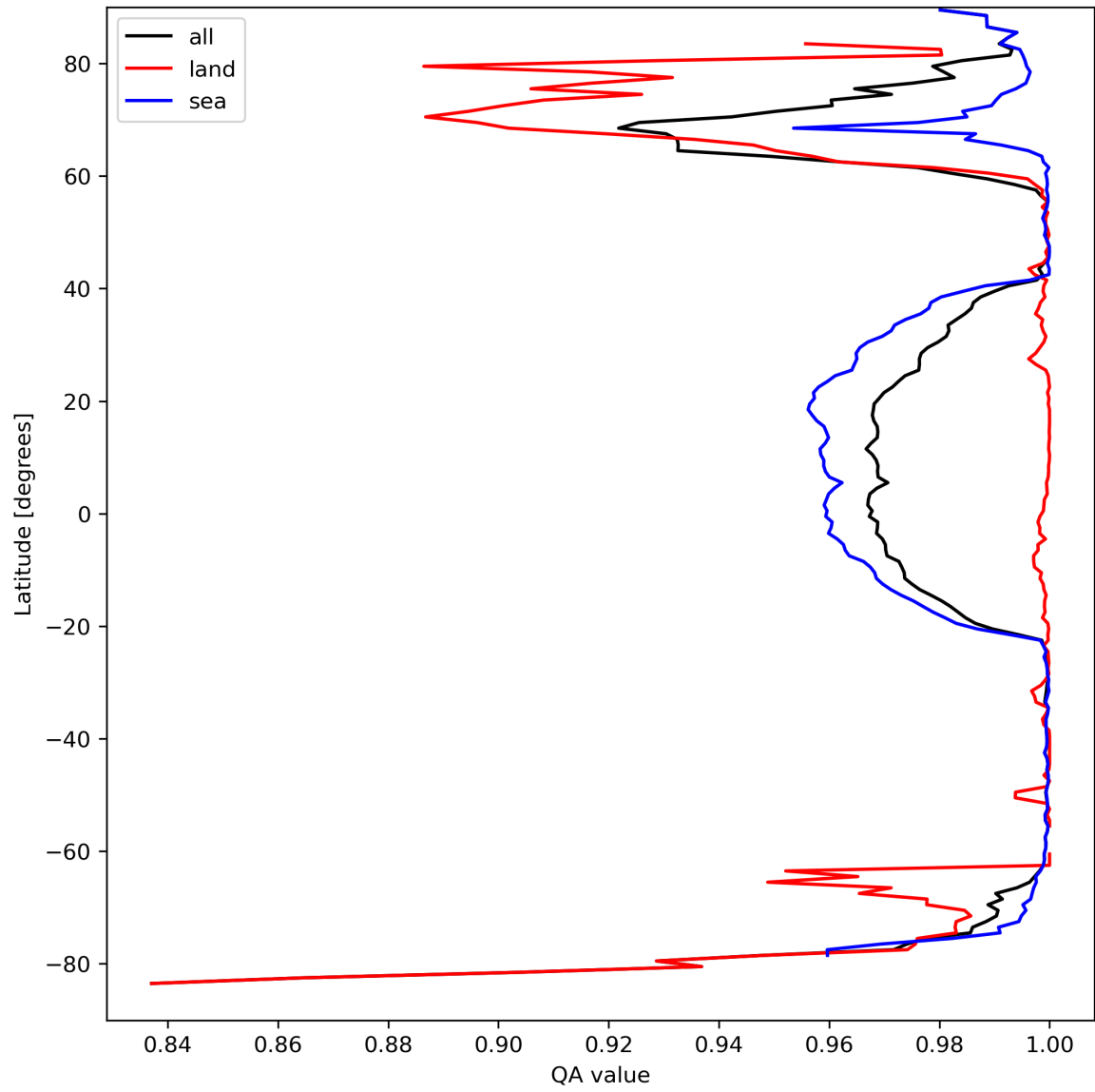
Figure 12: Zonal average of "QA value" for 2024-03-31 to 2024-04-02.
