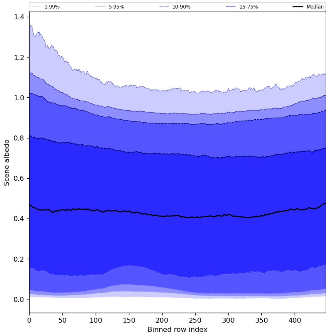
Figure 51: Along track statistics of “Scene albedo” for 2024-03-31 to 2024-04-02
