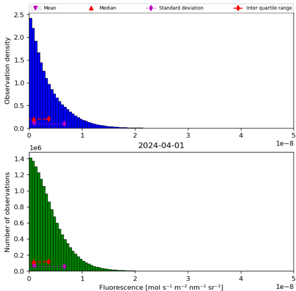
Figure 40: Histogram of “Fluorescence” for 2024-03-31 to 2024-04-02
