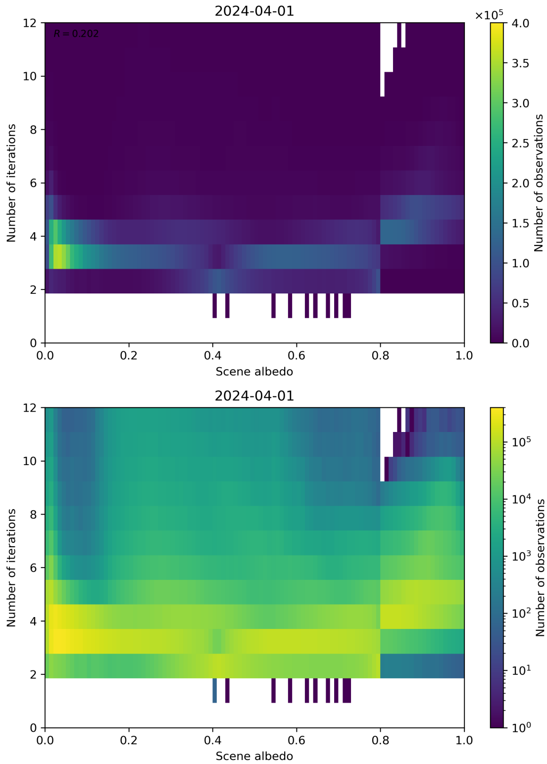
Figure 105: Scatter density plot of “Scene albedo” against “Number of iterations” for 2024-03-31 to 2024-04-02.
