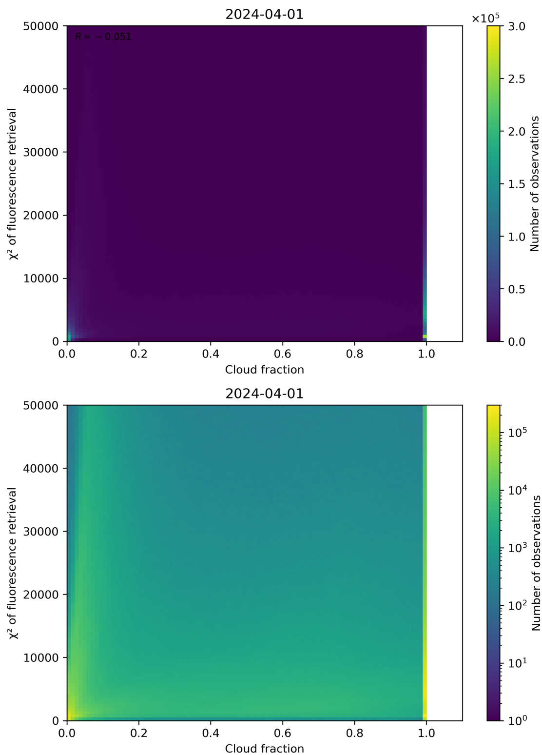
Figure 71: Scatter density plot of “Cloud fraction” against “ \chi^2 of fluorescence retrieval” for 2024-03-31 to 2024-04-02.
