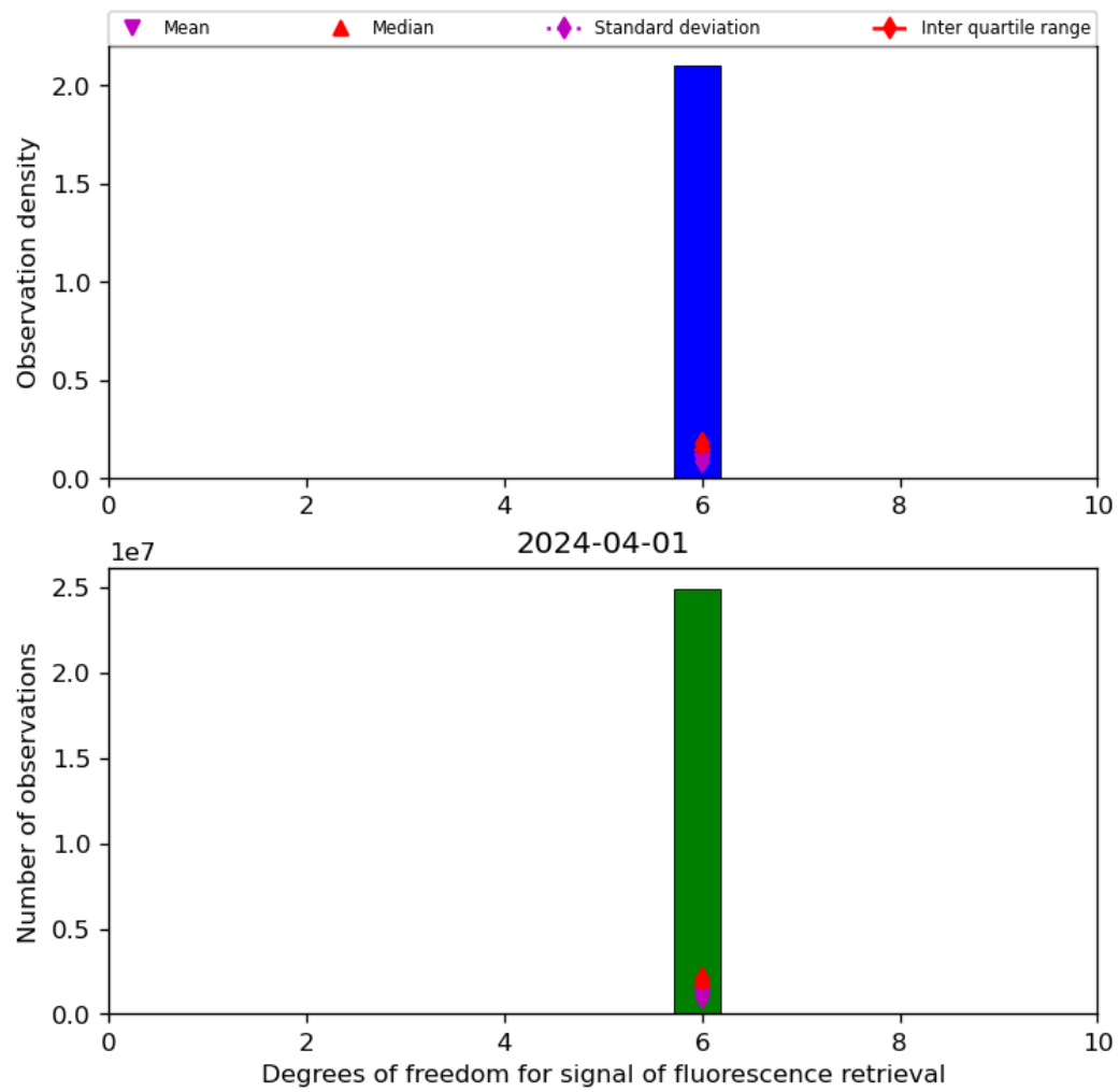
Figure 43: Histogram of “Degrees of freedom for signal of fluorescence retrieval” for 2024-03-31 to 2024-04-02
