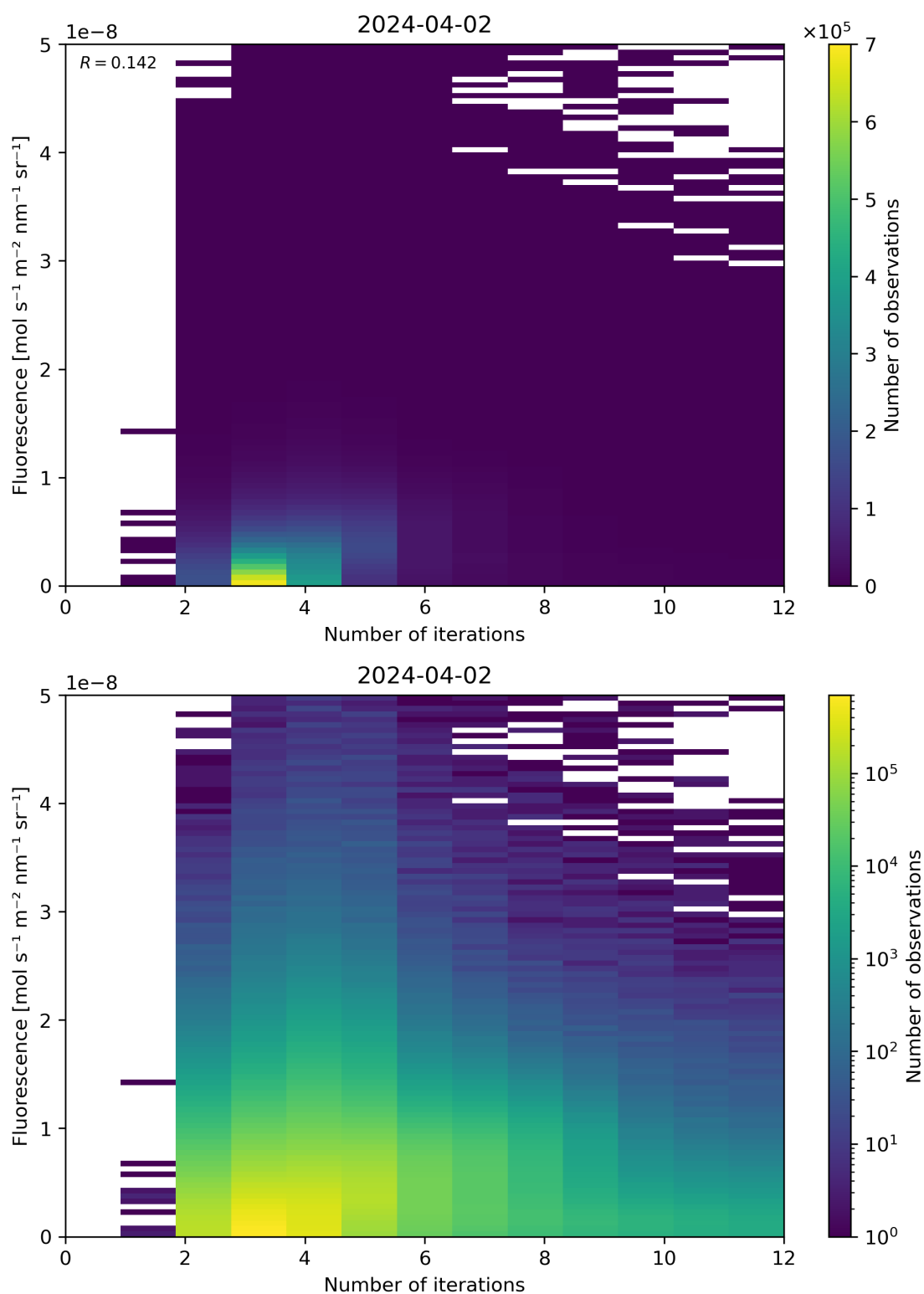
Figure 98: Scatter density plot of “Number of iterations” against “Fluorescence” for 2024-04-01 to 2024-04-03.
