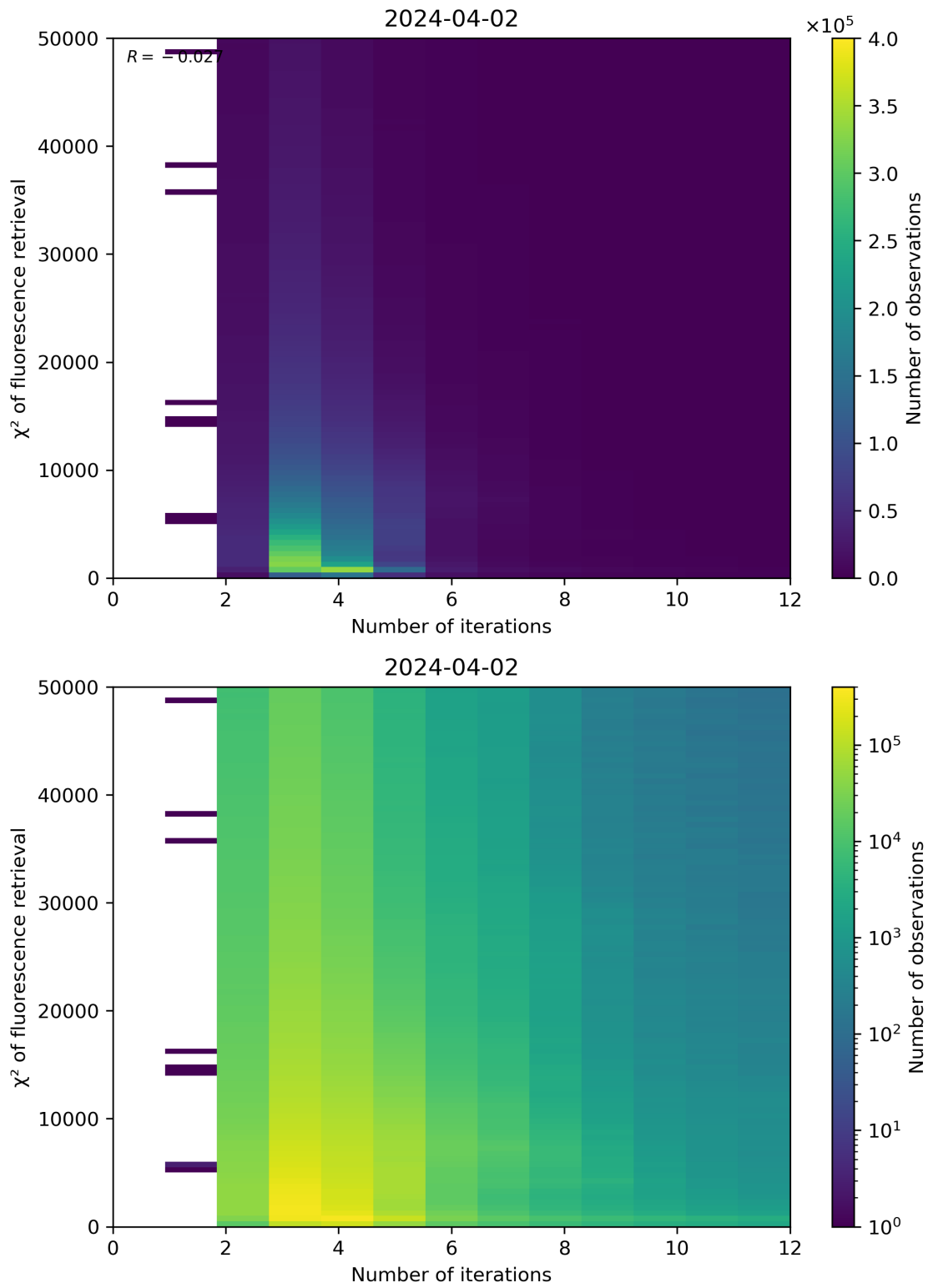
Figure 97: Scatter density plot of “Number of iterations” against “ \chi^2 of fluorescence retrieval” for 2024-04-01 to 2024-04-03.
