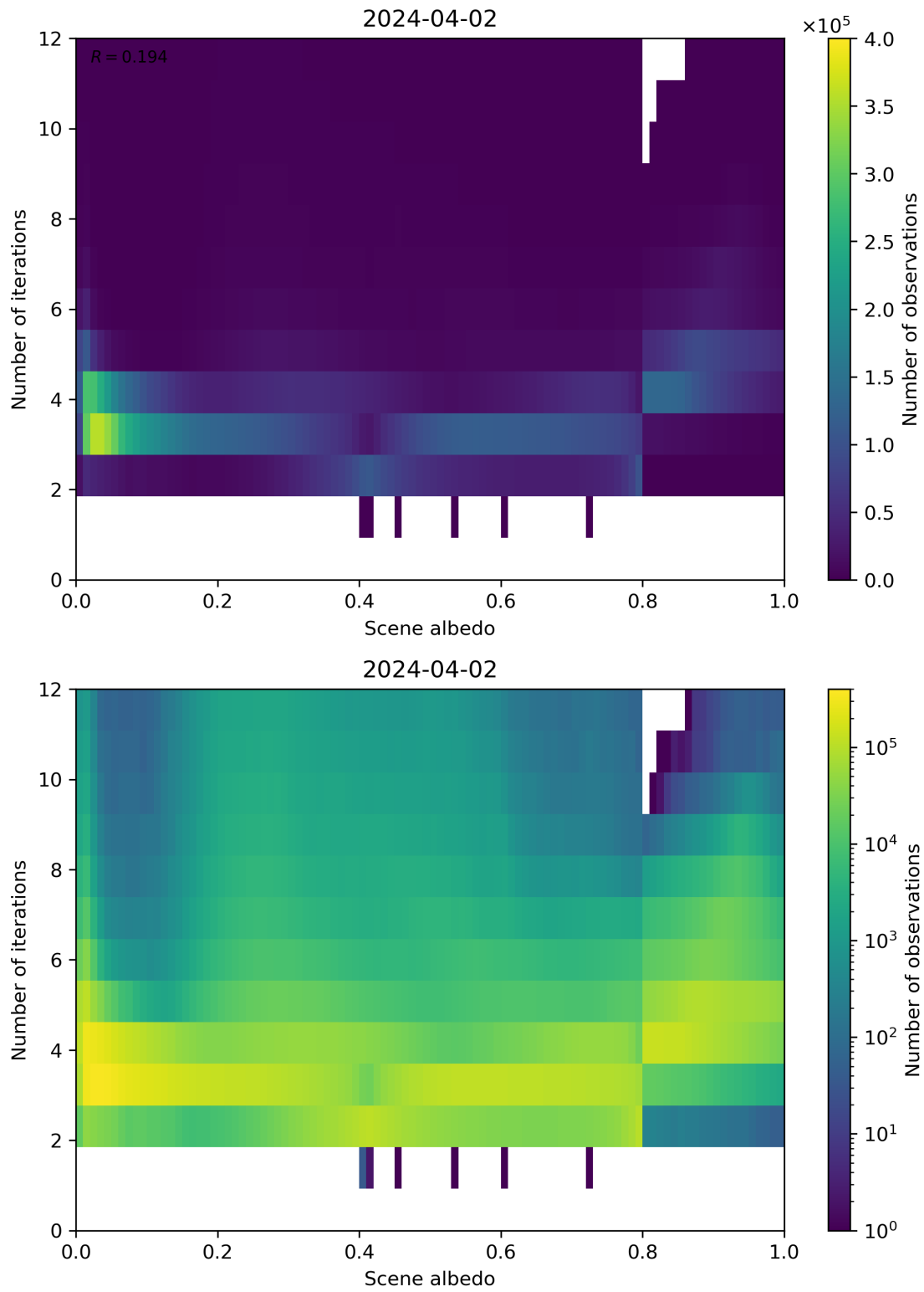
Figure 105: Scatter density plot of “Scene albedo” against “Number of iterations” for 2024-04-01 to 2024-04-03.
