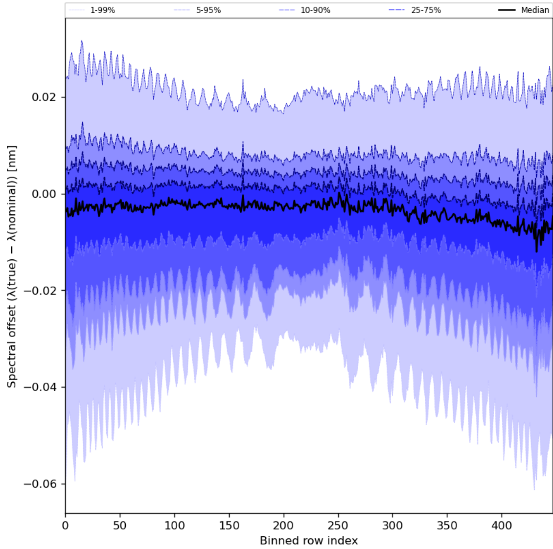
Figure 62: Along track statistics of “Spectral offset ( \lambda(\text{true}) - \lambda(\text{nominal}) )” for 2024-04-01 to 2024-04-03
