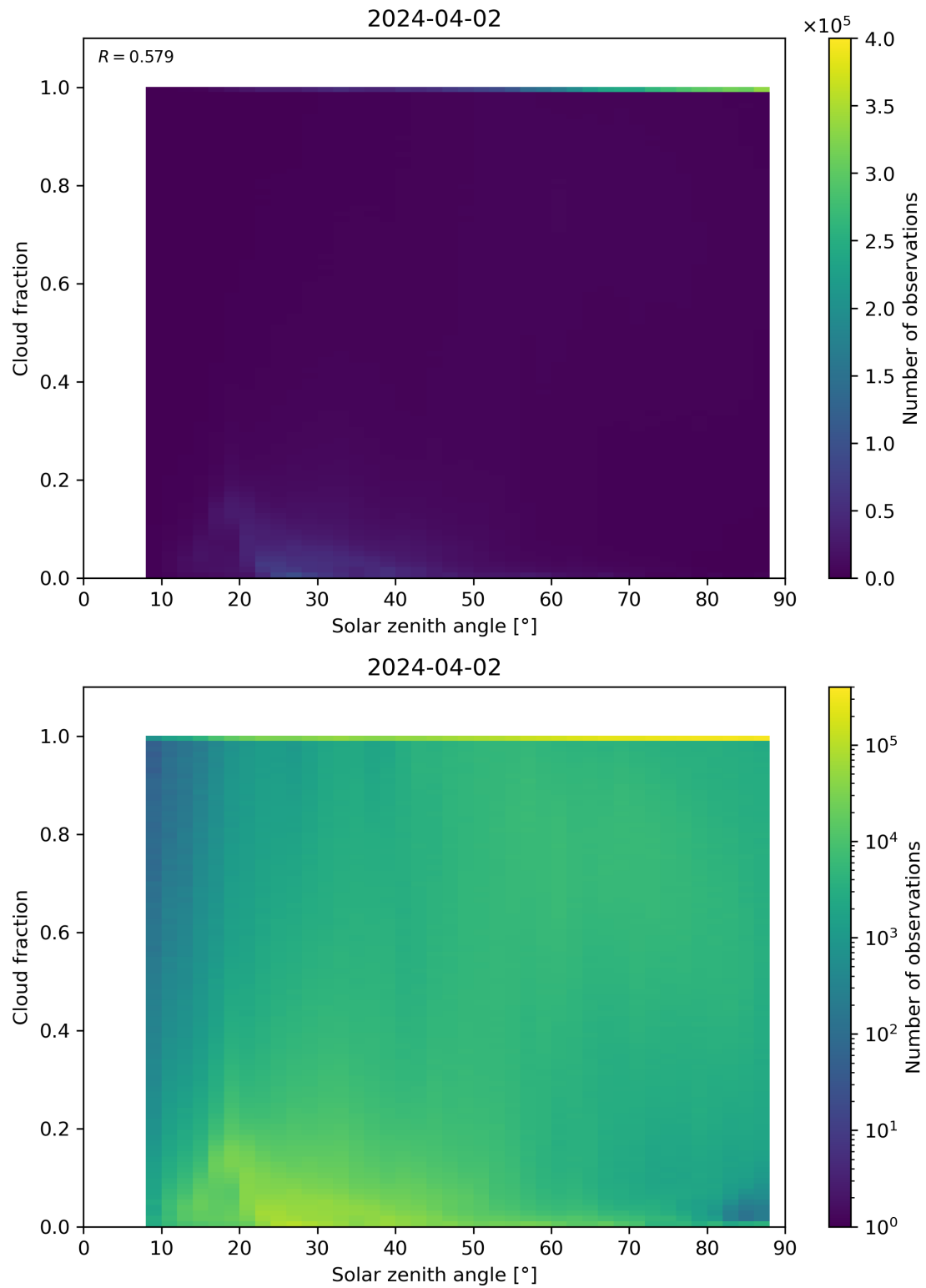
Figure 110: Scatter density plot of “Solar zenith angle” against “Cloud fraction” for 2024-04-01 to 2024-04-03.
