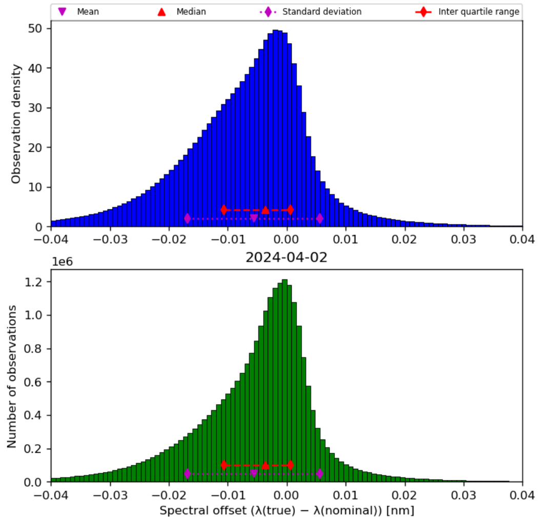
Figure 45: Histogram of “Spectral offset ( \lambda(\text{true}) - \lambda(\text{nominal}) )” for 2024-04-01 to 2024-04-03
