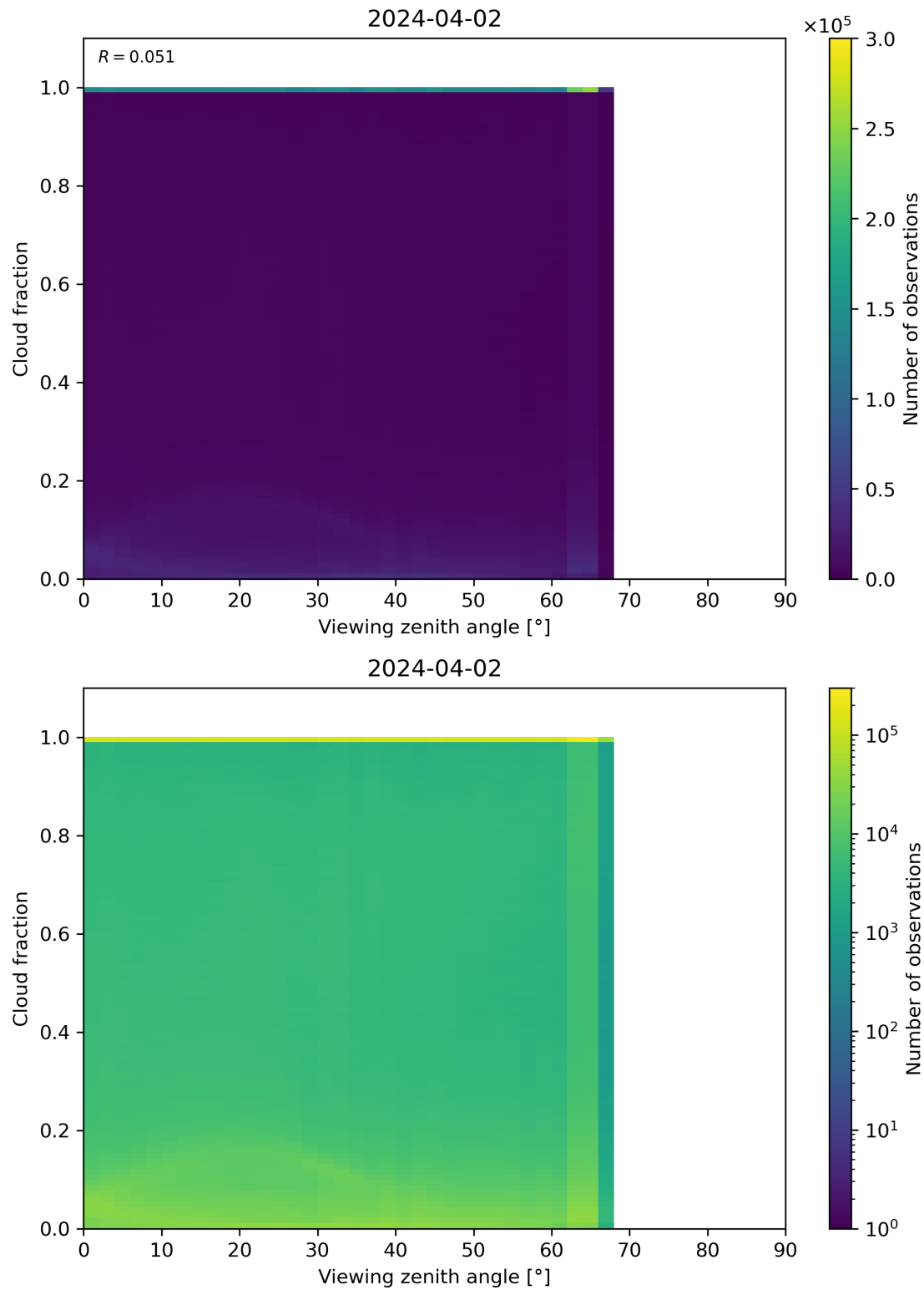
Figure 120: Scatter density plot of “Viewing zenith angle” against “Cloud fraction” for 2024-04-01 to 2024-04-03.
