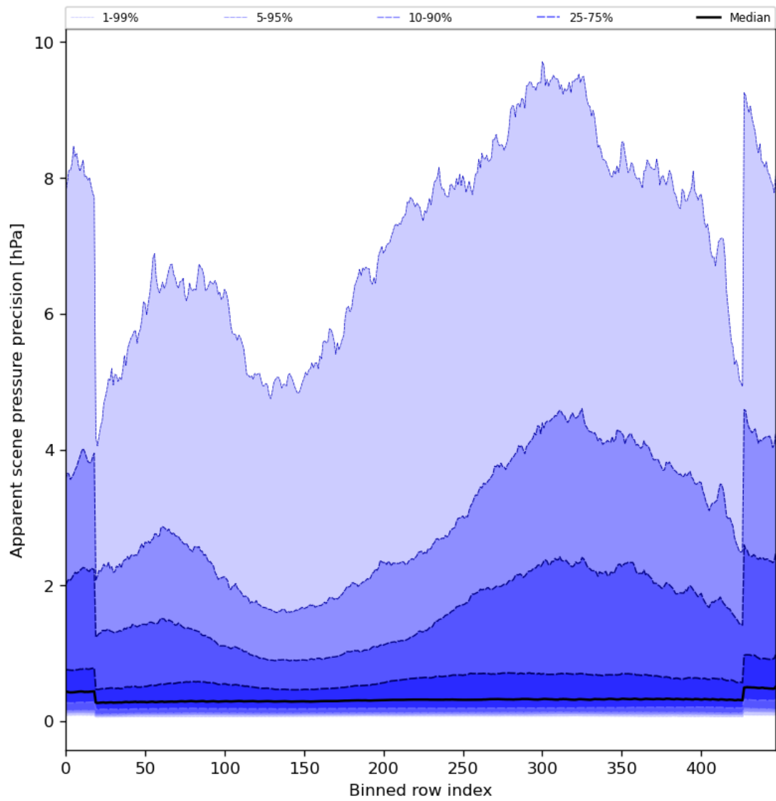
Figure 54: Along track statistics of “Apparent scene pressure precision” for 2024-04-01 to 2024-04-03
