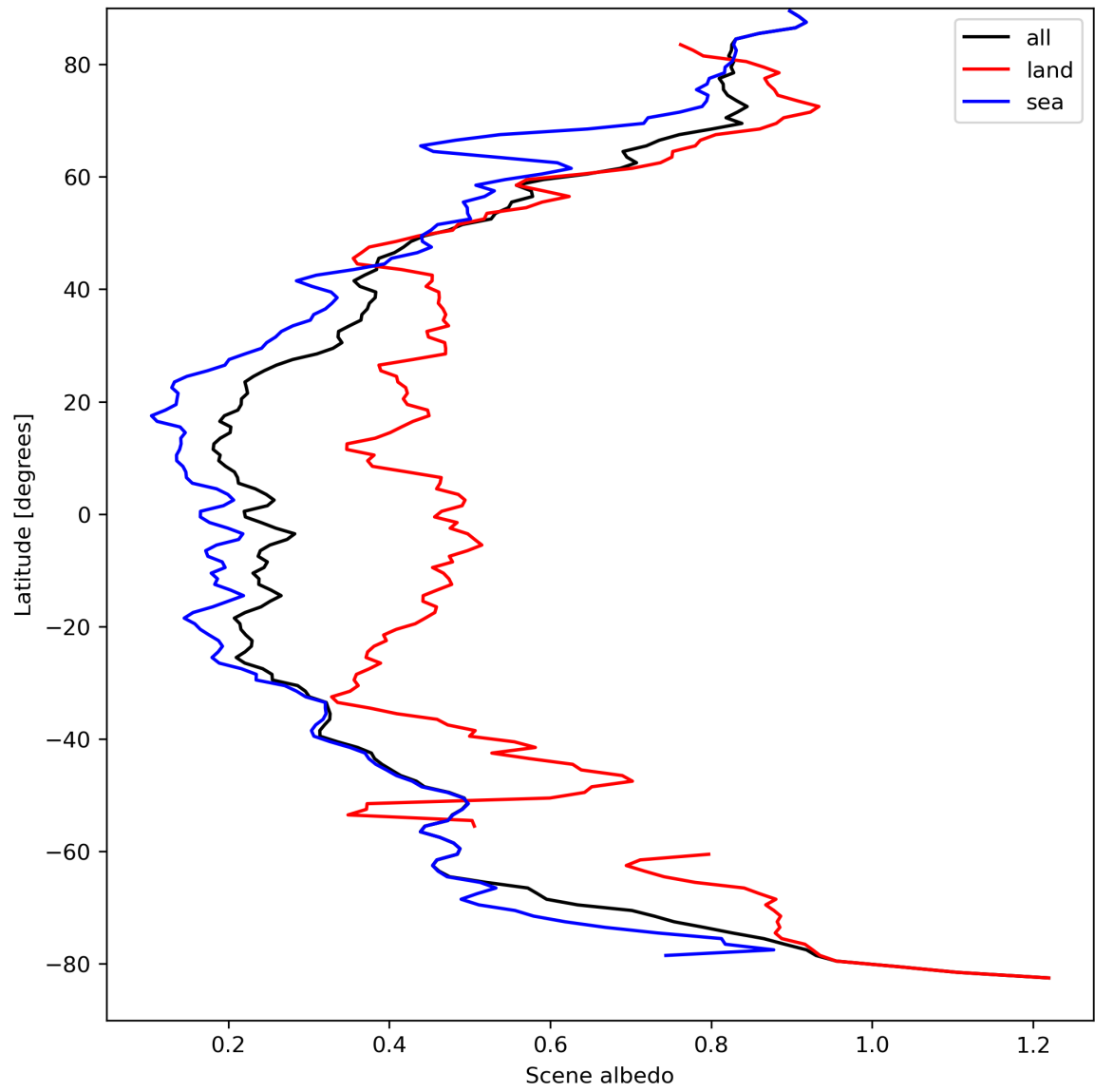
Figure 17: Zonal average of “Scene albedo” for 2024-04-01 to 2024-04-03.
