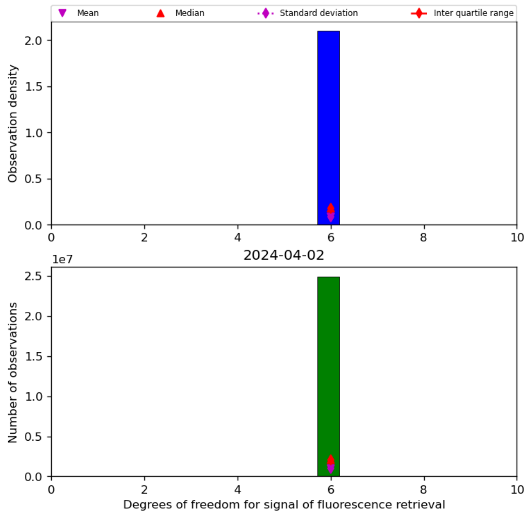
Figure 43: Histogram of “Degrees of freedom for signal of fluorescence retrieval” for 2024-04-01 to 2024-04-03
