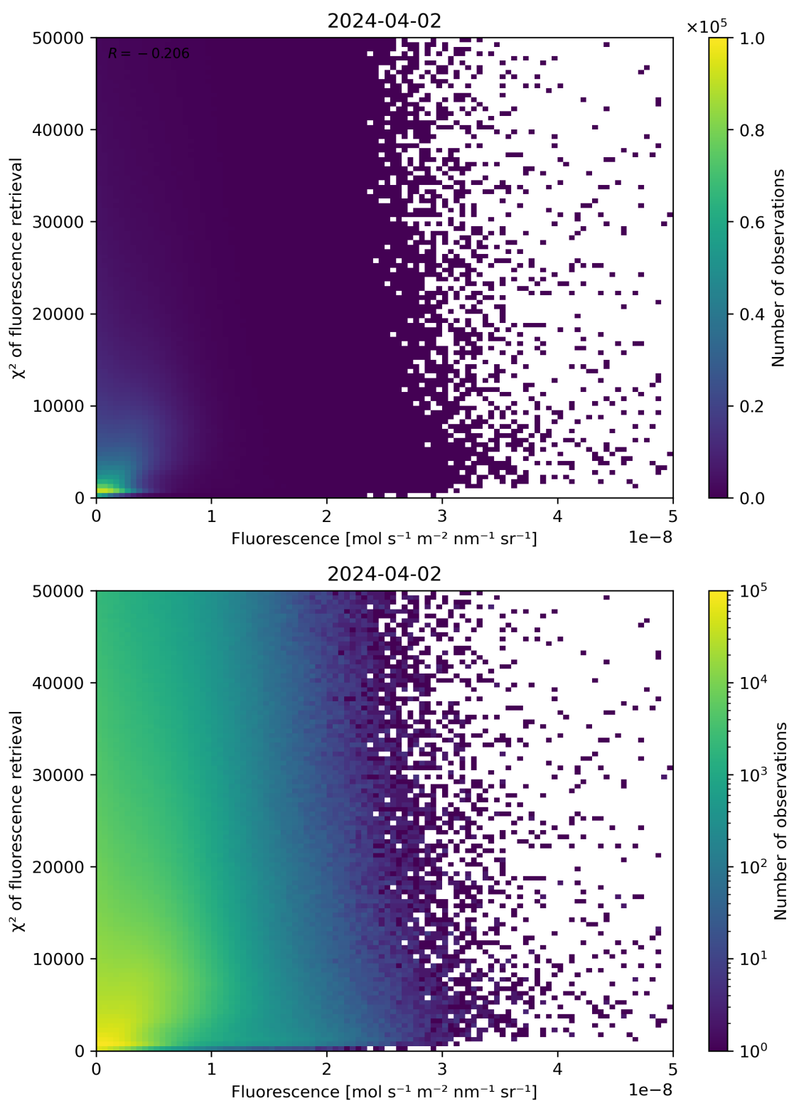
Figure 85: Scatter density plot of “Fluorescence” against “ \chi^2 of fluorescence retrieval” for 2024-04-01 to 2024-04-03.
