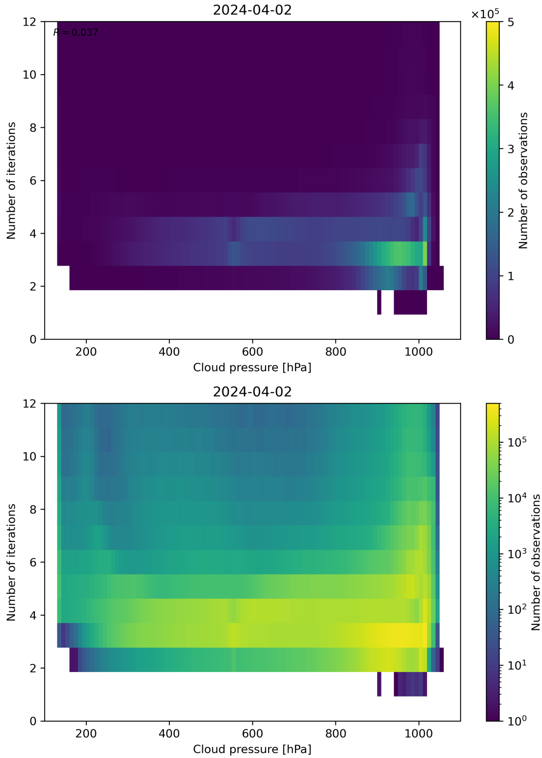
Figure 81: Scatter density plot of “Cloud pressure” against “Number of iterations” for 2024-04-01 to 2024-04-03.
