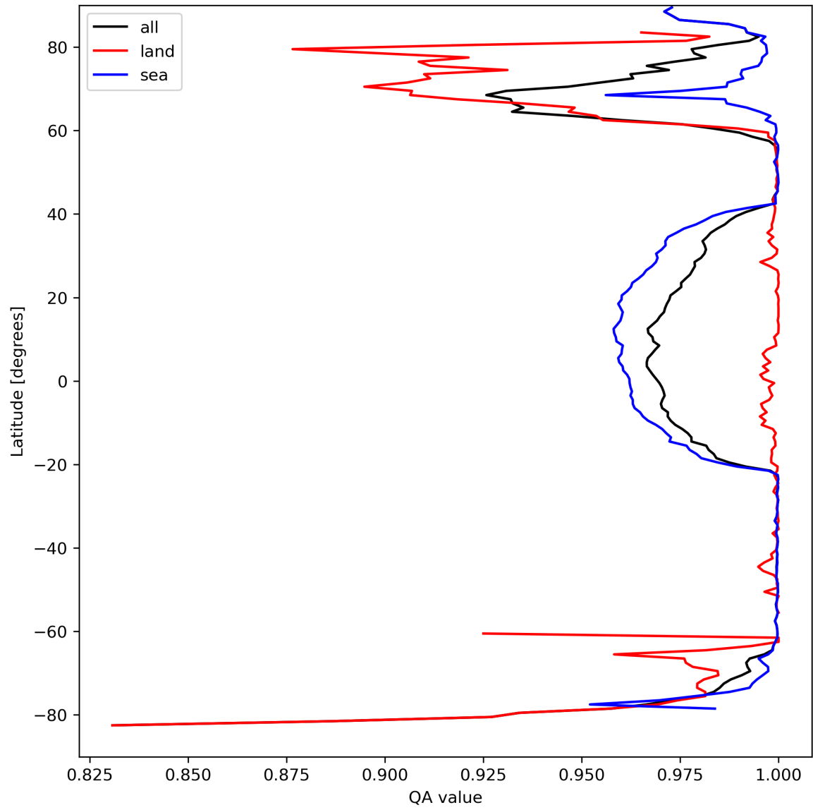
Figure 12: Zonal average of “QA value” for 2024-04-01 to 2024-04-03.
