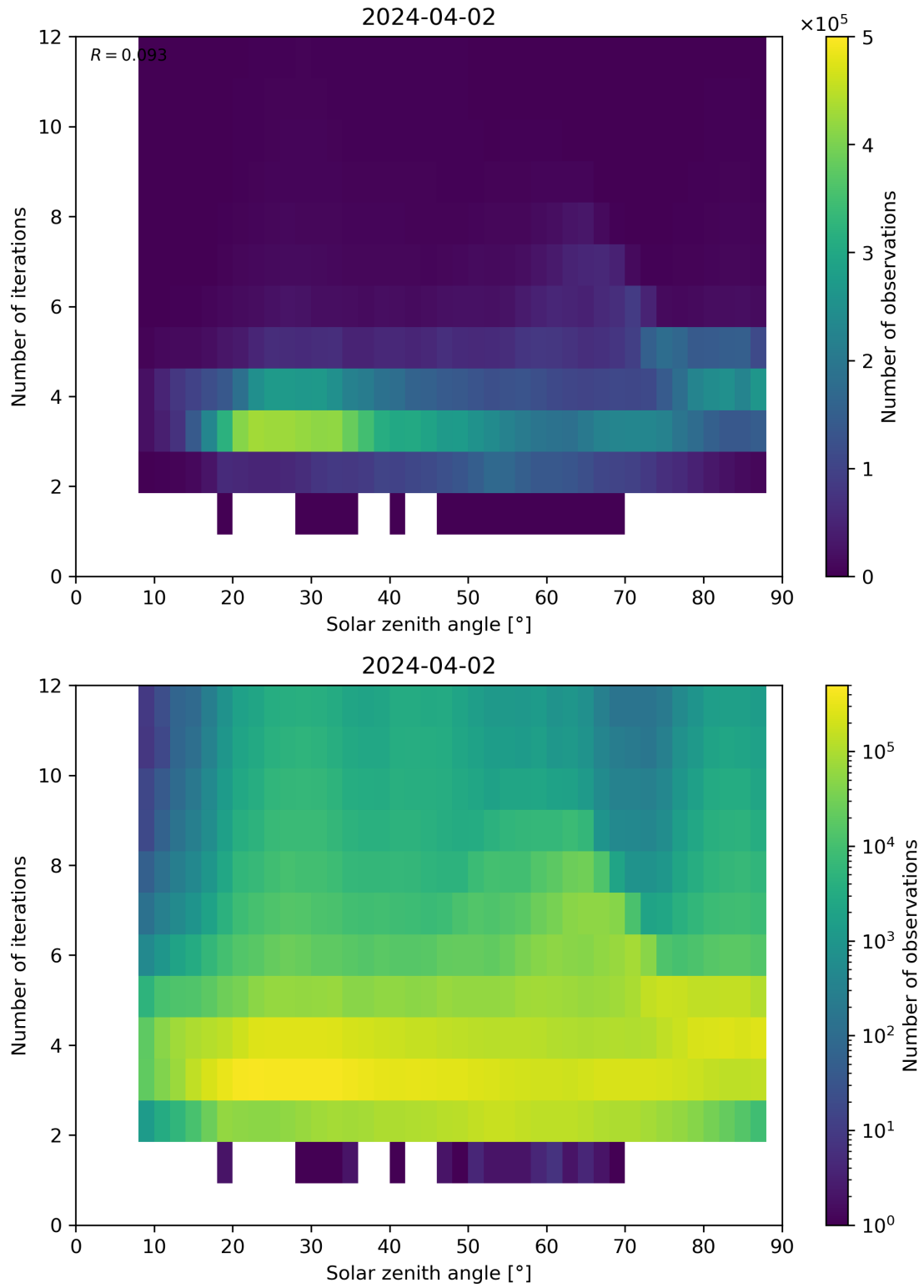
Figure 114: Scatter density plot of “Solar zenith angle” against “Number of iterations” for 2024-04-01 to 2024-04-03.
