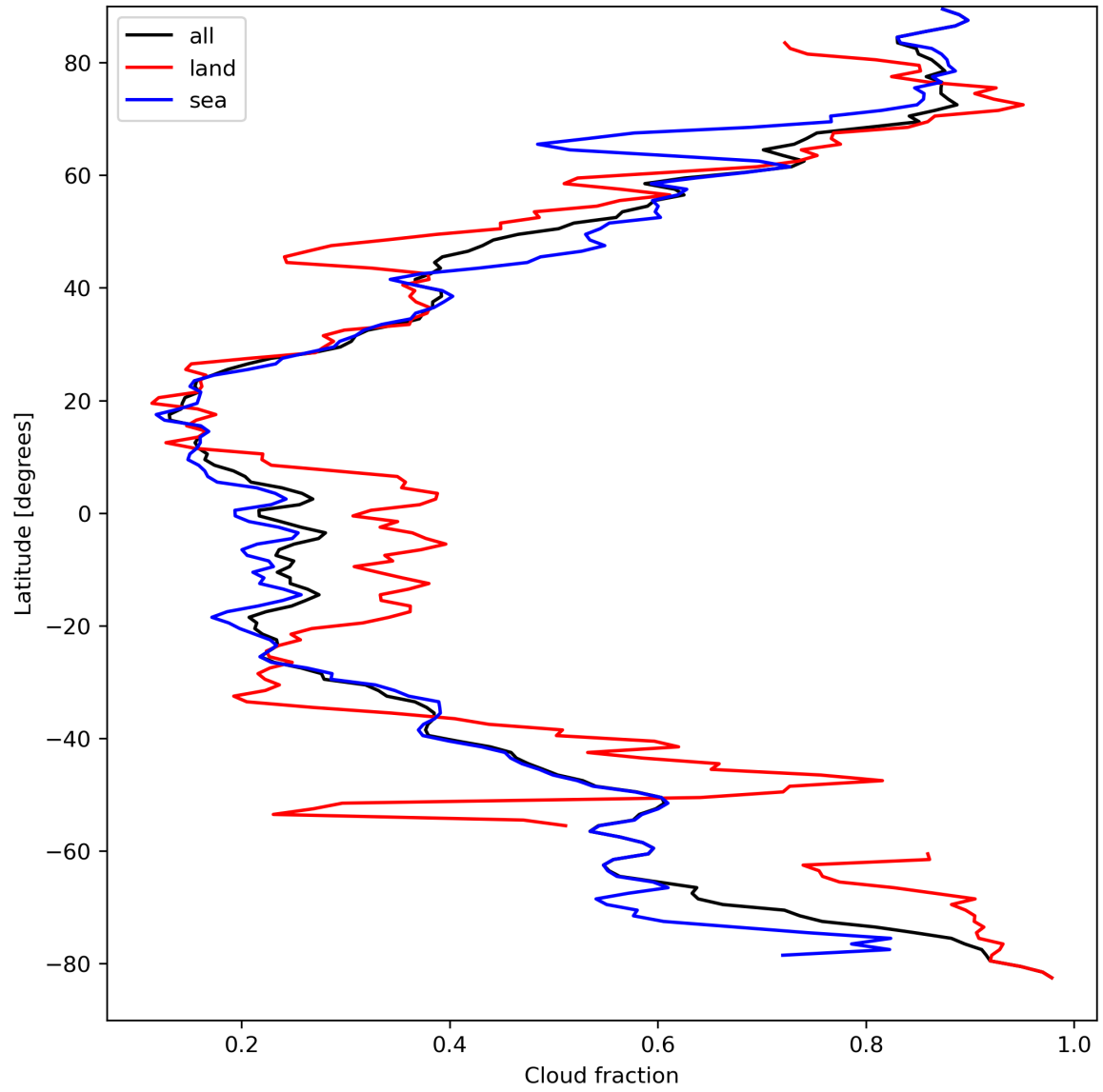
Figure 15: Zonal average of “Cloud fraction” for 2024-04-01 to 2024-04-03.
