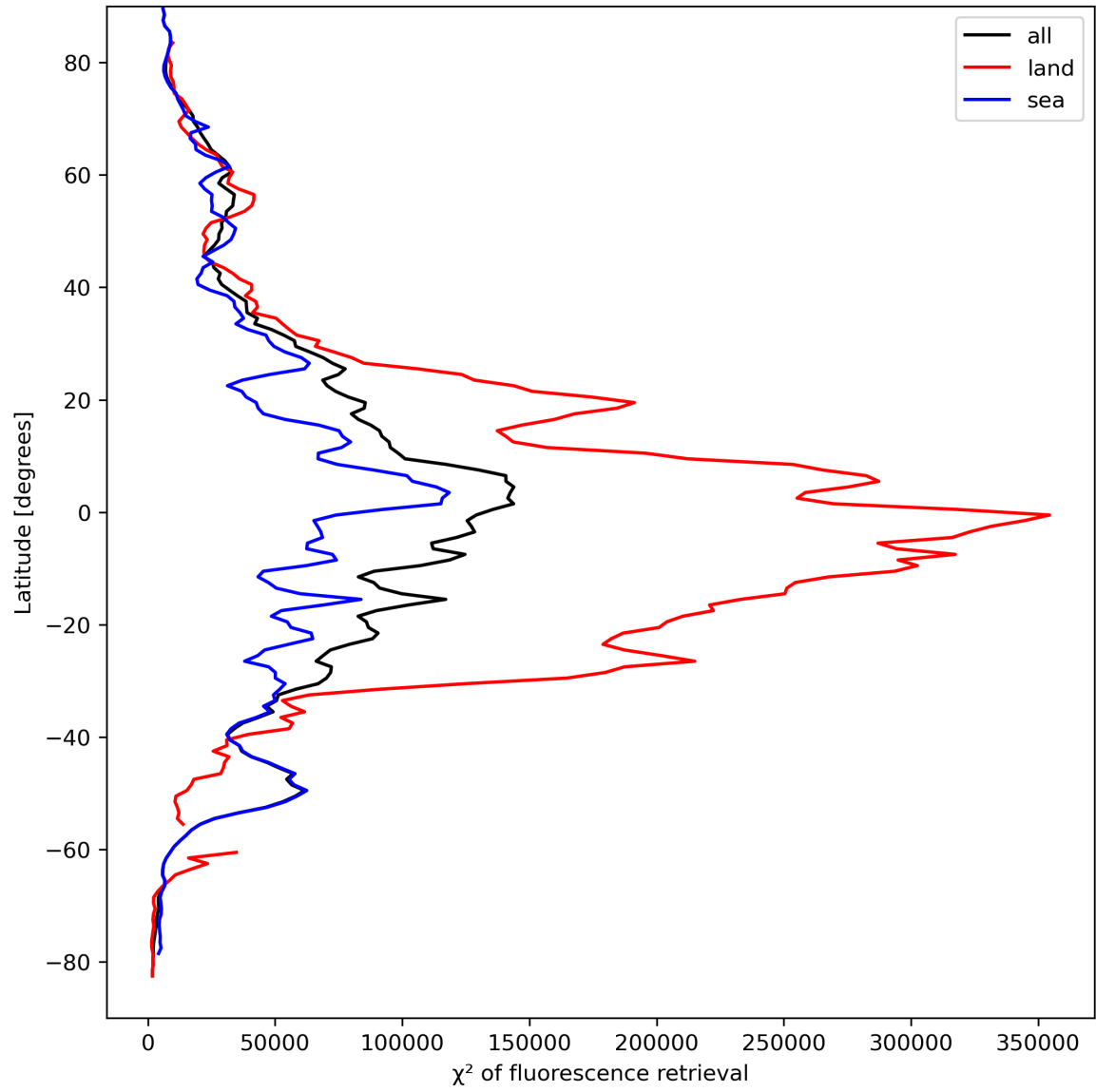
Figure 25: Zonal average of “ \chi^2 of fluorescence retrieval” for 2024-04-01 to 2024-04-03.
