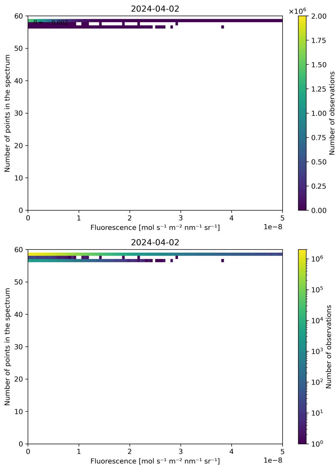
Figure 86: Scatter density plot of “Fluorescence” against “Number of points in the spectrum” for 2024-04-01 to 2024-04-03.
