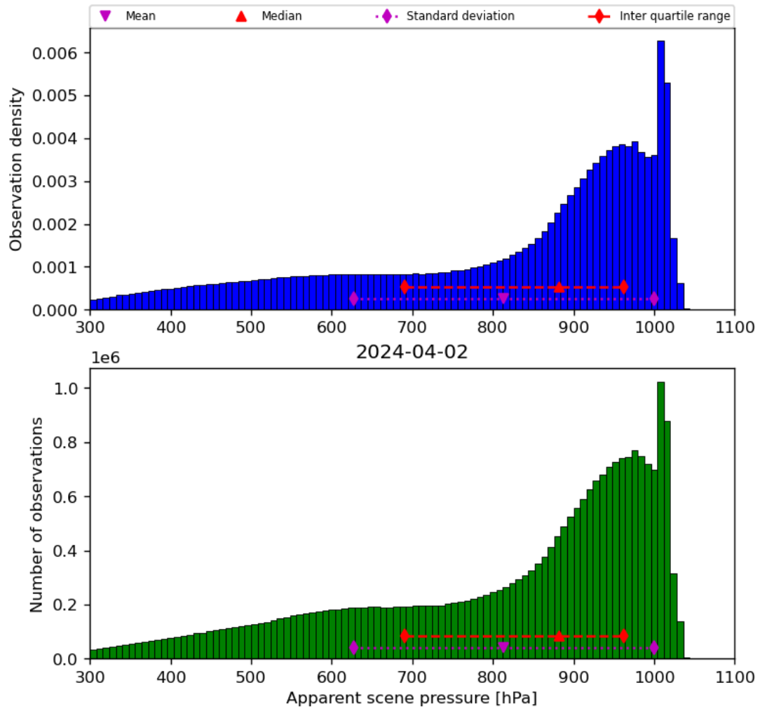
Figure 36: Histogram of “Apparent scene pressure” for 2024-04-01 to 2024-04-03
