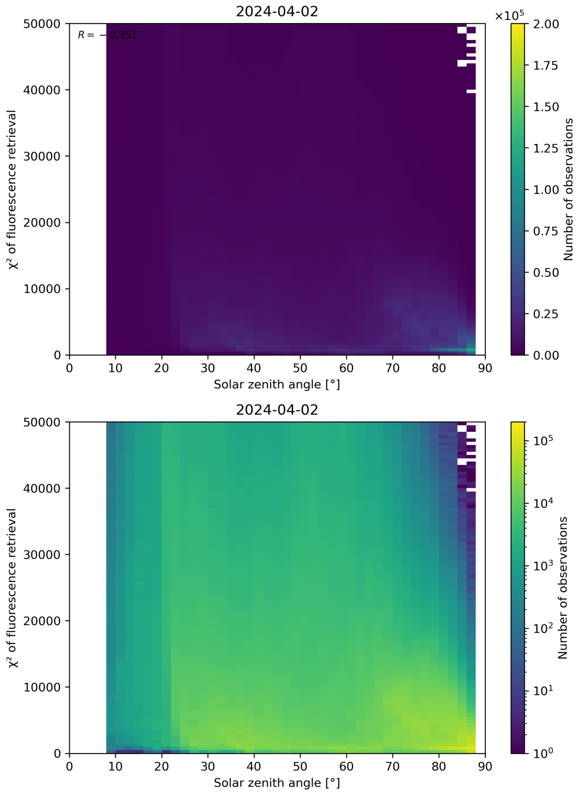
Figure 109: Scatter density plot of “Solar zenith angle” against “ \chi^2 of fluorescence retrieval” for 2024-04-01 to 2024-04-03.
