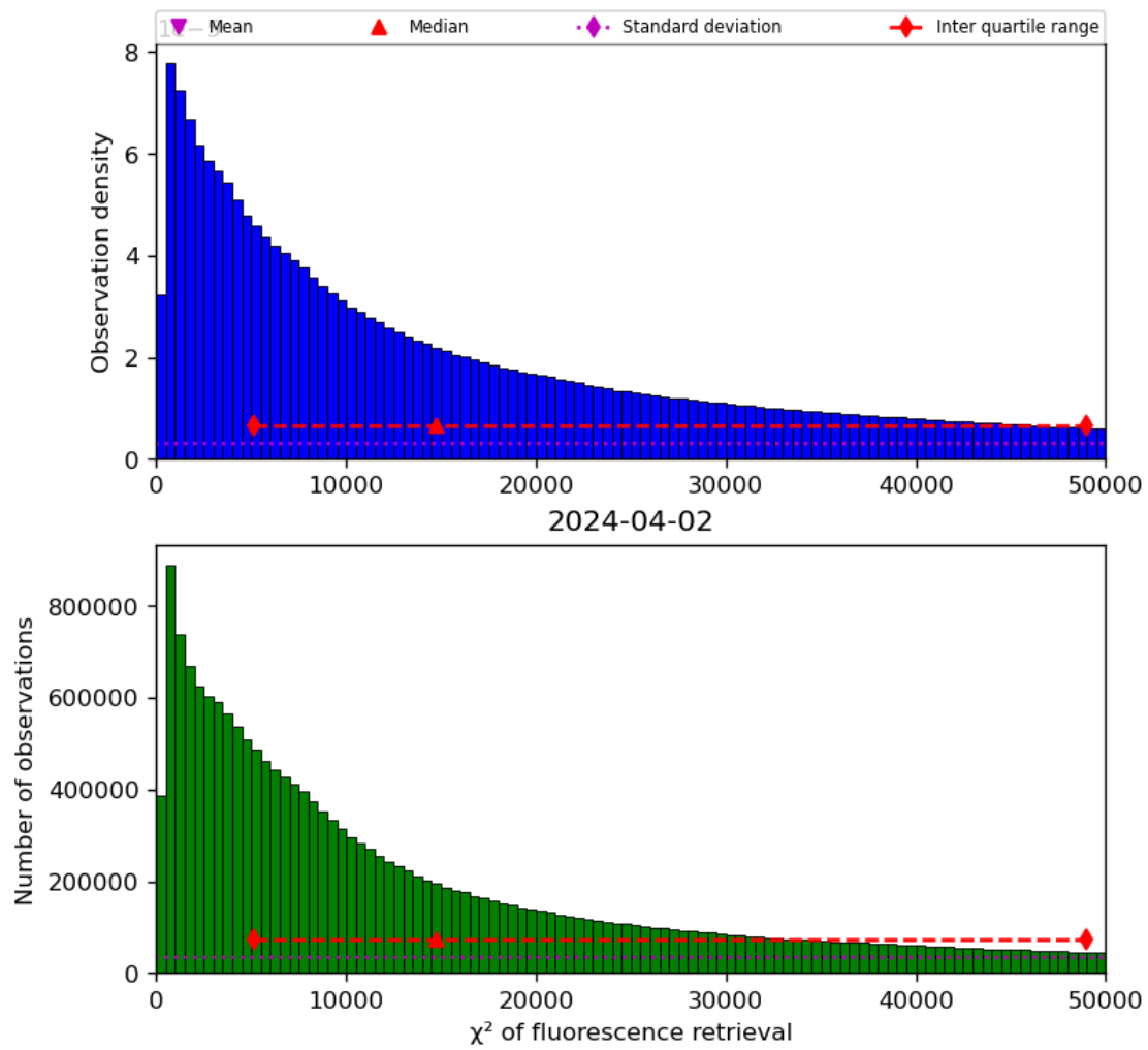
Figure 42: Histogram of “ \chi^2 of fluorescence retrieval” for 2024-04-01 to 2024-04-03
