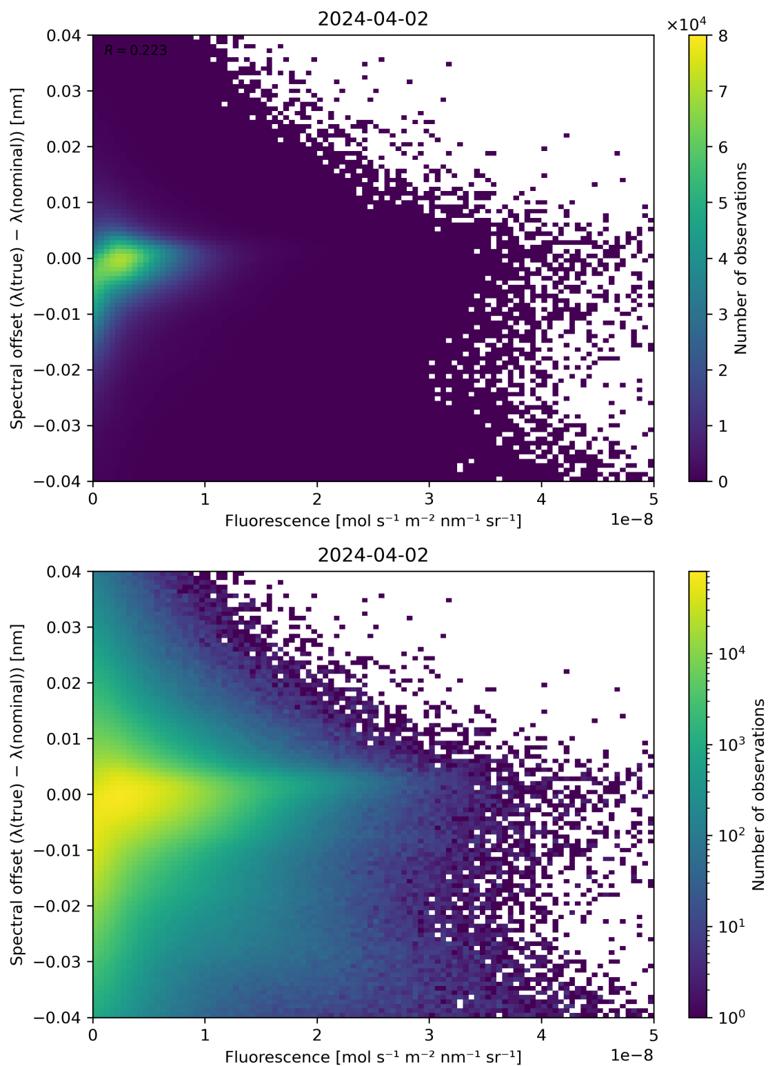
Figure 87: Scatter density plot of “Fluorescence” against “Spectral offset ( \lambda(\text{true}) - \lambda(\text{nominal}) )” for 2024-04-01 to 2024-04-03.
