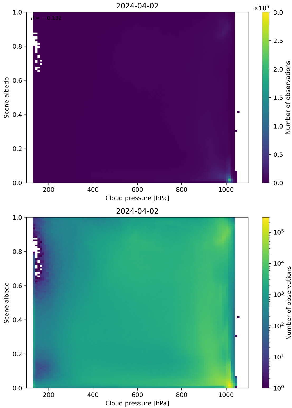
Figure 83: Scatter density plot of “Cloud pressure” against “Scene albedo” for 2024-04-01 to 2024-04-03.
