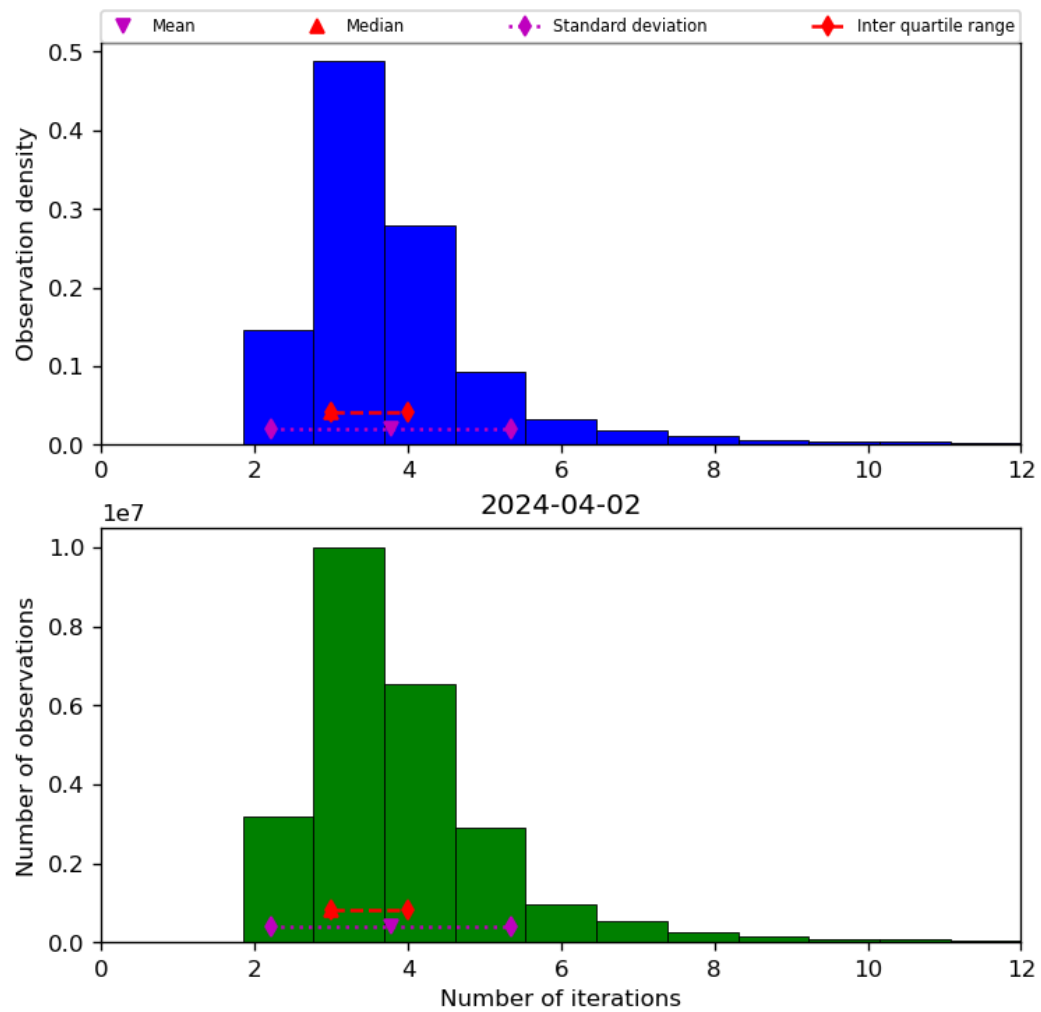
Figure 39: Histogram of “Number of iterations” for 2024-04-01 to 2024-04-03
