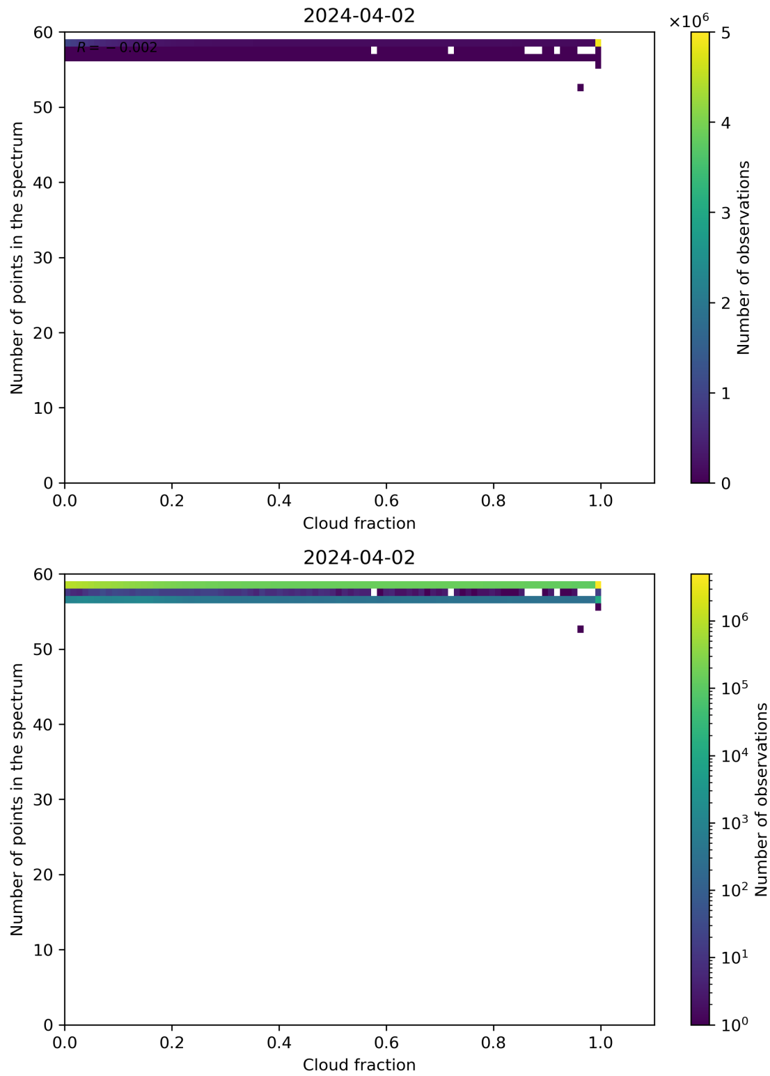
Figure 74: Scatter density plot of “Cloud fraction” against “Number of points in the spectrum” for 2024-04-01 to 2024-04-03.
