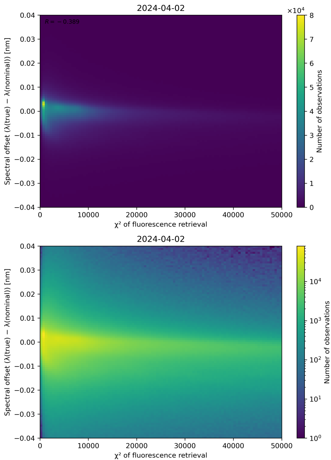
Figure 69: Scatter density plot of " \chi^2 of fluorescence retrieval" against "Spectral offset ( \lambda(\text{true}) - \lambda(\text{nominal})) " for 2024-04-01 to 2024-04-03.
