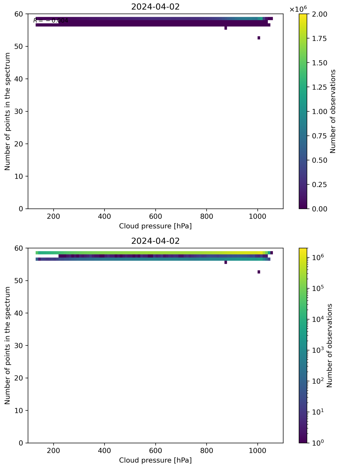
Figure 82: Scatter density plot of “Cloud pressure” against “Number of points in the spectrum” for 2024-04-01 to 2024-04-03.
