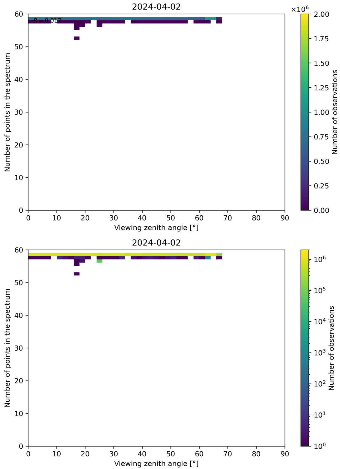
Figure 125: Scatter density plot of “Viewing zenith angle” against “Number of points in the spectrum” for 2024-04-01 to 2024-04-03.
