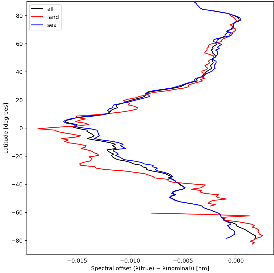
Figure 28: Zonal average of “Spectral offset ( \lambda(\text{true}) - \lambda(\text{nominal}) )” for 2024-04-01 to 2024-04-03.
