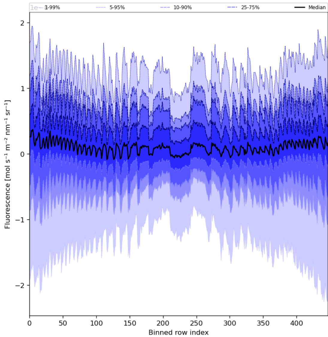
Figure 57: Along track statistics of “Fluorescence” for 2024-04-01 to 2024-04-03
