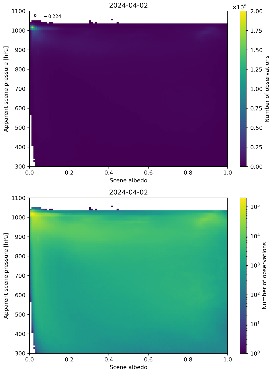
Figure 102: Scatter density plot of “Scene albedo” against “Apparent scene pressure” for 2024-04-01 to 2024-04-03.
