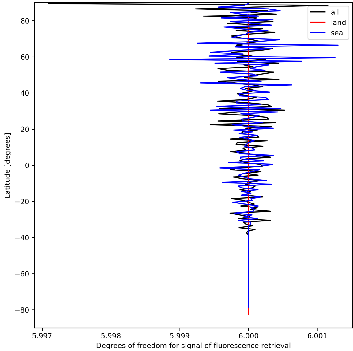
Figure 26: Zonal average of “Degrees of freedom for signal of fluorescence retrieval” for 2024-04-01 to 2024-04-03.
