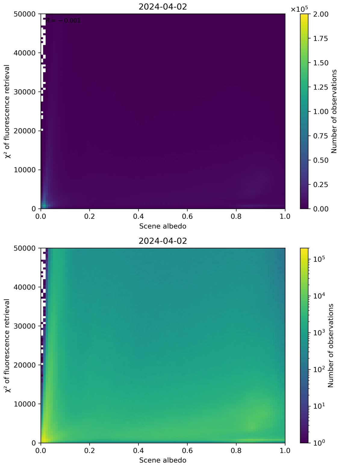
Figure 103: Scatter density plot of “Scene albedo” against “ \chi^2 of fluorescence retrieval” for 2024-04-01 to 2024-04-03.
