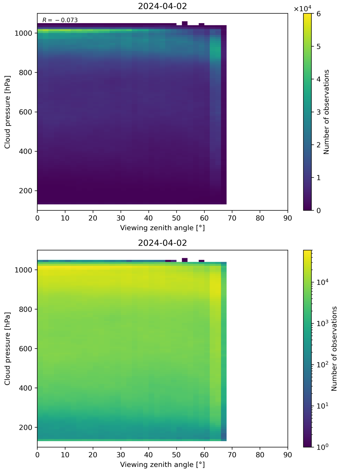
Figure 121: Scatter density plot of “Viewing zenith angle” against “Cloud pressure” for 2024-04-01 to 2024-04-03.
