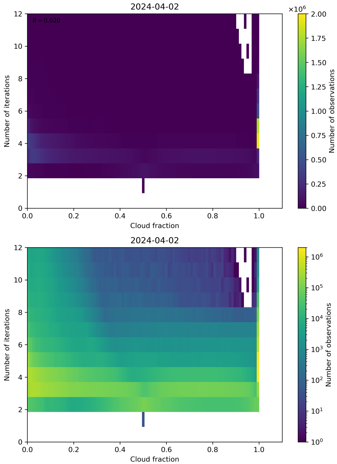
Figure 73: Scatter density plot of “Cloud fraction” against “Number of iterations” for 2024-04-01 to 2024-04-03.
