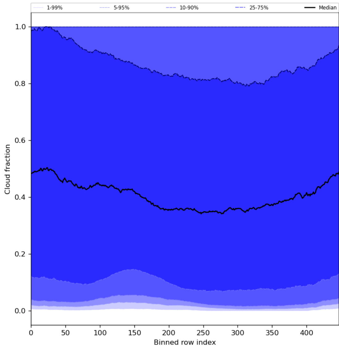
Figure 49: Along track statistics of “Cloud fraction” for 2024-04-01 to 2024-04-03
