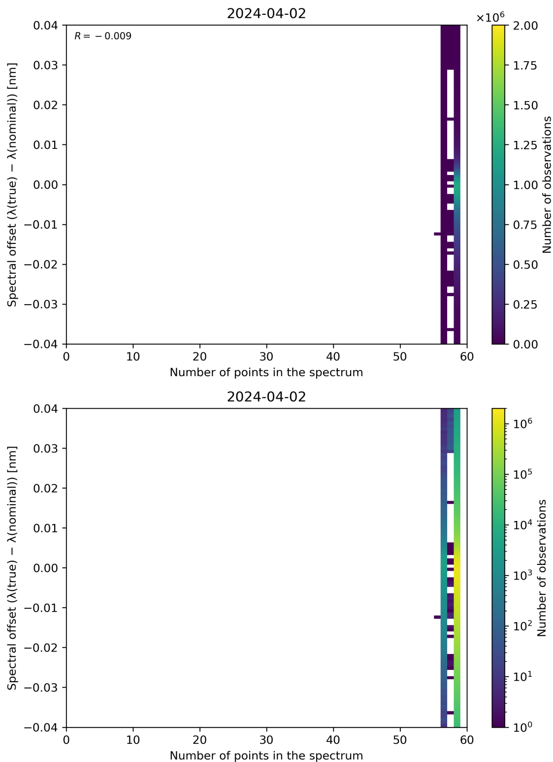
Figure 101: Scatter density plot of “Number of points in the spectrum” against “Spectral offset ( \lambda(\text{true}) - \lambda(\text{nominal}) )” for 2024-04-01 to 2024-04-03.
