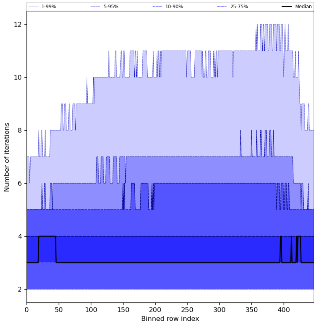
Figure 56: Along track statistics of “Number of iterations” for 2024-04-01 to 2024-04-03
