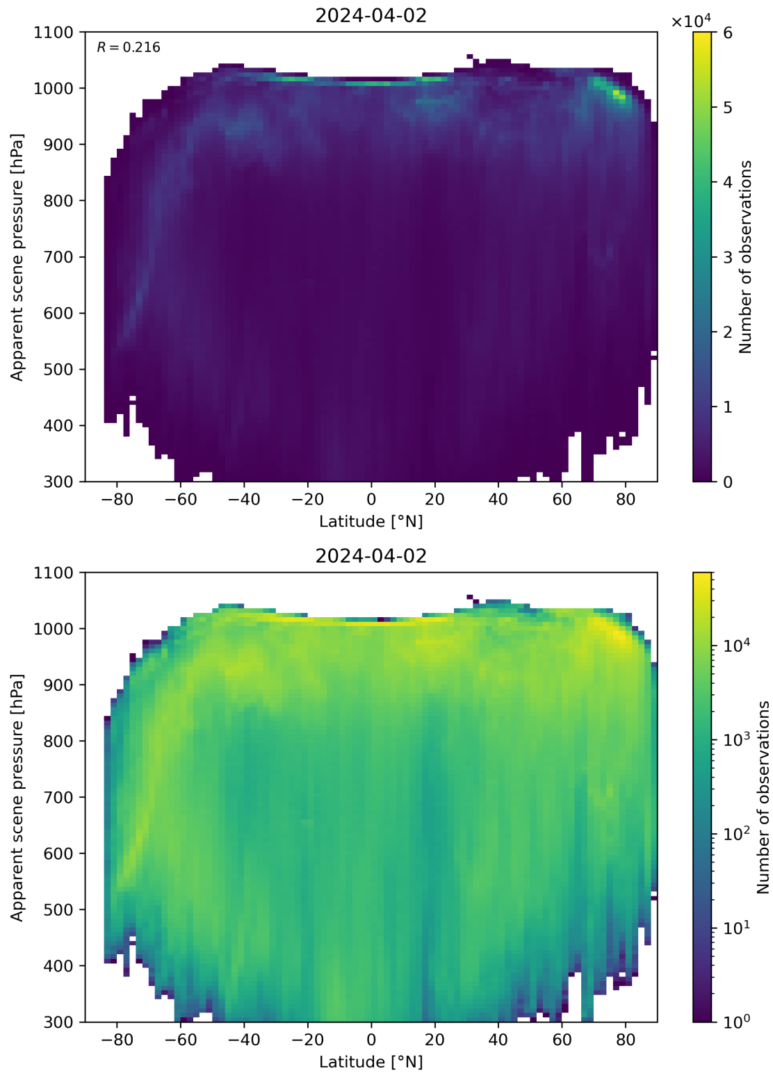
Figure 88: Scatter density plot of “Latitude” against “Apparent scene pressure” for 2024-04-01 to 2024-04-03.
