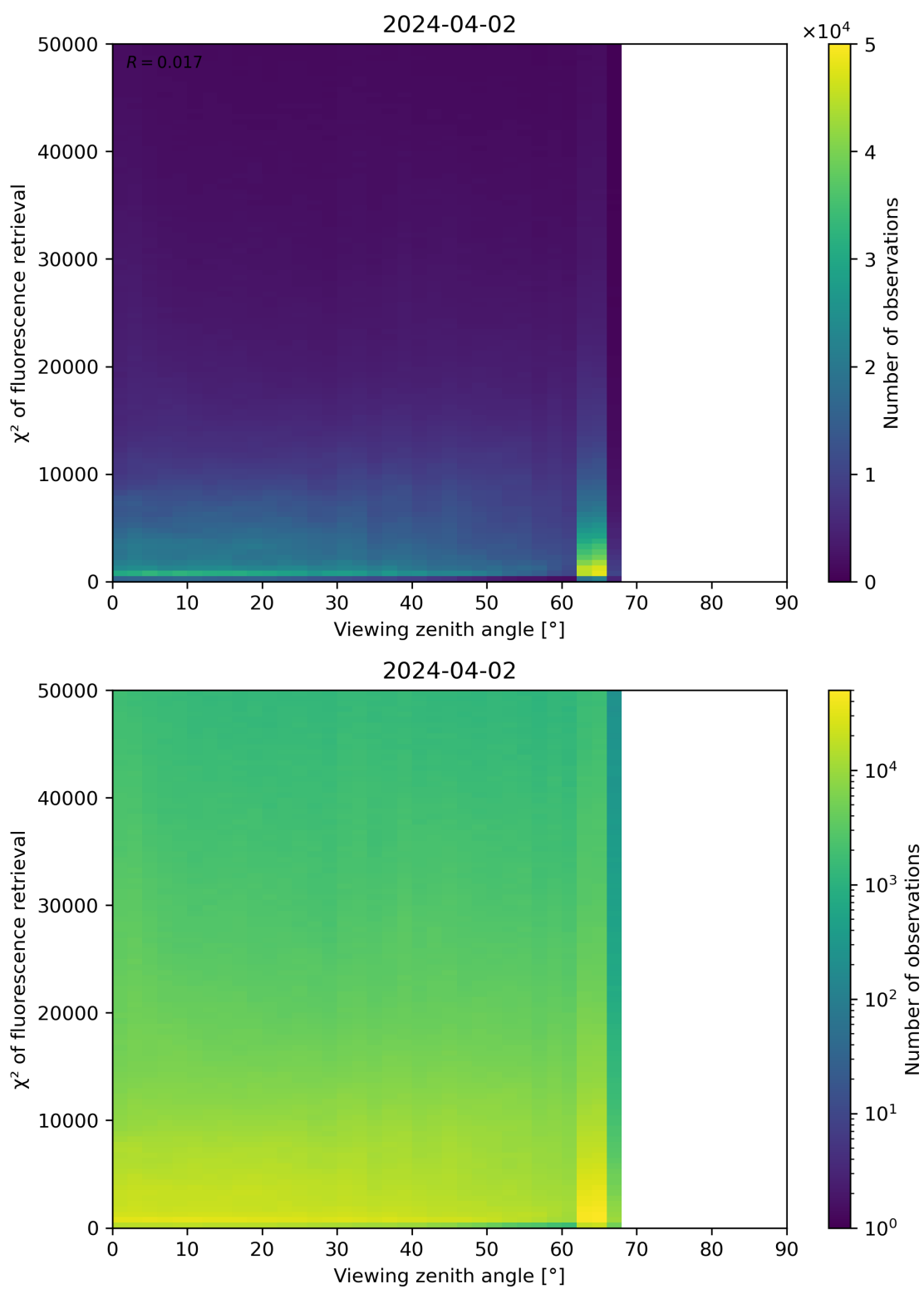
Figure 119: Scatter density plot of “Viewing zenith angle” against “ \chi^2 of fluorescence retrieval” for 2024-04-01 to 2024-04-03.
