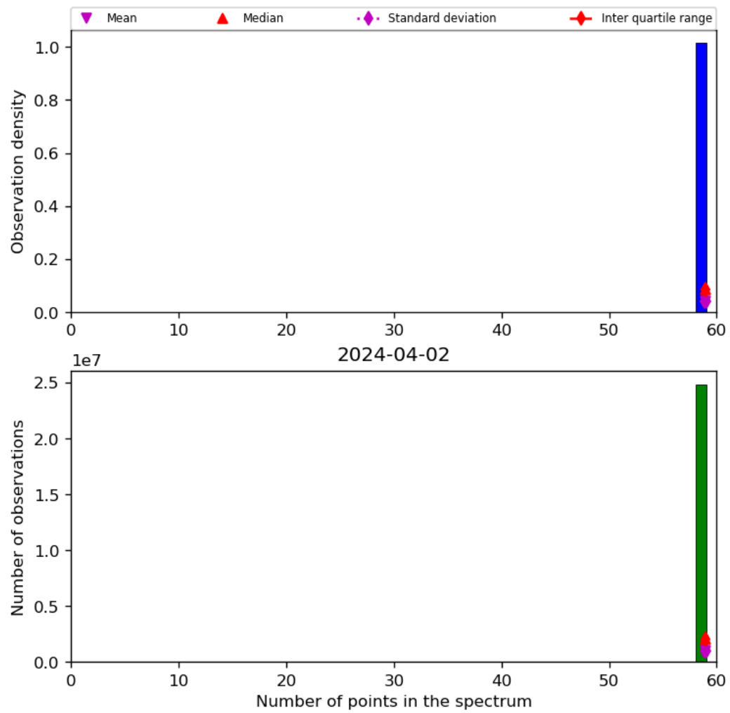
Figure 44: Histogram of "Number of points in the spectrum" for 2024-04-01 to 2024-04-03
