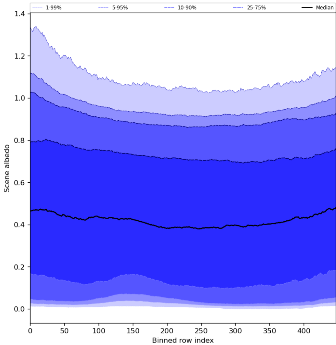
Figure 51: Along track statistics of “Scene albedo” for 2024-04-01 to 2024-04-03
