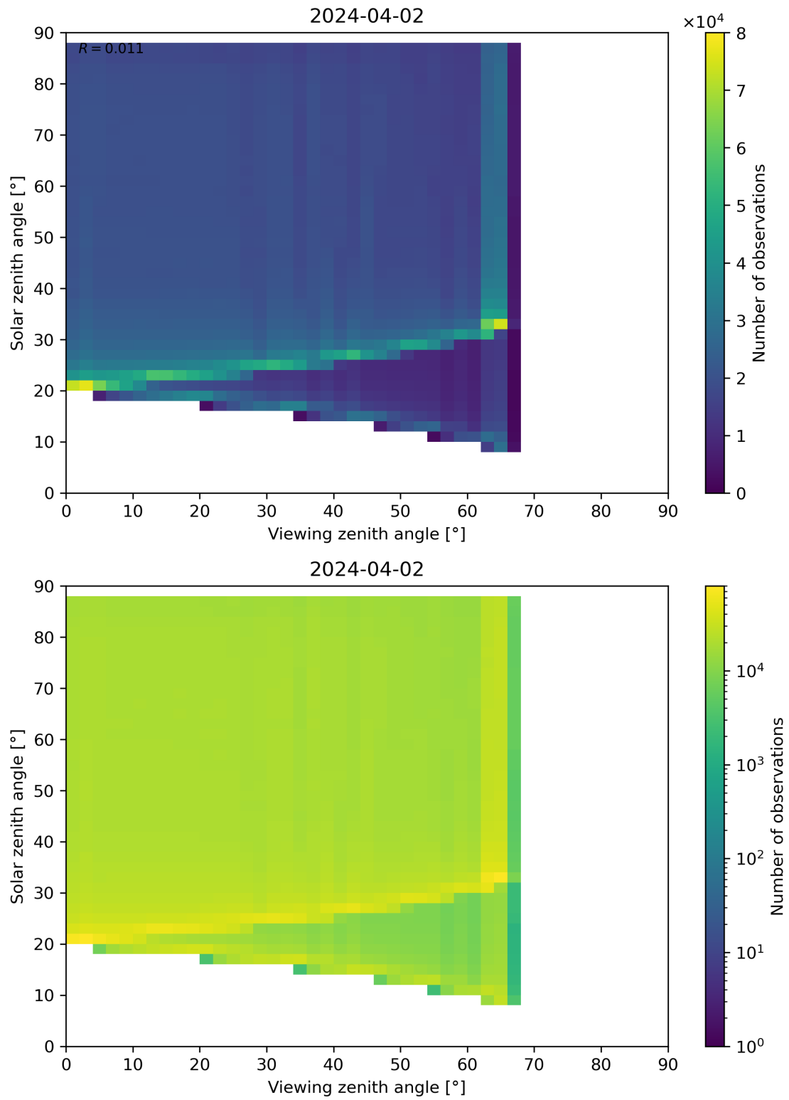
Figure 127: Scatter density plot of “Viewing zenith angle” against “Solar zenith angle” for 2024-04-01 to 2024-04-03.
