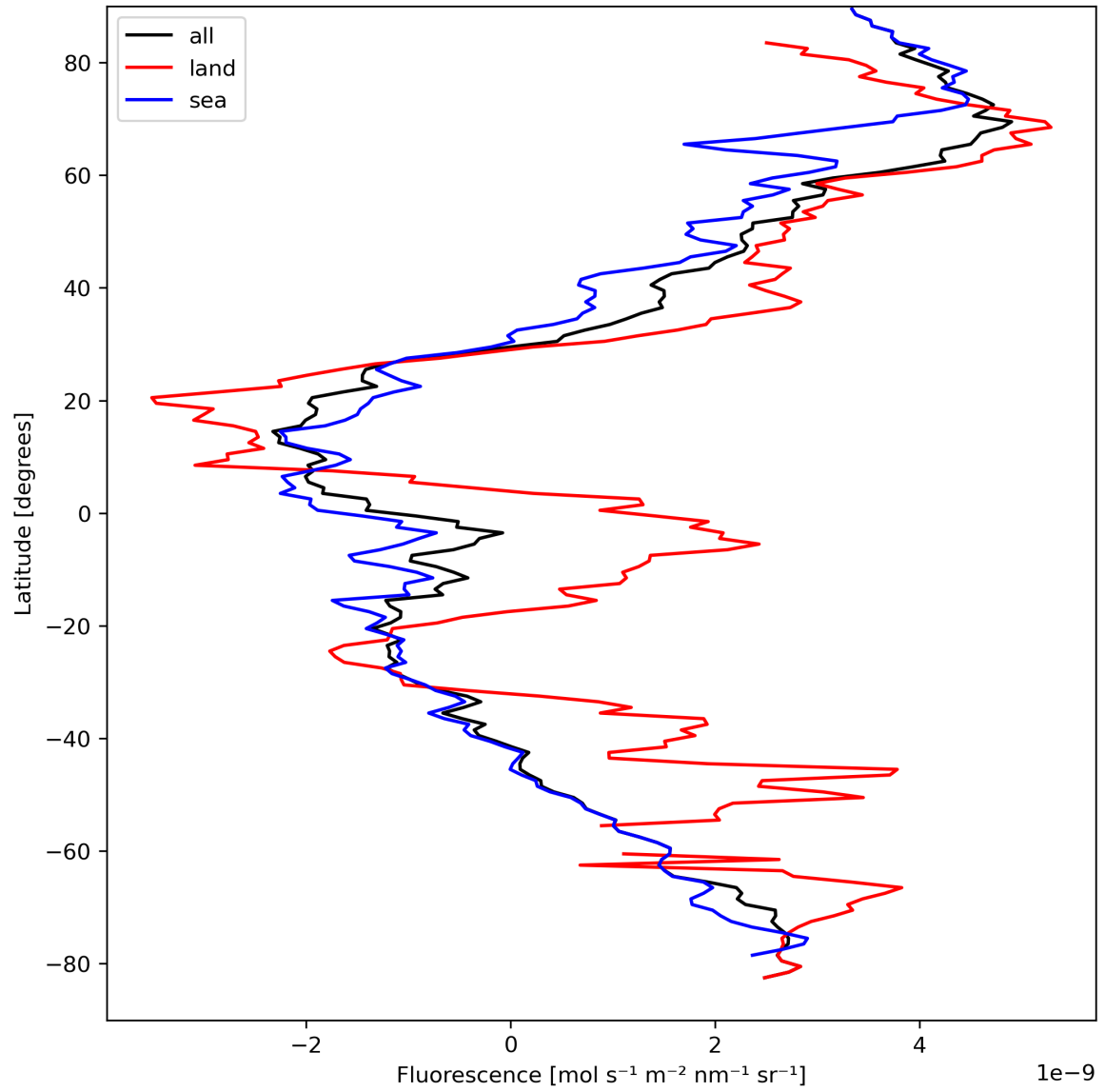
Figure 23: Zonal average of “Fluorescence” for 2024-04-01 to 2024-04-03.
