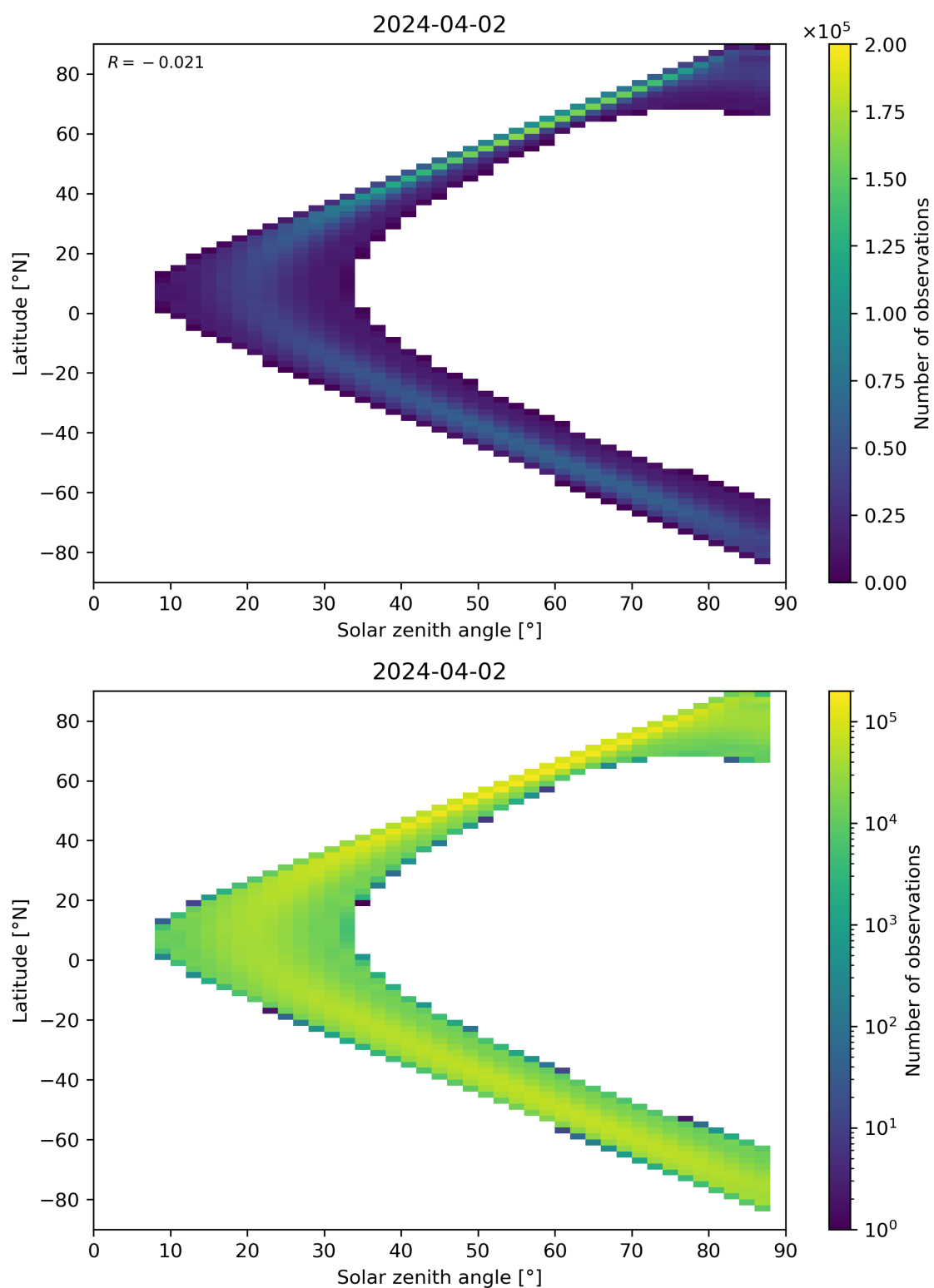
Figure 113: Scatter density plot of “Solar zenith angle” against “Latitude” for 2024-04-01 to 2024-04-03.
