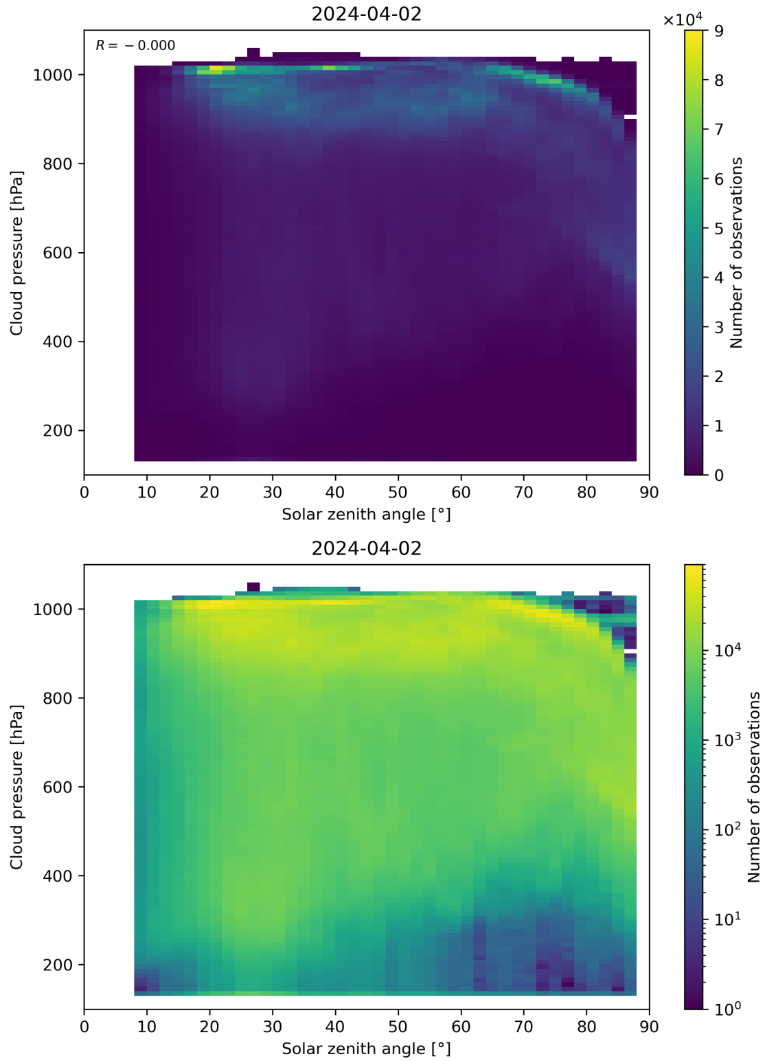
Figure 111: Scatter density plot of “Solar zenith angle” against “Cloud pressure” for 2024-04-01 to 2024-04-03.
