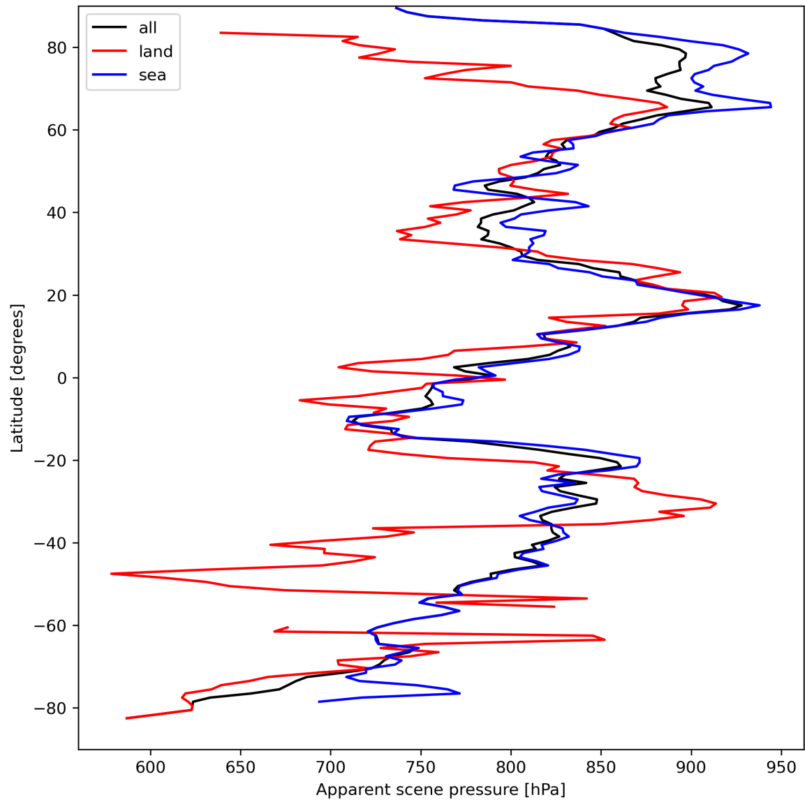
Figure 19: Zonal average of “Apparent scene pressure” for 2024-04-01 to 2024-04-03.
