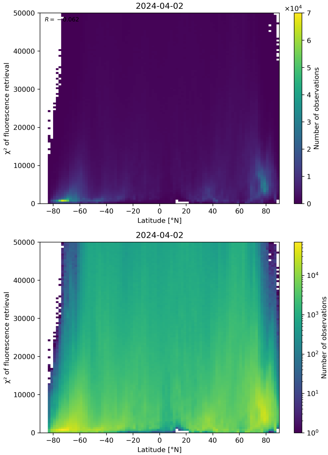
Figure 89: Scatter density plot of “Latitude” against “ \chi^2 of fluorescence retrieval” for 2024-04-01 to 2024-04-03.
