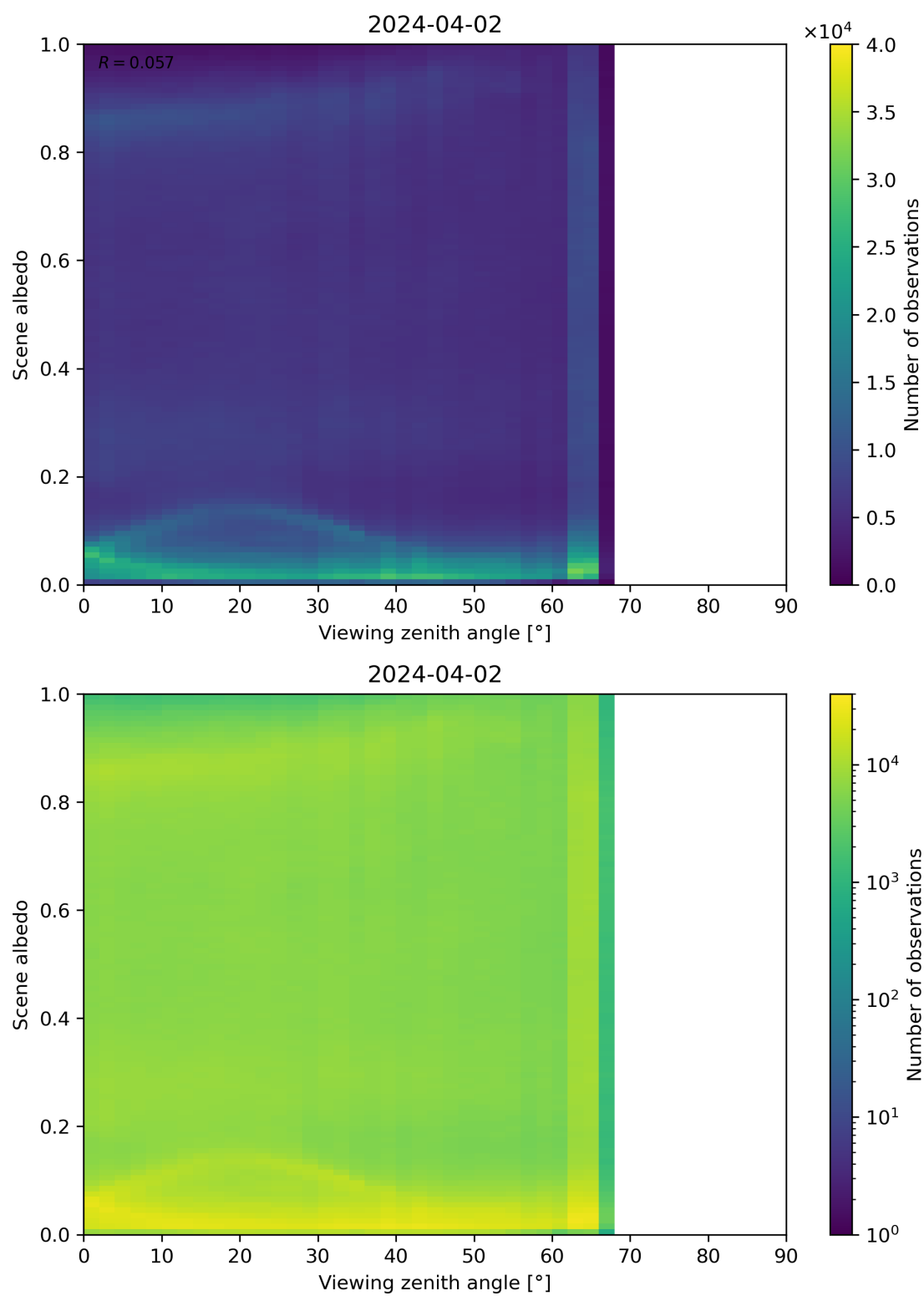
Figure 126: Scatter density plot of “Viewing zenith angle” against “Scene albedo” for 2024-04-01 to 2024-04-03.
