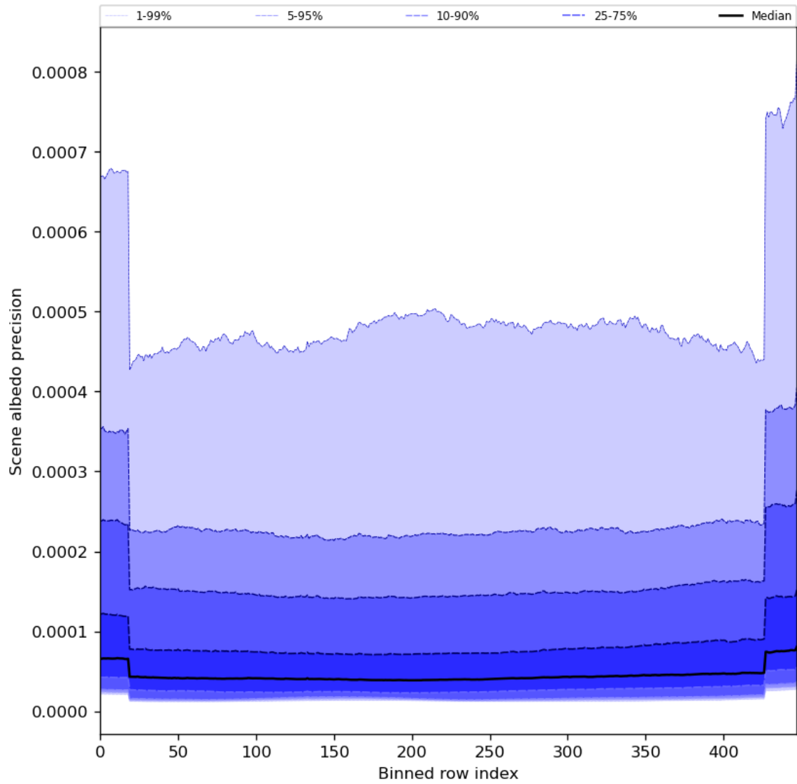
Figure 52: Along track statistics of “Scene albedo precision” for 2024-04-01 to 2024-04-03
