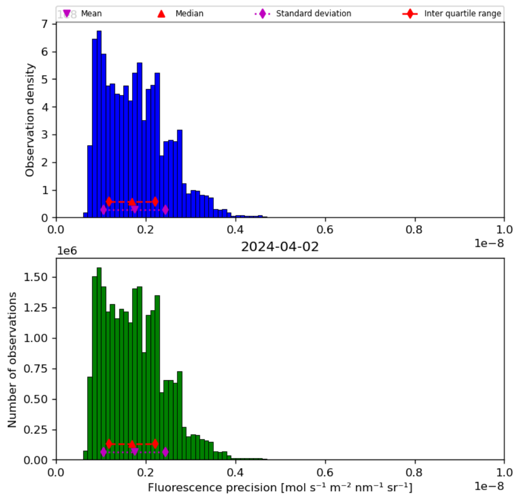
Figure 41: Histogram of “Fluorescence precision” for 2024-04-01 to 2024-04-03
