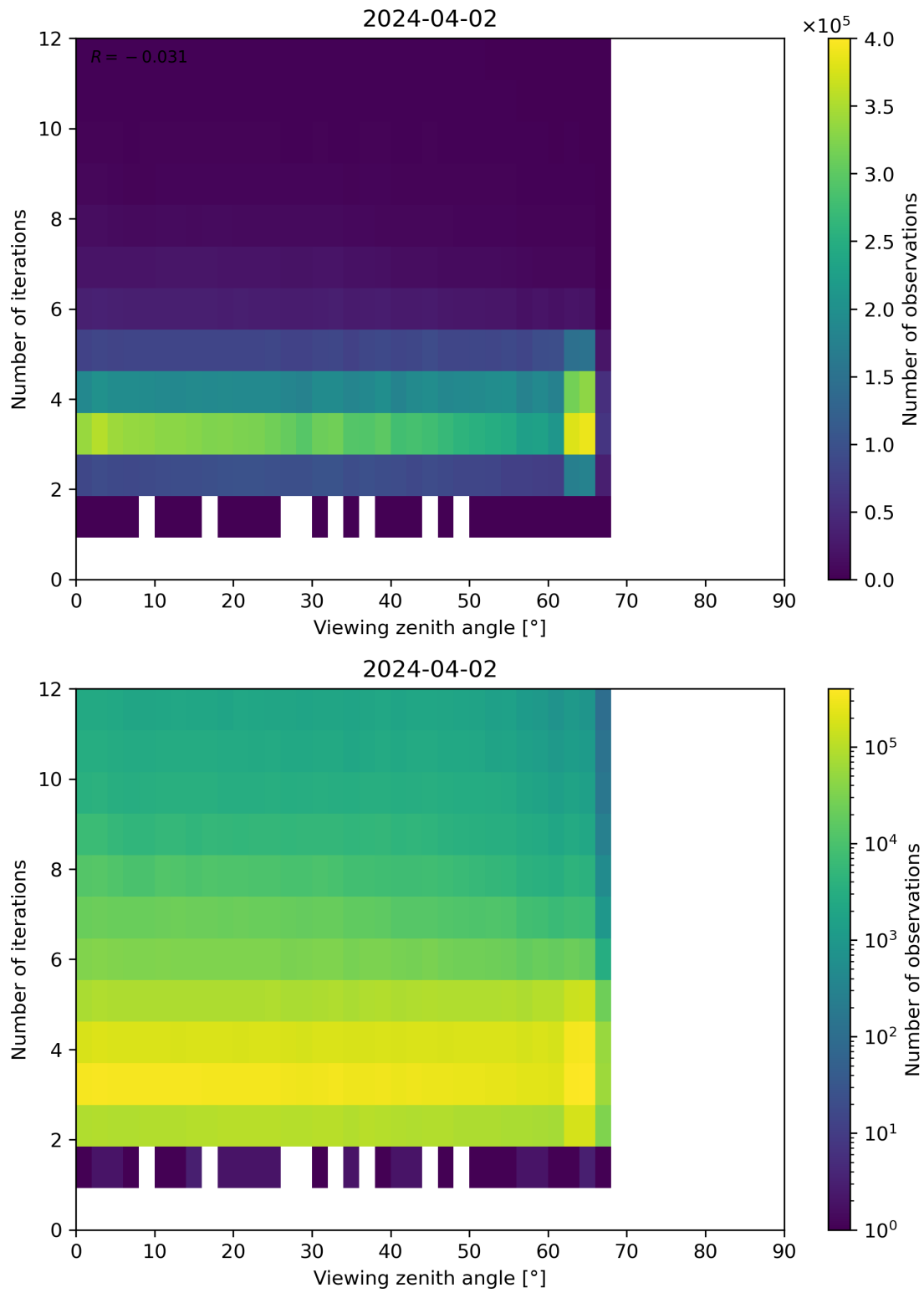
Figure 124: Scatter density plot of “Viewing zenith angle” against “Number of iterations” for 2024-04-01 to 2024-04-03.
