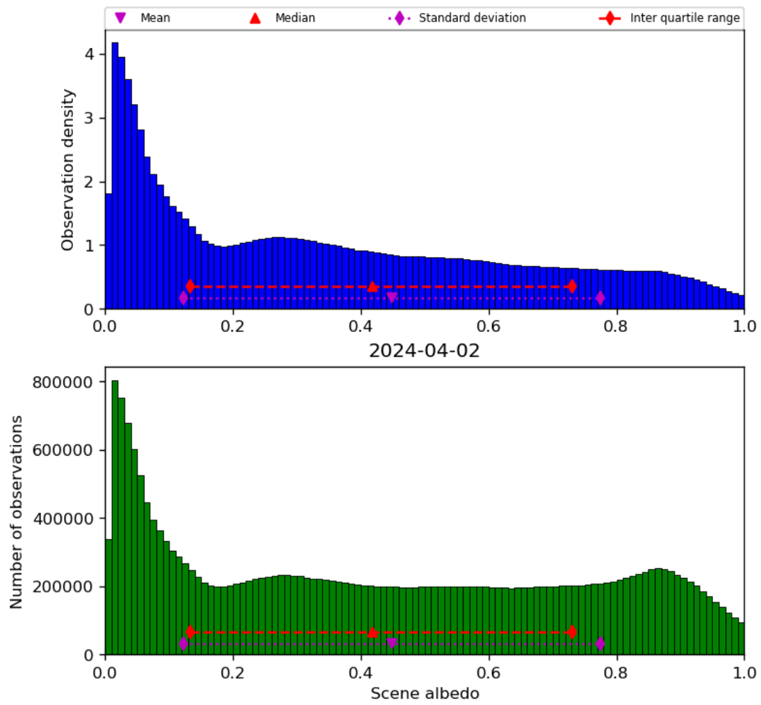
Figure 34: Histogram of “Scene albedo” for 2024-04-01 to 2024-04-03
