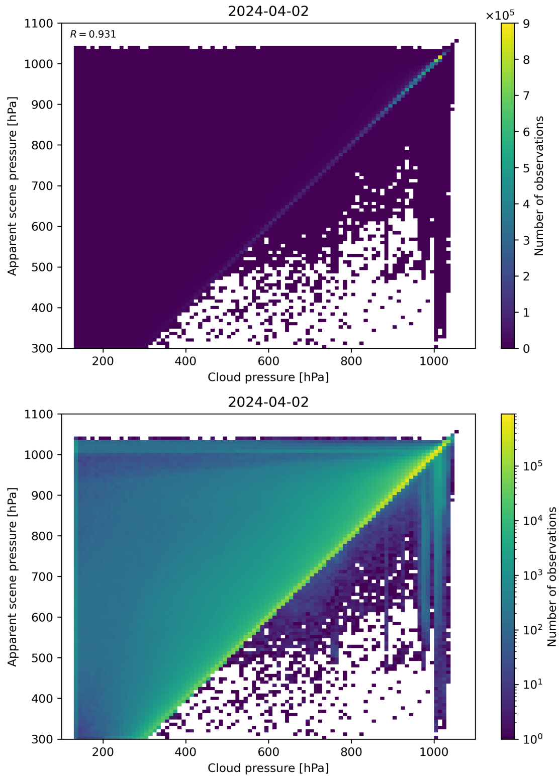
Figure 77: Scatter density plot of “Cloud pressure” against “Apparent scene pressure” for 2024-04-01 to 2024-04-03.
