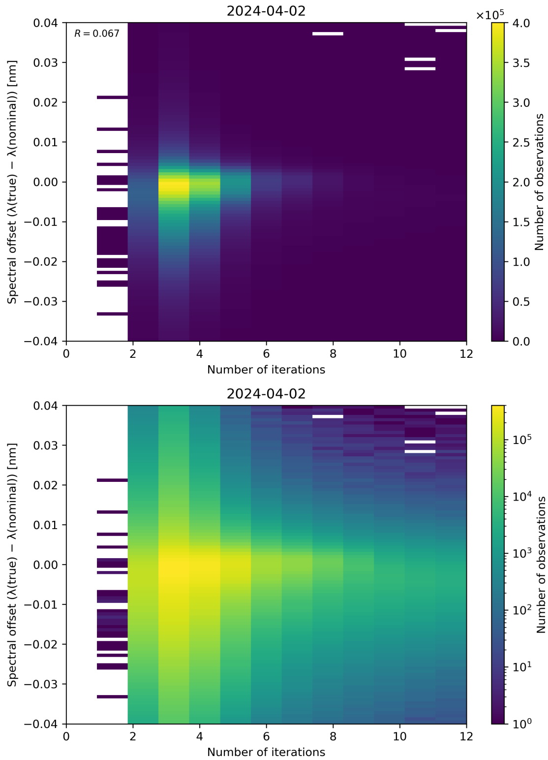
Figure 100: Scatter density plot of “Number of iterations” against “Spectral offset ( \lambda(\text{true}) - \lambda(\text{nominal}) )” for 2024-04-01 to 2024-04-03.
