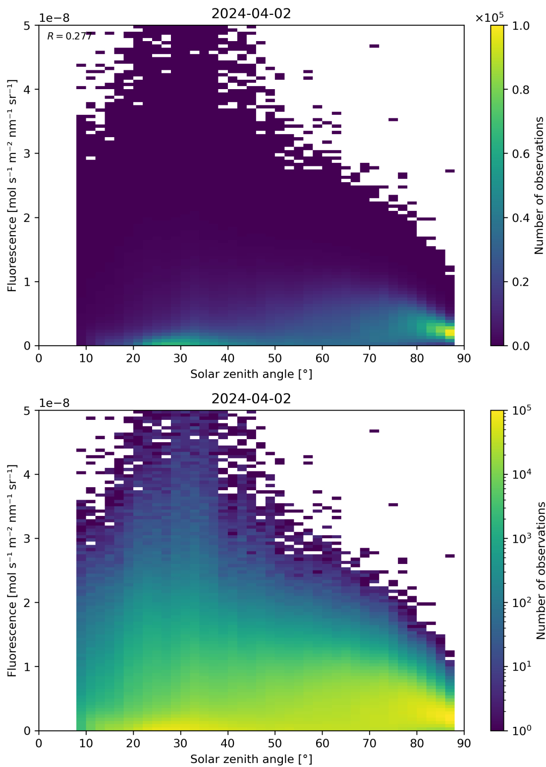
Figure 112: Scatter density plot of “Solar zenith angle” against “Fluorescence” for 2024-04-01 to 2024-04-03.
