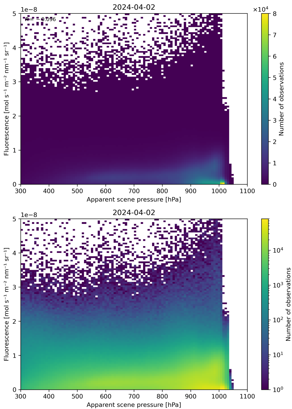
Figure 64: Scatter density plot of “Apparent scene pressure” against “Fluorescence” for 2024-04-01 to 2024-04-03.
