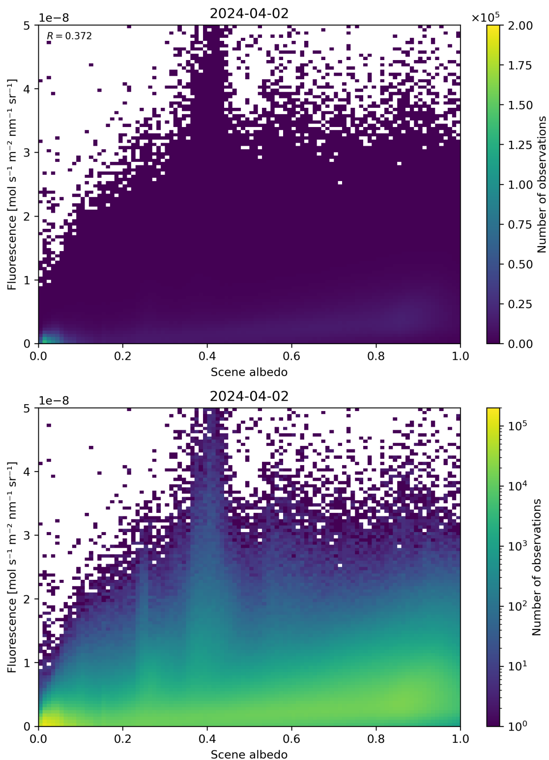
Figure 104: Scatter density plot of “Scene albedo” against “Fluorescence” for 2024-04-01 to 2024-04-03.
