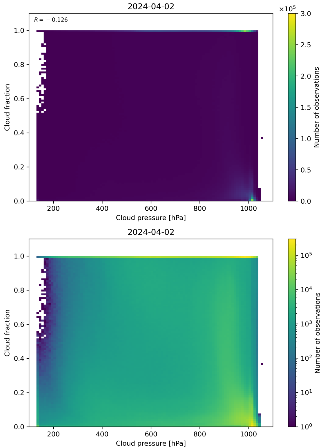
Figure 79: Scatter density plot of “Cloud pressure” against “Cloud fraction” for 2024-04-01 to 2024-04-03.
