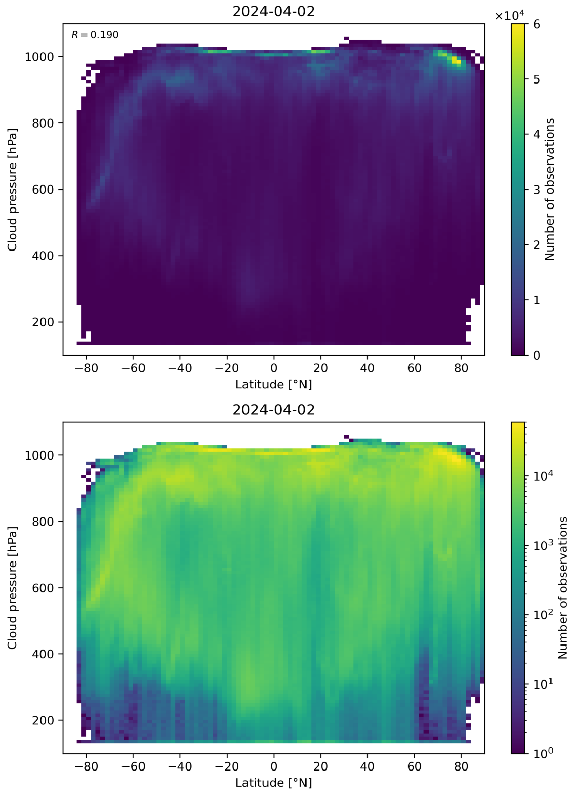
Figure 91: Scatter density plot of “Latitude” against “Cloud pressure” for 2024-04-01 to 2024-04-03.
