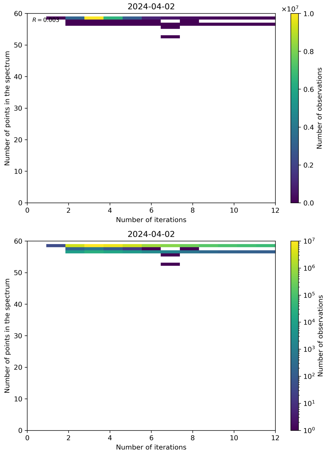
Figure 99: Scatter density plot of “Number of iterations” against “Number of points in the spectrum” for 2024-04-01 to 2024-04-03.
