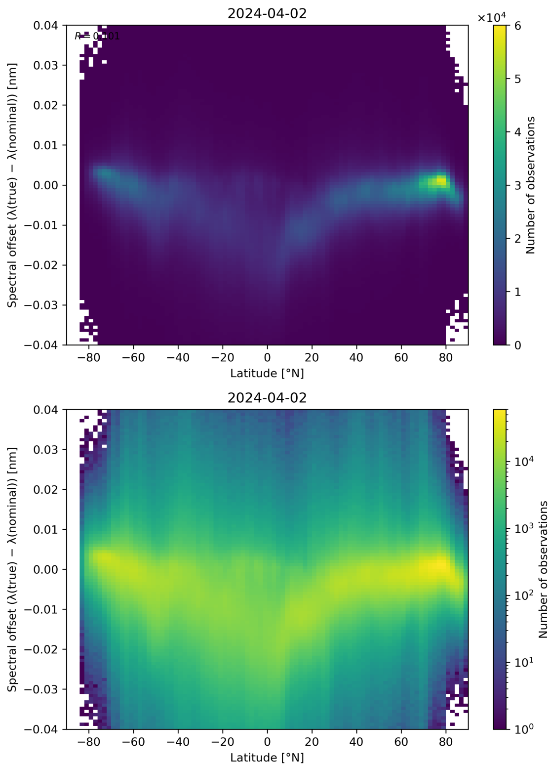
Figure 96: Scatter density plot of “Latitude” against “Spectral offset ( \lambda(\text{true}) - \lambda(\text{nominal}) )” for 2024-04-01 to 2024-04-03.
