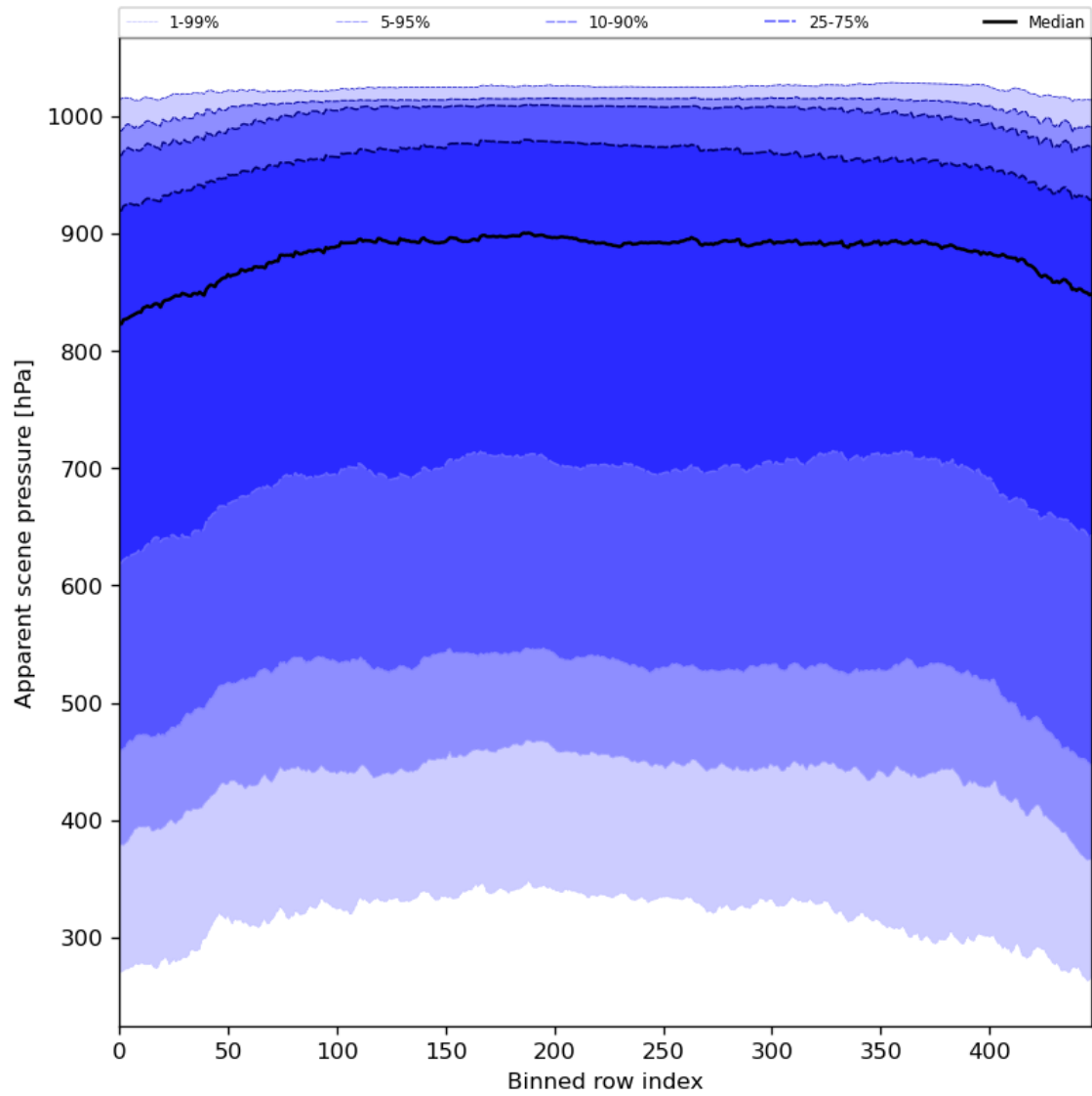
Figure 53: Along track statistics of “Apparent scene pressure” for 2024-04-01 to 2024-04-03
