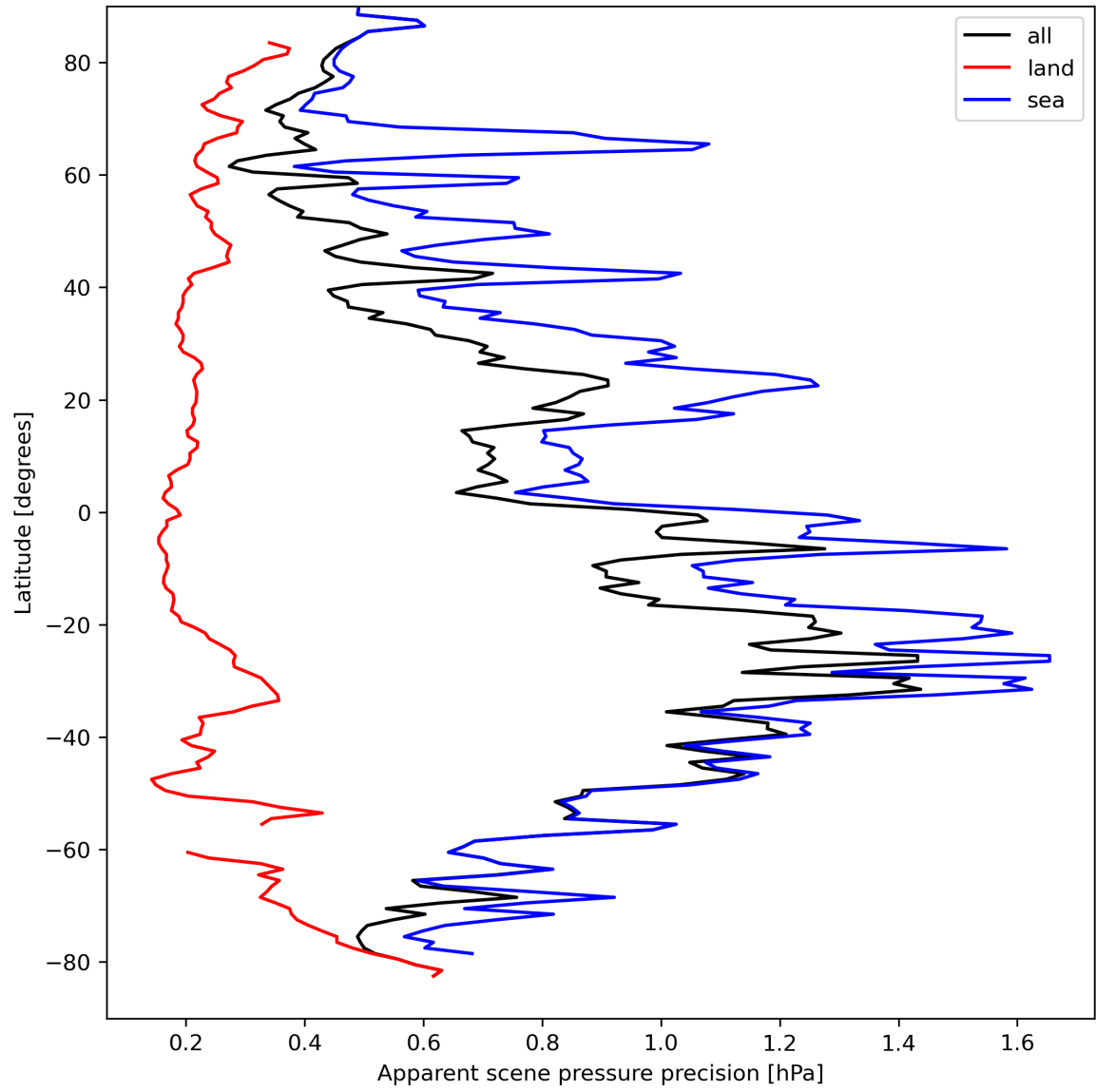
Figure 20: Zonal average of “Apparent scene pressure precision” for 2024-04-01 to 2024-04-03.
