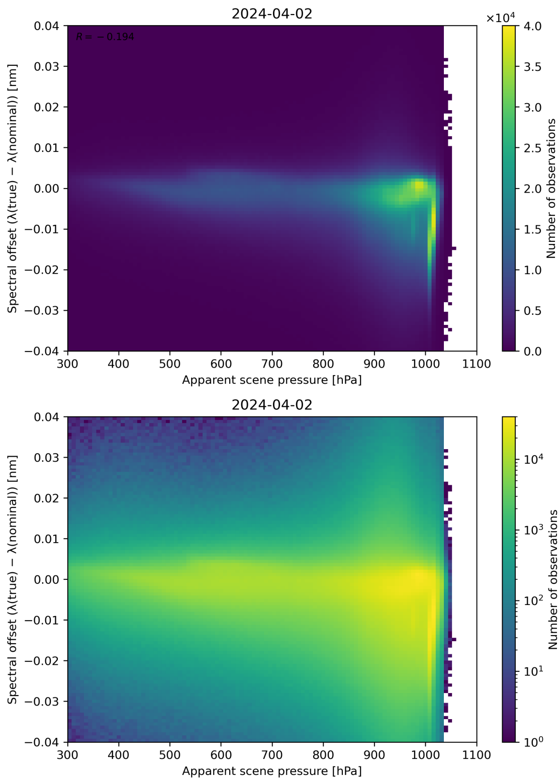
Figure 67: Scatter density plot of “Apparent scene pressure” against “Spectral offset ( \lambda(\text{true}) - \lambda(\text{nominal}) )” for 2024-04-01 to 2024-04-03.
