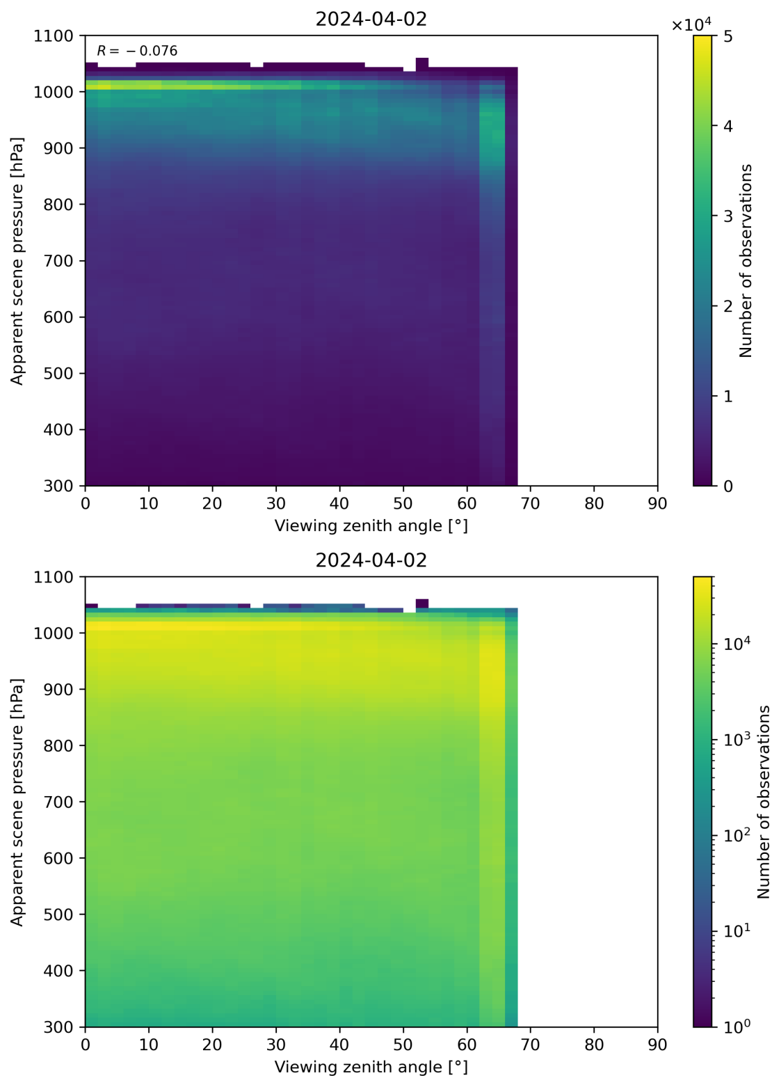
Figure 118: Scatter density plot of “Viewing zenith angle” against “Apparent scene pressure” for 2024-04-01 to 2024-04-03.
