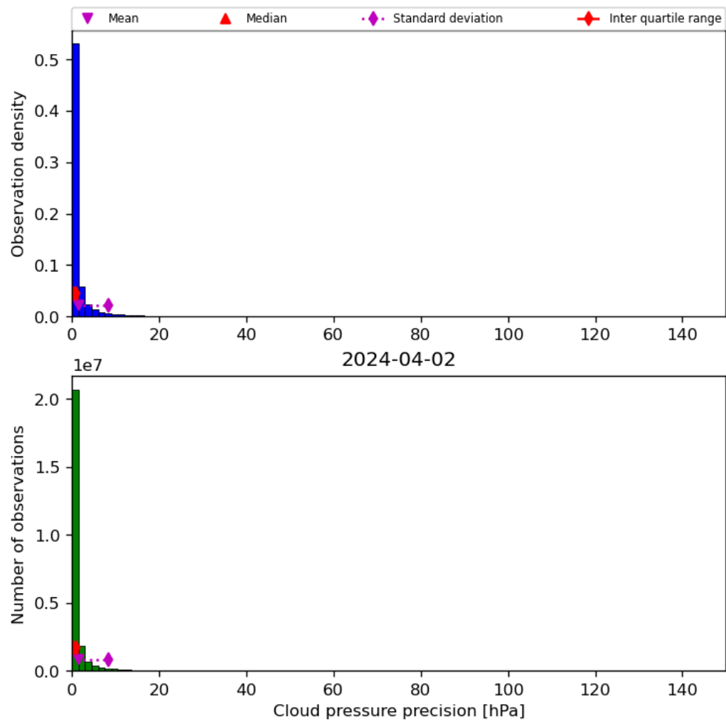
Figure 31: Histogram of “Cloud pressure precision” for 2024-04-01 to 2024-04-03
