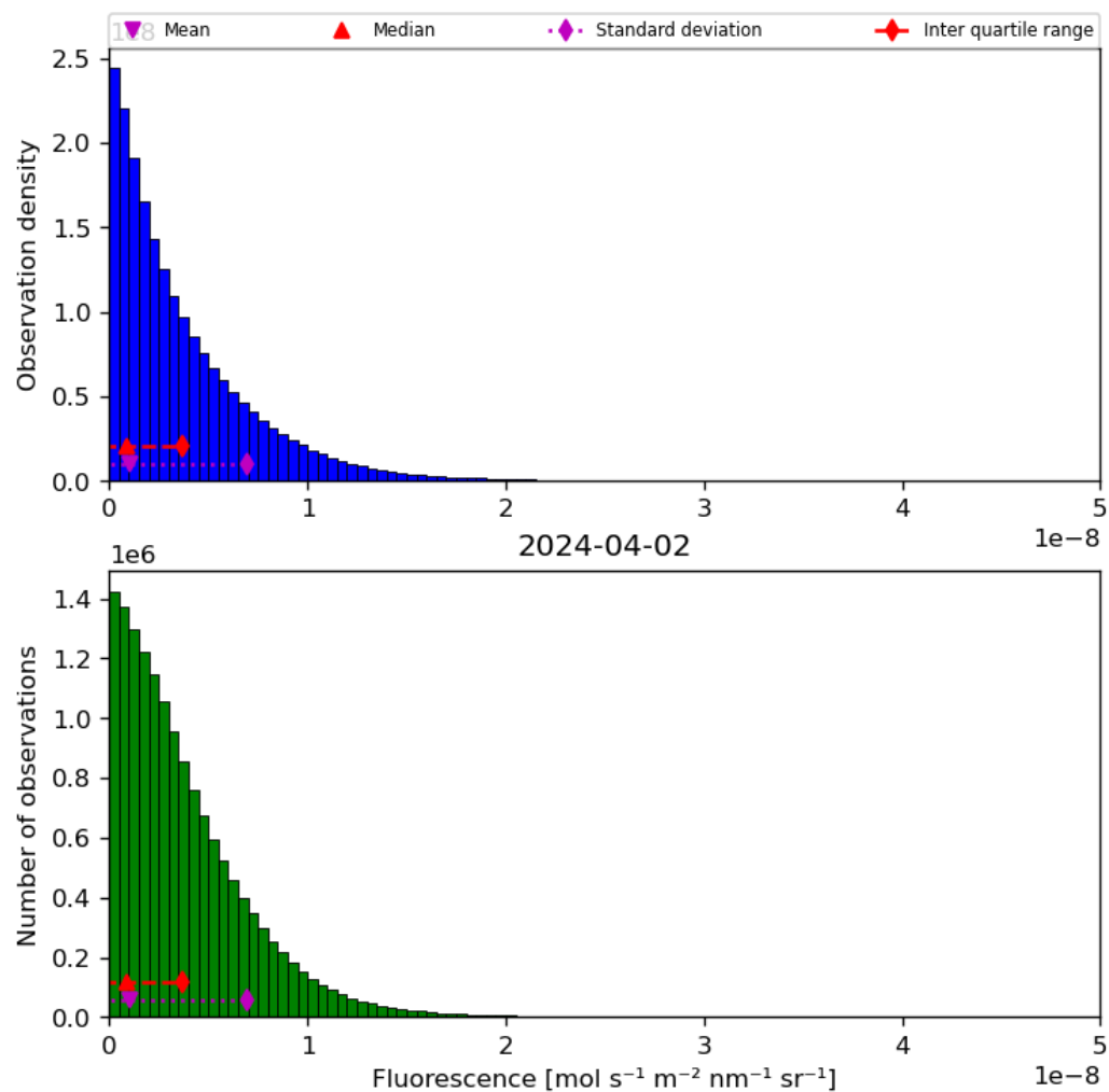
Figure 40: Histogram of “Fluorescence” for 2024-04-01 to 2024-04-03
