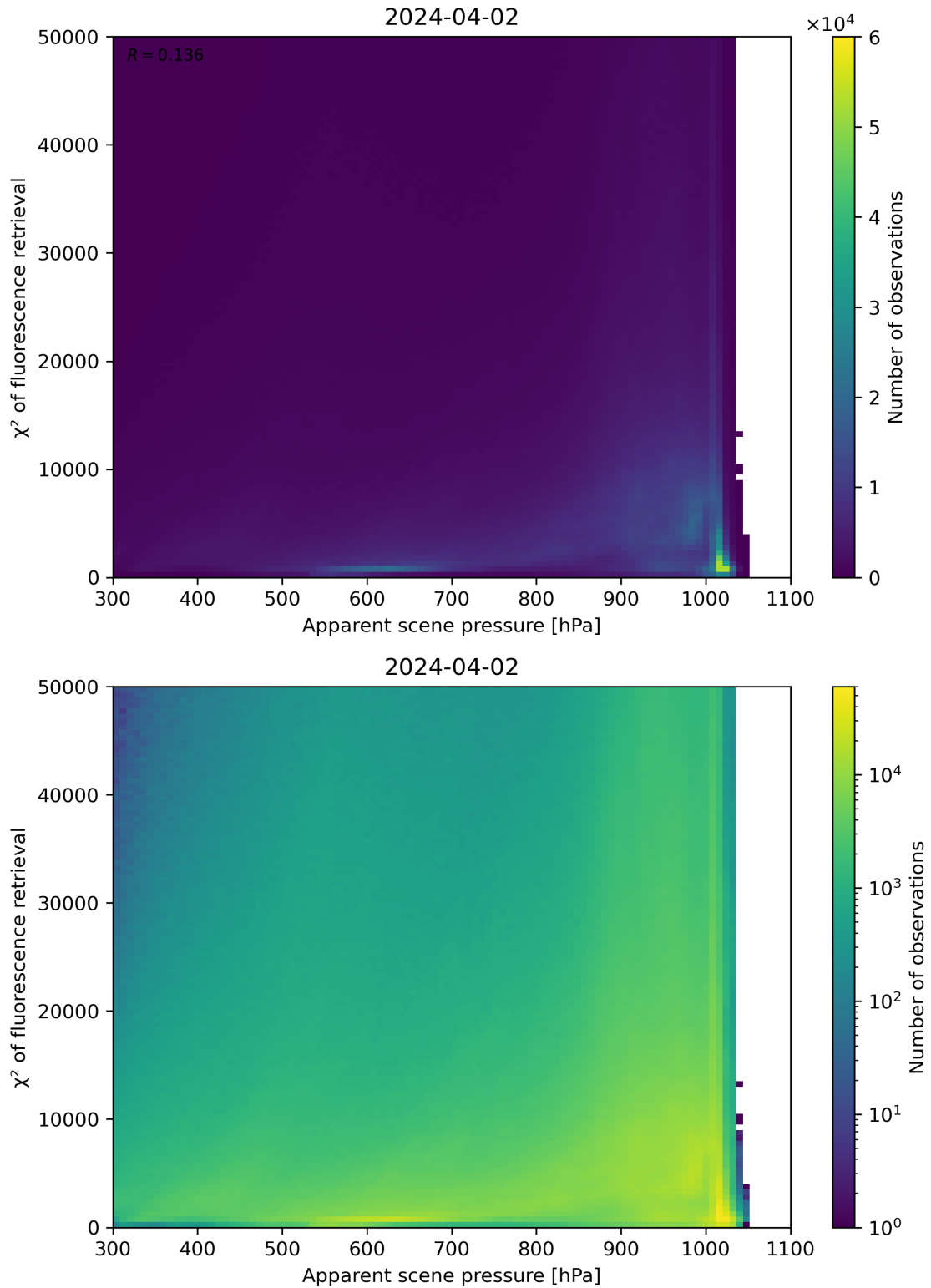
Figure 63: Scatter density plot of “Apparent scene pressure” against “ \chi^2 of fluorescence retrieval” for 2024-04-01 to 2024-04-03.
