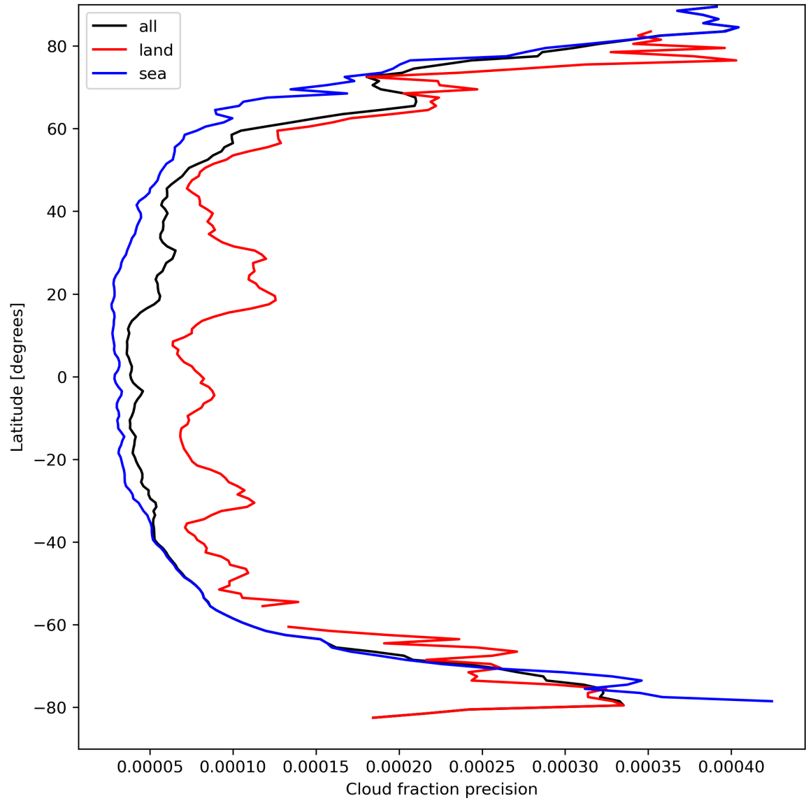
Figure 16: Zonal average of “Cloud fraction precision” for 2024-04-01 to 2024-04-03.
