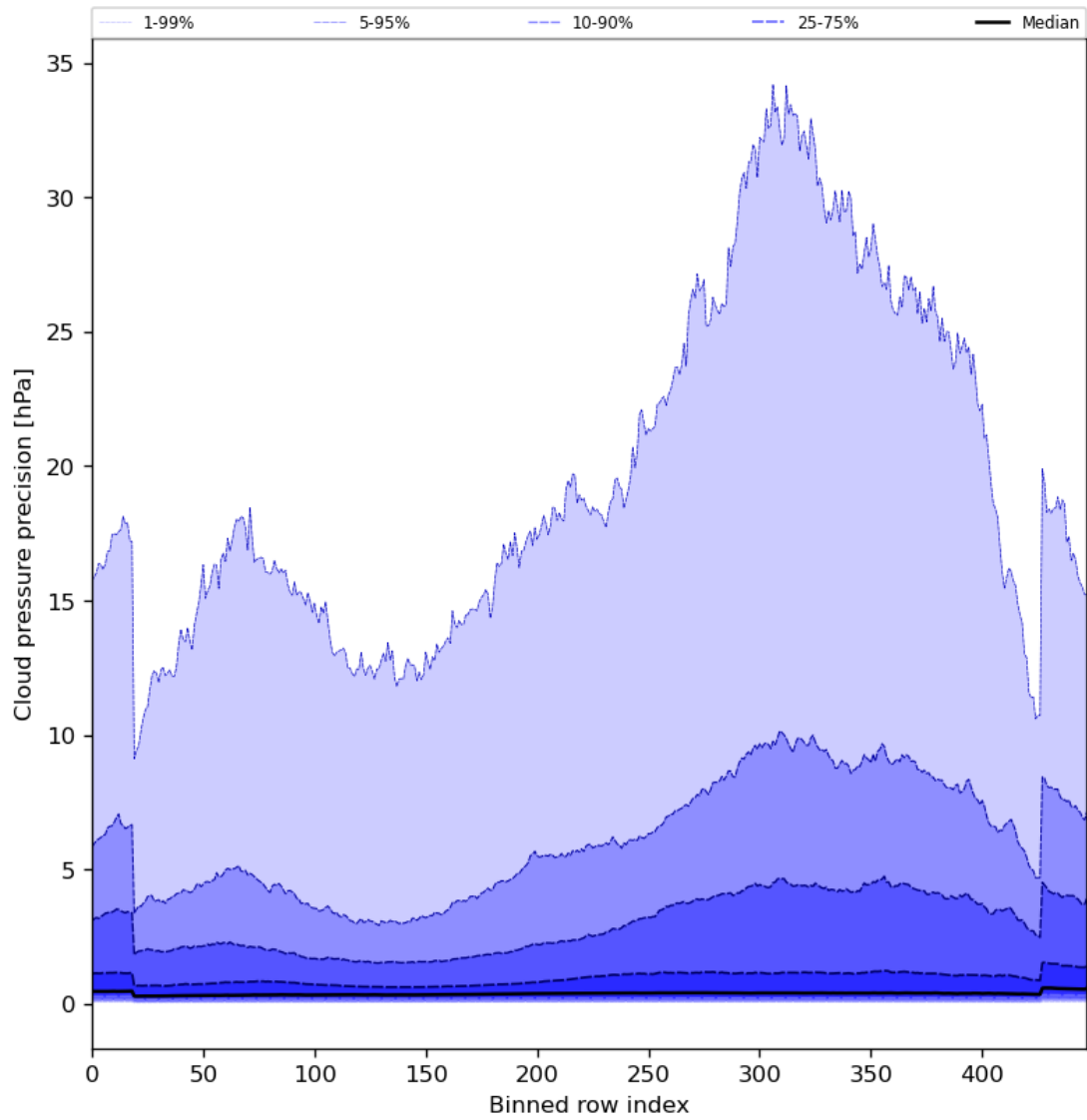
Figure 48: Along track statistics of “Cloud pressure precision” for 2024-04-01 to 2024-04-03
