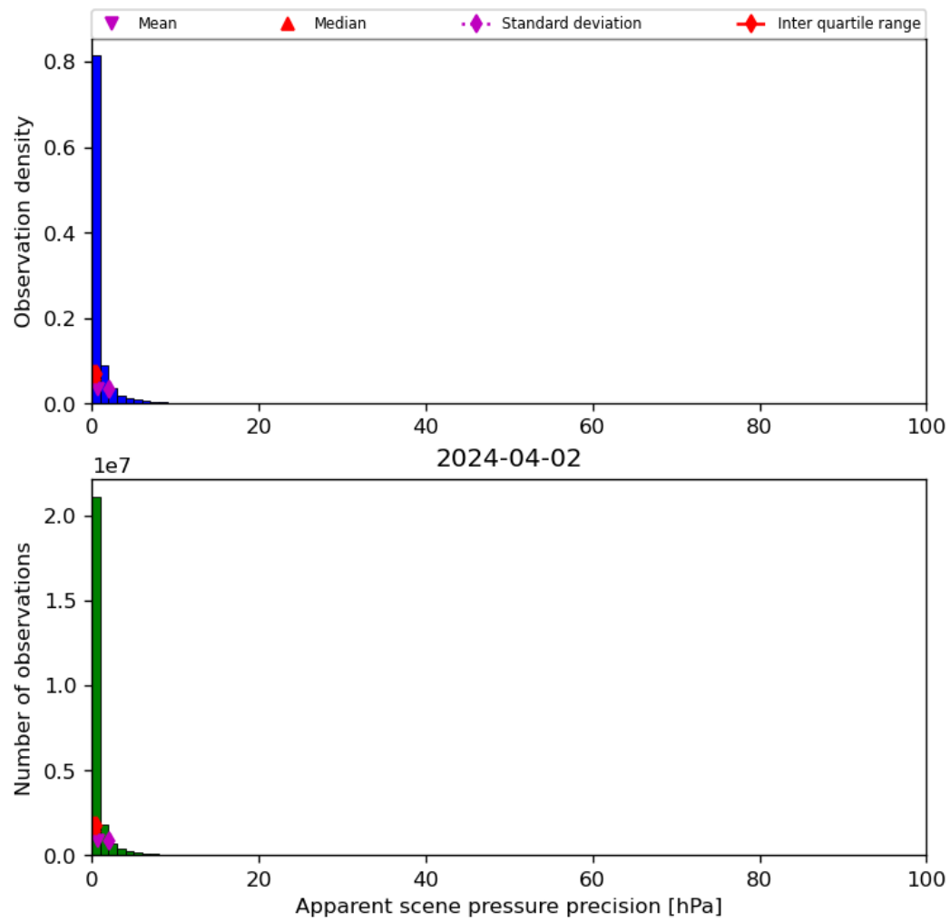
Figure 37: Histogram of “Apparent scene pressure precision” for 2024-04-01 to 2024-04-03
