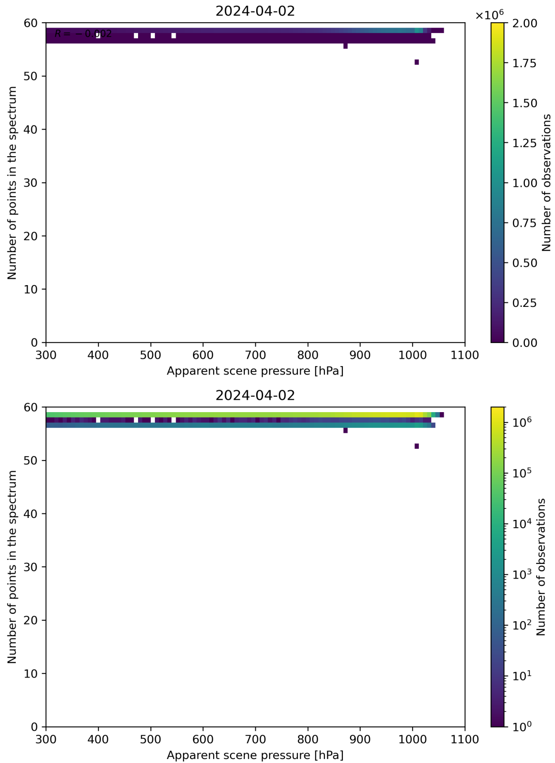
Figure 66: Scatter density plot of “Apparent scene pressure” against “Number of points in the spectrum” for 2024-04-01 to 2024-04-03.
