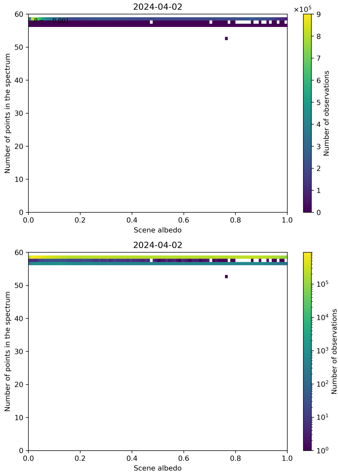
Figure 106: Scatter density plot of “Scene albedo” against “Number of points in the spectrum” for 2024-04-01 to 2024-04-03.
