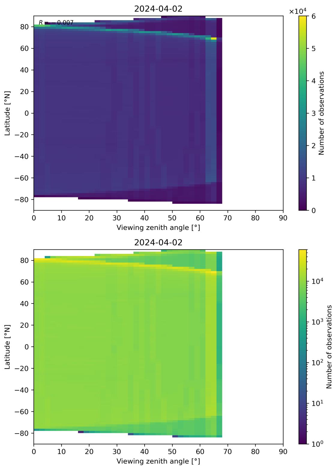
Figure 123: Scatter density plot of “Viewing zenith angle” against “Latitude” for 2024-04-01 to 2024-04-03.
