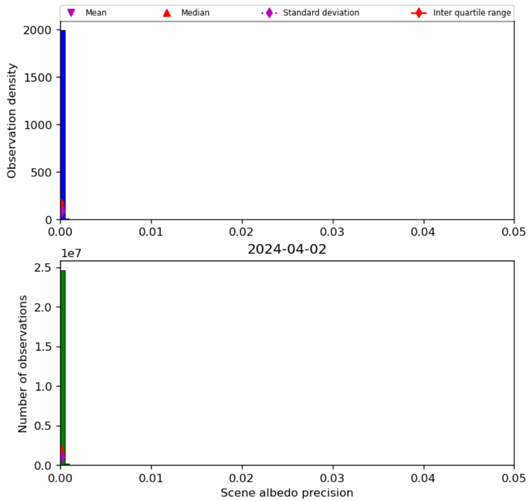
Figure 35: Histogram of “Scene albedo precision” for 2024-04-01 to 2024-04-03
