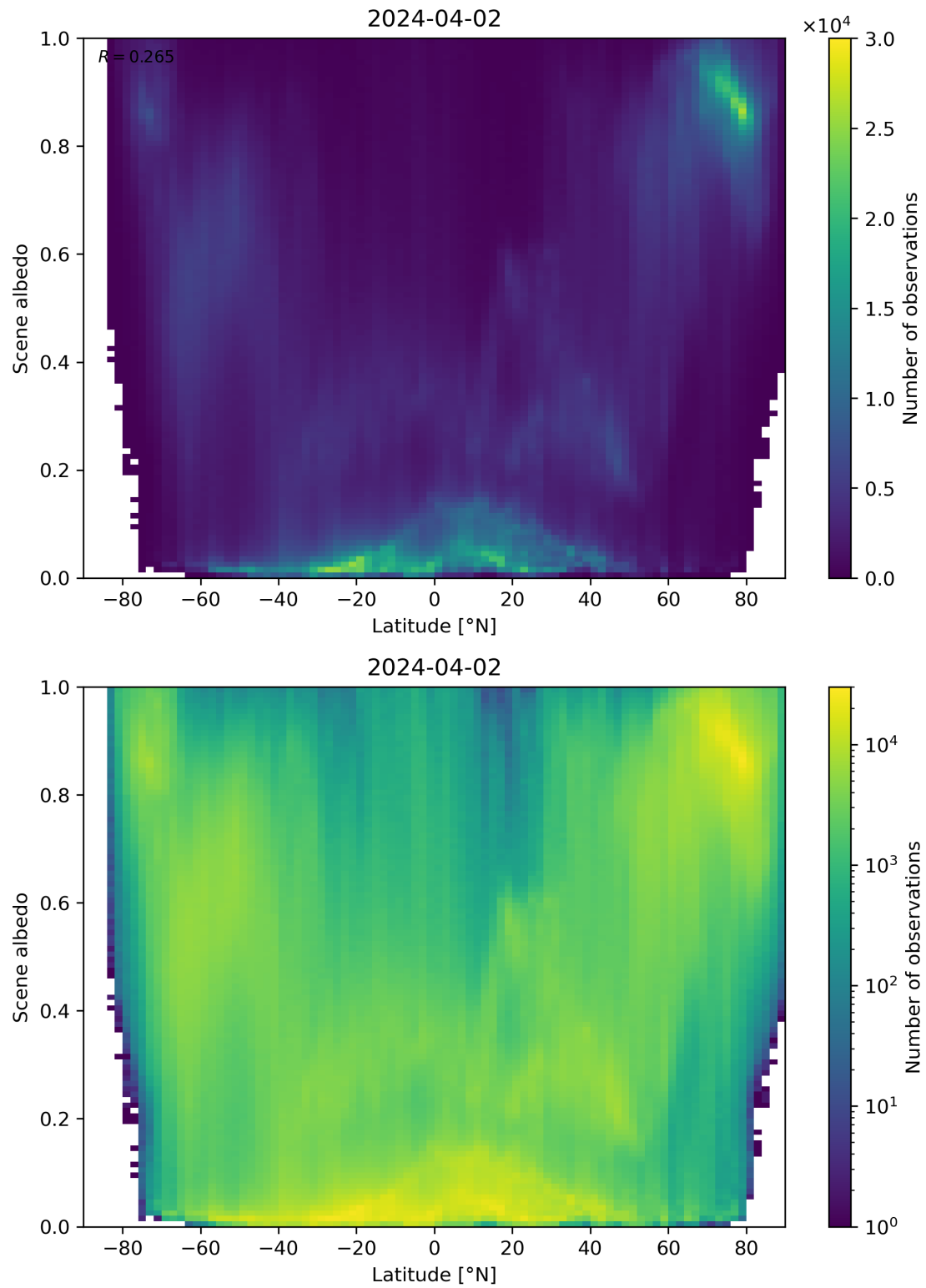
Figure 95: Scatter density plot of “Latitude” against “Scene albedo” for 2024-04-01 to 2024-04-03.
