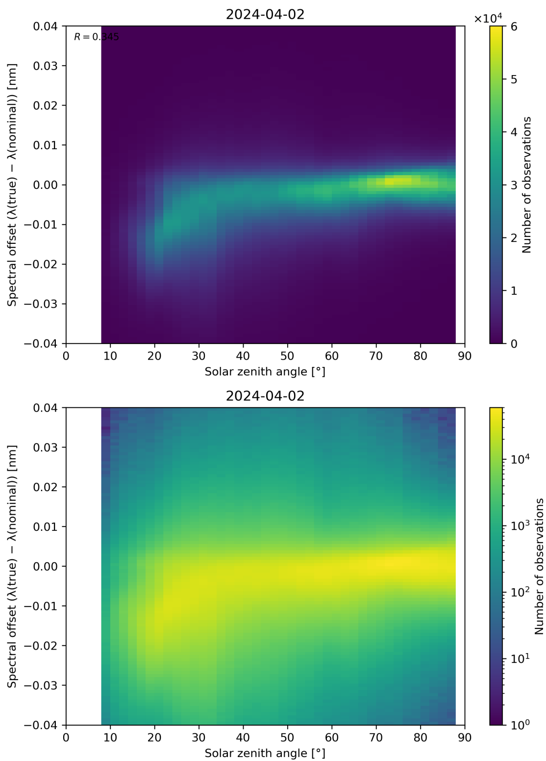
Figure 117: Scatter density plot of “Solar zenith angle” against “Spectral offset ( \lambda(\text{true}) - \lambda(\text{nominal}) )” for 2024-04-01 to 2024-04-03.
