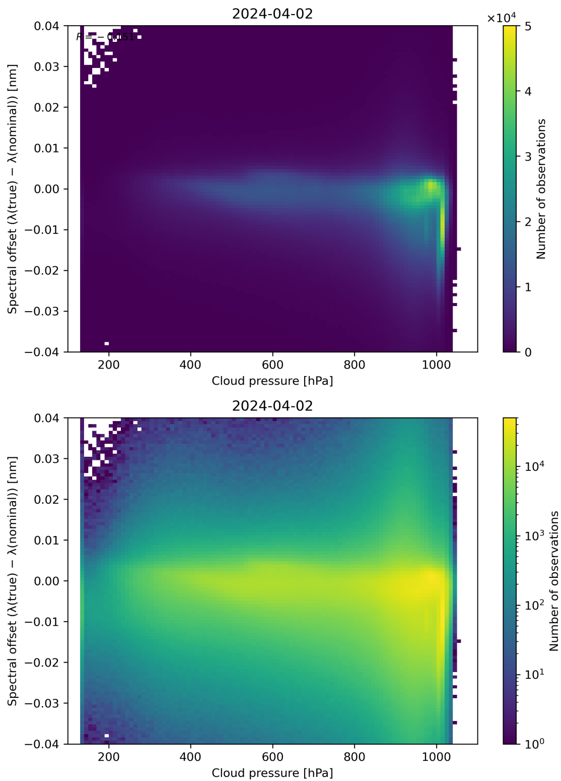
Figure 84: Scatter density plot of “Cloud pressure” against “Spectral offset ( \lambda(\text{true}) - \lambda(\text{nominal}) )” for 2024-04-01 to 2024-04-03.
