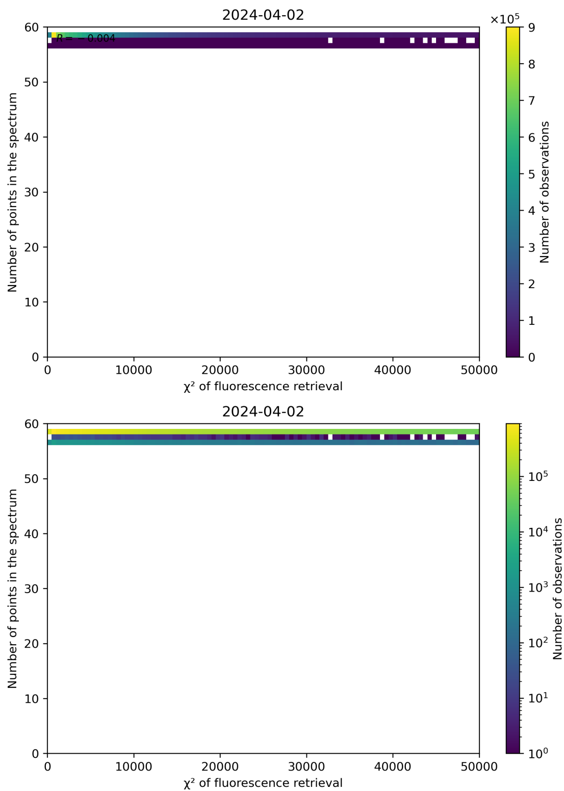
Figure 68: Scatter density plot of " \chi^2 of fluorescence retrieval" against "Number of points in the spectrum" for 2024-04-01 to 2024-04-03.
