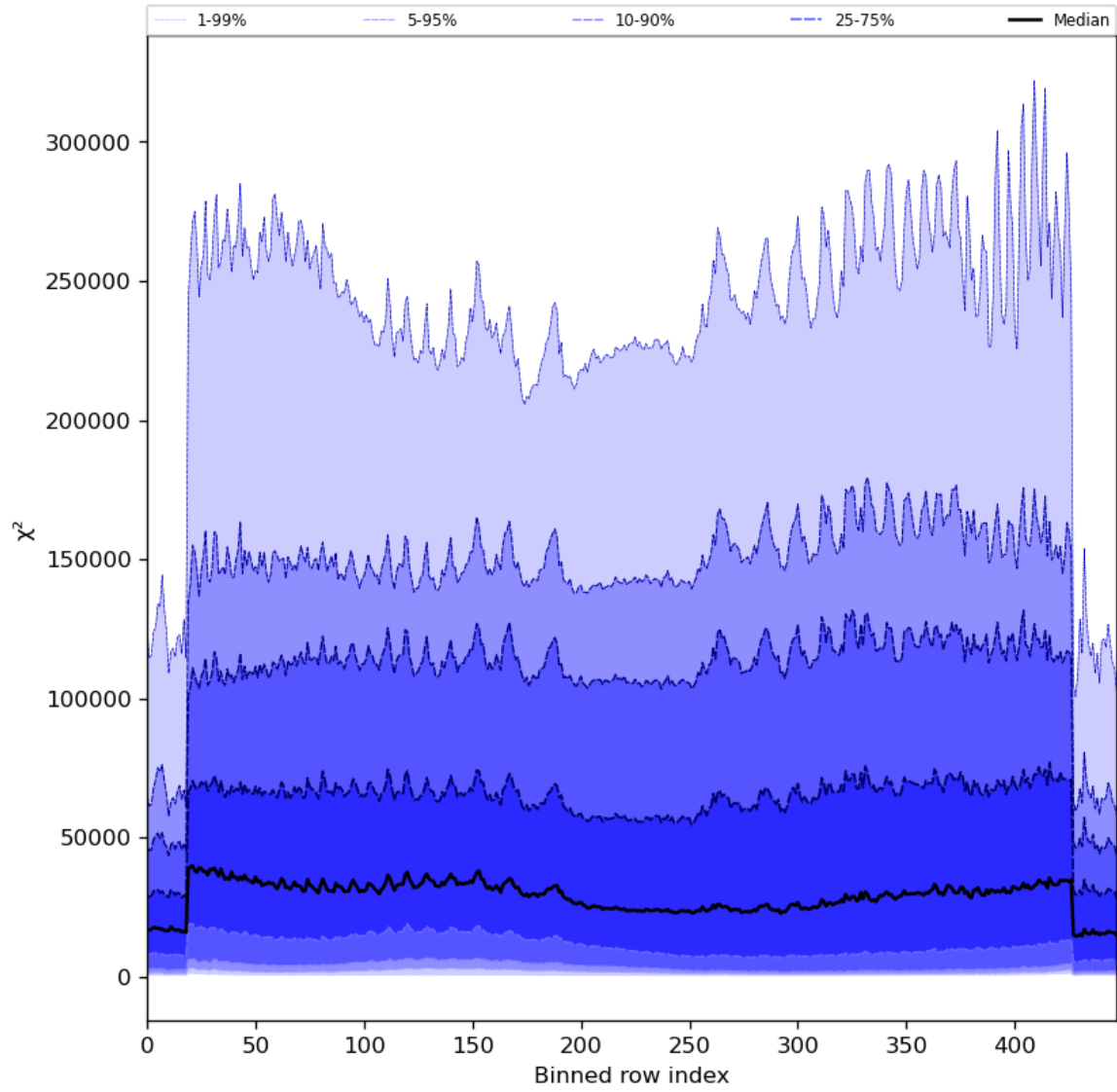
Figure 55: Along track statistics of “ \chi^2 ” for 2024-04-01 to 2024-04-03
