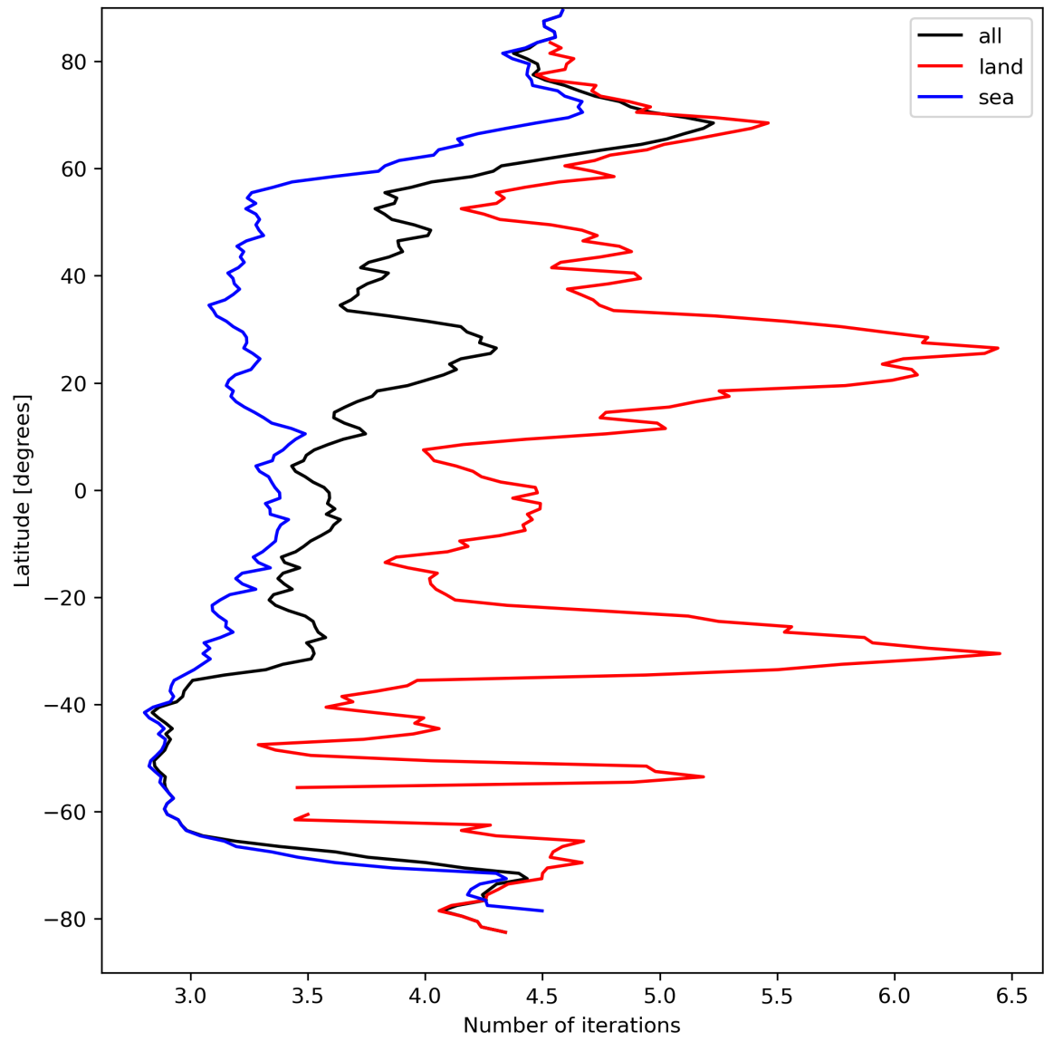
Figure 22: Zonal average of “Number of iterations” for 2024-04-01 to 2024-04-03.
