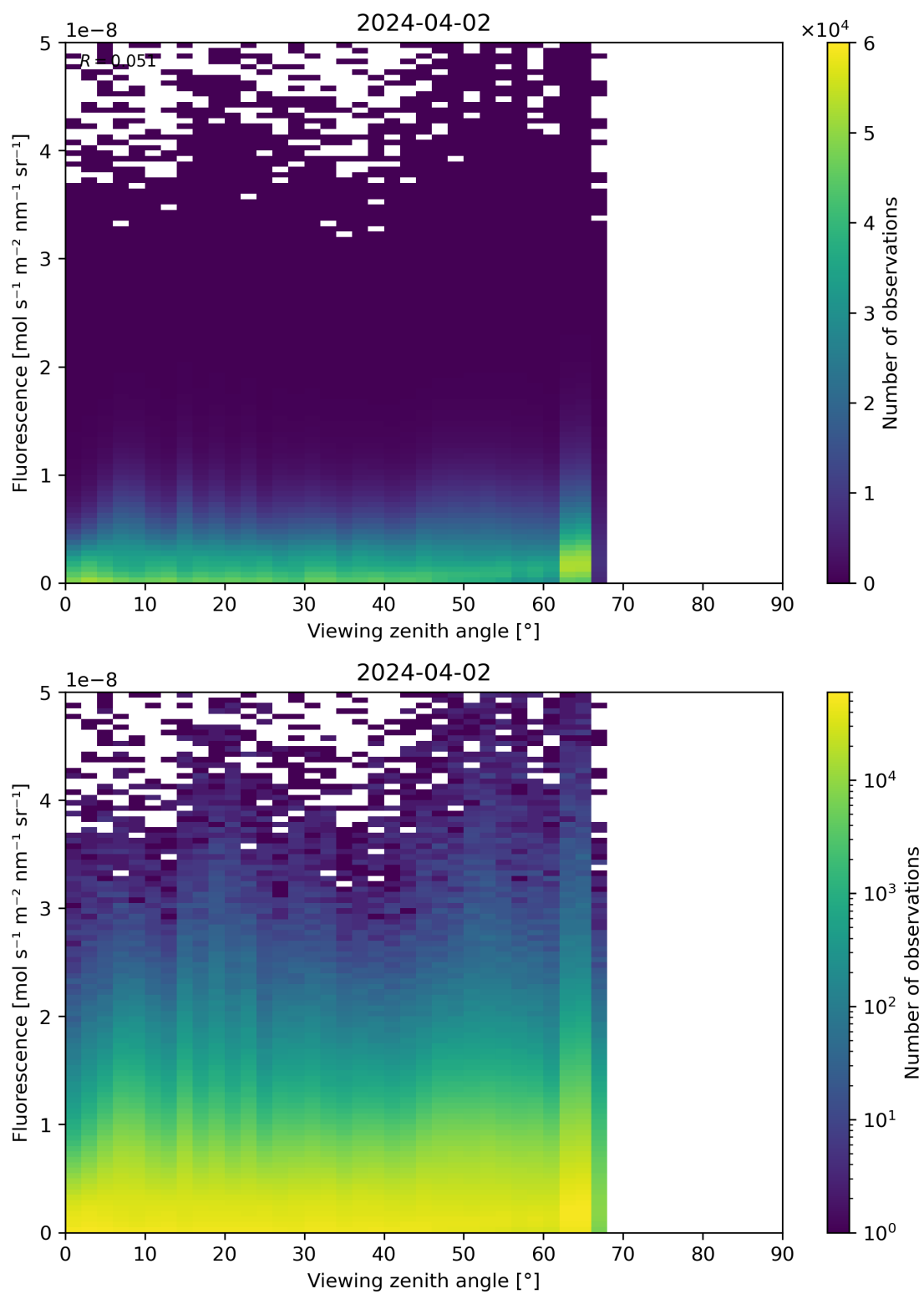
Figure 122: Scatter density plot of “Viewing zenith angle” against “Fluorescence” for 2024-04-01 to 2024-04-03.
