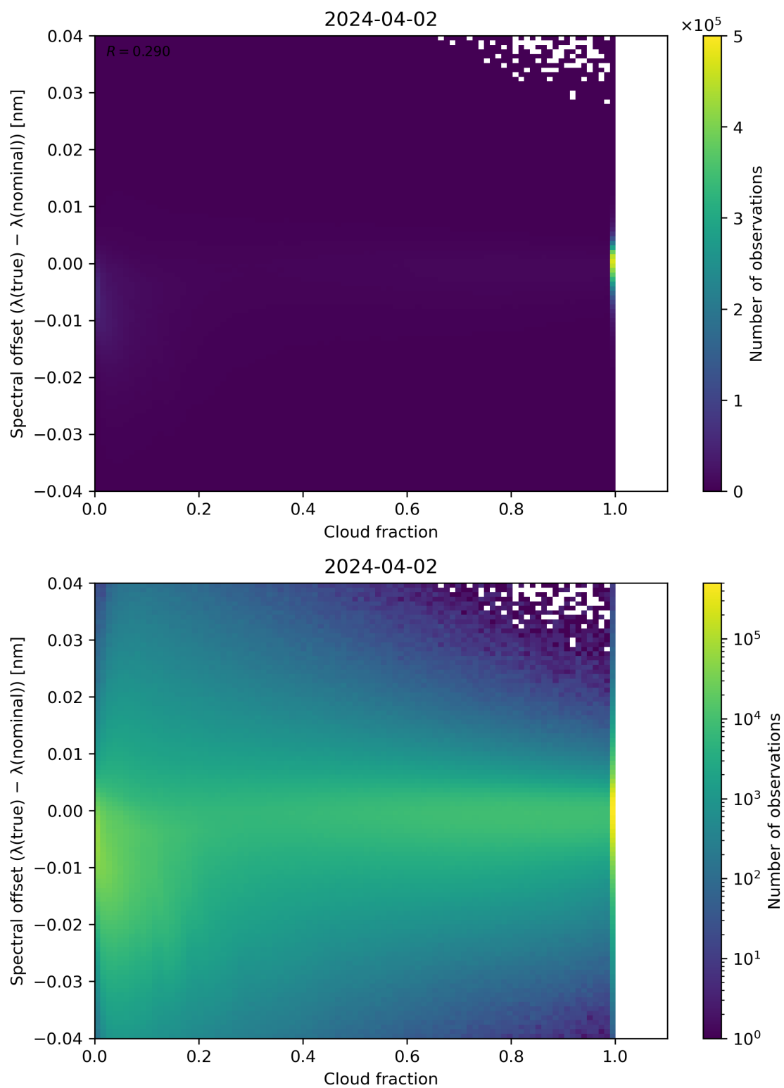
Figure 76: Scatter density plot of “Cloud fraction” against “Spectral offset ( \lambda(\text{true}) - \lambda(\text{nominal}) )” for 2024-04-01 to 2024-04-03.
