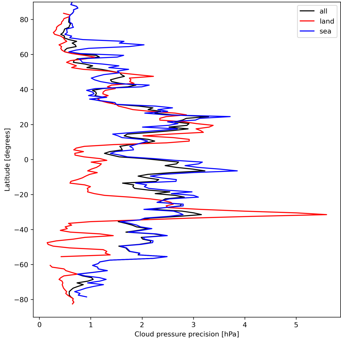
Figure 14: Zonal average of “Cloud pressure precision” for 2024-04-01 to 2024-04-03.
