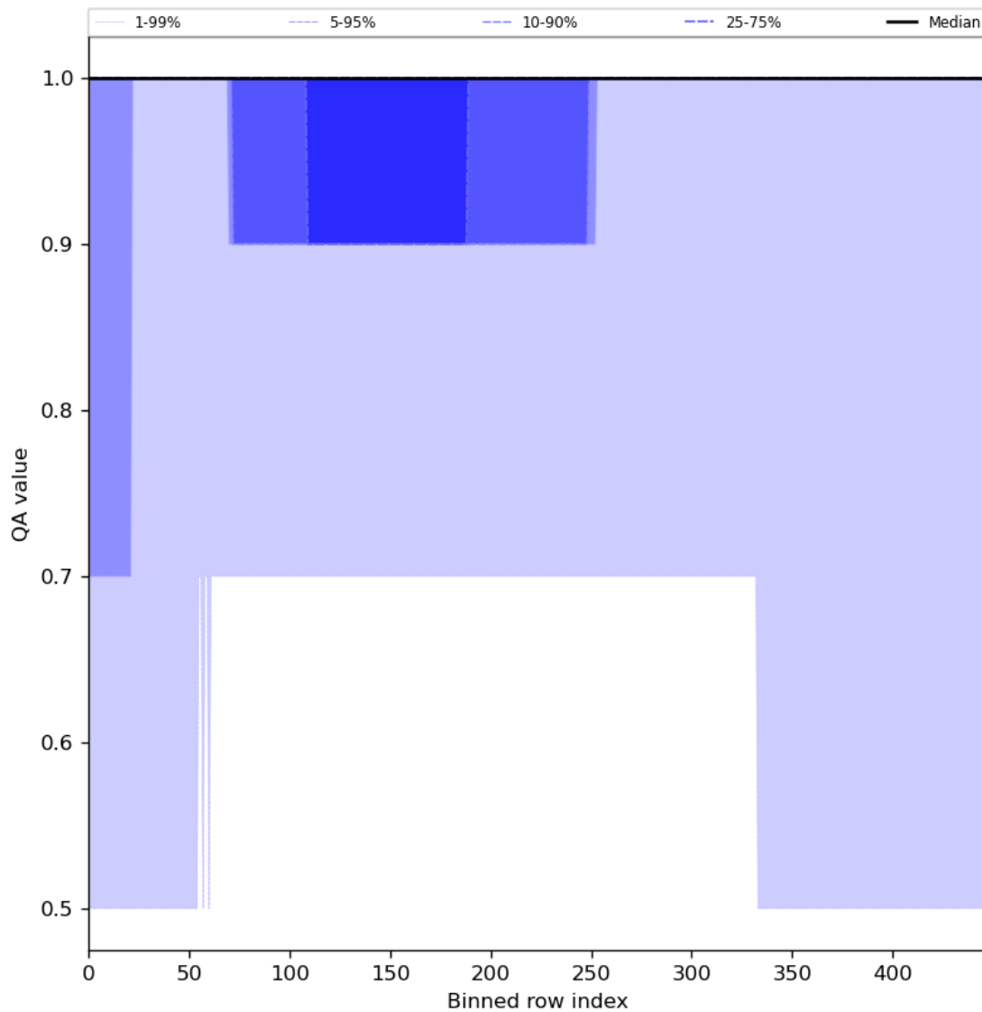
Figure 46: Along track statistics of “QA value” for 2024-04-01 to 2024-04-03
