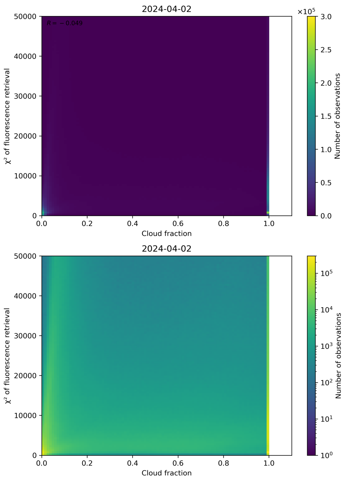
Figure 71: Scatter density plot of “Cloud fraction” against “ \chi^2 of fluorescence retrieval” for 2024-04-01 to 2024-04-03.
