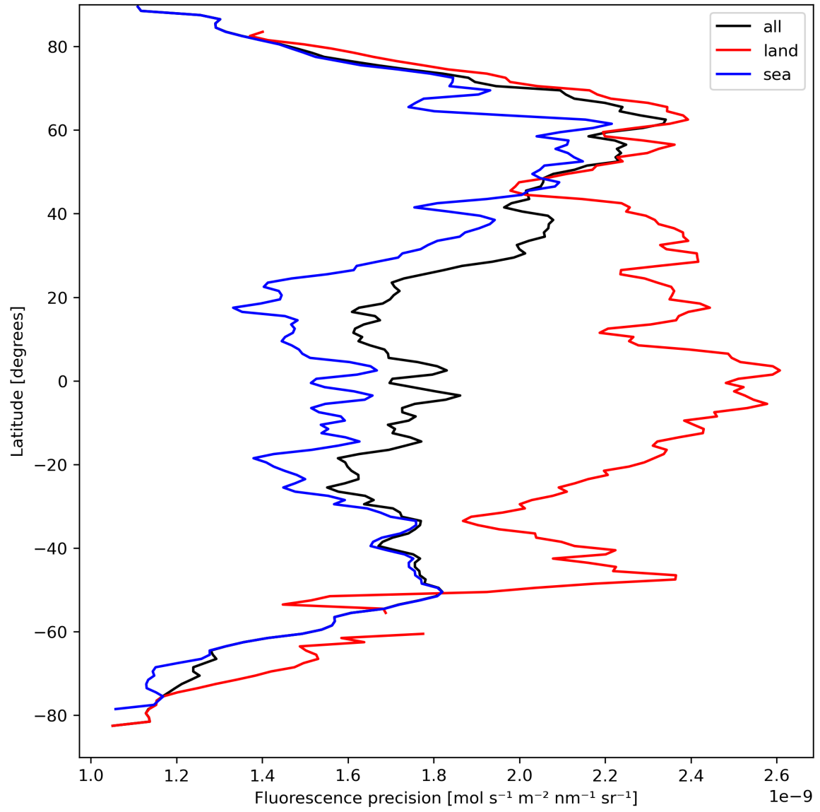
Figure 24: Zonal average of “Fluorescence precision” for 2024-04-01 to 2024-04-03.
