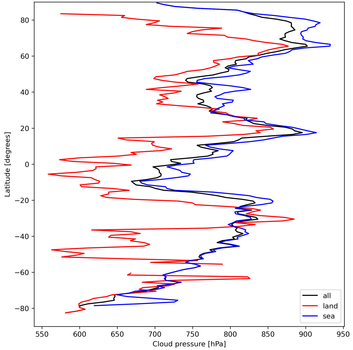
Figure 13: Zonal average of “Cloud pressure” for 2024-04-01 to 2024-04-03.
