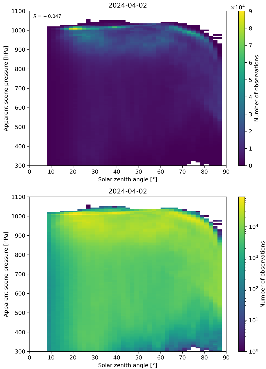
Figure 108: Scatter density plot of “Solar zenith angle” against “Apparent scene pressure” for 2024-04-01 to 2024-04-03.
