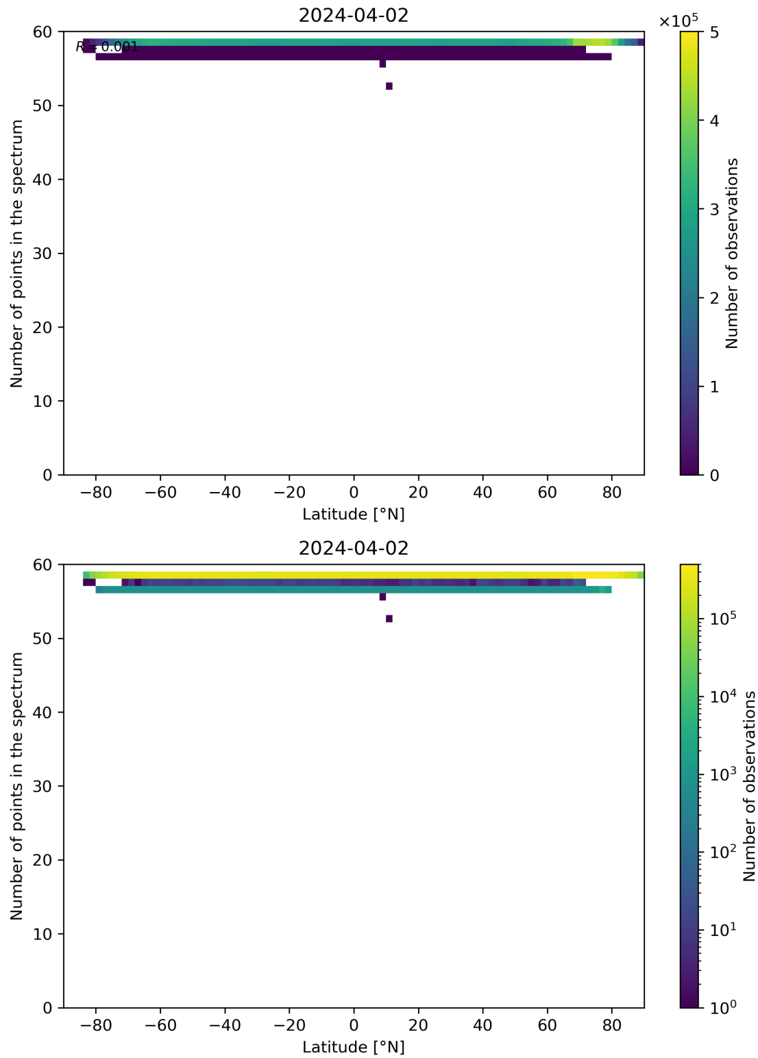
Figure 94: Scatter density plot of “Latitude” against “Number of points in the spectrum” for 2024-04-01 to 2024-04-03.
