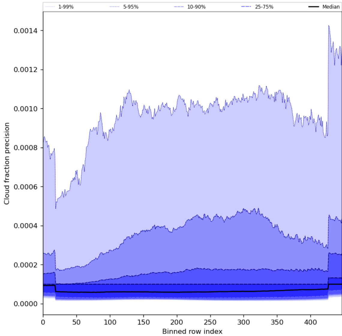
Figure 50: Along track statistics of “Cloud fraction precision” for 2024-04-01 to 2024-04-03
