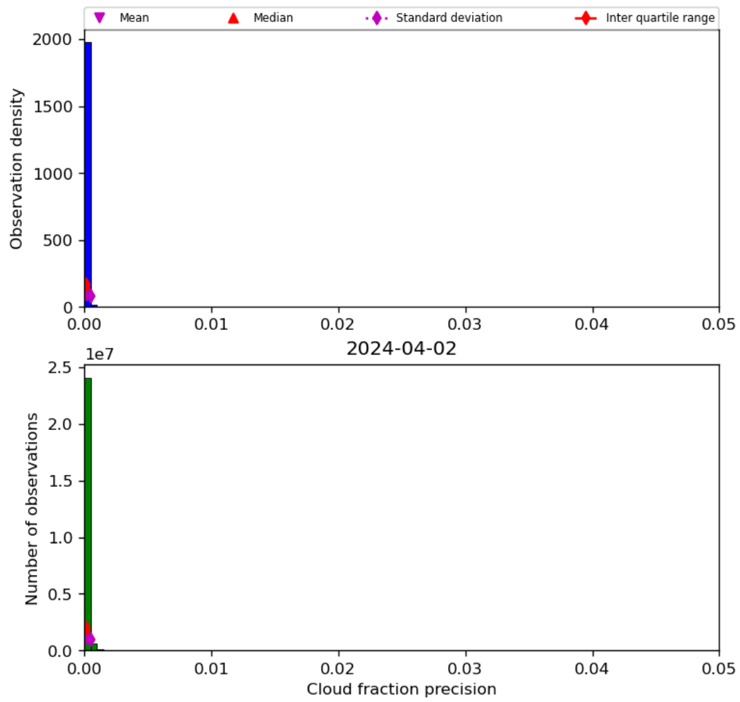
Figure 33: Histogram of “Cloud fraction precision” for 2024-04-01 to 2024-04-03
