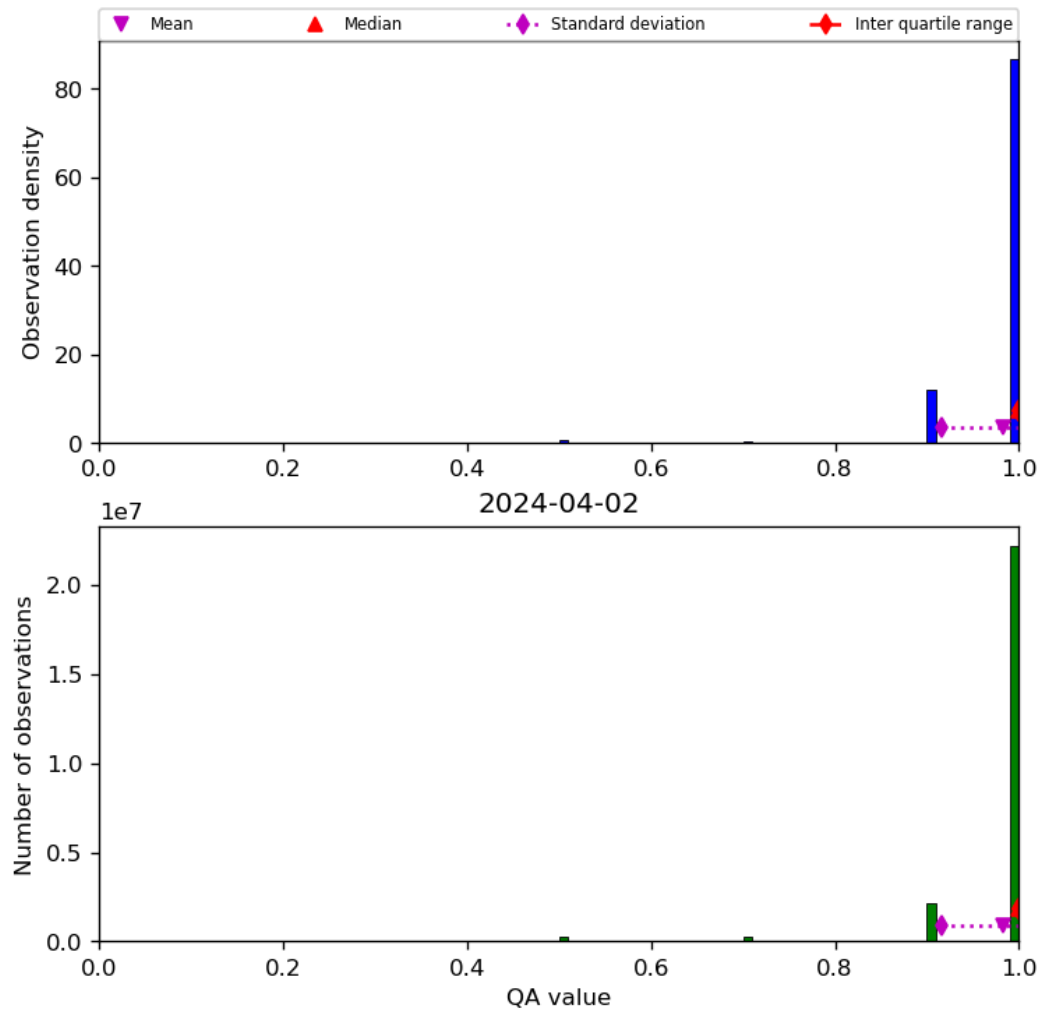
Figure 29: Histogram of “QA value” for 2024-04-01 to 2024-04-03
