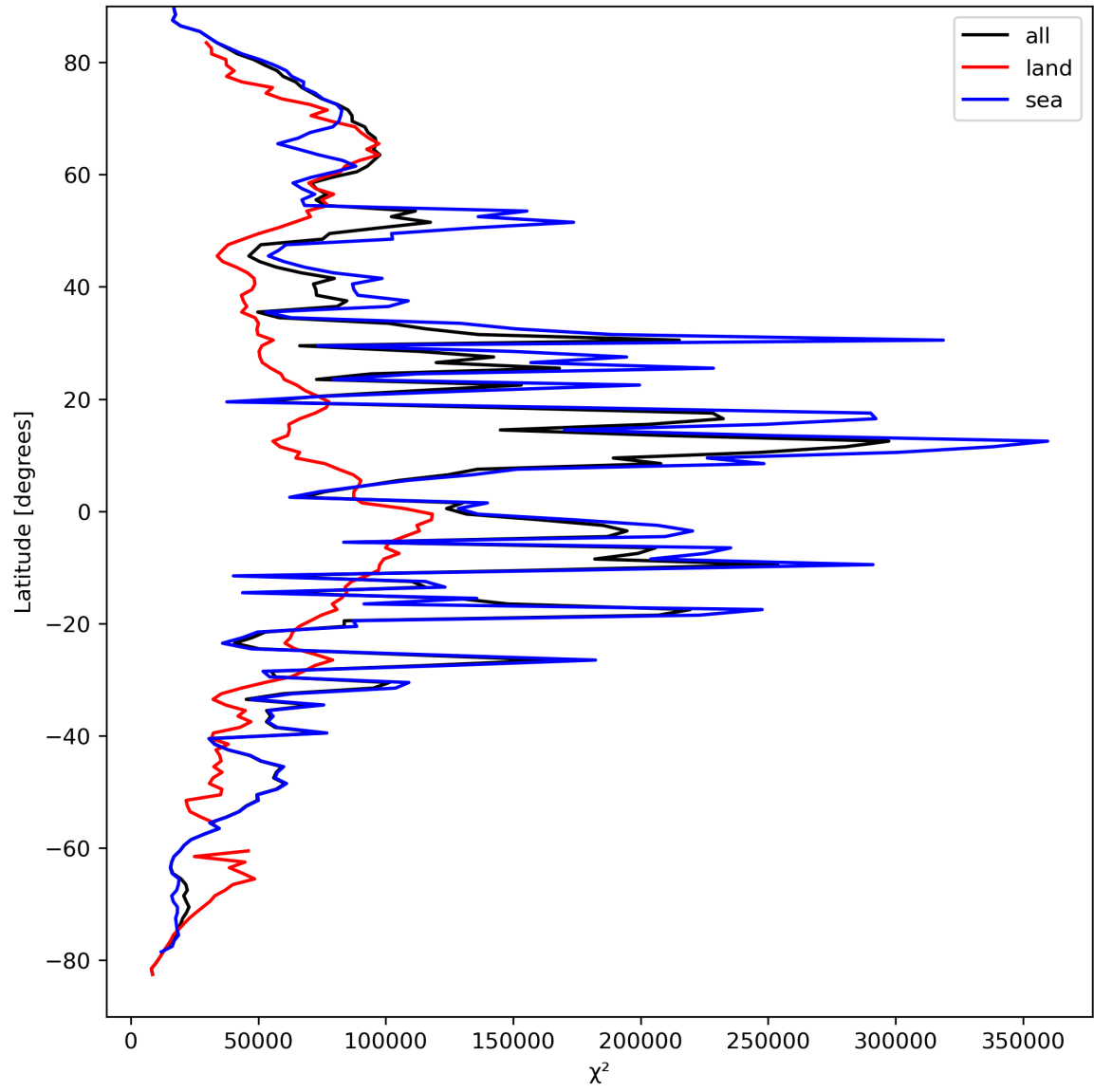
Figure 21: Zonal average of “ \chi^2 ” for 2024-04-01 to 2024-04-03.
