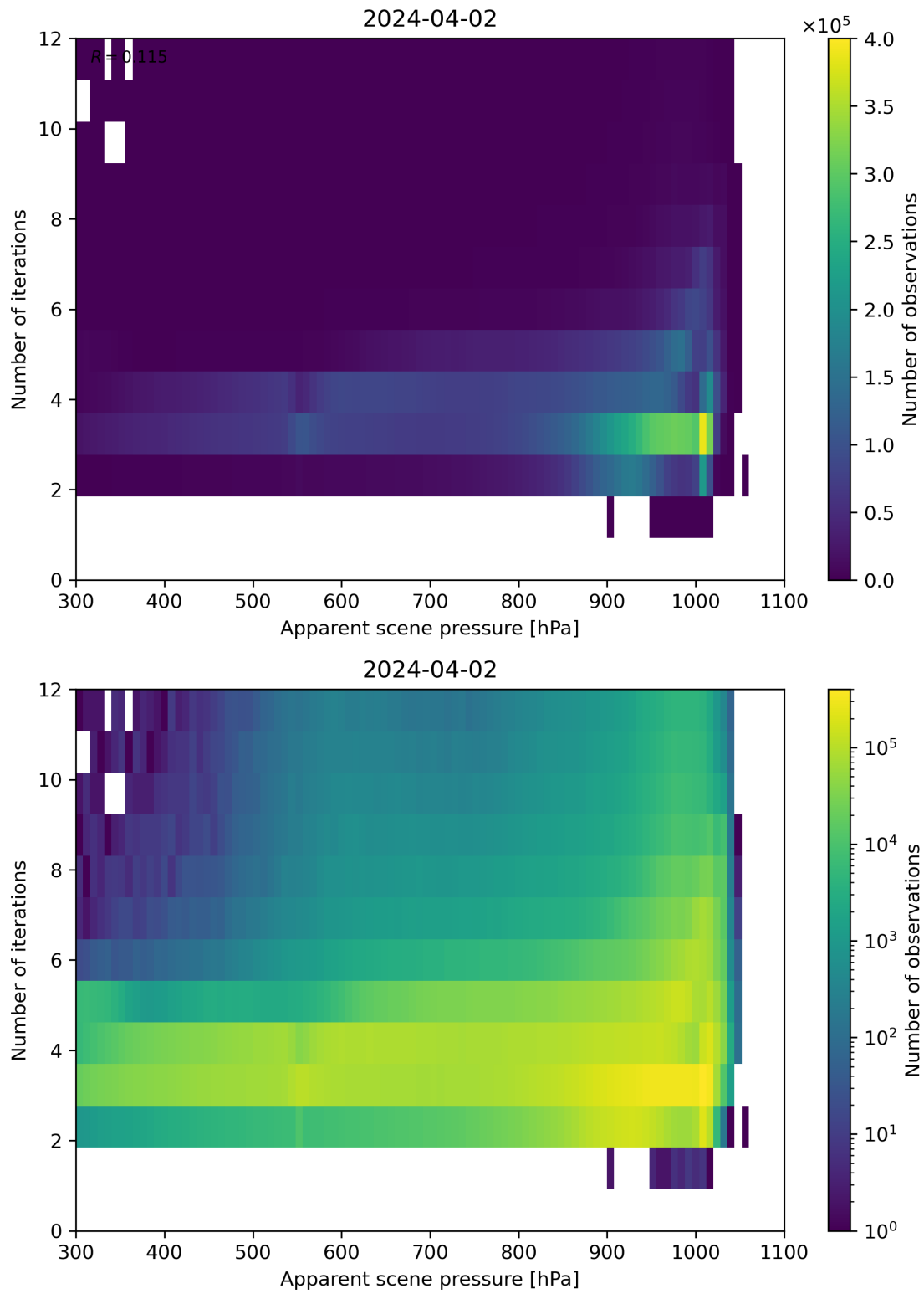
Figure 65: Scatter density plot of “Apparent scene pressure” against “Number of iterations” for 2024-04-01 to 2024-04-03.
