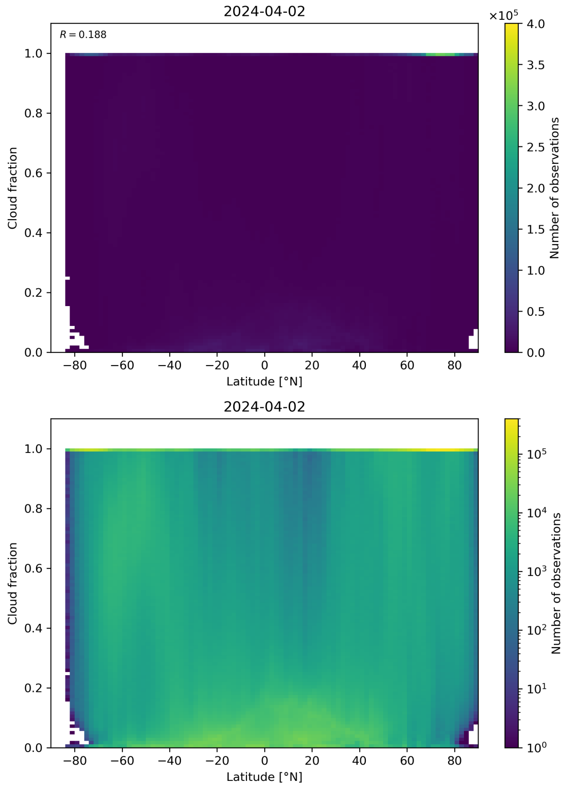
Figure 90: Scatter density plot of “Latitude” against “Cloud fraction” for 2024-04-01 to 2024-04-03.
