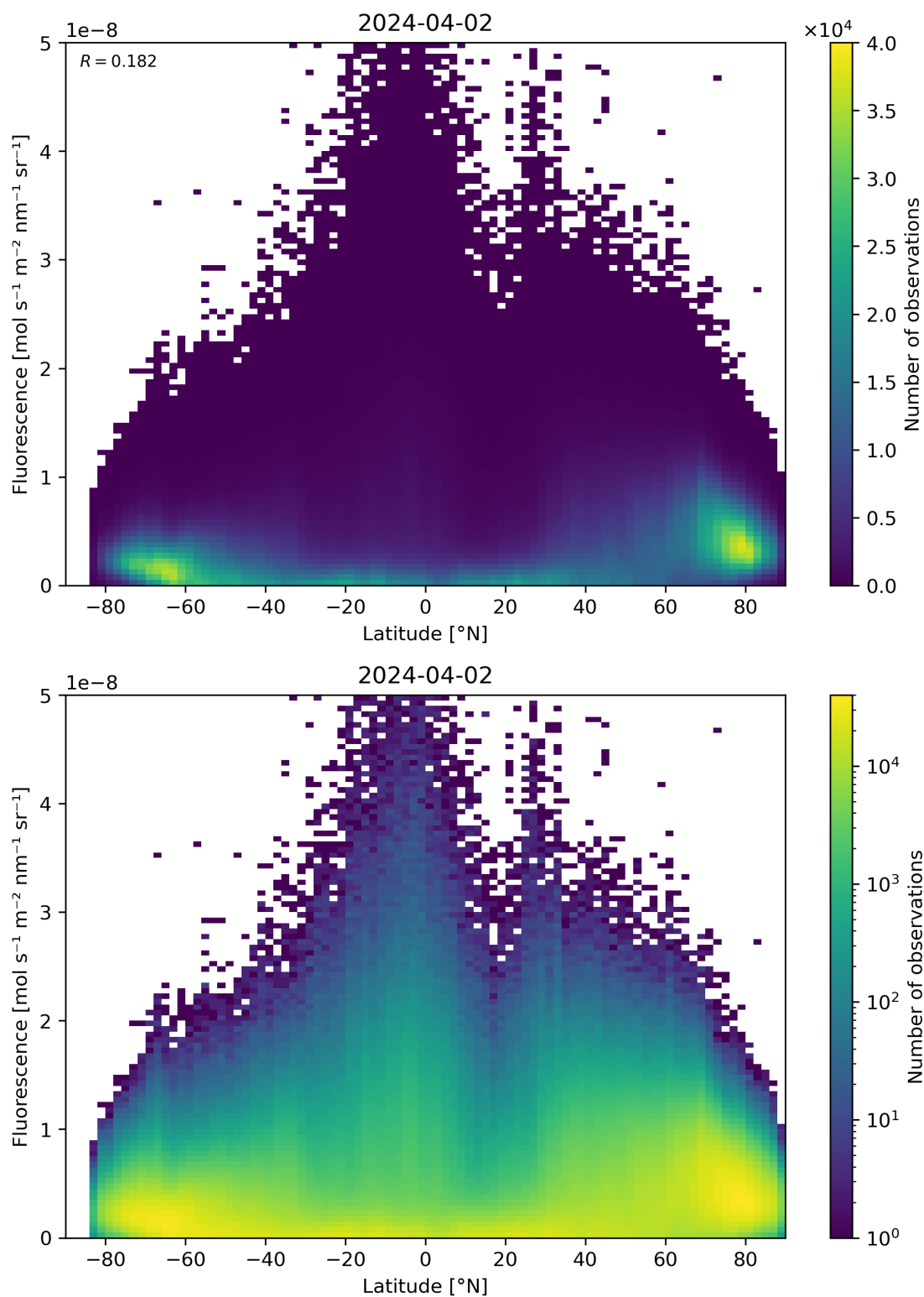
Figure 92: Scatter density plot of “Latitude” against “Fluorescence” for 2024-04-01 to 2024-04-03.
