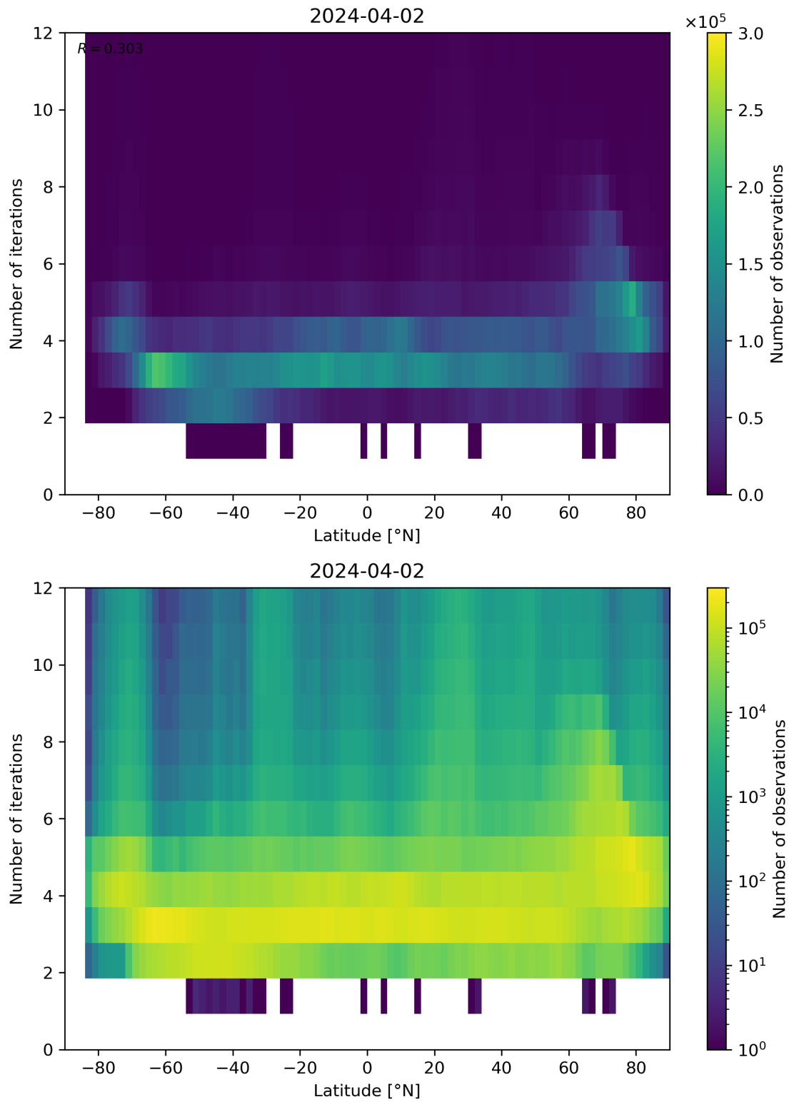
Figure 93: Scatter density plot of “Latitude” against “Number of iterations” for 2024-04-01 to 2024-04-03.
