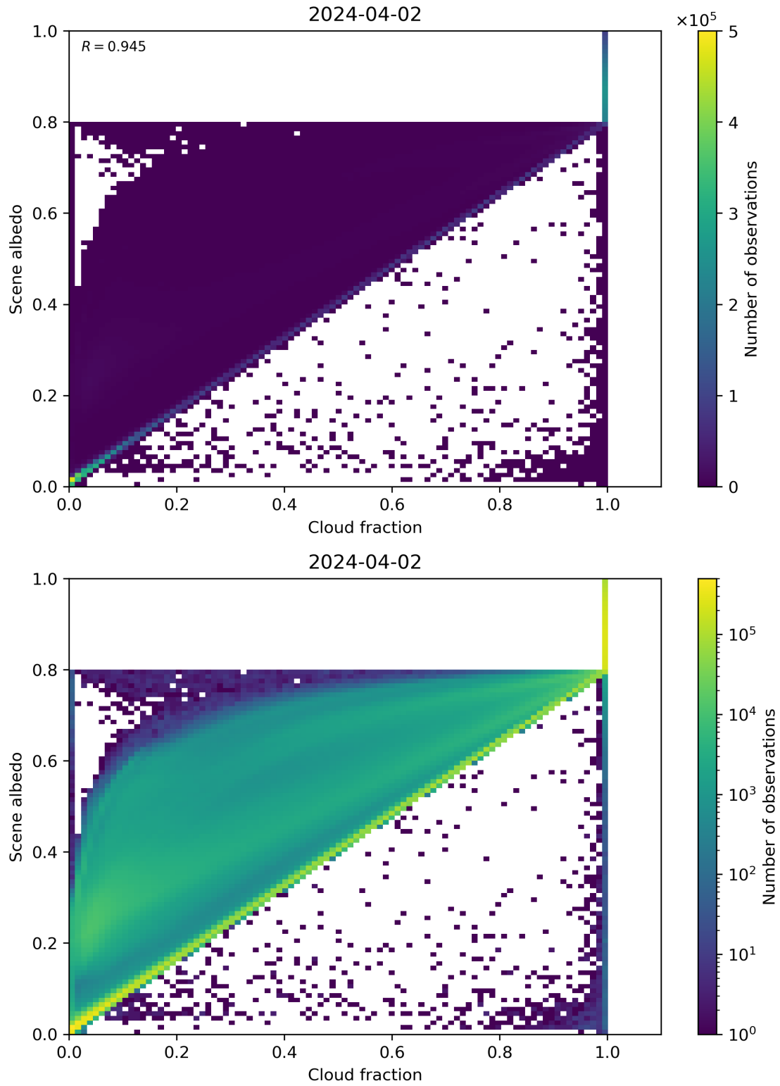
Figure 75: Scatter density plot of “Cloud fraction” against “Scene albedo” for 2024-04-01 to 2024-04-03.
