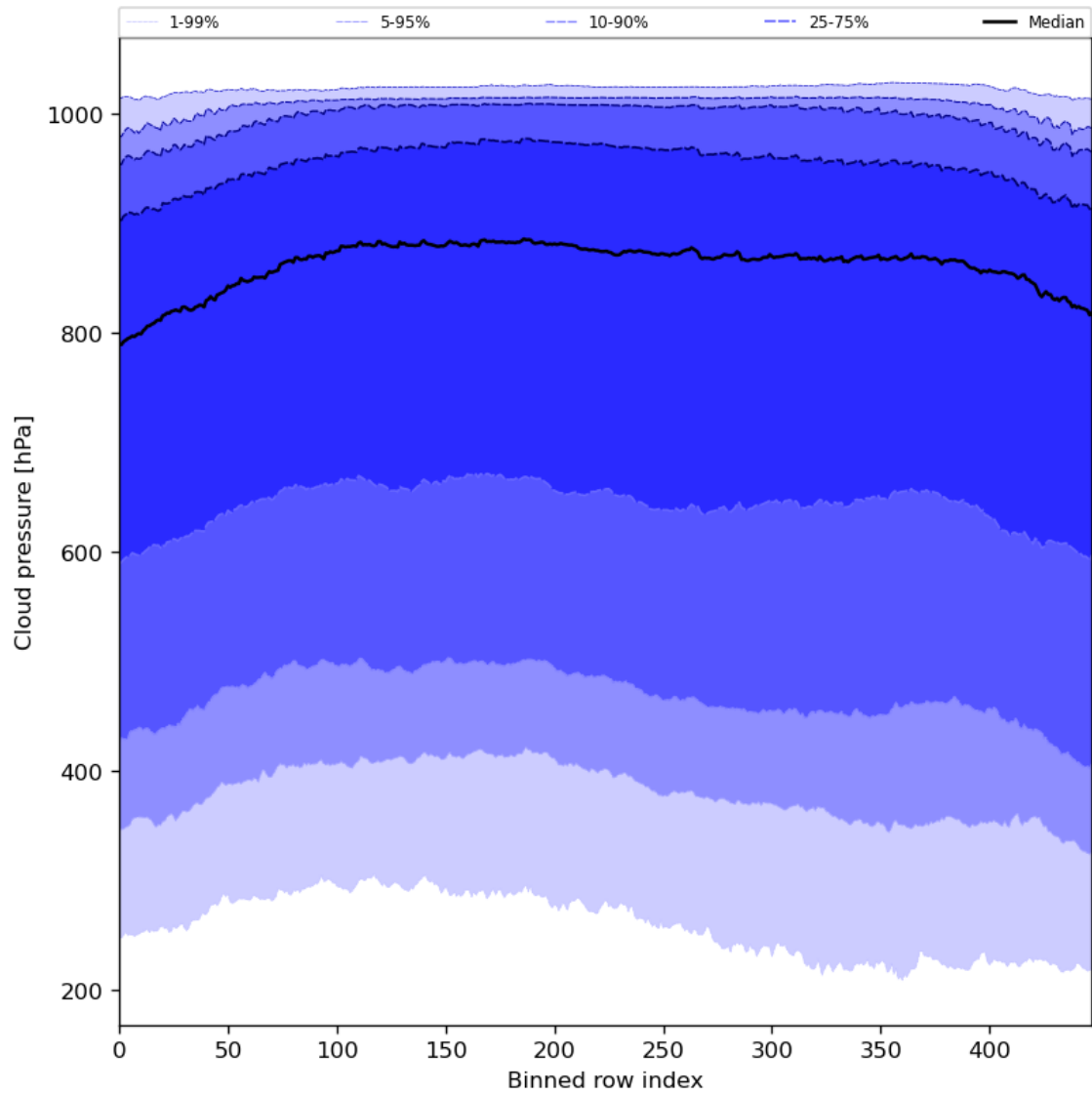
Figure 47: Along track statistics of “Cloud pressure” for 2024-04-01 to 2024-04-03
