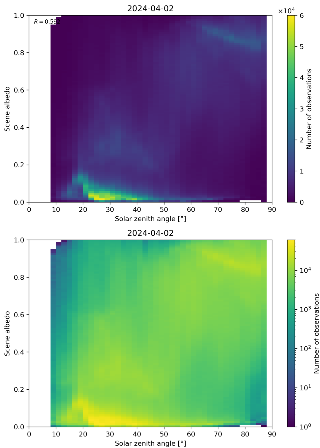
Figure 116: Scatter density plot of “Solar zenith angle” against “Scene albedo” for 2024-04-01 to 2024-04-03.
