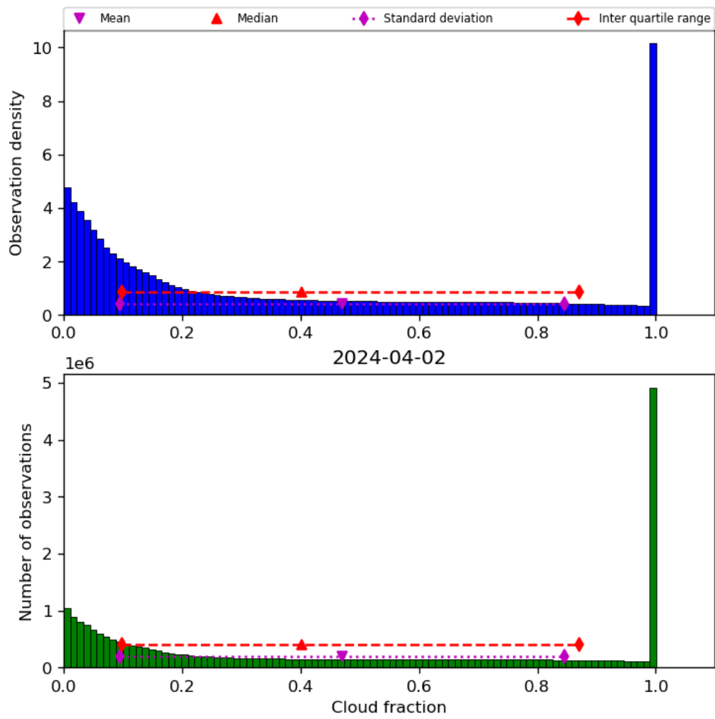
Figure 32: Histogram of “Cloud fraction” for 2024-04-01 to 2024-04-03
