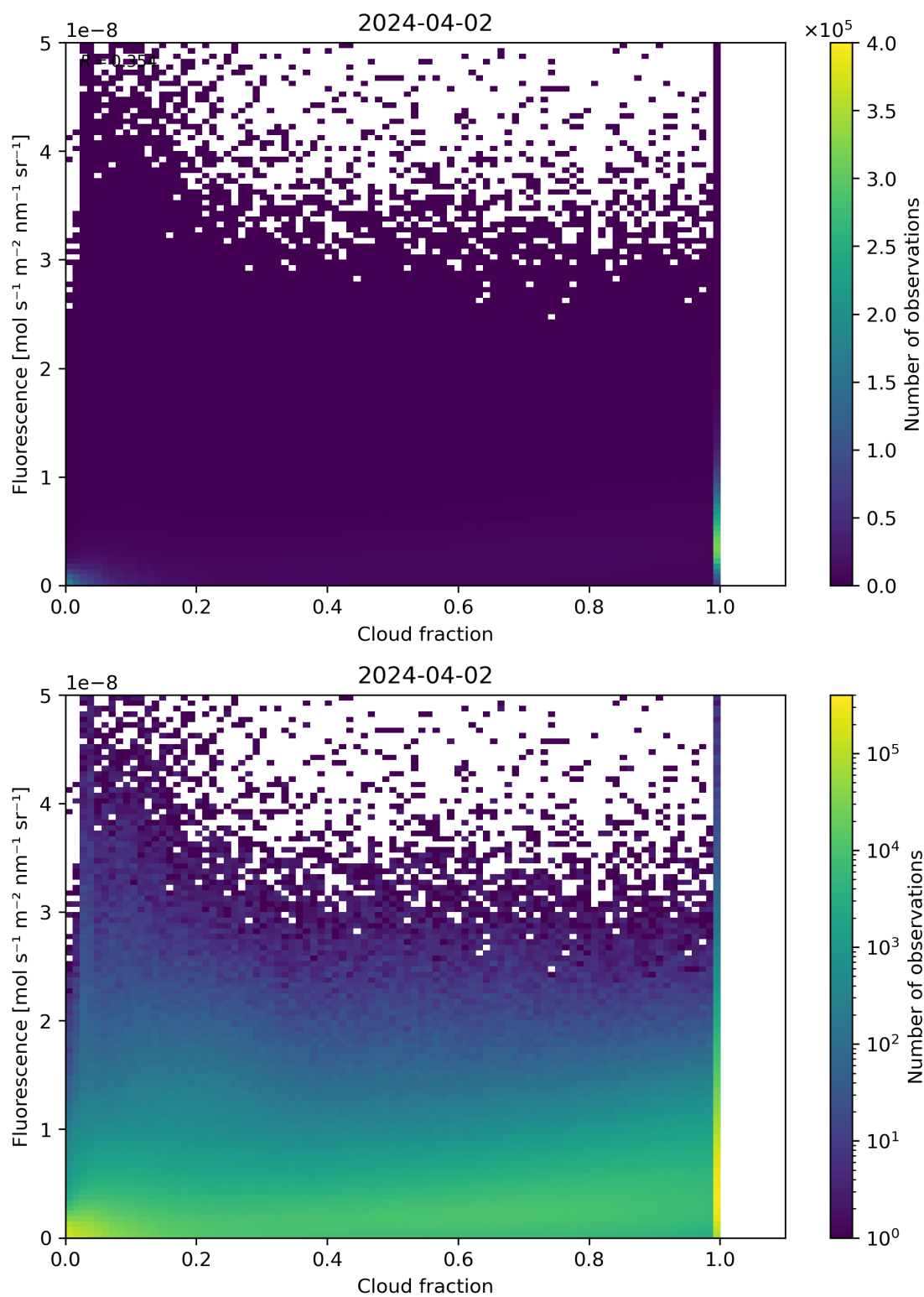
Figure 72: Scatter density plot of “Cloud fraction” against “Fluorescence” for 2024-04-01 to 2024-04-03.
