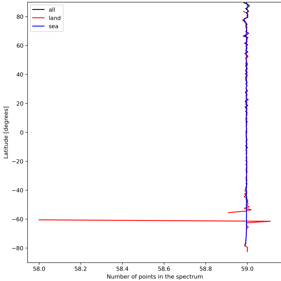
Figure 27: Zonal average of “Number of points in the spectrum” for 2024-04-01 to 2024-04-03.
