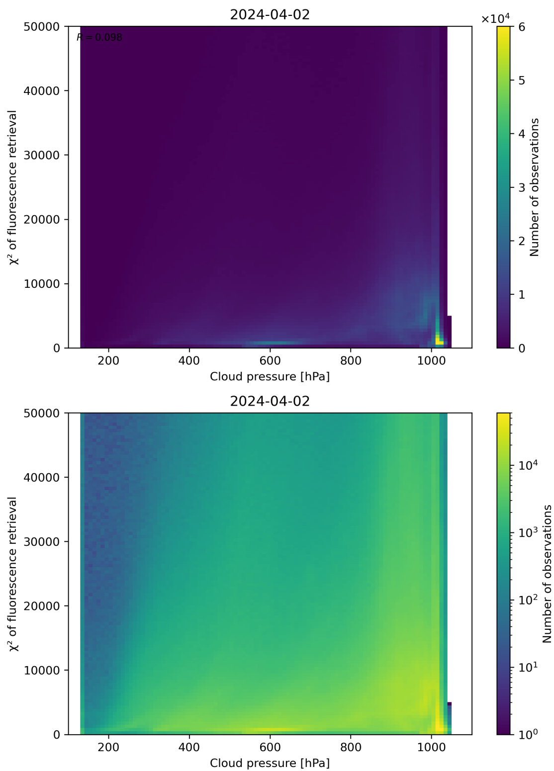
Figure 78: Scatter density plot of “Cloud pressure” against “ \chi^2 of fluorescence retrieval” for 2024-04-01 to 2024-04-03.
