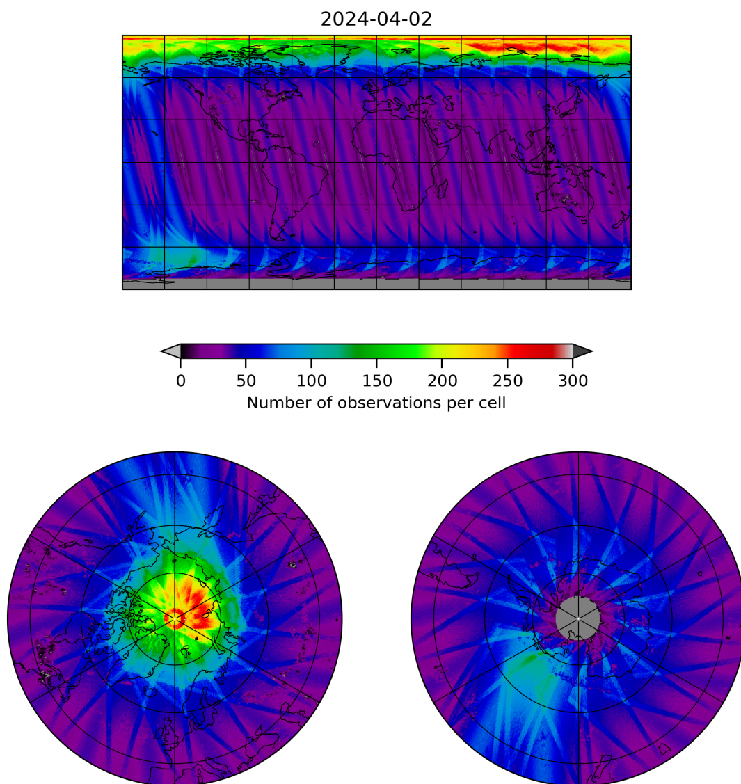
Figure 11: Map of the number of observations for 2024-04-01 to 2024-04-03
