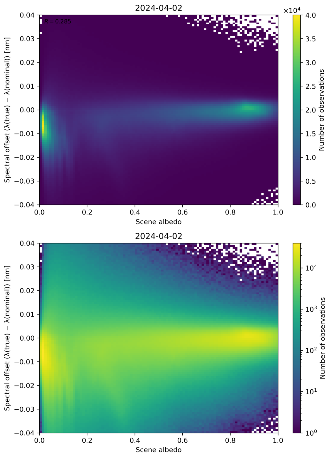
Figure 107: Scatter density plot of “Scene albedo” against “Spectral offset ( \lambda(\text{true}) - \lambda(\text{nominal}) )” for 2024-04-01 to 2024-04-03.
