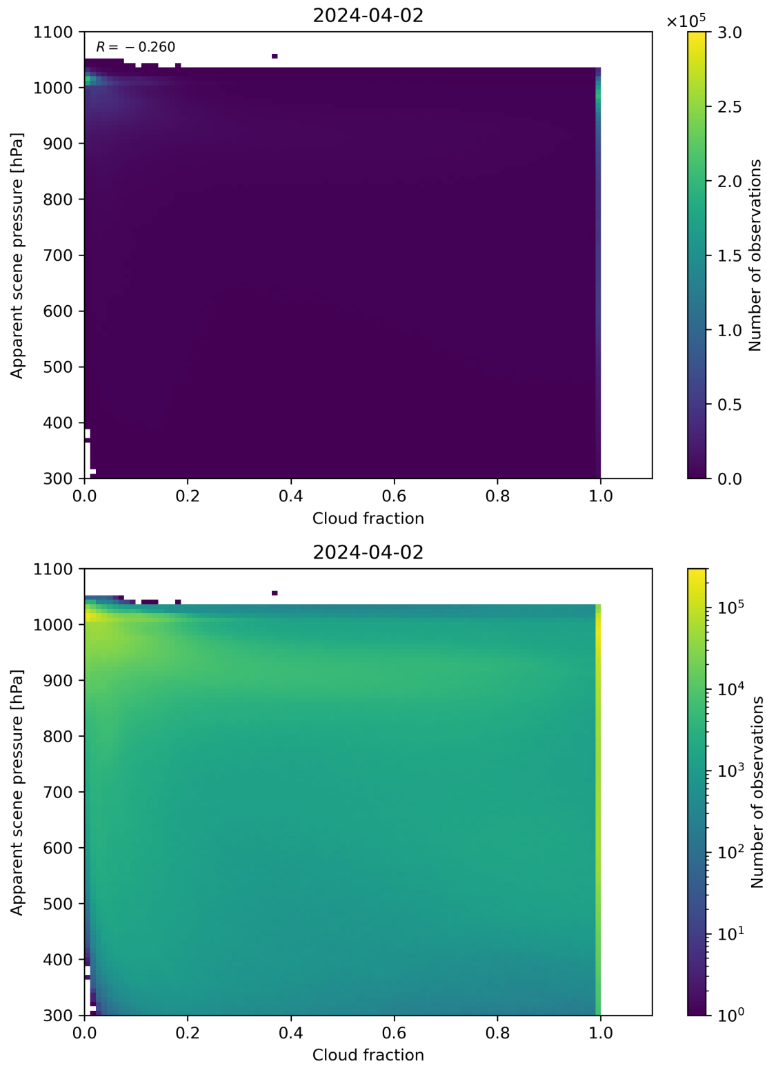
Figure 70: Scatter density plot of “Cloud fraction” against “Apparent scene pressure” for 2024-04-01 to 2024-04-03.
