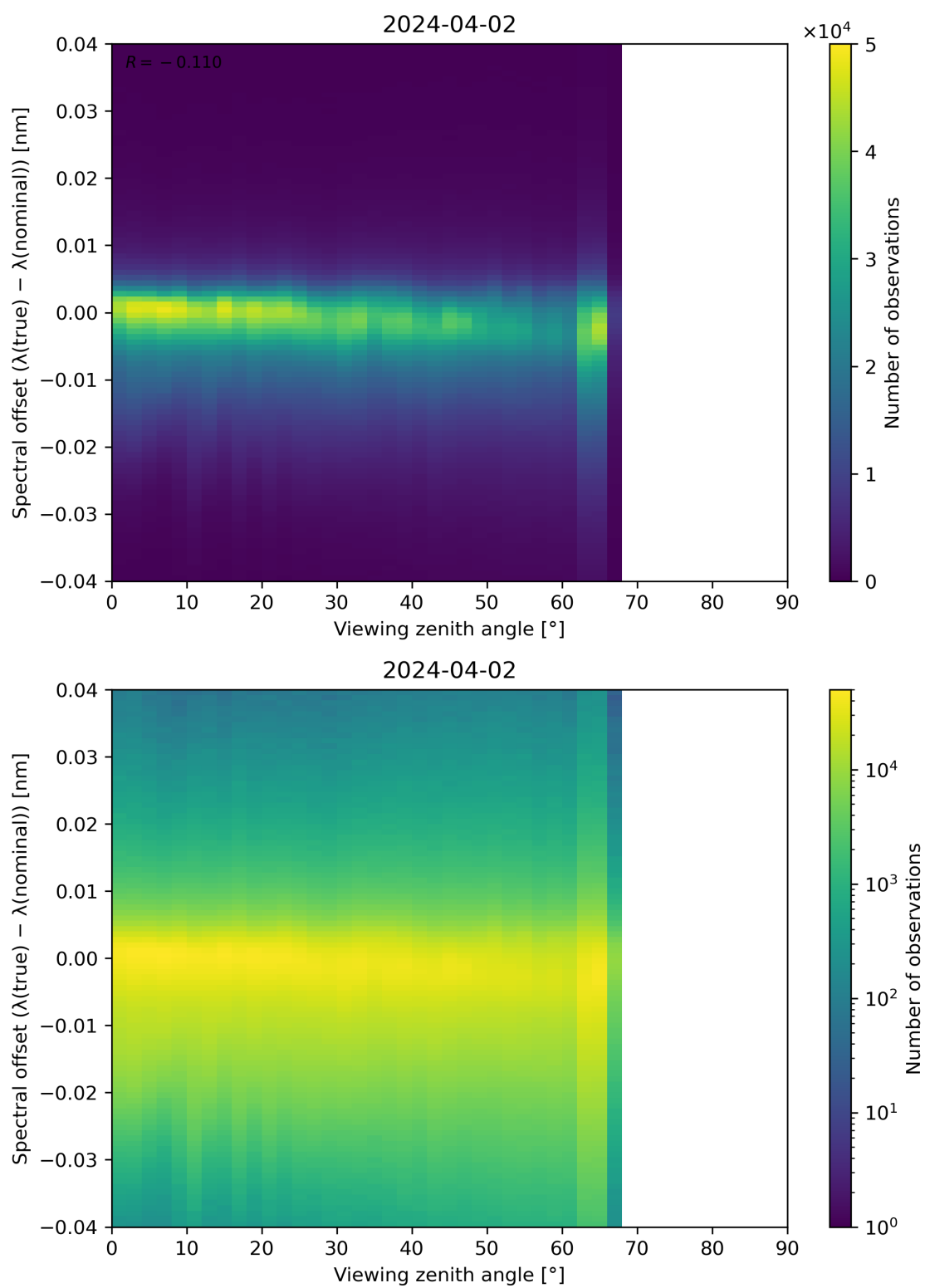
Figure 128: Scatter density plot of “Viewing zenith angle” against “Spectral offset ( \lambda(\text{true}) - \lambda(\text{nominal}) )” for 2024-04-01 to 2024-04-03.
