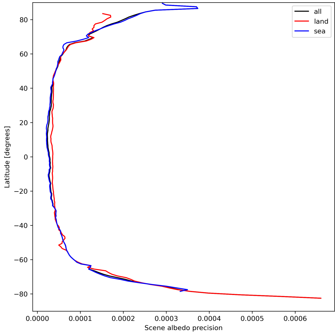
Figure 18: Zonal average of “Scene albedo precision” for 2024-04-01 to 2024-04-03.
