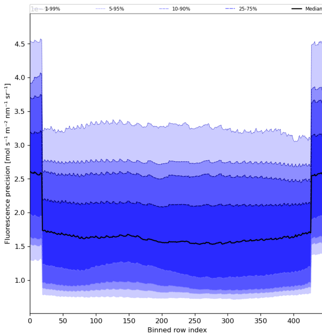
Figure 58: Along track statistics of “Fluorescence precision” for 2024-04-01 to 2024-04-03
