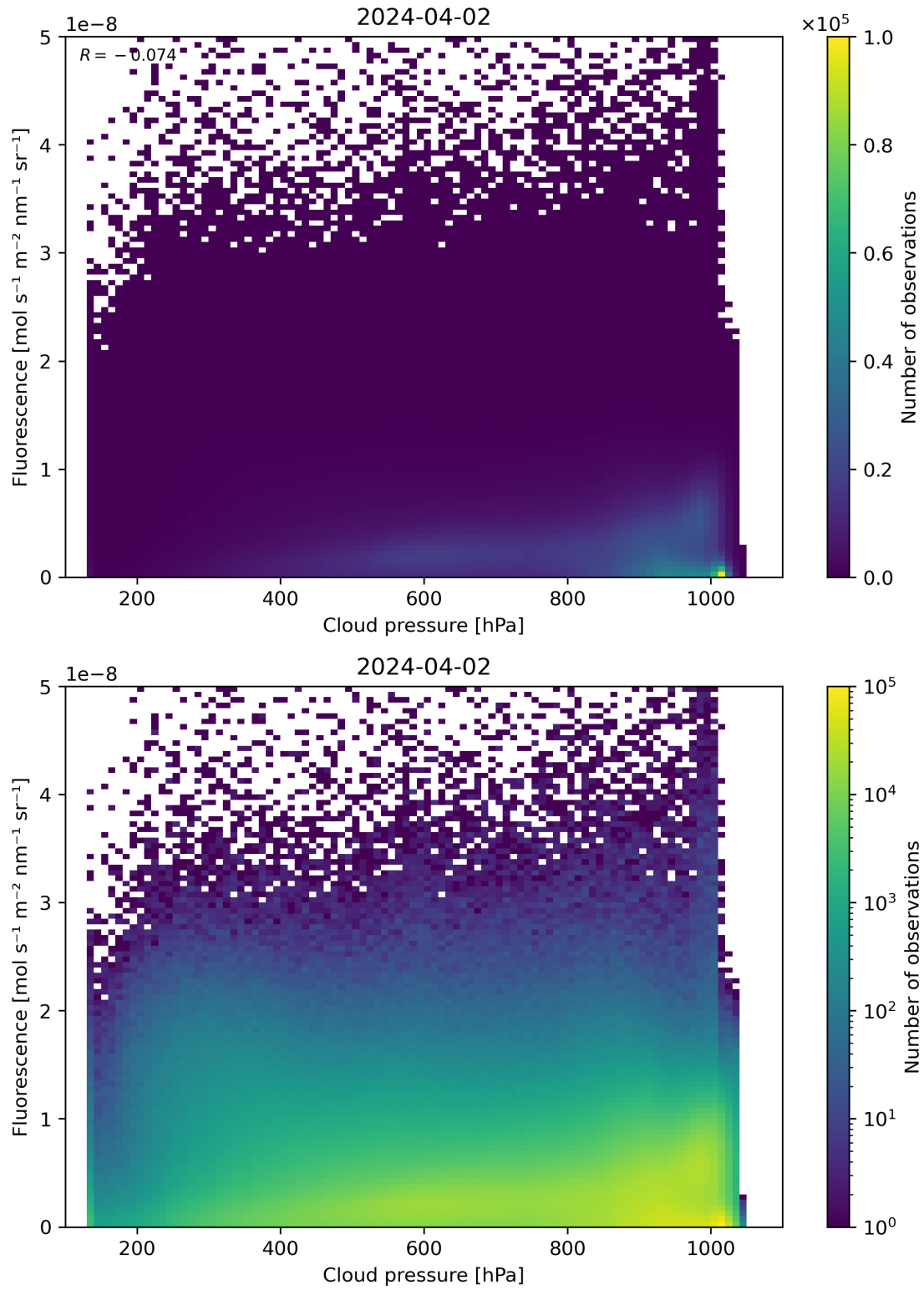
Figure 80: Scatter density plot of “Cloud pressure” against “Fluorescence” for 2024-04-01 to 2024-04-03.
