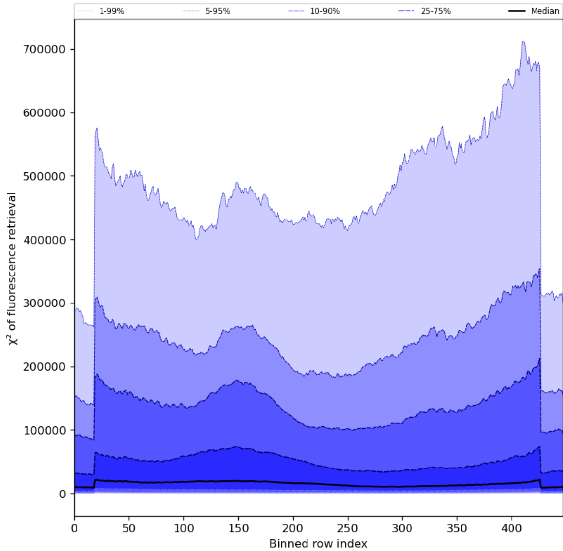
Figure 59: Along track statistics of “ \chi^2 of fluorescence retrieval” for 2024-04-01 to 2024-04-03
