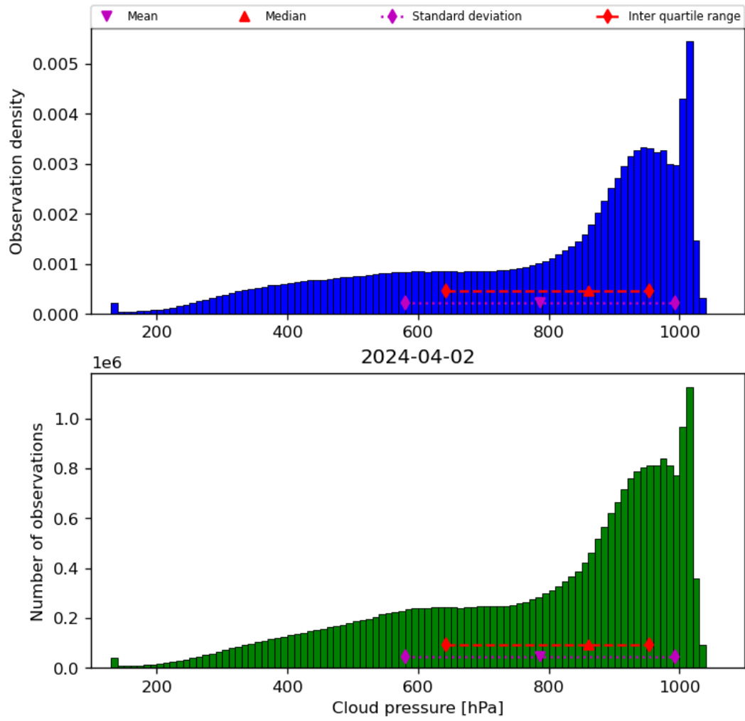
Figure 30: Histogram of “Cloud pressure” for 2024-04-01 to 2024-04-03
