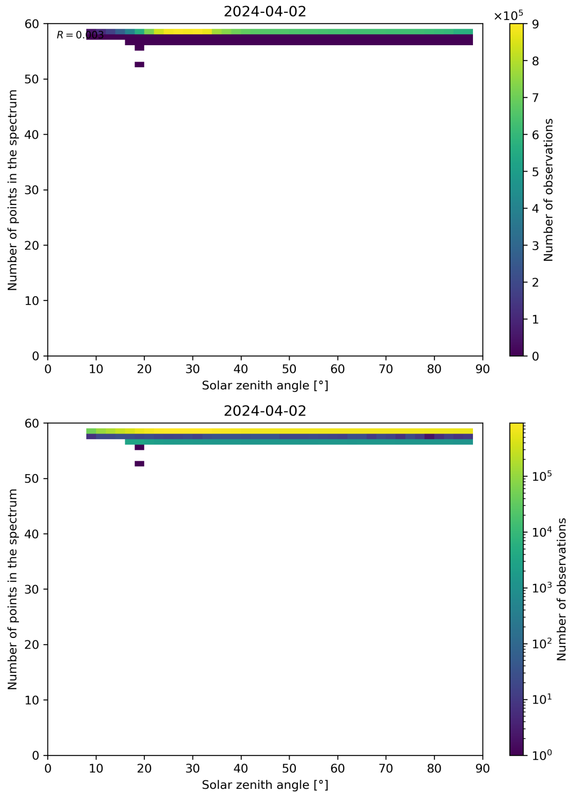
Figure 115: Scatter density plot of “Solar zenith angle” against “Number of points in the spectrum” for 2024-04-01 to 2024-04-03.
