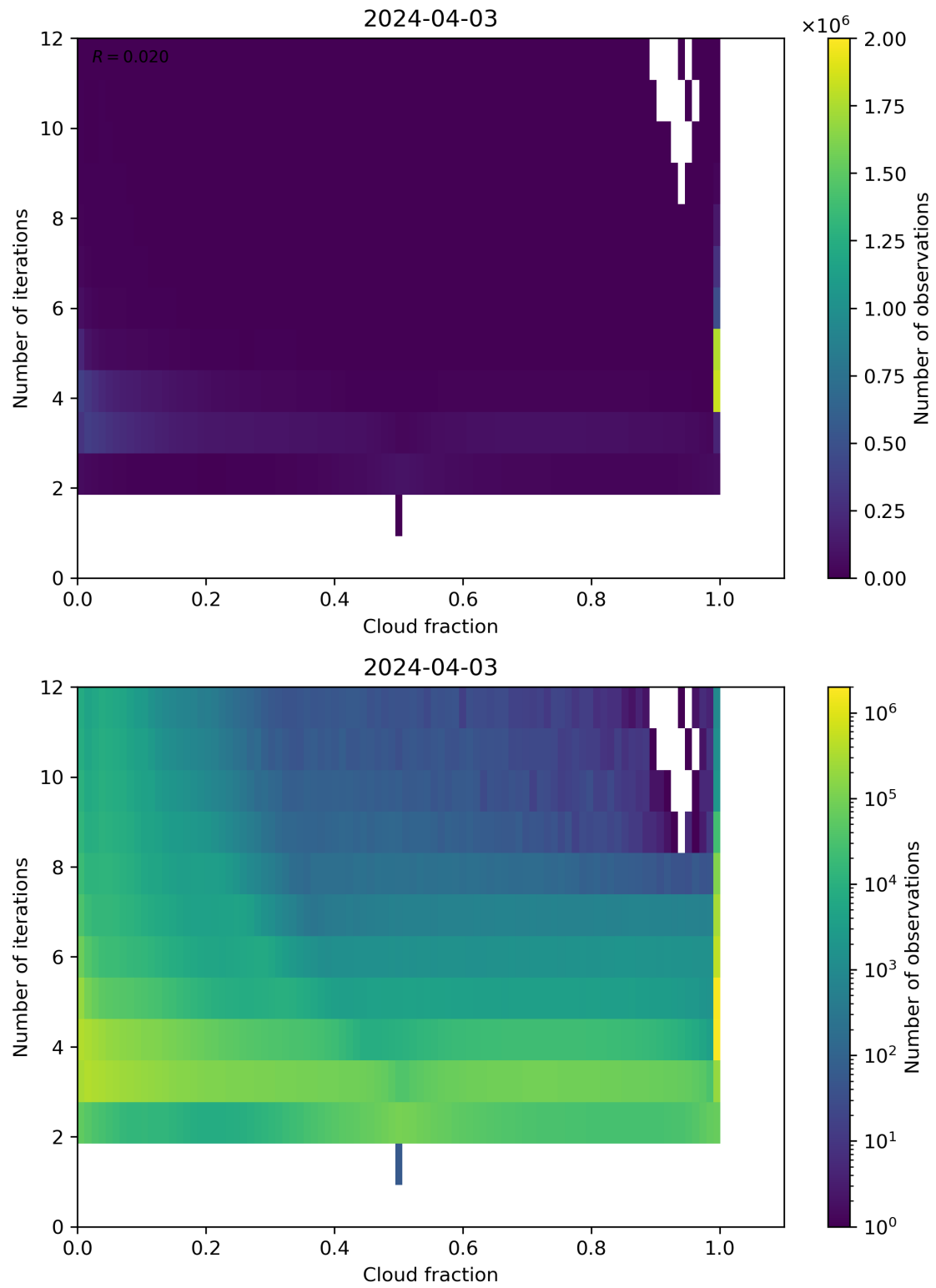
Figure 73: Scatter density plot of “Cloud fraction” against “Number of iterations” for 2024-04-02 to 2024-04-04.
