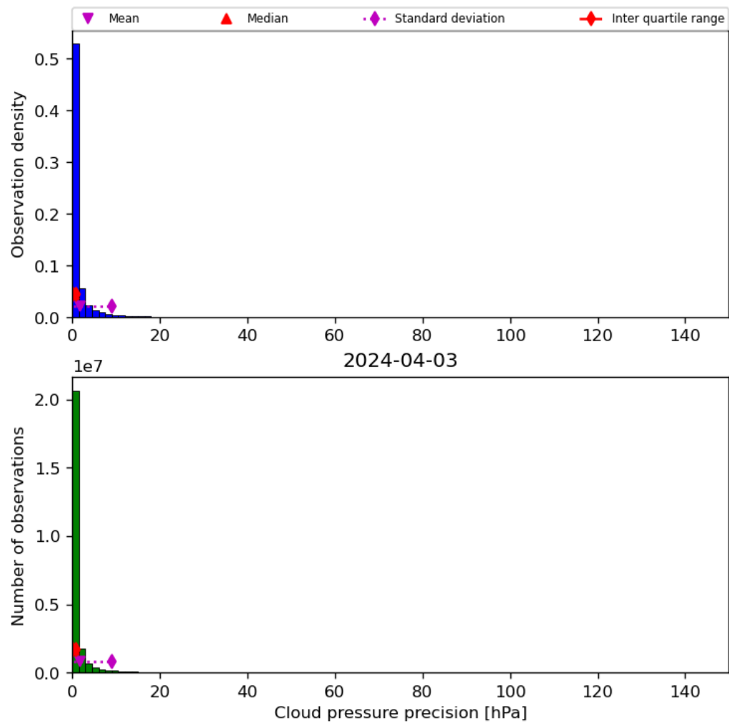
Figure 31: Histogram of “Cloud pressure precision” for 2024-04-02 to 2024-04-04
