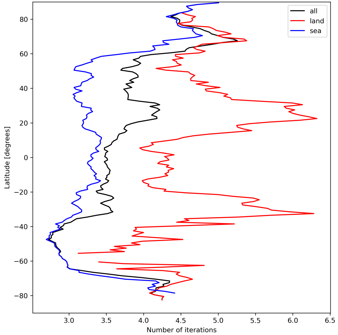
Figure 22: Zonal average of “Number of iterations” for 2024-04-02 to 2024-04-04.
