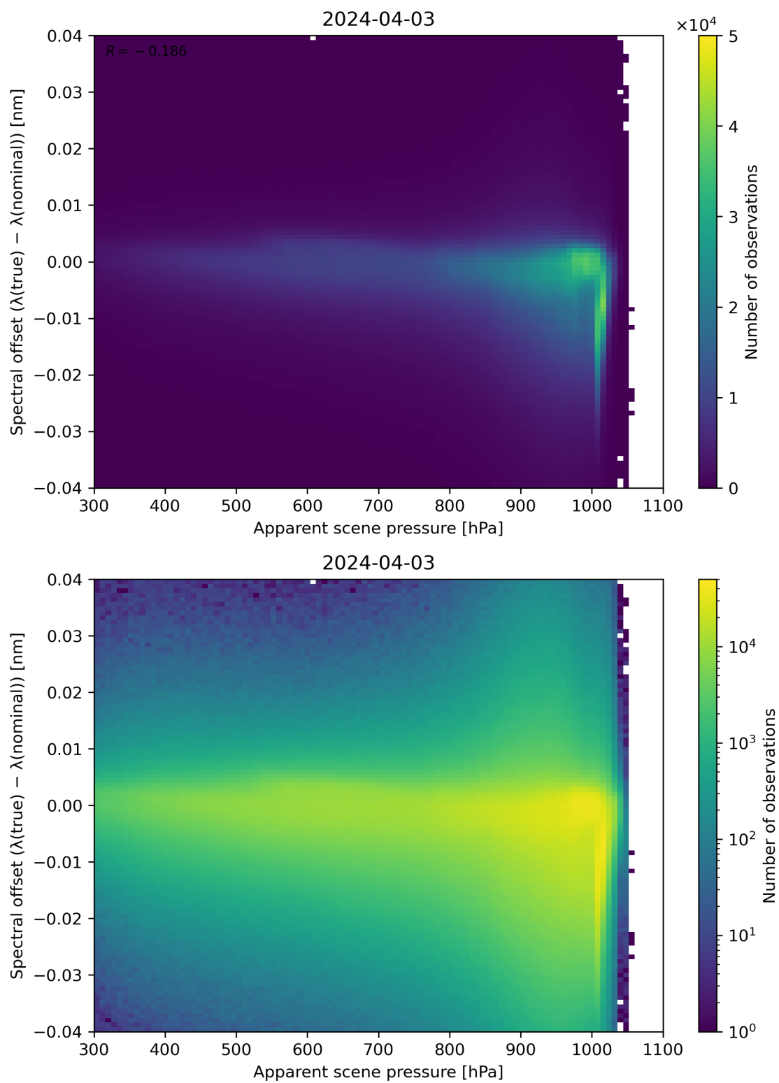
Figure 67: Scatter density plot of “Apparent scene pressure” against “Spectral offset ( \lambda(\text{true}) - \lambda(\text{nominal}) )” for 2024-04-02 to 2024-04-04.
