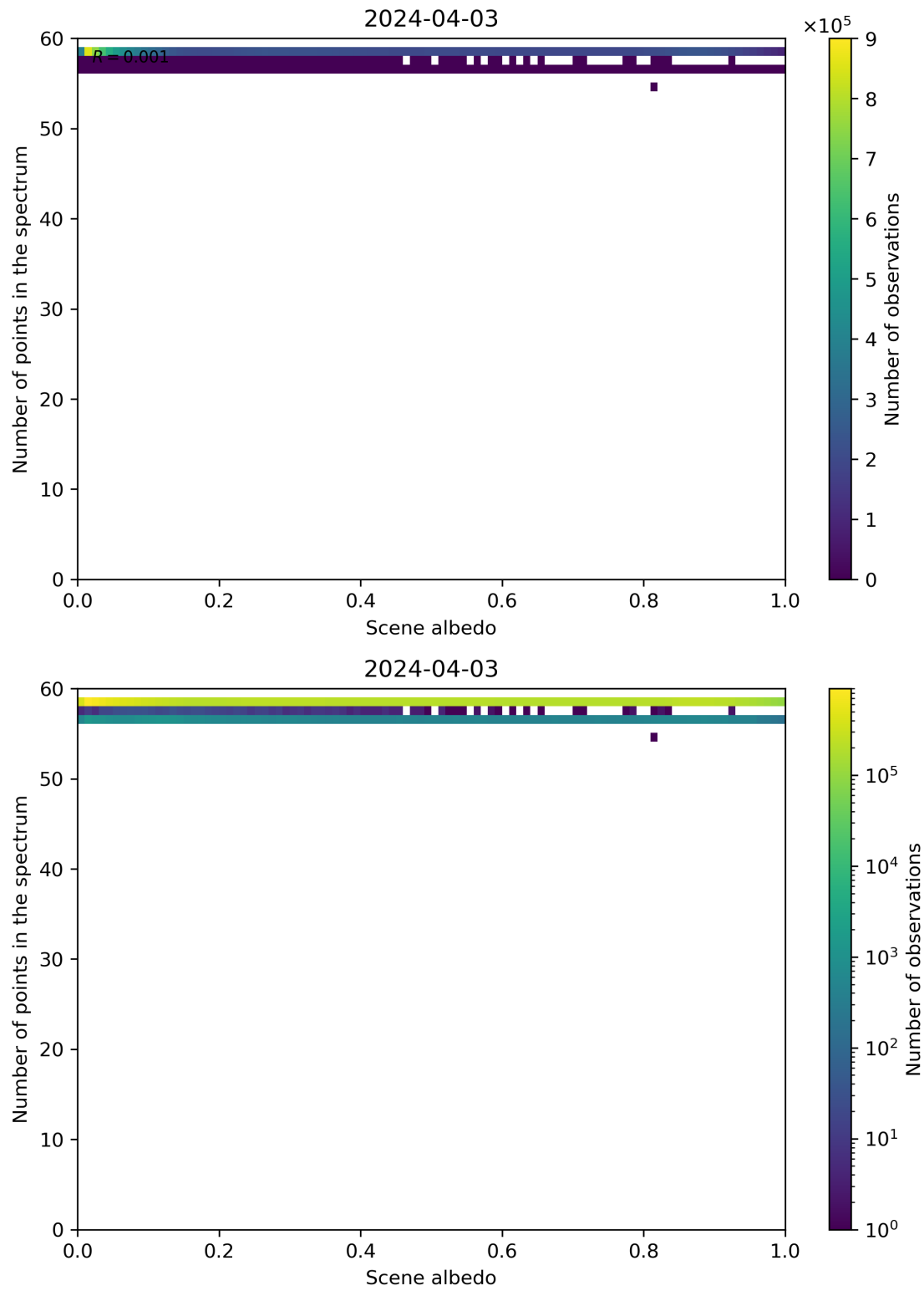
Figure 106: Scatter density plot of “Scene albedo” against “Number of points in the spectrum” for 2024-04-02 to 2024-04-04.
