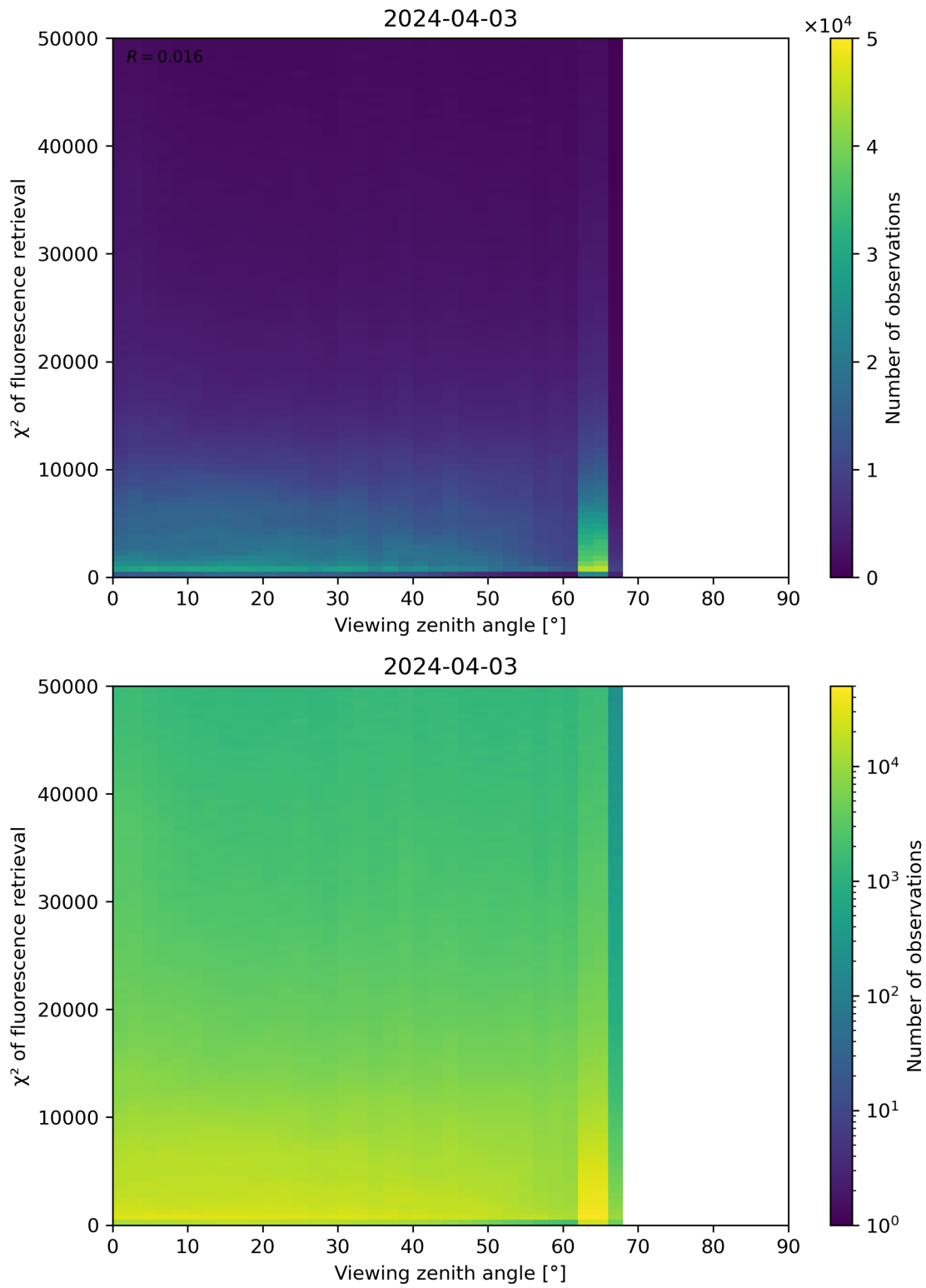
Figure 119: Scatter density plot of “Viewing zenith angle” against “ \chi^2 of fluorescence retrieval” for 2024-04-02 to 2024-04-04.
