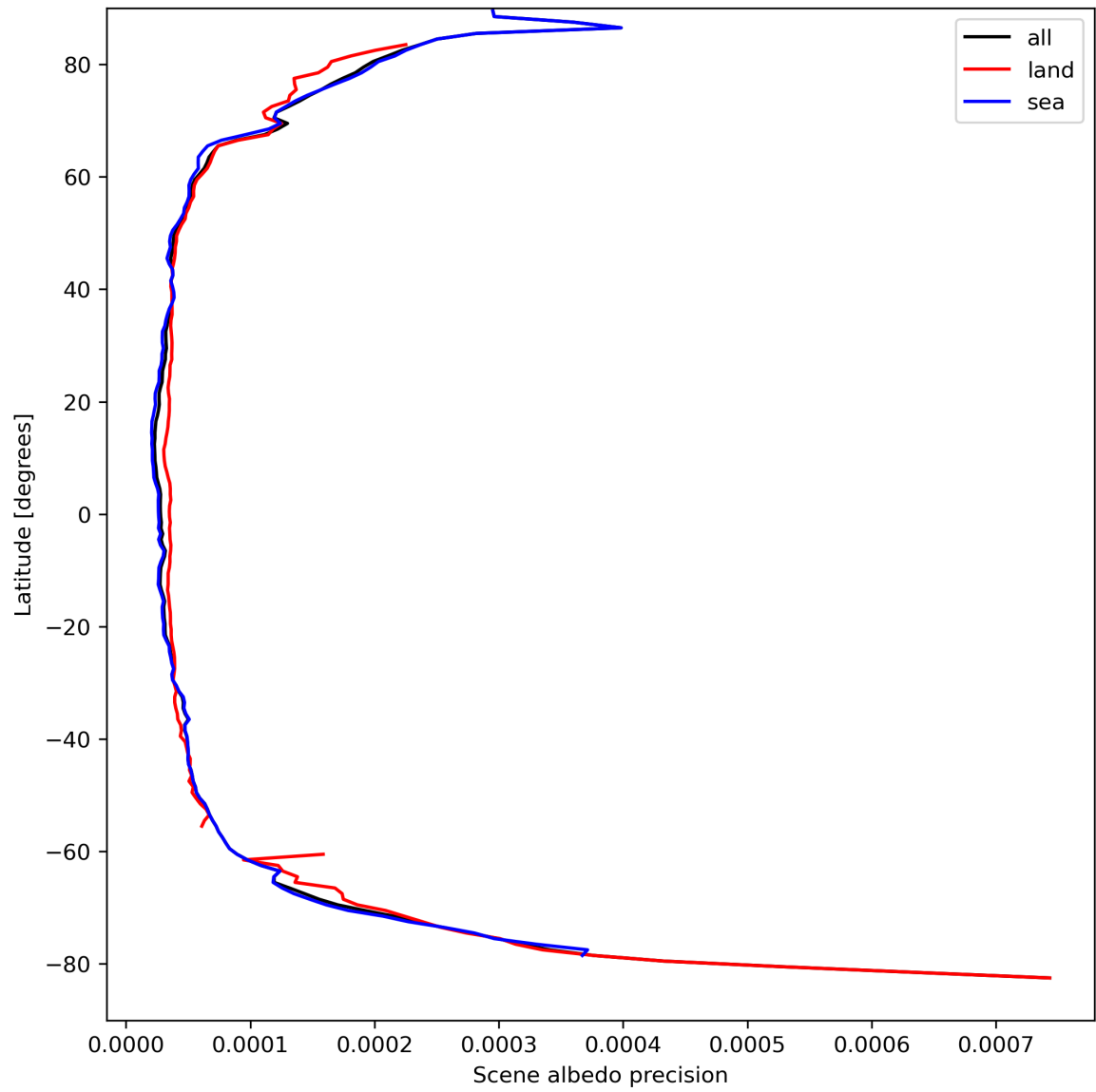
Figure 18: Zonal average of “Scene albedo precision” for 2024-04-02 to 2024-04-04.
