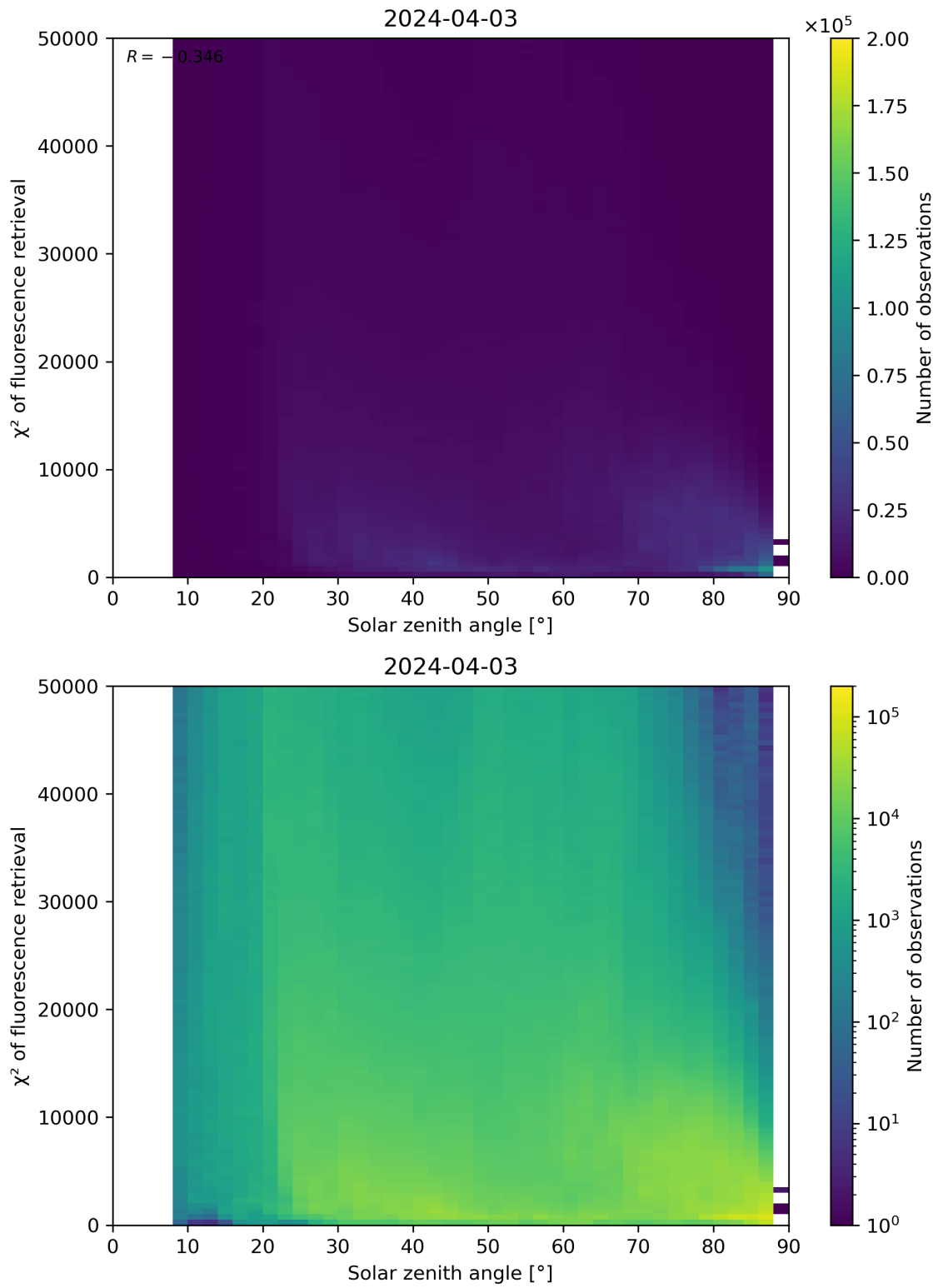
Figure 109: Scatter density plot of “Solar zenith angle” against “ \chi^2 of fluorescence retrieval” for 2024-04-02 to 2024-04-04.
