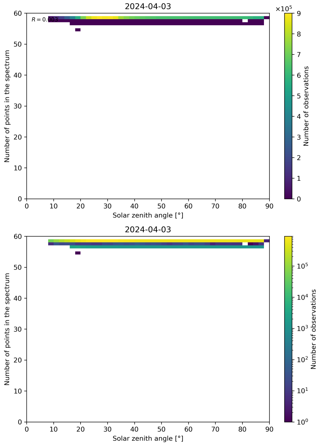
Figure 115: Scatter density plot of “Solar zenith angle” against “Number of points in the spectrum” for 2024-04-02 to 2024-04-04.
