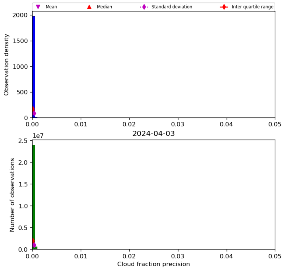
Figure 33: Histogram of “Cloud fraction precision” for 2024-04-02 to 2024-04-04
