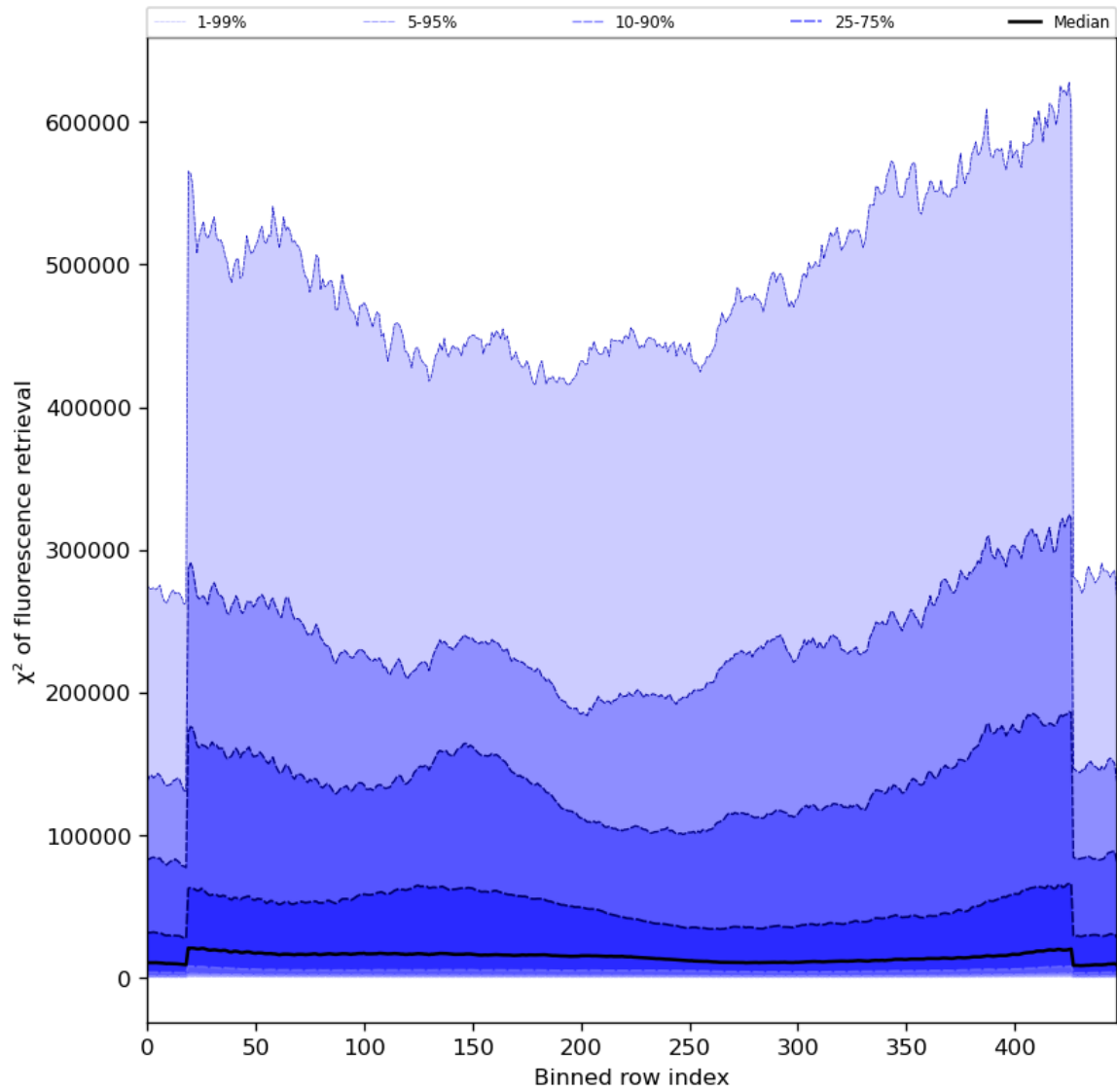
Figure 59: Along track statistics of “ \chi^2 of fluorescence retrieval” for 2024-04-02 to 2024-04-04
