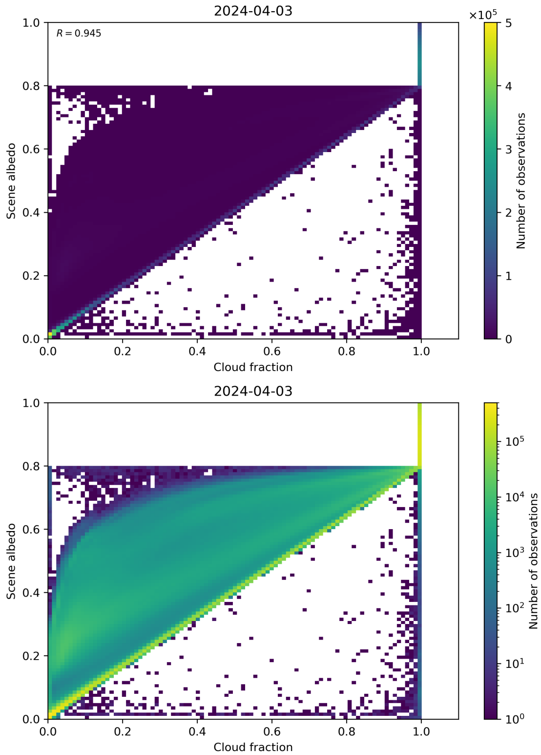
Figure 75: Scatter density plot of “Cloud fraction” against “Scene albedo” for 2024-04-02 to 2024-04-04.
