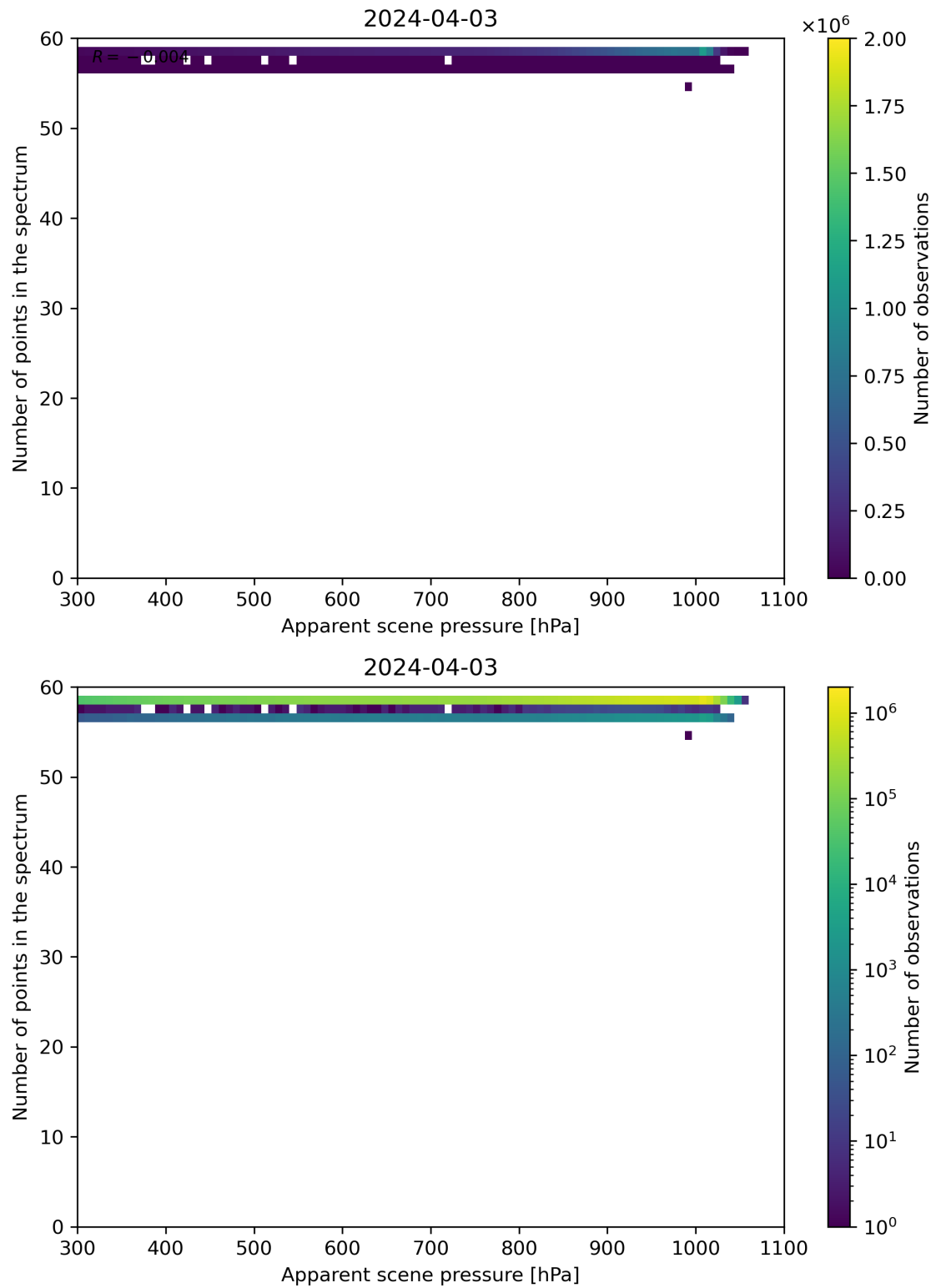
Figure 66: Scatter density plot of “Apparent scene pressure” against “Number of points in the spectrum” for 2024-04-02 to 2024-04-04.
