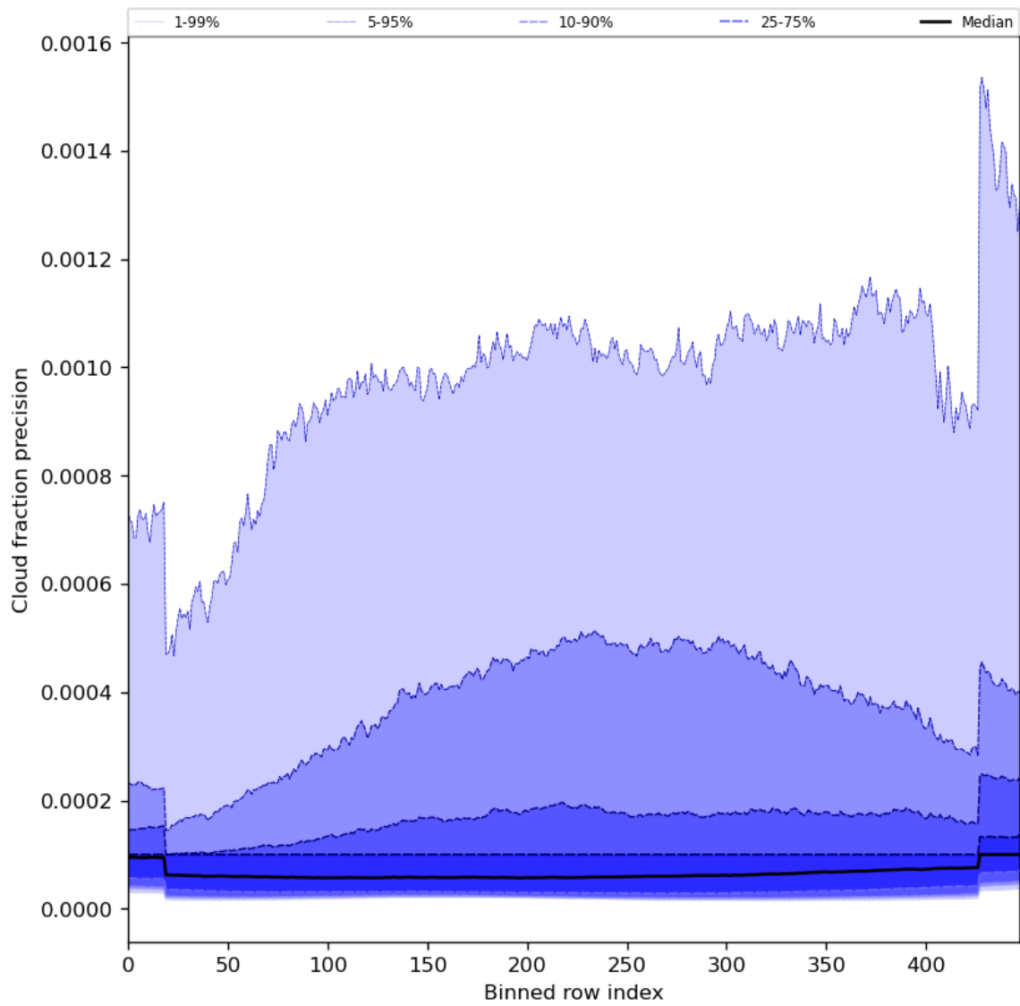
Figure 50: Along track statistics of “Cloud fraction precision” for 2024-04-02 to 2024-04-04
