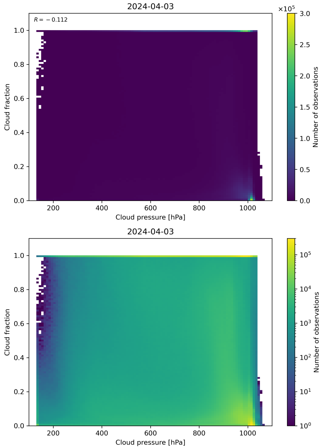
Figure 79: Scatter density plot of “Cloud pressure” against “Cloud fraction” for 2024-04-02 to 2024-04-04.
