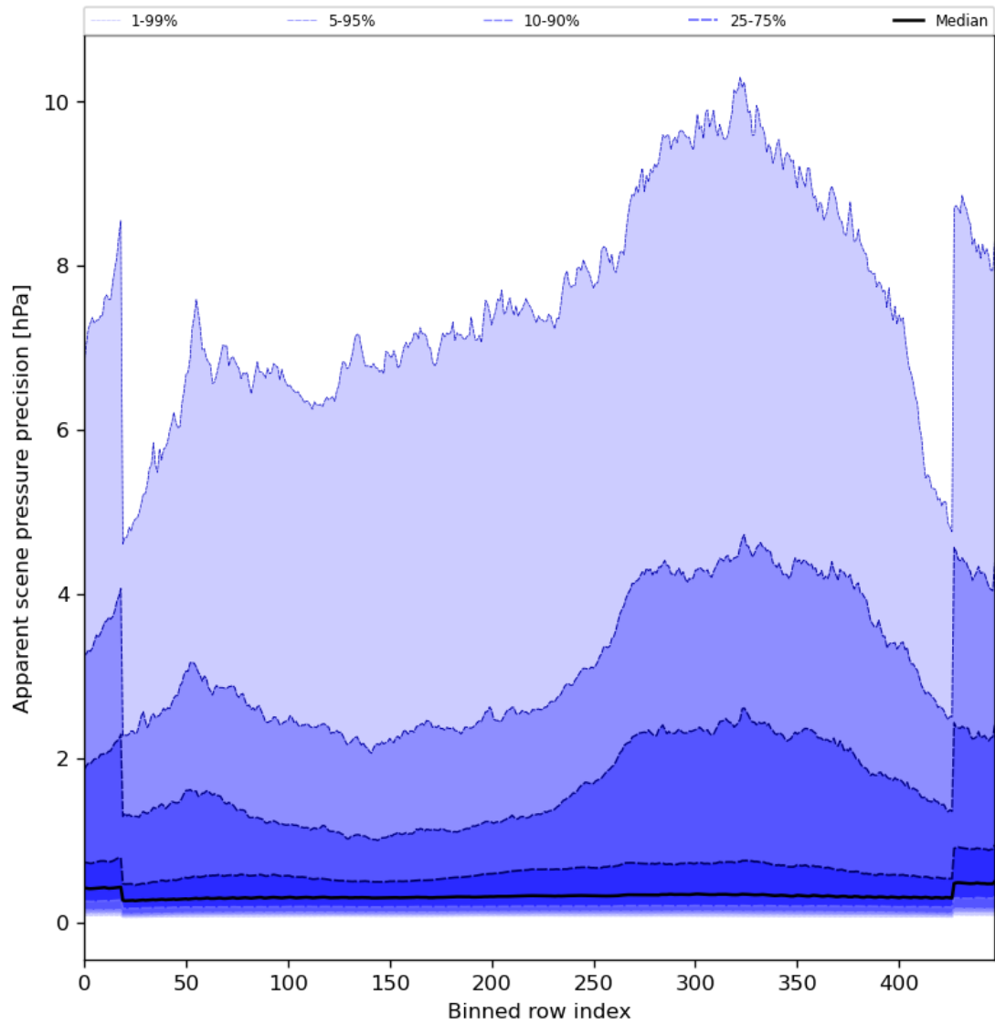
Figure 54: Along track statistics of “Apparent scene pressure precision” for 2024-04-02 to 2024-04-04
