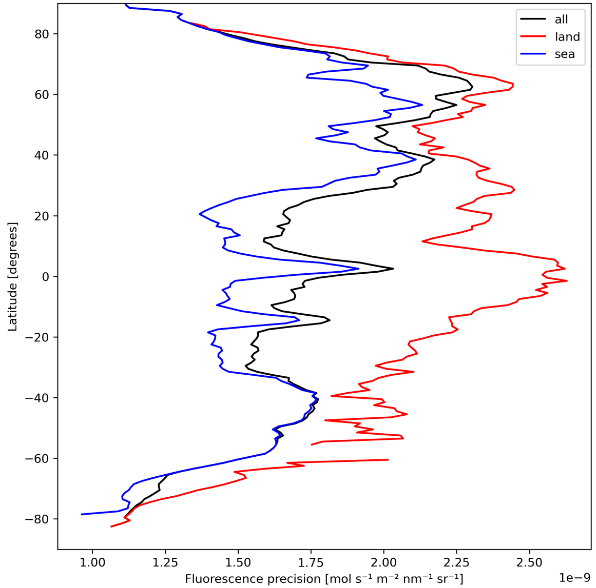
Figure 24: Zonal average of "Fluorescence precision" for 2024-04-02 to 2024-04-04.
