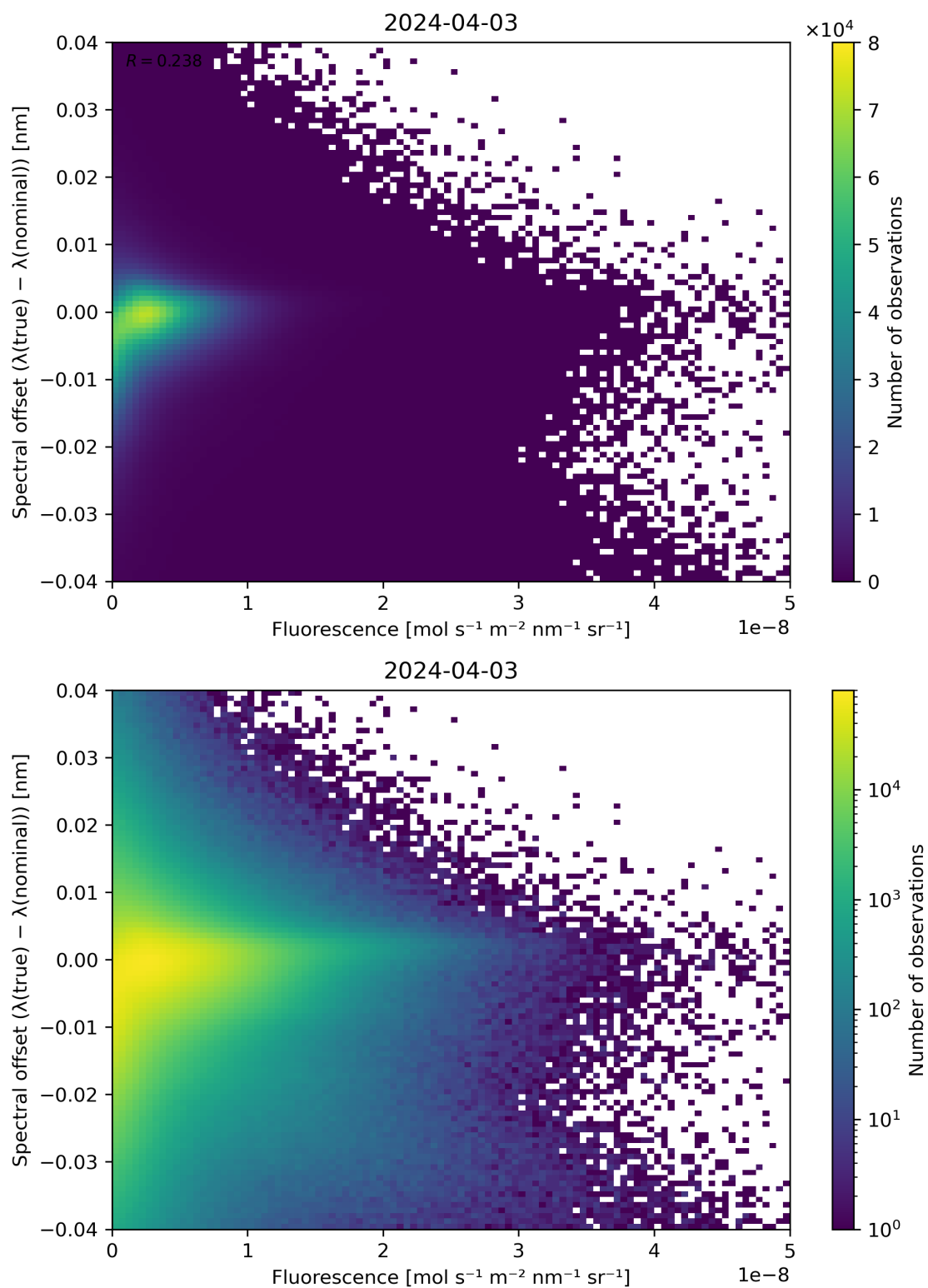
Figure 87: Scatter density plot of “Fluorescence” against “Spectral offset ( \lambda(\text{true}) - \lambda(\text{nominal}) )” for 2024-04-02 to 2024-04-04.
