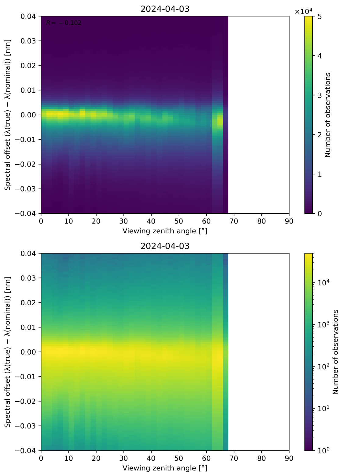
Figure 128: Scatter density plot of “Viewing zenith angle” against “Spectral offset ( \lambda(\text{true}) - \lambda(\text{nominal}) )” for 2024-04-02 to 2024-04-04.
