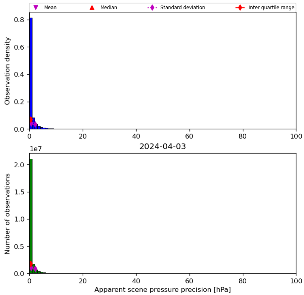
Figure 37: Histogram of “Apparent scene pressure precision” for 2024-04-02 to 2024-04-04
