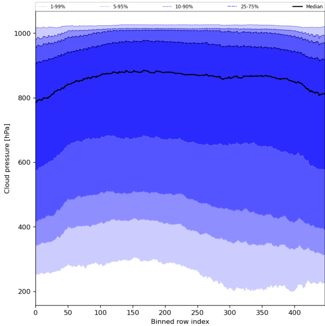
Figure 47: Along track statistics of “Cloud pressure” for 2024-04-02 to 2024-04-04
