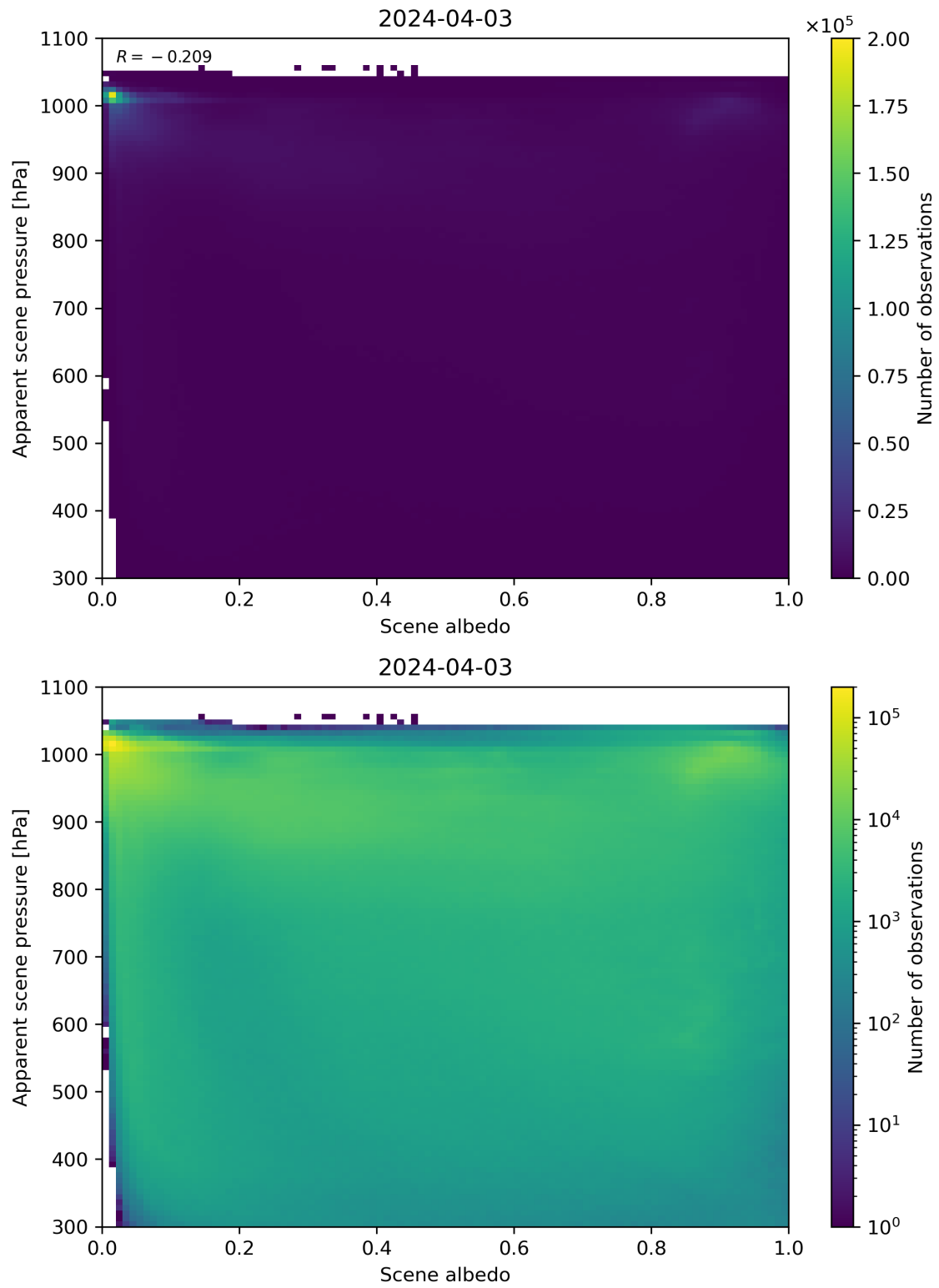
Figure 102: Scatter density plot of “Scene albedo” against “Apparent scene pressure” for 2024-04-02 to 2024-04-04.
