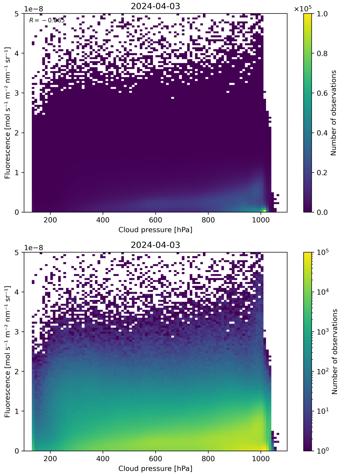
Figure 80: Scatter density plot of “Cloud pressure” against “Fluorescence” for 2024-04-02 to 2024-04-04.
