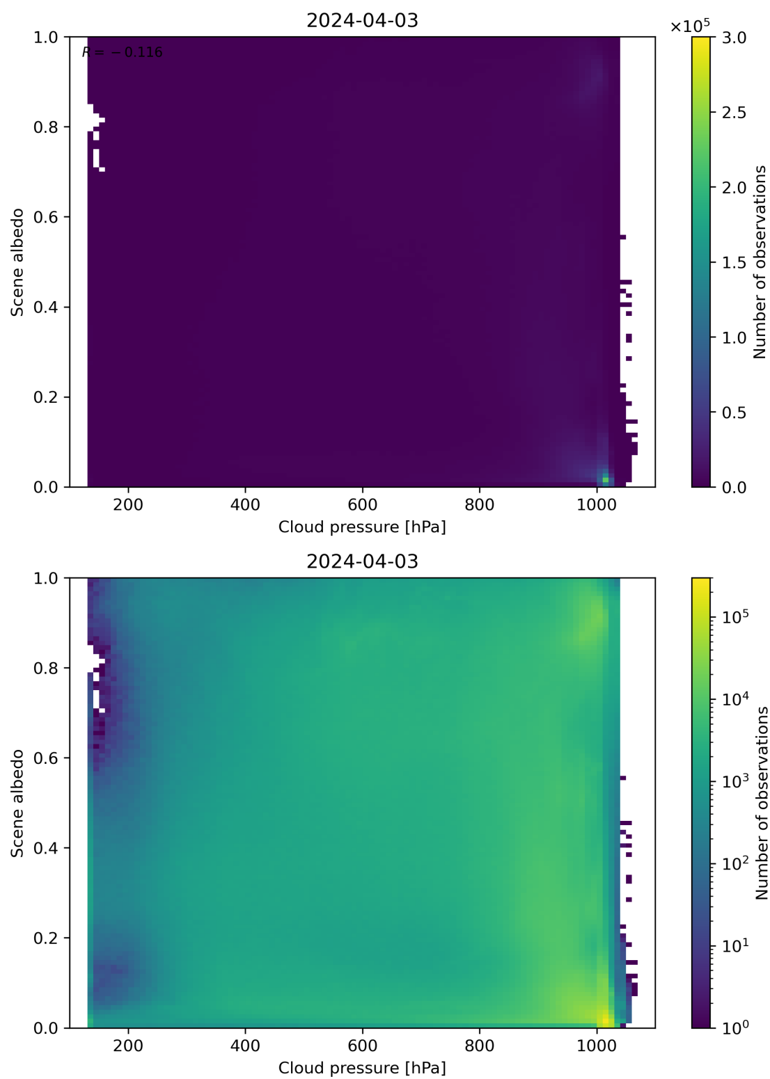
Figure 83: Scatter density plot of “Cloud pressure” against “Scene albedo” for 2024-04-02 to 2024-04-04.
