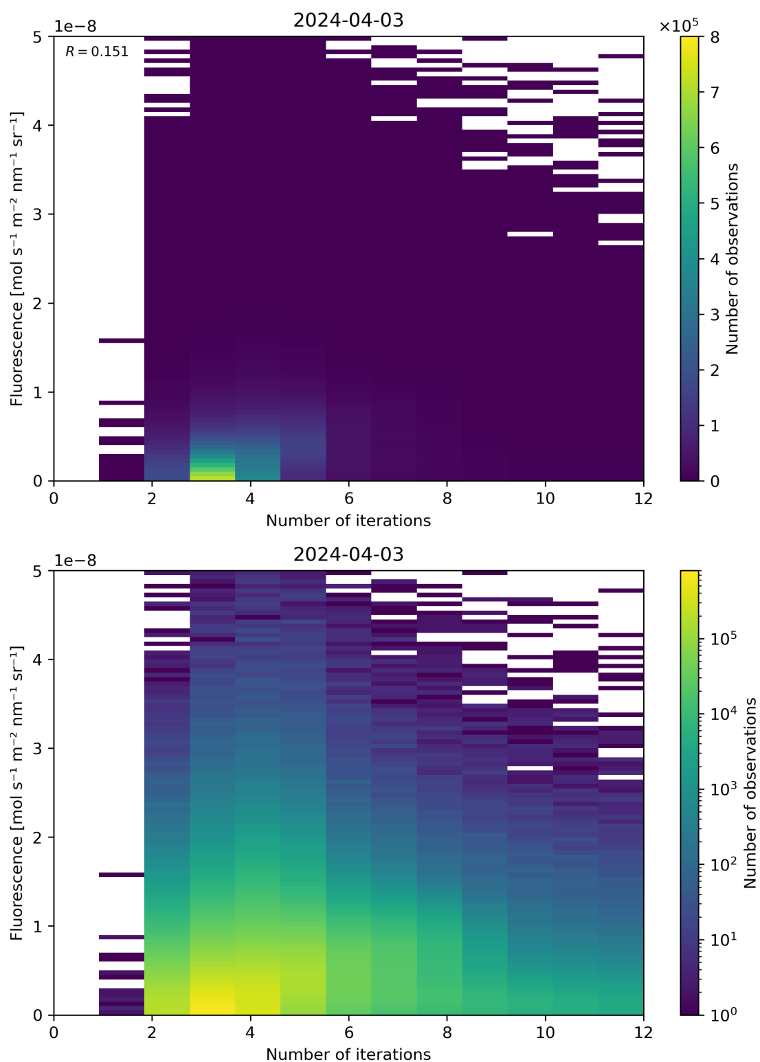
Figure 98: Scatter density plot of “Number of iterations” against “Fluorescence” for 2024-04-02 to 2024-04-04.
