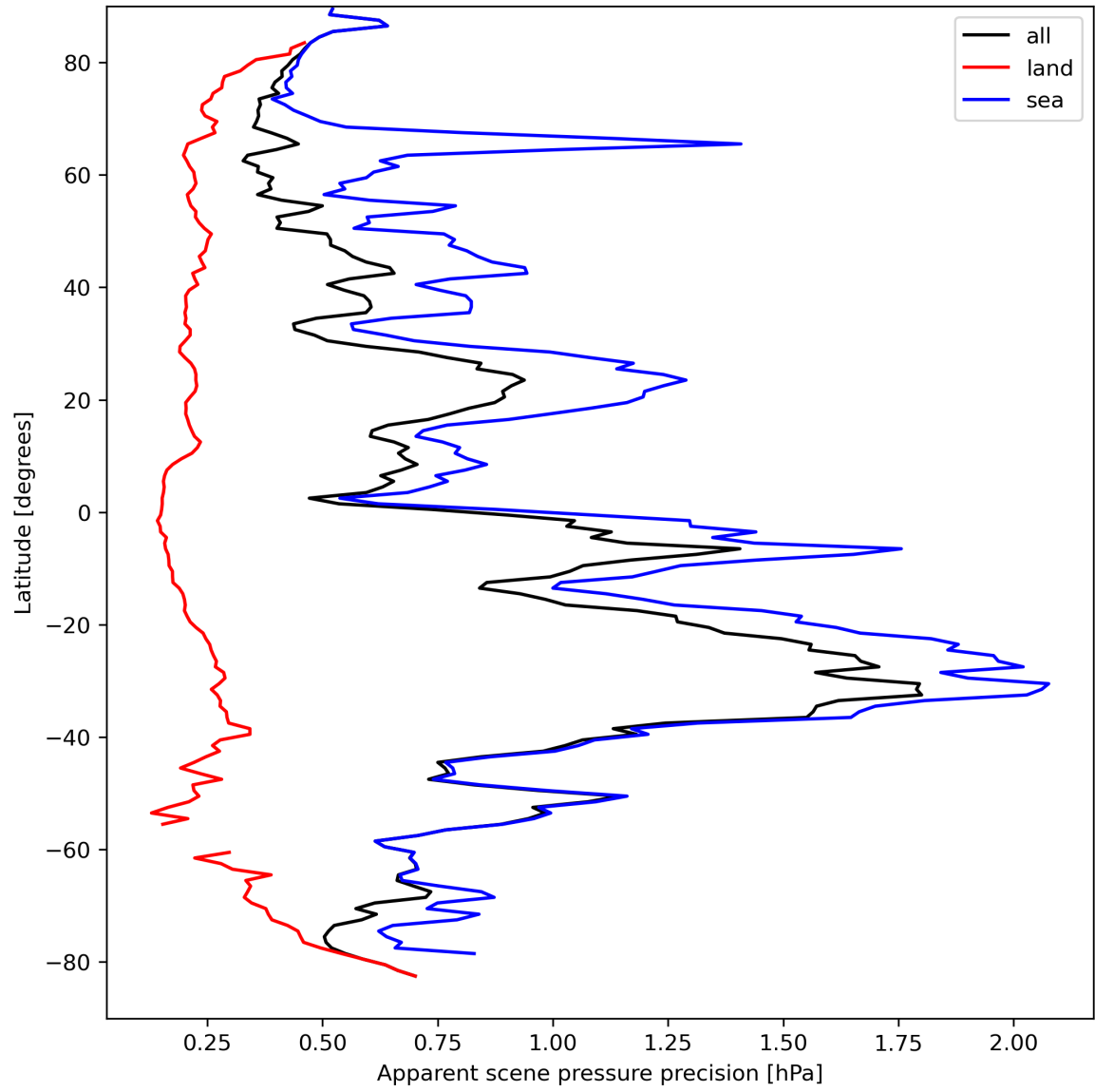
Figure 20: Zonal average of “Apparent scene pressure precision” for 2024-04-02 to 2024-04-04.
