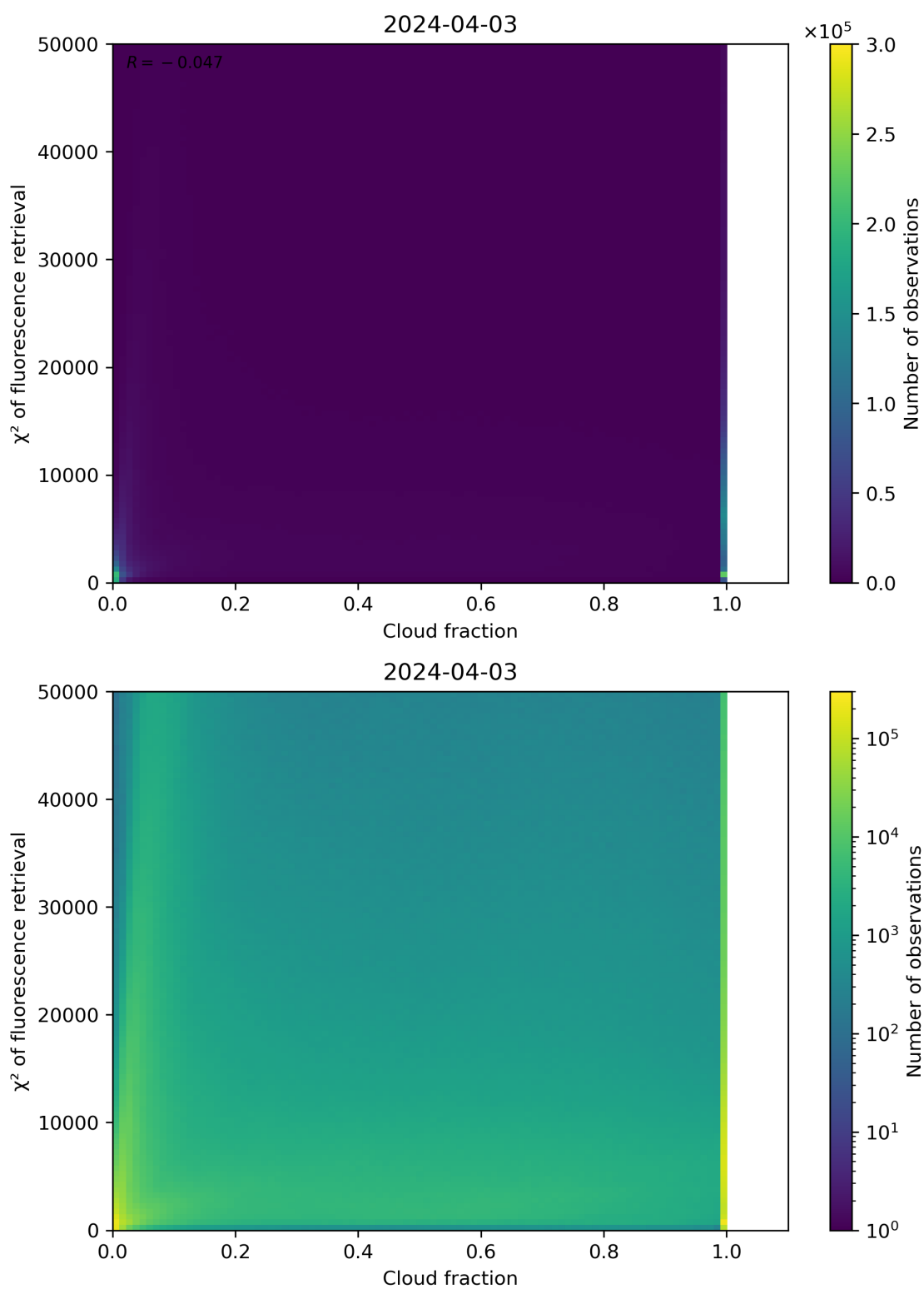
Figure 71: Scatter density plot of “Cloud fraction” against “ \chi^2 of fluorescence retrieval” for 2024-04-02 to 2024-04-04.
