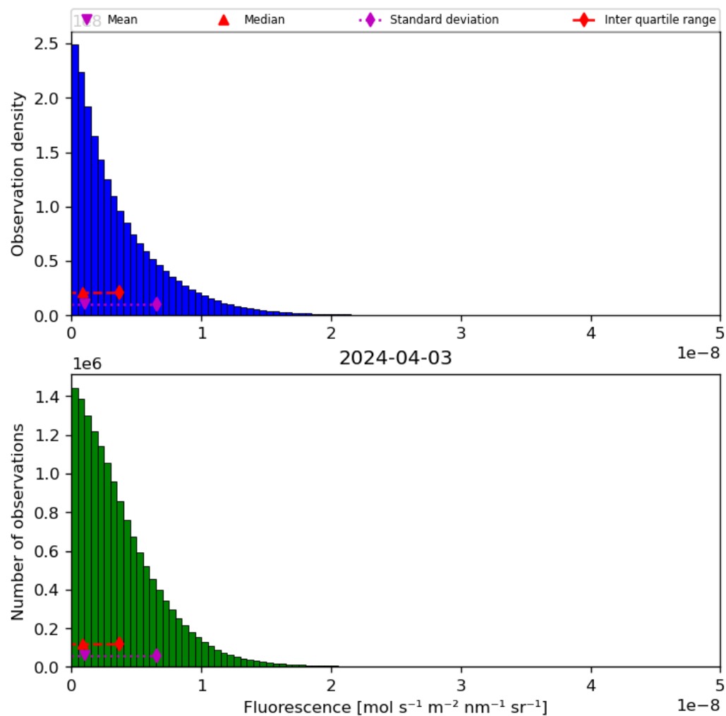
Figure 40: Histogram of “Fluorescence” for 2024-04-02 to 2024-04-04
