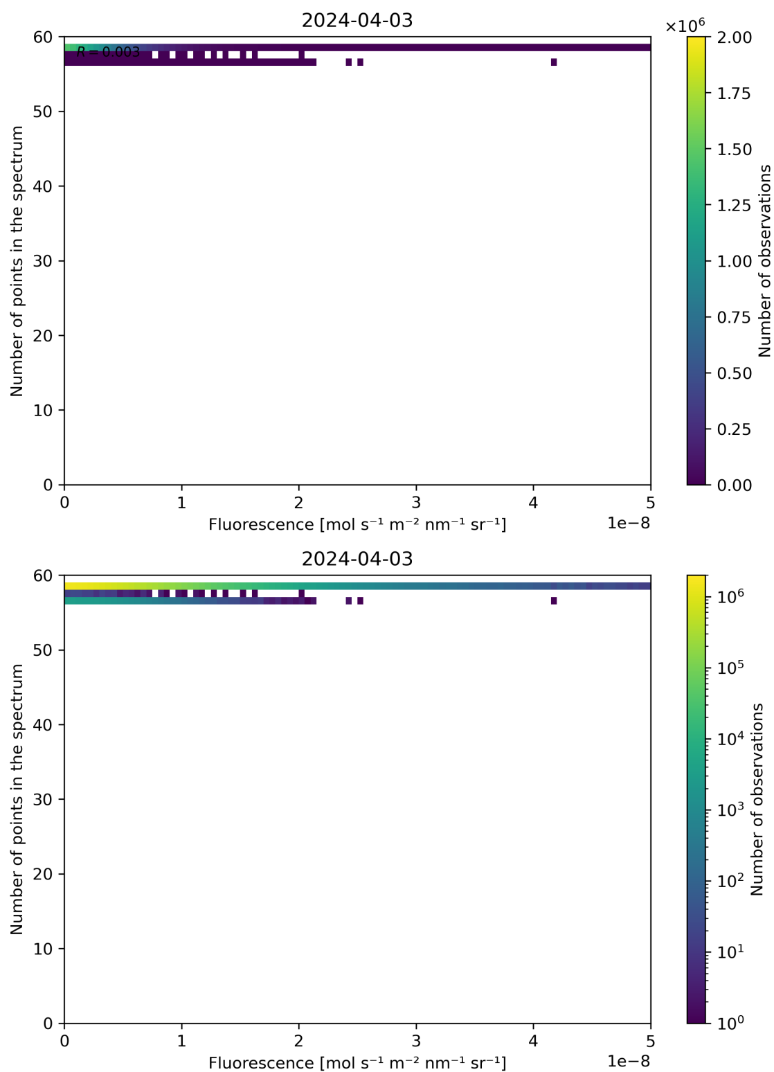
Figure 86: Scatter density plot of “Fluorescence” against “Number of points in the spectrum” for 2024-04-02 to 2024-04-04.
