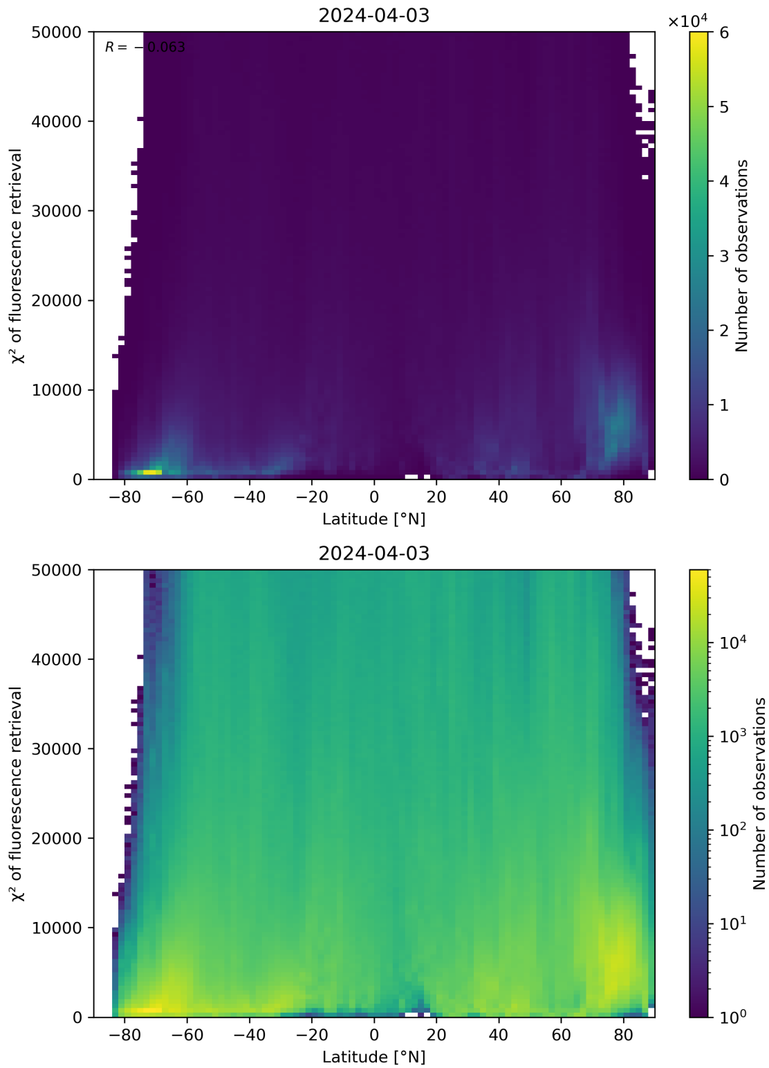
Figure 89: Scatter density plot of “Latitude” against “ \chi^2 of fluorescence retrieval” for 2024-04-02 to 2024-04-04.
