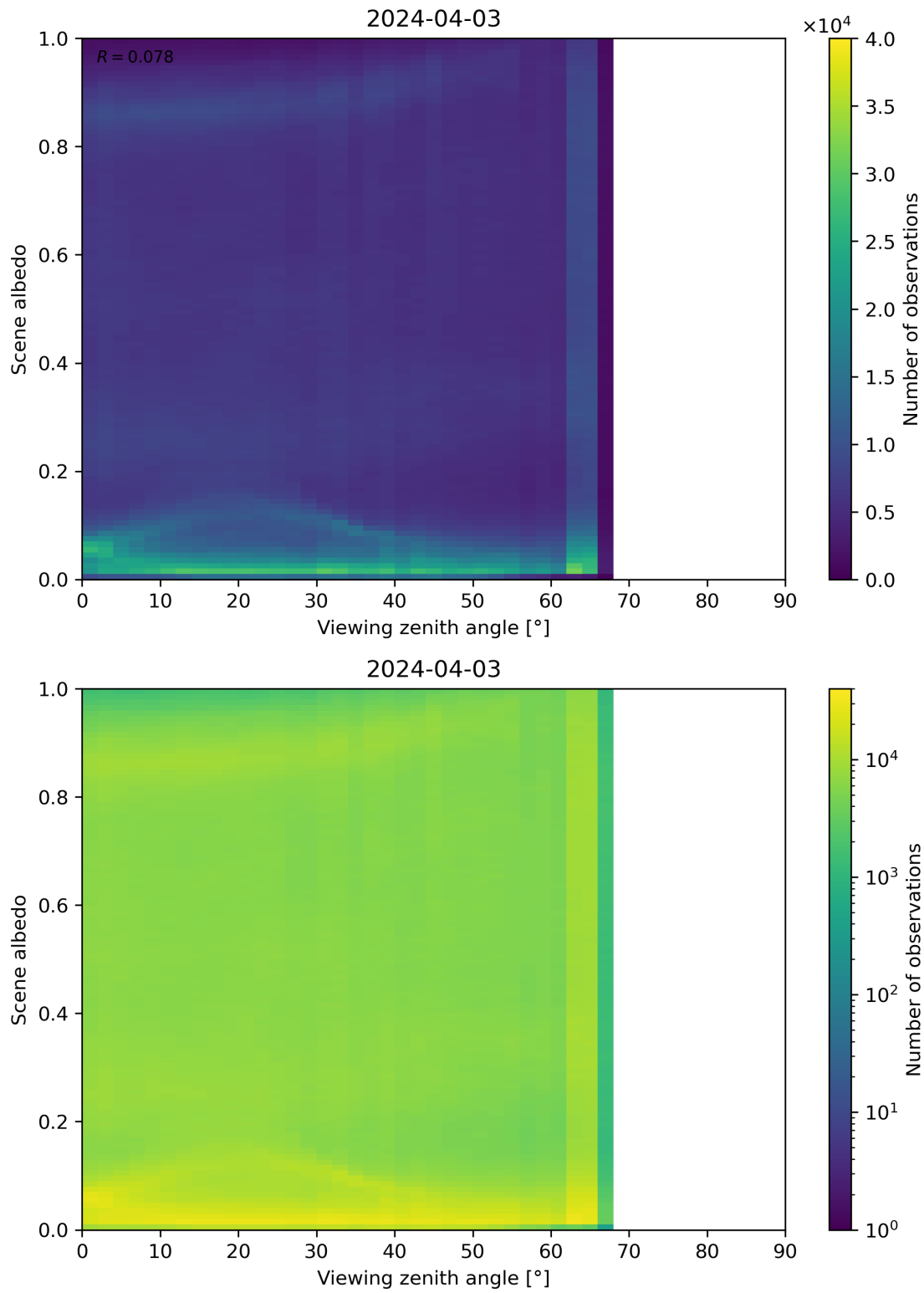
Figure 126: Scatter density plot of “Viewing zenith angle” against “Scene albedo” for 2024-04-02 to 2024-04-04.
