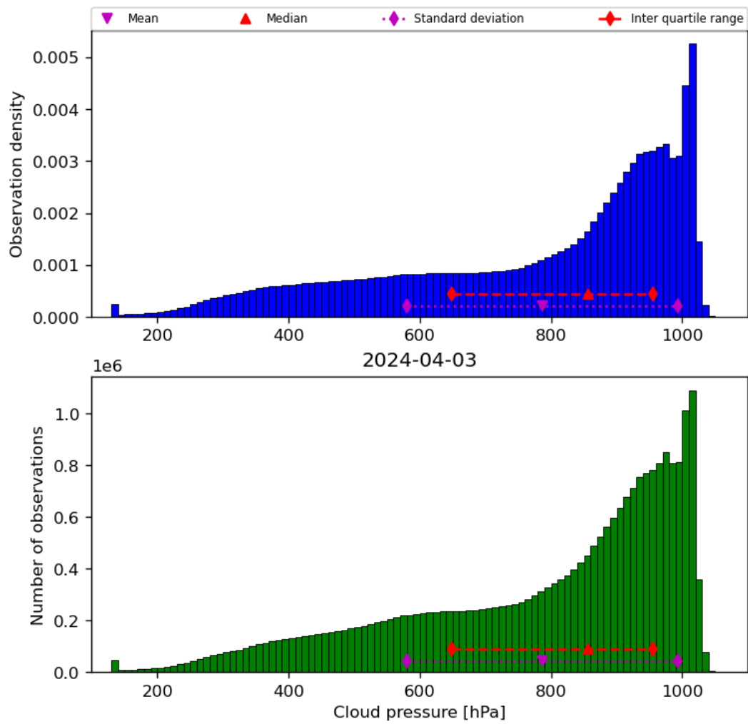
Figure 30: Histogram of “Cloud pressure” for 2024-04-02 to 2024-04-04
