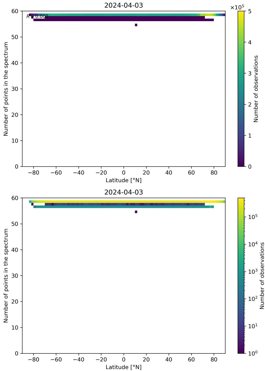
Figure 94: Scatter density plot of “Latitude” against “Number of points in the spectrum” for 2024-04-02 to 2024-04-04.
