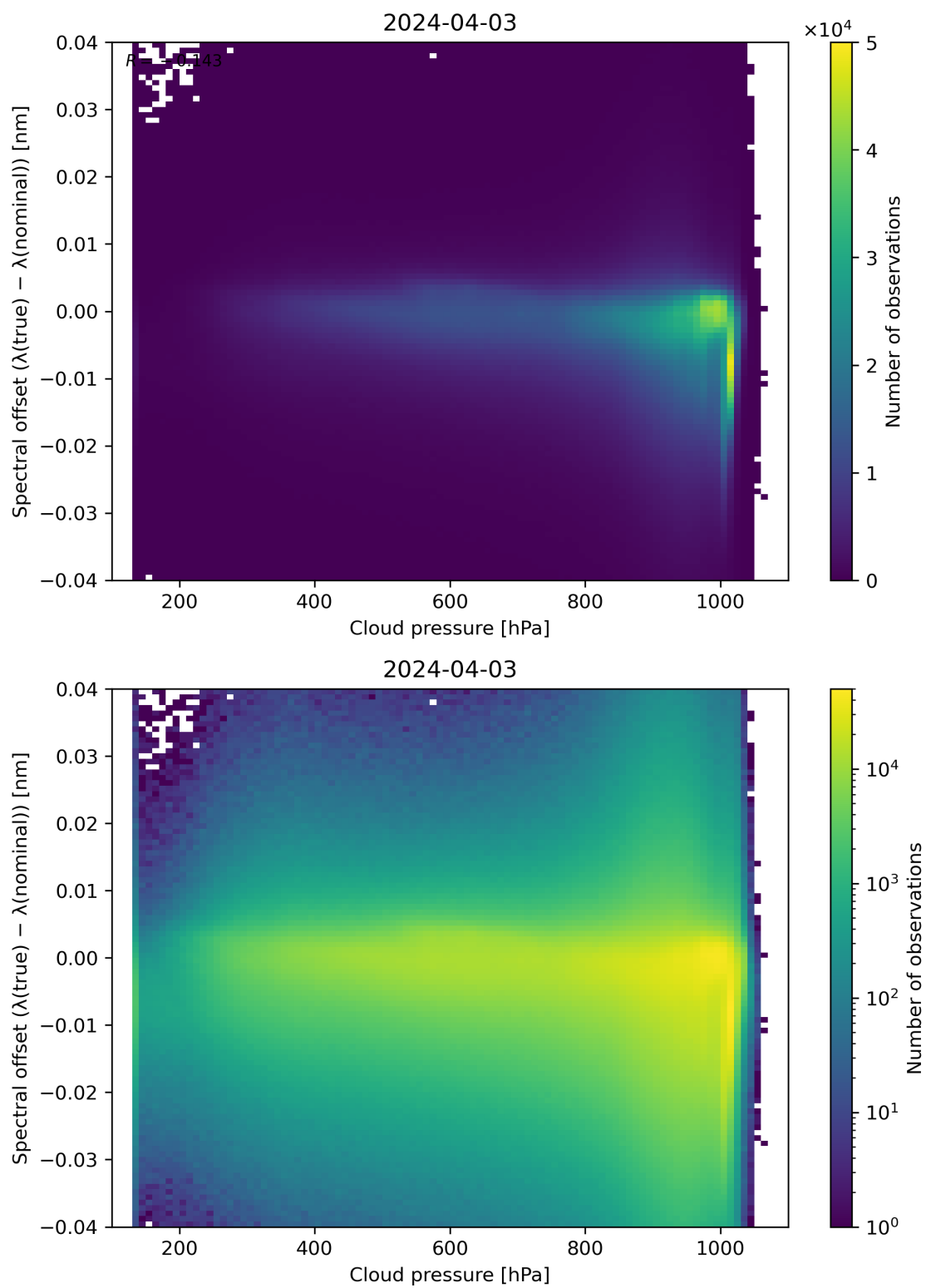
Figure 84: Scatter density plot of “Cloud pressure” against “Spectral offset ( \lambda(\text{true}) - \lambda(\text{nominal}) )” for 2024-04-02 to 2024-04-04.
