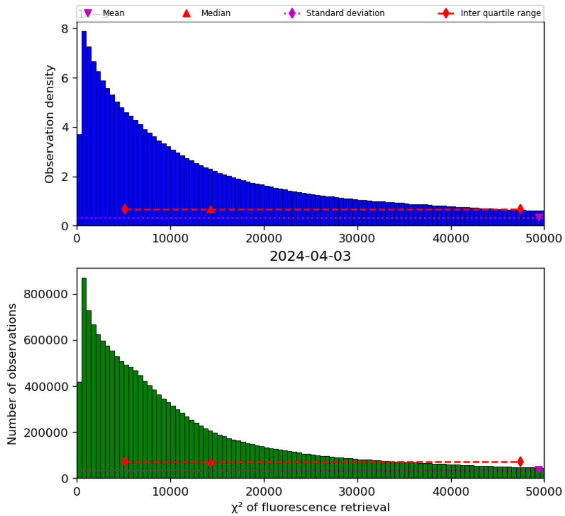
Figure 42: Histogram of “ \chi^2 of fluorescence retrieval” for 2024-04-02 to 2024-04-04
