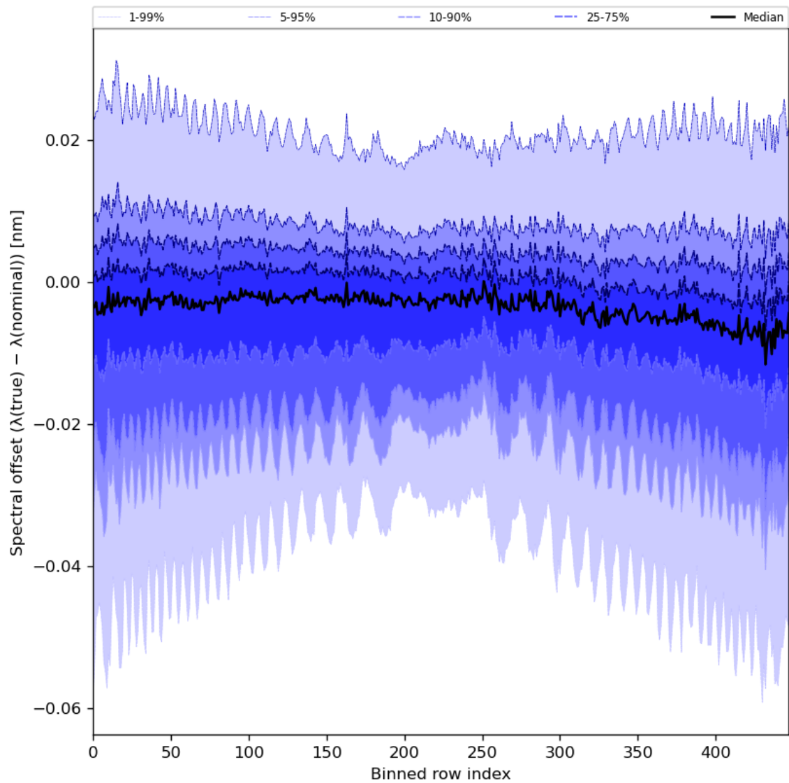
Figure 62: Along track statistics of “Spectral offset ( \lambda(\text{true}) - \lambda(\text{nominal}) )” for 2024-04-02 to 2024-04-04
