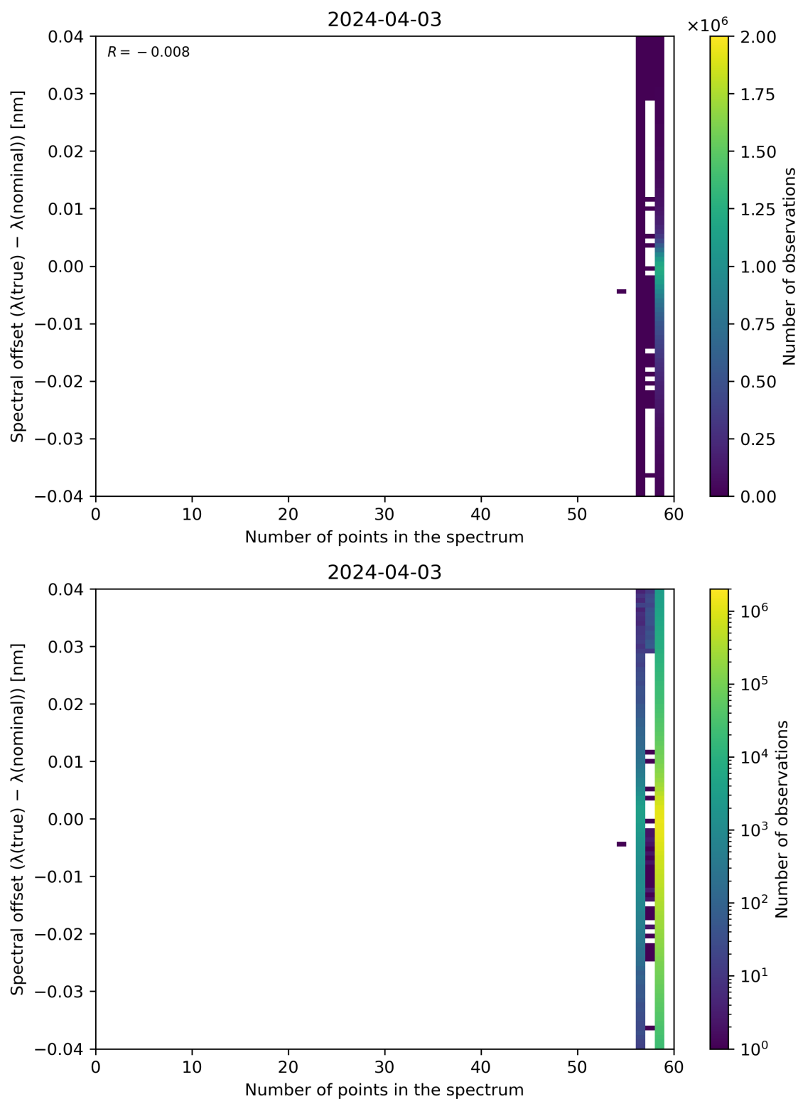
Figure 101: Scatter density plot of “Number of points in the spectrum” against “Spectral offset ( \lambda(\text{true}) - \lambda(\text{nominal}) )” for 2024-04-02 to 2024-04-04.
