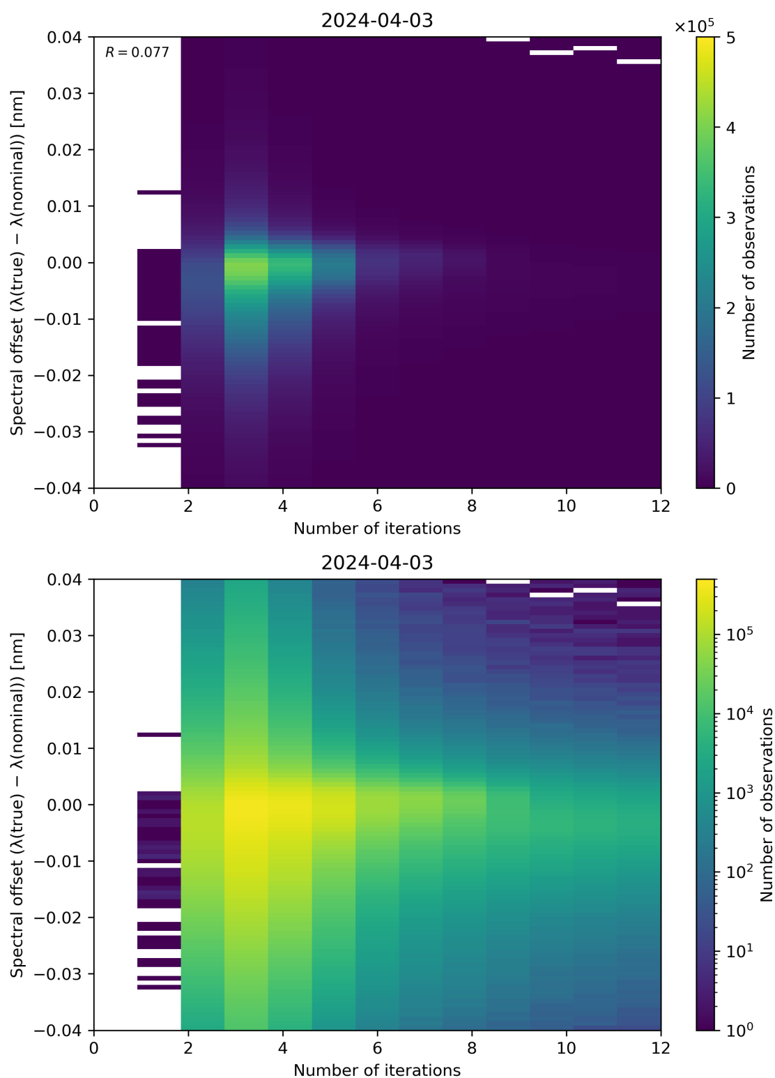
Figure 100: Scatter density plot of “Number of iterations” against “Spectral offset ( \lambda(\text{true}) - \lambda(\text{nominal}) )” for 2024-04-02 to 2024-04-04.
