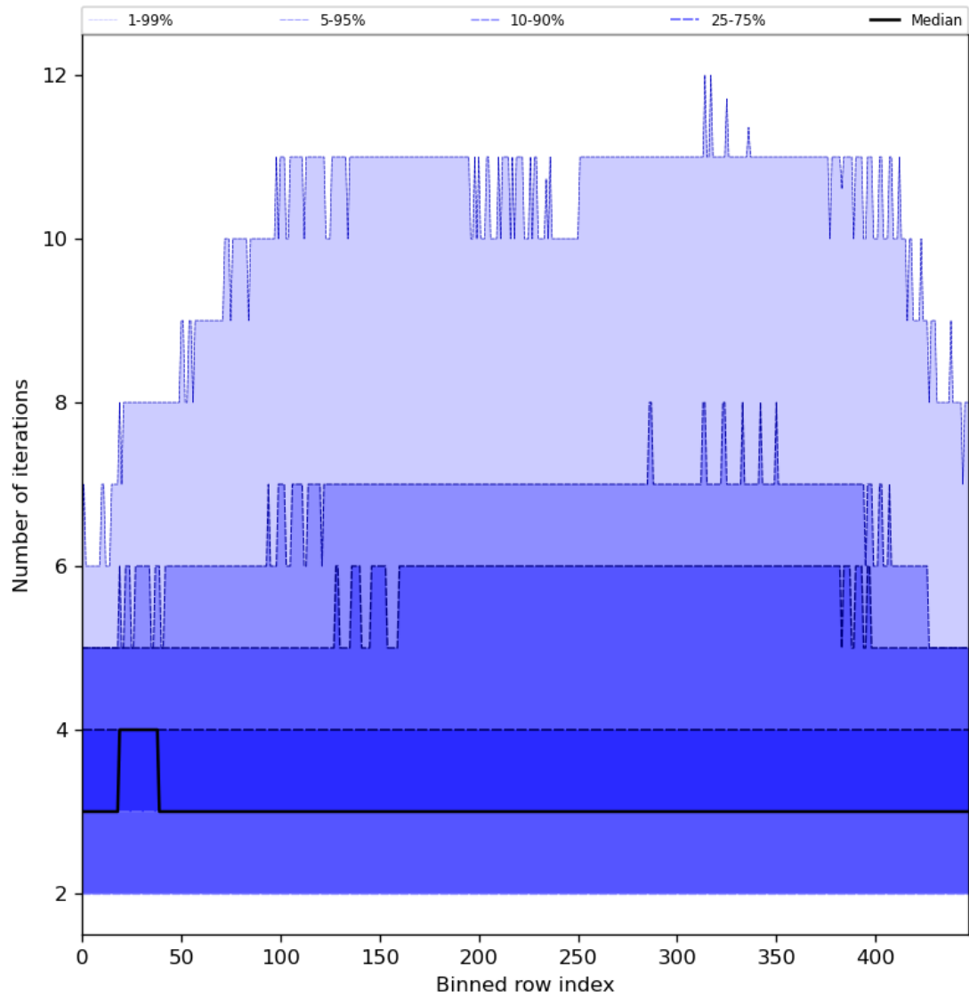
Figure 56: Along track statistics of “Number of iterations” for 2024-04-02 to 2024-04-04
