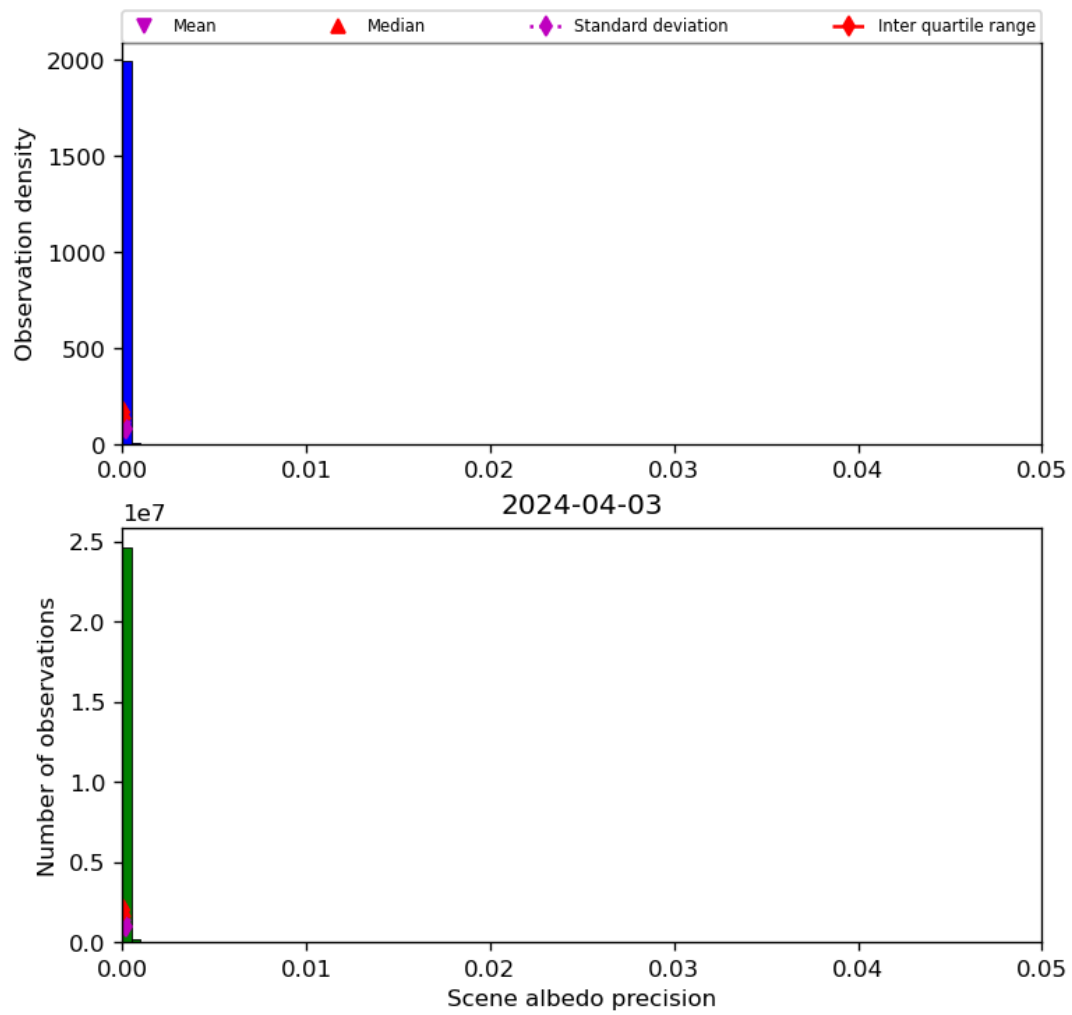
Figure 35: Histogram of “Scene albedo precision” for 2024-04-02 to 2024-04-04
