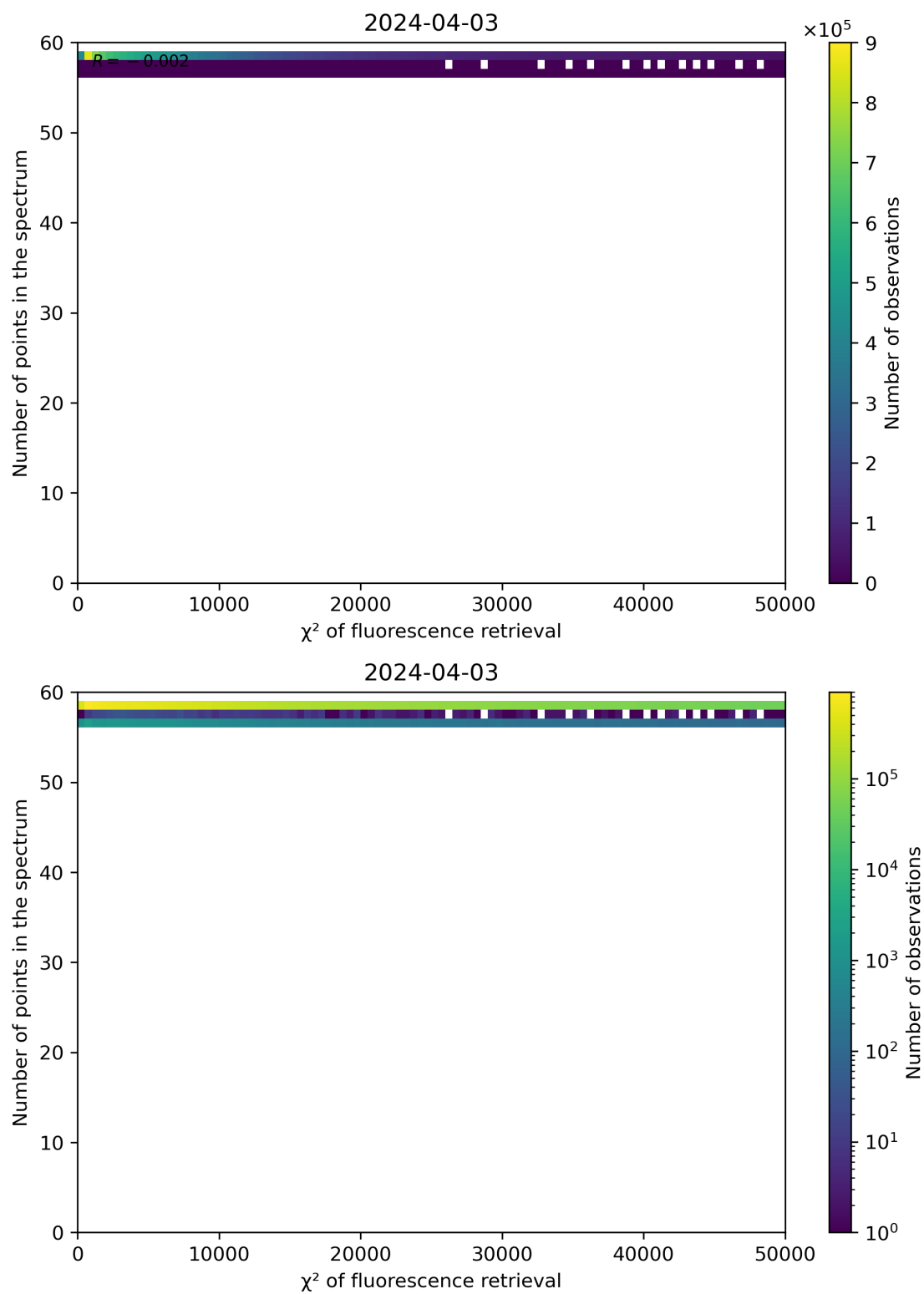
Figure 68: Scatter density plot of " \chi^2 of fluorescence retrieval" against "Number of points in the spectrum" for 2024-04-02 to 2024-04-04.
