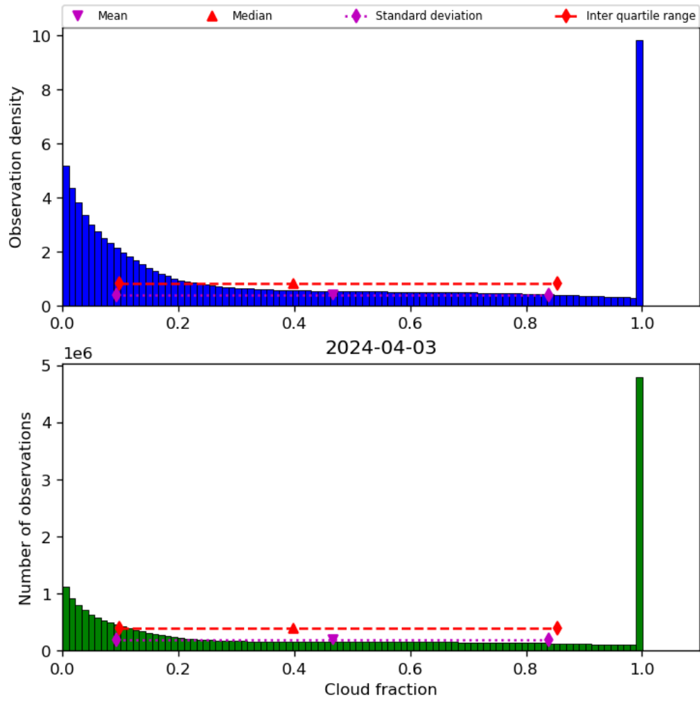
Figure 32: Histogram of "Cloud fraction" for 2024-04-02 to 2024-04-04
