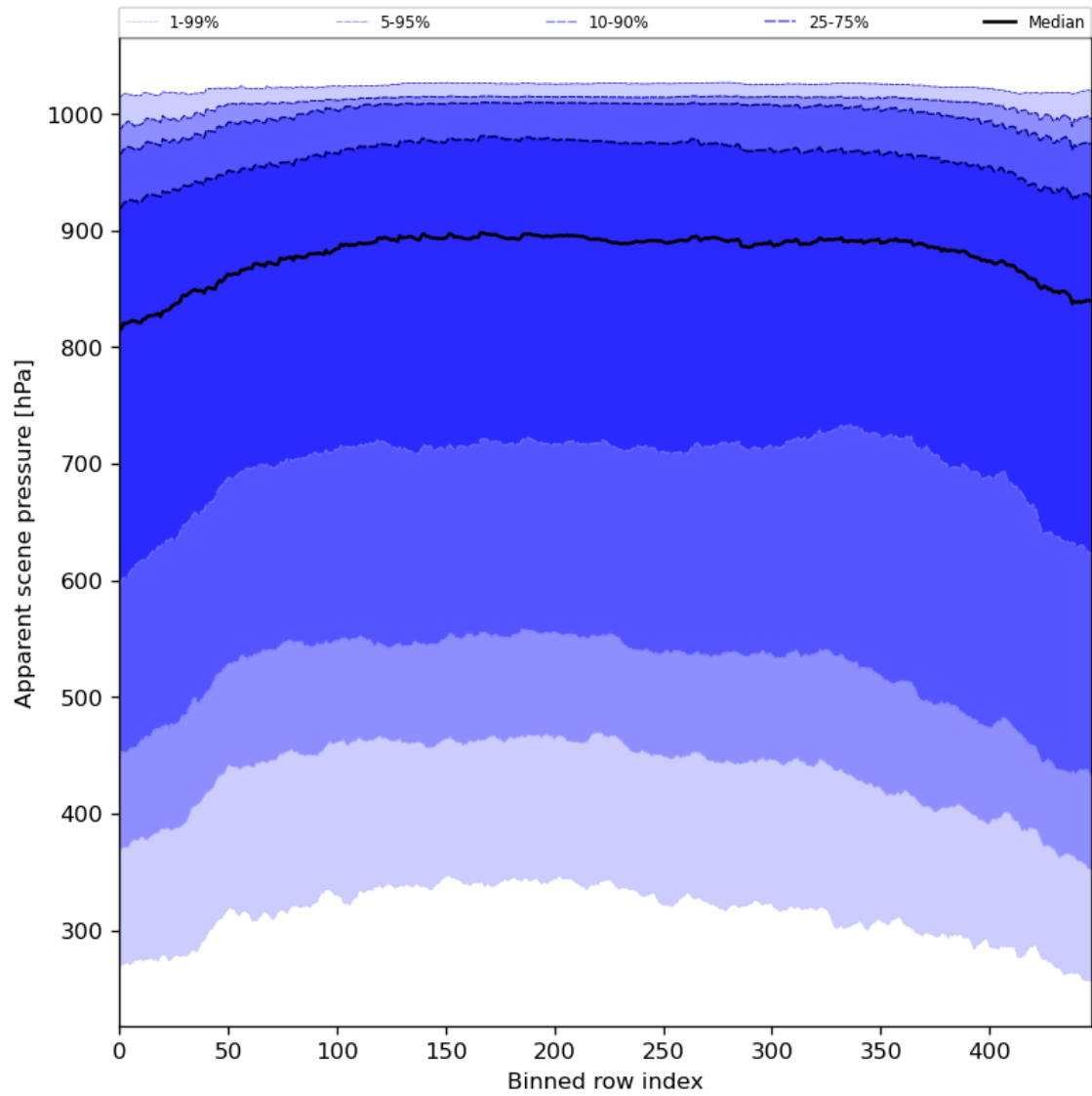
Figure 53: Along track statistics of “Apparent scene pressure” for 2024-04-02 to 2024-04-04
