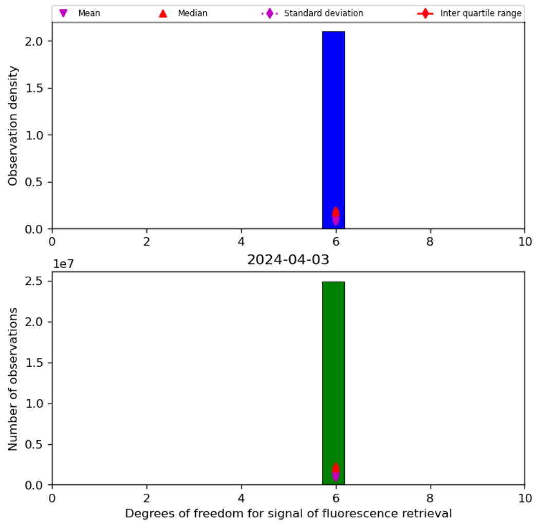
Figure 43: Histogram of “Degrees of freedom for signal of fluorescence retrieval” for 2024-04-02 to 2024-04-04
