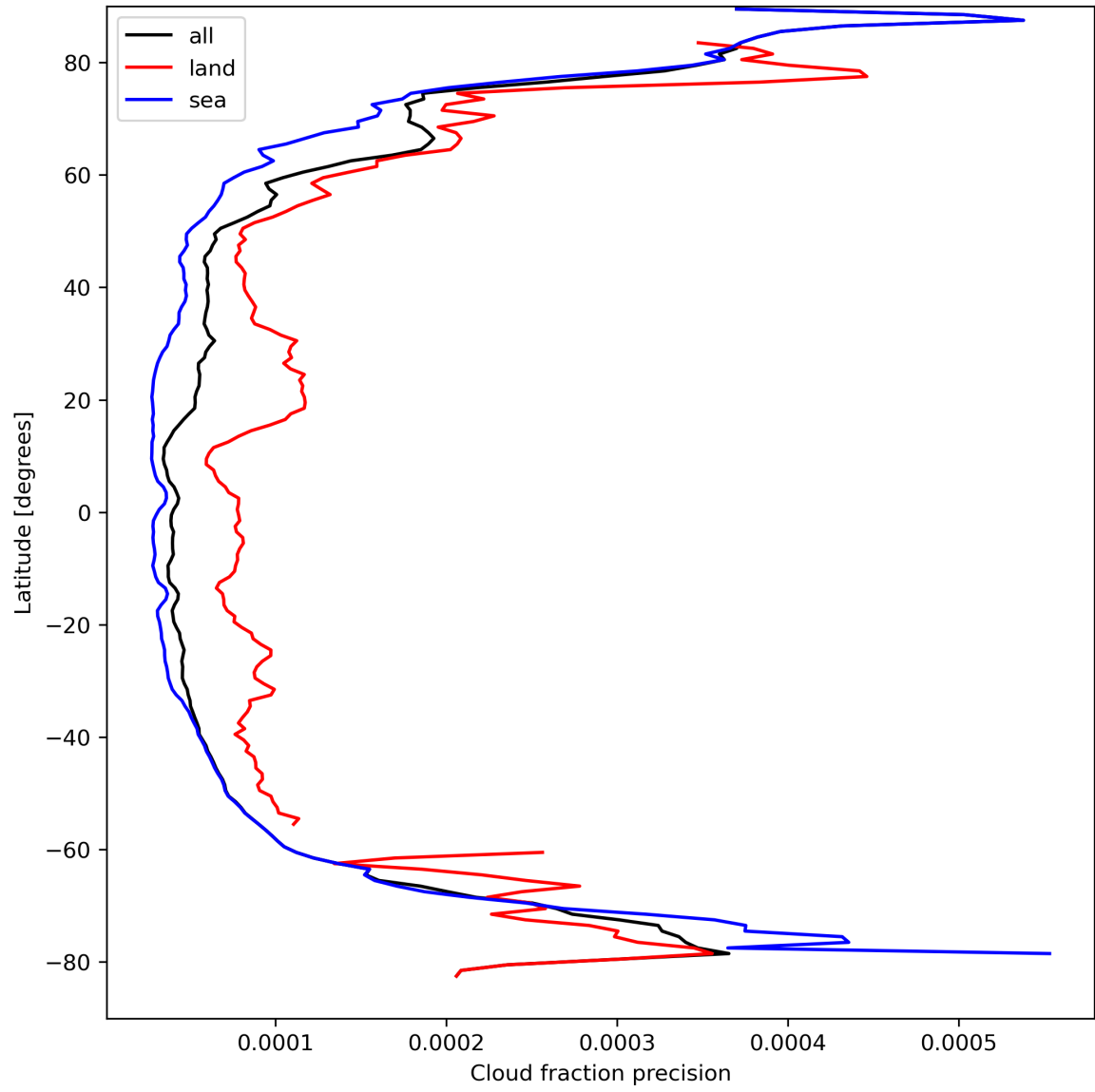
Figure 16: Zonal average of “Cloud fraction precision” for 2024-04-02 to 2024-04-04.
