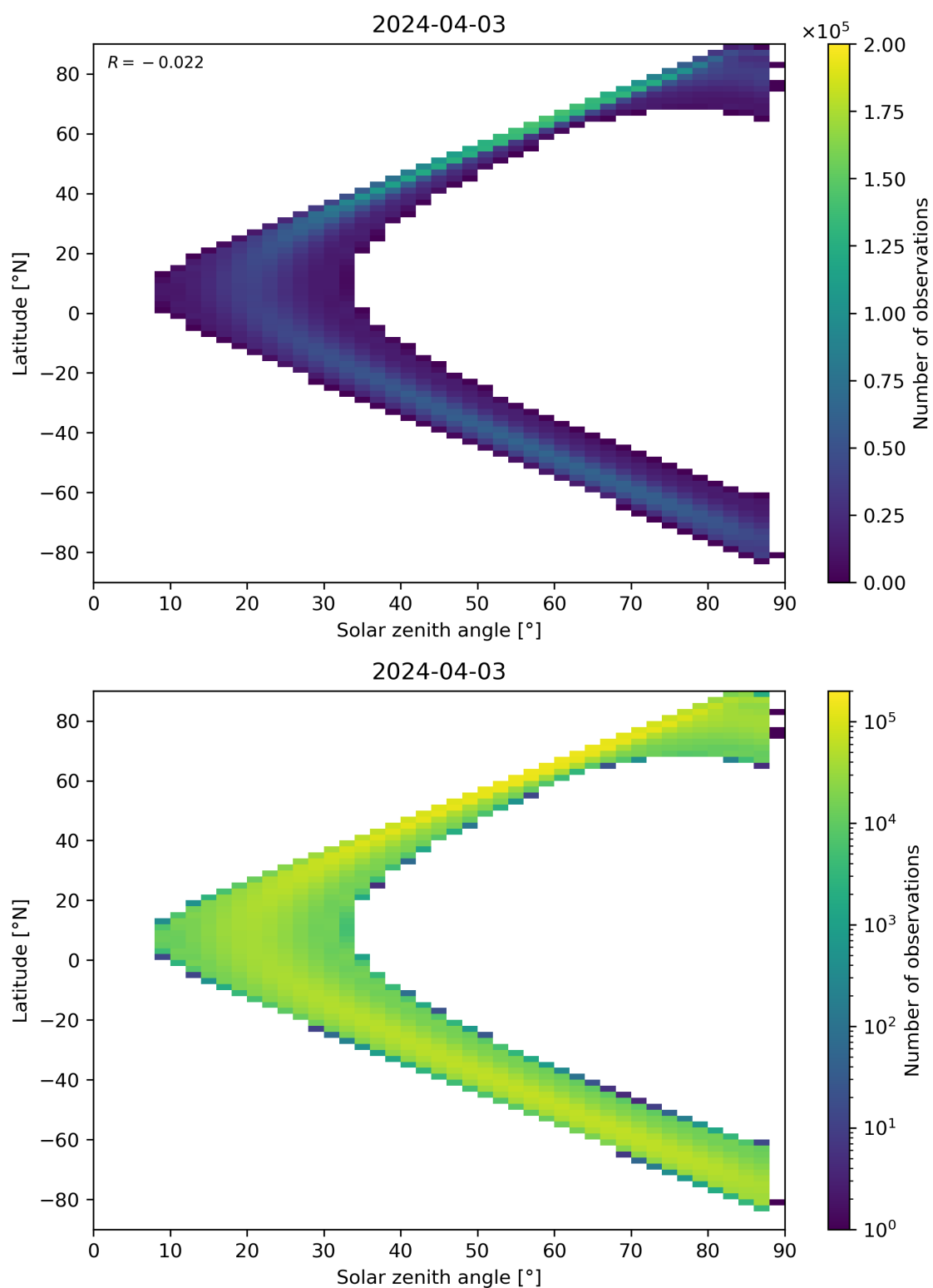
Figure 113: Scatter density plot of “Solar zenith angle” against “Latitude” for 2024-04-02 to 2024-04-04.
