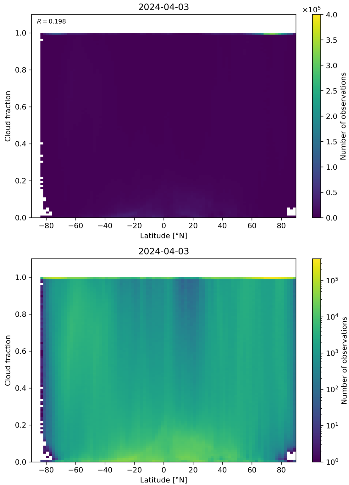
Figure 90: Scatter density plot of “Latitude” against “Cloud fraction” for 2024-04-02 to 2024-04-04.
