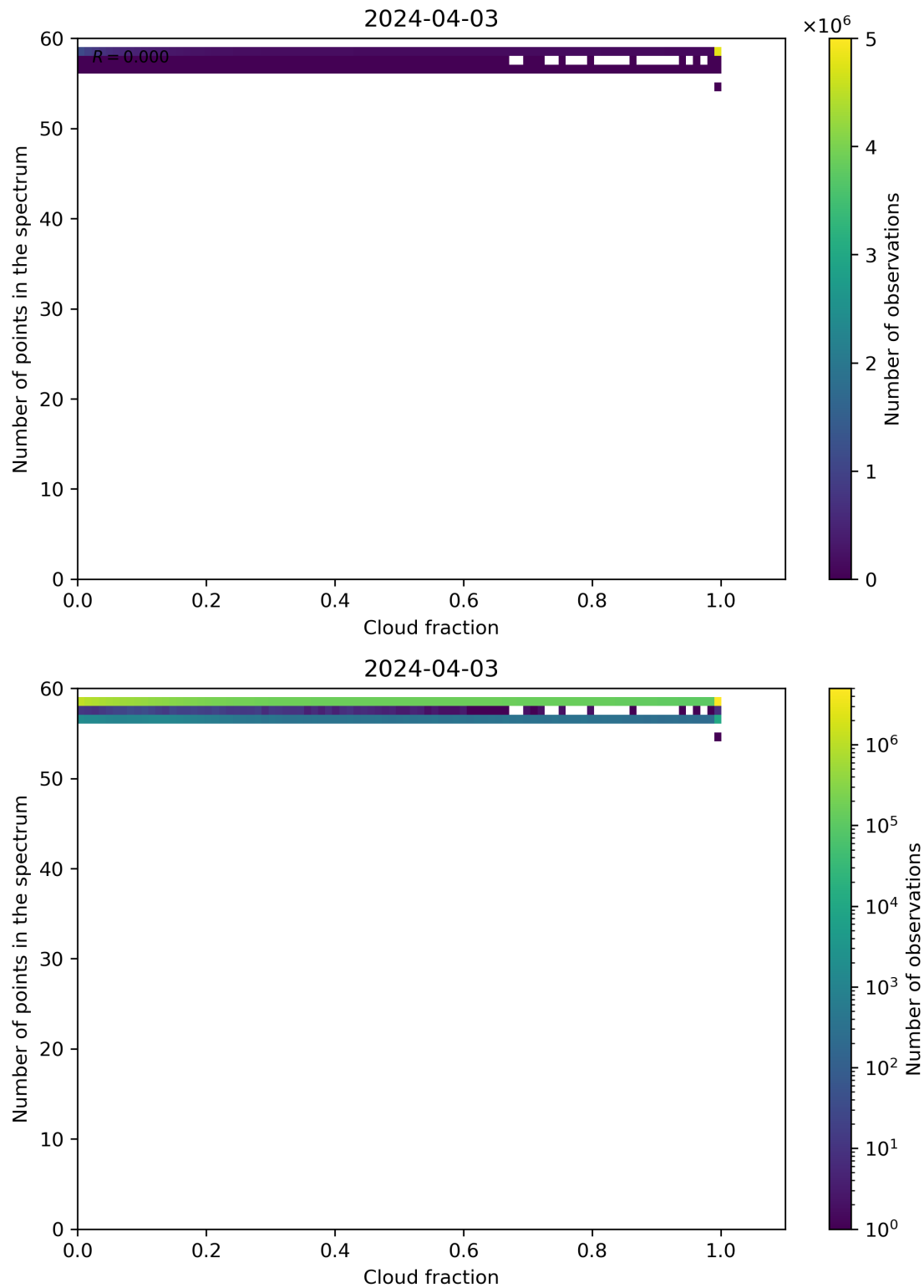
Figure 74: Scatter density plot of “Cloud fraction” against “Number of points in the spectrum” for 2024-04-02 to 2024-04-04.
