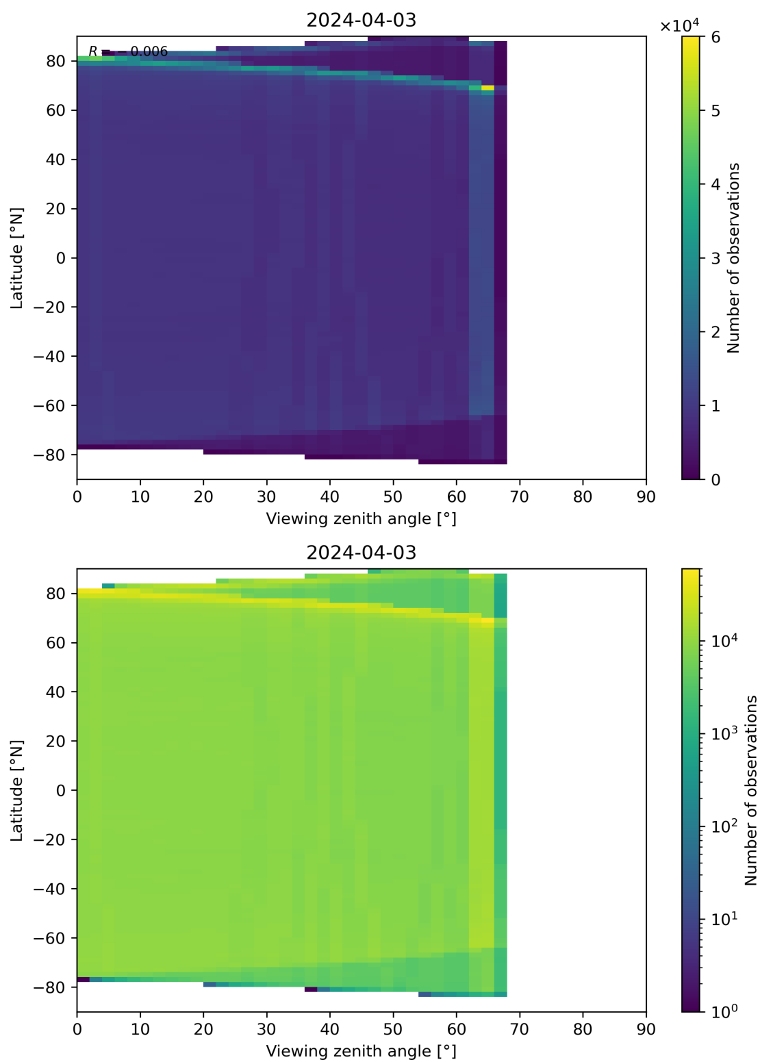
Figure 123: Scatter density plot of “Viewing zenith angle” against “Latitude” for 2024-04-02 to 2024-04-04.
