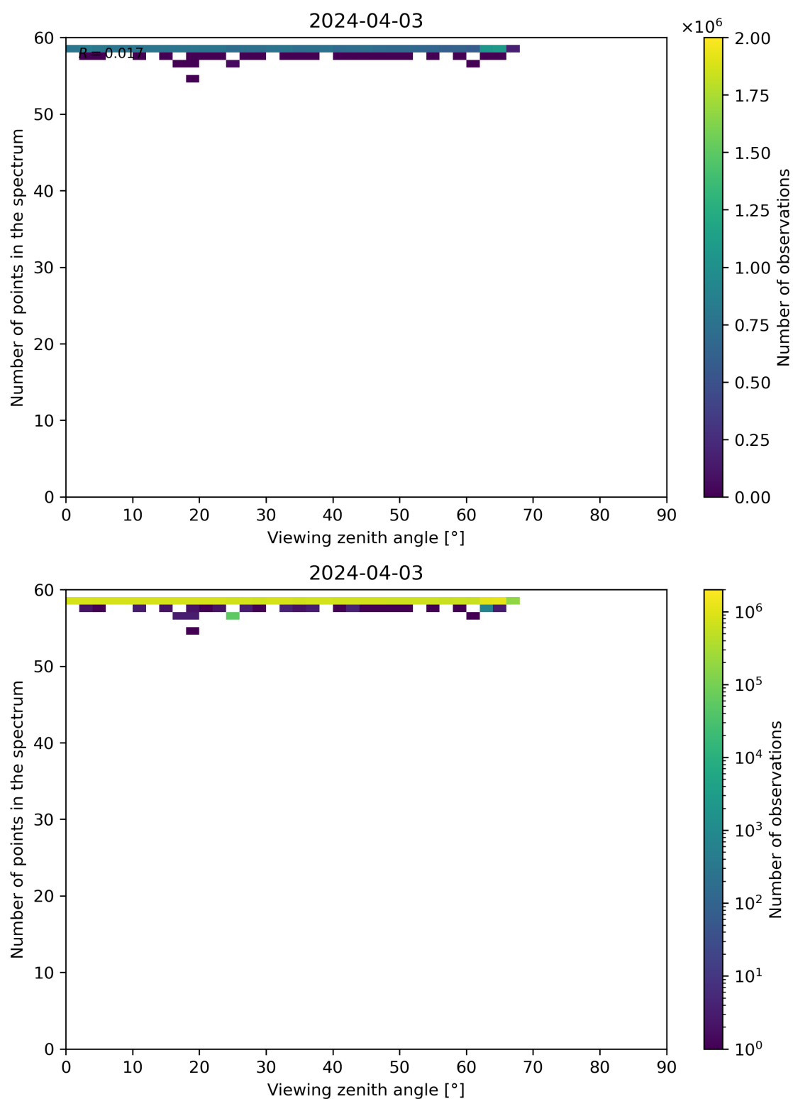
Figure 125: Scatter density plot of “Viewing zenith angle” against “Number of points in the spectrum” for 2024-04-02 to 2024-04-04.
