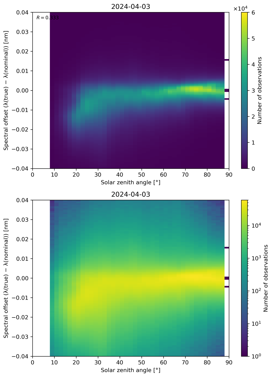
Figure 117: Scatter density plot of “Solar zenith angle” against “Spectral offset ( \lambda(\text{true}) - \lambda(\text{nominal}) )” for 2024-04-02 to 2024-04-04.
