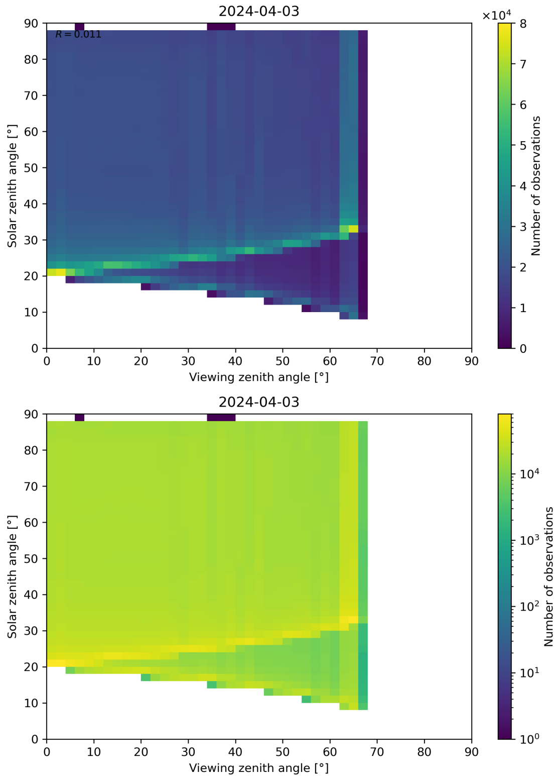
Figure 127: Scatter density plot of “Viewing zenith angle” against “Solar zenith angle” for 2024-04-02 to 2024-04-04.
