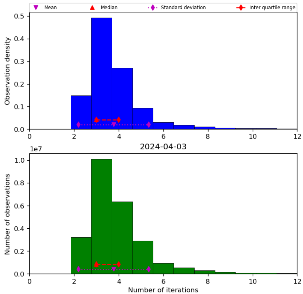
Figure 39: Histogram of “Number of iterations” for 2024-04-02 to 2024-04-04
