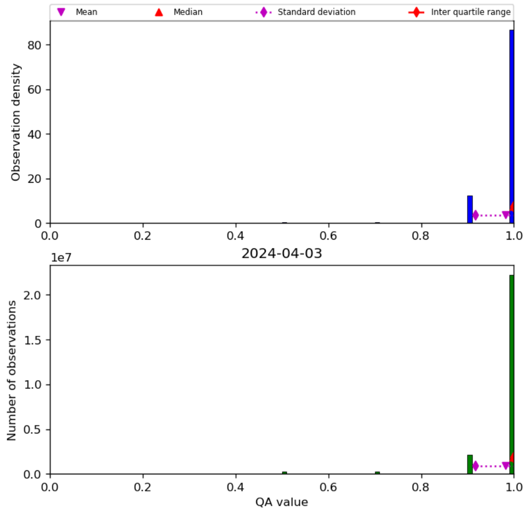
Figure 29: Histogram of “QA value” for 2024-04-02 to 2024-04-04
