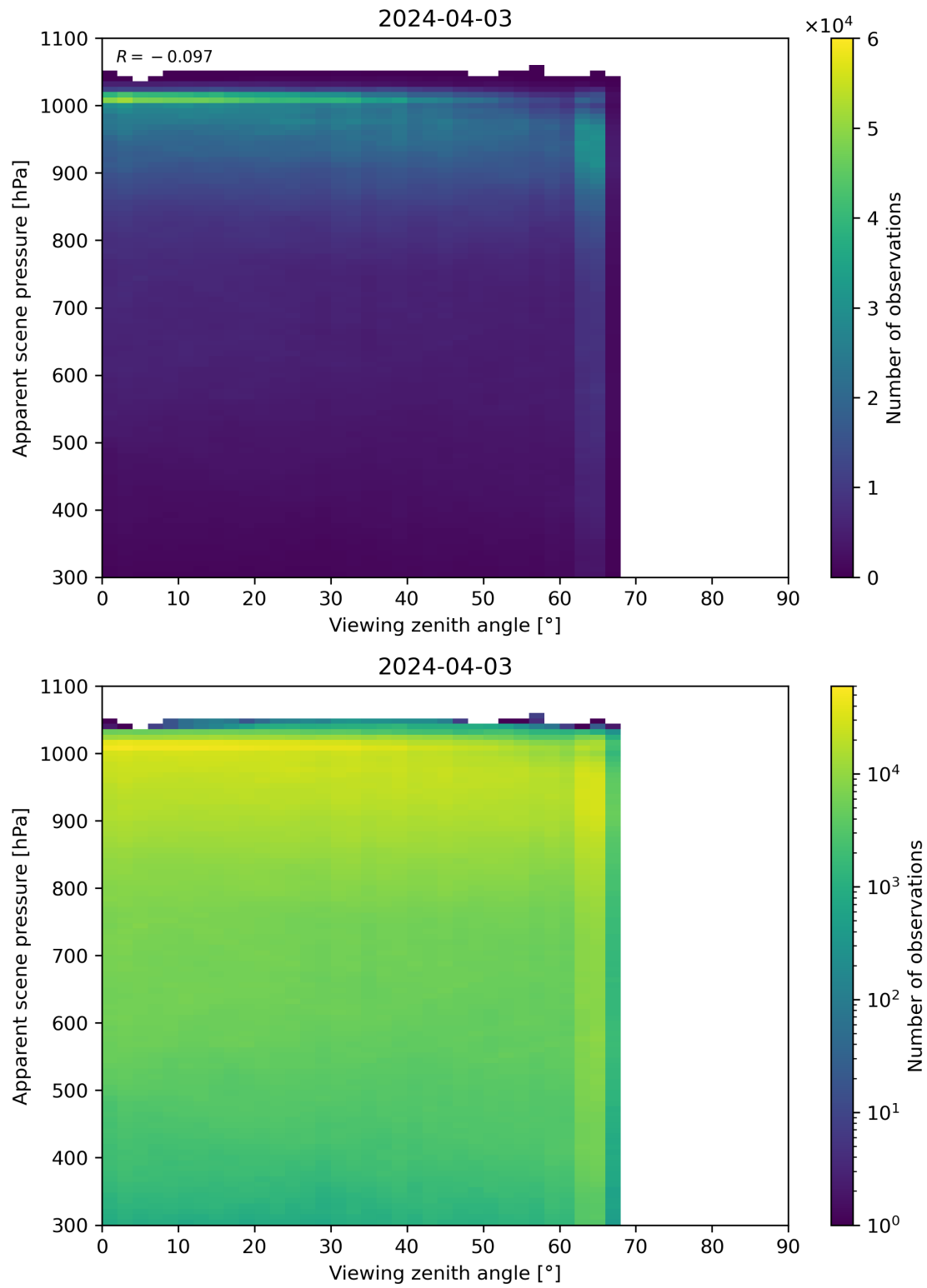
Figure 118: Scatter density plot of “Viewing zenith angle” against “Apparent scene pressure” for 2024-04-02 to 2024-04-04.
