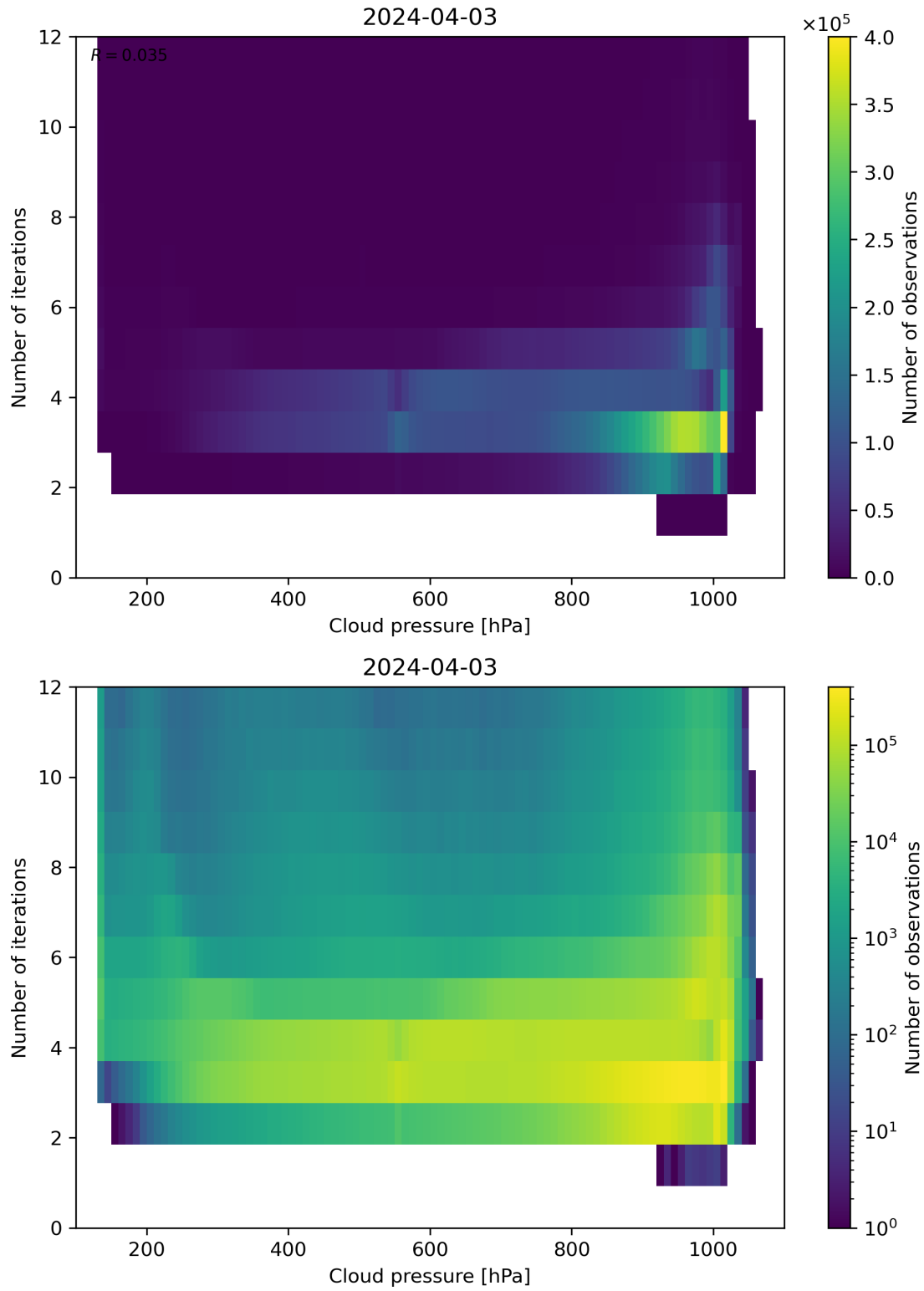
Figure 81: Scatter density plot of “Cloud pressure” against “Number of iterations” for 2024-04-02 to 2024-04-04.
