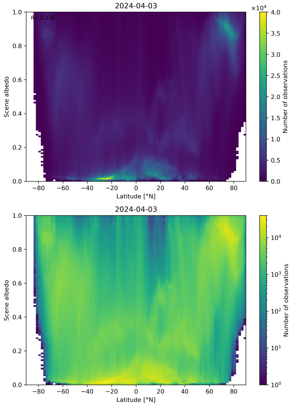
Figure 95: Scatter density plot of “Latitude” against “Scene albedo” for 2024-04-02 to 2024-04-04.
