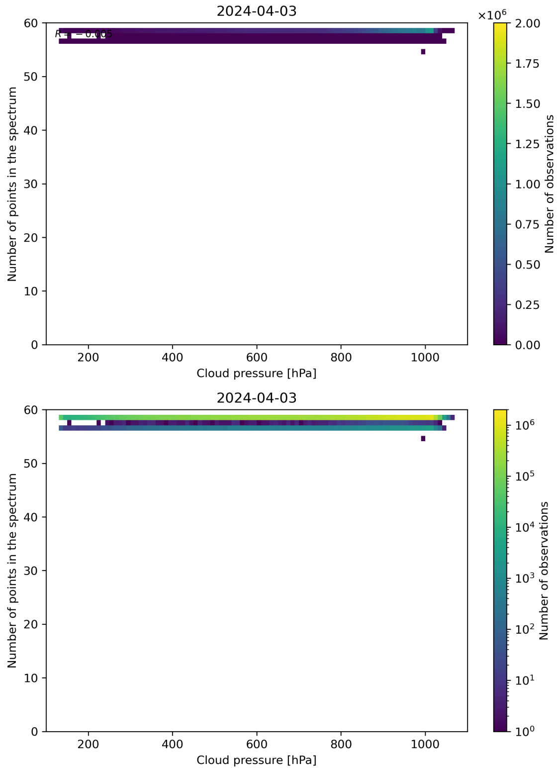
Figure 82: Scatter density plot of “Cloud pressure” against “Number of points in the spectrum” for 2024-04-02 to 2024-04-04.
