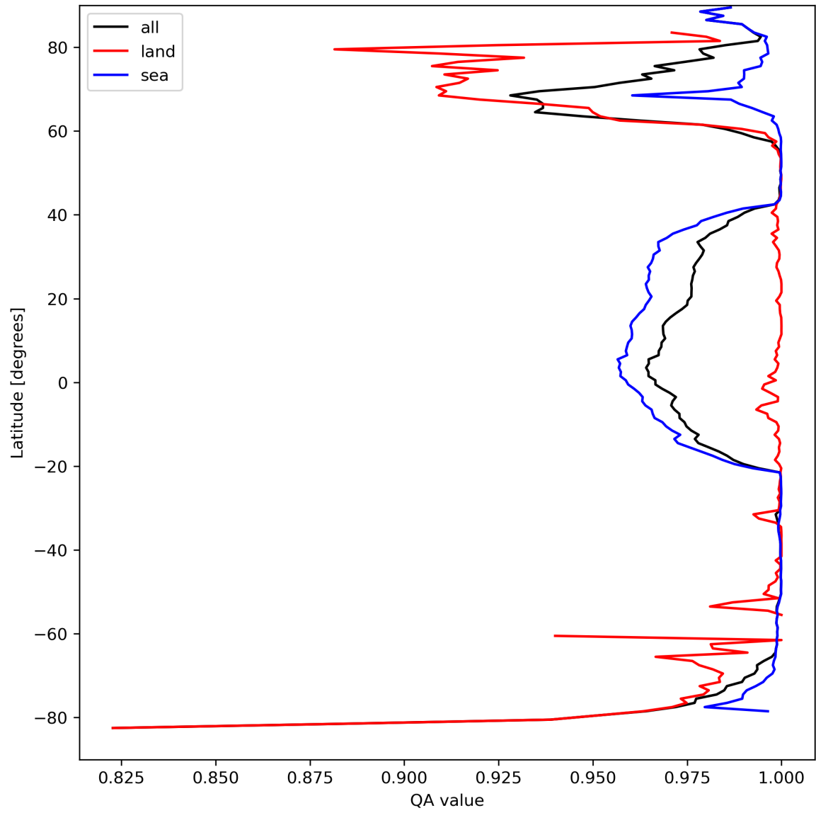
Figure 12: Zonal average of “QA value” for 2024-04-02 to 2024-04-04.
