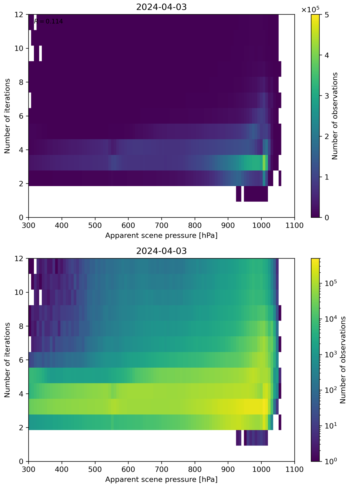
Figure 65: Scatter density plot of “Apparent scene pressure” against “Number of iterations” for 2024-04-02 to 2024-04-04.
