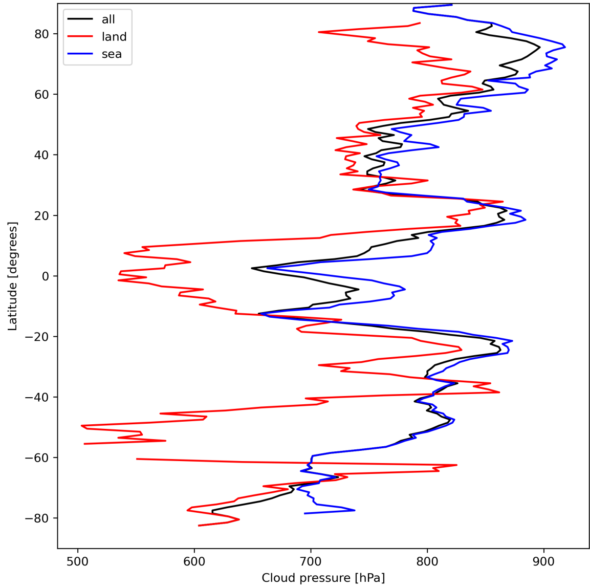
Figure 13: Zonal average of “Cloud pressure” for 2024-04-02 to 2024-04-04.
