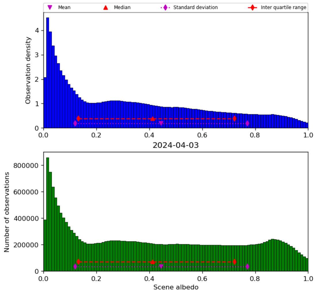
Figure 34: Histogram of “Scene albedo” for 2024-04-02 to 2024-04-04
