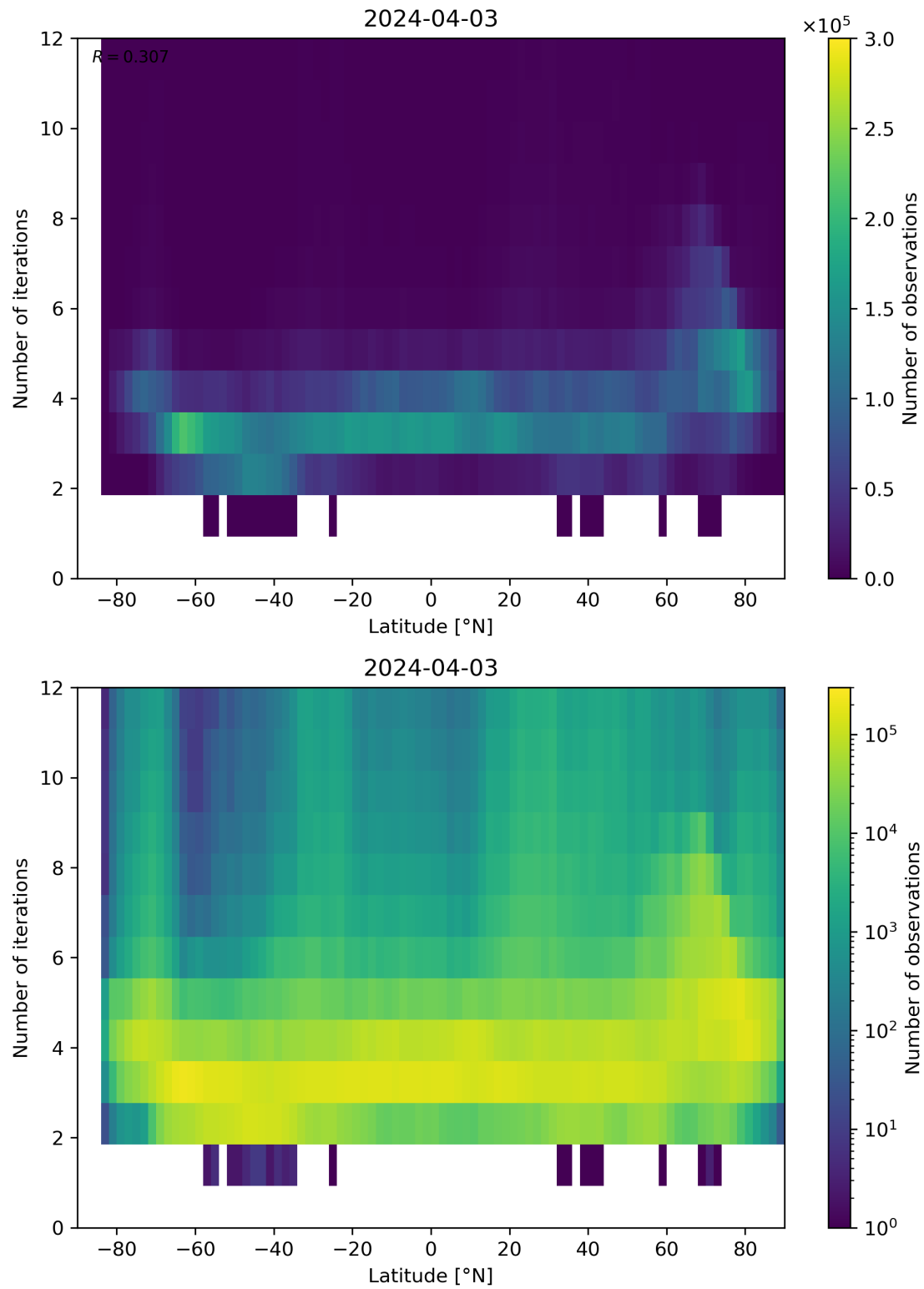
Figure 93: Scatter density plot of “Latitude” against “Number of iterations” for 2024-04-02 to 2024-04-04.
