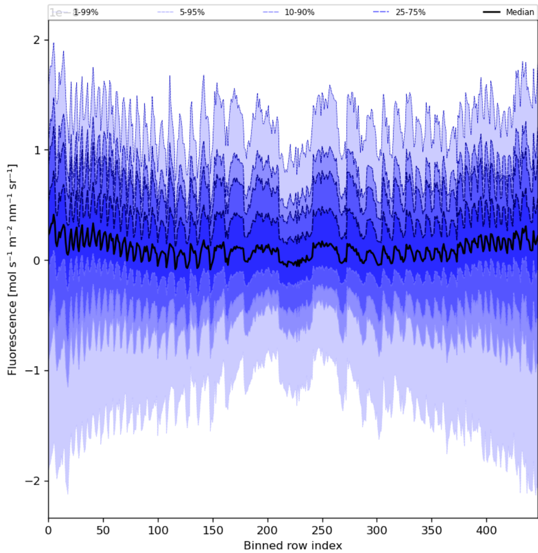
Figure 57: Along track statistics of “Fluorescence” for 2024-04-02 to 2024-04-04
