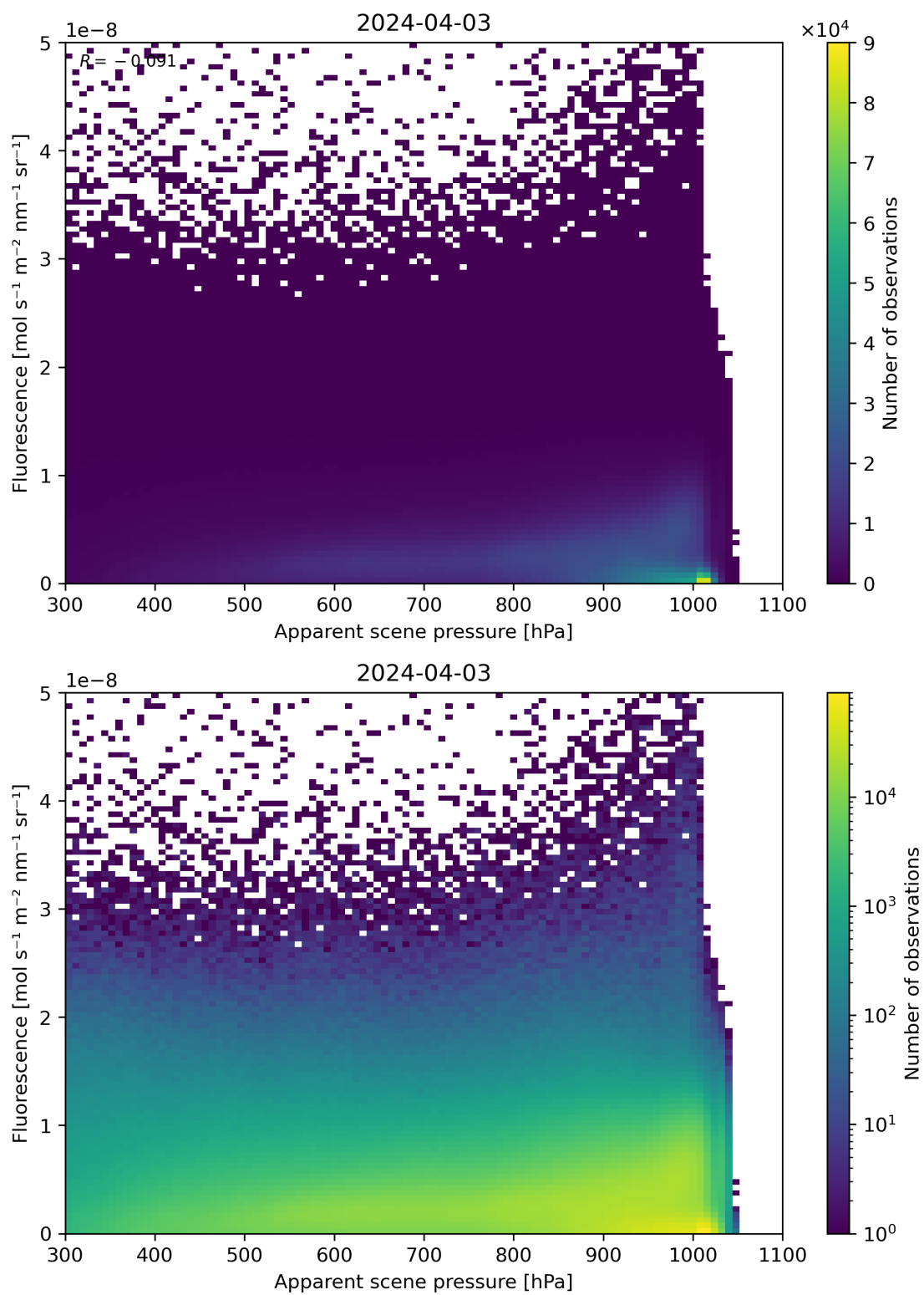
Figure 64: Scatter density plot of “Apparent scene pressure” against “Fluorescence” for 2024-04-02 to 2024-04-04.
