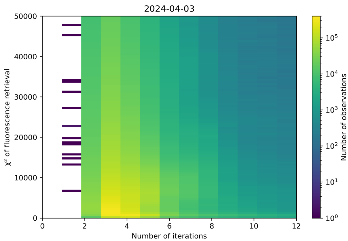
Figure 97: Scatter density plot of “Number of iterations” against “ \chi^2 of fluorescence retrieval” for 2024-04-02 to 2024-04-04.
