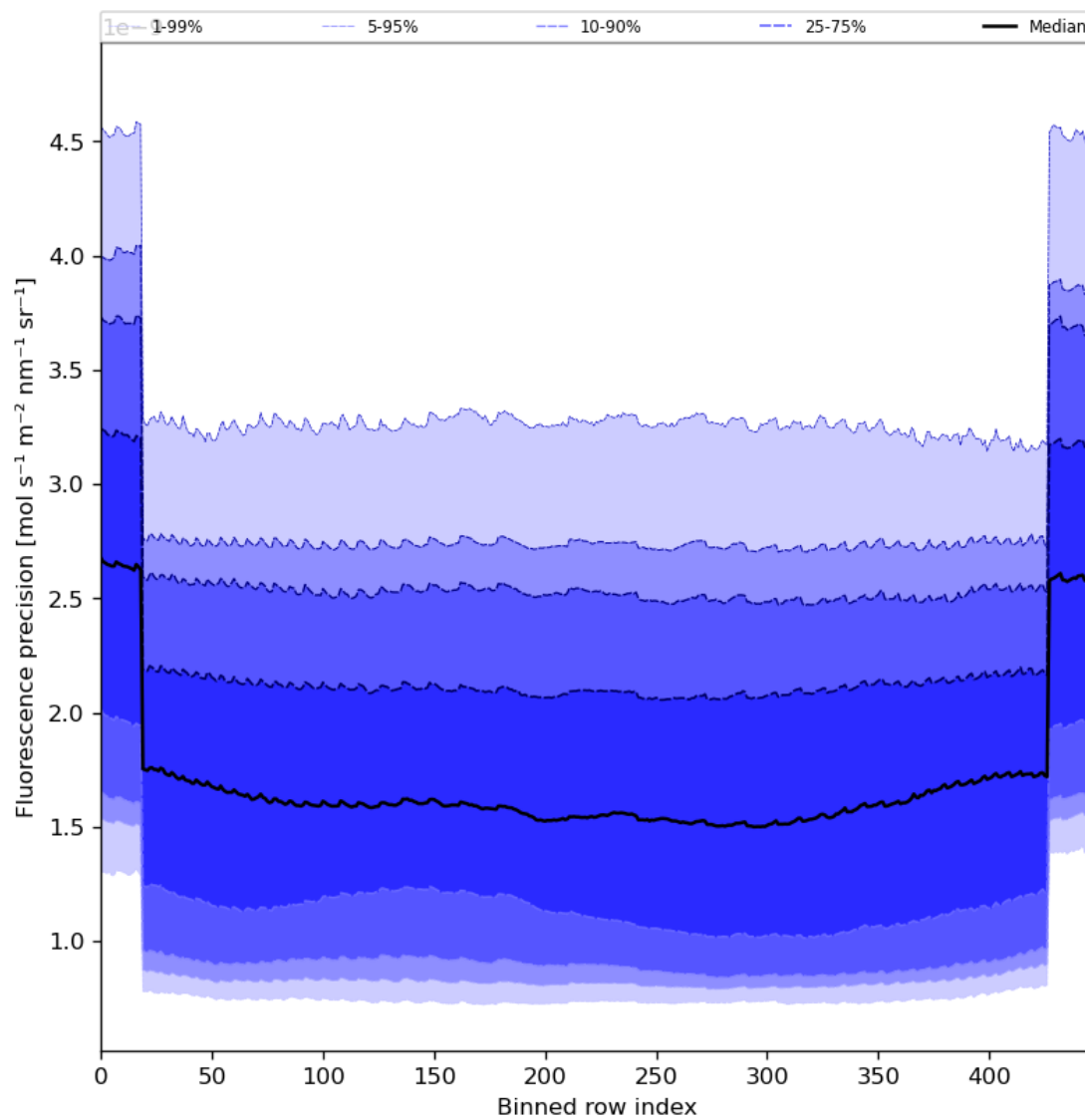
Figure 58: Along track statistics of “Fluorescence precision” for 2024-04-02 to 2024-04-04
