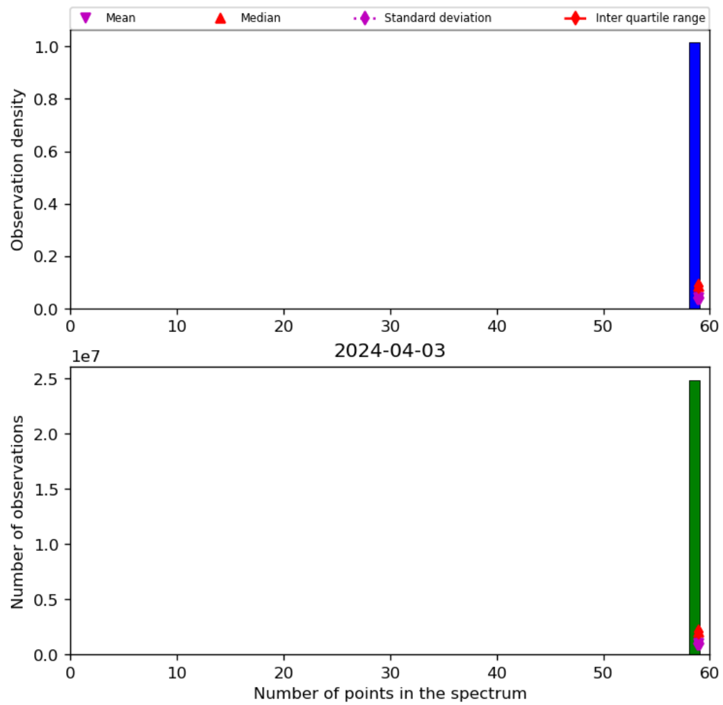
Figure 44: Histogram of “Number of points in the spectrum” for 2024-04-02 to 2024-04-04
