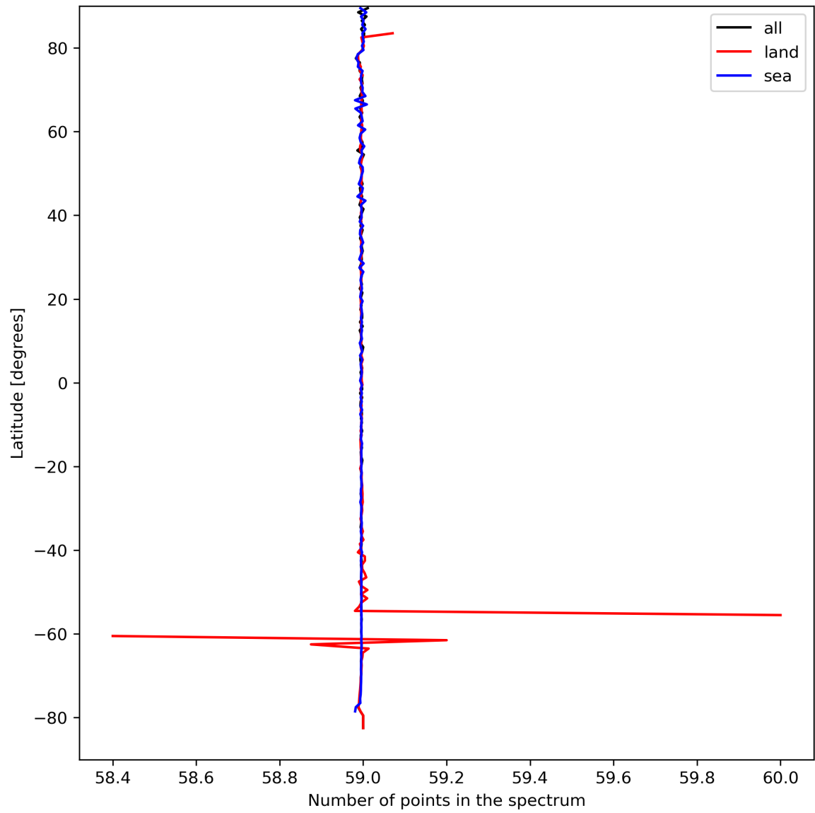
Figure 27: Zonal average of “Number of points in the spectrum” for 2024-04-02 to 2024-04-04.
