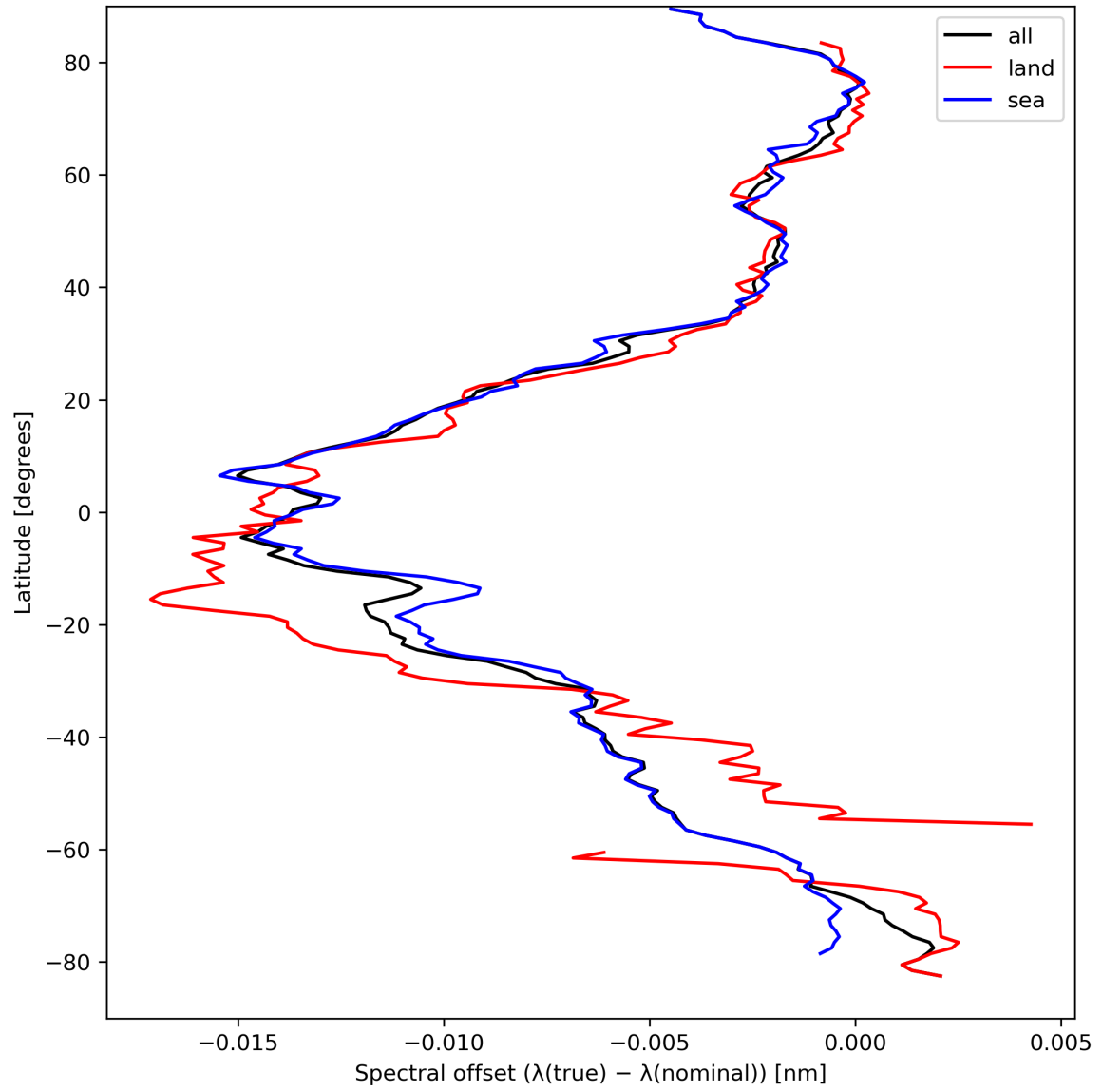
Figure 28: Zonal average of “Spectral offset ( \lambda(\text{true}) - \lambda(\text{nominal}) )” for 2024-04-02 to 2024-04-04.
