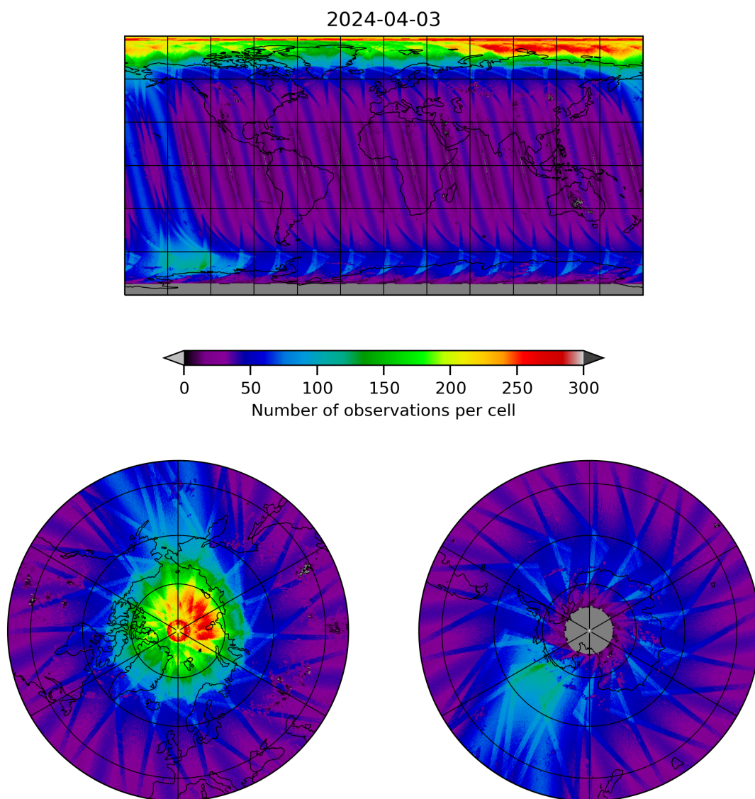
Figure 11: Map of the number of observations for 2024-04-02 to 2024-04-04
