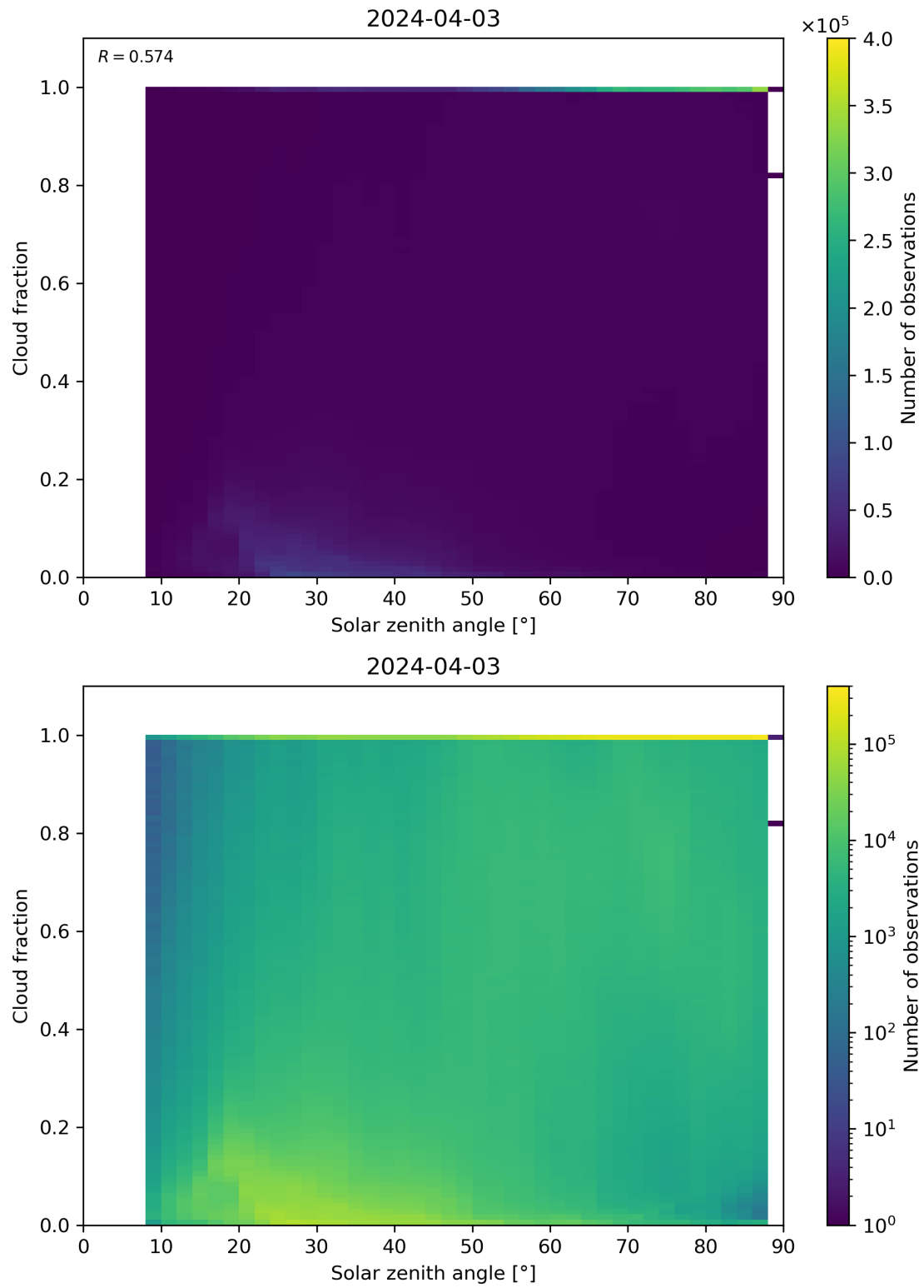
Figure 110: Scatter density plot of “Solar zenith angle” against “Cloud fraction” for 2024-04-02 to 2024-04-04.
