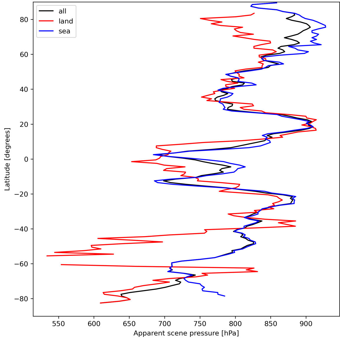
Figure 19: Zonal average of “Apparent scene pressure” for 2024-04-02 to 2024-04-04.
