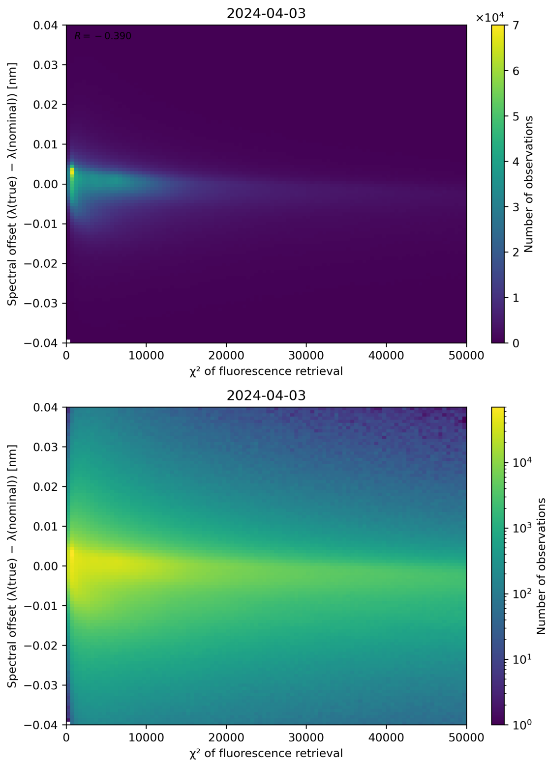
Figure 69: Scatter density plot of " \chi^2 of fluorescence retrieval" against "Spectral offset ( \lambda(\text{true}) - \lambda(\text{nominal}) )" for 2024-04-02 to 2024-04-04.
