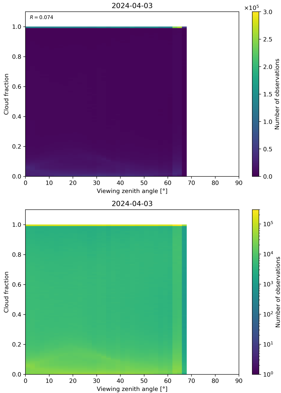
Figure 120: Scatter density plot of “Viewing zenith angle” against “Cloud fraction” for 2024-04-02 to 2024-04-04.
