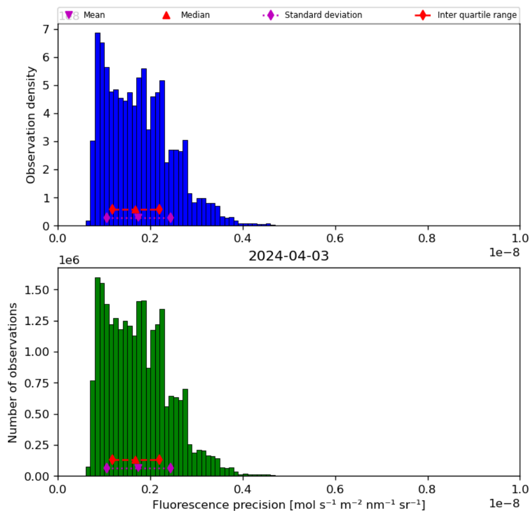
Figure 41: Histogram of “Fluorescence precision” for 2024-04-02 to 2024-04-04
