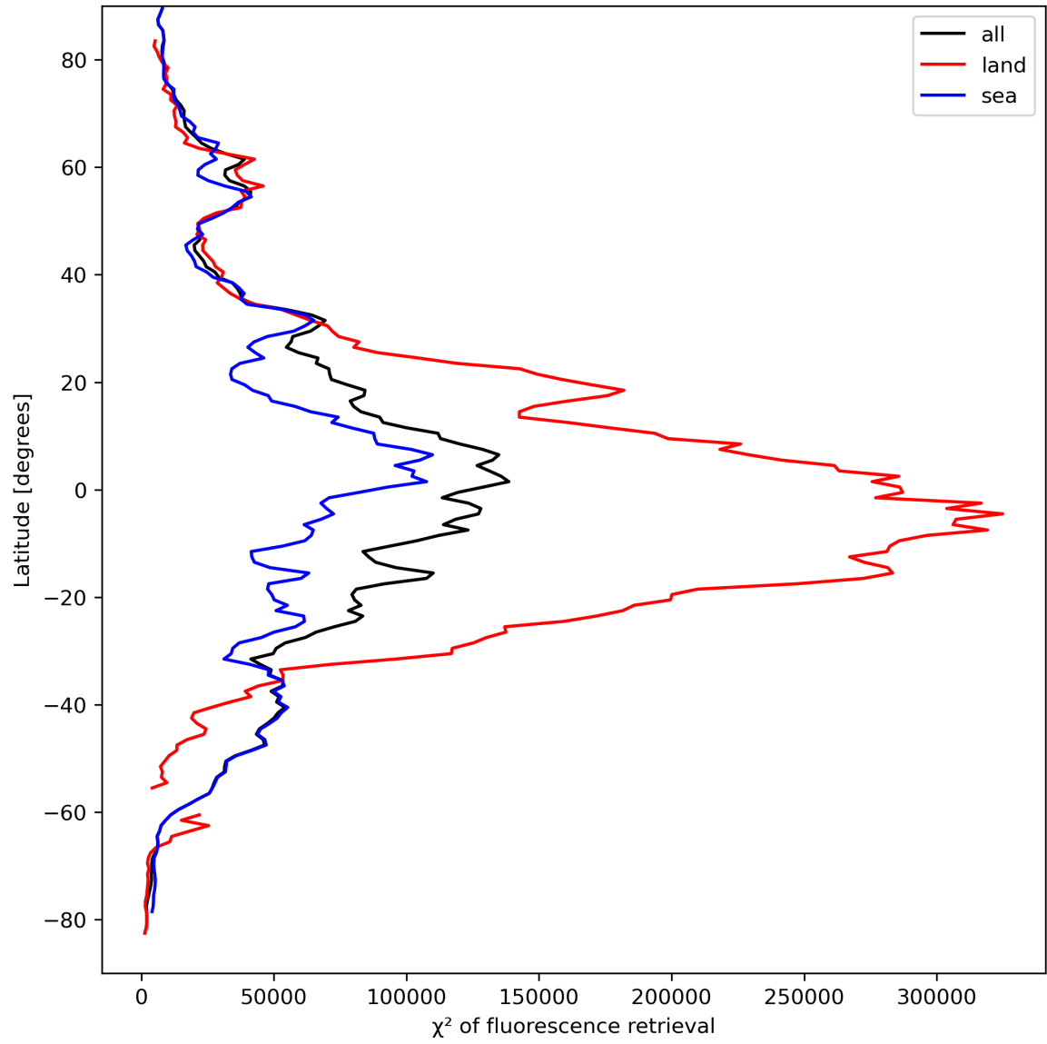
Figure 25: Zonal average of “ \chi^2 of fluorescence retrieval” for 2024-04-02 to 2024-04-04.
