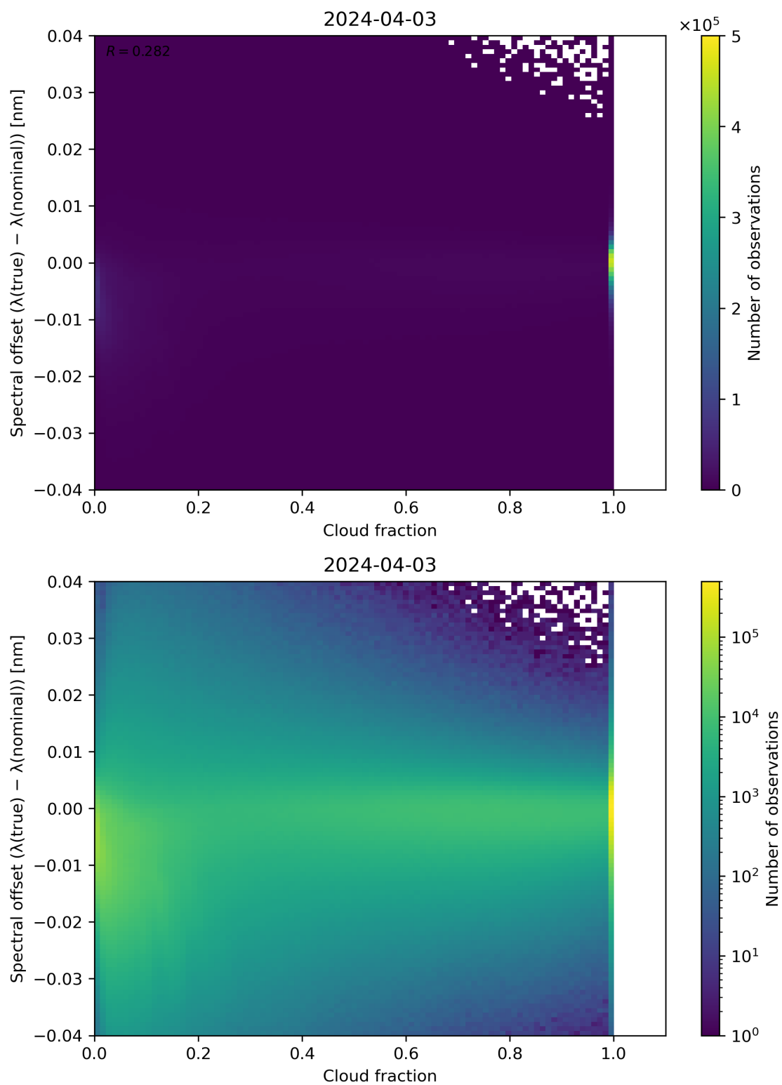
Figure 76: Scatter density plot of “Cloud fraction” against “Spectral offset ( \lambda(\text{true}) - \lambda(\text{nominal}) )” for 2024-04-02 to 2024-04-04.
