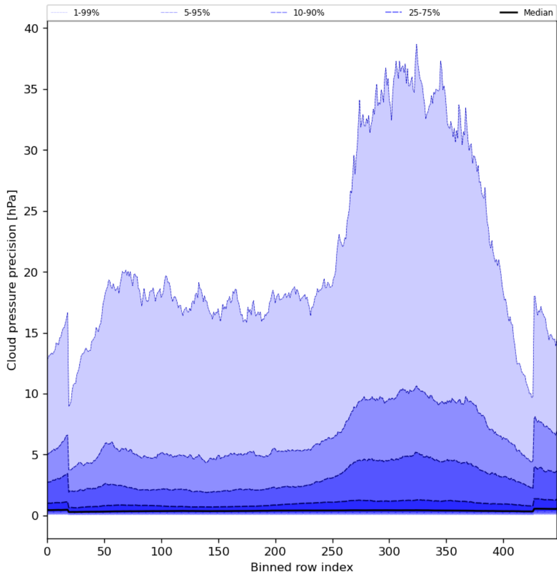
Figure 48: Along track statistics of “Cloud pressure precision” for 2024-04-02 to 2024-04-04
