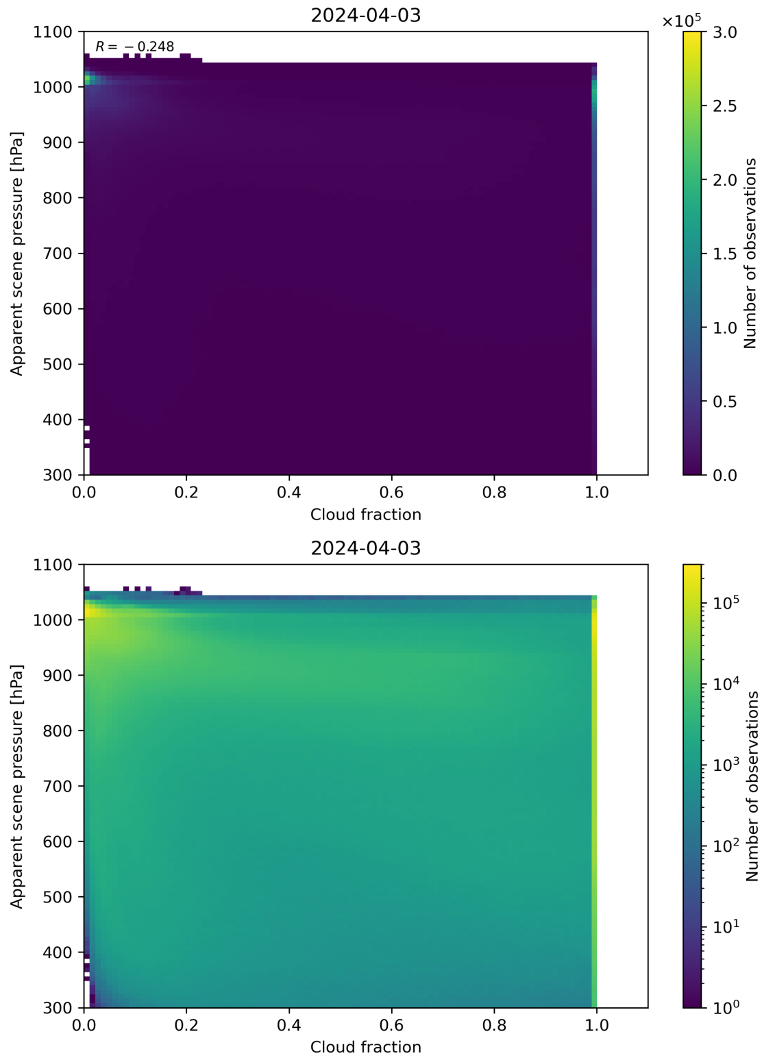
Figure 70: Scatter density plot of “Cloud fraction” against “Apparent scene pressure” for 2024-04-02 to 2024-04-04.
