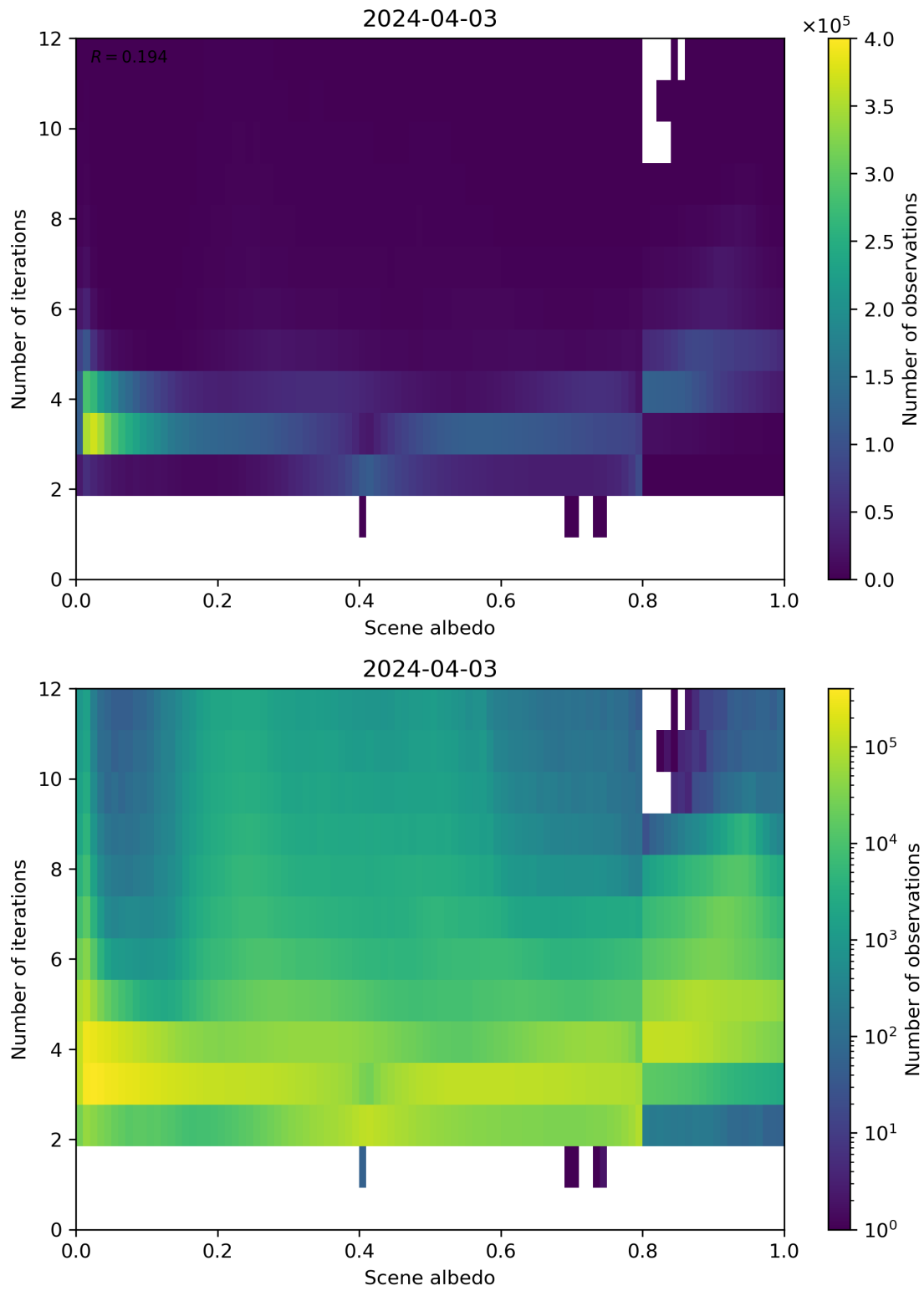
Figure 105: Scatter density plot of “Scene albedo” against “Number of iterations” for 2024-04-02 to 2024-04-04.
