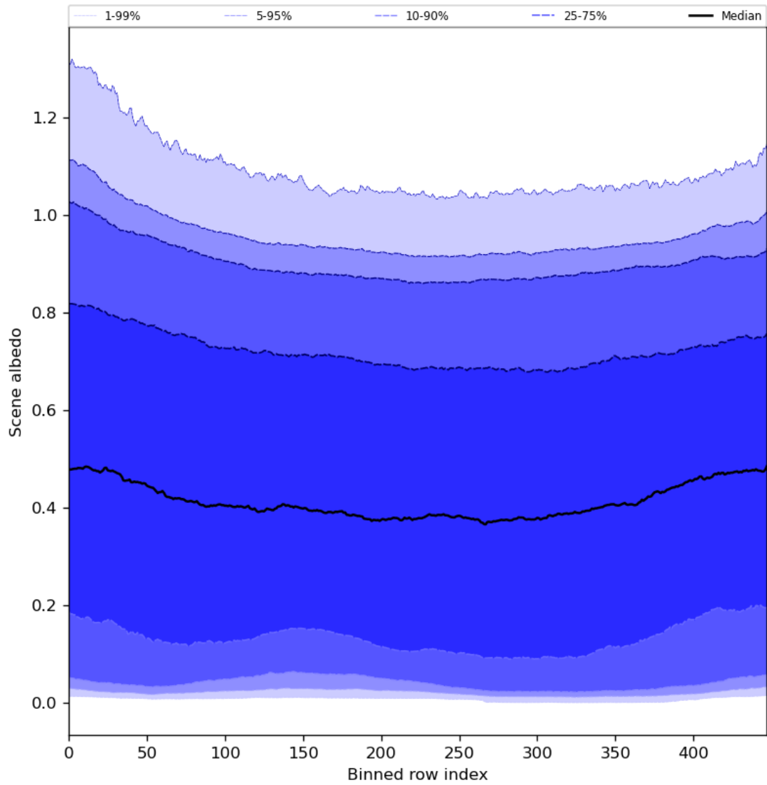
Figure 51: Along track statistics of “Scene albedo” for 2024-04-02 to 2024-04-04
