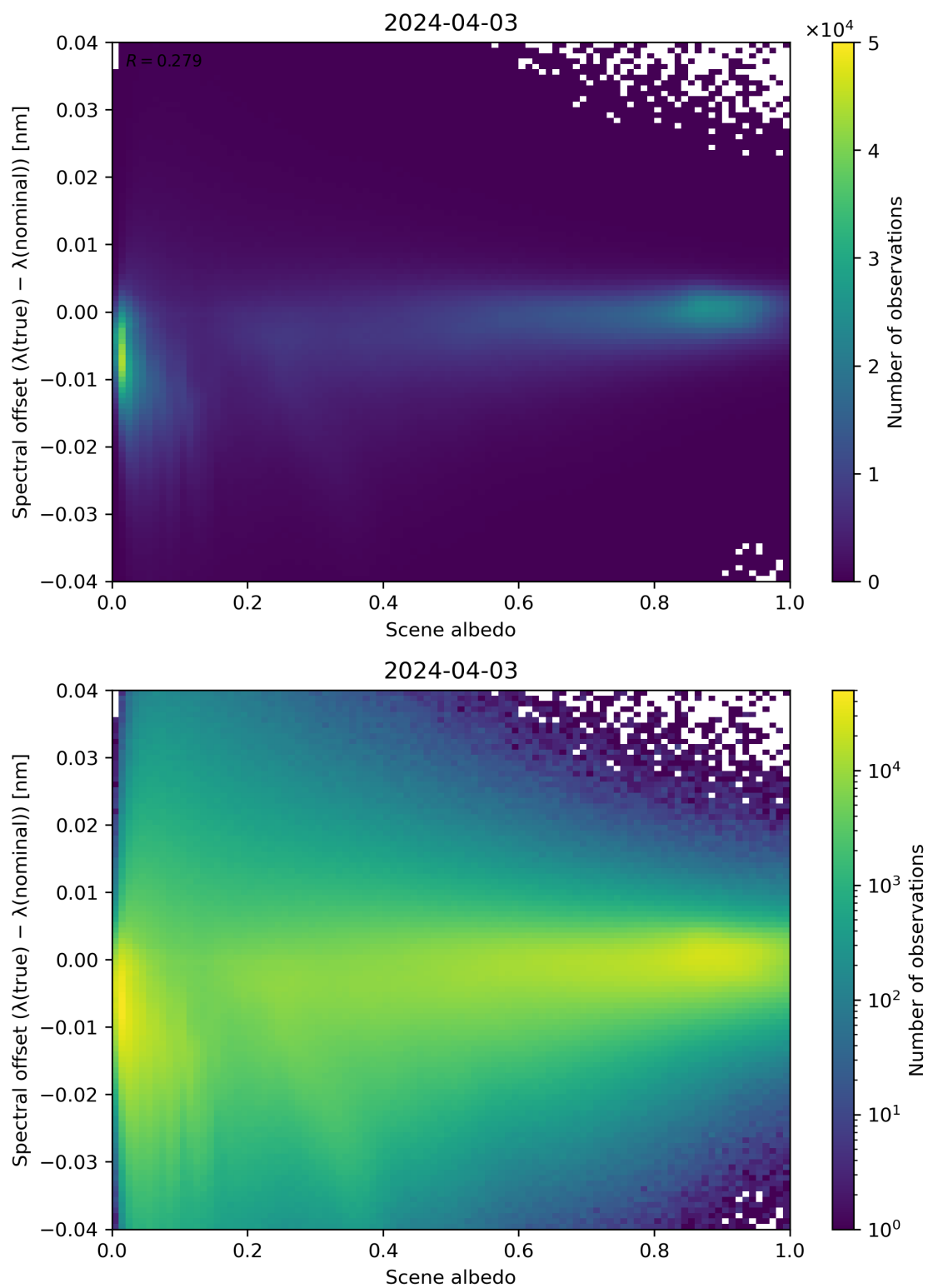
Figure 107: Scatter density plot of “Scene albedo” against “Spectral offset ( \lambda(\text{true}) - \lambda(\text{nominal}) )” for 2024-04-02 to 2024-04-04.
