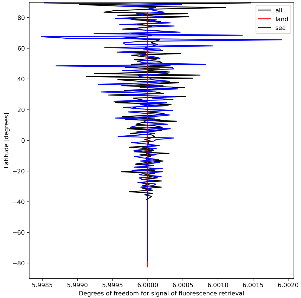
Figure 26: Zonal average of “Degrees of freedom for signal of fluorescence retrieval” for 2024-04-02 to 2024-04-04.
