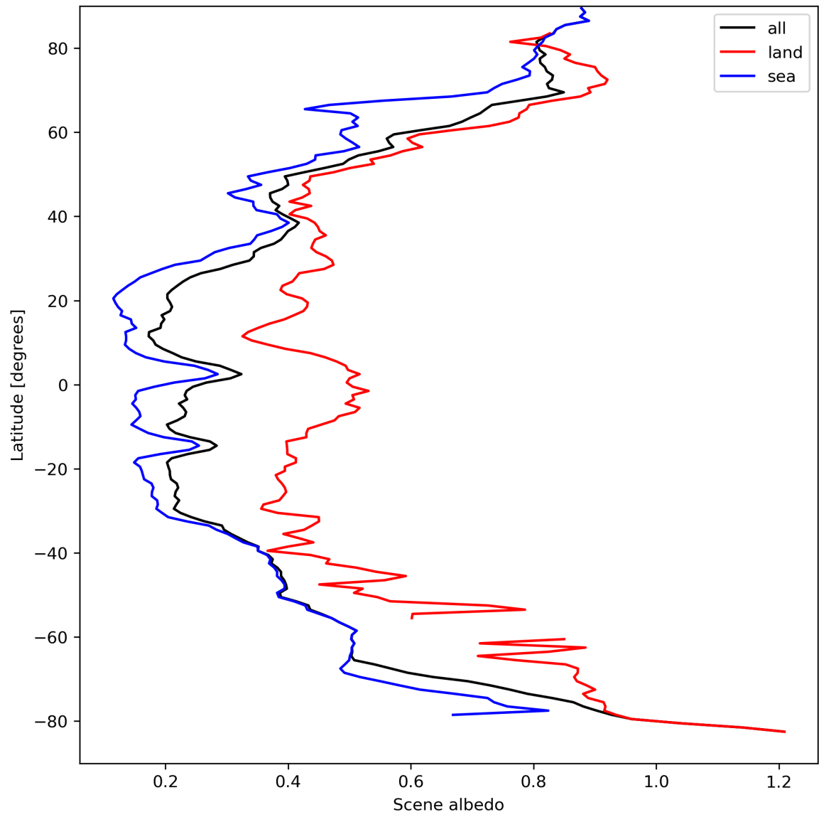
Figure 17: Zonal average of “Scene albedo” for 2024-04-02 to 2024-04-04.
