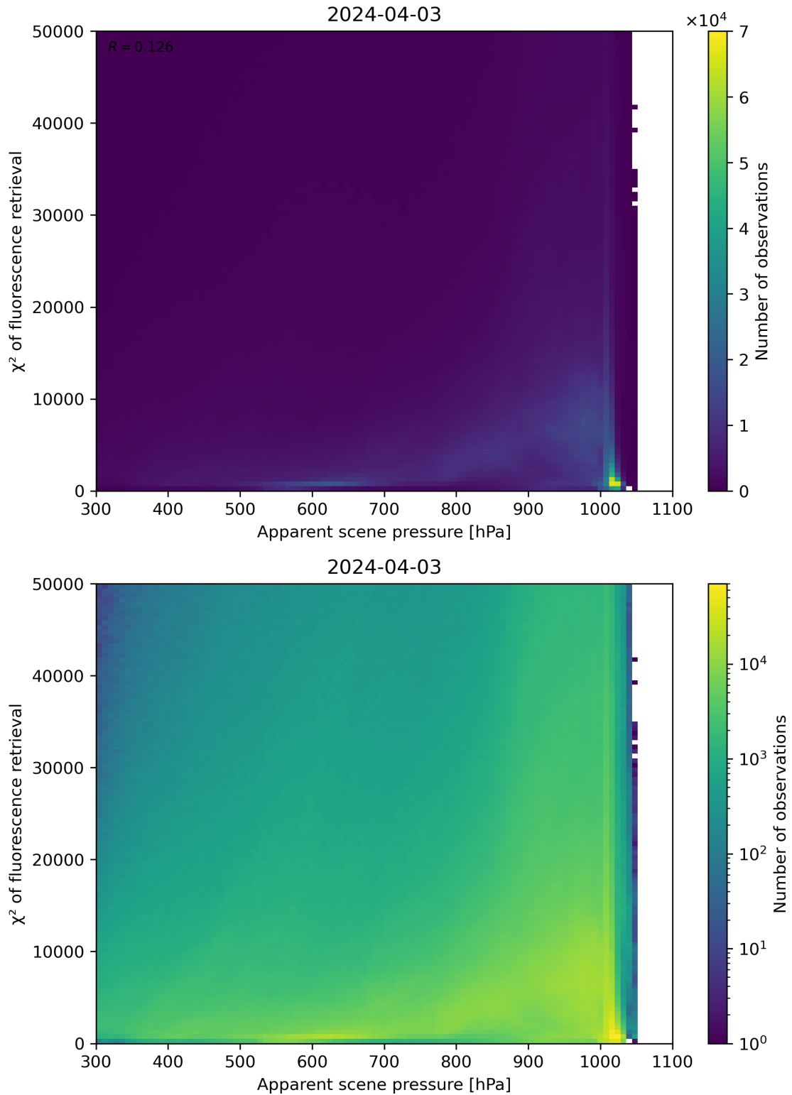
Figure 63: Scatter density plot of “Apparent scene pressure” against “ \chi^2 of fluorescence retrieval” for 2024-04-02 to 2024-04-04.
