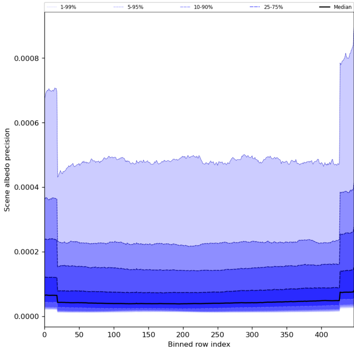
Figure 52: Along track statistics of “Scene albedo precision” for 2024-04-02 to 2024-04-04
