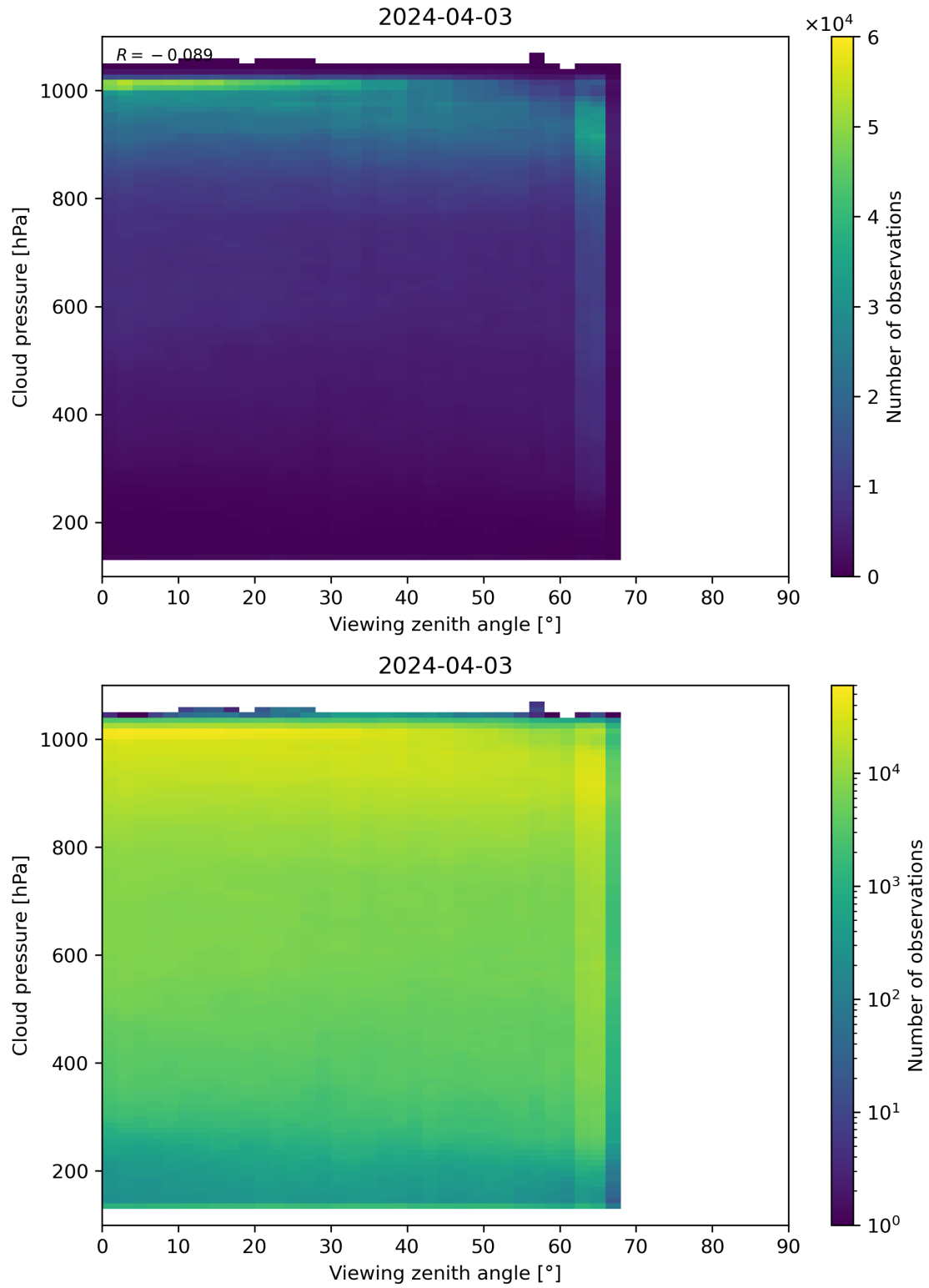
Figure 121: Scatter density plot of “Viewing zenith angle” against “Cloud pressure” for 2024-04-02 to 2024-04-04.
