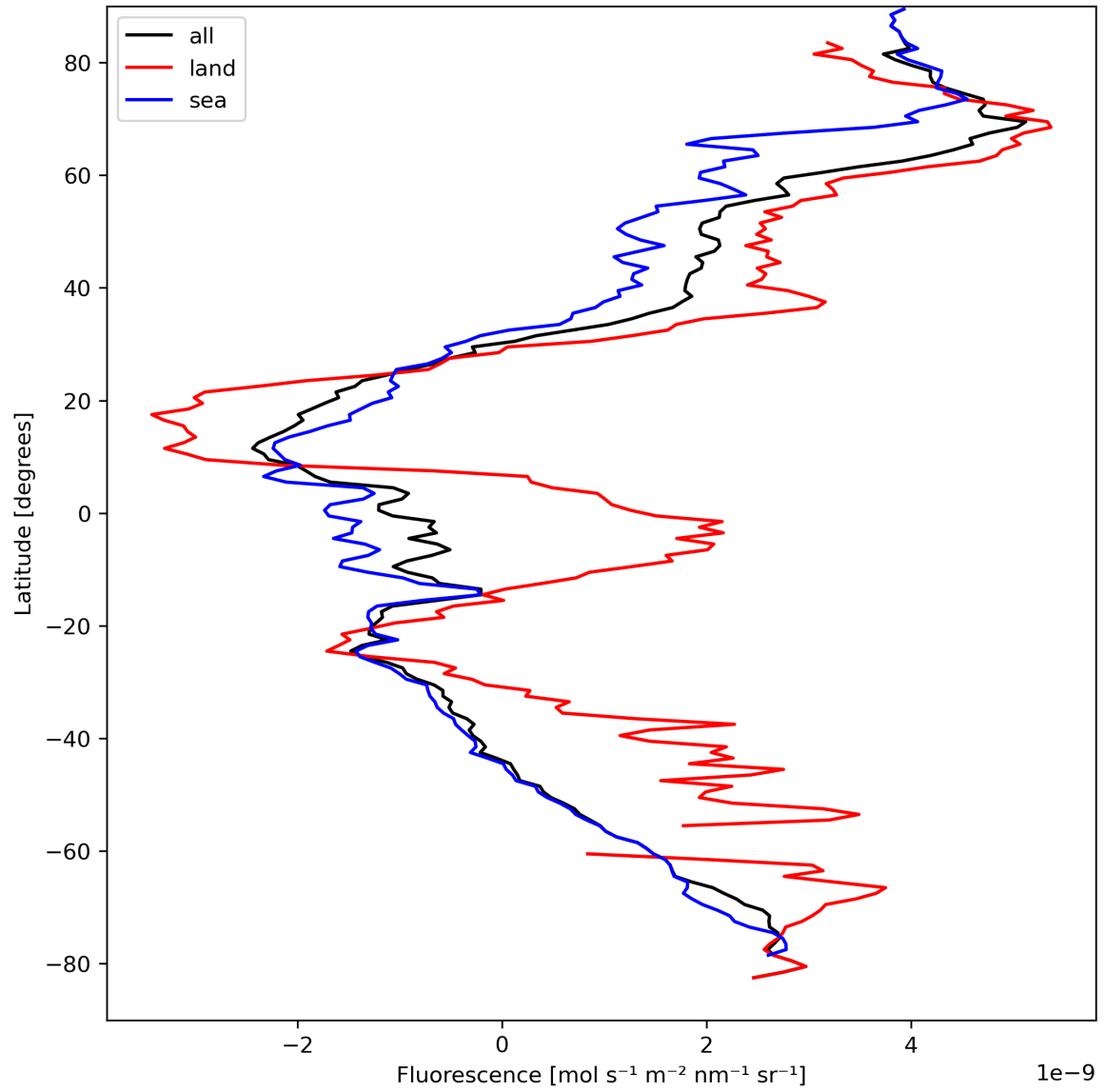
Figure 23: Zonal average of “Fluorescence” for 2024-04-02 to 2024-04-04.
