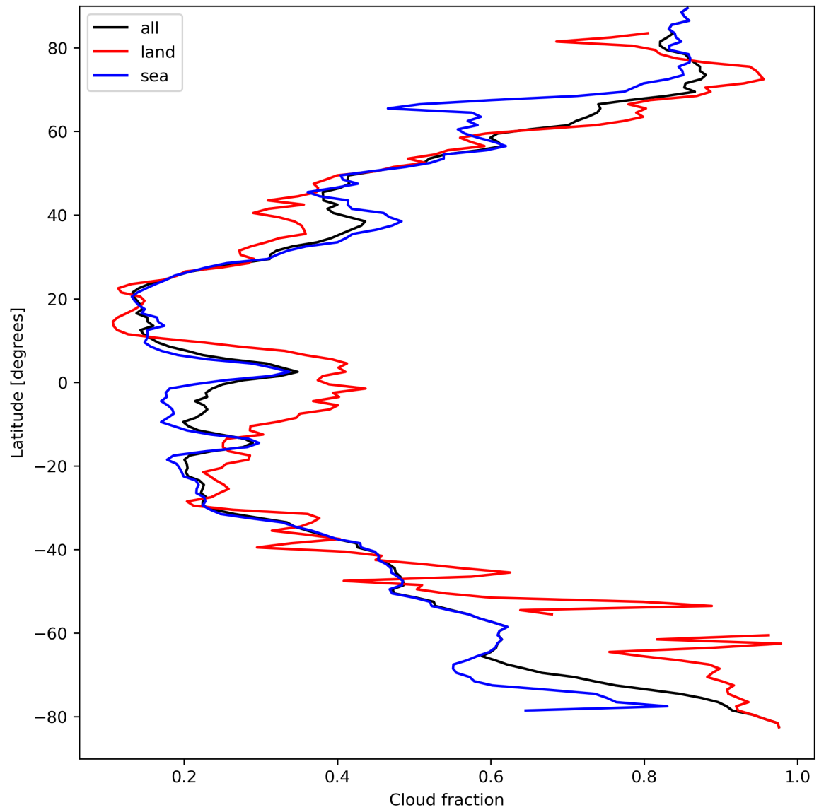
Figure 15: Zonal average of “Cloud fraction” for 2024-04-02 to 2024-04-04.
