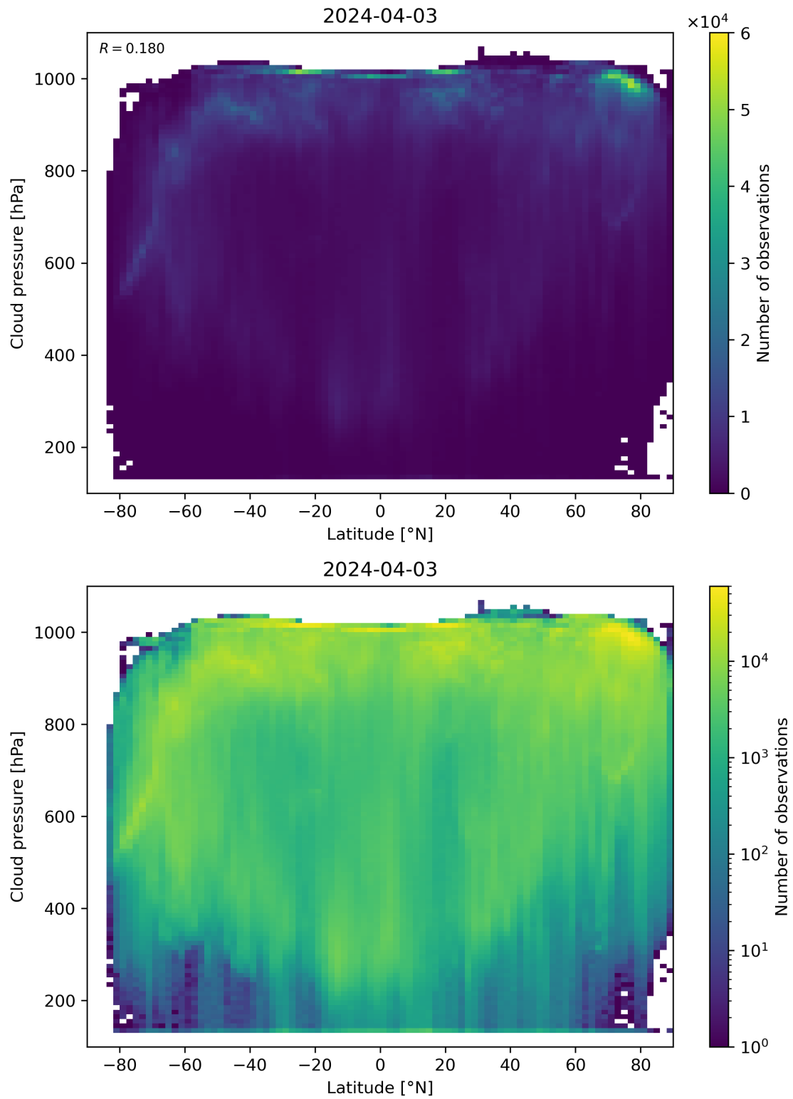
Figure 91: Scatter density plot of “Latitude” against “Cloud pressure” for 2024-04-02 to 2024-04-04.
