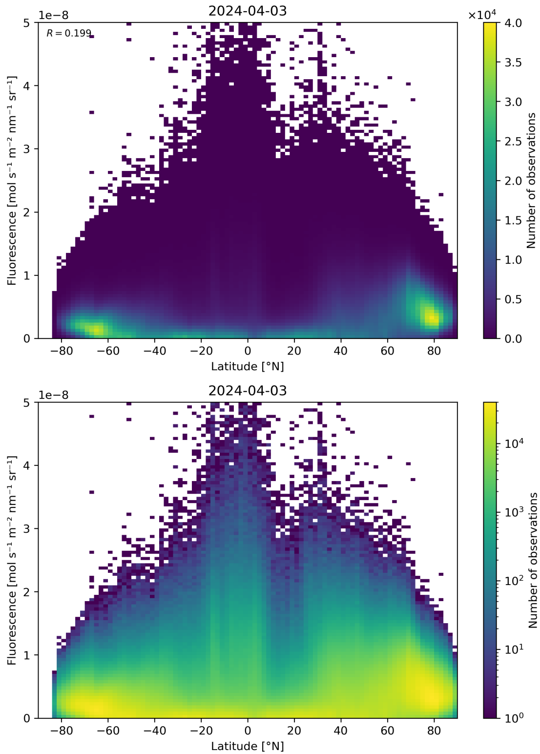
Figure 92: Scatter density plot of “Latitude” against “Fluorescence” for 2024-04-02 to 2024-04-04.
