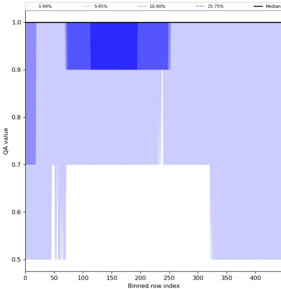
Figure 46: Along track statistics of “QA value” for 2024-04-02 to 2024-04-04
