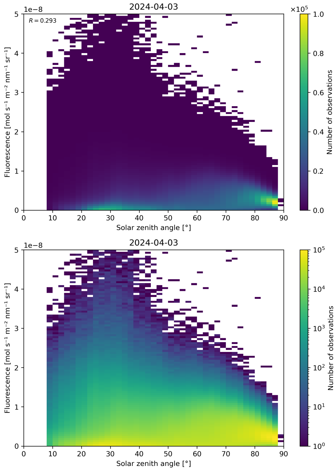
Figure 112: Scatter density plot of “Solar zenith angle” against “Fluorescence” for 2024-04-02 to 2024-04-04.
