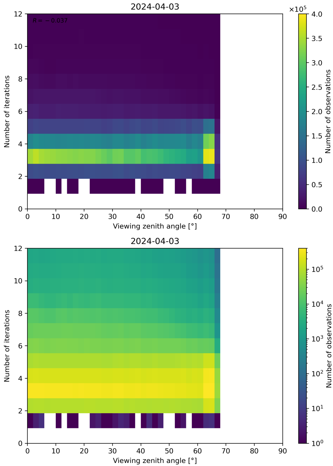
Figure 124: Scatter density plot of “Viewing zenith angle” against “Number of iterations” for 2024-04-02 to 2024-04-04.
