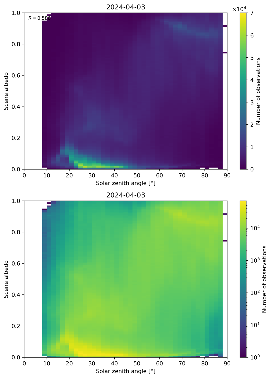
Figure 116: Scatter density plot of “Solar zenith angle” against “Scene albedo” for 2024-04-02 to 2024-04-04.
