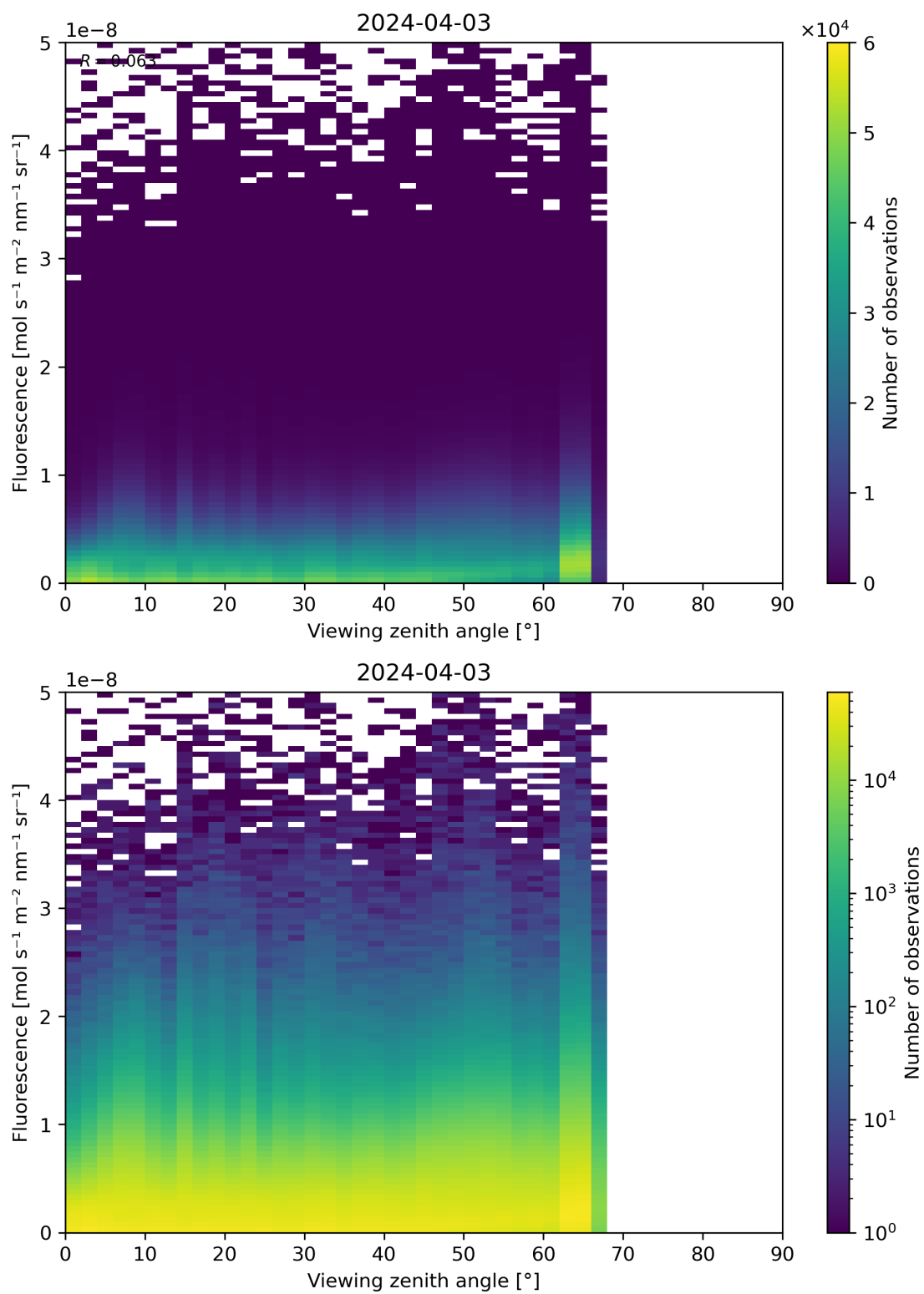
Figure 122: Scatter density plot of “Viewing zenith angle” against “Fluorescence” for 2024-04-02 to 2024-04-04.
