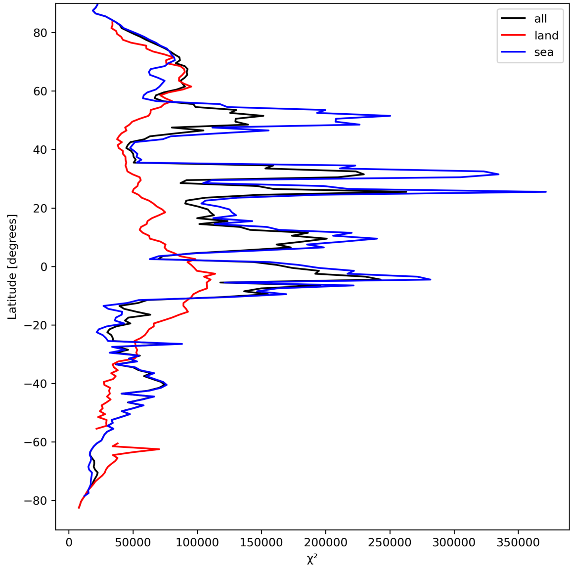
Figure 21: Zonal average of “ \chi^2 ” for 2024-04-02 to 2024-04-04.
