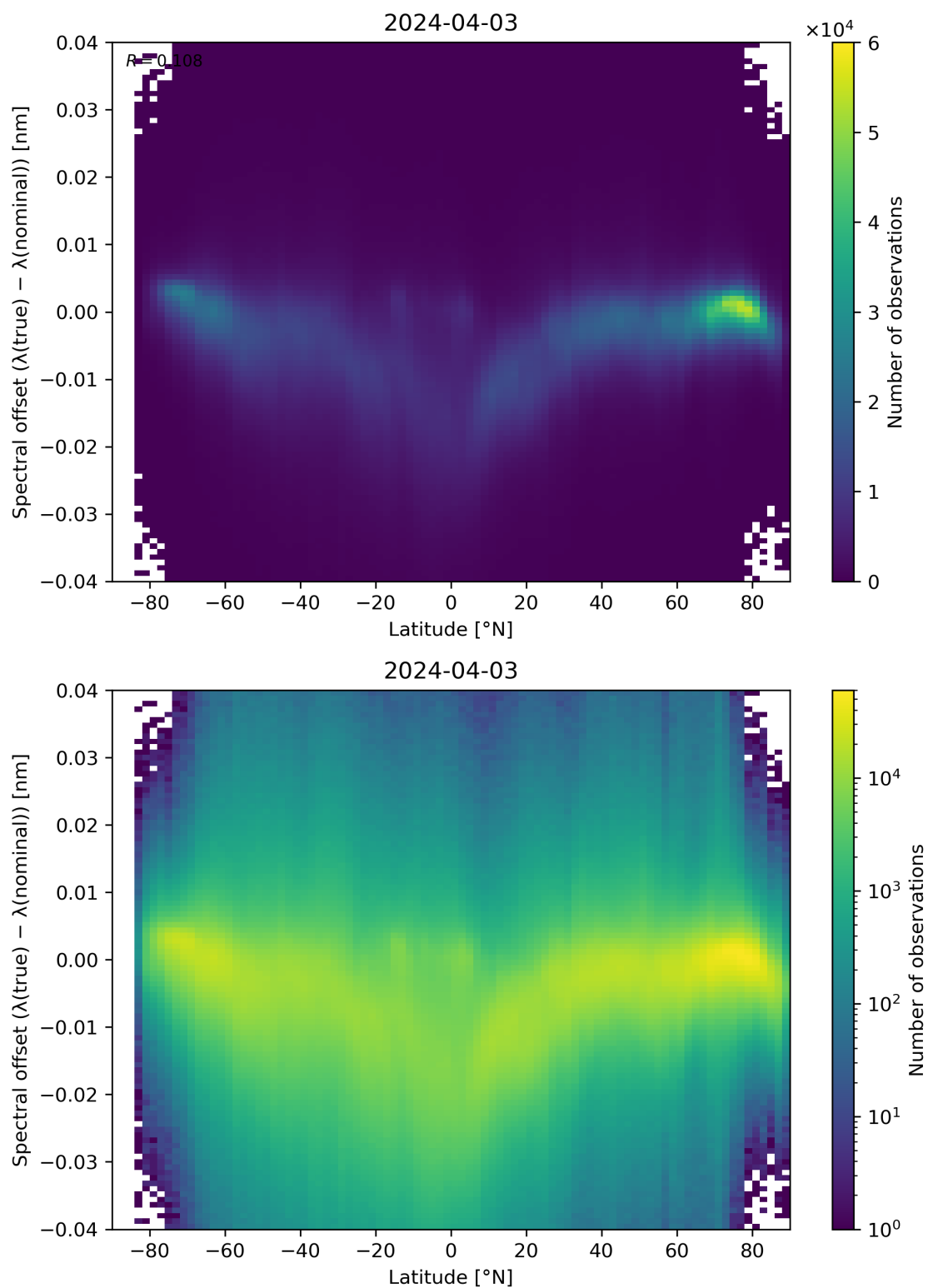
Figure 96: Scatter density plot of “Latitude” against “Spectral offset ( \lambda(\text{true}) - \lambda(\text{nominal}) )” for 2024-04-02 to 2024-04-04.
