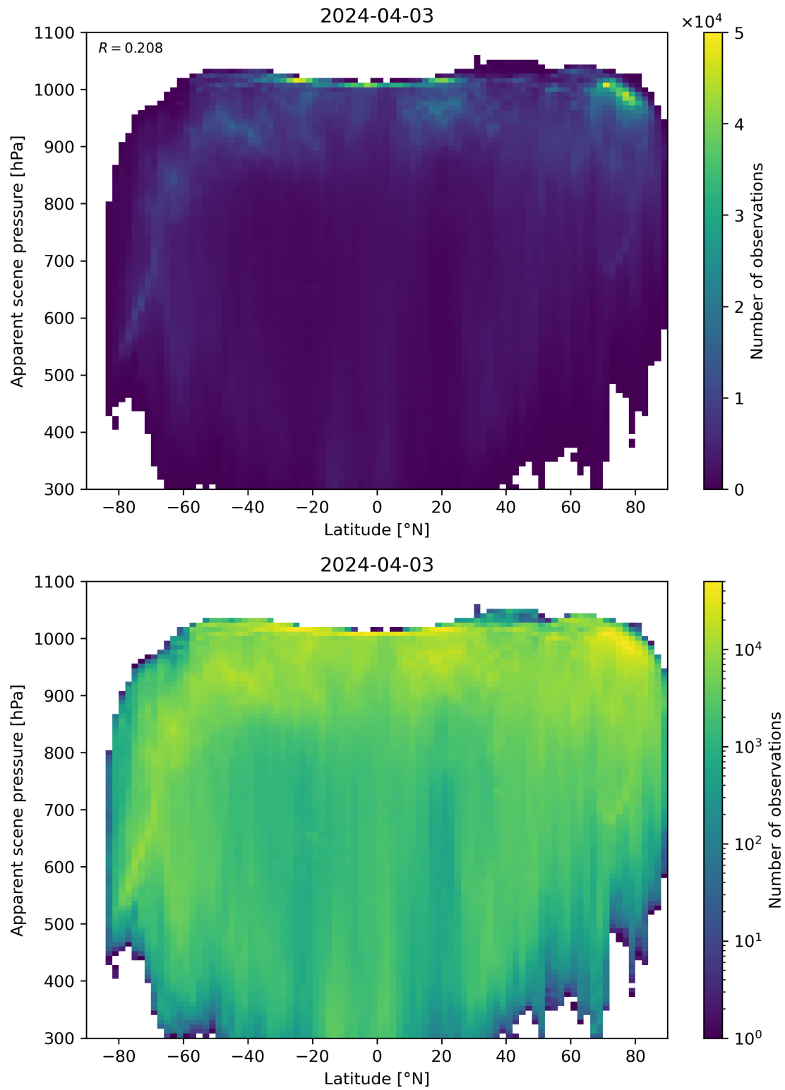
Figure 88: Scatter density plot of “Latitude” against “Apparent scene pressure” for 2024-04-02 to 2024-04-04.
