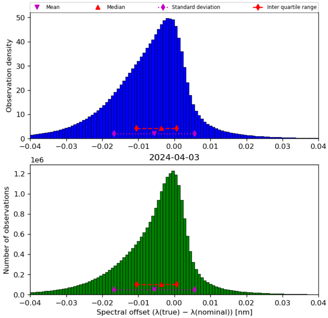
Figure 45: Histogram of “Spectral offset ( \lambda(\text{true}) - \lambda(\text{nominal}) )” for 2024-04-02 to 2024-04-04
