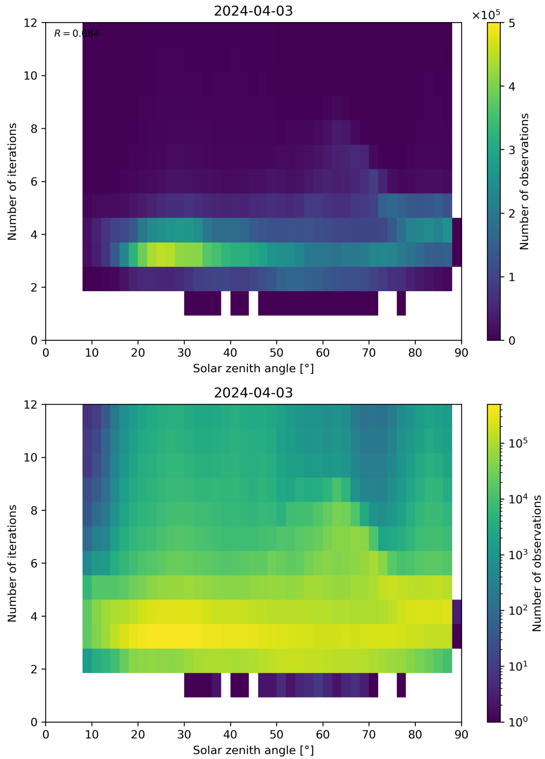
Figure 114: Scatter density plot of “Solar zenith angle” against “Number of iterations” for 2024-04-02 to 2024-04-04.
