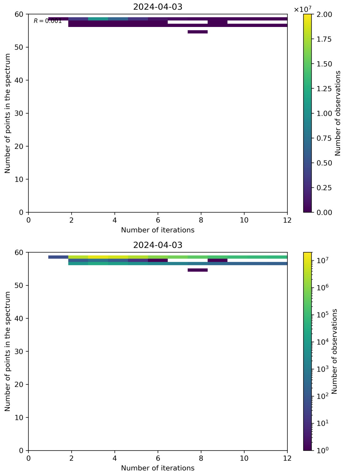
Figure 99: Scatter density plot of “Number of iterations” against “Number of points in the spectrum” for 2024-04-02 to 2024-04-04.
