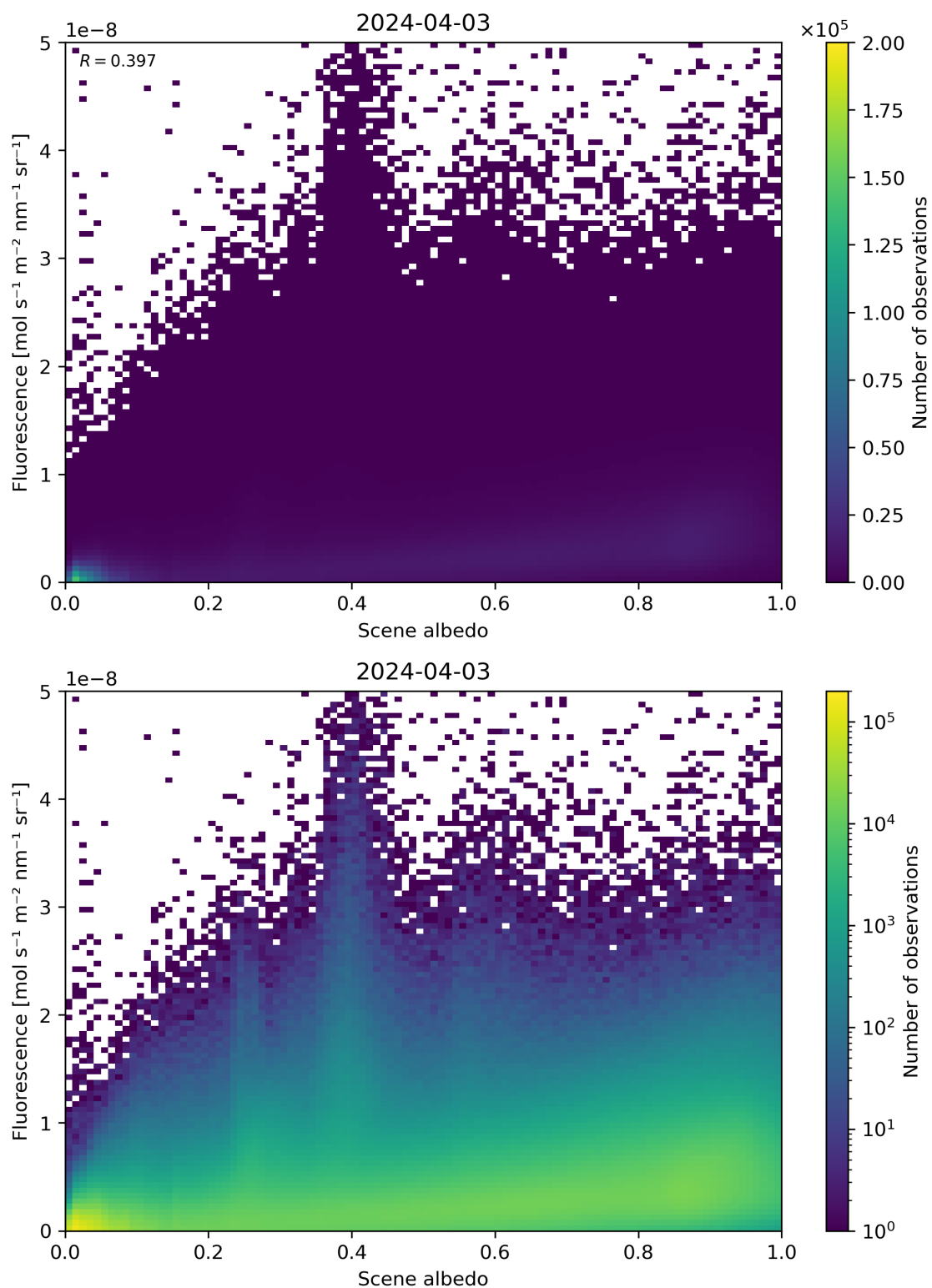
Figure 104: Scatter density plot of “Scene albedo” against “Fluorescence” for 2024-04-02 to 2024-04-04.
