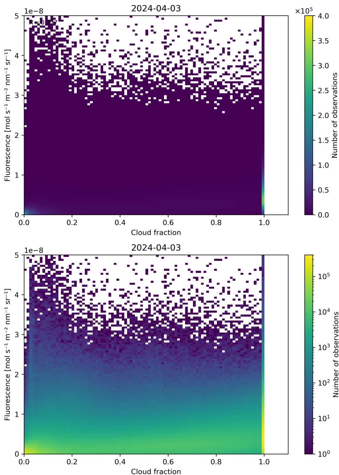
Figure 72: Scatter density plot of “Cloud fraction” against “Fluorescence” for 2024-04-02 to 2024-04-04.
