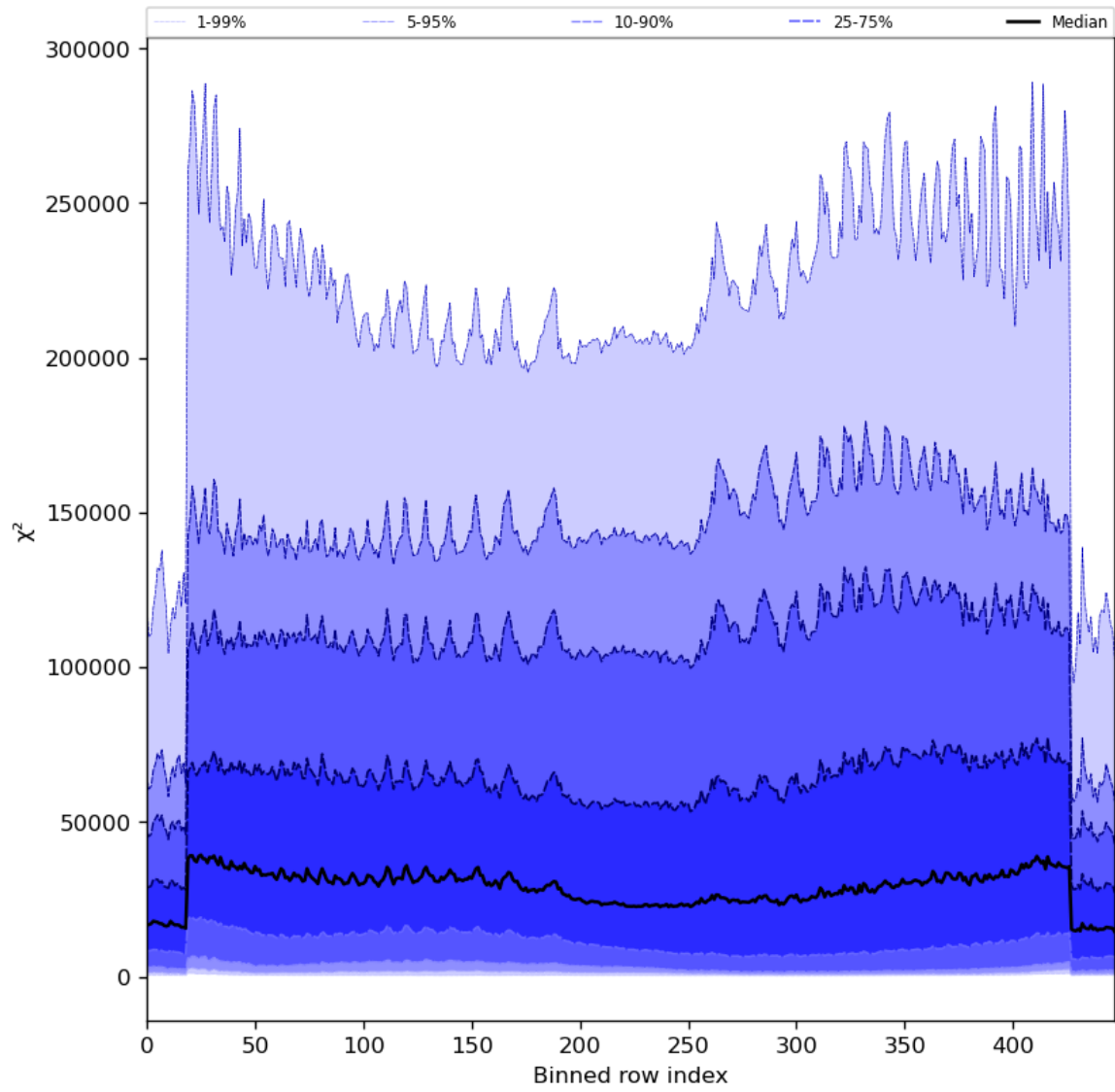
Figure 55: Along track statistics of “ \chi^2 ” for 2024-04-02 to 2024-04-04
