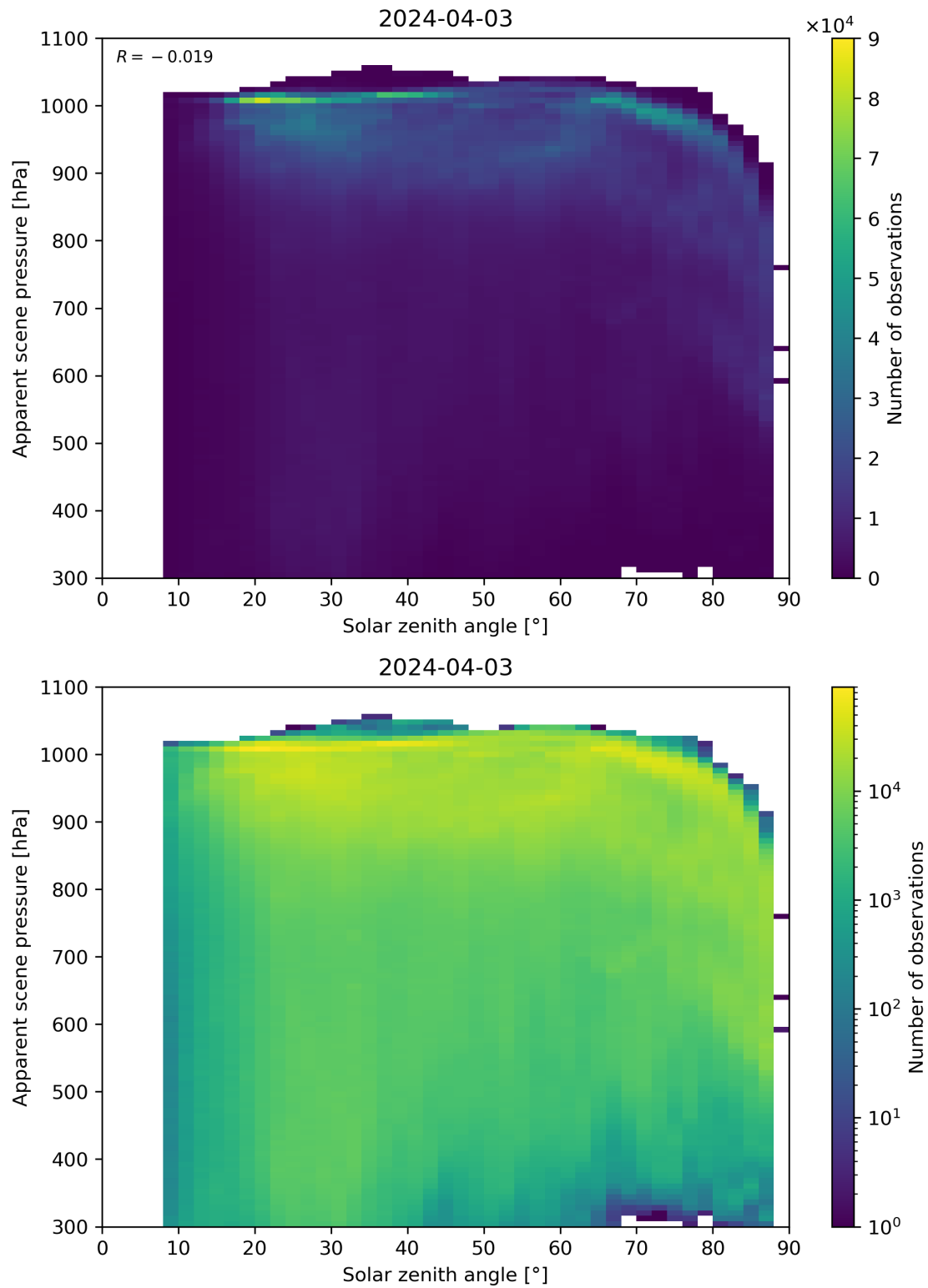
Figure 108: Scatter density plot of “Solar zenith angle” against “Apparent scene pressure” for 2024-04-02 to 2024-04-04.
