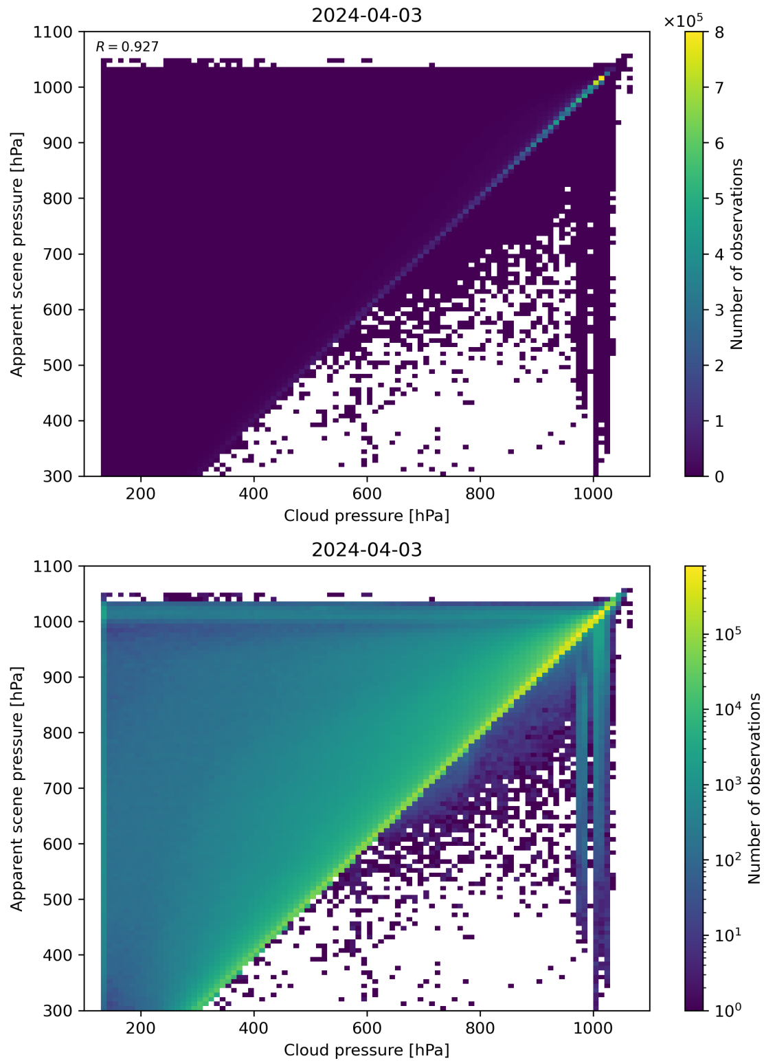
Figure 77: Scatter density plot of “Cloud pressure” against “Apparent scene pressure” for 2024-04-02 to 2024-04-04.
