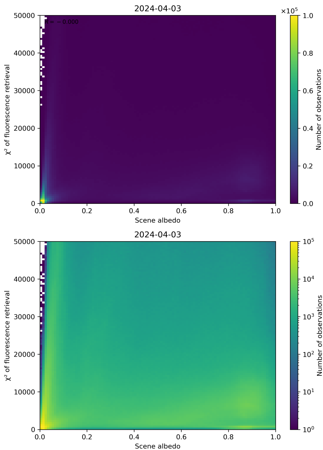
Figure 103: Scatter density plot of “Scene albedo” against “ \chi^2 of fluorescence retrieval” for 2024-04-02 to 2024-04-04.
