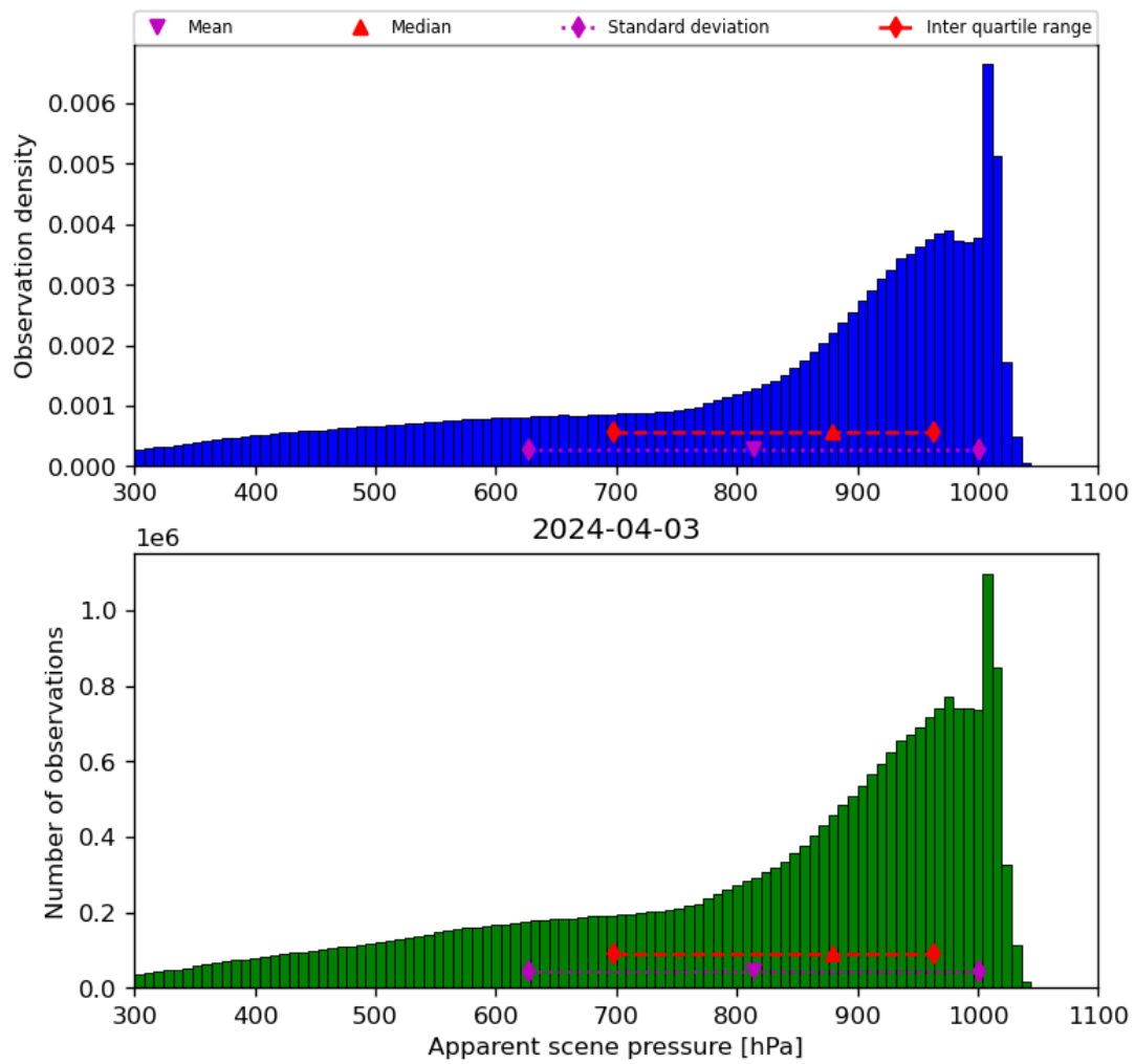
Figure 36: Histogram of “Apparent scene pressure” for 2024-04-02 to 2024-04-04
