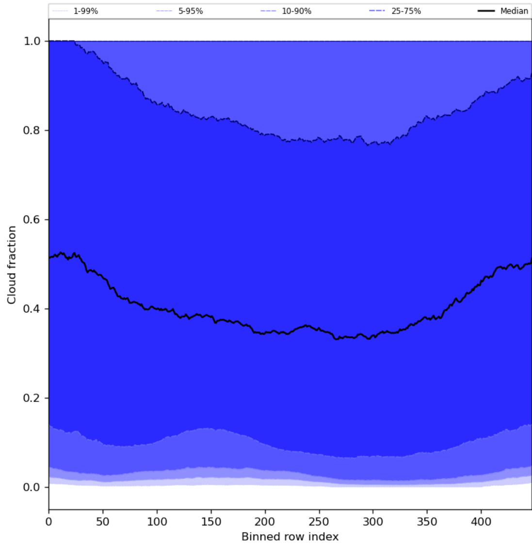
Figure 49: Along track statistics of “Cloud fraction” for 2024-04-02 to 2024-04-04
