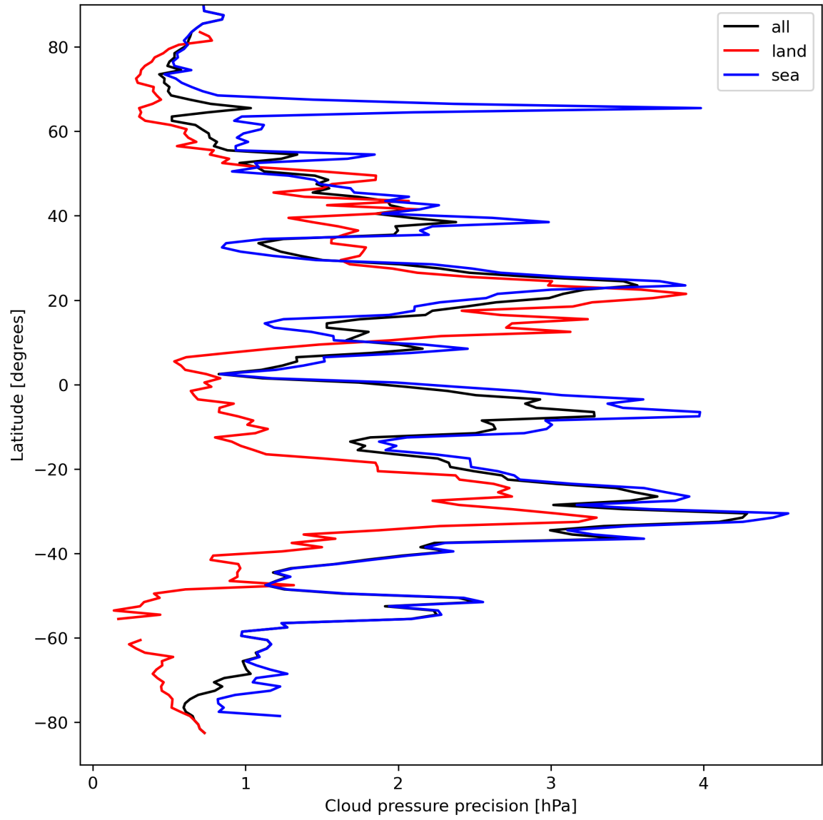
Figure 14: Zonal average of “Cloud pressure precision” for 2024-04-02 to 2024-04-04.
