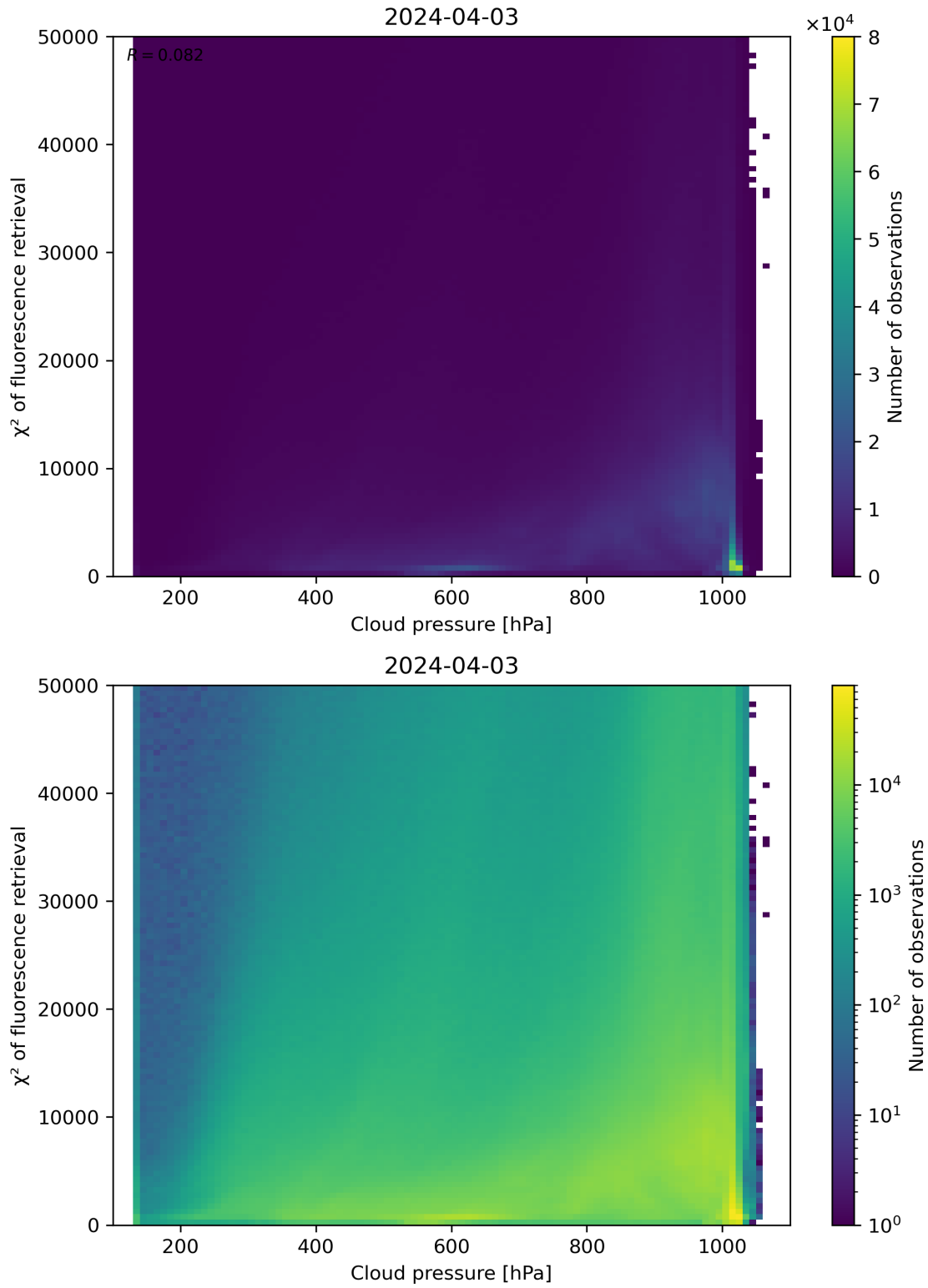
Figure 78: Scatter density plot of “Cloud pressure” against “ \chi^2 of fluorescence retrieval” for 2024-04-02 to 2024-04-04.
