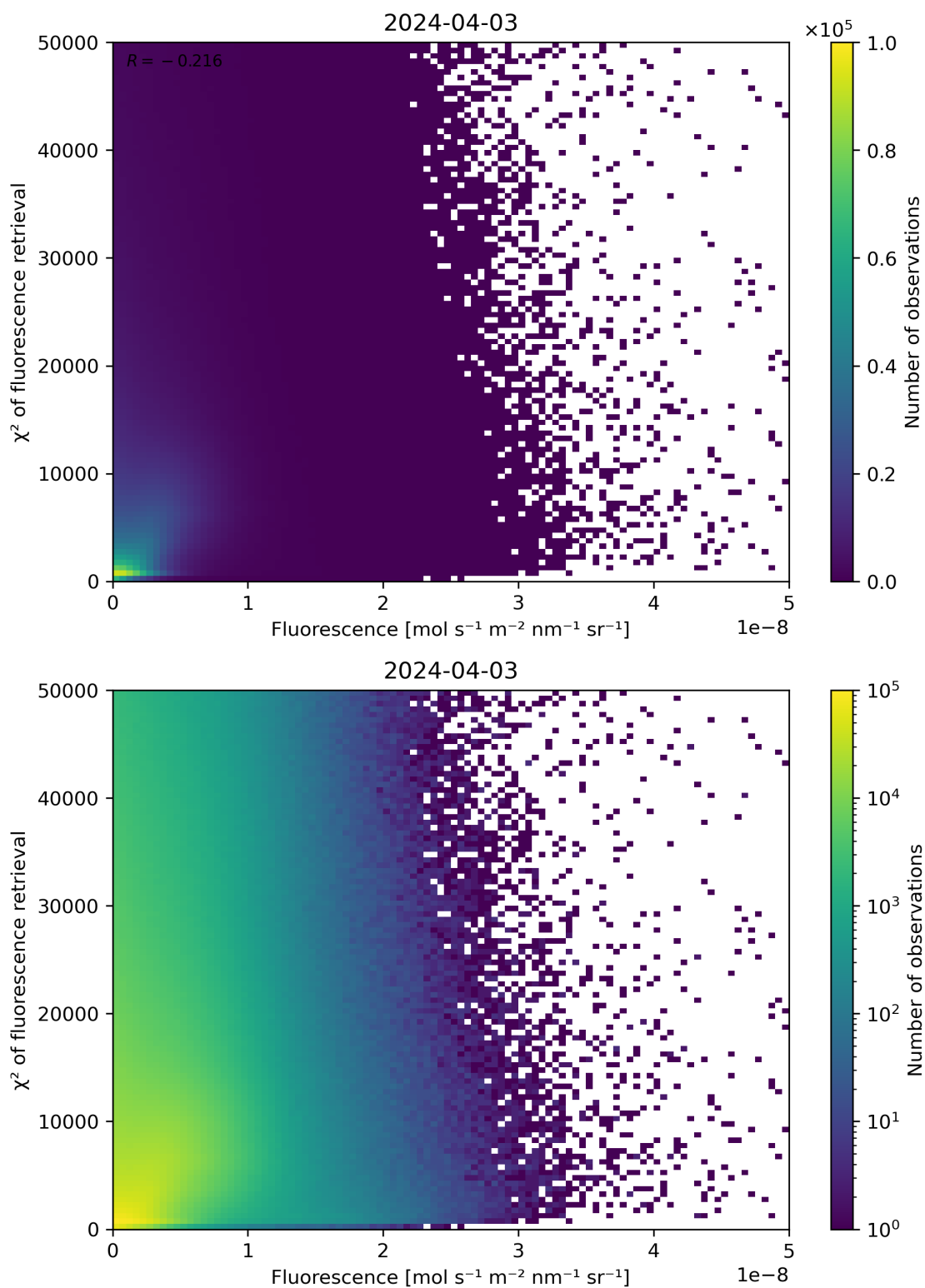
Figure 85: Scatter density plot of “Fluorescence” against “ \chi^2 of fluorescence retrieval” for 2024-04-02 to 2024-04-04.
