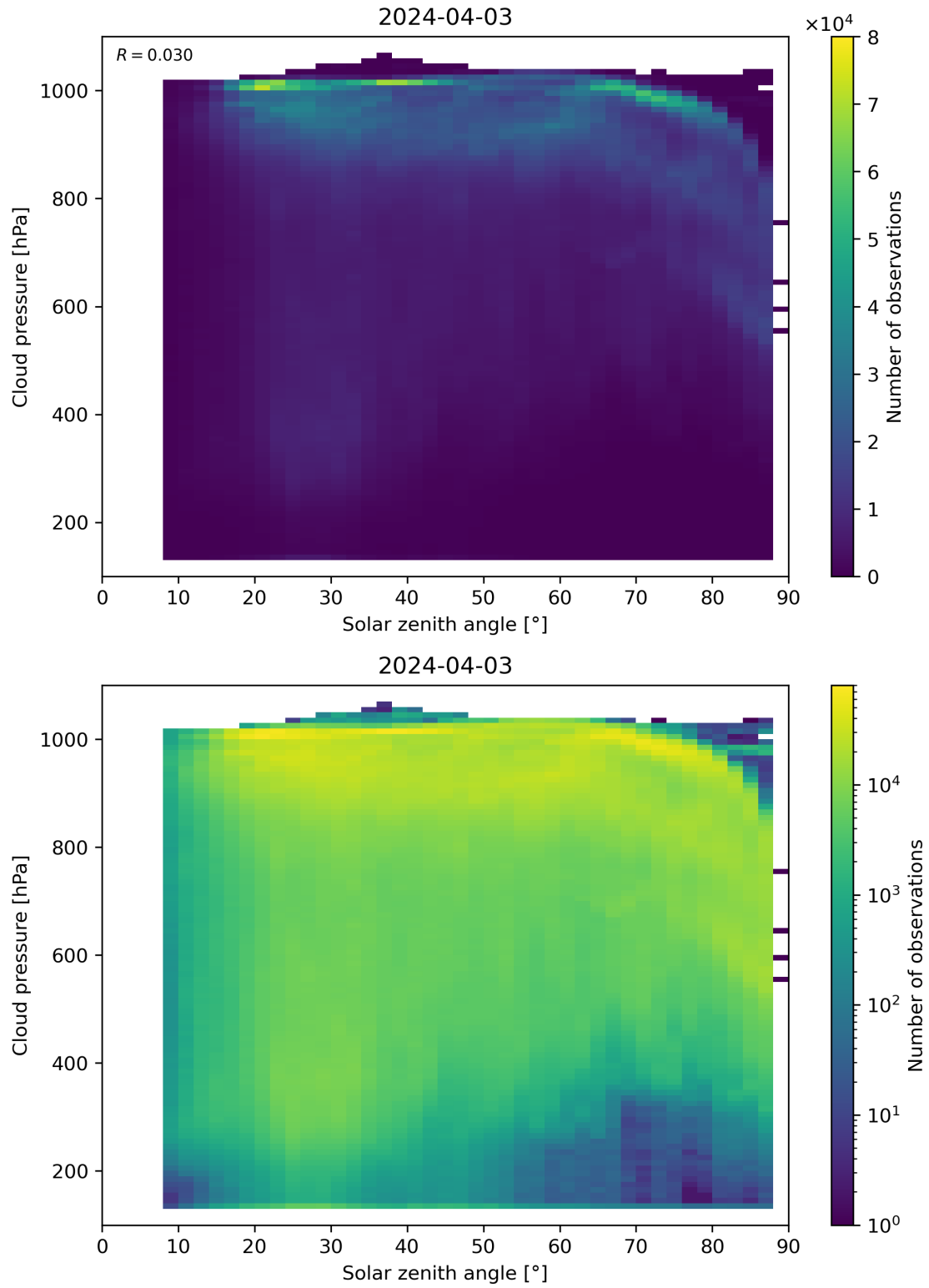
Figure 111: Scatter density plot of “Solar zenith angle” against “Cloud pressure” for 2024-04-02 to 2024-04-04.
