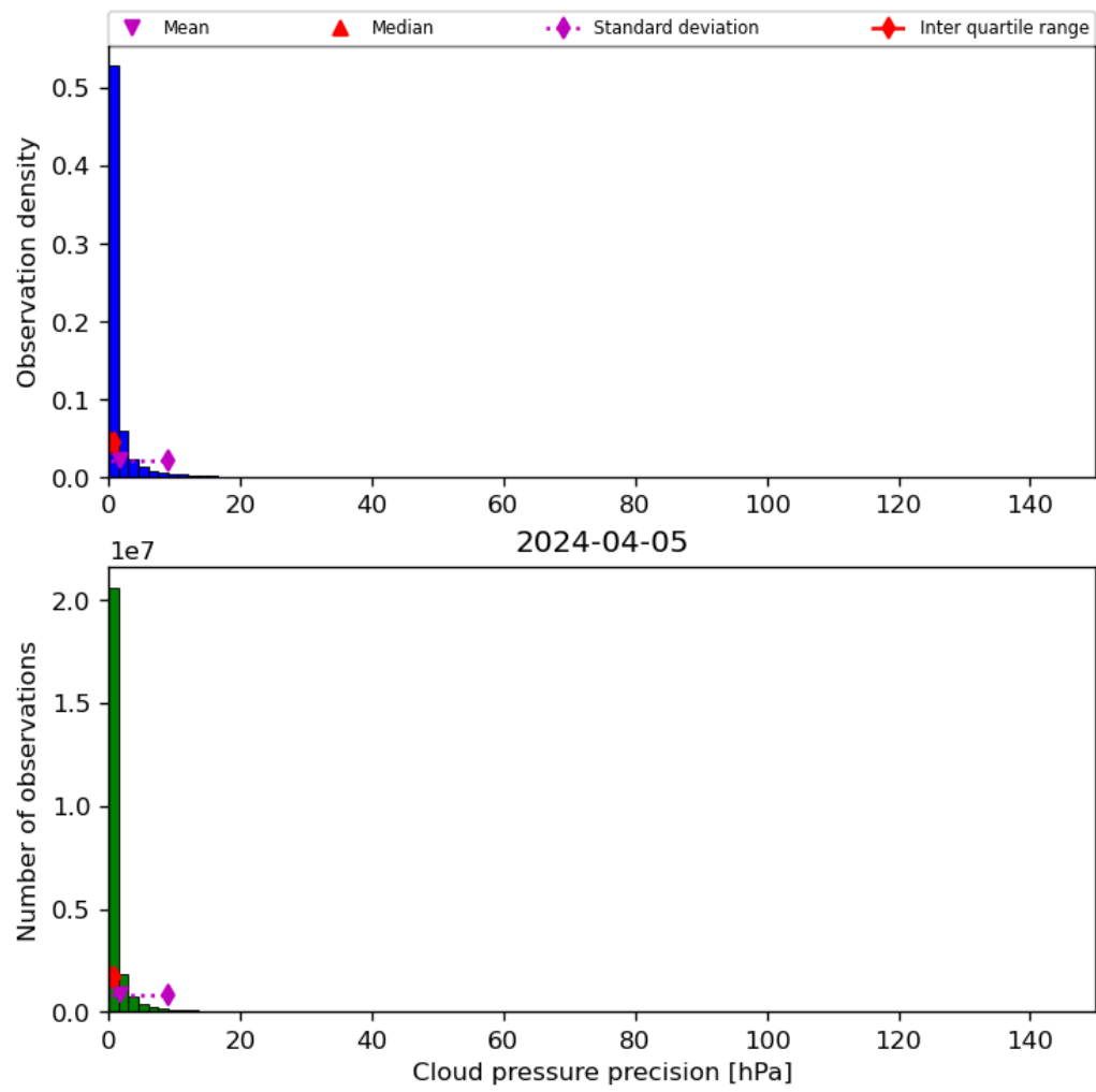
Figure 31: Histogram of “Cloud pressure precision” for 2024-04-05 to 2024-04-06
