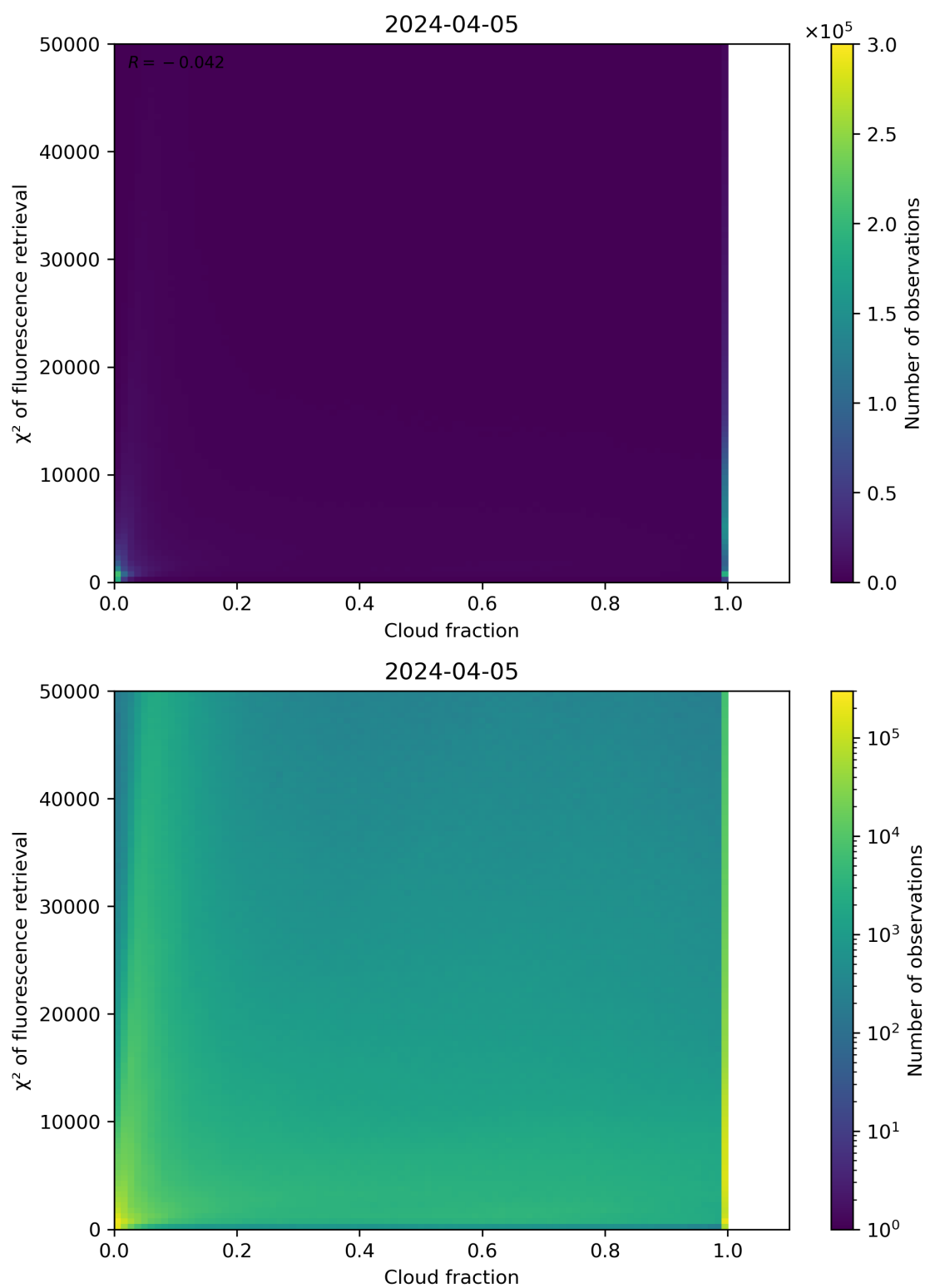
Figure 71: Scatter density plot of “Cloud fraction” against “ \chi^2 of fluorescence retrieval” for 2024-04-05 to 2024-04-06.
