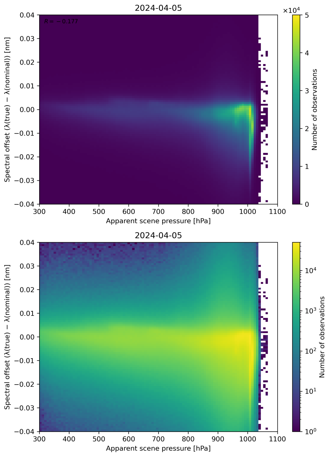
Figure 67: Scatter density plot of “Apparent scene pressure” against “Spectral offset ( \lambda(\text{true}) - \lambda(\text{nominal}) )” for 2024-04-05 to 2024-04-06.
