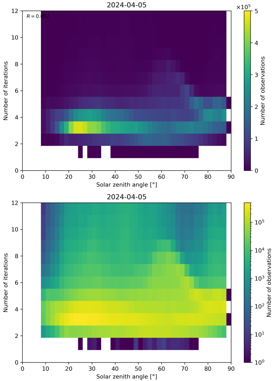
Figure 114: Scatter density plot of “Solar zenith angle” against “Number of iterations” for 2024-04-05 to 2024-04-06.
