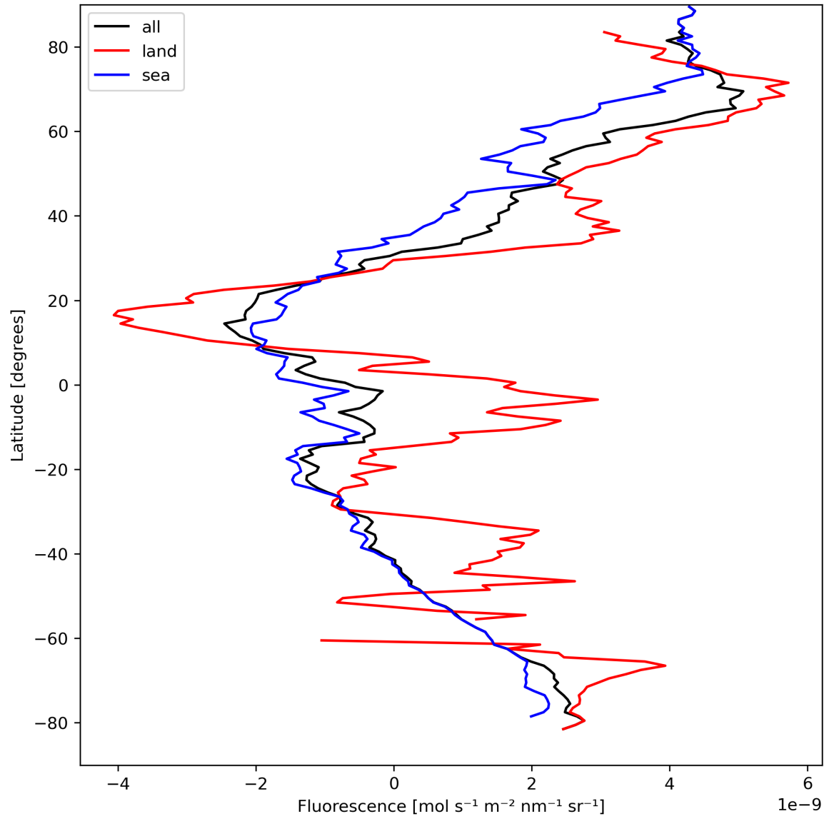
Figure 23: Zonal average of “Fluorescence” for 2024-04-05 to 2024-04-06.
