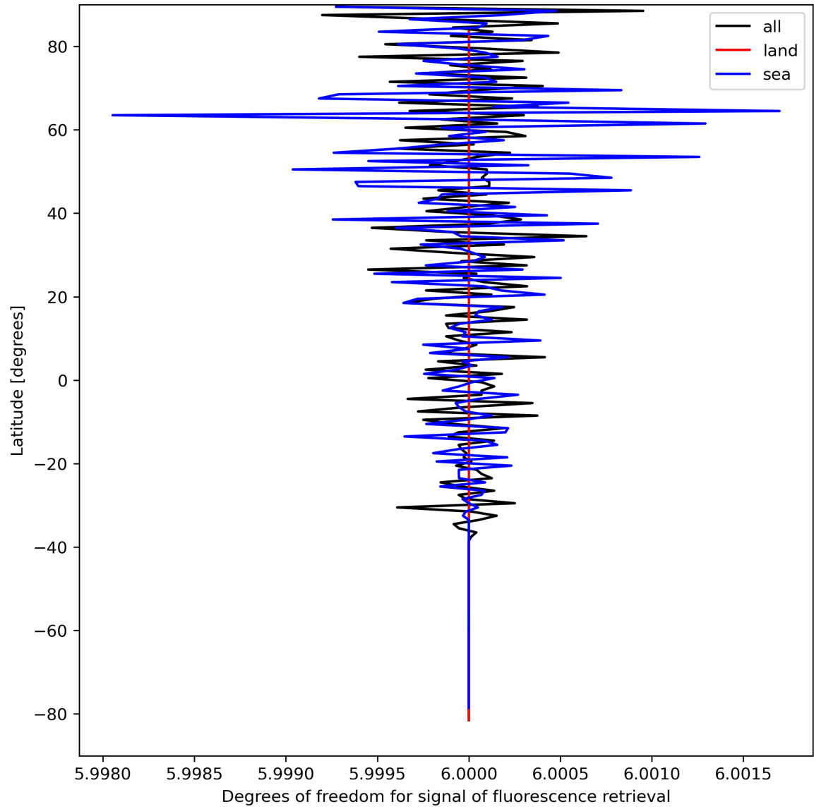
Figure 26: Zonal average of “Degrees of freedom for signal of fluorescence retrieval” for 2024-04-05 to 2024-04-06.
