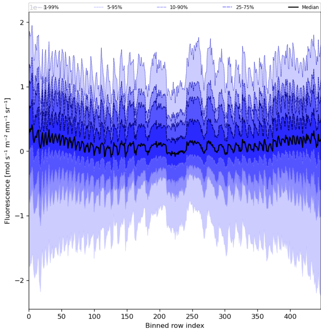
Figure 57: Along track statistics of “Fluorescence” for 2024-04-05 to 2024-04-06
