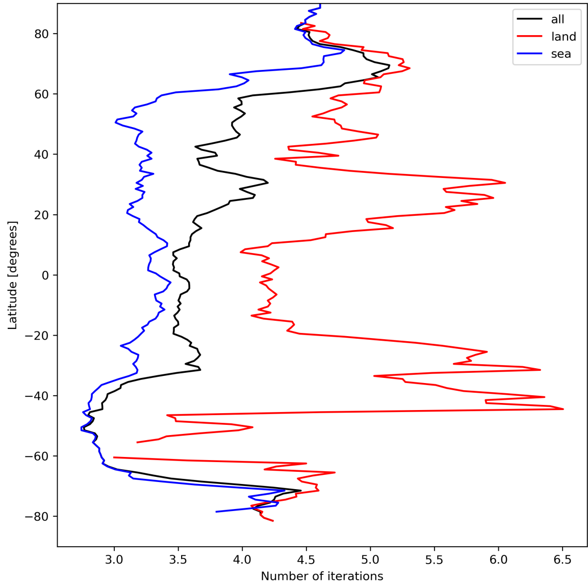
Figure 22: Zonal average of “Number of iterations” for 2024-04-05 to 2024-04-06.
