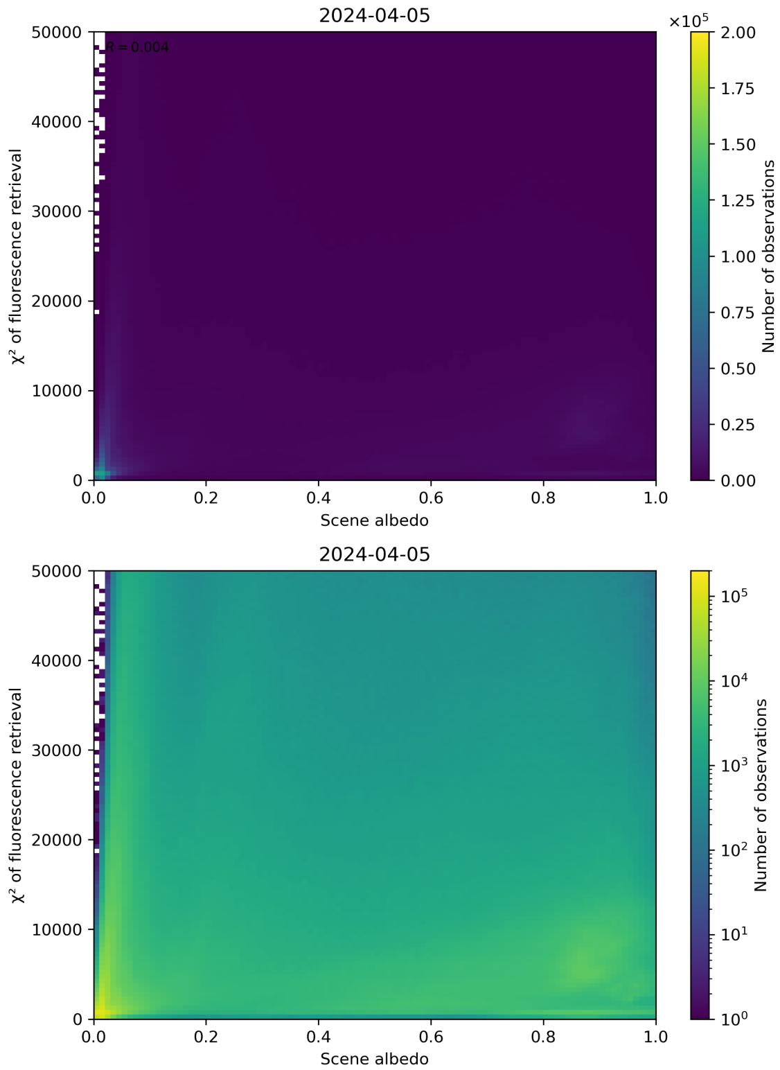
Figure 103: Scatter density plot of “Scene albedo” against “ \chi^2 of fluorescence retrieval” for 2024-04-05 to 2024-04-06.
