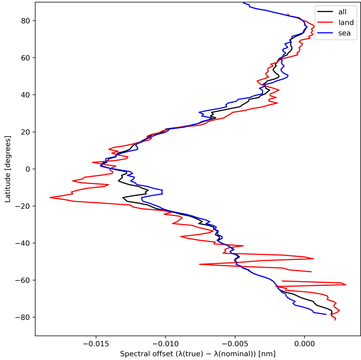
Figure 28: Zonal average of “Spectral offset ( \lambda(\text{true}) - \lambda(\text{nominal}) )” for 2024-04-05 to 2024-04-06.
