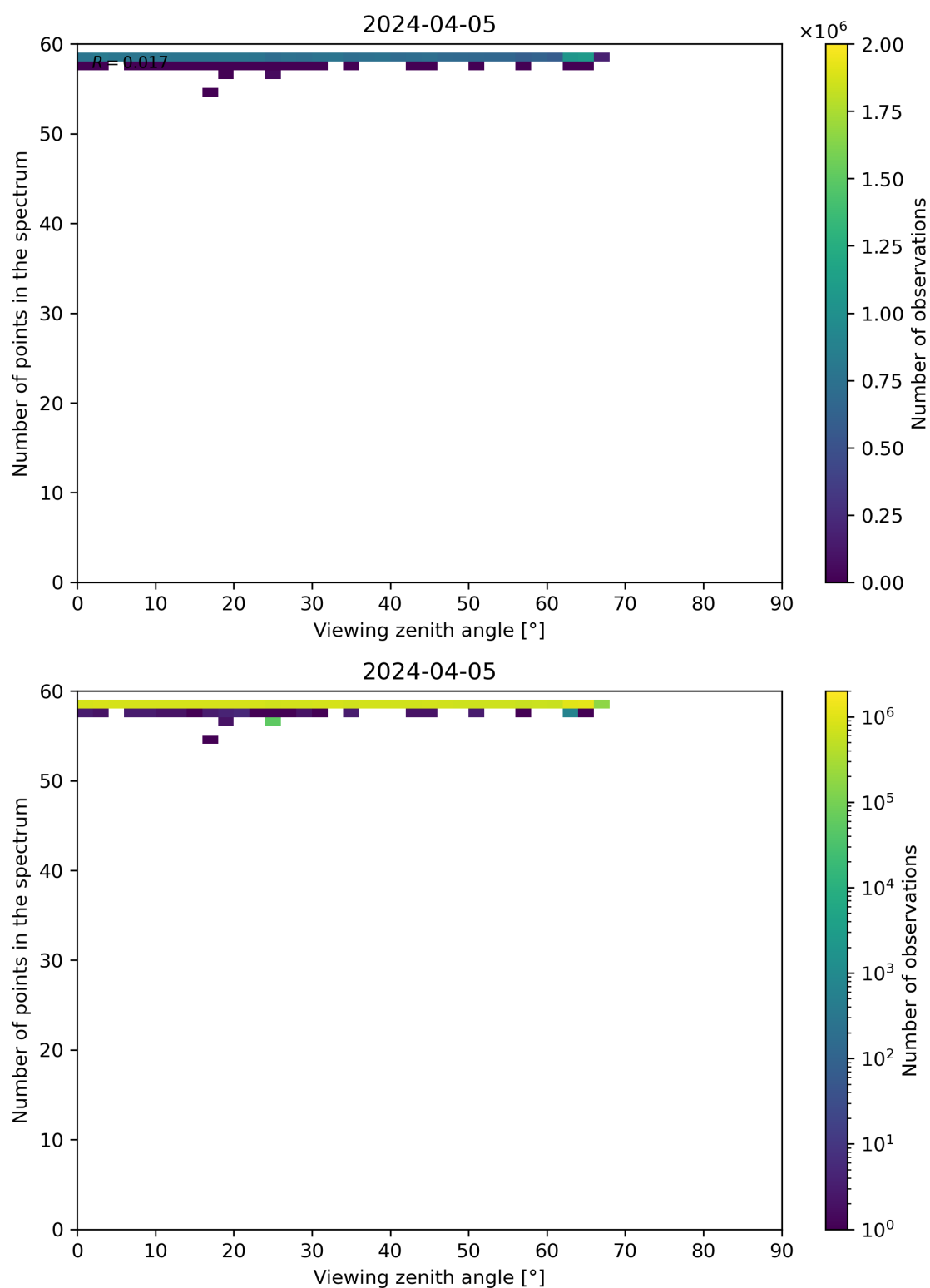
Figure 125: Scatter density plot of “Viewing zenith angle” against “Number of points in the spectrum” for 2024-04-05 to 2024-04-06.
