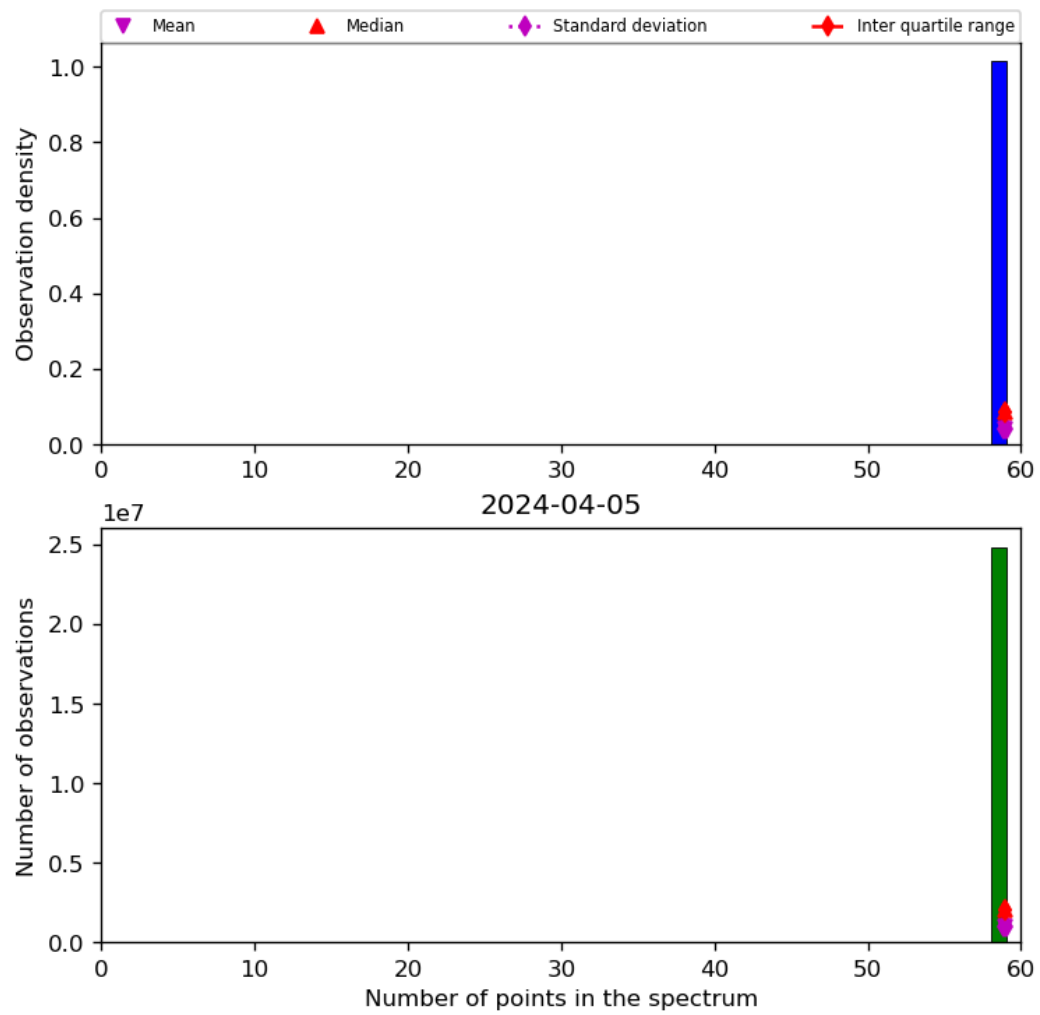
Figure 44: Histogram of “Number of points in the spectrum” for 2024-04-05 to 2024-04-06
