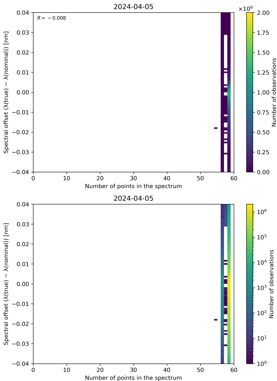
Figure 101: Scatter density plot of “Number of points in the spectrum” against “Spectral offset ( \lambda(\text{true}) - \lambda(\text{nominal}) )” for 2024-04-05 to 2024-04-06.
