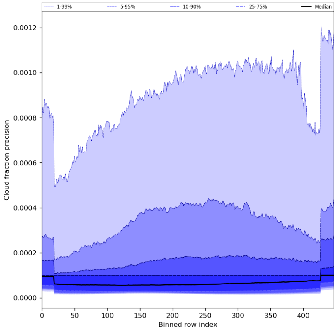
Figure 50: Along track statistics of “Cloud fraction precision” for 2024-04-05 to 2024-04-06
