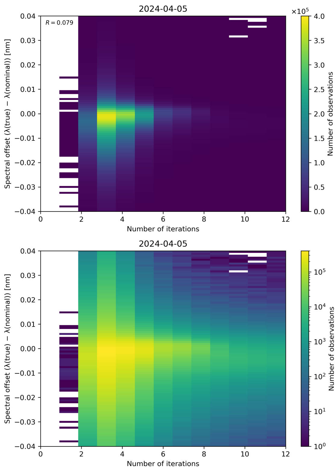
Figure 100: Scatter density plot of “Number of iterations” against “Spectral offset ( \lambda(\text{true}) - \lambda(\text{nominal}) )” for 2024-04-05 to 2024-04-06.
