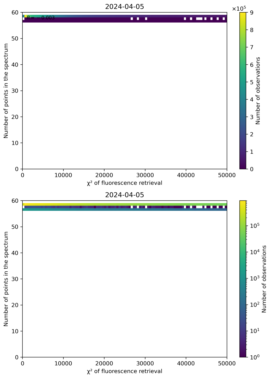
Figure 68: Scatter density plot of " \chi^2 of fluorescence retrieval" against "Number of points in the spectrum" for 2024-04-05 to 2024-04-06.
