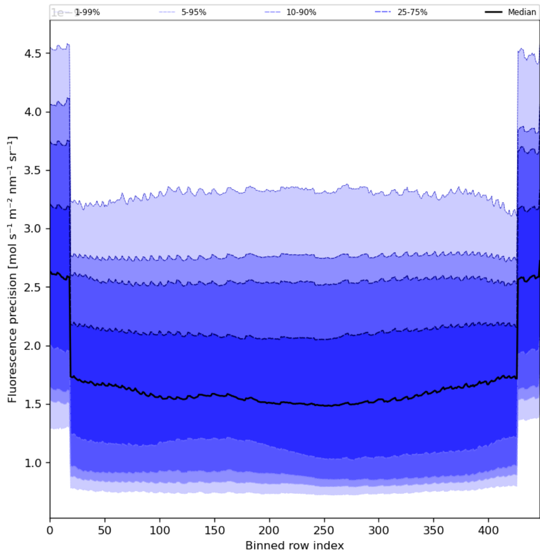
Figure 58: Along track statistics of “Fluorescence precision” for 2024-04-05 to 2024-04-06
