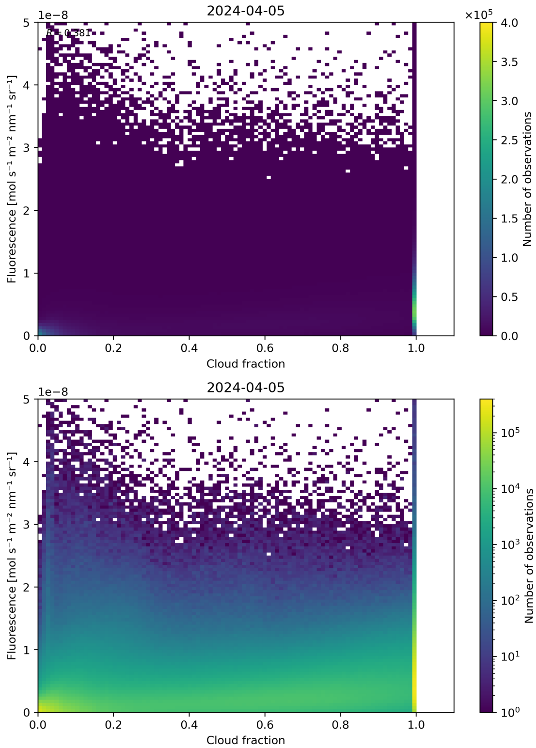
Figure 72: Scatter density plot of “Cloud fraction” against “Fluorescence” for 2024-04-05 to 2024-04-06.
