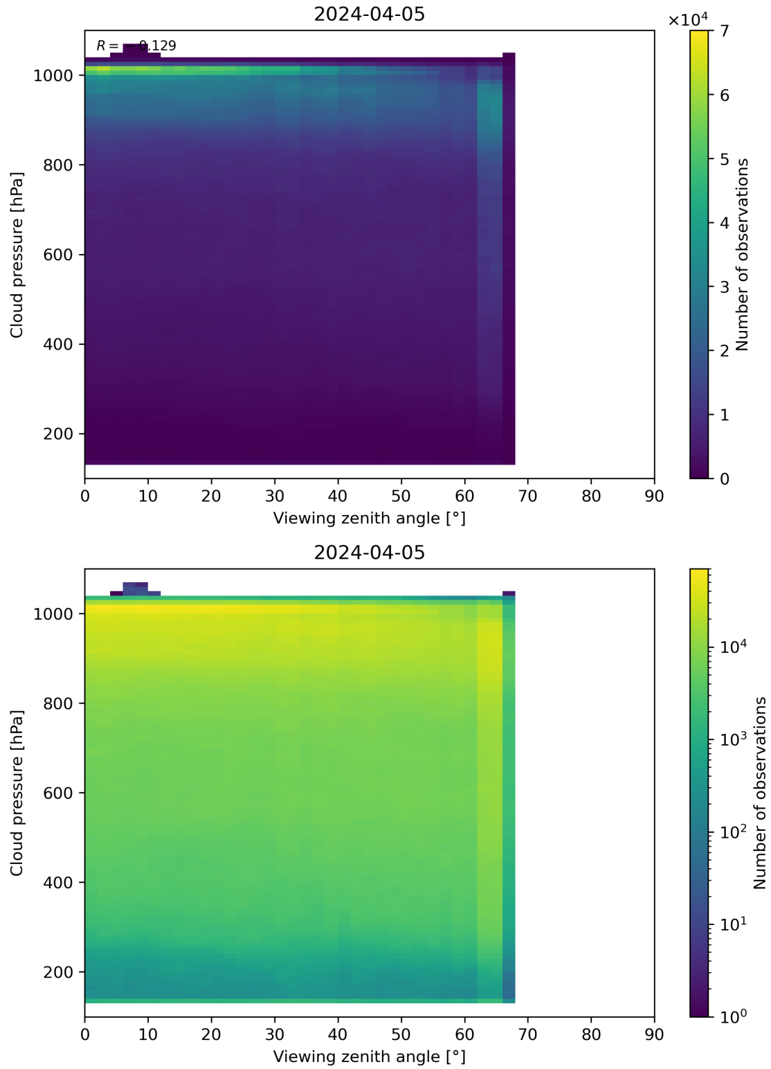
Figure 121: Scatter density plot of “Viewing zenith angle” against “Cloud pressure” for 2024-04-05 to 2024-04-06.
