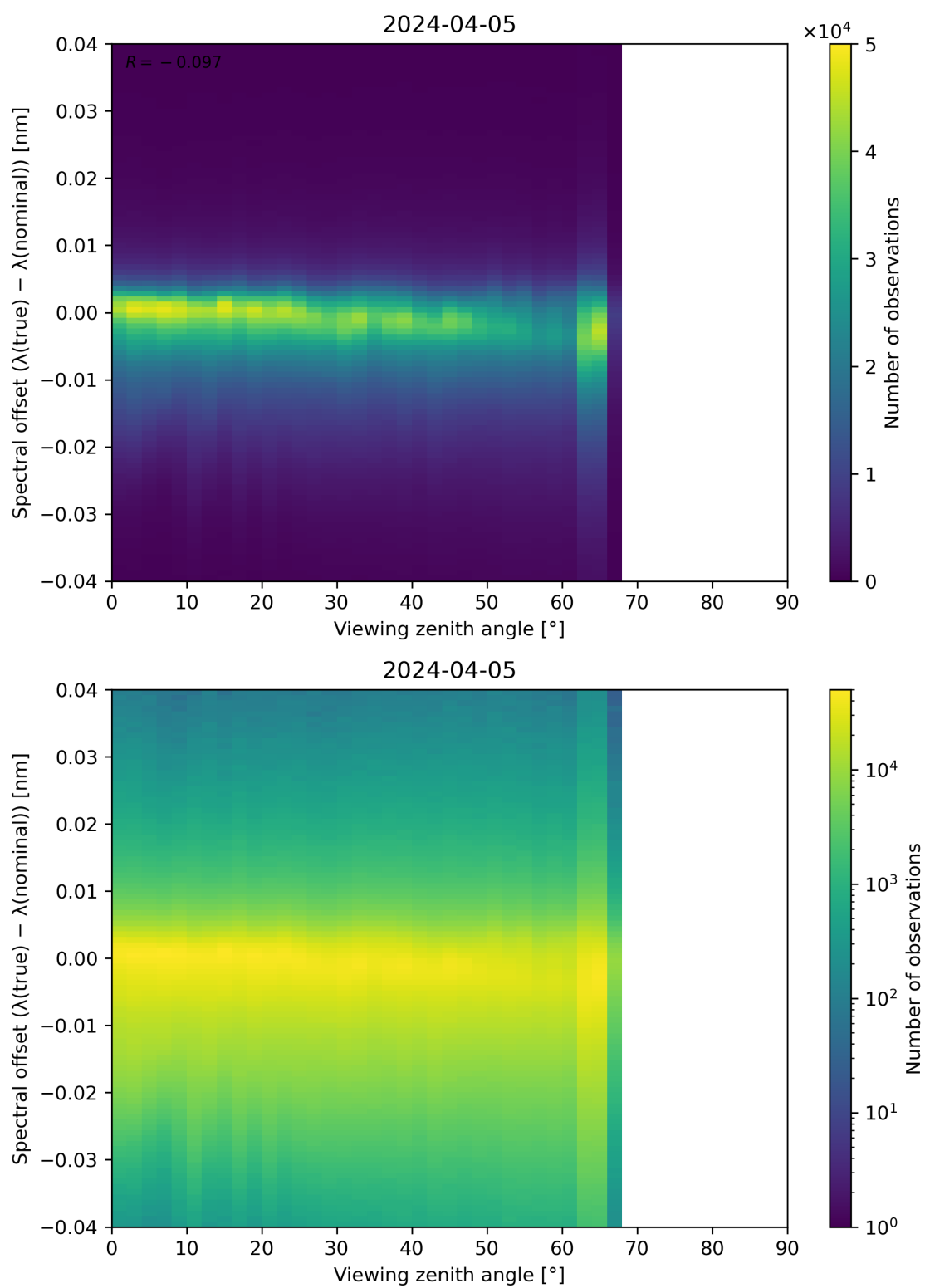
Figure 128: Scatter density plot of “Viewing zenith angle” against “Spectral offset ( \lambda(\text{true}) - \lambda(\text{nominal}) )” for 2024-04-05 to 2024-04-06.
