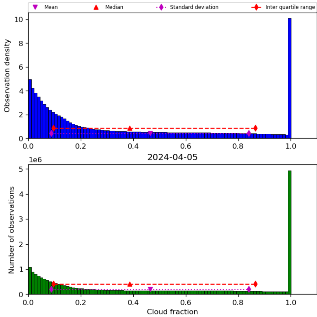
Figure 32: Histogram of “Cloud fraction” for 2024-04-05 to 2024-04-06
