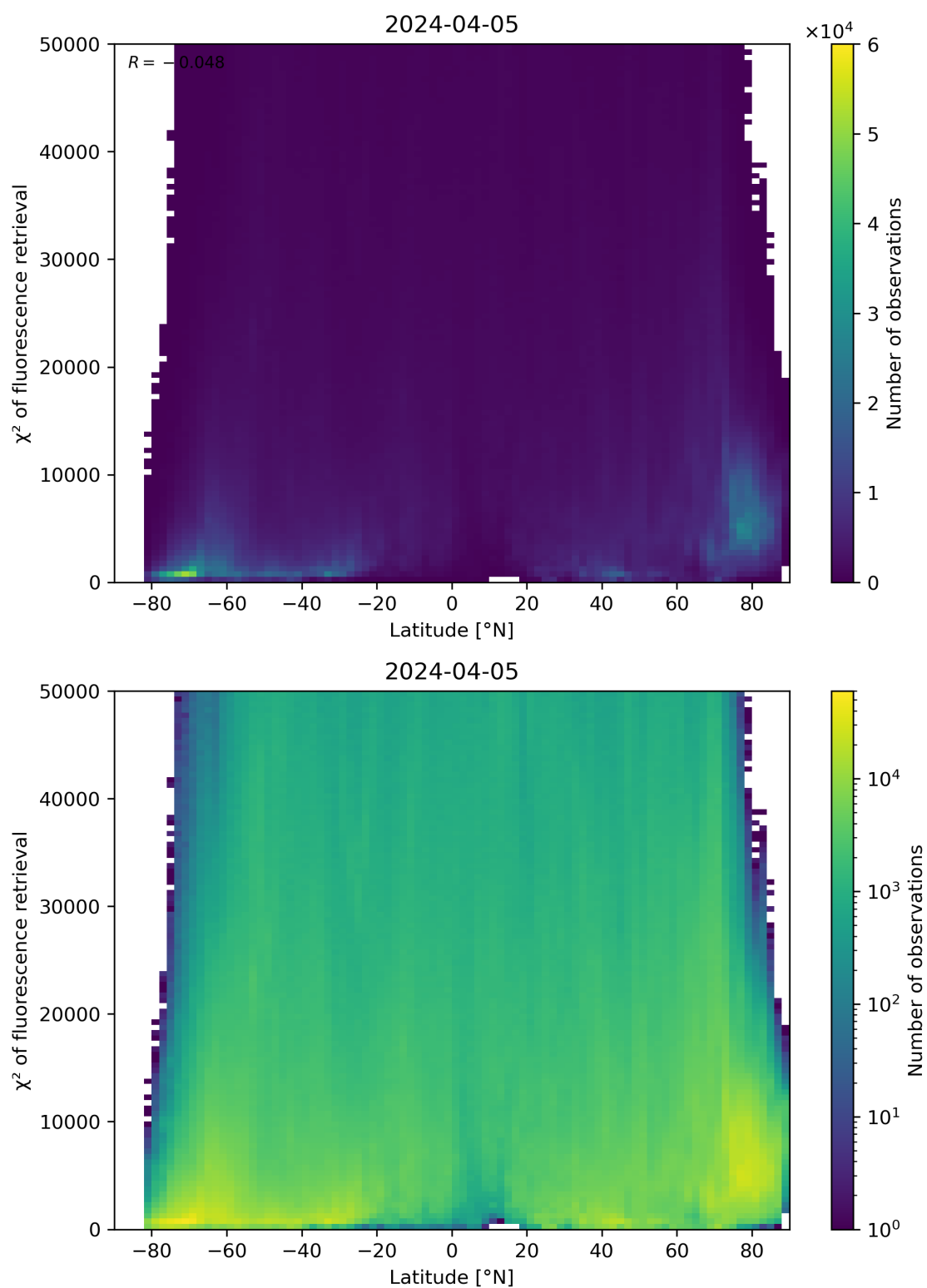
Figure 89: Scatter density plot of “Latitude” against “ \chi^2 of fluorescence retrieval” for 2024-04-05 to 2024-04-06.
