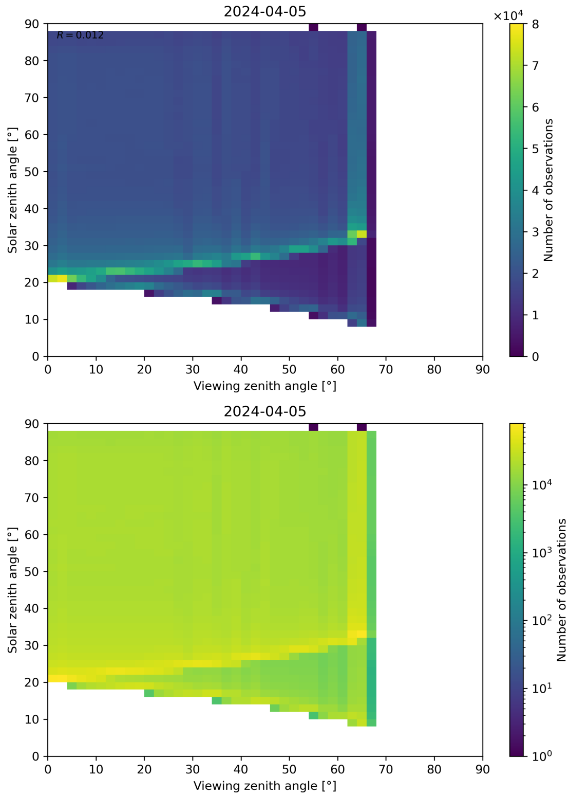
Figure 127: Scatter density plot of “Viewing zenith angle” against “Solar zenith angle” for 2024-04-05 to 2024-04-06.
