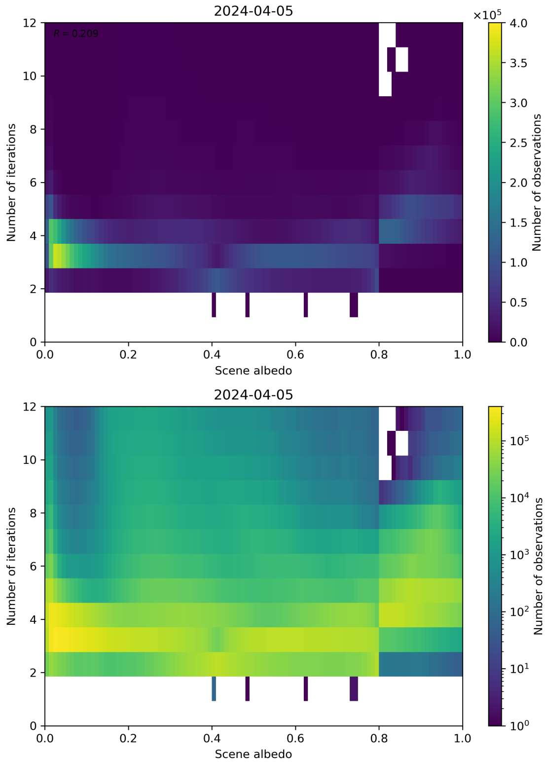
Figure 105: Scatter density plot of “Scene albedo” against “Number of iterations” for 2024-04-05 to 2024-04-06.
