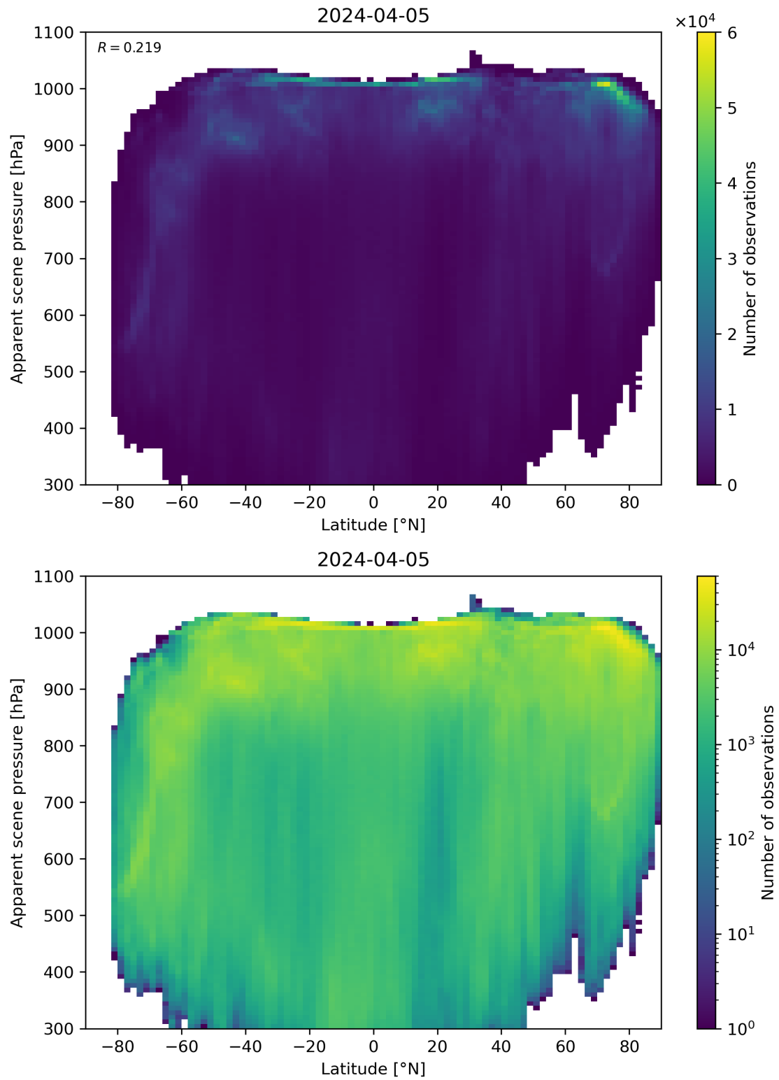
Figure 88: Scatter density plot of “Latitude” against “Apparent scene pressure” for 2024-04-05 to 2024-04-06.
