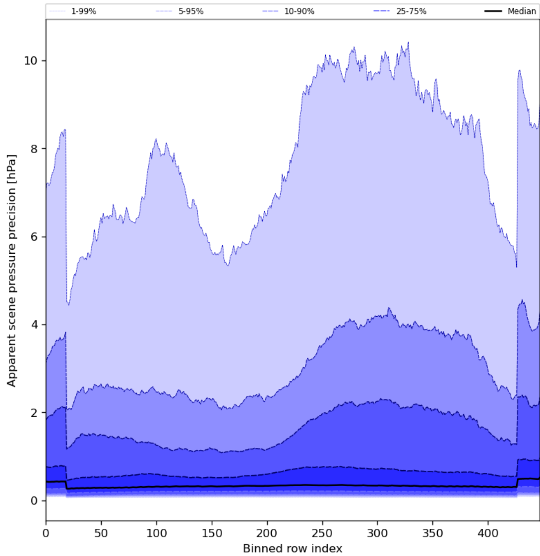
Figure 54: Along track statistics of “Apparent scene pressure precision” for 2024-04-05 to 2024-04-06
