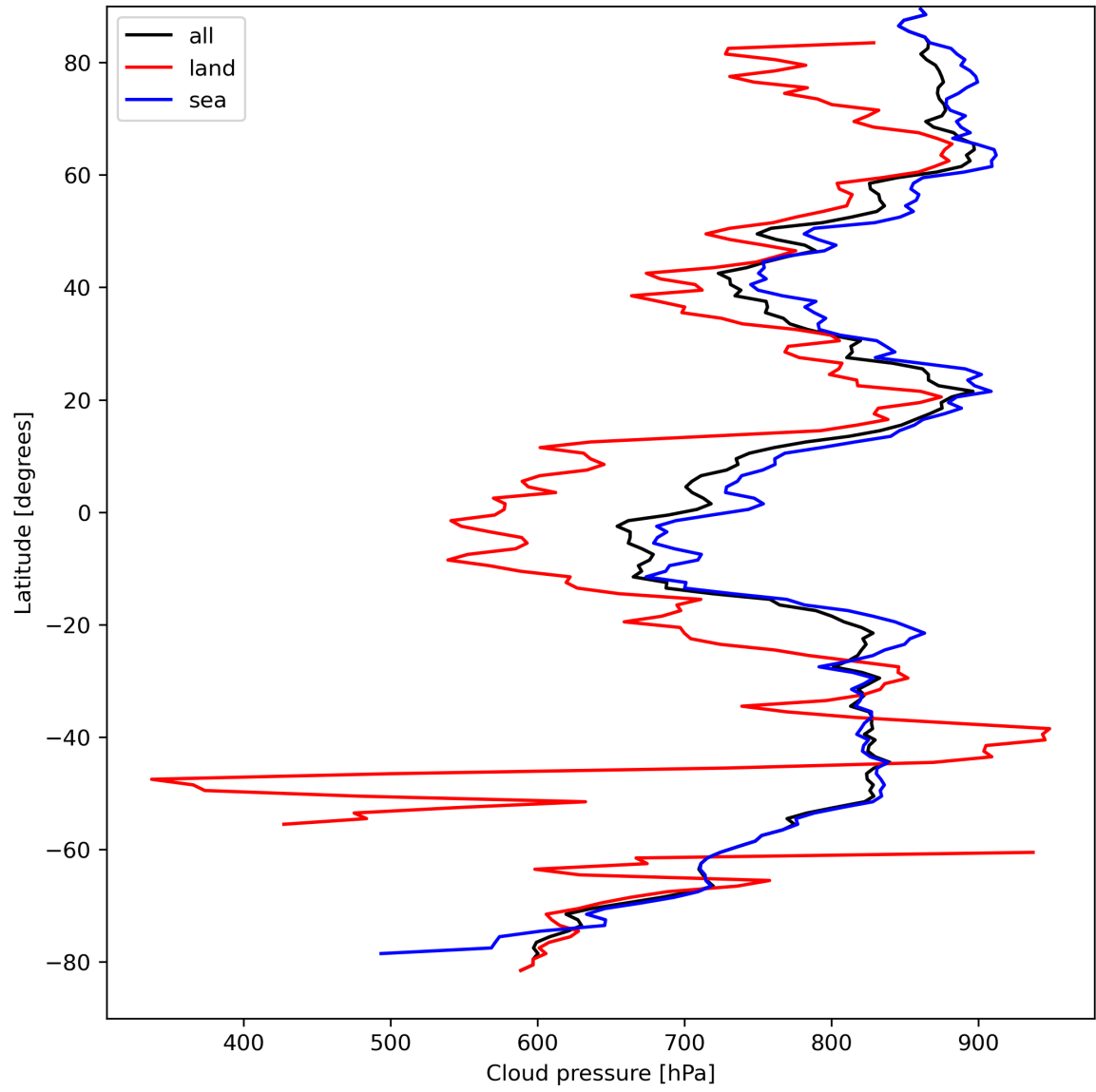
Figure 13: Zonal average of “Cloud pressure” for 2024-04-05 to 2024-04-06.
