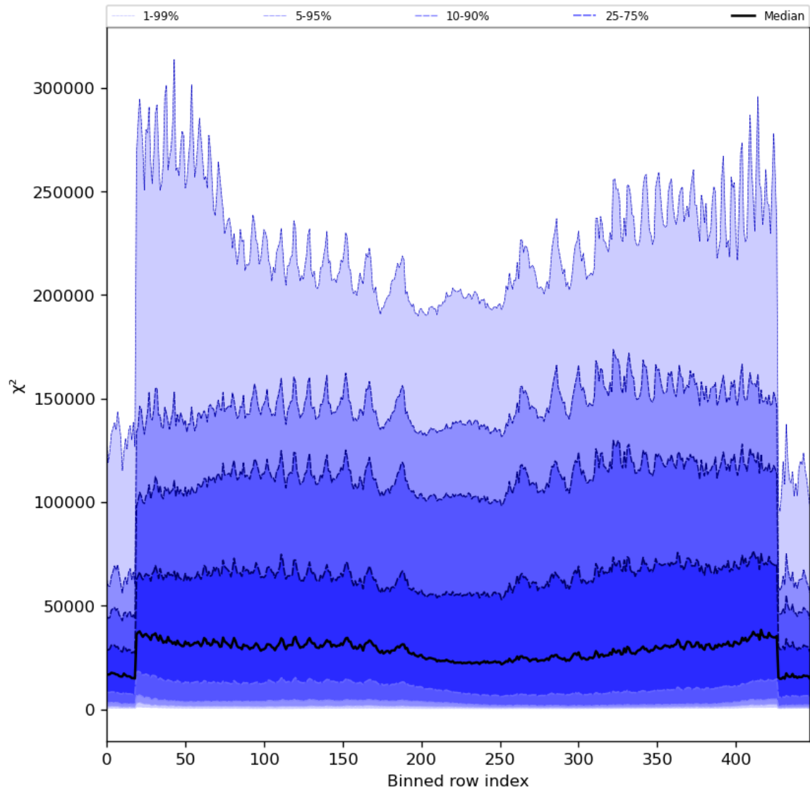
Figure 55: Along track statistics of “ \chi^2 ” for 2024-04-05 to 2024-04-06
