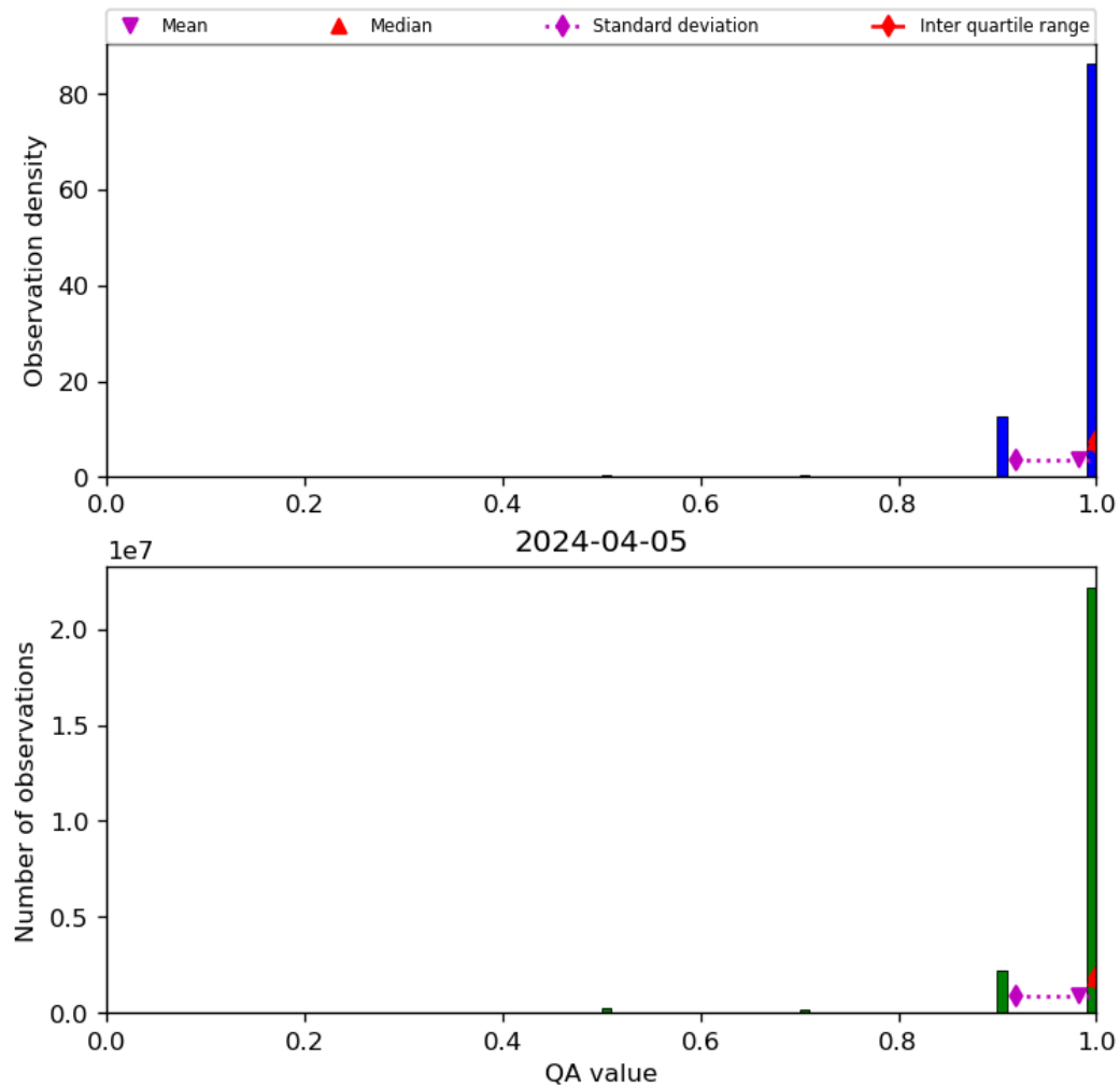
Figure 29: Histogram of “QA value” for 2024-04-05 to 2024-04-06
