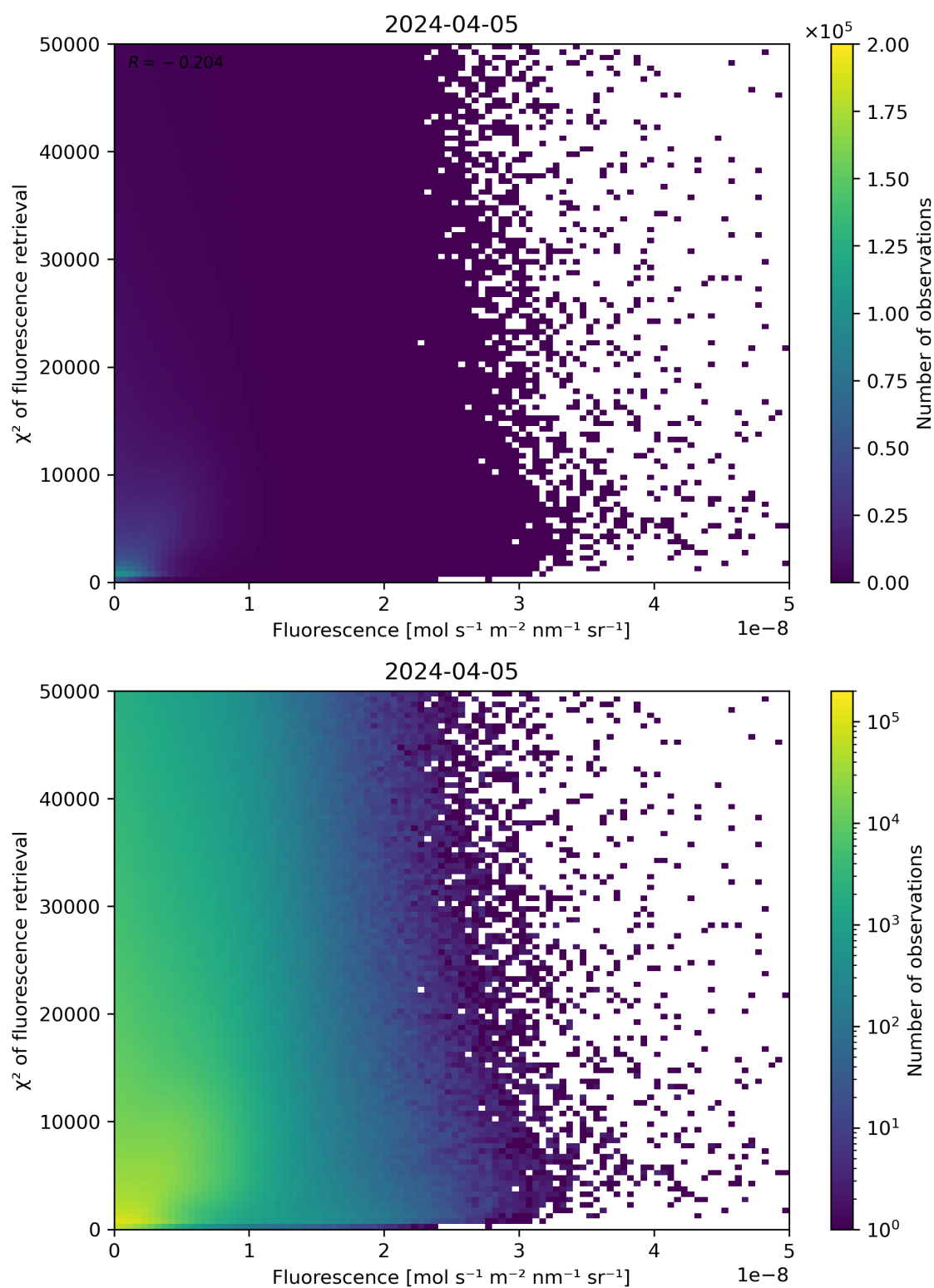
Figure 85: Scatter density plot of “Fluorescence” against “ \chi^2 of fluorescence retrieval” for 2024-04-05 to 2024-04-06.
