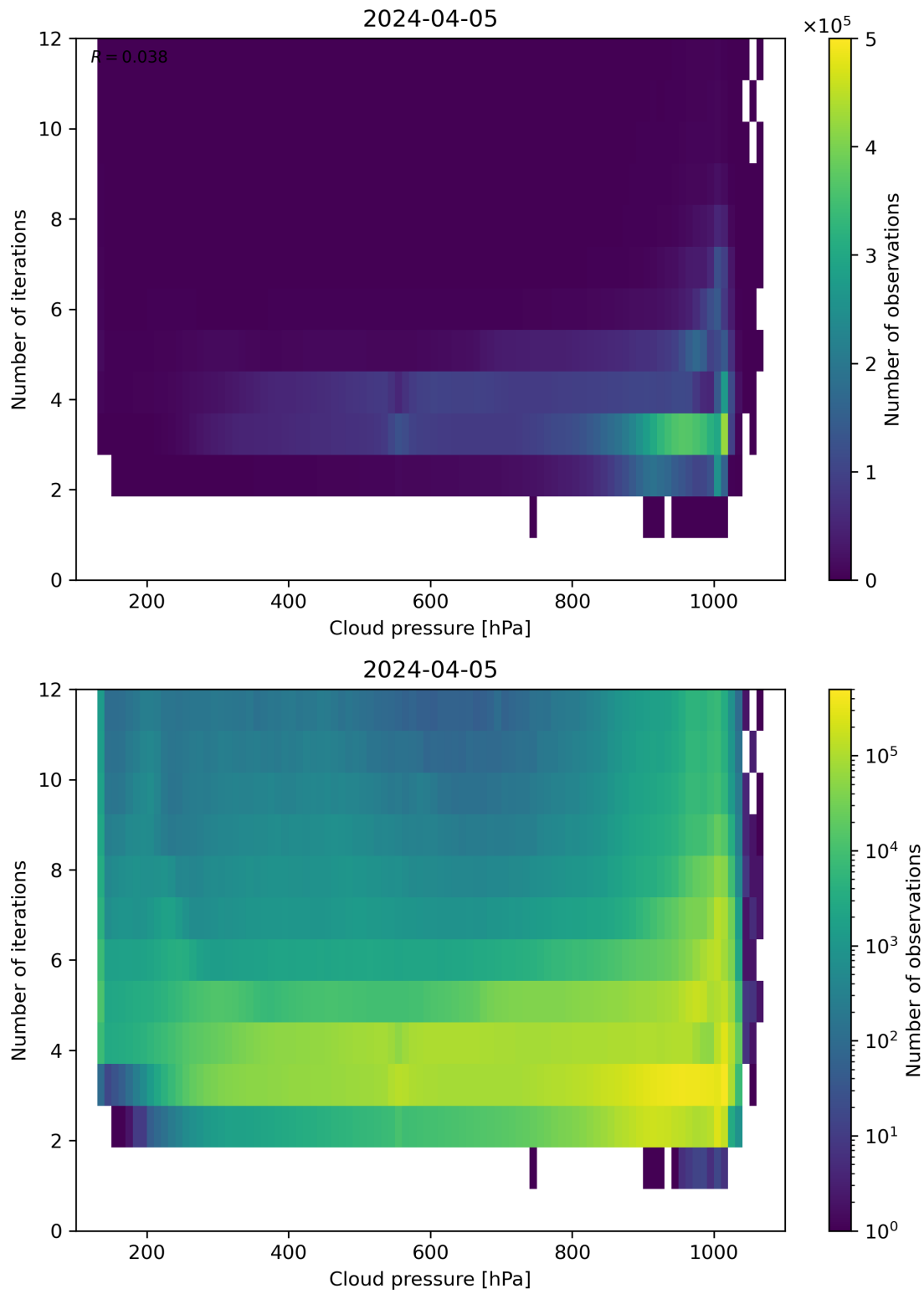
Figure 81: Scatter density plot of “Cloud pressure” against “Number of iterations” for 2024-04-05 to 2024-04-06.
