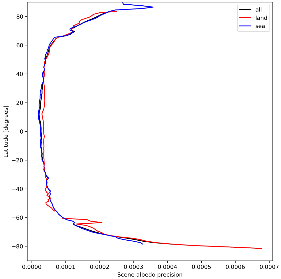
Figure 18: Zonal average of “Scene albedo precision” for 2024-04-05 to 2024-04-06.
