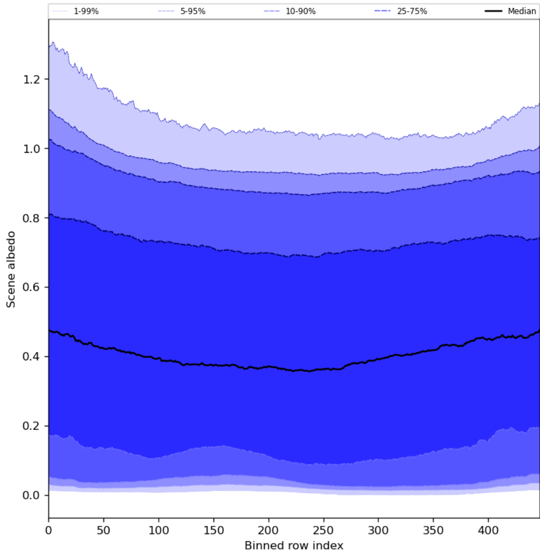
Figure 51: Along track statistics of “Scene albedo” for 2024-04-05 to 2024-04-06
