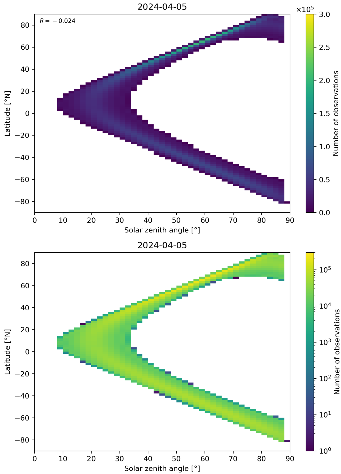
Figure 113: Scatter density plot of “Solar zenith angle” against “Latitude” for 2024-04-05 to 2024-04-06.
