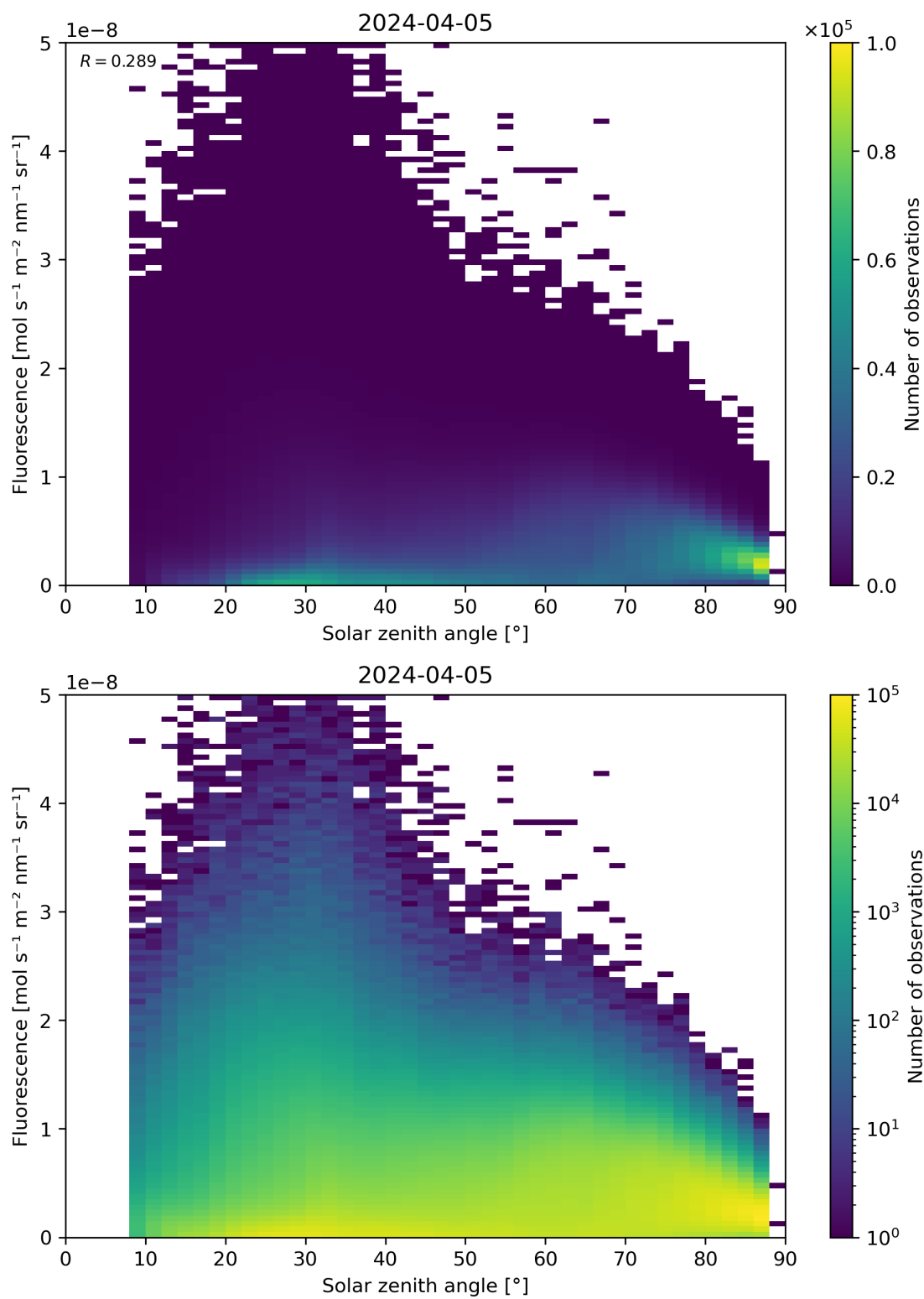
Figure 112: Scatter density plot of “Solar zenith angle” against “Fluorescence” for 2024-04-05 to 2024-04-06.
