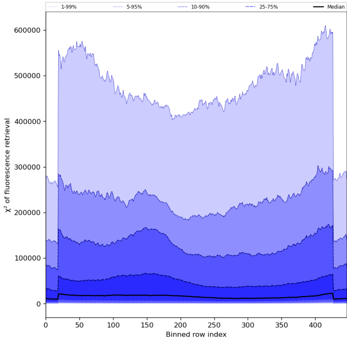
Figure 59: Along track statistics of “ \chi^2 of fluorescence retrieval” for 2024-04-05 to 2024-04-06
