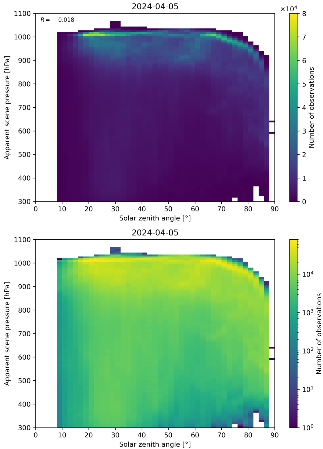
Figure 108: Scatter density plot of “Solar zenith angle” against “Apparent scene pressure” for 2024-04-05 to 2024-04-06.
