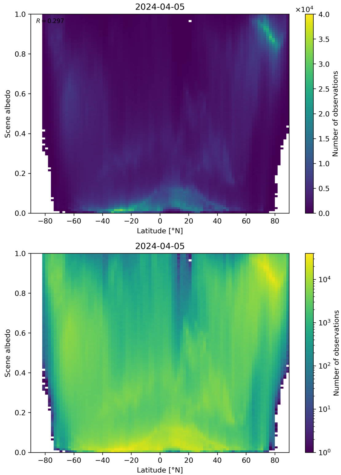
Figure 95: Scatter density plot of “Latitude” against “Scene albedo” for 2024-04-05 to 2024-04-06.
