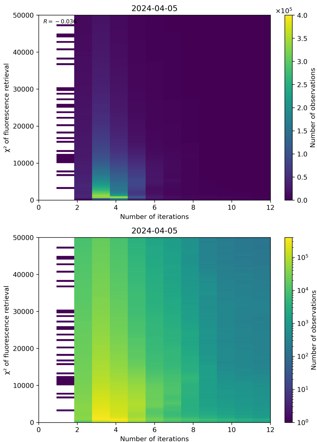
Figure 97: Scatter density plot of “Number of iterations” against “ \chi^2 of fluorescence retrieval” for 2024-04-05 to 2024-04-06.
