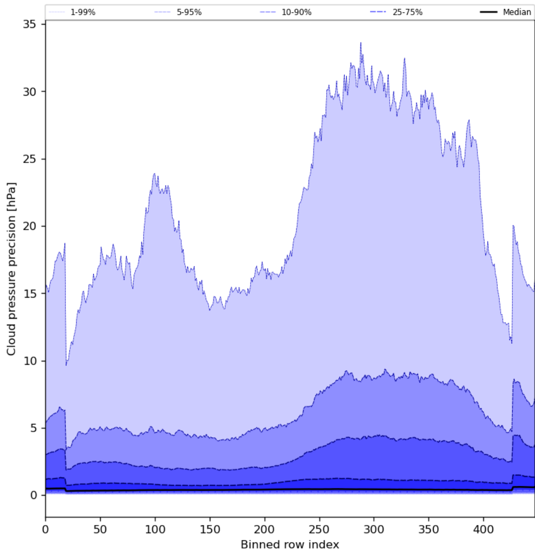
Figure 48: Along track statistics of “Cloud pressure precision” for 2024-04-05 to 2024-04-06
