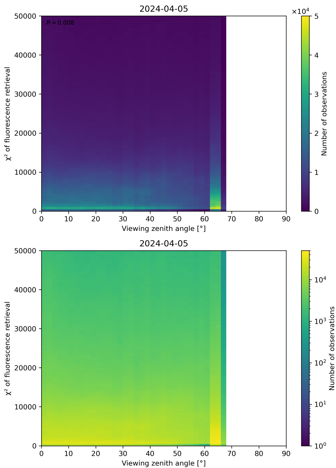
Figure 119: Scatter density plot of “Viewing zenith angle” against “ \chi^2 of fluorescence retrieval” for 2024-04-05 to 2024-04-06.
