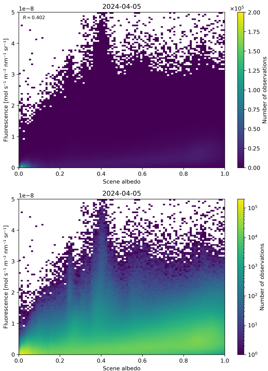
Figure 104: Scatter density plot of “Scene albedo” against “Fluorescence” for 2024-04-05 to 2024-04-06.
