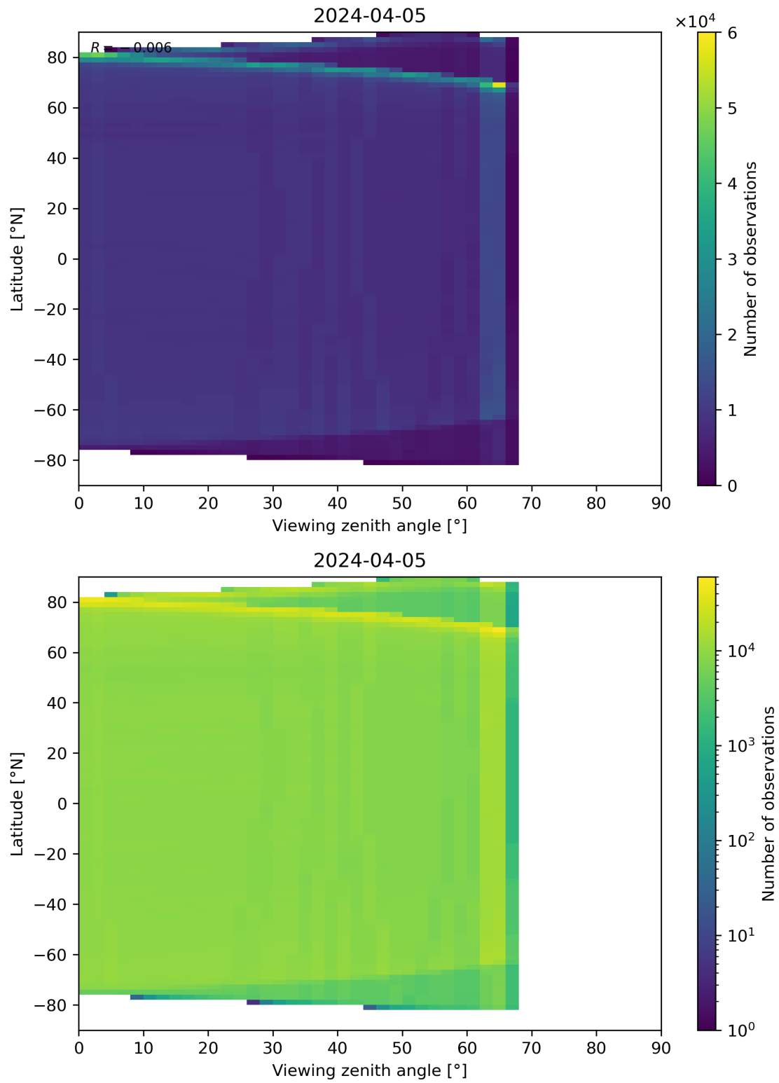
Figure 123: Scatter density plot of “Viewing zenith angle” against “Latitude” for 2024-04-05 to 2024-04-06.
