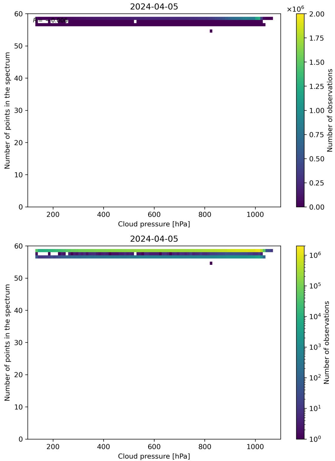
Figure 82: Scatter density plot of “Cloud pressure” against “Number of points in the spectrum” for 2024-04-05 to 2024-04-06.
