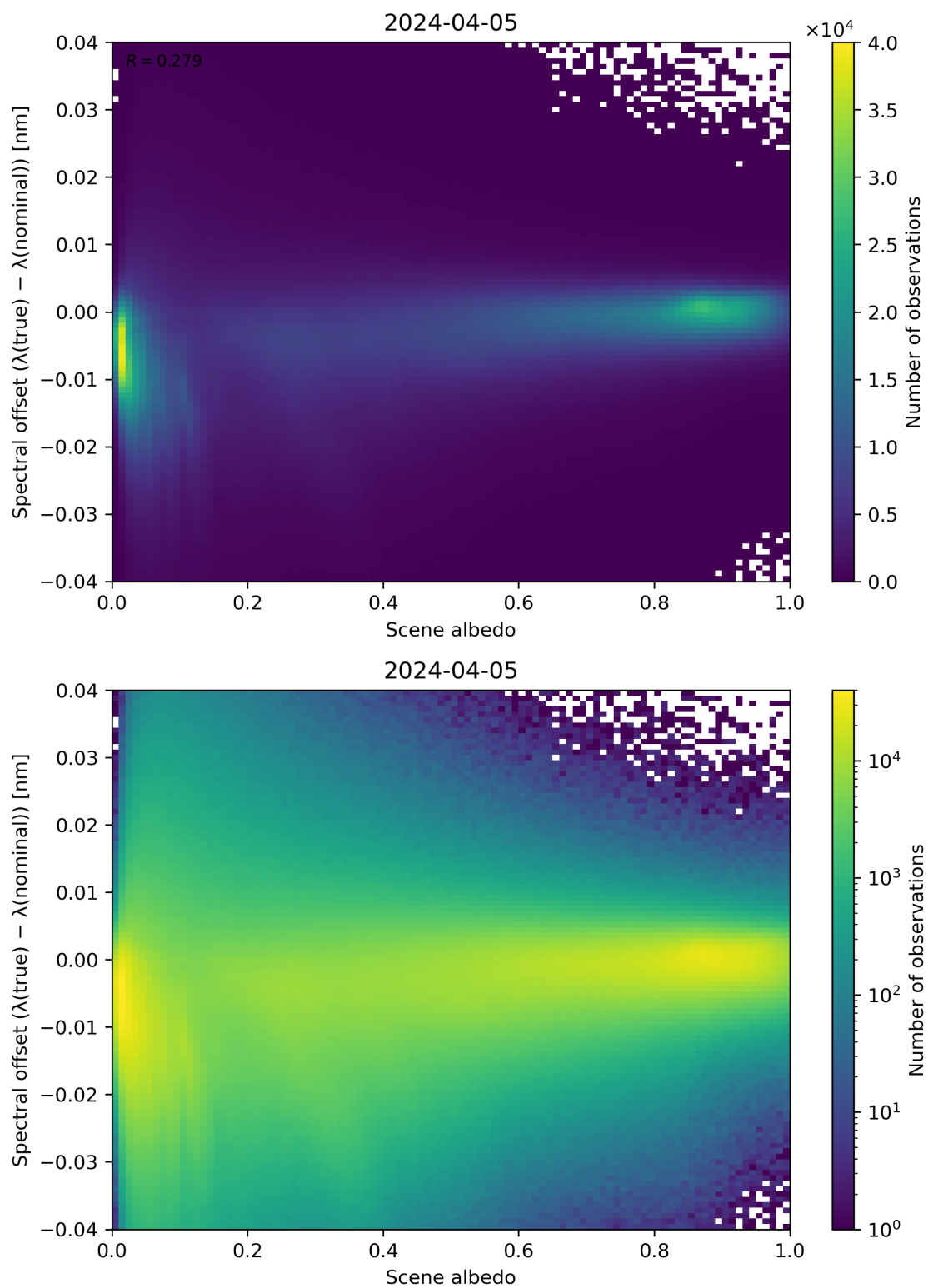
Figure 107: Scatter density plot of “Scene albedo” against “Spectral offset ( \lambda(\text{true}) - \lambda(\text{nominal}) )” for 2024-04-05 to 2024-04-06.
