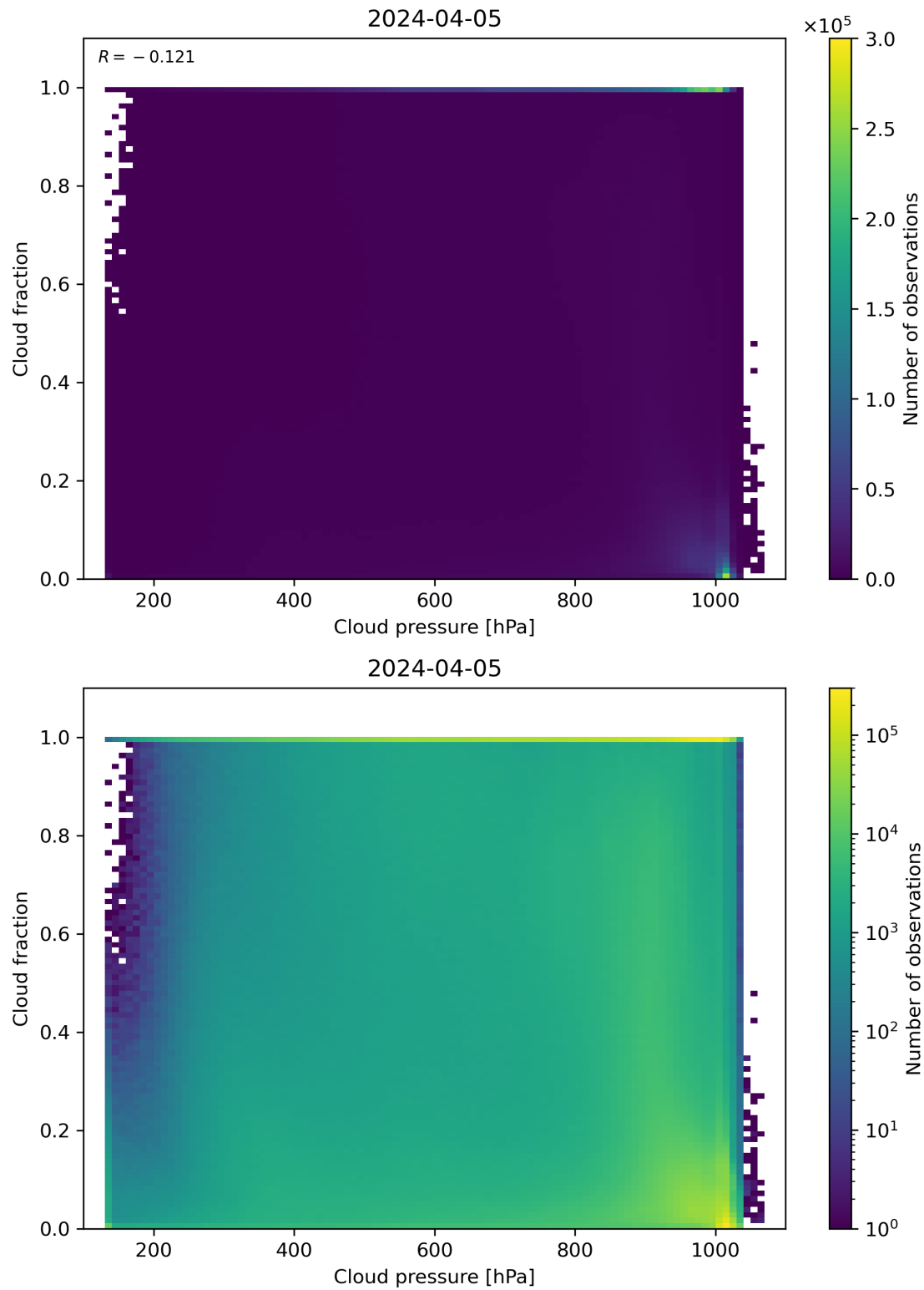
Figure 79: Scatter density plot of “Cloud pressure” against “Cloud fraction” for 2024-04-05 to 2024-04-06.
