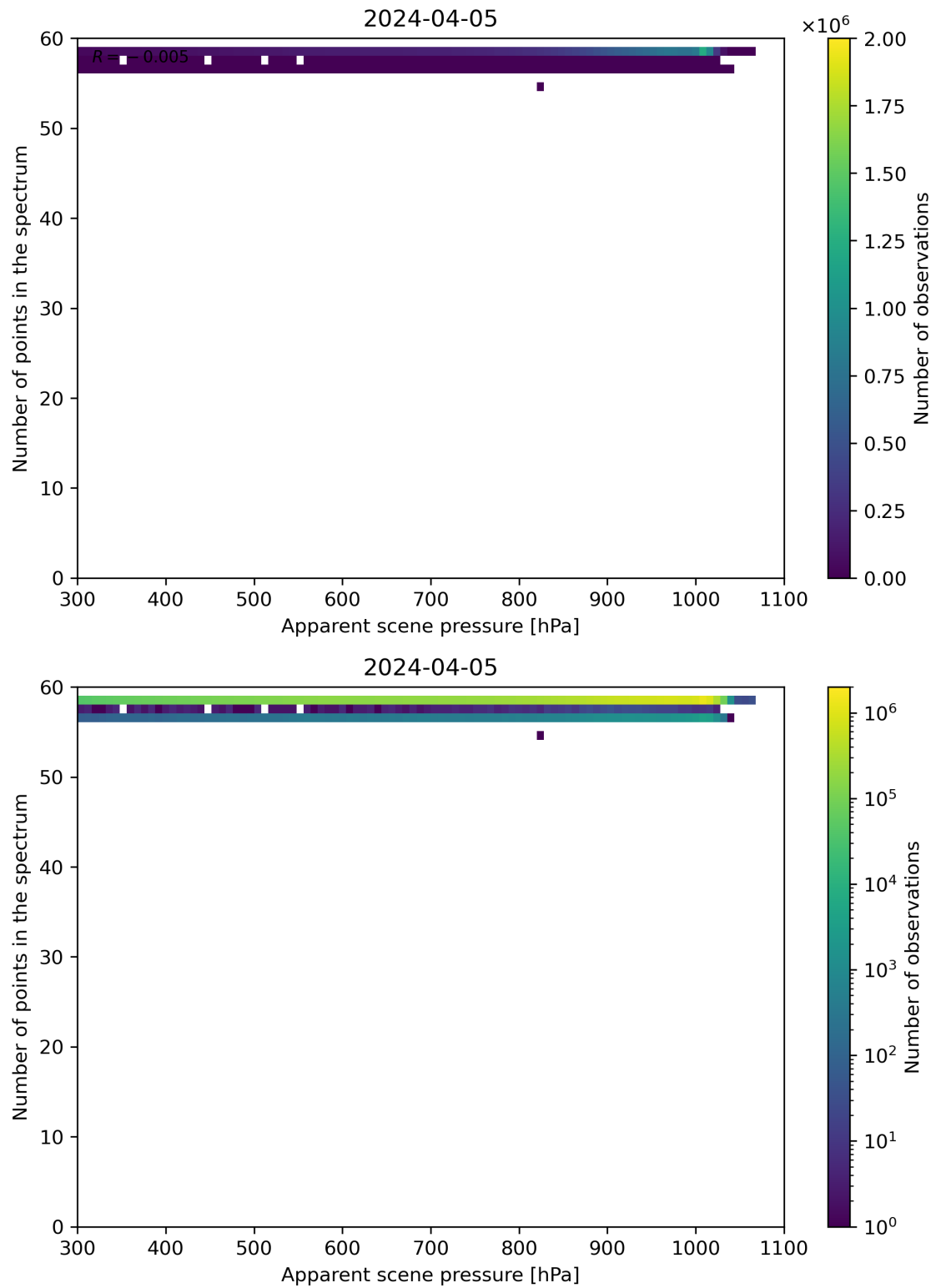
Figure 66: Scatter density plot of “Apparent scene pressure” against “Number of points in the spectrum” for 2024-04-05 to 2024-04-06.
