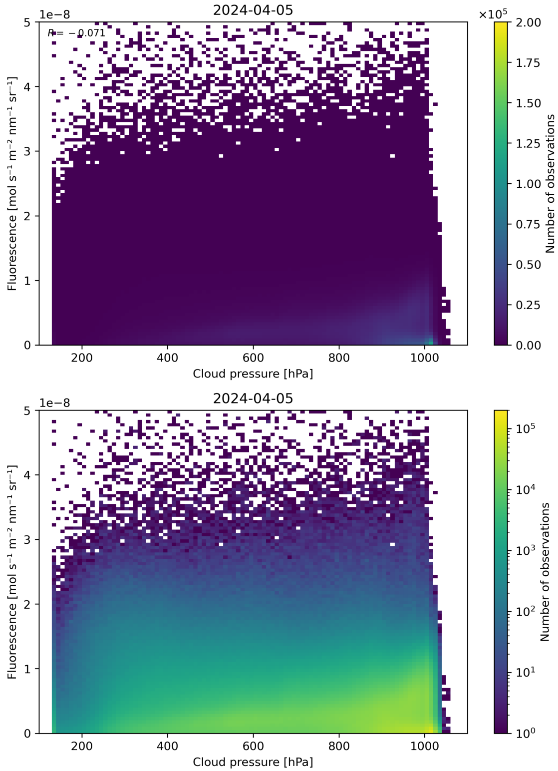
Figure 80: Scatter density plot of “Cloud pressure” against “Fluorescence” for 2024-04-05 to 2024-04-06.
