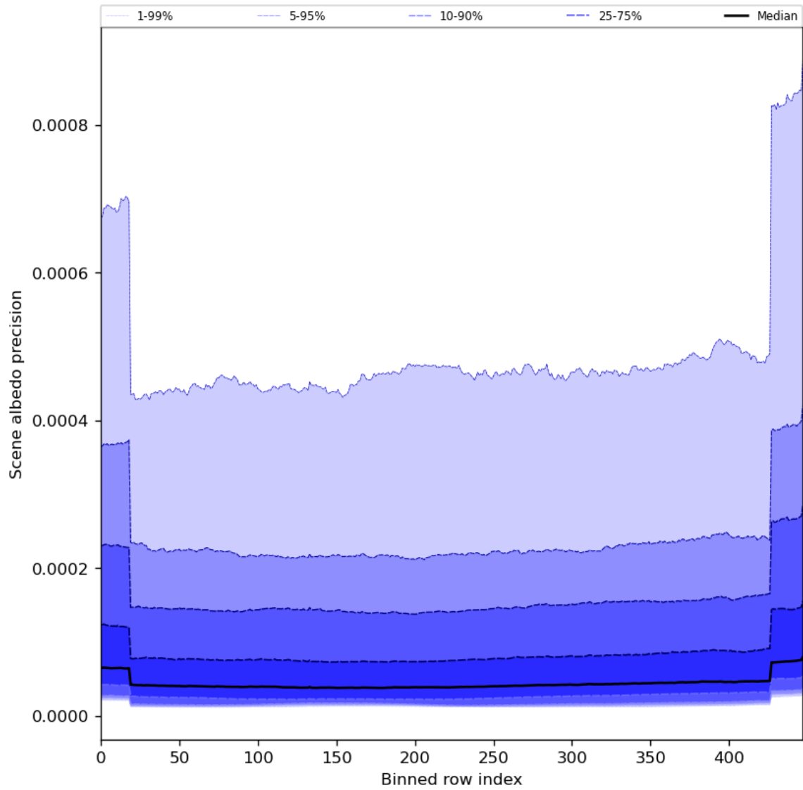
Figure 52: Along track statistics of “Scene albedo precision” for 2024-04-05 to 2024-04-06
