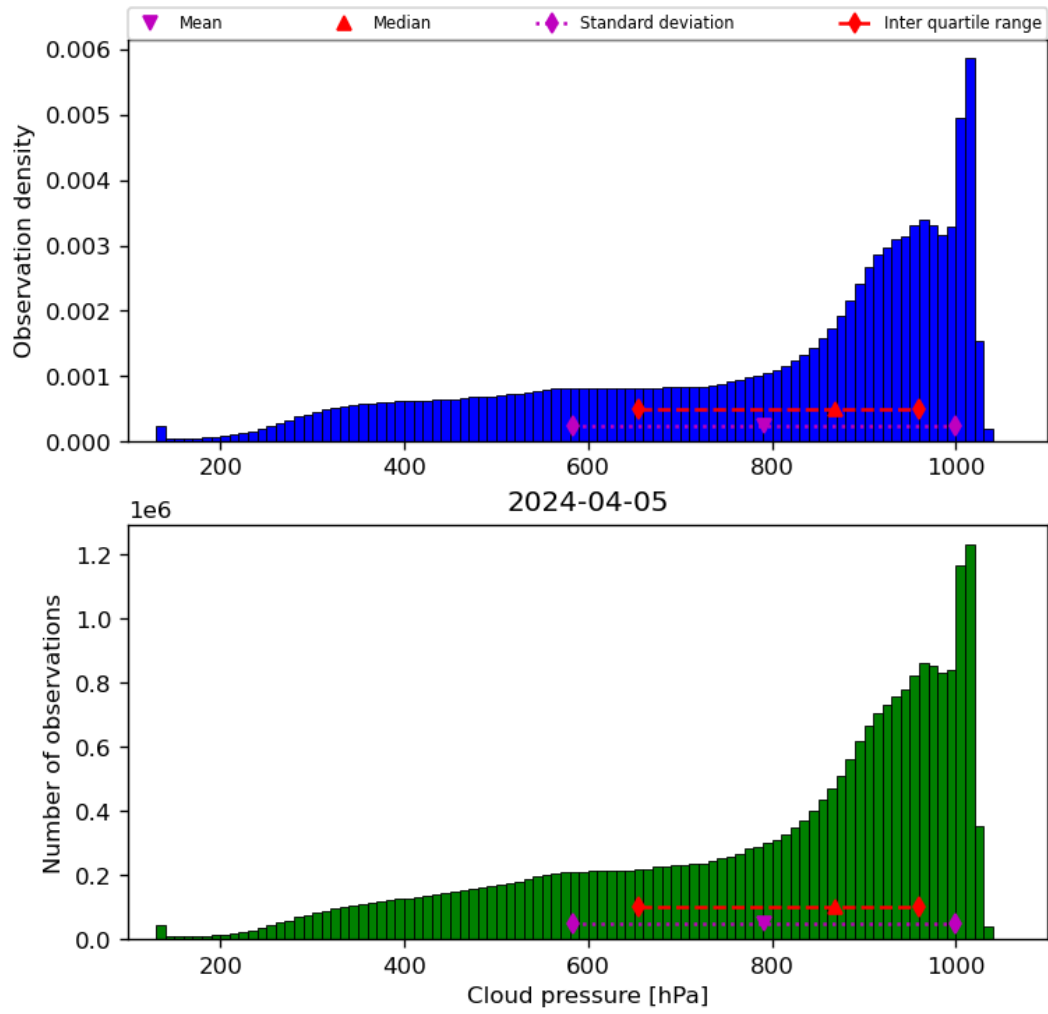
Figure 30: Histogram of “Cloud pressure” for 2024-04-05 to 2024-04-06
