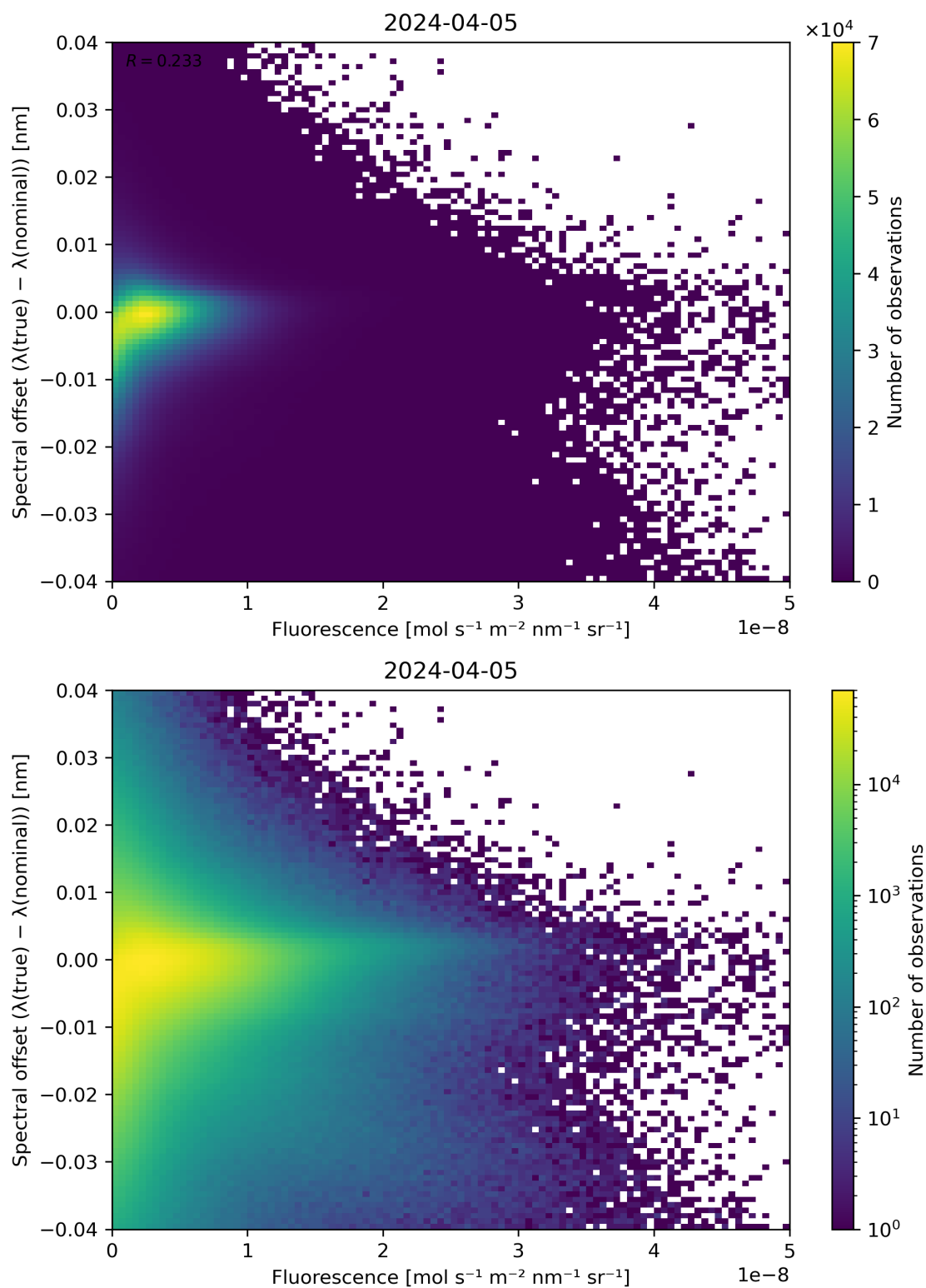
Figure 87: Scatter density plot of “Fluorescence” against “Spectral offset ( \lambda(\text{true}) - \lambda(\text{nominal}) )” for 2024-04-05 to 2024-04-06.
