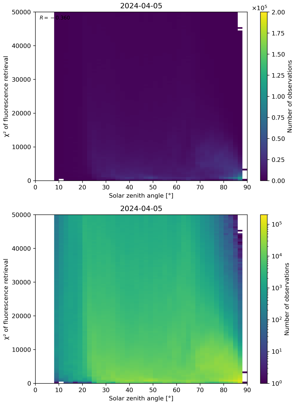
Figure 109: Scatter density plot of “Solar zenith angle” against “ \chi^2 of fluorescence retrieval” for 2024-04-05 to 2024-04-06.
