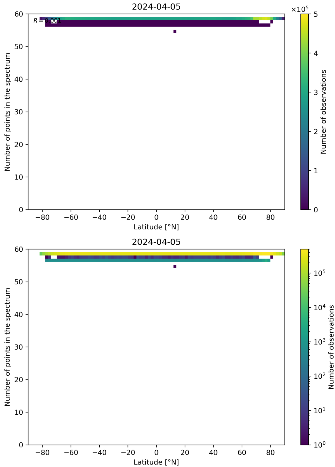
Figure 94: Scatter density plot of “Latitude” against “Number of points in the spectrum” for 2024-04-05 to 2024-04-06.
