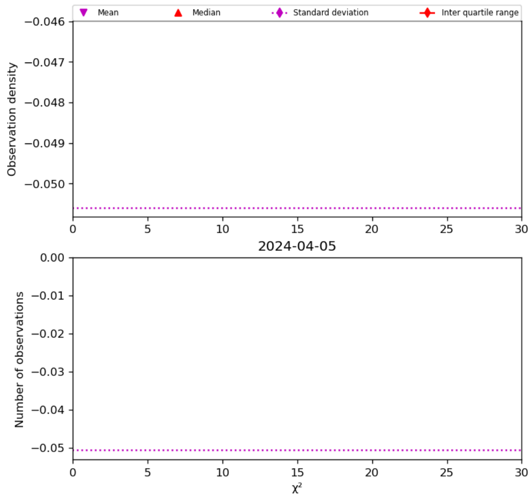
Figure 38: Histogram of “ \chi^2 ” for 2024-04-05 to 2024-04-06
