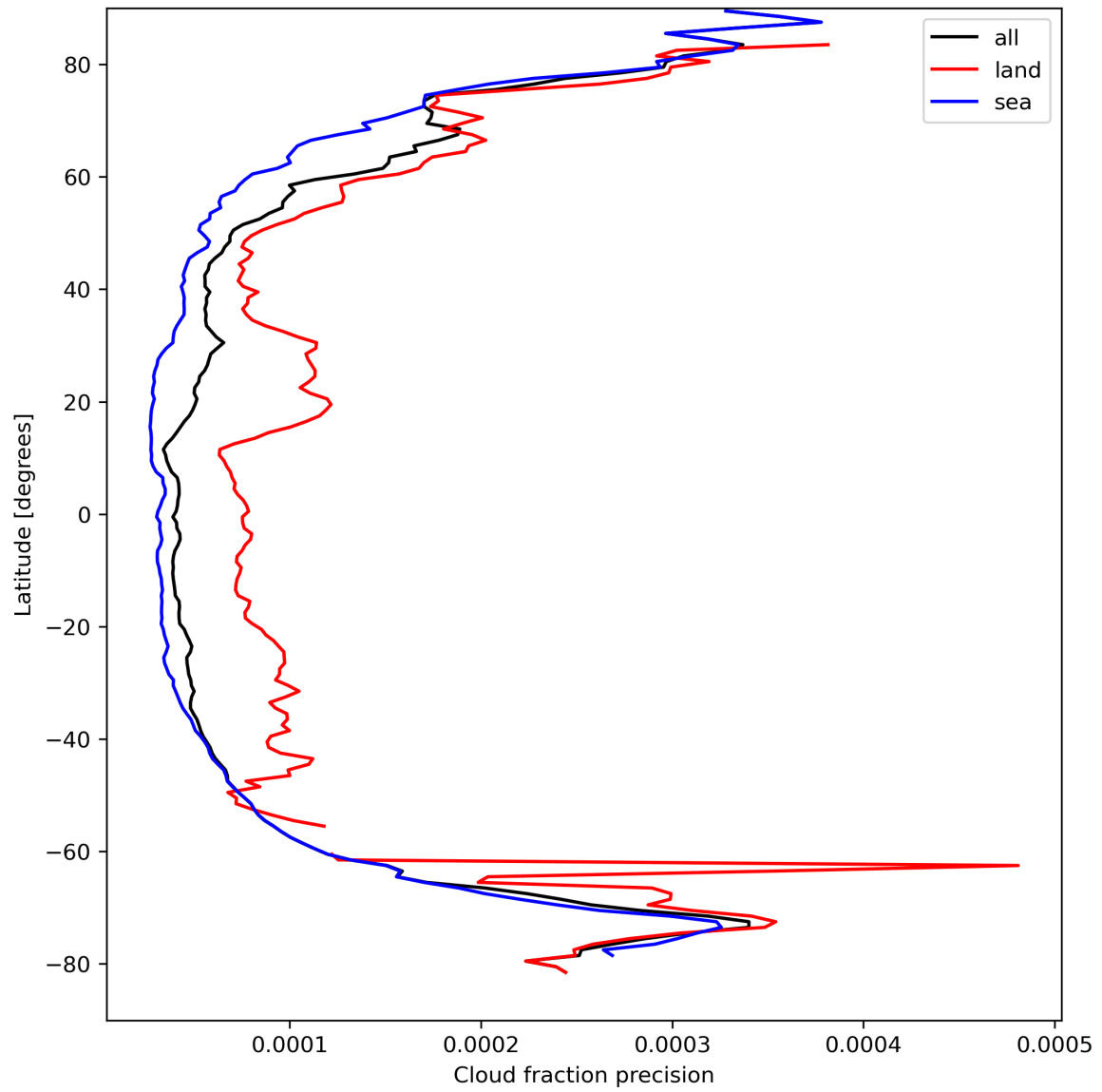
Figure 16: Zonal average of “Cloud fraction precision” for 2024-04-05 to 2024-04-06.
