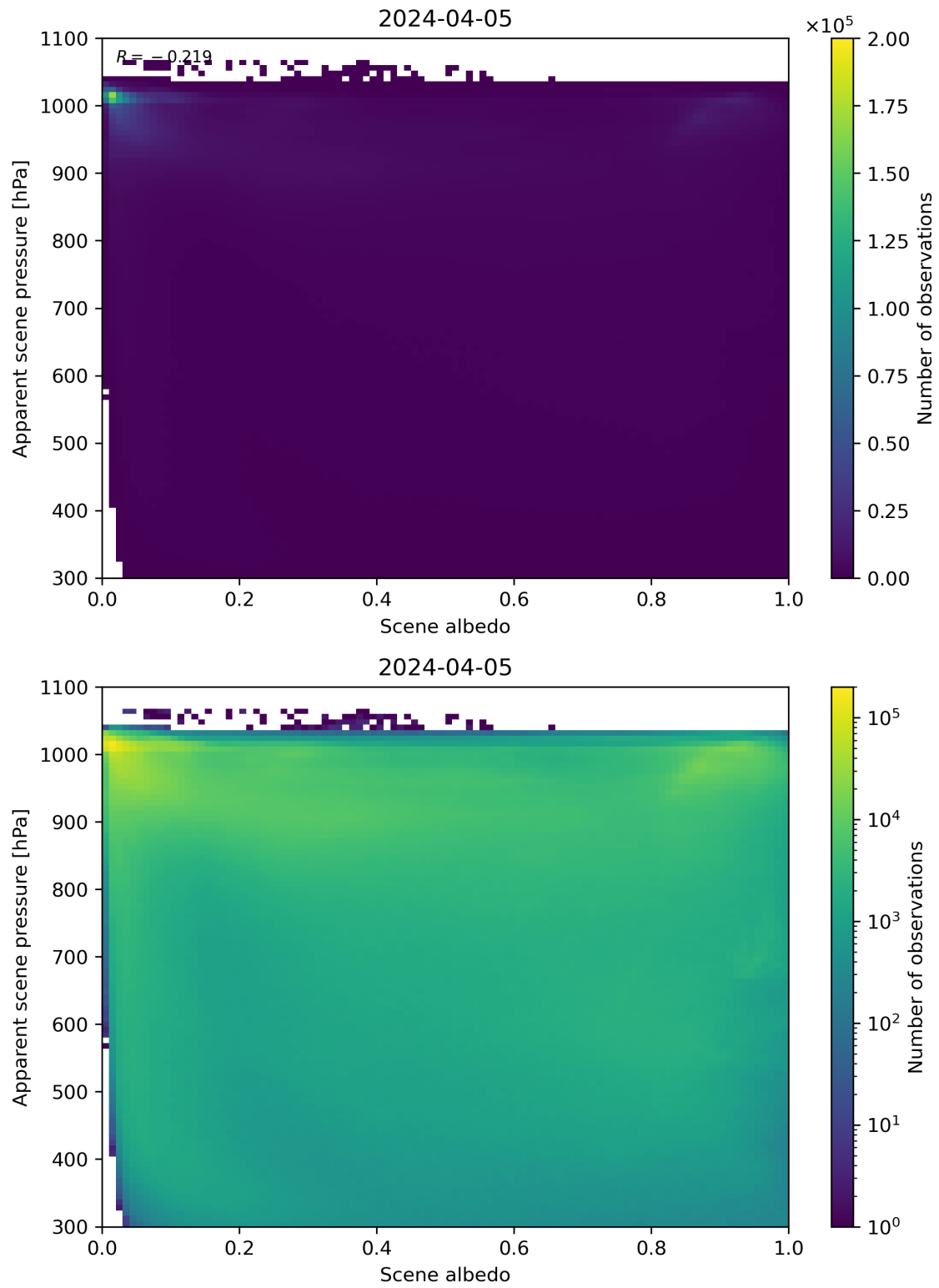
Figure 102: Scatter density plot of “Scene albedo” against “Apparent scene pressure” for 2024-04-05 to 2024-04-06.
