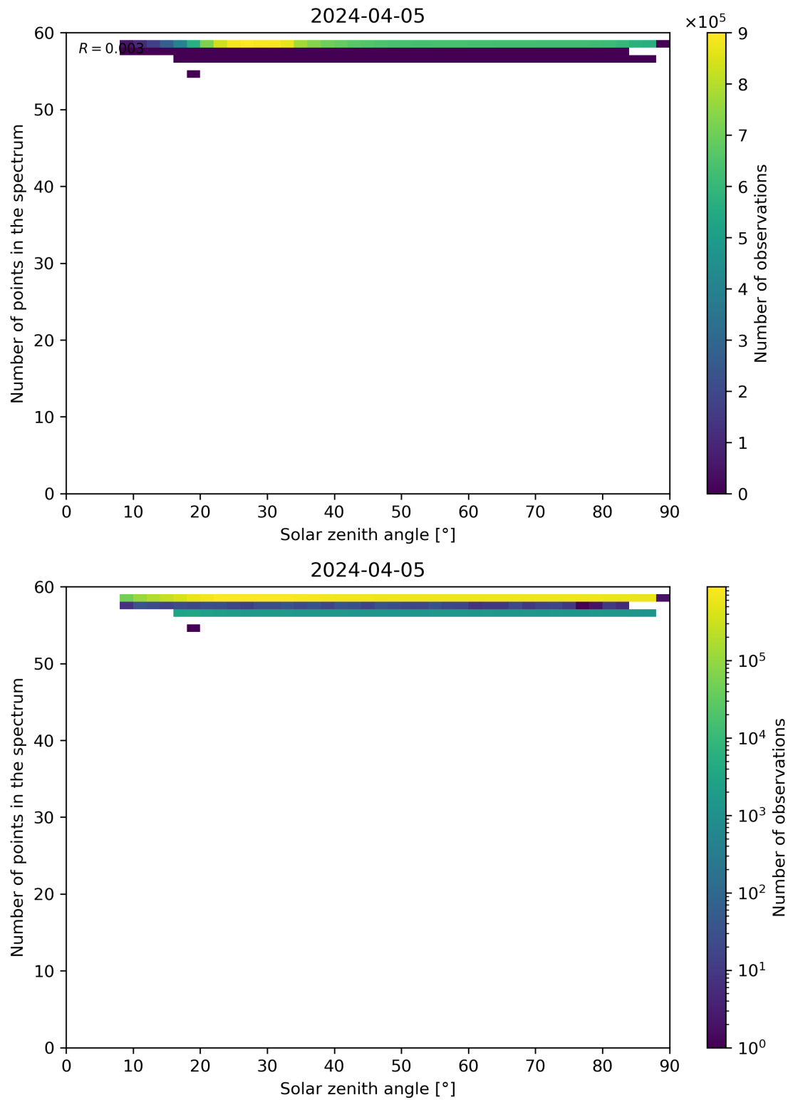
Figure 115: Scatter density plot of “Solar zenith angle” against “Number of points in the spectrum” for 2024-04-05 to 2024-04-06.
