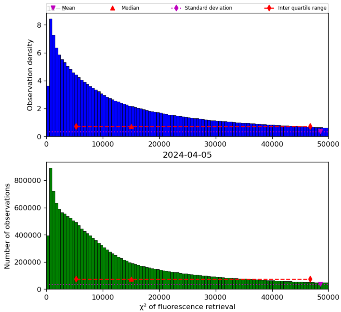
Figure 42: Histogram of “ \chi^2 of fluorescence retrieval” for 2024-04-05 to 2024-04-06
