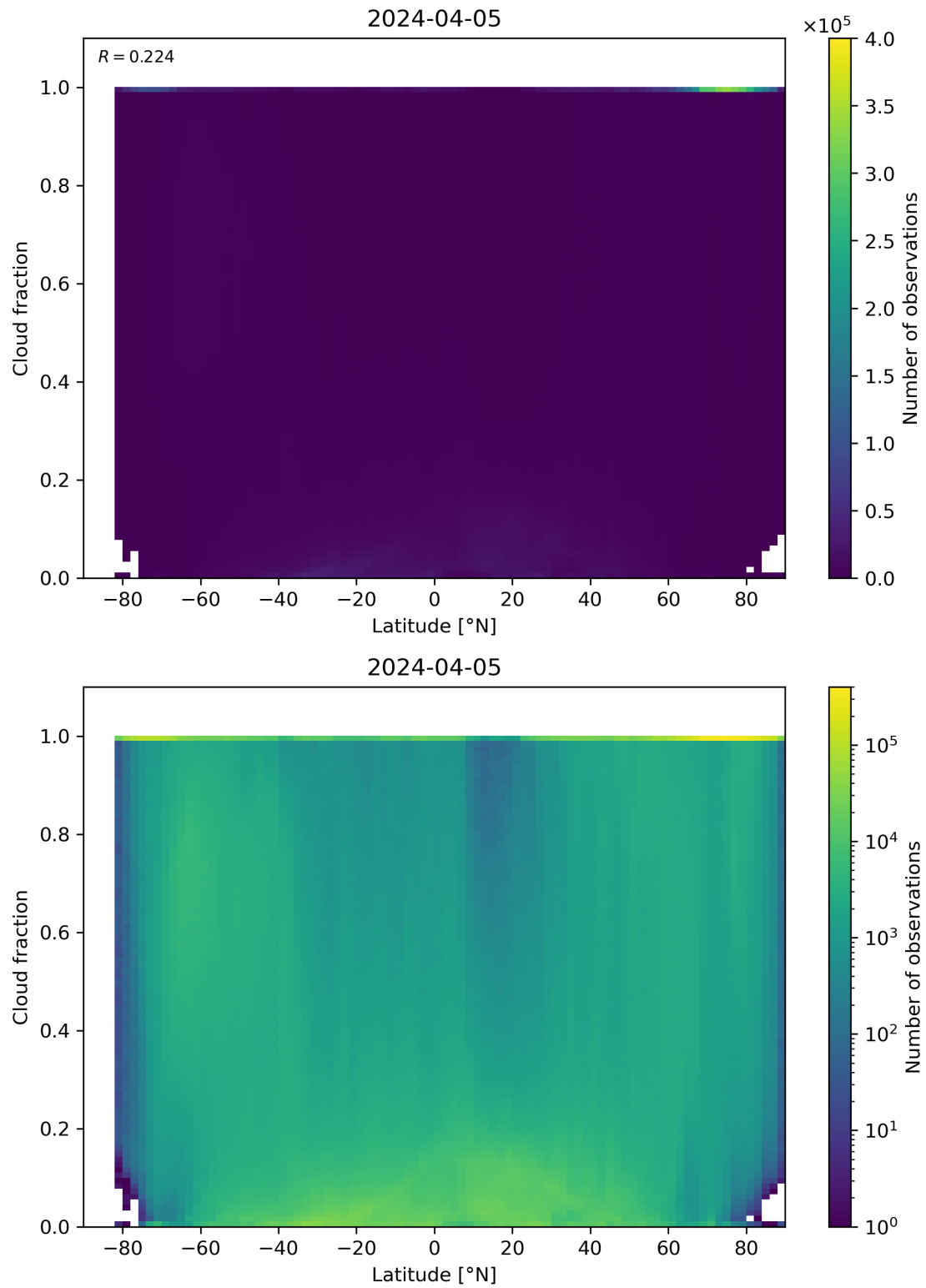
Figure 90: Scatter density plot of “Latitude” against “Cloud fraction” for 2024-04-05 to 2024-04-06.
