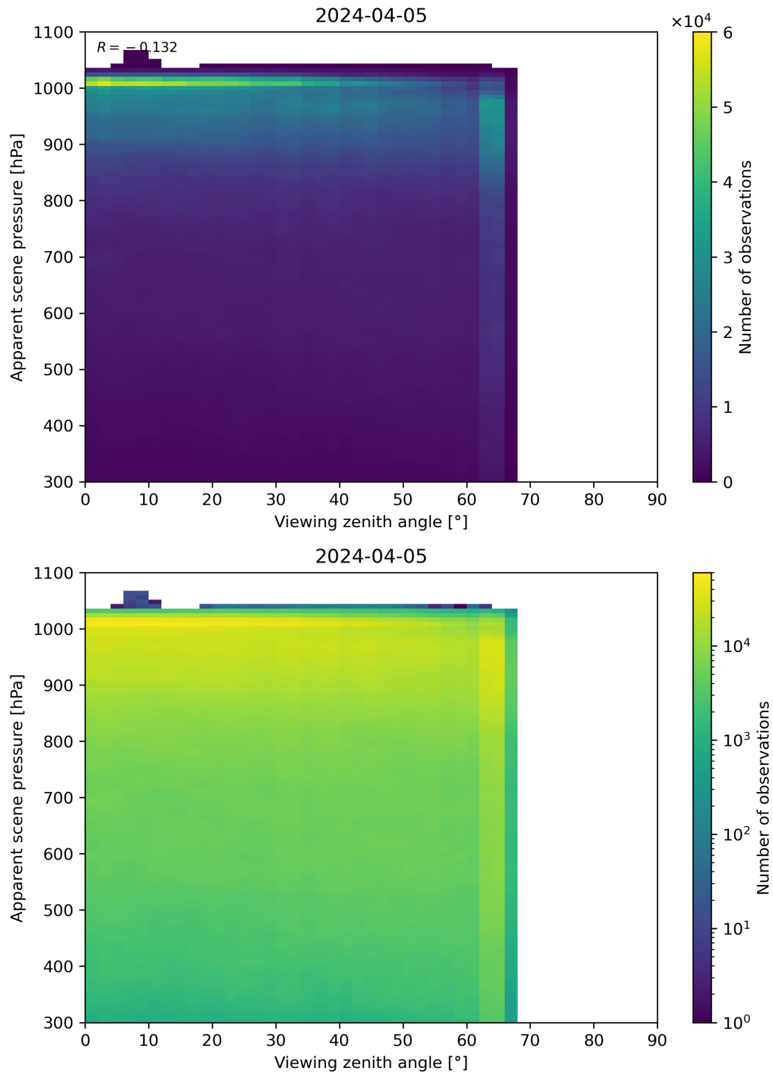
Figure 118: Scatter density plot of “Viewing zenith angle” against “Apparent scene pressure” for 2024-04-05 to 2024-04-06.
