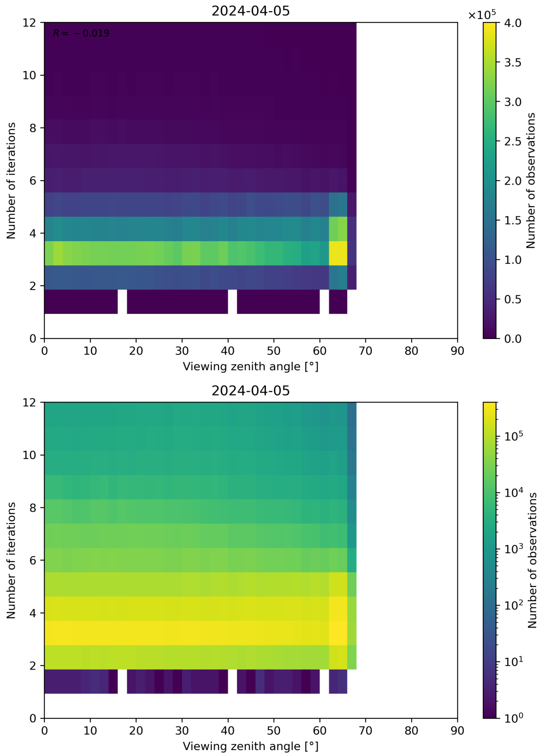
Figure 124: Scatter density plot of “Viewing zenith angle” against “Number of iterations” for 2024-04-05 to 2024-04-06.
