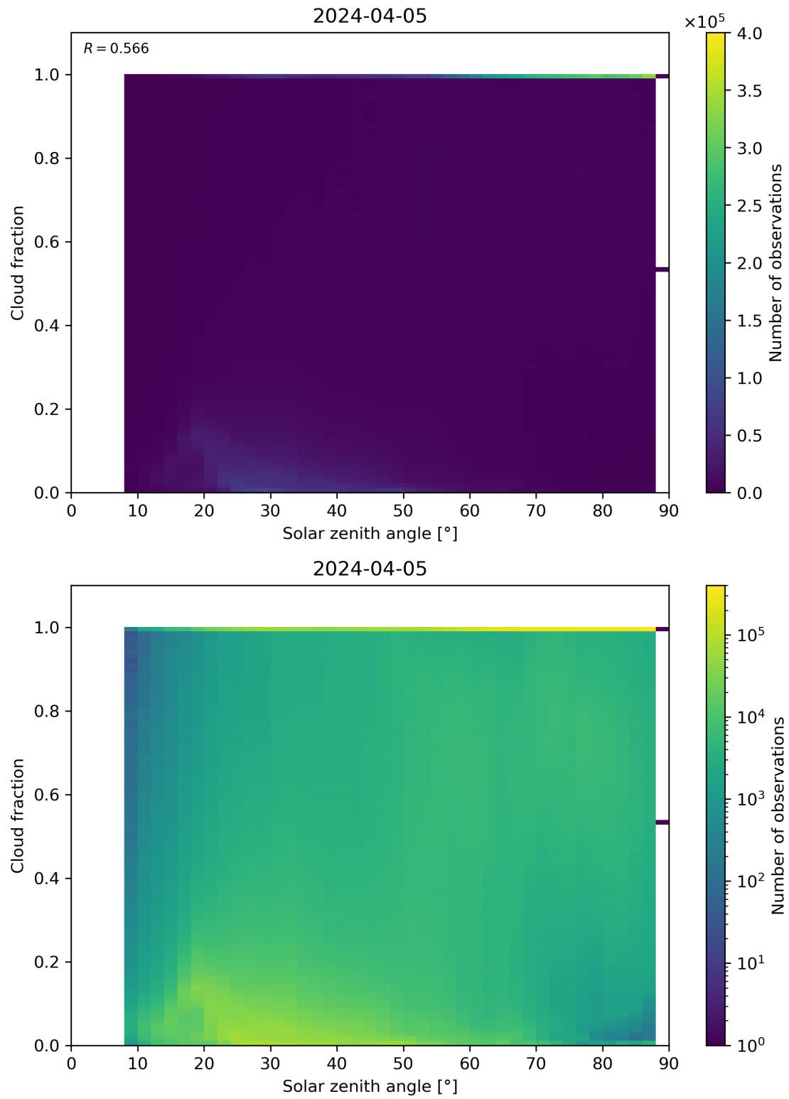
Figure 110: Scatter density plot of “Solar zenith angle” against “Cloud fraction” for 2024-04-05 to 2024-04-06.
