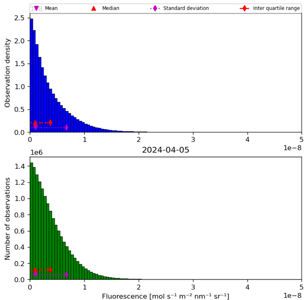
Figure 40: Histogram of “Fluorescence” for 2024-04-05 to 2024-04-06
