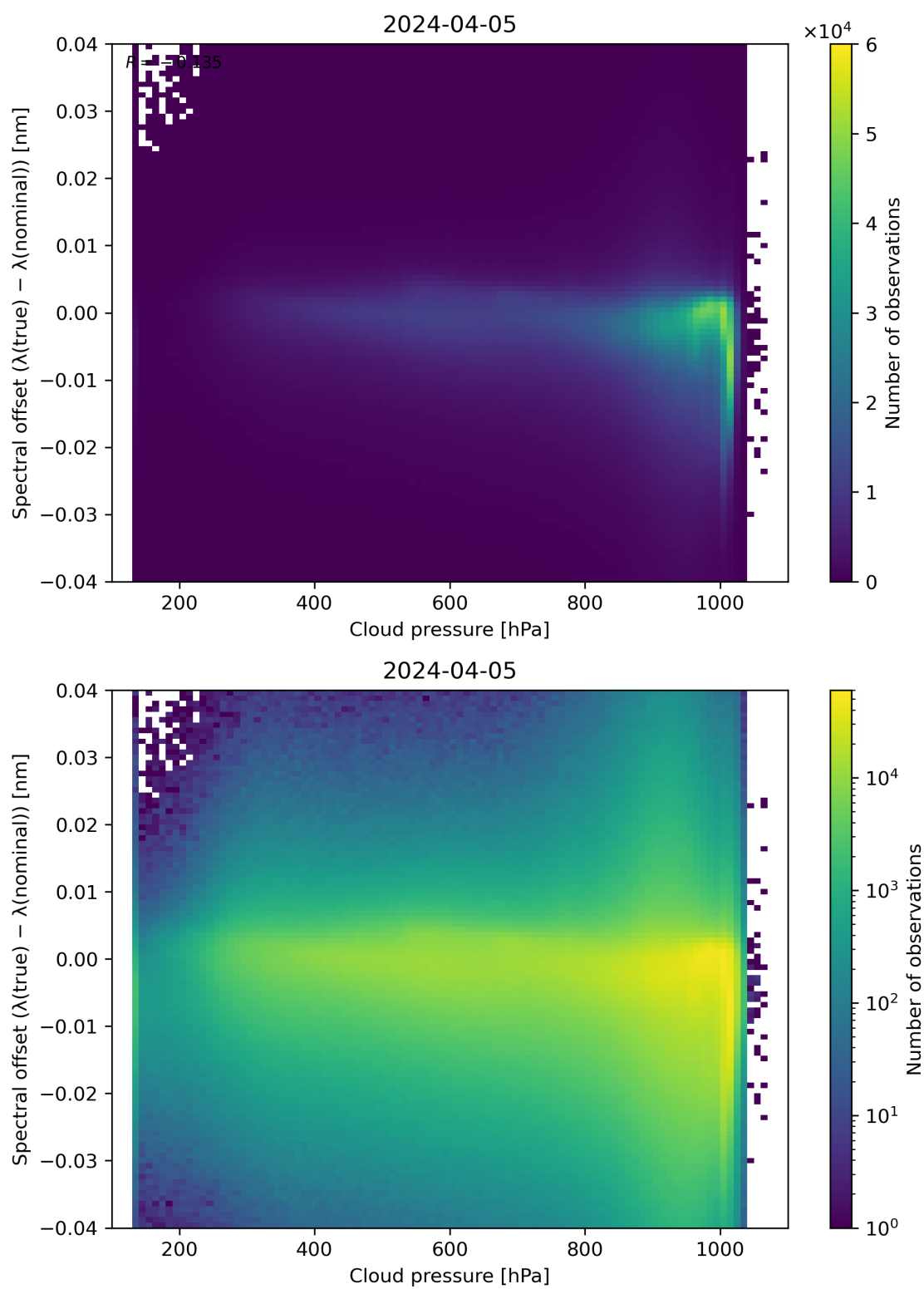
Figure 84: Scatter density plot of “Cloud pressure” against “Spectral offset ( \lambda(\text{true}) - \lambda(\text{nominal}) )” for 2024-04-05 to 2024-04-06.
