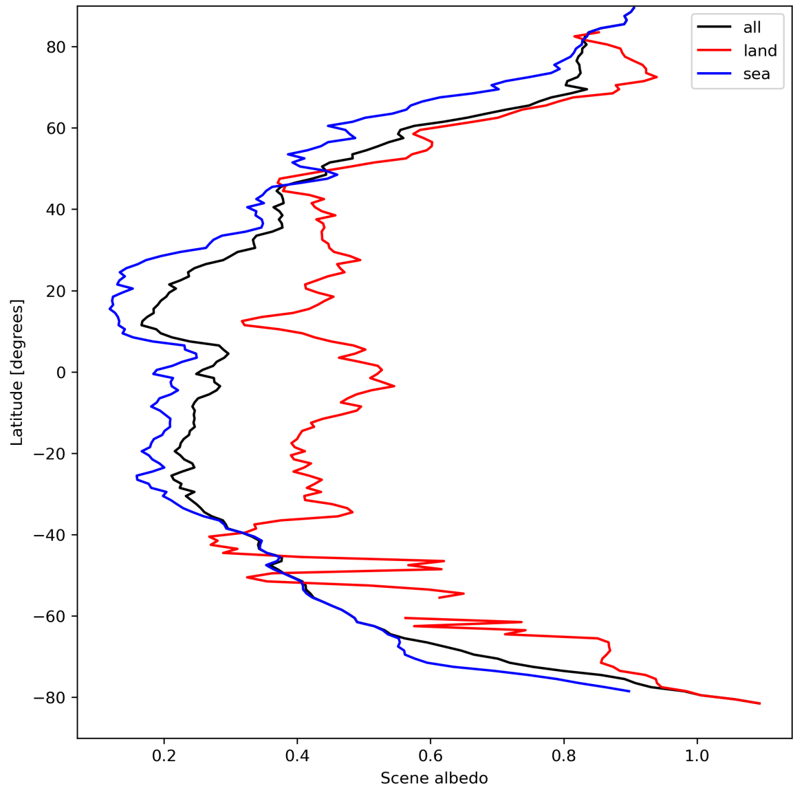
Figure 17: Zonal average of “Scene albedo” for 2024-04-05 to 2024-04-06.
