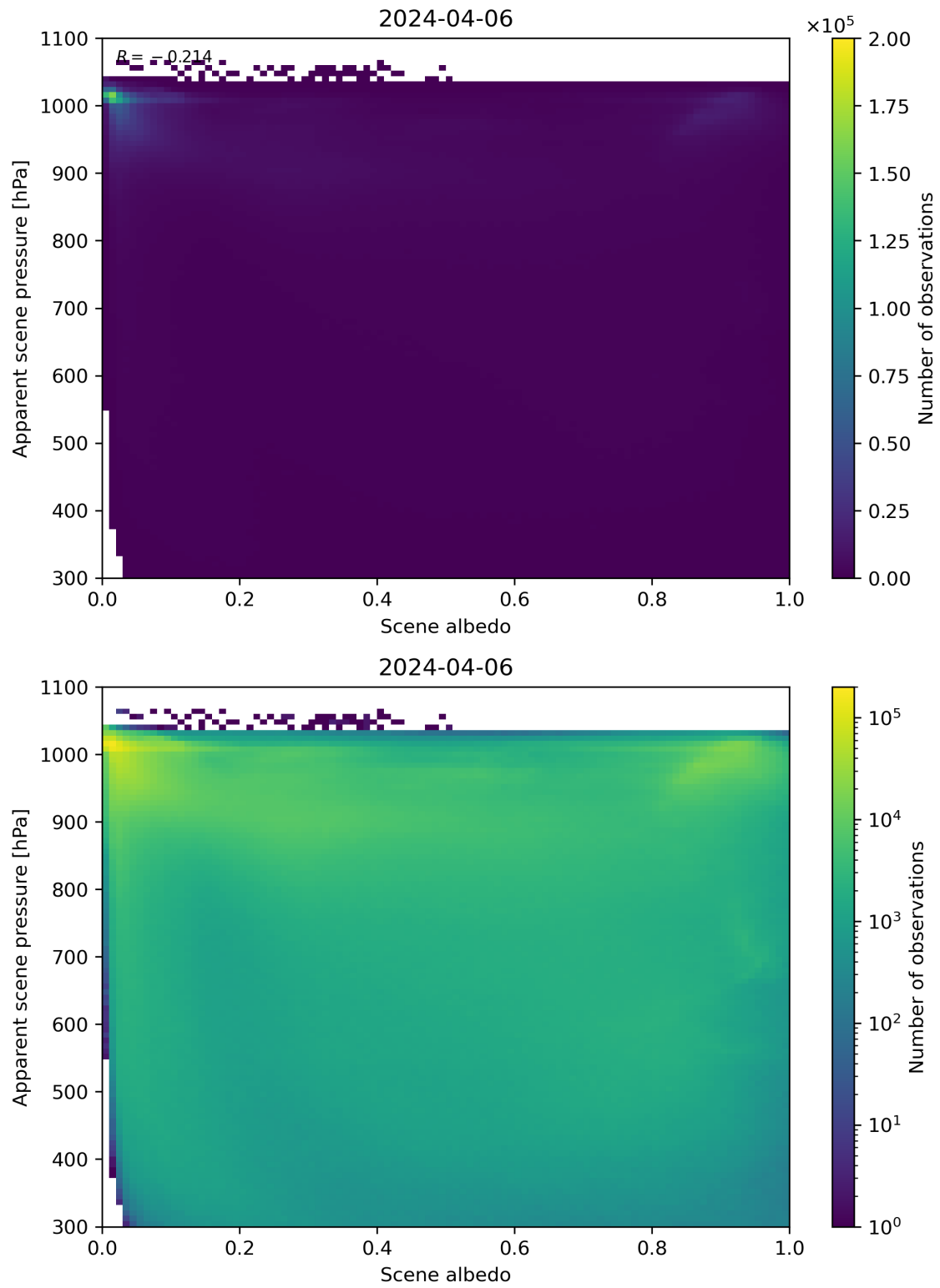
Figure 102: Scatter density plot of “Scene albedo” against “Apparent scene pressure” for 2024-04-05 to 2024-04-07.
