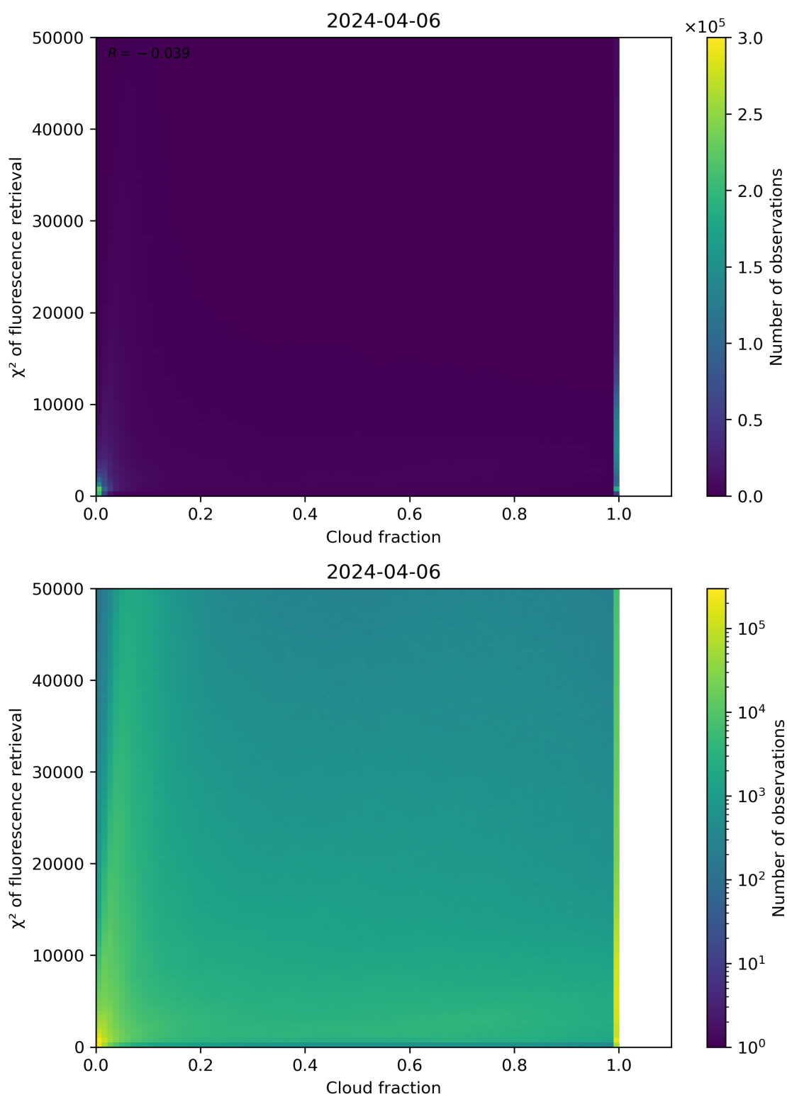
Figure 71: Scatter density plot of “Cloud fraction” against “ \chi^2 of fluorescence retrieval” for 2024-04-05 to 2024-04-07.
