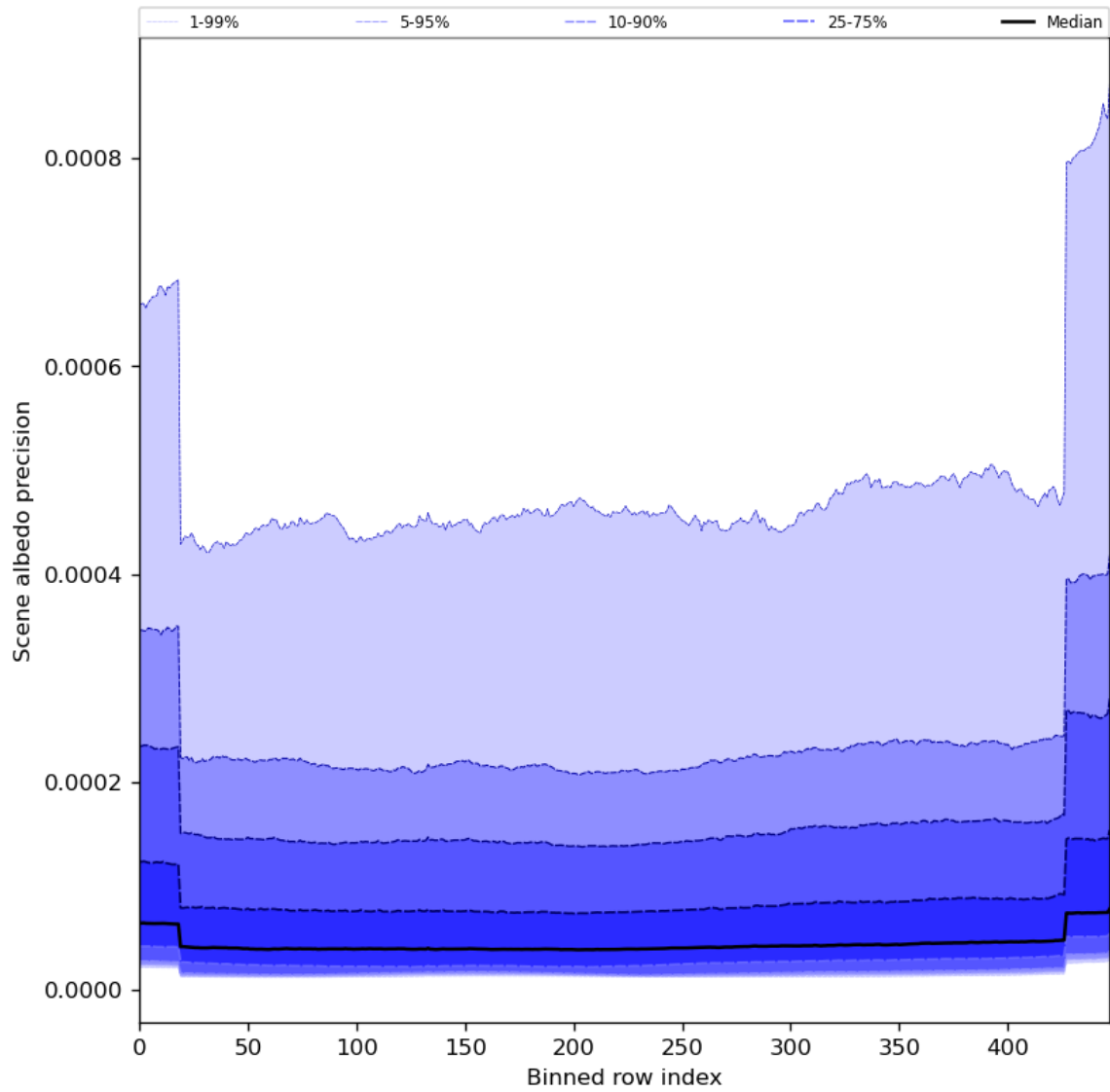
Figure 52: Along track statistics of “Scene albedo precision” for 2024-04-05 to 2024-04-07
