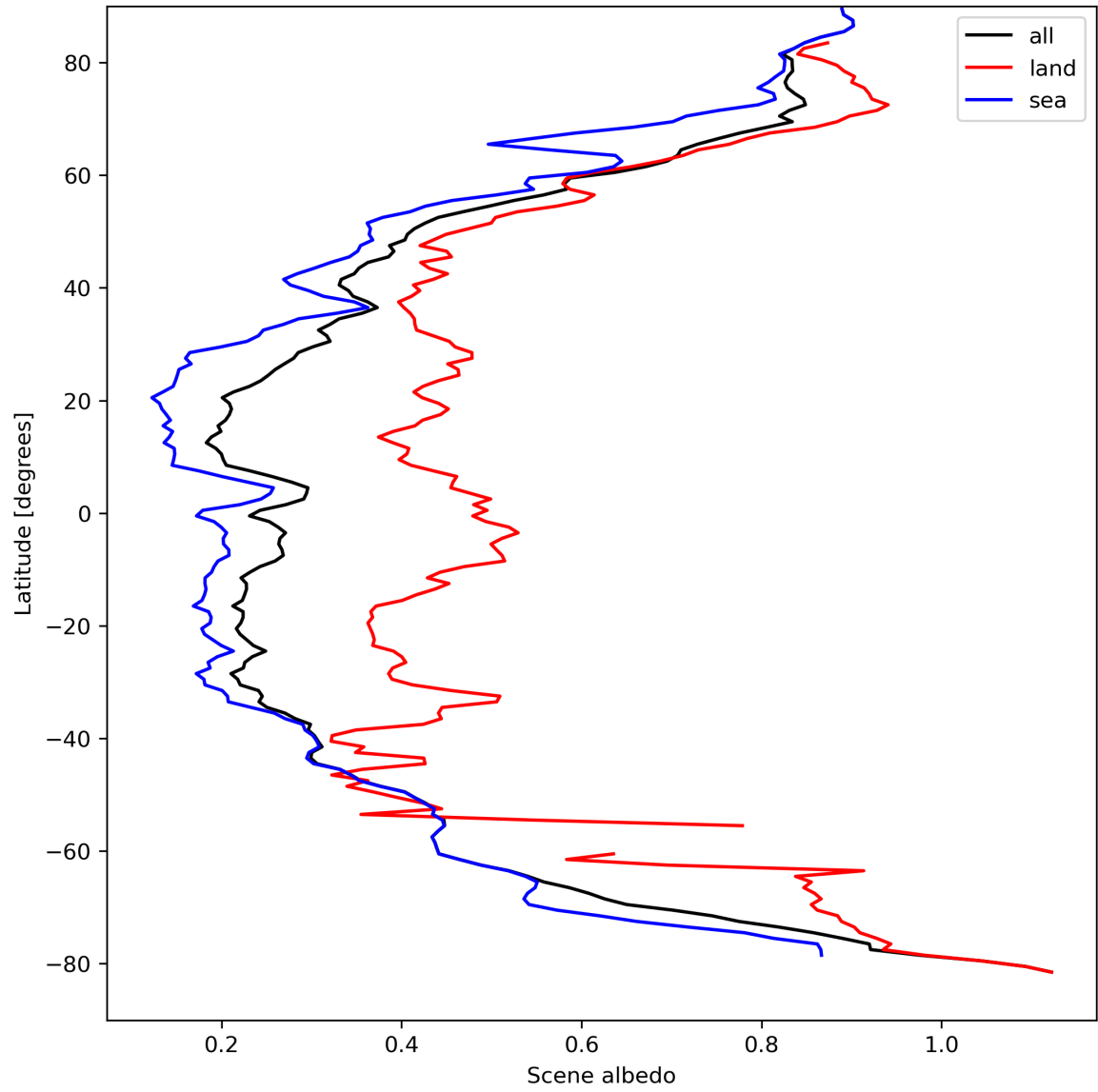
Figure 17: Zonal average of “Scene albedo” for 2024-04-05 to 2024-04-07.
