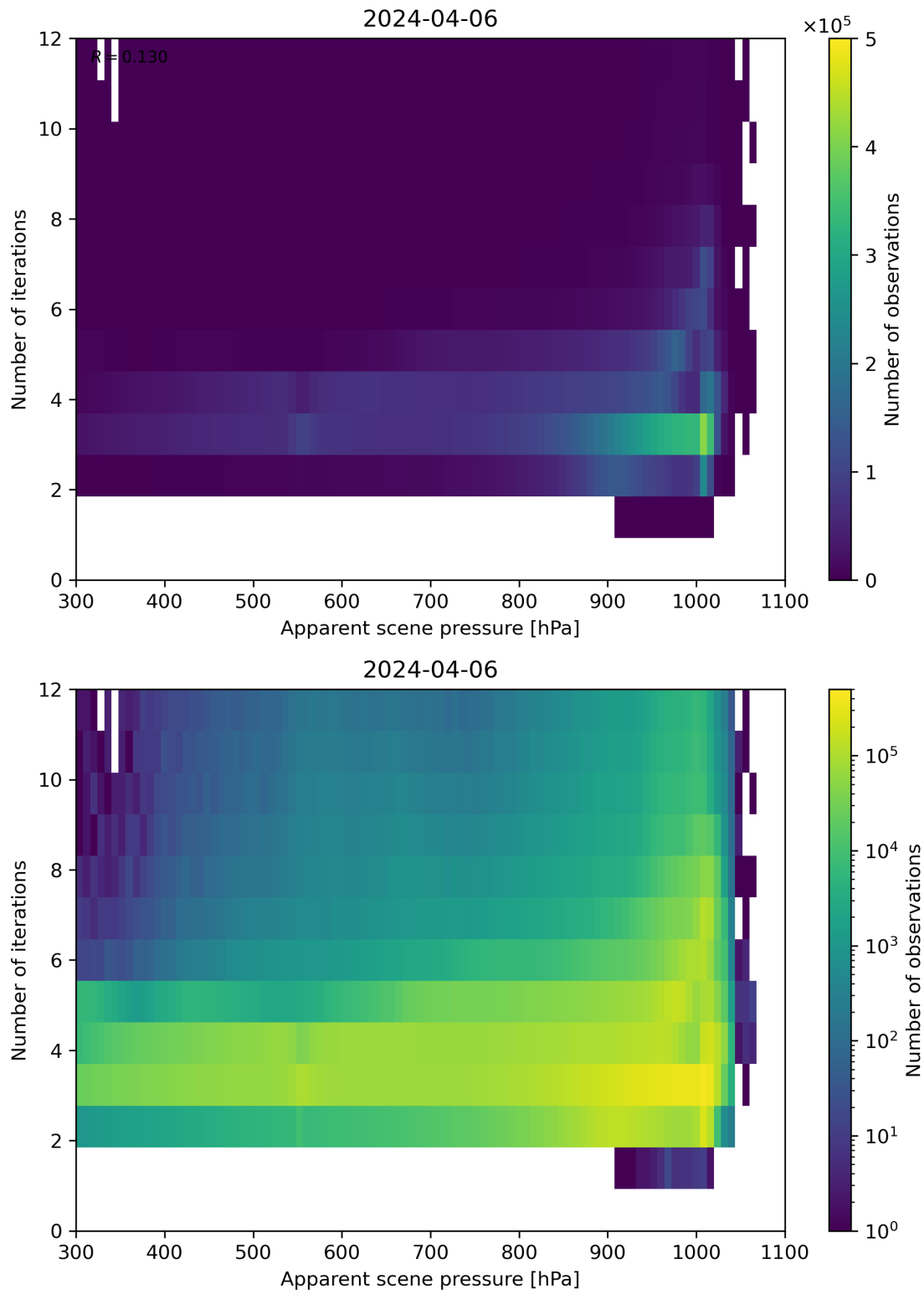
Figure 65: Scatter density plot of “Apparent scene pressure” against “Number of iterations” for 2024-04-05 to 2024-04-07.
