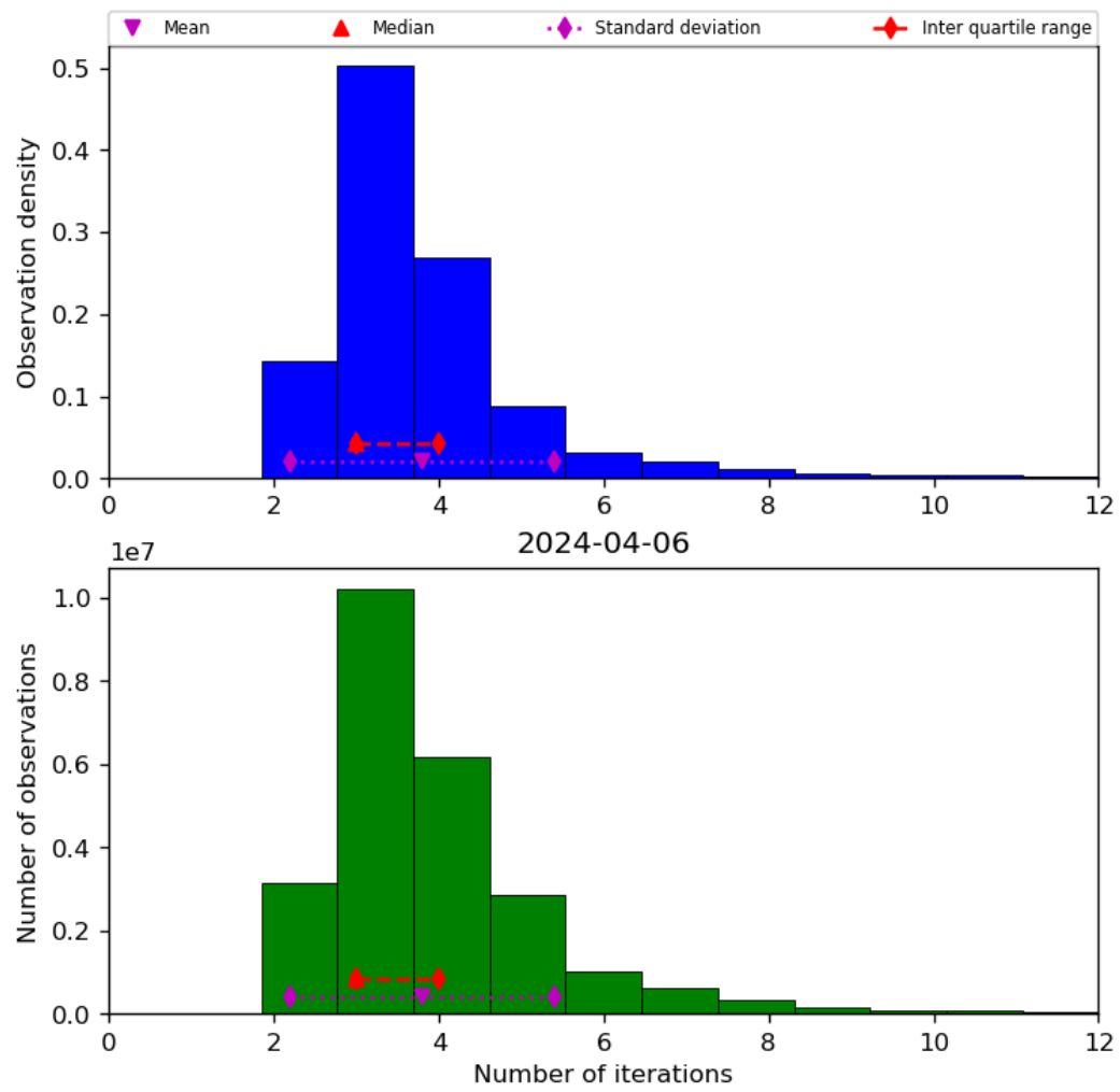
Figure 39: Histogram of “Number of iterations” for 2024-04-05 to 2024-04-07
