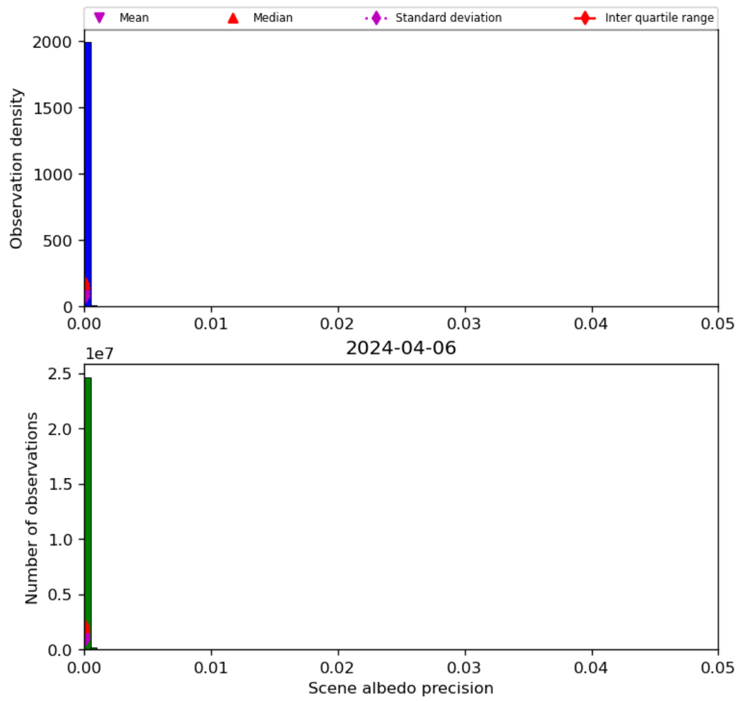
Figure 35: Histogram of “Scene albedo precision” for 2024-04-05 to 2024-04-07
