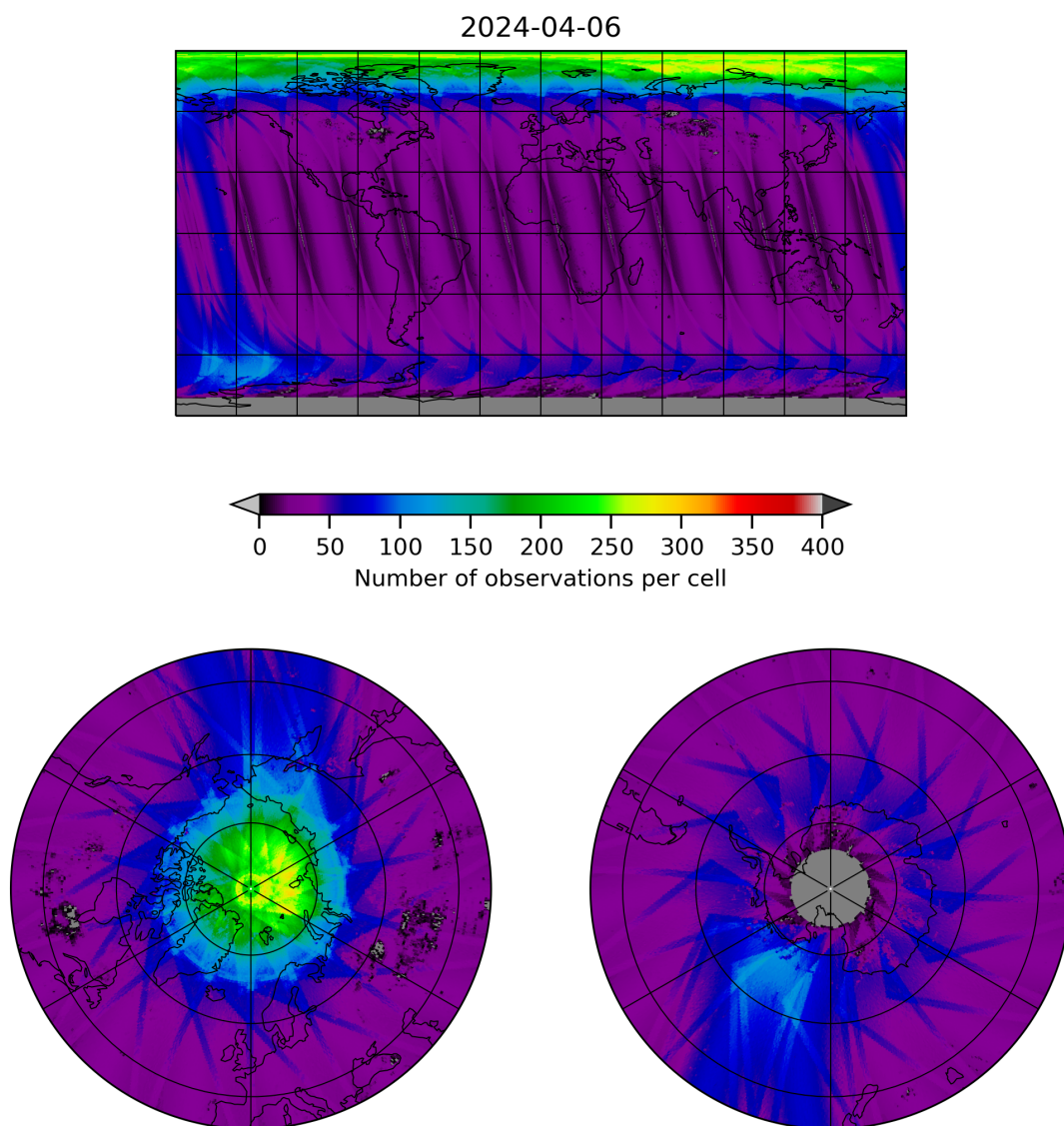
Figure 11: Map of the number of observations for 2024-04-05 to 2024-04-07
