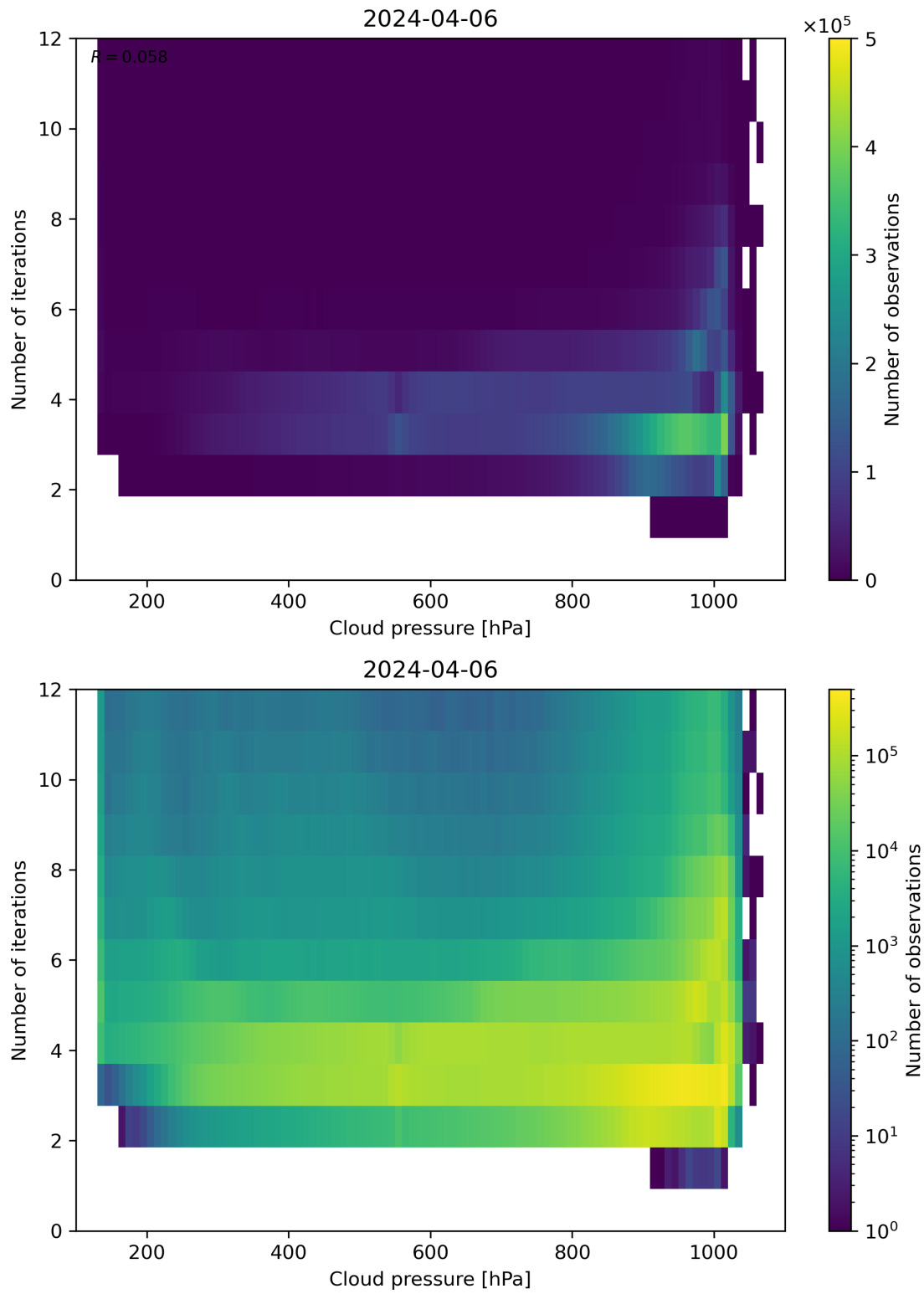
Figure 81: Scatter density plot of “Cloud pressure” against “Number of iterations” for 2024-04-05 to 2024-04-07.
