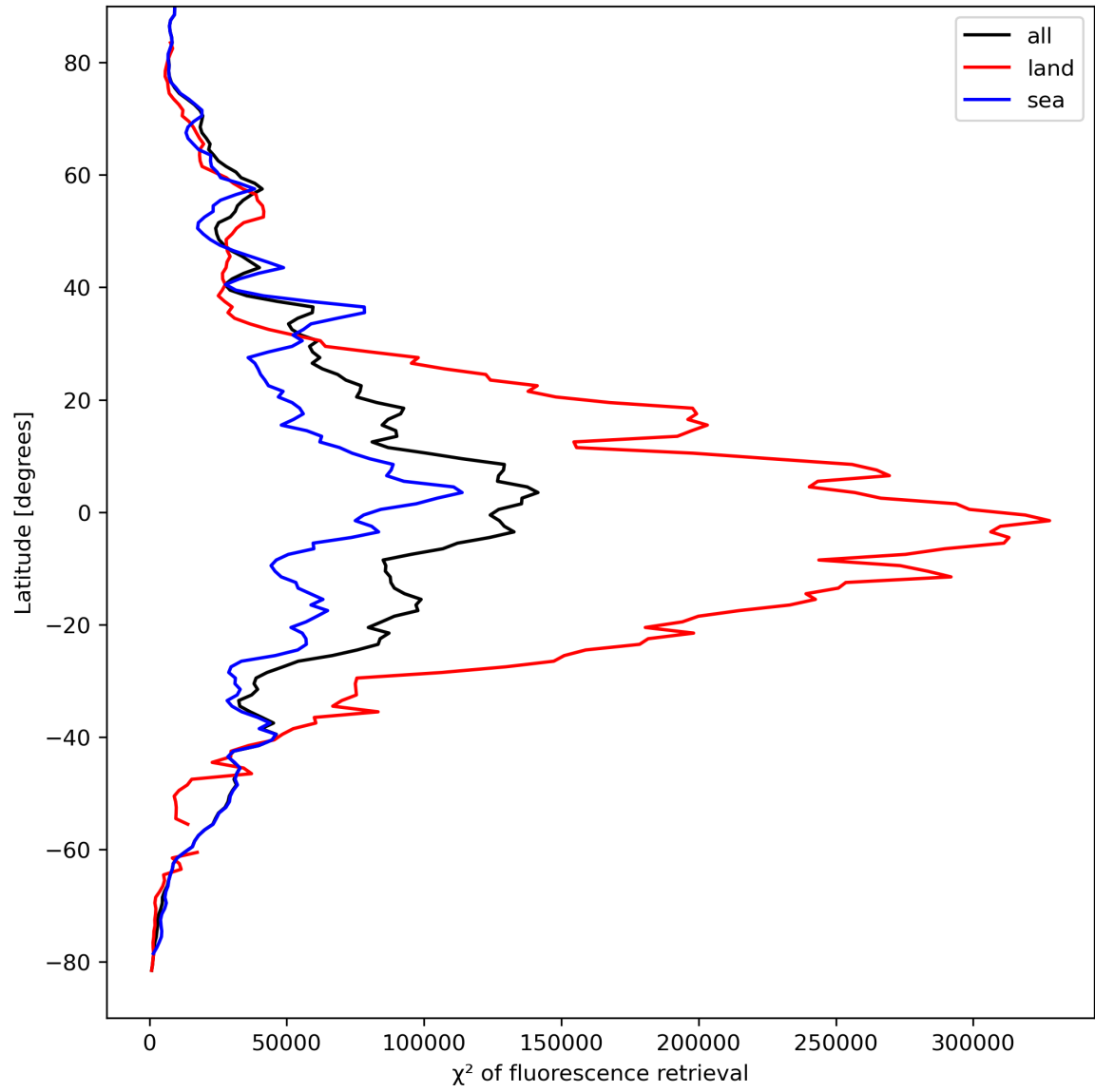
Figure 25: Zonal average of “ \chi^2 of fluorescence retrieval” for 2024-04-05 to 2024-04-07.
