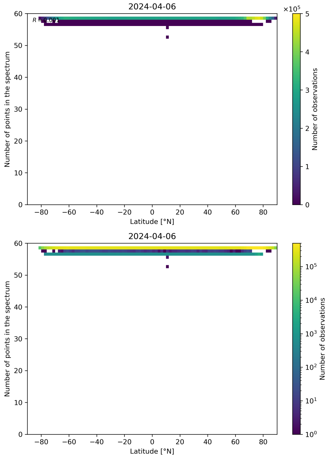
Figure 94: Scatter density plot of “Latitude” against “Number of points in the spectrum” for 2024-04-05 to 2024-04-07.
