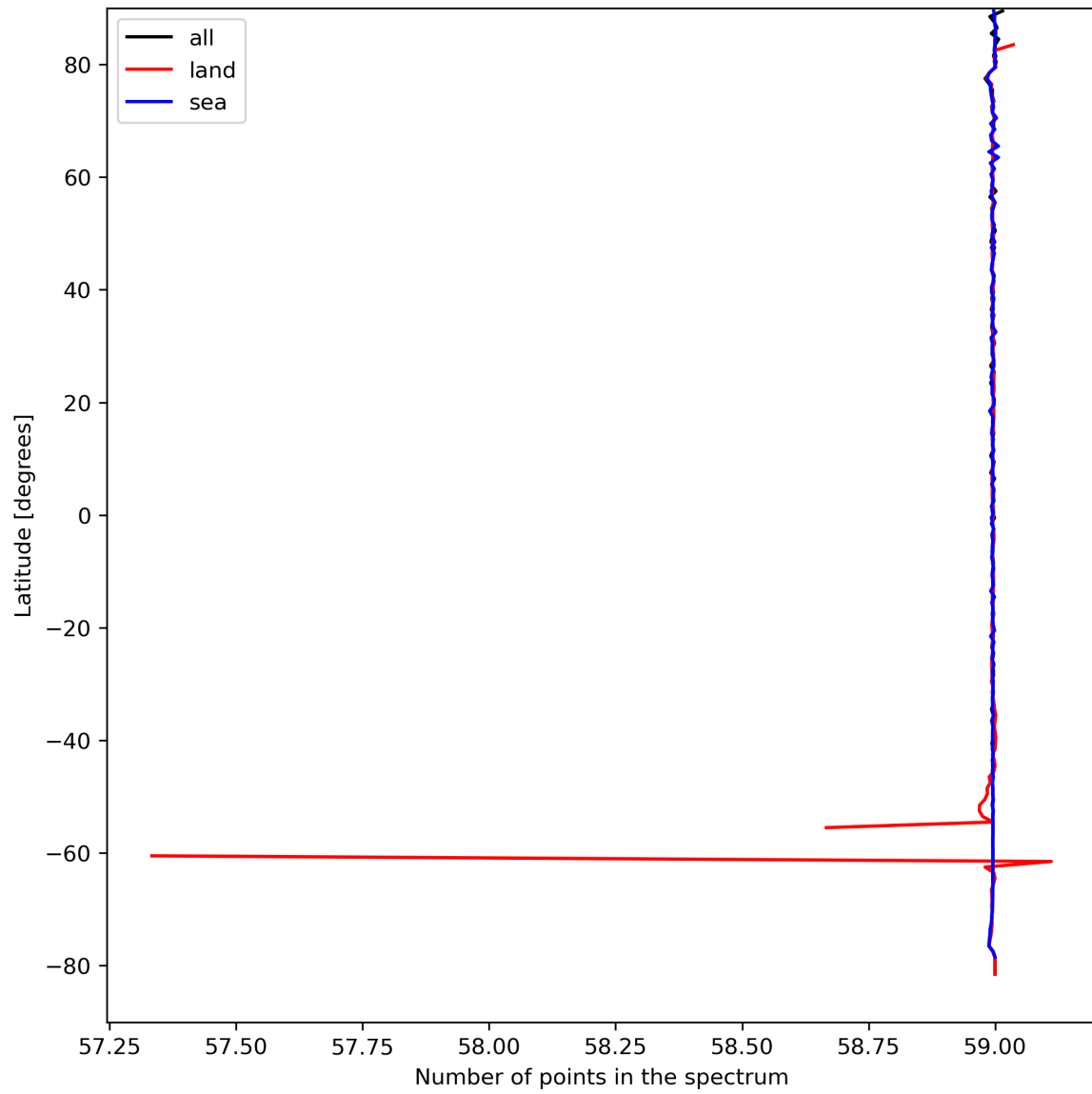
Figure 27: Zonal average of “Number of points in the spectrum” for 2024-04-05 to 2024-04-07.
