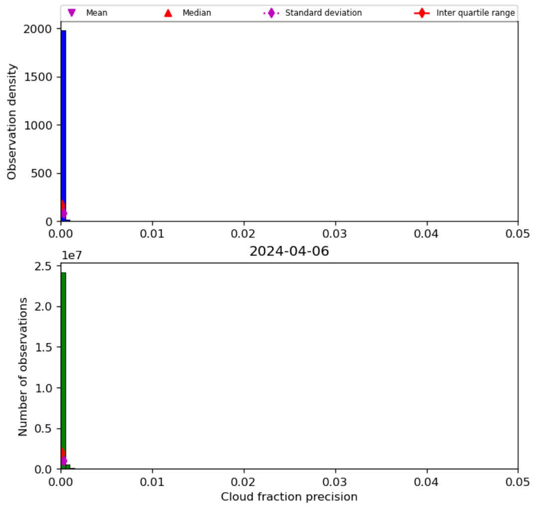
Figure 33: Histogram of “Cloud fraction precision” for 2024-04-05 to 2024-04-07
