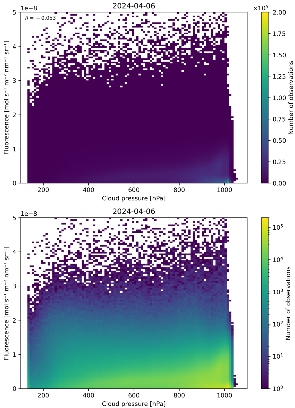
Figure 80: Scatter density plot of “Cloud pressure” against “Fluorescence” for 2024-04-05 to 2024-04-07.
