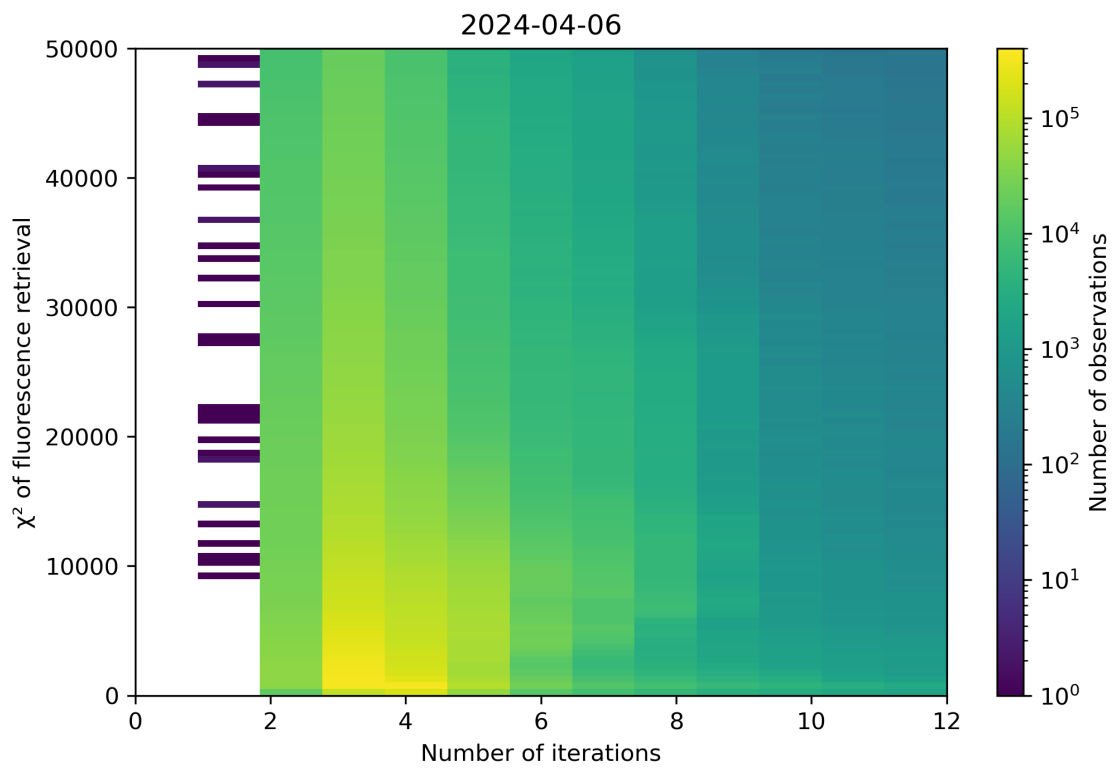
Figure 97: Scatter density plot of “Number of iterations” against “ \chi^2 of fluorescence retrieval” for 2024-04-05 to 2024-04-07.
