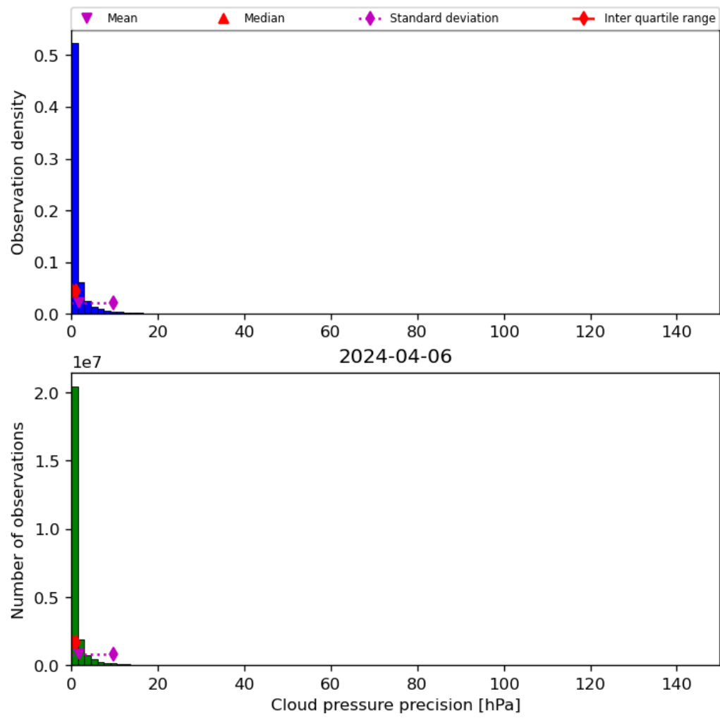
Figure 31: Histogram of “Cloud pressure precision” for 2024-04-05 to 2024-04-07
