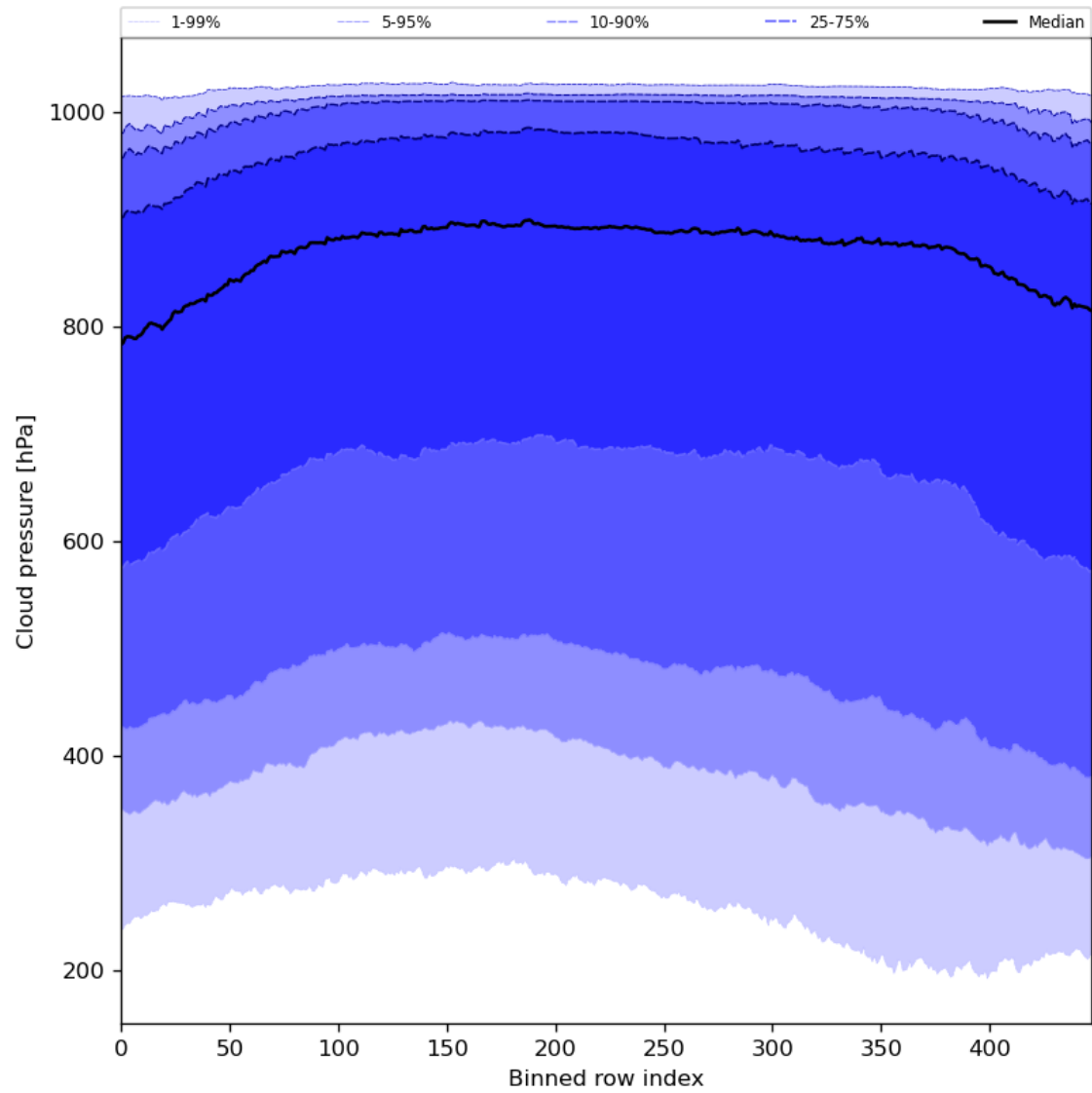
Figure 47: Along track statistics of “Cloud pressure” for 2024-04-05 to 2024-04-07
