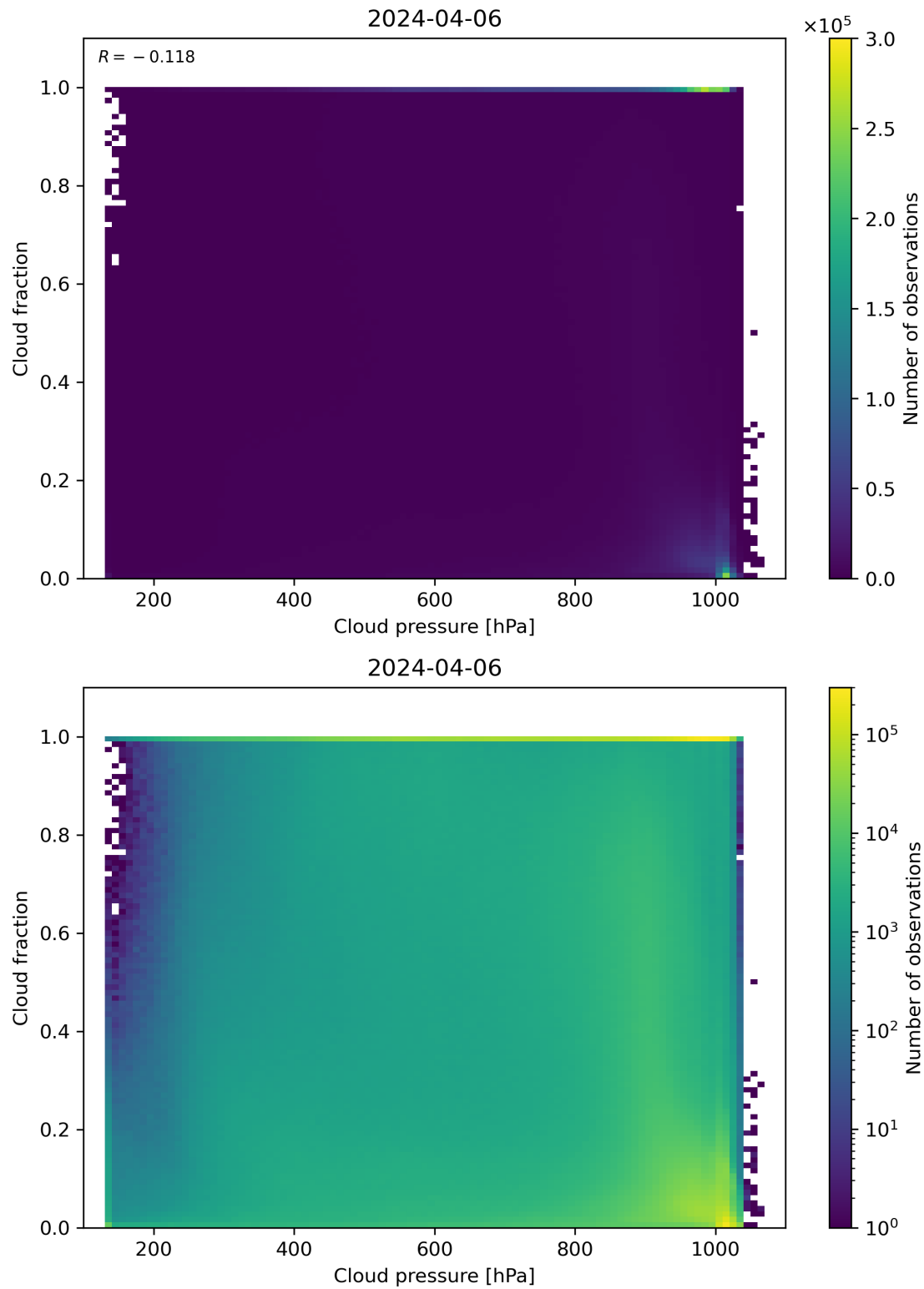
Figure 79: Scatter density plot of “Cloud pressure” against “Cloud fraction” for 2024-04-05 to 2024-04-07.
