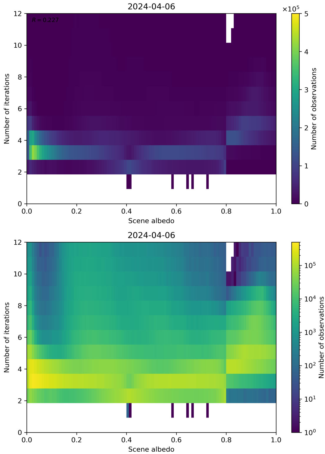
Figure 105: Scatter density plot of “Scene albedo” against “Number of iterations” for 2024-04-05 to 2024-04-07.
