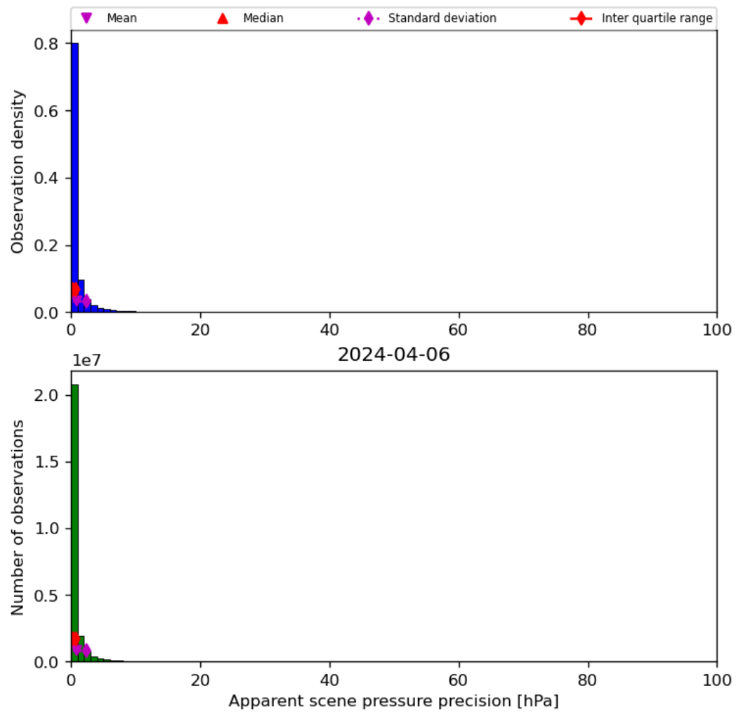
Figure 37: Histogram of “Apparent scene pressure precision” for 2024-04-05 to 2024-04-07
