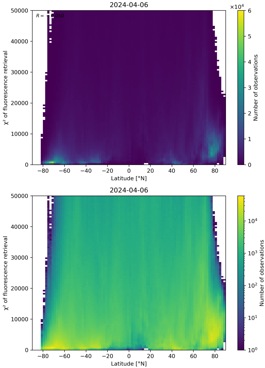
Figure 89: Scatter density plot of “Latitude” against “ \chi^2 of fluorescence retrieval” for 2024-04-05 to 2024-04-07.
