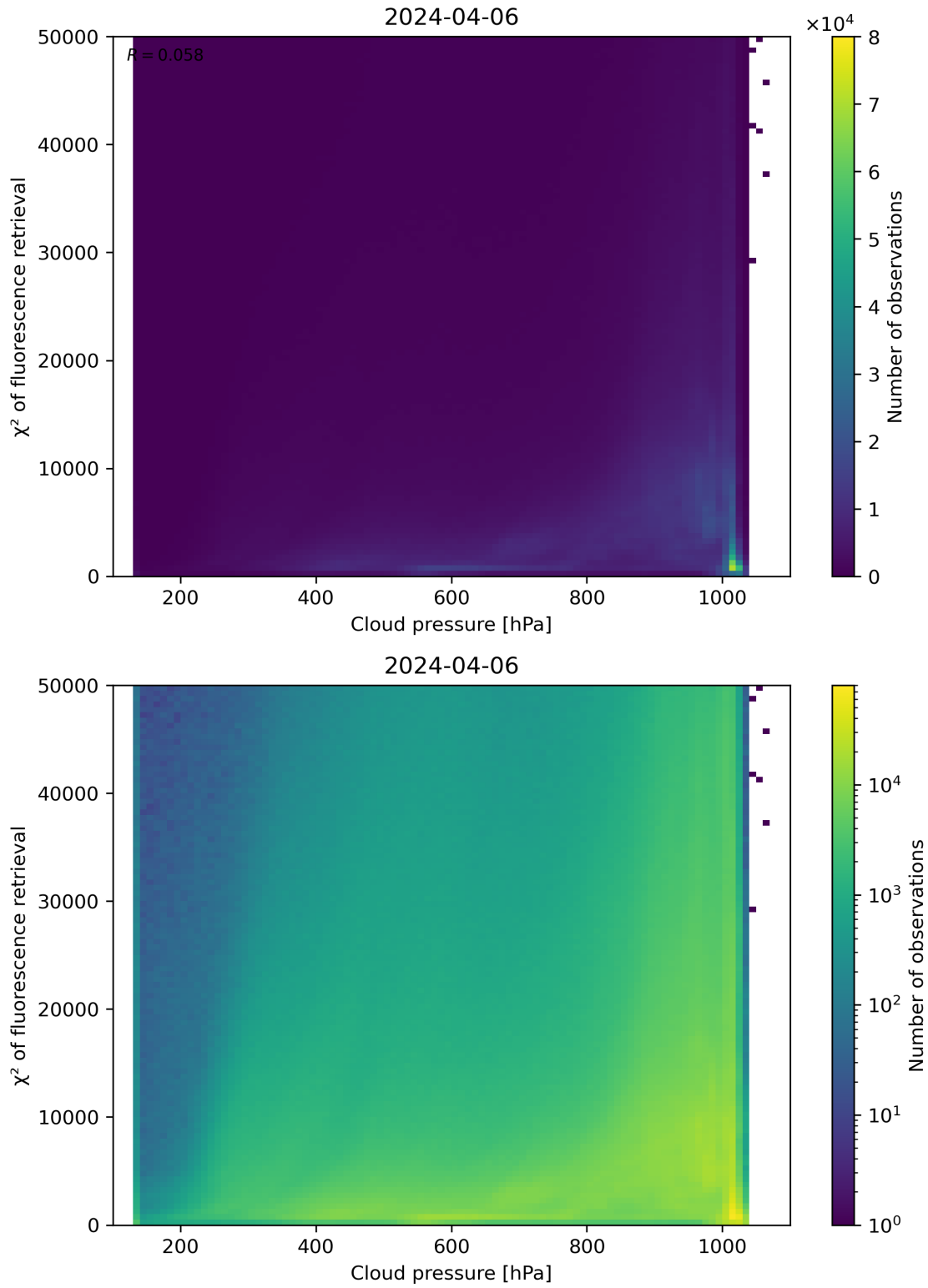
Figure 78: Scatter density plot of “Cloud pressure” against “ \chi^2 of fluorescence retrieval” for 2024-04-05 to 2024-04-07.
