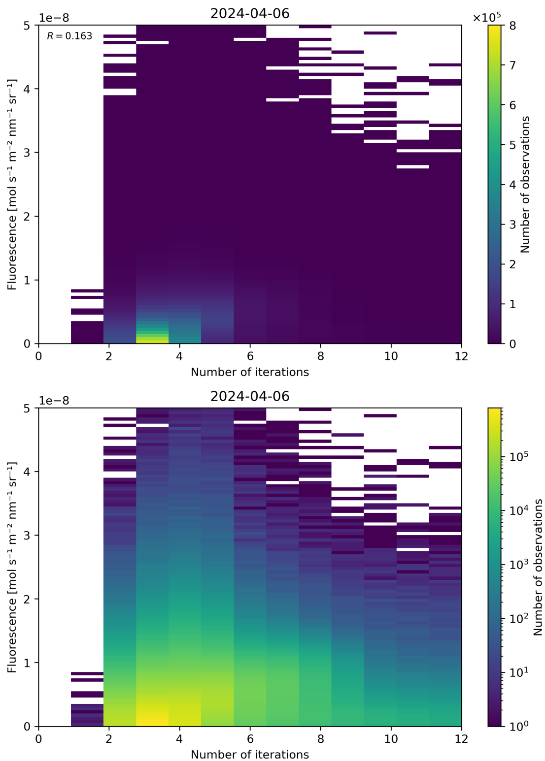
Figure 98: Scatter density plot of “Number of iterations” against “Fluorescence” for 2024-04-05 to 2024-04-07.
