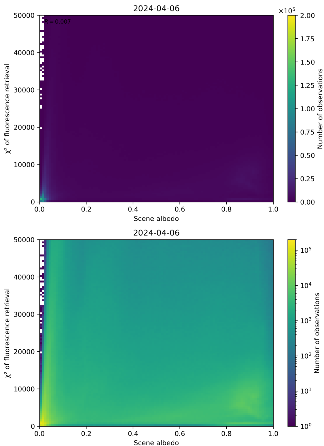
Figure 103: Scatter density plot of “Scene albedo” against “ \chi^2 of fluorescence retrieval” for 2024-04-05 to 2024-04-07.
