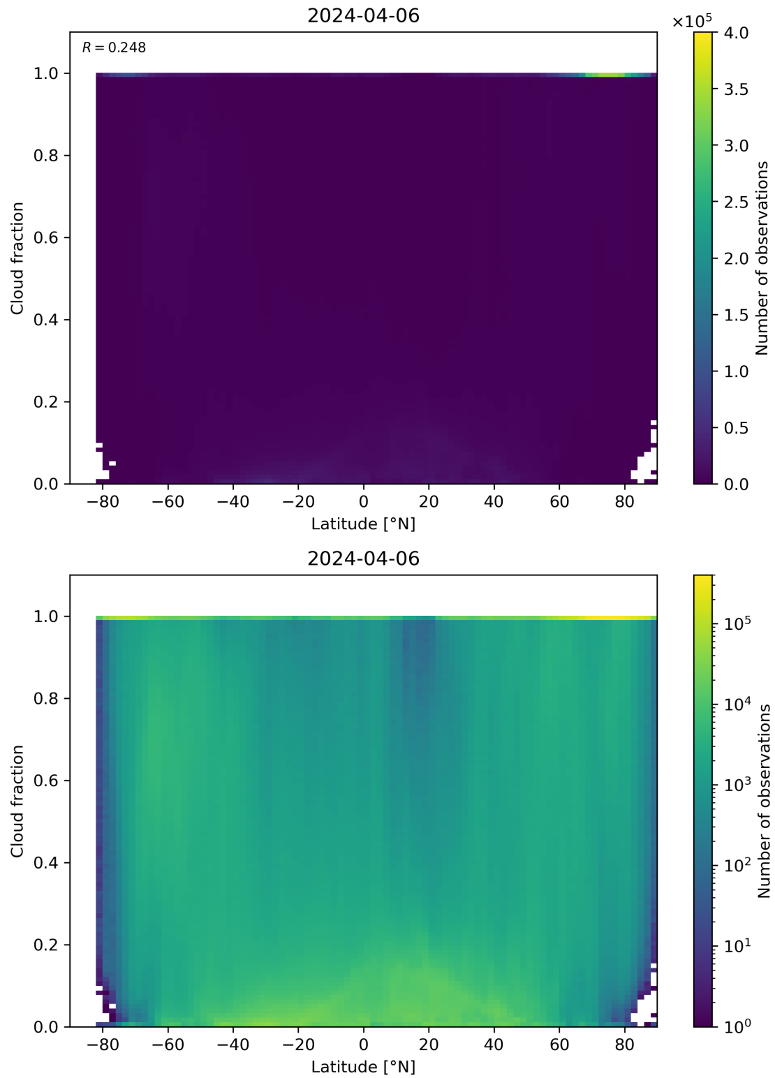
Figure 90: Scatter density plot of “Latitude” against “Cloud fraction” for 2024-04-05 to 2024-04-07.
