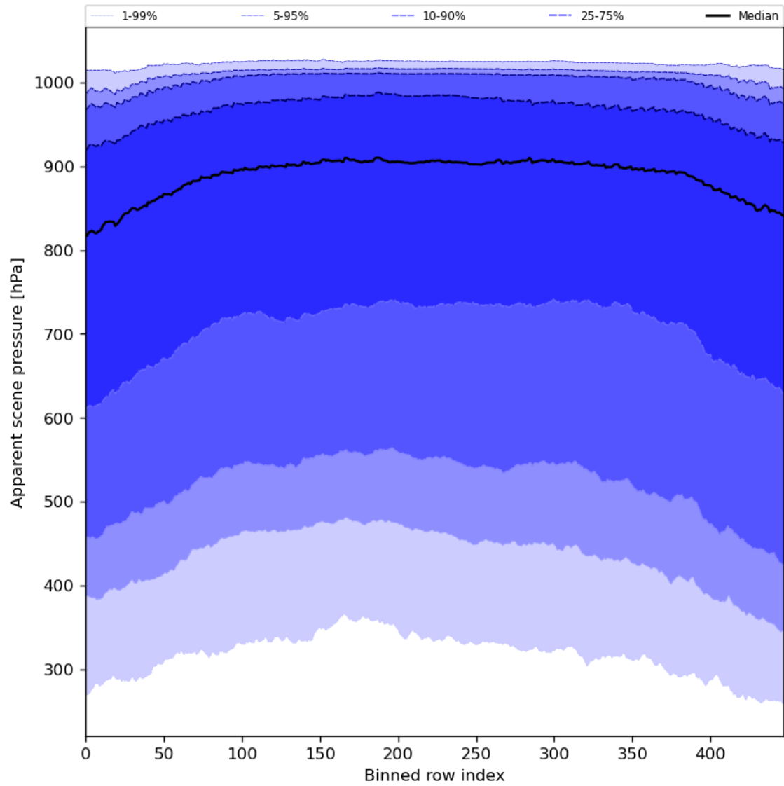
Figure 53: Along track statistics of “Apparent scene pressure” for 2024-04-05 to 2024-04-07
