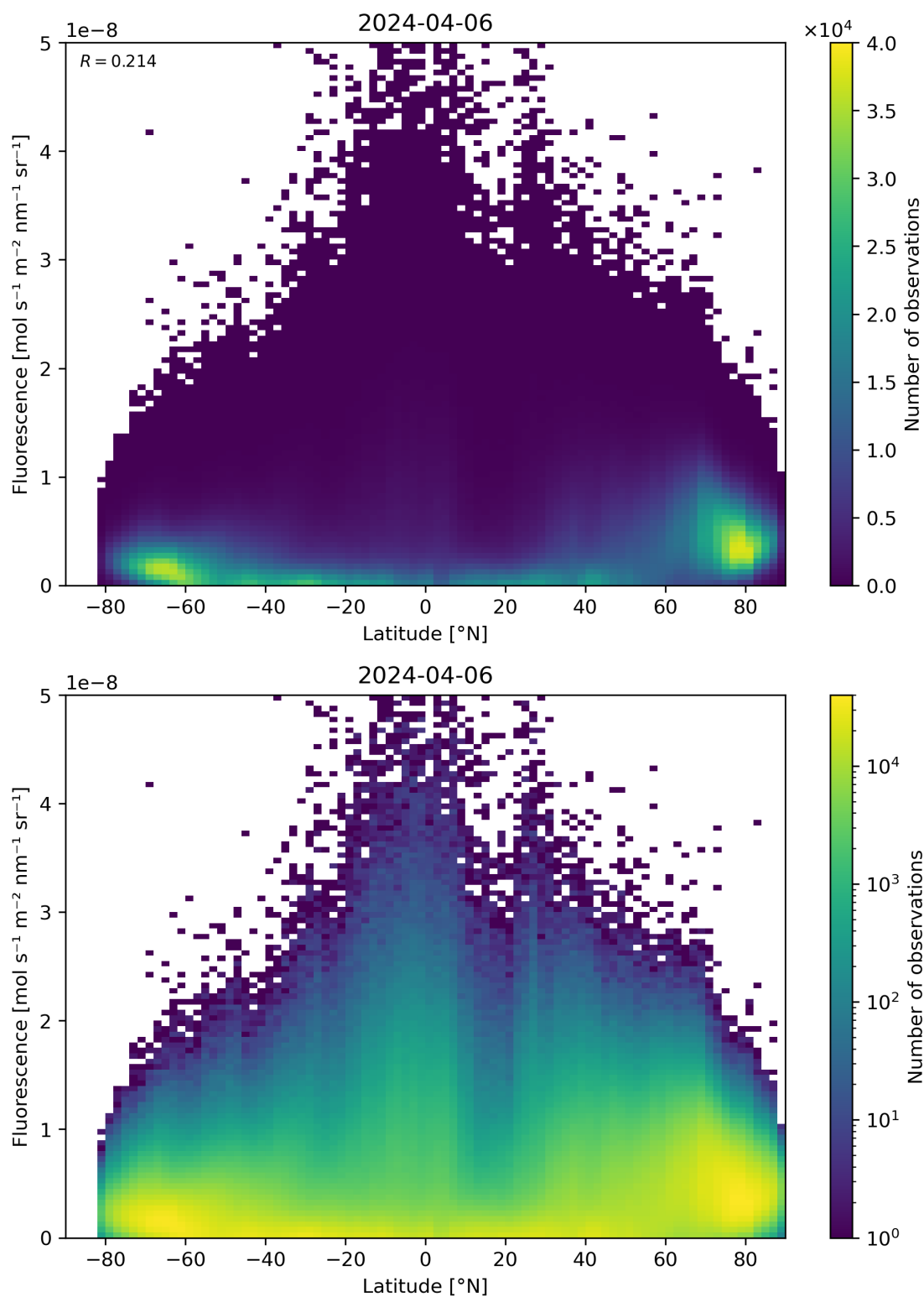
Figure 92: Scatter density plot of “Latitude” against “Fluorescence” for 2024-04-05 to 2024-04-07.
