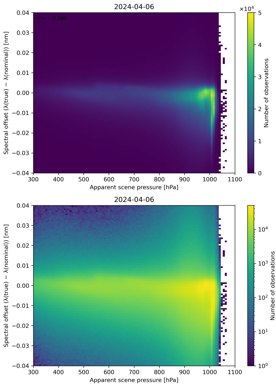
Figure 67: Scatter density plot of “Apparent scene pressure” against “Spectral offset ( \lambda(\text{true}) - \lambda(\text{nominal}) )” for 2024-04-05 to 2024-04-07.
