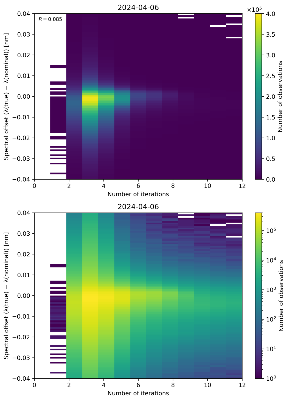
Figure 100: Scatter density plot of “Number of iterations” against “Spectral offset ( \lambda(\text{true}) - \lambda(\text{nominal}) )” for 2024-04-05 to 2024-04-07.
