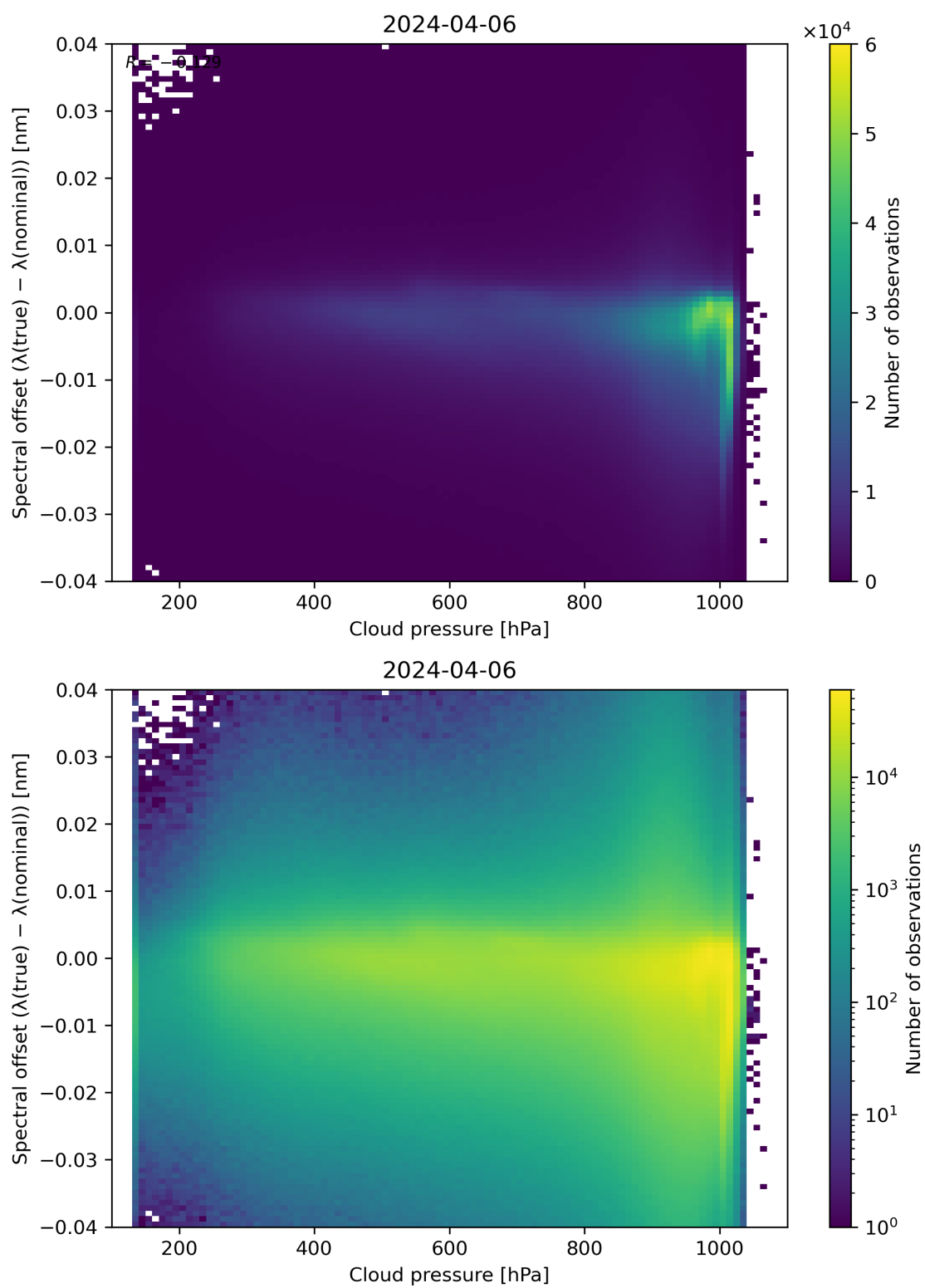
Figure 84: Scatter density plot of “Cloud pressure” against “Spectral offset ( \lambda(\text{true}) - \lambda(\text{nominal}) )” for 2024-04-05 to 2024-04-07.
