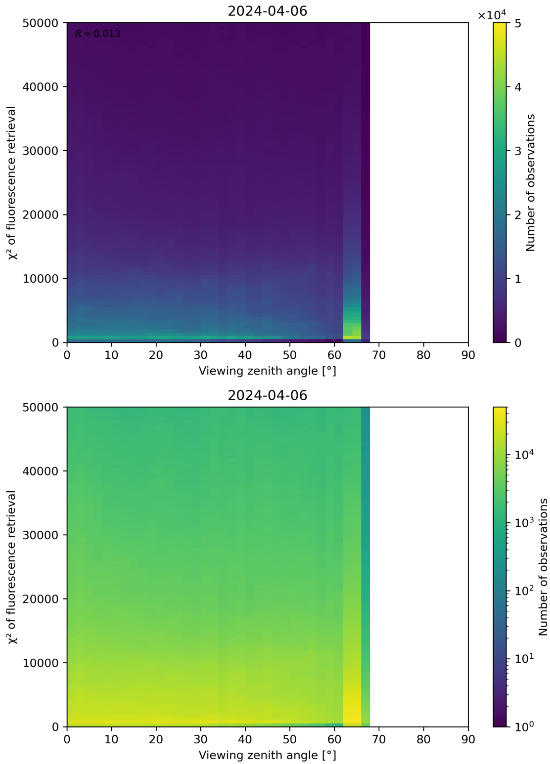
Figure 119: Scatter density plot of “Viewing zenith angle” against “ \chi^2 of fluorescence retrieval” for 2024-04-05 to 2024-04-07.
