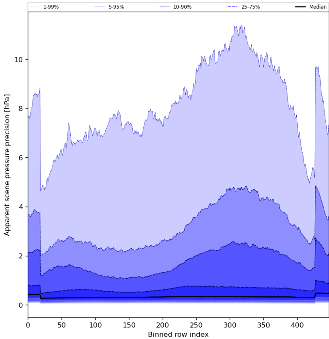
Figure 54: Along track statistics of “Apparent scene pressure precision” for 2024-04-05 to 2024-04-07
