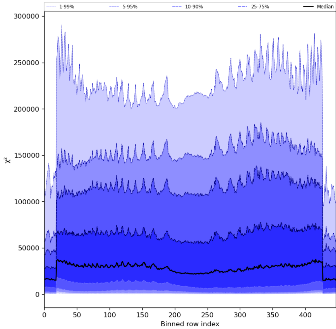
Figure 55: Along track statistics of “ \chi^2 ” for 2024-04-05 to 2024-04-07
