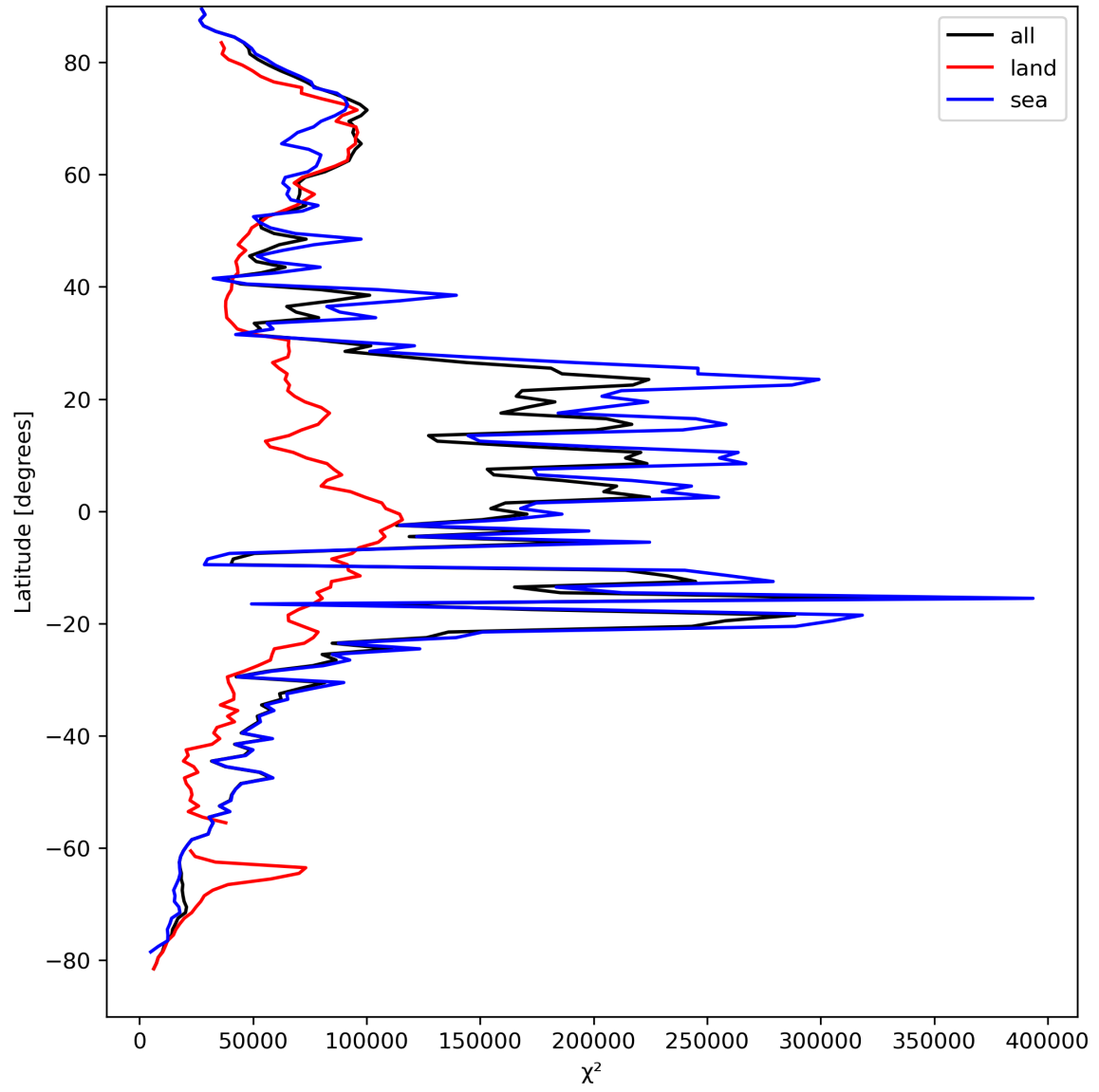
Figure 21: Zonal average of “ \chi^2 ” for 2024-04-05 to 2024-04-07.
