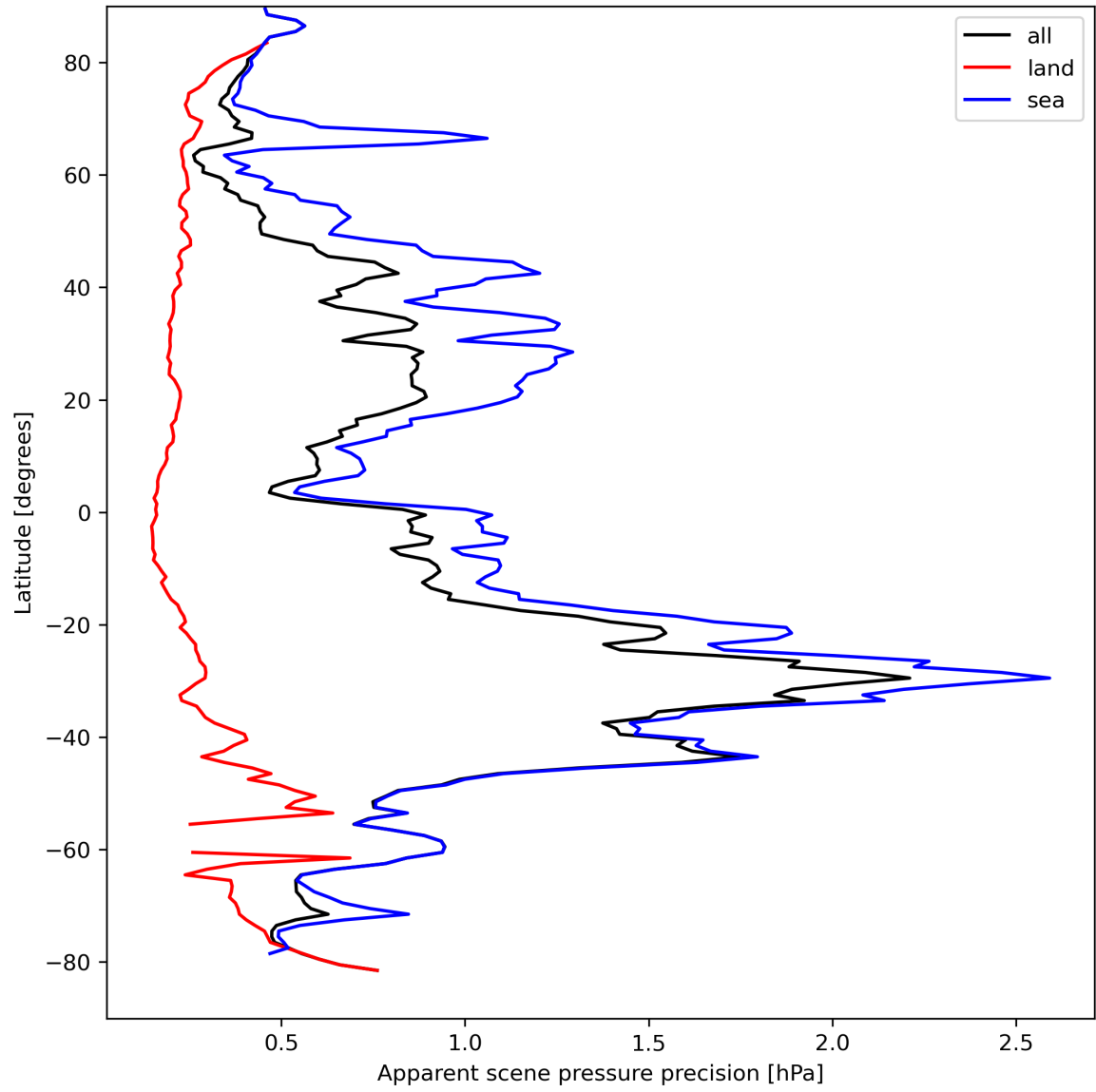
Figure 20: Zonal average of “Apparent scene pressure precision” for 2024-04-05 to 2024-04-07.
