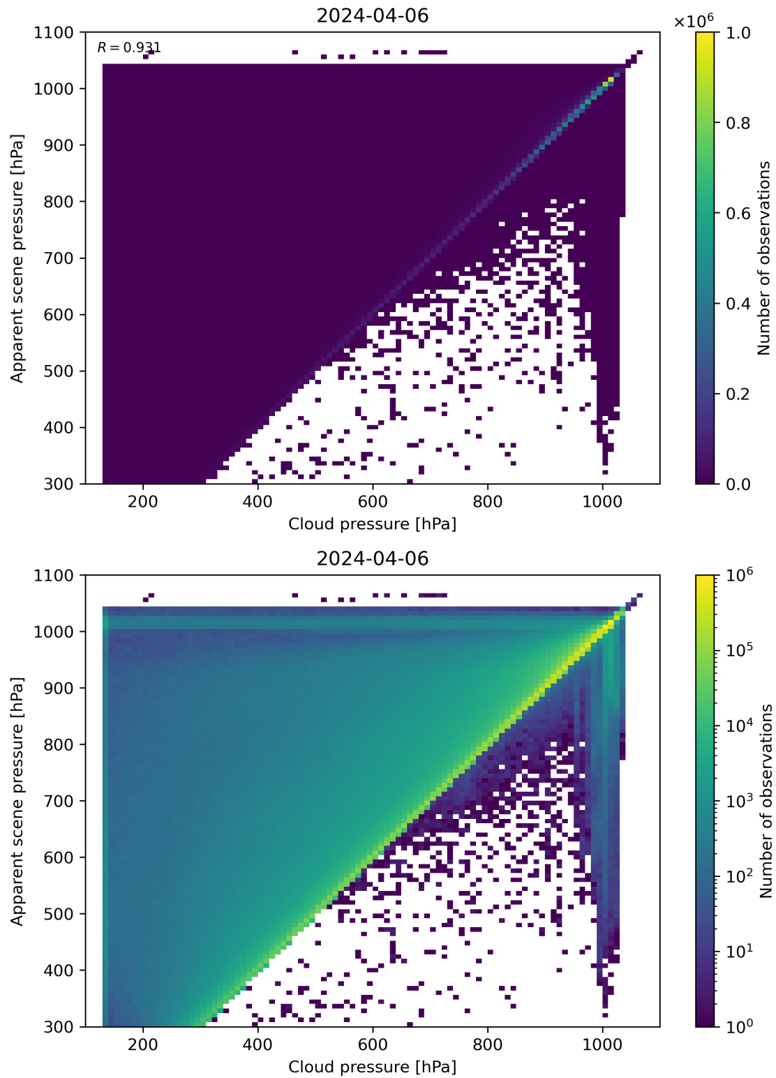
Figure 77: Scatter density plot of “Cloud pressure” against “Apparent scene pressure” for 2024-04-05 to 2024-04-07.
