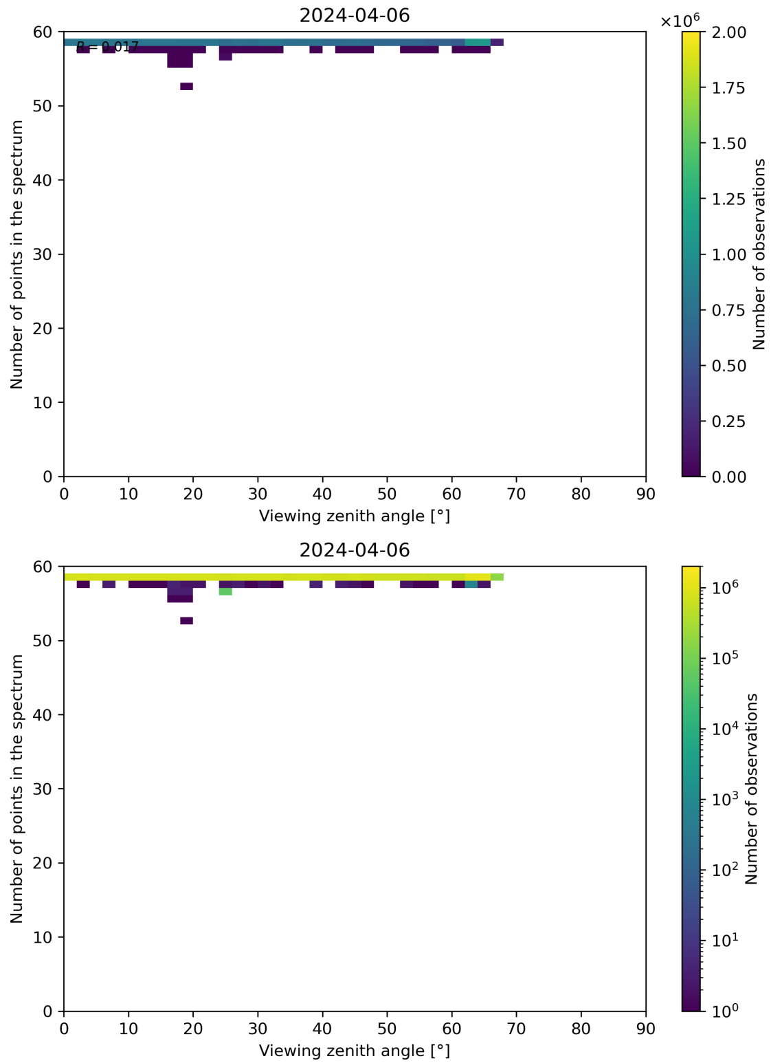
Figure 125: Scatter density plot of “Viewing zenith angle” against “Number of points in the spectrum” for 2024-04-05 to 2024-04-07.
