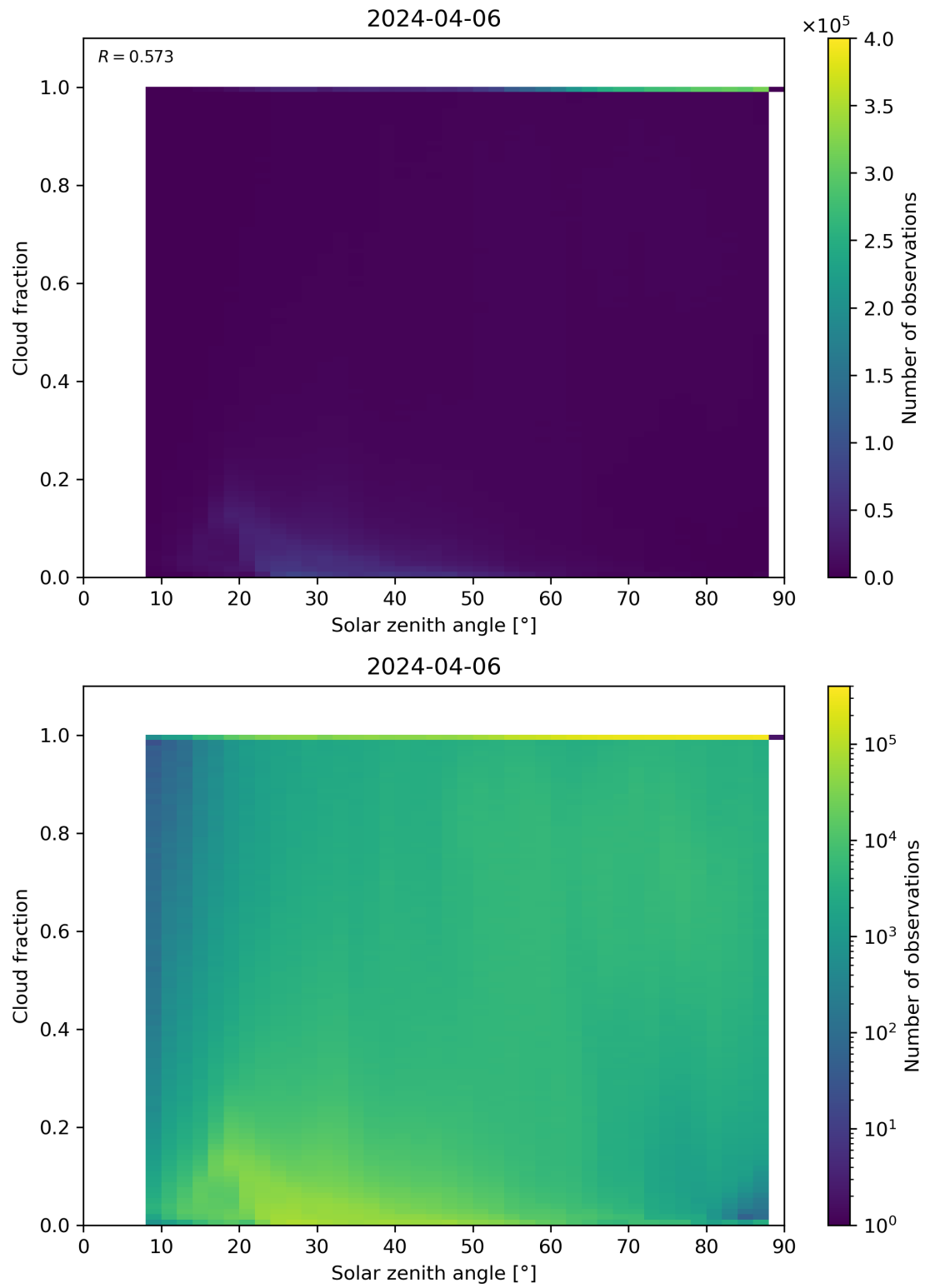
Figure 110: Scatter density plot of “Solar zenith angle” against “Cloud fraction” for 2024-04-05 to 2024-04-07.
