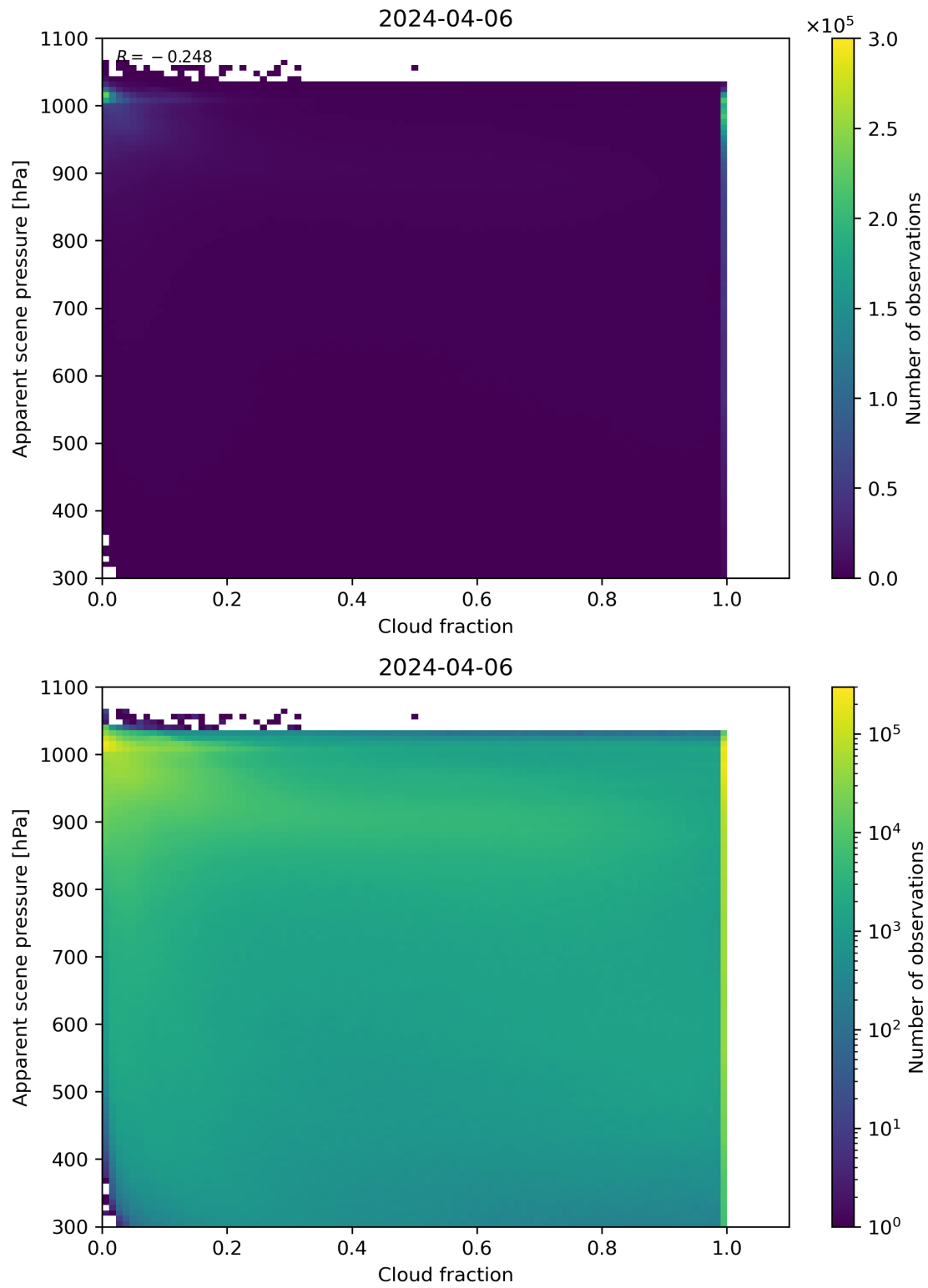
Figure 70: Scatter density plot of “Cloud fraction” against “Apparent scene pressure” for 2024-04-05 to 2024-04-07.
