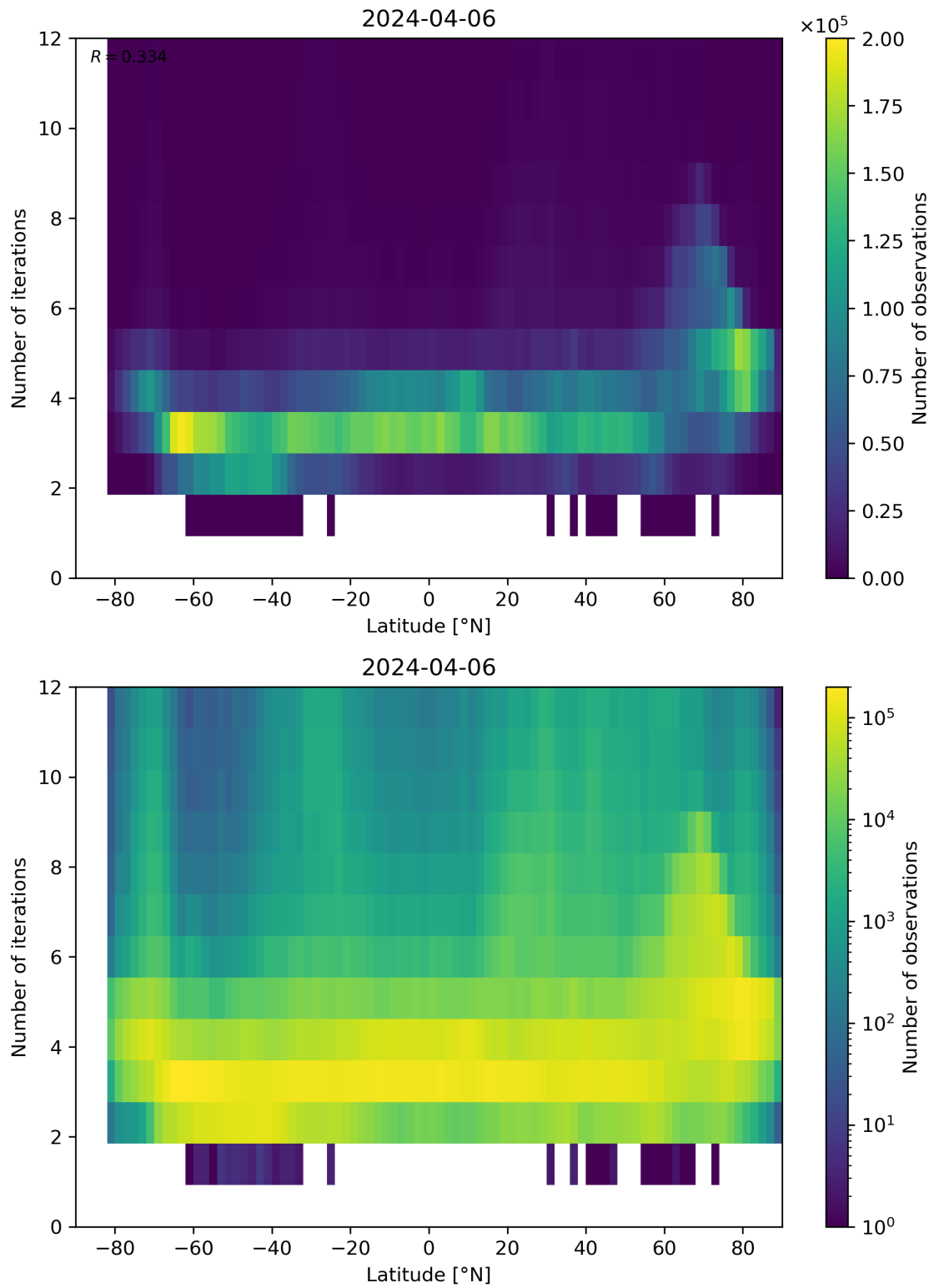
Figure 93: Scatter density plot of “Latitude” against “Number of iterations” for 2024-04-05 to 2024-04-07.
