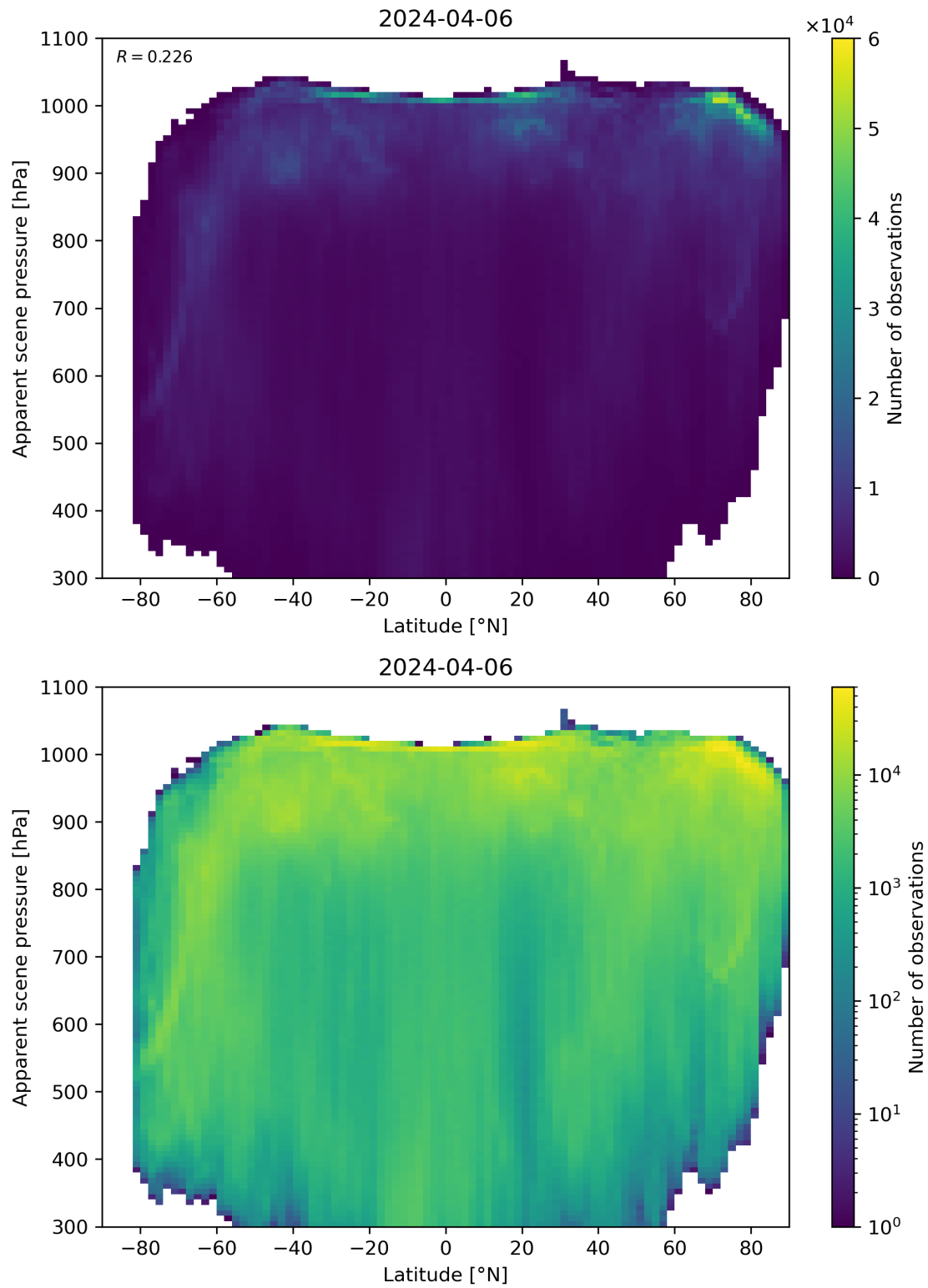
Figure 88: Scatter density plot of “Latitude” against “Apparent scene pressure” for 2024-04-05 to 2024-04-07.
