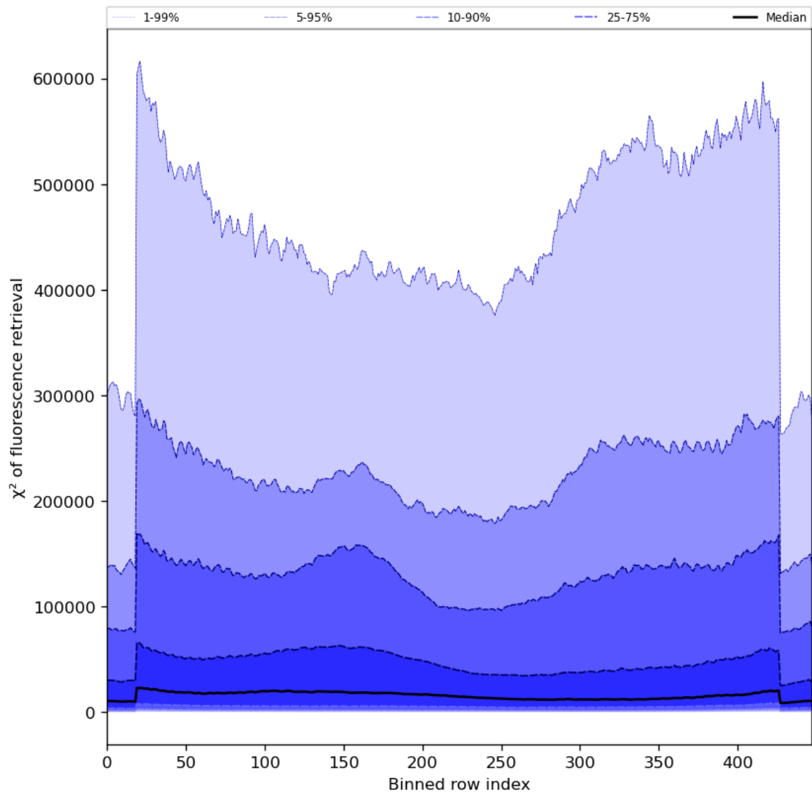
Figure 59: Along track statistics of “ \chi^2 of fluorescence retrieval” for 2024-04-05 to 2024-04-07
