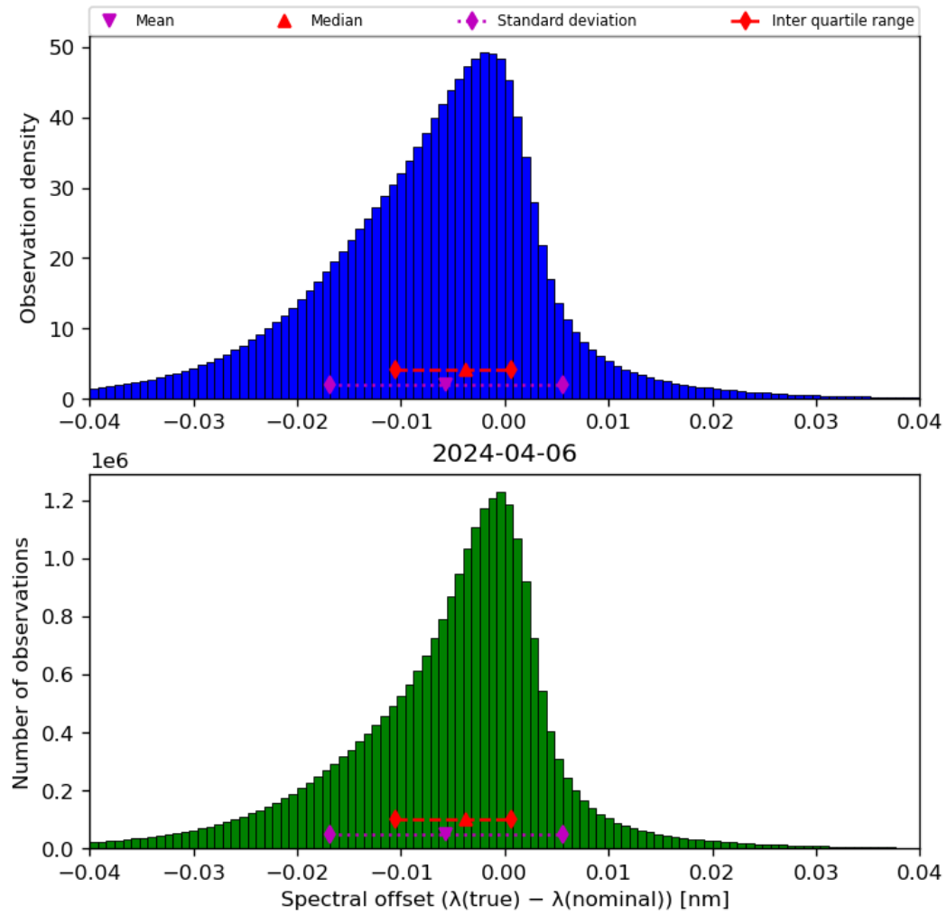
Figure 45: Histogram of “Spectral offset ( \lambda(\text{true}) - \lambda(\text{nominal}) )” for 2024-04-05 to 2024-04-07
