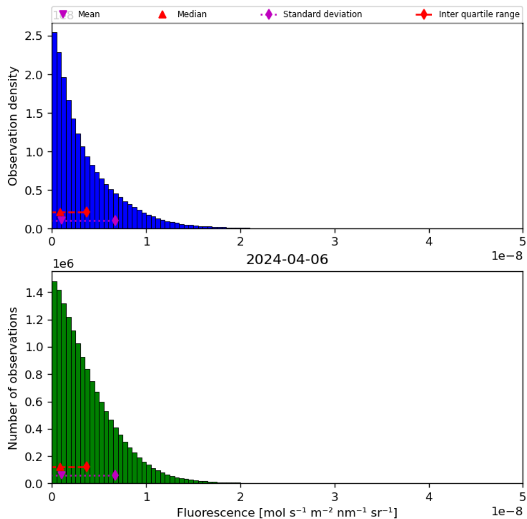
Figure 40: Histogram of “Fluorescence” for 2024-04-05 to 2024-04-07
