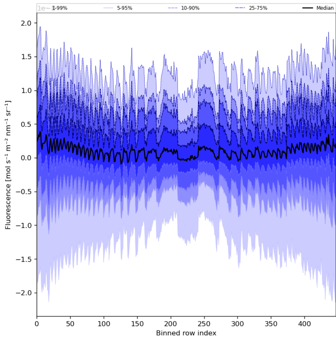
Figure 57: Along track statistics of “Fluorescence” for 2024-04-05 to 2024-04-07
