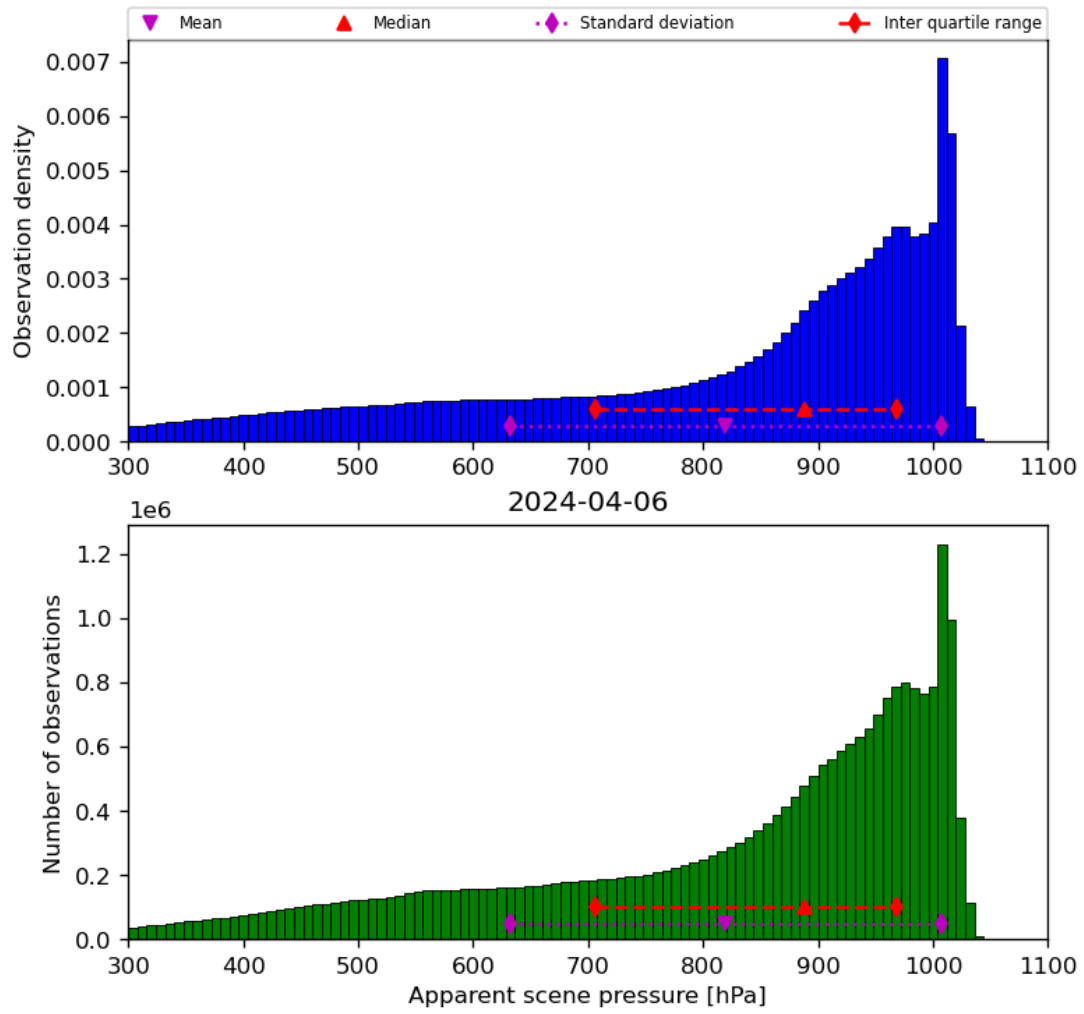
Figure 36: Histogram of “Apparent scene pressure” for 2024-04-05 to 2024-04-07
