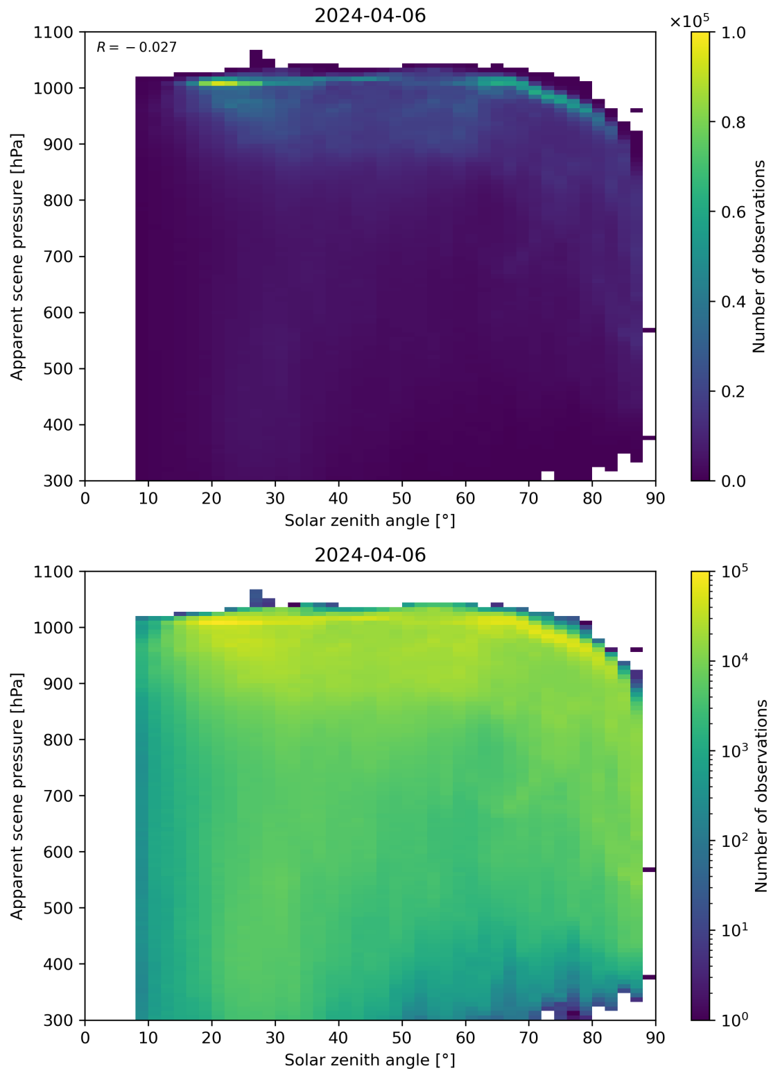
Figure 108: Scatter density plot of “Solar zenith angle” against “Apparent scene pressure” for 2024-04-05 to 2024-04-07.
