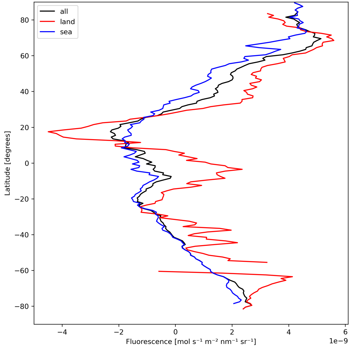
Figure 23: Zonal average of “Fluorescence” for 2024-04-05 to 2024-04-07.
