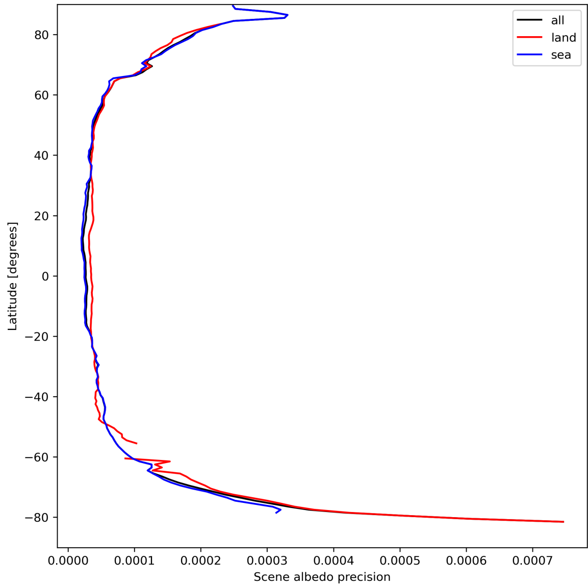
Figure 18: Zonal average of “Scene albedo precision” for 2024-04-05 to 2024-04-07.
