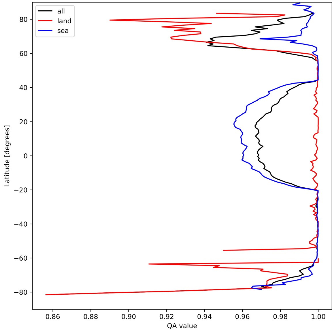
Figure 12: Zonal average of "QA value" for 2024-04-05 to 2024-04-07.
