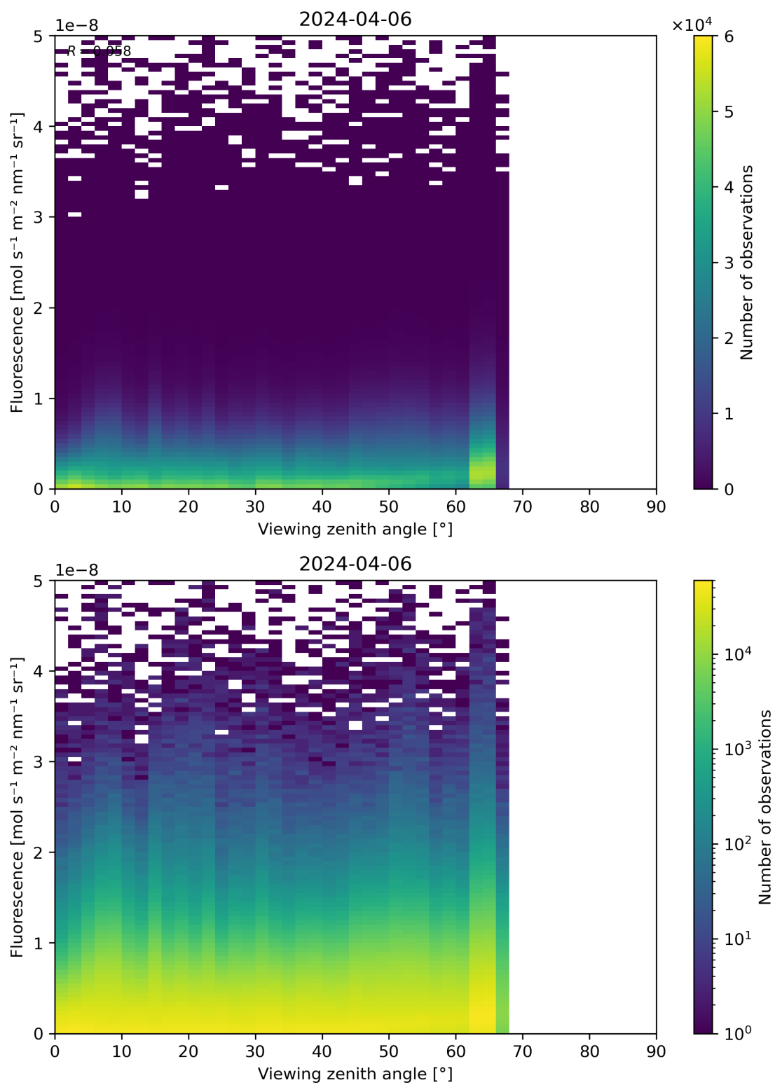
Figure 122: Scatter density plot of “Viewing zenith angle” against “Fluorescence” for 2024-04-05 to 2024-04-07.
