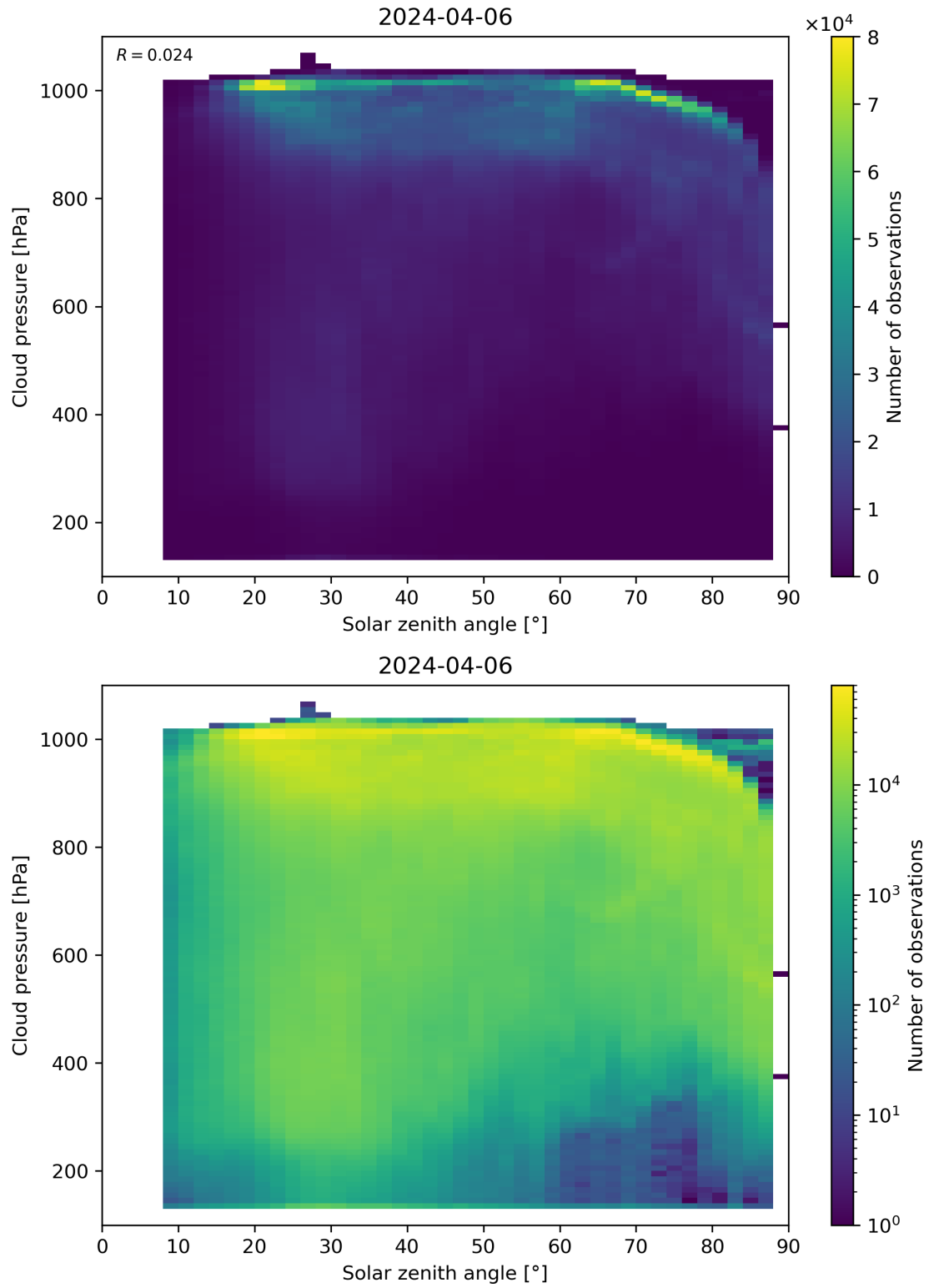
Figure 111: Scatter density plot of “Solar zenith angle” against “Cloud pressure” for 2024-04-05 to 2024-04-07.
