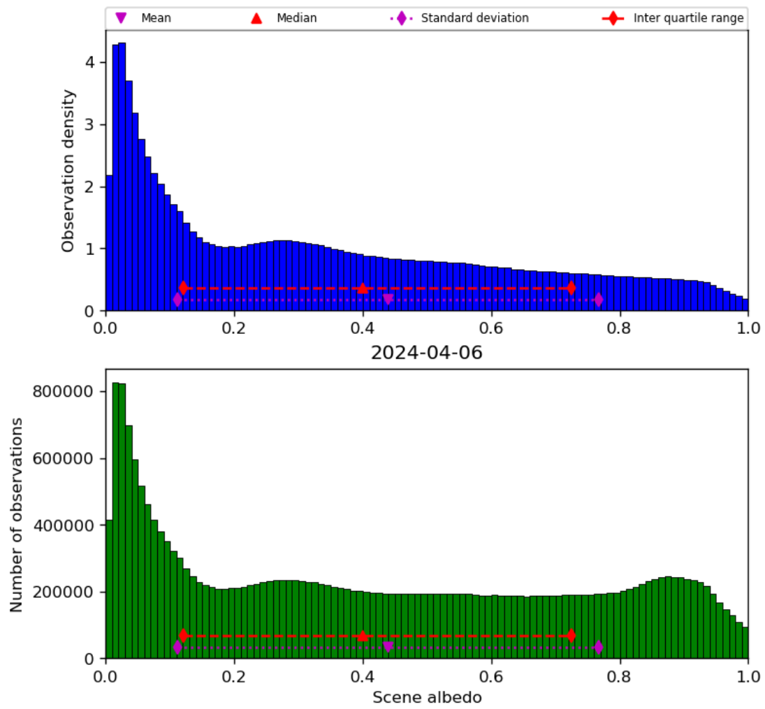
Figure 34: Histogram of “Scene albedo” for 2024-04-05 to 2024-04-07
