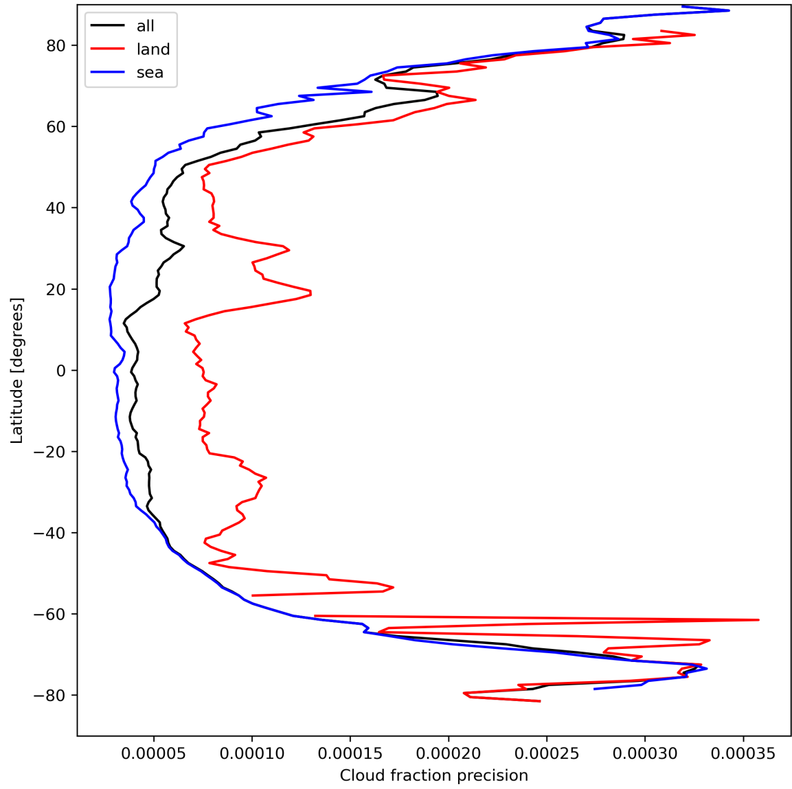
Figure 16: Zonal average of “Cloud fraction precision” for 2024-04-05 to 2024-04-07.
