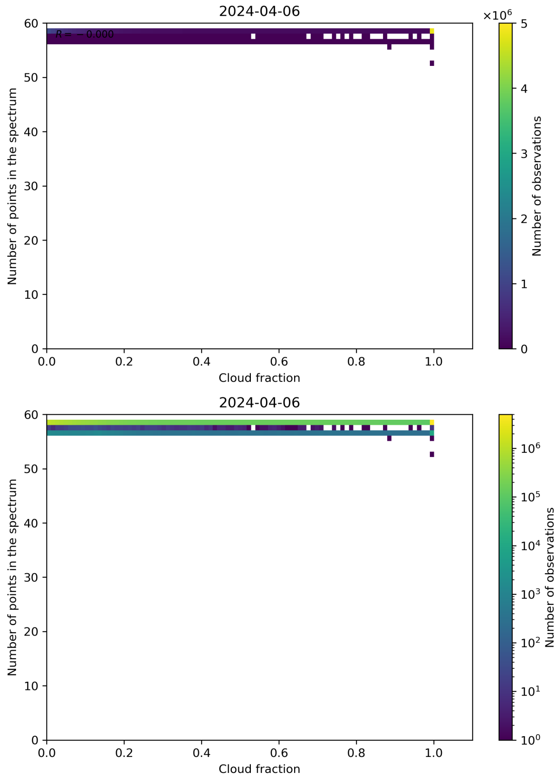
Figure 74: Scatter density plot of “Cloud fraction” against “Number of points in the spectrum” for 2024-04-05 to 2024-04-07.
