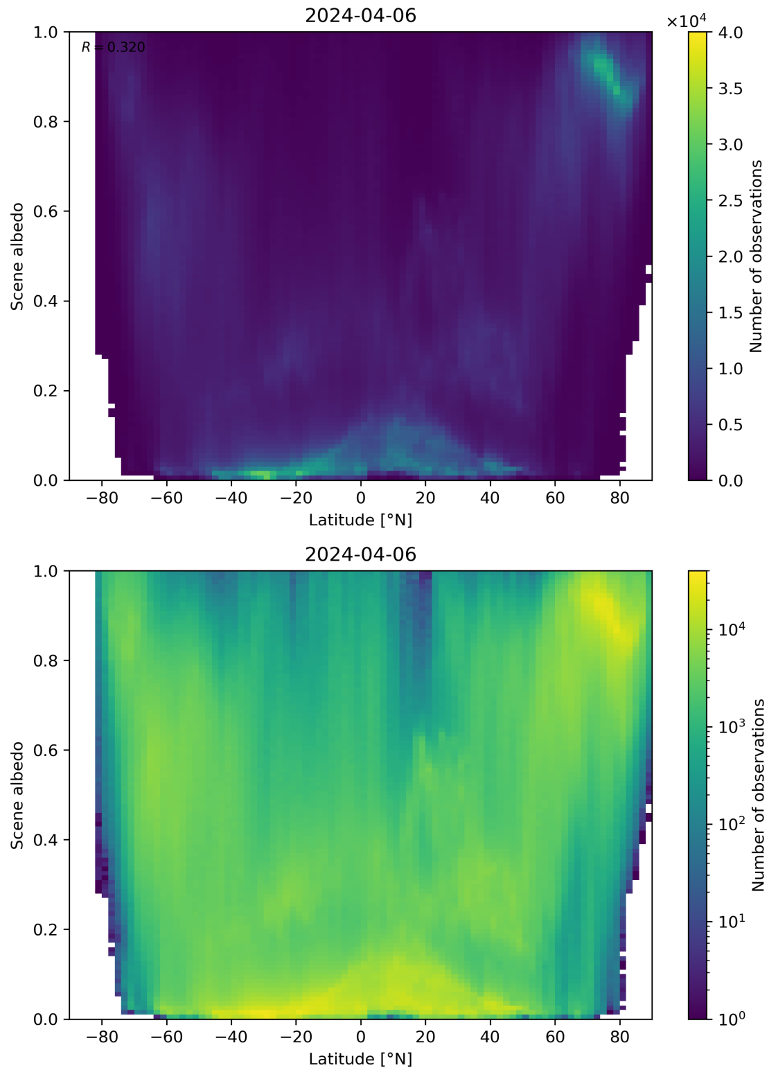
Figure 95: Scatter density plot of “Latitude” against “Scene albedo” for 2024-04-05 to 2024-04-07.
