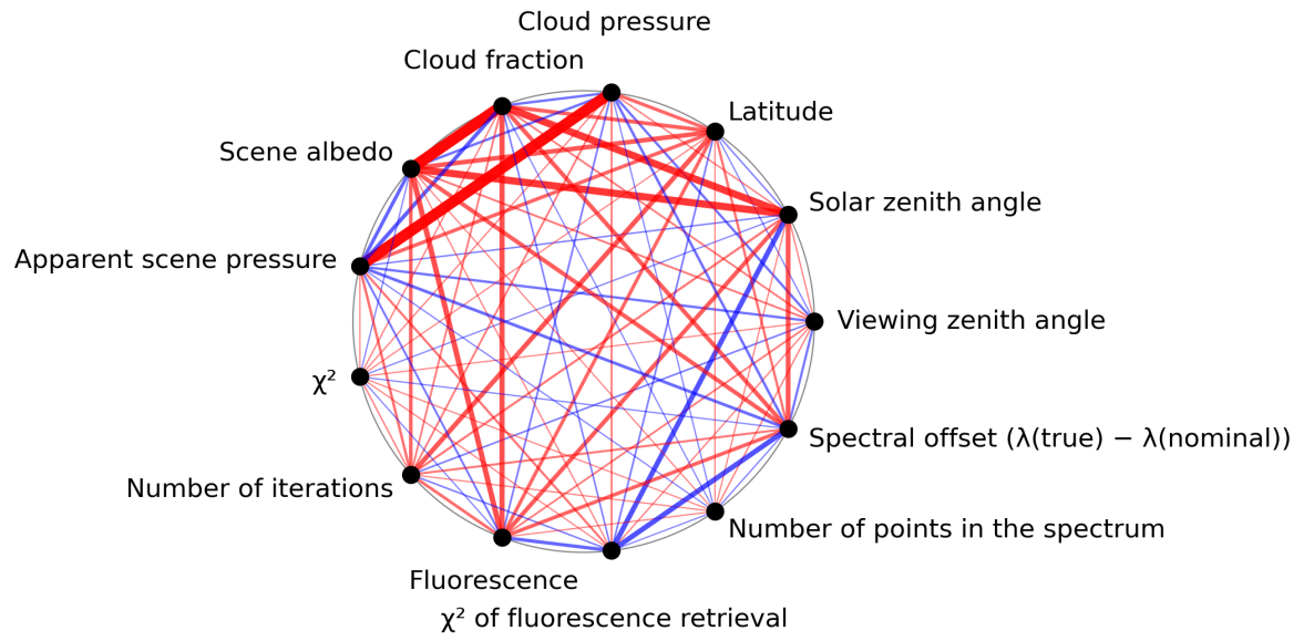
Figure 1: Map of correlation graph for 2024-04-05 to 2024-04-07.
