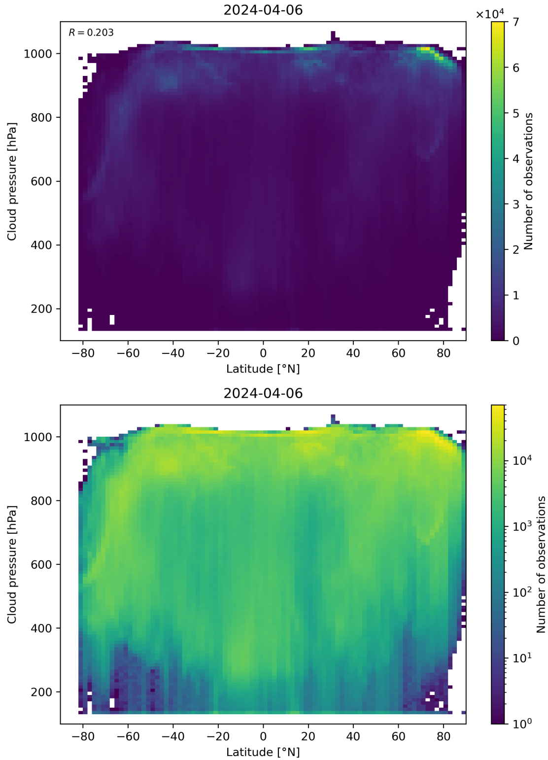
Figure 91: Scatter density plot of “Latitude” against “Cloud pressure” for 2024-04-05 to 2024-04-07.
