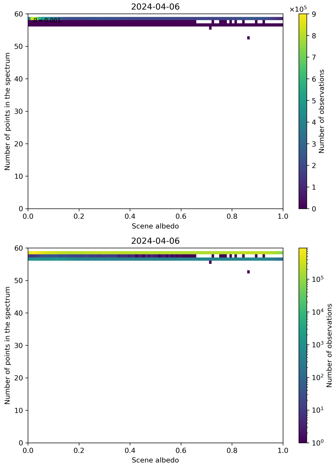
Figure 106: Scatter density plot of “Scene albedo” against “Number of points in the spectrum” for 2024-04-05 to 2024-04-07.
