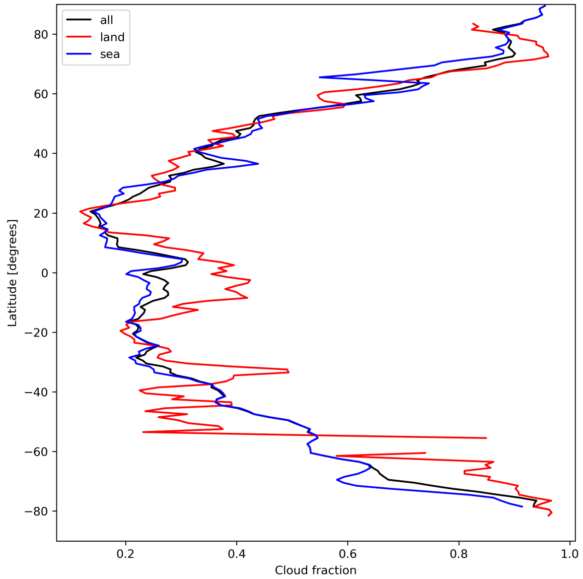
Figure 15: Zonal average of “Cloud fraction” for 2024-04-05 to 2024-04-07.
