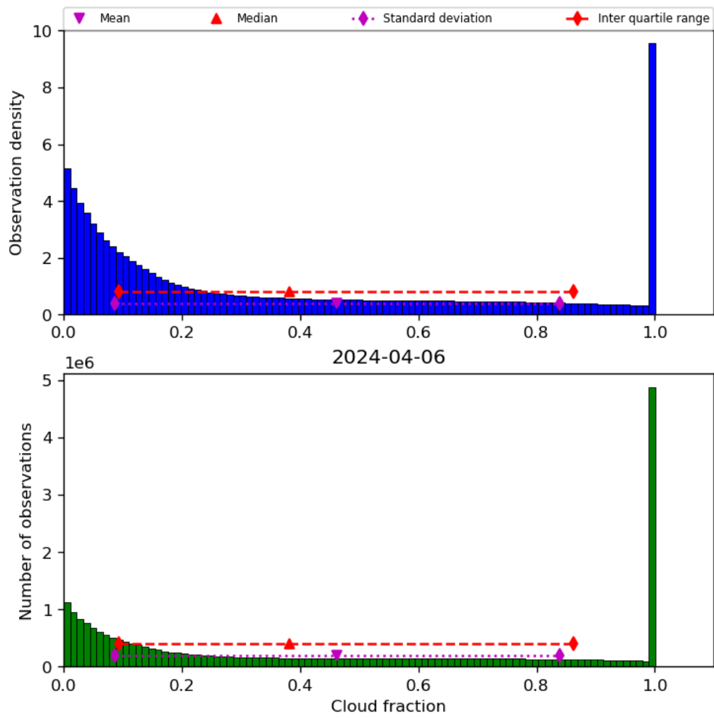
Figure 32: Histogram of “Cloud fraction” for 2024-04-05 to 2024-04-07
