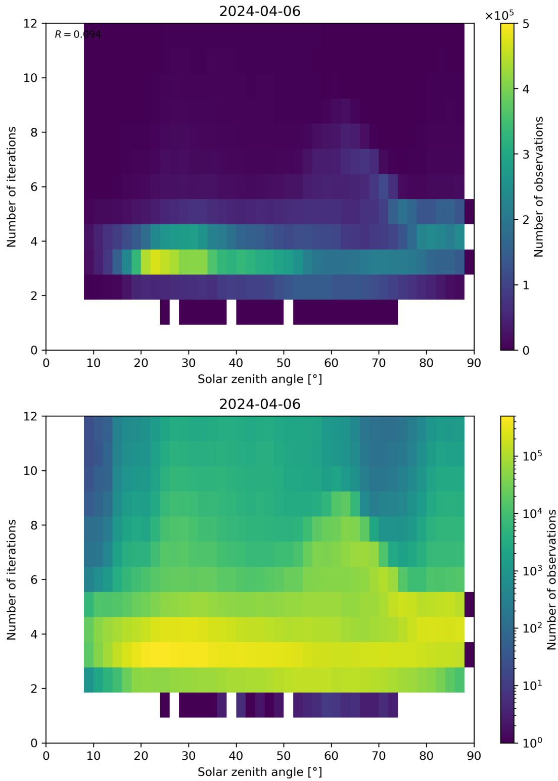
Figure 114: Scatter density plot of “Solar zenith angle” against “Number of iterations” for 2024-04-05 to 2024-04-07.
