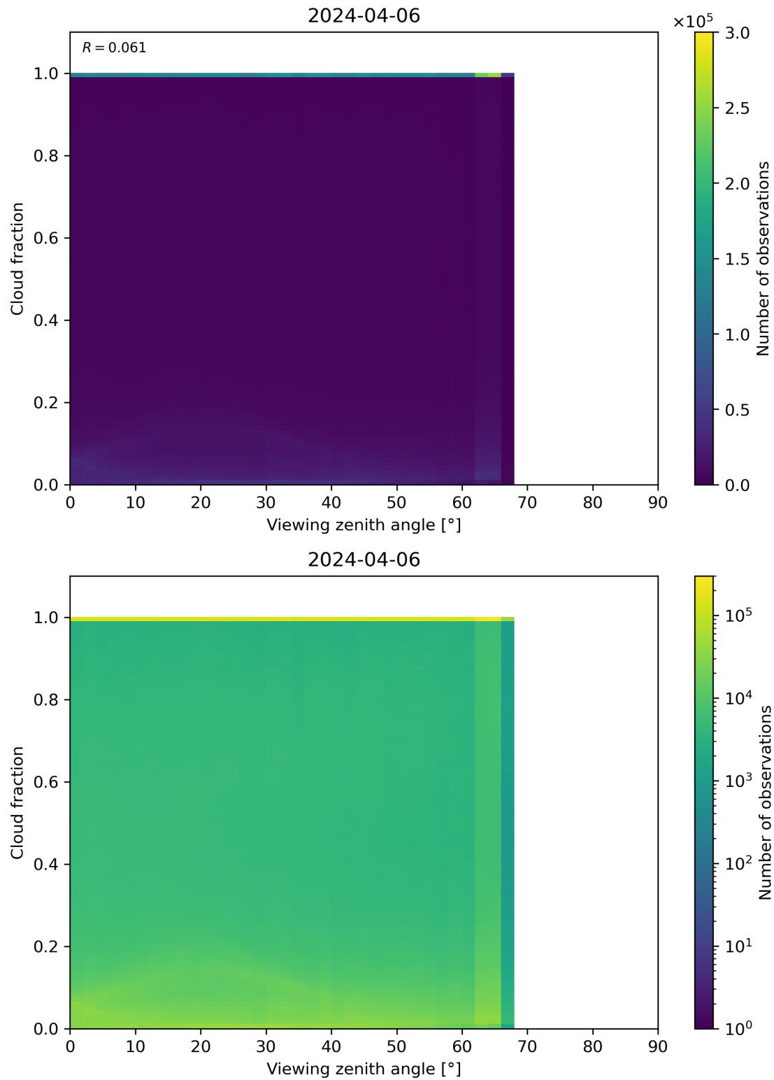
Figure 120: Scatter density plot of “Viewing zenith angle” against “Cloud fraction” for 2024-04-05 to 2024-04-07.
