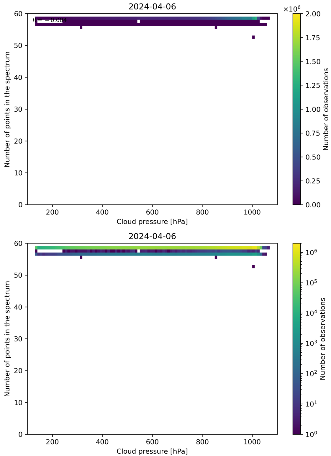
Figure 82: Scatter density plot of “Cloud pressure” against “Number of points in the spectrum” for 2024-04-05 to 2024-04-07.
