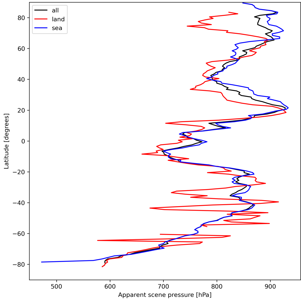
Figure 19: Zonal average of “Apparent scene pressure” for 2024-04-05 to 2024-04-07.
