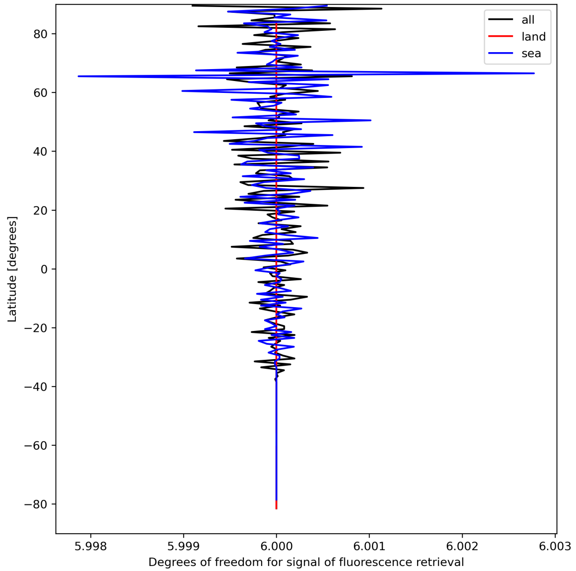
Figure 26: Zonal average of “Degrees of freedom for signal of fluorescence retrieval” for 2024-04-05 to 2024-04-07.
