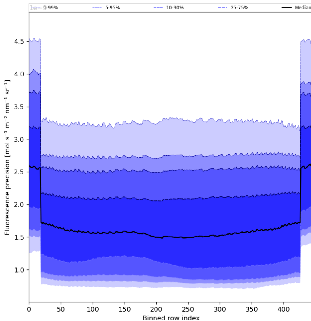
Figure 58: Along track statistics of “Fluorescence precision” for 2024-04-05 to 2024-04-07
