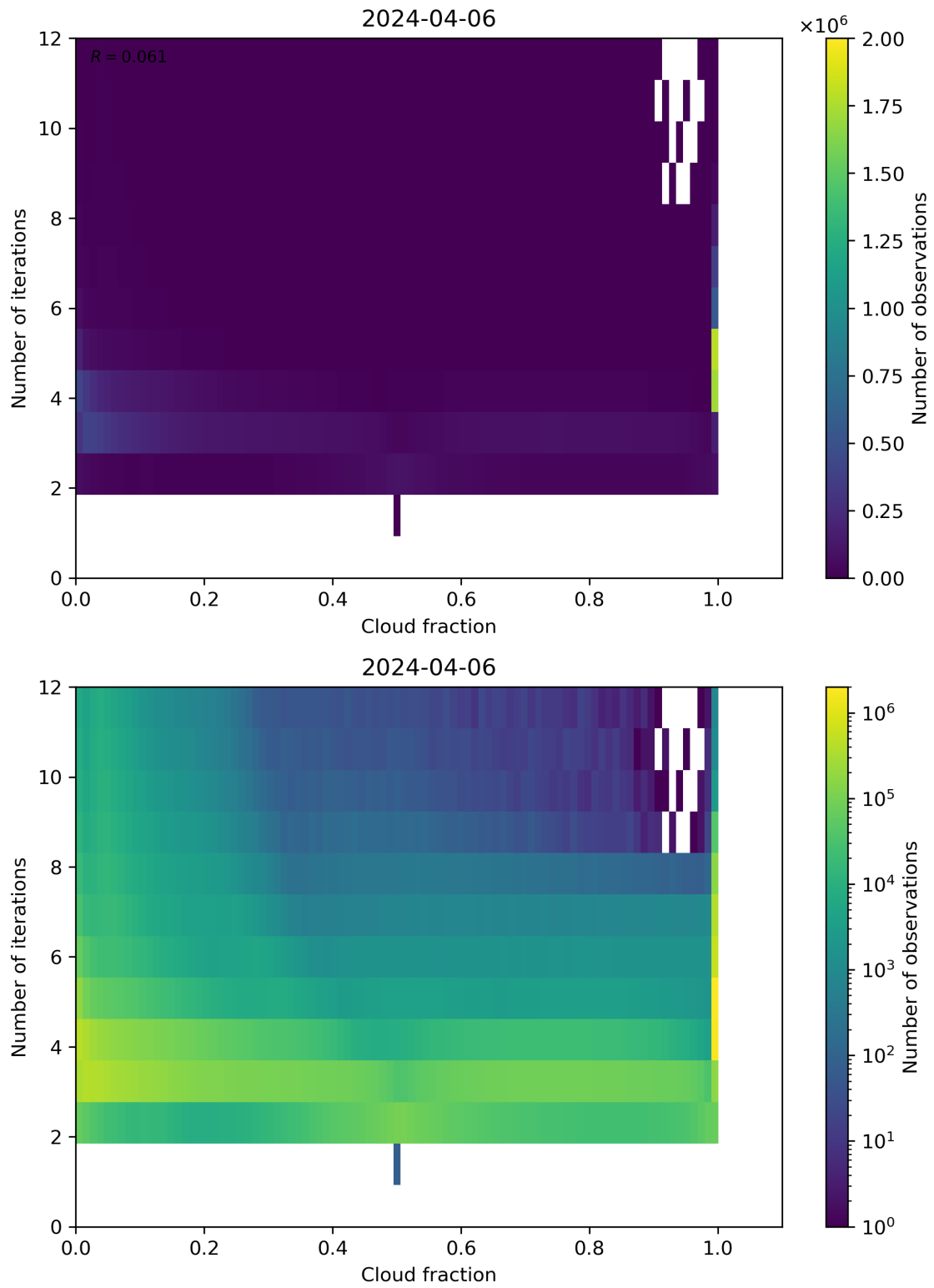
Figure 73: Scatter density plot of “Cloud fraction” against “Number of iterations” for 2024-04-05 to 2024-04-07.
