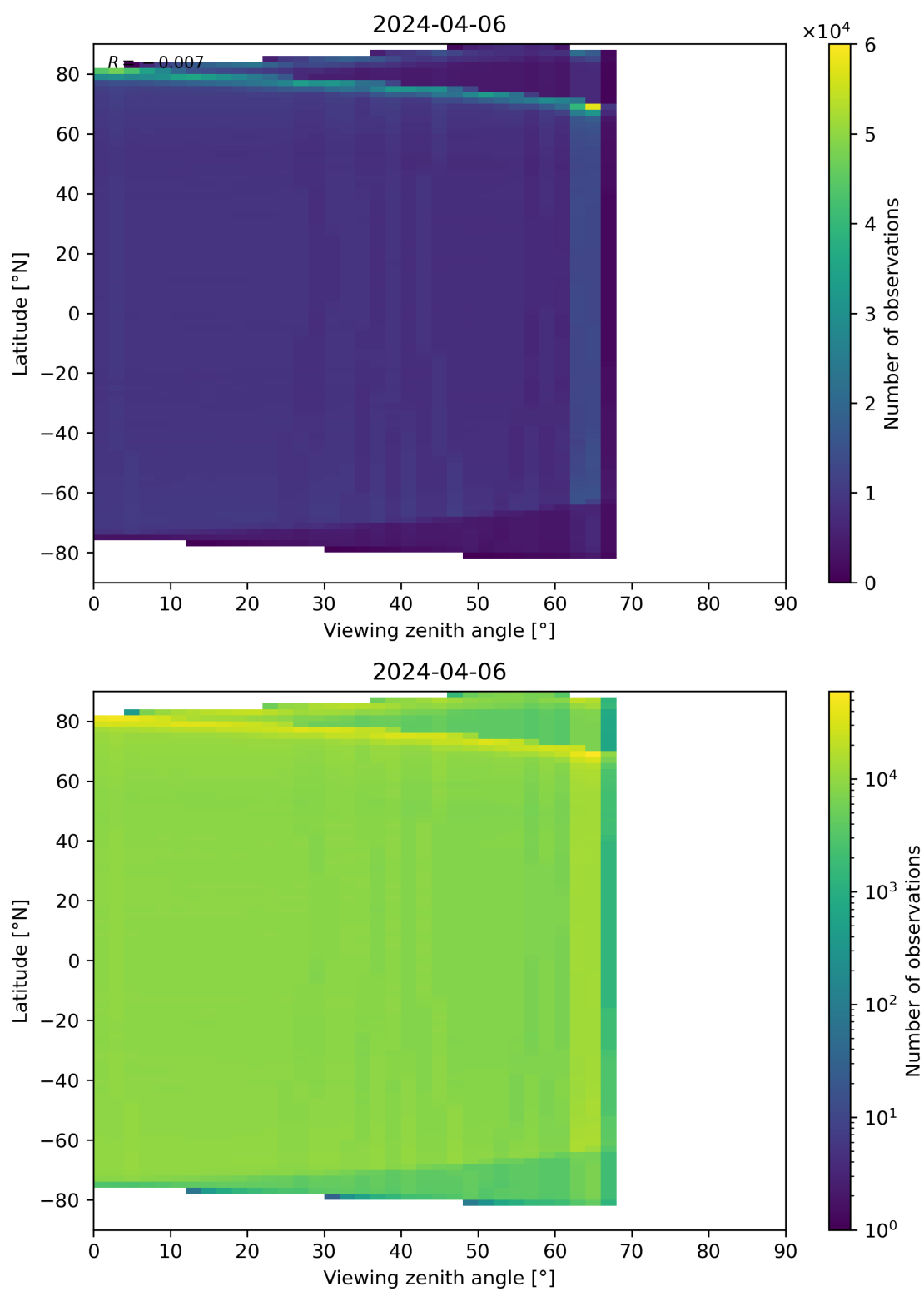
Figure 123: Scatter density plot of “Viewing zenith angle” against “Latitude” for 2024-04-05 to 2024-04-07.
