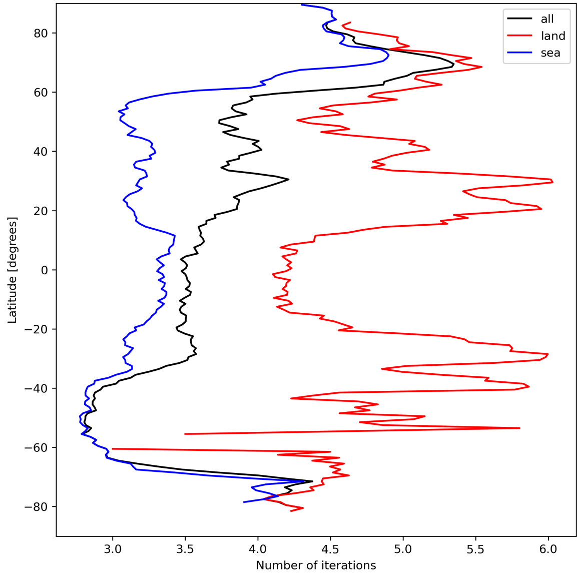
Figure 22: Zonal average of “Number of iterations” for 2024-04-05 to 2024-04-07.
