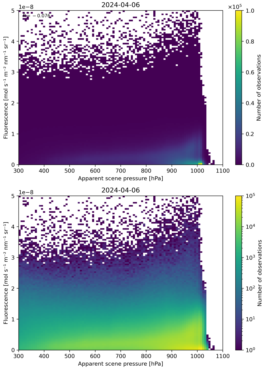
Figure 64: Scatter density plot of “Apparent scene pressure” against “Fluorescence” for 2024-04-05 to 2024-04-07.
