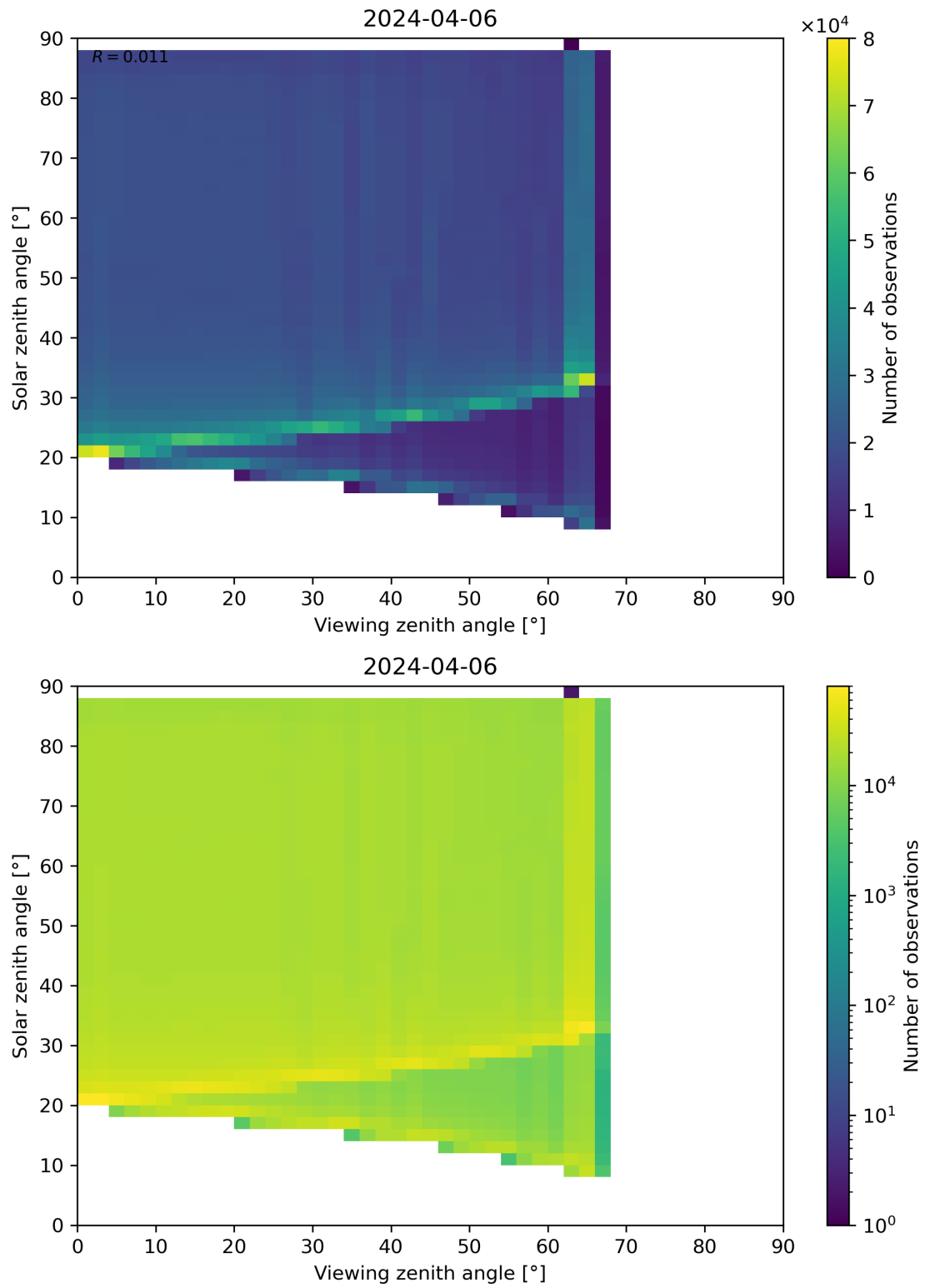
Figure 127: Scatter density plot of “Viewing zenith angle” against “Solar zenith angle” for 2024-04-05 to 2024-04-07.
