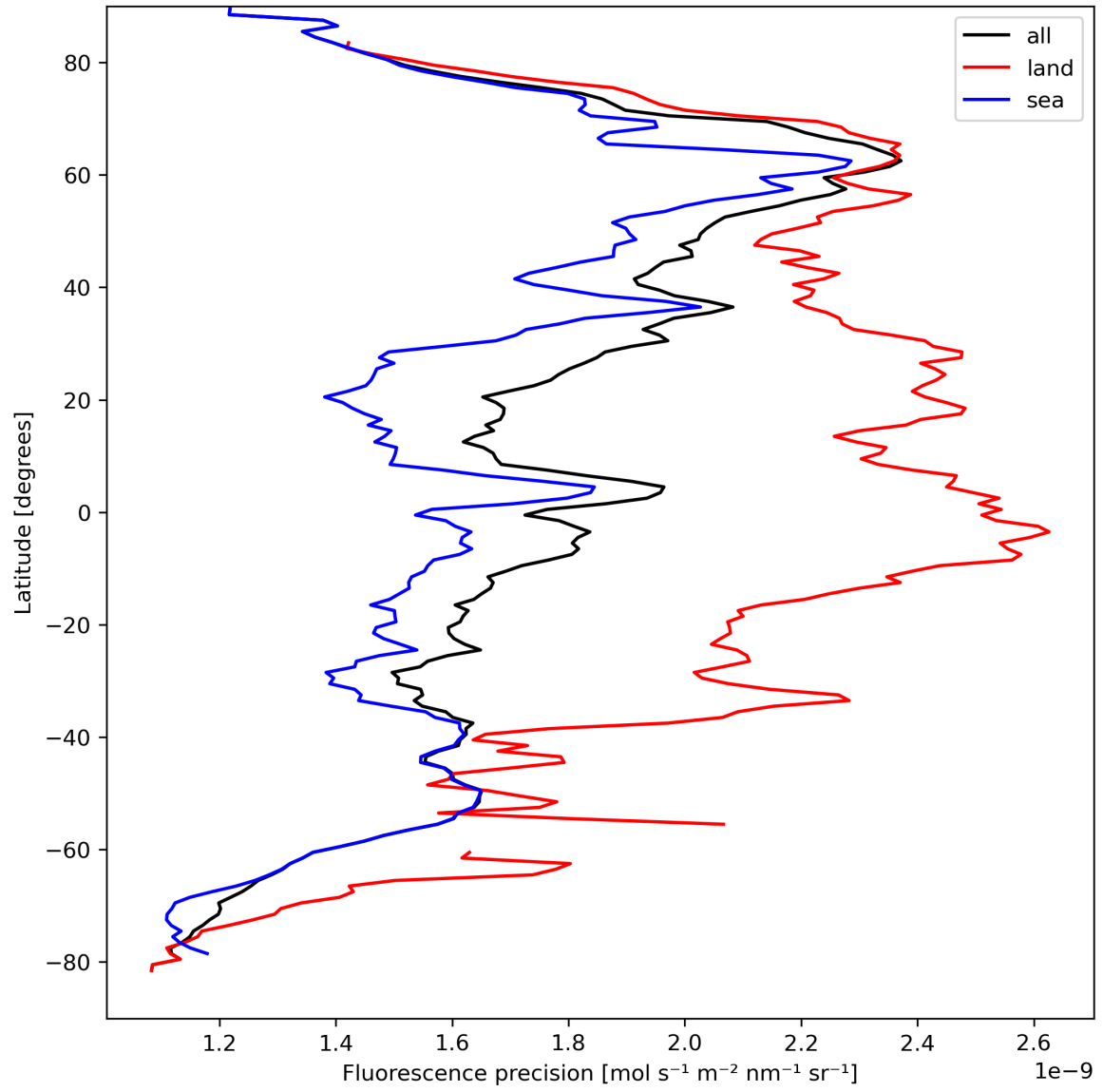
Figure 24: Zonal average of “Fluorescence precision” for 2024-04-05 to 2024-04-07.
