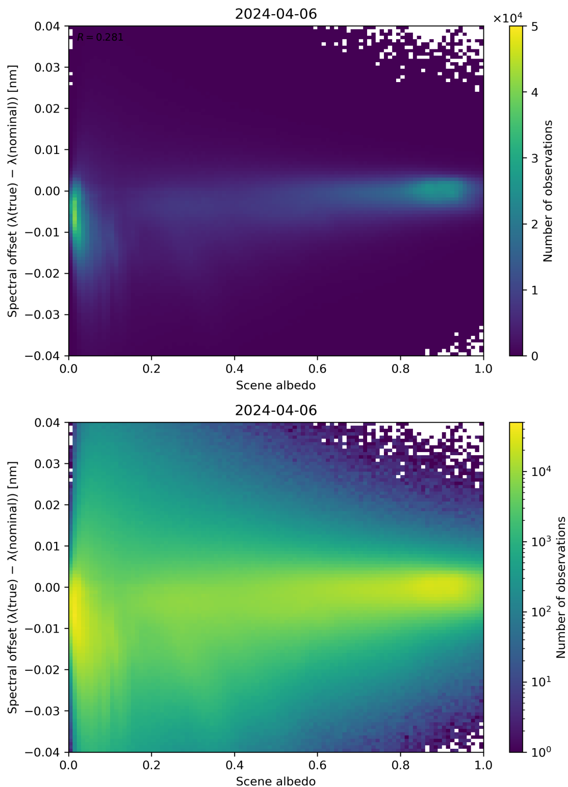
Figure 107: Scatter density plot of “Scene albedo” against “Spectral offset ( \lambda(\text{true}) - \lambda(\text{nominal}) )” for 2024-04-05 to 2024-04-07.
