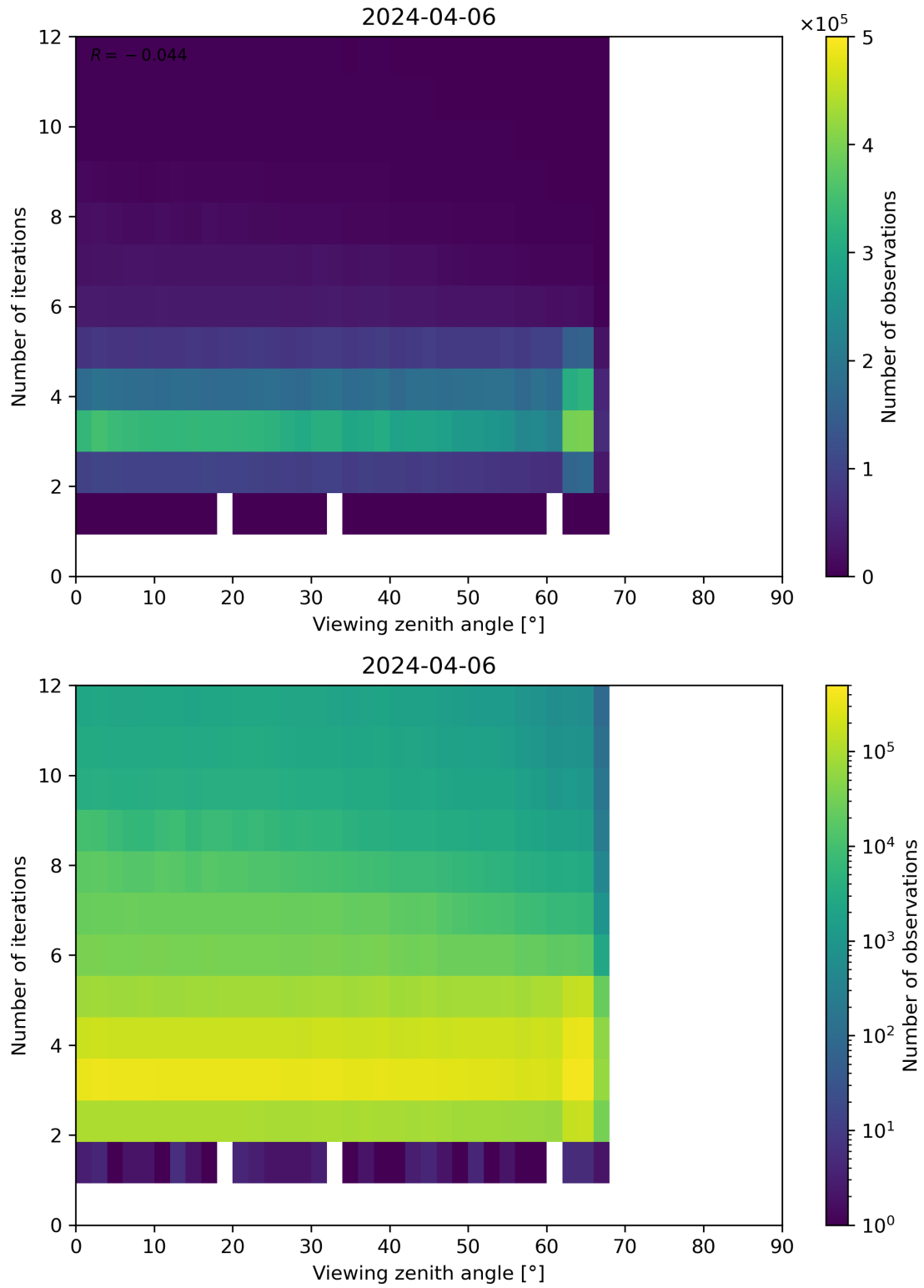
Figure 124: Scatter density plot of “Viewing zenith angle” against “Number of iterations” for 2024-04-05 to 2024-04-07.
