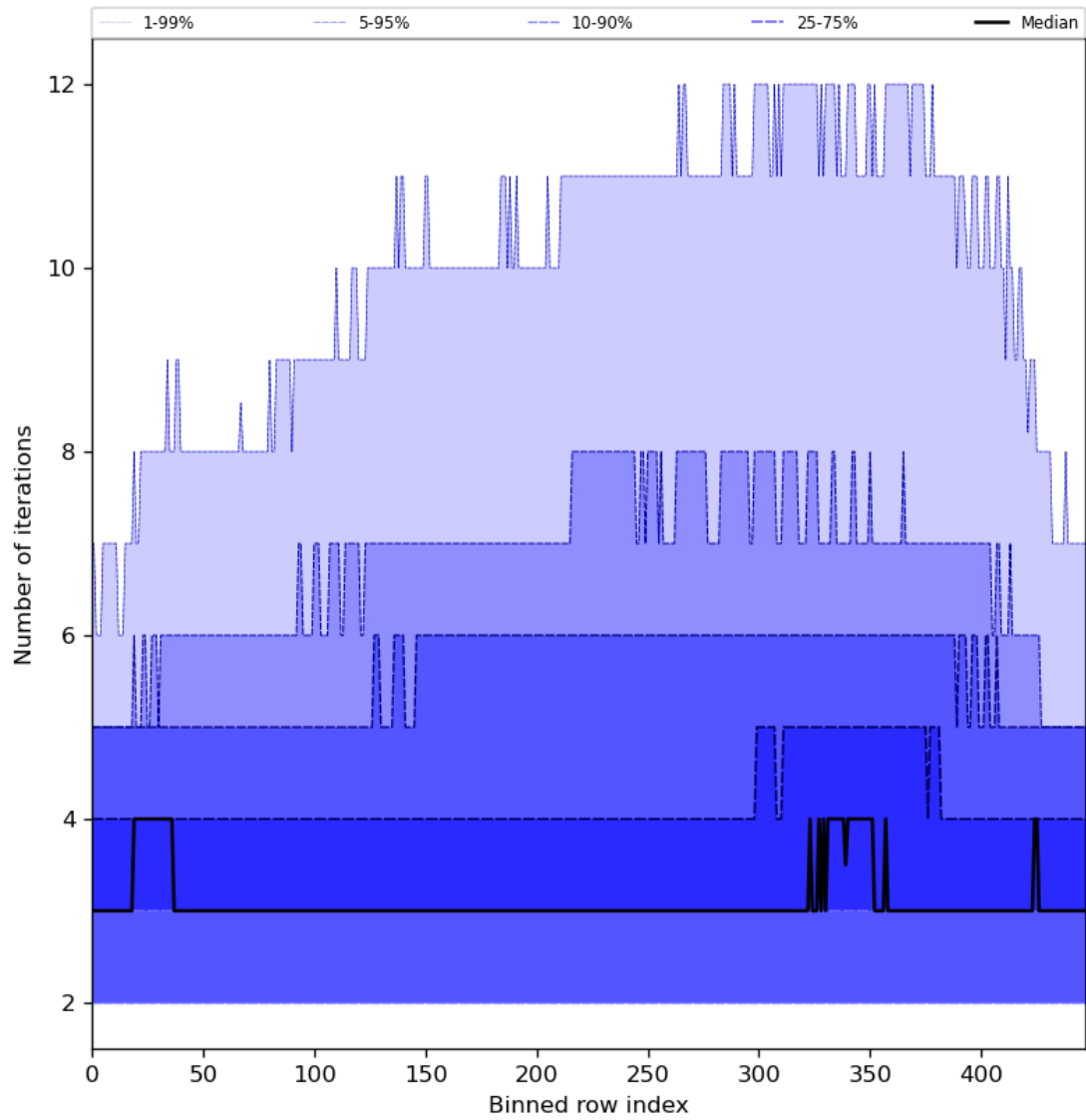
Figure 56: Along track statistics of “Number of iterations” for 2024-04-05 to 2024-04-07
