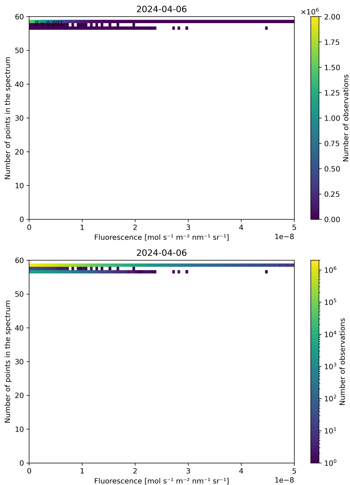
Figure 86: Scatter density plot of “Fluorescence” against “Number of points in the spectrum” for 2024-04-05 to 2024-04-07.
