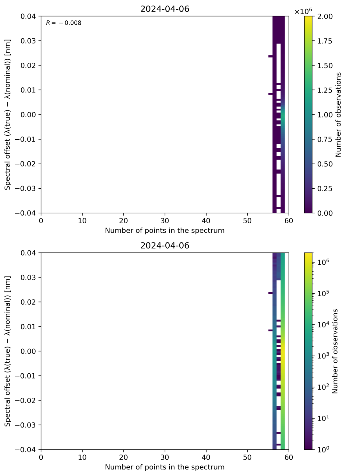
Figure 101: Scatter density plot of “Number of points in the spectrum” against “Spectral offset ( \lambda(\text{true}) - \lambda(\text{nominal}) )” for 2024-04-05 to 2024-04-07.
