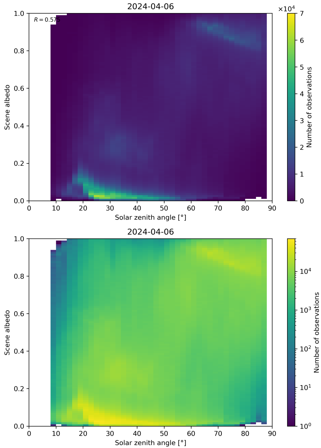
Figure 116: Scatter density plot of “Solar zenith angle” against “Scene albedo” for 2024-04-05 to 2024-04-07.
