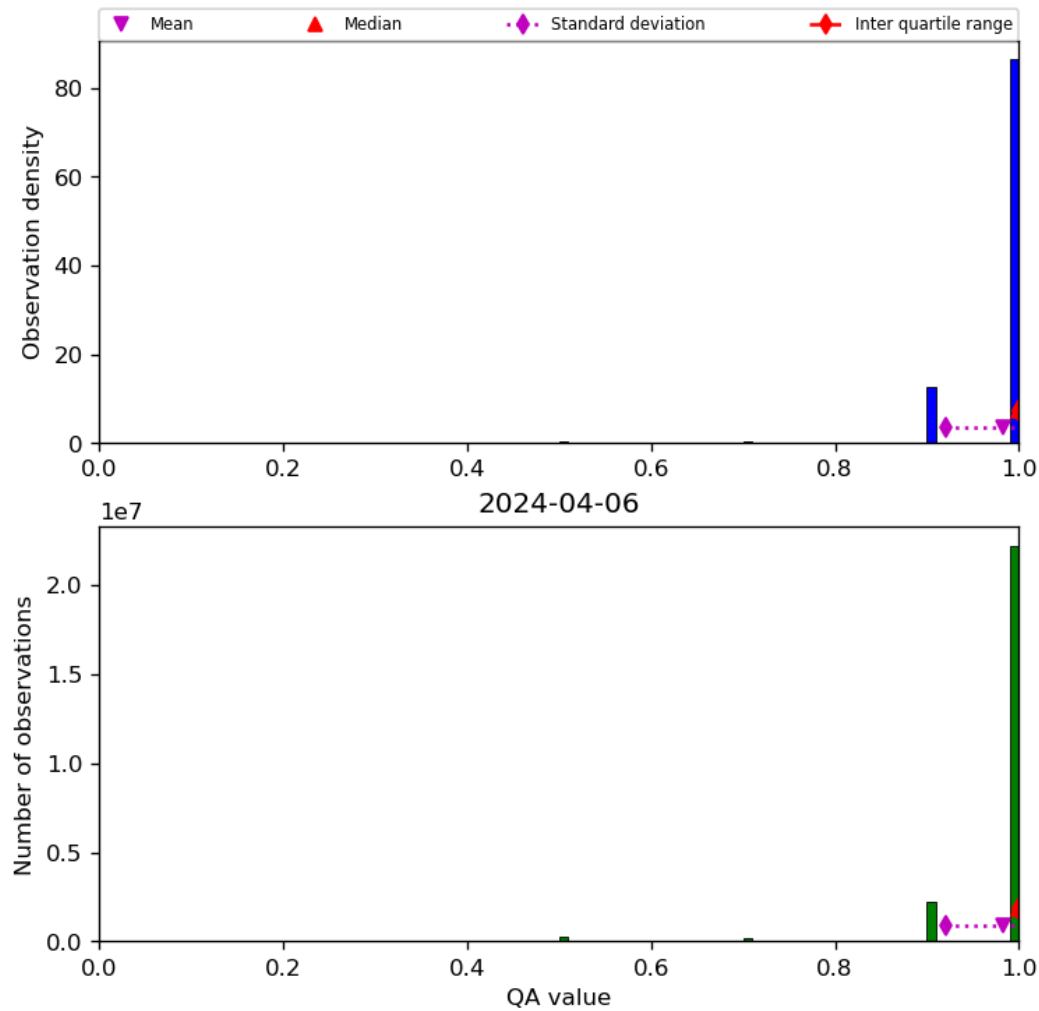
Figure 29: Histogram of “QA value” for 2024-04-05 to 2024-04-07
