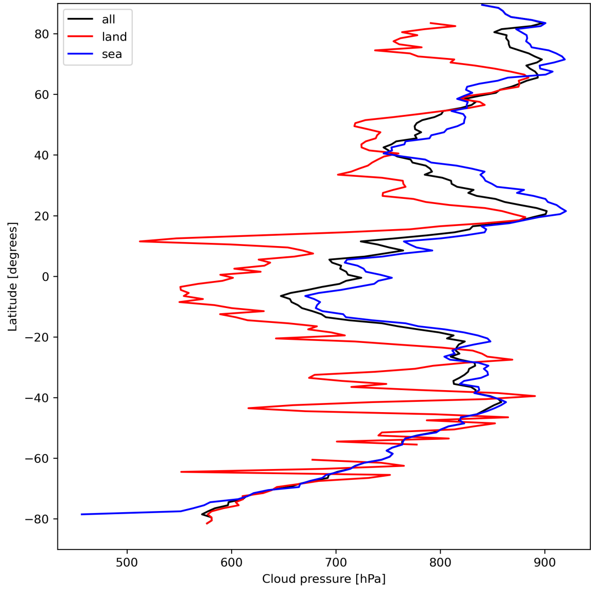
Figure 13: Zonal average of “Cloud pressure” for 2024-04-05 to 2024-04-07.
