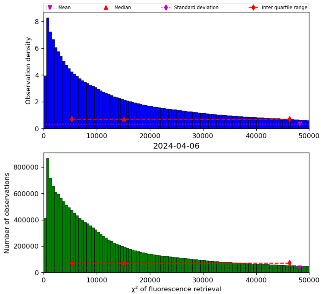
Figure 42: Histogram of “ \chi^2 of fluorescence retrieval” for 2024-04-05 to 2024-04-07
