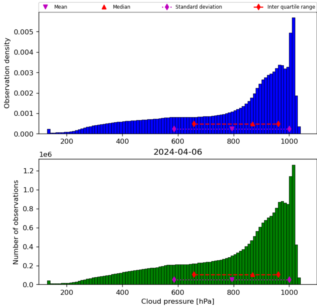
Figure 30: Histogram of “Cloud pressure” for 2024-04-05 to 2024-04-07
