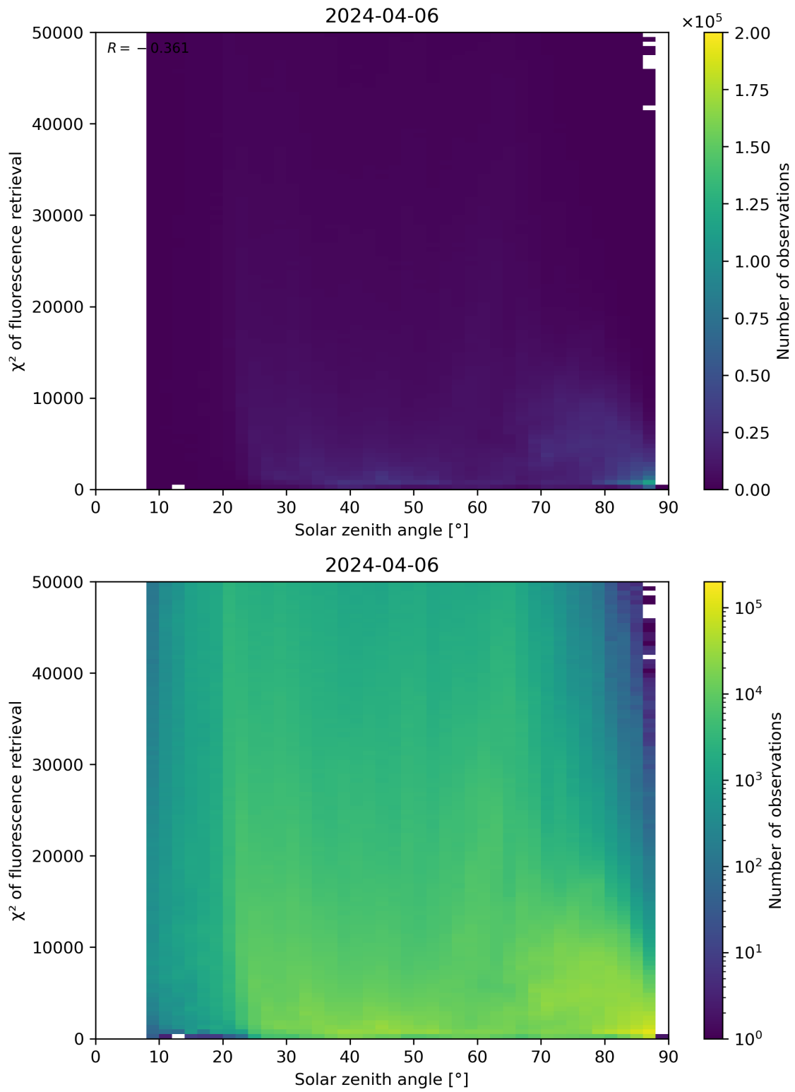
Figure 109: Scatter density plot of “Solar zenith angle” against “ \chi^2 of fluorescence retrieval” for 2024-04-05 to 2024-04-07.
