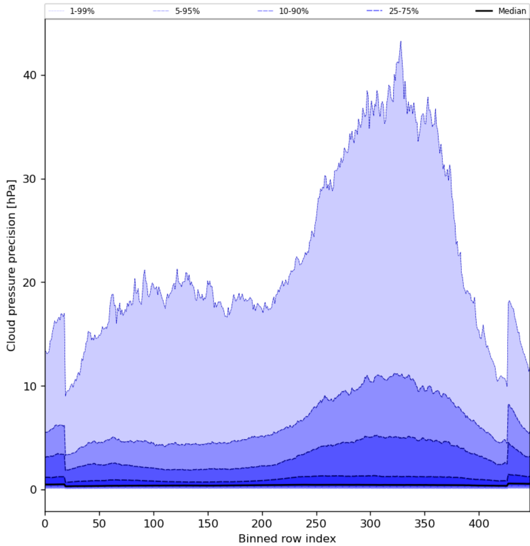
Figure 48: Along track statistics of “Cloud pressure precision” for 2024-04-05 to 2024-04-07
