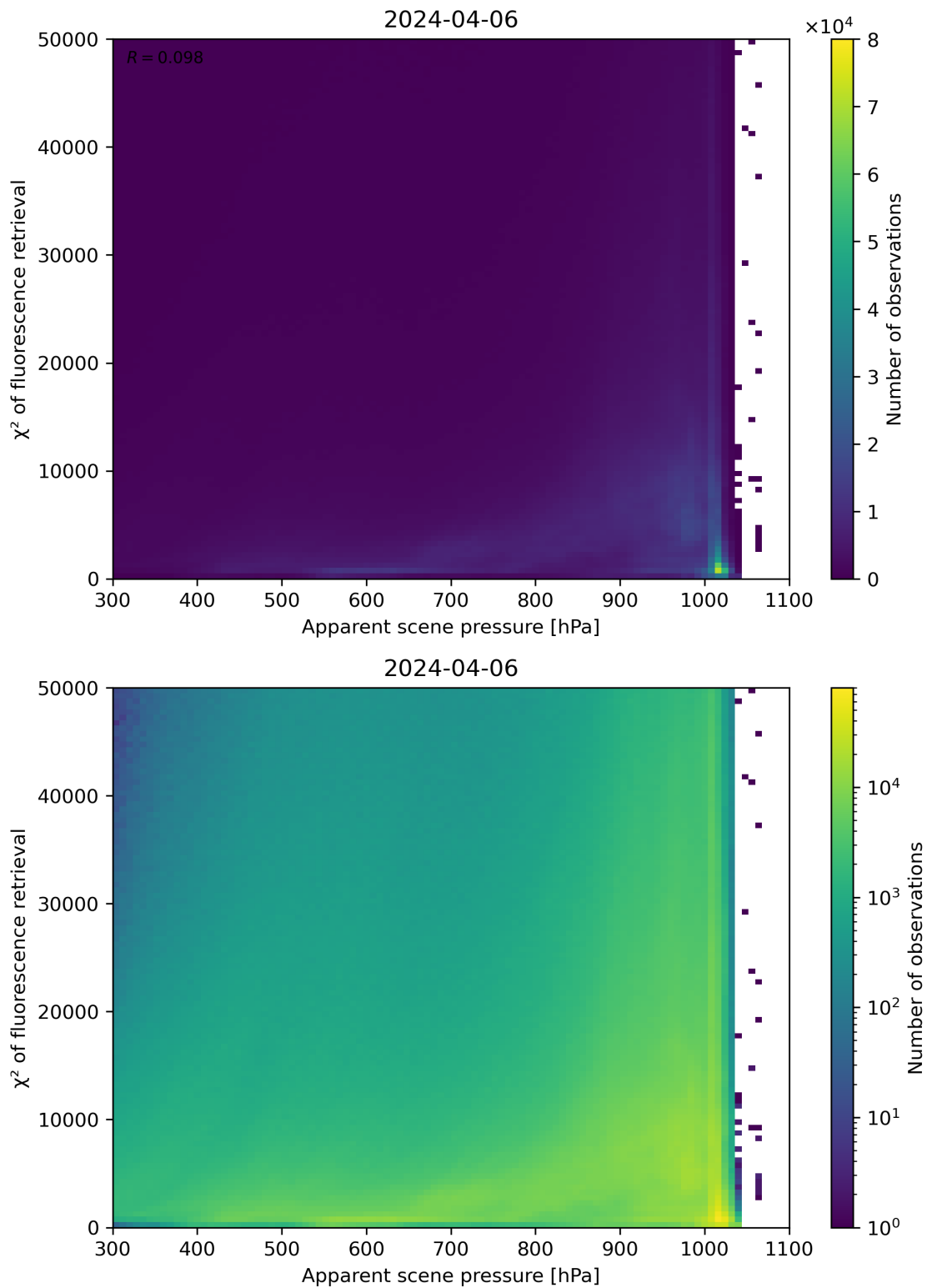
Figure 63: Scatter density plot of “Apparent scene pressure” against “ \chi^2 of fluorescence retrieval” for 2024-04-05 to 2024-04-07.
