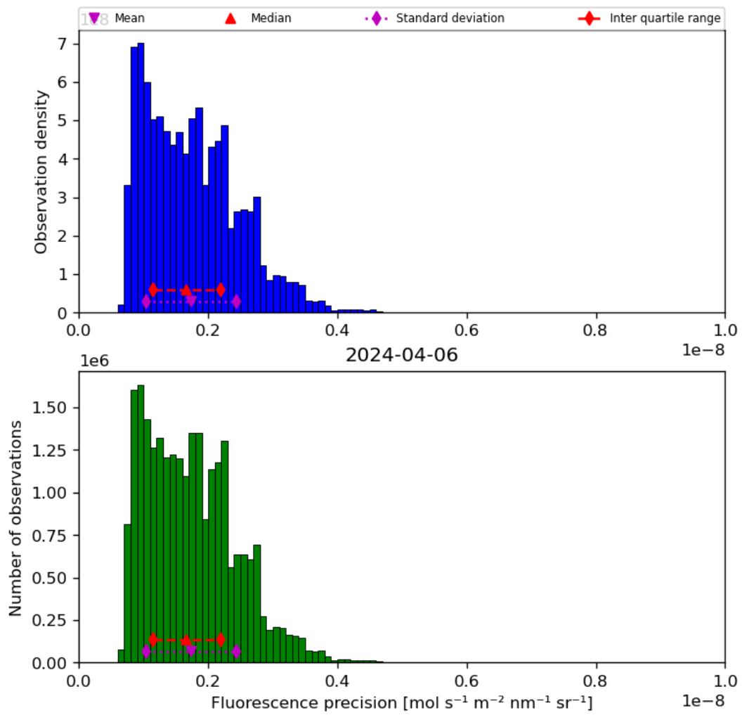
Figure 41: Histogram of “Fluorescence precision” for 2024-04-05 to 2024-04-07
