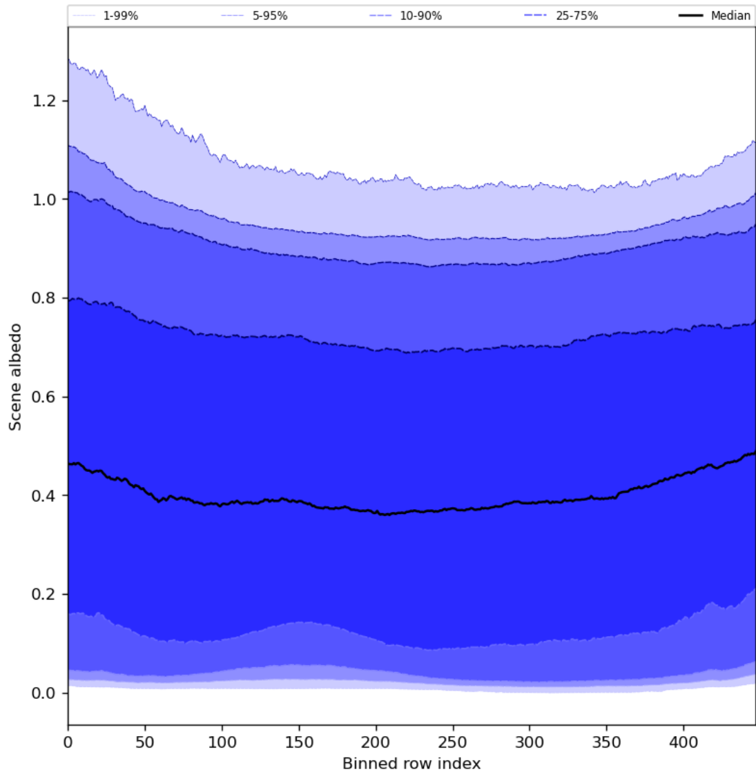
Figure 51: Along track statistics of “Scene albedo” for 2024-04-05 to 2024-04-07
