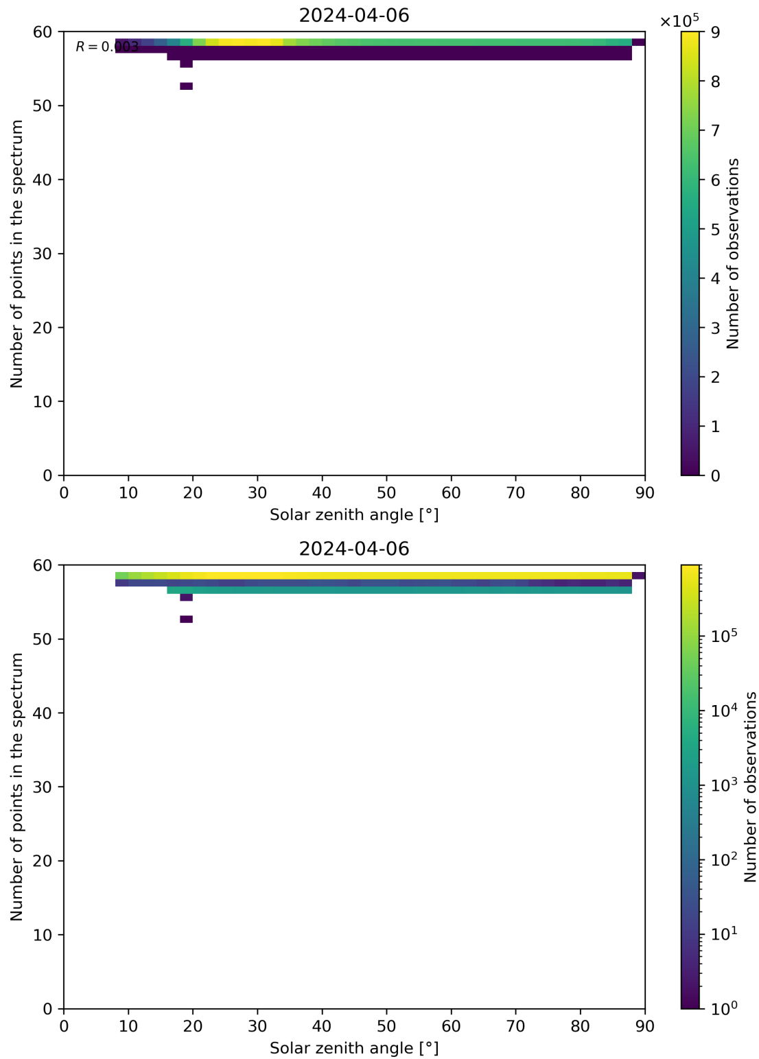
Figure 115: Scatter density plot of “Solar zenith angle” against “Number of points in the spectrum” for 2024-04-05 to 2024-04-07.
