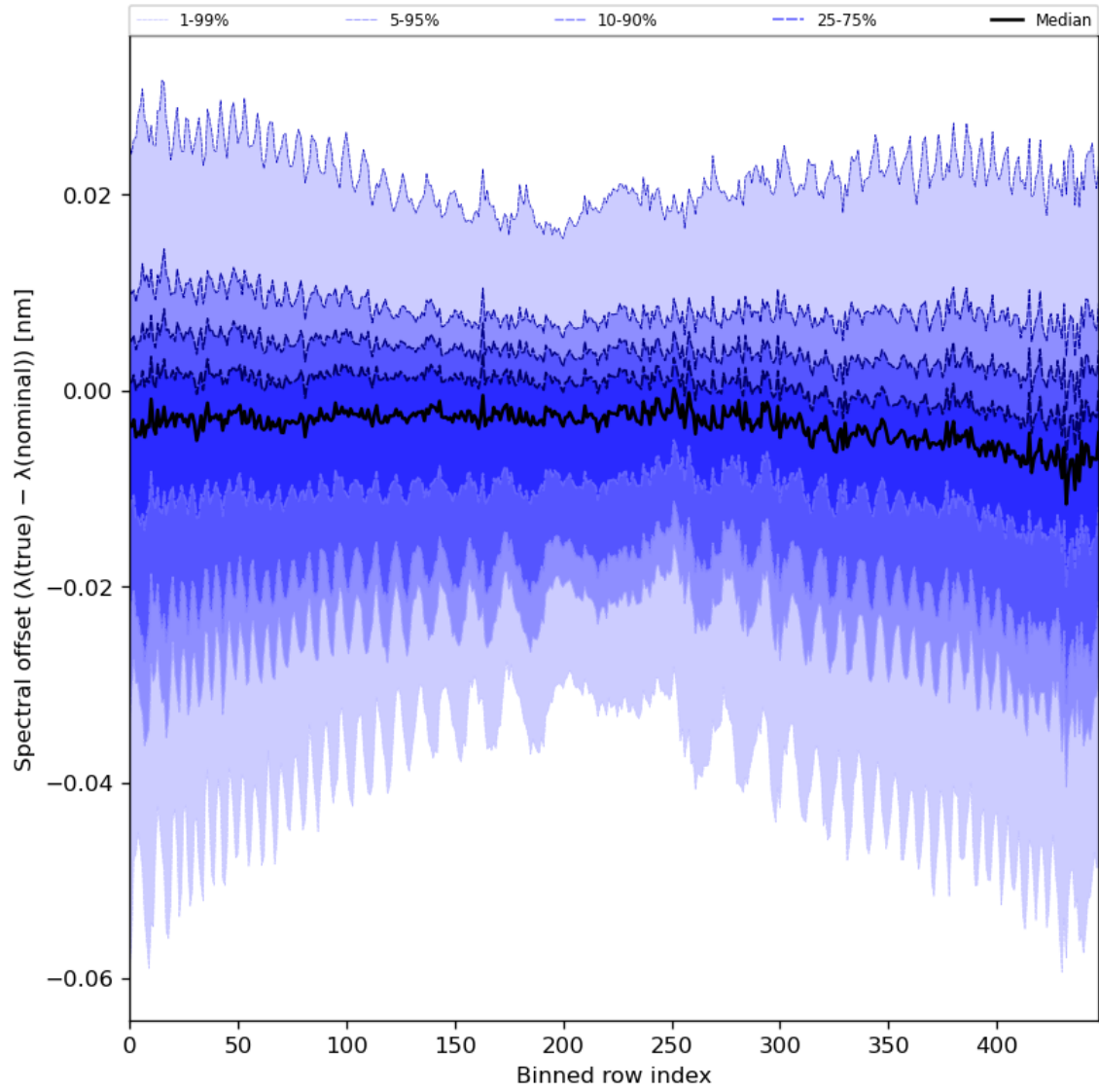
Figure 62: Along track statistics of “Spectral offset ( \lambda(\text{true}) - \lambda(\text{nominal}) )” for 2024-04-05 to 2024-04-07
