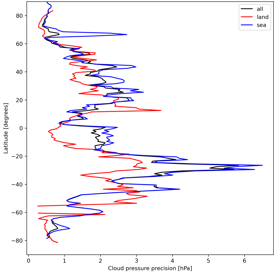
Figure 14: Zonal average of “Cloud pressure precision” for 2024-04-05 to 2024-04-07.
