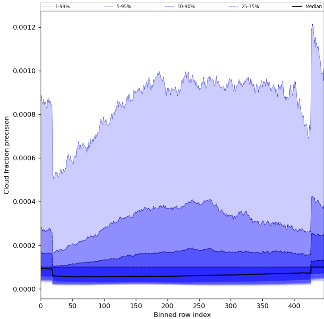
Figure 50: Along track statistics of “Cloud fraction precision” for 2024-04-05 to 2024-04-07
