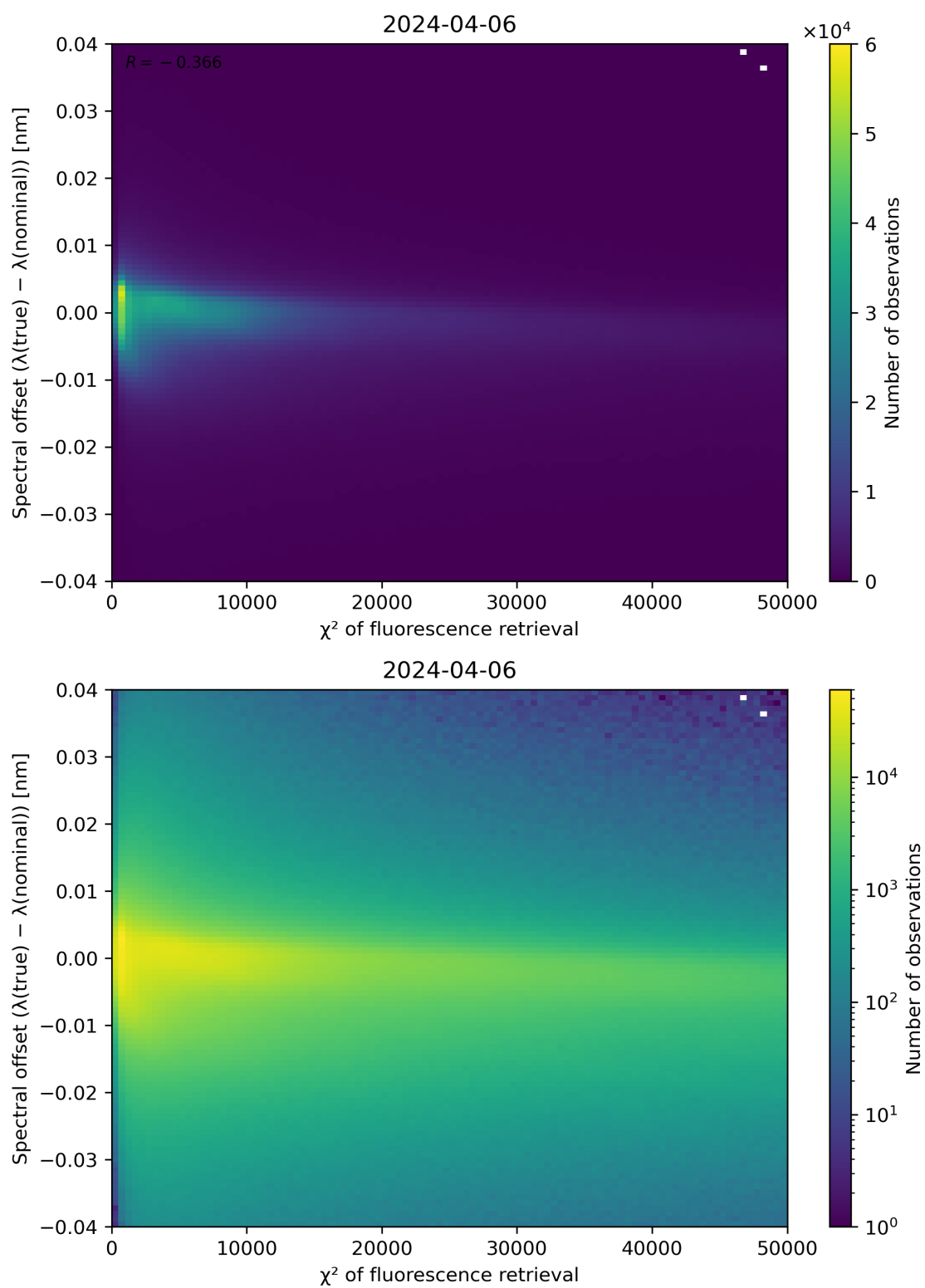
Figure 69: Scatter density plot of " \chi^2 of fluorescence retrieval" against "Spectral offset ( \lambda(\text{true}) - \lambda(\text{nominal})) " for 2024-04-05 to 2024-04-07.
