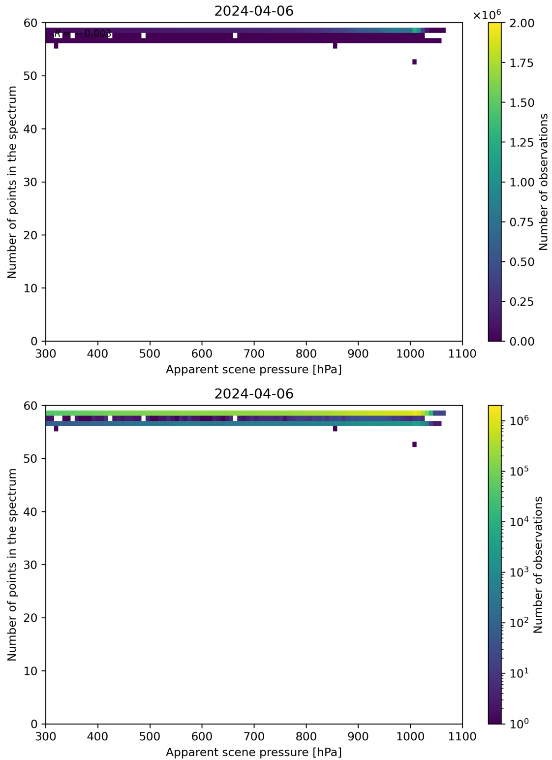
Figure 66: Scatter density plot of “Apparent scene pressure” against “Number of points in the spectrum” for 2024-04-05 to 2024-04-07.
