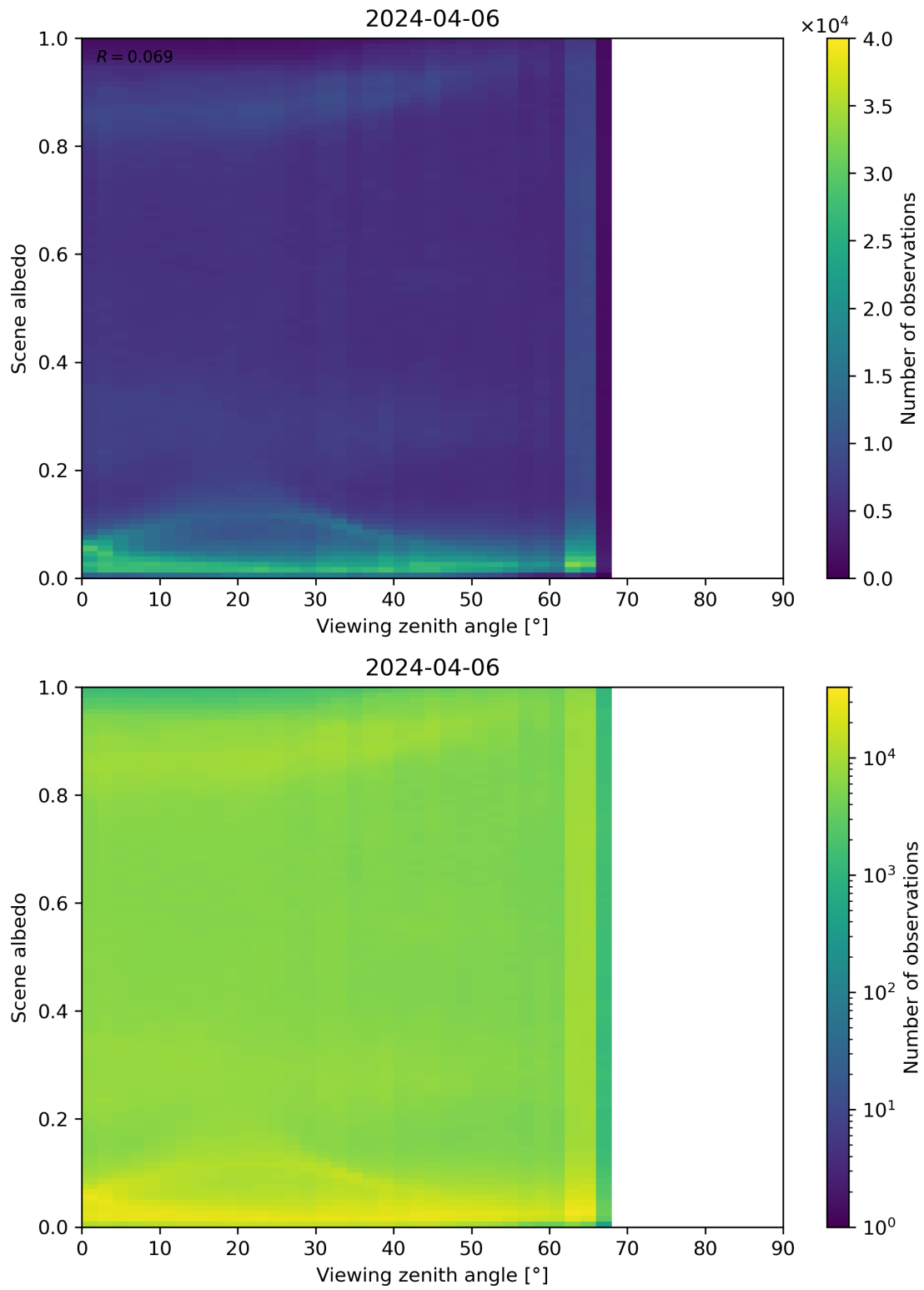
Figure 126: Scatter density plot of “Viewing zenith angle” against “Scene albedo” for 2024-04-05 to 2024-04-07.
