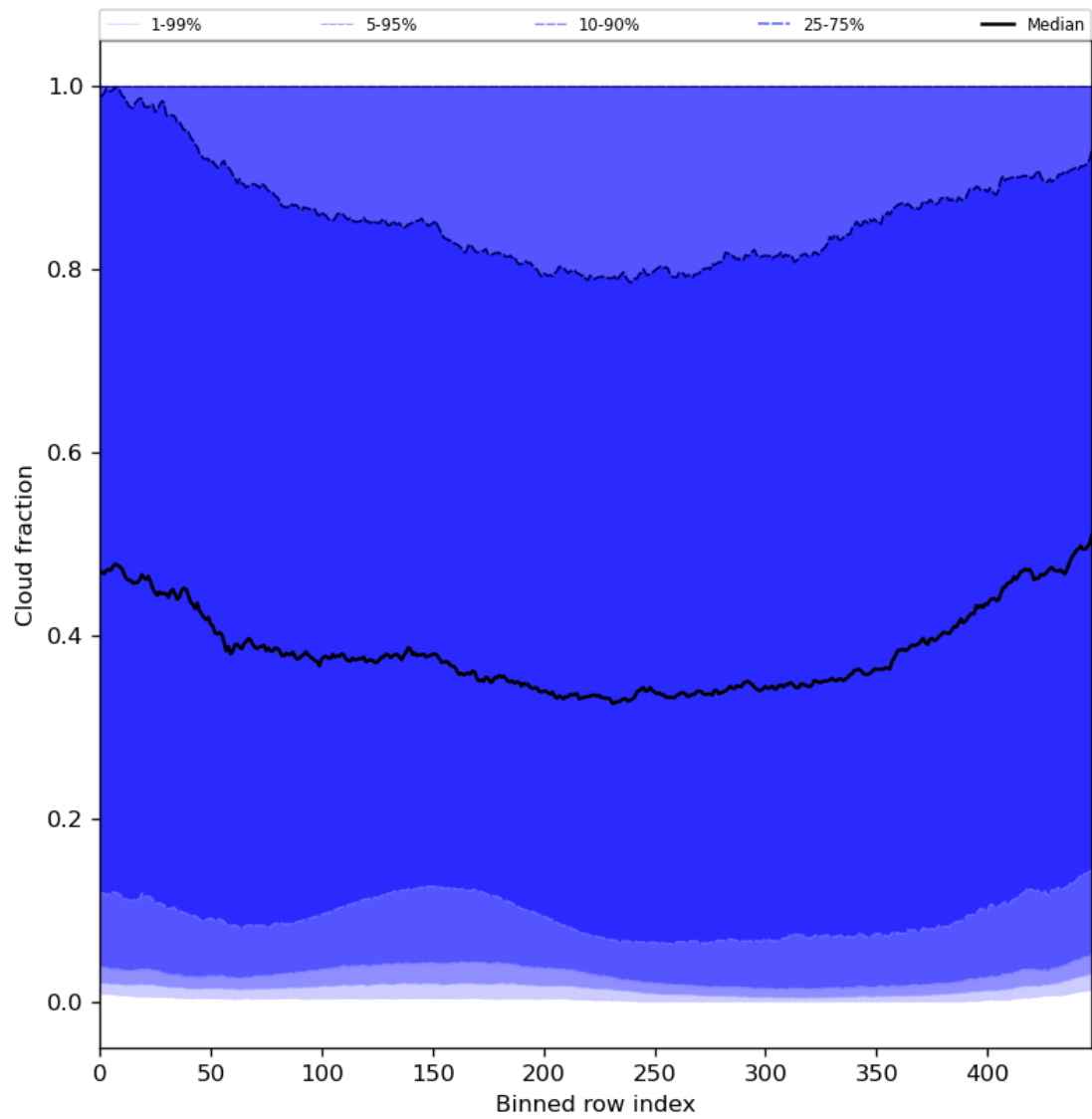
Figure 49: Along track statistics of “Cloud fraction” for 2024-04-05 to 2024-04-07
