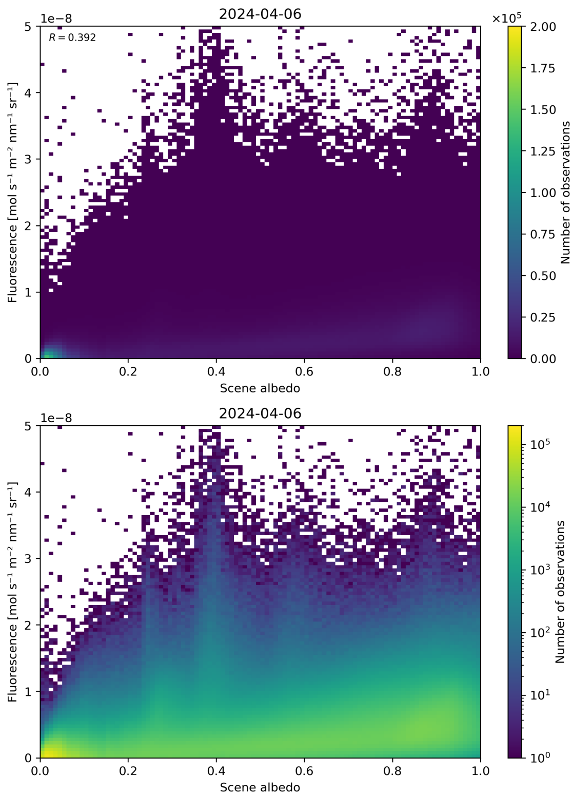
Figure 104: Scatter density plot of “Scene albedo” against “Fluorescence” for 2024-04-05 to 2024-04-07.
