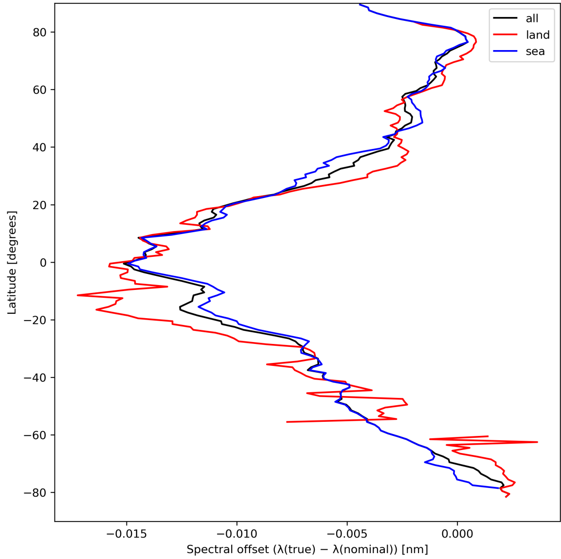
Figure 28: Zonal average of “Spectral offset ( \lambda(\text{true}) - \lambda(\text{nominal}) )” for 2024-04-05 to 2024-04-07.
