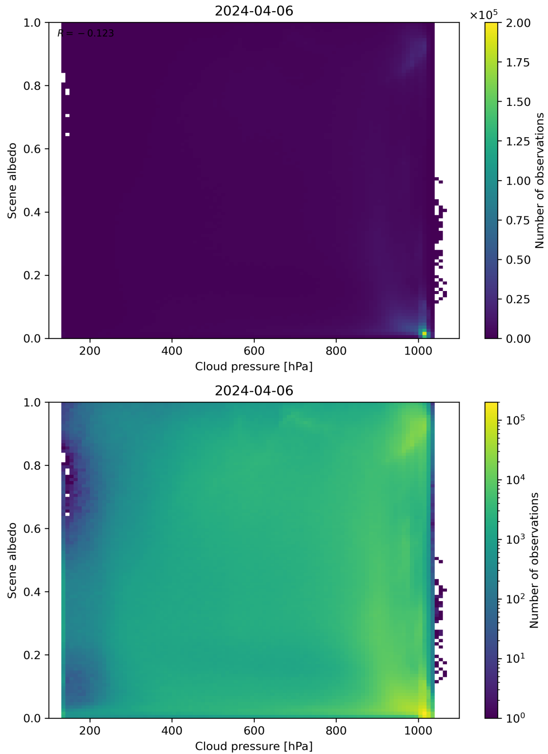
Figure 83: Scatter density plot of “Cloud pressure” against “Scene albedo” for 2024-04-05 to 2024-04-07.
