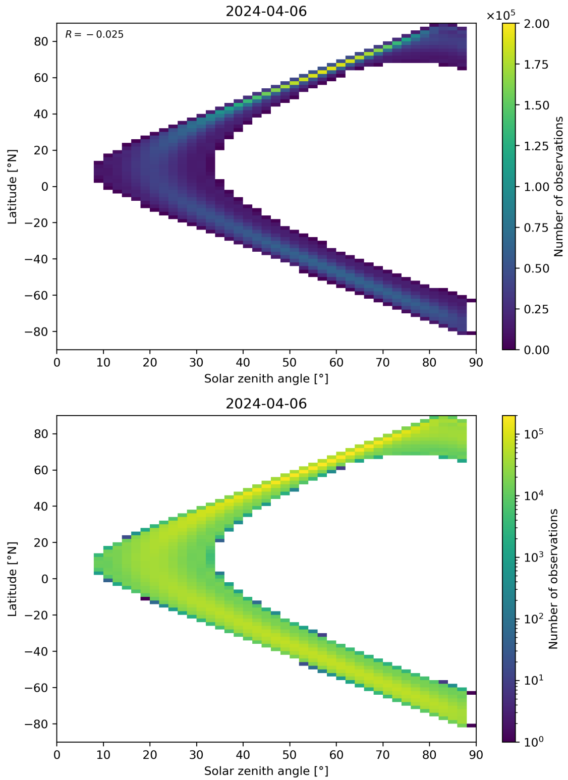
Figure 113: Scatter density plot of “Solar zenith angle” against “Latitude” for 2024-04-05 to 2024-04-07.
