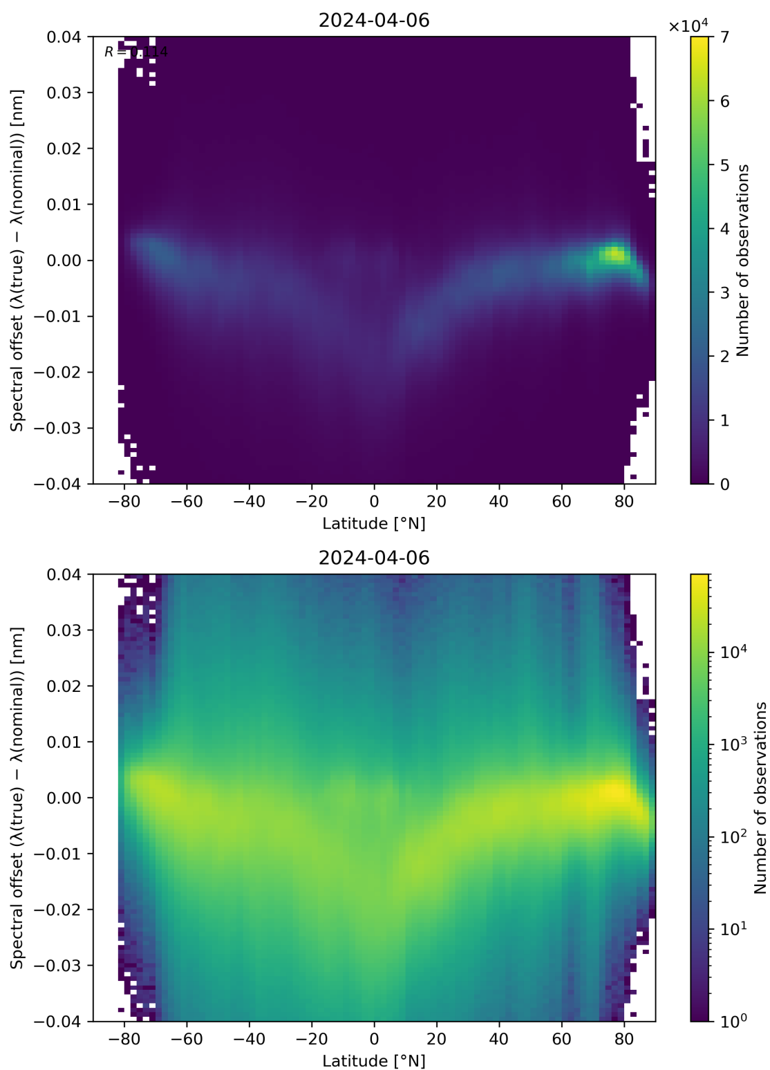
Figure 96: Scatter density plot of “Latitude” against “Spectral offset ( \lambda(\text{true}) - \lambda(\text{nominal}) )” for 2024-04-05 to 2024-04-07.
