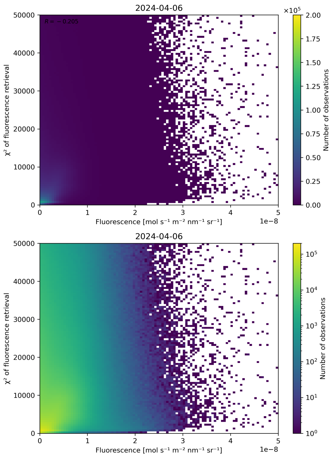
Figure 85: Scatter density plot of “Fluorescence” against “ \chi^2 of fluorescence retrieval” for 2024-04-05 to 2024-04-07.
