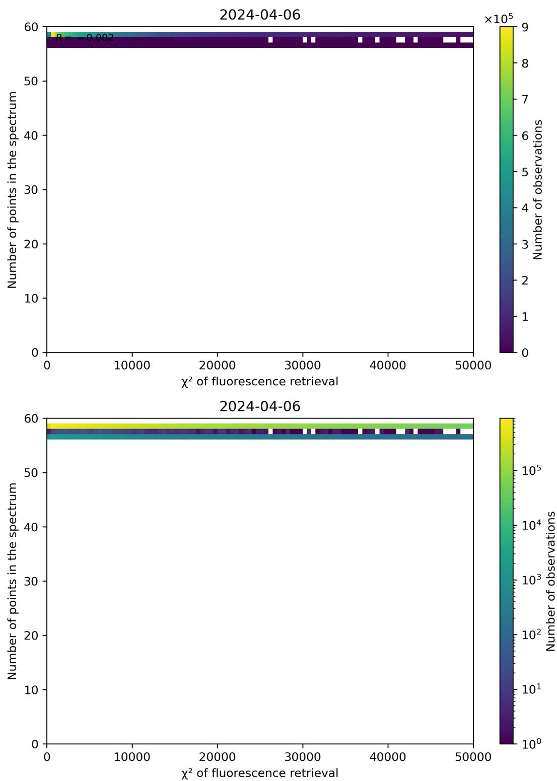
Figure 68: Scatter density plot of " \chi^2 of fluorescence retrieval" against "Number of points in the spectrum" for 2024-04-05 to 2024-04-07.
