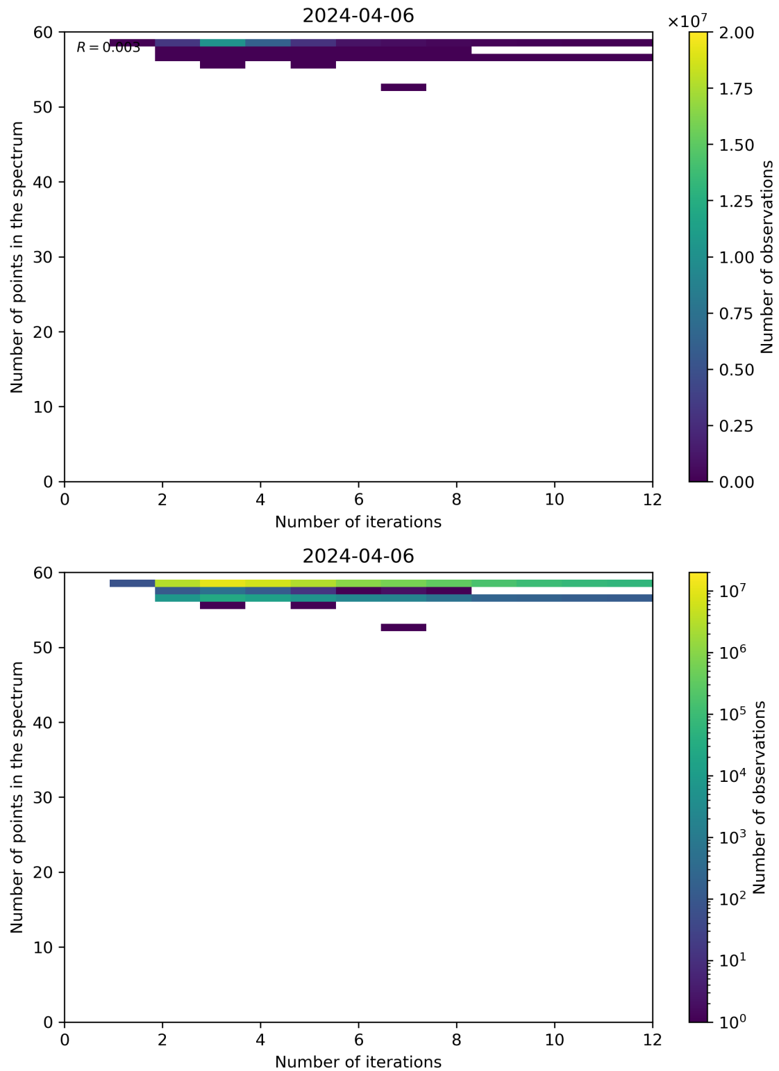
Figure 99: Scatter density plot of “Number of iterations” against “Number of points in the spectrum” for 2024-04-05 to 2024-04-07.
