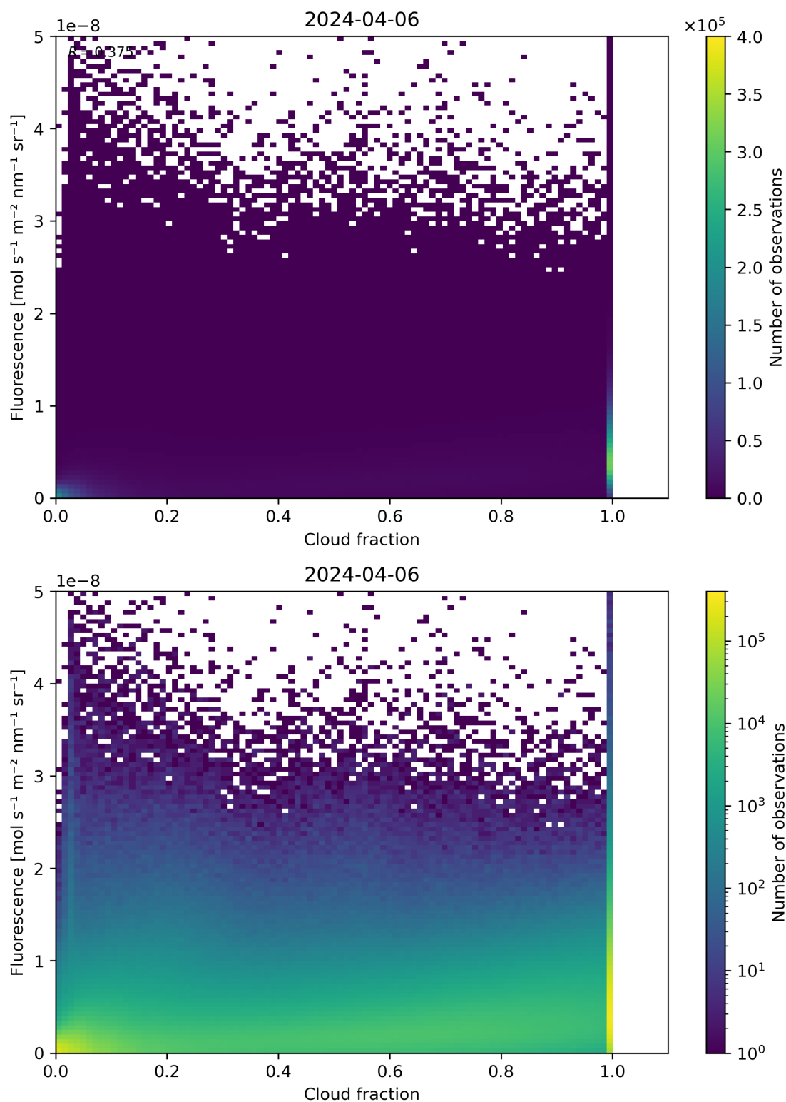
Figure 72: Scatter density plot of “Cloud fraction” against “Fluorescence” for 2024-04-05 to 2024-04-07.
