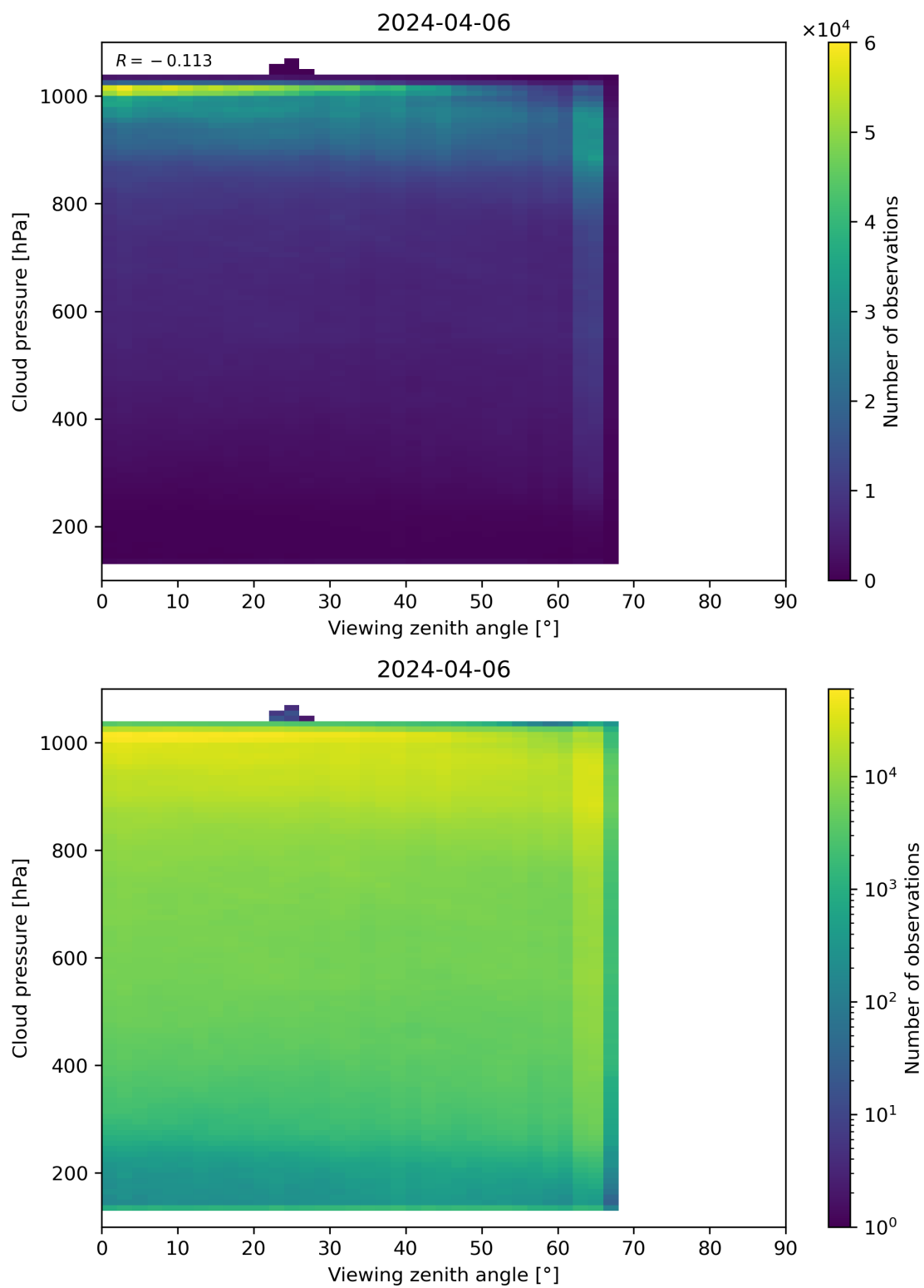
Figure 121: Scatter density plot of “Viewing zenith angle” against “Cloud pressure” for 2024-04-05 to 2024-04-07.
