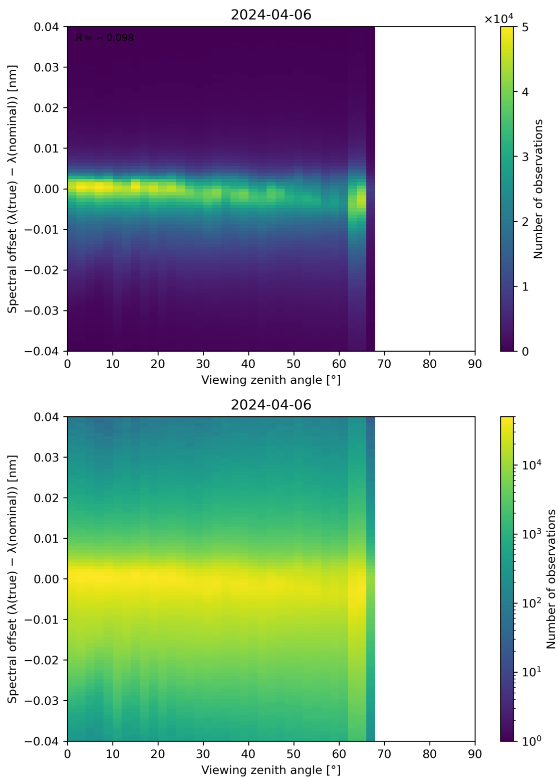
Figure 128: Scatter density plot of “Viewing zenith angle” against “Spectral offset ( \lambda(\text{true}) - \lambda(\text{nominal}) )” for 2024-04-05 to 2024-04-07.
