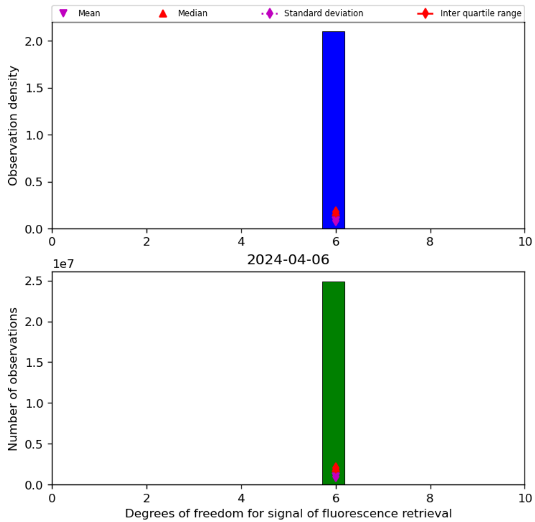
Figure 43: Histogram of “Degrees of freedom for signal of fluorescence retrieval” for 2024-04-05 to 2024-04-07
