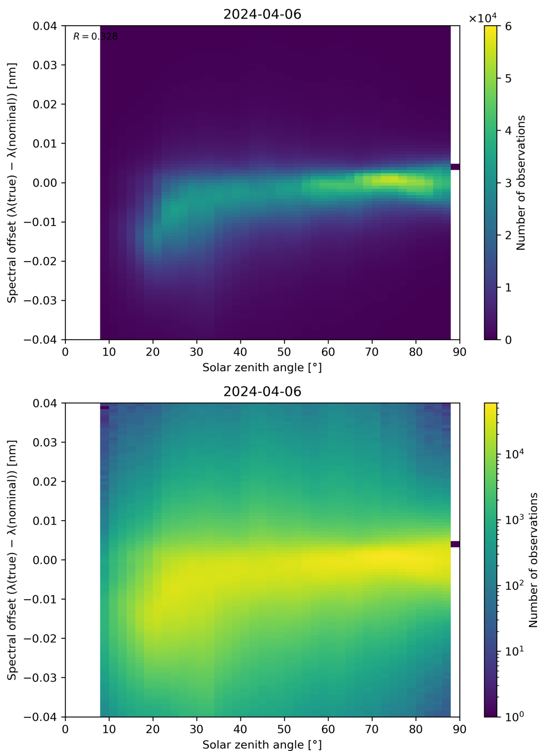
Figure 117: Scatter density plot of “Solar zenith angle” against “Spectral offset ( \lambda(\text{true}) - \lambda(\text{nominal}) )” for 2024-04-05 to 2024-04-07.
