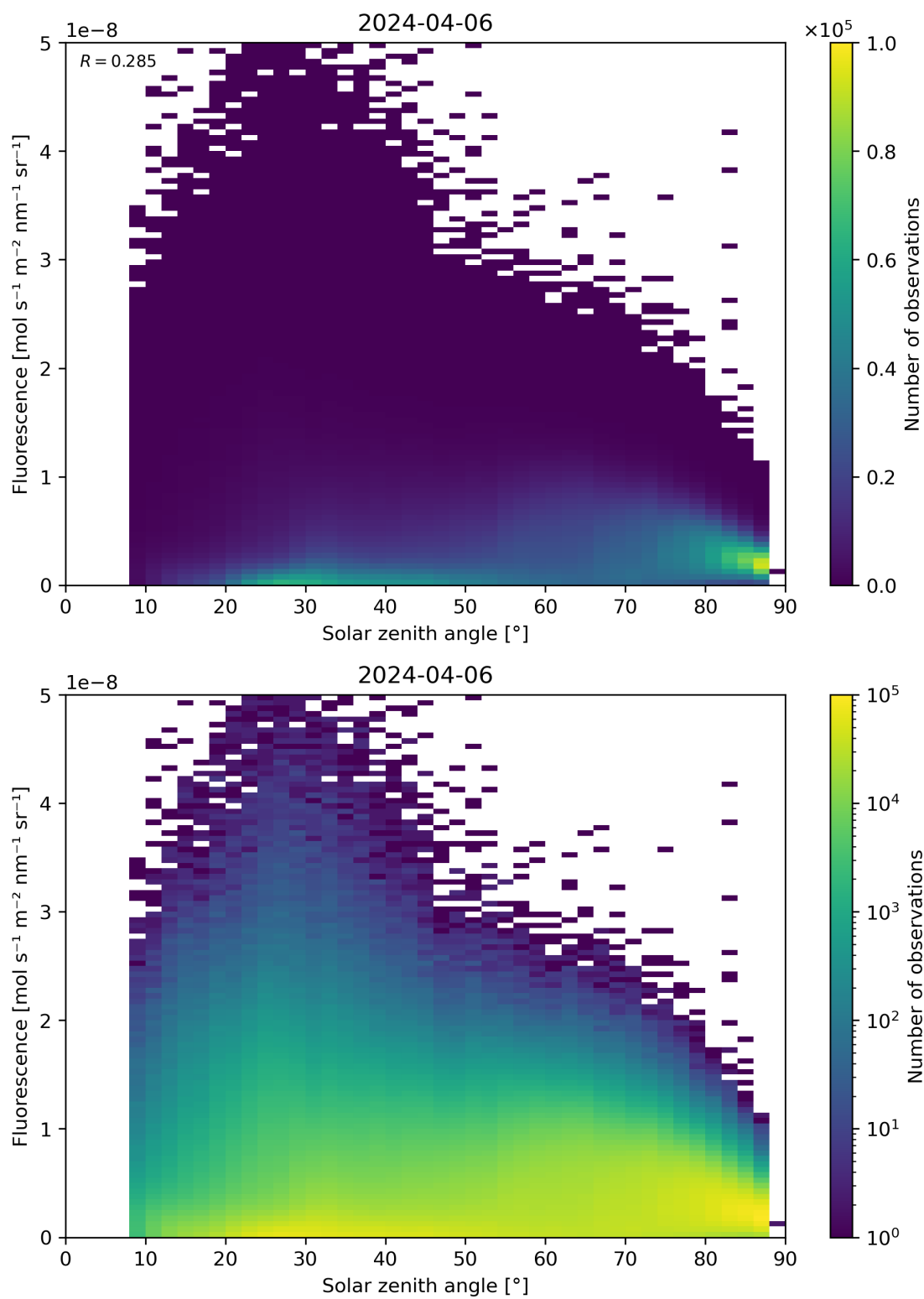
Figure 112: Scatter density plot of “Solar zenith angle” against “Fluorescence” for 2024-04-05 to 2024-04-07.
