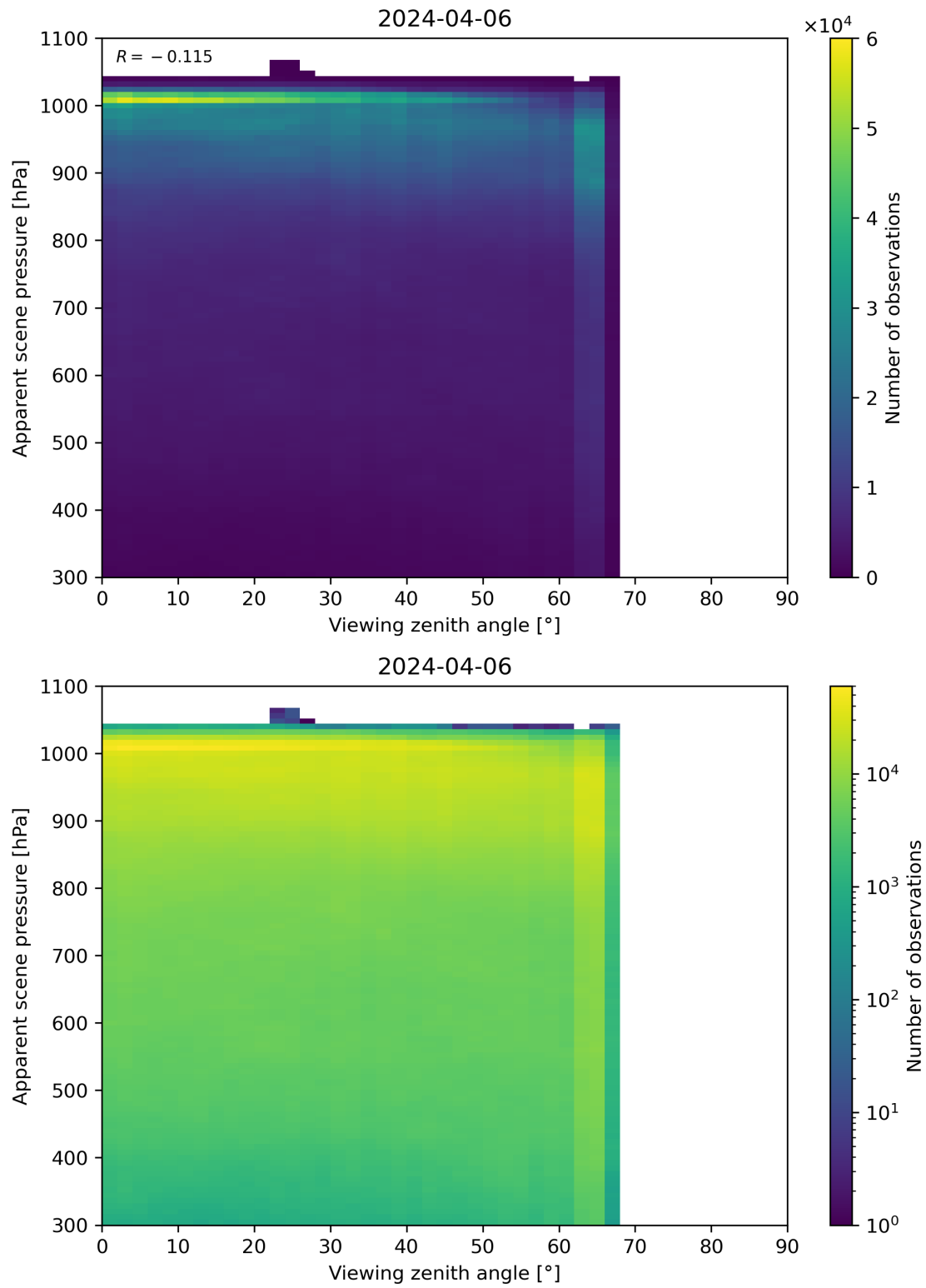
Figure 118: Scatter density plot of “Viewing zenith angle” against “Apparent scene pressure” for 2024-04-05 to 2024-04-07.
