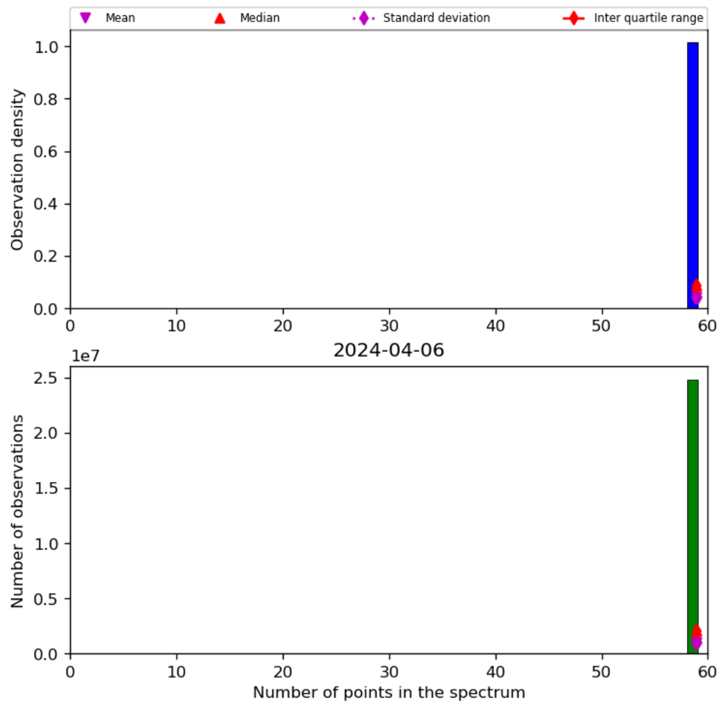
Figure 44: Histogram of "Number of points in the spectrum" for 2024-04-05 to 2024-04-07
