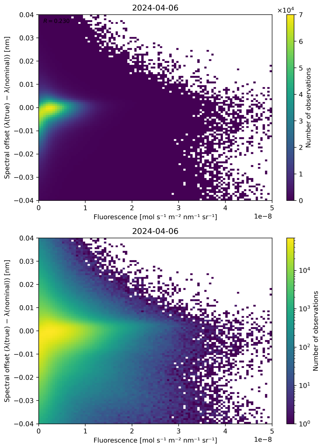
Figure 87: Scatter density plot of “Fluorescence” against “Spectral offset ( \lambda(\text{true}) - \lambda(\text{nominal}) )” for 2024-04-05 to 2024-04-07.
