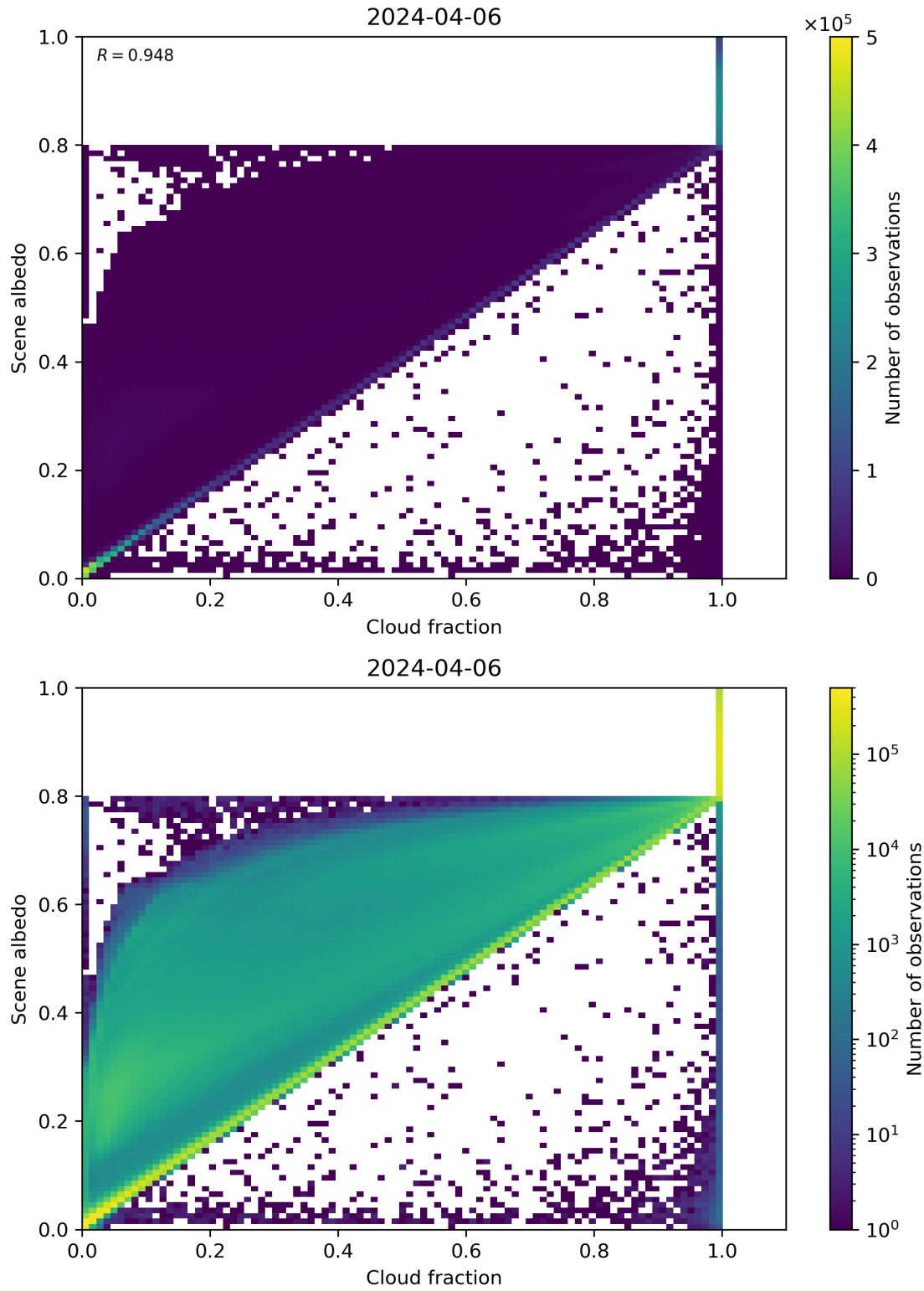
Figure 75: Scatter density plot of “Cloud fraction” against “Scene albedo” for 2024-04-05 to 2024-04-07.
