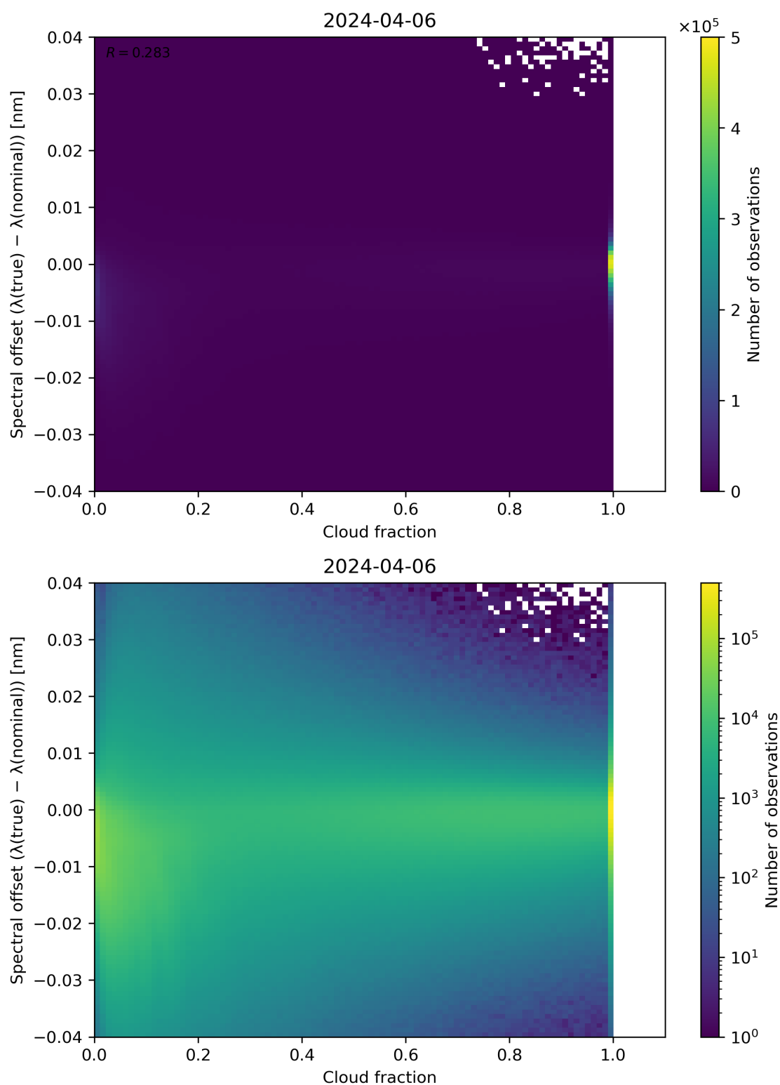
Figure 76: Scatter density plot of “Cloud fraction” against “Spectral offset ( \lambda(\text{true}) - \lambda(\text{nominal}) )” for 2024-04-05 to 2024-04-07.
