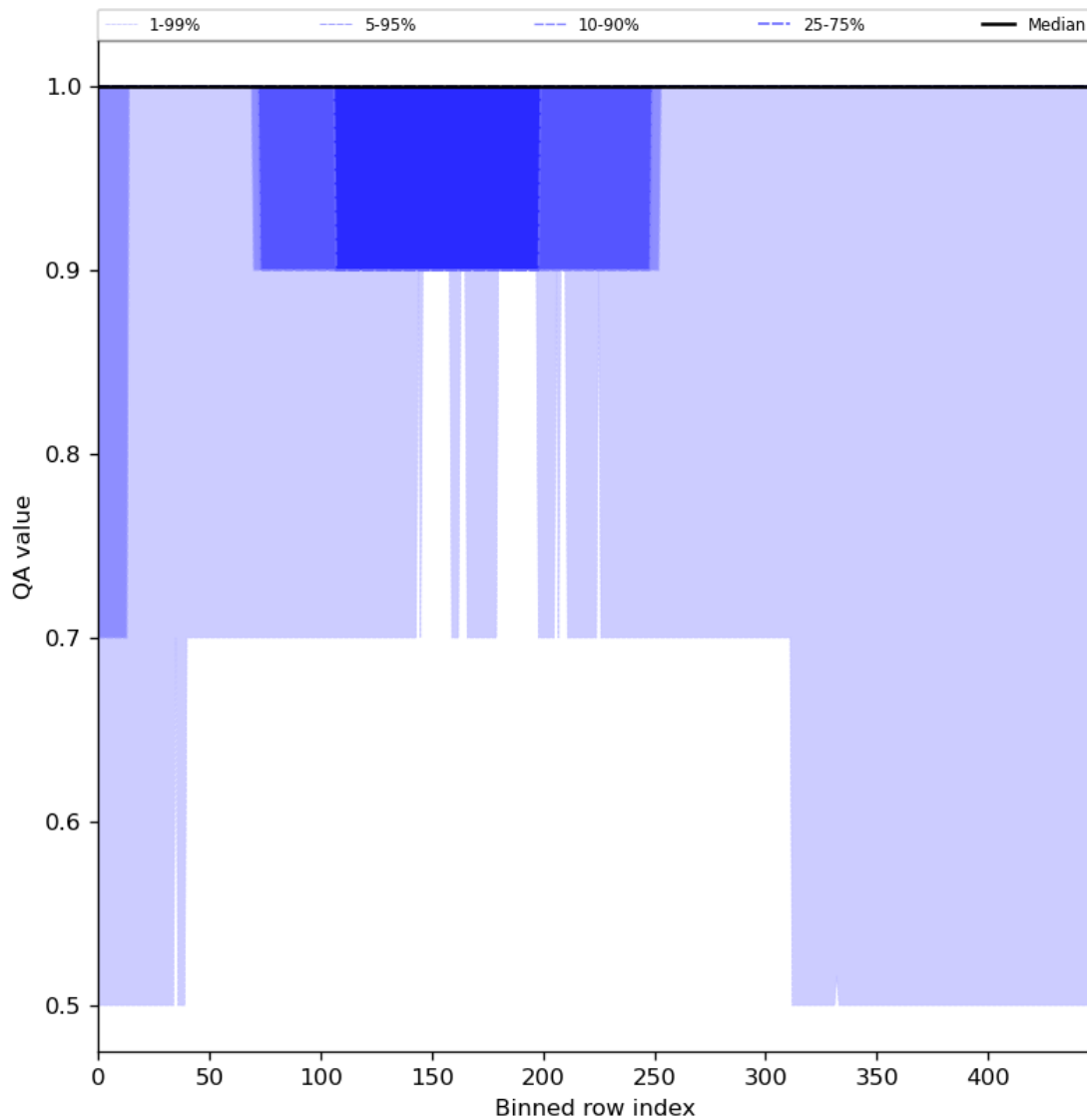
Figure 46: Along track statistics of “QA value” for 2024-04-05 to 2024-04-07
