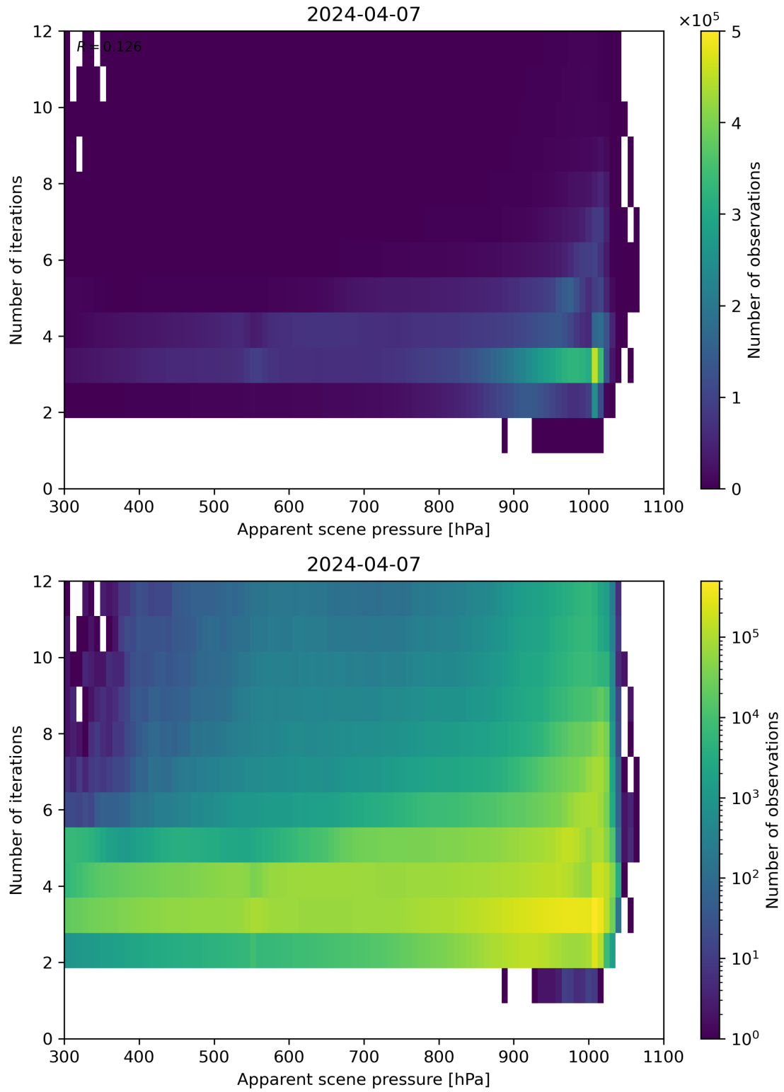
Figure 65: Scatter density plot of “Apparent scene pressure” against “Number of iterations” for 2024-04-06 to 2024-04-08.
