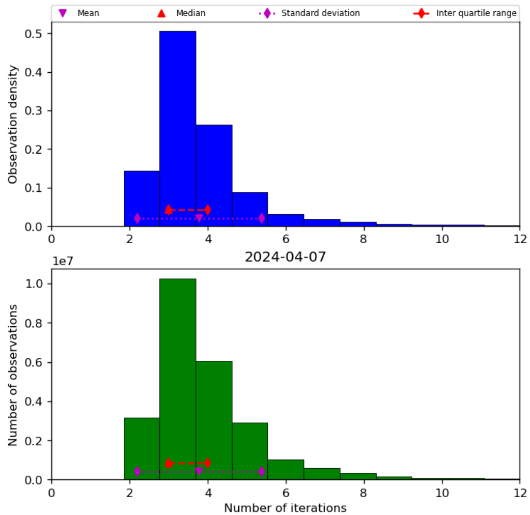
Figure 39: Histogram of “Number of iterations” for 2024-04-06 to 2024-04-08
