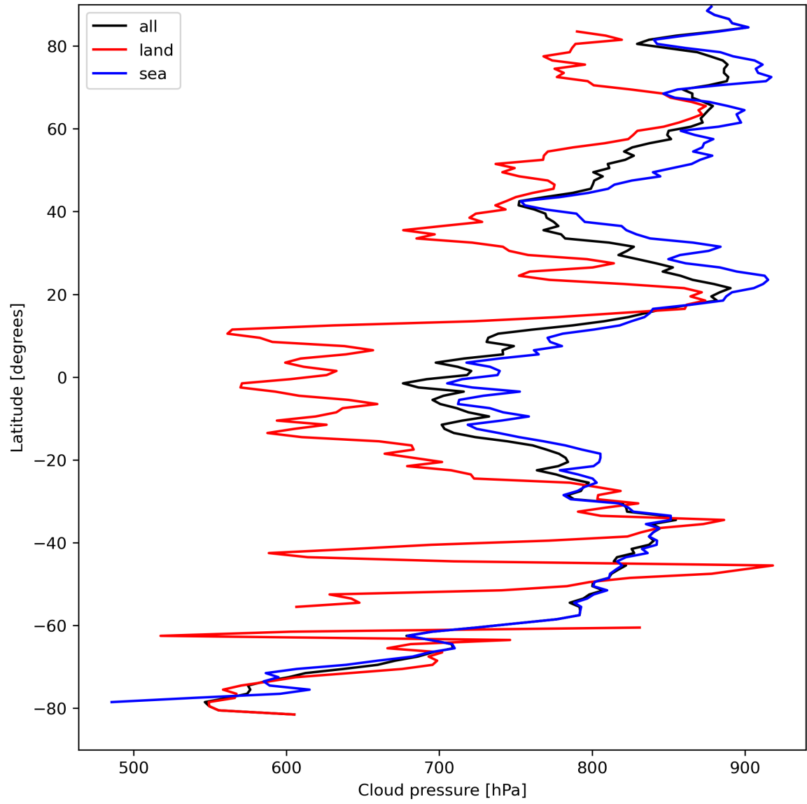
Figure 13: Zonal average of “Cloud pressure” for 2024-04-06 to 2024-04-08.
