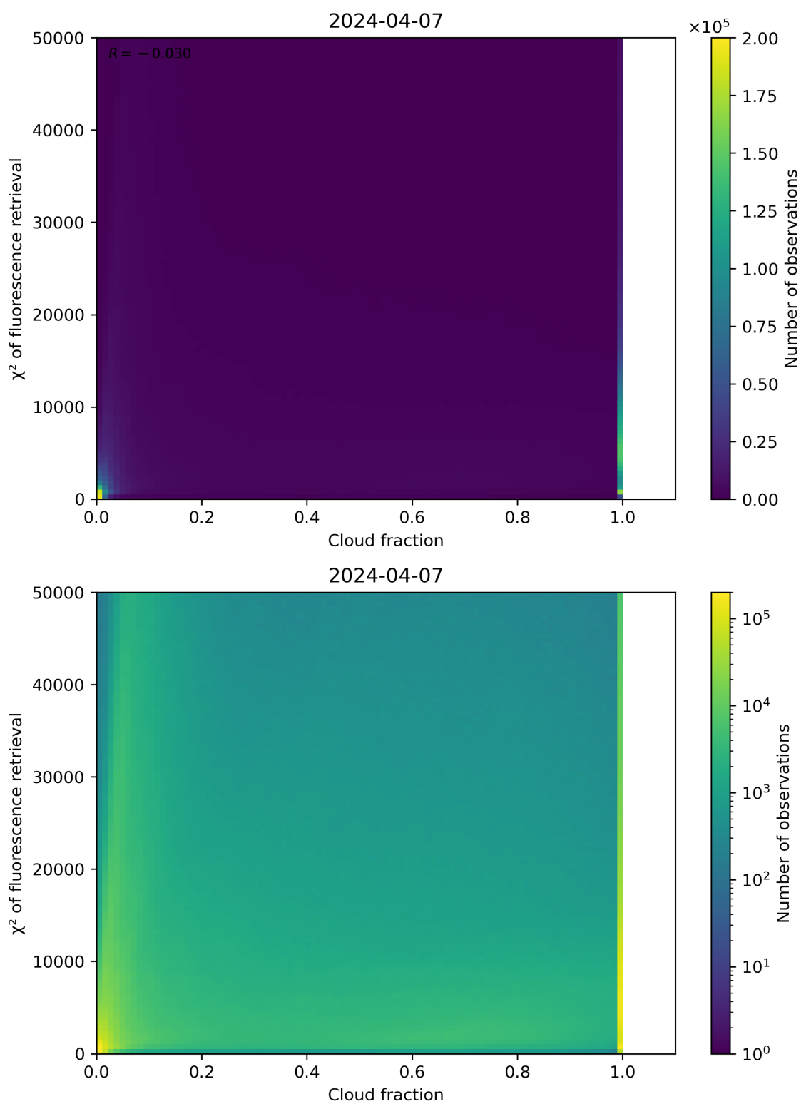
Figure 71: Scatter density plot of “Cloud fraction” against “ \chi^2 of fluorescence retrieval” for 2024-04-06 to 2024-04-08.
