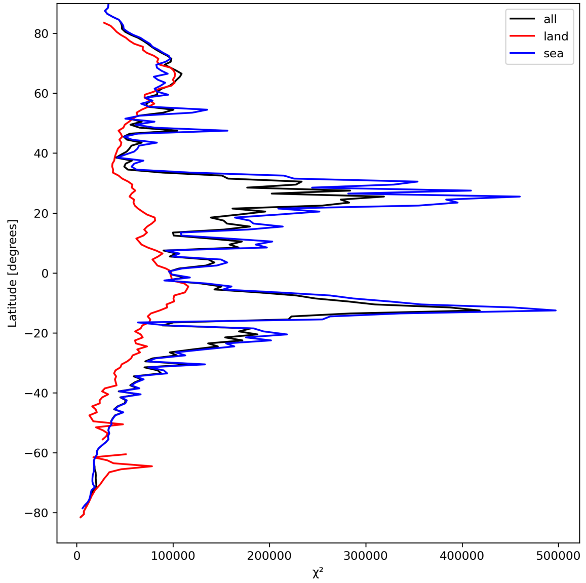
Figure 21: Zonal average of “ \chi^2 ” for 2024-04-06 to 2024-04-08.
