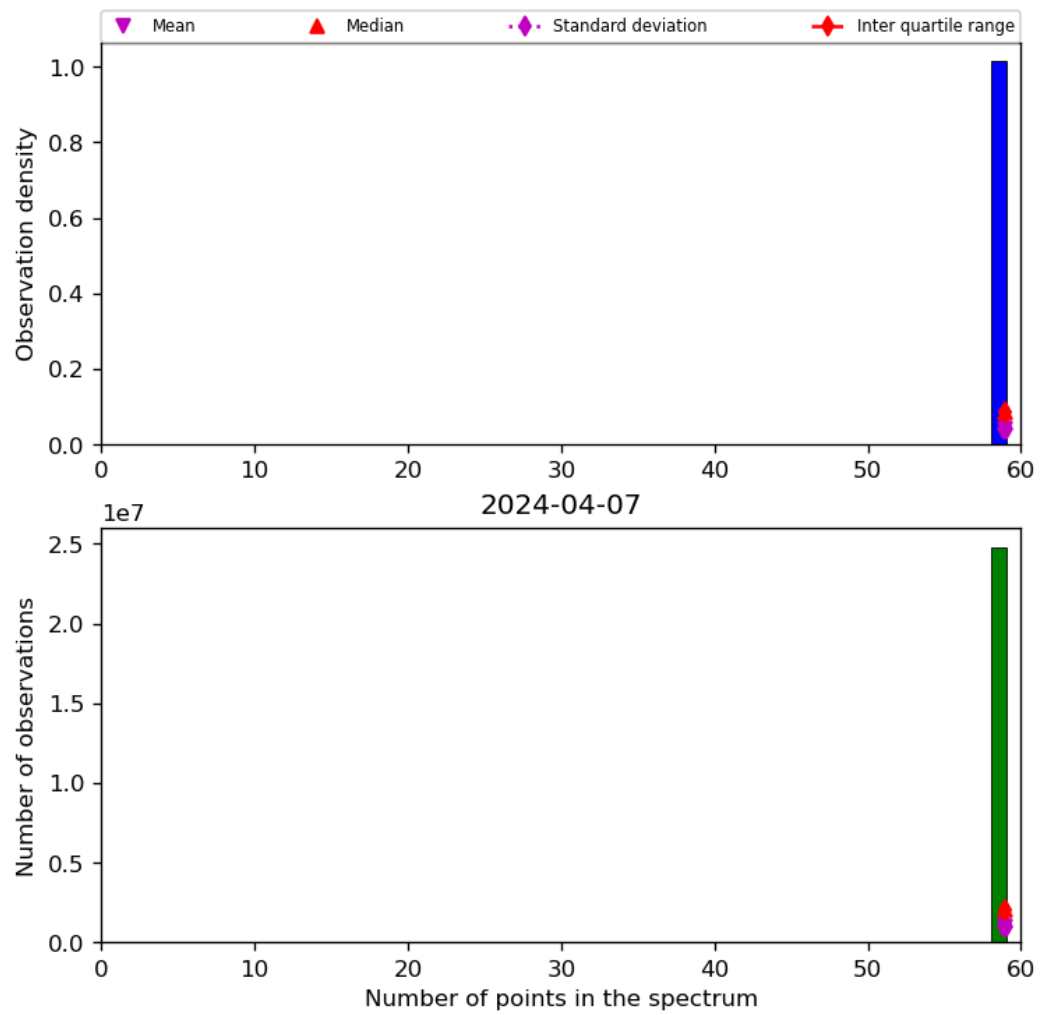
Figure 44: Histogram of “Number of points in the spectrum” for 2024-04-06 to 2024-04-08
