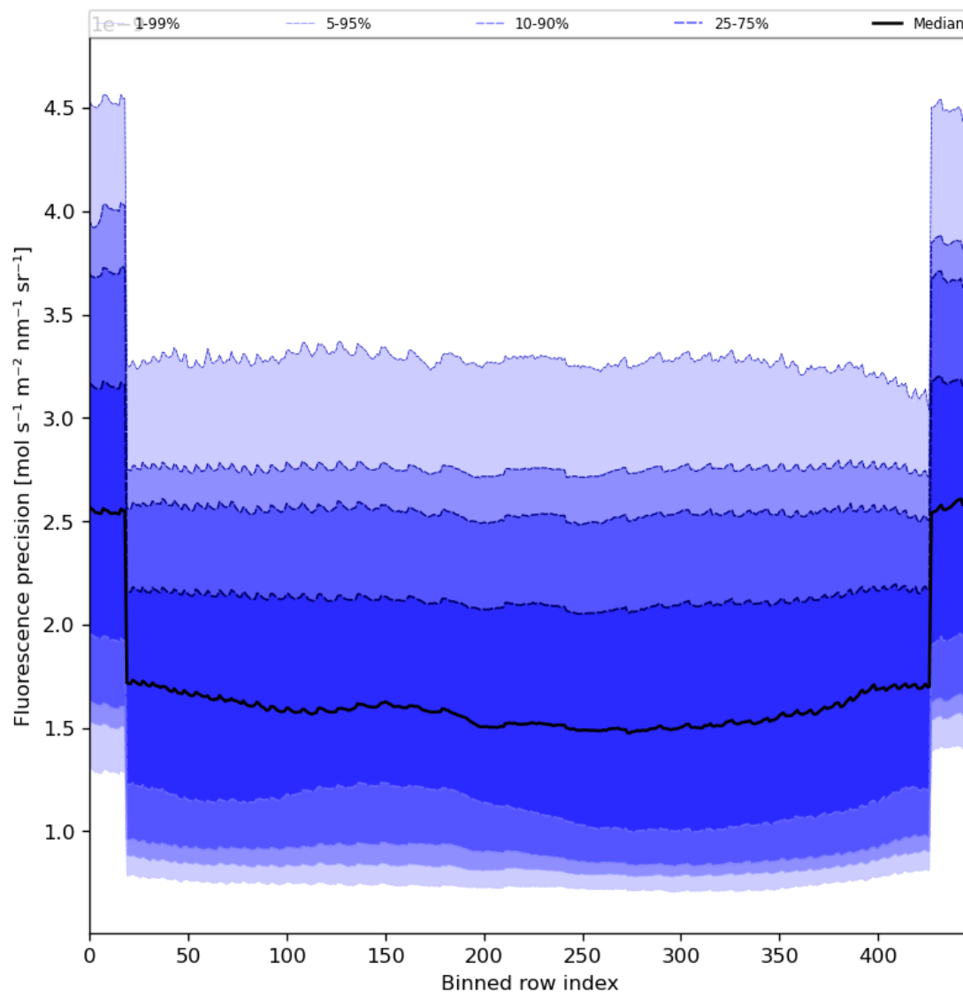
Figure 58: Along track statistics of “Fluorescence precision” for 2024-04-06 to 2024-04-08
