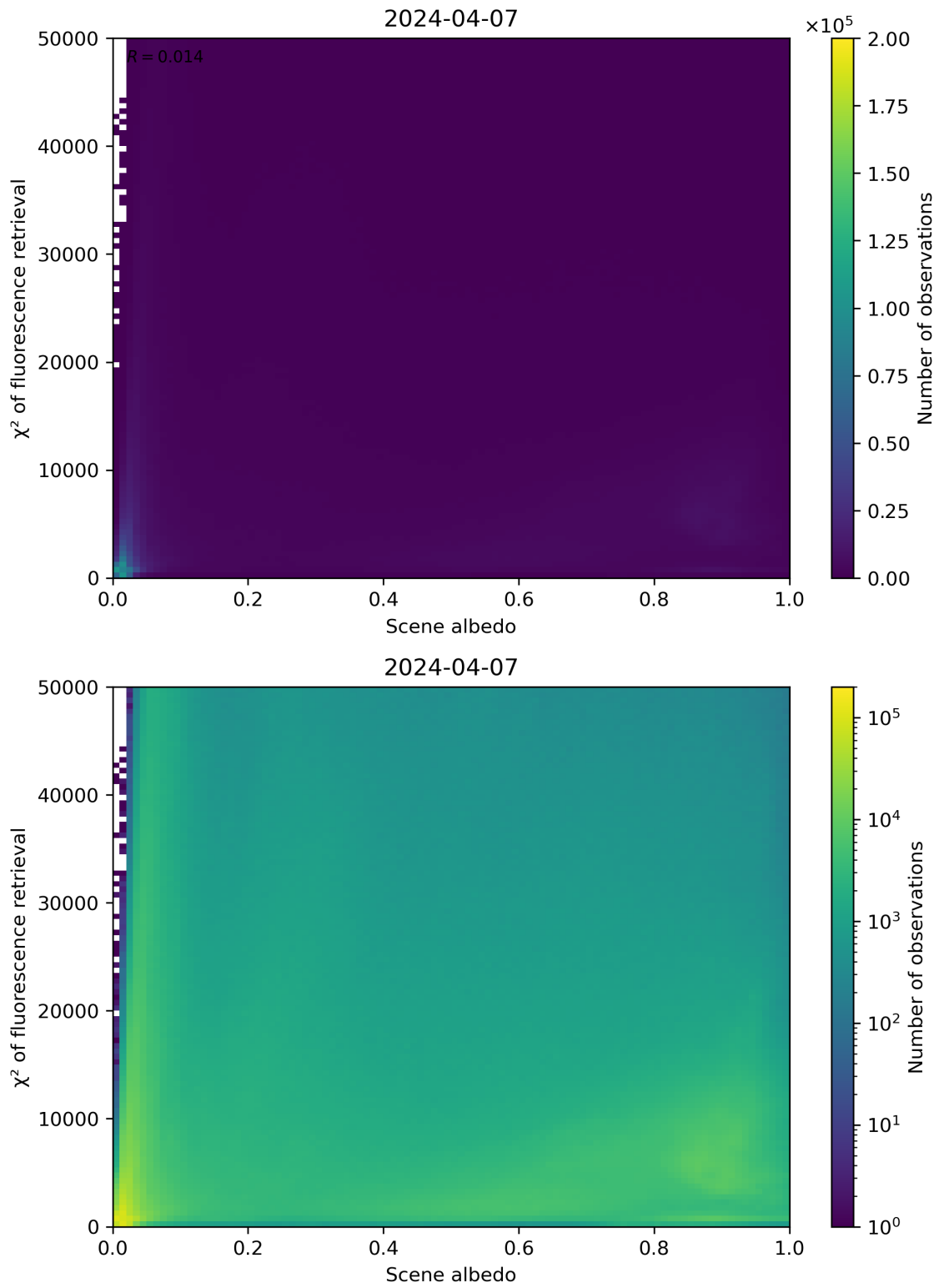
Figure 103: Scatter density plot of “Scene albedo” against “ \chi^2 of fluorescence retrieval” for 2024-04-06 to 2024-04-08.
