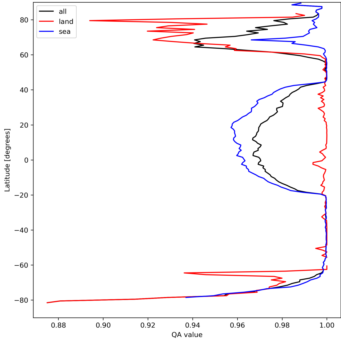
Figure 12: Zonal average of "QA value" for 2024-04-06 to 2024-04-08.
