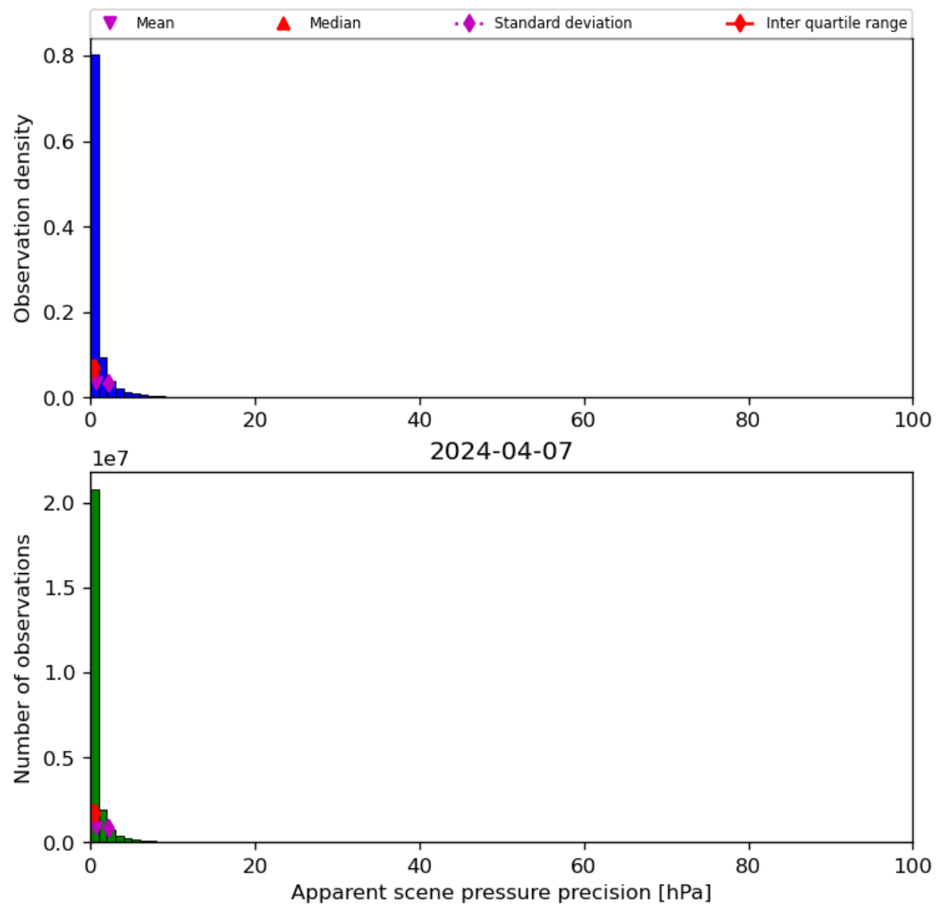
Figure 37: Histogram of “Apparent scene pressure precision” for 2024-04-06 to 2024-04-08
