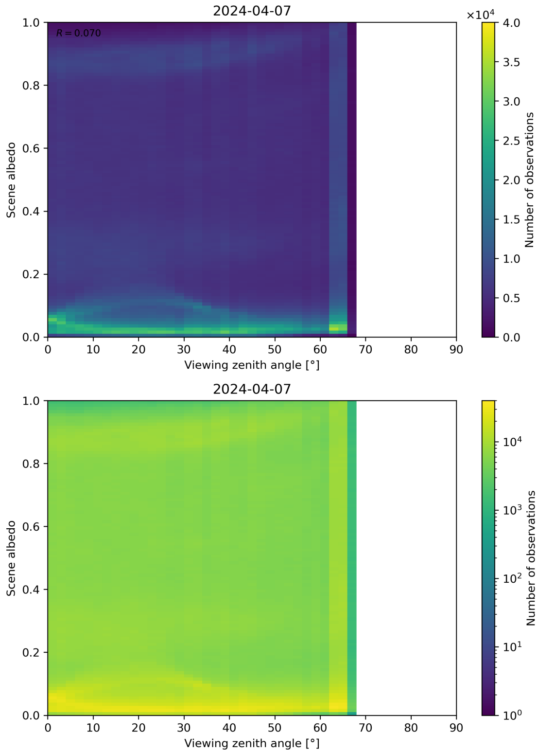
Figure 126: Scatter density plot of “Viewing zenith angle” against “Scene albedo” for 2024-04-06 to 2024-04-08.
