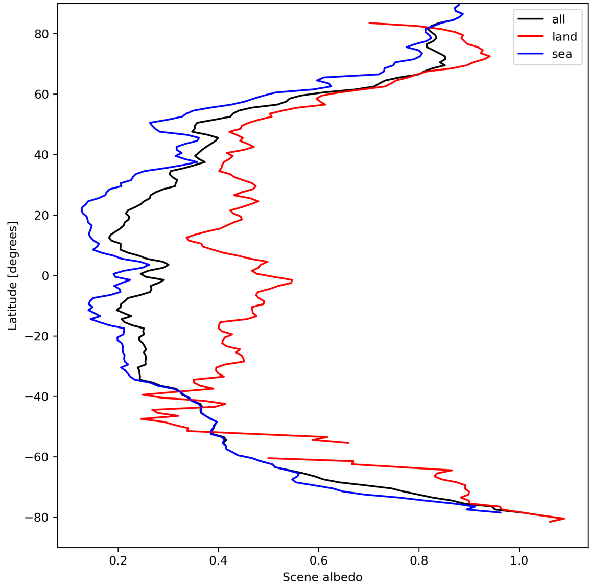
Figure 17: Zonal average of “Scene albedo” for 2024-04-06 to 2024-04-08.
