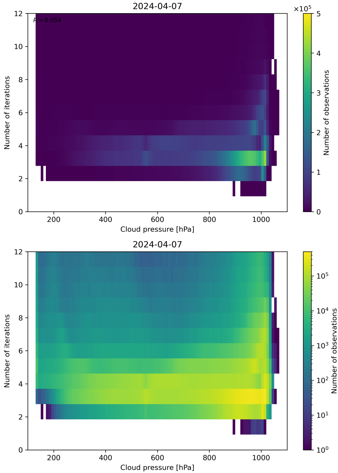
Figure 81: Scatter density plot of “Cloud pressure” against “Number of iterations” for 2024-04-06 to 2024-04-08.
