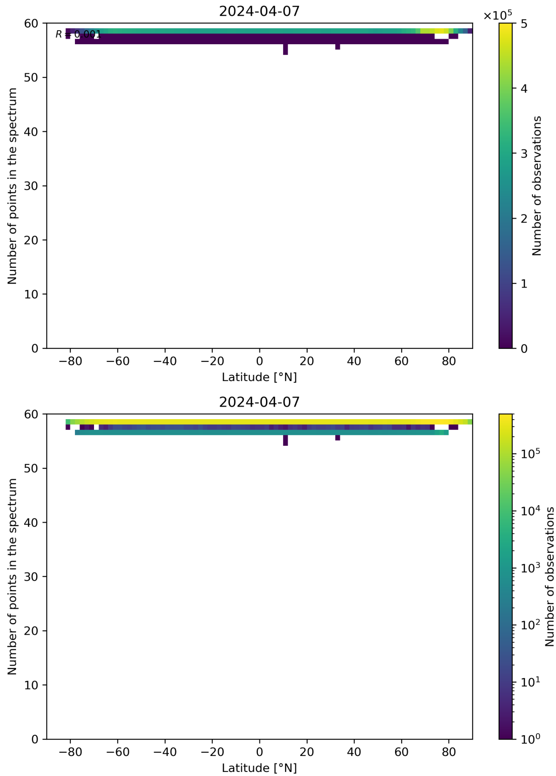
Figure 94: Scatter density plot of “Latitude” against “Number of points in the spectrum” for 2024-04-06 to 2024-04-08.
