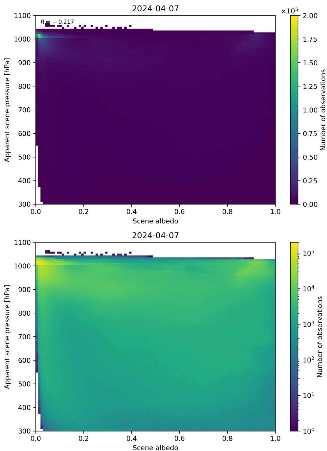
Figure 102: Scatter density plot of “Scene albedo” against “Apparent scene pressure” for 2024-04-06 to 2024-04-08.
