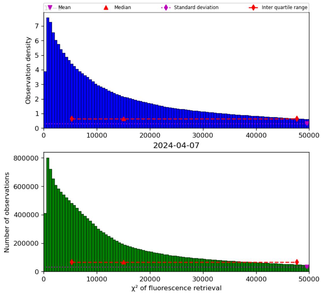
Figure 42: Histogram of “ \chi^2 of fluorescence retrieval” for 2024-04-06 to 2024-04-08
