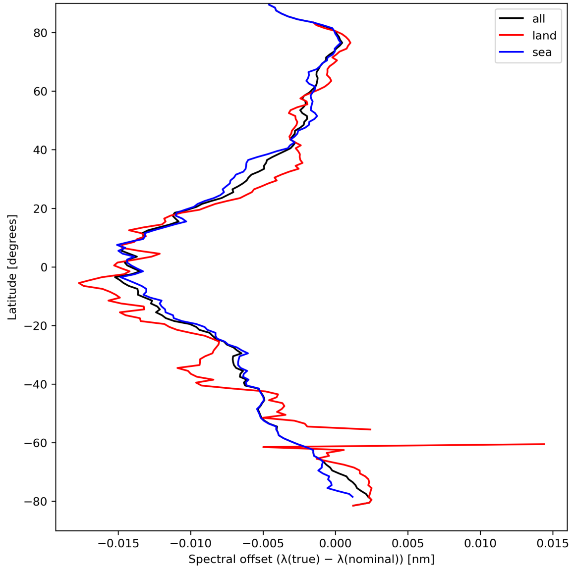
Figure 28: Zonal average of “Spectral offset ( \lambda(\text{true}) - \lambda(\text{nominal}) )” for 2024-04-06 to 2024-04-08.
