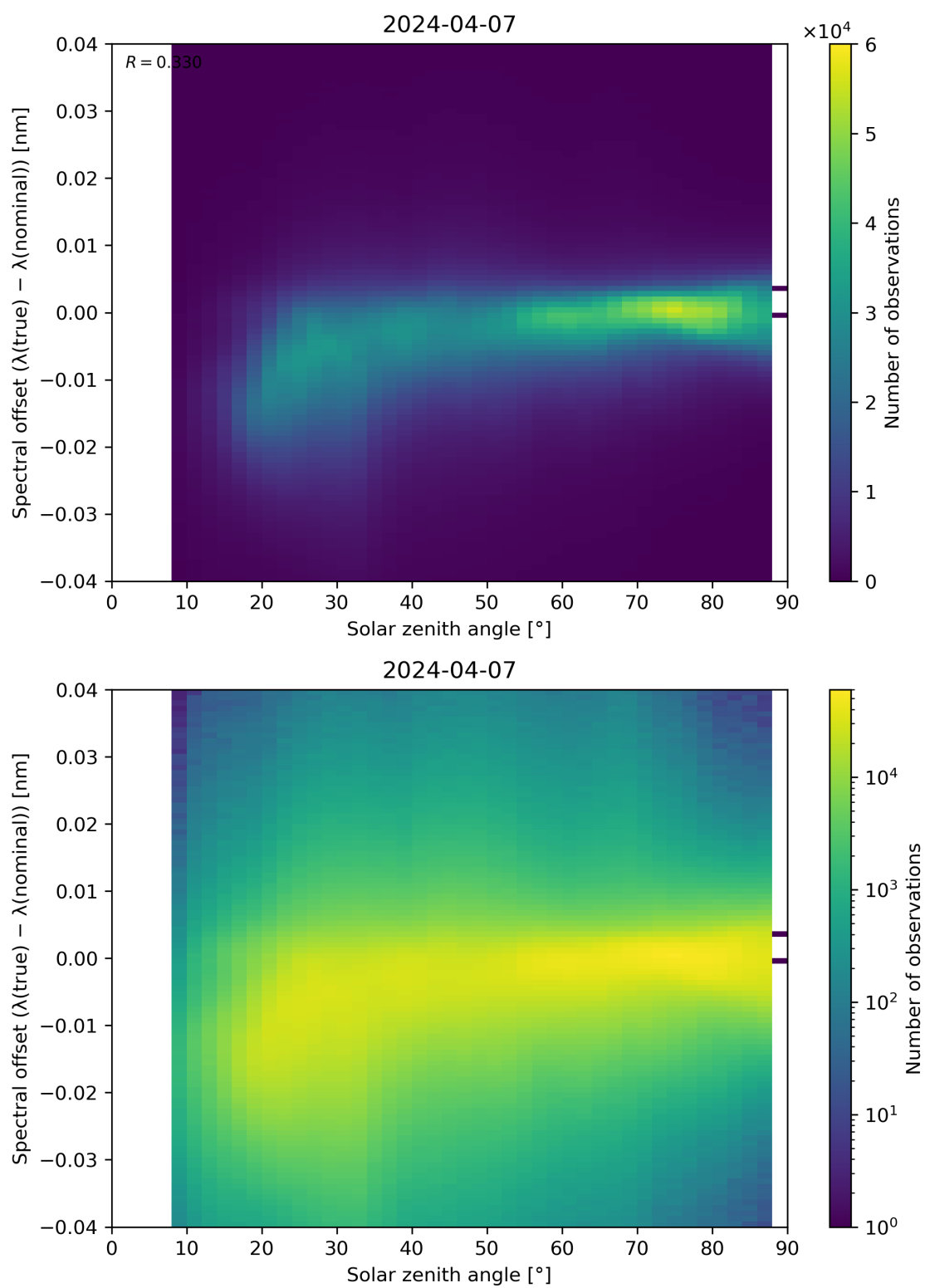
Figure 117: Scatter density plot of “Solar zenith angle” against “Spectral offset ( \lambda(\text{true}) - \lambda(\text{nominal}) )” for 2024-04-06 to 2024-04-08.
