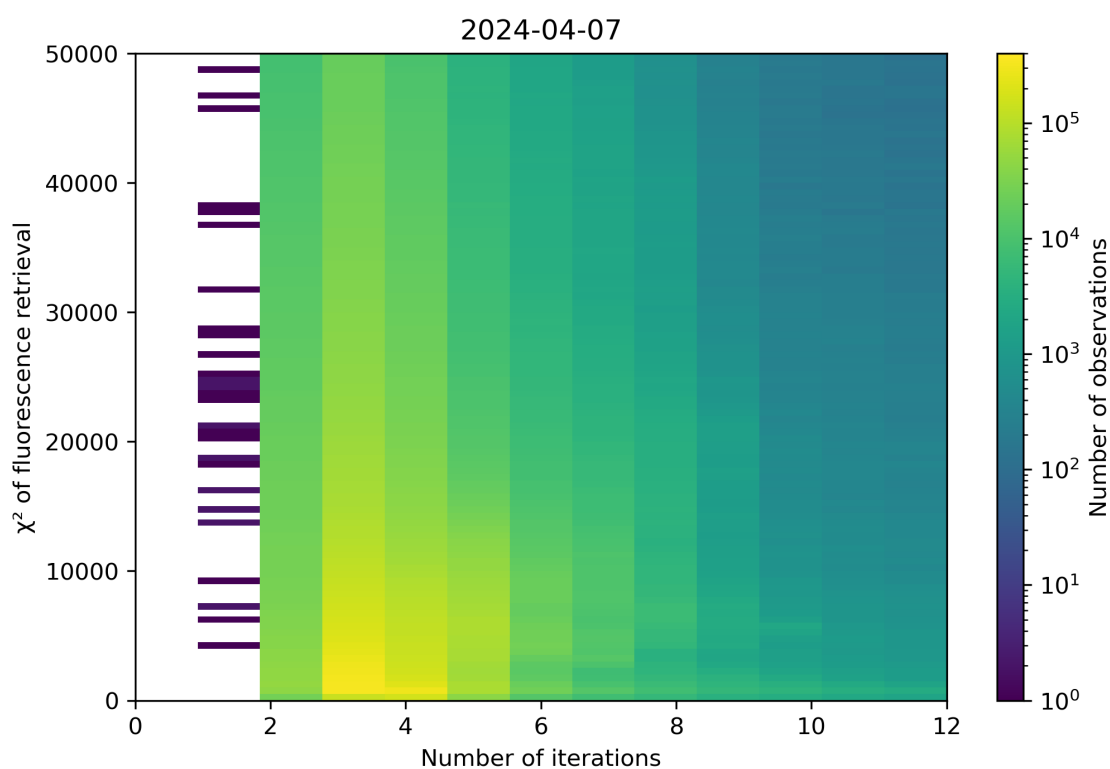
Figure 97: Scatter density plot of “Number of iterations” against “ \chi^2 of fluorescence retrieval” for 2024-04-06 to 2024-04-08.
