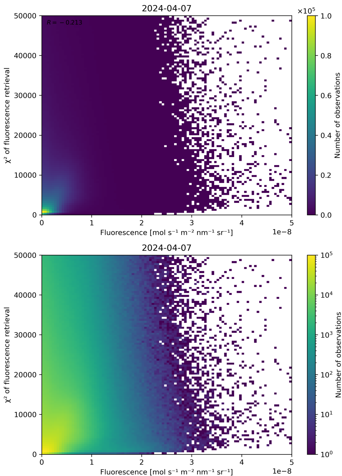
Figure 85: Scatter density plot of “Fluorescence” against “ \chi^2 of fluorescence retrieval” for 2024-04-06 to 2024-04-08.
