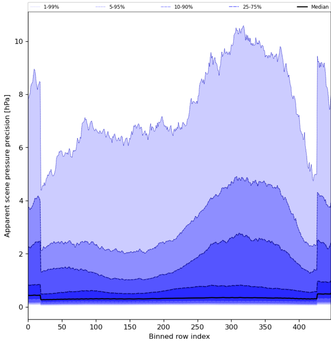
Figure 54: Along track statistics of “Apparent scene pressure precision” for 2024-04-06 to 2024-04-08
