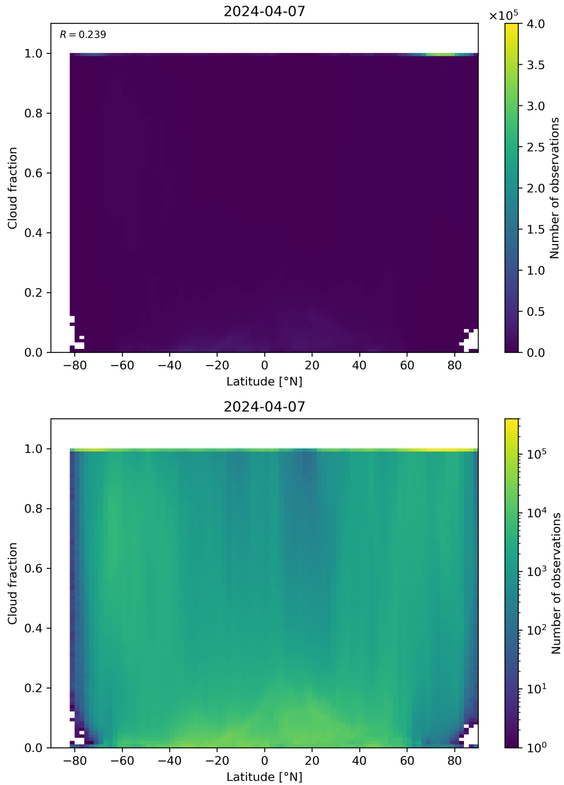
Figure 90: Scatter density plot of “Latitude” against “Cloud fraction” for 2024-04-06 to 2024-04-08.
