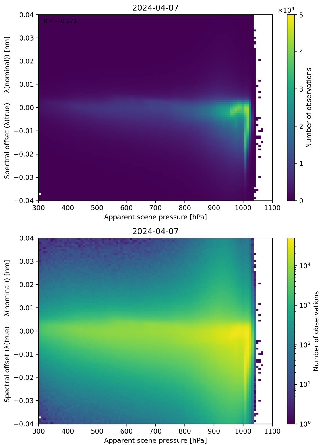
Figure 67: Scatter density plot of “Apparent scene pressure” against “Spectral offset ( \lambda(\text{true}) - \lambda(\text{nominal}) )” for 2024-04-06 to 2024-04-08.
