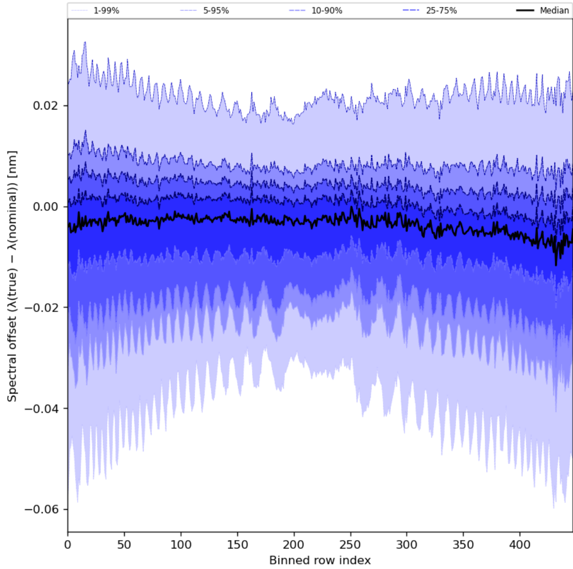
Figure 62: Along track statistics of “Spectral offset ( \lambda(\text{true}) - \lambda(\text{nominal}) )” for 2024-04-06 to 2024-04-08
