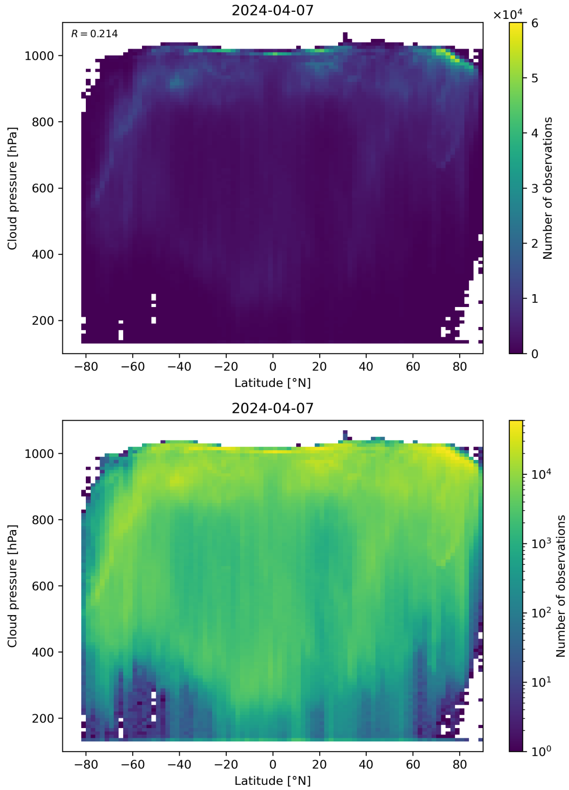
Figure 91: Scatter density plot of “Latitude” against “Cloud pressure” for 2024-04-06 to 2024-04-08.
