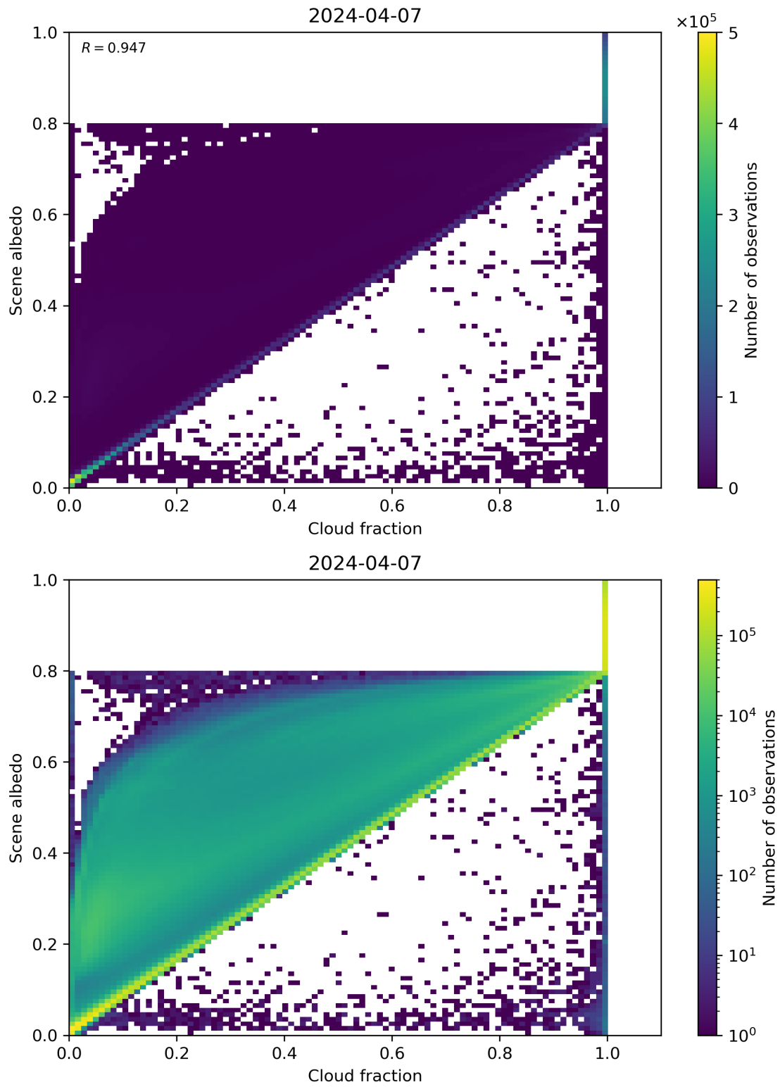
Figure 75: Scatter density plot of “Cloud fraction” against “Scene albedo” for 2024-04-06 to 2024-04-08.
