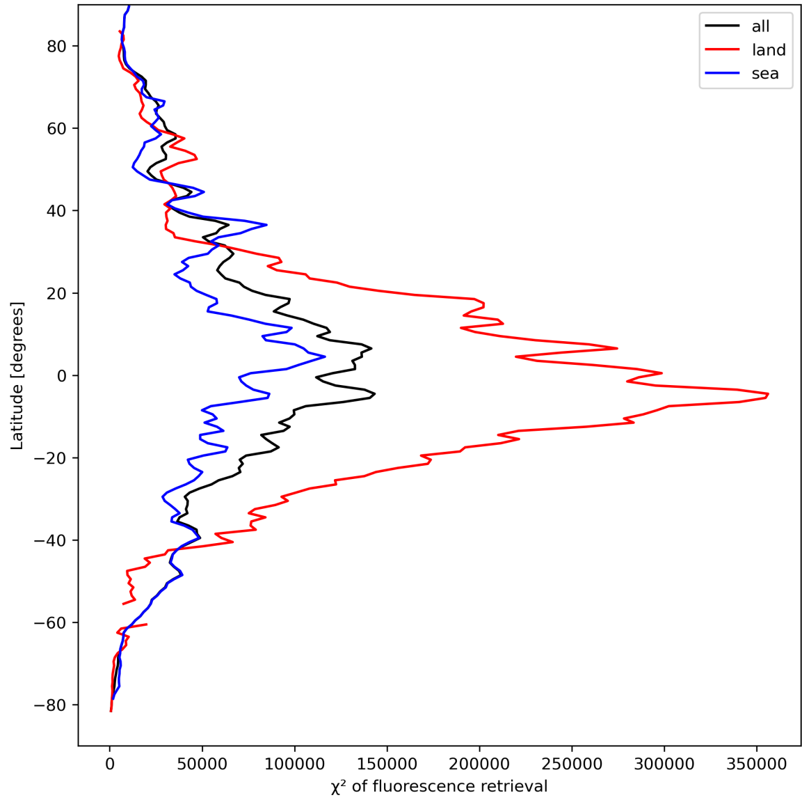
Figure 25: Zonal average of “ \chi^2 of fluorescence retrieval” for 2024-04-06 to 2024-04-08.
