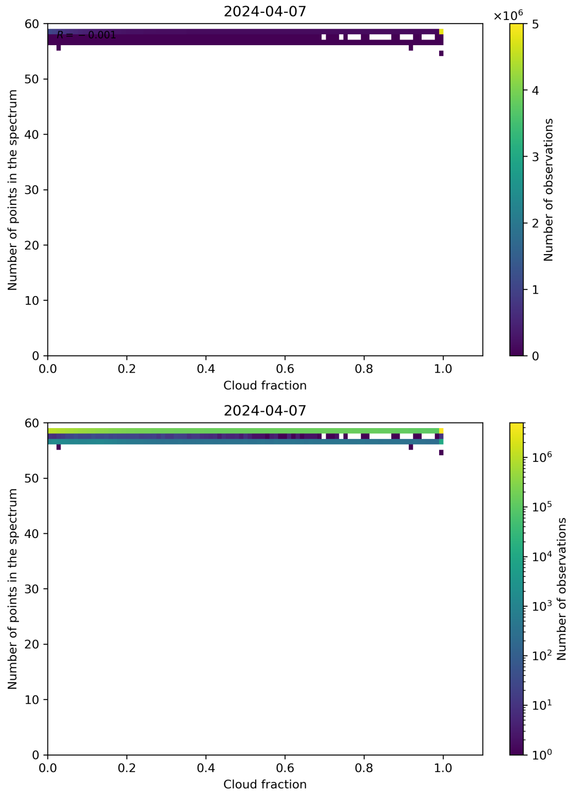
Figure 74: Scatter density plot of “Cloud fraction” against “Number of points in the spectrum” for 2024-04-06 to 2024-04-08.
