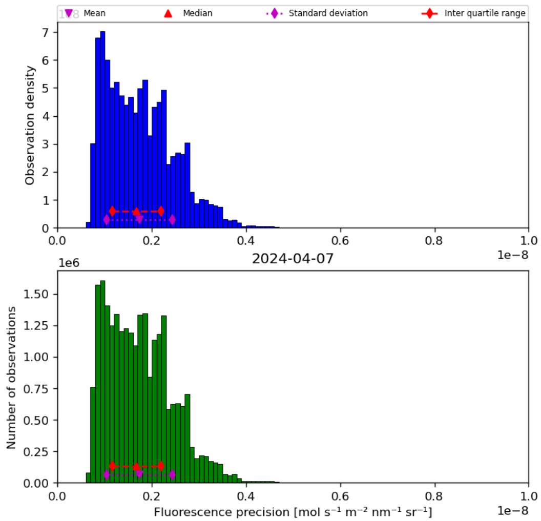
Figure 41: Histogram of “Fluorescence precision” for 2024-04-06 to 2024-04-08
