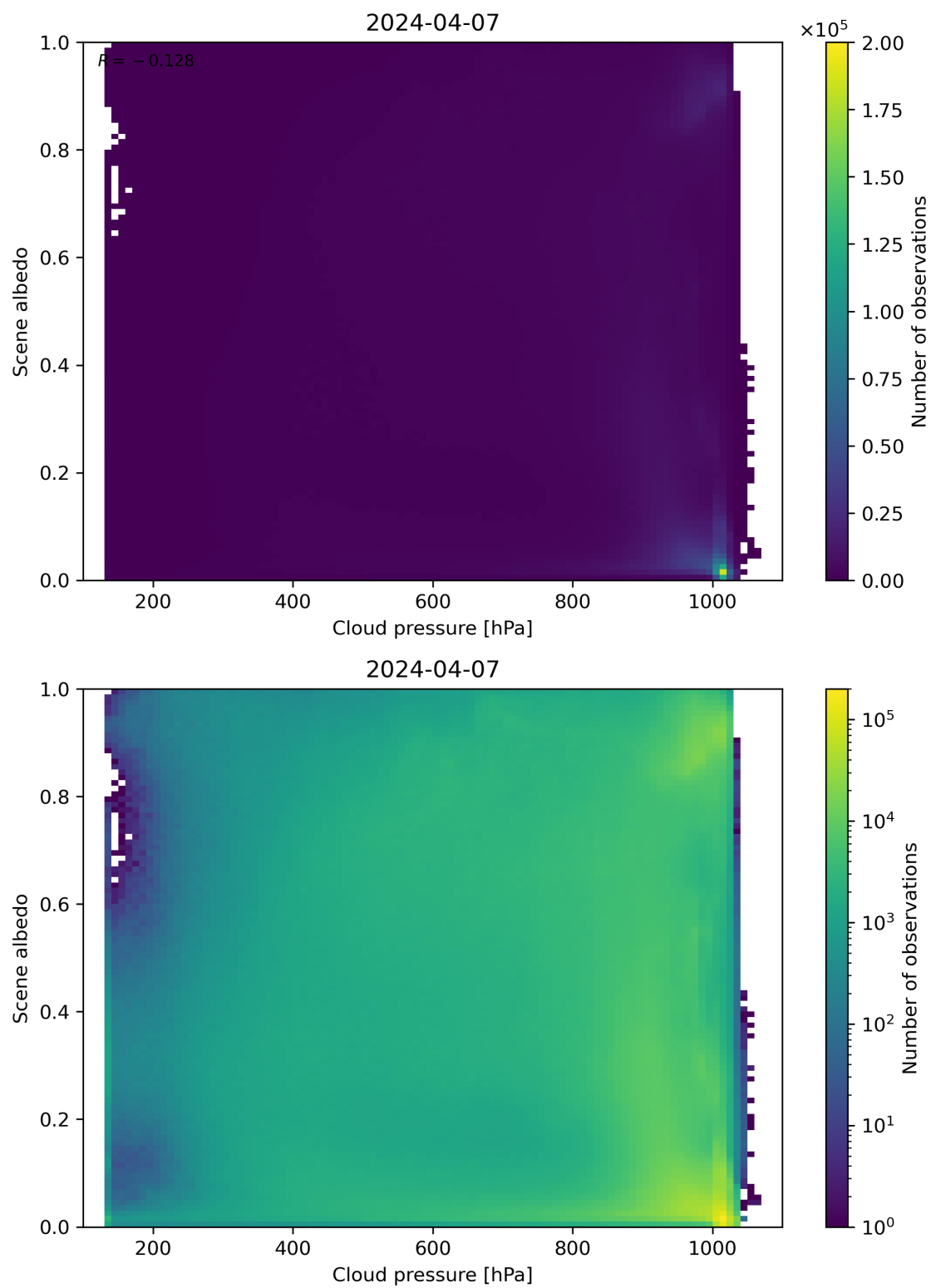
Figure 83: Scatter density plot of “Cloud pressure” against “Scene albedo” for 2024-04-06 to 2024-04-08.
