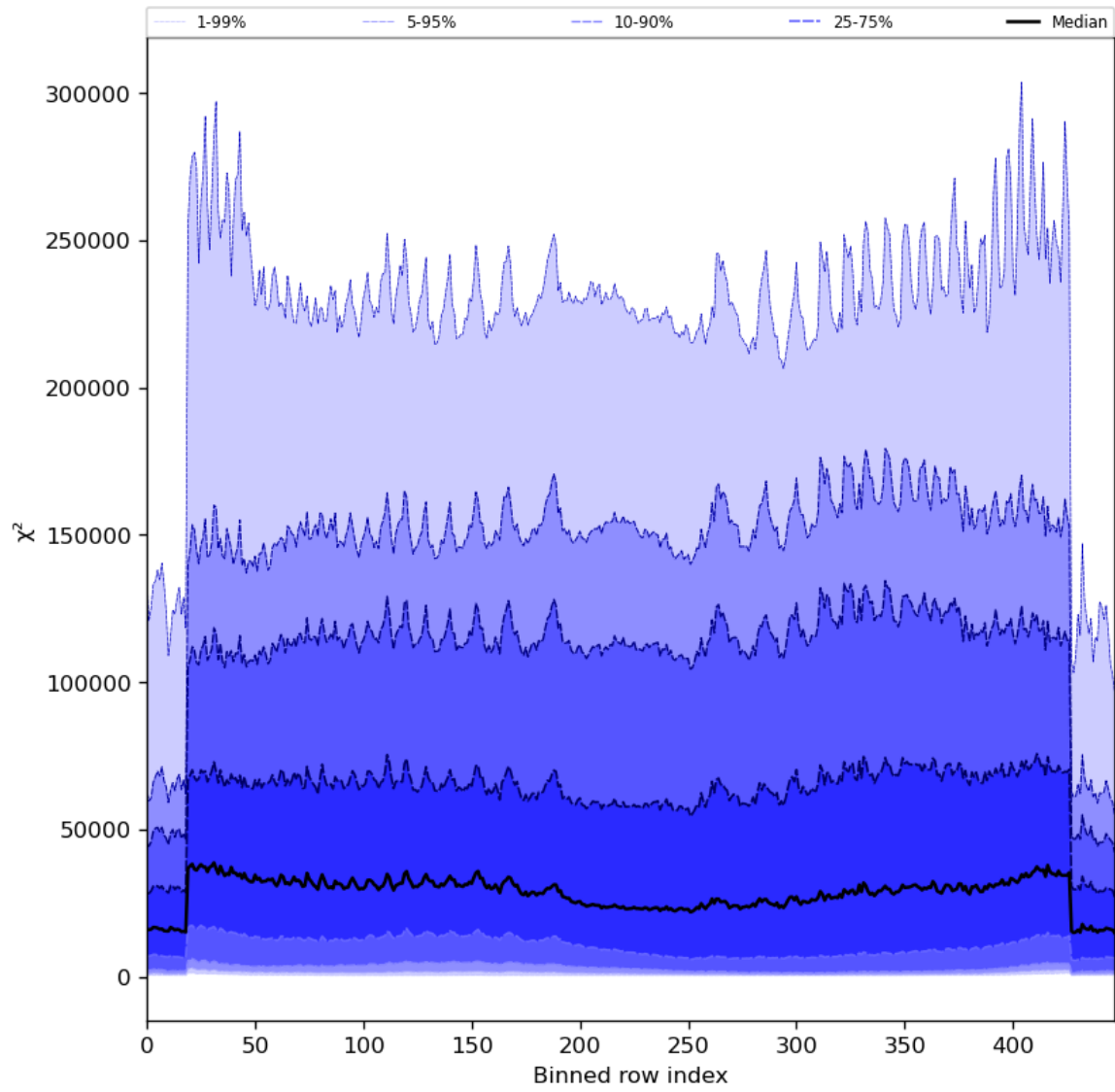
Figure 55: Along track statistics of “ \chi^2 ” for 2024-04-06 to 2024-04-08
