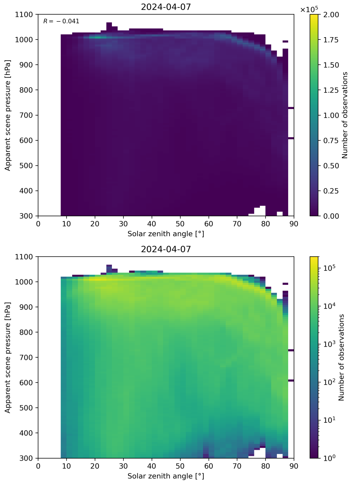
Figure 108: Scatter density plot of “Solar zenith angle” against “Apparent scene pressure” for 2024-04-06 to 2024-04-08.
