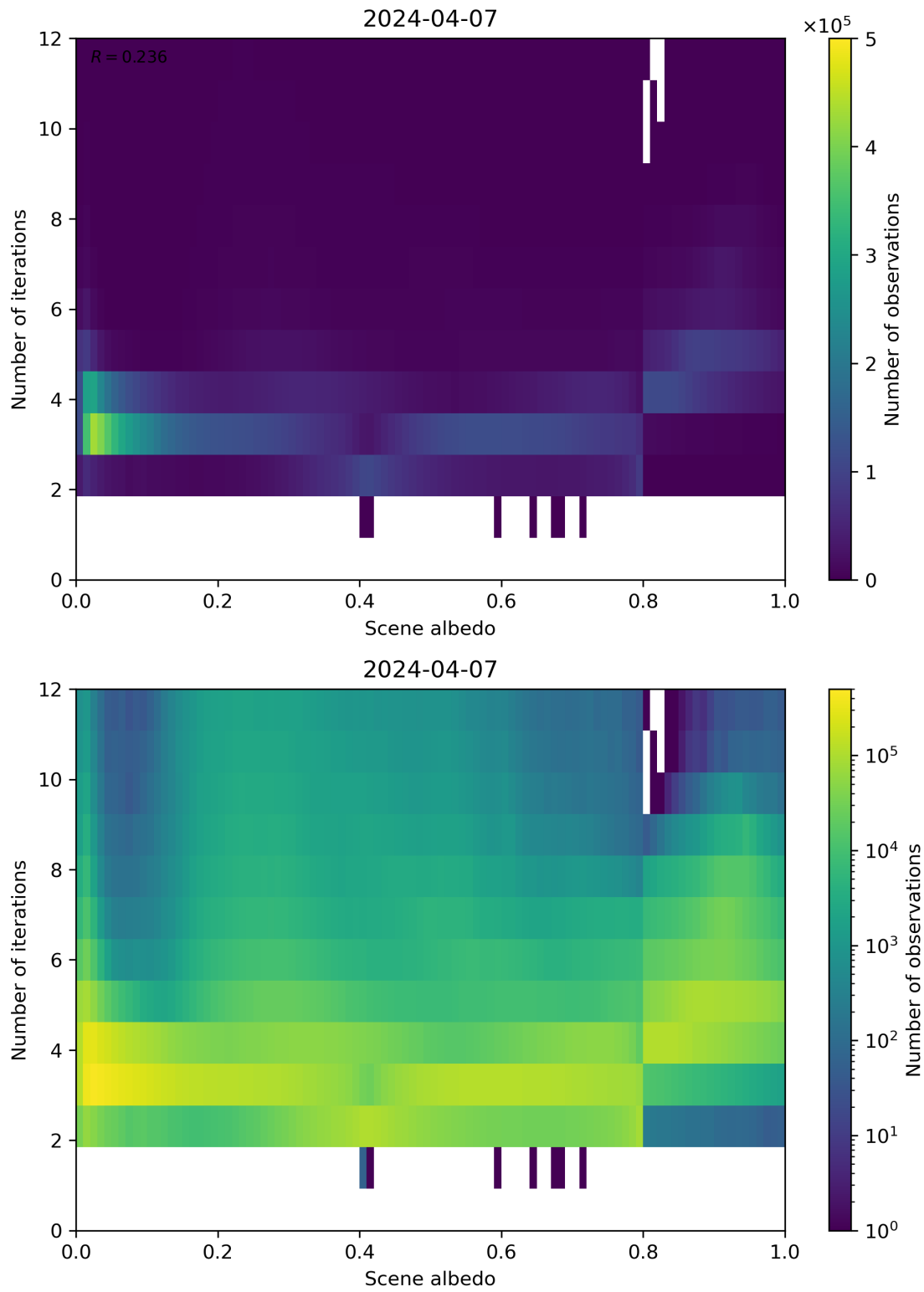
Figure 105: Scatter density plot of “Scene albedo” against “Number of iterations” for 2024-04-06 to 2024-04-08.
