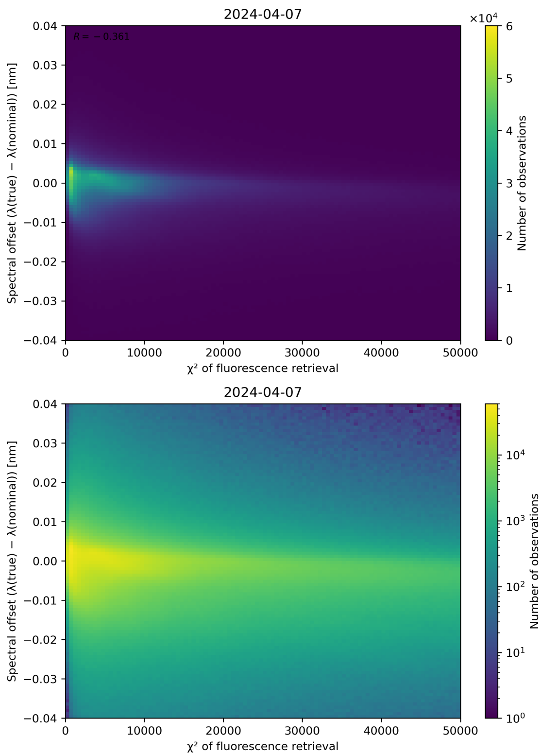
Figure 69: Scatter density plot of " \chi^2 of fluorescence retrieval" against "Spectral offset ( \lambda(\text{true}) - \lambda(\text{nominal}) )" for 2024-04-06 to 2024-04-08.
