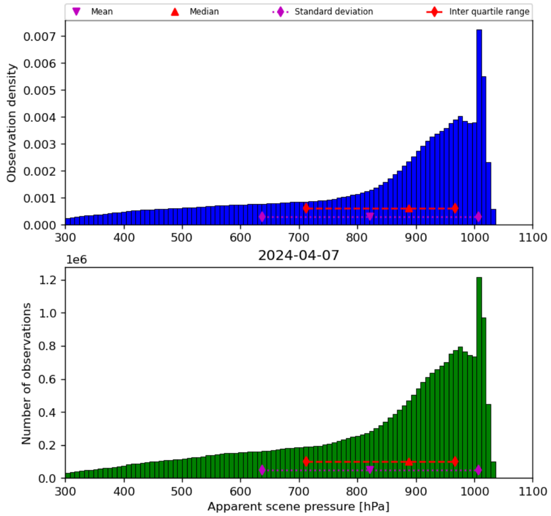
Figure 36: Histogram of “Apparent scene pressure” for 2024-04-06 to 2024-04-08
