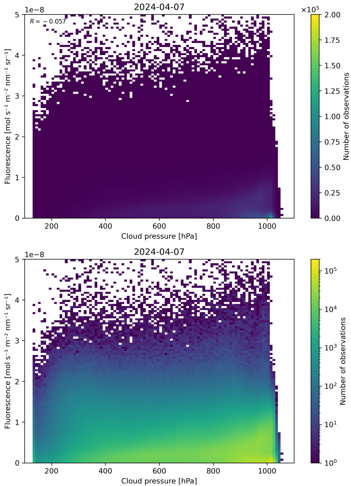
Figure 80: Scatter density plot of “Cloud pressure” against “Fluorescence” for 2024-04-06 to 2024-04-08.
