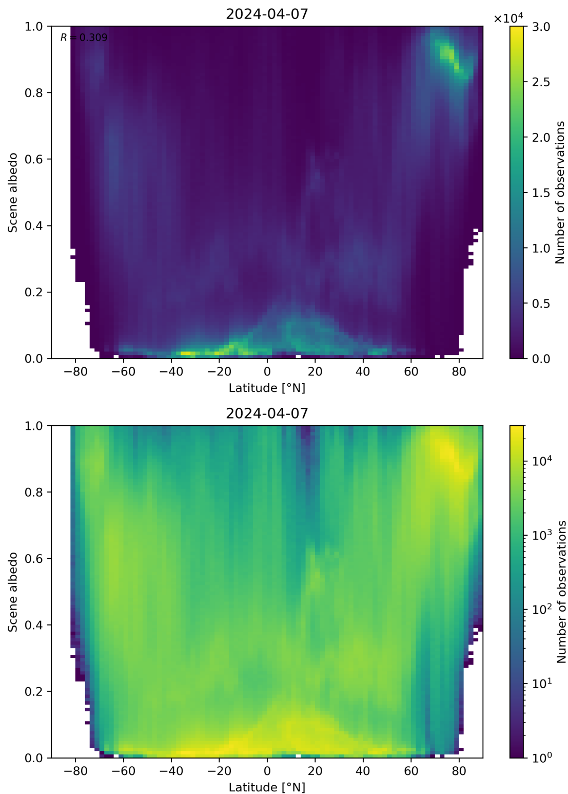
Figure 95: Scatter density plot of “Latitude” against “Scene albedo” for 2024-04-06 to 2024-04-08.
