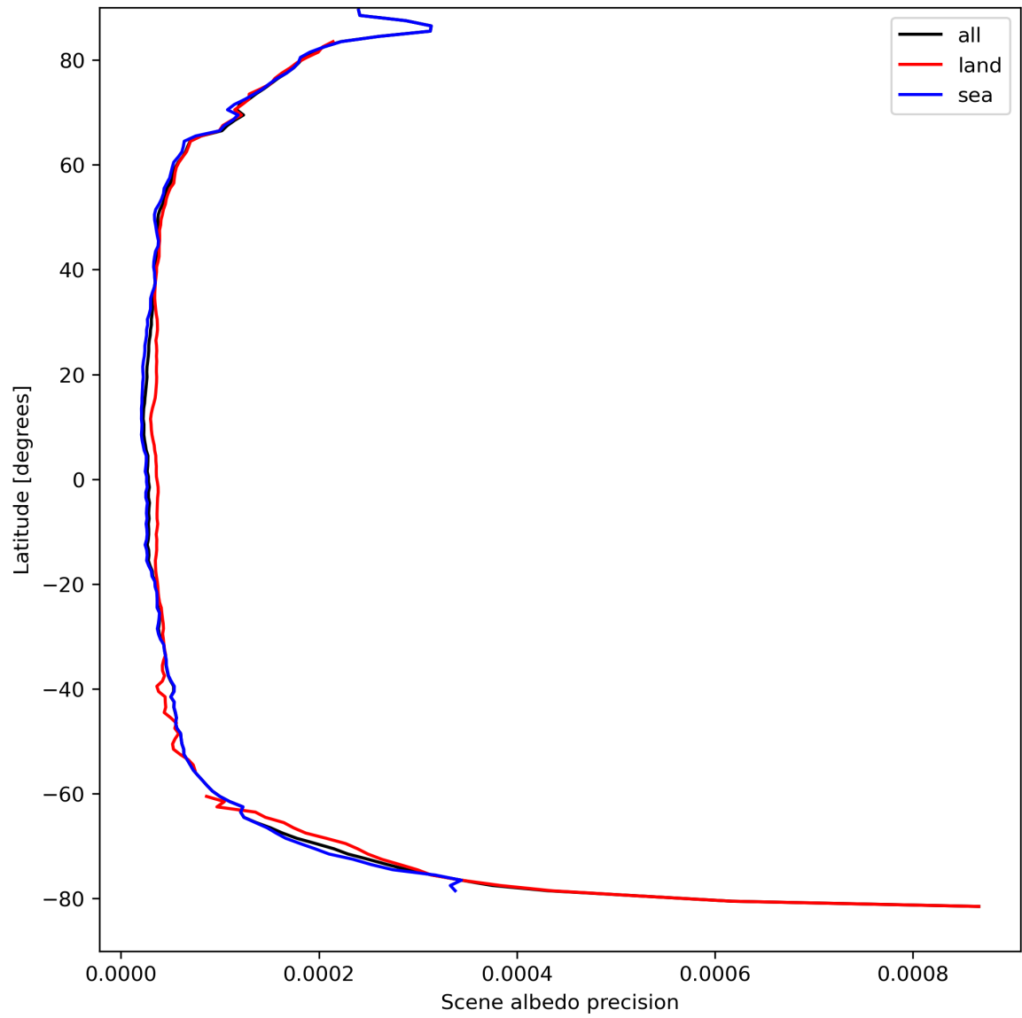
Figure 18: Zonal average of “Scene albedo precision” for 2024-04-06 to 2024-04-08.
