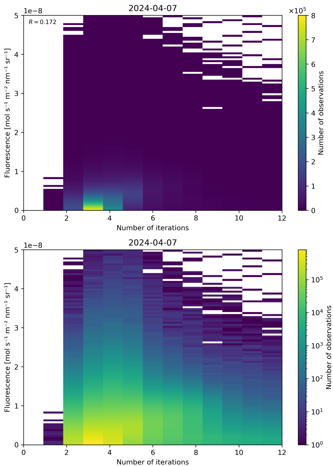
Figure 98: Scatter density plot of “Number of iterations” against “Fluorescence” for 2024-04-06 to 2024-04-08.
