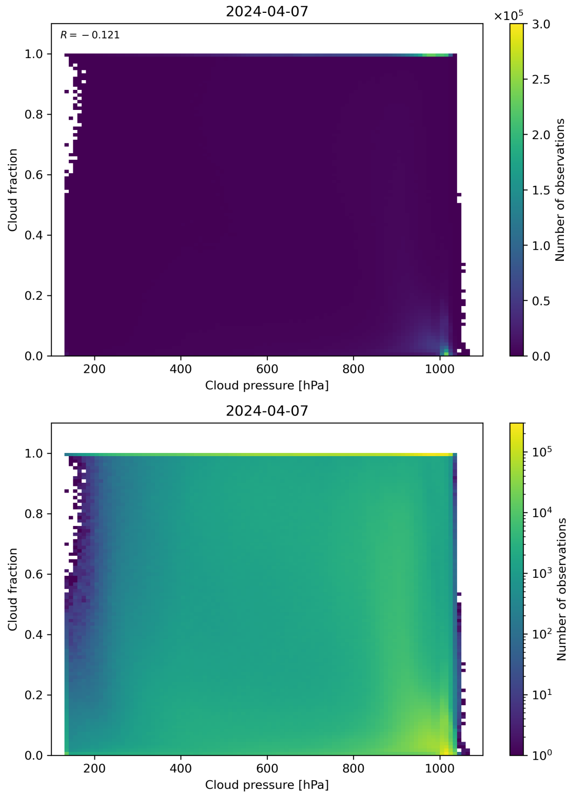
Figure 79: Scatter density plot of “Cloud pressure” against “Cloud fraction” for 2024-04-06 to 2024-04-08.
