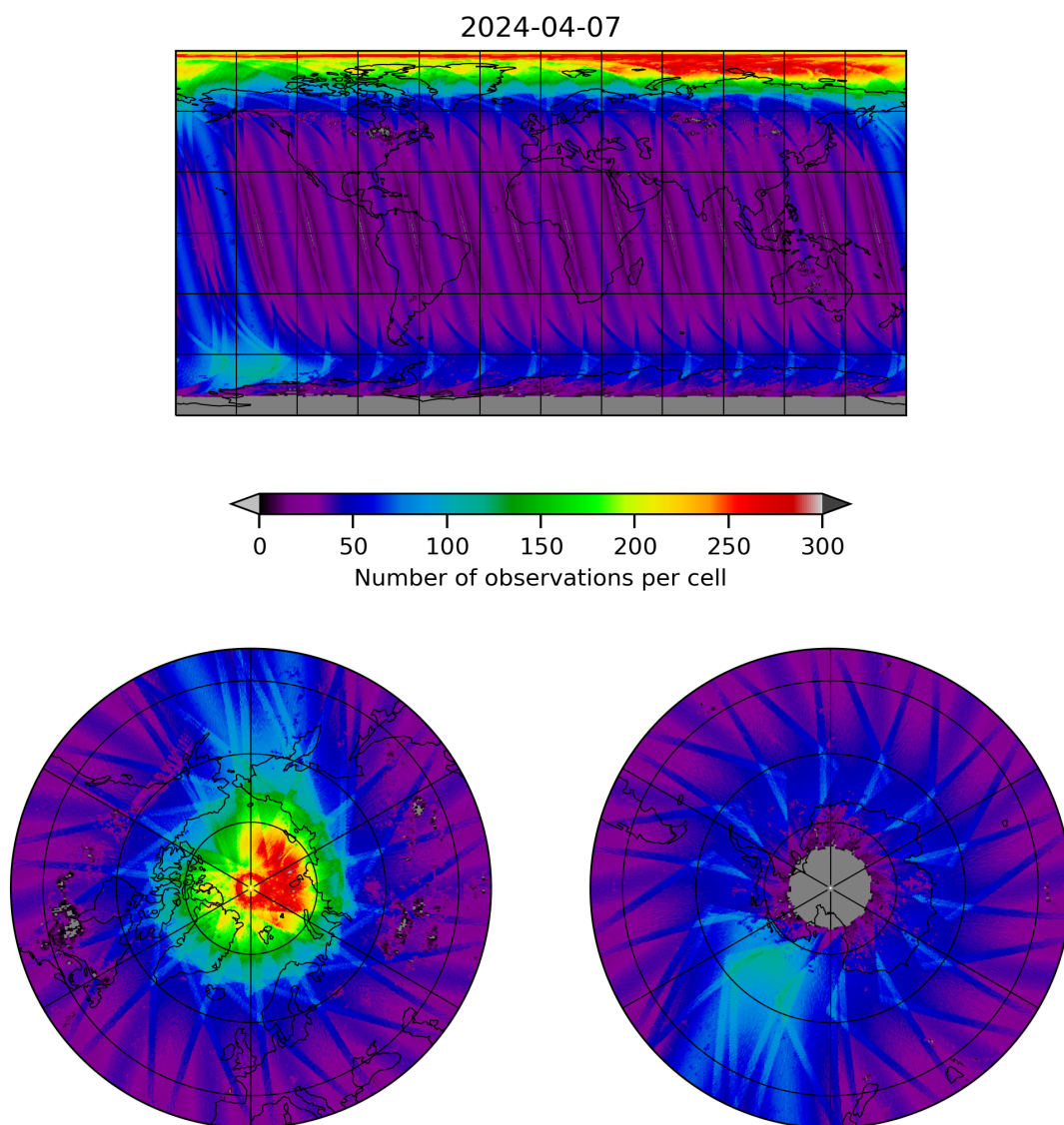
Figure 11: Map of the number of observations for 2024-04-06 to 2024-04-08
