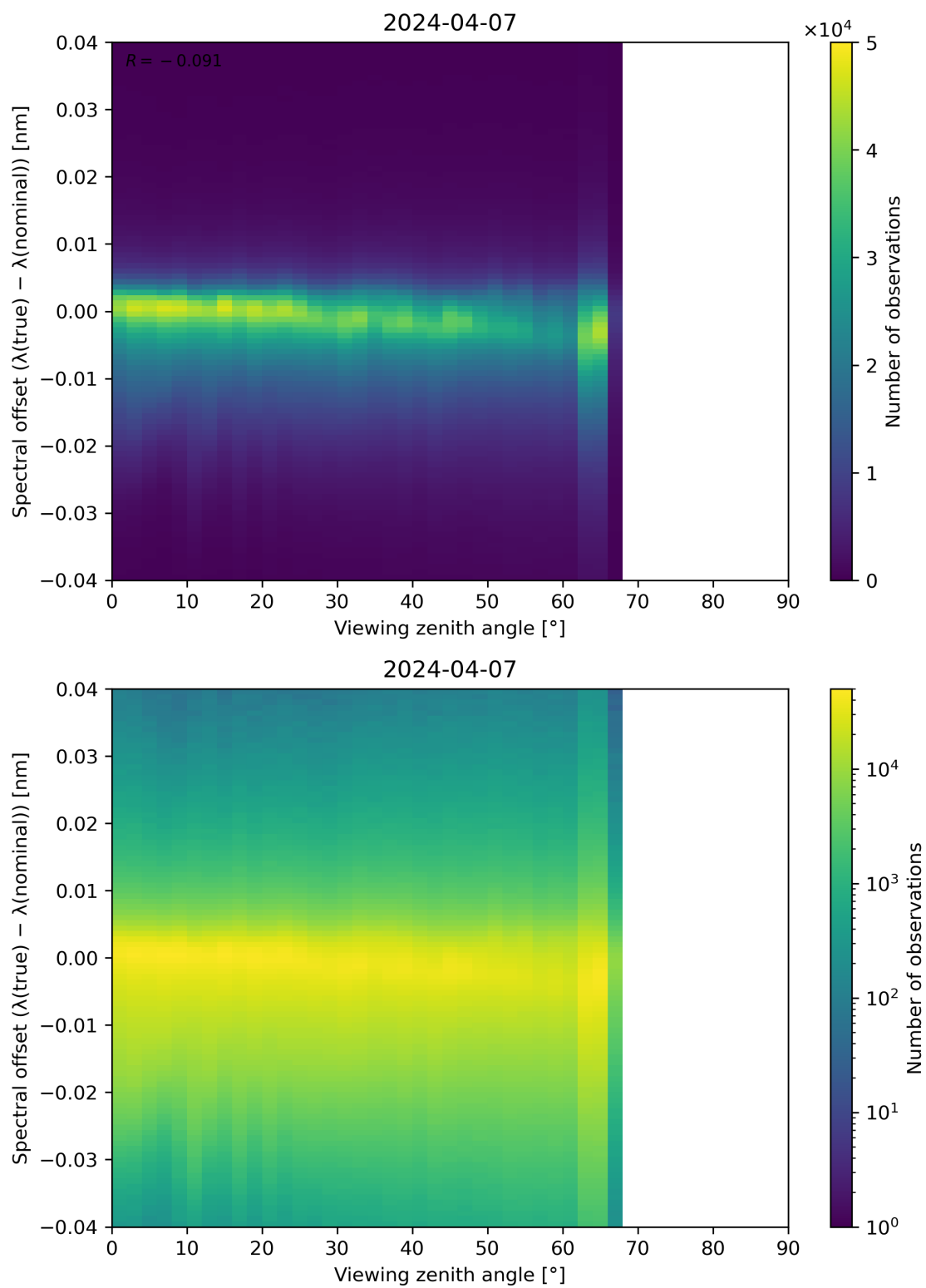
Figure 128: Scatter density plot of “Viewing zenith angle” against “Spectral offset ( \lambda(\text{true}) - \lambda(\text{nominal}) )” for 2024-04-06 to 2024-04-08.
