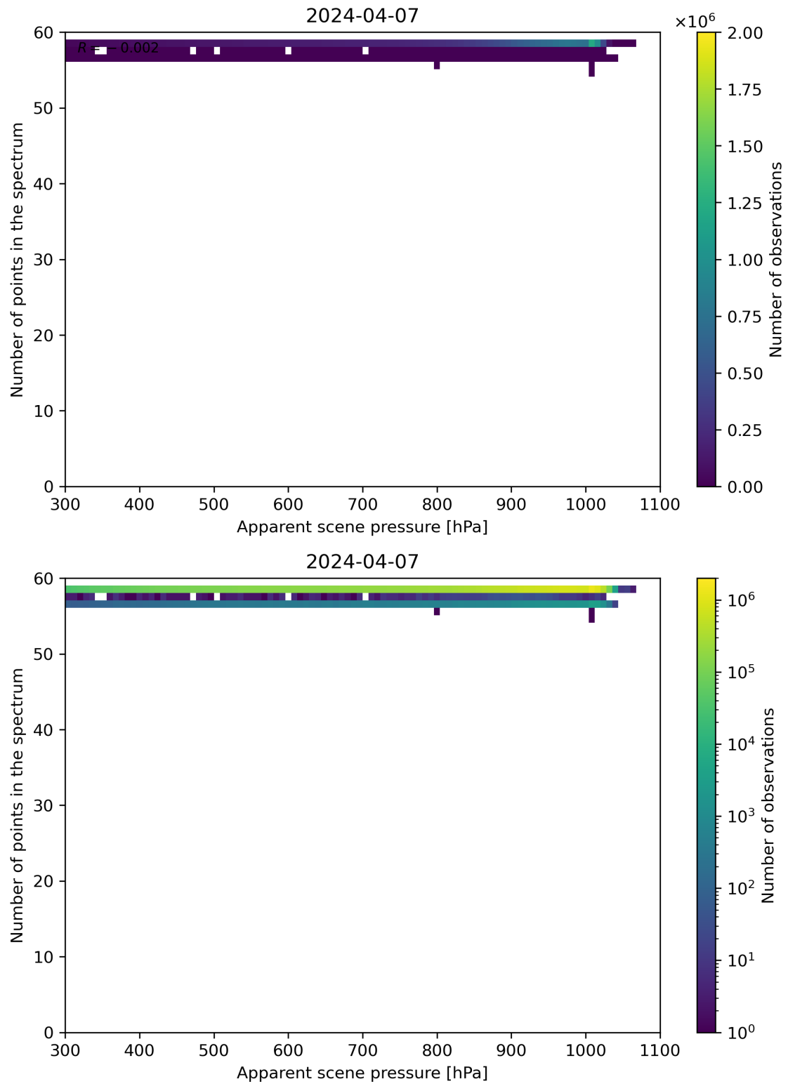
Figure 66: Scatter density plot of “Apparent scene pressure” against “Number of points in the spectrum” for 2024-04-06 to 2024-04-08.
