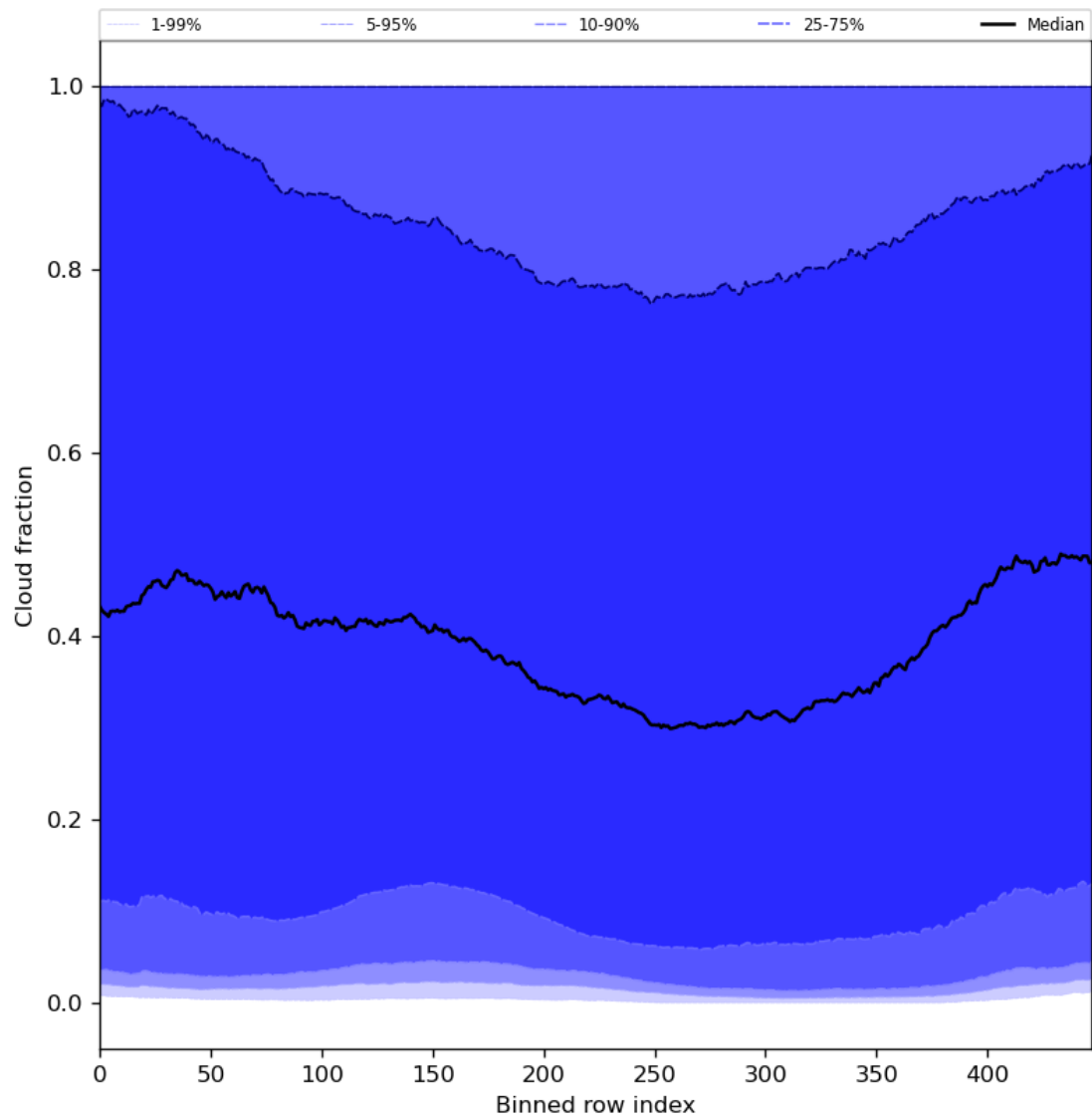
Figure 49: Along track statistics of “Cloud fraction” for 2024-04-06 to 2024-04-08
