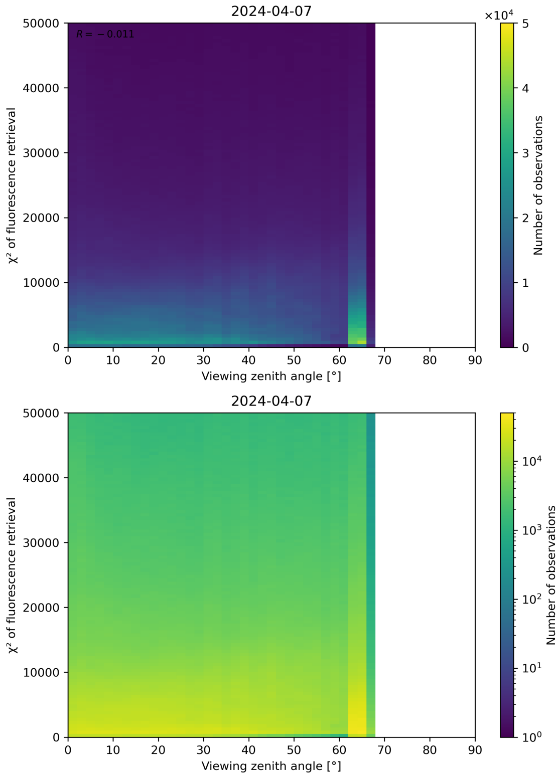
Figure 119: Scatter density plot of “Viewing zenith angle” against “ \chi^2 of fluorescence retrieval” for 2024-04-06 to 2024-04-08.
