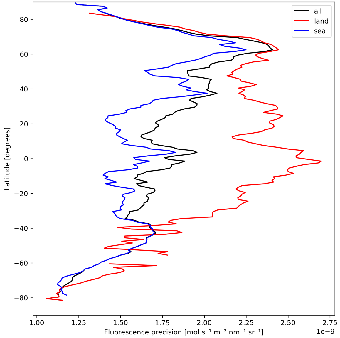
Figure 24: Zonal average of “Fluorescence precision” for 2024-04-06 to 2024-04-08.
