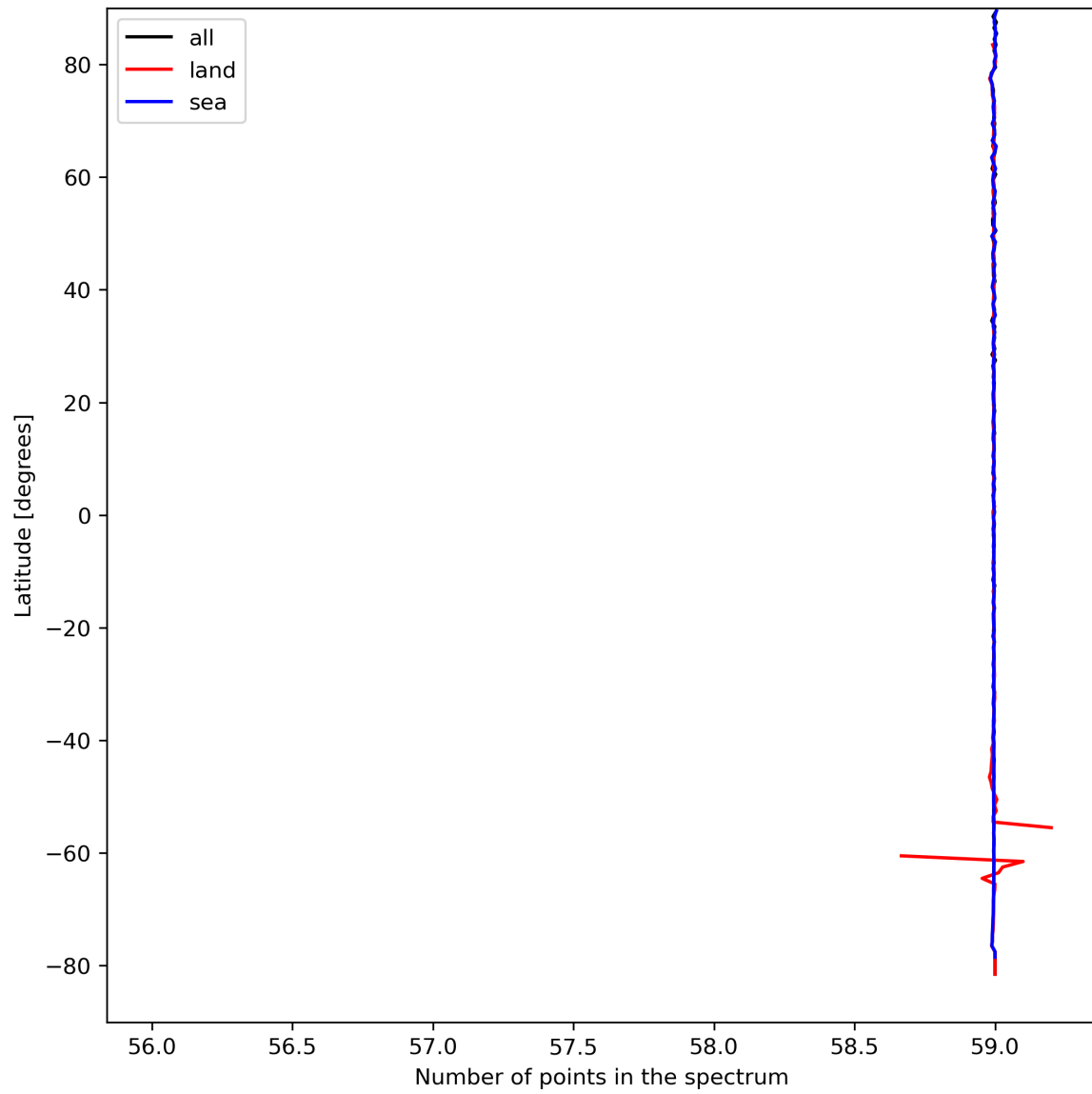
Figure 27: Zonal average of “Number of points in the spectrum” for 2024-04-06 to 2024-04-08.
