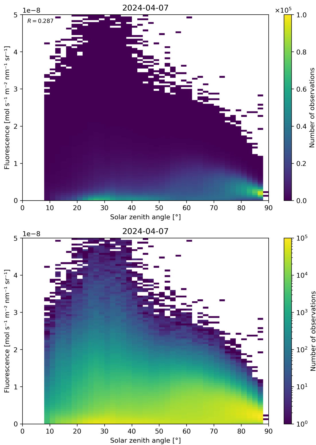
Figure 112: Scatter density plot of “Solar zenith angle” against “Fluorescence” for 2024-04-06 to 2024-04-08.
