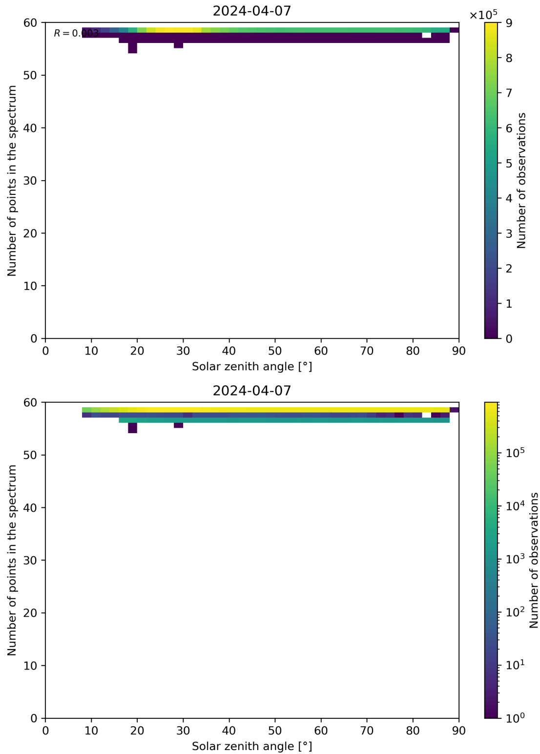
Figure 115: Scatter density plot of “Solar zenith angle” against “Number of points in the spectrum” for 2024-04-06 to 2024-04-08.
