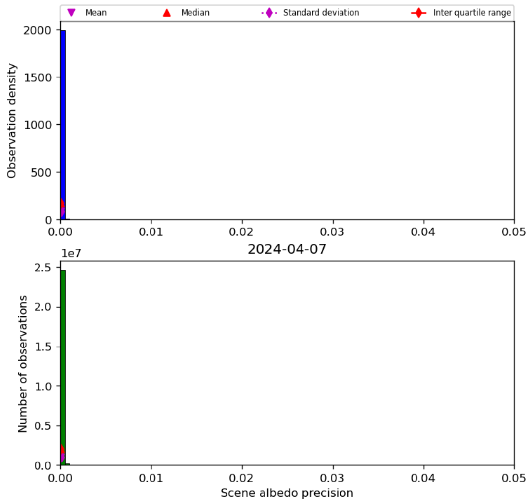
Figure 35: Histogram of “Scene albedo precision” for 2024-04-06 to 2024-04-08
