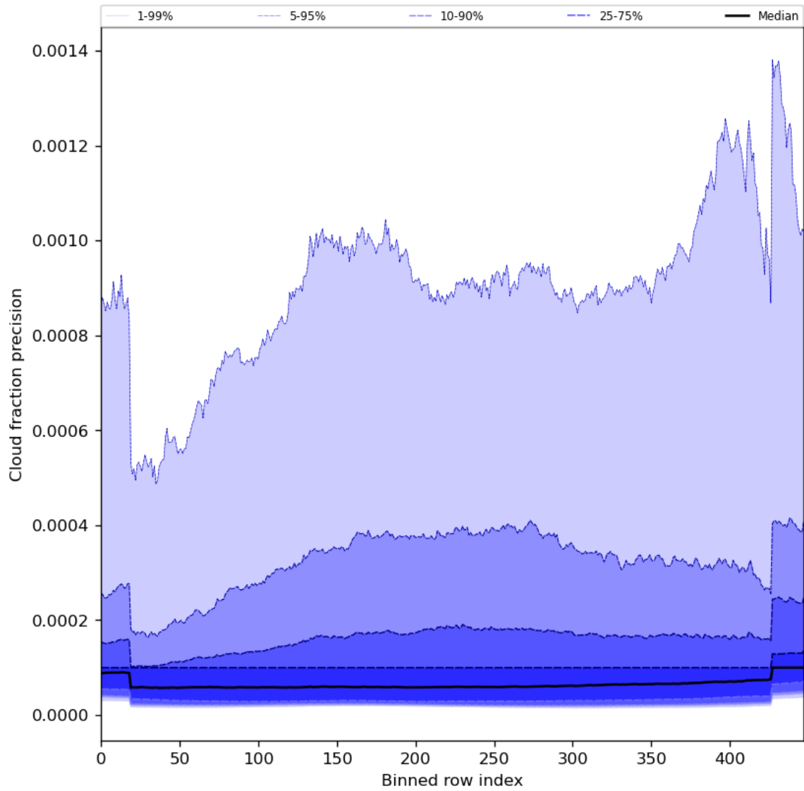
Figure 50: Along track statistics of “Cloud fraction precision” for 2024-04-06 to 2024-04-08
