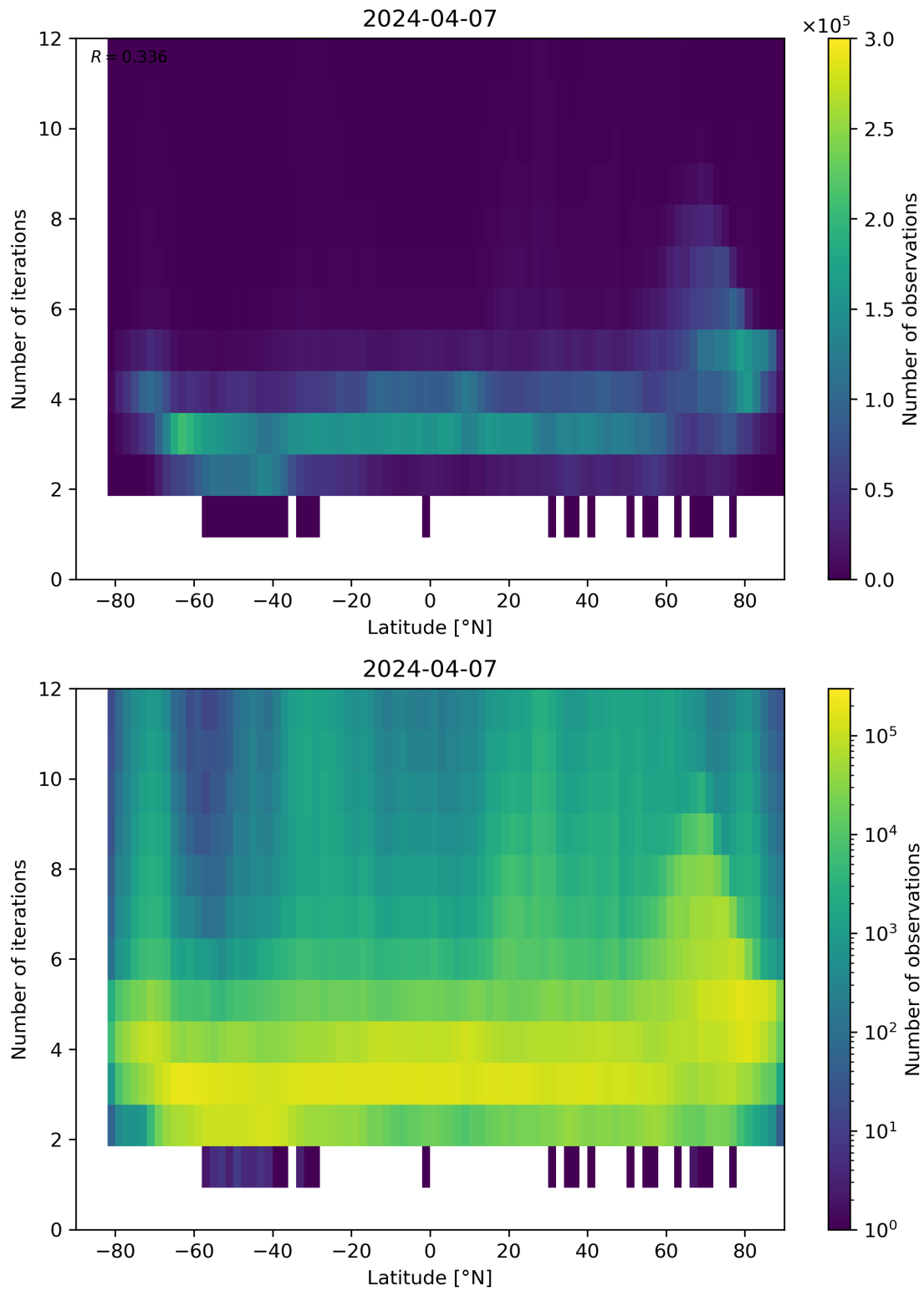
Figure 93: Scatter density plot of “Latitude” against “Number of iterations” for 2024-04-06 to 2024-04-08.
