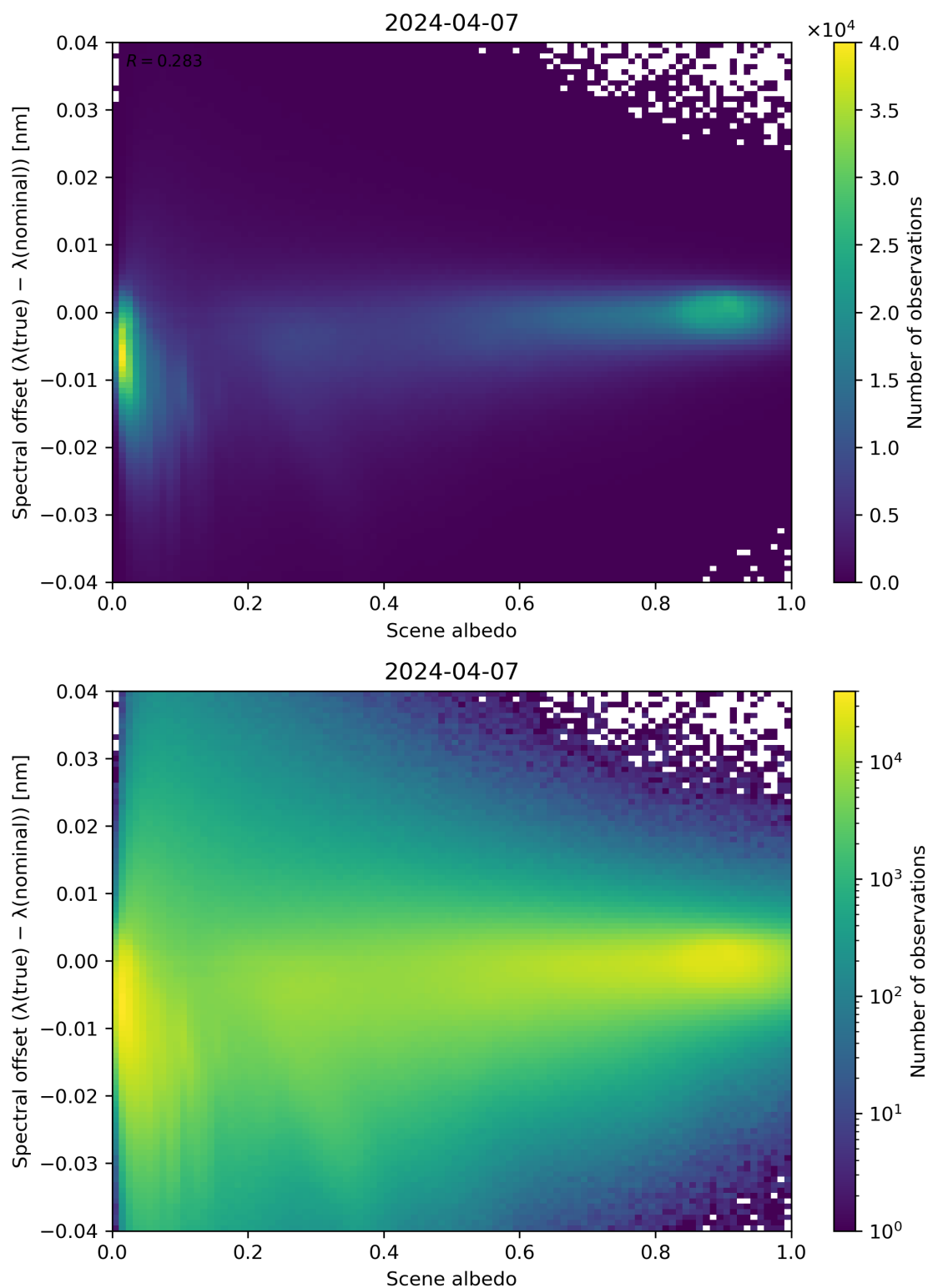
Figure 107: Scatter density plot of “Scene albedo” against “Spectral offset ( \lambda(\text{true}) - \lambda(\text{nominal}) )” for 2024-04-06 to 2024-04-08.
