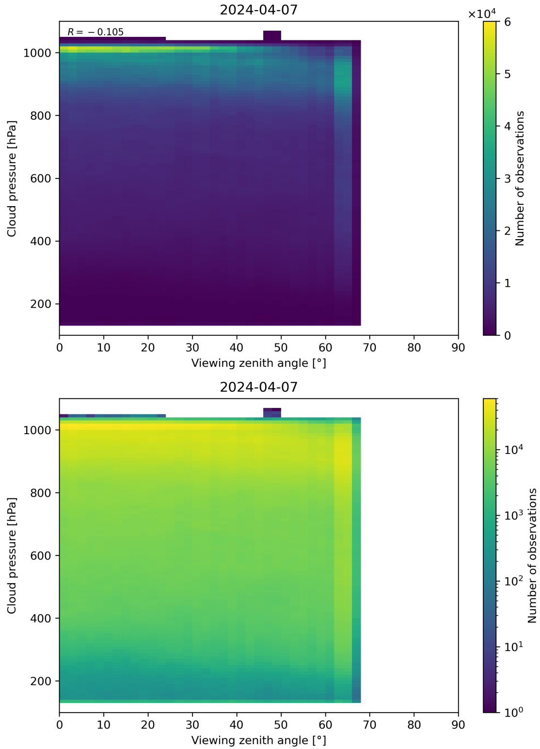
Figure 121: Scatter density plot of “Viewing zenith angle” against “Cloud pressure” for 2024-04-06 to 2024-04-08.
