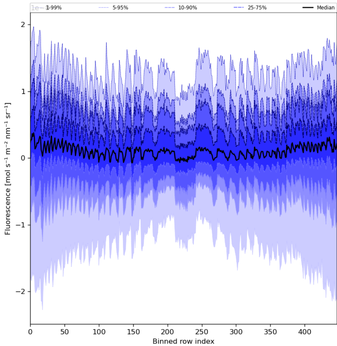
Figure 57: Along track statistics of “Fluorescence” for 2024-04-06 to 2024-04-08
