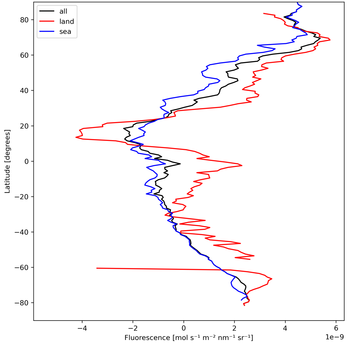
Figure 23: Zonal average of “Fluorescence” for 2024-04-06 to 2024-04-08.
