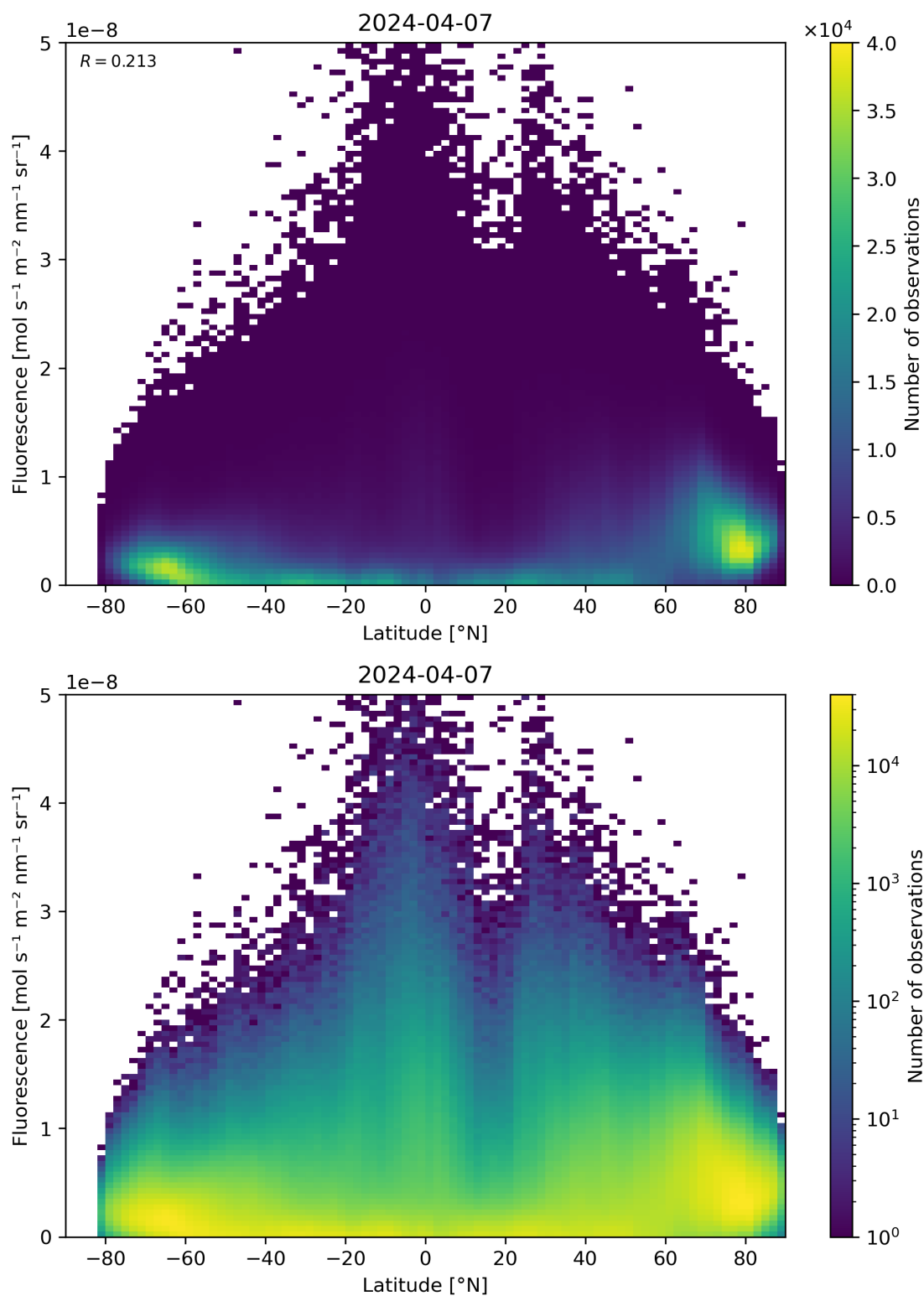
Figure 92: Scatter density plot of “Latitude” against “Fluorescence” for 2024-04-06 to 2024-04-08.
