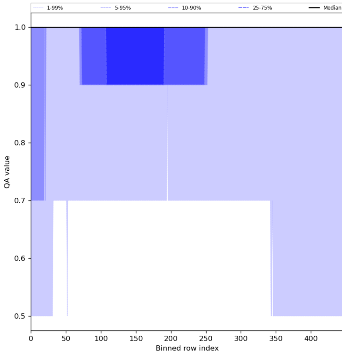
Figure 46: Along track statistics of “QA value” for 2024-04-06 to 2024-04-08
