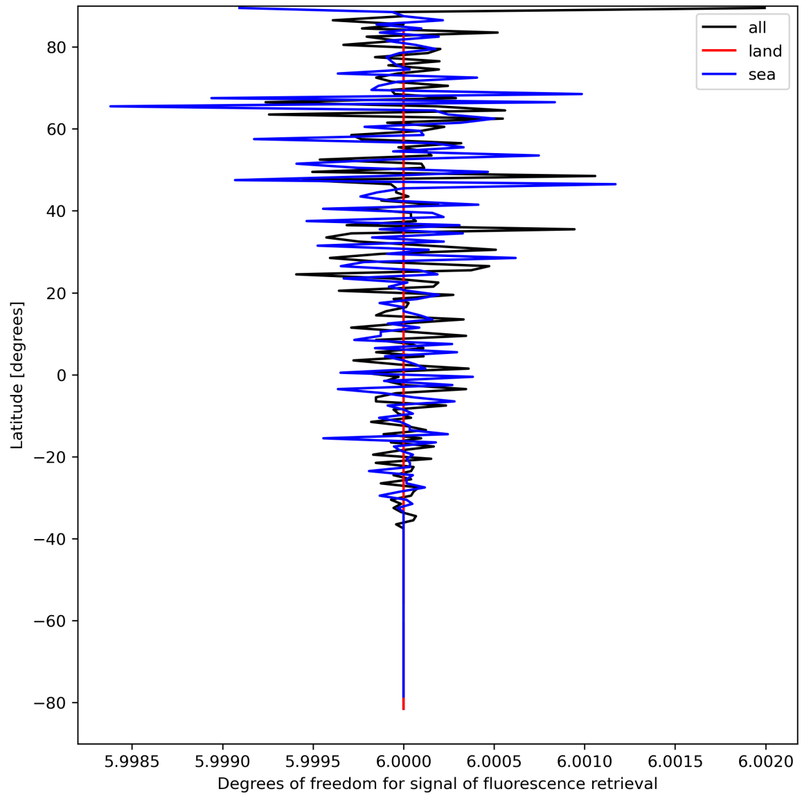
Figure 26: Zonal average of “Degrees of freedom for signal of fluorescence retrieval” for 2024-04-06 to 2024-04-08.
