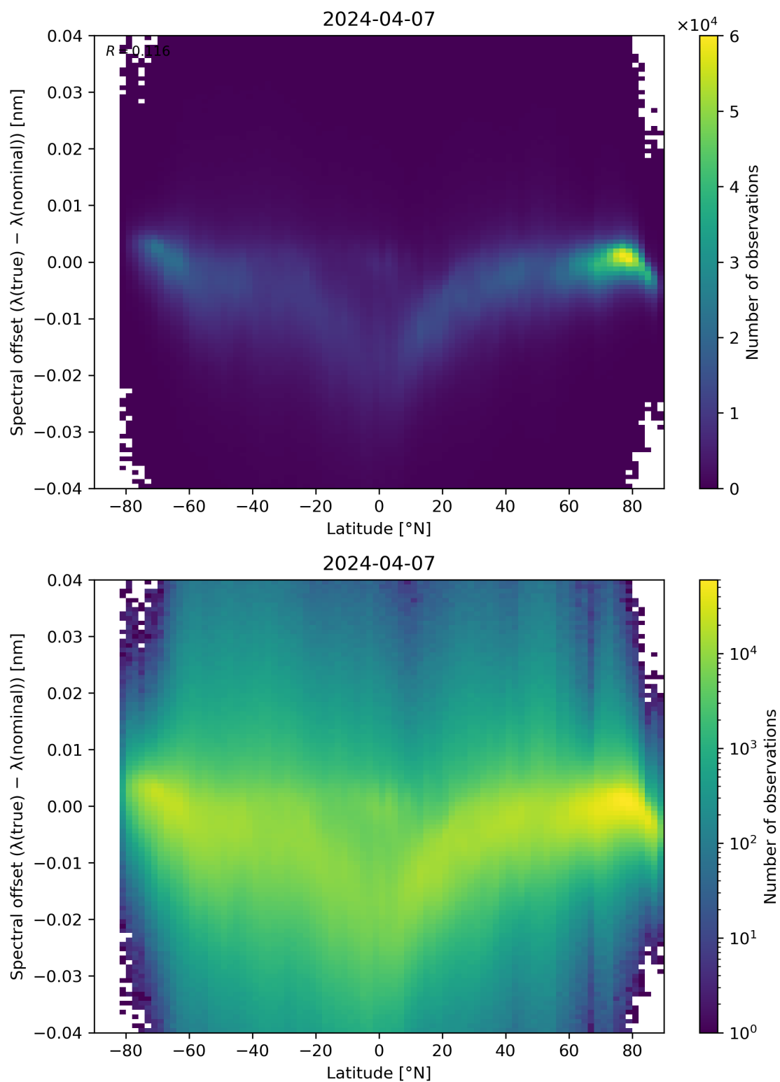
Figure 96: Scatter density plot of “Latitude” against “Spectral offset ( \lambda(\text{true}) - \lambda(\text{nominal}) )” for 2024-04-06 to 2024-04-08.
