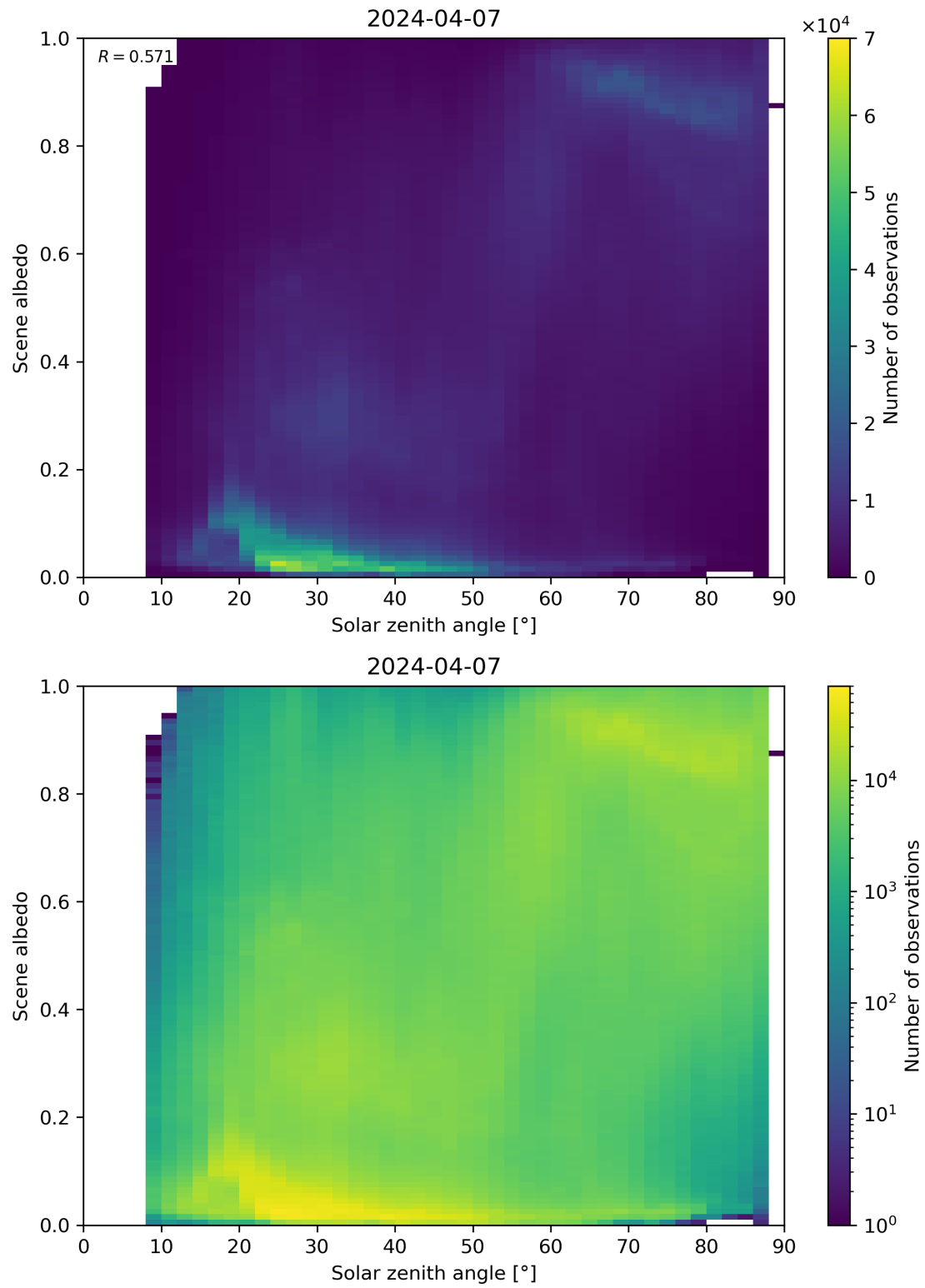
Figure 116: Scatter density plot of “Solar zenith angle” against “Scene albedo” for 2024-04-06 to 2024-04-08.
