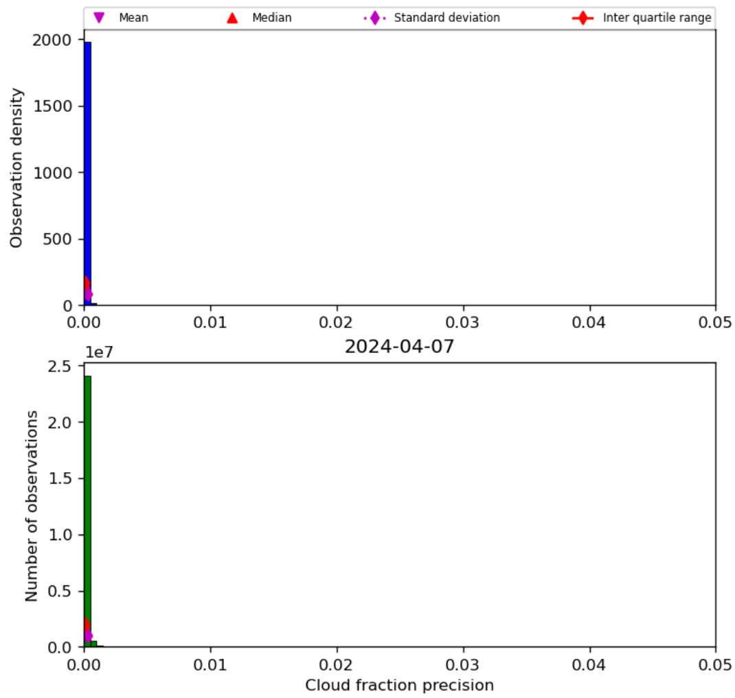
Figure 33: Histogram of “Cloud fraction precision” for 2024-04-06 to 2024-04-08
