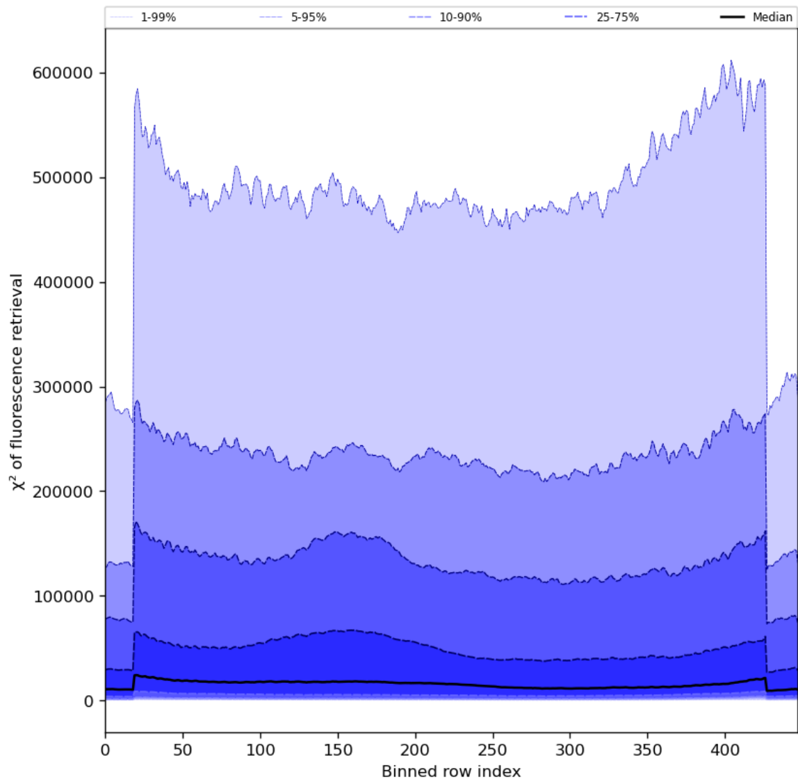
Figure 59: Along track statistics of “ \chi^2 of fluorescence retrieval” for 2024-04-06 to 2024-04-08
