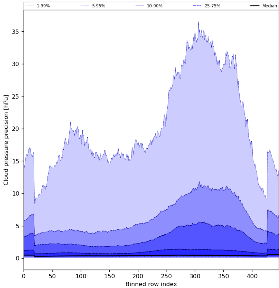
Figure 48: Along track statistics of “Cloud pressure precision” for 2024-04-06 to 2024-04-08
