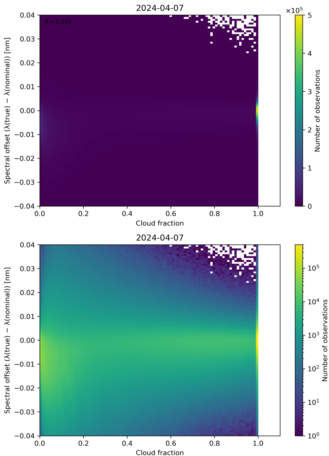
Figure 76: Scatter density plot of “Cloud fraction” against “Spectral offset ( \lambda(\text{true}) - \lambda(\text{nominal}) )” for 2024-04-06 to 2024-04-08.
