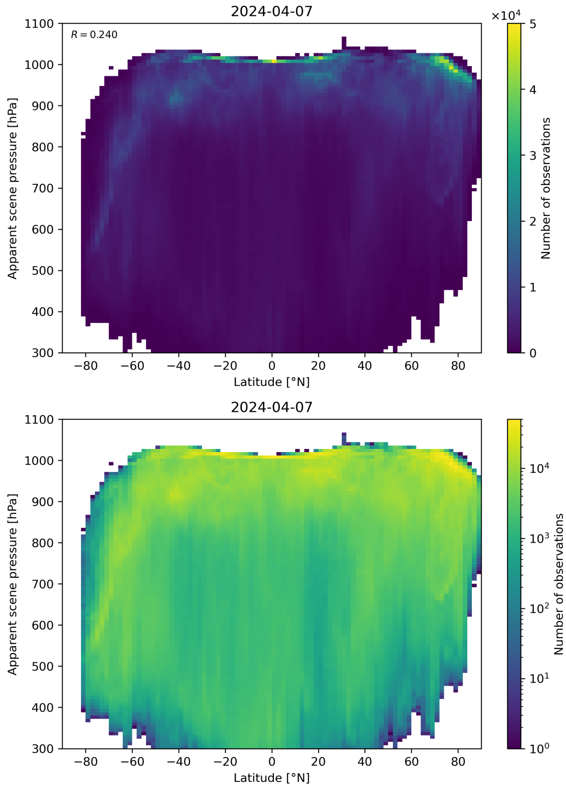
Figure 88: Scatter density plot of “Latitude” against “Apparent scene pressure” for 2024-04-06 to 2024-04-08.
