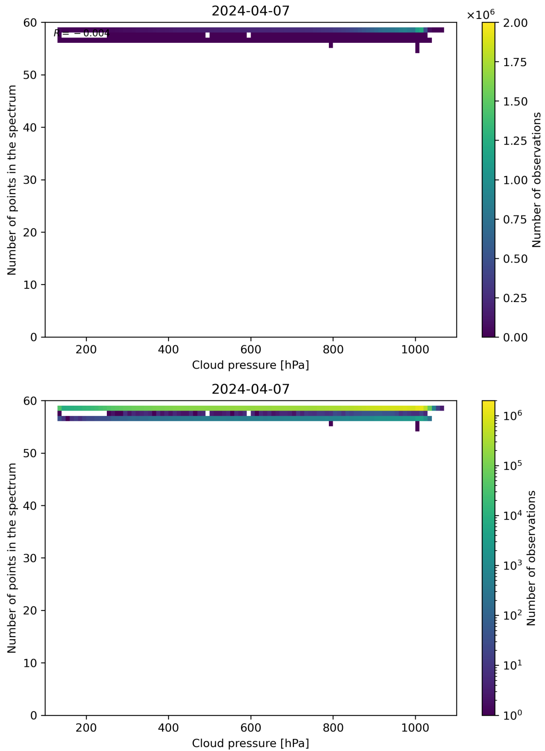
Figure 82: Scatter density plot of “Cloud pressure” against “Number of points in the spectrum” for 2024-04-06 to 2024-04-08.
