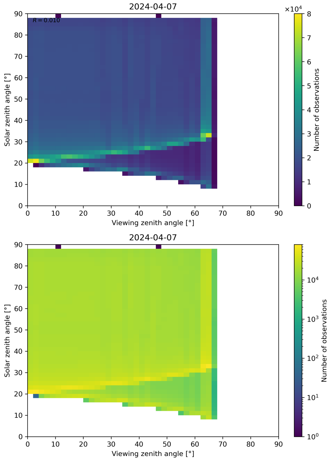
Figure 127: Scatter density plot of “Viewing zenith angle” against “Solar zenith angle” for 2024-04-06 to 2024-04-08.
