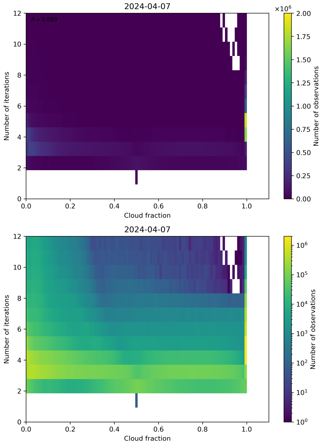
Figure 73: Scatter density plot of “Cloud fraction” against “Number of iterations” for 2024-04-06 to 2024-04-08.
