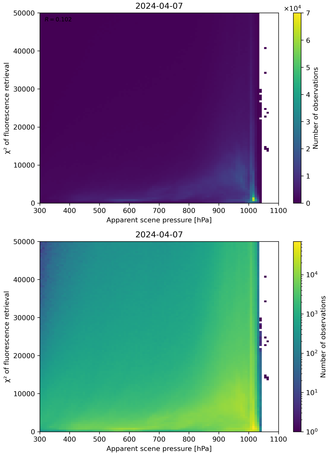
Figure 63: Scatter density plot of “Apparent scene pressure” against “ \chi^2 of fluorescence retrieval” for 2024-04-06 to 2024-04-08.
