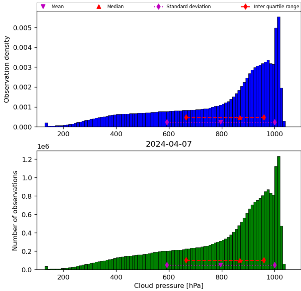
Figure 30: Histogram of “Cloud pressure” for 2024-04-06 to 2024-04-08
