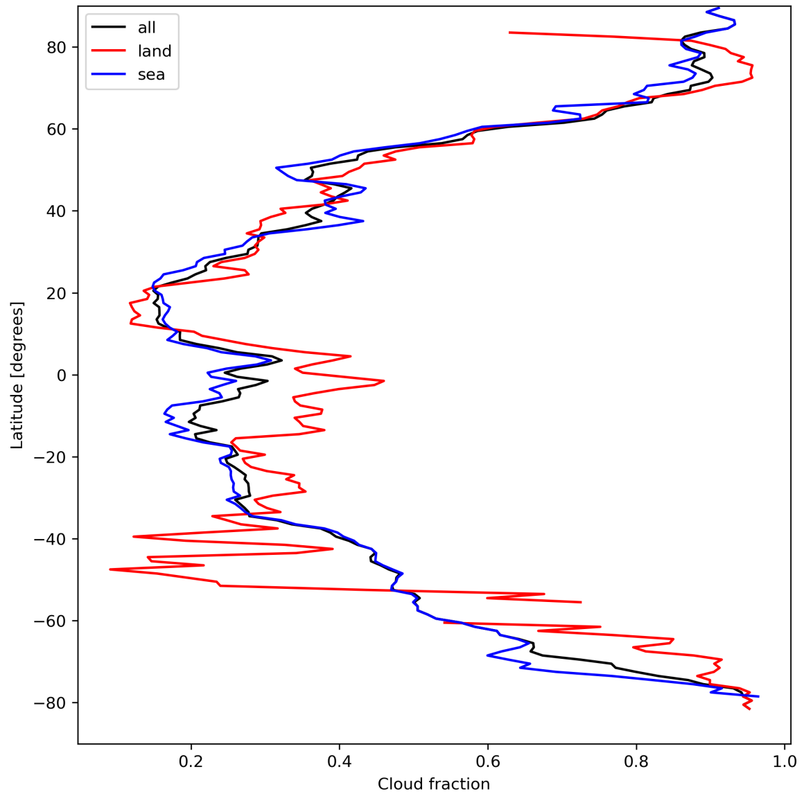
Figure 15: Zonal average of “Cloud fraction” for 2024-04-06 to 2024-04-08.
