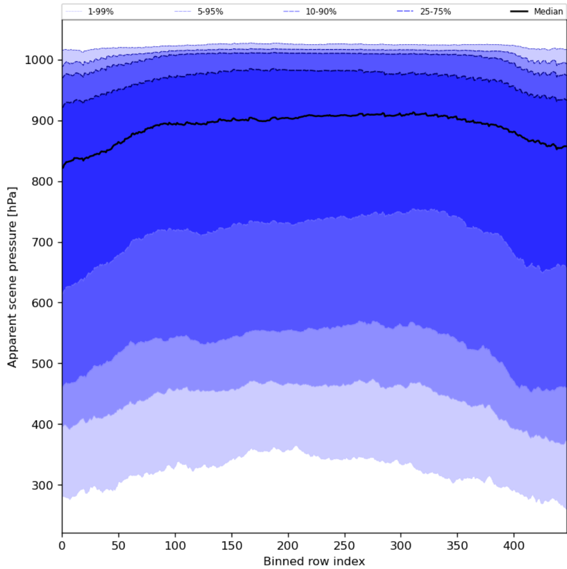
Figure 53: Along track statistics of “Apparent scene pressure” for 2024-04-06 to 2024-04-08
