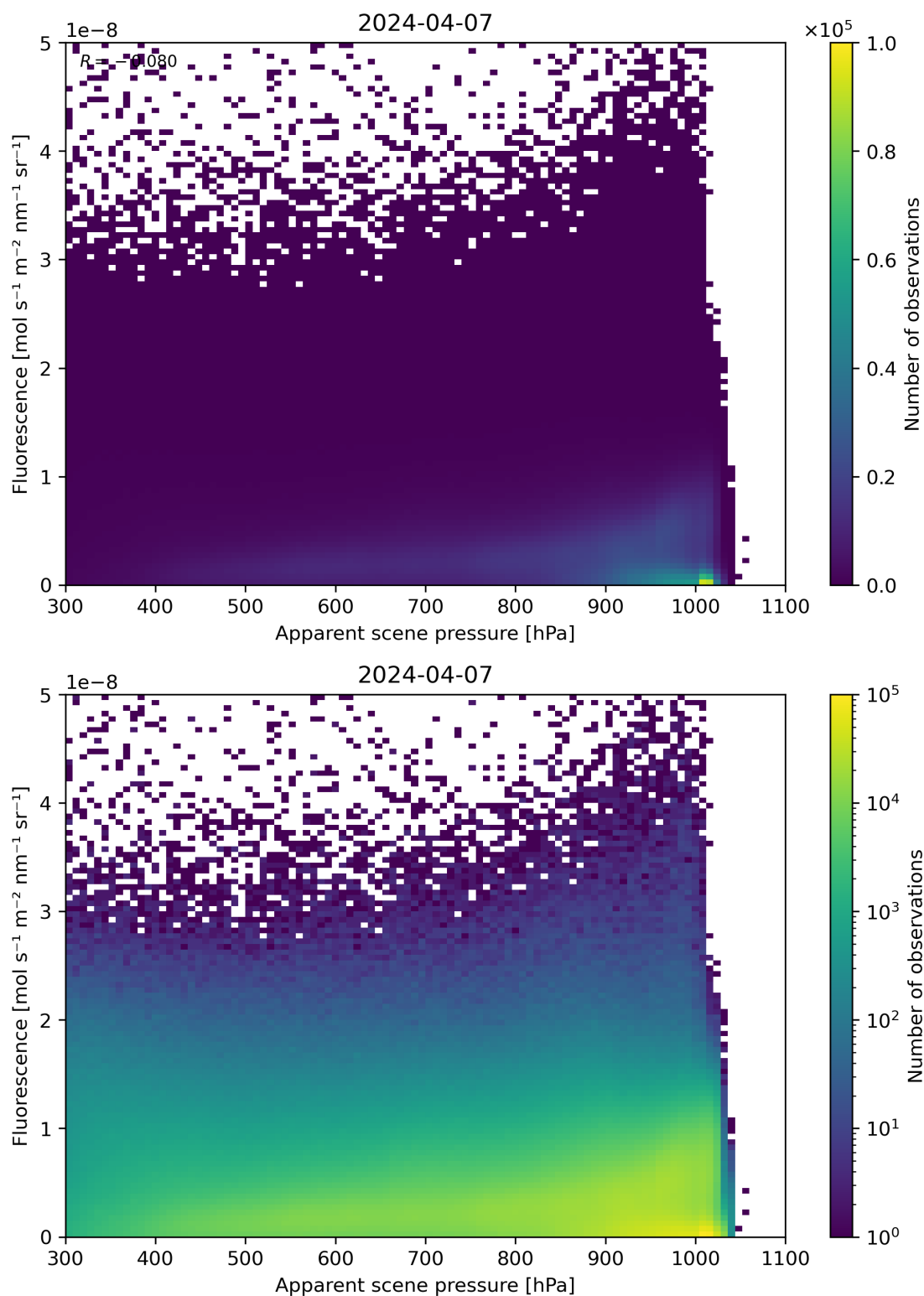
Figure 64: Scatter density plot of “Apparent scene pressure” against “Fluorescence” for 2024-04-06 to 2024-04-08.
