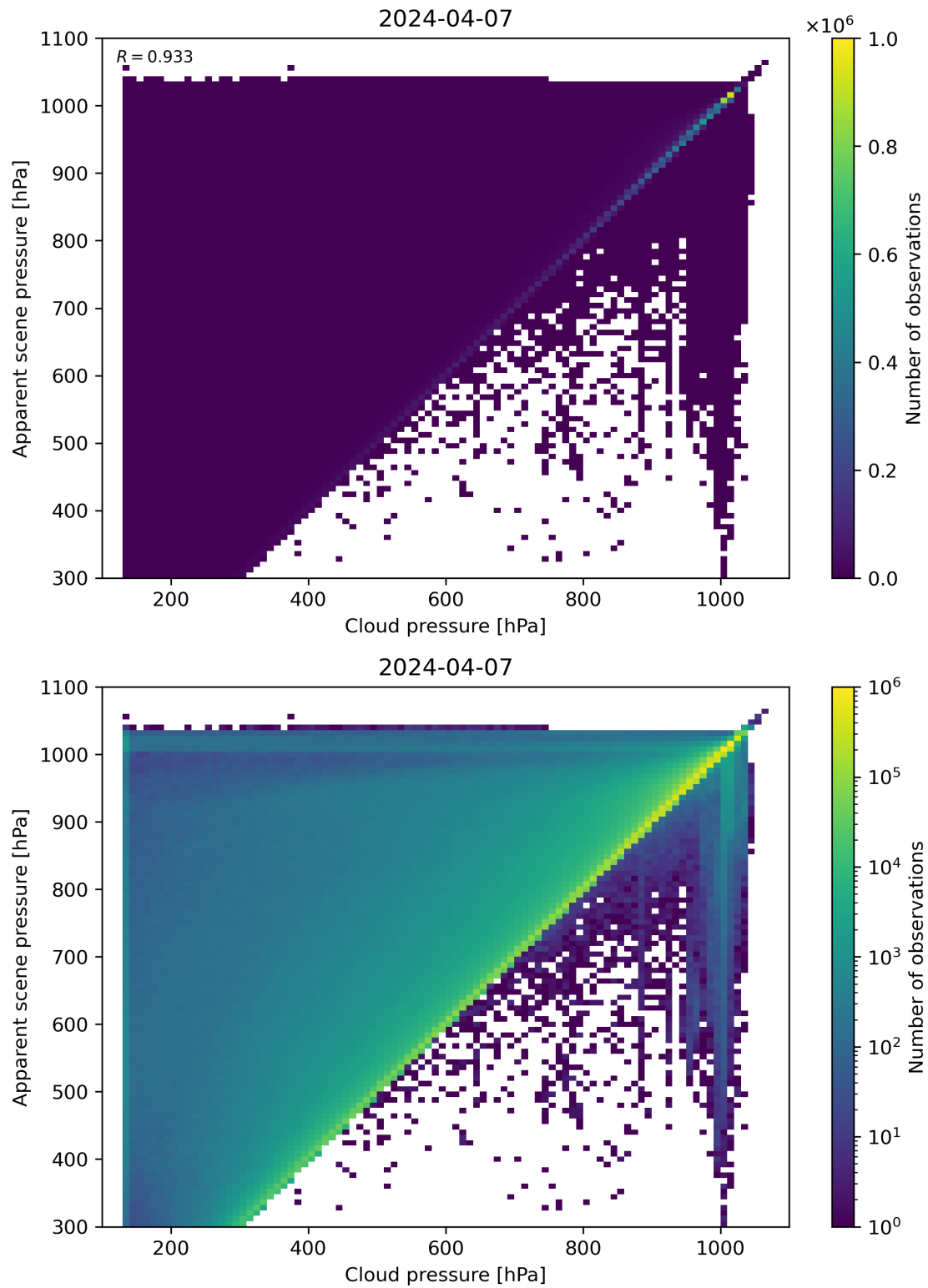
Figure 77: Scatter density plot of “Cloud pressure” against “Apparent scene pressure” for 2024-04-06 to 2024-04-08.
