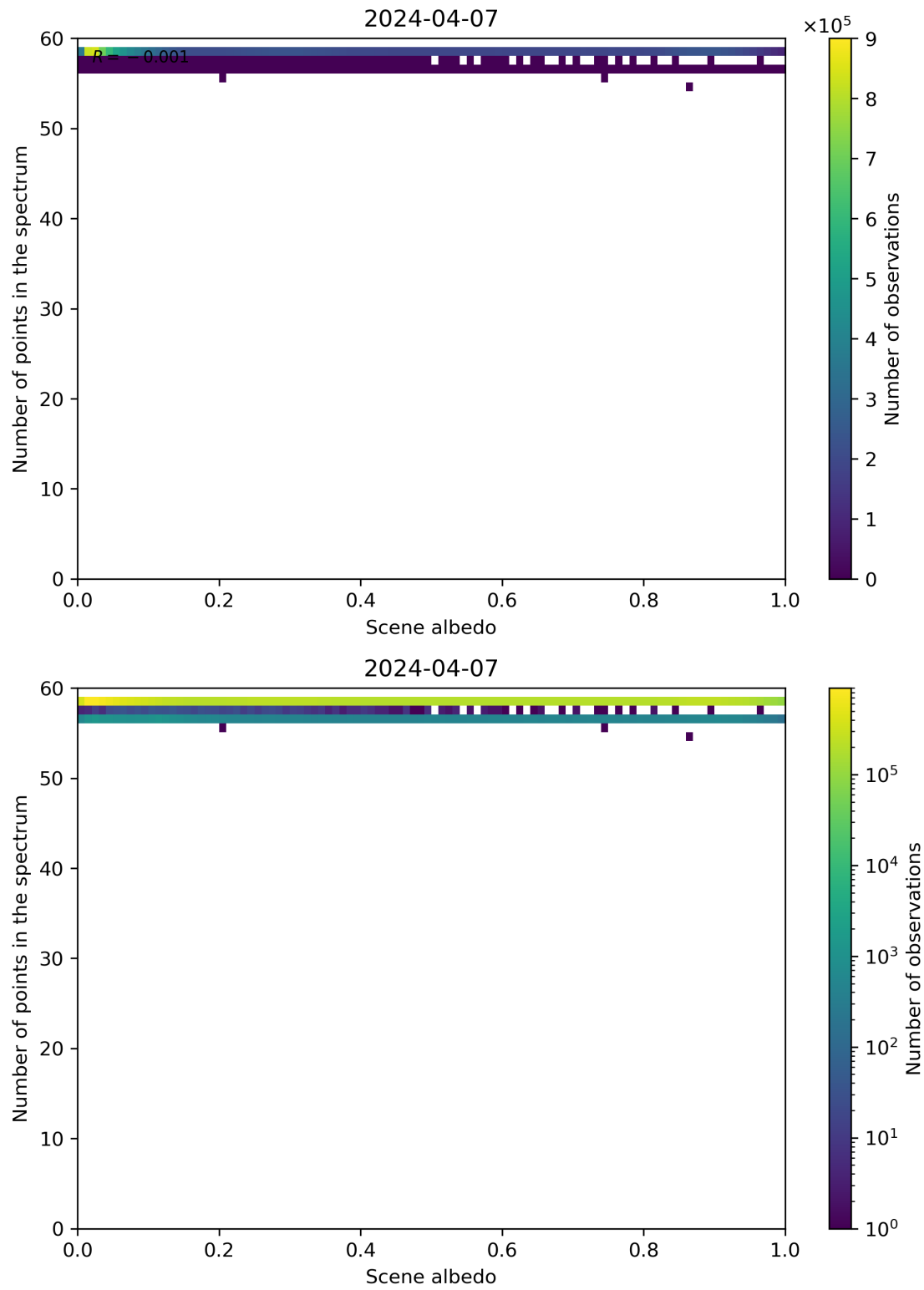
Figure 106: Scatter density plot of “Scene albedo” against “Number of points in the spectrum” for 2024-04-06 to 2024-04-08.
