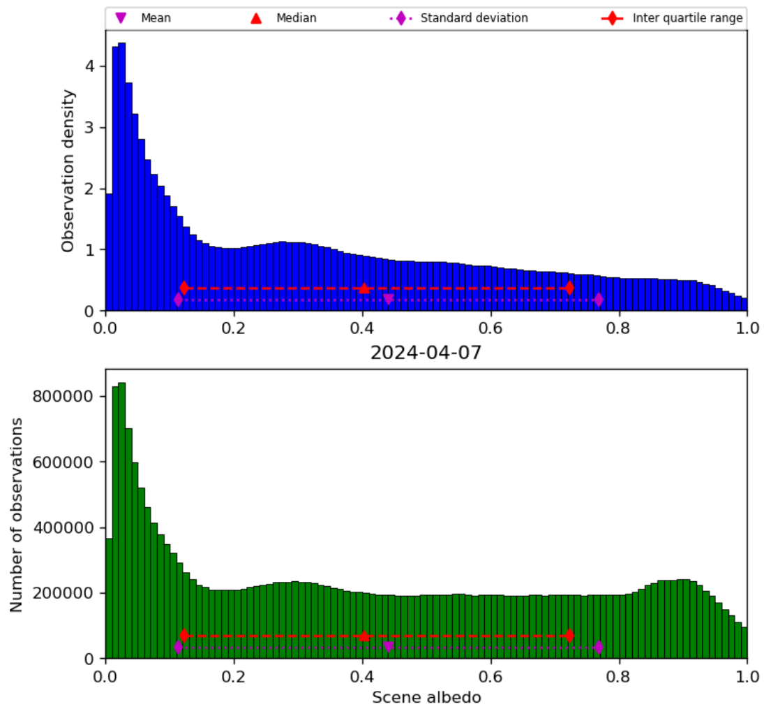
Figure 34: Histogram of “Scene albedo” for 2024-04-06 to 2024-04-08
