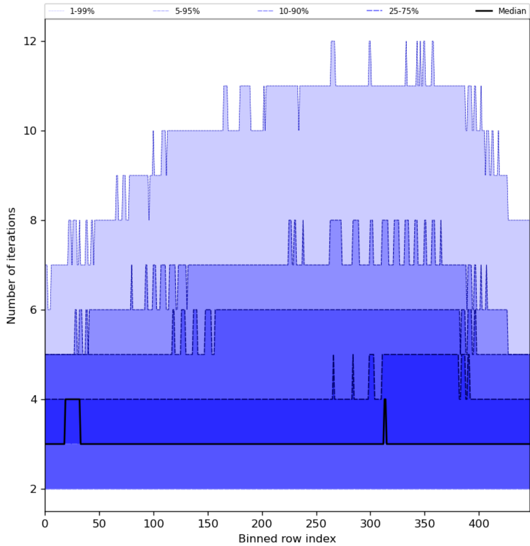
Figure 56: Along track statistics of “Number of iterations” for 2024-04-06 to 2024-04-08
