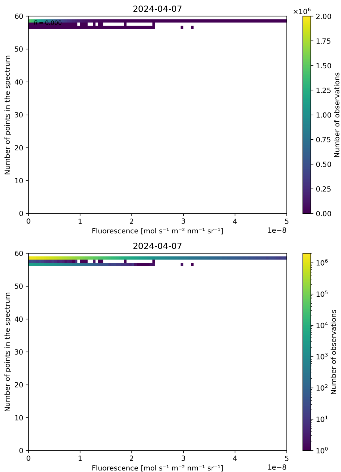
Figure 86: Scatter density plot of “Fluorescence” against “Number of points in the spectrum” for 2024-04-06 to 2024-04-08.
