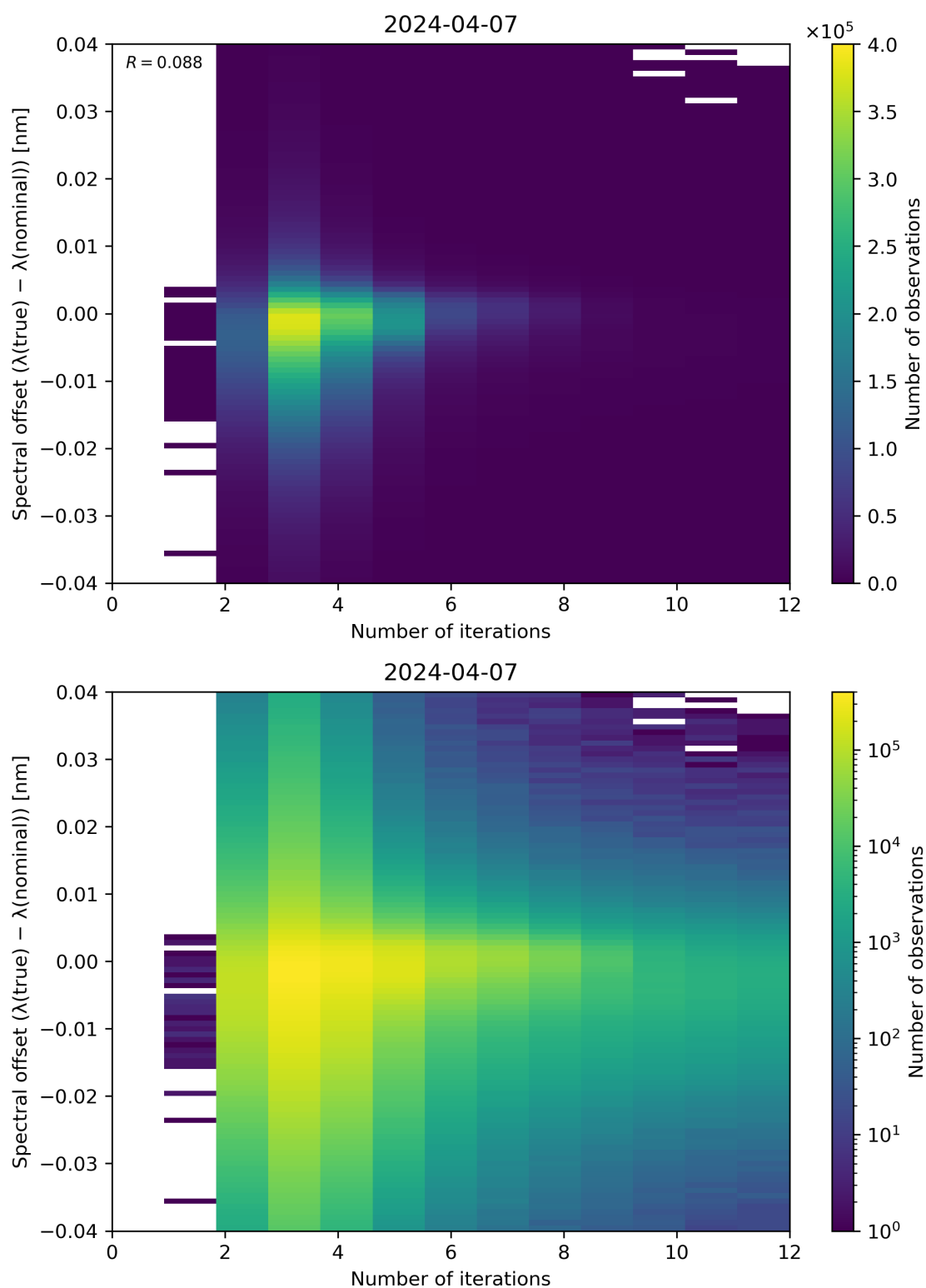
Figure 100: Scatter density plot of “Number of iterations” against “Spectral offset ( \lambda(\text{true}) - \lambda(\text{nominal}) )” for 2024-04-06 to 2024-04-08.
