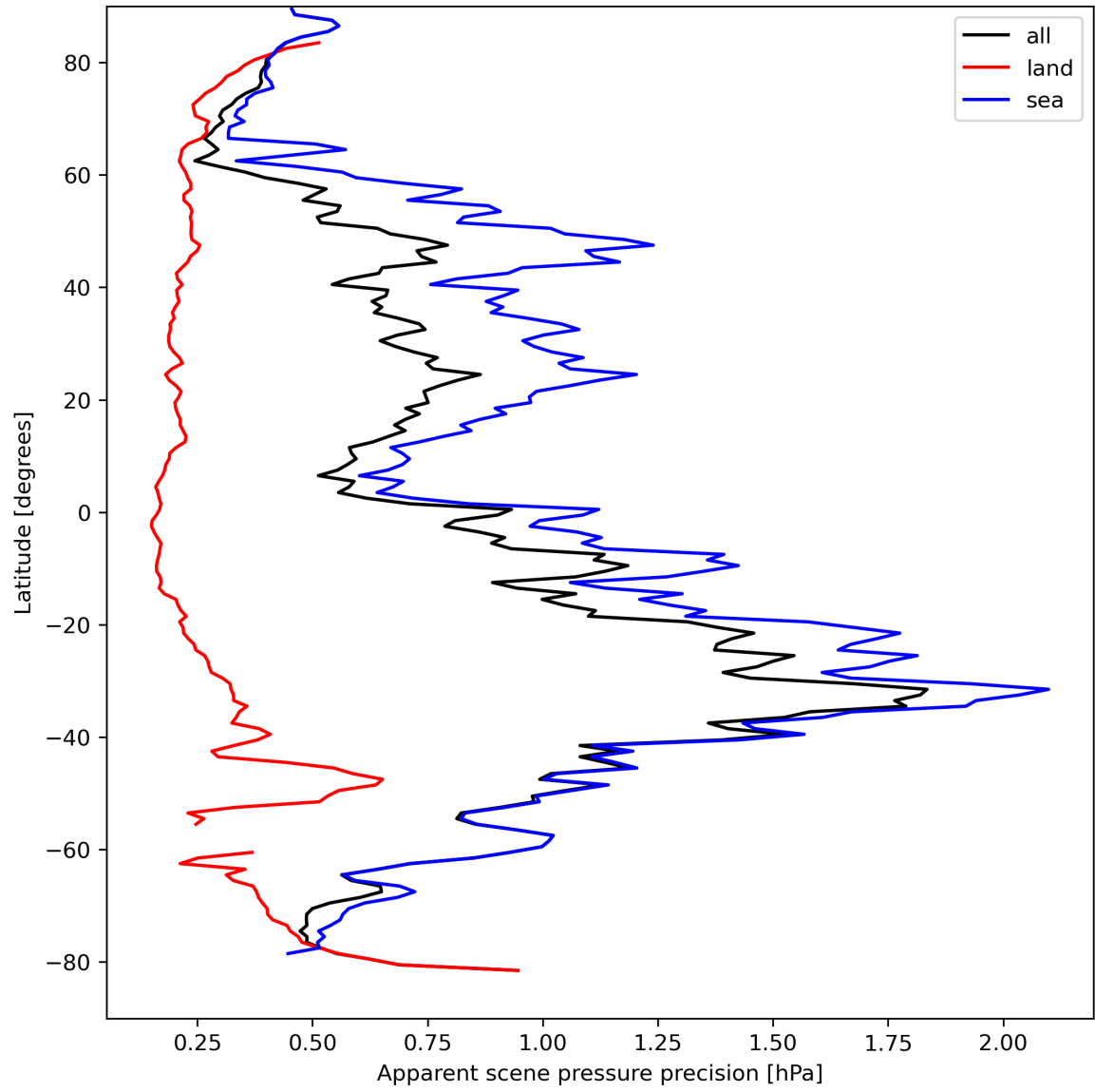
Figure 20: Zonal average of “Apparent scene pressure precision” for 2024-04-06 to 2024-04-08.
