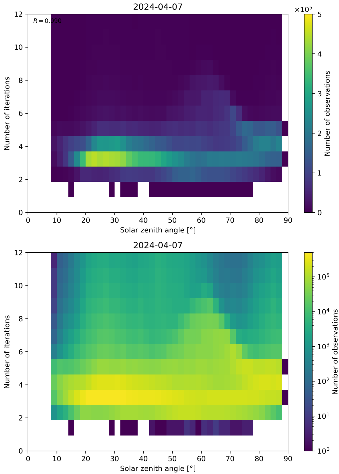
Figure 114: Scatter density plot of “Solar zenith angle” against “Number of iterations” for 2024-04-06 to 2024-04-08.
