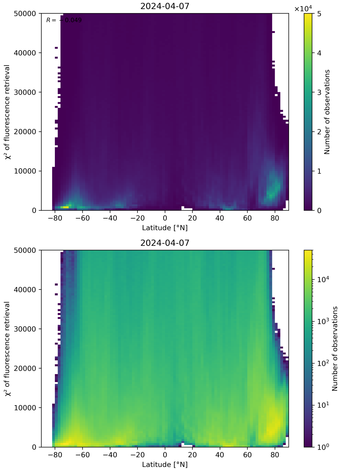
Figure 89: Scatter density plot of “Latitude” against “ \chi^2 of fluorescence retrieval” for 2024-04-06 to 2024-04-08.
