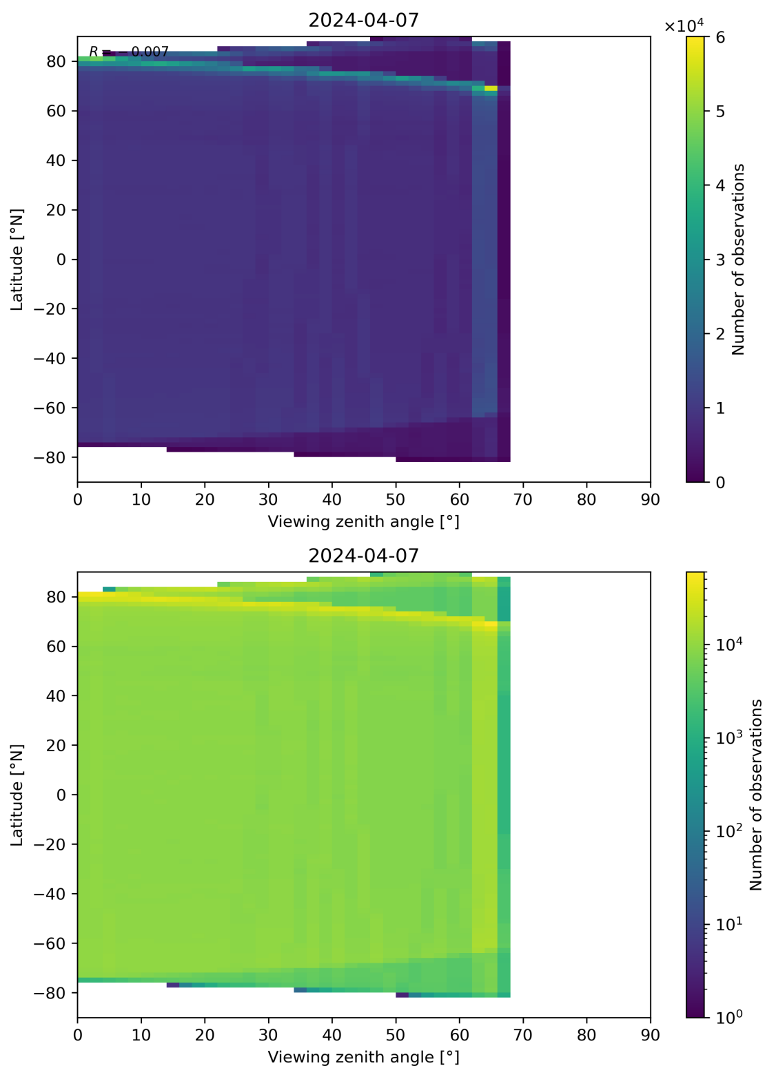
Figure 123: Scatter density plot of “Viewing zenith angle” against “Latitude” for 2024-04-06 to 2024-04-08.
