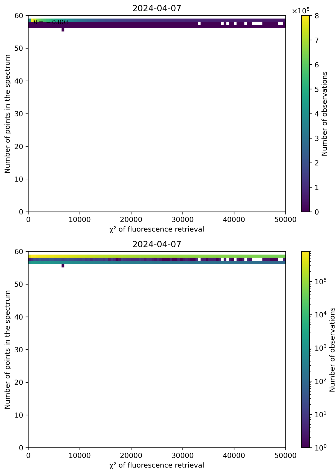
Figure 68: Scatter density plot of " \chi^2 of fluorescence retrieval" against "Number of points in the spectrum" for 2024-04-06 to 2024-04-08.
