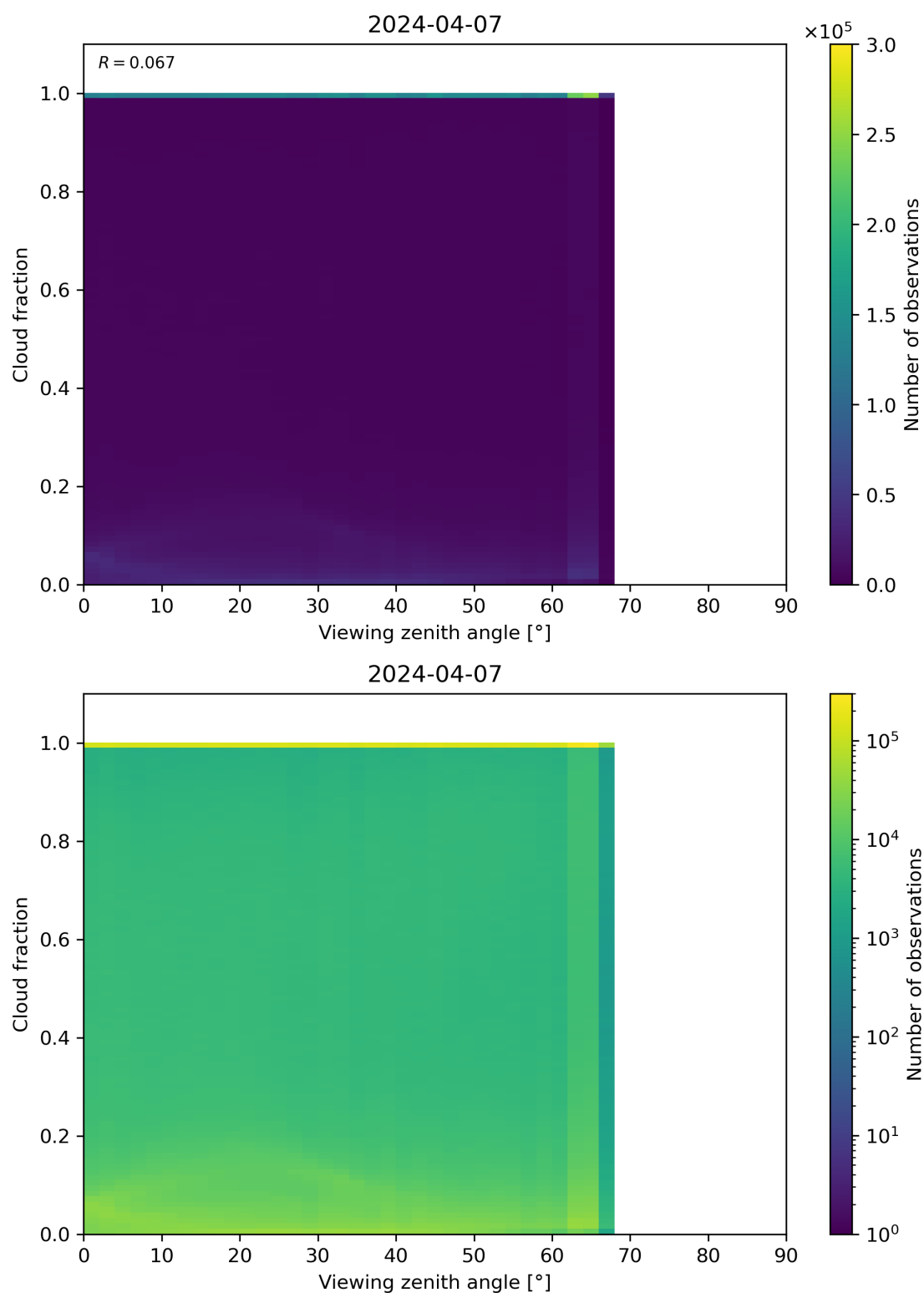
Figure 120: Scatter density plot of “Viewing zenith angle” against “Cloud fraction” for 2024-04-06 to 2024-04-08.
