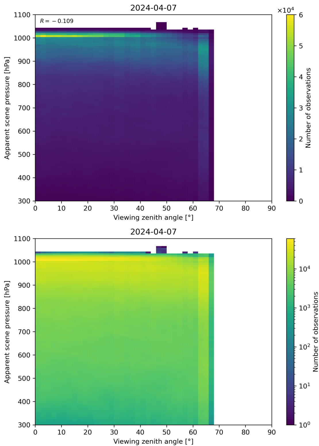
Figure 118: Scatter density plot of “Viewing zenith angle” against “Apparent scene pressure” for 2024-04-06 to 2024-04-08.
