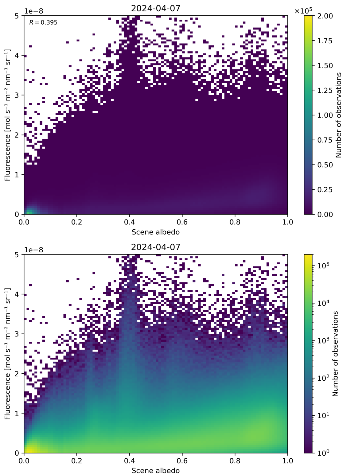
Figure 104: Scatter density plot of “Scene albedo” against “Fluorescence” for 2024-04-06 to 2024-04-08.
