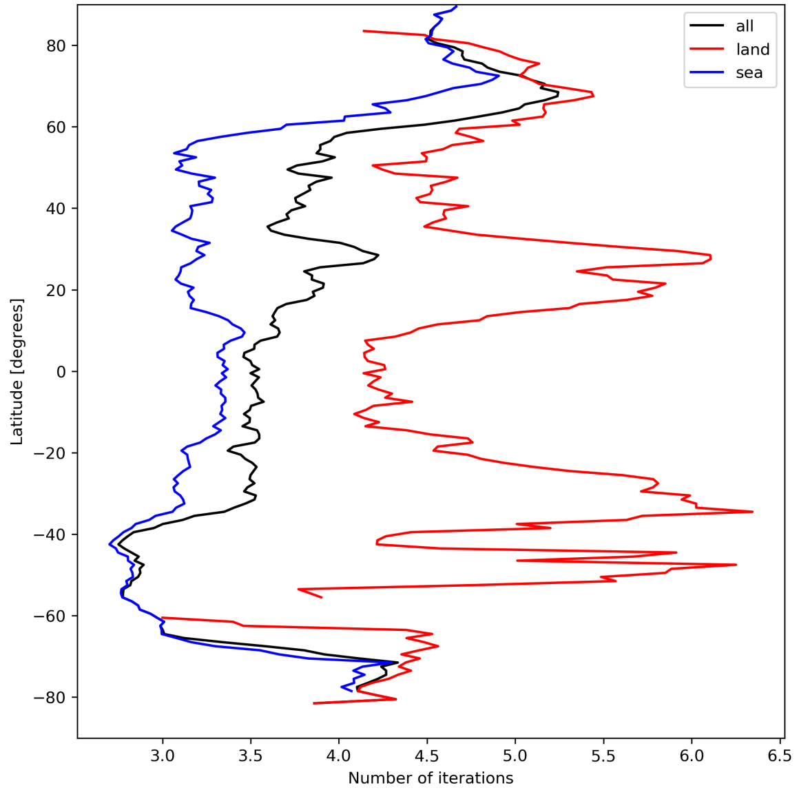
Figure 22: Zonal average of “Number of iterations” for 2024-04-06 to 2024-04-08.
