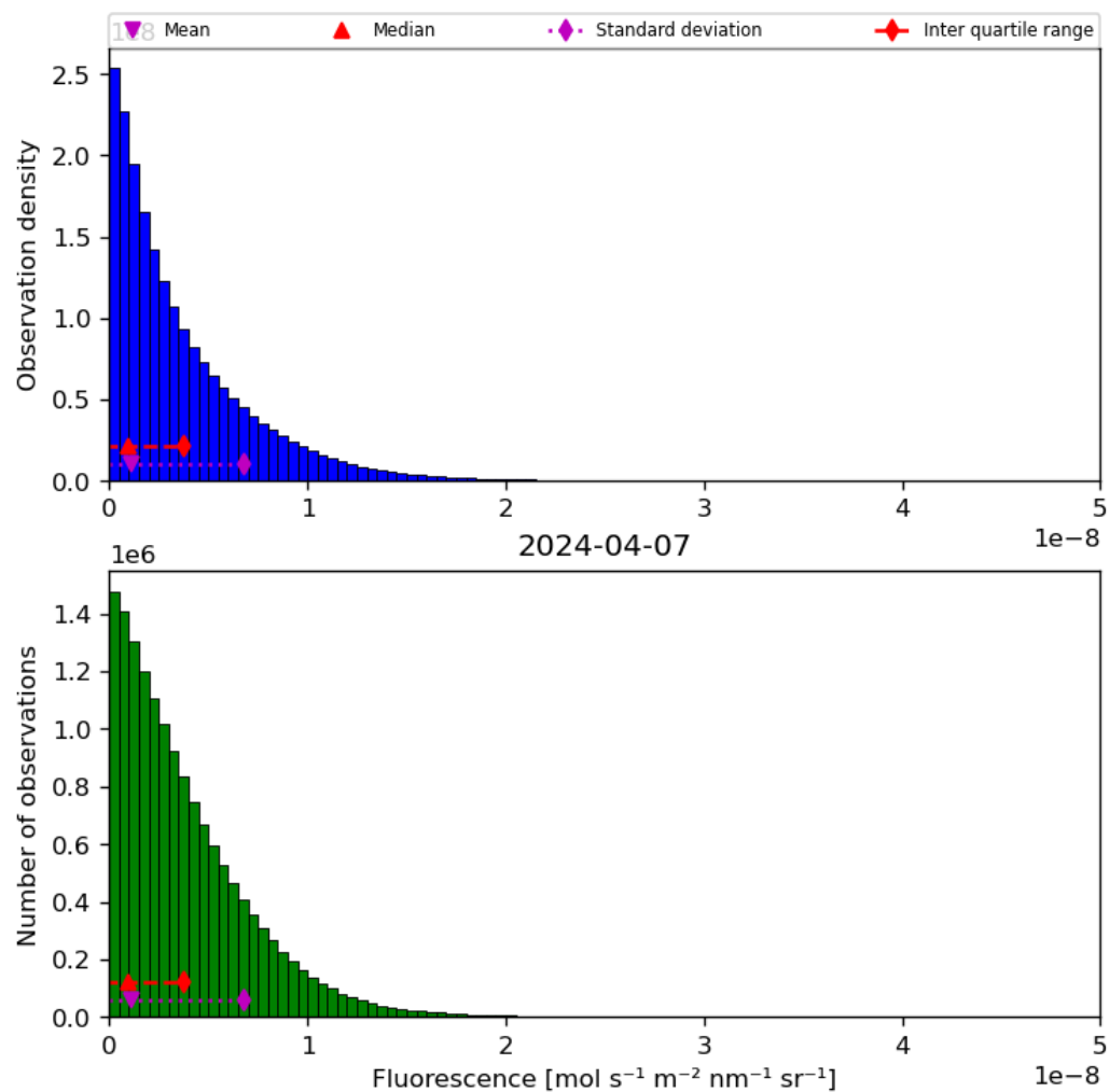
Figure 40: Histogram of “Fluorescence” for 2024-04-06 to 2024-04-08
