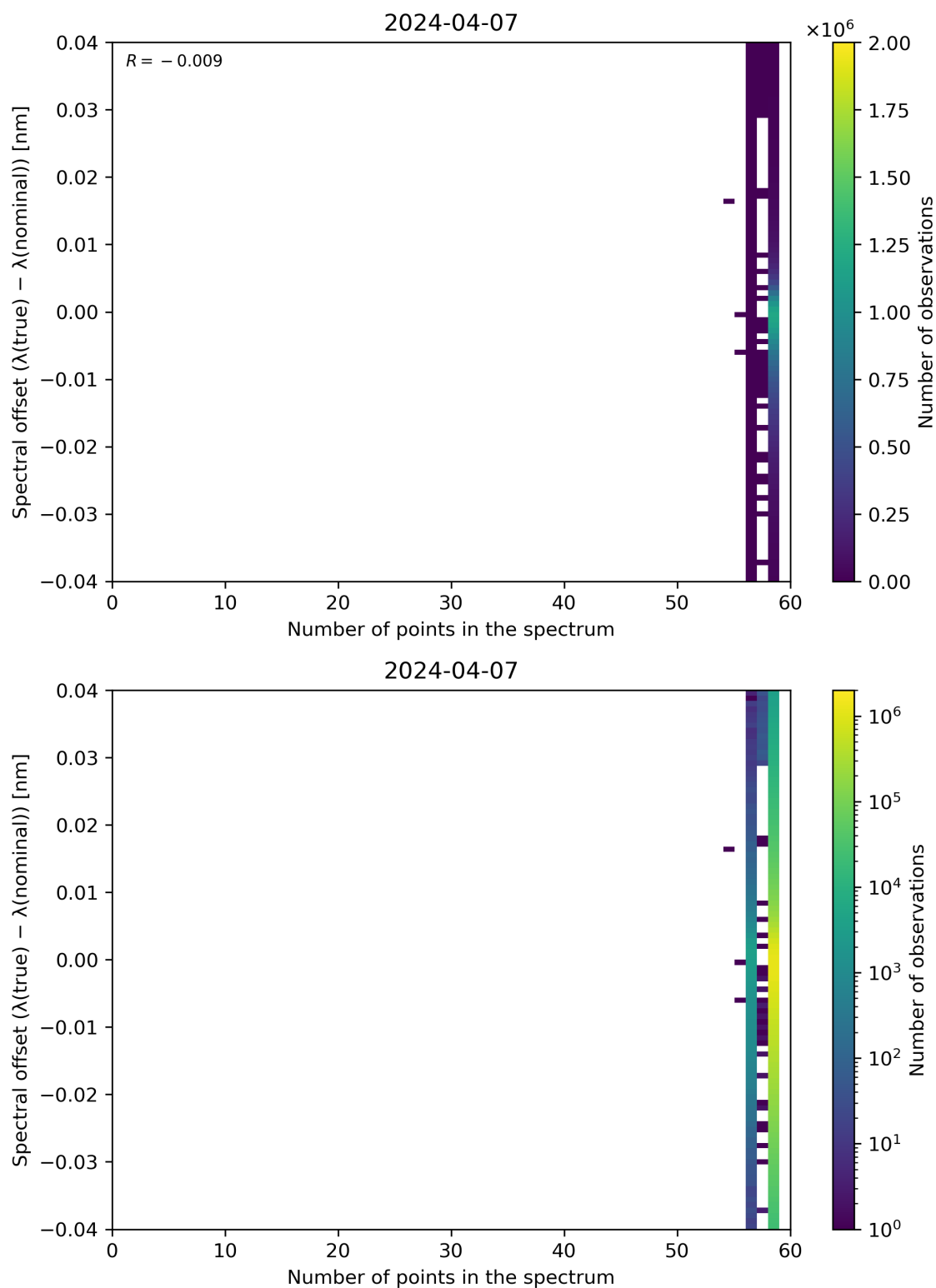
Figure 101: Scatter density plot of “Number of points in the spectrum” against “Spectral offset ( \lambda(\text{true}) - \lambda(\text{nominal}) )” for 2024-04-06 to 2024-04-08.
