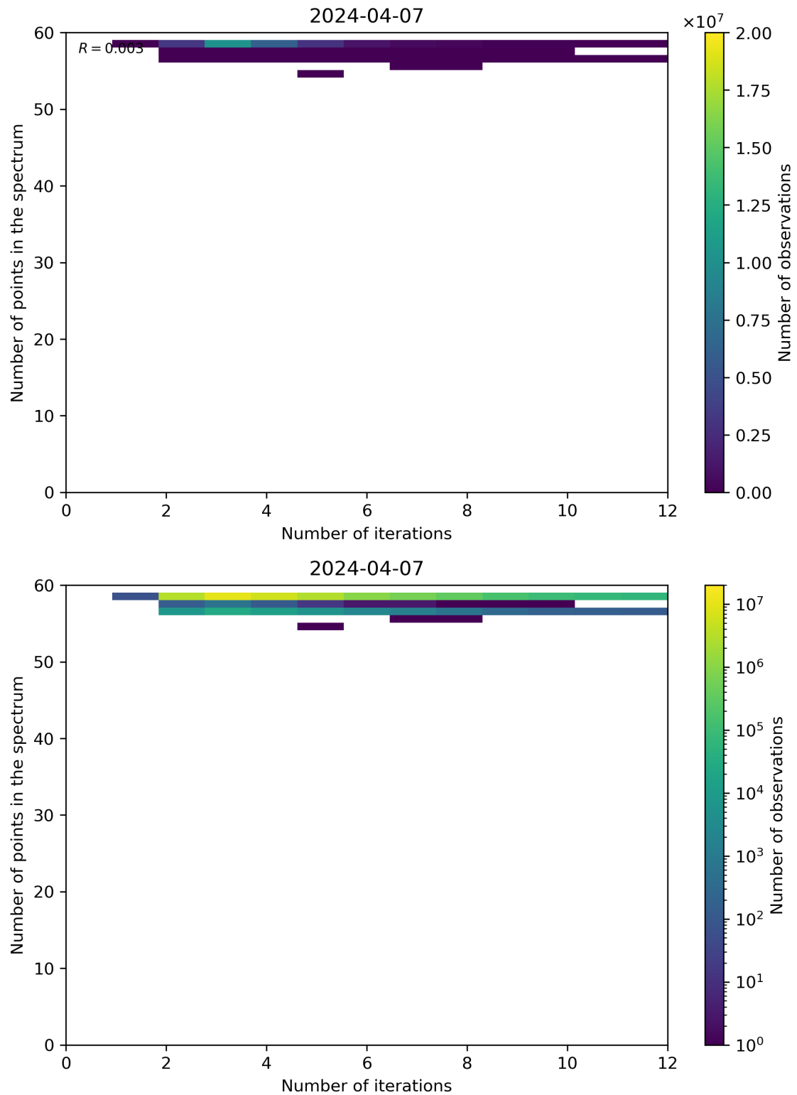
Figure 99: Scatter density plot of “Number of iterations” against “Number of points in the spectrum” for 2024-04-06 to 2024-04-08.
