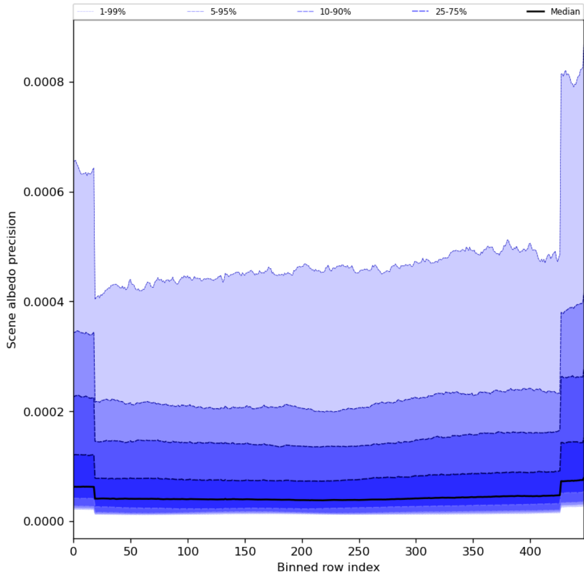
Figure 52: Along track statistics of “Scene albedo precision” for 2024-04-06 to 2024-04-08
