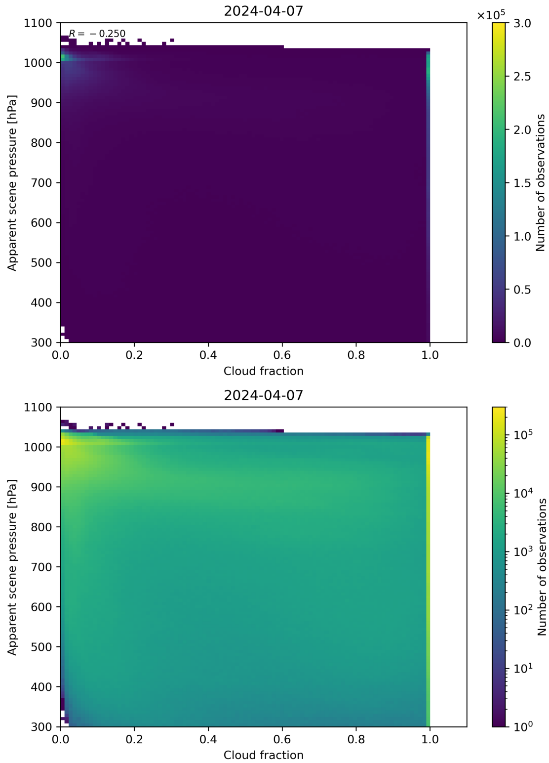
Figure 70: Scatter density plot of “Cloud fraction” against “Apparent scene pressure” for 2024-04-06 to 2024-04-08.
