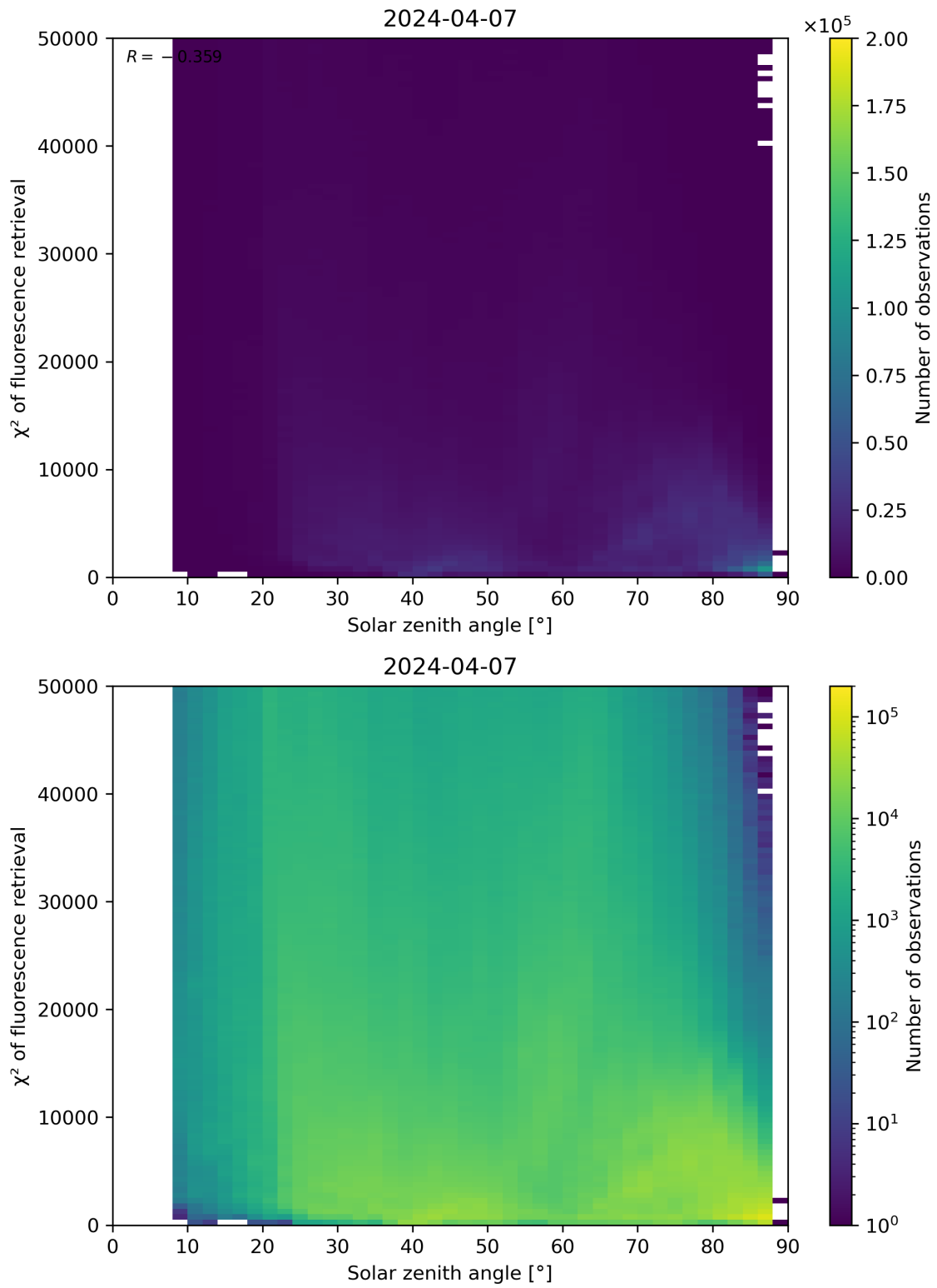
Figure 109: Scatter density plot of “Solar zenith angle” against “ \chi^2 of fluorescence retrieval” for 2024-04-06 to 2024-04-08.
