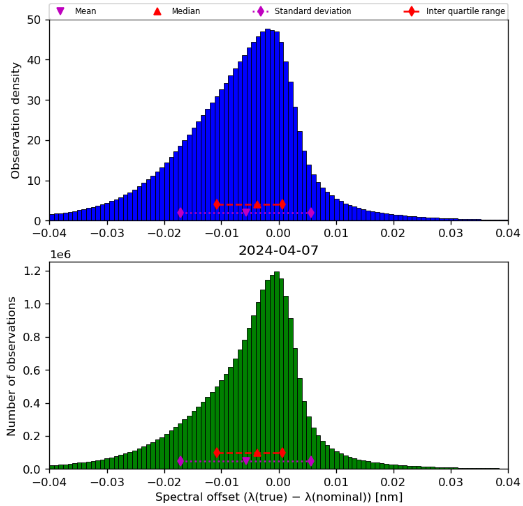
Figure 45: Histogram of “Spectral offset ( \lambda(\text{true}) - \lambda(\text{nominal}) )” for 2024-04-06 to 2024-04-08
