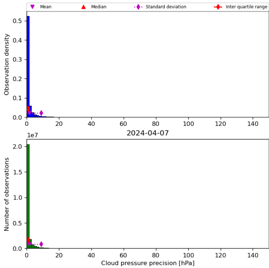
Figure 31: Histogram of “Cloud pressure precision” for 2024-04-06 to 2024-04-08
