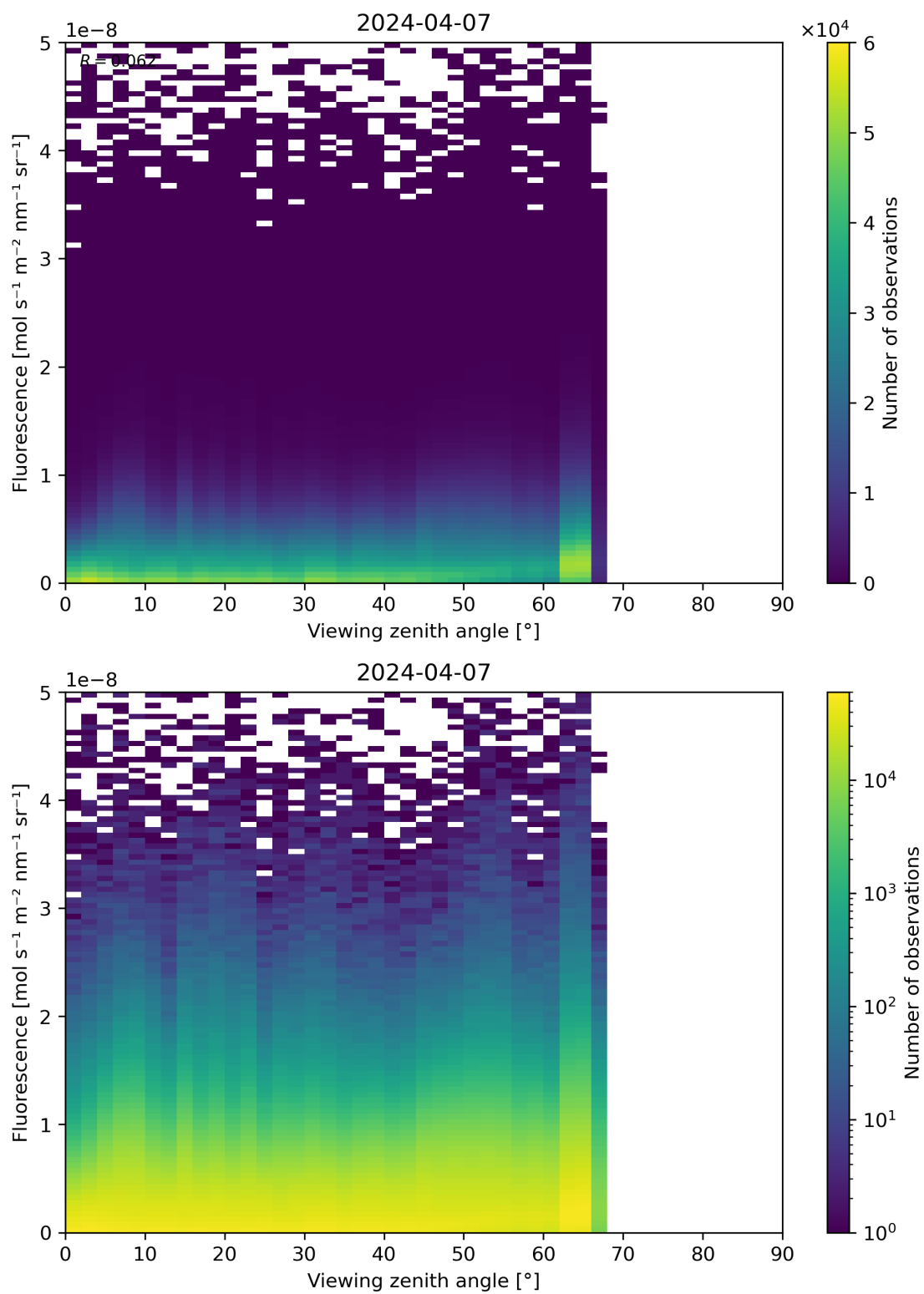
Figure 122: Scatter density plot of “Viewing zenith angle” against “Fluorescence” for 2024-04-06 to 2024-04-08.
