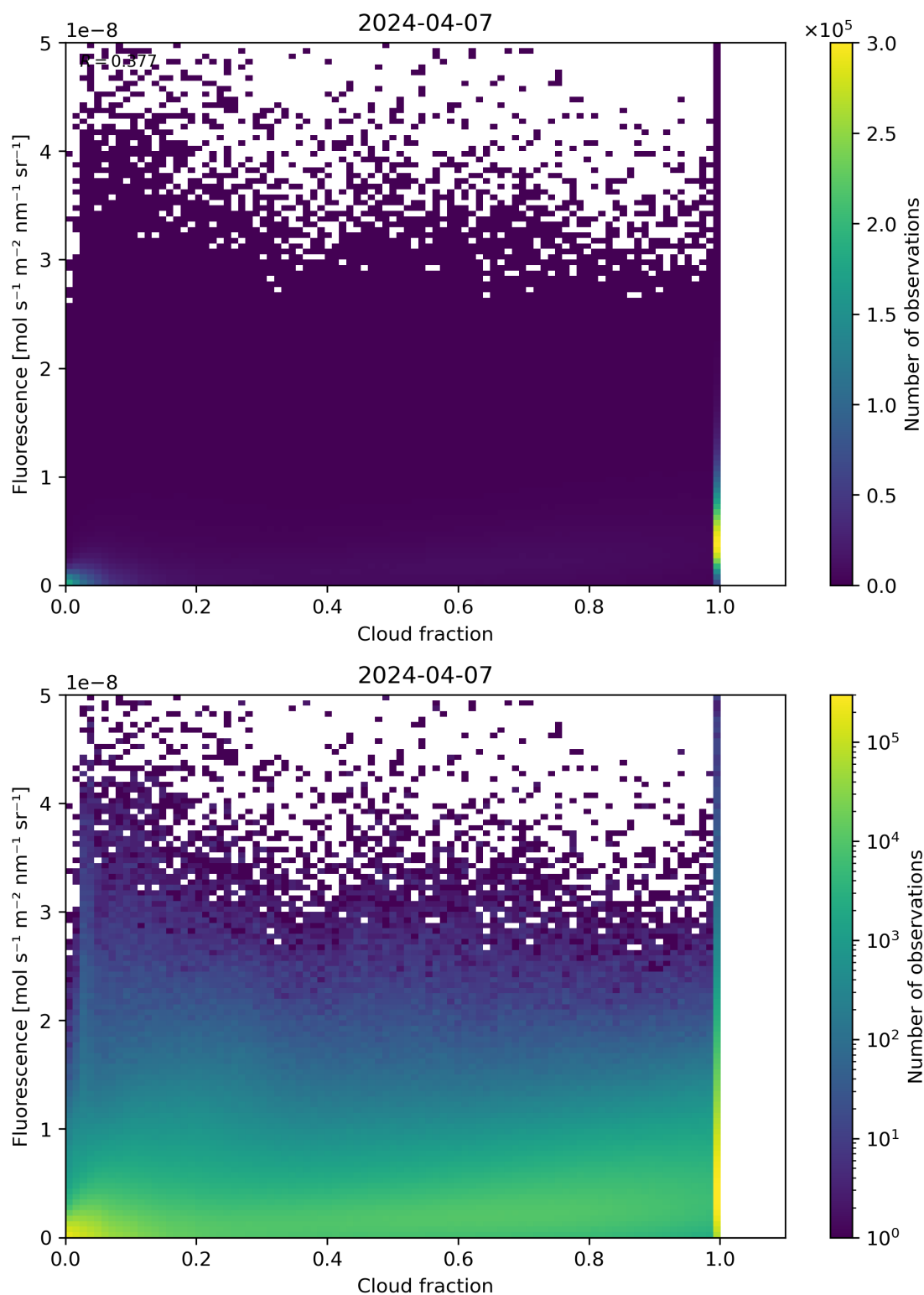
Figure 72: Scatter density plot of “Cloud fraction” against “Fluorescence” for 2024-04-06 to 2024-04-08.
