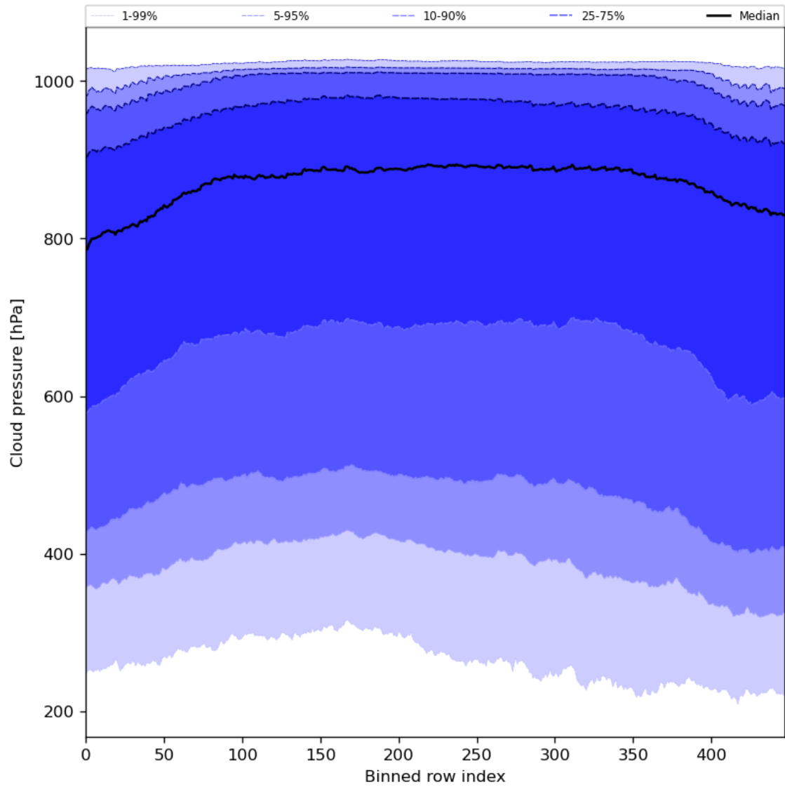
Figure 47: Along track statistics of “Cloud pressure” for 2024-04-06 to 2024-04-08
