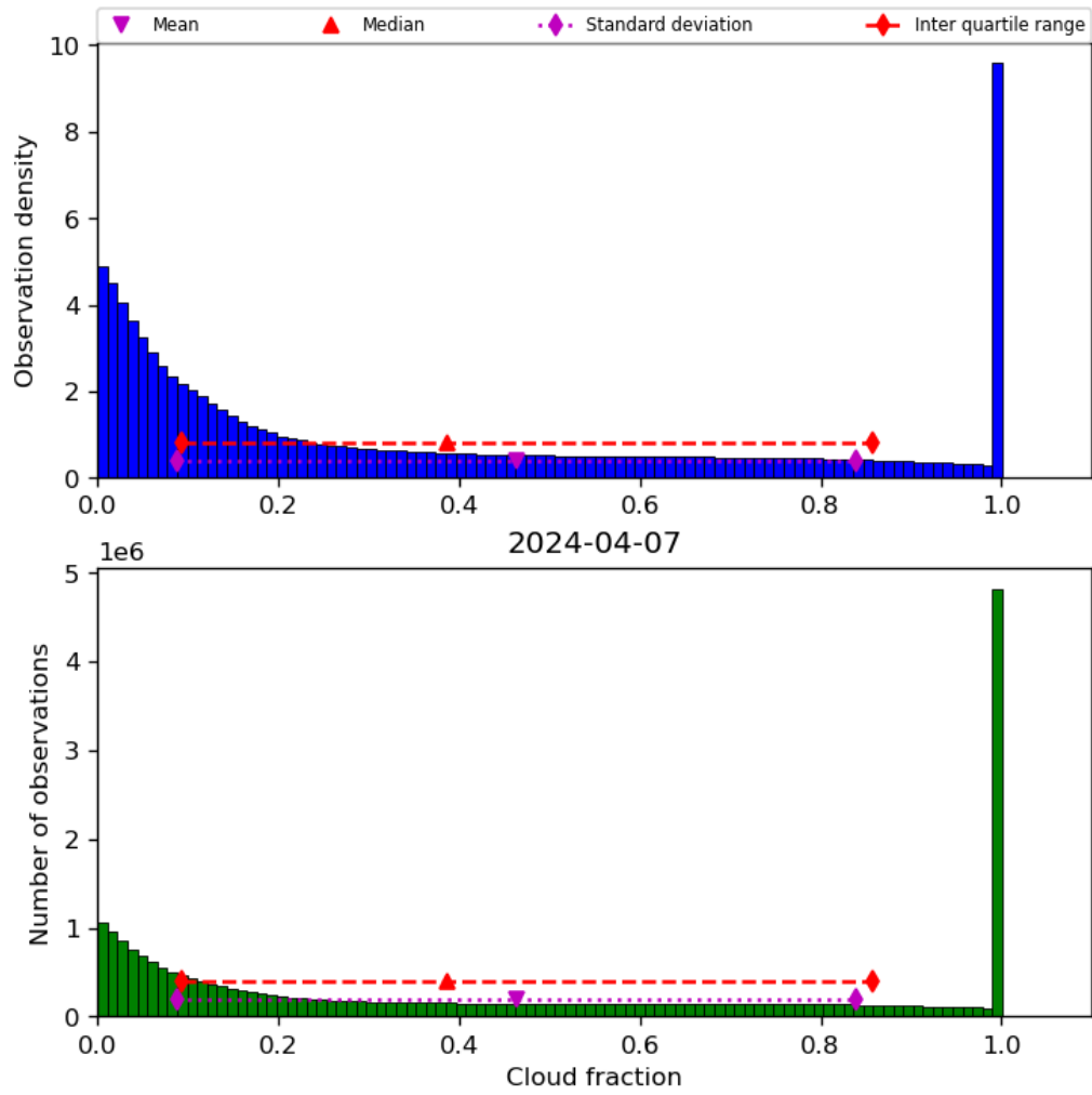
Figure 32: Histogram of “Cloud fraction” for 2024-04-06 to 2024-04-08
