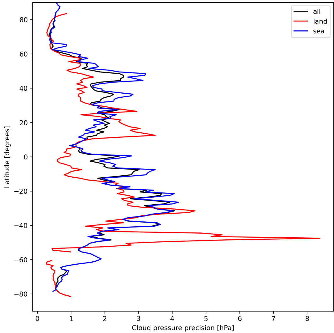
Figure 14: Zonal average of “Cloud pressure precision” for 2024-04-06 to 2024-04-08.
