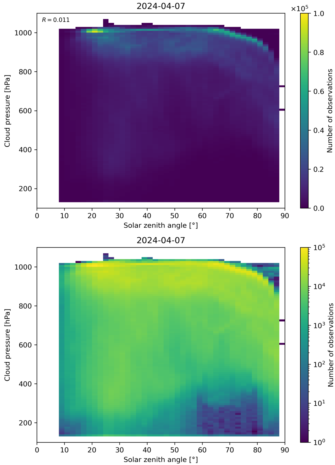
Figure 111: Scatter density plot of “Solar zenith angle” against “Cloud pressure” for 2024-04-06 to 2024-04-08.
