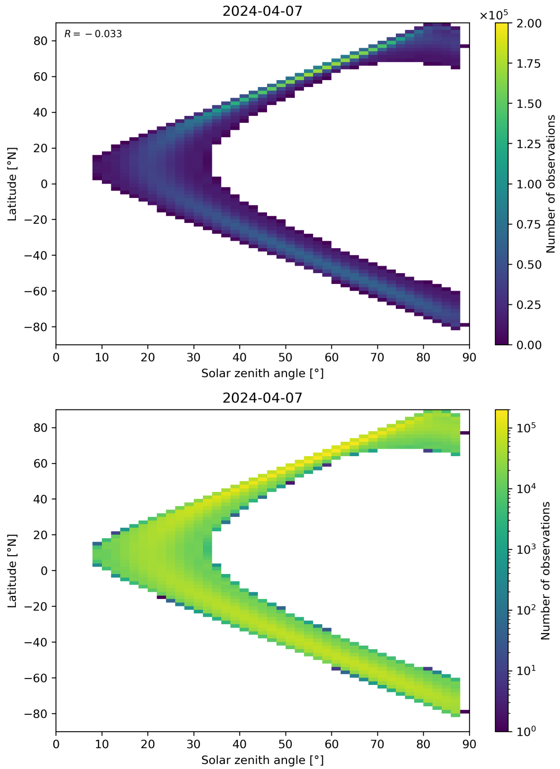
Figure 113: Scatter density plot of “Solar zenith angle” against “Latitude” for 2024-04-06 to 2024-04-08.
