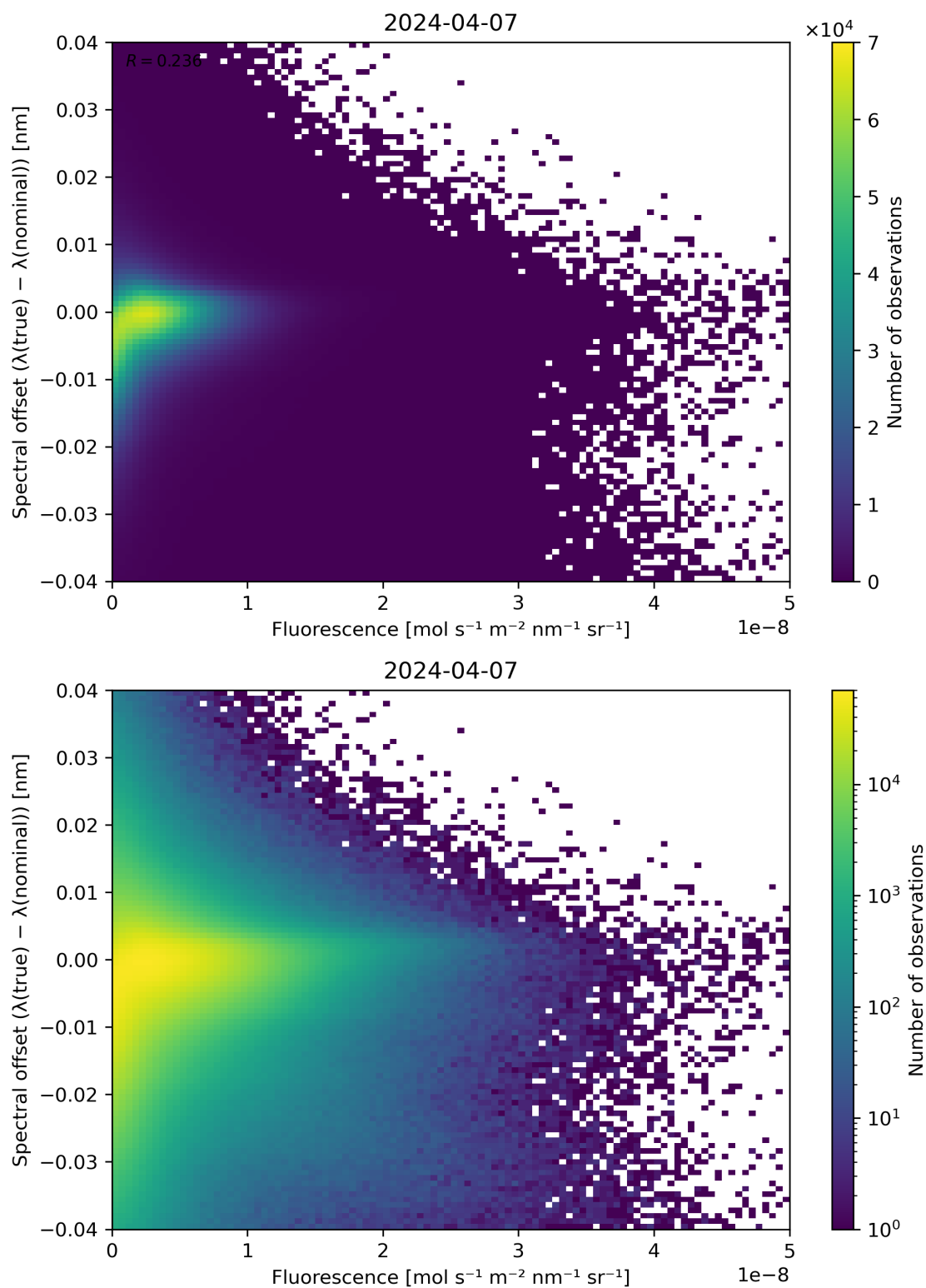
Figure 87: Scatter density plot of “Fluorescence” against “Spectral offset ( \lambda(\text{true}) - \lambda(\text{nominal}) )” for 2024-04-06 to 2024-04-08.
