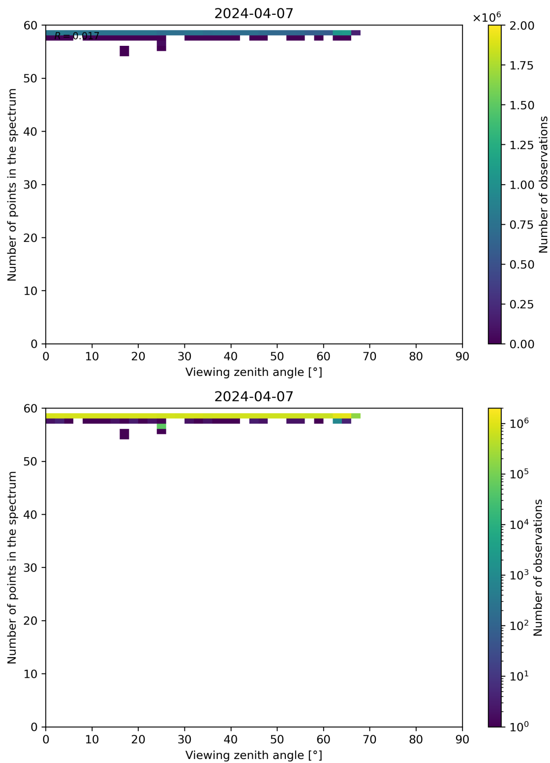
Figure 125: Scatter density plot of “Viewing zenith angle” against “Number of points in the spectrum” for 2024-04-06 to 2024-04-08.
