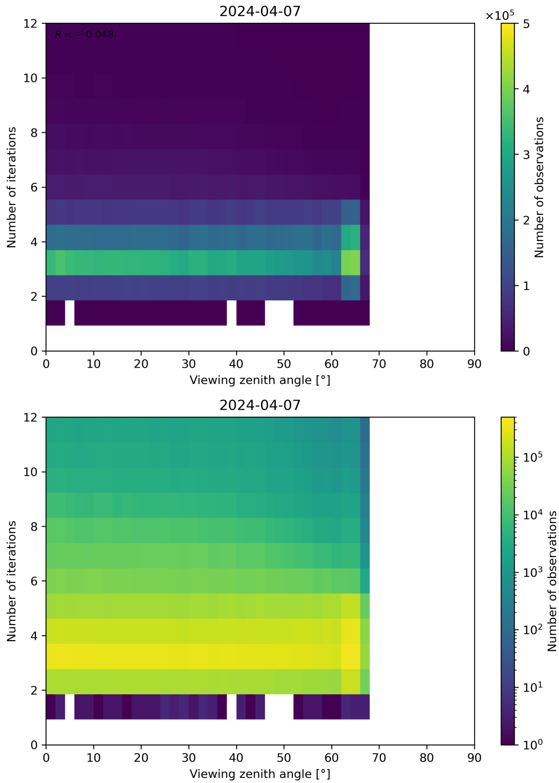
Figure 124: Scatter density plot of “Viewing zenith angle” against “Number of iterations” for 2024-04-06 to 2024-04-08.
