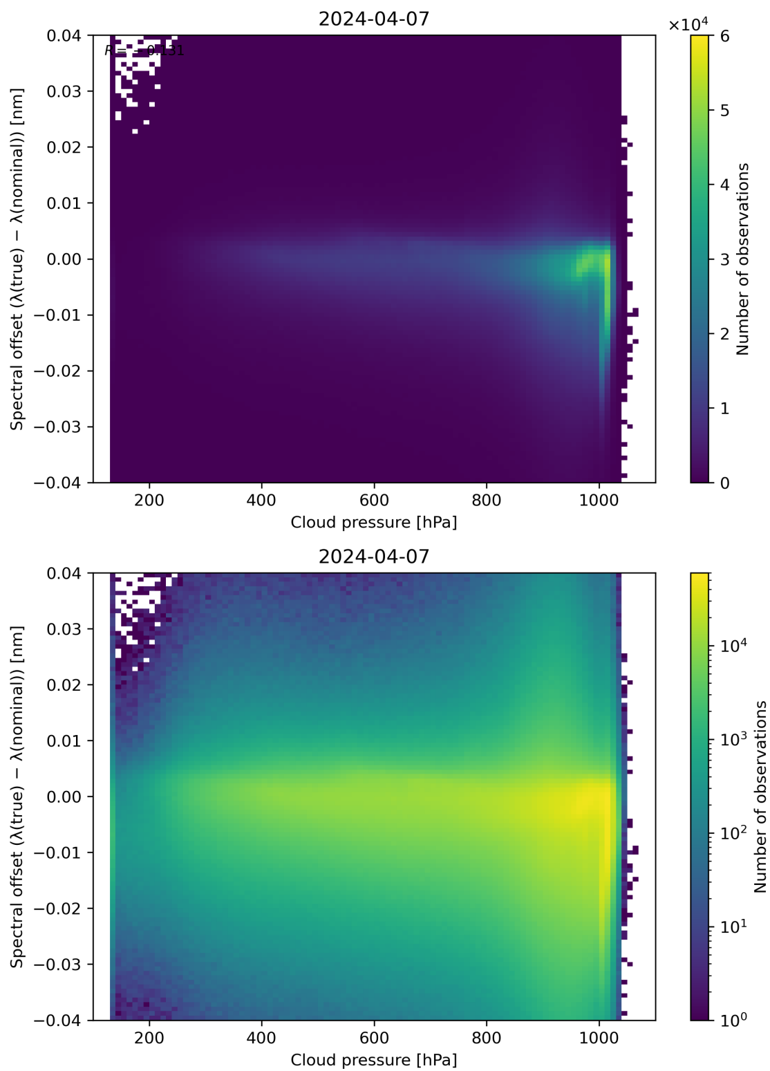
Figure 84: Scatter density plot of “Cloud pressure” against “Spectral offset ( \lambda(\text{true}) - \lambda(\text{nominal}) )” for 2024-04-06 to 2024-04-08.
