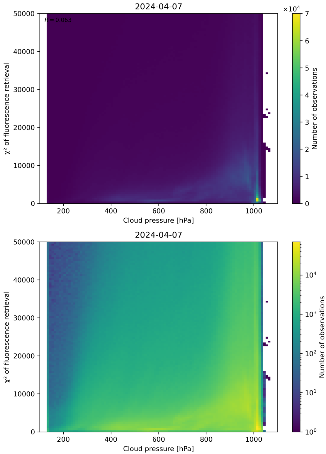
Figure 78: Scatter density plot of “Cloud pressure” against “ \chi^2 of fluorescence retrieval” for 2024-04-06 to 2024-04-08.
