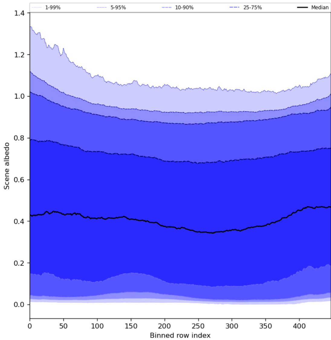
Figure 51: Along track statistics of “Scene albedo” for 2024-04-06 to 2024-04-08
