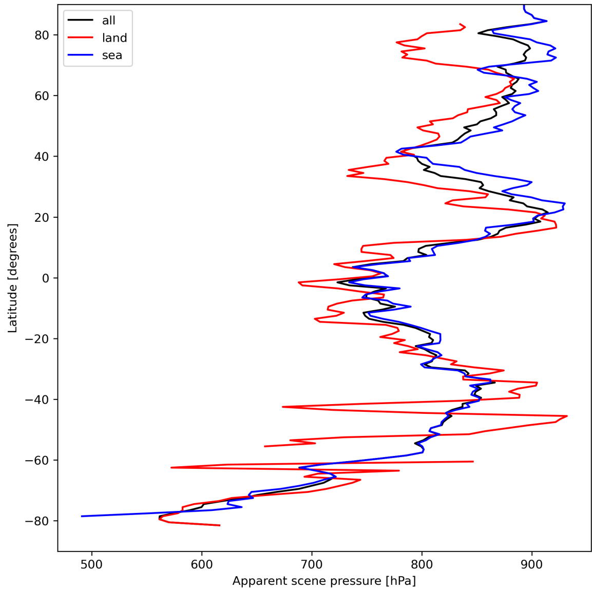
Figure 19: Zonal average of “Apparent scene pressure” for 2024-04-06 to 2024-04-08.
