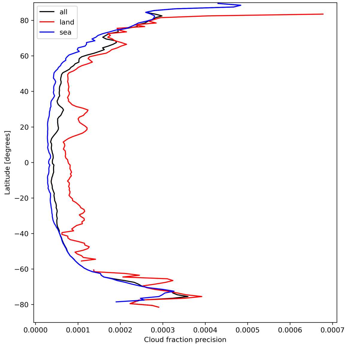
Figure 16: Zonal average of “Cloud fraction precision” for 2024-04-06 to 2024-04-08.
