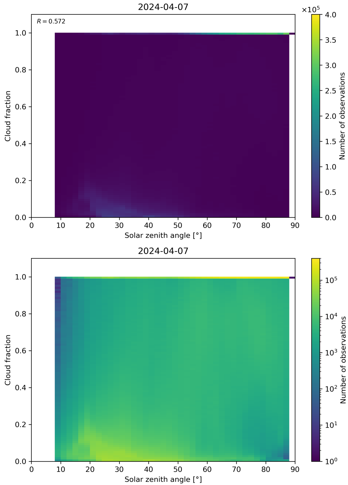
Figure 110: Scatter density plot of “Solar zenith angle” against “Cloud fraction” for 2024-04-06 to 2024-04-08.
