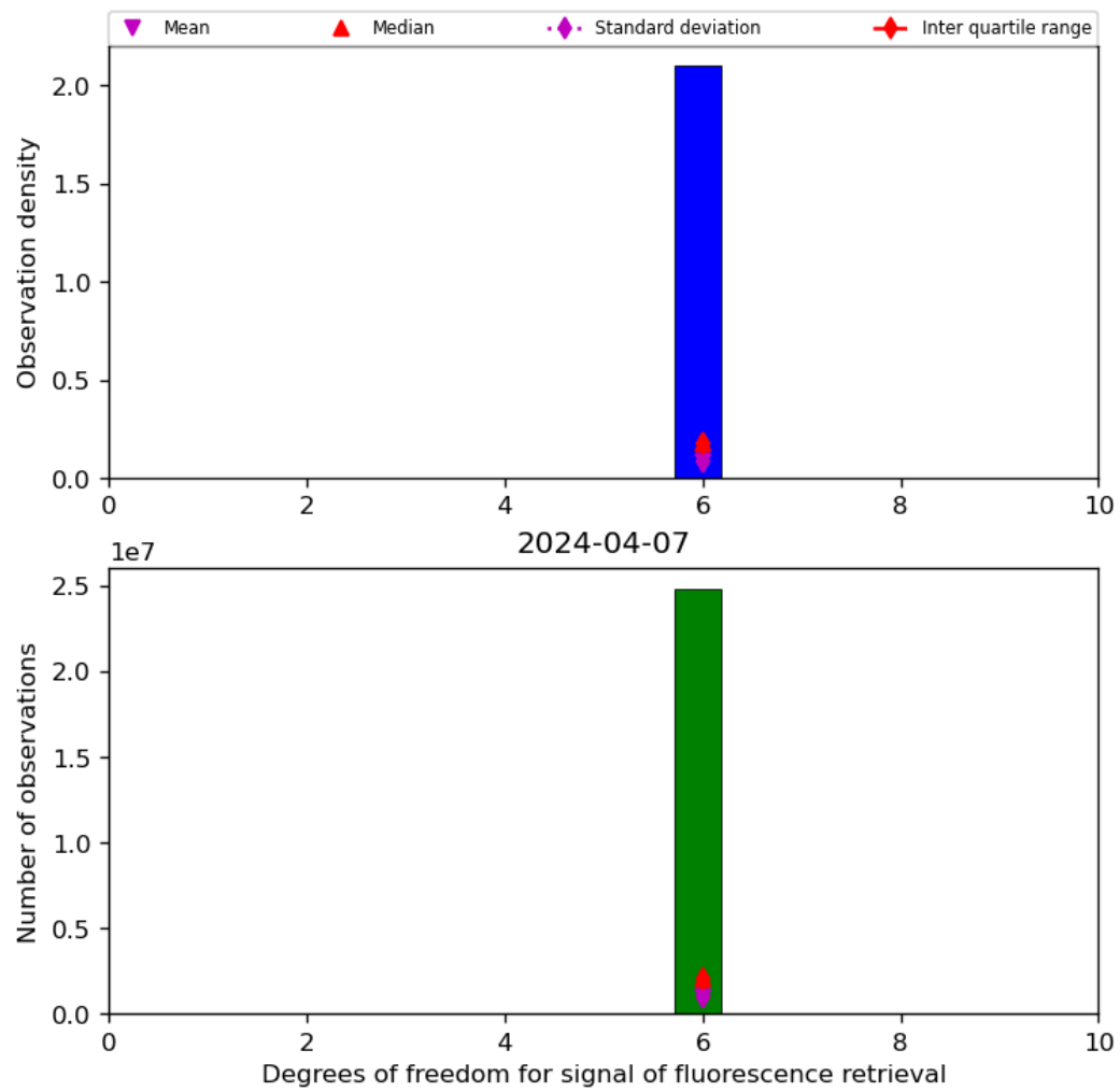
Figure 43: Histogram of “Degrees of freedom for signal of fluorescence retrieval” for 2024-04-06 to 2024-04-08
