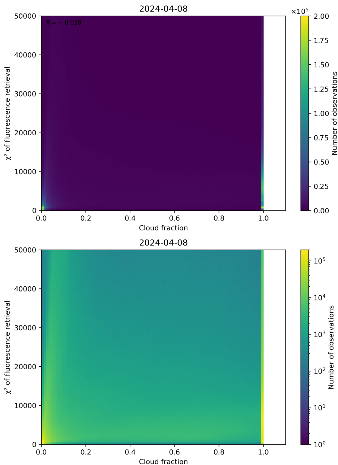
Figure 71: Scatter density plot of “Cloud fraction” against “ \chi^2 of fluorescence retrieval” for 2024-04-07 to 2024-04-09.
