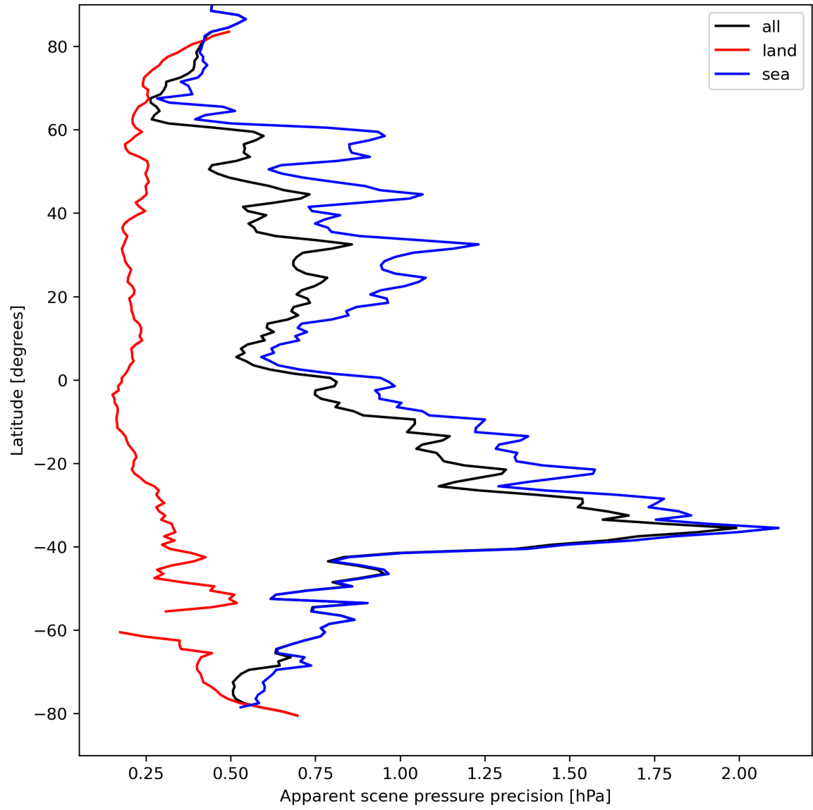
Figure 20: Zonal average of “Apparent scene pressure precision” for 2024-04-07 to 2024-04-09.
