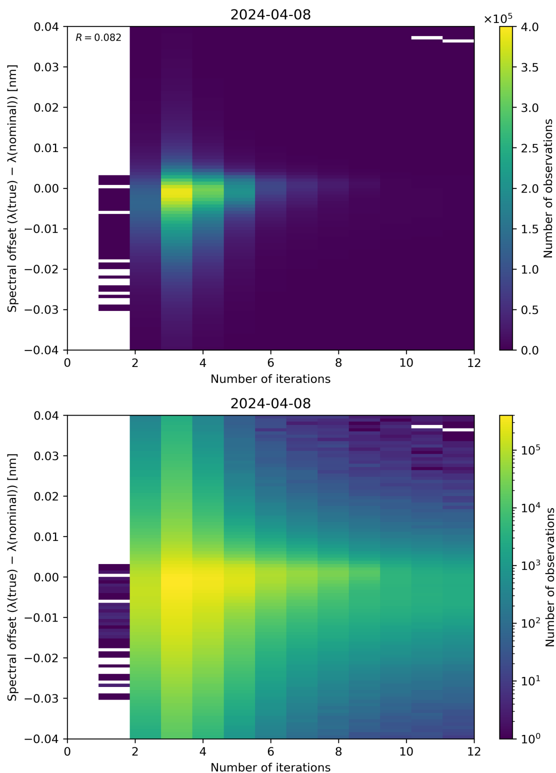
Figure 100: Scatter density plot of “Number of iterations” against “Spectral offset ( \lambda(\text{true}) - \lambda(\text{nominal}) )” for 2024-04-07 to 2024-04-09.
