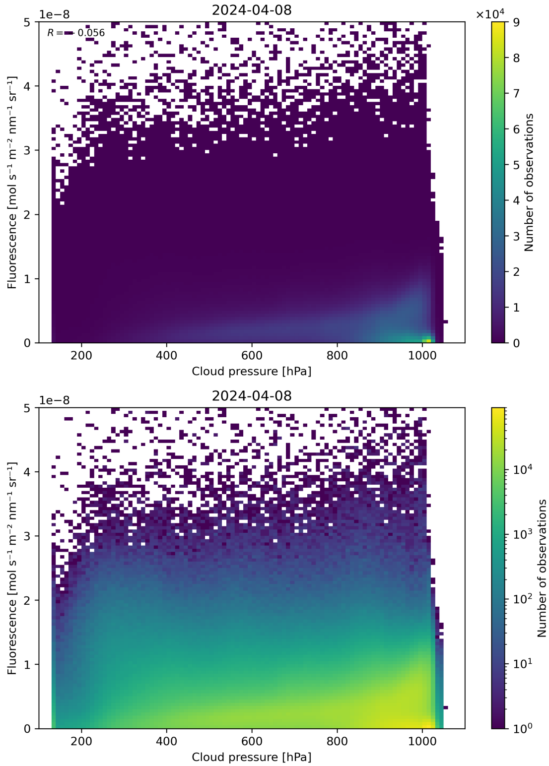
Figure 80: Scatter density plot of “Cloud pressure” against “Fluorescence” for 2024-04-07 to 2024-04-09.
