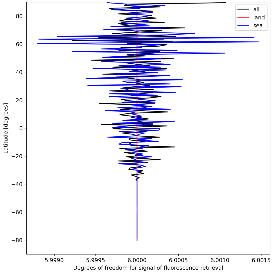
Figure 26: Zonal average of “Degrees of freedom for signal of fluorescence retrieval” for 2024-04-07 to 2024-04-09.
