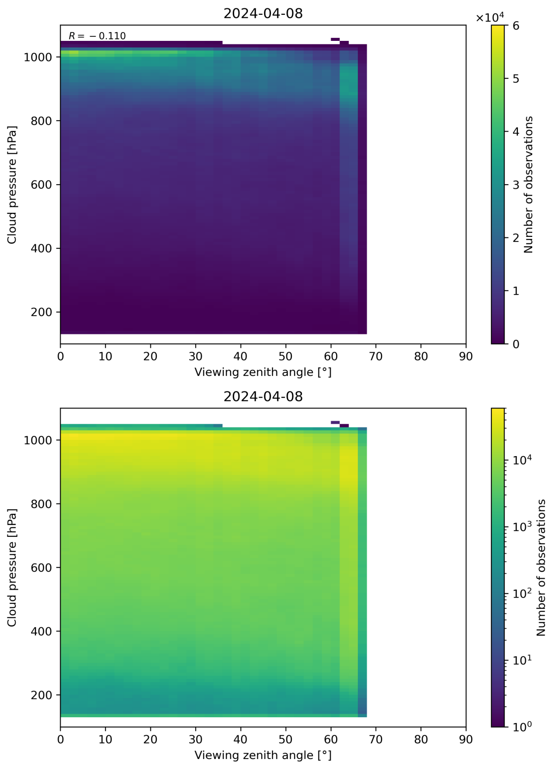
Figure 121: Scatter density plot of “Viewing zenith angle” against “Cloud pressure” for 2024-04-07 to 2024-04-09.
