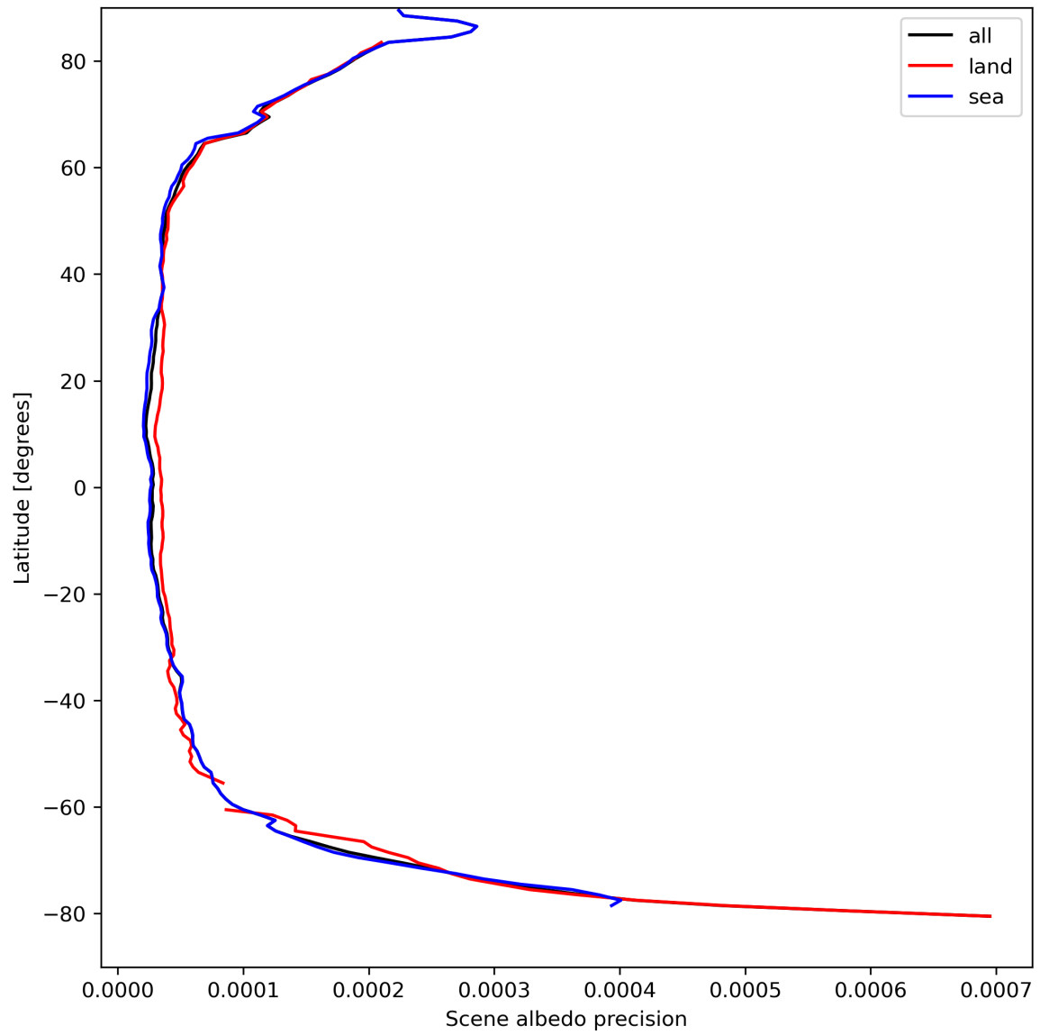
Figure 18: Zonal average of “Scene albedo precision” for 2024-04-07 to 2024-04-09.
