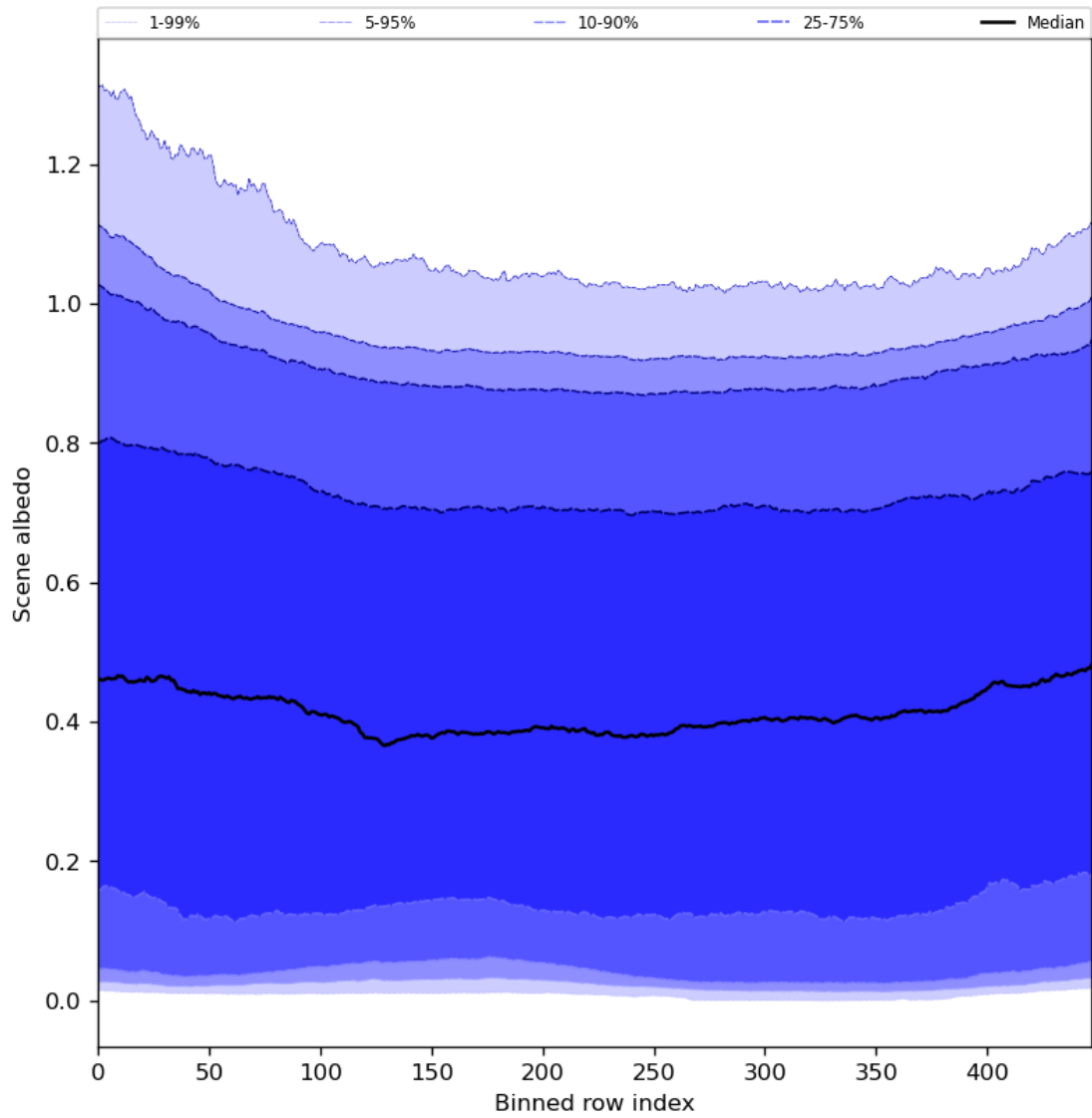
Figure 51: Along track statistics of “Scene albedo” for 2024-04-07 to 2024-04-09
