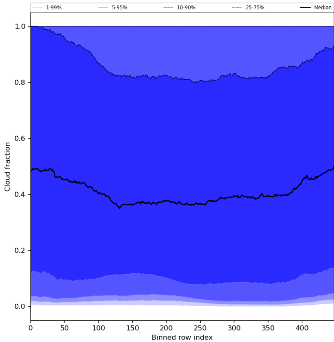
Figure 49: Along track statistics of “Cloud fraction” for 2024-04-07 to 2024-04-09
