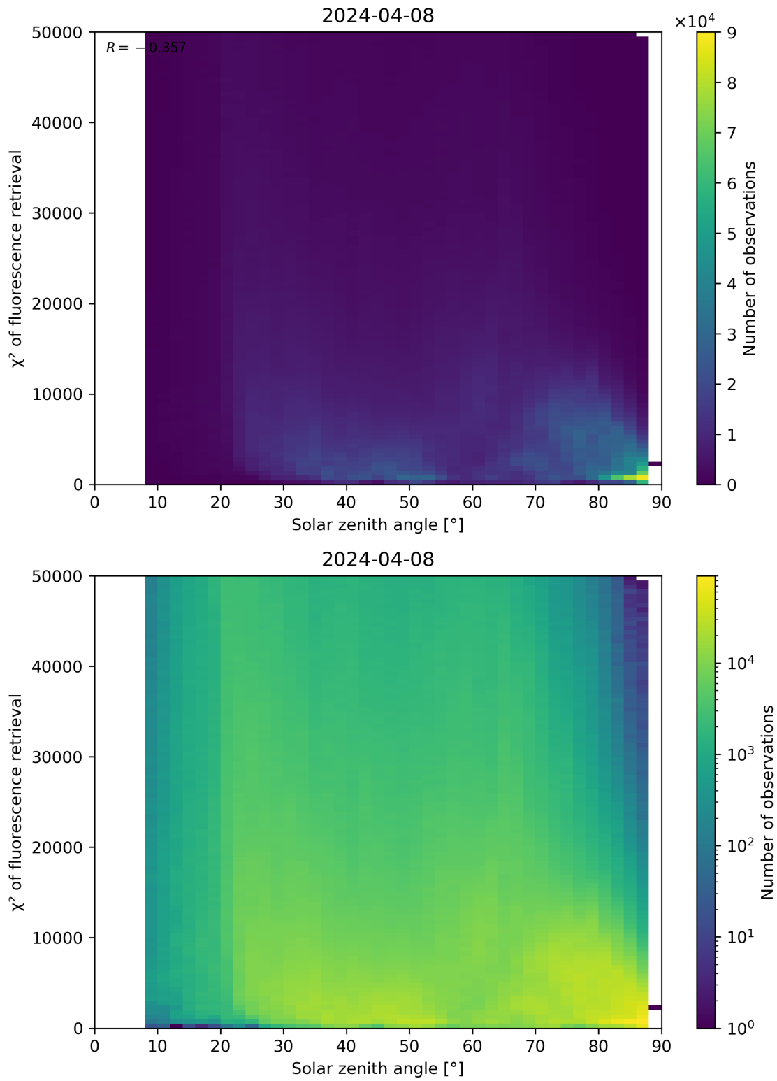
Figure 109: Scatter density plot of “Solar zenith angle” against “ \chi^2 of fluorescence retrieval” for 2024-04-07 to 2024-04-09.
