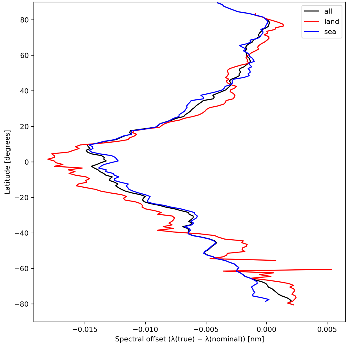
Figure 28: Zonal average of “Spectral offset ( \lambda(\text{true}) - \lambda(\text{nominal}) )” for 2024-04-07 to 2024-04-09.
