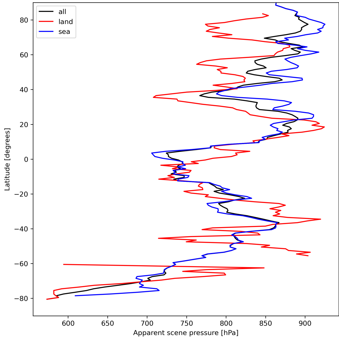
Figure 19: Zonal average of “Apparent scene pressure” for 2024-04-07 to 2024-04-09.
