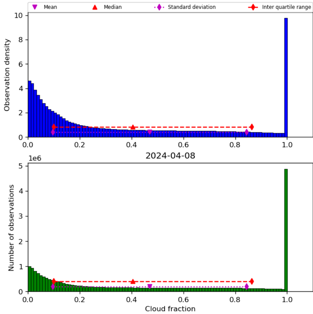
Figure 32: Histogram of “Cloud fraction” for 2024-04-07 to 2024-04-09
