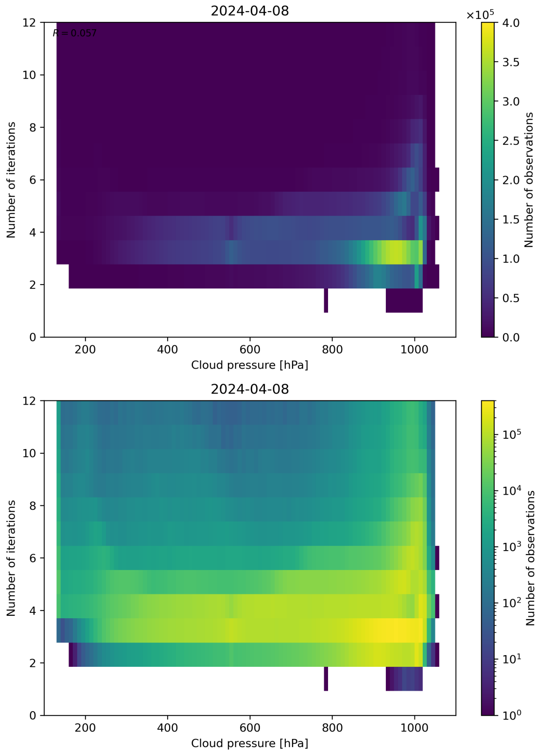
Figure 81: Scatter density plot of “Cloud pressure” against “Number of iterations” for 2024-04-07 to 2024-04-09.
