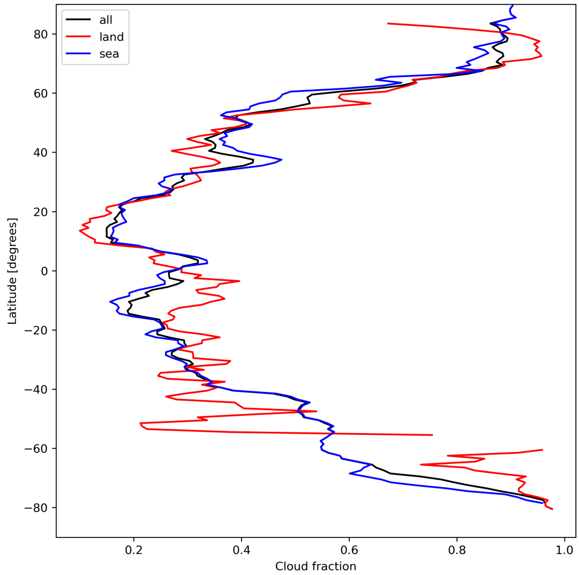
Figure 15: Zonal average of “Cloud fraction” for 2024-04-07 to 2024-04-09.
