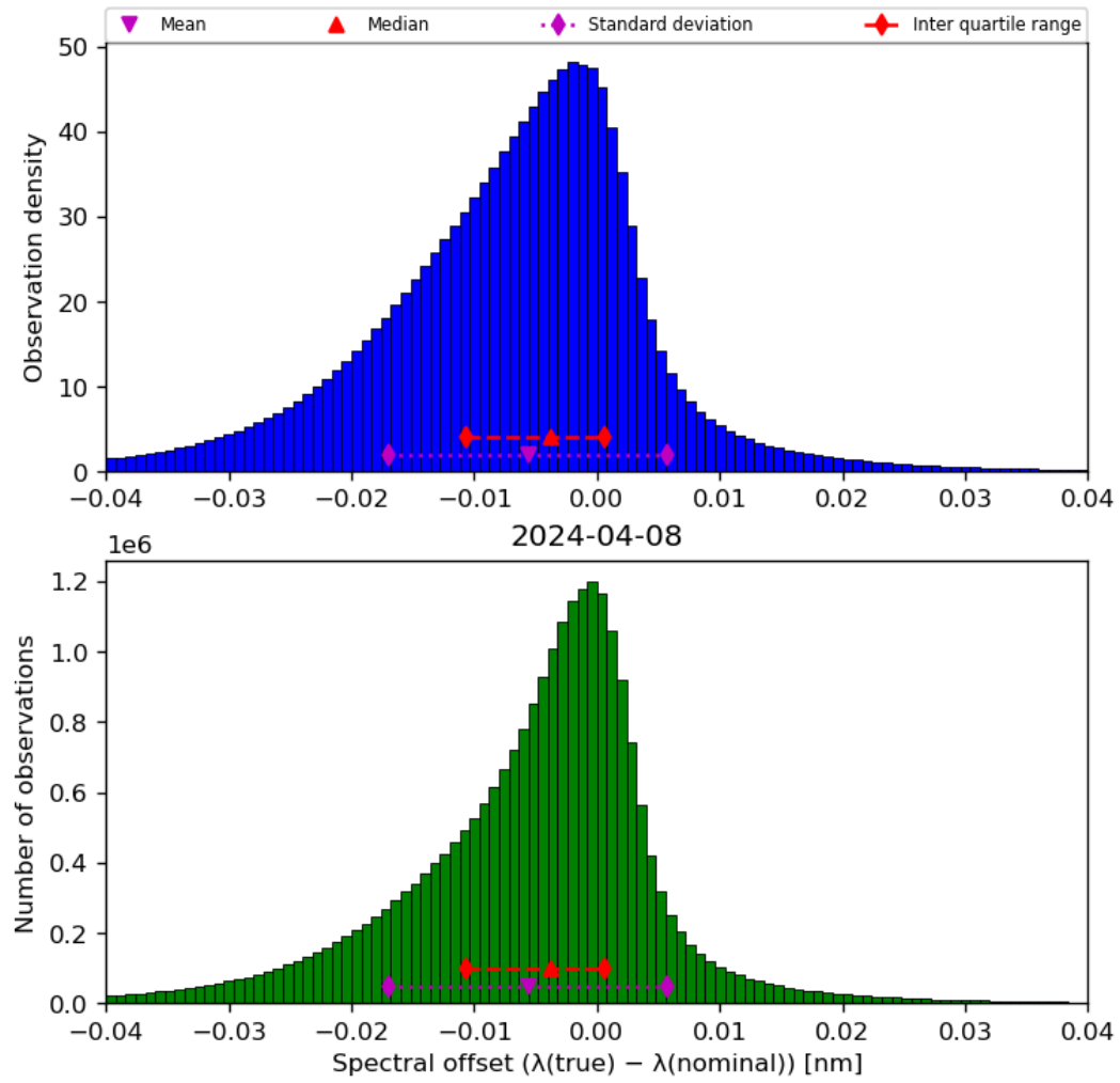
Figure 45: Histogram of “Spectral offset ( \lambda(\text{true}) - \lambda(\text{nominal}) )” for 2024-04-07 to 2024-04-09
