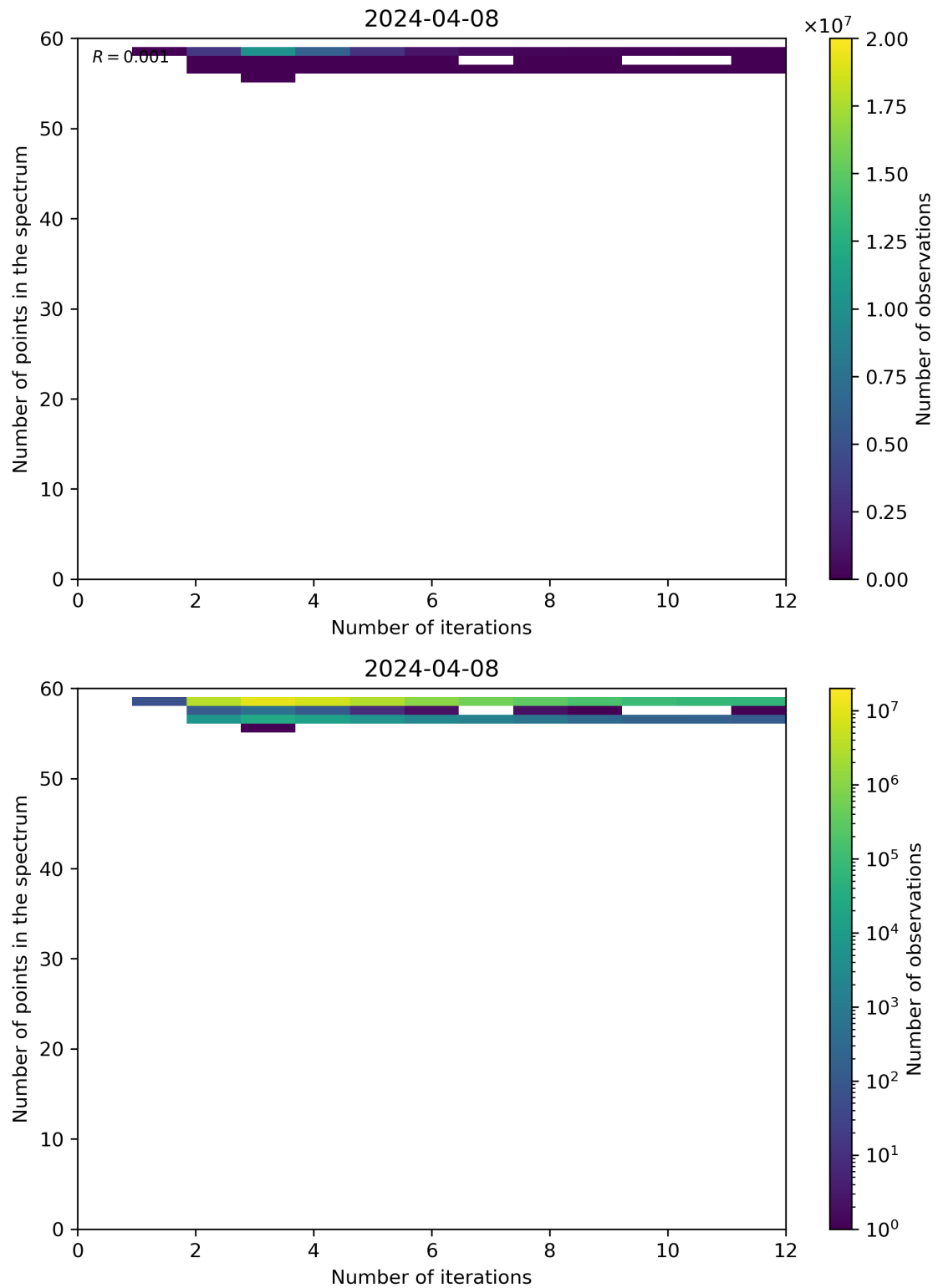
Figure 99: Scatter density plot of “Number of iterations” against “Number of points in the spectrum” for 2024-04-07 to 2024-04-09.
