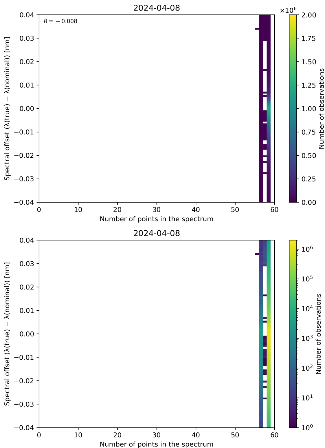
Figure 101: Scatter density plot of “Number of points in the spectrum” against “Spectral offset ( \lambda(\text{true}) - \lambda(\text{nominal}) )” for 2024-04-07 to 2024-04-09.
