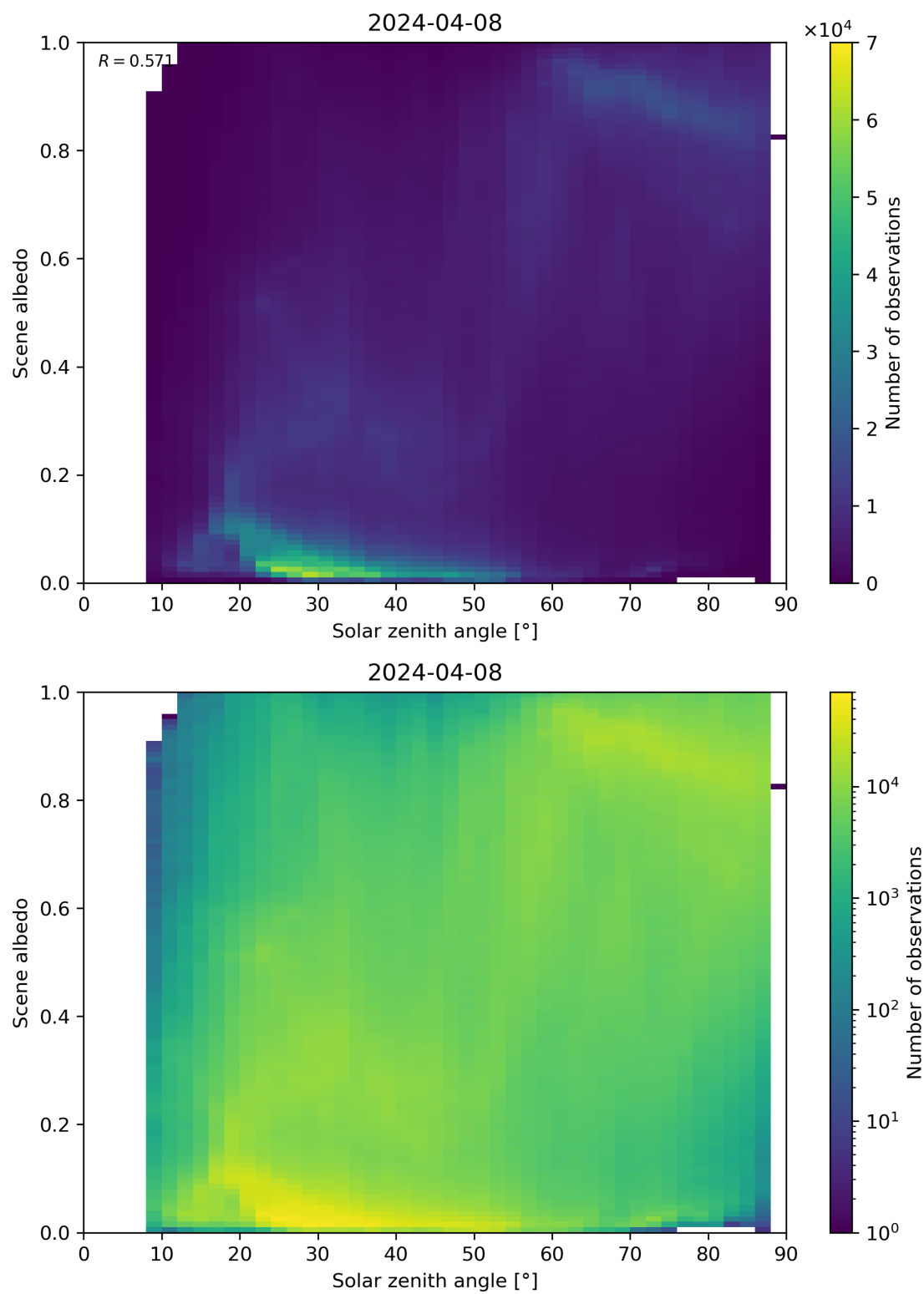
Figure 116: Scatter density plot of “Solar zenith angle” against “Scene albedo” for 2024-04-07 to 2024-04-09.
