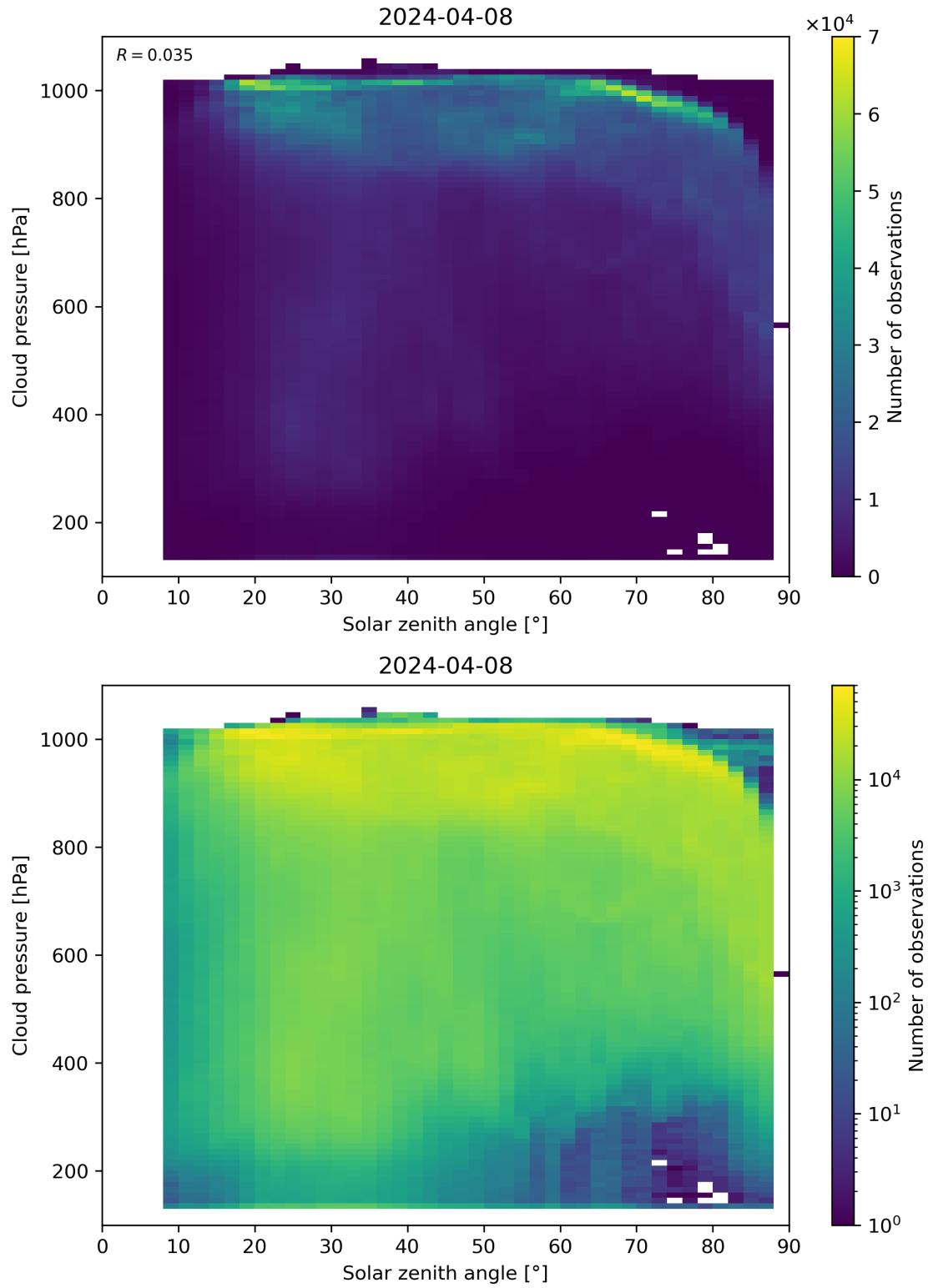
Figure 111: Scatter density plot of “Solar zenith angle” against “Cloud pressure” for 2024-04-07 to 2024-04-09.
