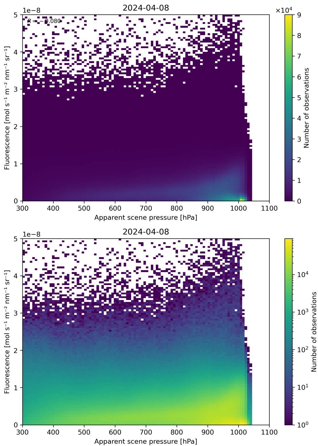
Figure 64: Scatter density plot of “Apparent scene pressure” against “Fluorescence” for 2024-04-07 to 2024-04-09.
