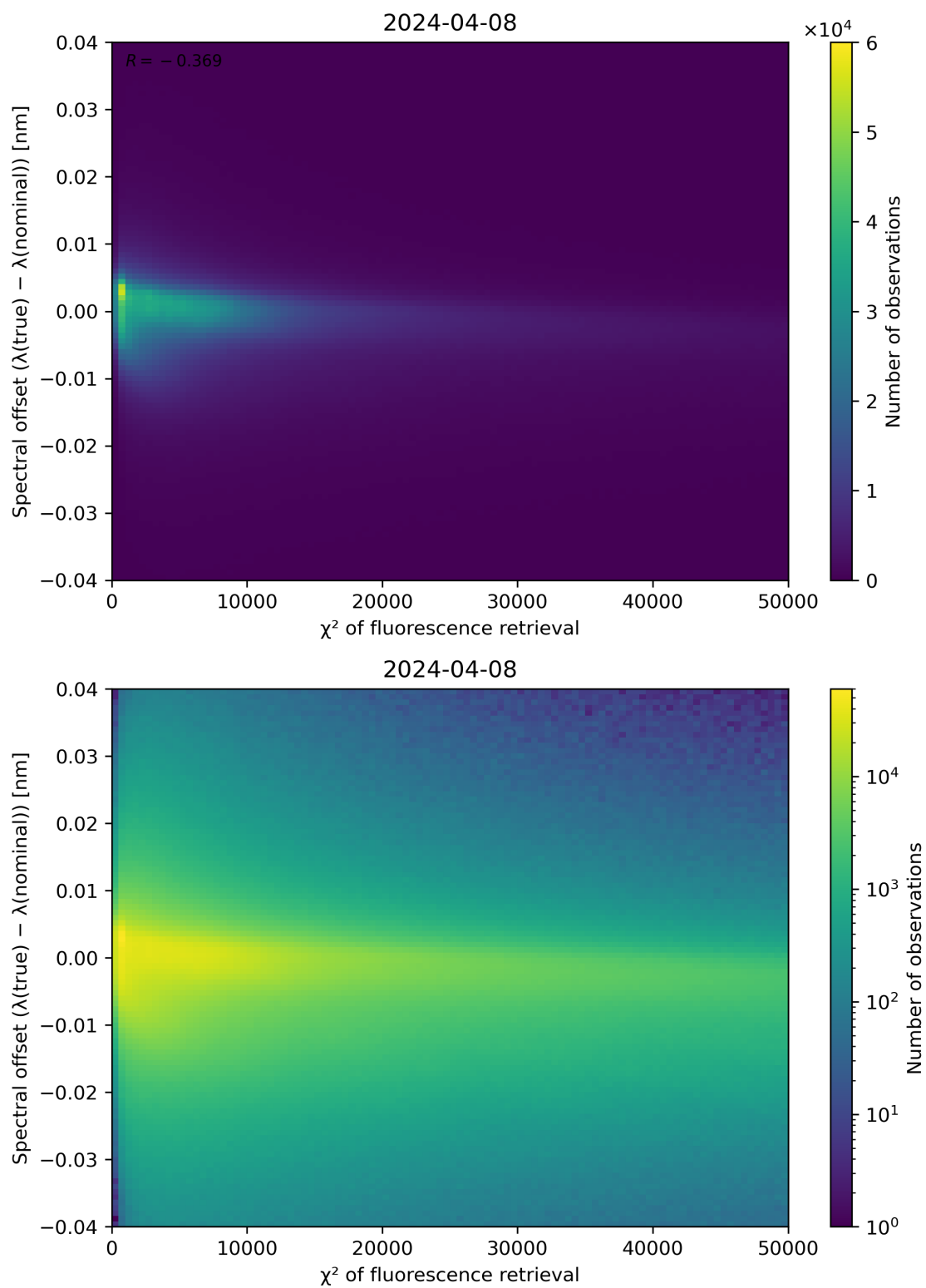
Figure 69: Scatter density plot of " \chi^2 of fluorescence retrieval" against "Spectral offset ( \lambda(\text{true}) - \lambda(\text{nominal}) )" for 2024-04-07 to 2024-04-09.
