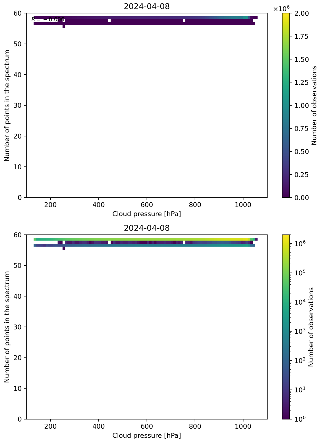
Figure 82: Scatter density plot of “Cloud pressure” against “Number of points in the spectrum” for 2024-04-07 to 2024-04-09.
