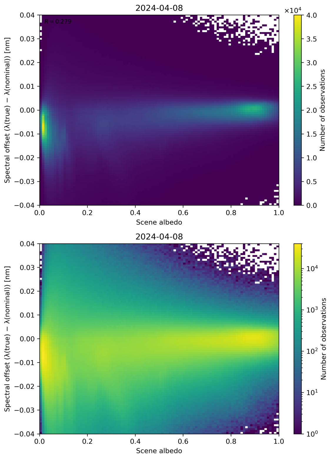
Figure 107: Scatter density plot of “Scene albedo” against “Spectral offset ( \lambda(\text{true}) - \lambda(\text{nominal}) )” for 2024-04-07 to 2024-04-09.
