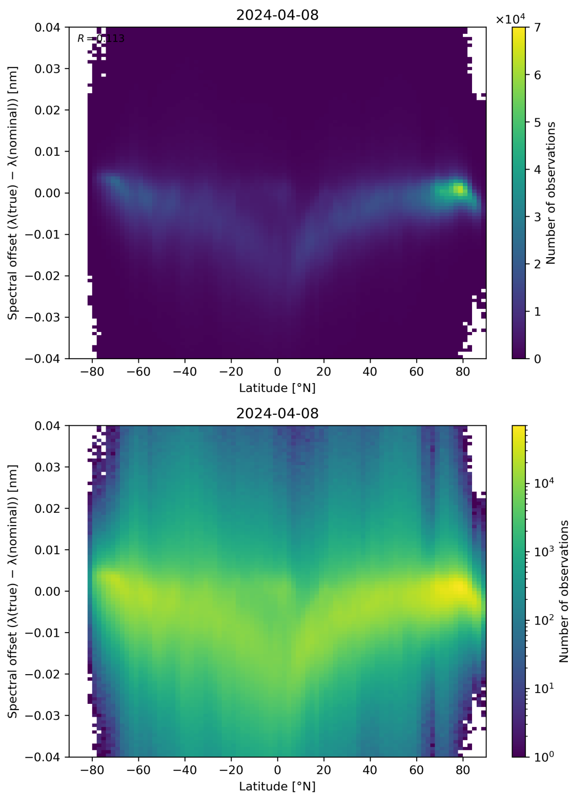
Figure 96: Scatter density plot of “Latitude” against “Spectral offset ( \lambda(\text{true}) - \lambda(\text{nominal}) )” for 2024-04-07 to 2024-04-09.
