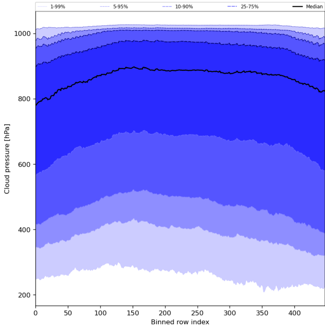
Figure 47: Along track statistics of “Cloud pressure” for 2024-04-07 to 2024-04-09
