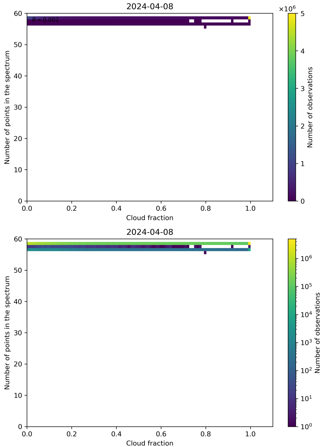
Figure 74: Scatter density plot of “Cloud fraction” against “Number of points in the spectrum” for 2024-04-07 to 2024-04-09.
