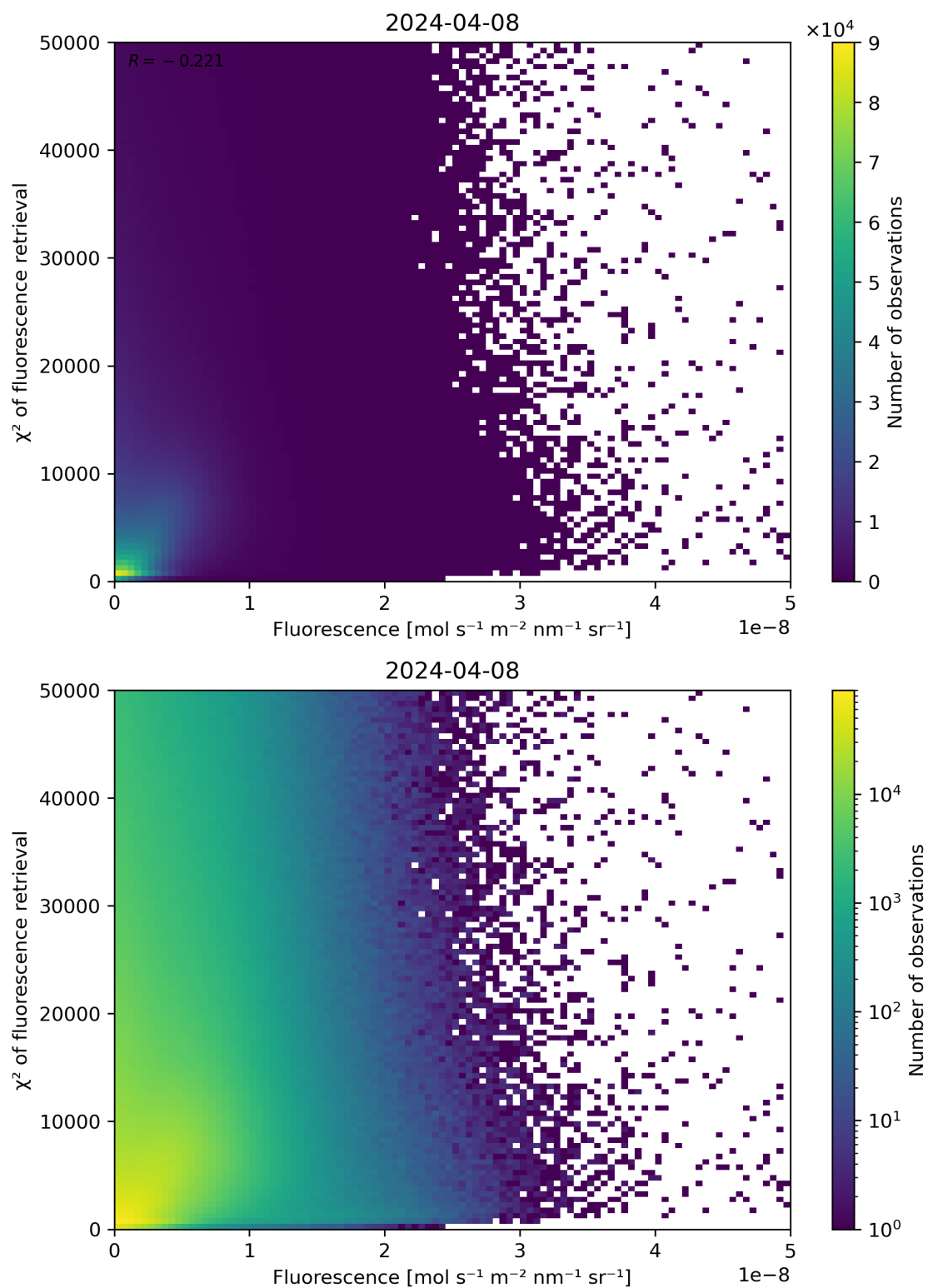
Figure 85: Scatter density plot of “Fluorescence” against “ \chi^2 of fluorescence retrieval” for 2024-04-07 to 2024-04-09.
