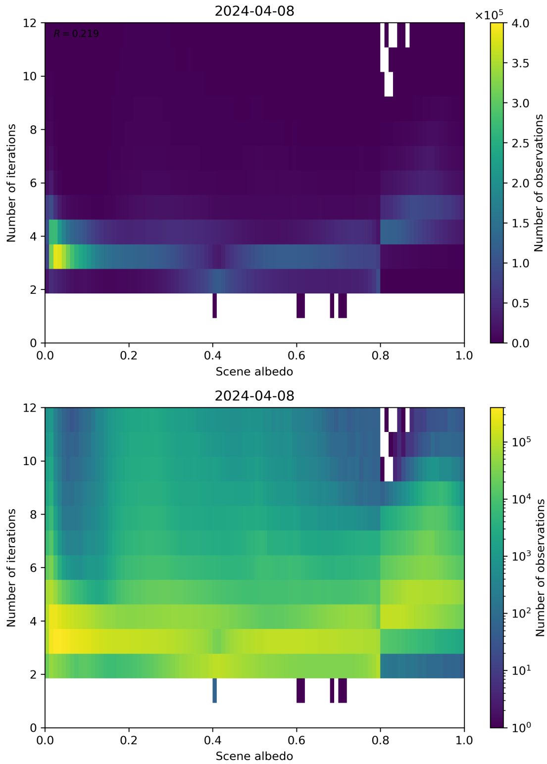
Figure 105: Scatter density plot of “Scene albedo” against “Number of iterations” for 2024-04-07 to 2024-04-09.
