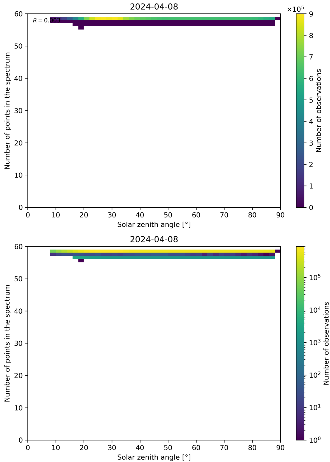
Figure 115: Scatter density plot of “Solar zenith angle” against “Number of points in the spectrum” for 2024-04-07 to 2024-04-09.
