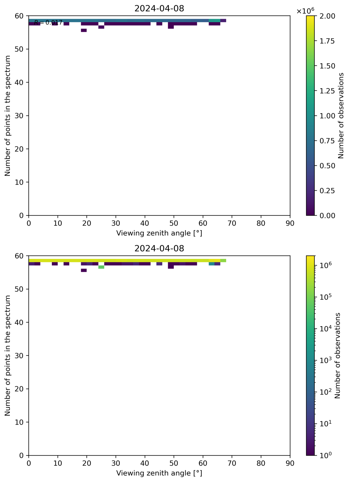
Figure 125: Scatter density plot of “Viewing zenith angle” against “Number of points in the spectrum” for 2024-04-07 to 2024-04-09.
