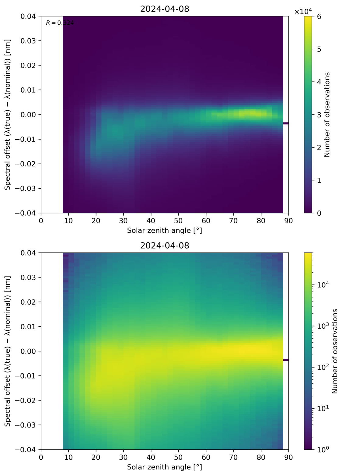
Figure 117: Scatter density plot of “Solar zenith angle” against “Spectral offset ( \lambda(\text{true}) - \lambda(\text{nominal}) )” for 2024-04-07 to 2024-04-09.
