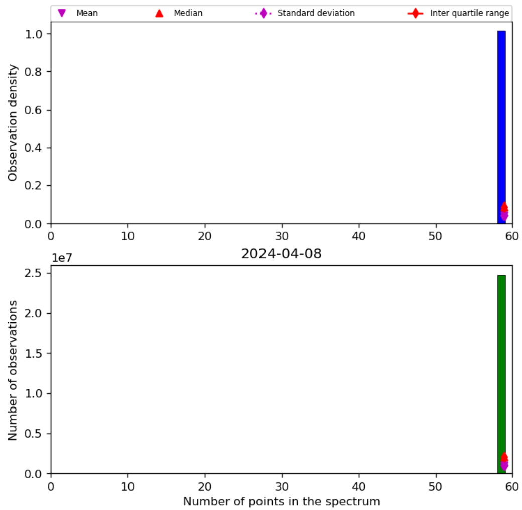
Figure 44: Histogram of “Number of points in the spectrum” for 2024-04-07 to 2024-04-09
