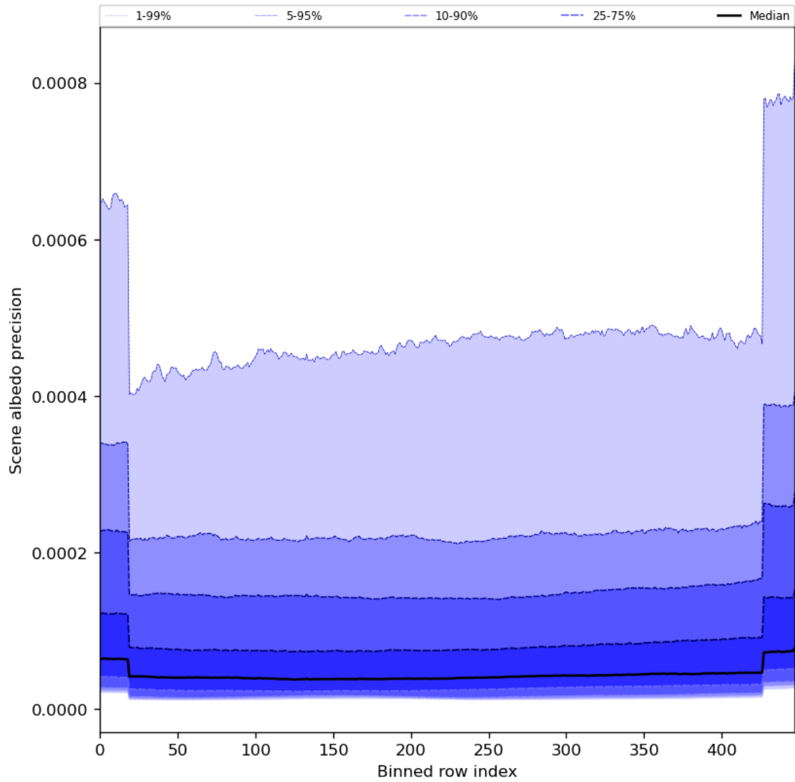
Figure 52: Along track statistics of “Scene albedo precision” for 2024-04-07 to 2024-04-09
