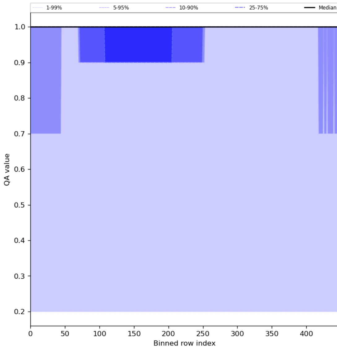
Figure 46: Along track statistics of “QA value” for 2024-04-07 to 2024-04-09
