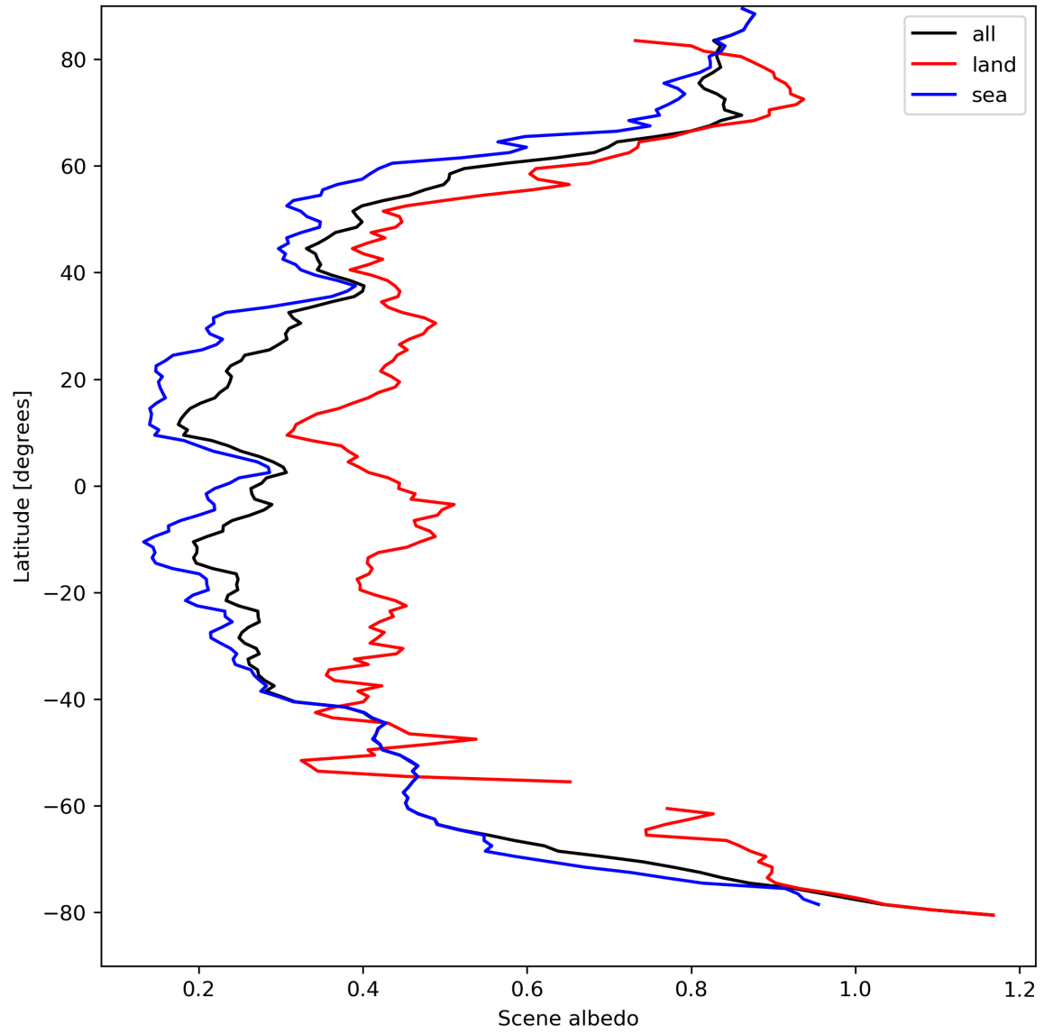
Figure 17: Zonal average of “Scene albedo” for 2024-04-07 to 2024-04-09.
