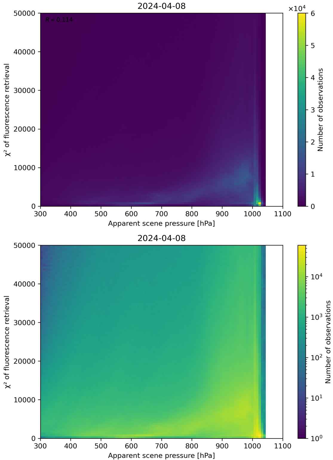
Figure 63: Scatter density plot of “Apparent scene pressure” against “ \chi^2 of fluorescence retrieval” for 2024-04-07 to 2024-04-09.
