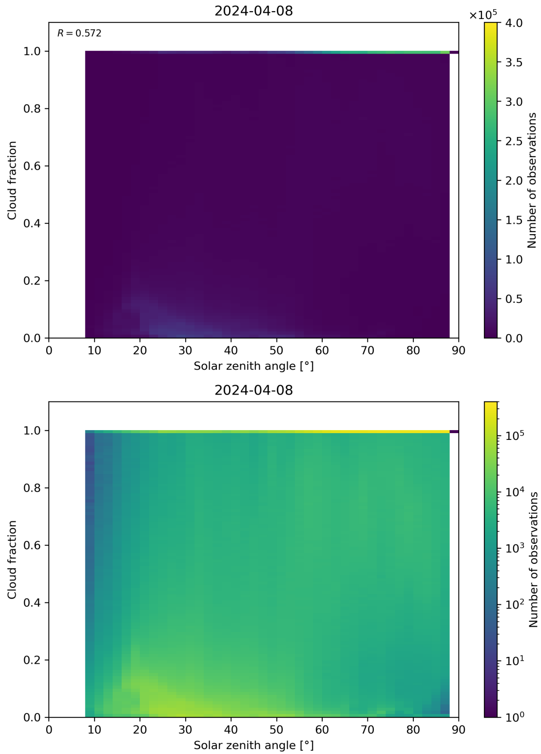
Figure 110: Scatter density plot of “Solar zenith angle” against “Cloud fraction” for 2024-04-07 to 2024-04-09.
