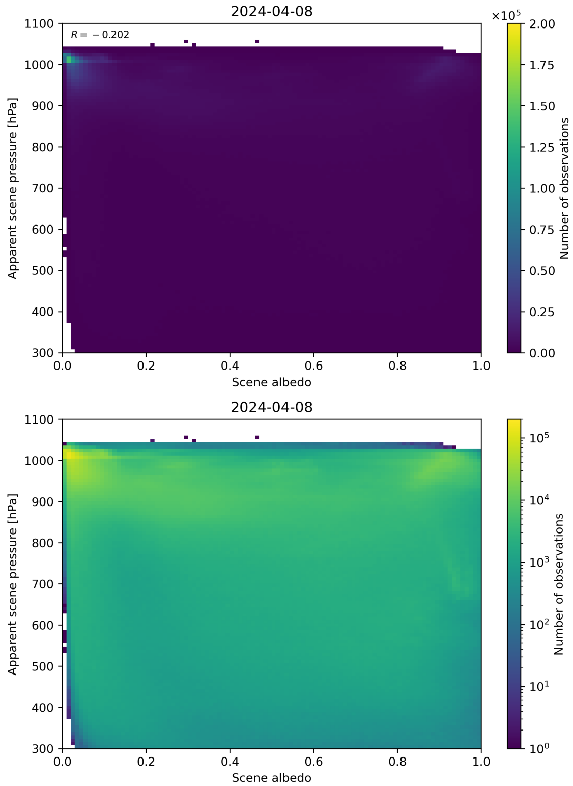
Figure 102: Scatter density plot of “Scene albedo” against “Apparent scene pressure” for 2024-04-07 to 2024-04-09.
