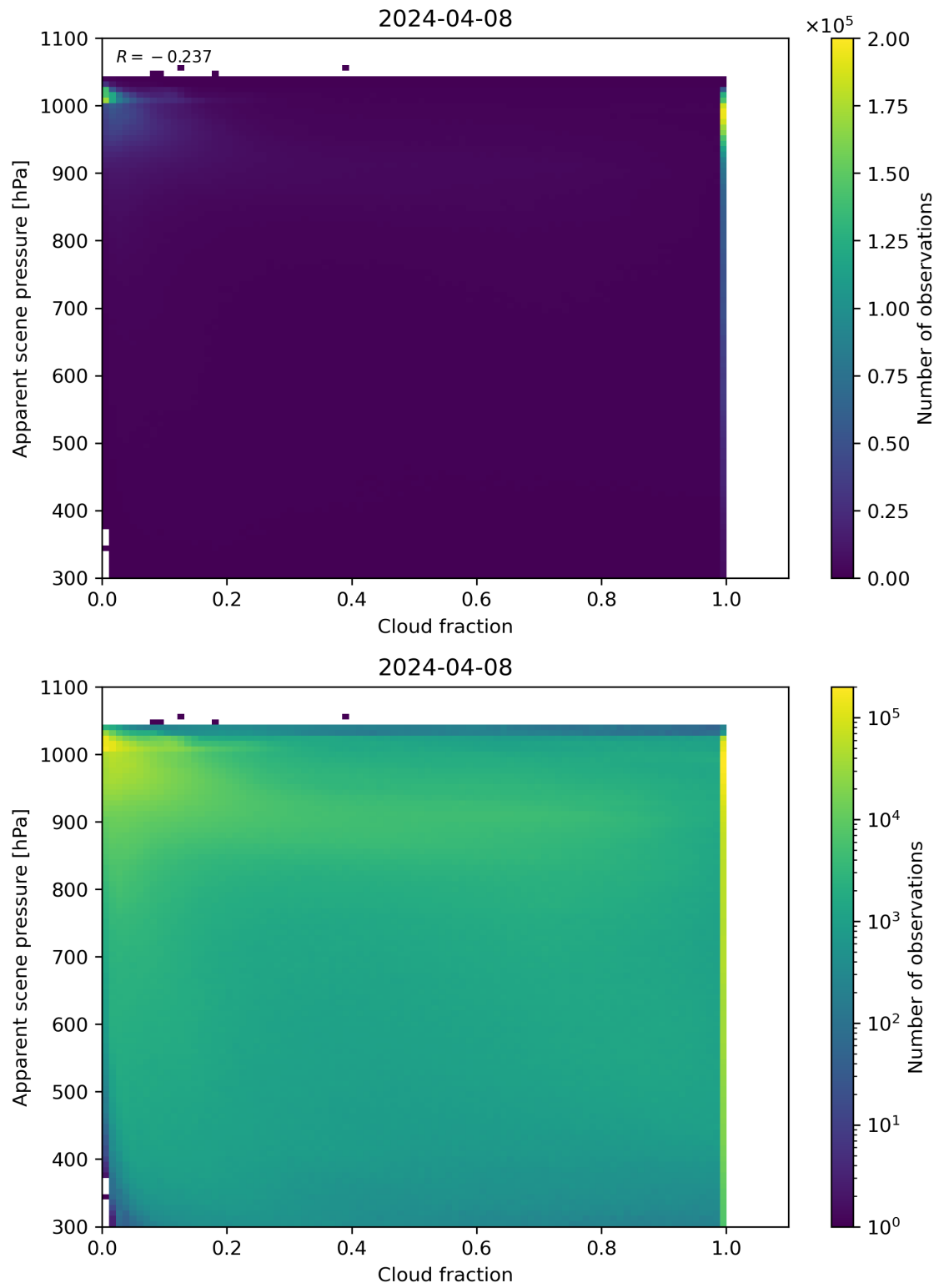
Figure 70: Scatter density plot of “Cloud fraction” against “Apparent scene pressure” for 2024-04-07 to 2024-04-09.
