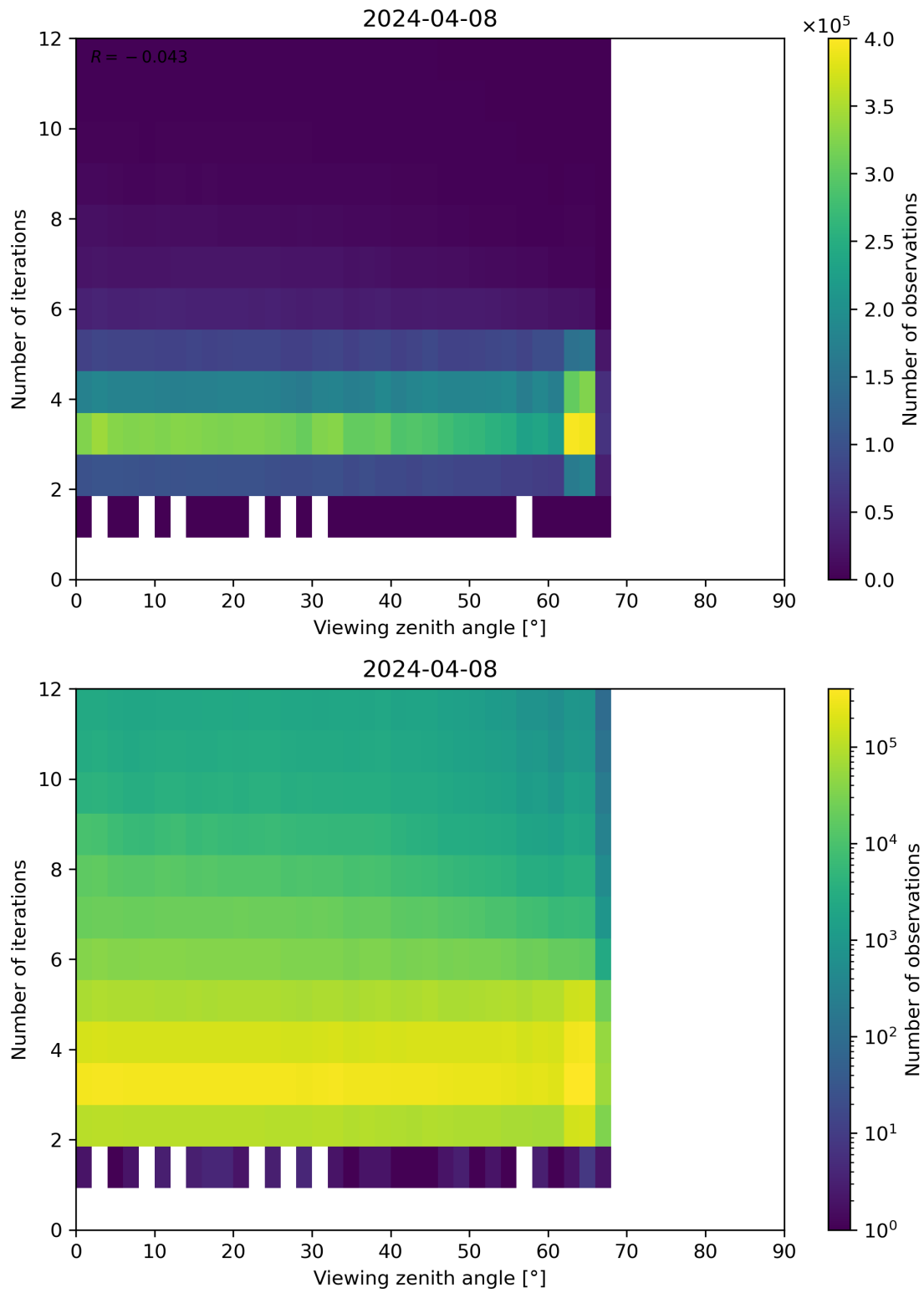
Figure 124: Scatter density plot of “Viewing zenith angle” against “Number of iterations” for 2024-04-07 to 2024-04-09.
