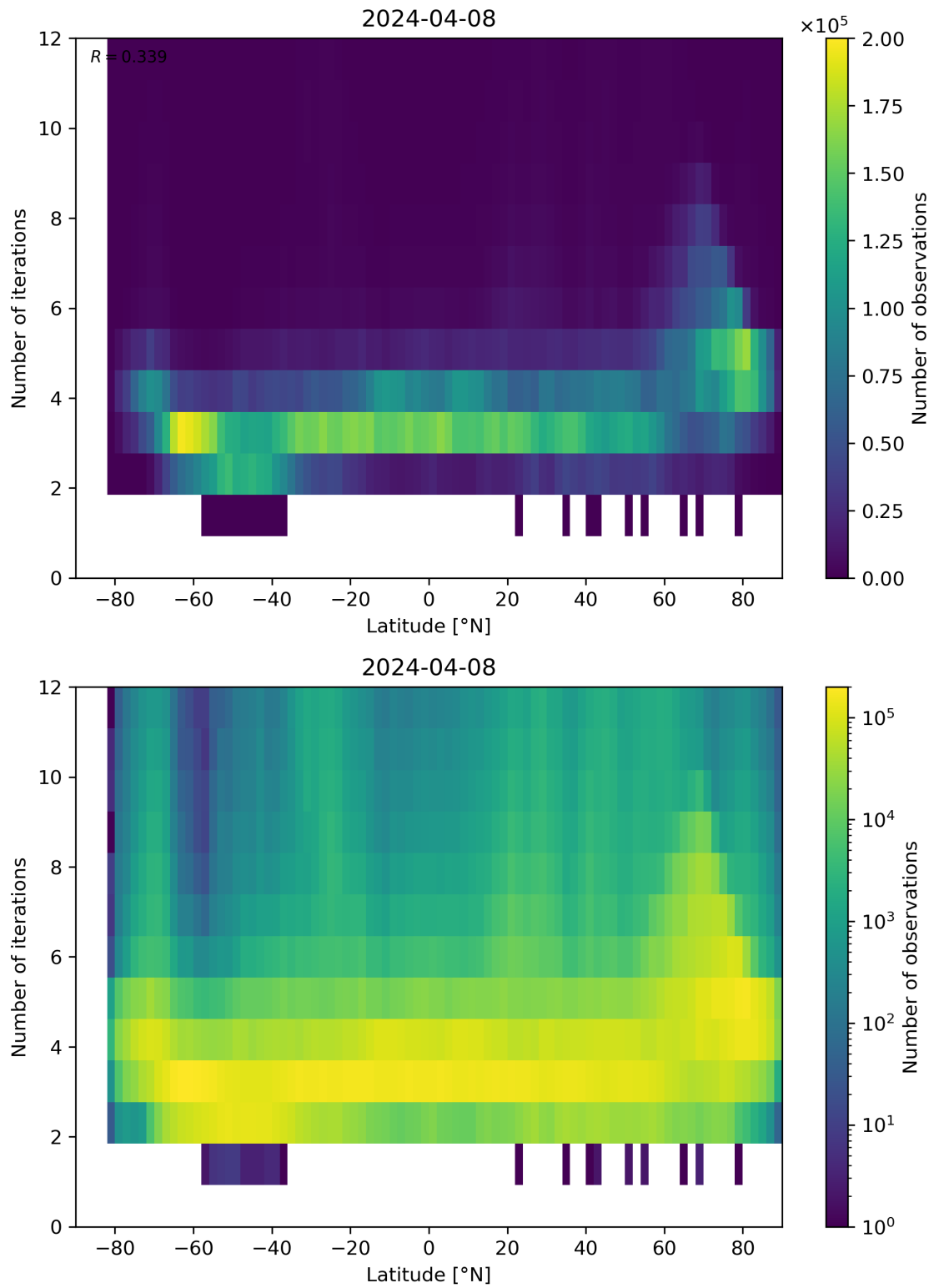
Figure 93: Scatter density plot of “Latitude” against “Number of iterations” for 2024-04-07 to 2024-04-09.
