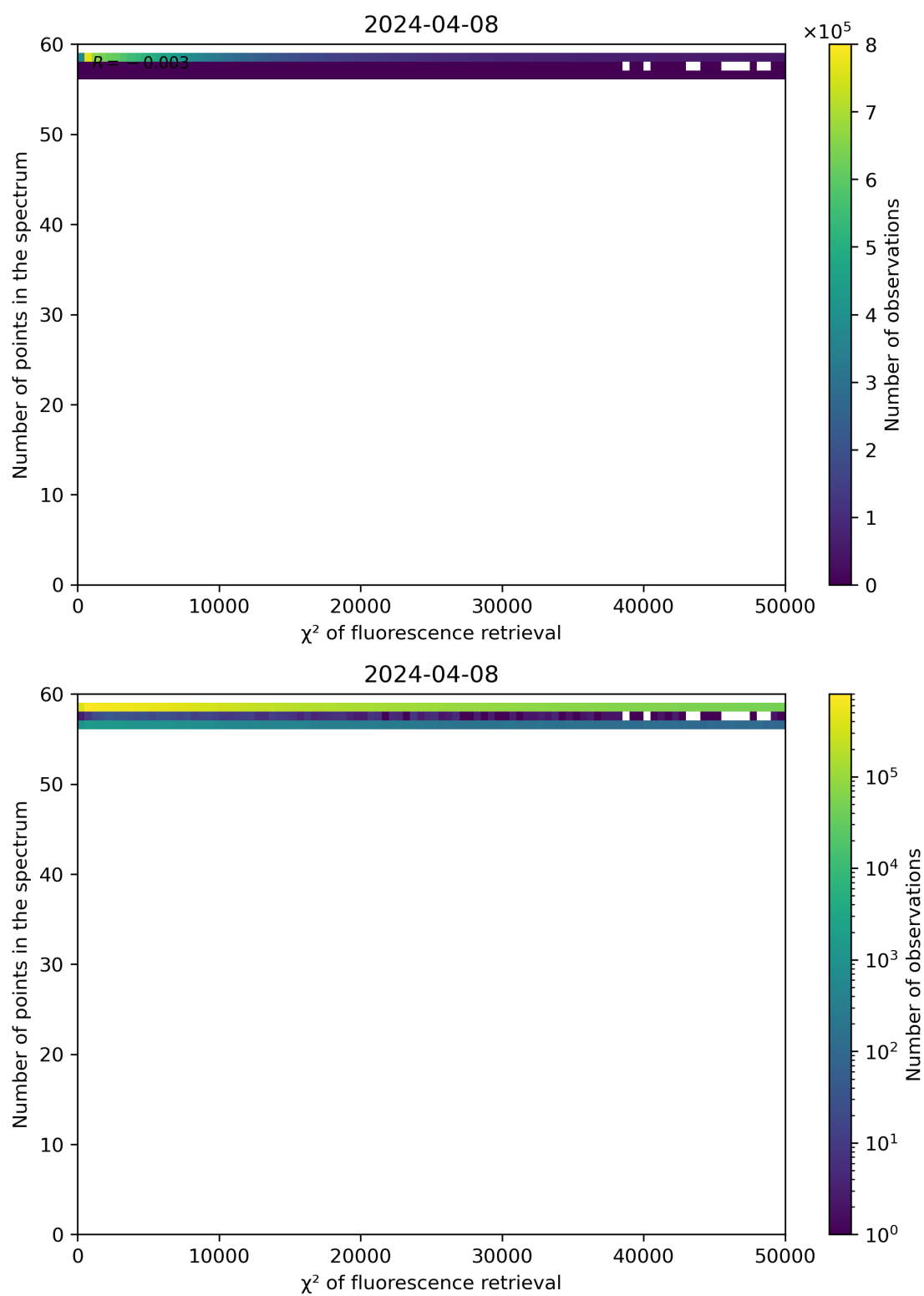
Figure 68: Scatter density plot of " \chi^2 of fluorescence retrieval" against "Number of points in the spectrum" for 2024-04-07 to 2024-04-09.
