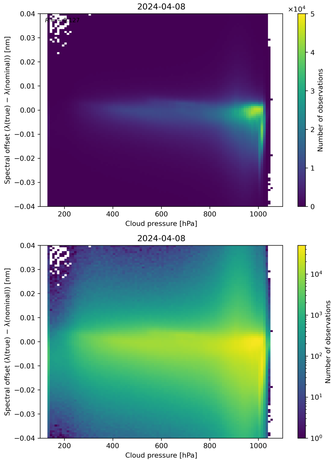
Figure 84: Scatter density plot of “Cloud pressure” against “Spectral offset ( \lambda(\text{true}) - \lambda(\text{nominal}) )” for 2024-04-07 to 2024-04-09.
