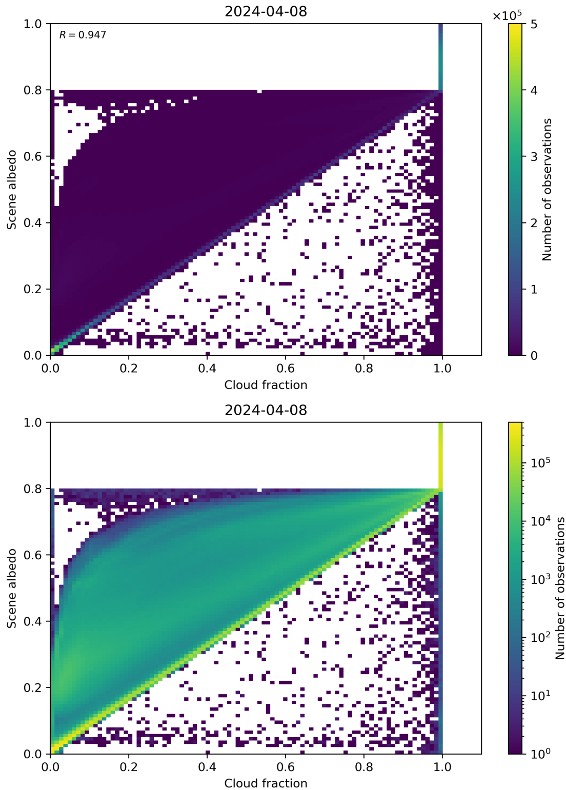
Figure 75: Scatter density plot of “Cloud fraction” against “Scene albedo” for 2024-04-07 to 2024-04-09.
