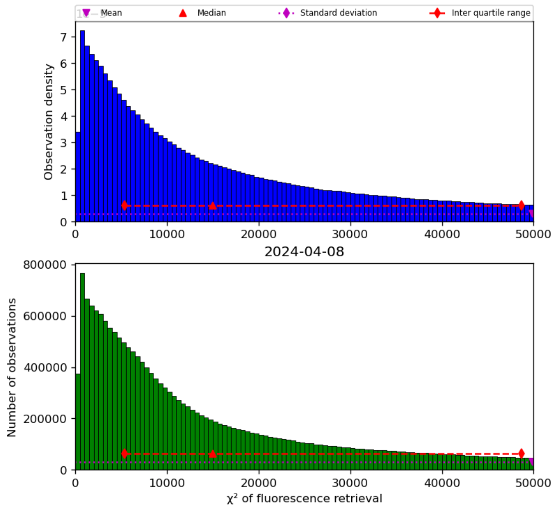
Figure 42: Histogram of “ \chi^2 of fluorescence retrieval” for 2024-04-07 to 2024-04-09
