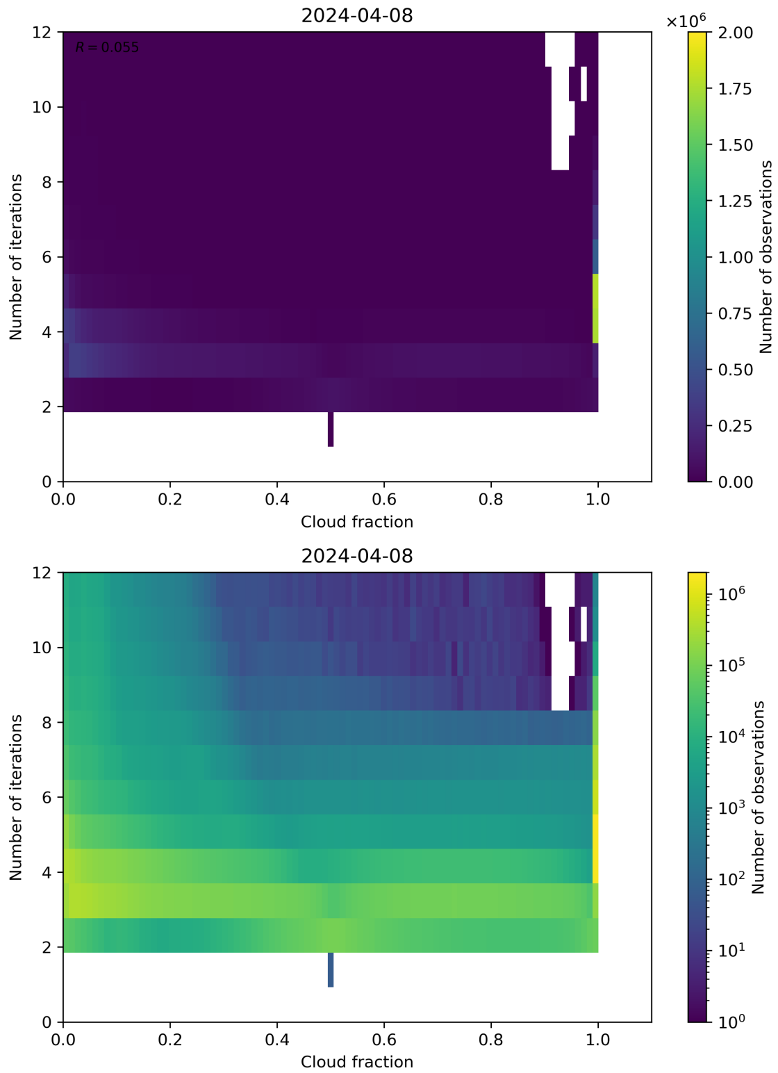
Figure 73: Scatter density plot of “Cloud fraction” against “Number of iterations” for 2024-04-07 to 2024-04-09.
