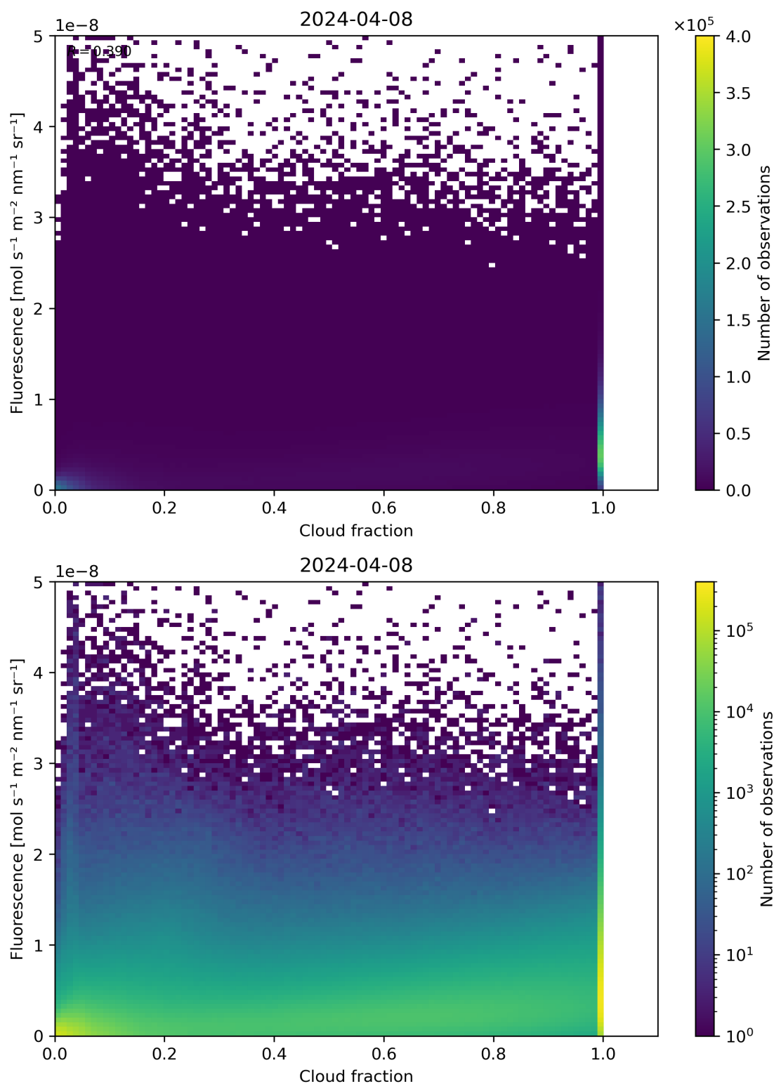
Figure 72: Scatter density plot of “Cloud fraction” against “Fluorescence” for 2024-04-07 to 2024-04-09.
