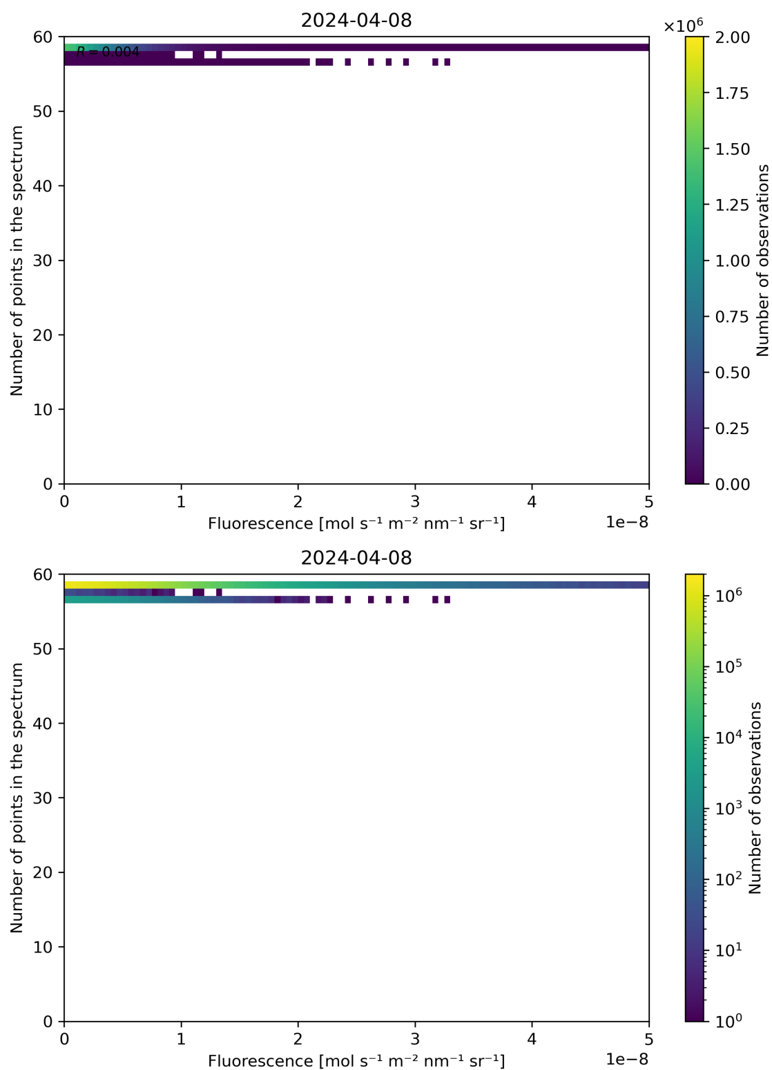
Figure 86: Scatter density plot of “Fluorescence” against “Number of points in the spectrum” for 2024-04-07 to 2024-04-09.
