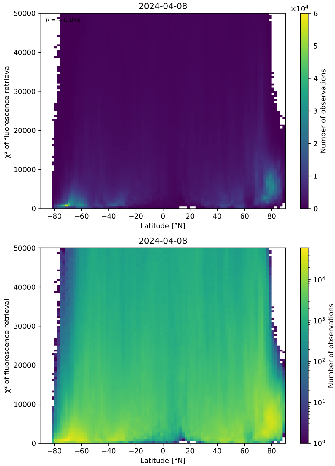
Figure 89: Scatter density plot of “Latitude” against “ \chi^2 of fluorescence retrieval” for 2024-04-07 to 2024-04-09.
