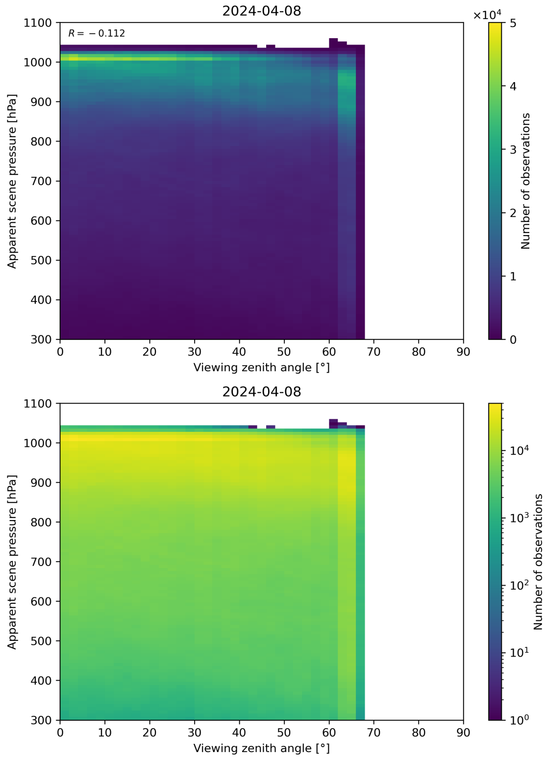
Figure 118: Scatter density plot of “Viewing zenith angle” against “Apparent scene pressure” for 2024-04-07 to 2024-04-09.
