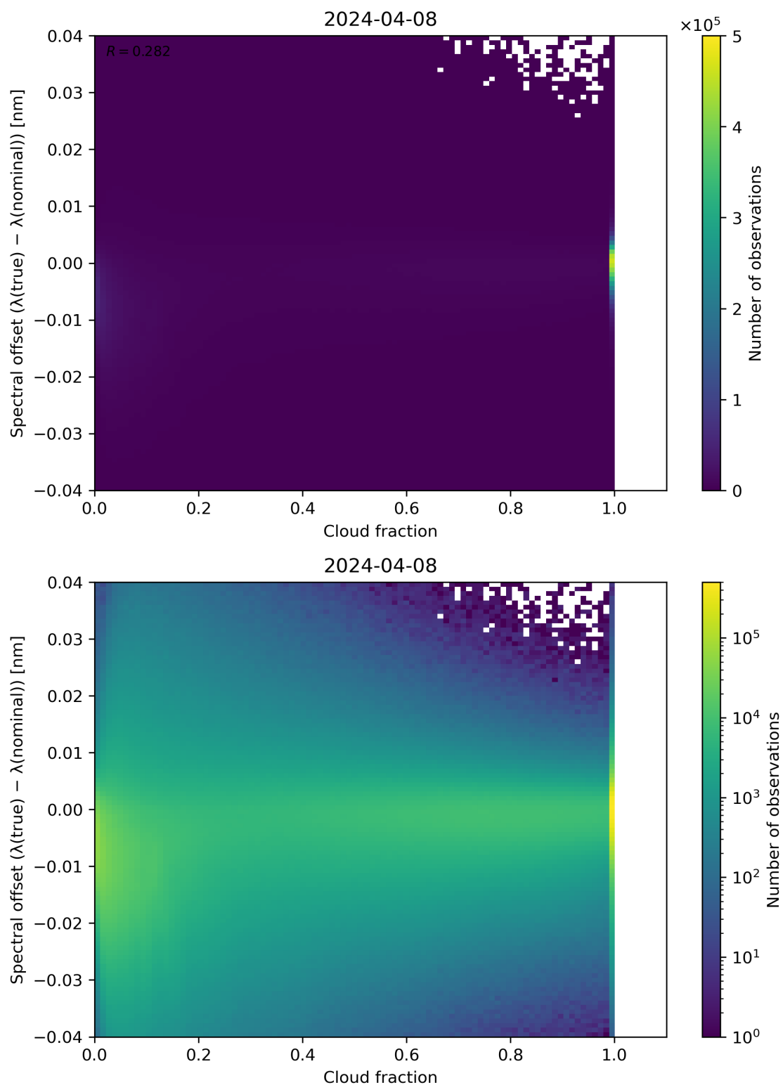
Figure 76: Scatter density plot of “Cloud fraction” against “Spectral offset ( \lambda(\text{true}) - \lambda(\text{nominal}) )” for 2024-04-07 to 2024-04-09.
