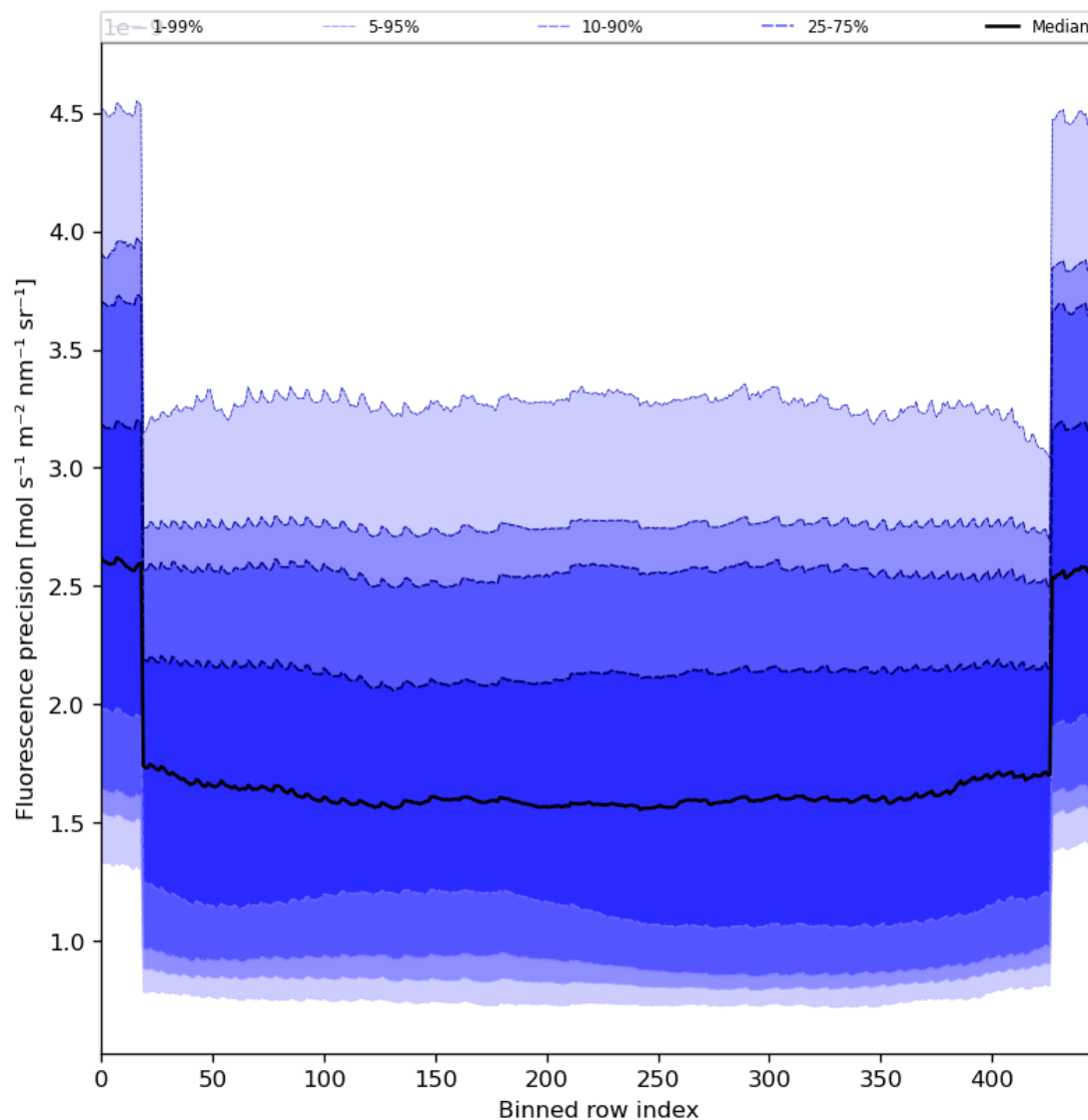
Figure 58: Along track statistics of “Fluorescence precision” for 2024-04-07 to 2024-04-09
