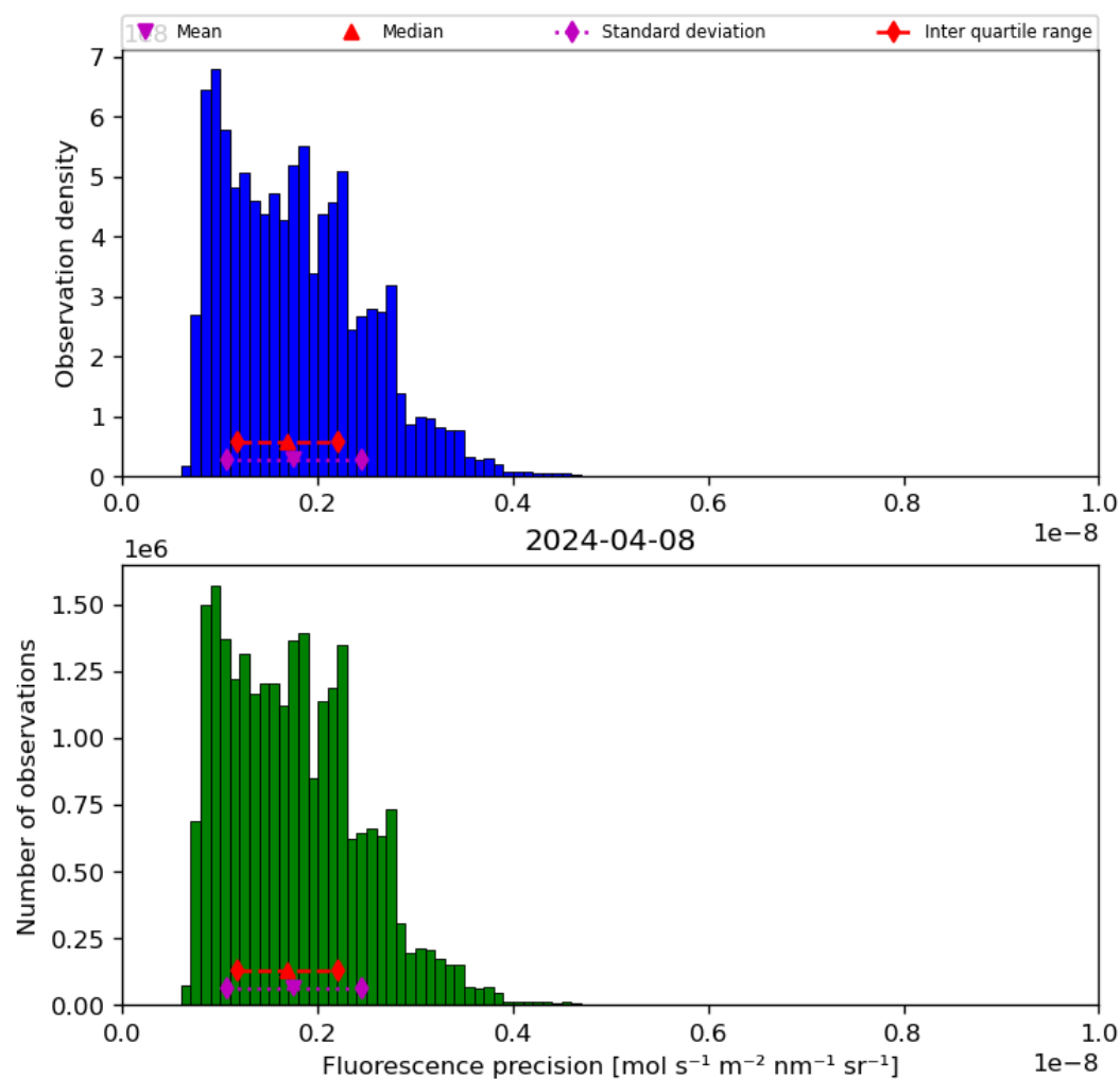
Figure 41: Histogram of “Fluorescence precision” for 2024-04-07 to 2024-04-09
