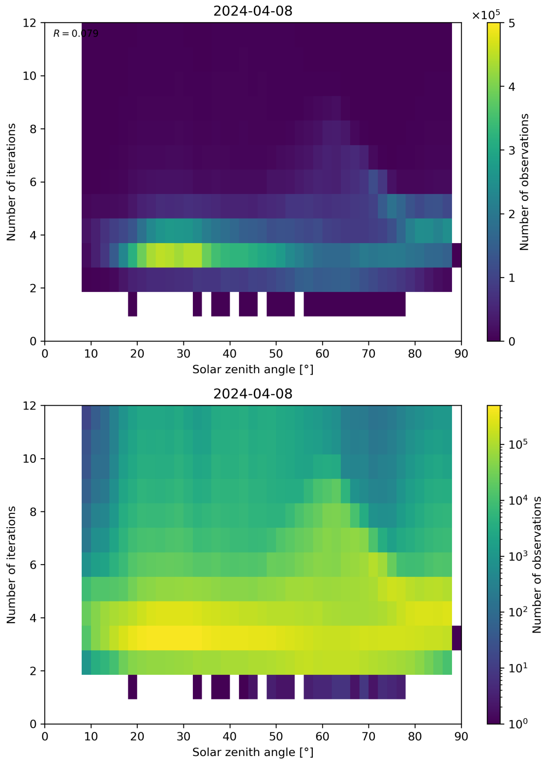
Figure 114: Scatter density plot of “Solar zenith angle” against “Number of iterations” for 2024-04-07 to 2024-04-09.
