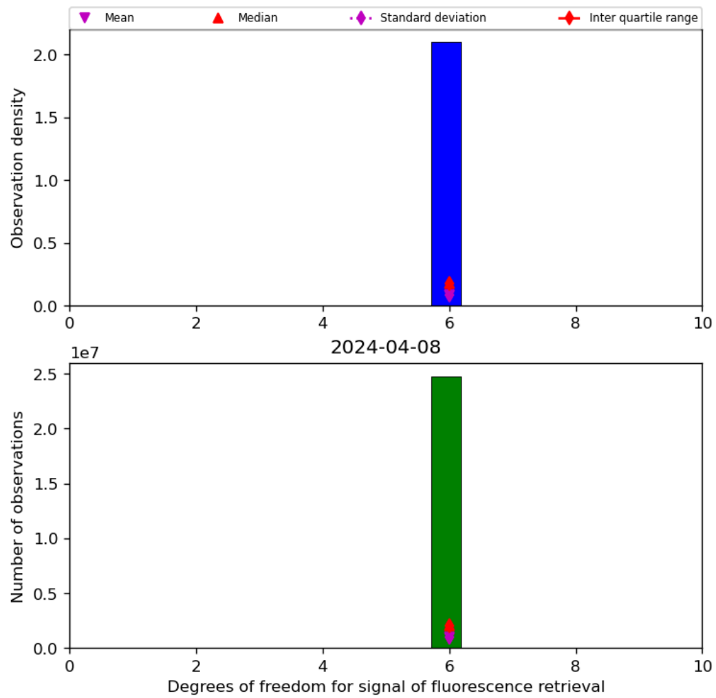
Figure 43: Histogram of “Degrees of freedom for signal of fluorescence retrieval” for 2024-04-07 to 2024-04-09
