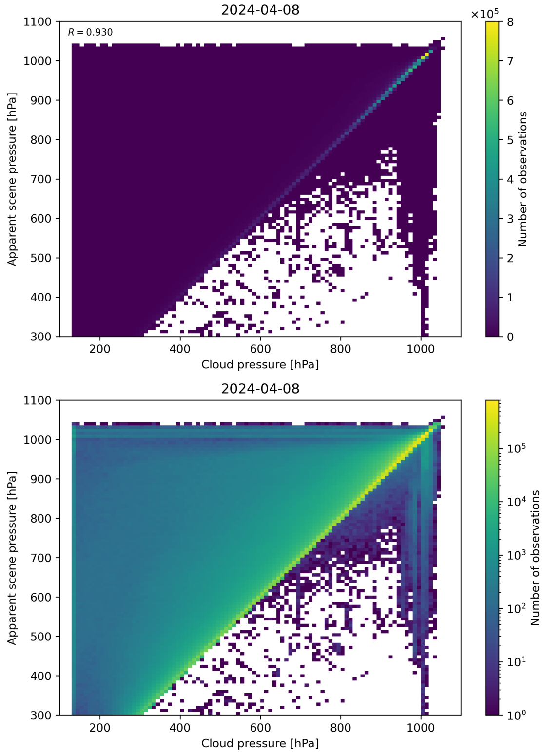
Figure 77: Scatter density plot of “Cloud pressure” against “Apparent scene pressure” for 2024-04-07 to 2024-04-09.
