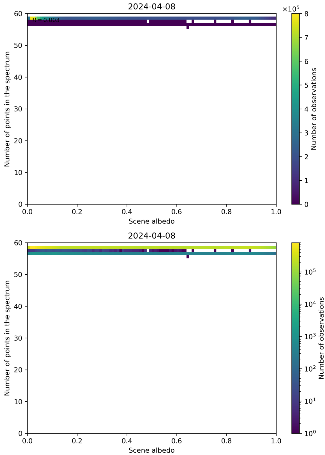
Figure 106: Scatter density plot of “Scene albedo” against “Number of points in the spectrum” for 2024-04-07 to 2024-04-09.
