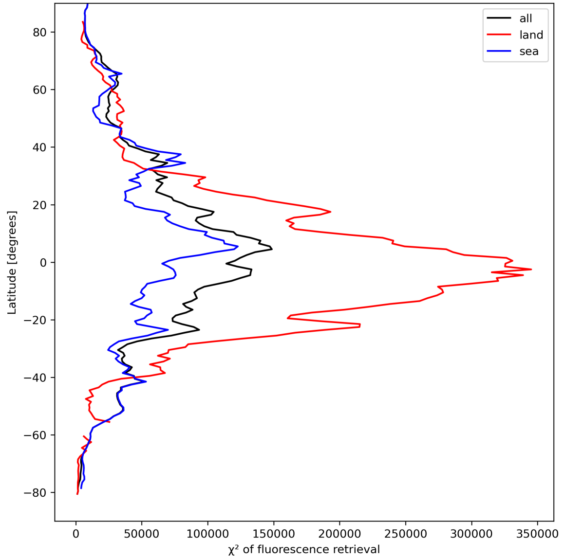
Figure 25: Zonal average of “ \chi^2 of fluorescence retrieval” for 2024-04-07 to 2024-04-09.
