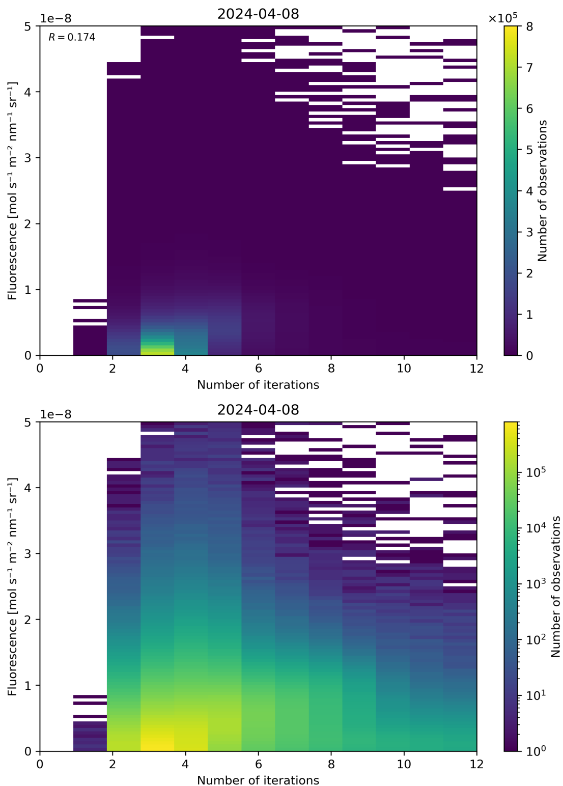
Figure 98: Scatter density plot of “Number of iterations” against “Fluorescence” for 2024-04-07 to 2024-04-09.
