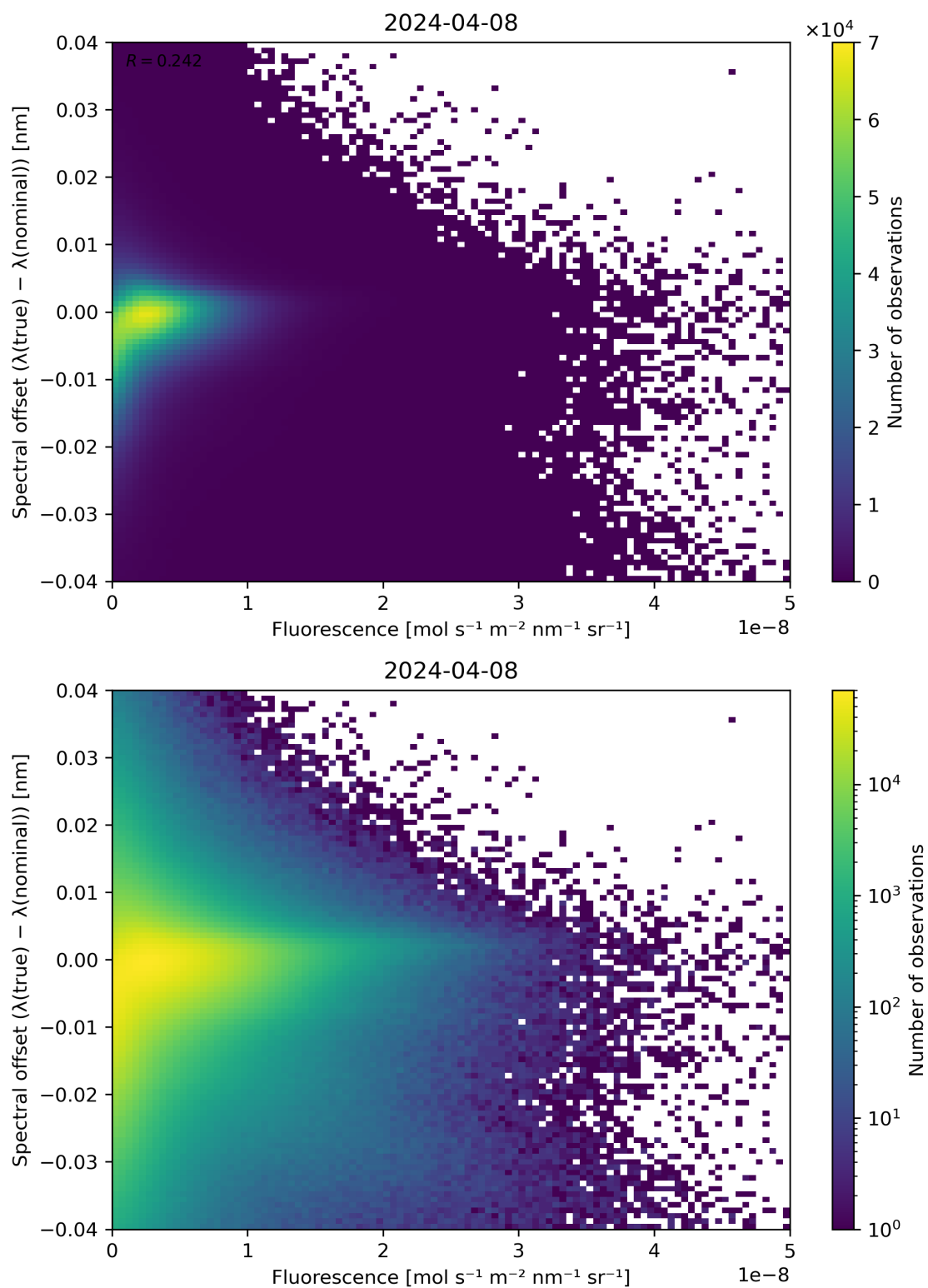
Figure 87: Scatter density plot of “Fluorescence” against “Spectral offset ( \lambda(\text{true}) - \lambda(\text{nominal}) )” for 2024-04-07 to 2024-04-09.
