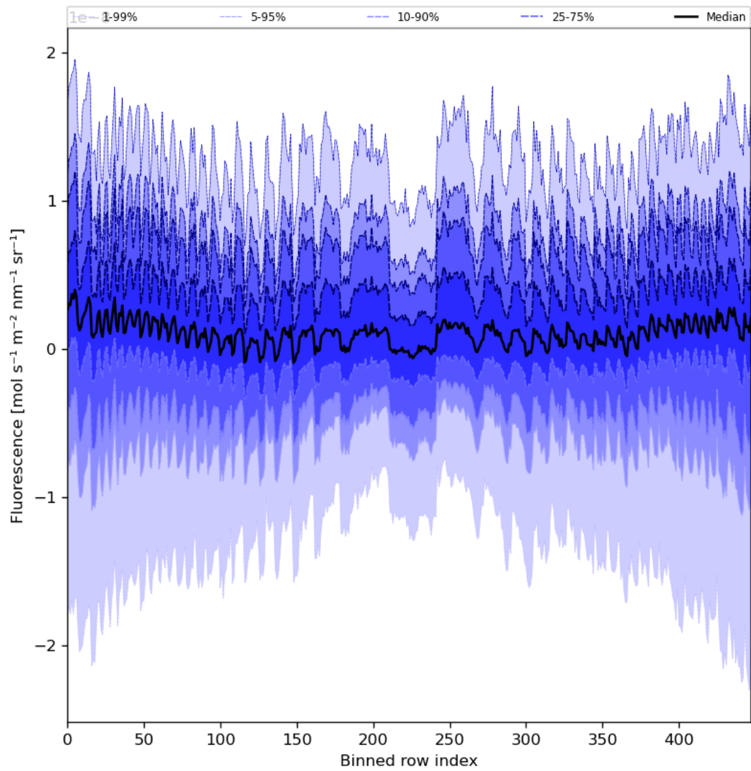
Figure 57: Along track statistics of “Fluorescence” for 2024-04-07 to 2024-04-09
