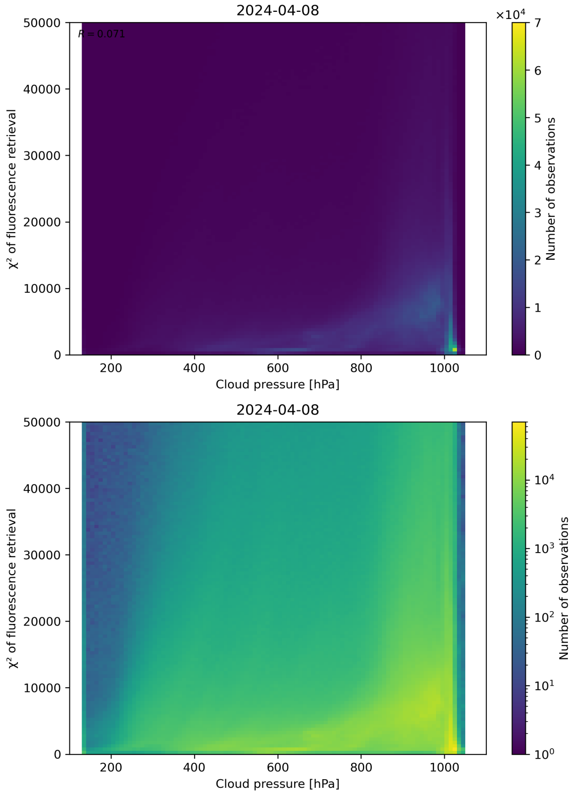
Figure 78: Scatter density plot of “Cloud pressure” against “ \chi^2 of fluorescence retrieval” for 2024-04-07 to 2024-04-09.
