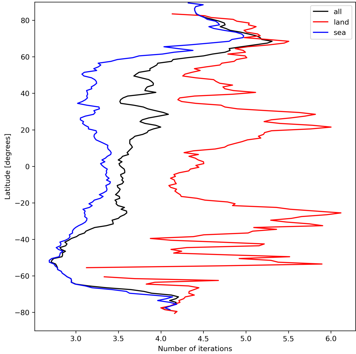
Figure 22: Zonal average of “Number of iterations” for 2024-04-07 to 2024-04-09.
