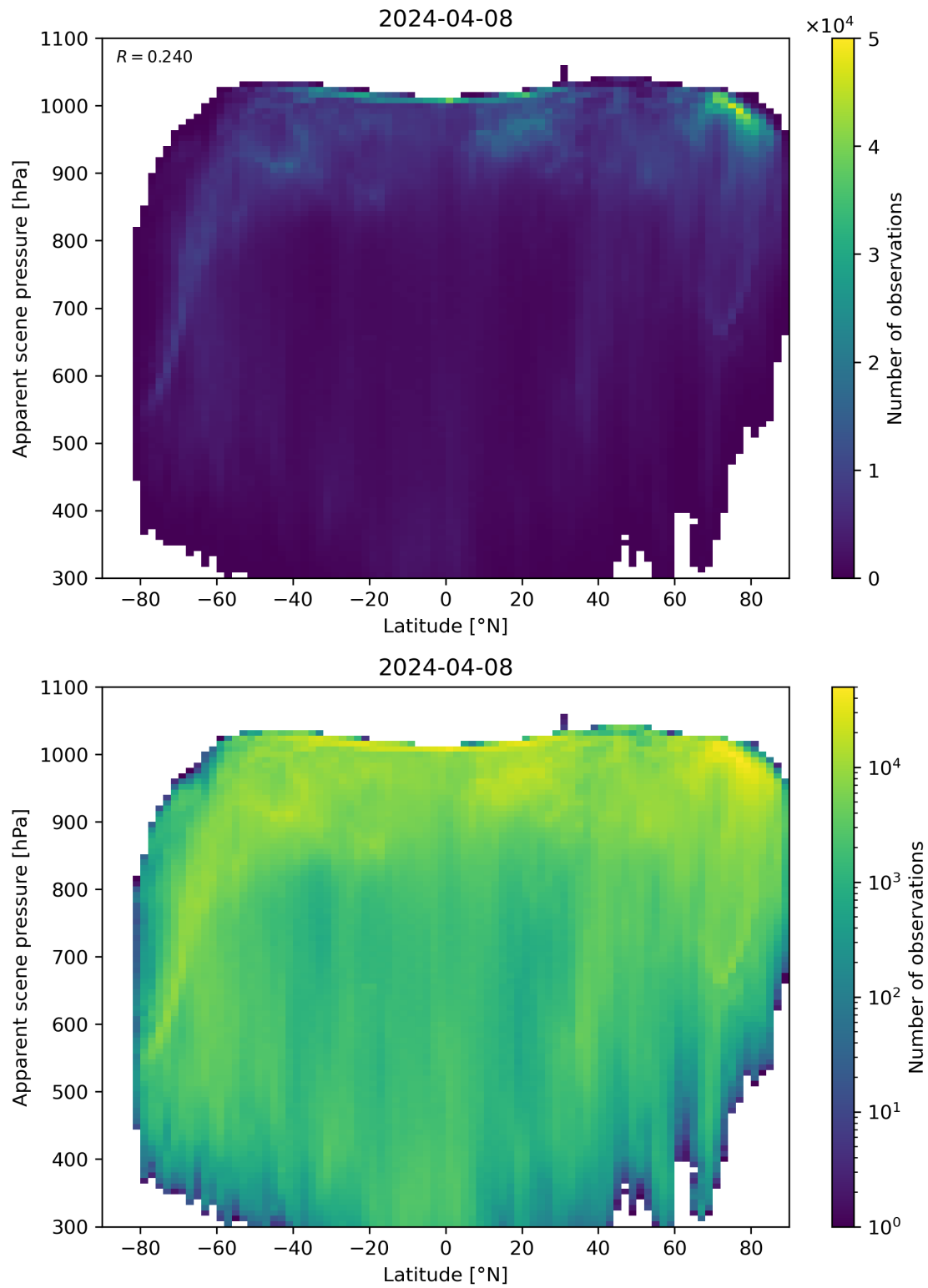
Figure 88: Scatter density plot of “Latitude” against “Apparent scene pressure” for 2024-04-07 to 2024-04-09.
