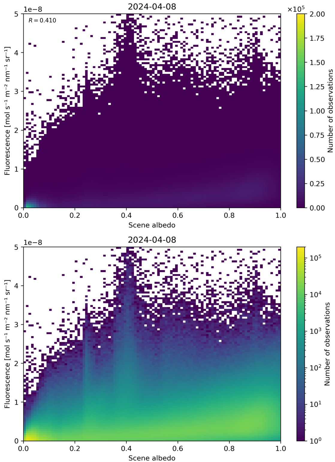
Figure 104: Scatter density plot of “Scene albedo” against “Fluorescence” for 2024-04-07 to 2024-04-09.
