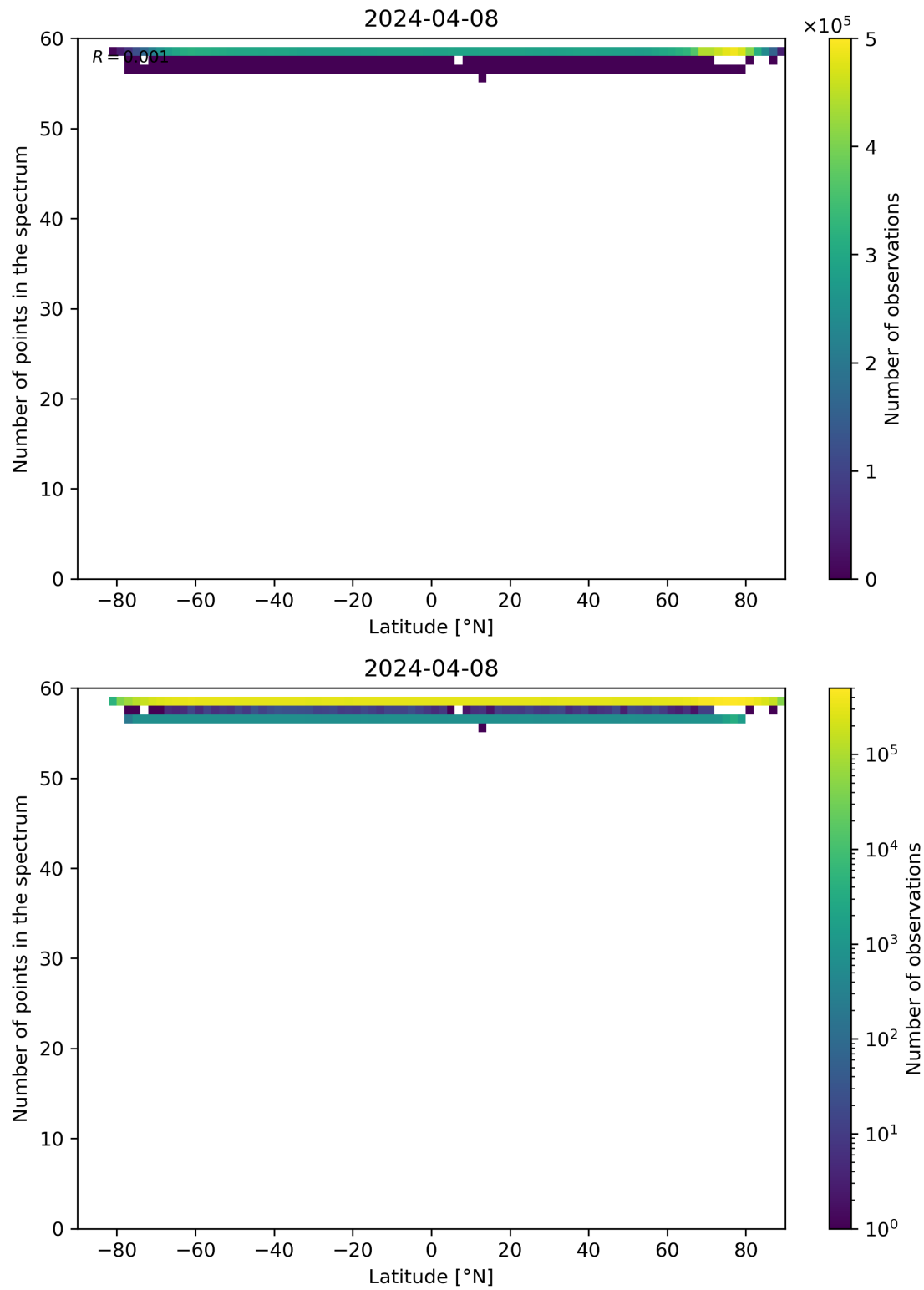
Figure 94: Scatter density plot of “Latitude” against “Number of points in the spectrum” for 2024-04-07 to 2024-04-09.
