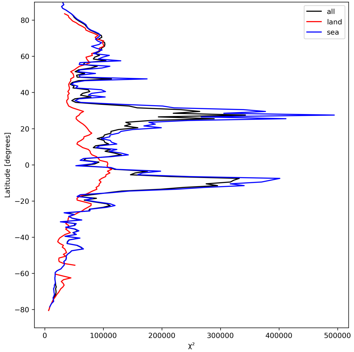
Figure 21: Zonal average of “ \chi^2 ” for 2024-04-07 to 2024-04-09.
