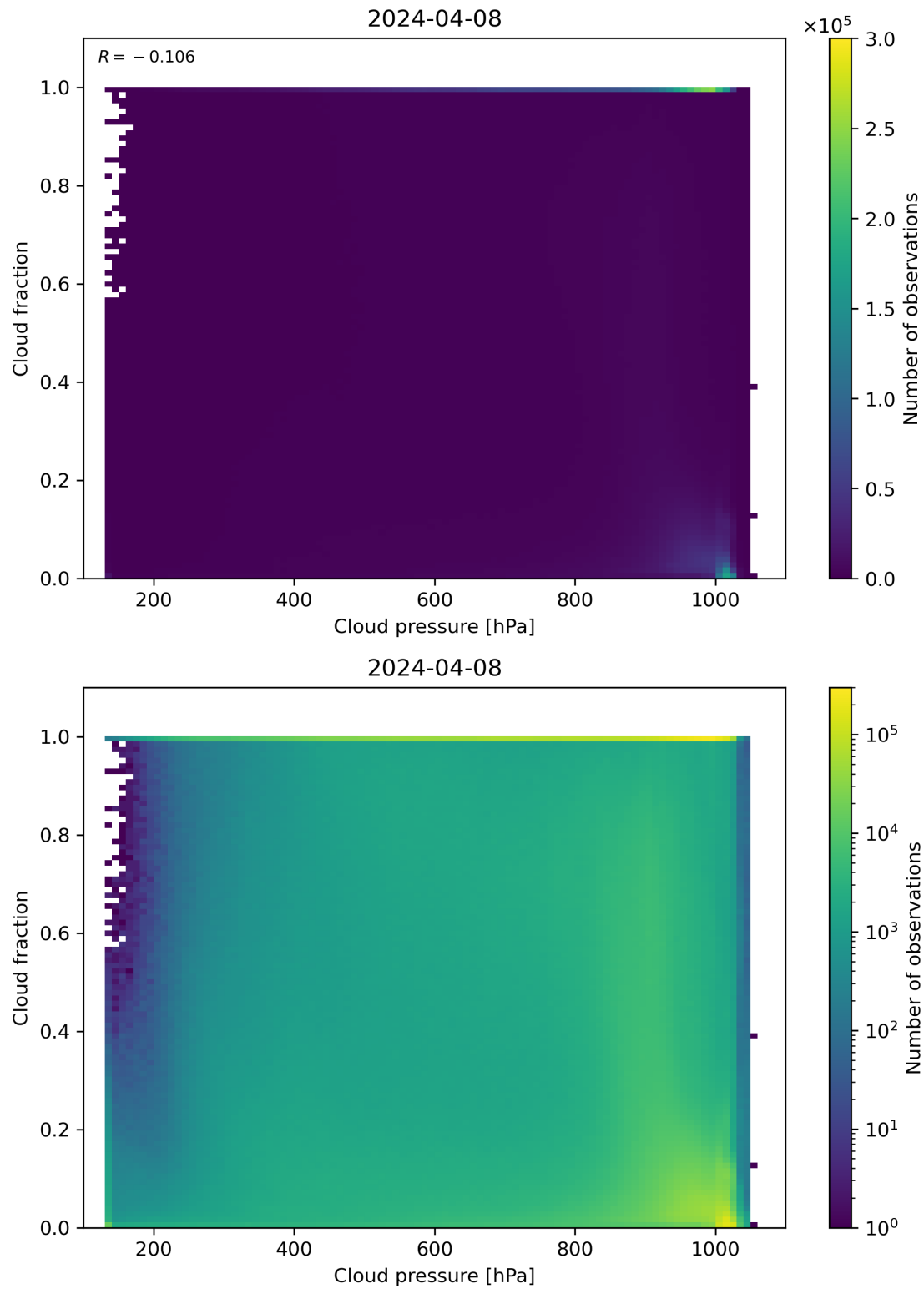
Figure 79: Scatter density plot of “Cloud pressure” against “Cloud fraction” for 2024-04-07 to 2024-04-09.
