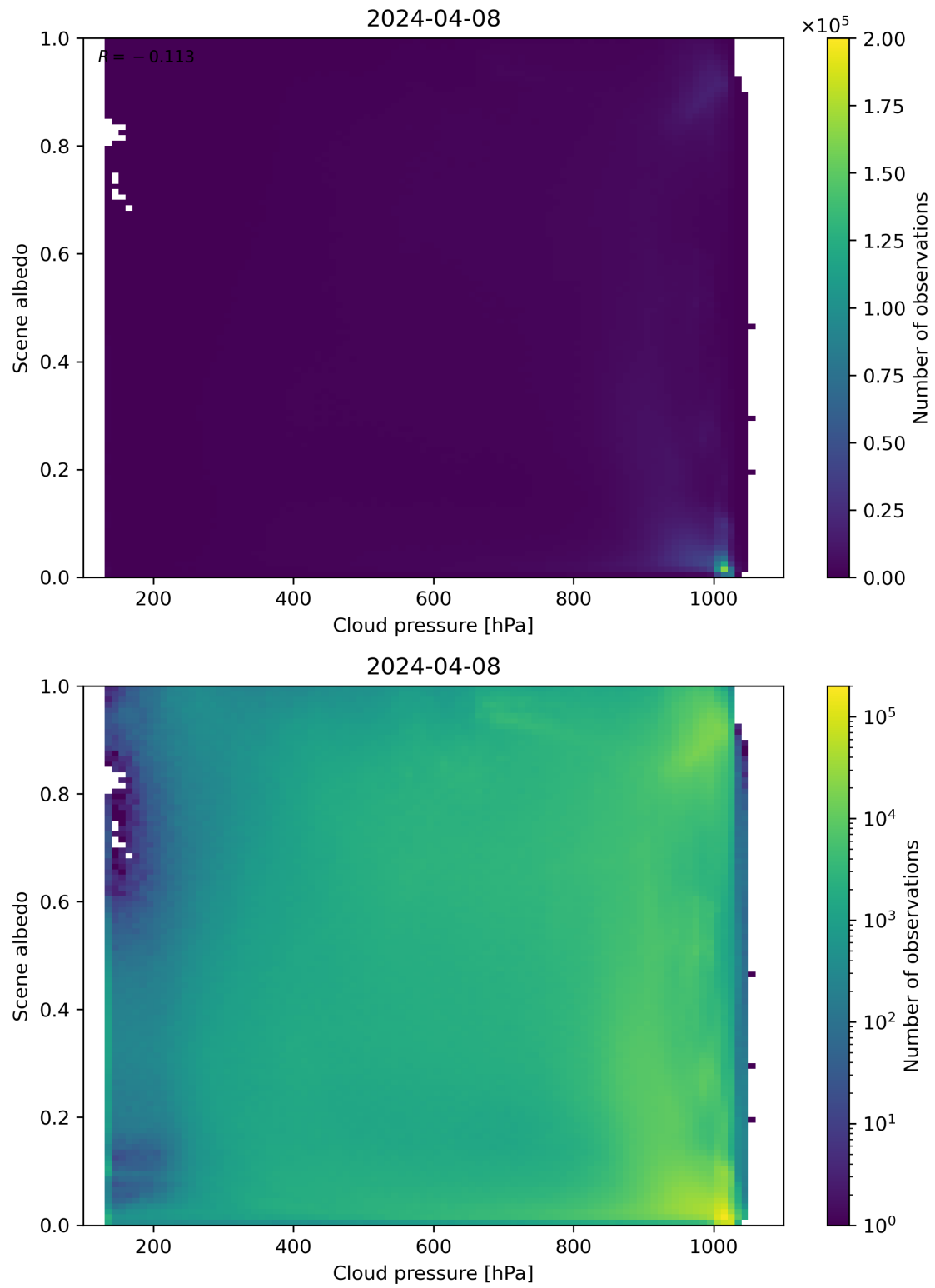
Figure 83: Scatter density plot of “Cloud pressure” against “Scene albedo” for 2024-04-07 to 2024-04-09.
