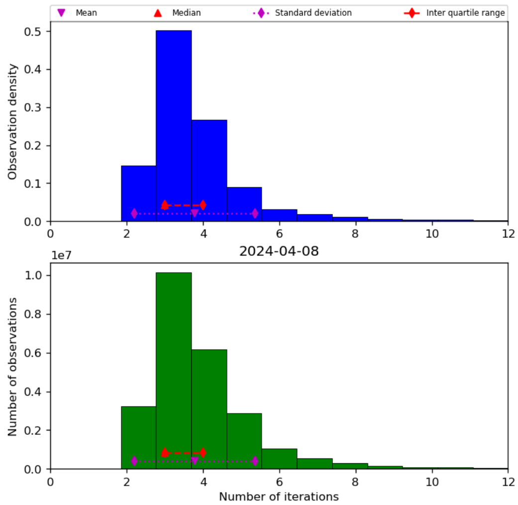
Figure 39: Histogram of “Number of iterations” for 2024-04-07 to 2024-04-09
