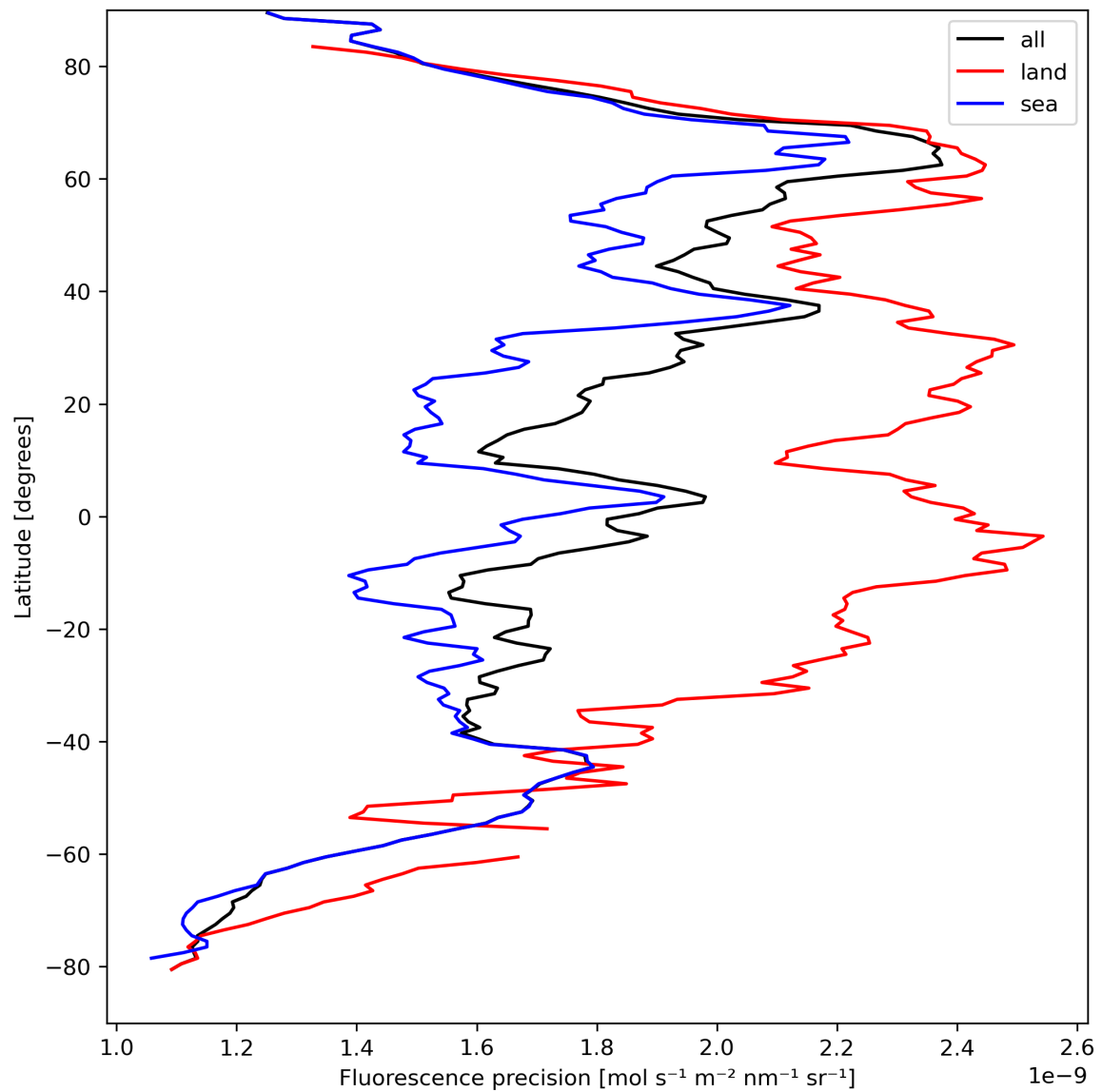
Figure 24: Zonal average of “Fluorescence precision” for 2024-04-07 to 2024-04-09.
