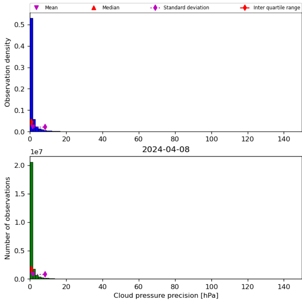
Figure 31: Histogram of “Cloud pressure precision” for 2024-04-07 to 2024-04-09
