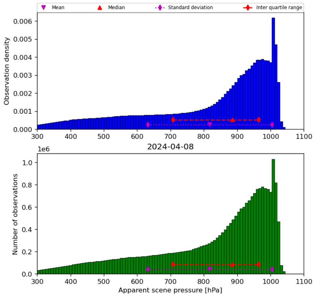
Figure 36: Histogram of “Apparent scene pressure” for 2024-04-07 to 2024-04-09
