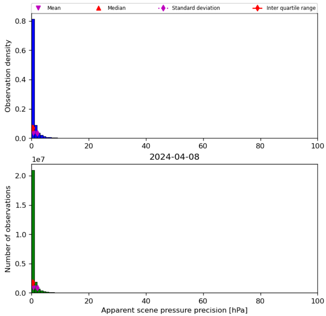
Figure 37: Histogram of “Apparent scene pressure precision” for 2024-04-07 to 2024-04-09
