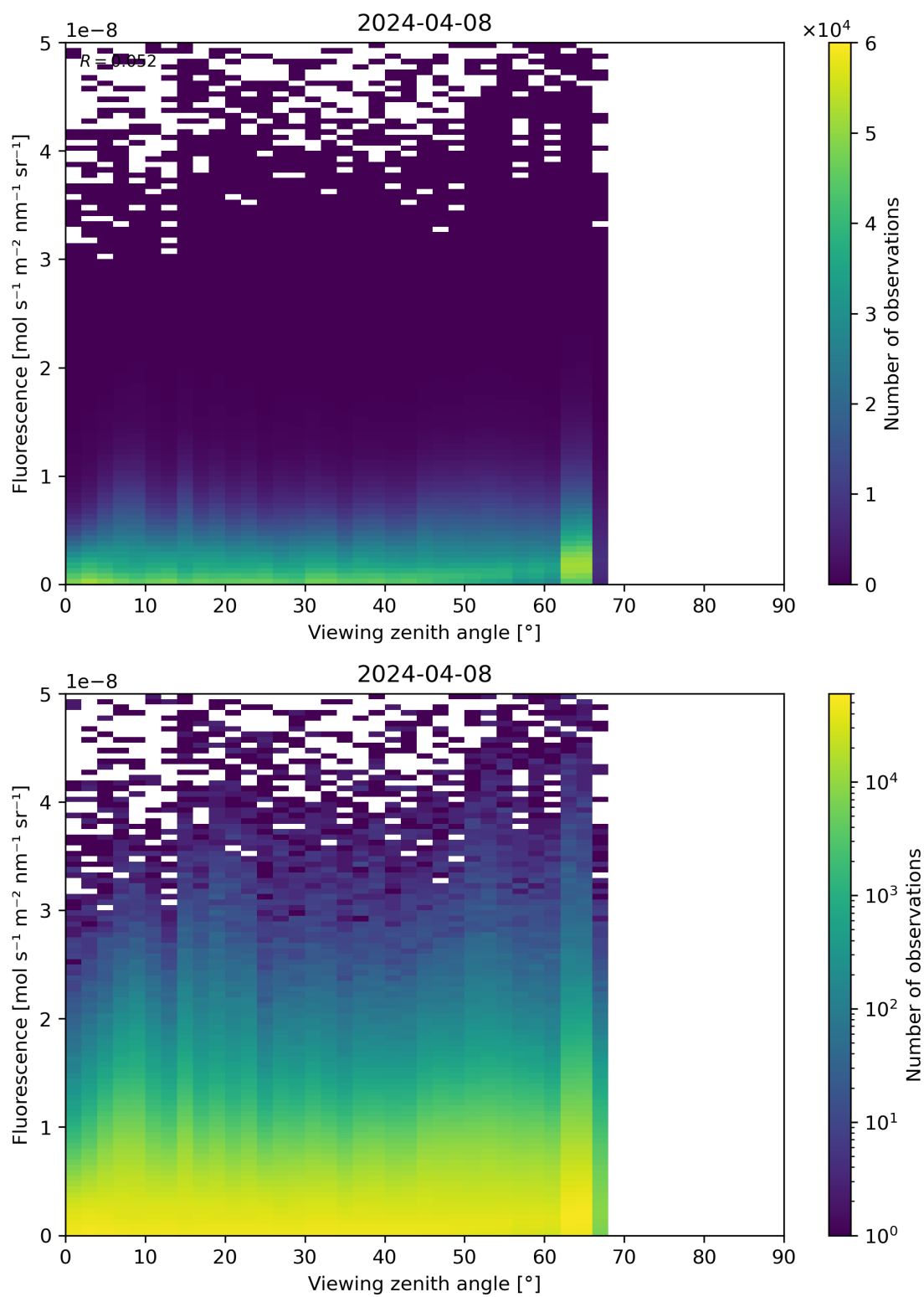
Figure 122: Scatter density plot of “Viewing zenith angle” against “Fluorescence” for 2024-04-07 to 2024-04-09.
