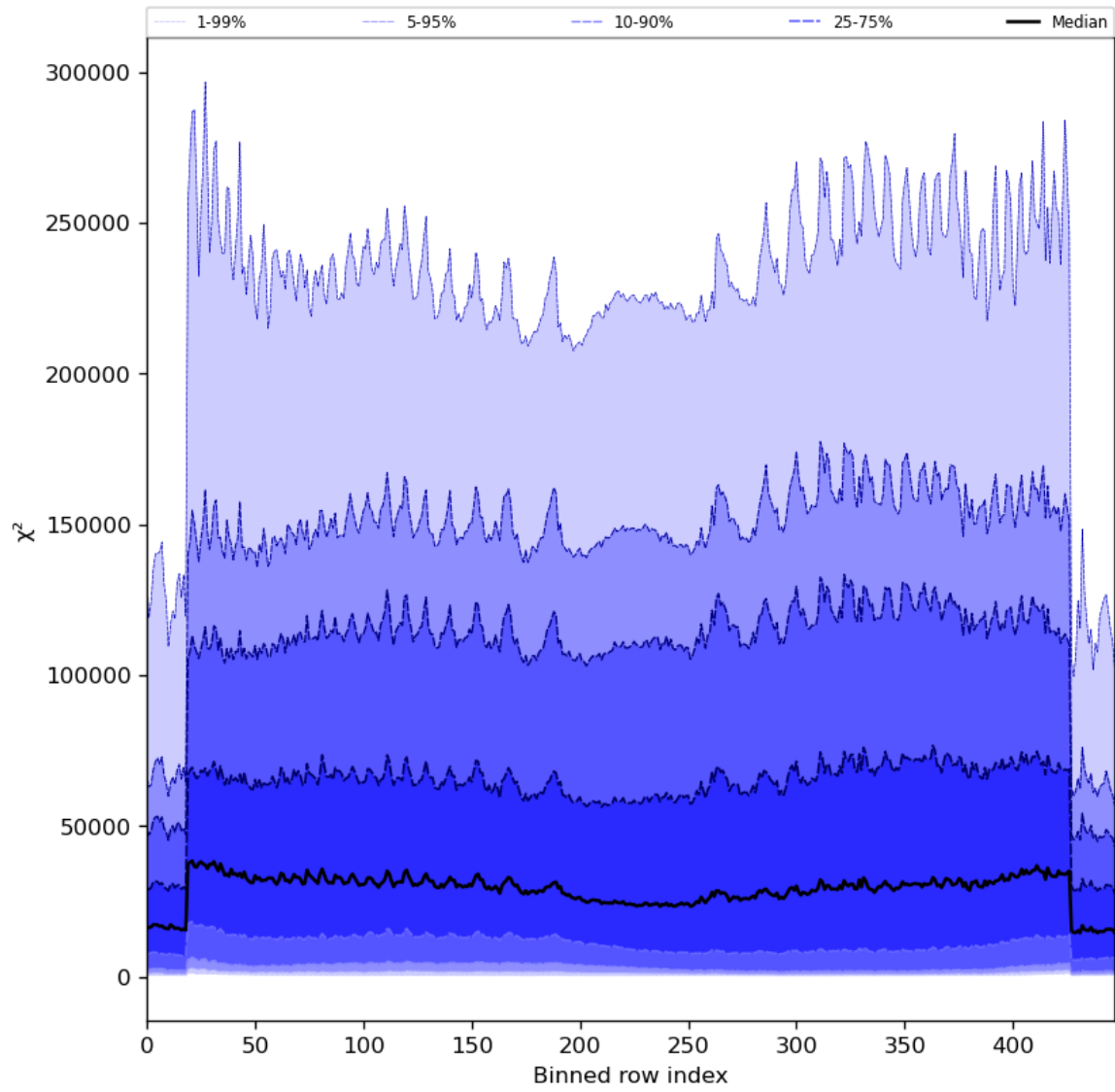
Figure 55: Along track statistics of “ \chi^2 ” for 2024-04-07 to 2024-04-09
