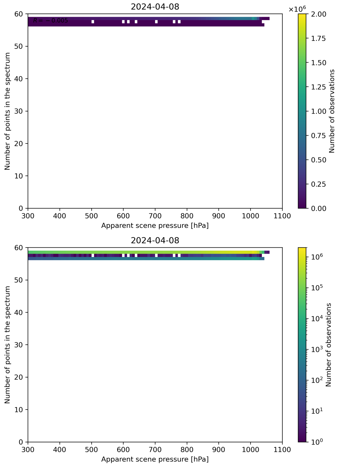
Figure 66: Scatter density plot of “Apparent scene pressure” against “Number of points in the spectrum” for 2024-04-07 to 2024-04-09.
