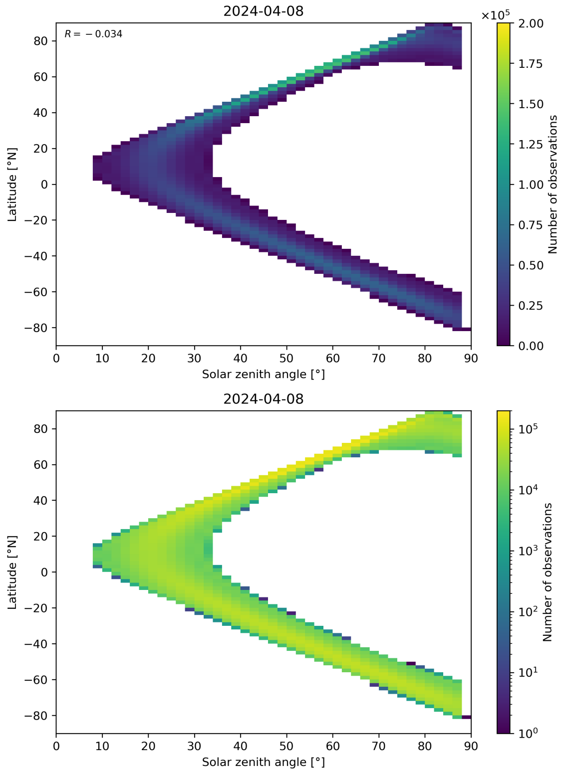
Figure 113: Scatter density plot of “Solar zenith angle” against “Latitude” for 2024-04-07 to 2024-04-09.
