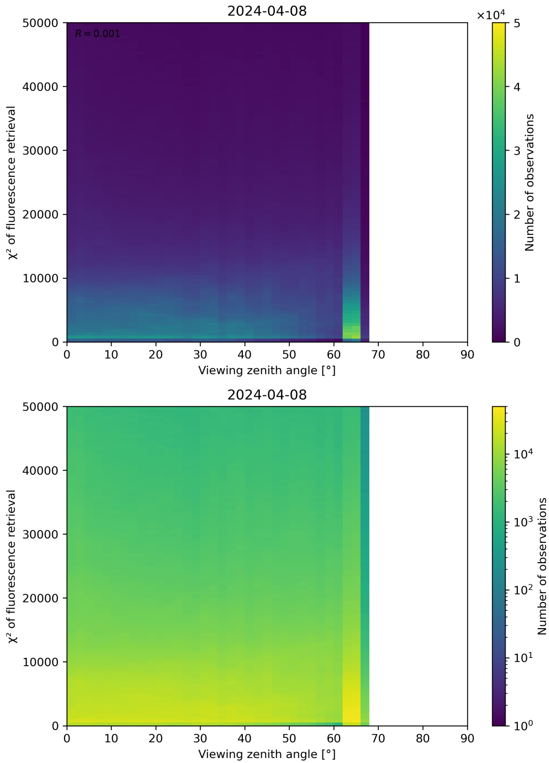
Figure 119: Scatter density plot of “Viewing zenith angle” against “ \chi^2 of fluorescence retrieval” for 2024-04-07 to 2024-04-09.
