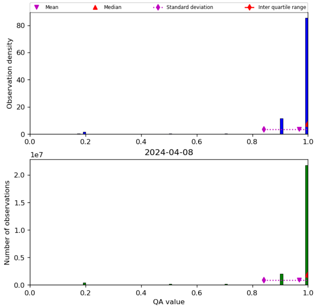
Figure 29: Histogram of “QA value” for 2024-04-07 to 2024-04-09
