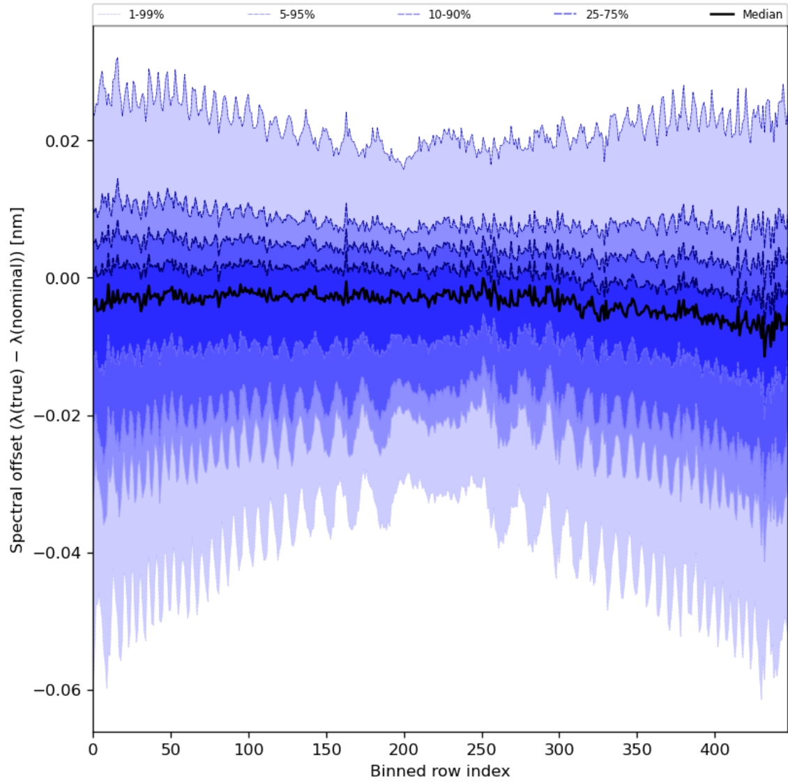
Figure 62: Along track statistics of “Spectral offset ( \lambda(\text{true}) - \lambda(\text{nominal}) )” for 2024-04-07 to 2024-04-09
