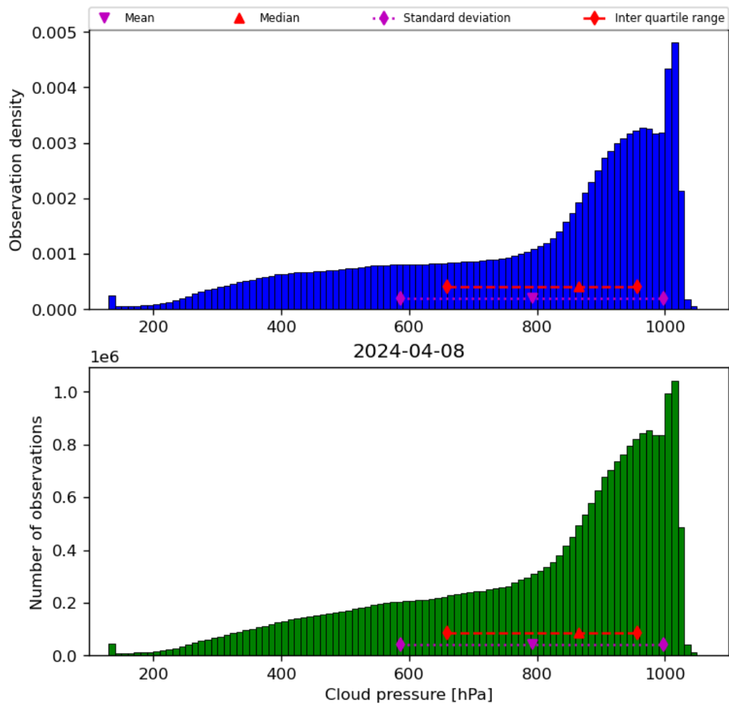
Figure 30: Histogram of “Cloud pressure” for 2024-04-07 to 2024-04-09
