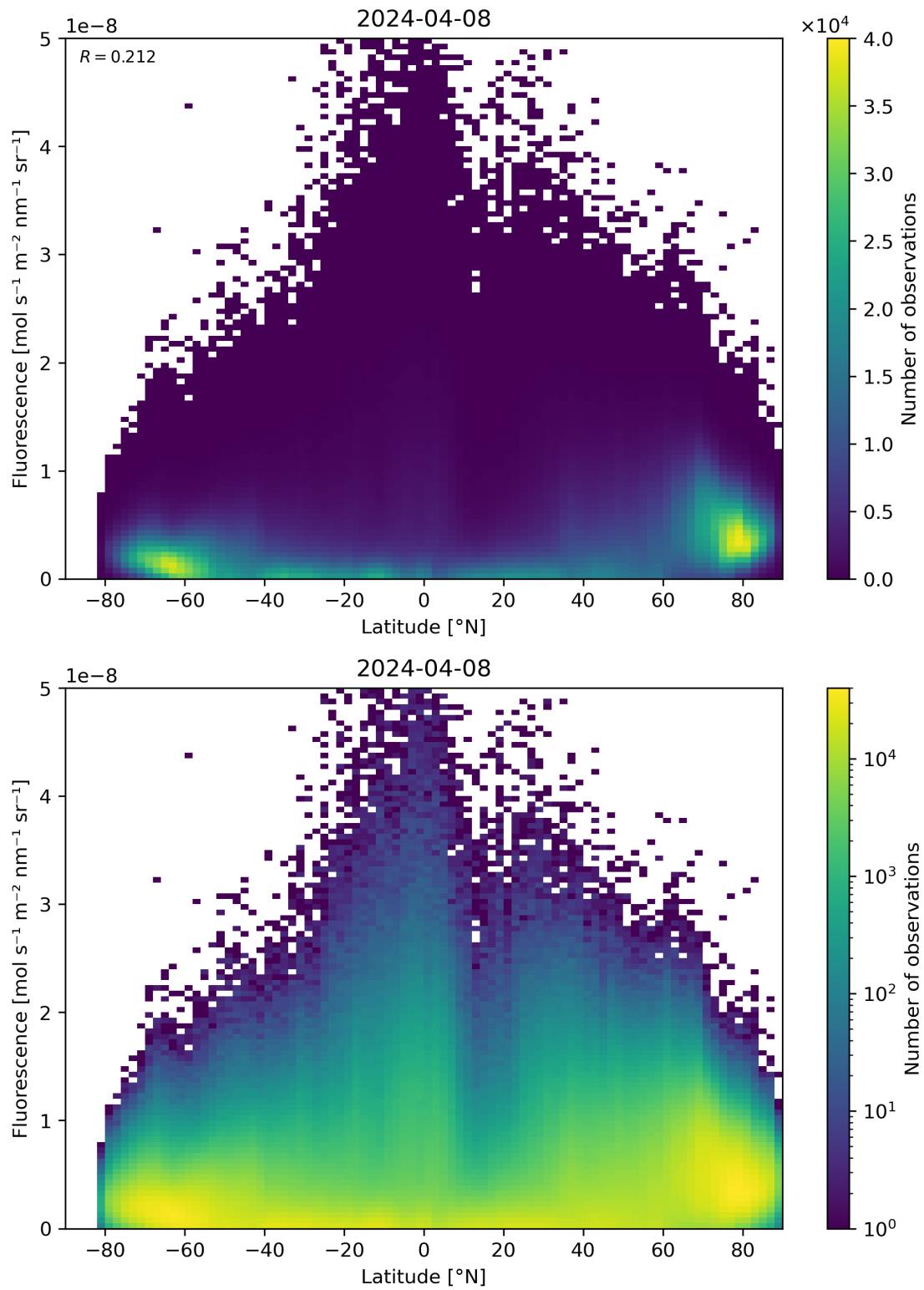
Figure 92: Scatter density plot of “Latitude” against “Fluorescence” for 2024-04-07 to 2024-04-09.
