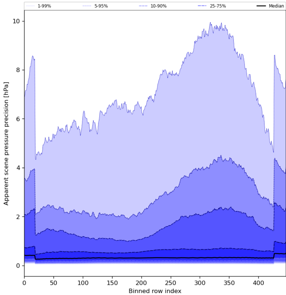
Figure 54: Along track statistics of “Apparent scene pressure precision” for 2024-04-07 to 2024-04-09
