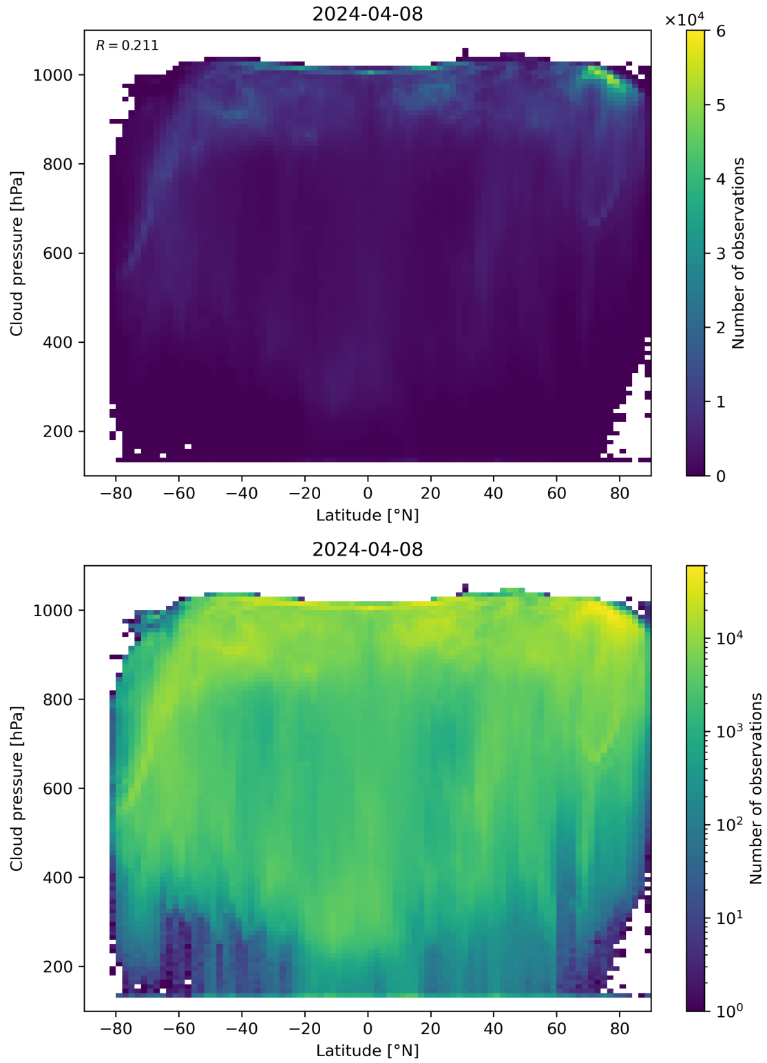
Figure 91: Scatter density plot of “Latitude” against “Cloud pressure” for 2024-04-07 to 2024-04-09.
