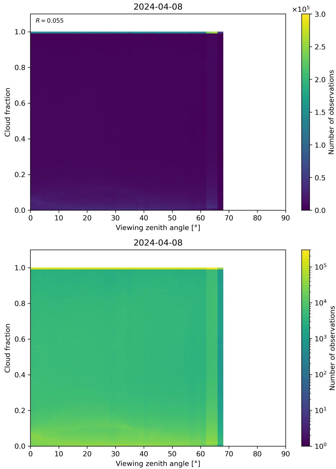
Figure 120: Scatter density plot of “Viewing zenith angle” against “Cloud fraction” for 2024-04-07 to 2024-04-09.
