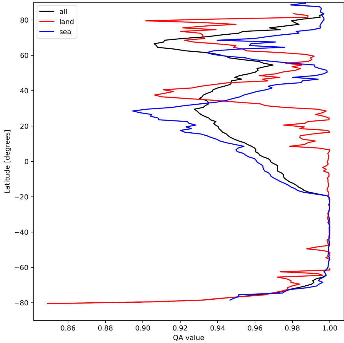
Figure 12: Zonal average of “QA value” for 2024-04-07 to 2024-04-09.
