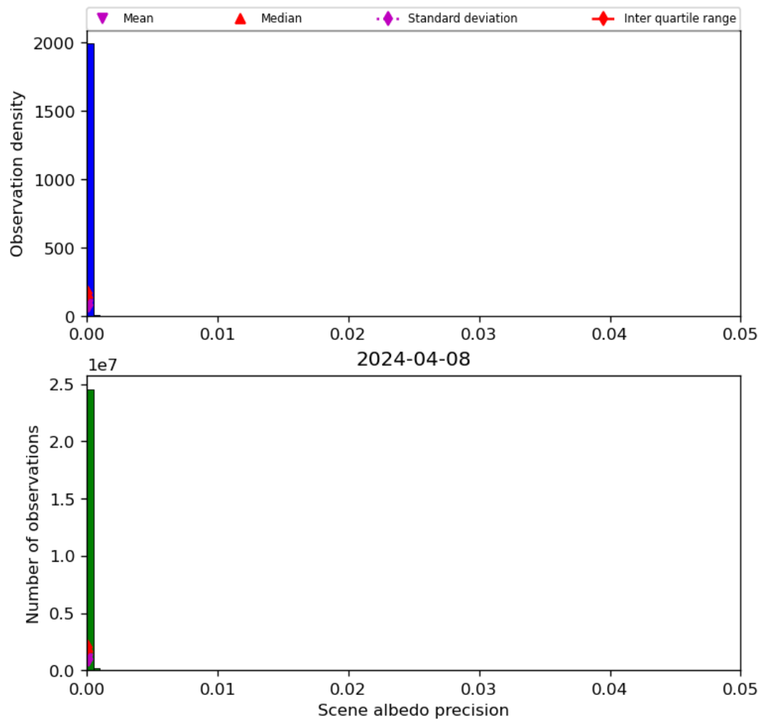
Figure 35: Histogram of “Scene albedo precision” for 2024-04-07 to 2024-04-09
