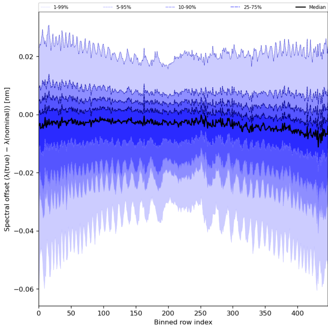
Figure 62: Along track statistics of “Spectral offset ( \lambda(\text{true}) - \lambda(\text{nominal}) )” for 2024-04-08 to 2024-04-10
