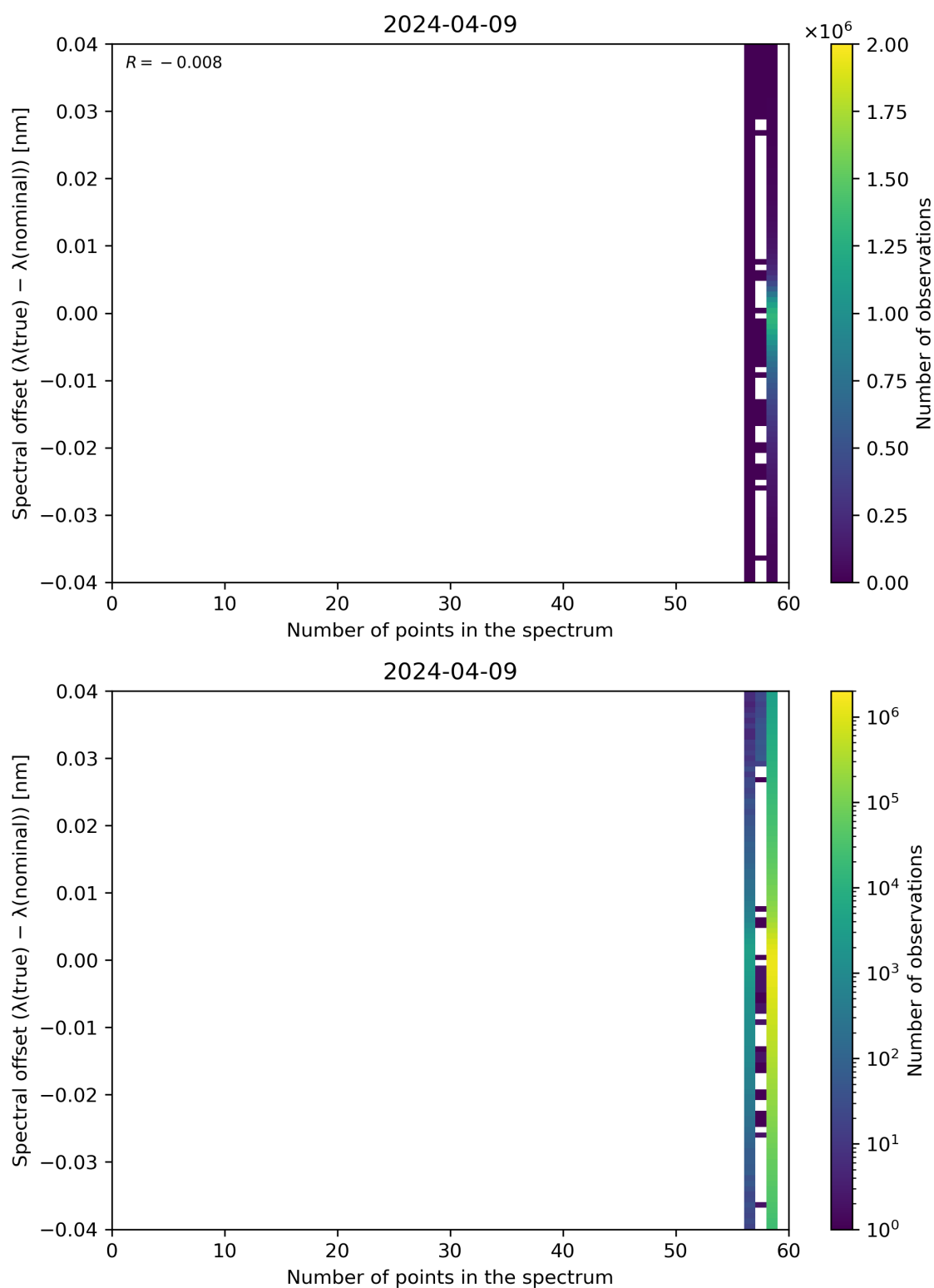
Figure 101: Scatter density plot of “Number of points in the spectrum” against “Spectral offset ( \lambda(\text{true}) - \lambda(\text{nominal}) )” for 2024-04-08 to 2024-04-10.
