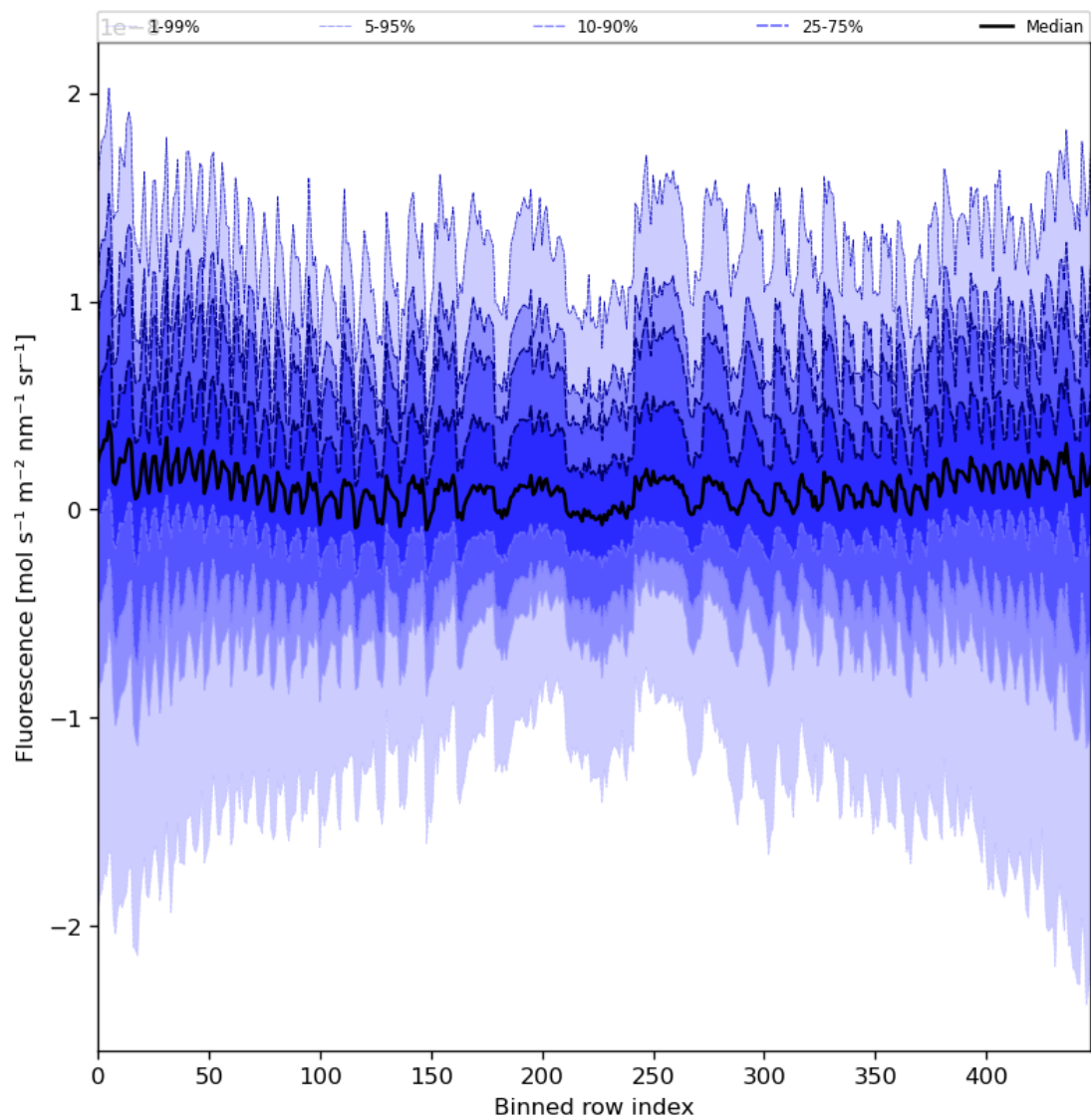
Figure 57: Along track statistics of "Fluorescence" for 2024-04-08 to 2024-04-10
