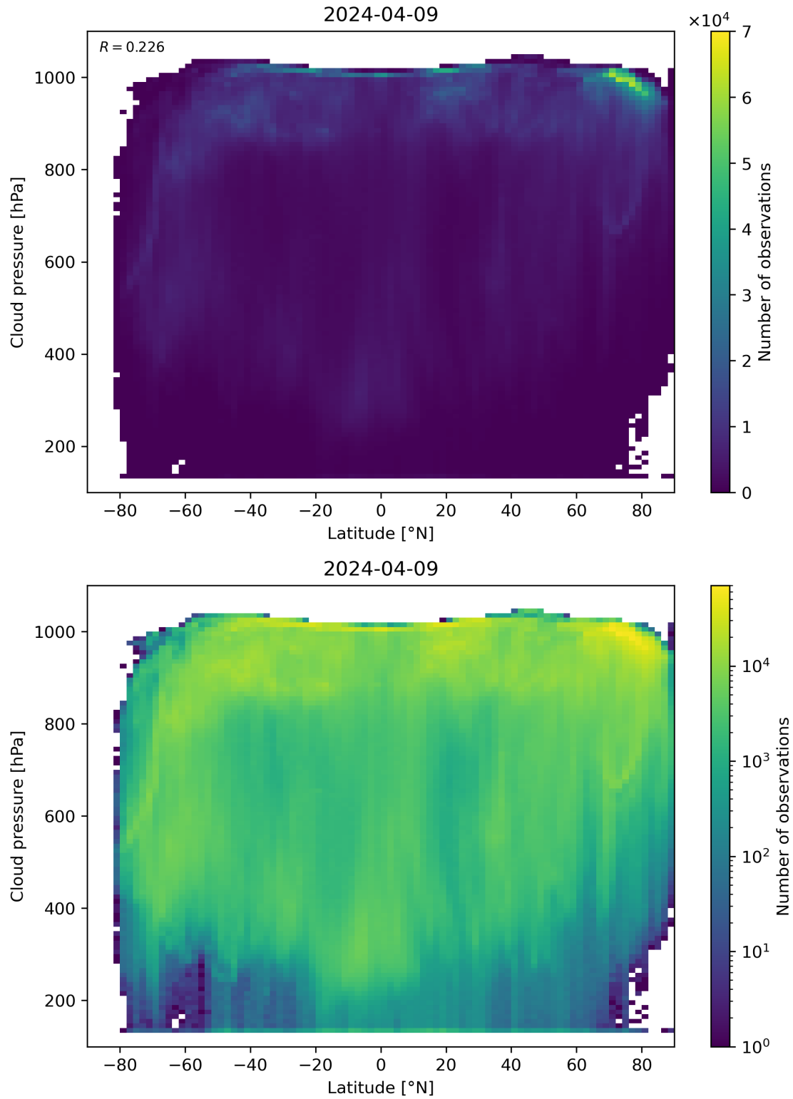
Figure 91: Scatter density plot of “Latitude” against “Cloud pressure” for 2024-04-08 to 2024-04-10.
