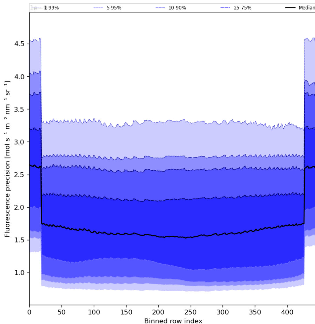
Figure 58: Along track statistics of “Fluorescence precision” for 2024-04-08 to 2024-04-10
