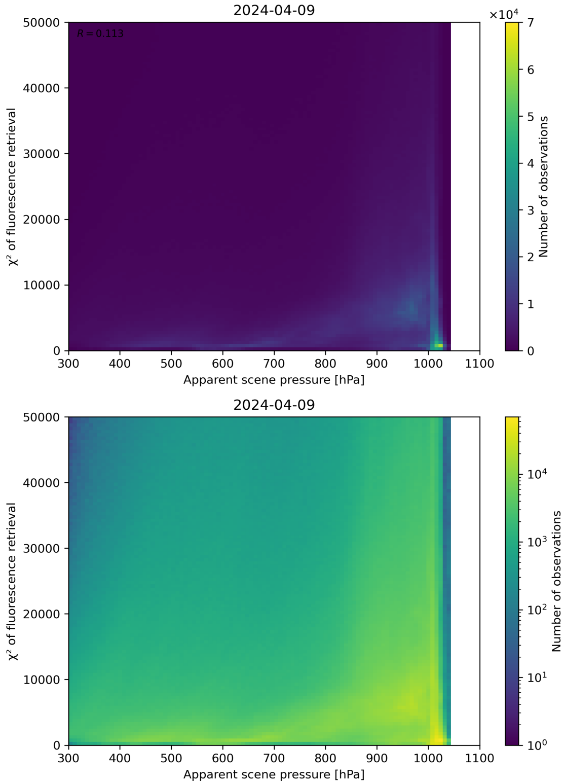
Figure 63: Scatter density plot of “Apparent scene pressure” against “ \chi^2 of fluorescence retrieval” for 2024-04-08 to 2024-04-10.
