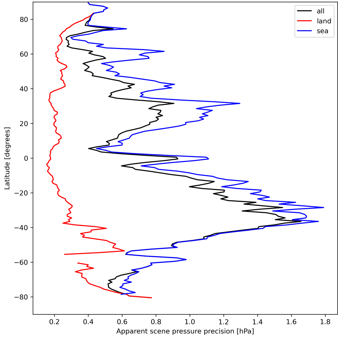
Figure 20: Zonal average of “Apparent scene pressure precision” for 2024-04-08 to 2024-04-10.
