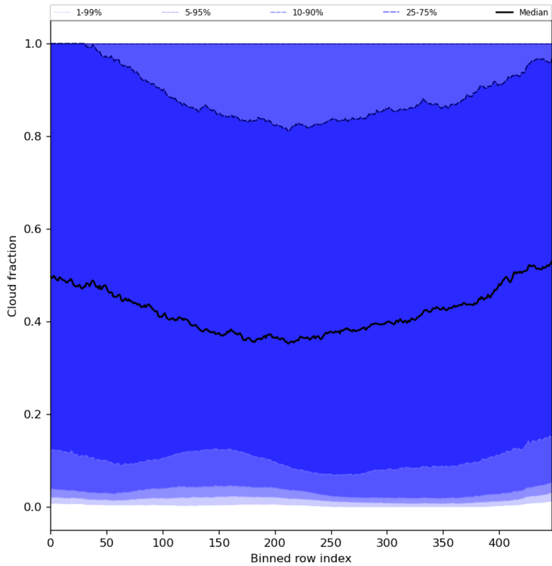
Figure 49: Along track statistics of “Cloud fraction” for 2024-04-08 to 2024-04-10
