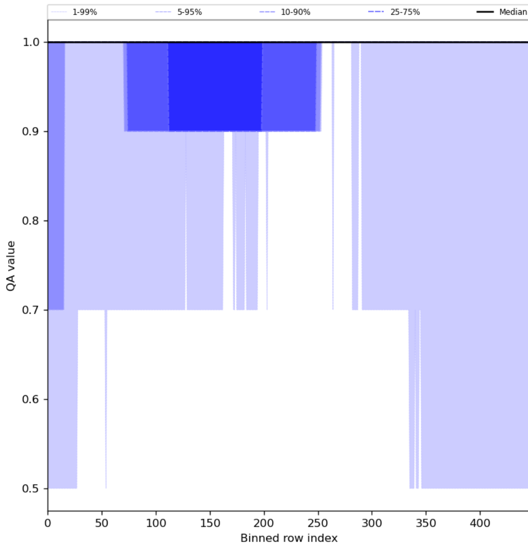
Figure 46: Along track statistics of “QA value” for 2024-04-08 to 2024-04-10
