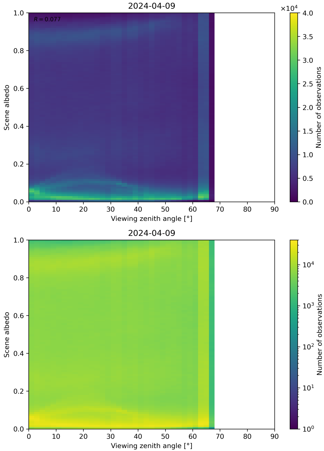
Figure 126: Scatter density plot of “Viewing zenith angle” against “Scene albedo” for 2024-04-08 to 2024-04-10.
