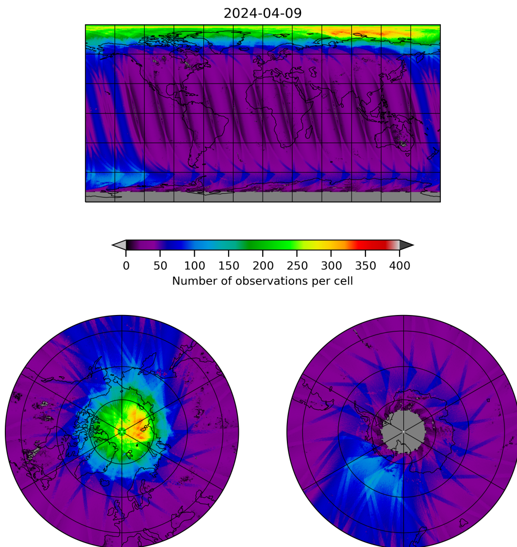
Figure 11: Map of the number of observations for 2024-04-08 to 2024-04-10
