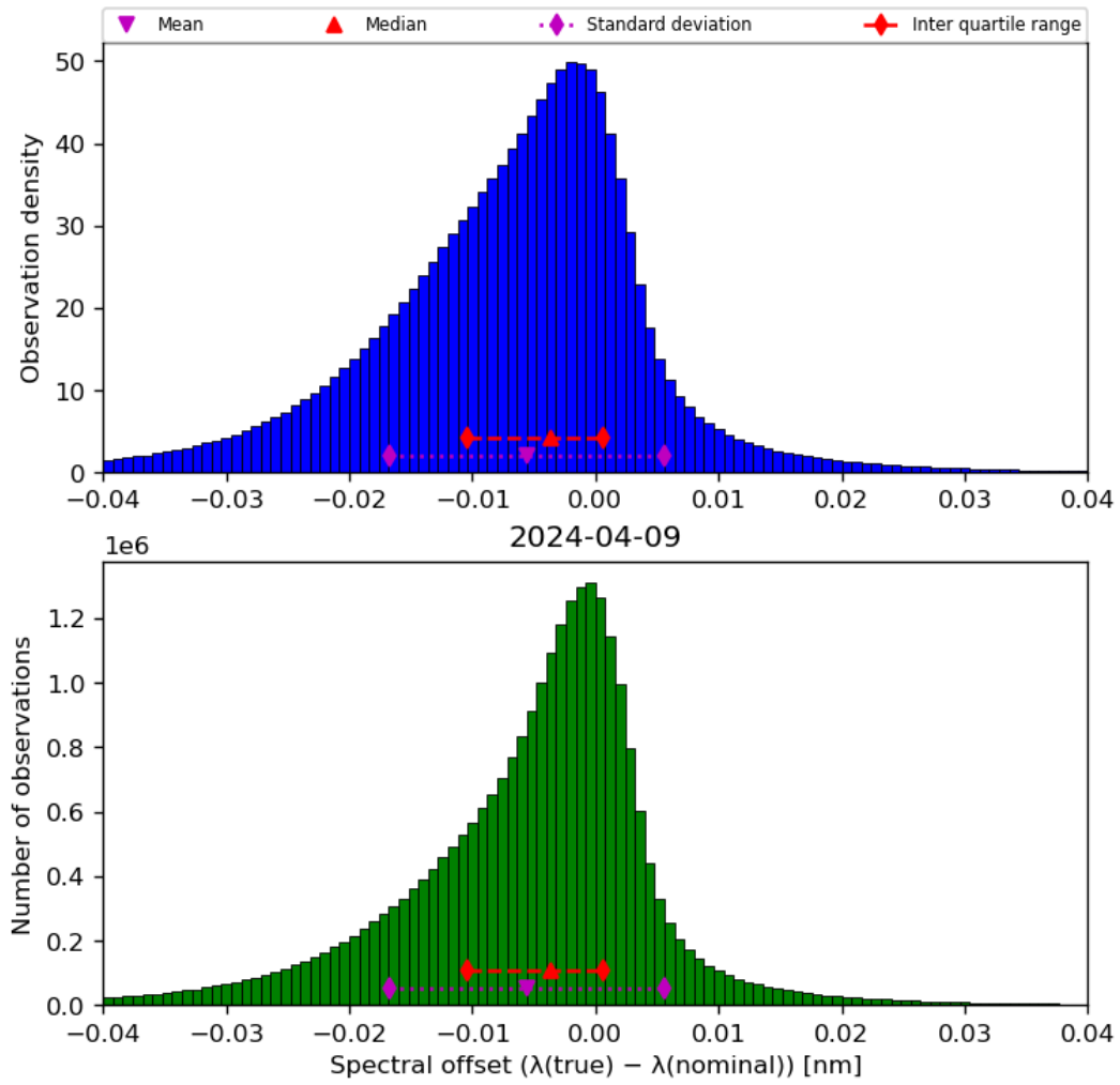
Figure 45: Histogram of “Spectral offset ( \lambda(\text{true}) - \lambda(\text{nominal}) )” for 2024-04-08 to 2024-04-10
