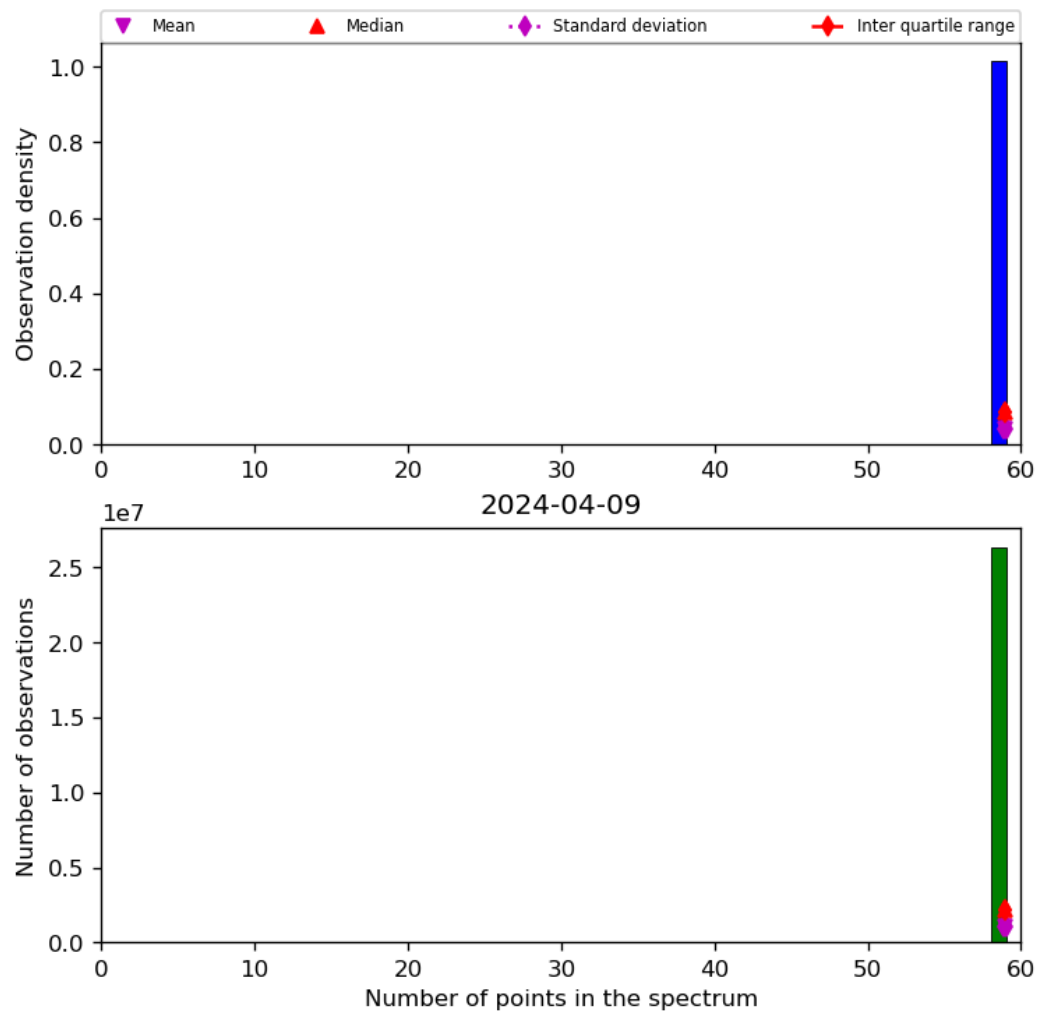
Figure 44: Histogram of “Number of points in the spectrum” for 2024-04-08 to 2024-04-10
