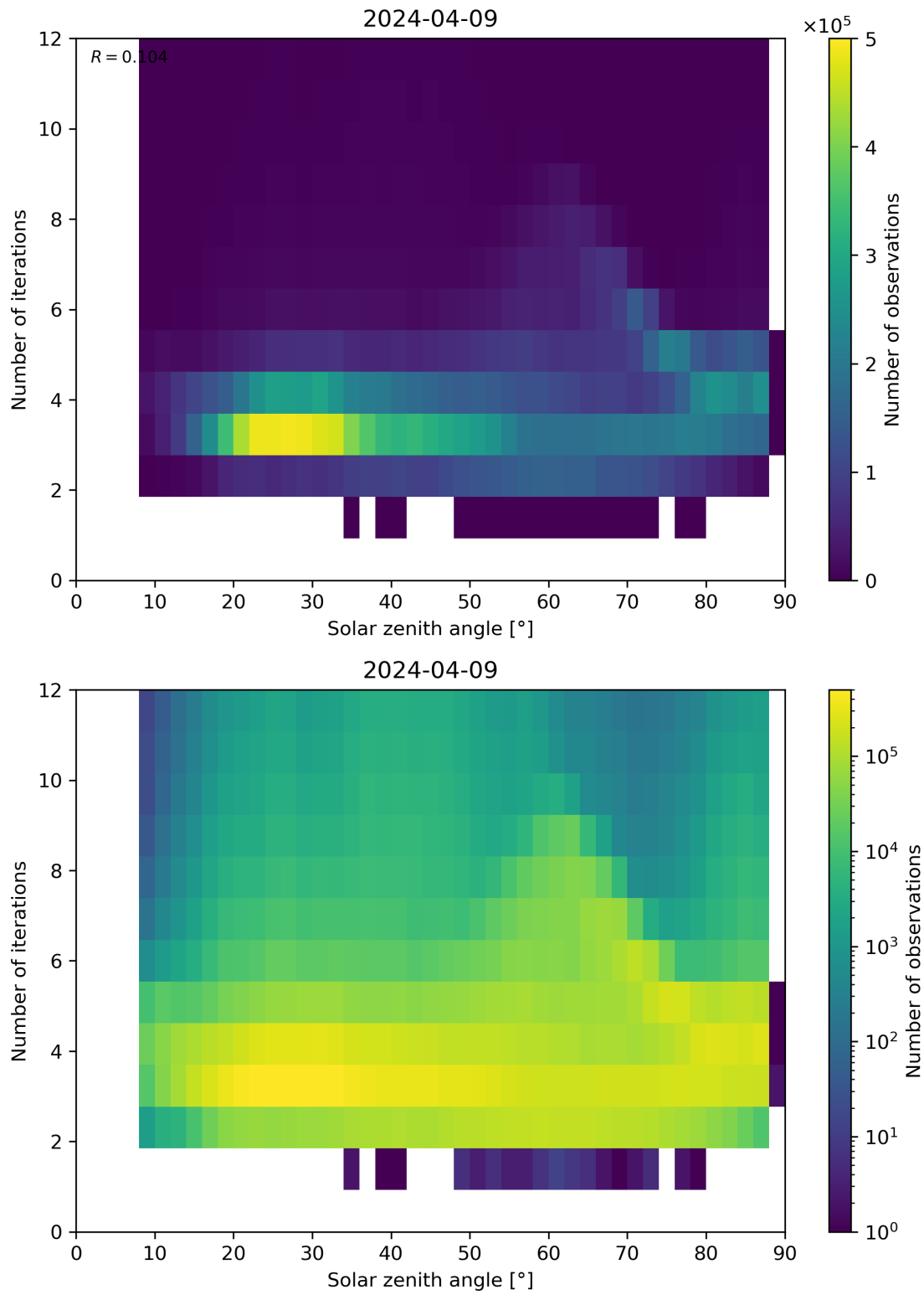
Figure 114: Scatter density plot of “Solar zenith angle” against “Number of iterations” for 2024-04-08 to 2024-04-10.
