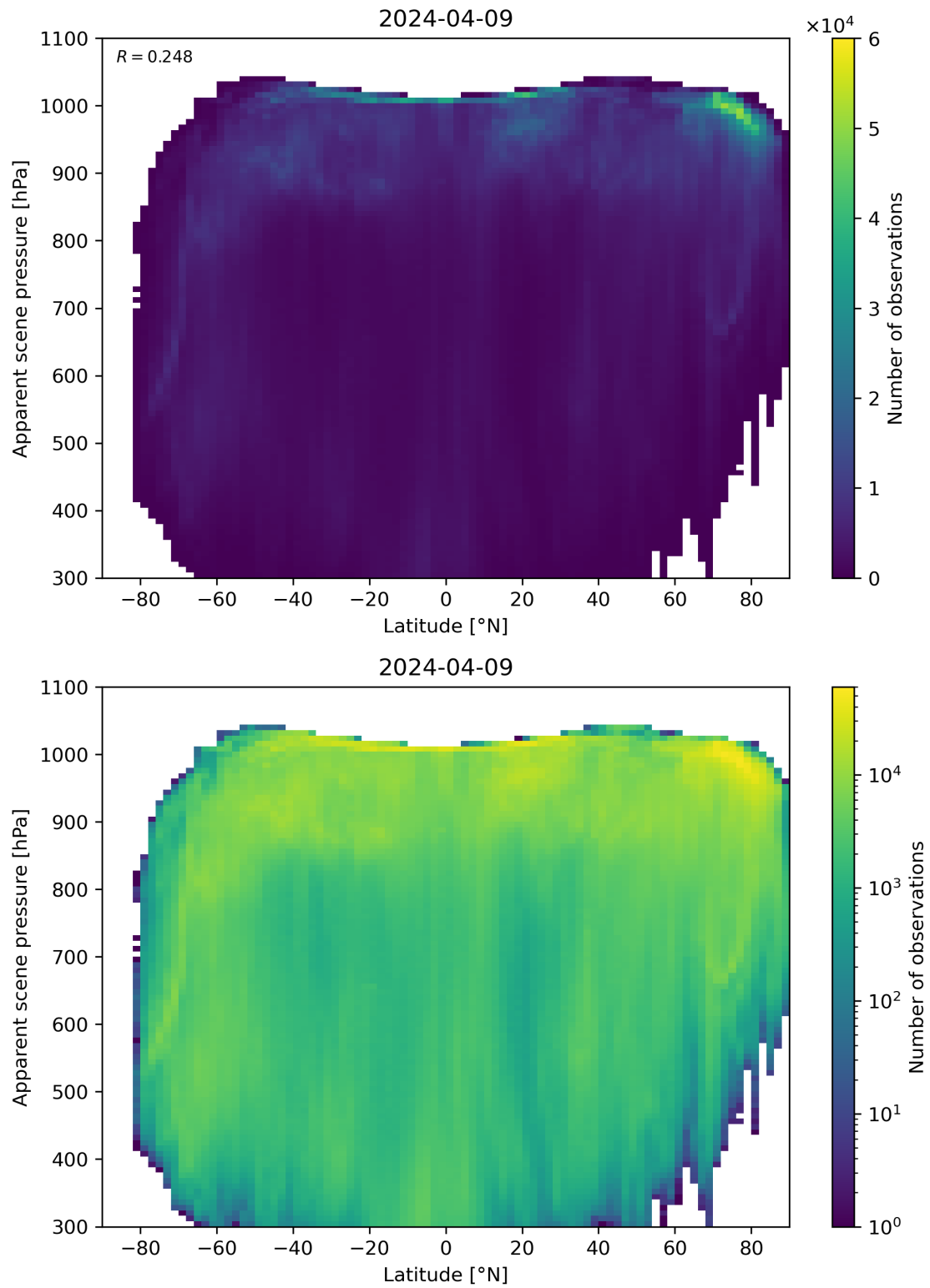
Figure 88: Scatter density plot of “Latitude” against “Apparent scene pressure” for 2024-04-08 to 2024-04-10.
