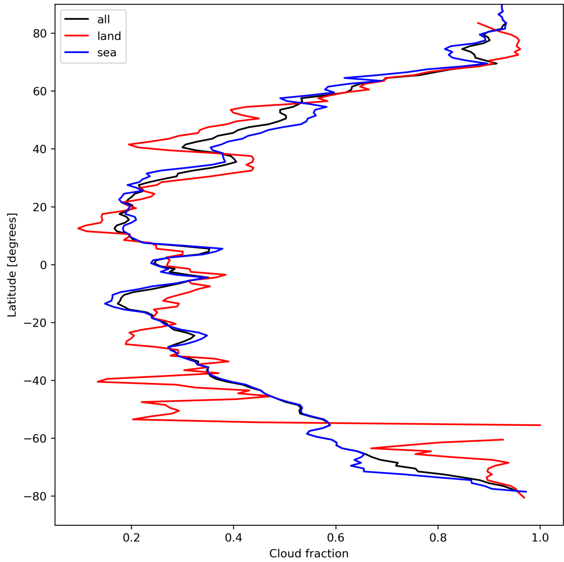
Figure 15: Zonal average of “Cloud fraction” for 2024-04-08 to 2024-04-10.
