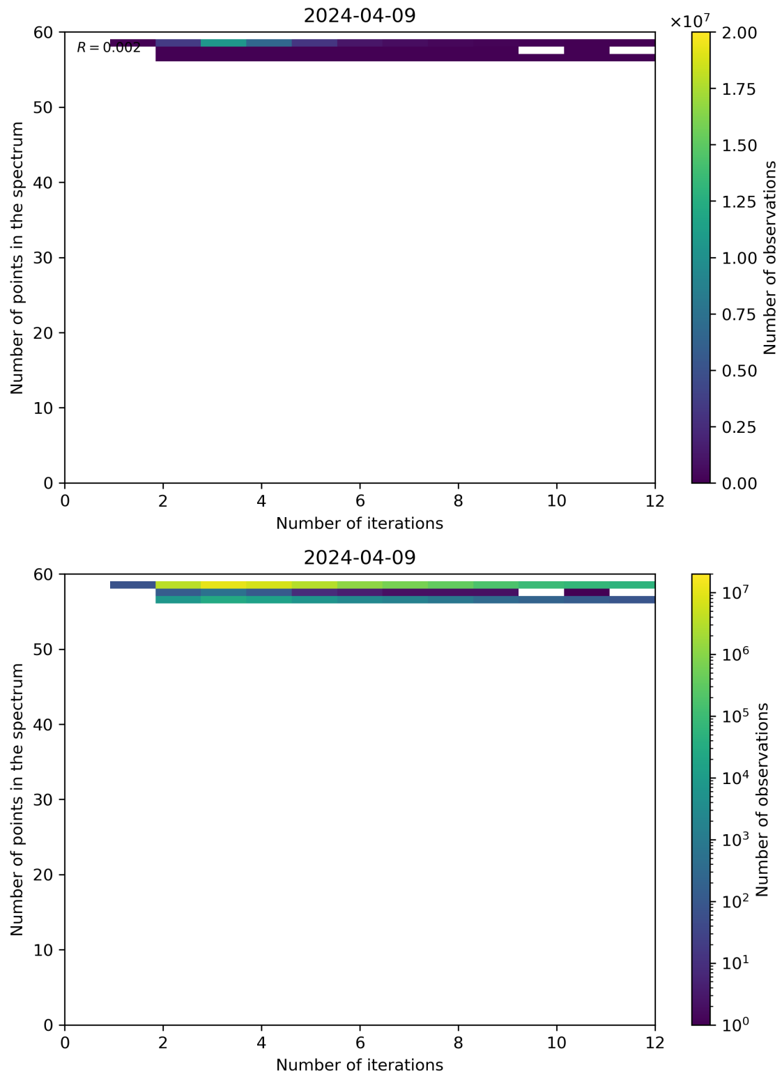
Figure 99: Scatter density plot of “Number of iterations” against “Number of points in the spectrum” for 2024-04-08 to 2024-04-10.
