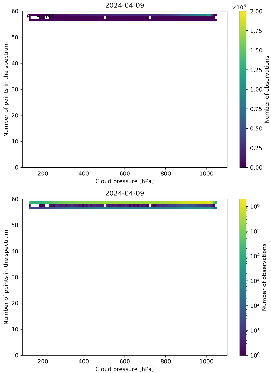
Figure 82: Scatter density plot of “Cloud pressure” against “Number of points in the spectrum” for 2024-04-08 to 2024-04-10.
