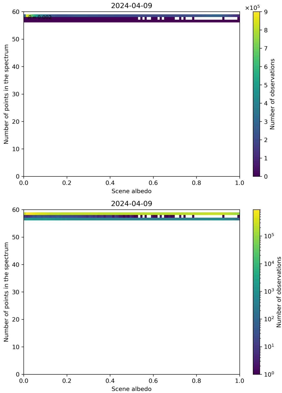
Figure 106: Scatter density plot of “Scene albedo” against “Number of points in the spectrum” for 2024-04-08 to 2024-04-10.
