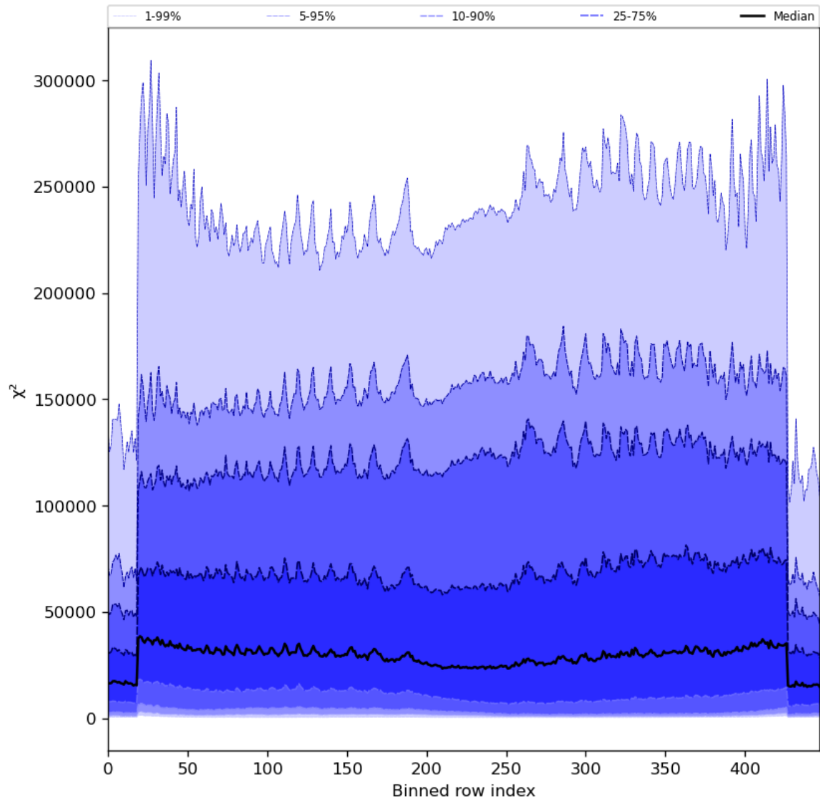
Figure 55: Along track statistics of “ \chi^2 ” for 2024-04-08 to 2024-04-10
