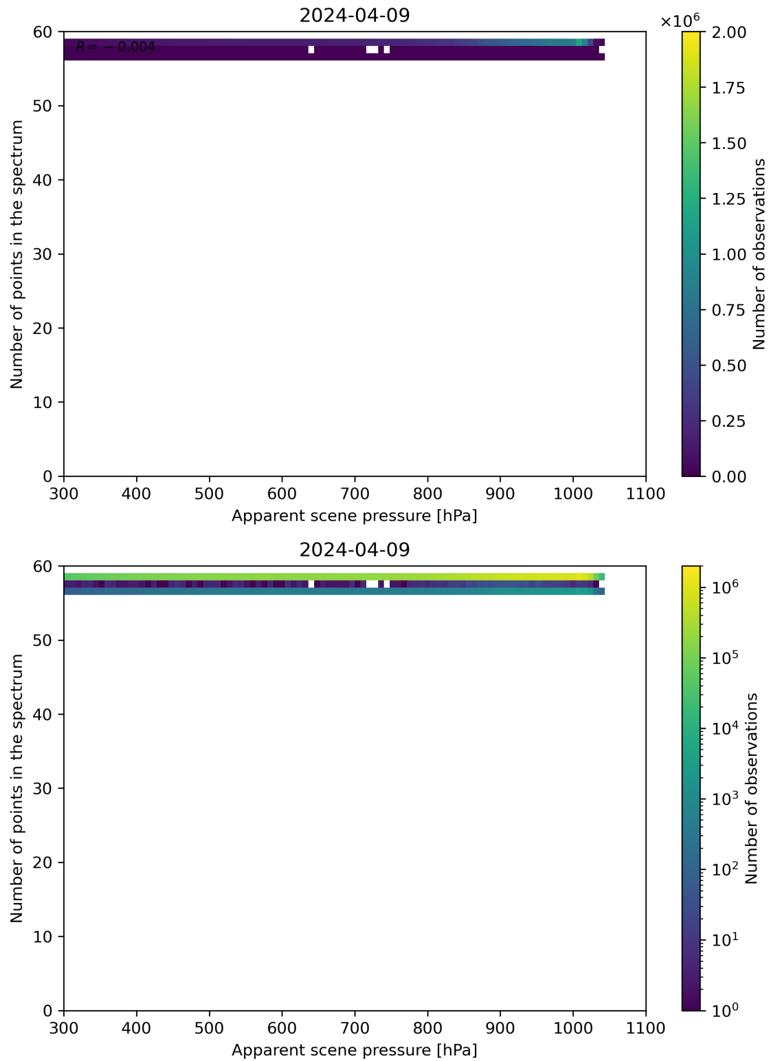
Figure 66: Scatter density plot of “Apparent scene pressure” against “Number of points in the spectrum” for 2024-04-08 to 2024-04-10.
