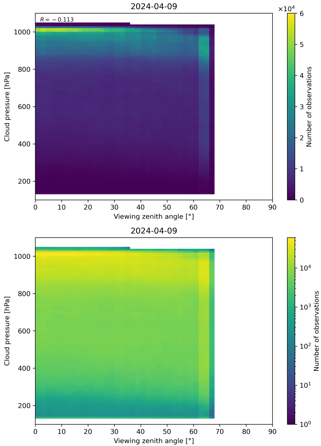
Figure 121: Scatter density plot of “Viewing zenith angle” against “Cloud pressure” for 2024-04-08 to 2024-04-10.
