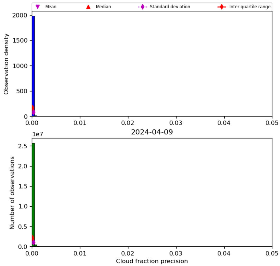
Figure 33: Histogram of “Cloud fraction precision” for 2024-04-08 to 2024-04-10
