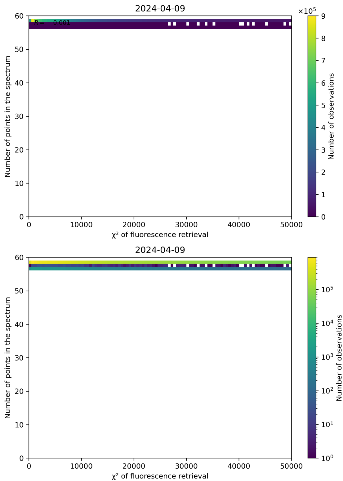
Figure 68: Scatter density plot of " \chi^2 of fluorescence retrieval" against "Number of points in the spectrum" for 2024-04-08 to 2024-04-10.
