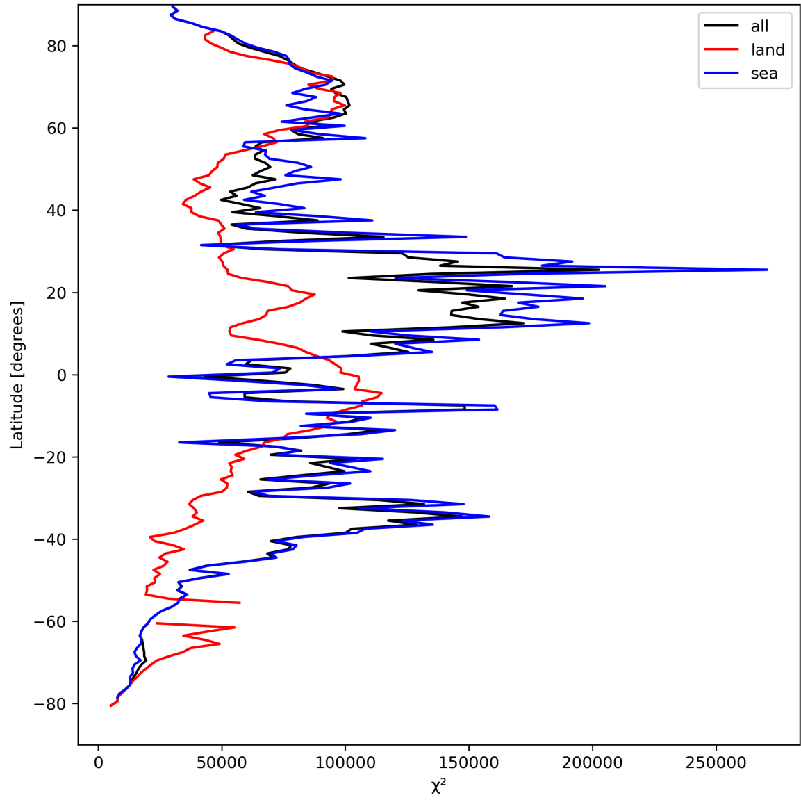
Figure 21: Zonal average of “ \chi^2 ” for 2024-04-08 to 2024-04-10.
