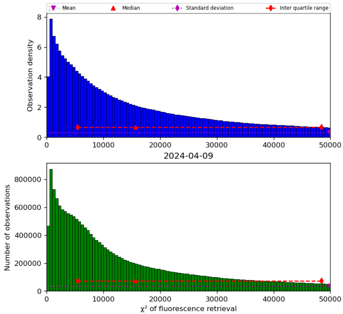
Figure 42: Histogram of “ \chi^2 of fluorescence retrieval” for 2024-04-08 to 2024-04-10
