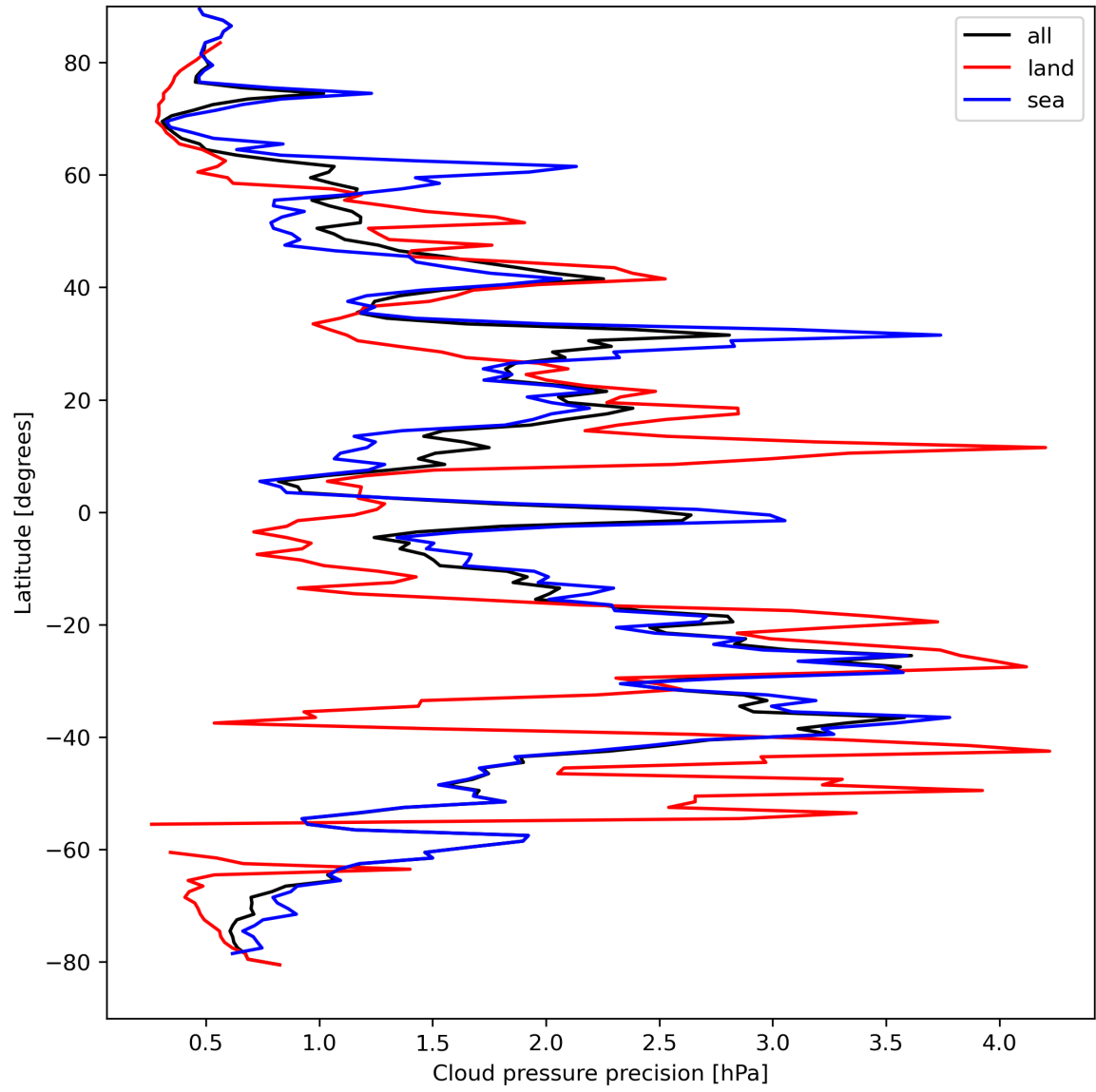
Figure 14: Zonal average of “Cloud pressure precision” for 2024-04-08 to 2024-04-10.
