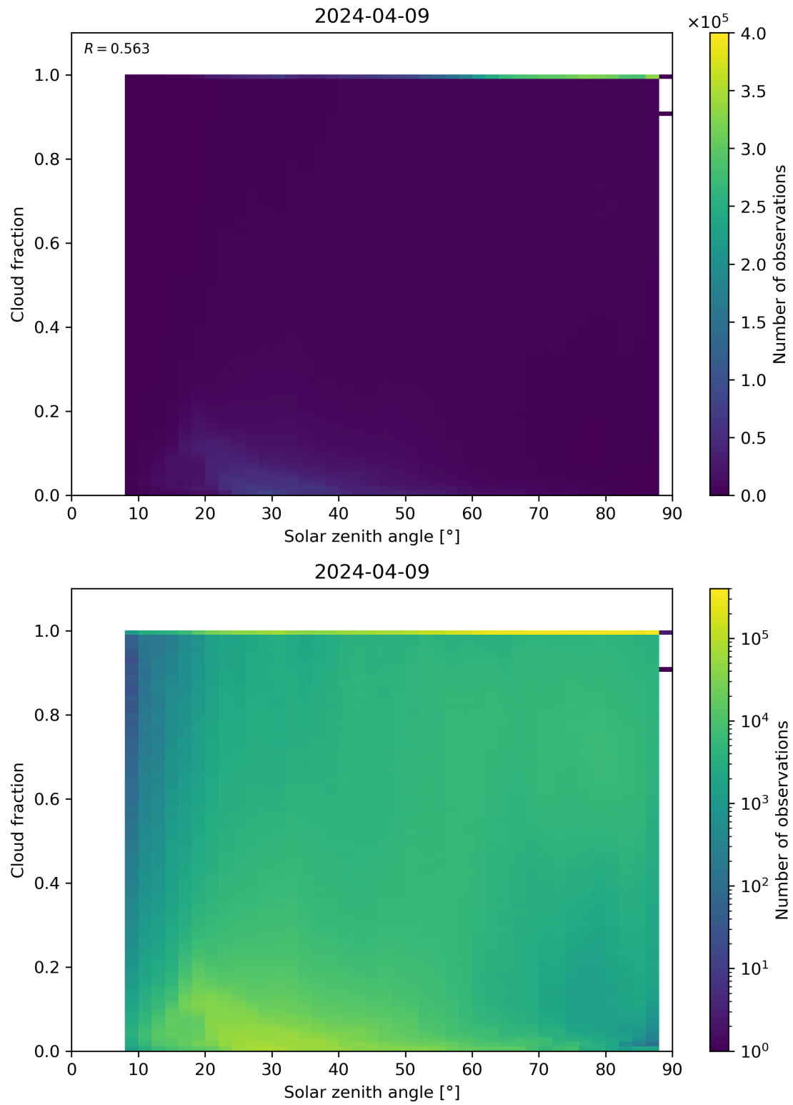
Figure 110: Scatter density plot of “Solar zenith angle” against “Cloud fraction” for 2024-04-08 to 2024-04-10.
