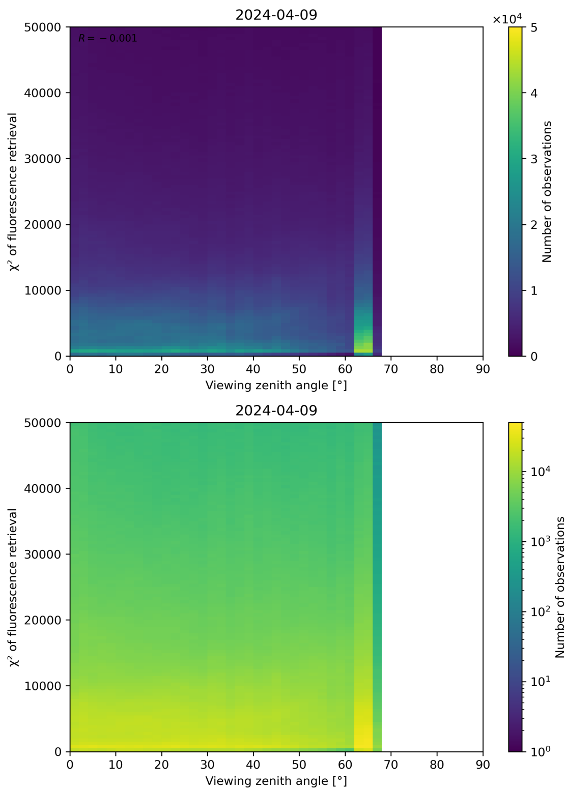
Figure 119: Scatter density plot of “Viewing zenith angle” against “ \chi^2 of fluorescence retrieval” for 2024-04-08 to 2024-04-10.
