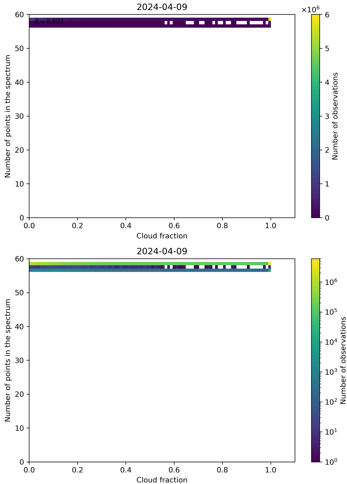
Figure 74: Scatter density plot of “Cloud fraction” against “Number of points in the spectrum” for 2024-04-08 to 2024-04-10.
