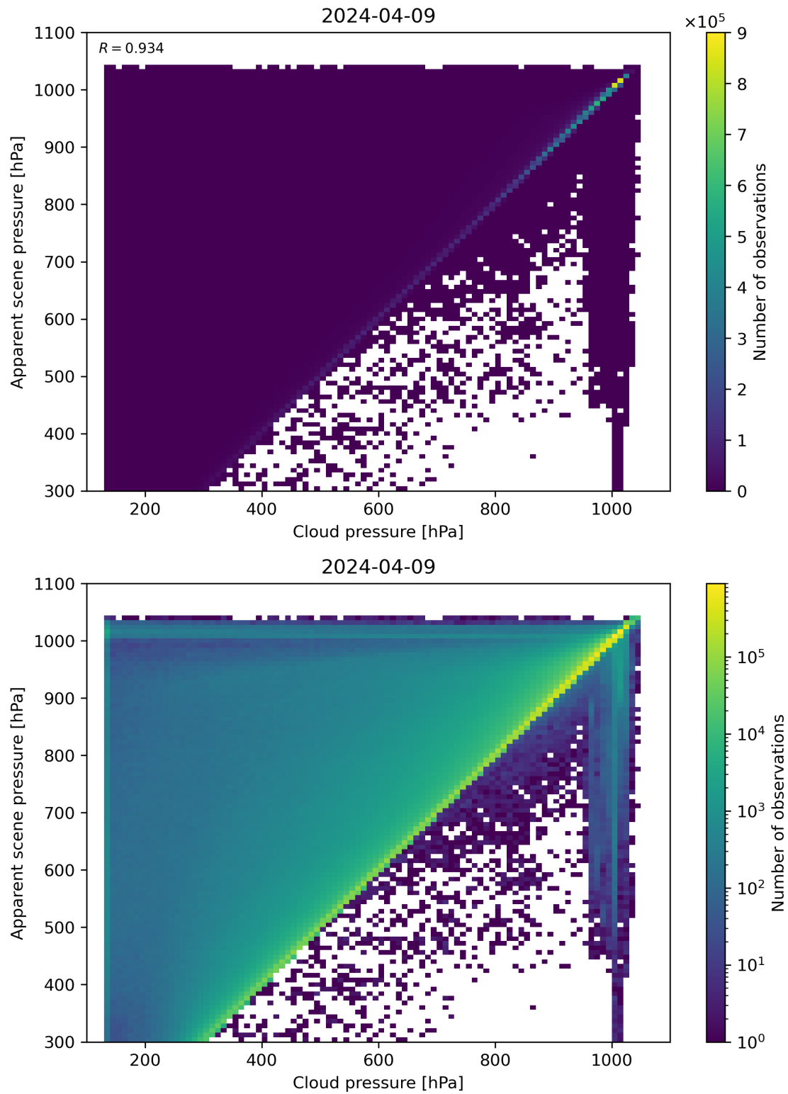
Figure 77: Scatter density plot of “Cloud pressure” against “Apparent scene pressure” for 2024-04-08 to 2024-04-10.
