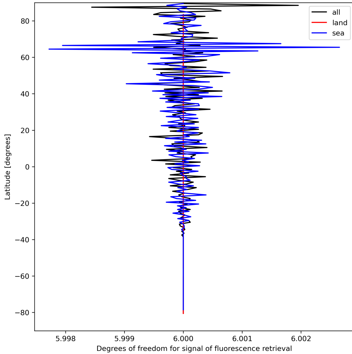
Figure 26: Zonal average of “Degrees of freedom for signal of fluorescence retrieval” for 2024-04-08 to 2024-04-10.
