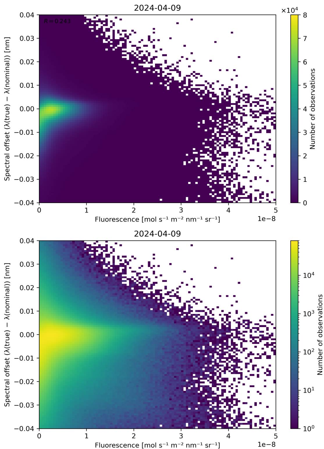
Figure 87: Scatter density plot of “Fluorescence” against “Spectral offset ( \lambda(\text{true}) - \lambda(\text{nominal}) )” for 2024-04-08 to 2024-04-10.
