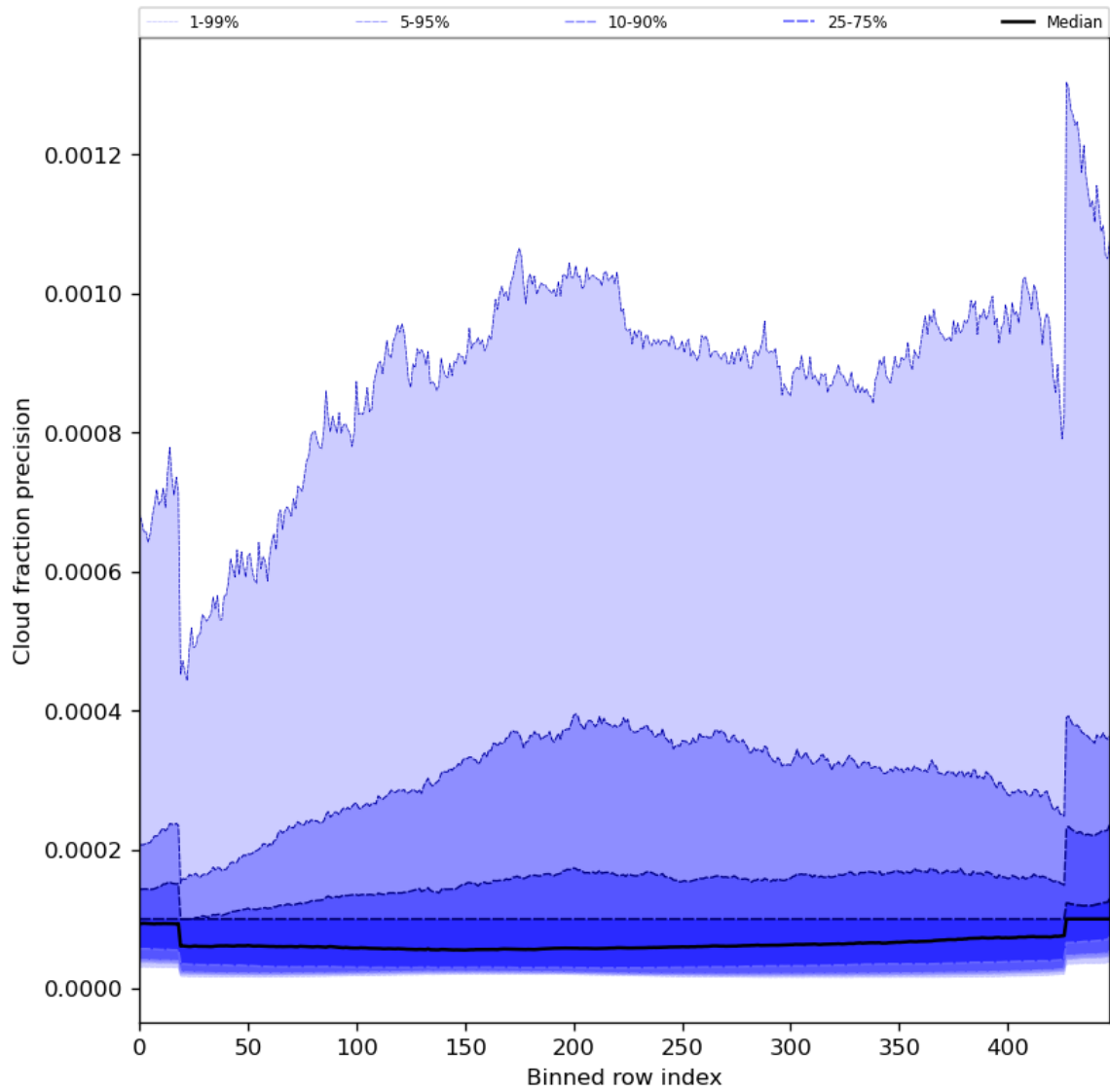
Figure 50: Along track statistics of “Cloud fraction precision” for 2024-04-08 to 2024-04-10
