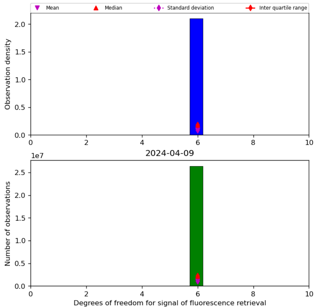
Figure 43: Histogram of “Degrees of freedom for signal of fluorescence retrieval” for 2024-04-08 to 2024-04-10
