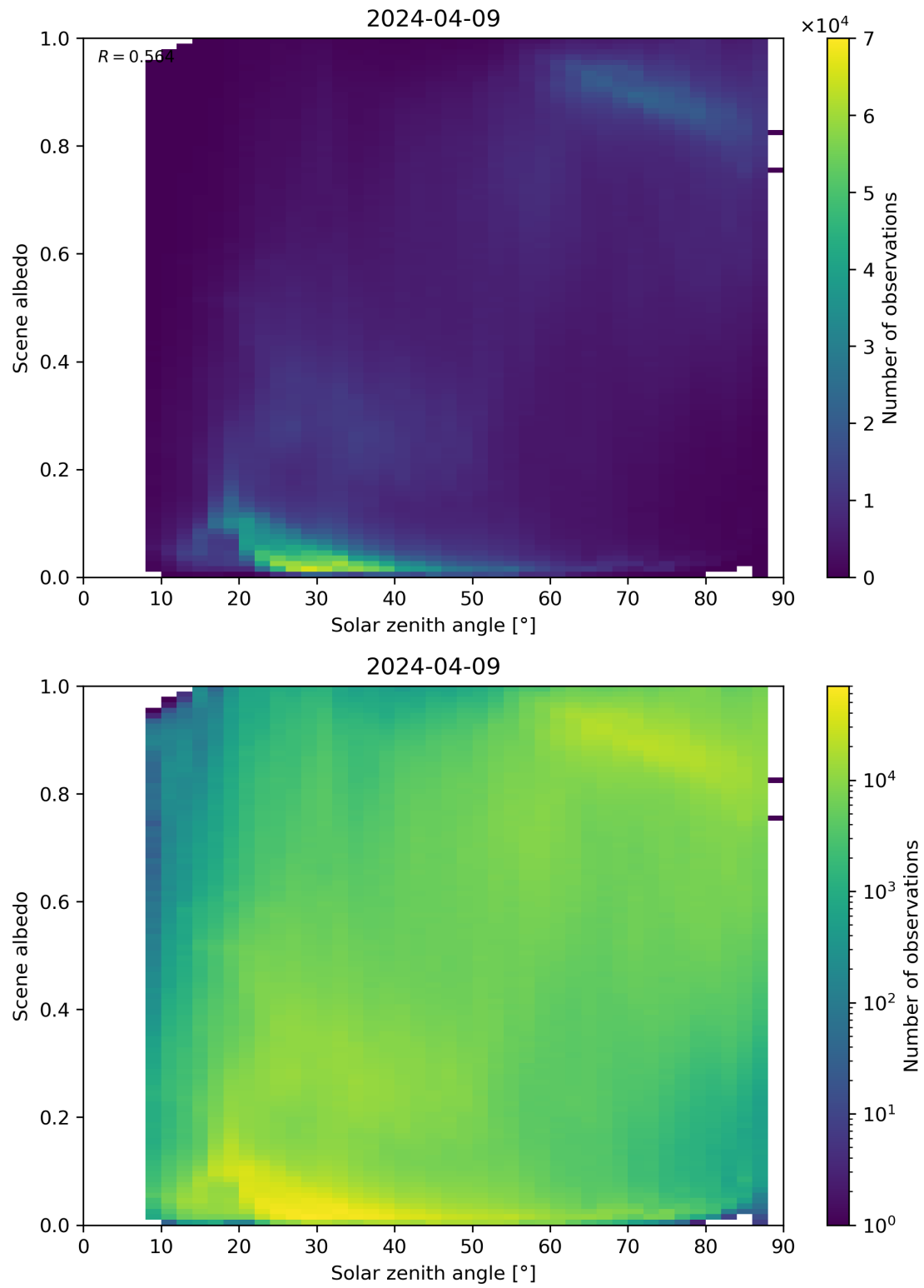
Figure 116: Scatter density plot of “Solar zenith angle” against “Scene albedo” for 2024-04-08 to 2024-04-10.
