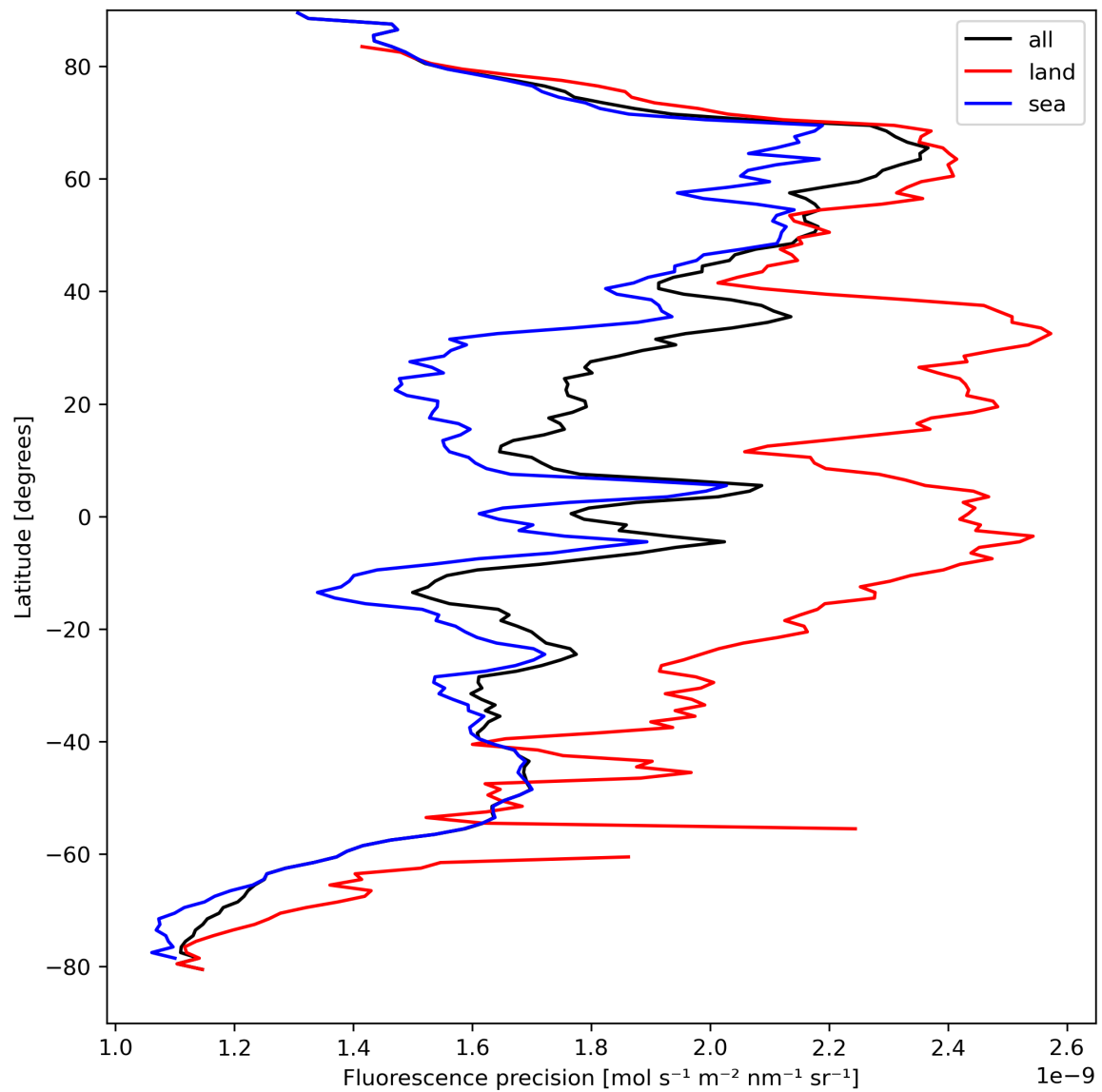
Figure 24: Zonal average of “Fluorescence precision” for 2024-04-08 to 2024-04-10.
