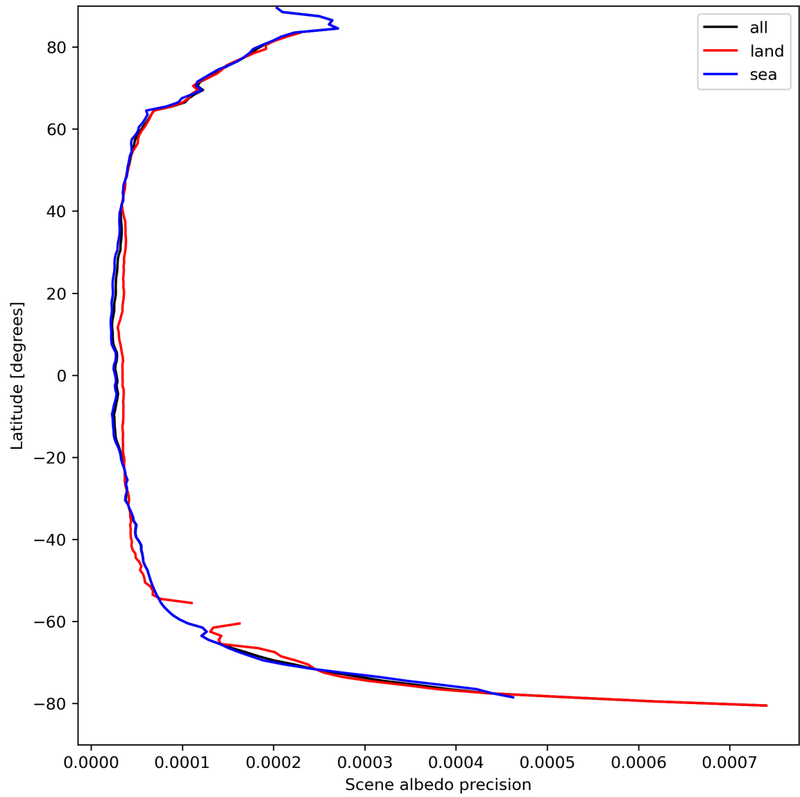
Figure 18: Zonal average of “Scene albedo precision” for 2024-04-08 to 2024-04-10.
