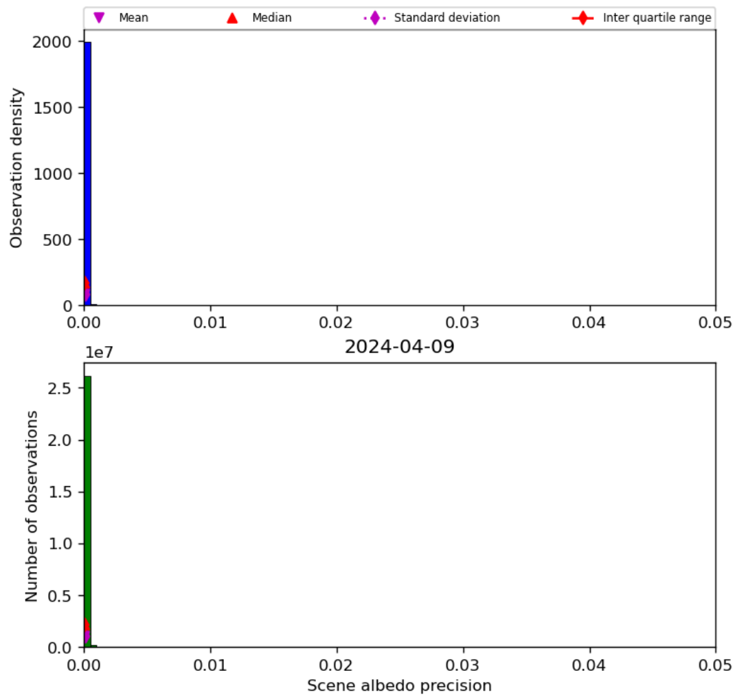
Figure 35: Histogram of “Scene albedo precision” for 2024-04-08 to 2024-04-10
