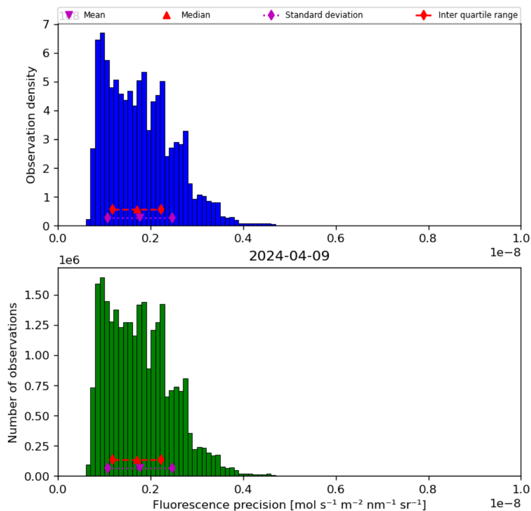
Figure 41: Histogram of “Fluorescence precision” for 2024-04-08 to 2024-04-10
