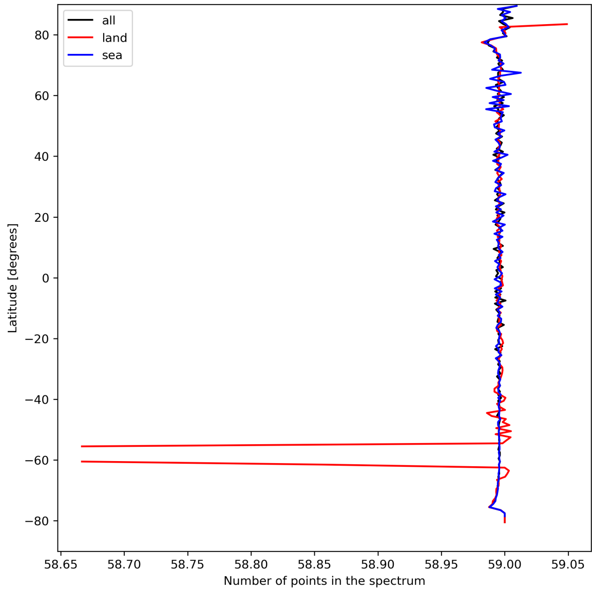
Figure 27: Zonal average of “Number of points in the spectrum” for 2024-04-08 to 2024-04-10.
