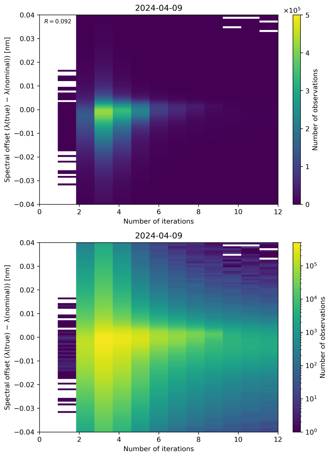
Figure 100: Scatter density plot of “Number of iterations” against “Spectral offset ( \lambda(\text{true}) - \lambda(\text{nominal}) )” for 2024-04-08 to 2024-04-10.
