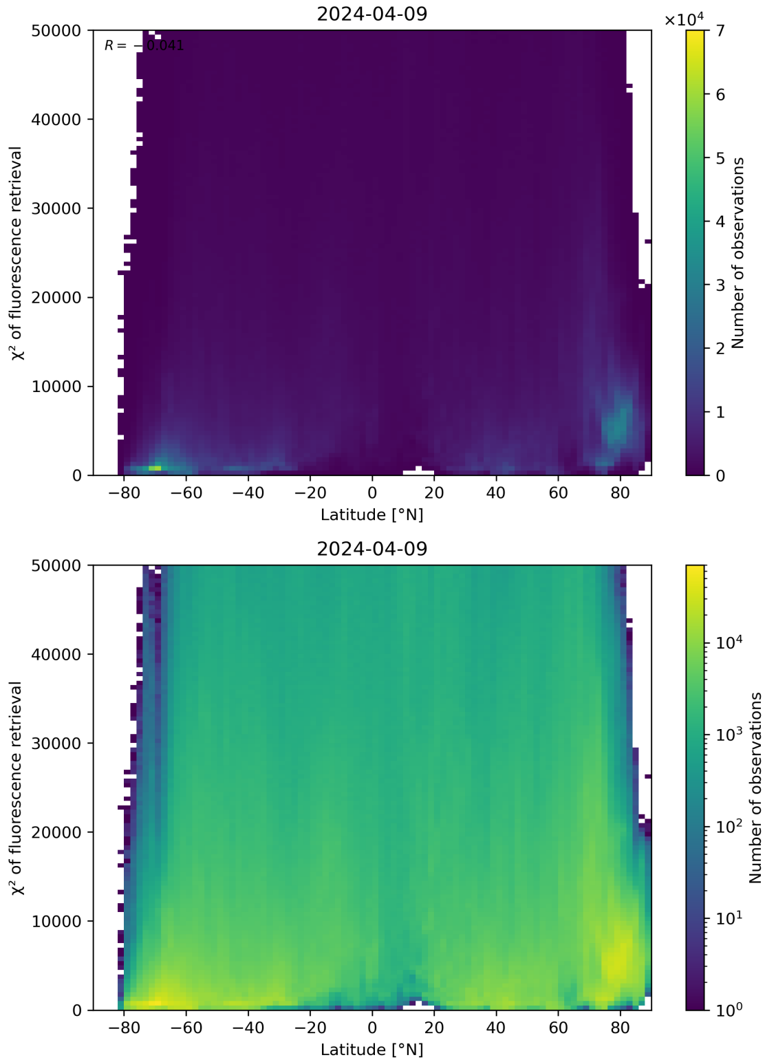
Figure 89: Scatter density plot of “Latitude” against “ \chi^2 of fluorescence retrieval” for 2024-04-08 to 2024-04-10.
