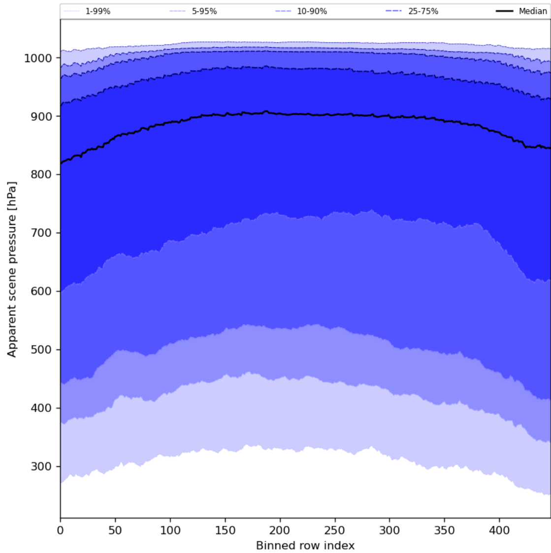
Figure 53: Along track statistics of “Apparent scene pressure” for 2024-04-08 to 2024-04-10
