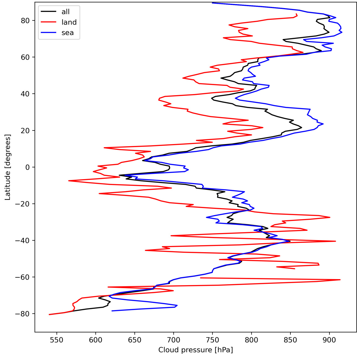
Figure 13: Zonal average of “Cloud pressure” for 2024-04-08 to 2024-04-10.
