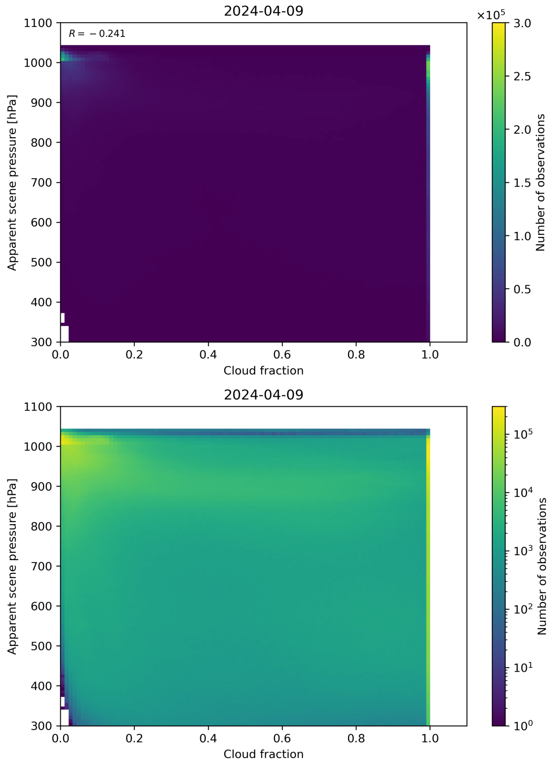
Figure 70: Scatter density plot of “Cloud fraction” against “Apparent scene pressure” for 2024-04-08 to 2024-04-10.
