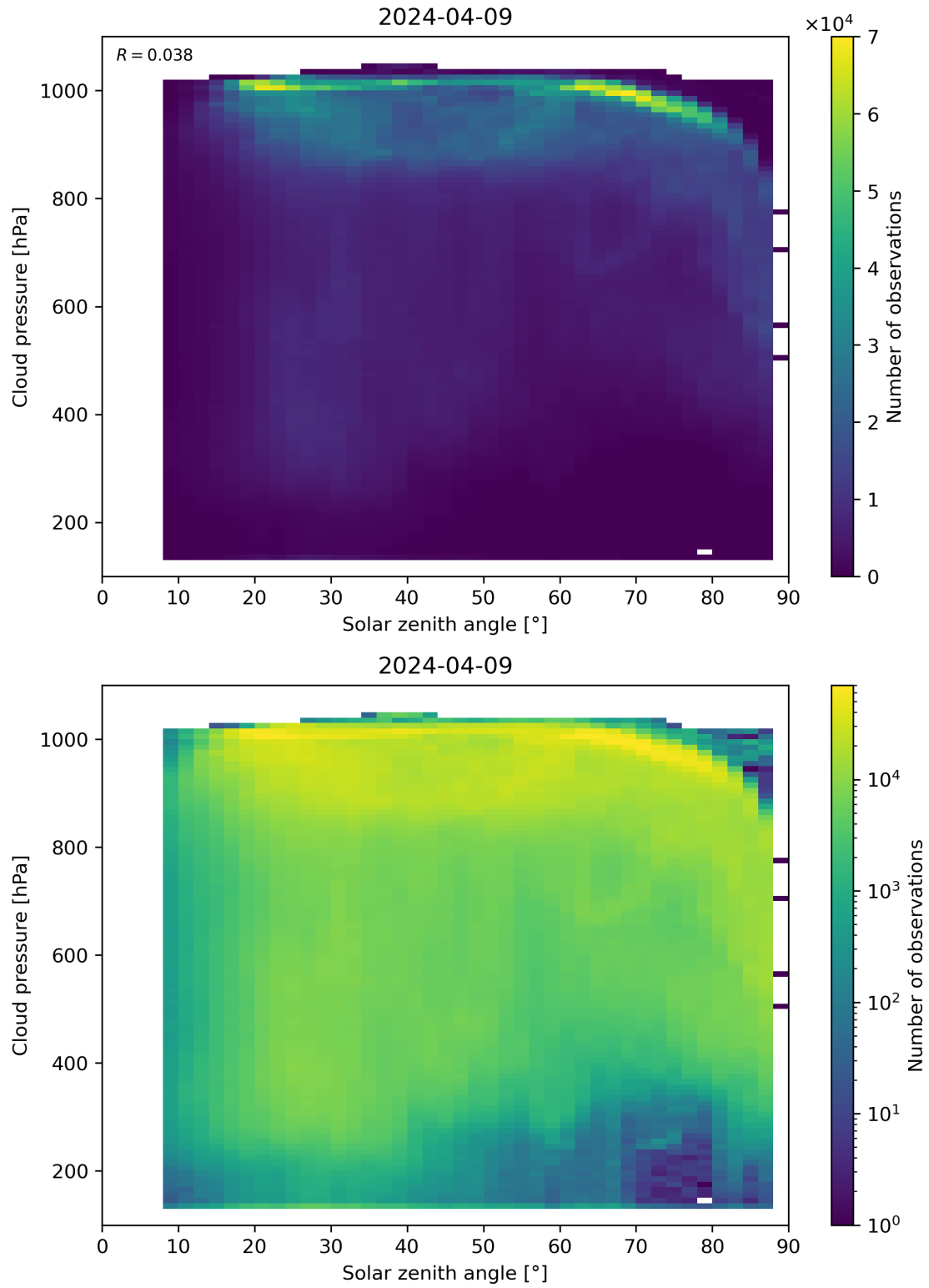
Figure 111: Scatter density plot of “Solar zenith angle” against “Cloud pressure” for 2024-04-08 to 2024-04-10.
