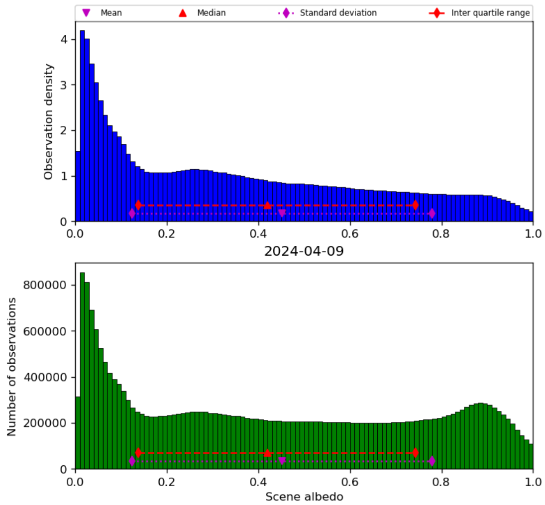
Figure 34: Histogram of “Scene albedo” for 2024-04-08 to 2024-04-10
