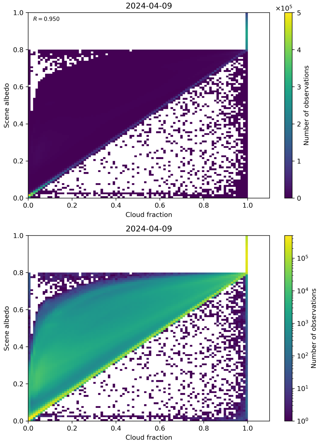
Figure 75: Scatter density plot of “Cloud fraction” against “Scene albedo” for 2024-04-08 to 2024-04-10.
