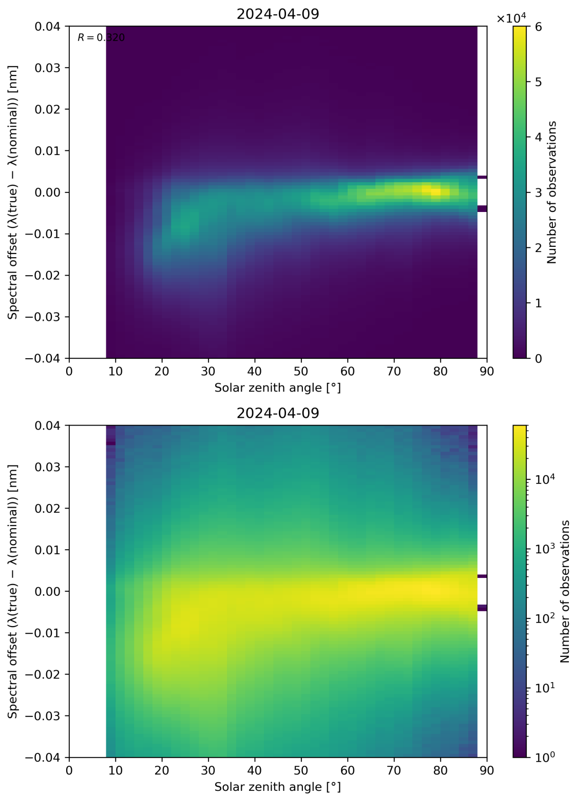
Figure 117: Scatter density plot of “Solar zenith angle” against “Spectral offset ( \lambda(\text{true}) - \lambda(\text{nominal}) )” for 2024-04-08 to 2024-04-10.
