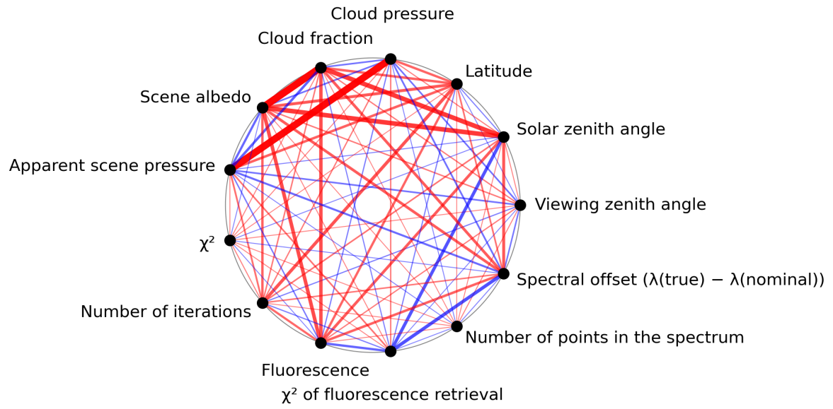
Figure 1: Map of correlation graph for 2024-04-08 to 2024-04-10.
