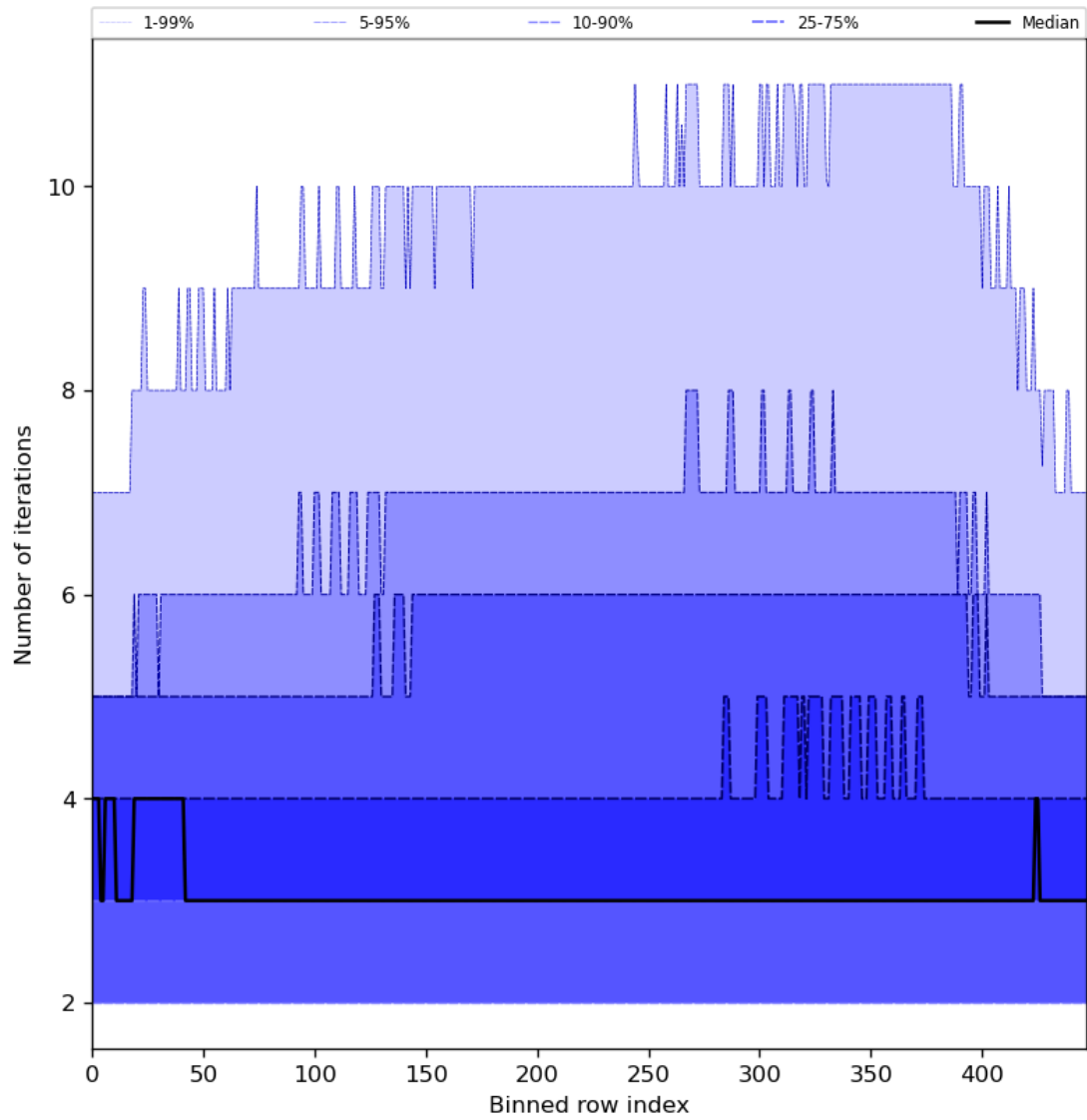
Figure 56: Along track statistics of “Number of iterations” for 2024-04-08 to 2024-04-10
