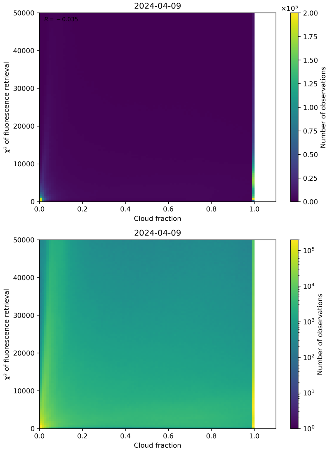
Figure 71: Scatter density plot of “Cloud fraction” against “ \chi^2 of fluorescence retrieval” for 2024-04-08 to 2024-04-10.
