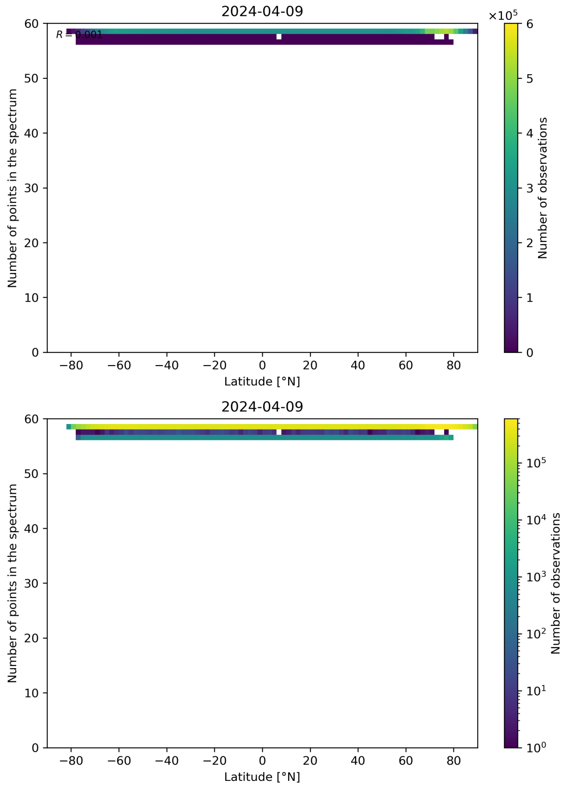
Figure 94: Scatter density plot of “Latitude” against “Number of points in the spectrum” for 2024-04-08 to 2024-04-10.
