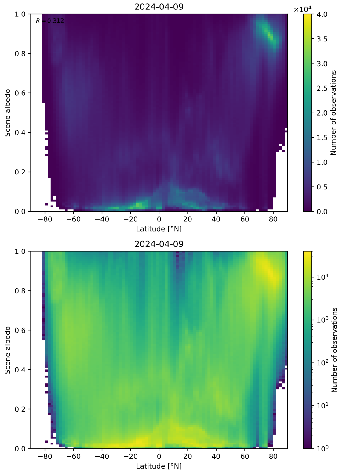
Figure 95: Scatter density plot of “Latitude” against “Scene albedo” for 2024-04-08 to 2024-04-10.
