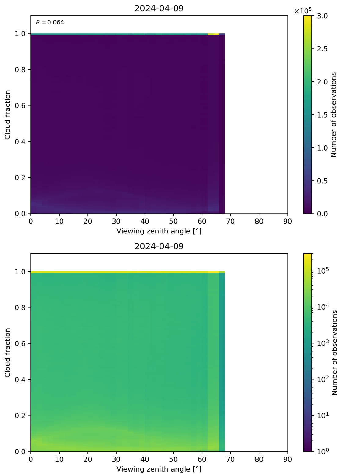
Figure 120: Scatter density plot of “Viewing zenith angle” against “Cloud fraction” for 2024-04-08 to 2024-04-10.
