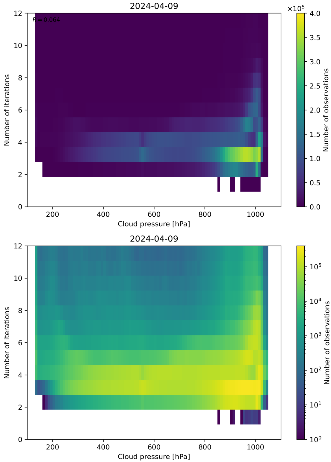
Figure 81: Scatter density plot of “Cloud pressure” against “Number of iterations” for 2024-04-08 to 2024-04-10.
