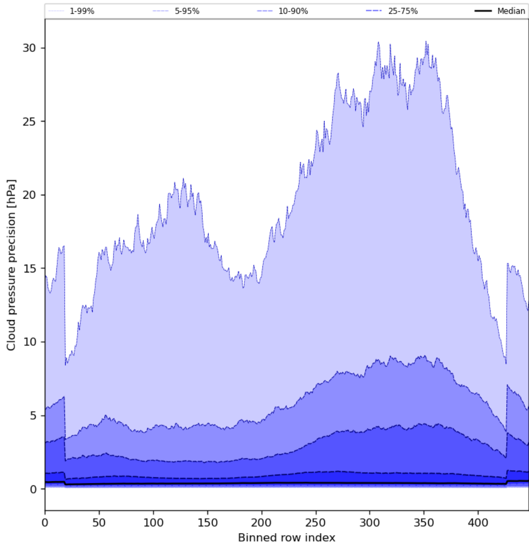
Figure 48: Along track statistics of “Cloud pressure precision” for 2024-04-08 to 2024-04-10
