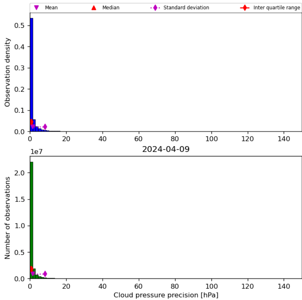
Figure 31: Histogram of “Cloud pressure precision” for 2024-04-08 to 2024-04-10
