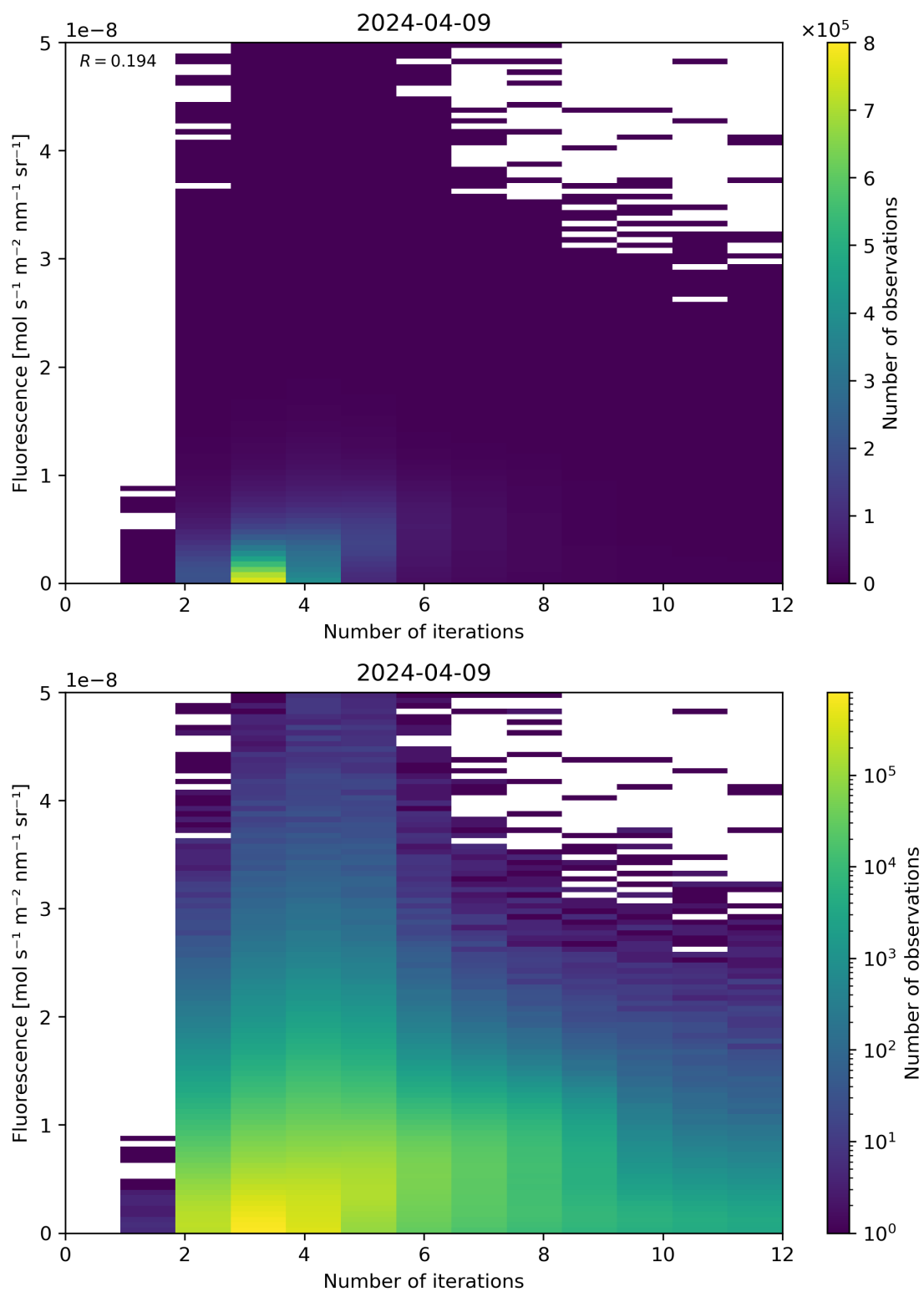
Figure 98: Scatter density plot of “Number of iterations” against “Fluorescence” for 2024-04-08 to 2024-04-10.
