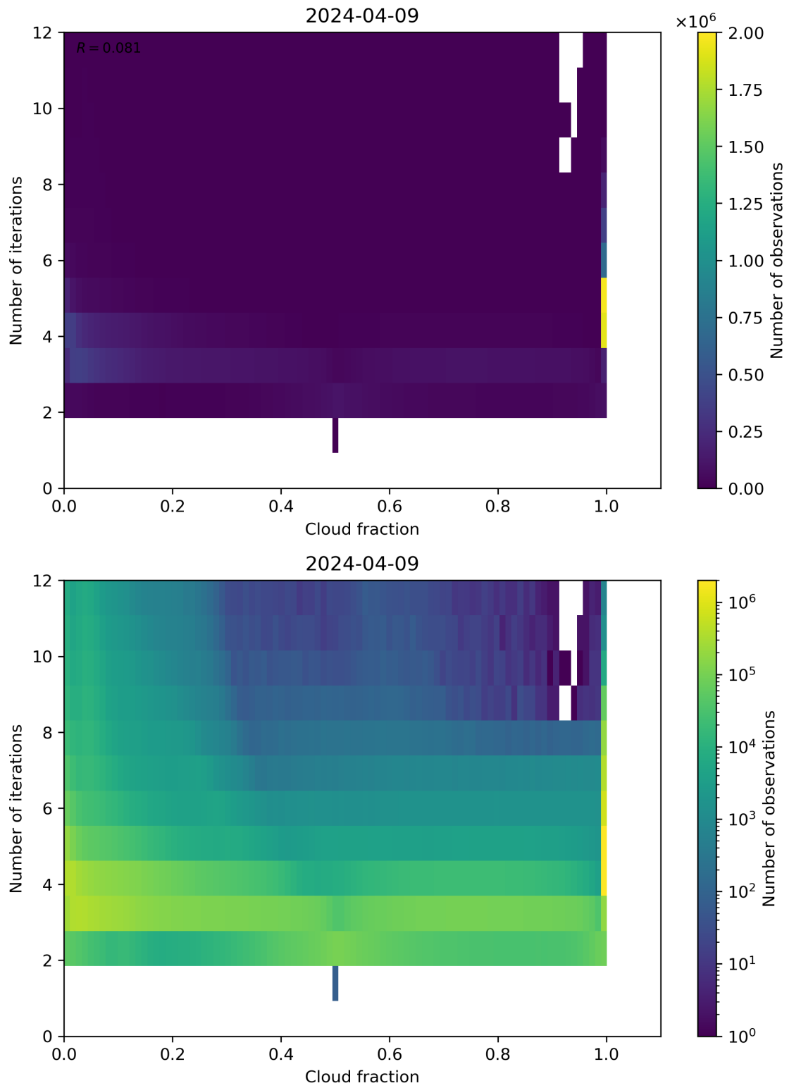
Figure 73: Scatter density plot of “Cloud fraction” against “Number of iterations” for 2024-04-08 to 2024-04-10.
