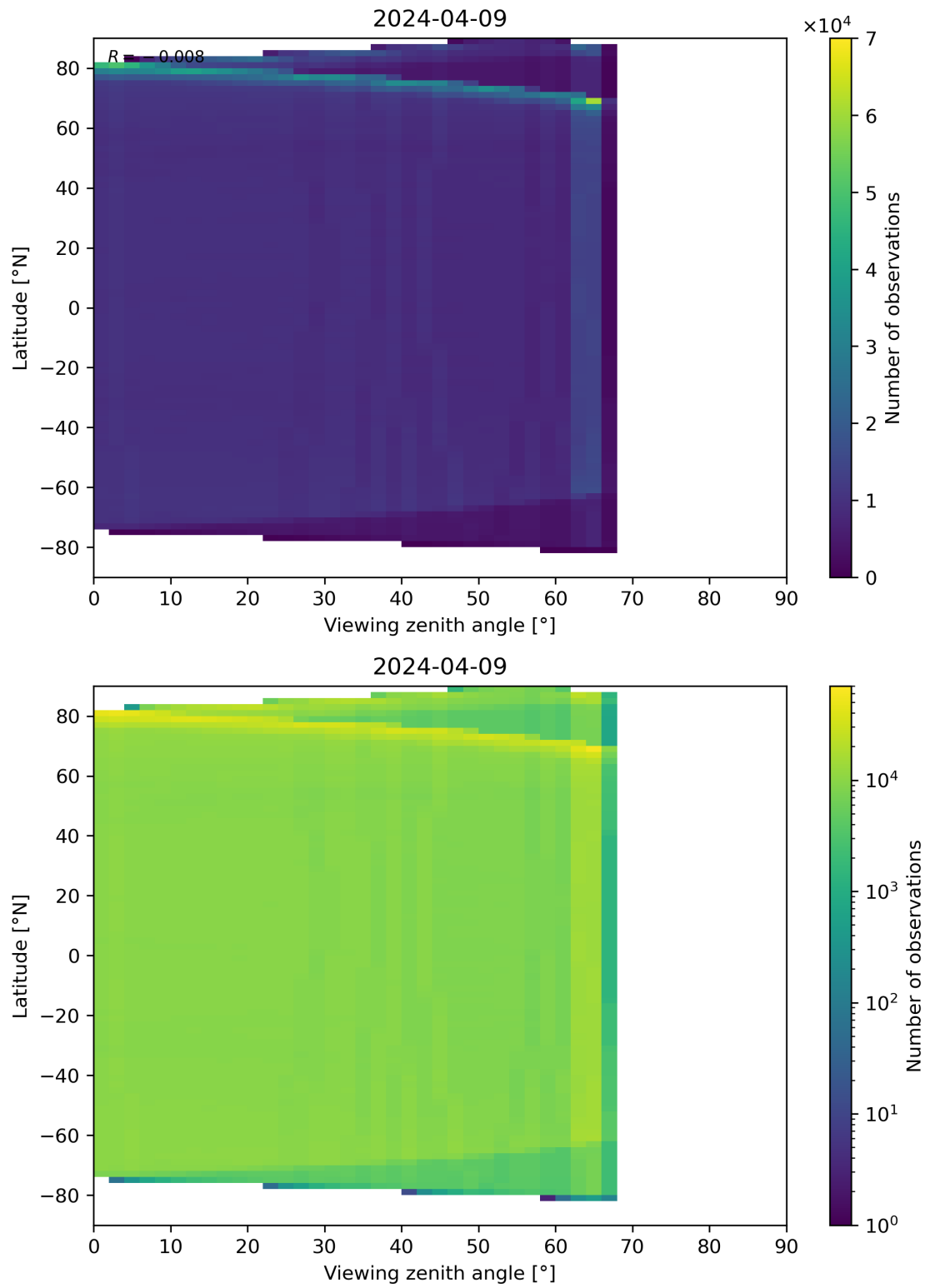
Figure 123: Scatter density plot of “Viewing zenith angle” against “Latitude” for 2024-04-08 to 2024-04-10.
