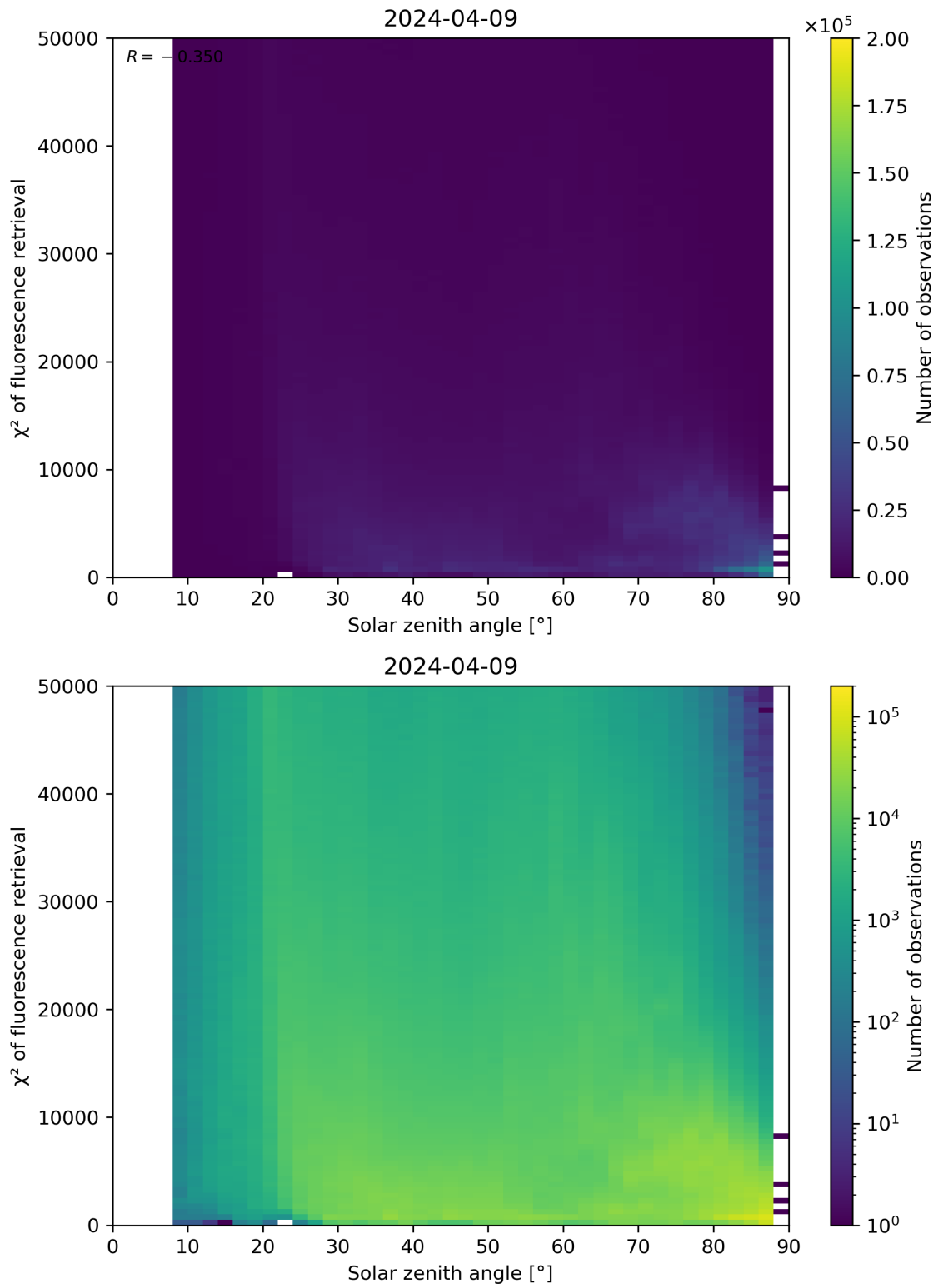
Figure 109: Scatter density plot of “Solar zenith angle” against “ \chi^2 of fluorescence retrieval” for 2024-04-08 to 2024-04-10.
