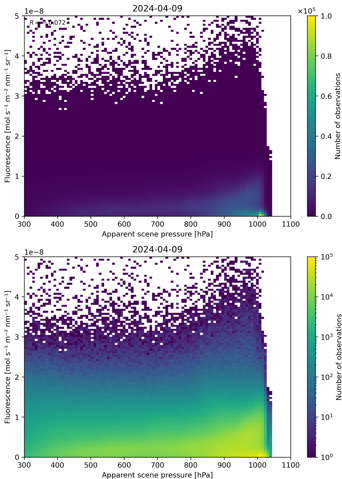
Figure 64: Scatter density plot of “Apparent scene pressure” against “Fluorescence” for 2024-04-08 to 2024-04-10.
