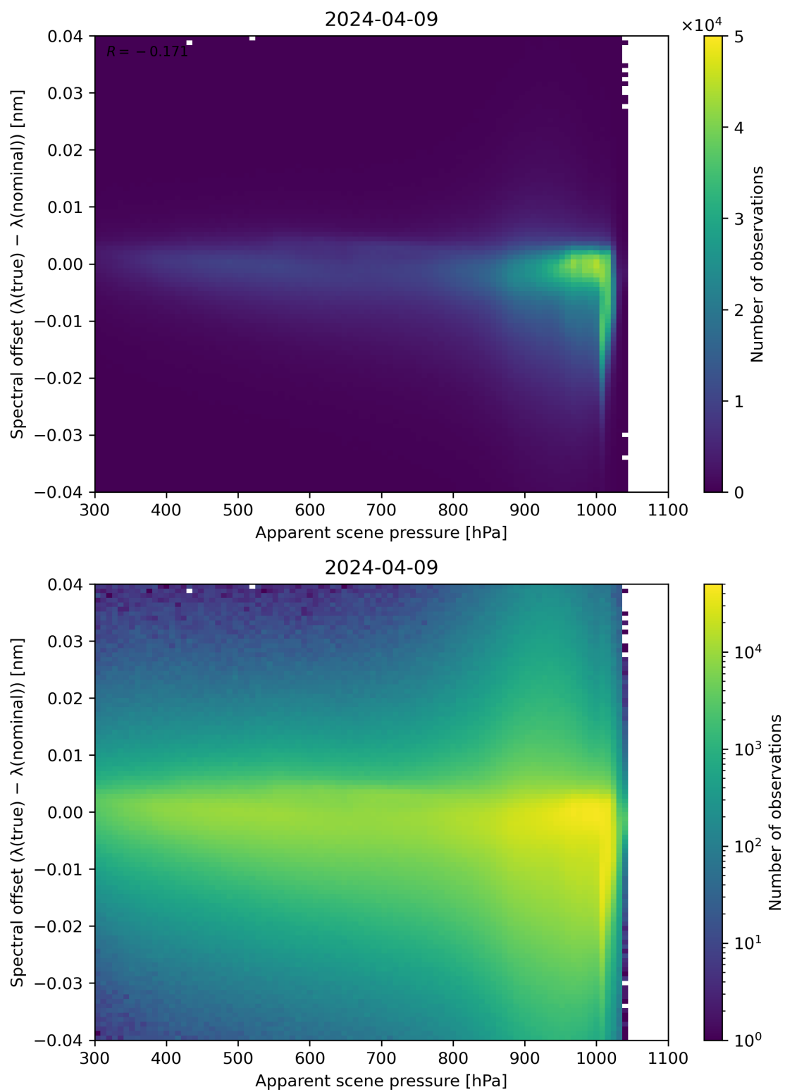
Figure 67: Scatter density plot of “Apparent scene pressure” against “Spectral offset ( \lambda(\text{true}) - \lambda(\text{nominal}) )” for 2024-04-08 to 2024-04-10.
