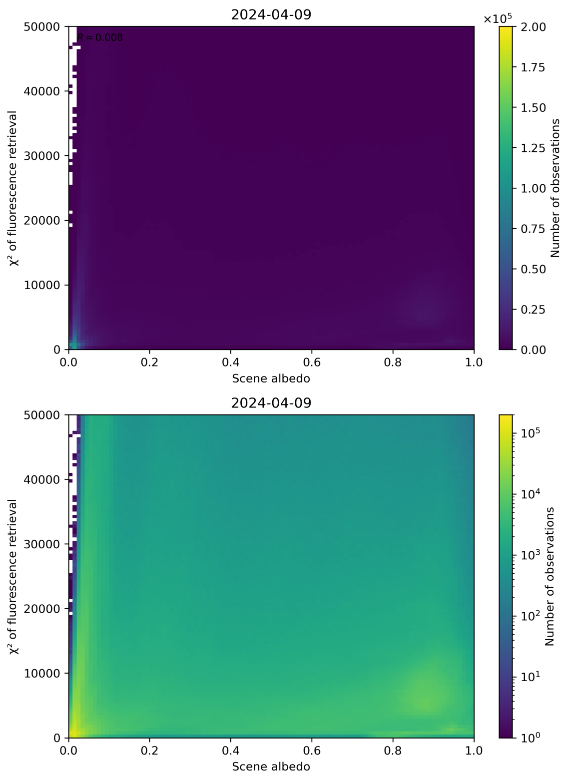
Figure 103: Scatter density plot of “Scene albedo” against “ \chi^2 of fluorescence retrieval” for 2024-04-08 to 2024-04-10.
