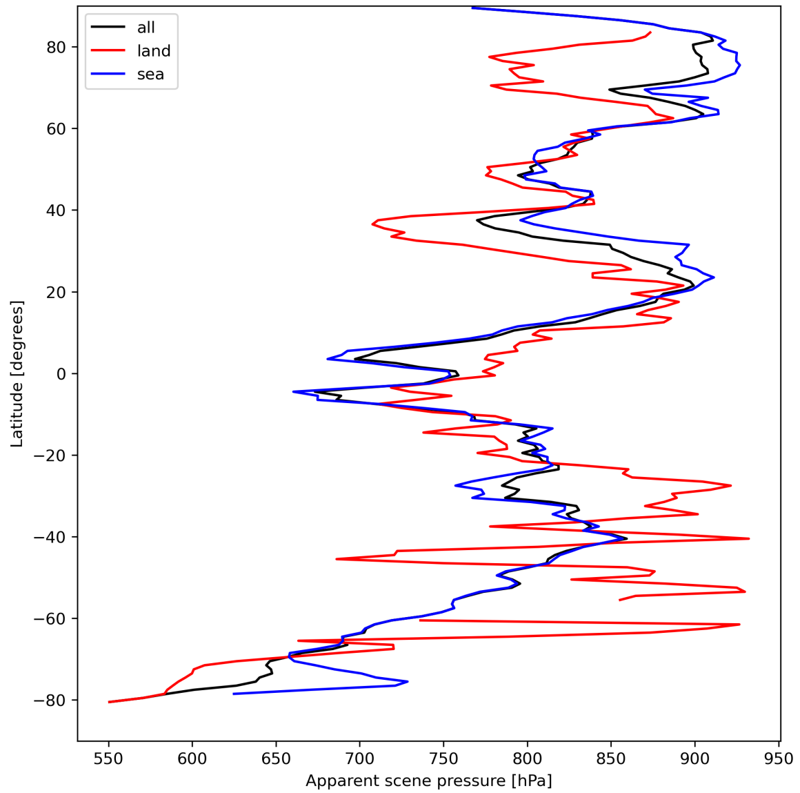
Figure 19: Zonal average of “Apparent scene pressure” for 2024-04-08 to 2024-04-10.
