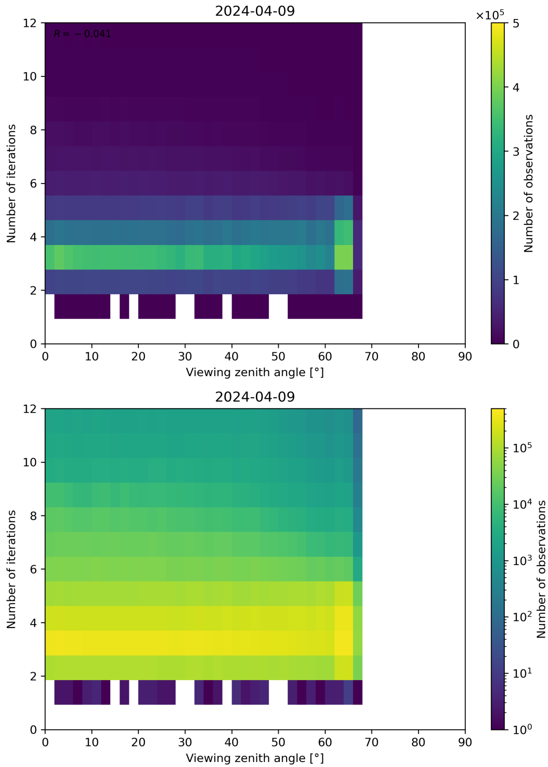
Figure 124: Scatter density plot of “Viewing zenith angle” against “Number of iterations” for 2024-04-08 to 2024-04-10.
