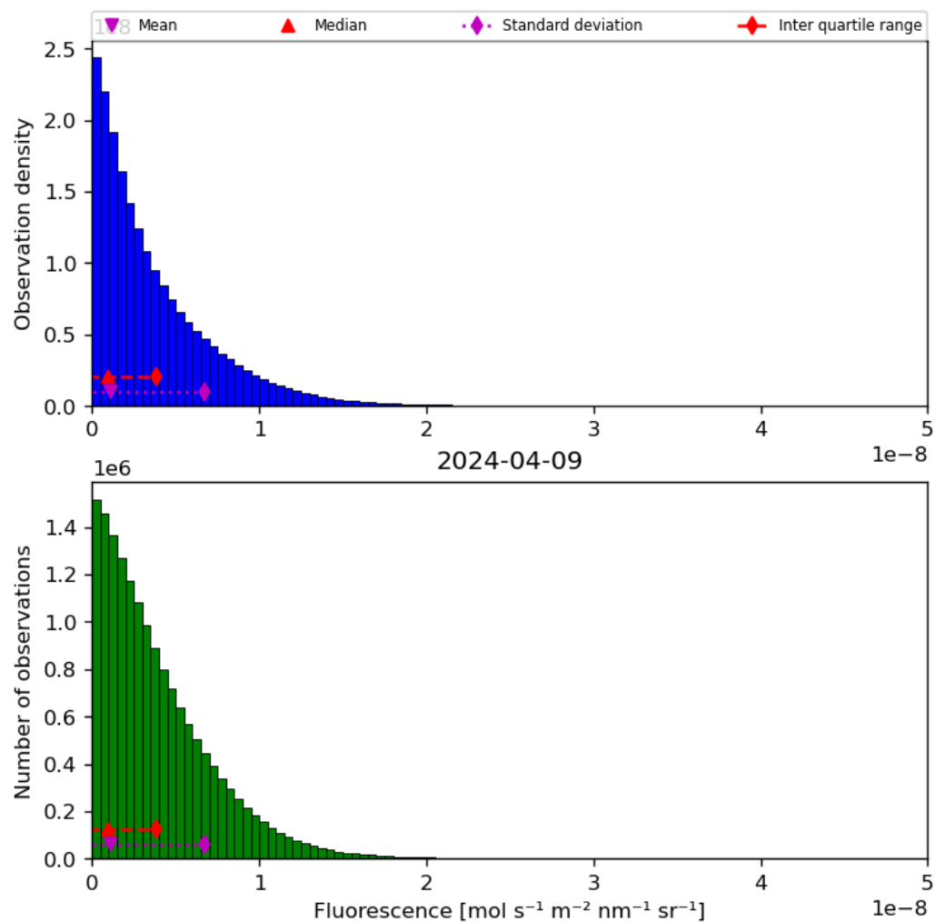
Figure 40: Histogram of “Fluorescence” for 2024-04-08 to 2024-04-10
