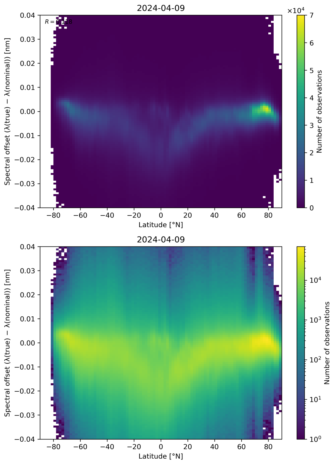
Figure 96: Scatter density plot of “Latitude” against “Spectral offset ( \lambda(\text{true}) - \lambda(\text{nominal}) )” for 2024-04-08 to 2024-04-10.
