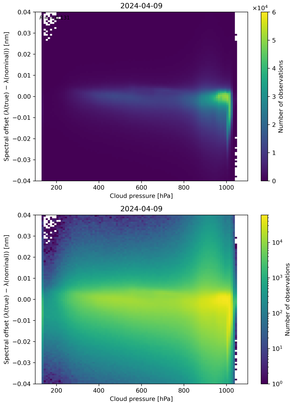
Figure 84: Scatter density plot of “Cloud pressure” against “Spectral offset ( \lambda(\text{true}) - \lambda(\text{nominal}) )” for 2024-04-08 to 2024-04-10.
