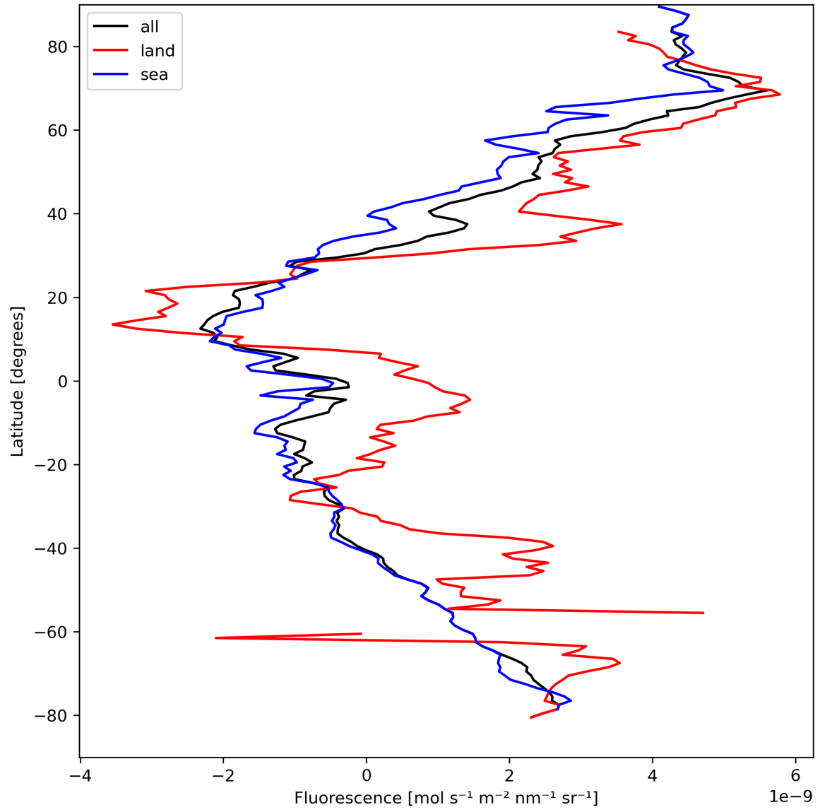
Figure 23: Zonal average of “Fluorescence” for 2024-04-08 to 2024-04-10.
