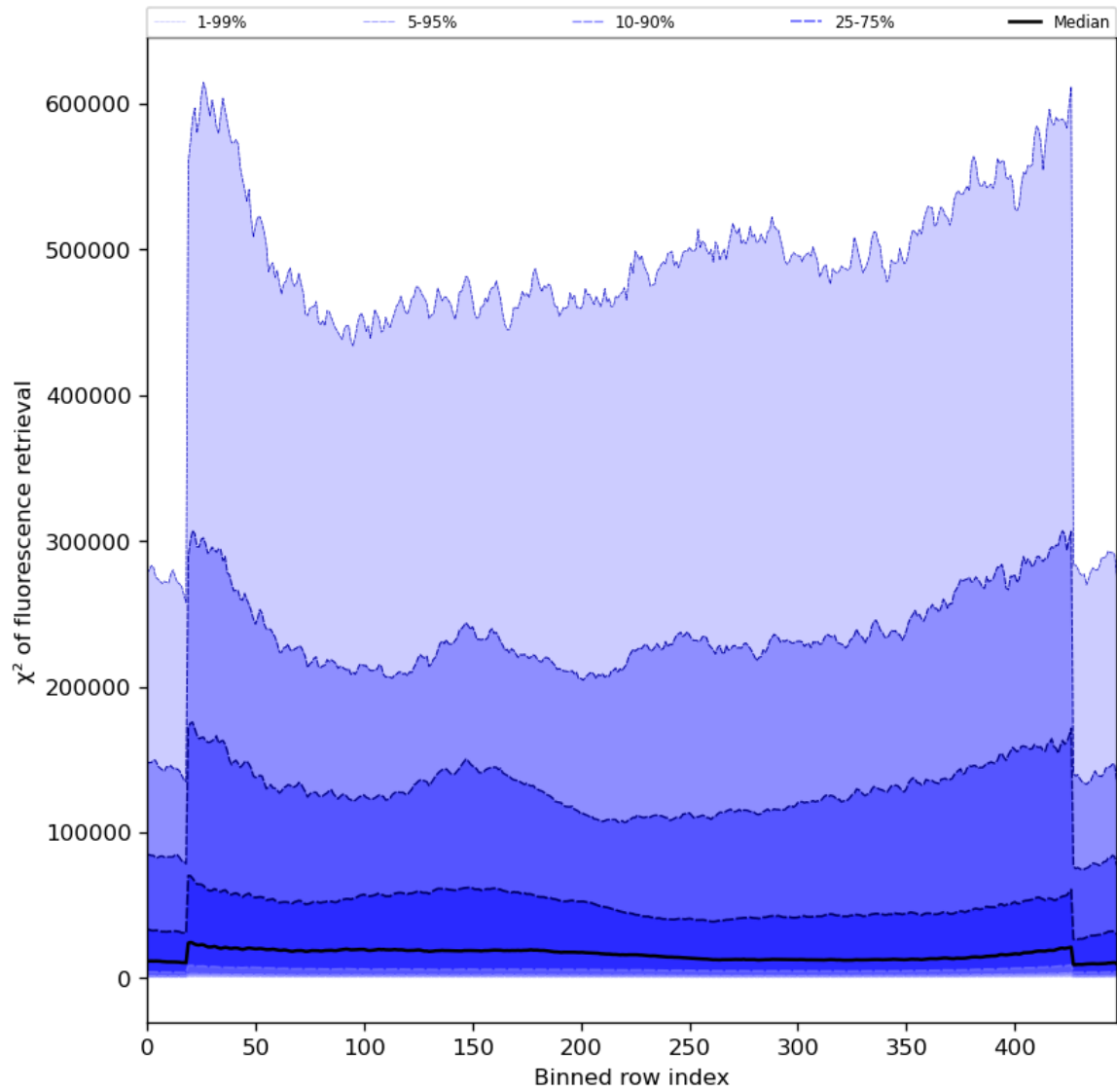
Figure 59: Along track statistics of “ \chi^2 of fluorescence retrieval” for 2024-04-08 to 2024-04-10
