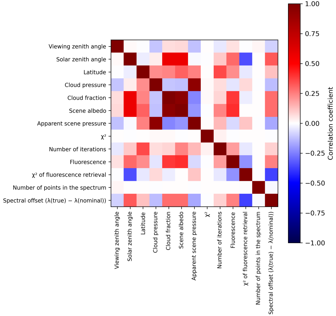
Figure 2: Map of correlation matrix for 2024-04-08 to 2024-04-10.
