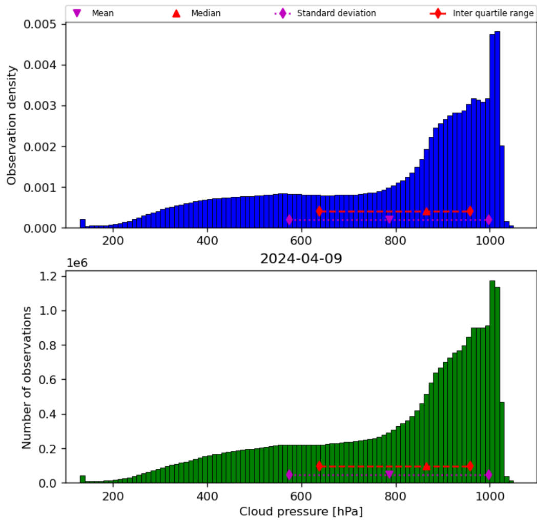
Figure 30: Histogram of “Cloud pressure” for 2024-04-08 to 2024-04-10
