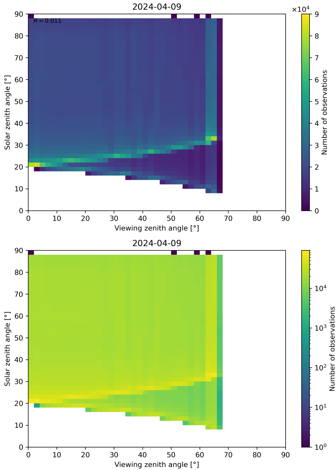
Figure 127: Scatter density plot of “Viewing zenith angle” against “Solar zenith angle” for 2024-04-08 to 2024-04-10.
