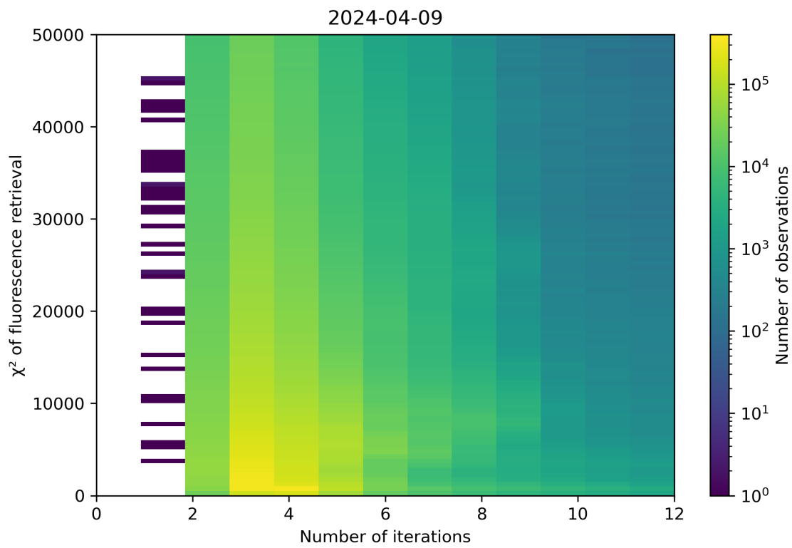
Figure 97: Scatter density plot of “Number of iterations” against “ \chi^2 of fluorescence retrieval” for 2024-04-08 to 2024-04-10.
