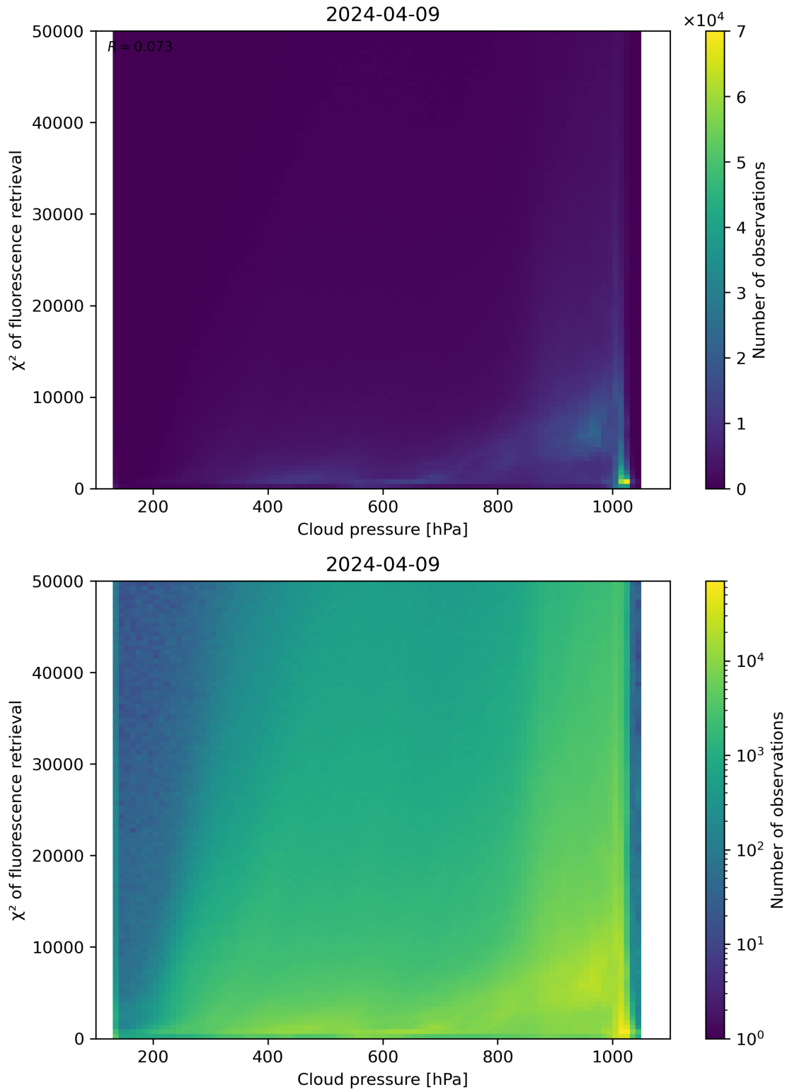
Figure 78: Scatter density plot of “Cloud pressure” against “ \chi^2 of fluorescence retrieval” for 2024-04-08 to 2024-04-10.
