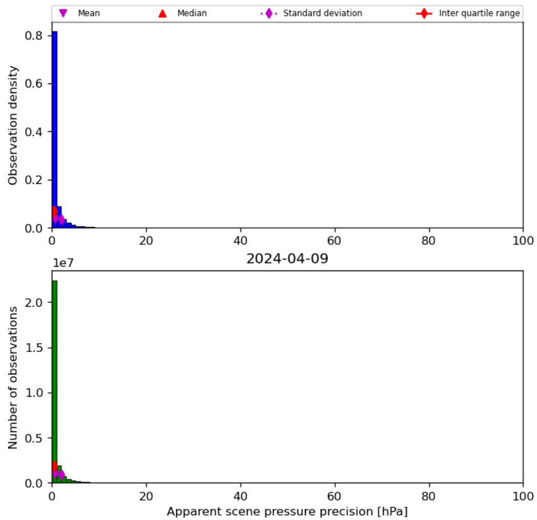
Figure 37: Histogram of “Apparent scene pressure precision” for 2024-04-08 to 2024-04-10
