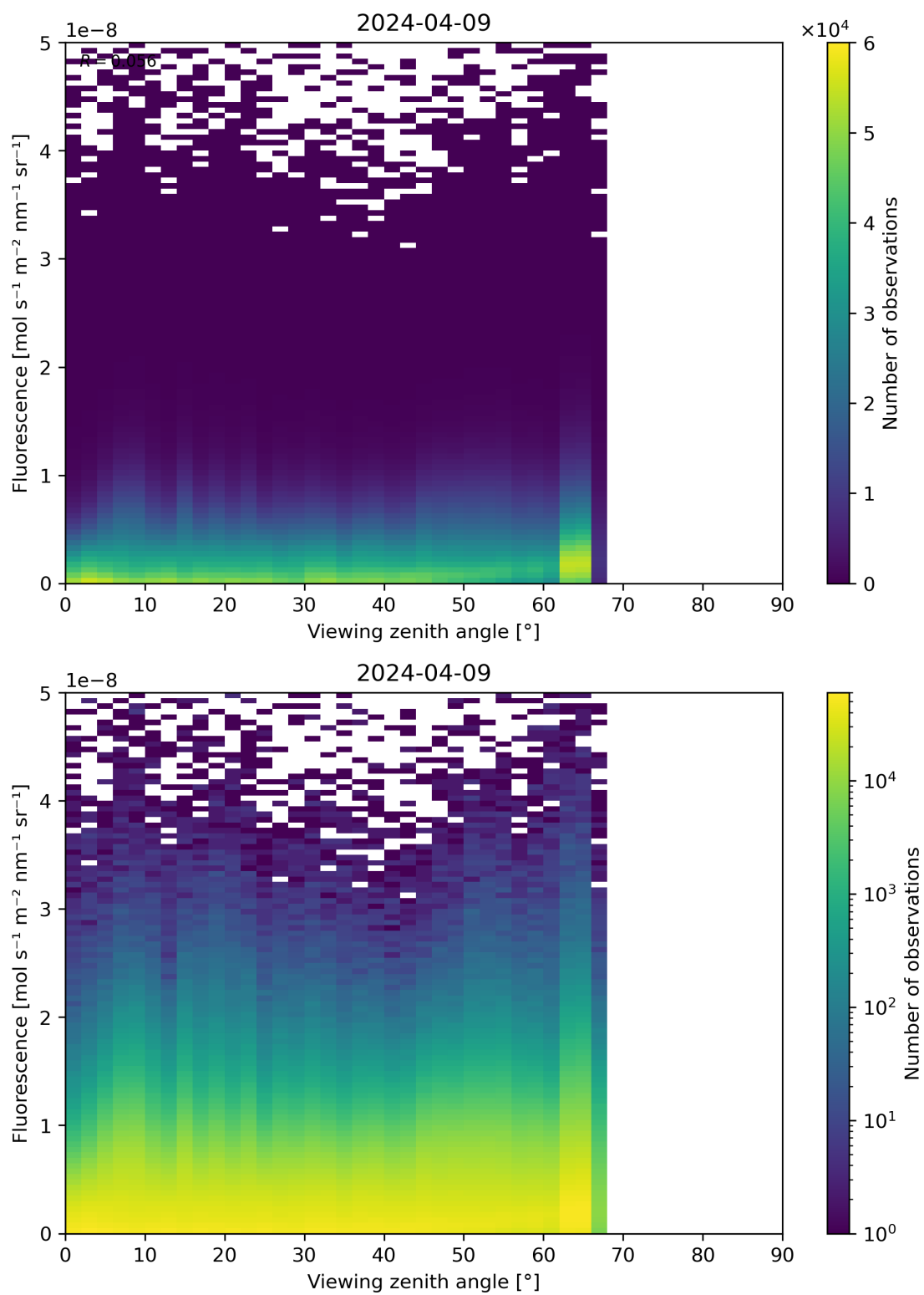
Figure 122: Scatter density plot of “Viewing zenith angle” against “Fluorescence” for 2024-04-08 to 2024-04-10.
