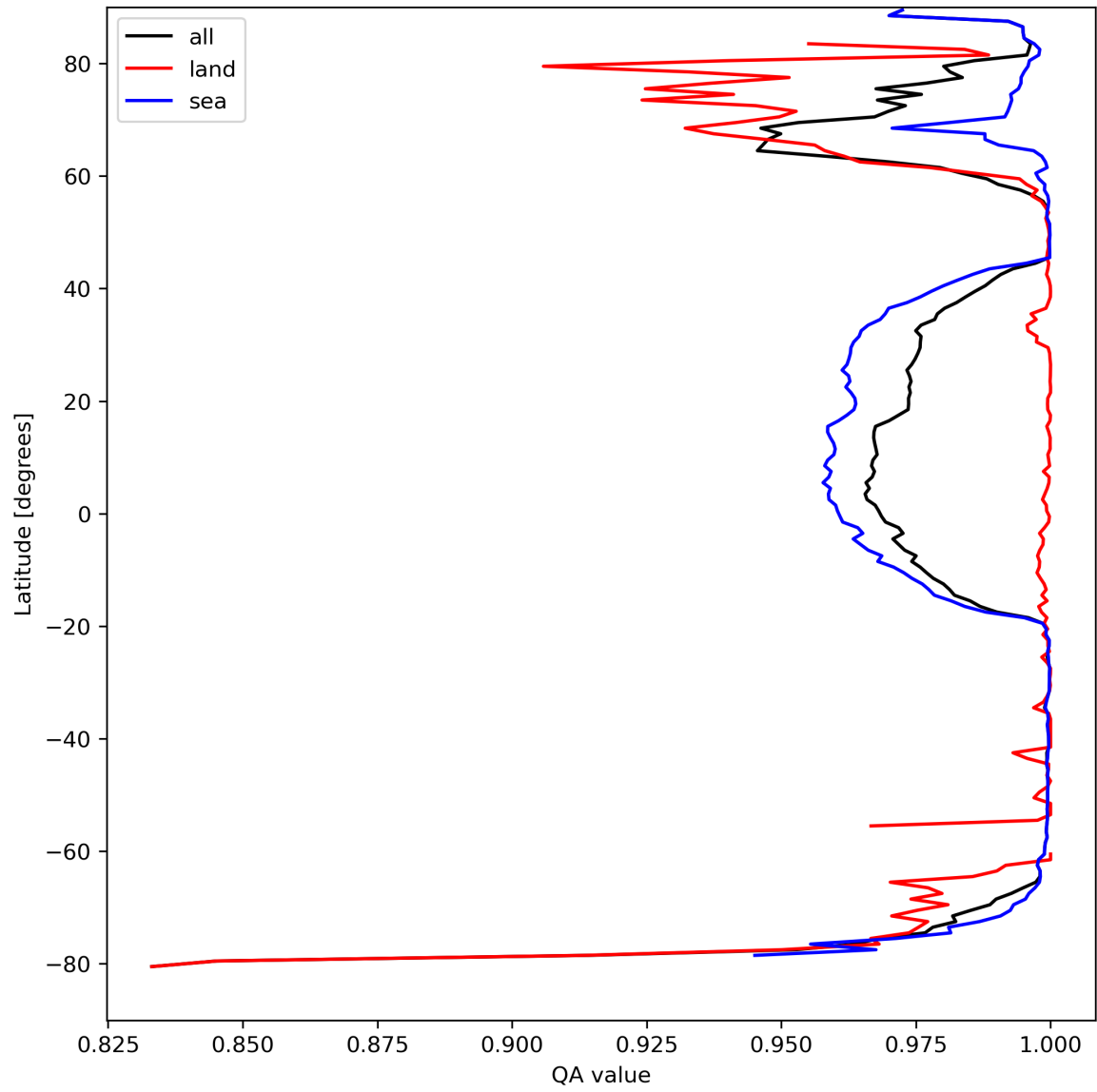
Figure 12: Zonal average of “QA value” for 2024-04-08 to 2024-04-10.
