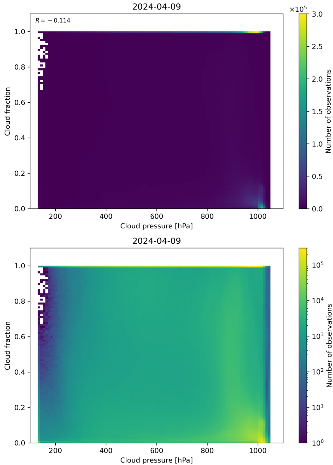
Figure 79: Scatter density plot of “Cloud pressure” against “Cloud fraction” for 2024-04-08 to 2024-04-10.
