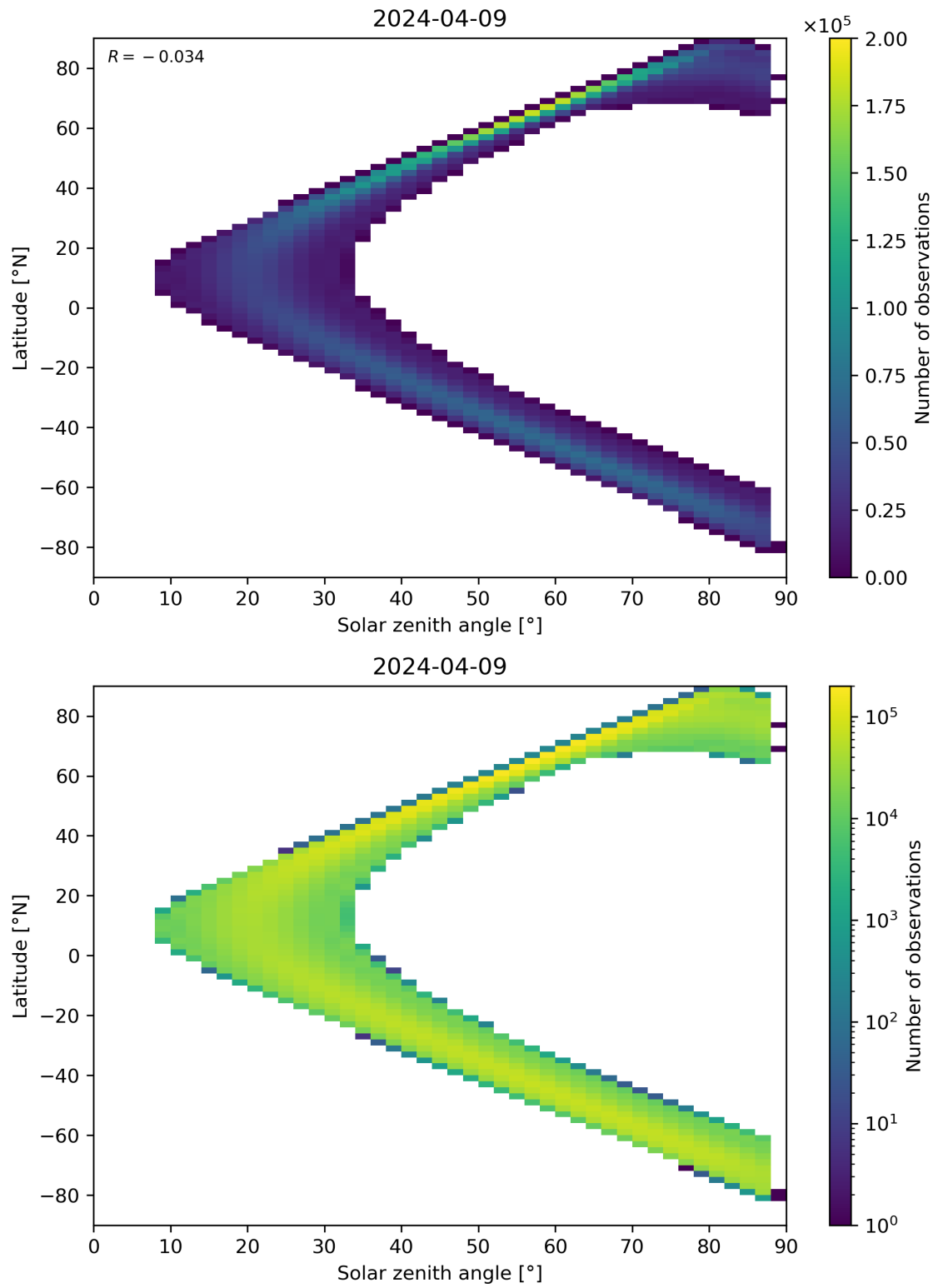
Figure 113: Scatter density plot of “Solar zenith angle” against “Latitude” for 2024-04-08 to 2024-04-10.
