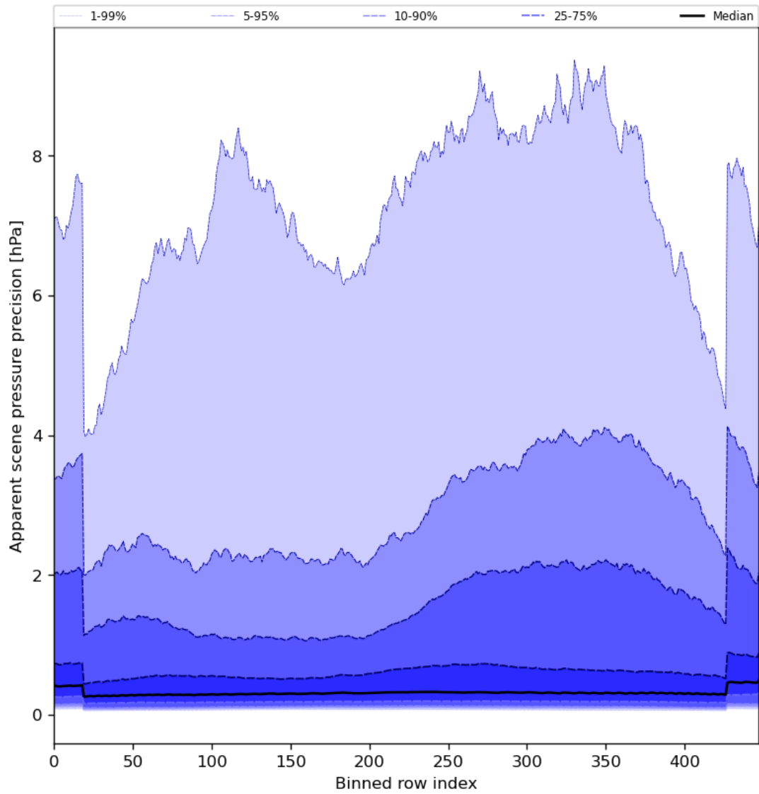
Figure 54: Along track statistics of “Apparent scene pressure precision” for 2024-04-08 to 2024-04-10
