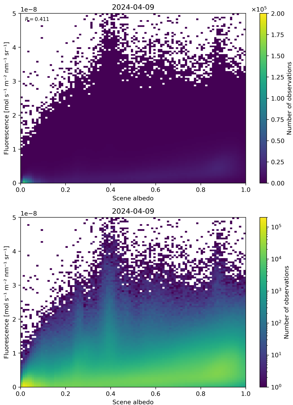
Figure 104: Scatter density plot of “Scene albedo” against “Fluorescence” for 2024-04-08 to 2024-04-10.
