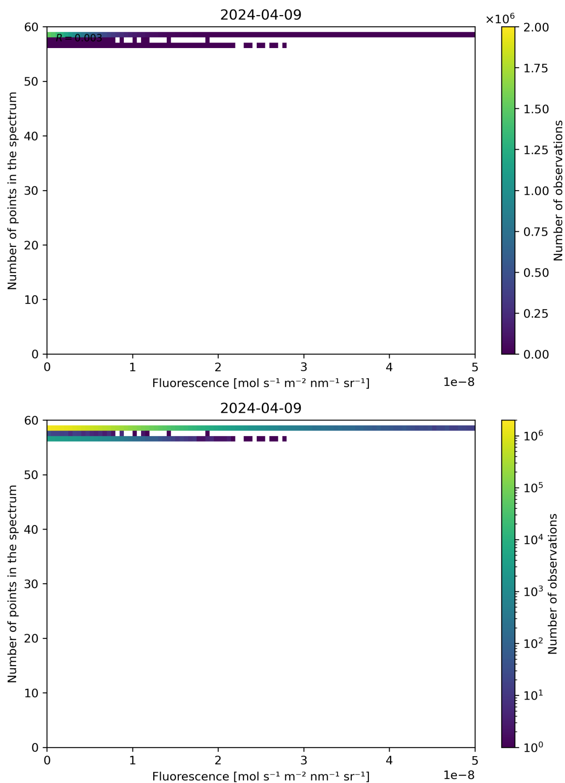
Figure 86: Scatter density plot of “Fluorescence” against “Number of points in the spectrum” for 2024-04-08 to 2024-04-10.
