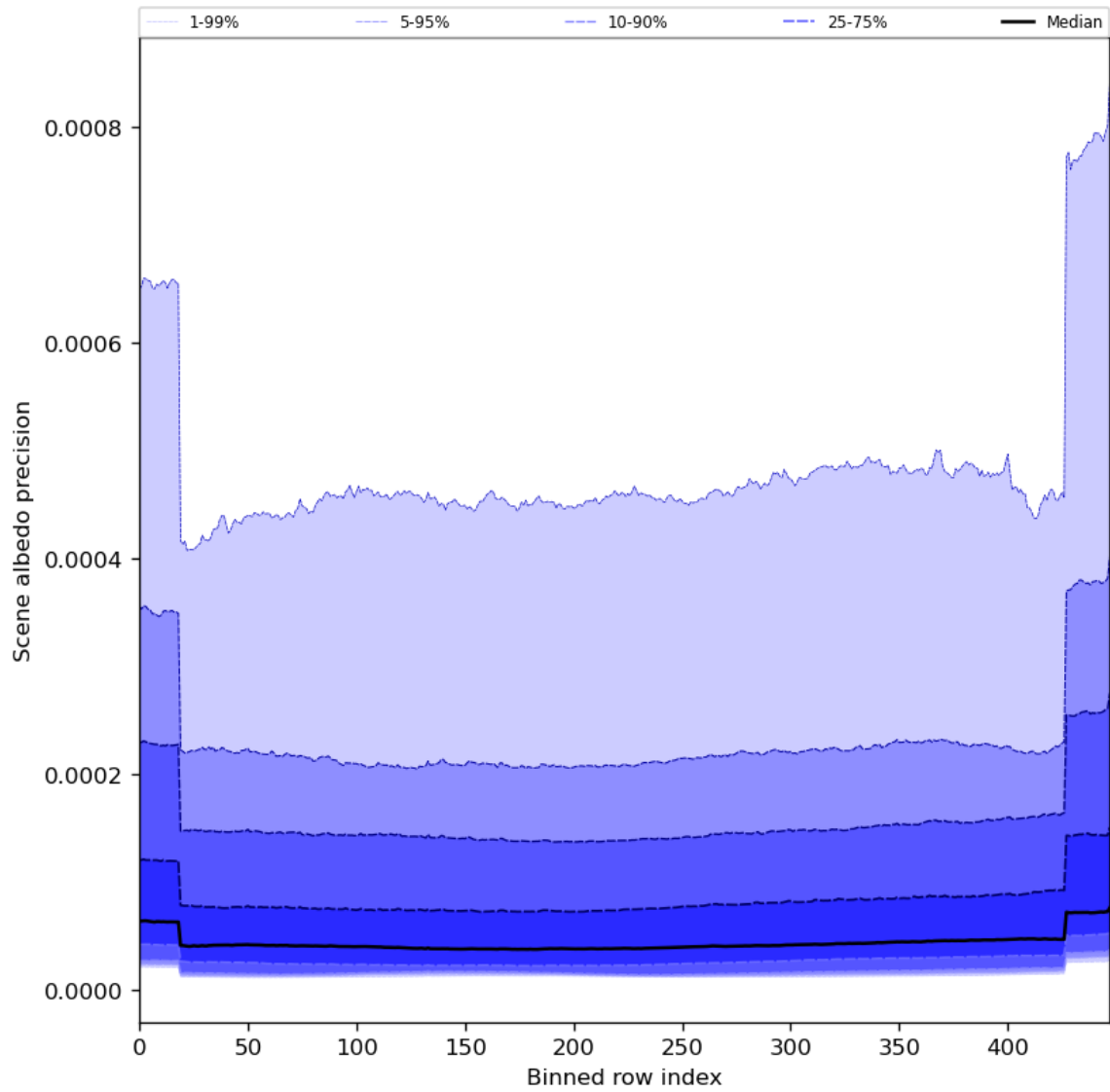
Figure 52: Along track statistics of “Scene albedo precision” for 2024-04-08 to 2024-04-10
