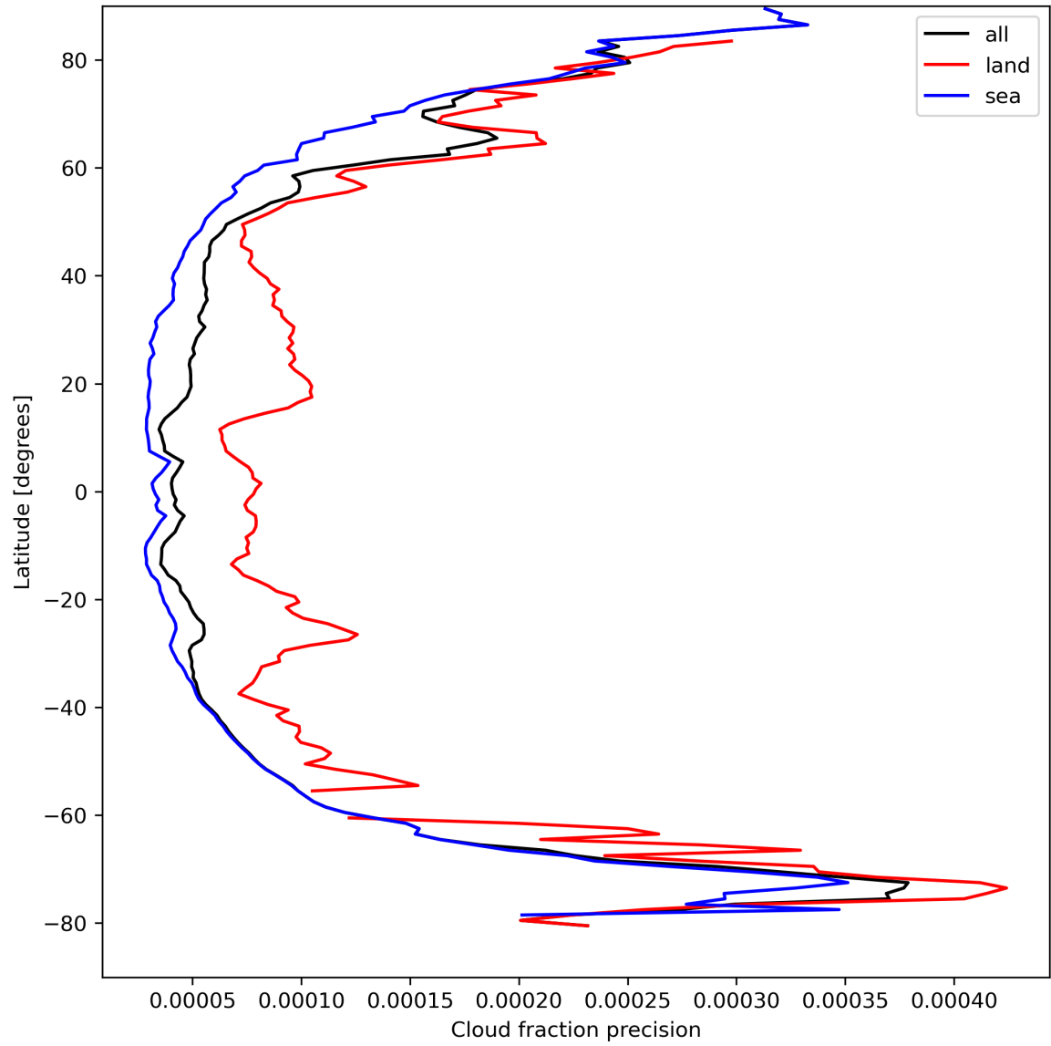
Figure 16: Zonal average of “Cloud fraction precision” for 2024-04-08 to 2024-04-10.
