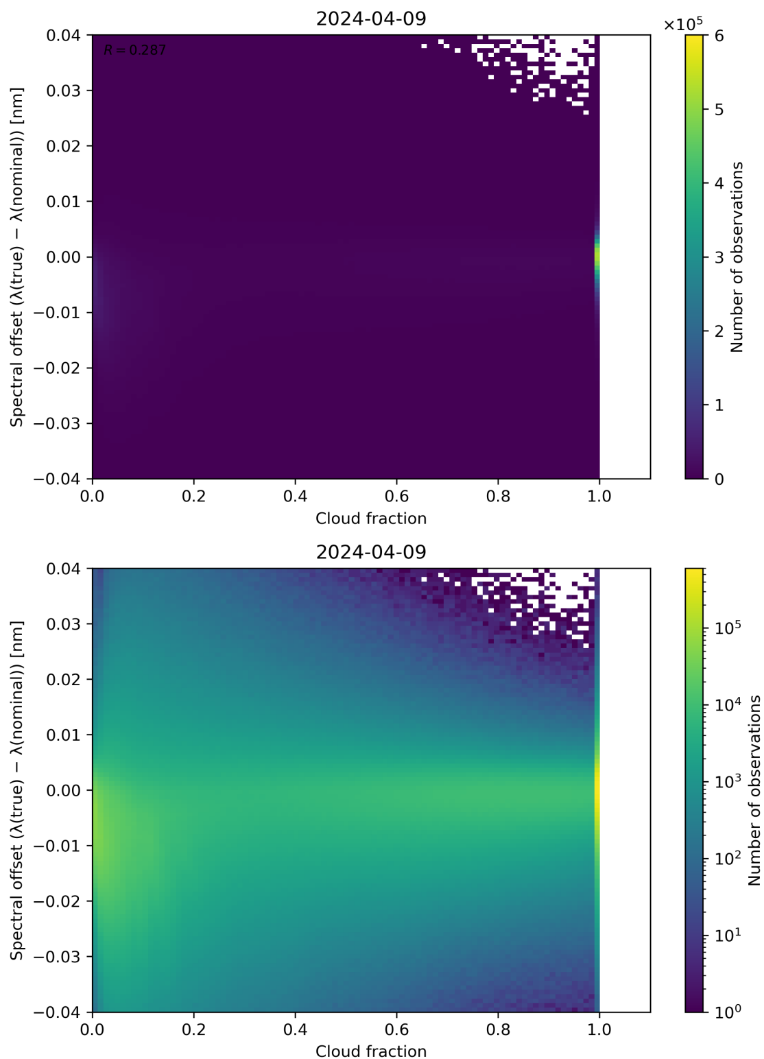
Figure 76: Scatter density plot of “Cloud fraction” against “Spectral offset ( \lambda(\text{true}) - \lambda(\text{nominal}) )” for 2024-04-08 to 2024-04-10.
