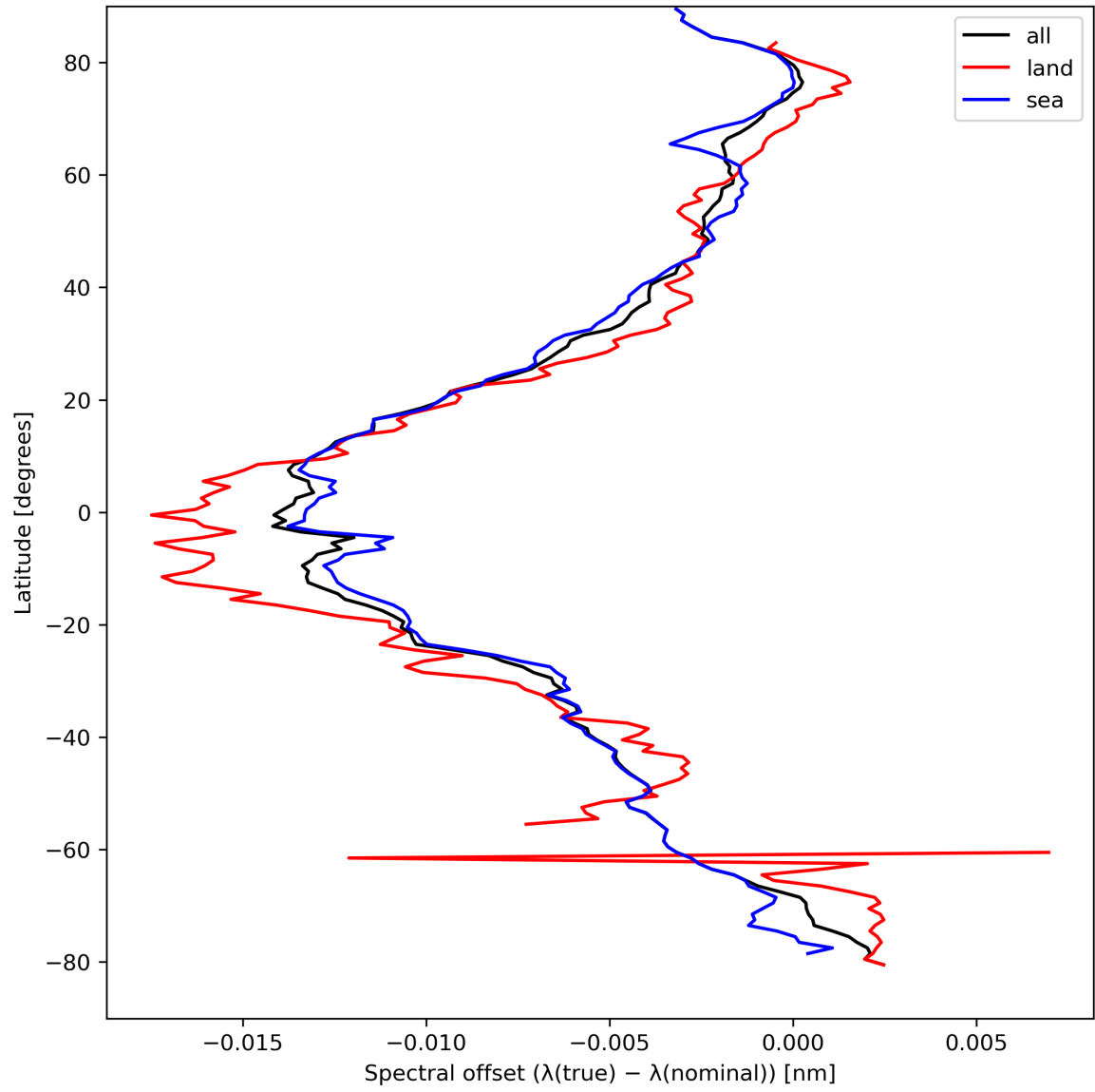
Figure 28: Zonal average of “Spectral offset ( \lambda(\text{true}) - \lambda(\text{nominal}) )” for 2024-04-08 to 2024-04-10.
