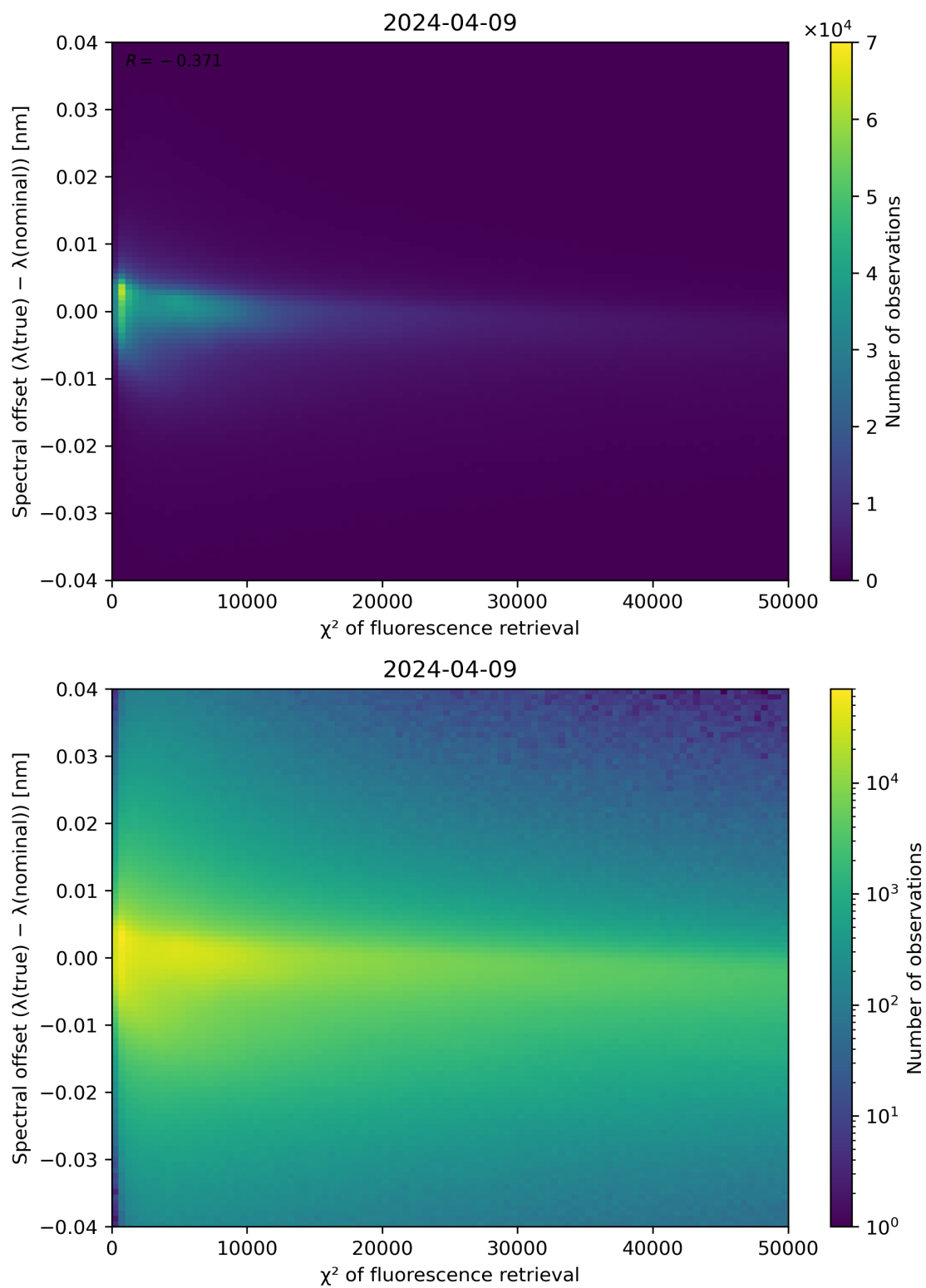
Figure 69: Scatter density plot of " \chi^2 of fluorescence retrieval" against "Spectral offset ( \lambda(\text{true}) - \lambda(\text{nominal}) )" for 2024-04-08 to 2024-04-10.
