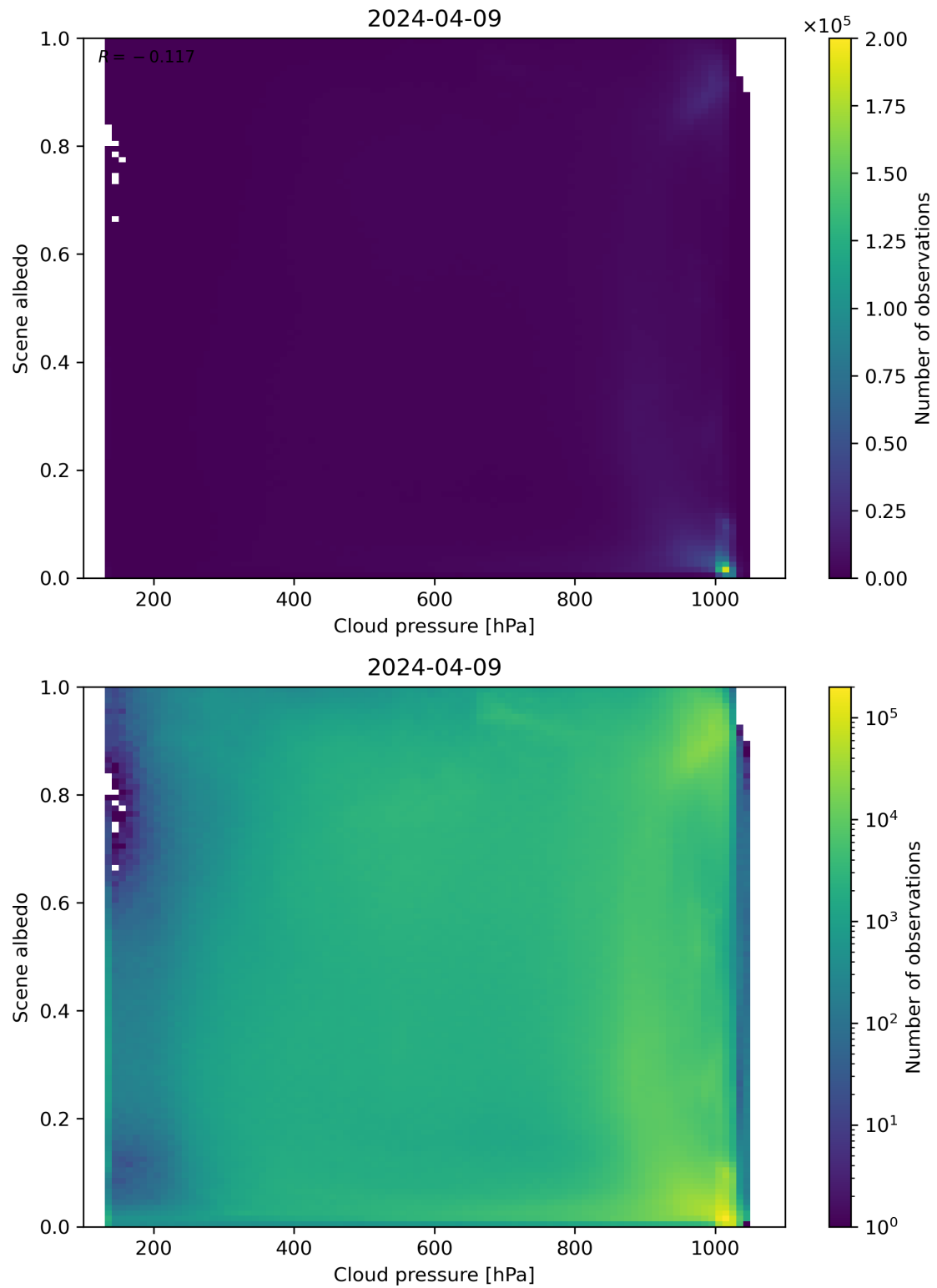
Figure 83: Scatter density plot of “Cloud pressure” against “Scene albedo” for 2024-04-08 to 2024-04-10.
