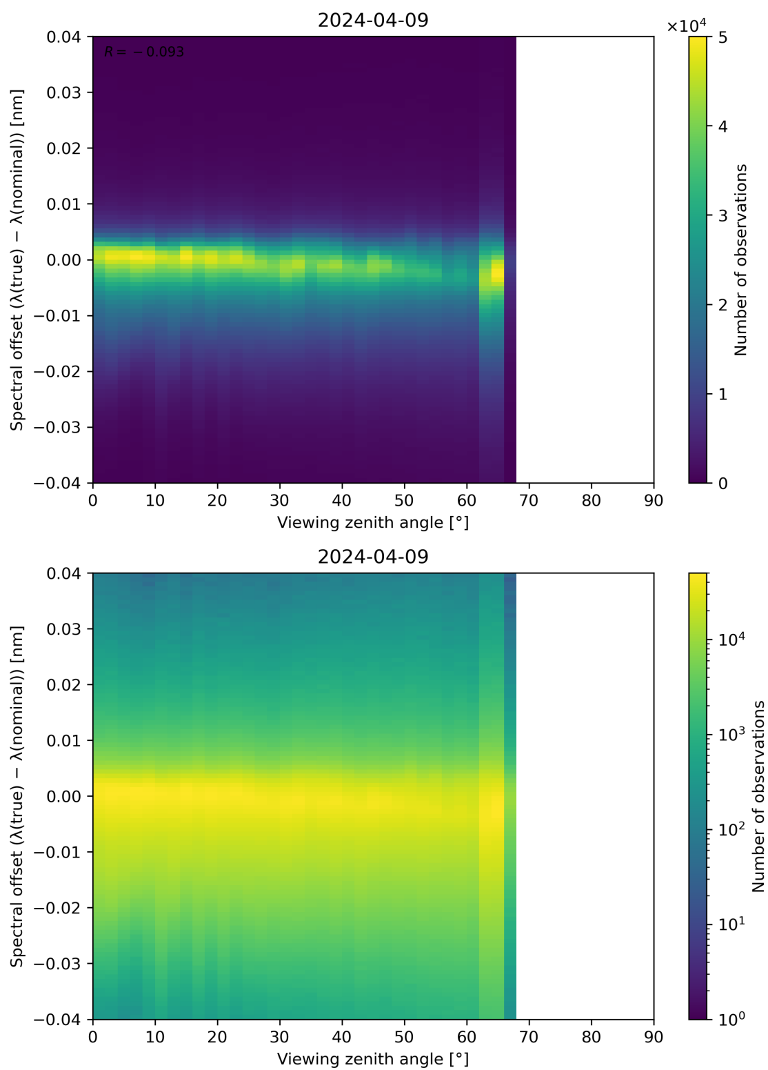
Figure 128: Scatter density plot of “Viewing zenith angle” against “Spectral offset ( \lambda(\text{true}) - \lambda(\text{nominal}) )” for 2024-04-08 to 2024-04-10.
