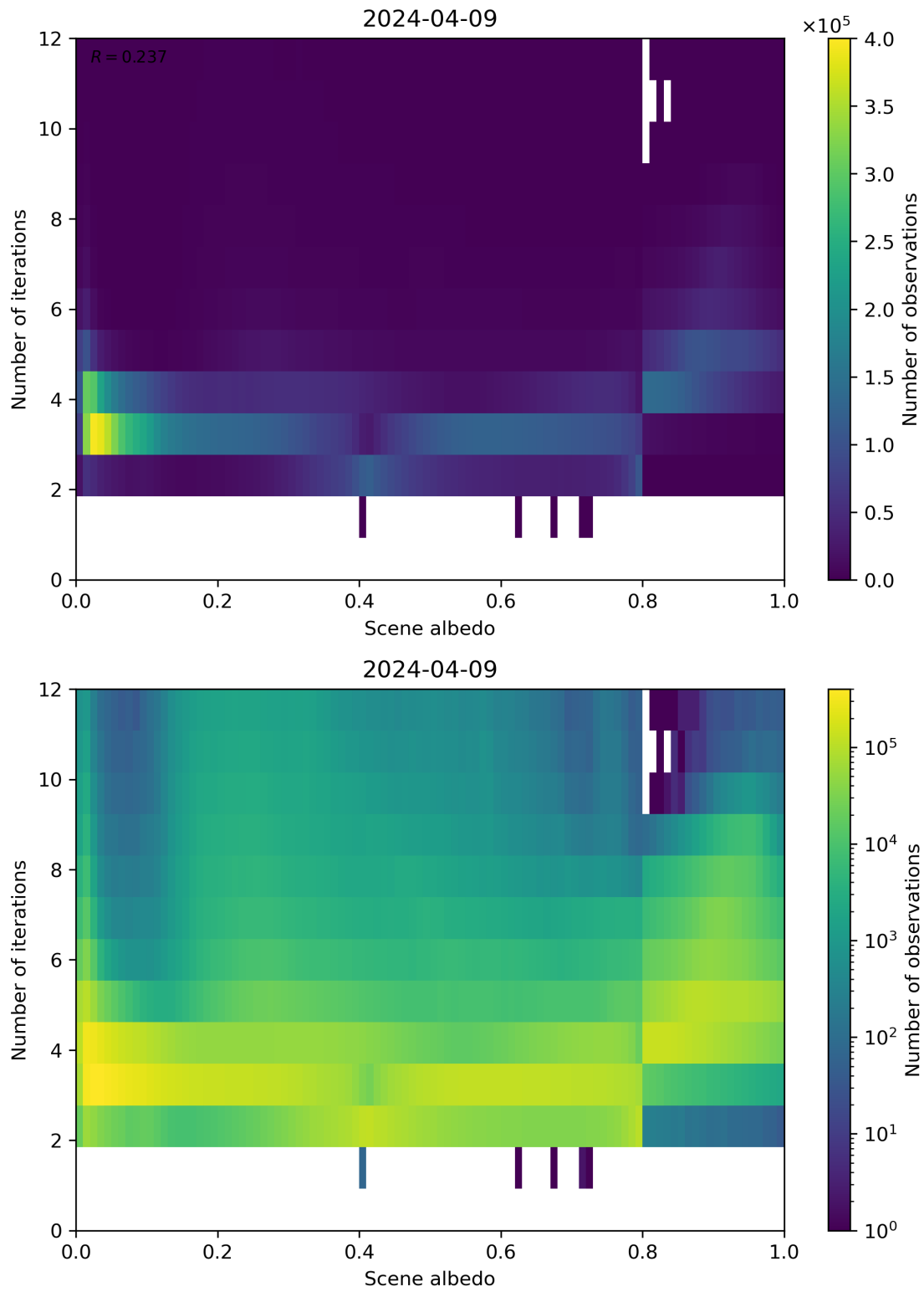
Figure 105: Scatter density plot of “Scene albedo” against “Number of iterations” for 2024-04-08 to 2024-04-10.
