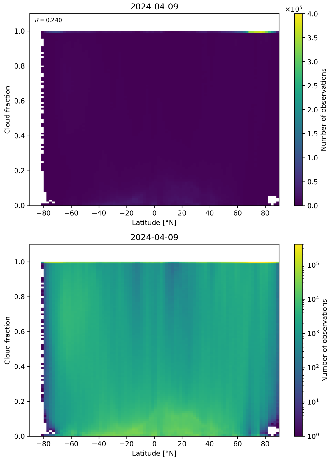
Figure 90: Scatter density plot of “Latitude” against “Cloud fraction” for 2024-04-08 to 2024-04-10.
