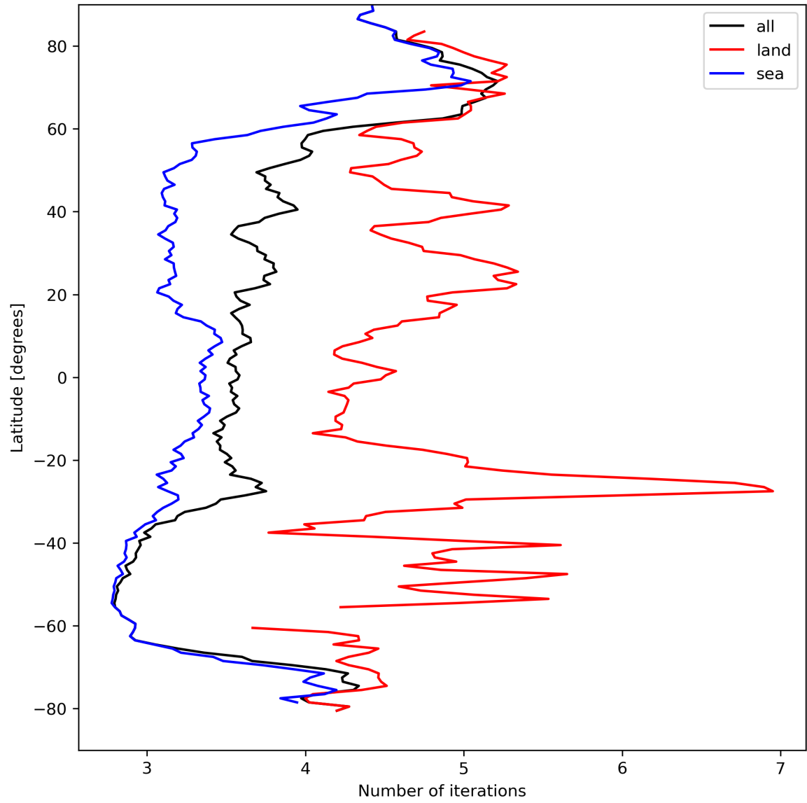
Figure 22: Zonal average of “Number of iterations” for 2024-04-08 to 2024-04-10.
