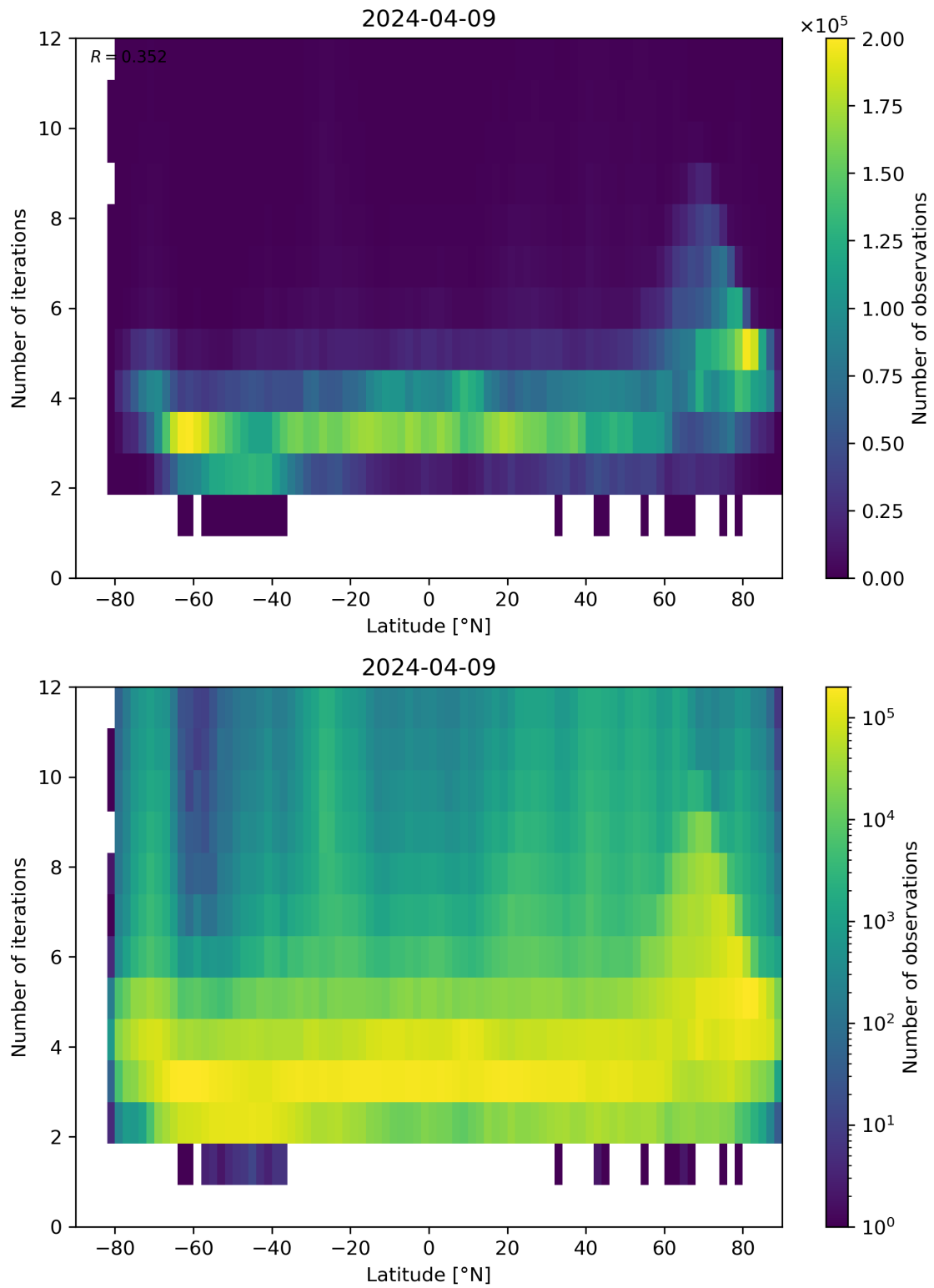
Figure 93: Scatter density plot of “Latitude” against “Number of iterations” for 2024-04-08 to 2024-04-10.
