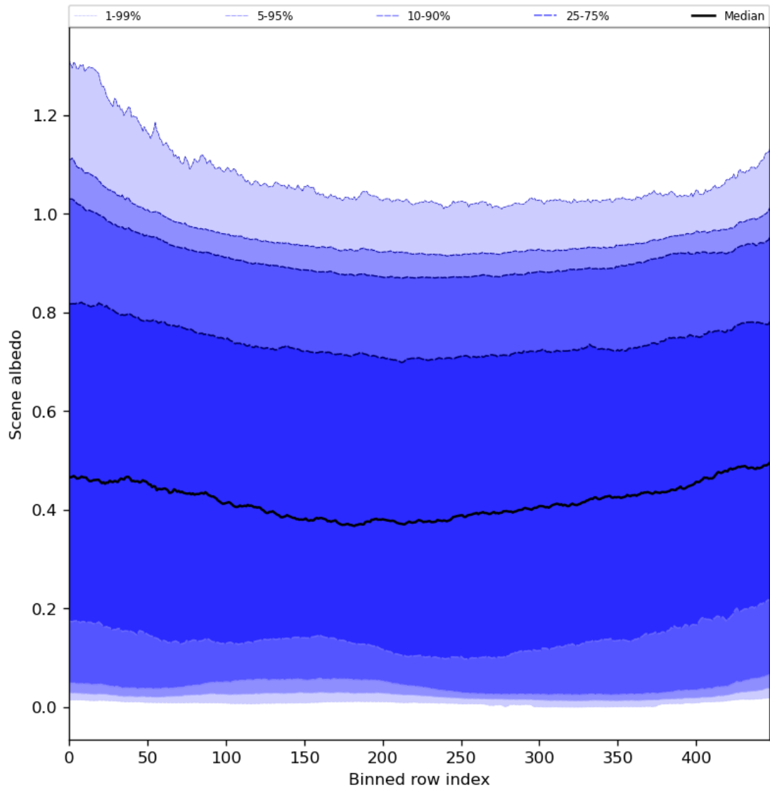
Figure 51: Along track statistics of “Scene albedo” for 2024-04-08 to 2024-04-10
