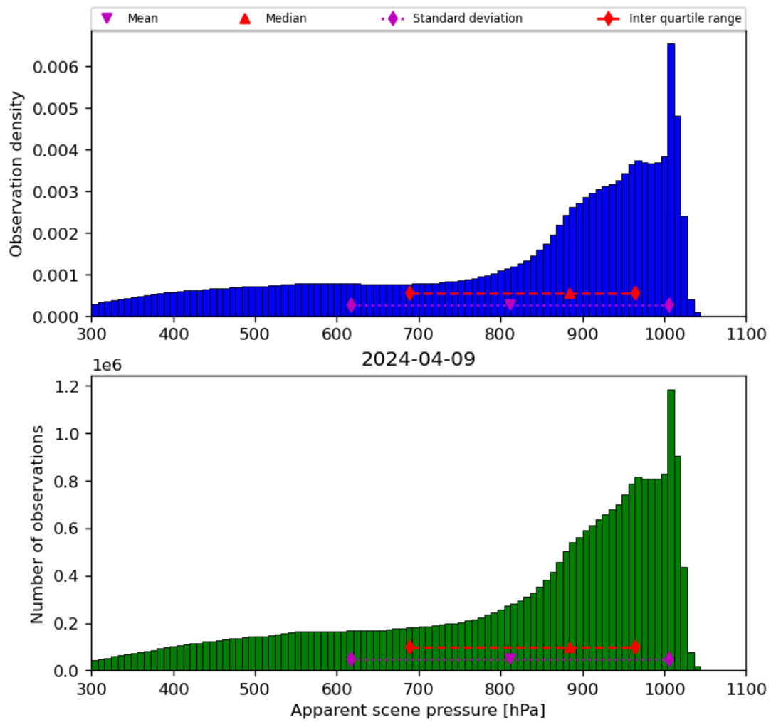
Figure 36: Histogram of “Apparent scene pressure” for 2024-04-08 to 2024-04-10
