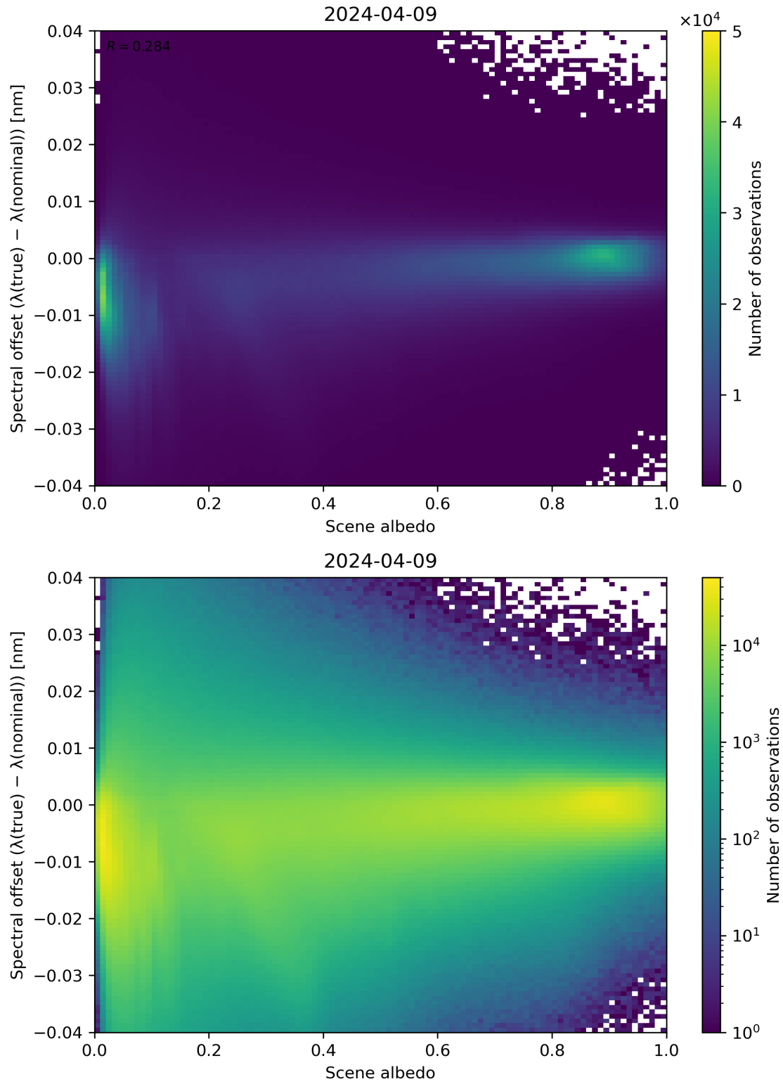
Figure 107: Scatter density plot of “Scene albedo” against “Spectral offset ( \lambda(\text{true}) - \lambda(\text{nominal}) )” for 2024-04-08 to 2024-04-10.
