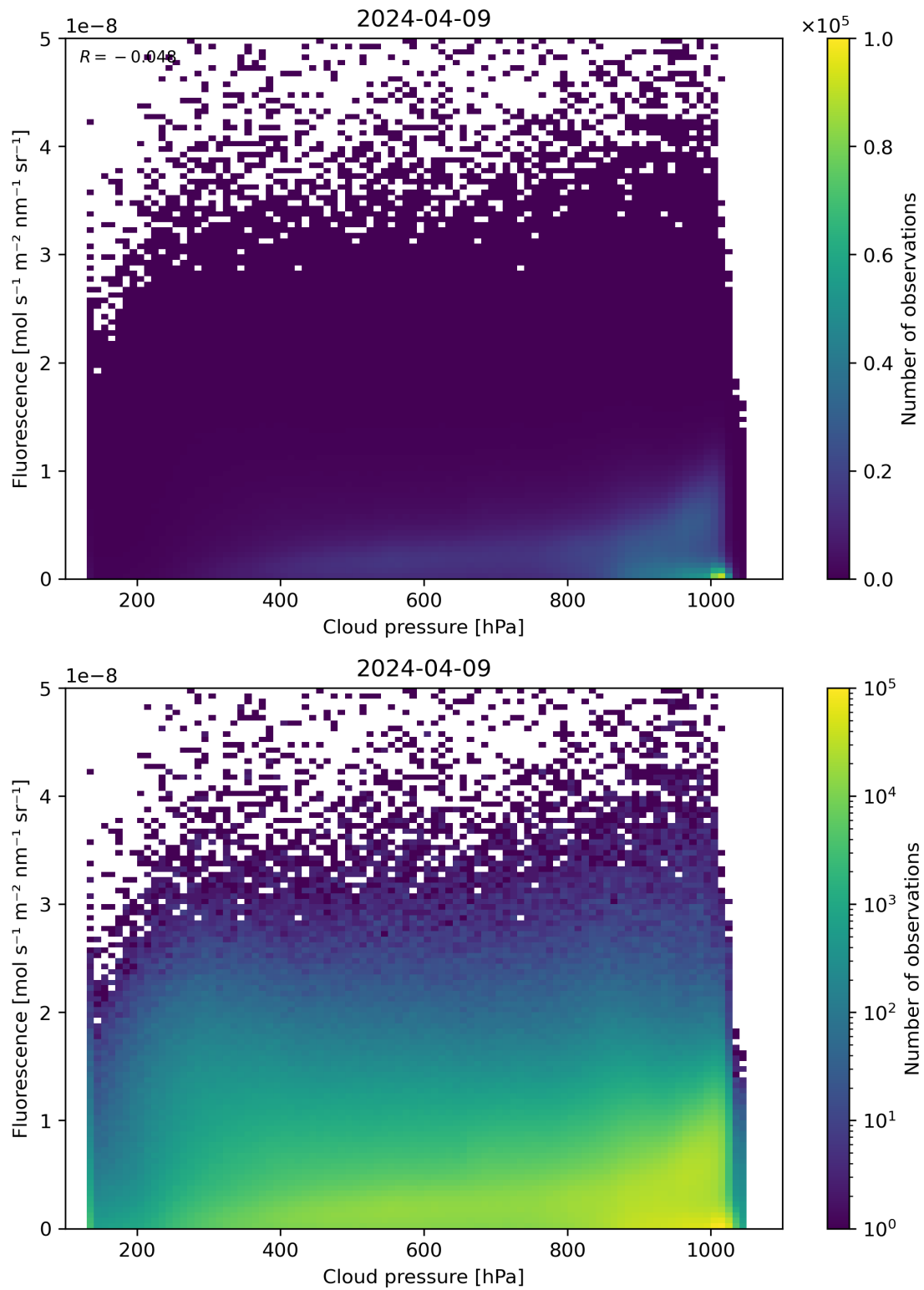
Figure 80: Scatter density plot of “Cloud pressure” against “Fluorescence” for 2024-04-08 to 2024-04-10.
