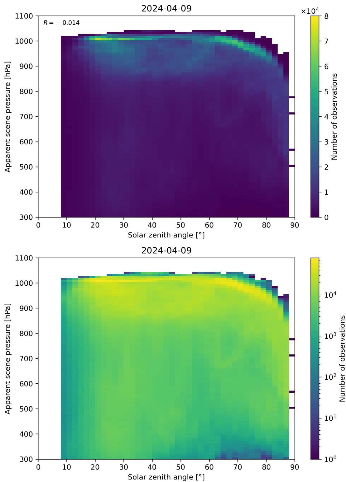
Figure 108: Scatter density plot of “Solar zenith angle” against “Apparent scene pressure” for 2024-04-08 to 2024-04-10.
