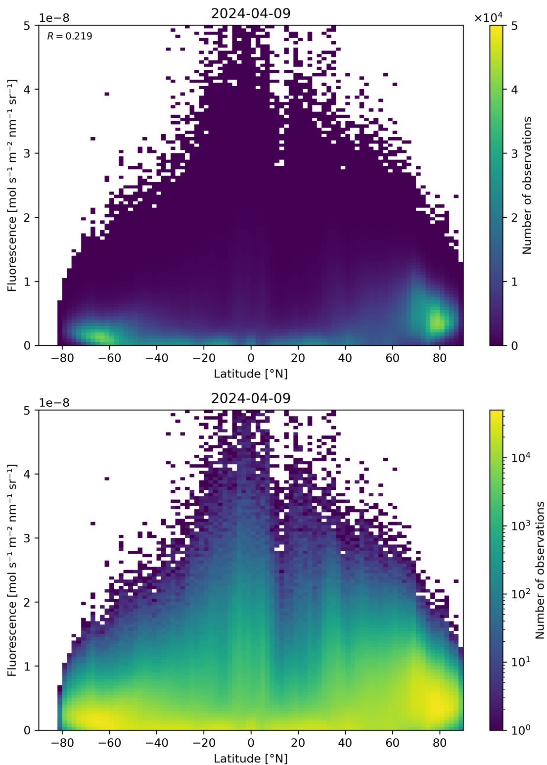
Figure 92: Scatter density plot of “Latitude” against “Fluorescence” for 2024-04-08 to 2024-04-10.
