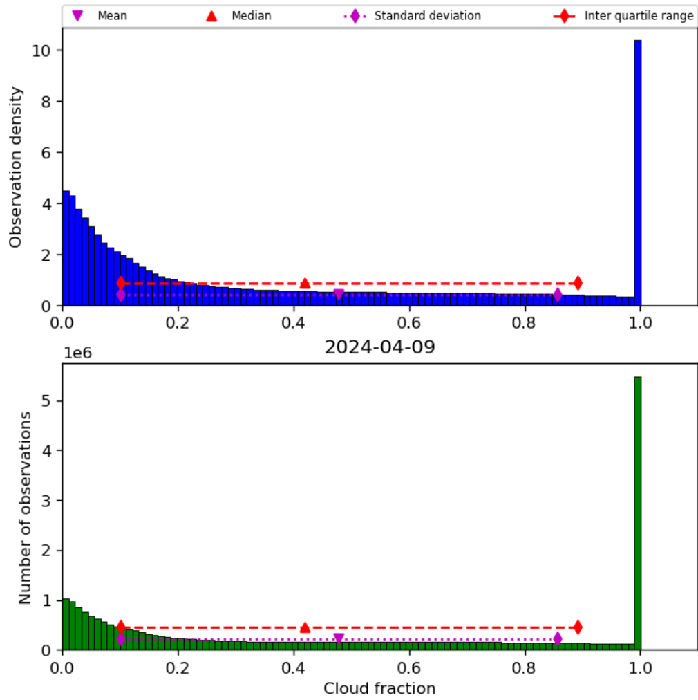
Figure 32: Histogram of “Cloud fraction” for 2024-04-08 to 2024-04-10
