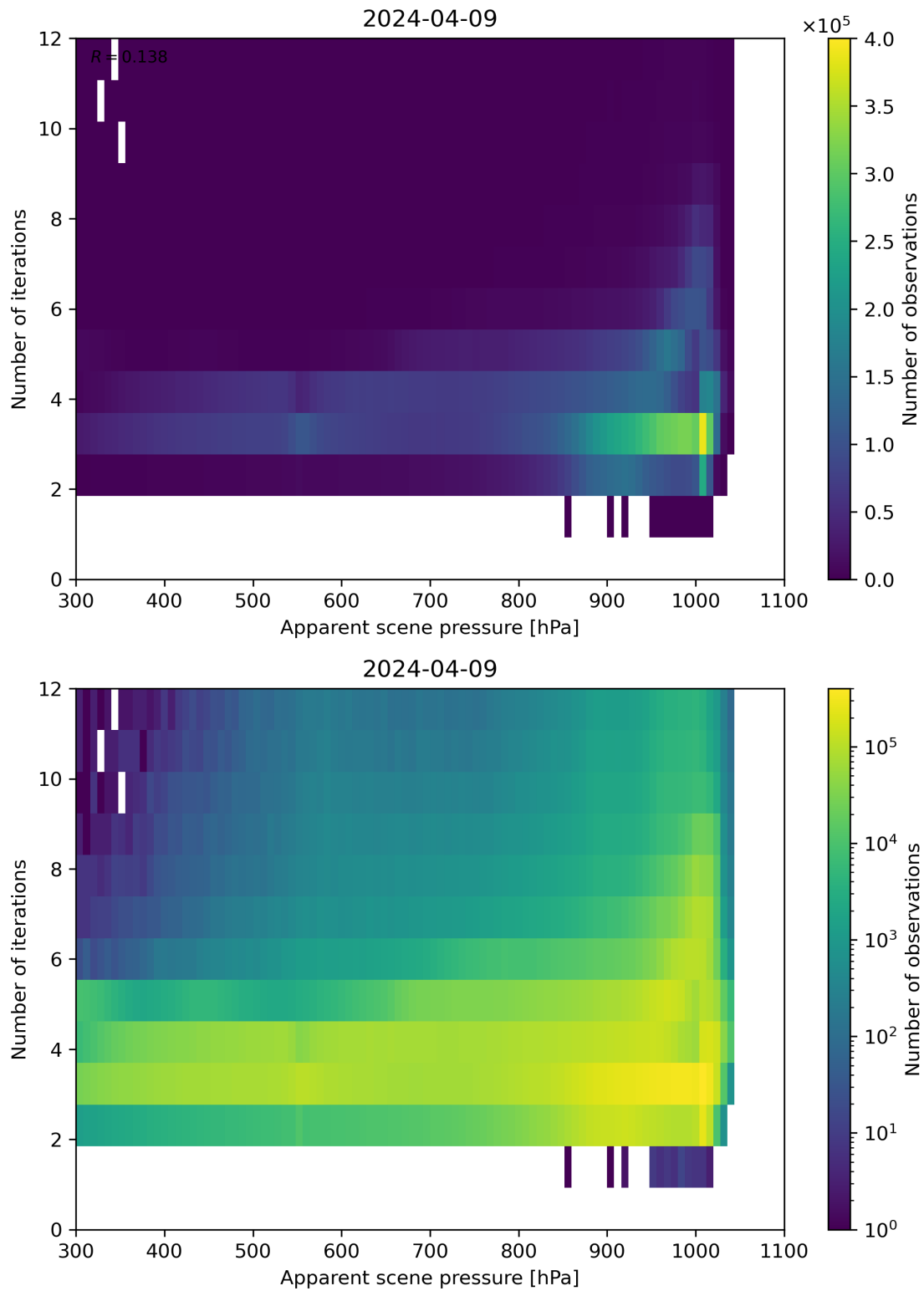
Figure 65: Scatter density plot of “Apparent scene pressure” against “Number of iterations” for 2024-04-08 to 2024-04-10.
