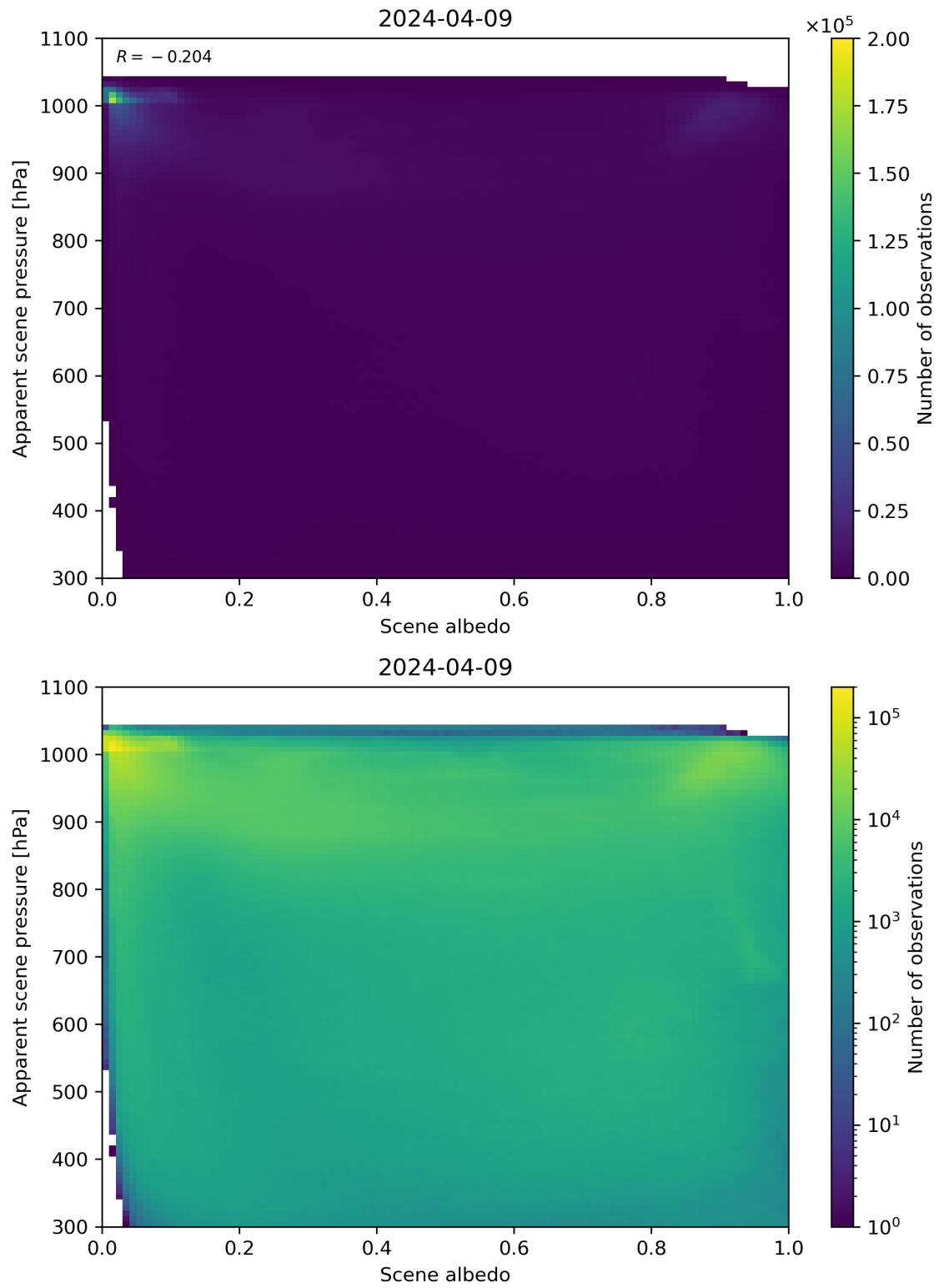
Figure 102: Scatter density plot of “Scene albedo” against “Apparent scene pressure” for 2024-04-08 to 2024-04-10.
