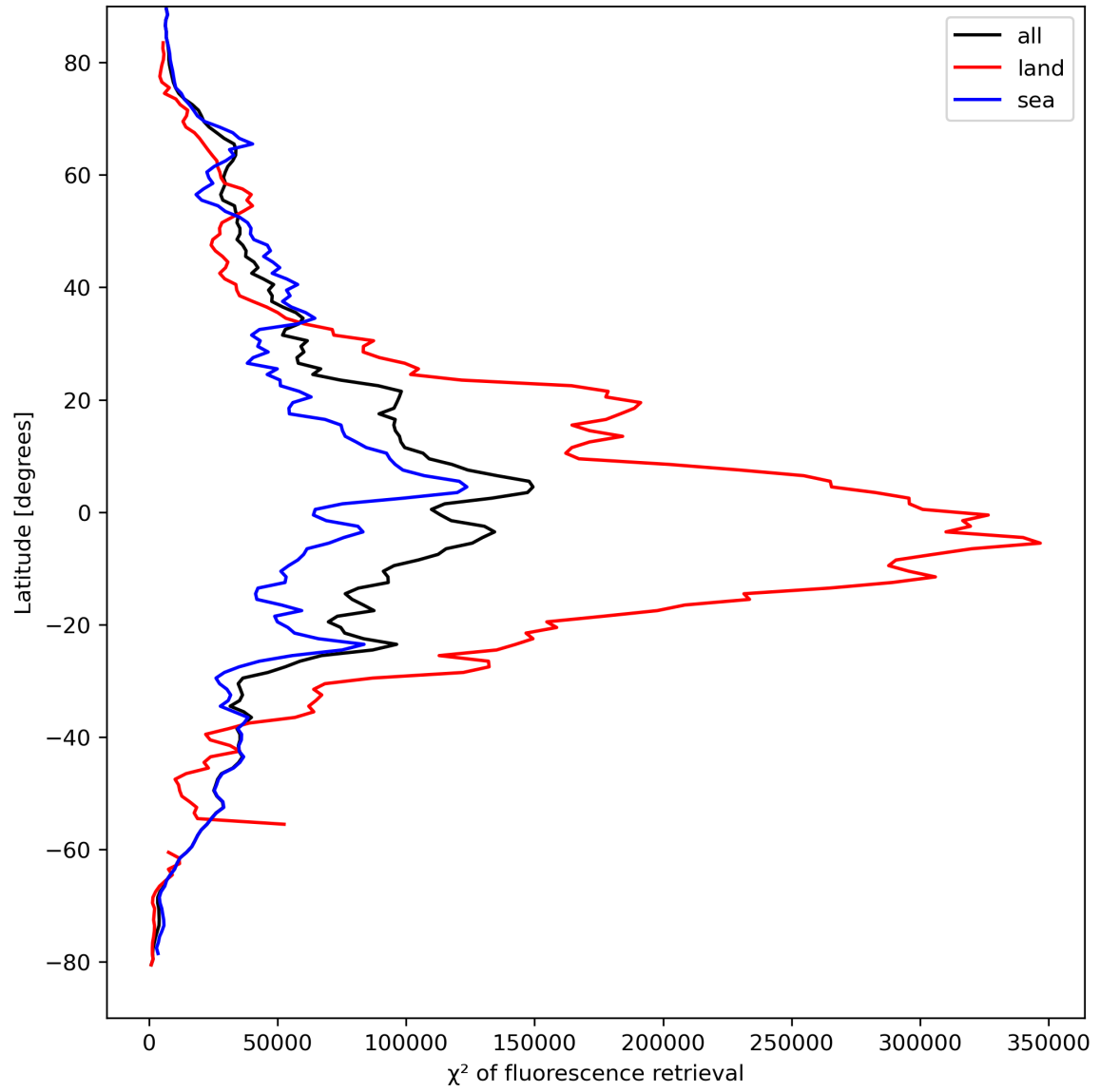
Figure 25: Zonal average of “ \chi^2 of fluorescence retrieval” for 2024-04-08 to 2024-04-10.
