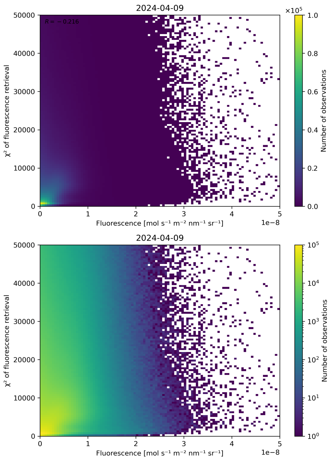
Figure 85: Scatter density plot of “Fluorescence” against “ \chi^2 of fluorescence retrieval” for 2024-04-08 to 2024-04-10.
