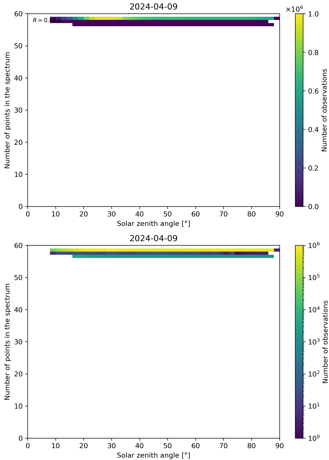
Figure 115: Scatter density plot of “Solar zenith angle” against “Number of points in the spectrum” for 2024-04-08 to 2024-04-10.
