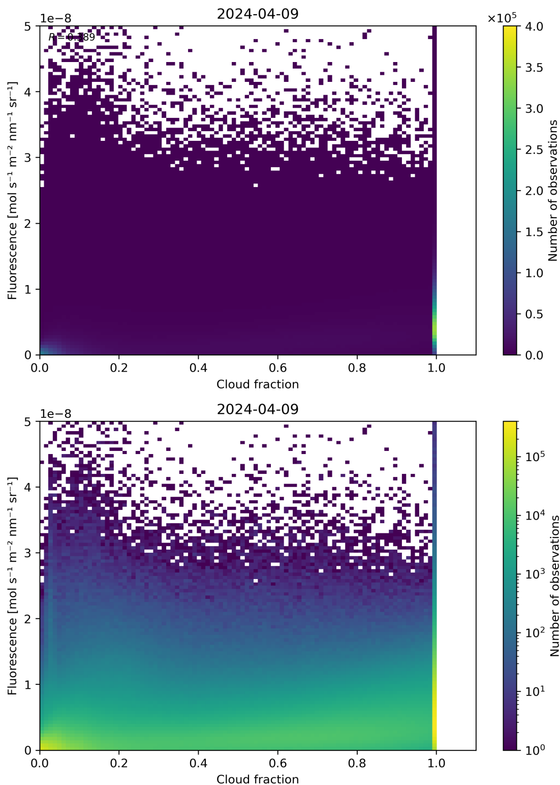
Figure 72: Scatter density plot of “Cloud fraction” against “Fluorescence” for 2024-04-08 to 2024-04-10.
