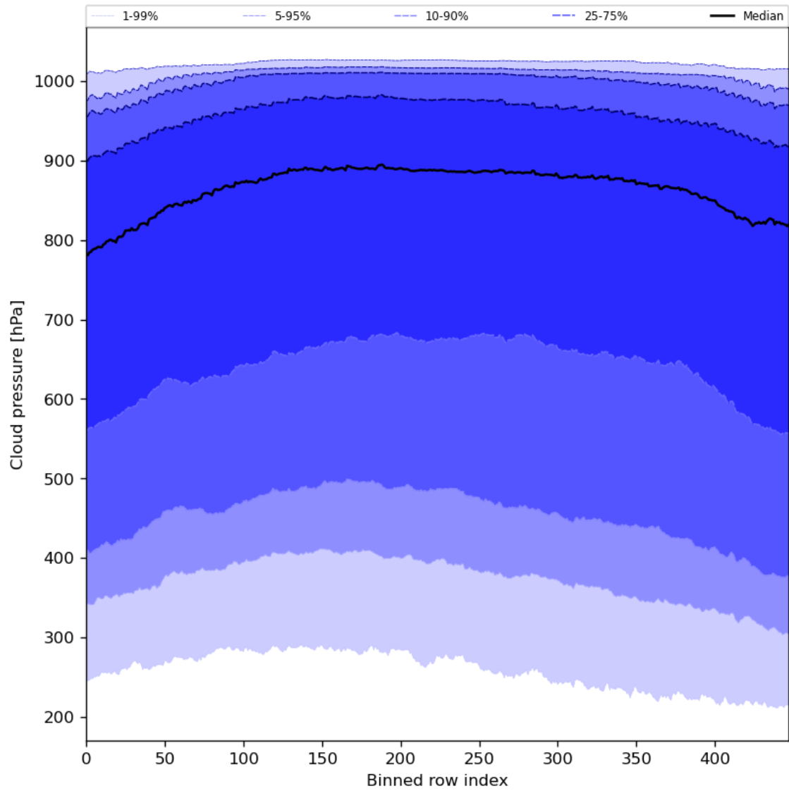
Figure 47: Along track statistics of “Cloud pressure” for 2024-04-08 to 2024-04-10
