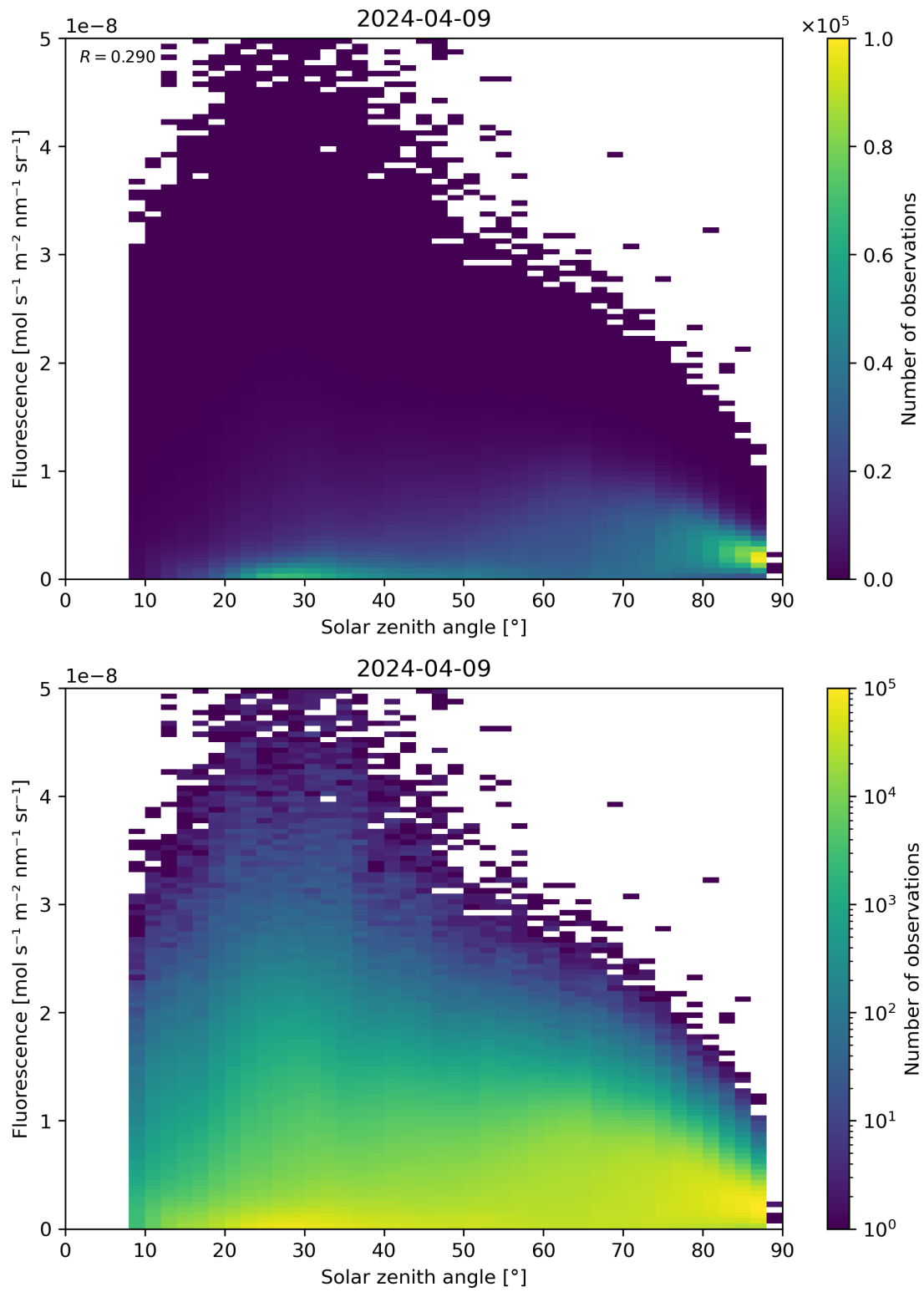
Figure 112: Scatter density plot of “Solar zenith angle” against “Fluorescence” for 2024-04-08 to 2024-04-10.
