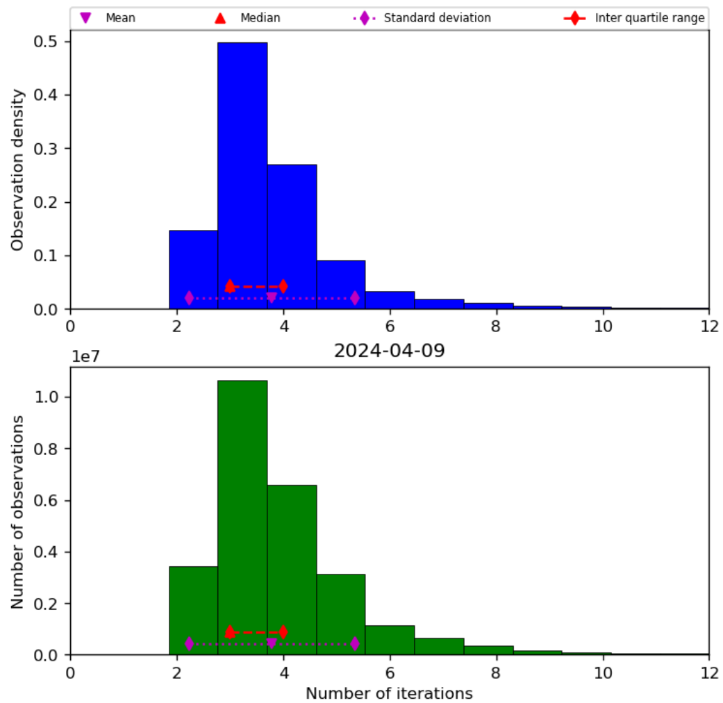
Figure 39: Histogram of “Number of iterations” for 2024-04-08 to 2024-04-10
