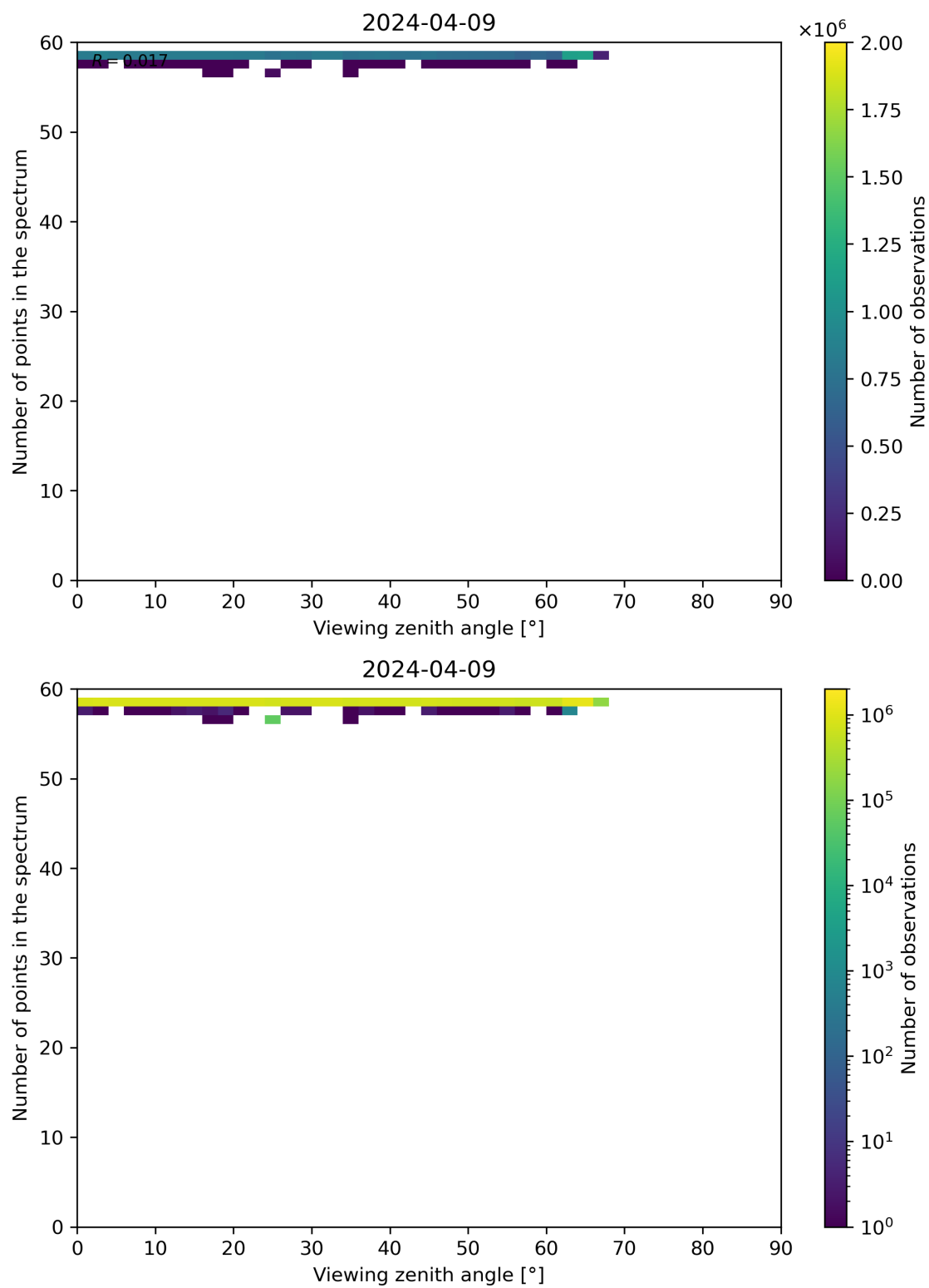
Figure 125: Scatter density plot of “Viewing zenith angle” against “Number of points in the spectrum” for 2024-04-08 to 2024-04-10.
