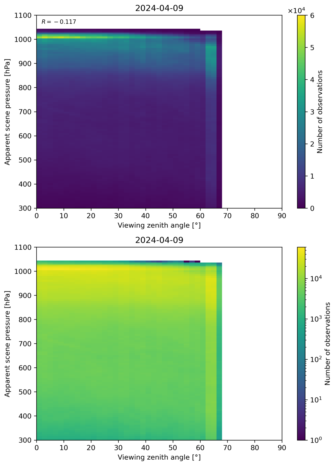
Figure 118: Scatter density plot of “Viewing zenith angle” against “Apparent scene pressure” for 2024-04-08 to 2024-04-10.
