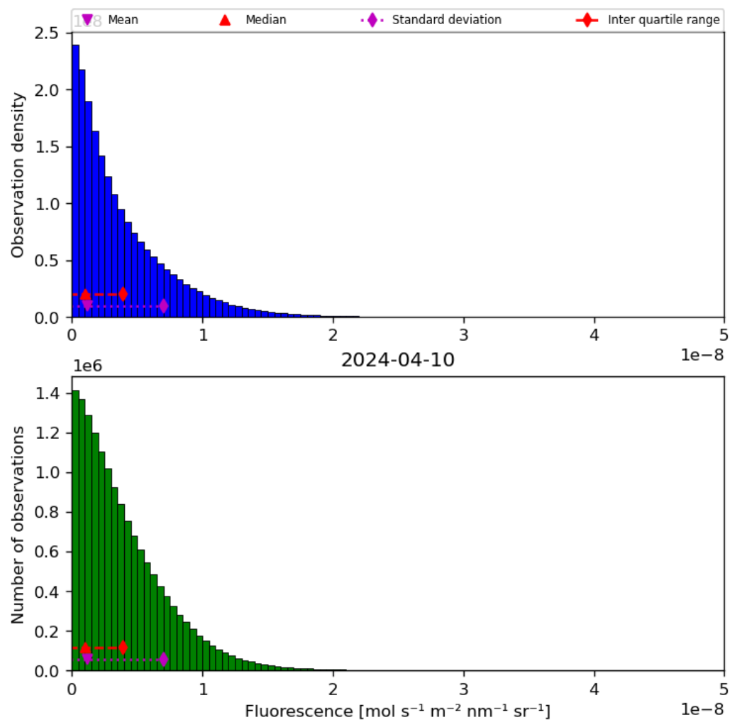
Figure 40: Histogram of “Fluorescence” for 2024-04-10 to 2024-04-11
