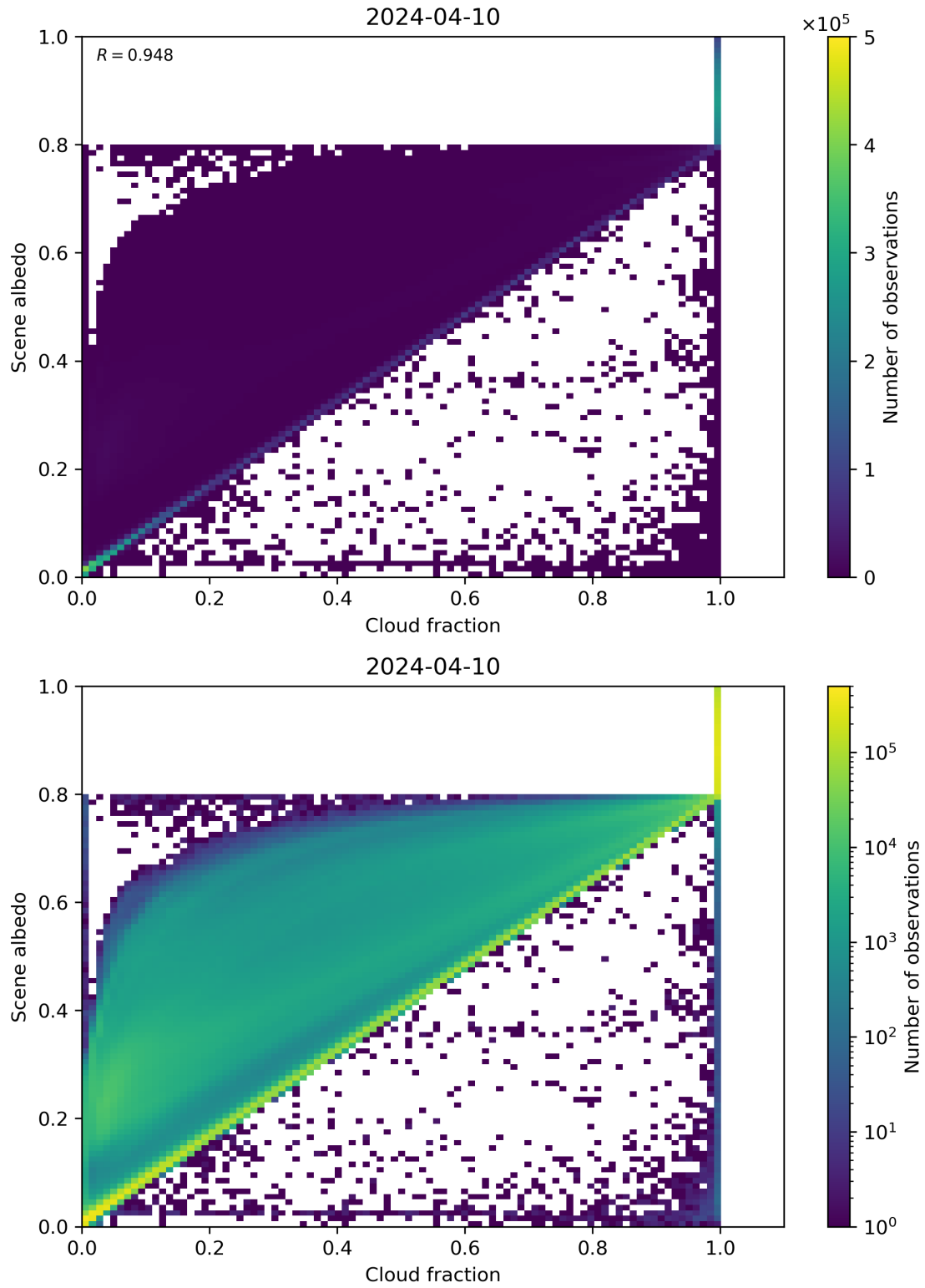
Figure 75: Scatter density plot of “Cloud fraction” against “Scene albedo” for 2024-04-10 to 2024-04-11.
