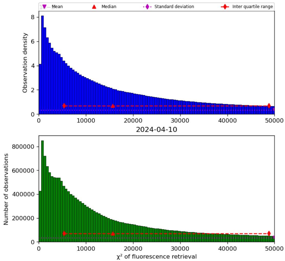
Figure 42: Histogram of “ \chi^2 of fluorescence retrieval” for 2024-04-10 to 2024-04-11
