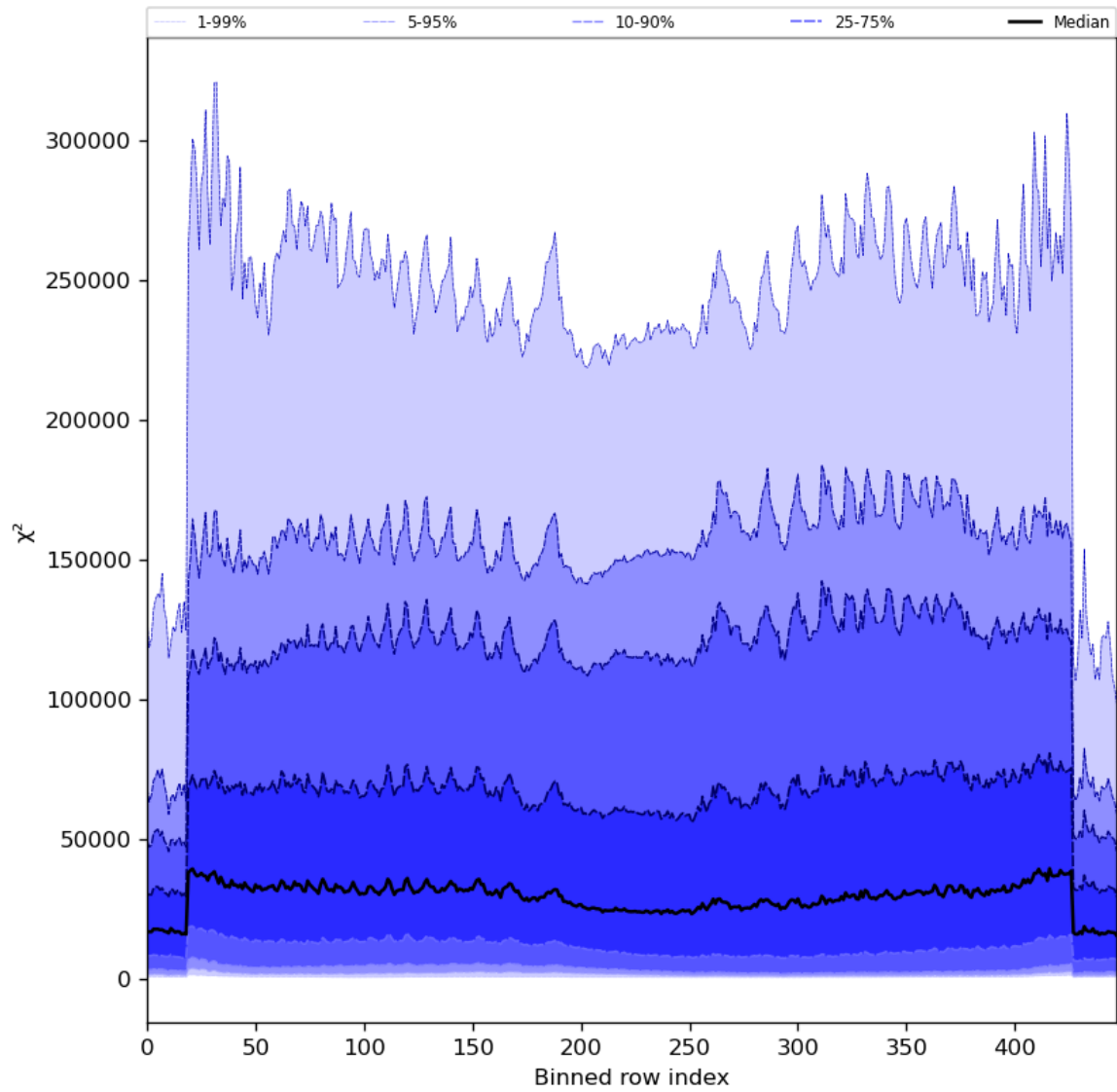
Figure 55: Along track statistics of “ \chi^2 ” for 2024-04-10 to 2024-04-11
