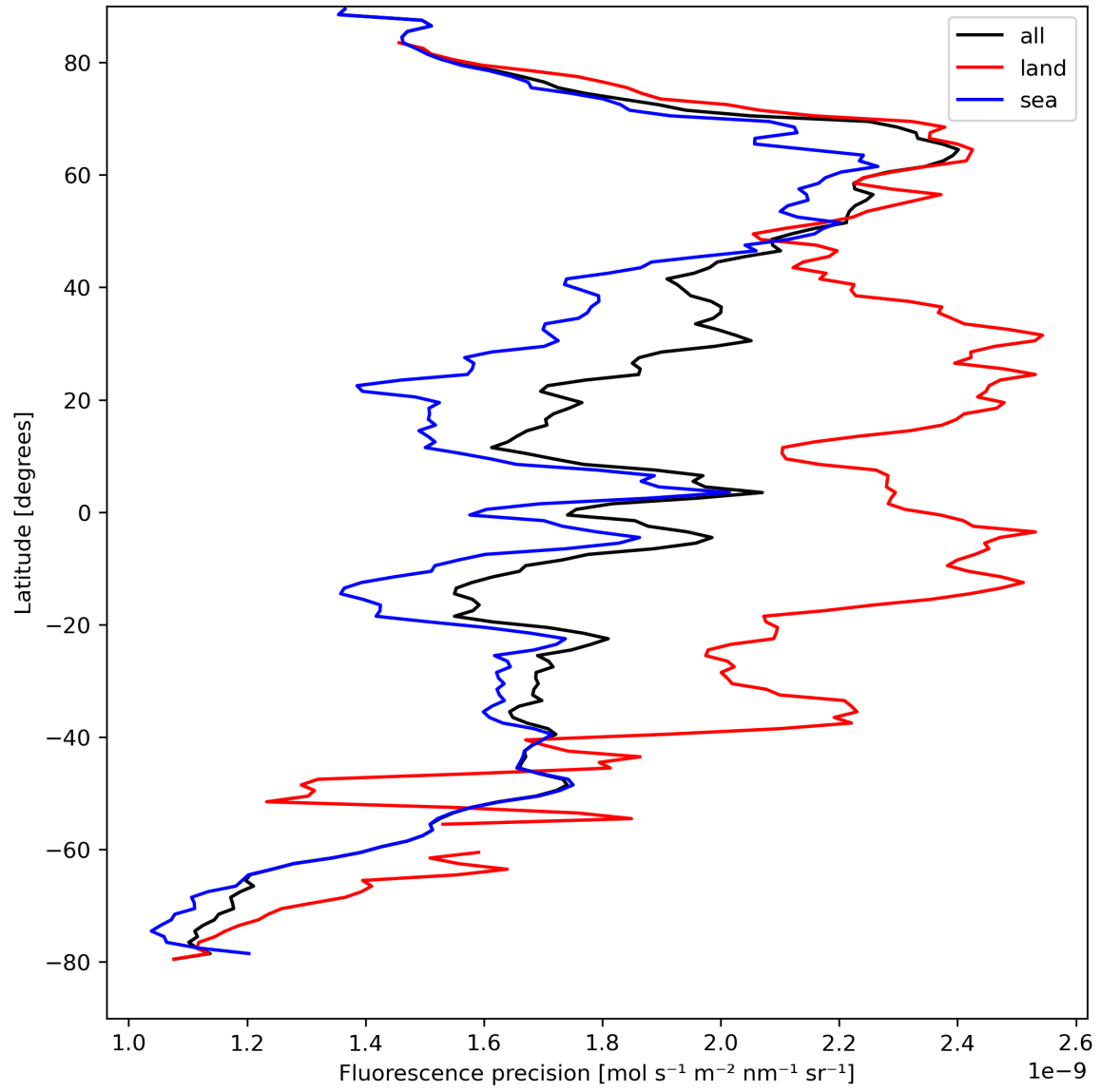
Figure 24: Zonal average of "Fluorescence precision" for 2024-04-10 to 2024-04-11.
