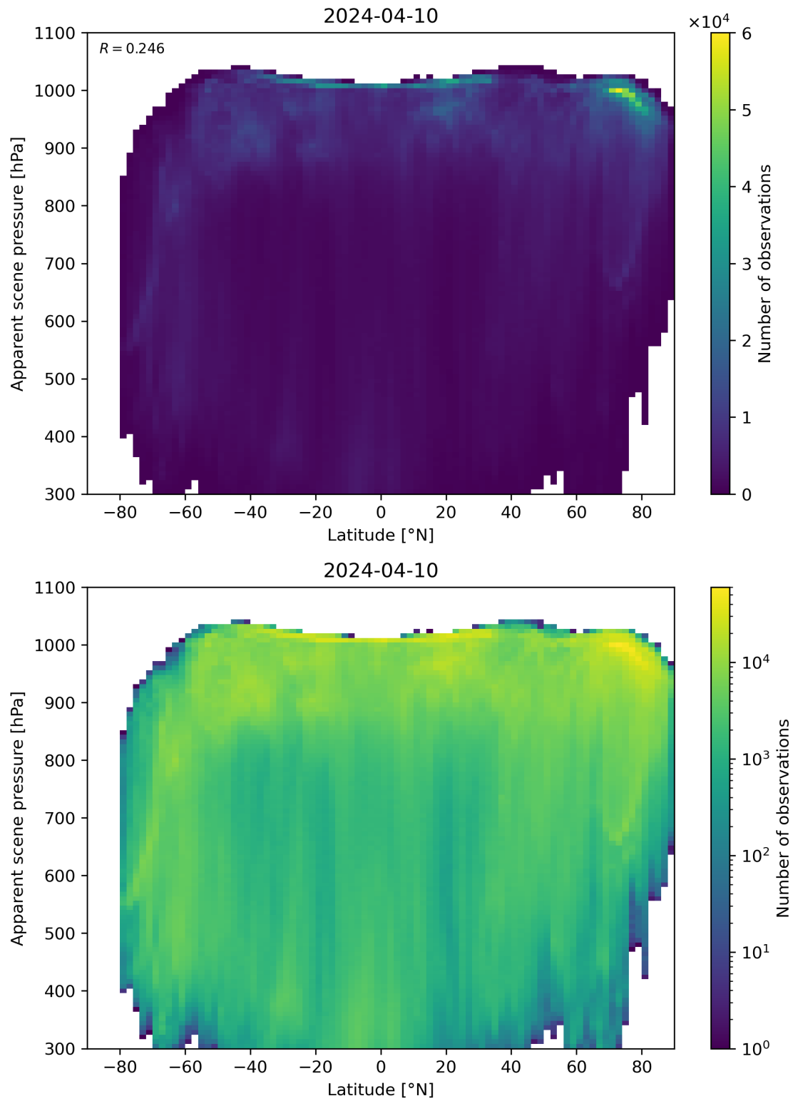
Figure 88: Scatter density plot of “Latitude” against “Apparent scene pressure” for 2024-04-10 to 2024-04-11.
