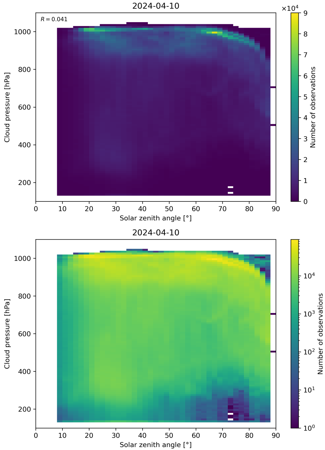
Figure 111: Scatter density plot of “Solar zenith angle” against “Cloud pressure” for 2024-04-10 to 2024-04-11.
