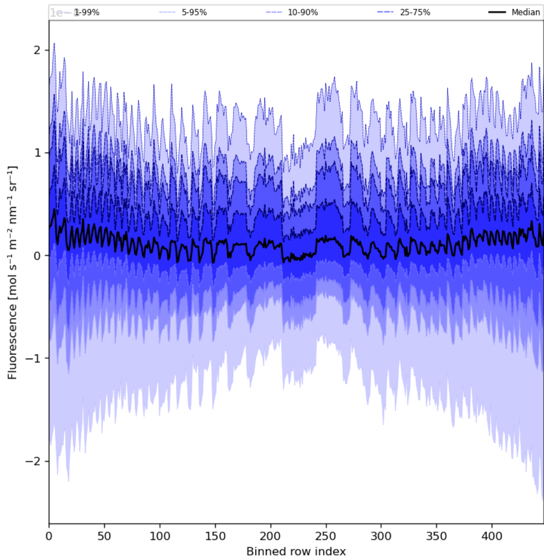
Figure 57: Along track statistics of “Fluorescence” for 2024-04-10 to 2024-04-11
