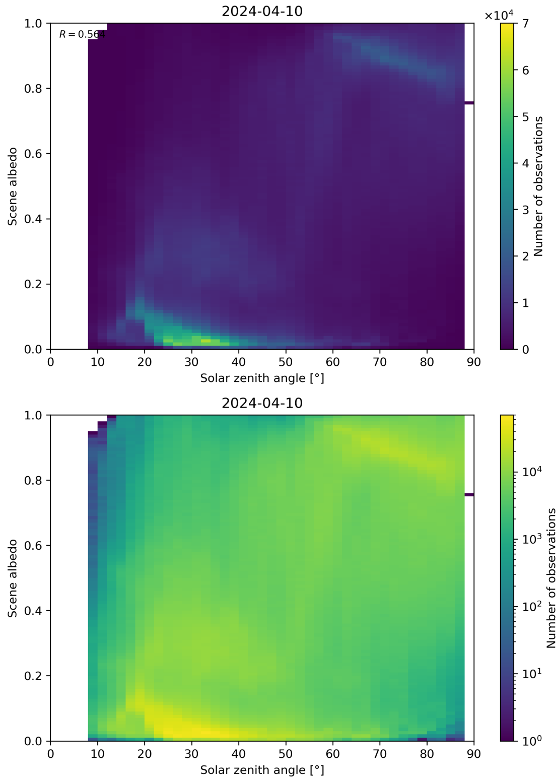
Figure 116: Scatter density plot of “Solar zenith angle” against “Scene albedo” for 2024-04-10 to 2024-04-11.
