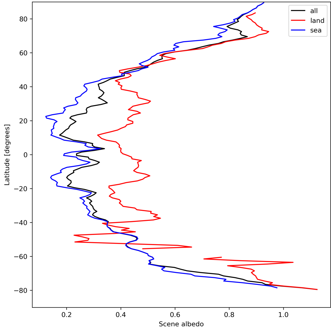
Figure 17: Zonal average of “Scene albedo” for 2024-04-10 to 2024-04-11.
