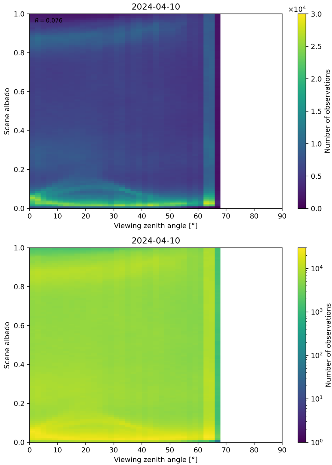
Figure 126: Scatter density plot of “Viewing zenith angle” against “Scene albedo” for 2024-04-10 to 2024-04-11.
