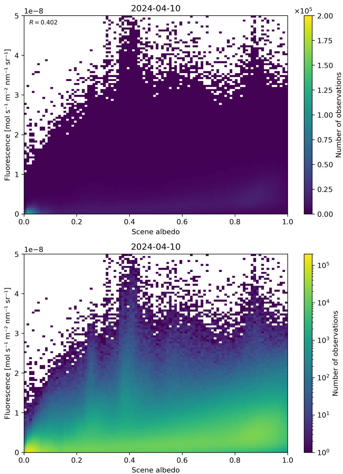
Figure 104: Scatter density plot of “Scene albedo” against “Fluorescence” for 2024-04-10 to 2024-04-11.
