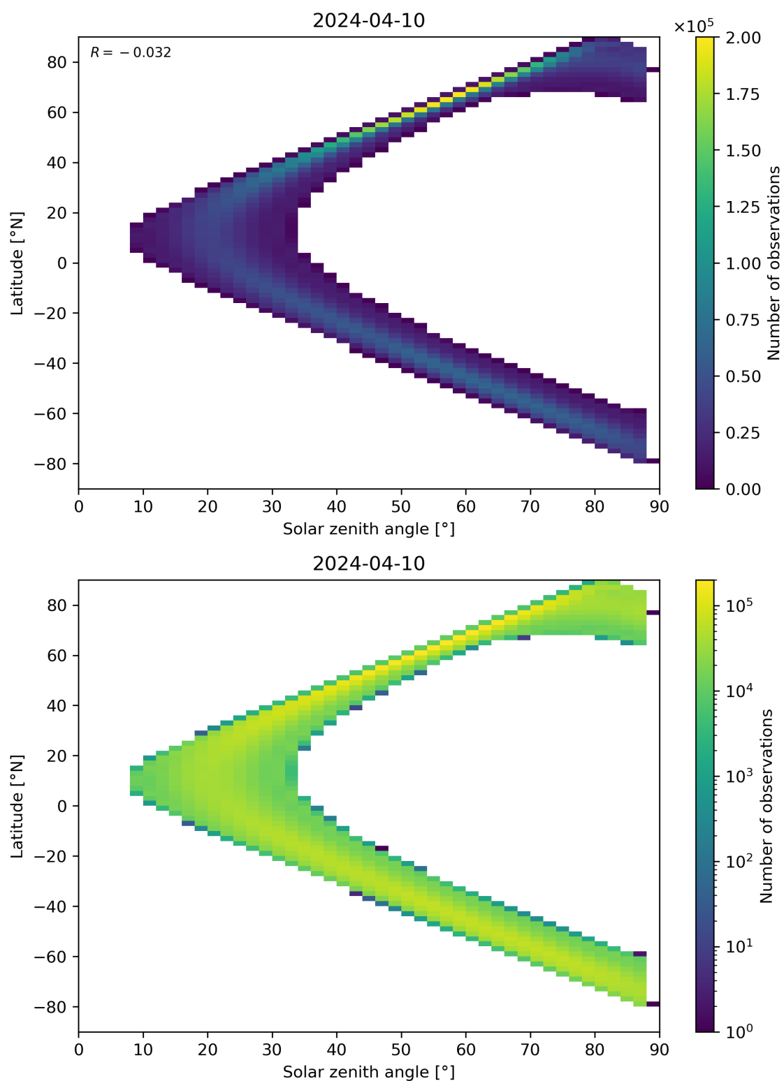
Figure 113: Scatter density plot of “Solar zenith angle” against “Latitude” for 2024-04-10 to 2024-04-11.
