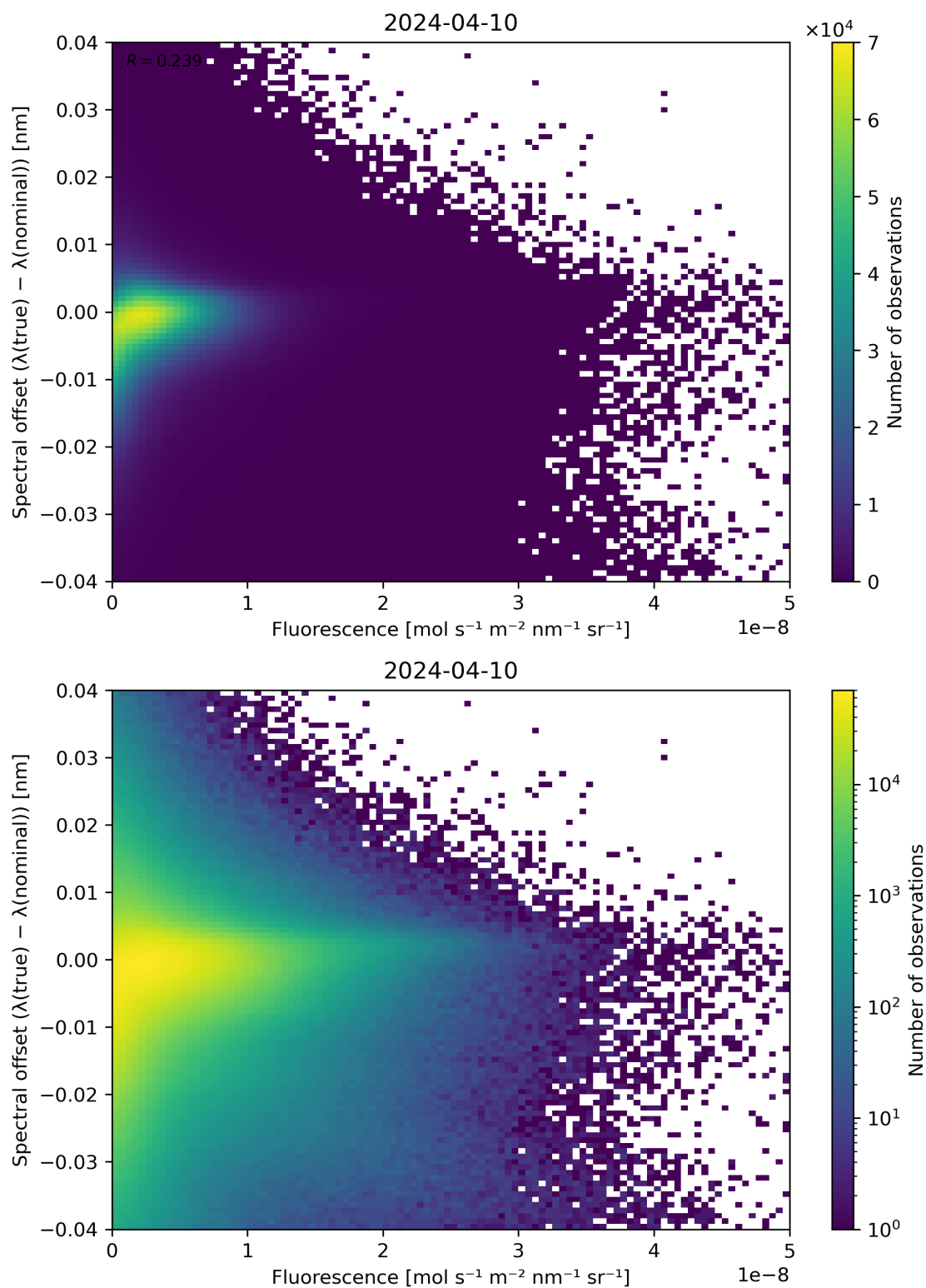
Figure 87: Scatter density plot of “Fluorescence” against “Spectral offset ( \lambda(\text{true}) - \lambda(\text{nominal}) )” for 2024-04-10 to 2024-04-11.
