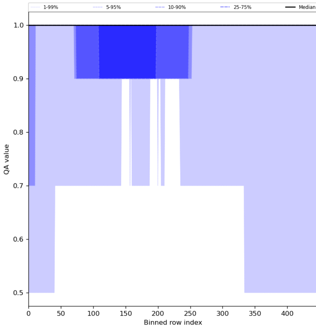
Figure 46: Along track statistics of “QA value” for 2024-04-10 to 2024-04-11
