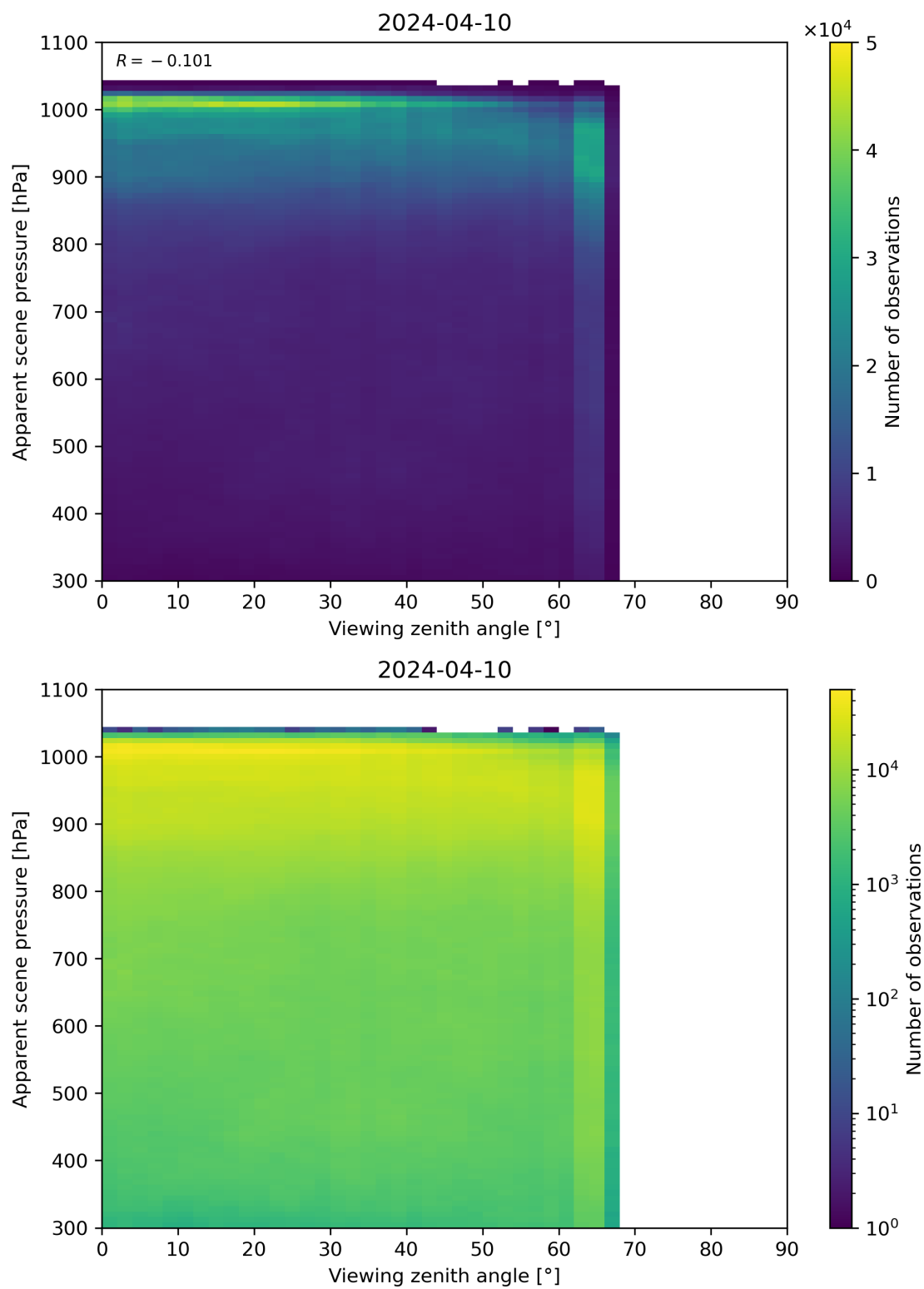
Figure 118: Scatter density plot of “Viewing zenith angle” against “Apparent scene pressure” for 2024-04-10 to 2024-04-11.
