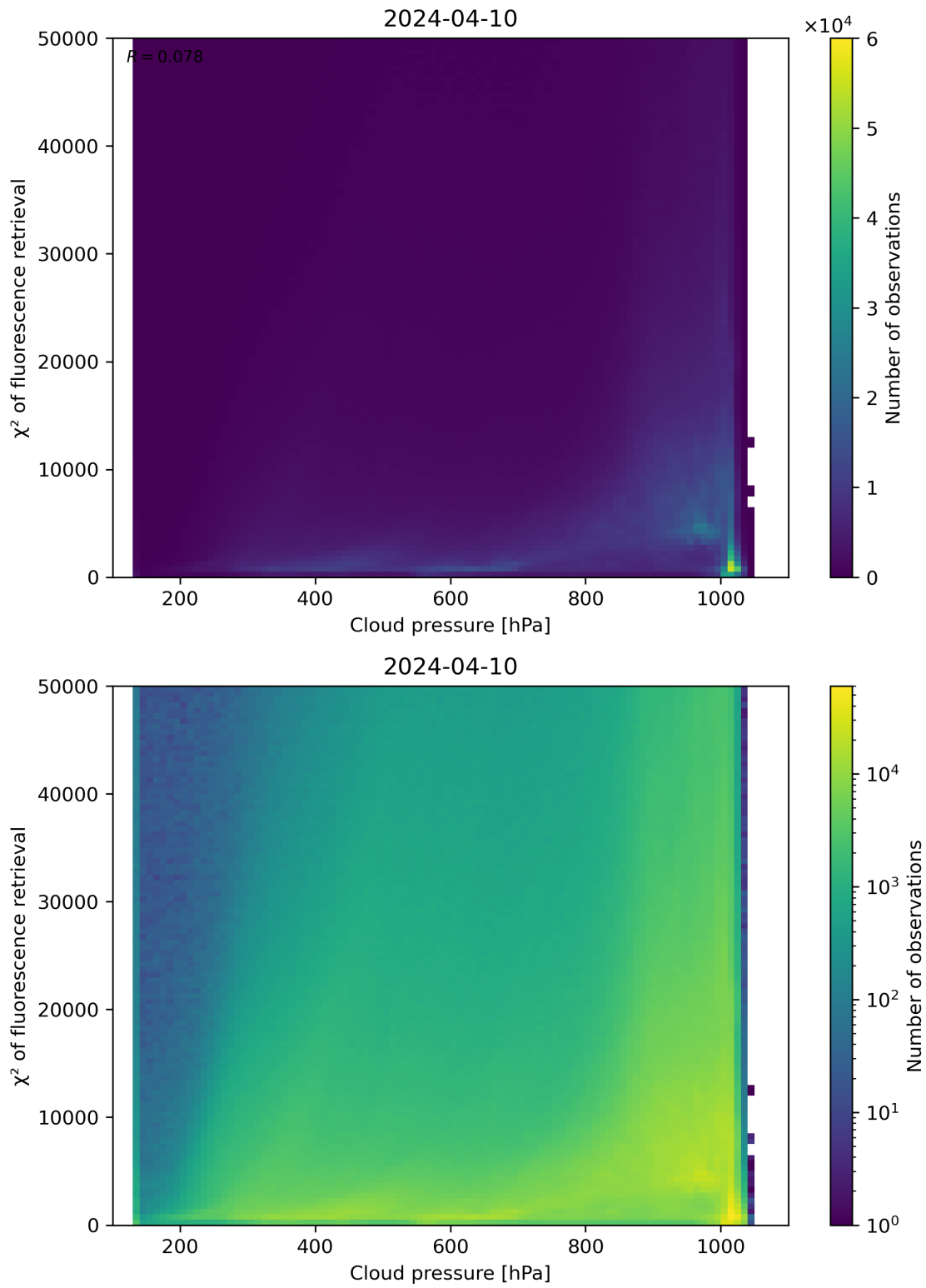
Figure 78: Scatter density plot of “Cloud pressure” against “ \chi^2 of fluorescence retrieval” for 2024-04-10 to 2024-04-11.
