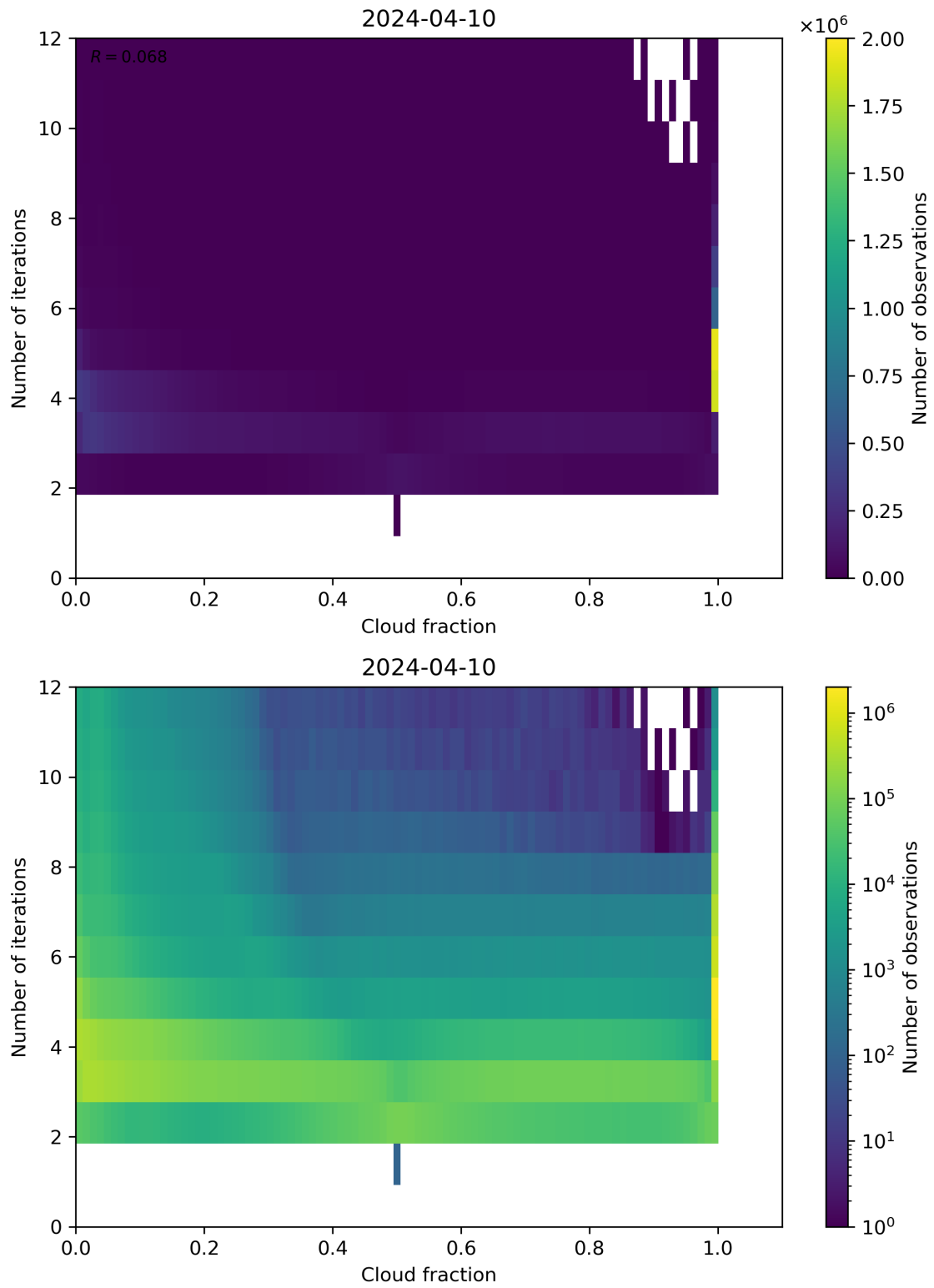
Figure 73: Scatter density plot of “Cloud fraction” against “Number of iterations” for 2024-04-10 to 2024-04-11.
