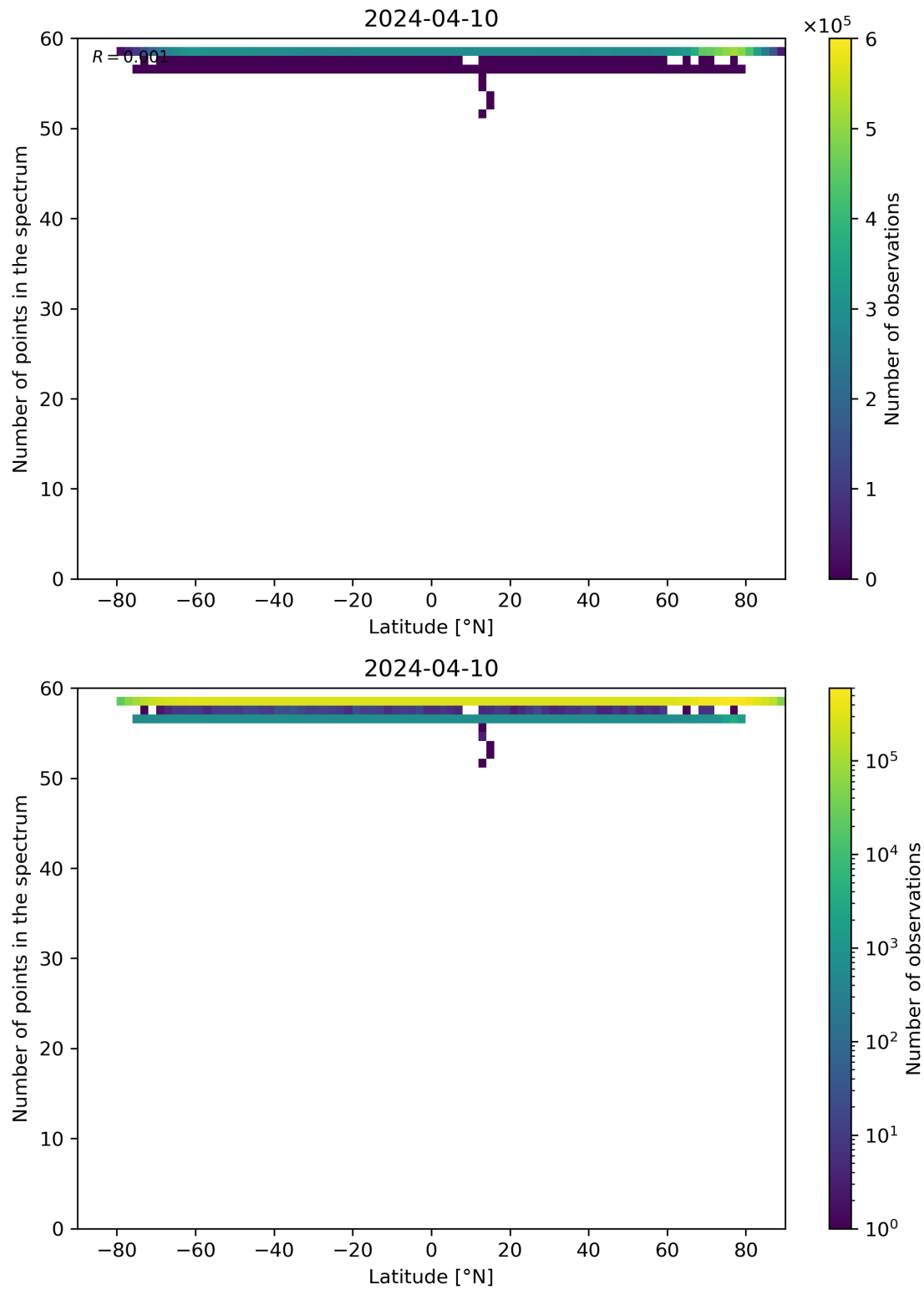
Figure 94: Scatter density plot of “Latitude” against “Number of points in the spectrum” for 2024-04-10 to 2024-04-11.
