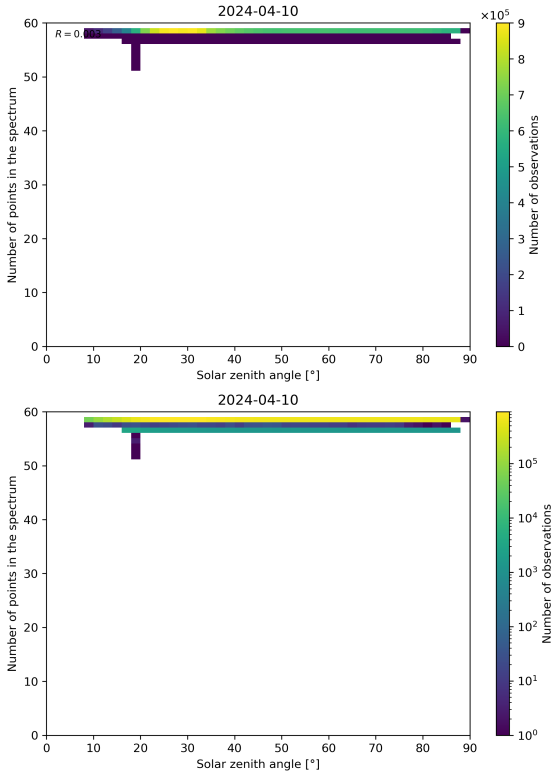
Figure 115: Scatter density plot of “Solar zenith angle” against “Number of points in the spectrum” for 2024-04-10 to 2024-04-11.
