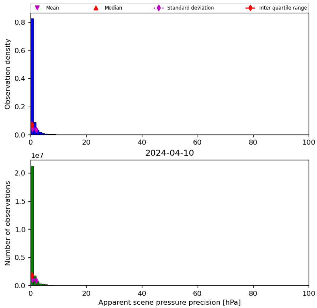
Figure 37: Histogram of “Apparent scene pressure precision” for 2024-04-10 to 2024-04-11
