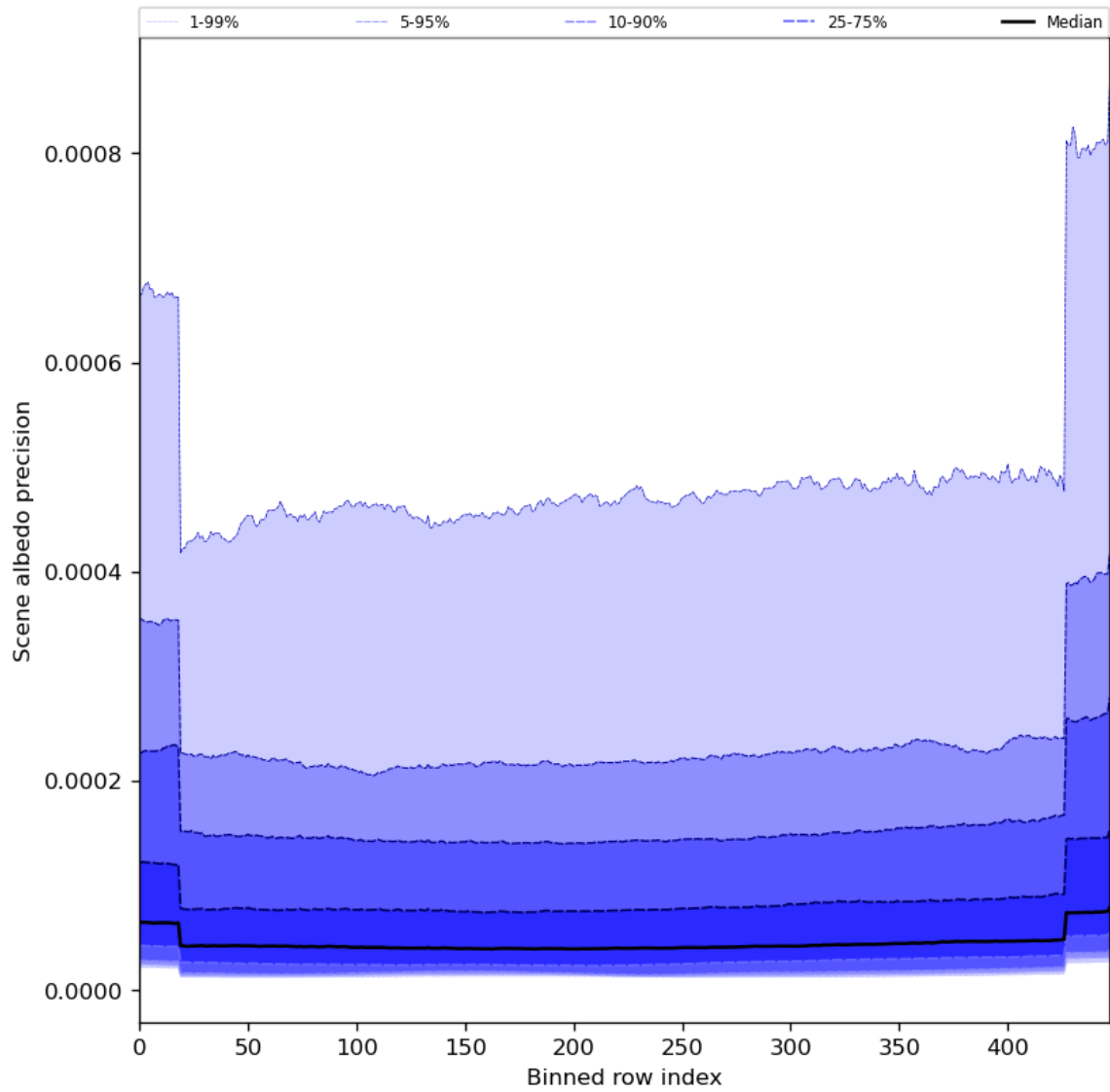
Figure 52: Along track statistics of “Scene albedo precision” for 2024-04-10 to 2024-04-11
