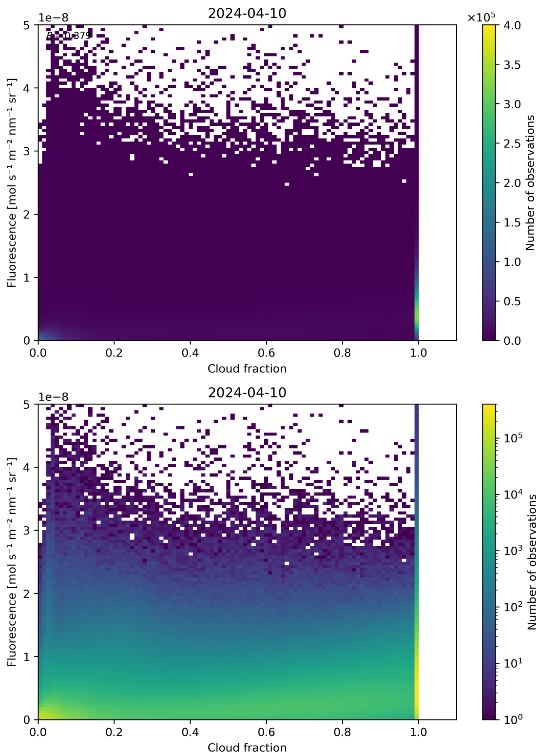
Figure 72: Scatter density plot of “Cloud fraction” against “Fluorescence” for 2024-04-10 to 2024-04-11.
