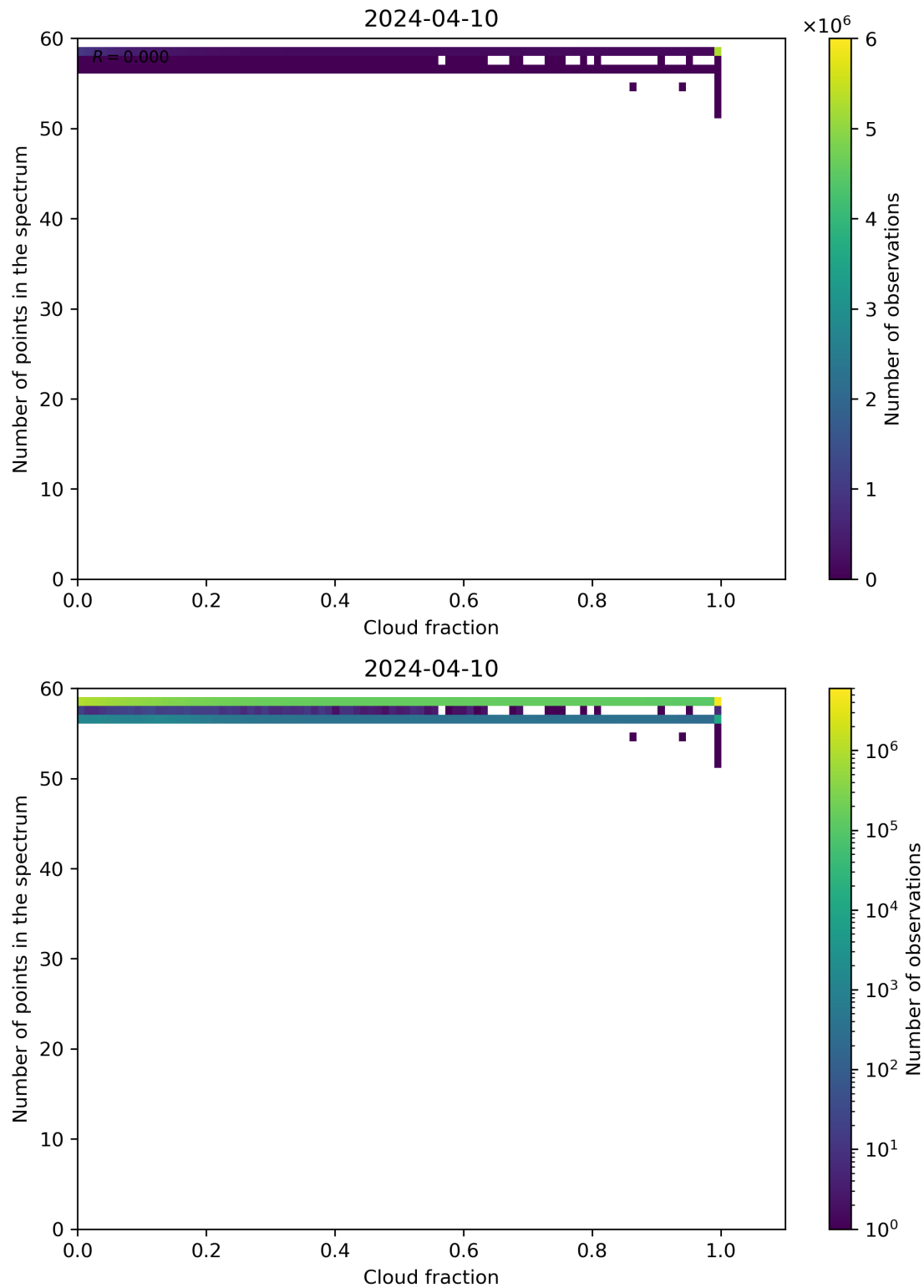
Figure 74: Scatter density plot of “Cloud fraction” against “Number of points in the spectrum” for 2024-04-10 to 2024-04-11.
