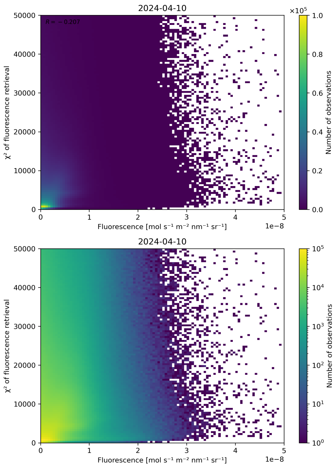
Figure 85: Scatter density plot of “Fluorescence” against “ \chi^2 of fluorescence retrieval” for 2024-04-10 to 2024-04-11.
