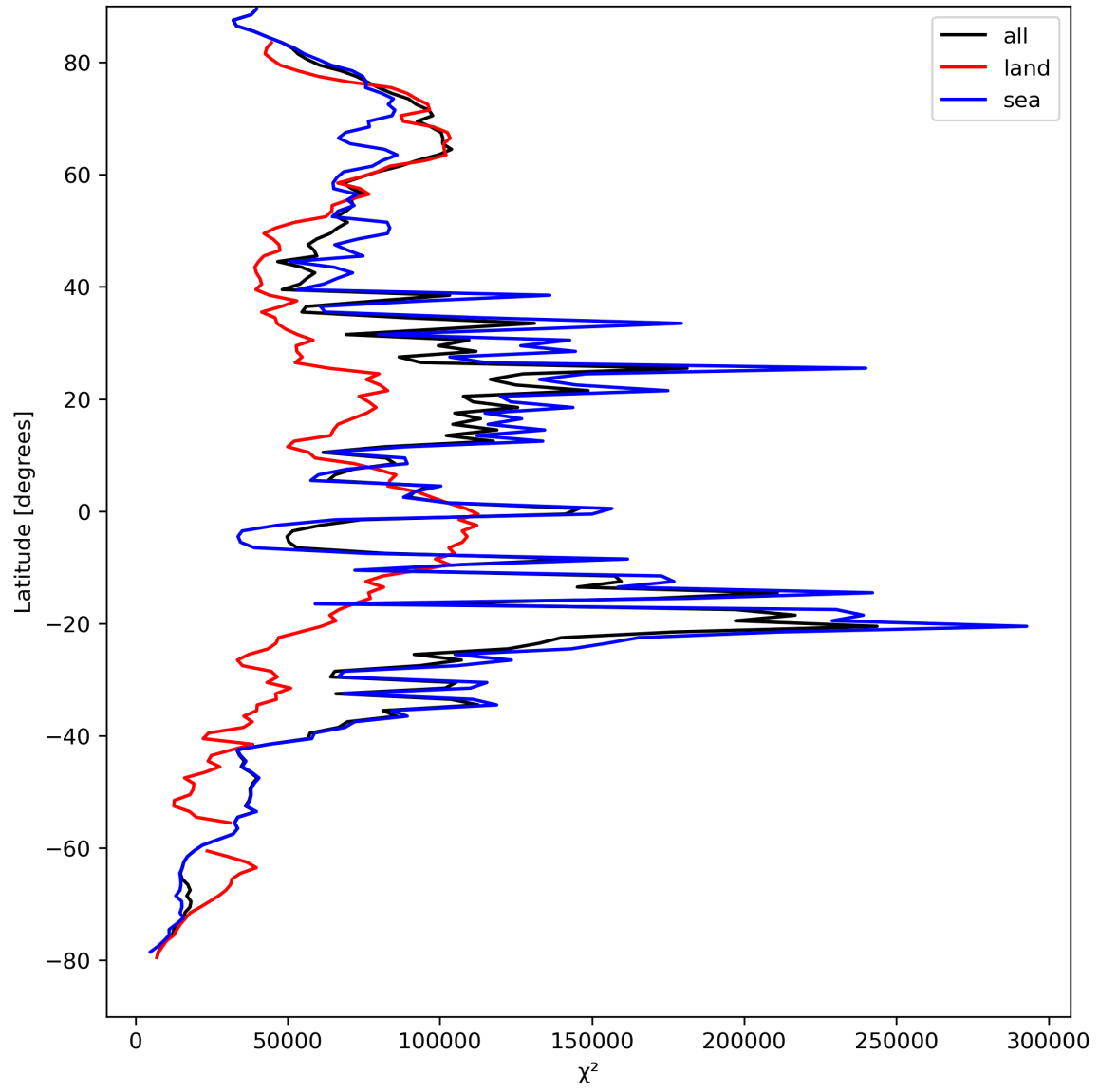
Figure 21: Zonal average of “ \chi^2 ” for 2024-04-10 to 2024-04-11.
