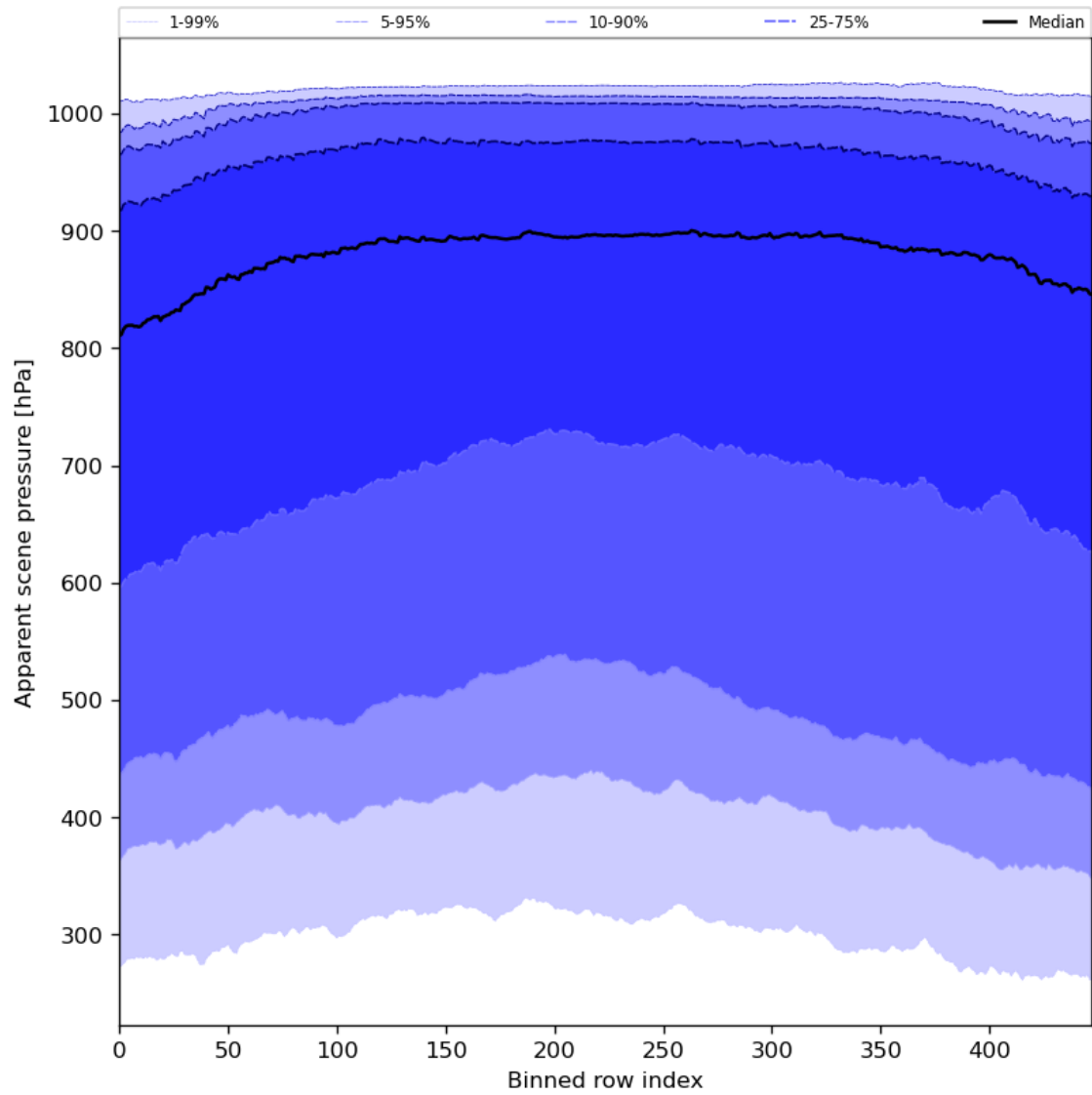
Figure 53: Along track statistics of “Apparent scene pressure” for 2024-04-10 to 2024-04-11
