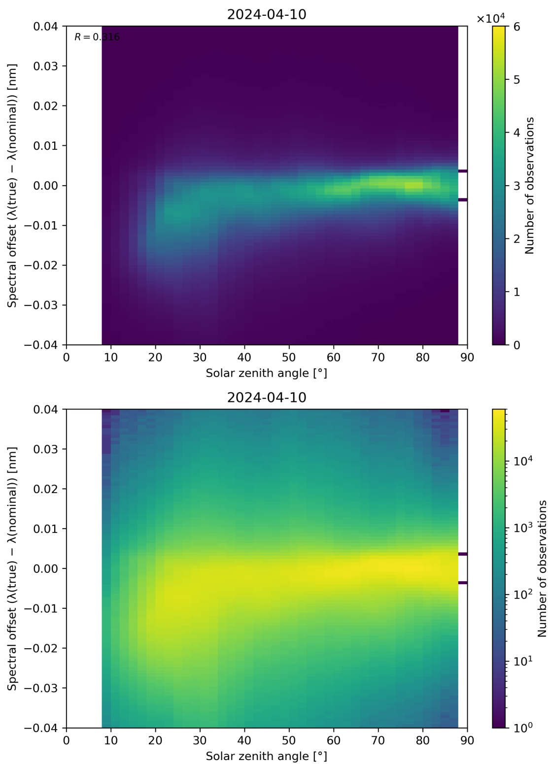
Figure 117: Scatter density plot of “Solar zenith angle” against “Spectral offset ( \lambda(\text{true}) - \lambda(\text{nominal}) )” for 2024-04-10 to 2024-04-11.
