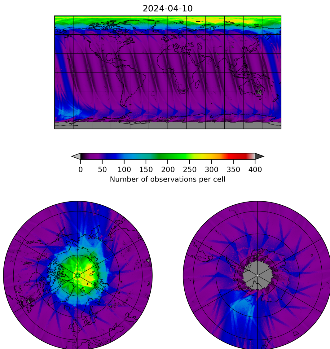
Figure 11: Map of the number of observations for 2024-04-10 to 2024-04-11
