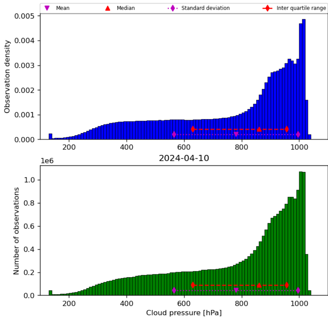
Figure 30: Histogram of “Cloud pressure” for 2024-04-10 to 2024-04-11
