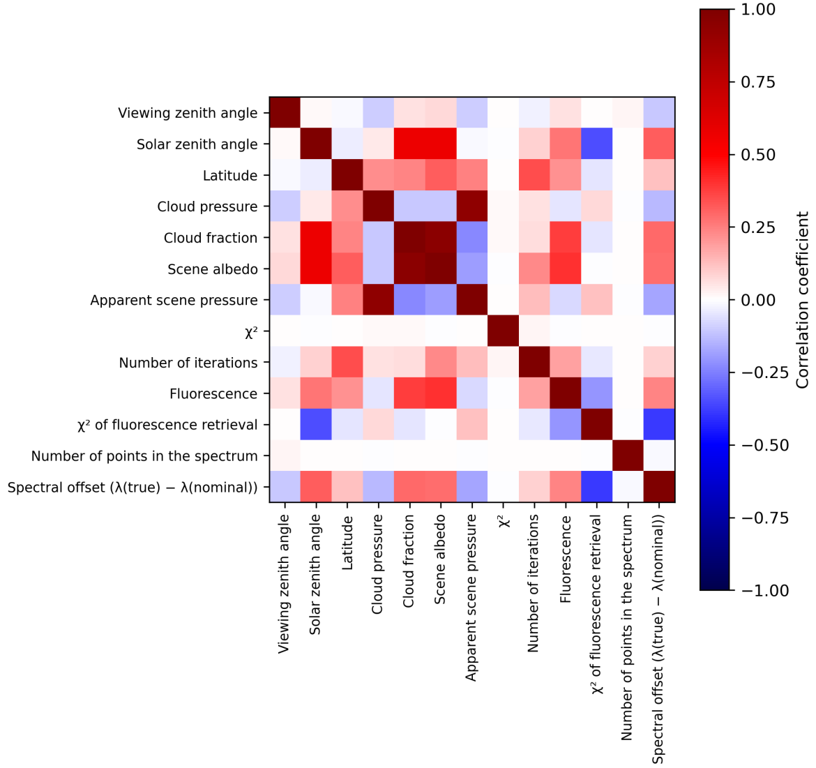
Figure 2: Map of correlation matrix for 2024-04-10 to 2024-04-11.
