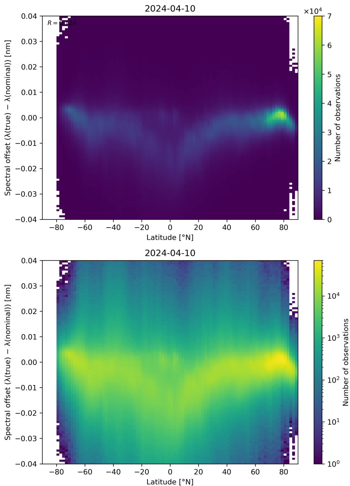
Figure 96: Scatter density plot of “Latitude” against “Spectral offset ( \lambda(\text{true}) - \lambda(\text{nominal}) )” for 2024-04-10 to 2024-04-11.
