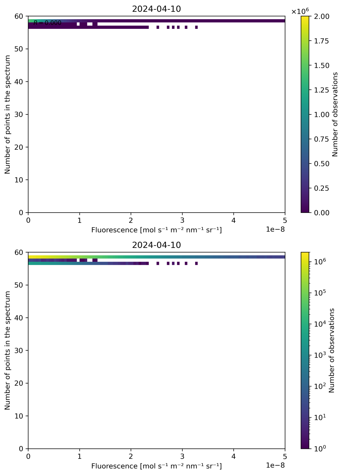
Figure 86: Scatter density plot of “Fluorescence” against “Number of points in the spectrum” for 2024-04-10 to 2024-04-11.
