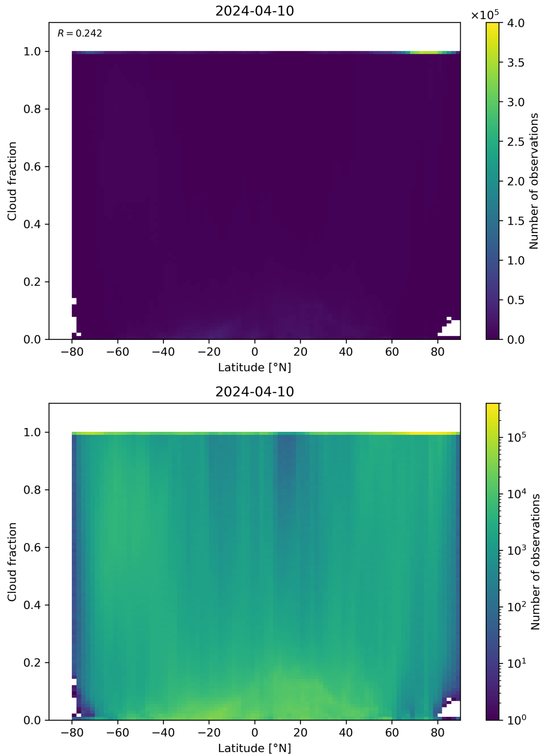
Figure 90: Scatter density plot of “Latitude” against “Cloud fraction” for 2024-04-10 to 2024-04-11.
