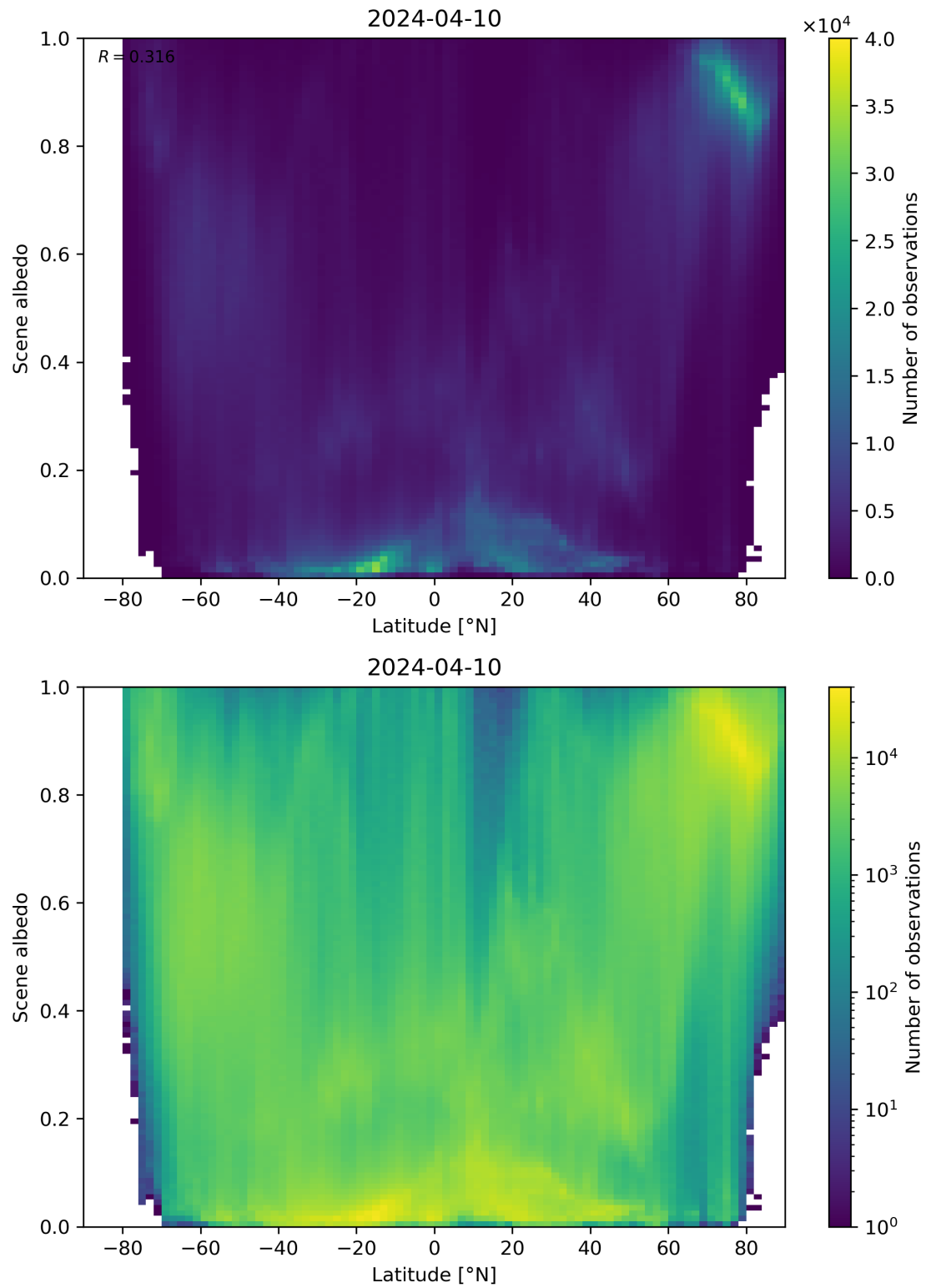
Figure 95: Scatter density plot of “Latitude” against “Scene albedo” for 2024-04-10 to 2024-04-11.
