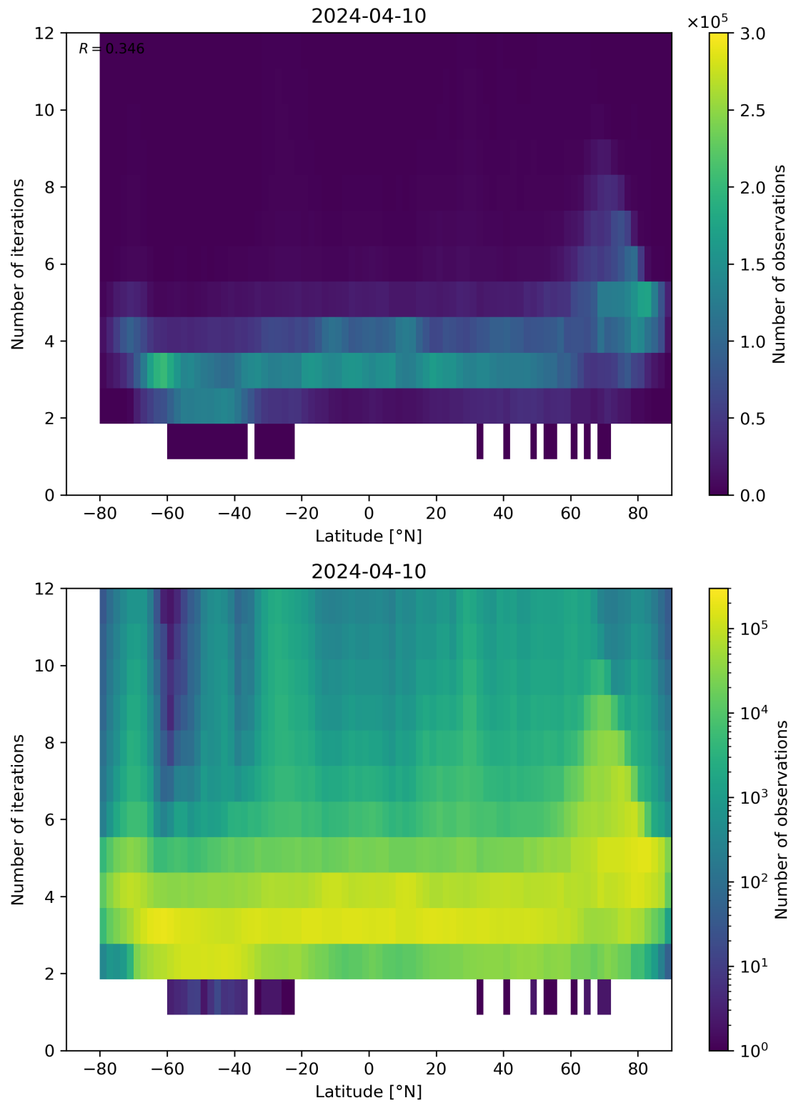
Figure 93: Scatter density plot of “Latitude” against “Number of iterations” for 2024-04-10 to 2024-04-11.
