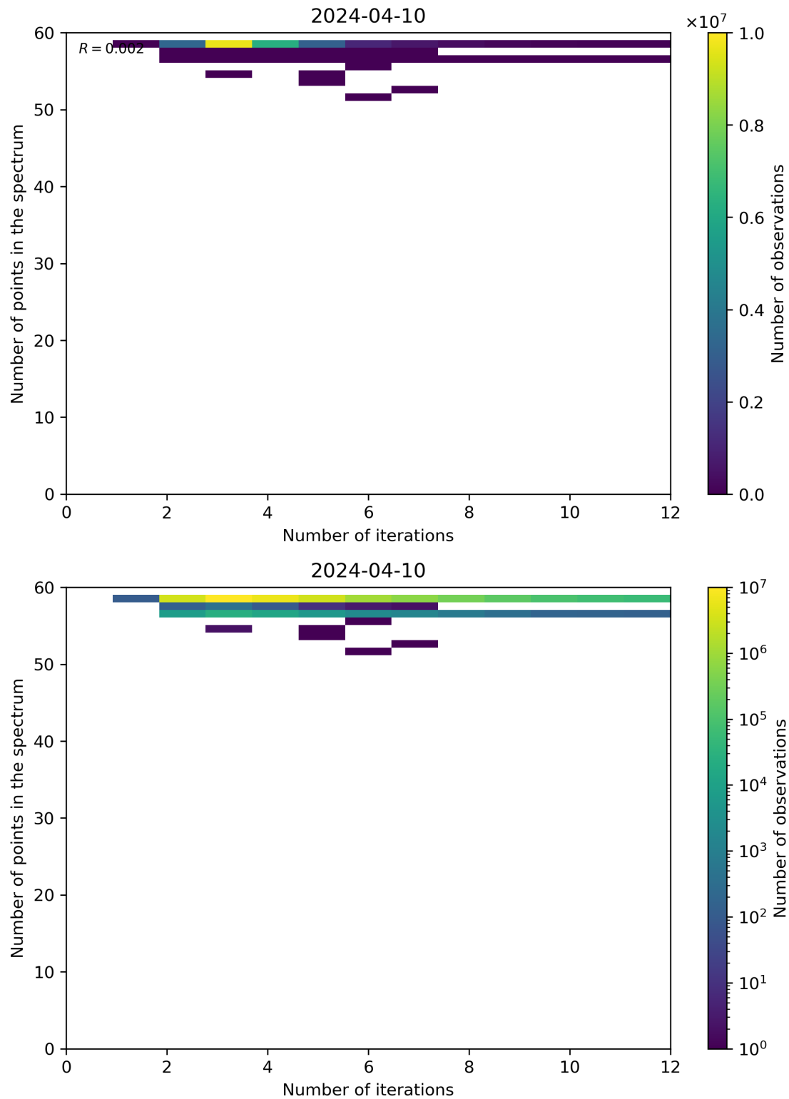
Figure 99: Scatter density plot of “Number of iterations” against “Number of points in the spectrum” for 2024-04-10 to 2024-04-11.
