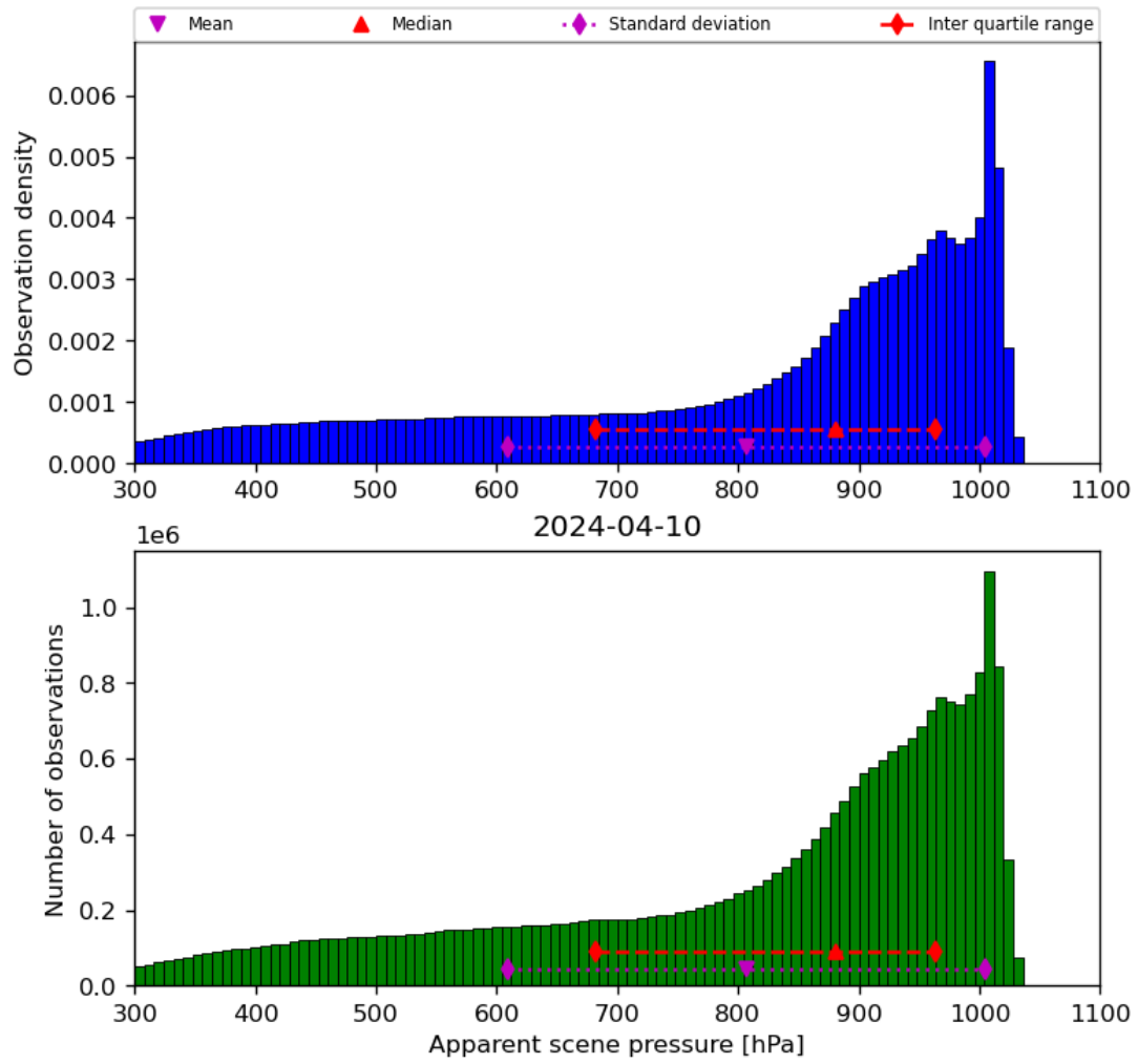
Figure 36: Histogram of “Apparent scene pressure” for 2024-04-10 to 2024-04-11
