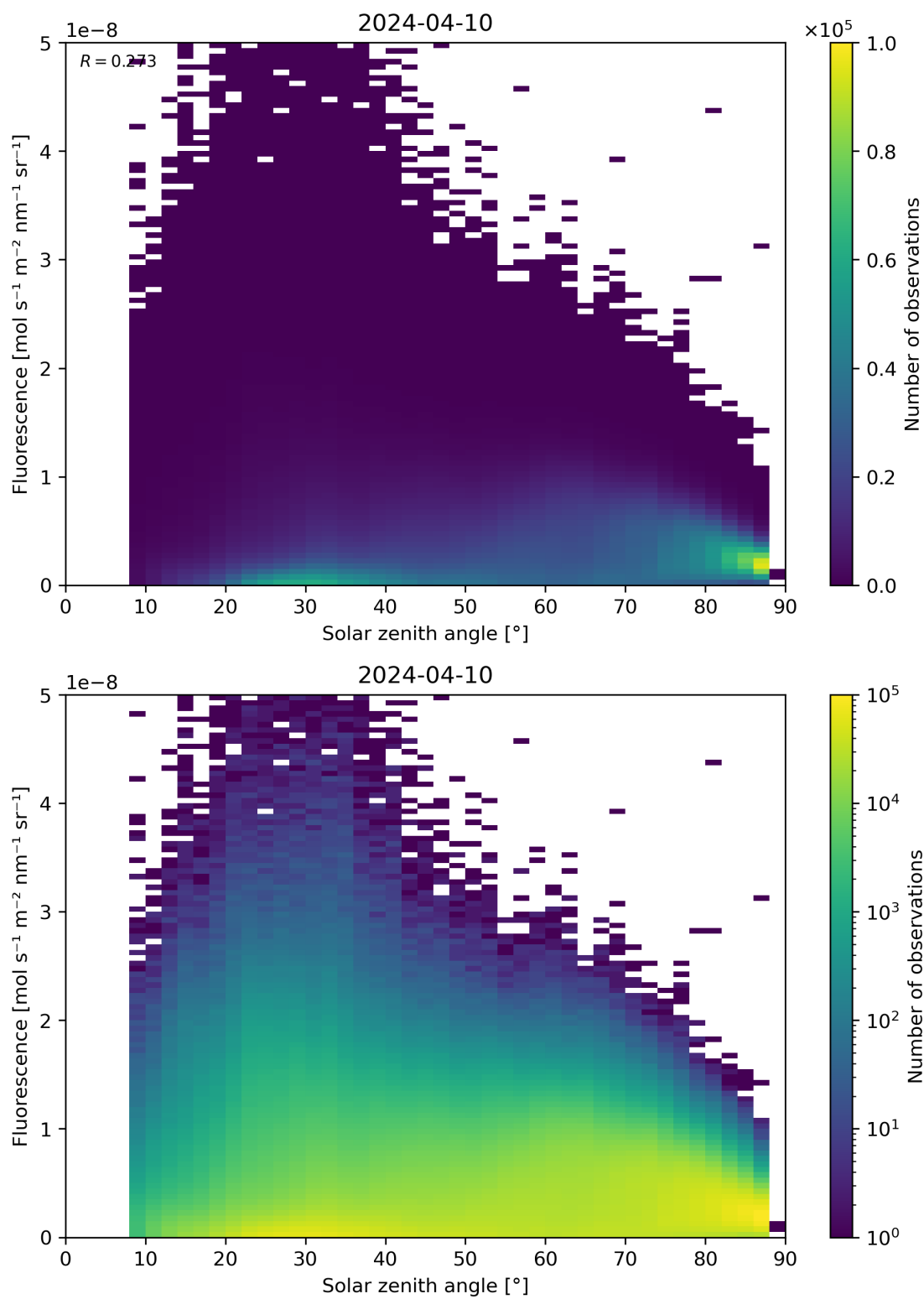
Figure 112: Scatter density plot of “Solar zenith angle” against “Fluorescence” for 2024-04-10 to 2024-04-11.
