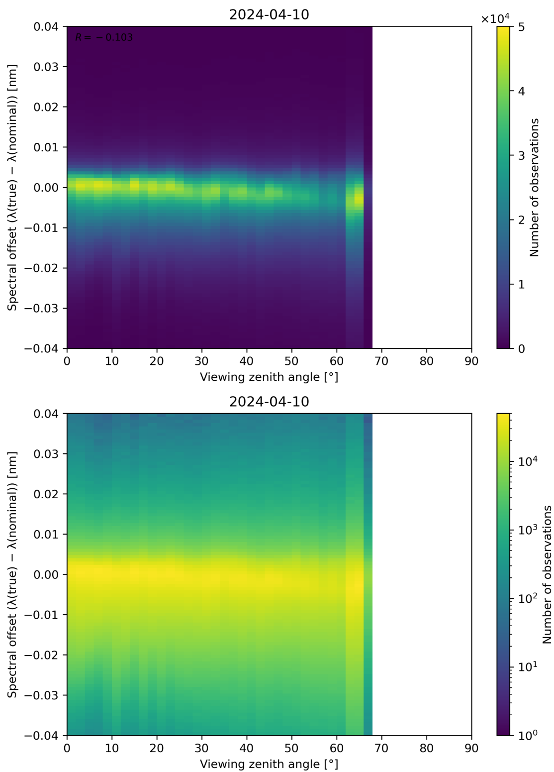
Figure 128: Scatter density plot of “Viewing zenith angle” against “Spectral offset ( \lambda(\text{true}) - \lambda(\text{nominal}) )” for 2024-04-10 to 2024-04-11.
