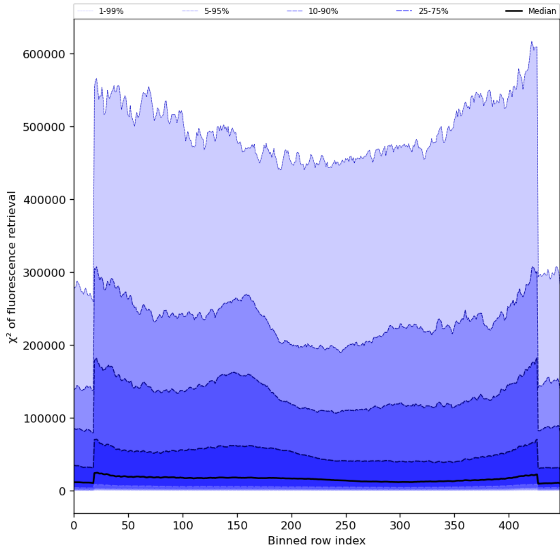
Figure 59: Along track statistics of “ \chi^2 of fluorescence retrieval” for 2024-04-10 to 2024-04-11
