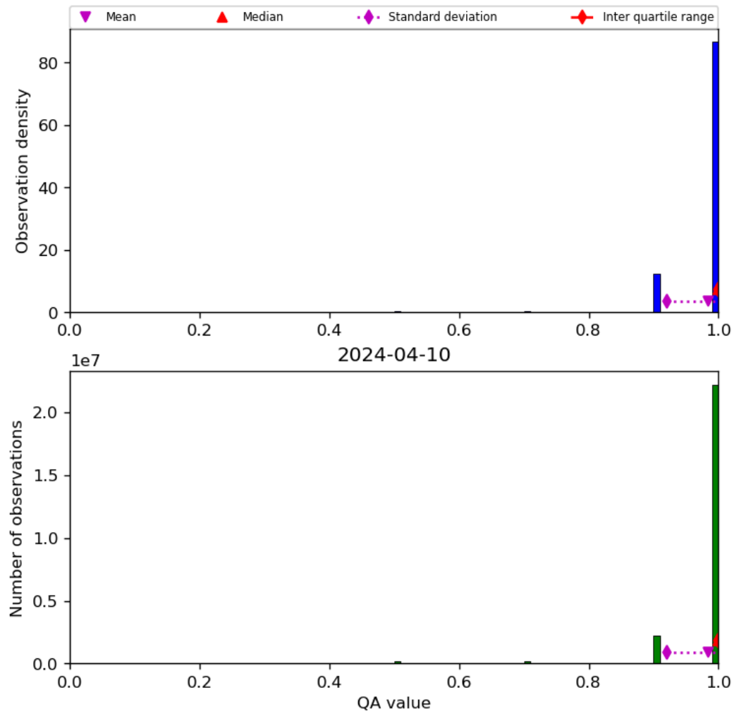
Figure 29: Histogram of “QA value” for 2024-04-10 to 2024-04-11
