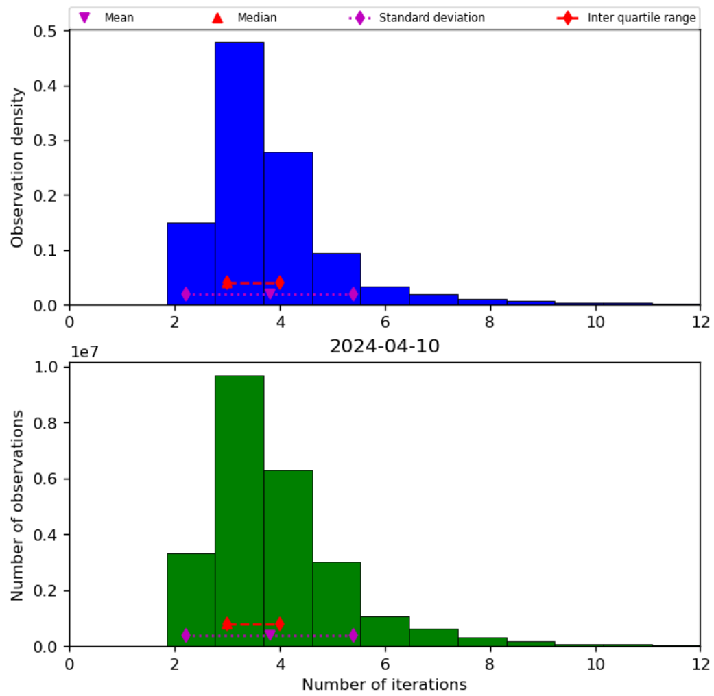
Figure 39: Histogram of “Number of iterations” for 2024-04-10 to 2024-04-11
