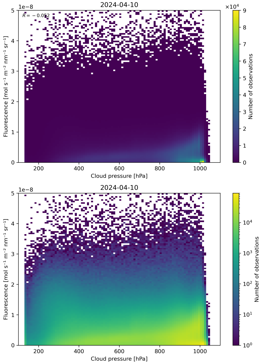
Figure 80: Scatter density plot of “Cloud pressure” against “Fluorescence” for 2024-04-10 to 2024-04-11.
