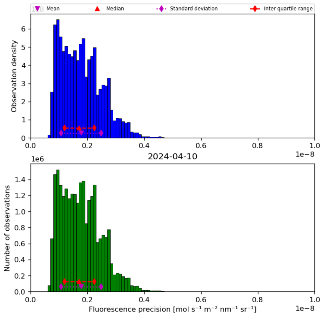
Figure 41: Histogram of “Fluorescence precision” for 2024-04-10 to 2024-04-11
