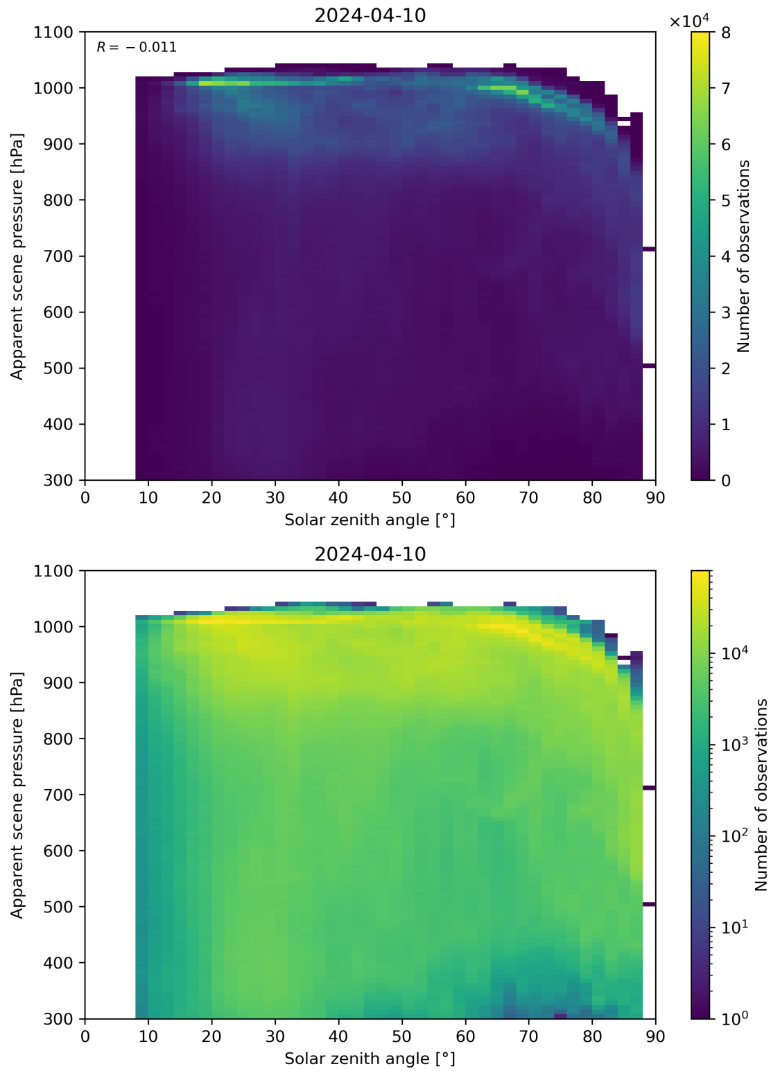
Figure 108: Scatter density plot of “Solar zenith angle” against “Apparent scene pressure” for 2024-04-10 to 2024-04-11.
