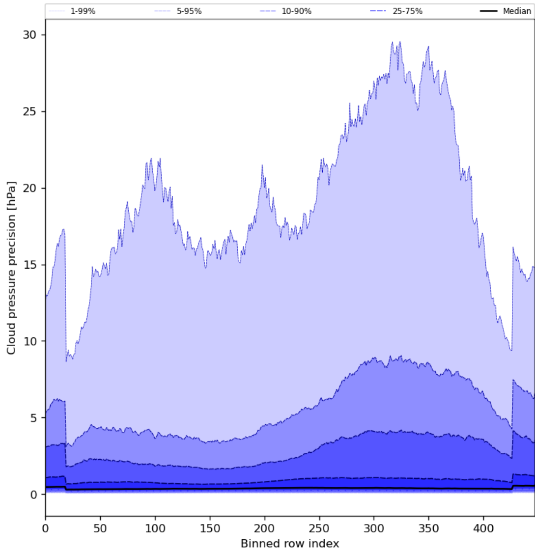
Figure 48: Along track statistics of “Cloud pressure precision” for 2024-04-10 to 2024-04-11
