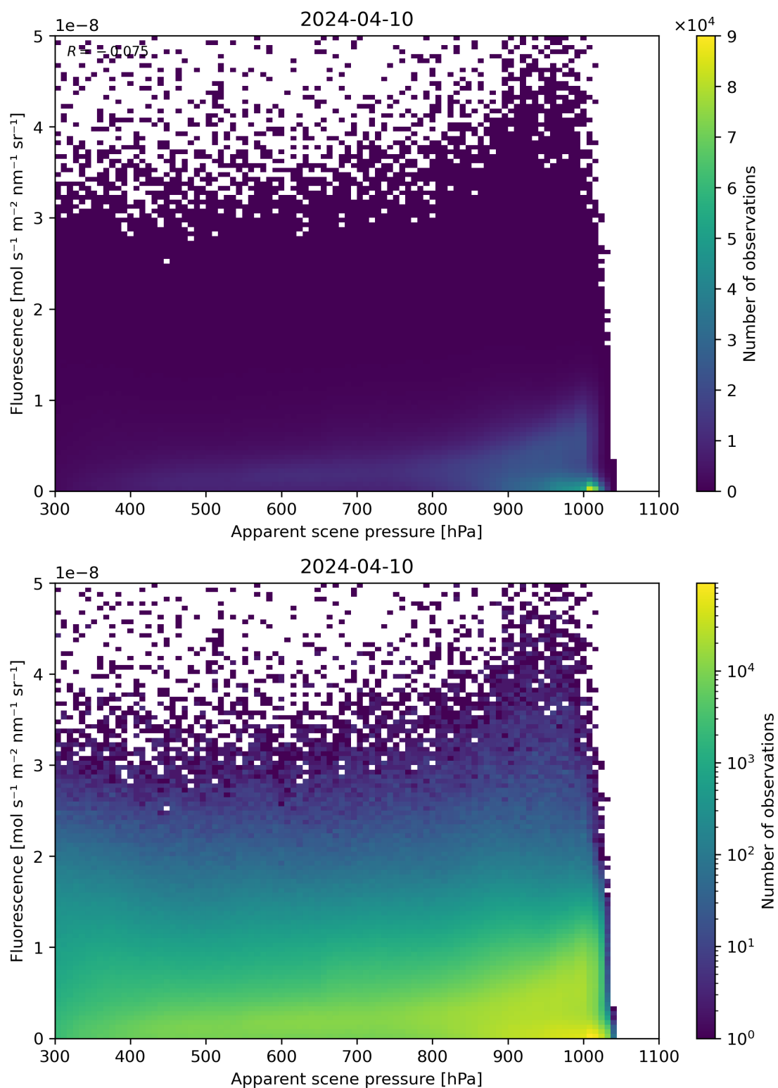
Figure 64: Scatter density plot of “Apparent scene pressure” against “Fluorescence” for 2024-04-10 to 2024-04-11.
