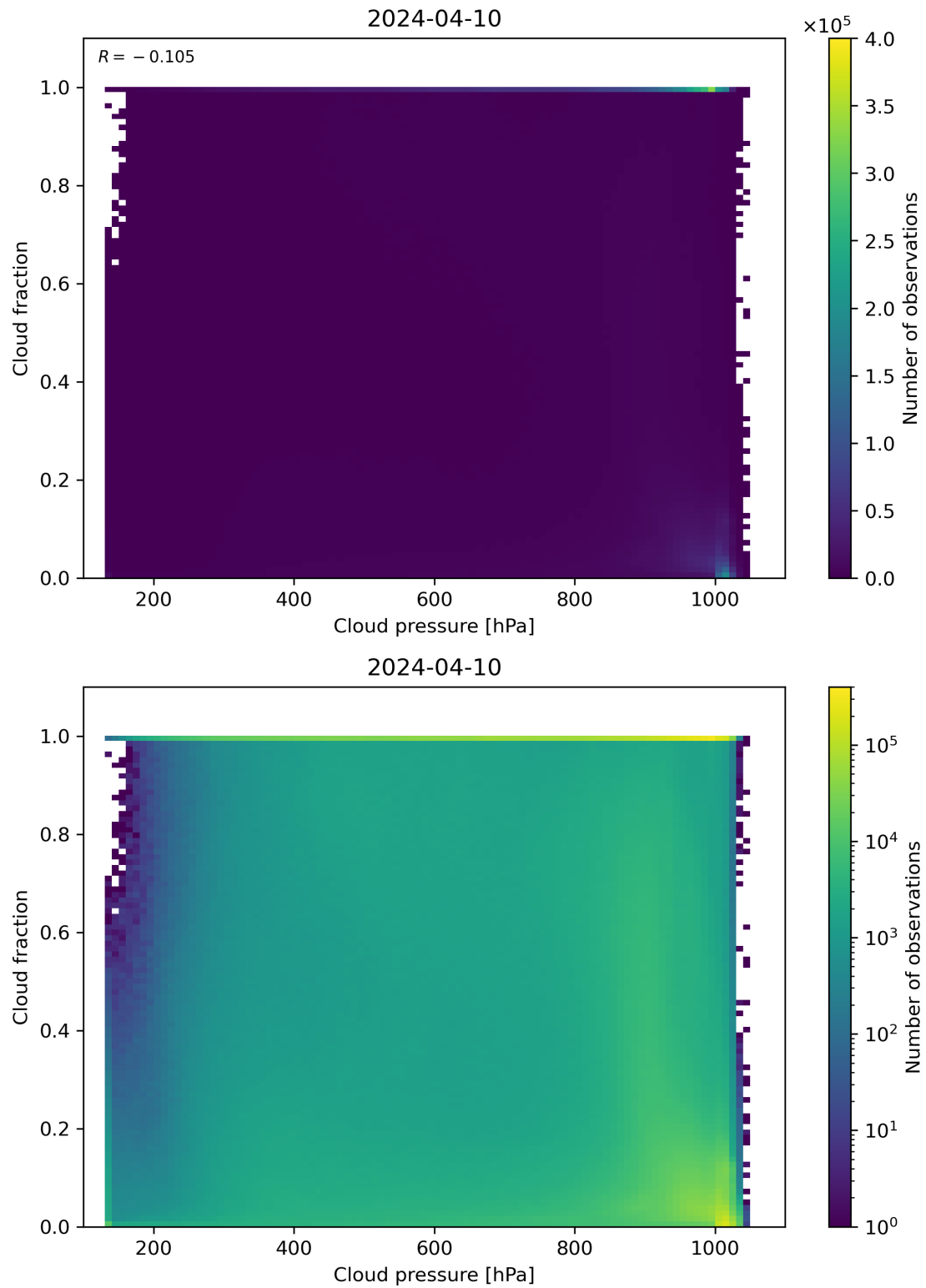
Figure 79: Scatter density plot of “Cloud pressure” against “Cloud fraction” for 2024-04-10 to 2024-04-11.
