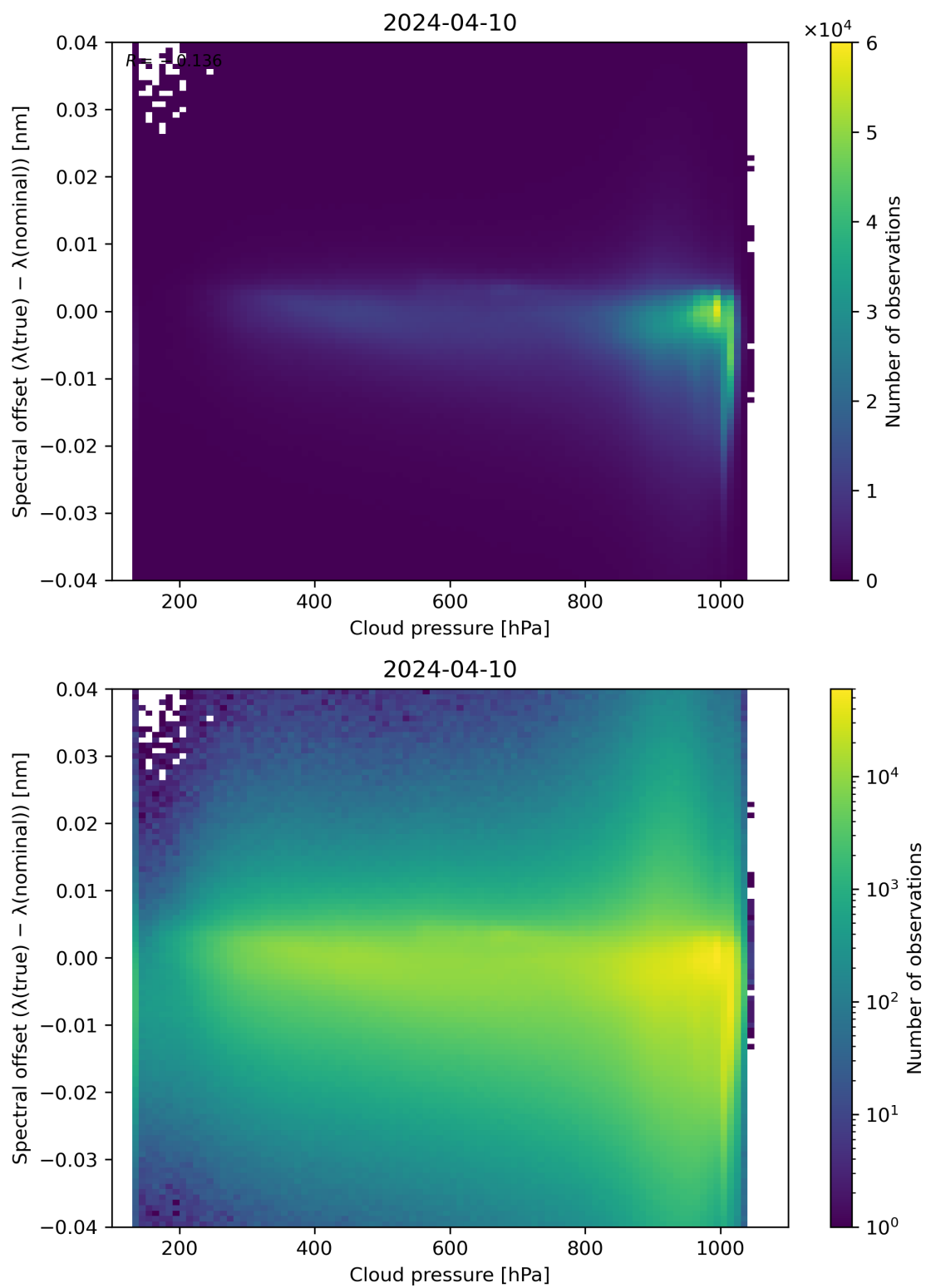
Figure 84: Scatter density plot of “Cloud pressure” against “Spectral offset ( \lambda(\text{true}) - \lambda(\text{nominal}) )” for 2024-04-10 to 2024-04-11.
