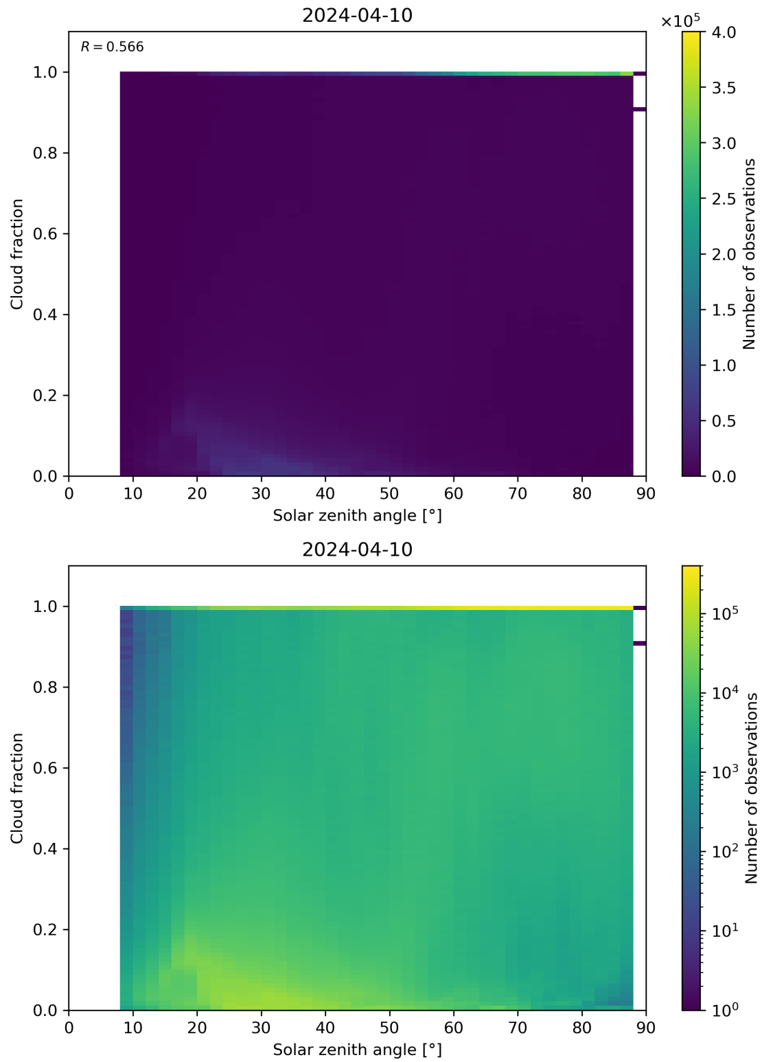
Figure 110: Scatter density plot of “Solar zenith angle” against “Cloud fraction” for 2024-04-10 to 2024-04-11.
