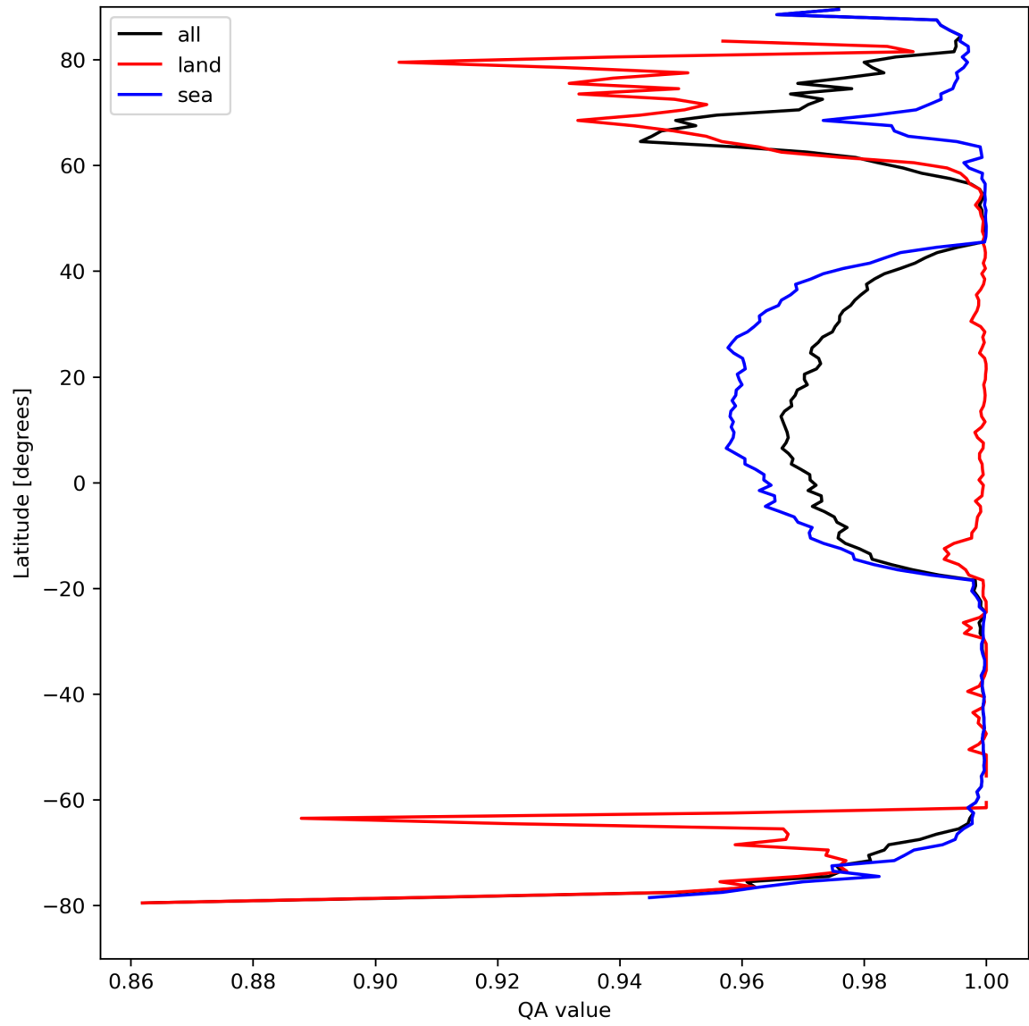
Figure 12: Zonal average of “QA value” for 2024-04-10 to 2024-04-11.
