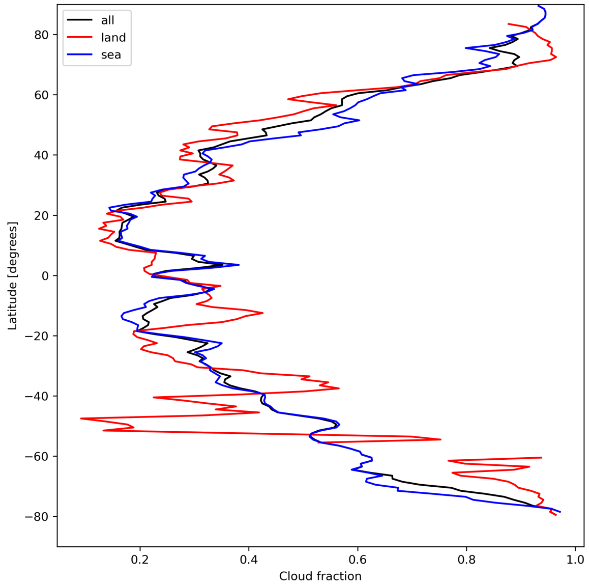
Figure 15: Zonal average of “Cloud fraction” for 2024-04-10 to 2024-04-11.
