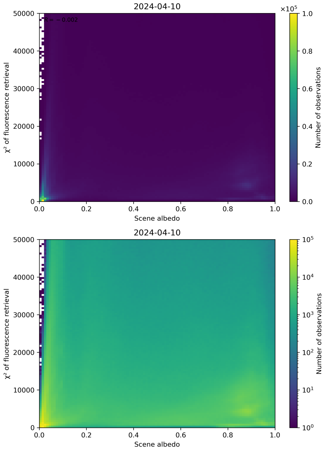
Figure 103: Scatter density plot of “Scene albedo” against “ \chi^2 of fluorescence retrieval” for 2024-04-10 to 2024-04-11.
