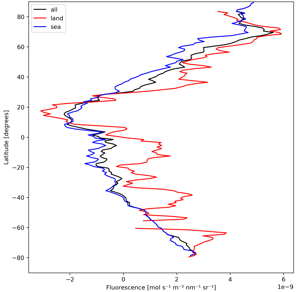
Figure 23: Zonal average of “Fluorescence” for 2024-04-10 to 2024-04-11.
