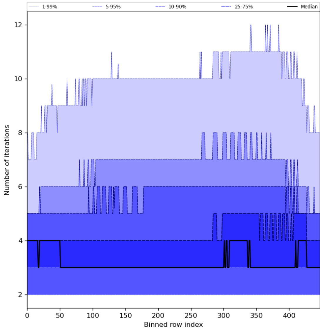
Figure 56: Along track statistics of “Number of iterations” for 2024-04-10 to 2024-04-11
