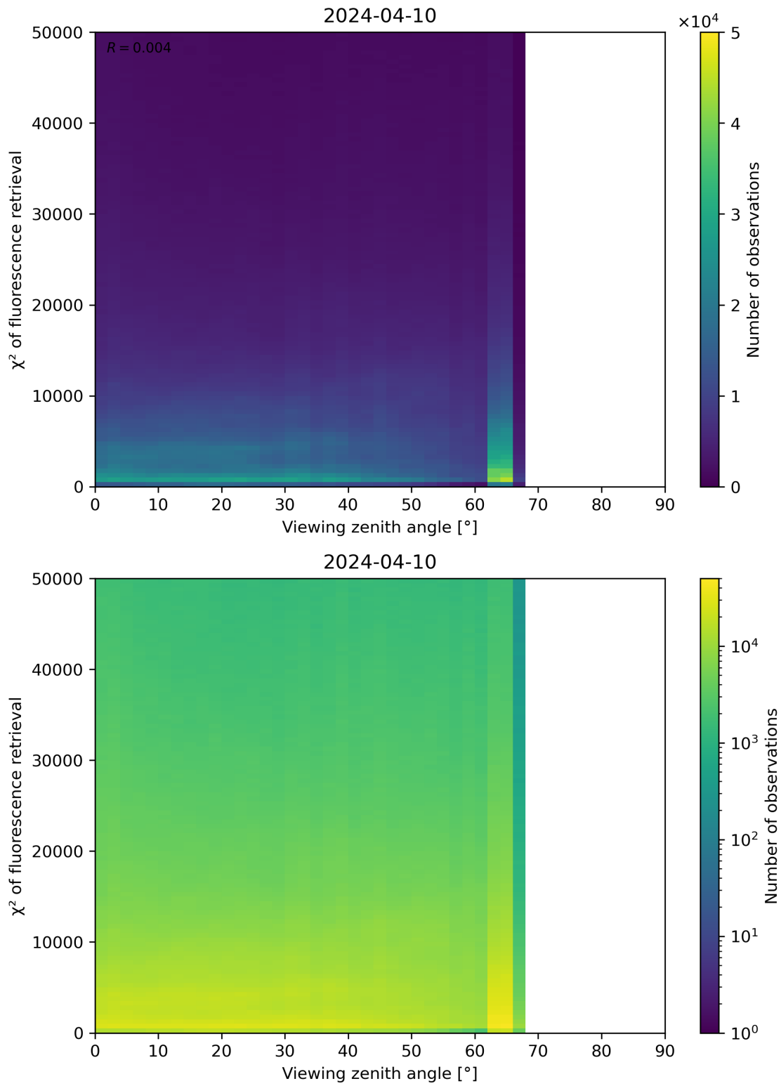
Figure 119: Scatter density plot of “Viewing zenith angle” against “ \chi^2 of fluorescence retrieval” for 2024-04-10 to 2024-04-11.
