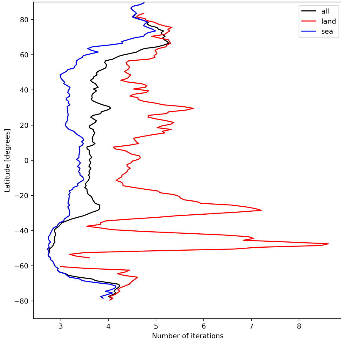
Figure 22: Zonal average of “Number of iterations” for 2024-04-10 to 2024-04-11.
