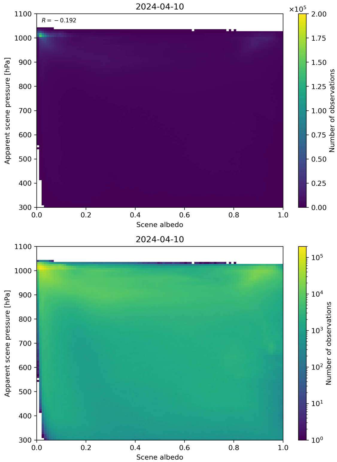
Figure 102: Scatter density plot of “Scene albedo” against “Apparent scene pressure” for 2024-04-10 to 2024-04-11.
