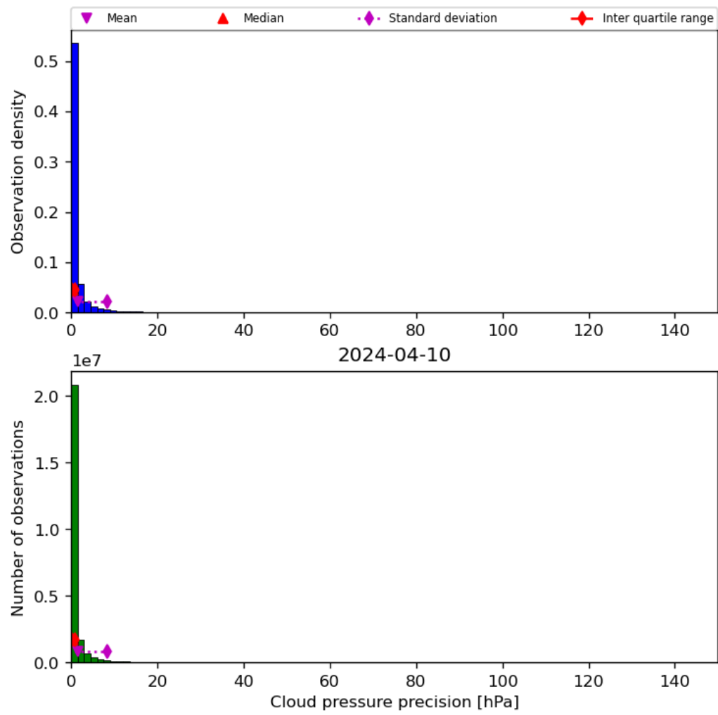
Figure 31: Histogram of “Cloud pressure precision” for 2024-04-10 to 2024-04-11
