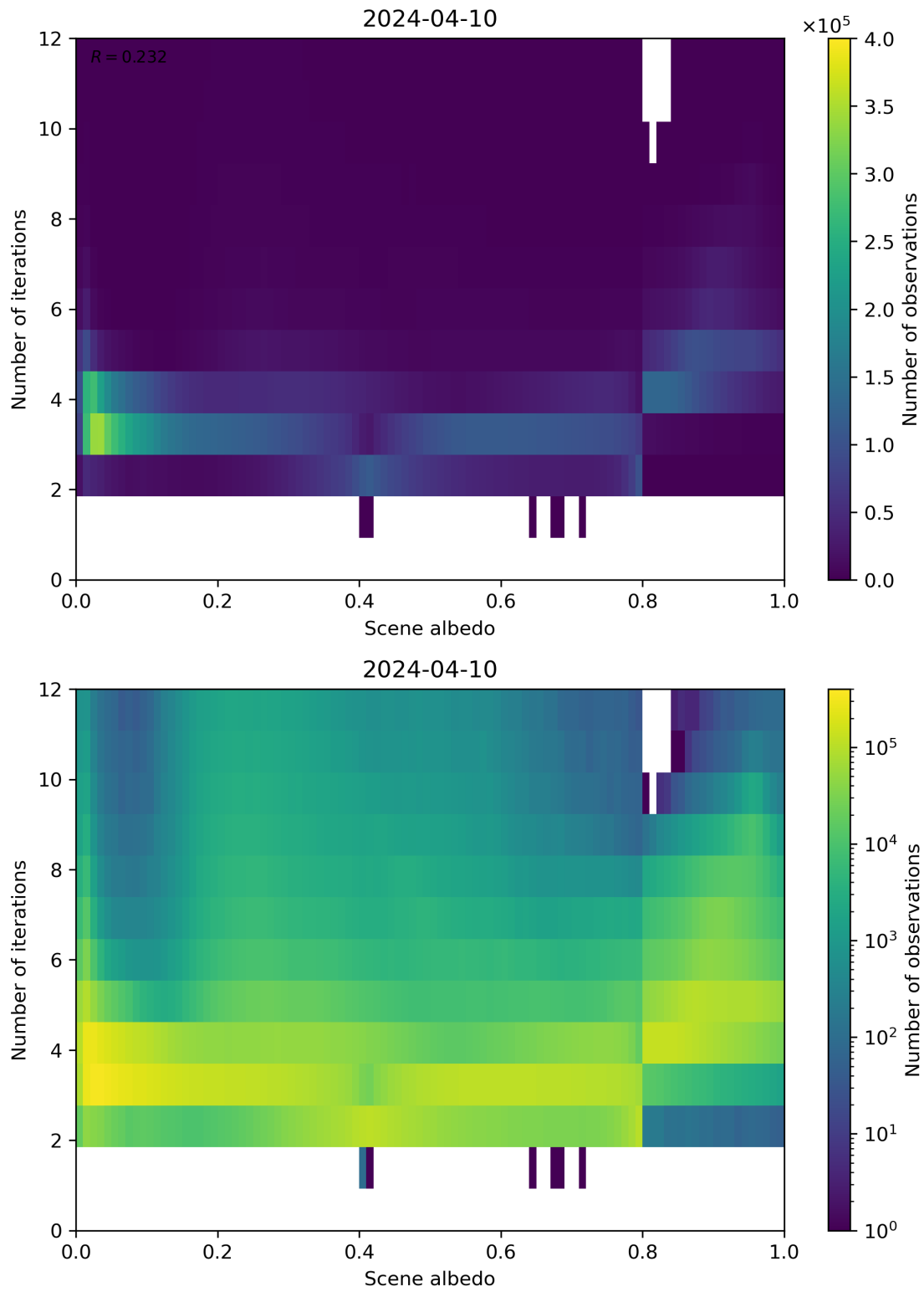
Figure 105: Scatter density plot of “Scene albedo” against “Number of iterations” for 2024-04-10 to 2024-04-11.
