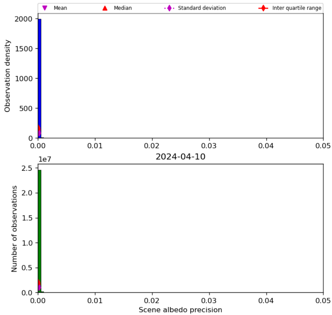
Figure 35: Histogram of “Scene albedo precision” for 2024-04-10 to 2024-04-11
