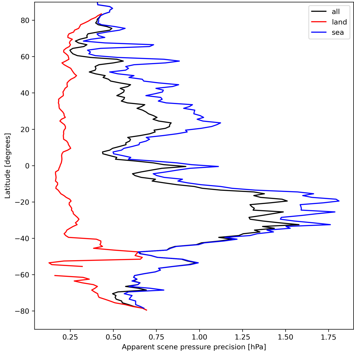
Figure 20: Zonal average of “Apparent scene pressure precision” for 2024-04-10 to 2024-04-11.
