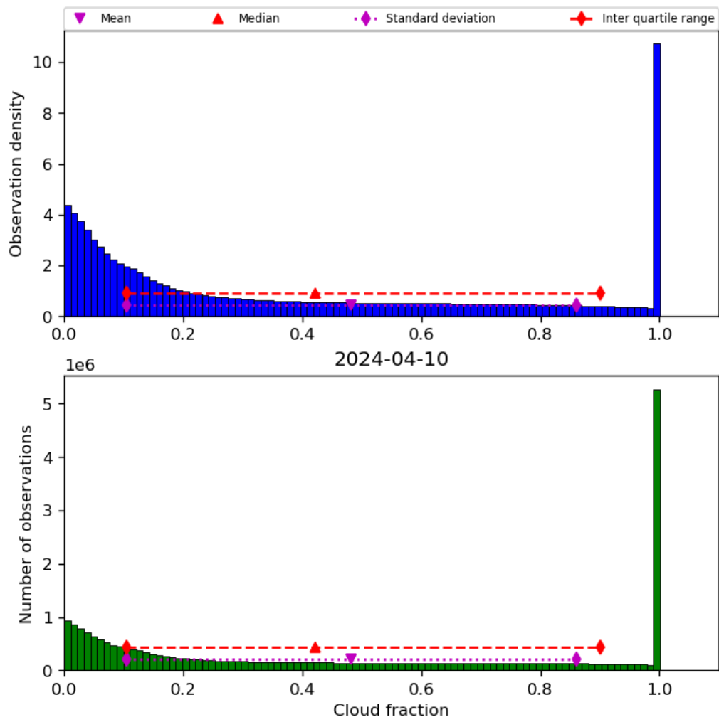
Figure 32: Histogram of “Cloud fraction” for 2024-04-10 to 2024-04-11
