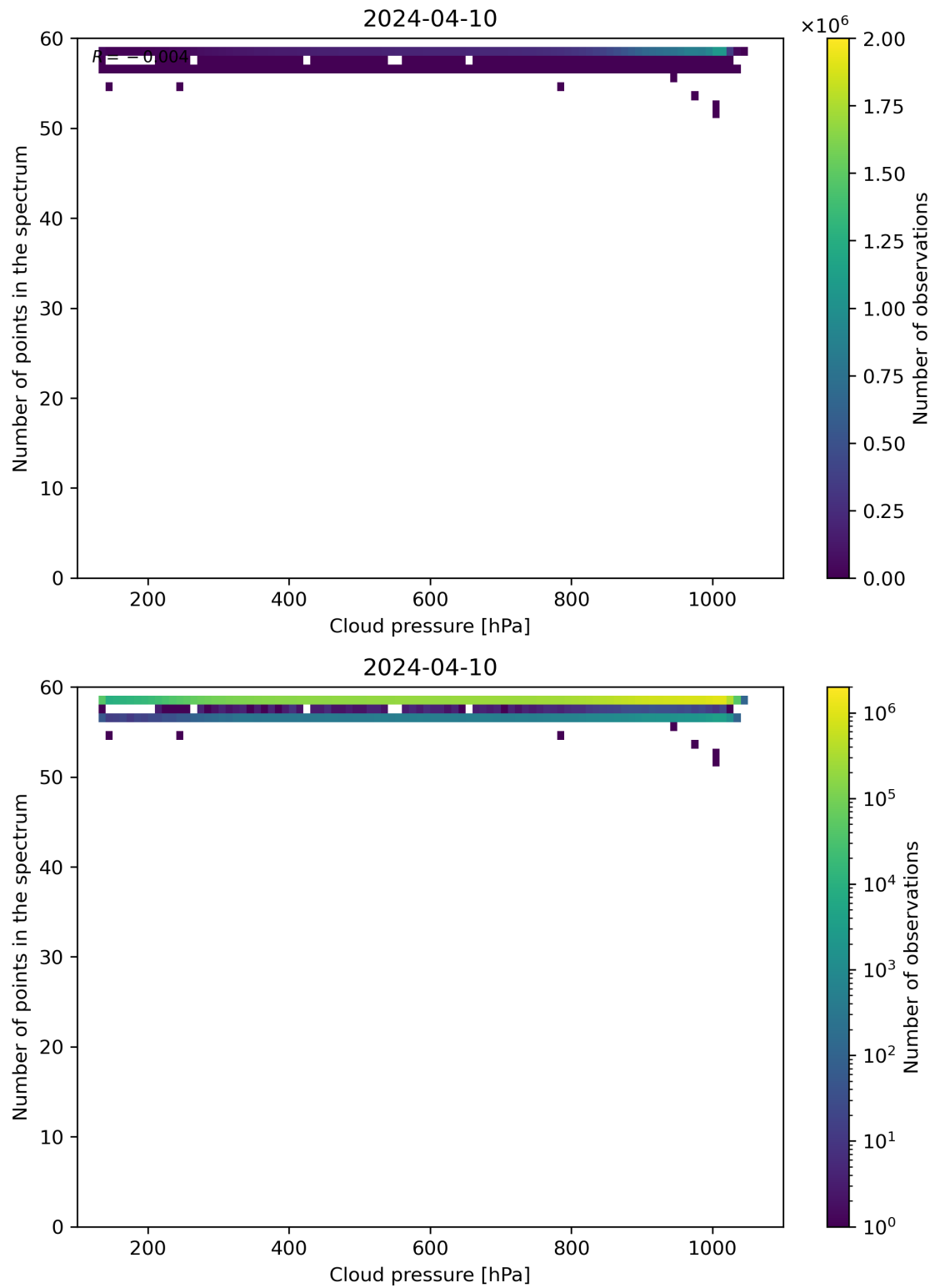
Figure 82: Scatter density plot of “Cloud pressure” against “Number of points in the spectrum” for 2024-04-10 to 2024-04-11.
