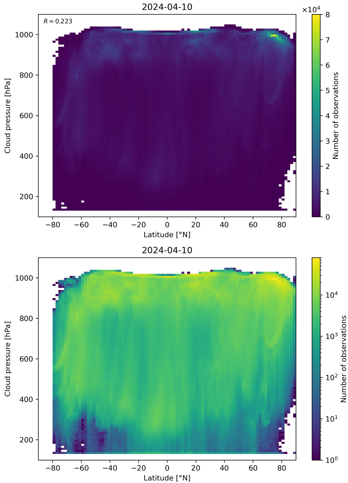
Figure 91: Scatter density plot of “Latitude” against “Cloud pressure” for 2024-04-10 to 2024-04-11.
