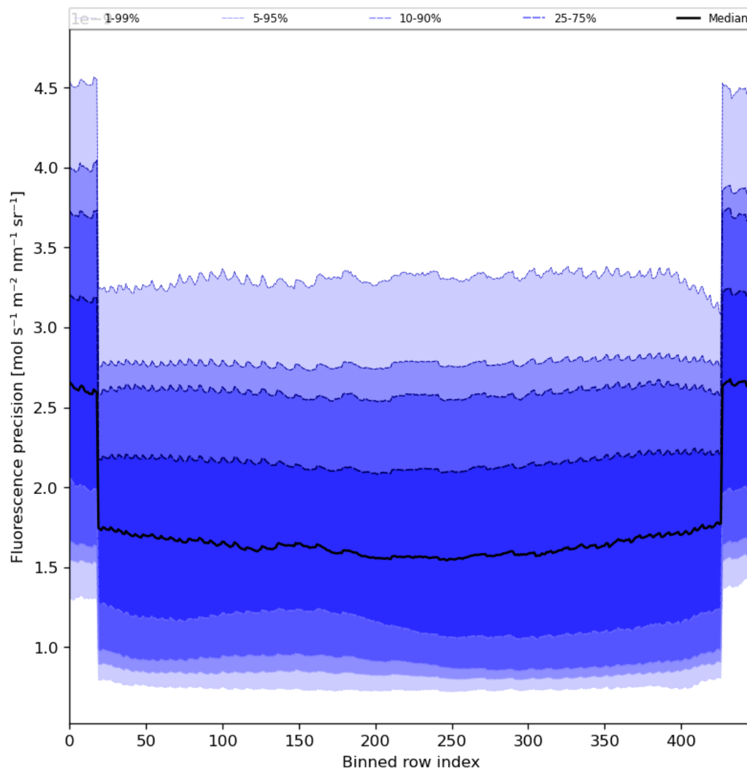
Figure 58: Along track statistics of “Fluorescence precision” for 2024-04-10 to 2024-04-11
