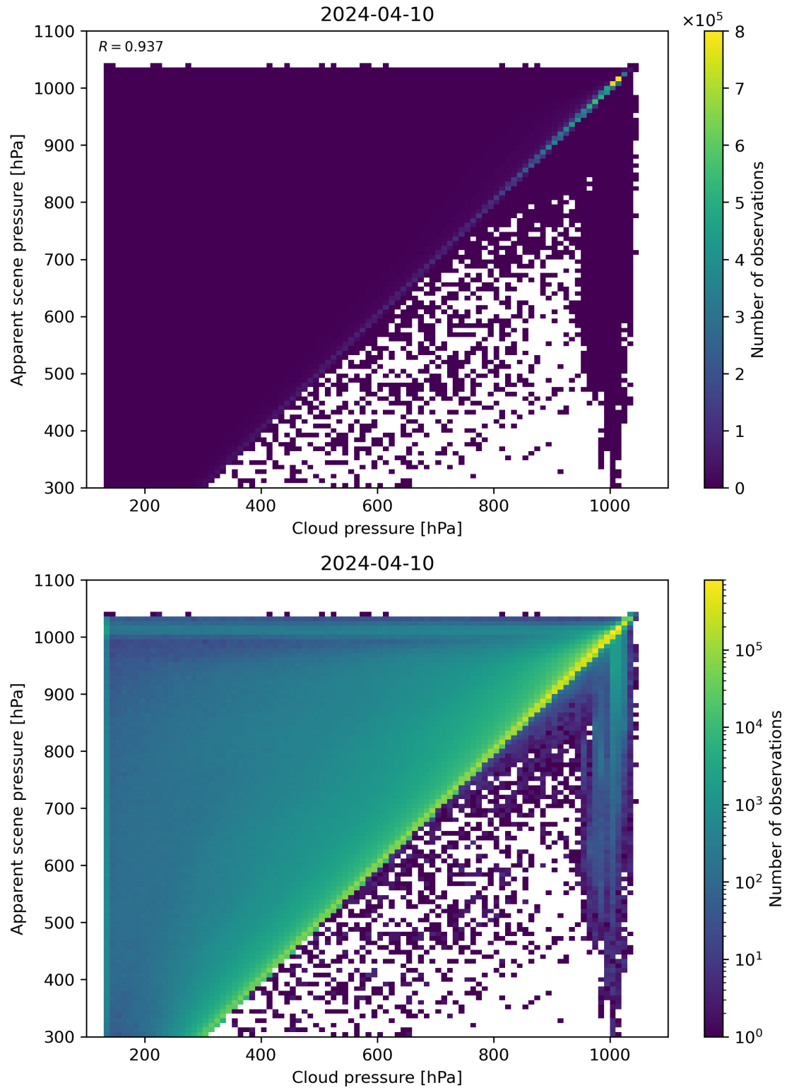
Figure 77: Scatter density plot of “Cloud pressure” against “Apparent scene pressure” for 2024-04-10 to 2024-04-11.
