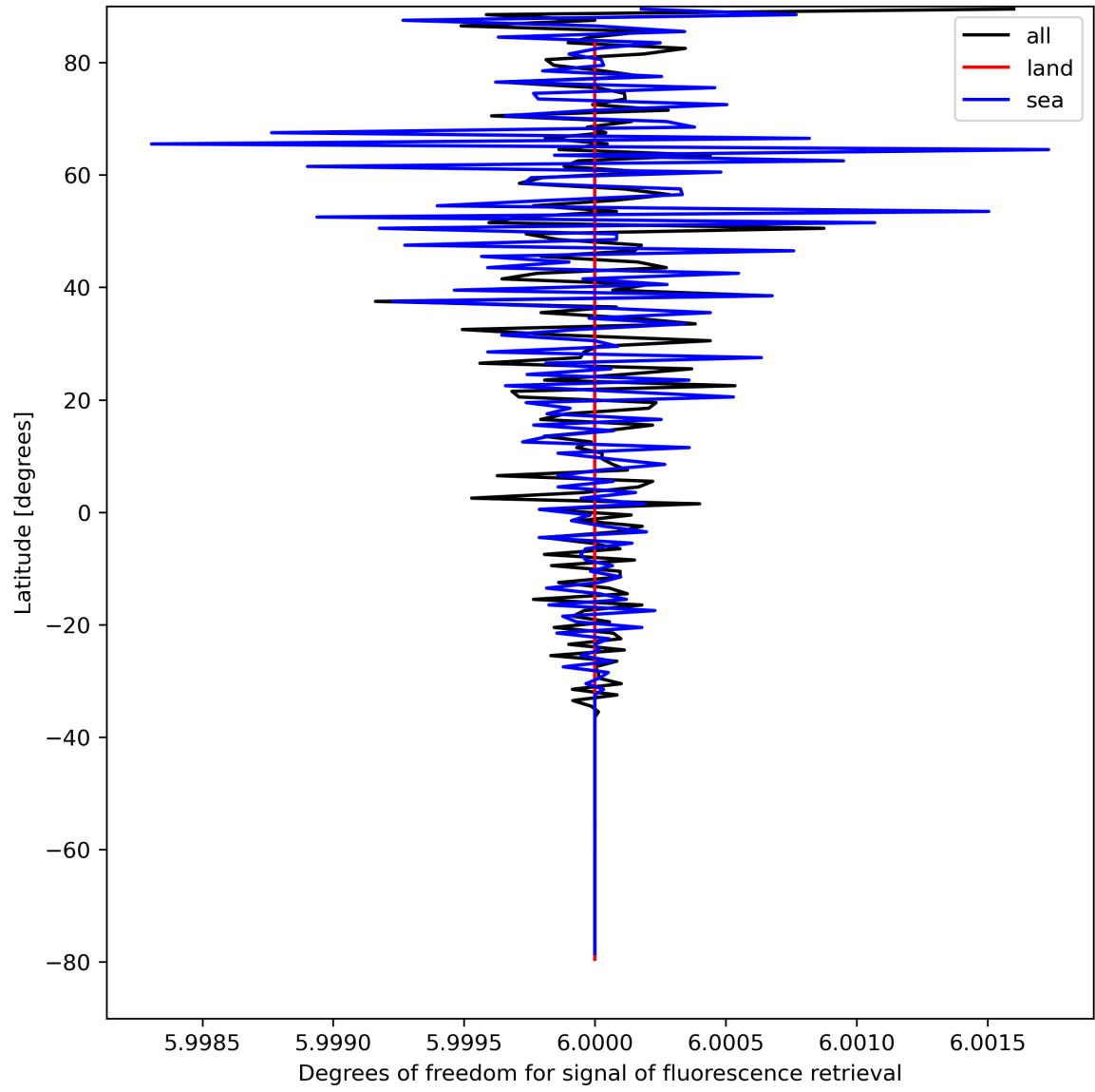
Figure 26: Zonal average of “Degrees of freedom for signal of fluorescence retrieval” for 2024-04-10 to 2024-04-11.
