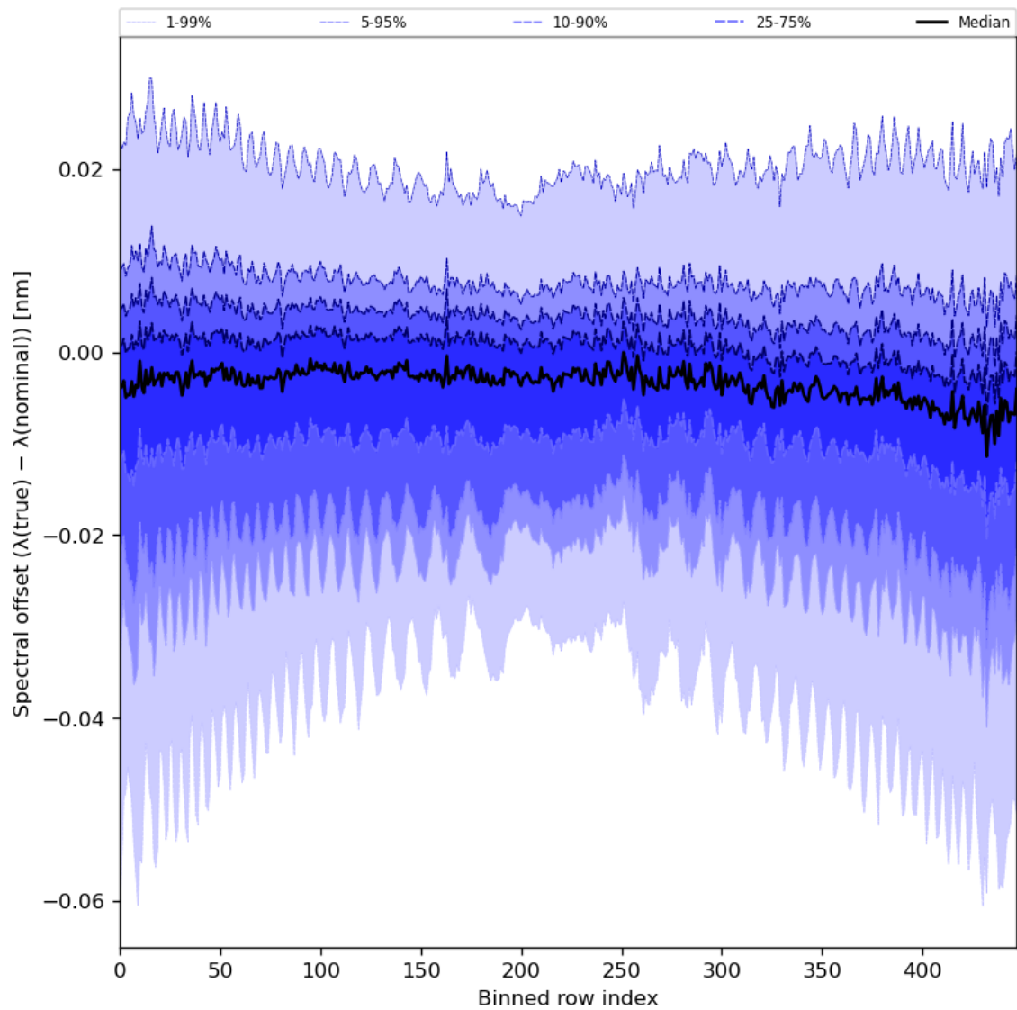
Figure 62: Along track statistics of “Spectral offset ( \lambda(\text{true}) - \lambda(\text{nominal}) )” for 2024-04-10 to 2024-04-11
