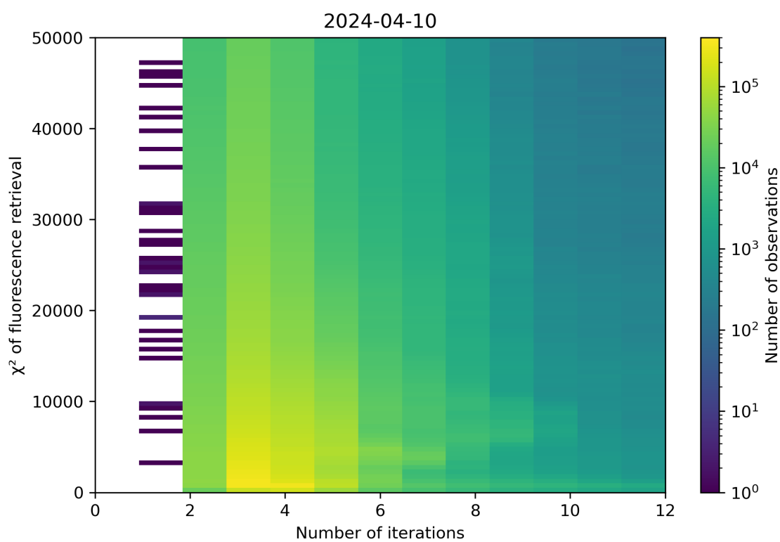
Figure 97: Scatter density plot of “Number of iterations” against “ \chi^2 of fluorescence retrieval” for 2024-04-10 to 2024-04-11.
