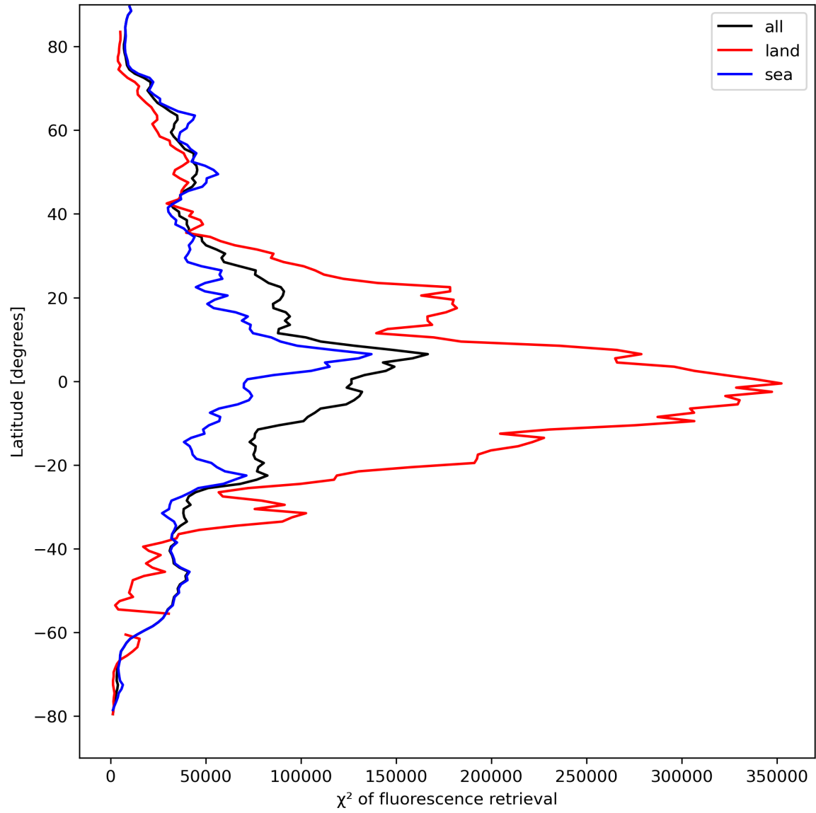
Figure 25: Zonal average of “ \chi^2 of fluorescence retrieval” for 2024-04-10 to 2024-04-11.
