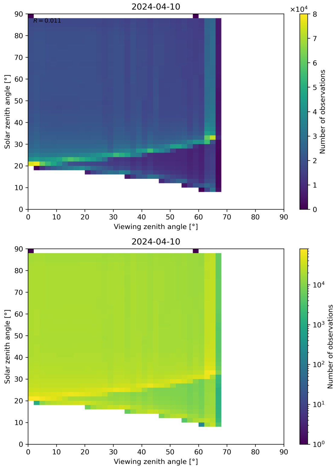
Figure 127: Scatter density plot of “Viewing zenith angle” against “Solar zenith angle” for 2024-04-10 to 2024-04-11.
