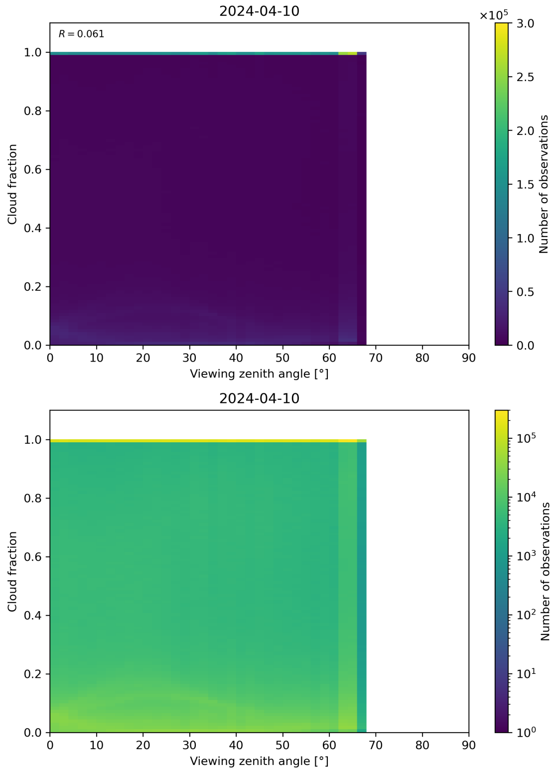
Figure 120: Scatter density plot of “Viewing zenith angle” against “Cloud fraction” for 2024-04-10 to 2024-04-11.
