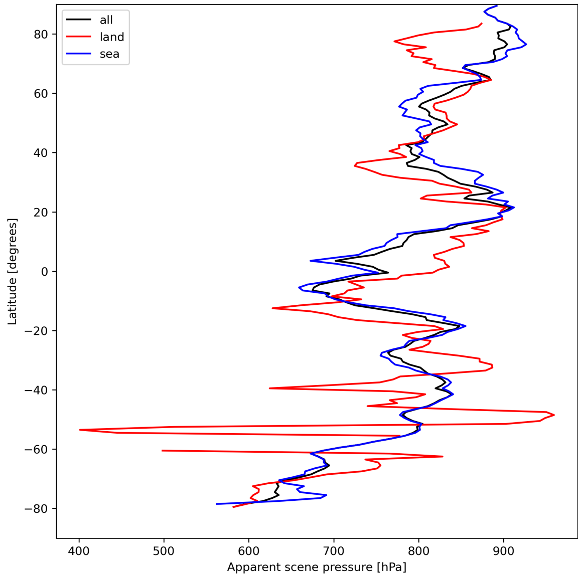
Figure 19: Zonal average of “Apparent scene pressure” for 2024-04-10 to 2024-04-11.
