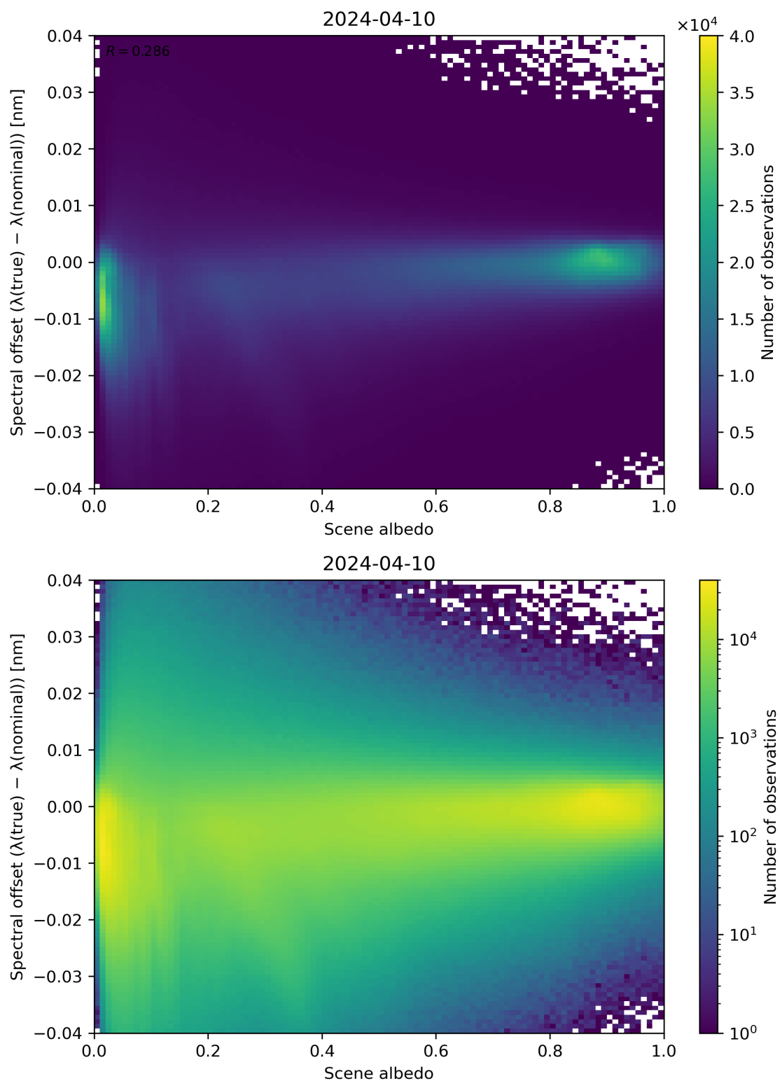
Figure 107: Scatter density plot of “Scene albedo” against “Spectral offset ( \lambda(\text{true}) - \lambda(\text{nominal}) )” for 2024-04-10 to 2024-04-11.
