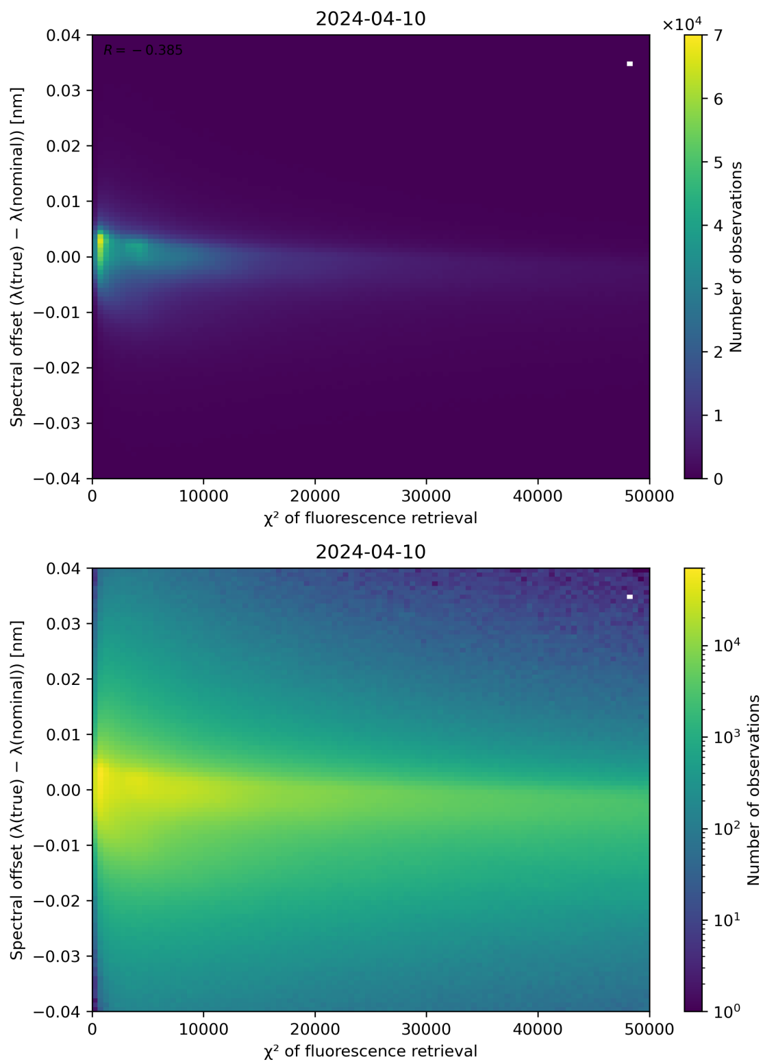
Figure 69: Scatter density plot of " \chi^2 of fluorescence retrieval" against "Spectral offset ( \lambda(\text{true}) - \lambda(\text{nominal}) )" for 2024-04-10 to 2024-04-11.
