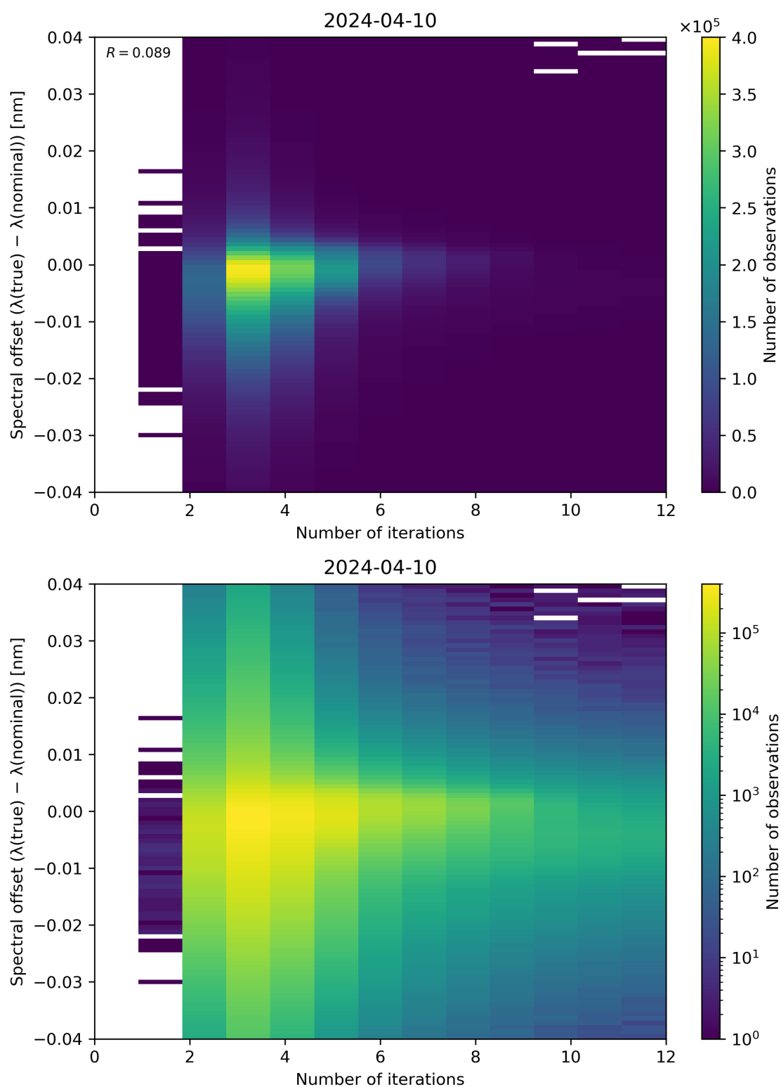
Figure 100: Scatter density plot of “Number of iterations” against “Spectral offset ( \lambda(\text{true}) - \lambda(\text{nominal}) )” for 2024-04-10 to 2024-04-11.
