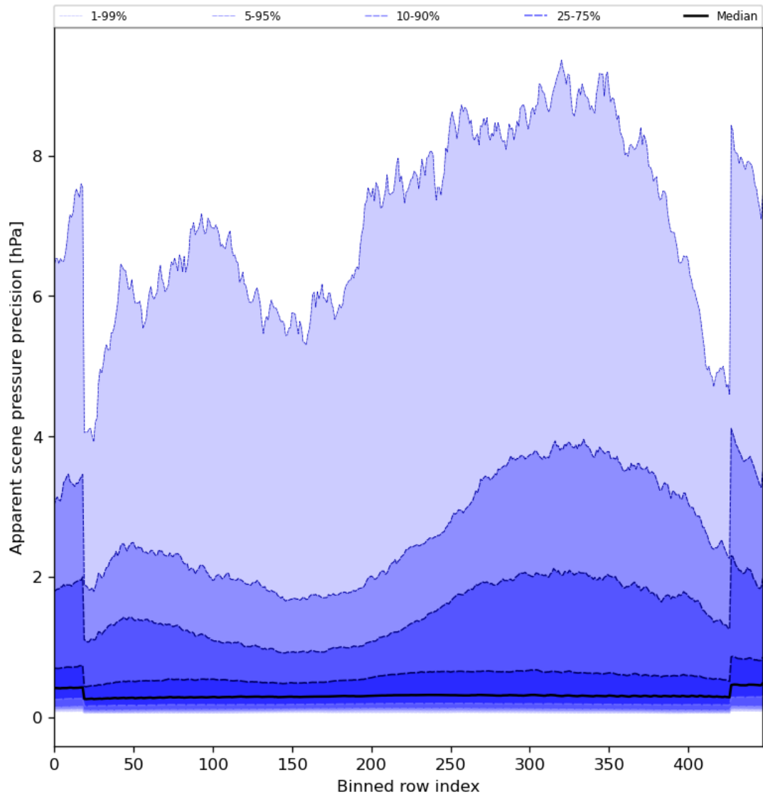
Figure 54: Along track statistics of “Apparent scene pressure precision” for 2024-04-10 to 2024-04-11
