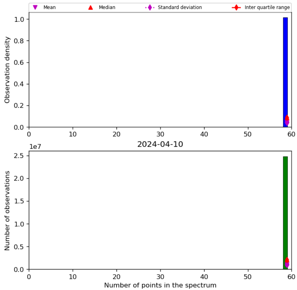
Figure 44: Histogram of “Number of points in the spectrum” for 2024-04-10 to 2024-04-11
