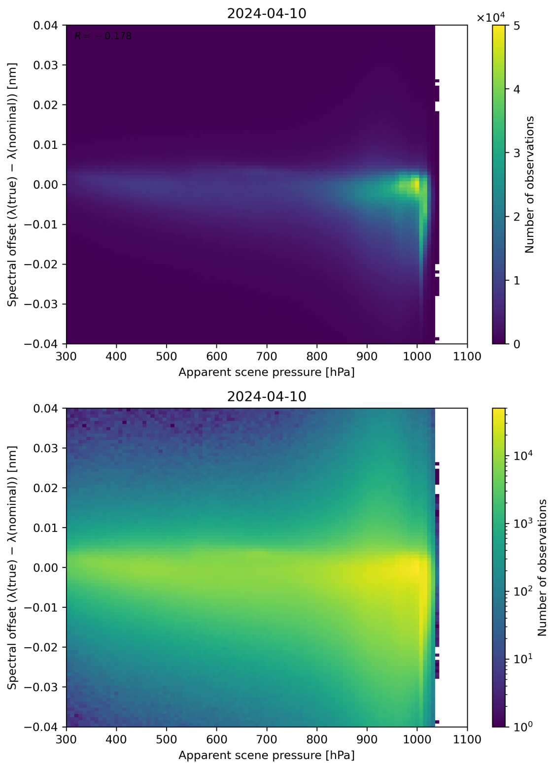
Figure 67: Scatter density plot of “Apparent scene pressure” against “Spectral offset ( \lambda(\text{true}) - \lambda(\text{nominal}) )” for 2024-04-10 to 2024-04-11.
