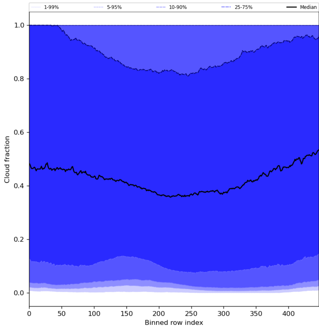
Figure 49: Along track statistics of “Cloud fraction” for 2024-04-10 to 2024-04-11
