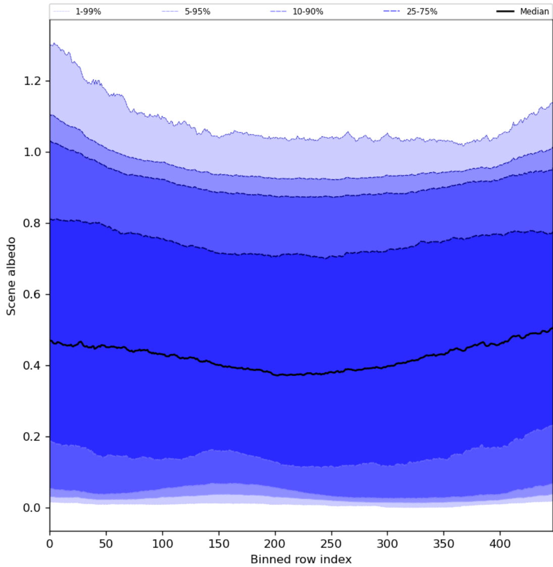
Figure 51: Along track statistics of “Scene albedo” for 2024-04-10 to 2024-04-11
