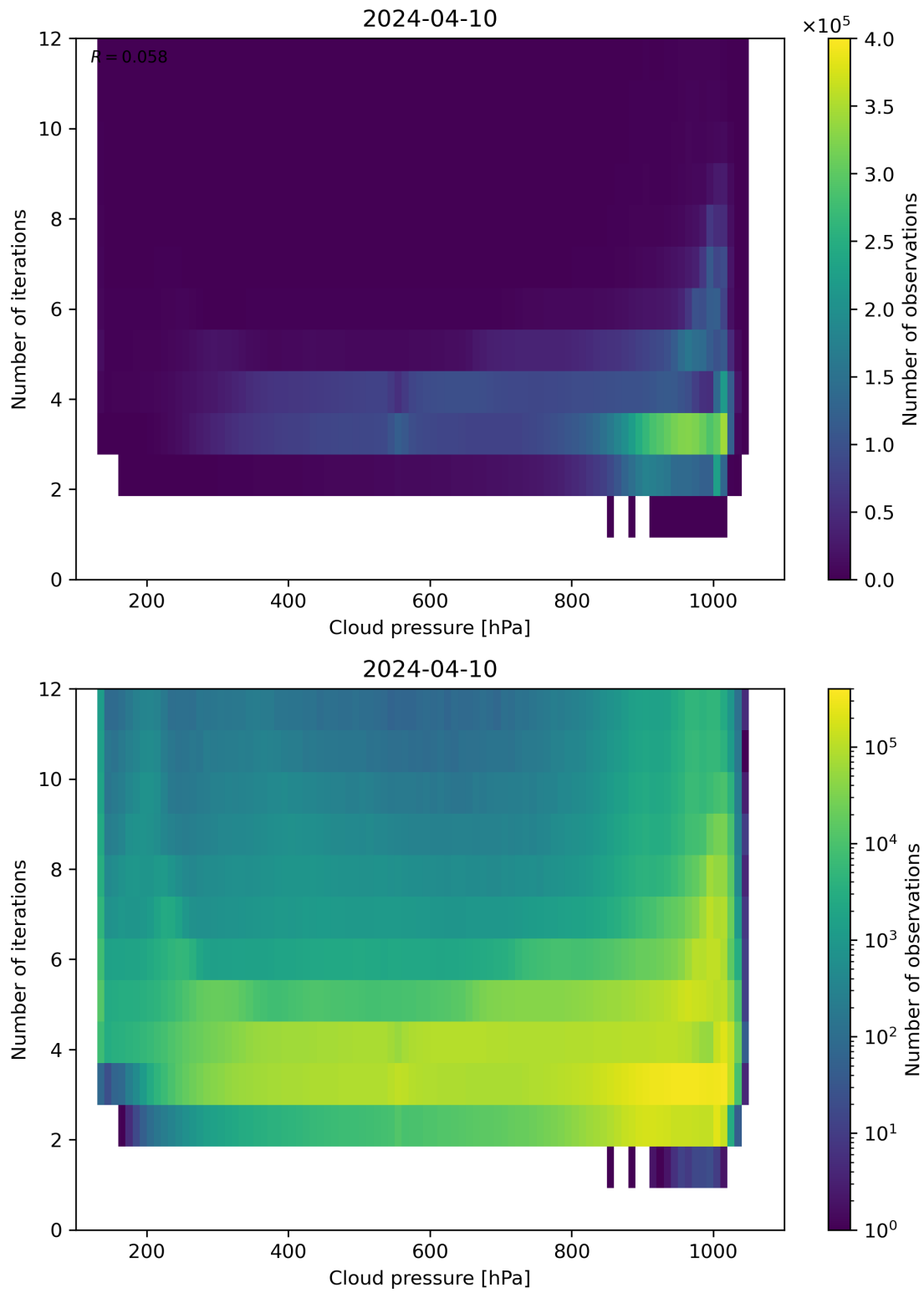
Figure 81: Scatter density plot of “Cloud pressure” against “Number of iterations” for 2024-04-10 to 2024-04-11.
