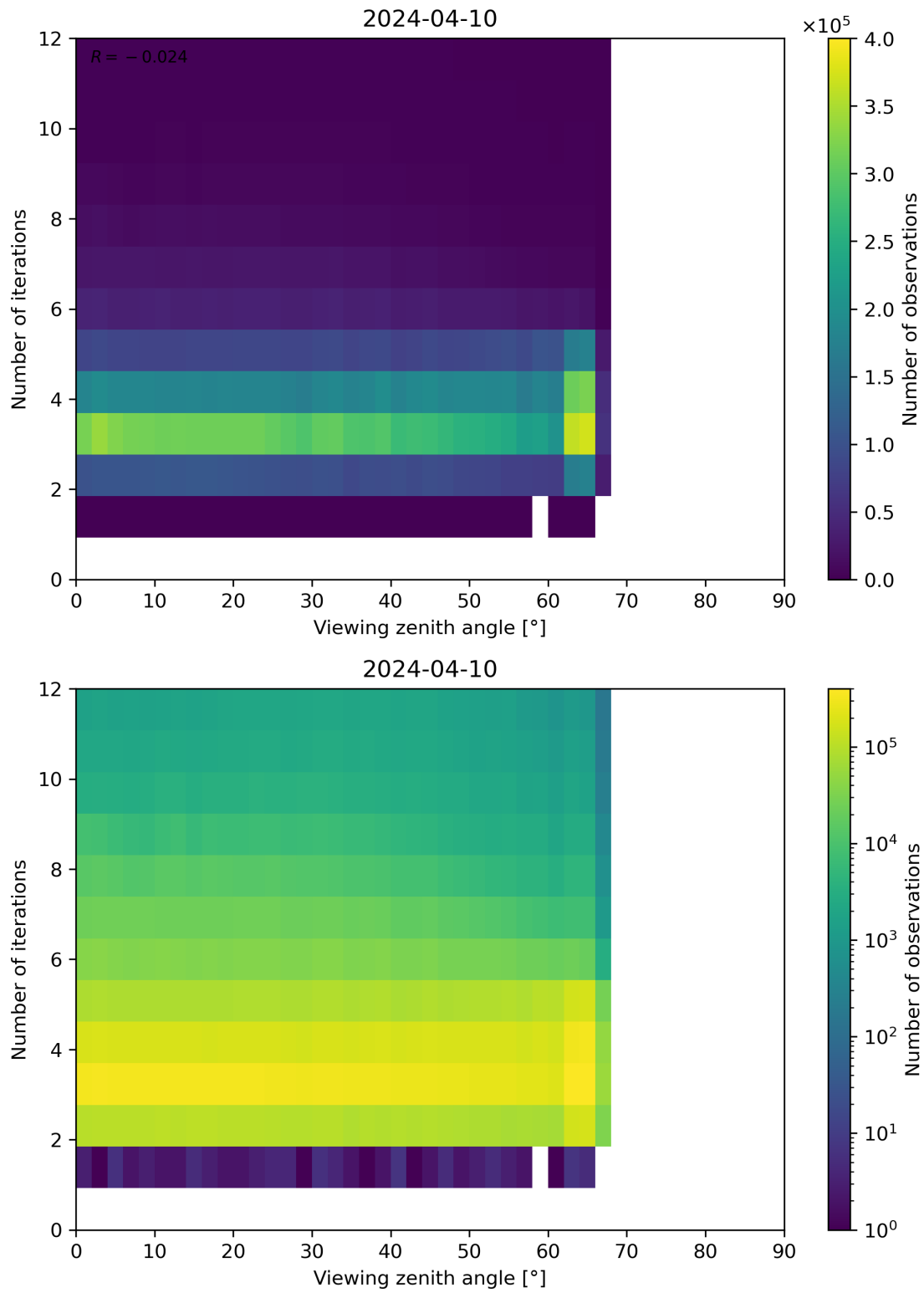
Figure 124: Scatter density plot of “Viewing zenith angle” against “Number of iterations” for 2024-04-10 to 2024-04-11.
