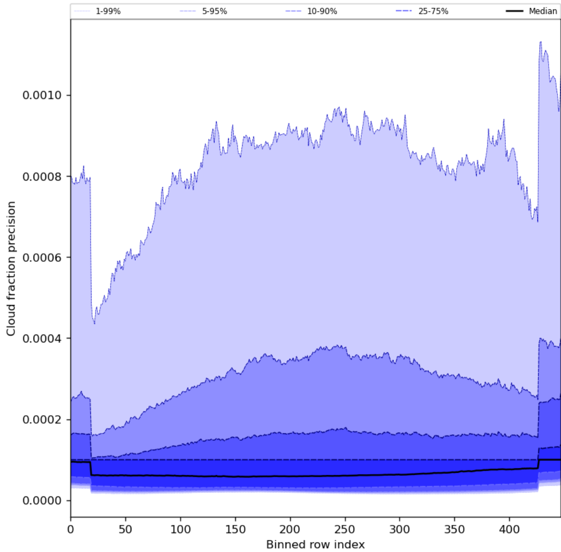
Figure 50: Along track statistics of “Cloud fraction precision” for 2024-04-10 to 2024-04-11
