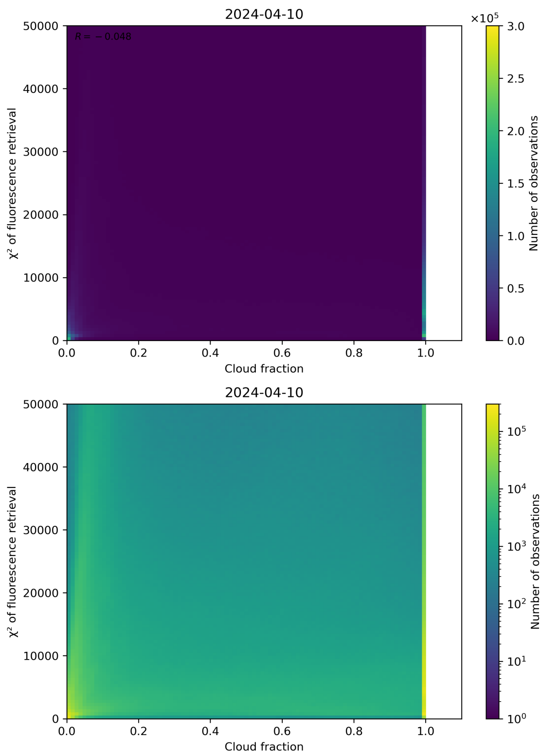
Figure 71: Scatter density plot of “Cloud fraction” against “ \chi^2 of fluorescence retrieval” for 2024-04-10 to 2024-04-11.
