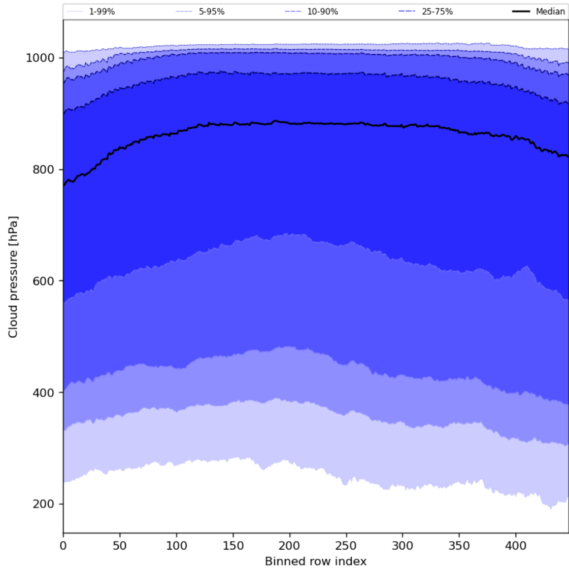
Figure 47: Along track statistics of “Cloud pressure” for 2024-04-10 to 2024-04-11
