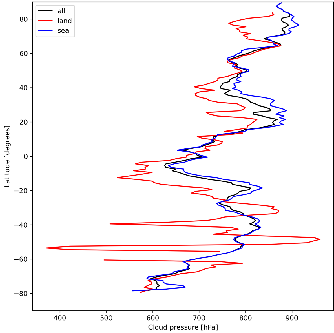
Figure 13: Zonal average of “Cloud pressure” for 2024-04-10 to 2024-04-11.
