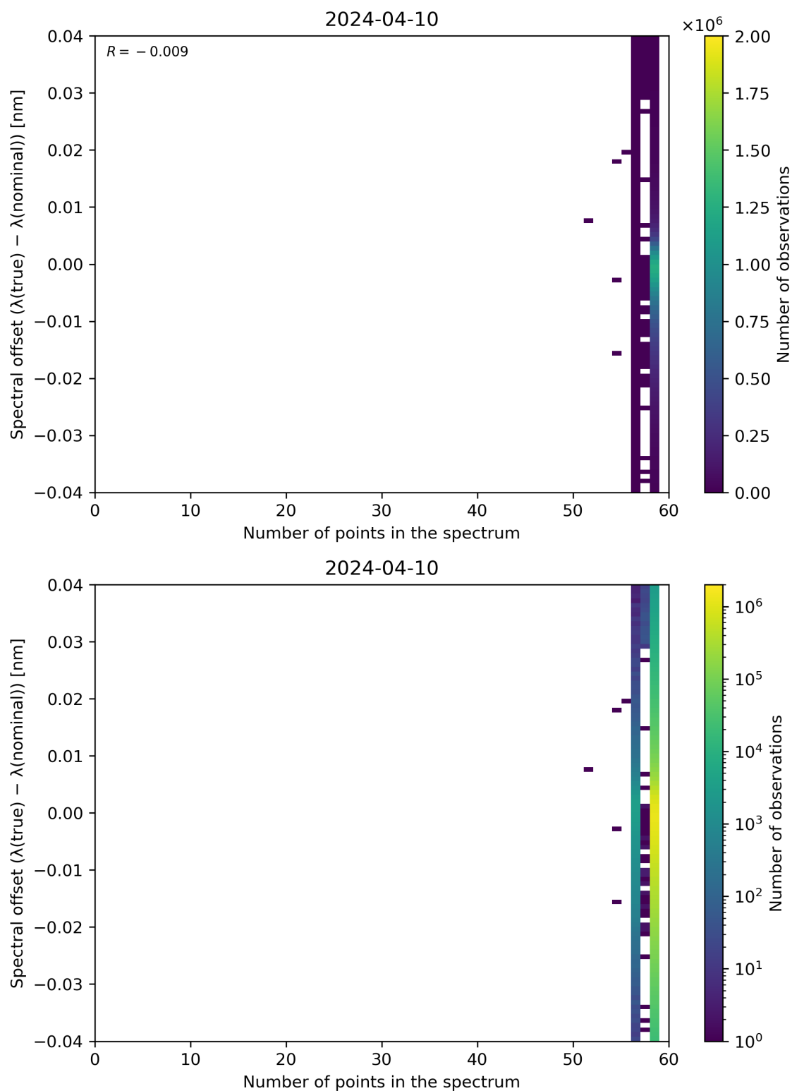
Figure 101: Scatter density plot of “Number of points in the spectrum” against “Spectral offset ( \lambda(\text{true}) - \lambda(\text{nominal}) )” for 2024-04-10 to 2024-04-11.
