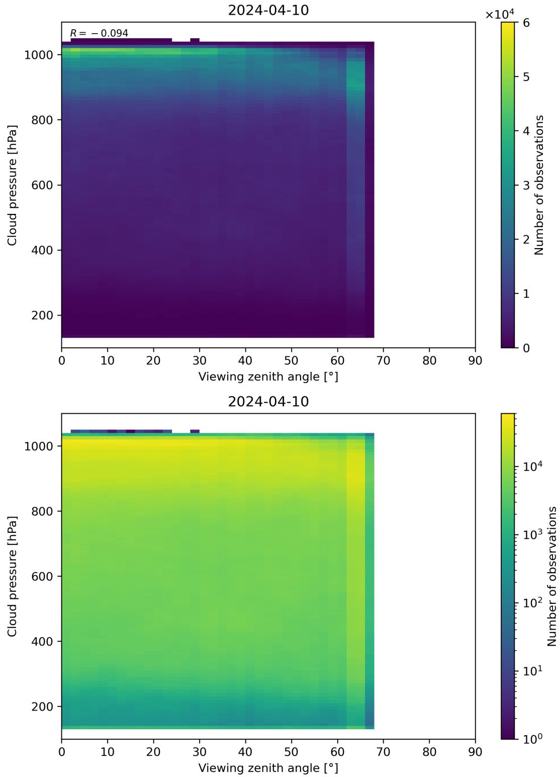
Figure 121: Scatter density plot of “Viewing zenith angle” against “Cloud pressure” for 2024-04-10 to 2024-04-11.
