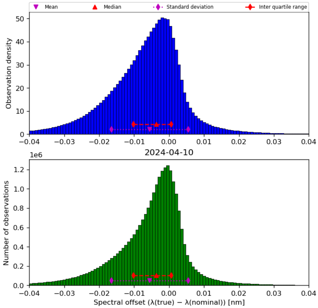
Figure 45: Histogram of “Spectral offset ( \lambda(\text{true}) - \lambda(\text{nominal}) )” for 2024-04-10 to 2024-04-11
