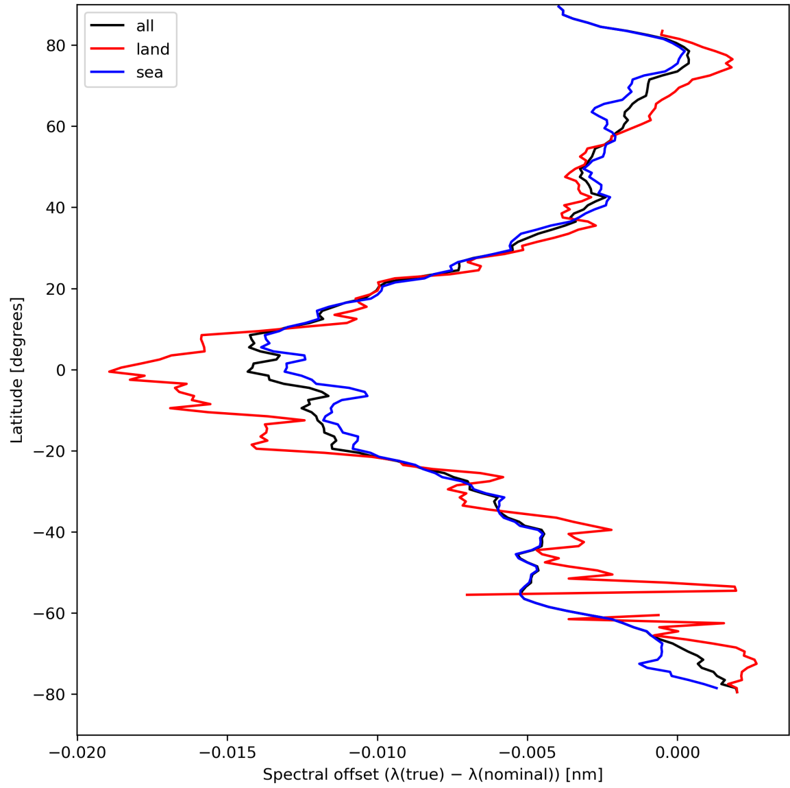
Figure 28: Zonal average of “Spectral offset ( \lambda(\text{true}) - \lambda(\text{nominal}) )” for 2024-04-10 to 2024-04-11.
