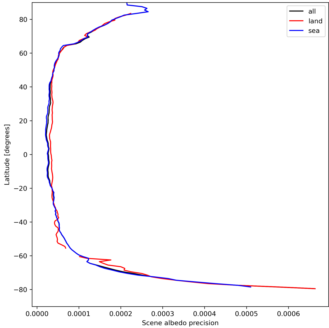
Figure 18: Zonal average of “Scene albedo precision” for 2024-04-10 to 2024-04-11.
