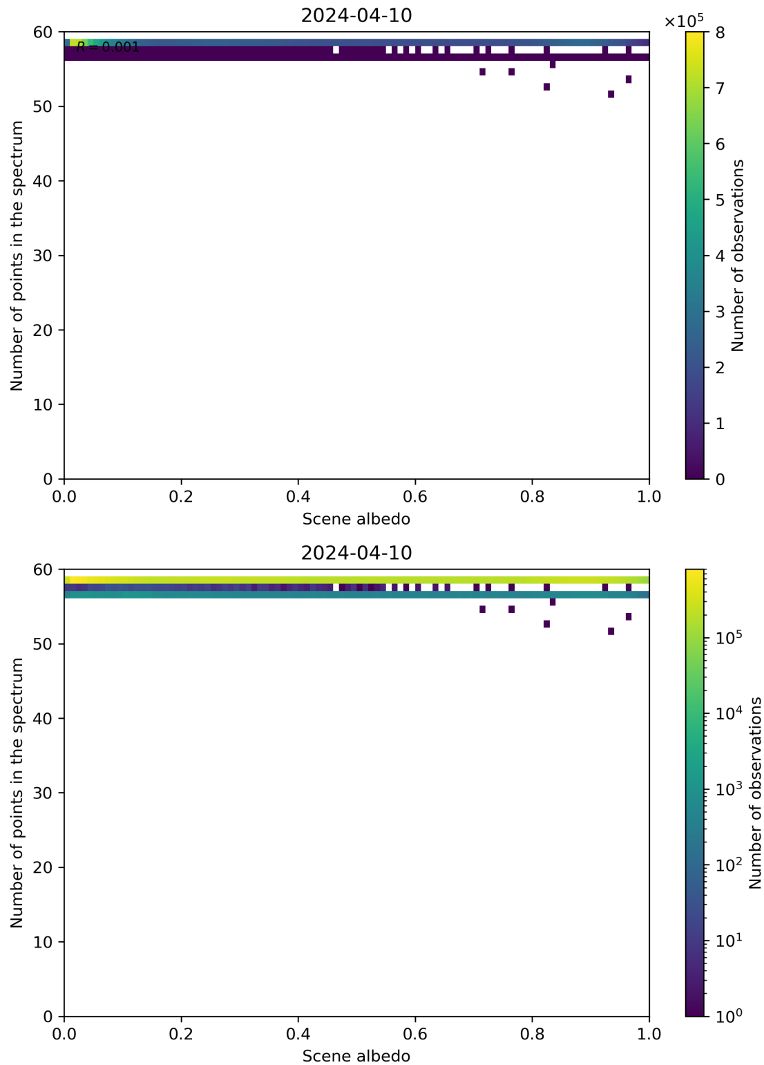
Figure 106: Scatter density plot of “Scene albedo” against “Number of points in the spectrum” for 2024-04-10 to 2024-04-11.
