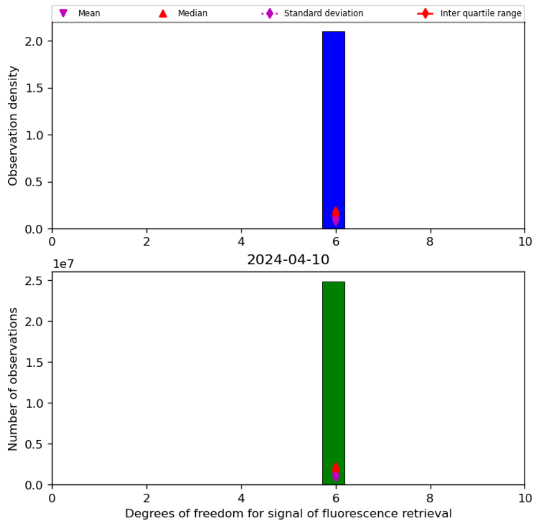
Figure 43: Histogram of “Degrees of freedom for signal of fluorescence retrieval” for 2024-04-10 to 2024-04-11
