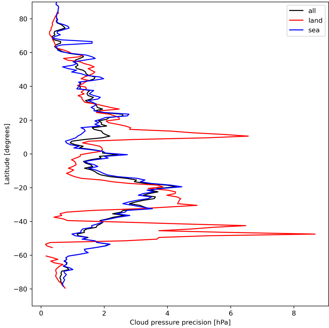
Figure 14: Zonal average of “Cloud pressure precision” for 2024-04-10 to 2024-04-11.
