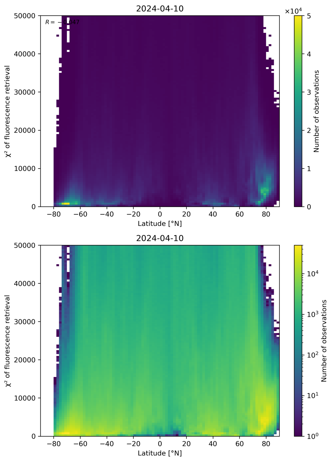
Figure 89: Scatter density plot of “Latitude” against “ \chi^2 of fluorescence retrieval” for 2024-04-10 to 2024-04-11.
