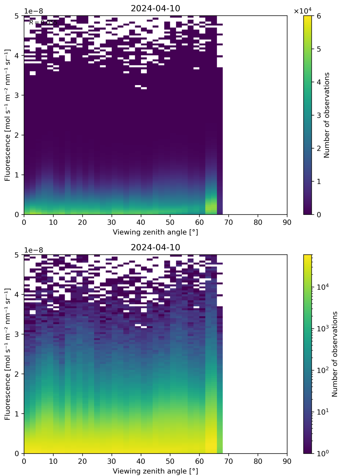
Figure 122: Scatter density plot of “Viewing zenith angle” against “Fluorescence” for 2024-04-10 to 2024-04-11.
