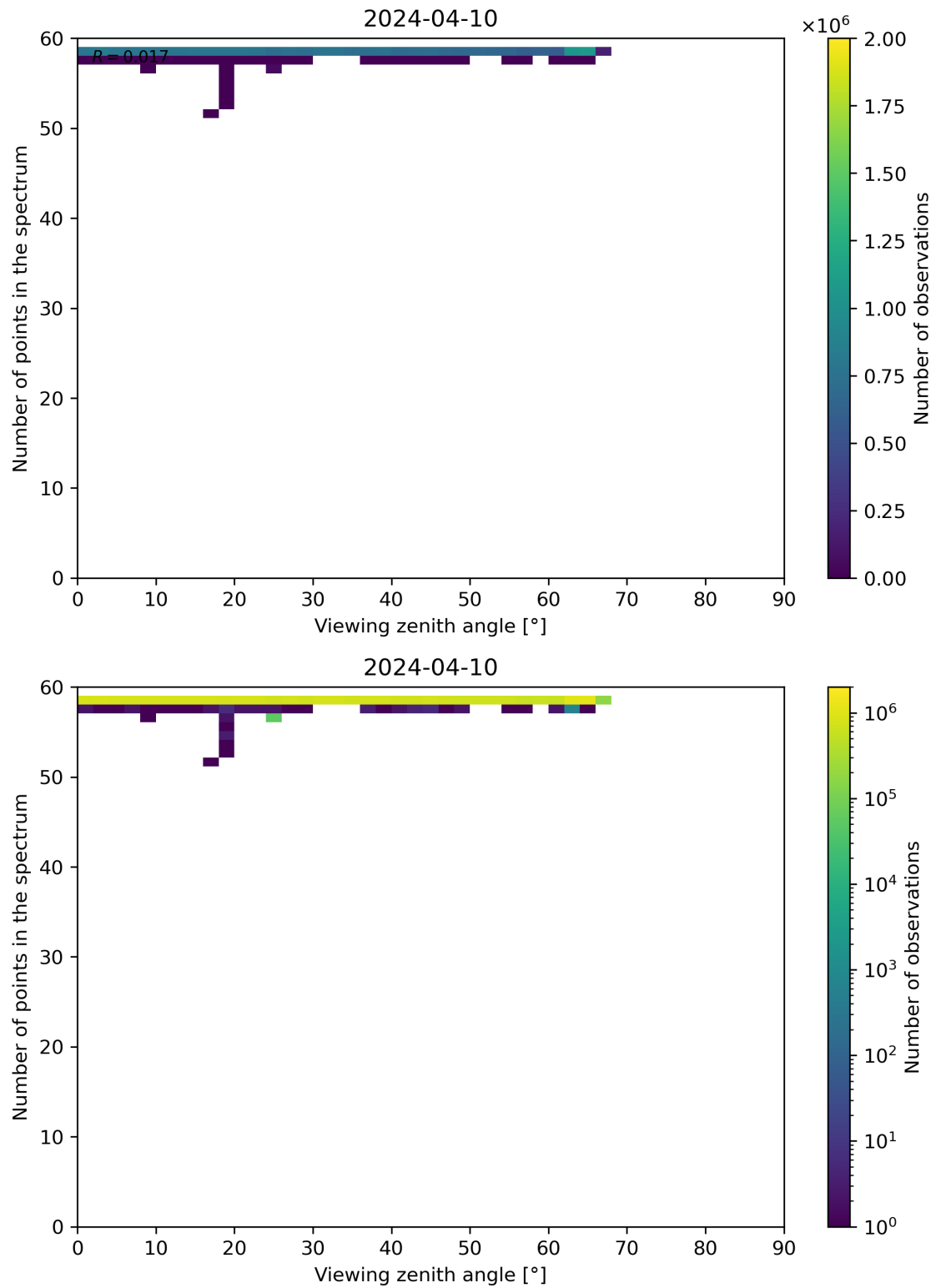
Figure 125: Scatter density plot of “Viewing zenith angle” against “Number of points in the spectrum” for 2024-04-10 to 2024-04-11.
