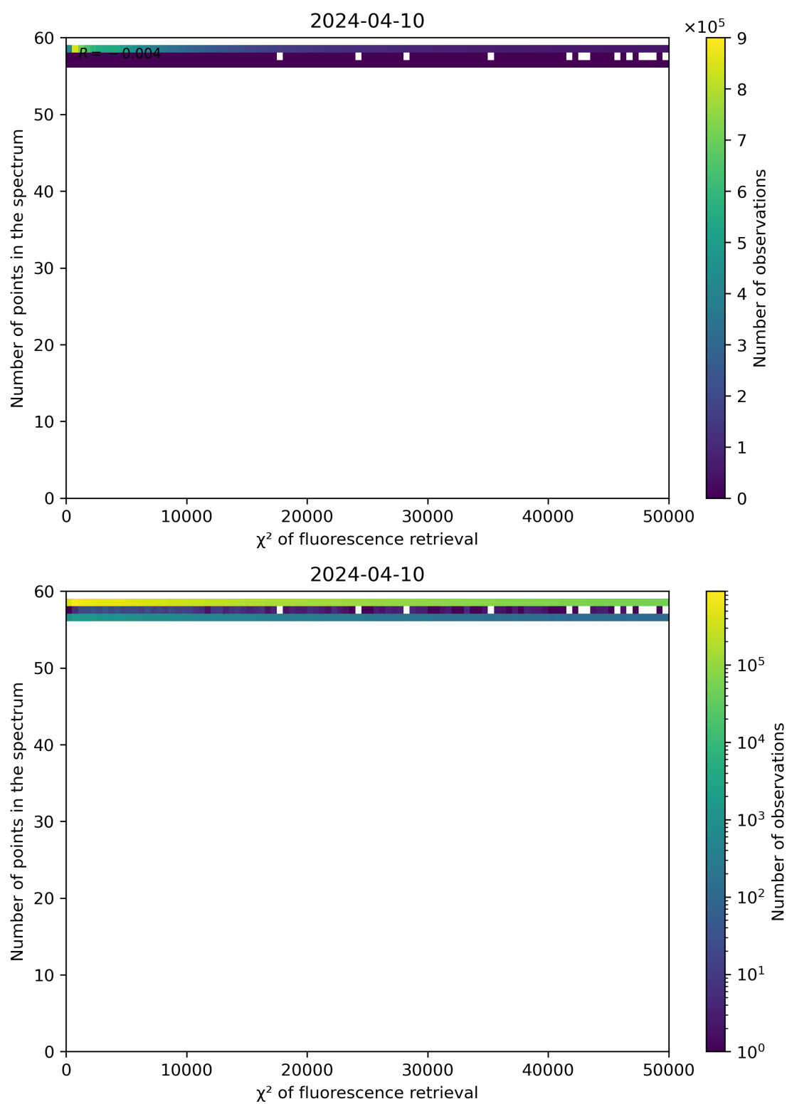
Figure 68: Scatter density plot of " \chi^2 of fluorescence retrieval" against "Number of points in the spectrum" for 2024-04-10 to 2024-04-11.
