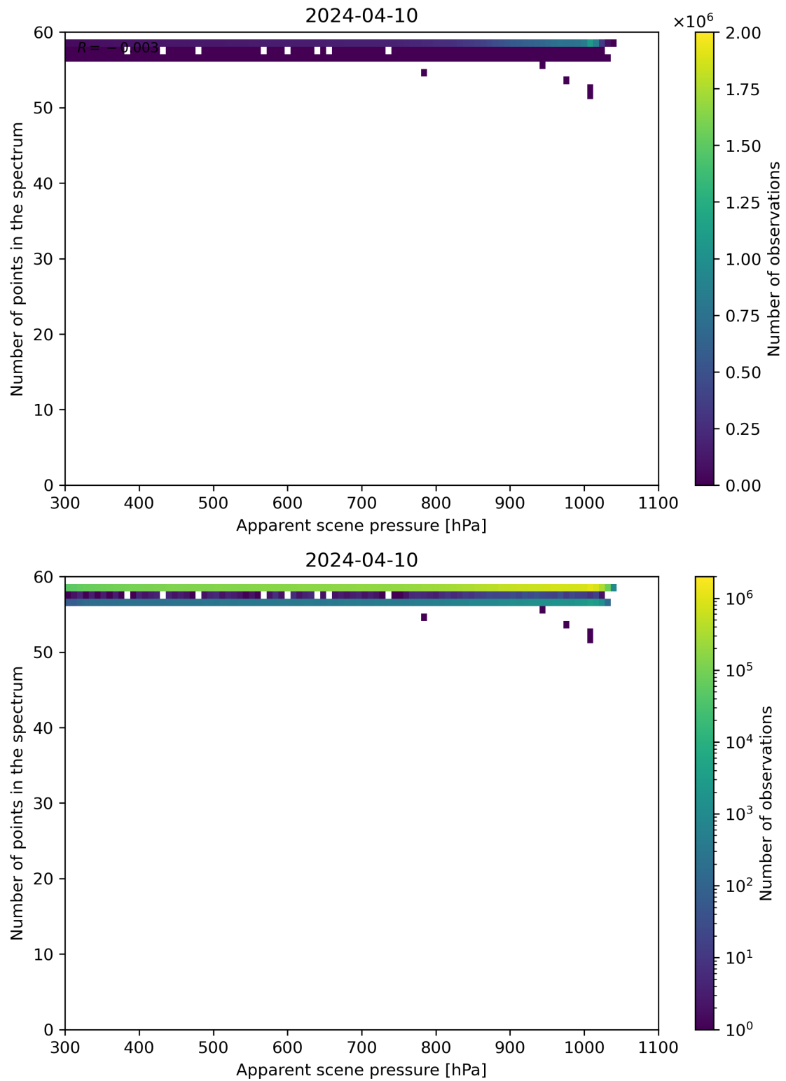
Figure 66: Scatter density plot of “Apparent scene pressure” against “Number of points in the spectrum” for 2024-04-10 to 2024-04-11.
