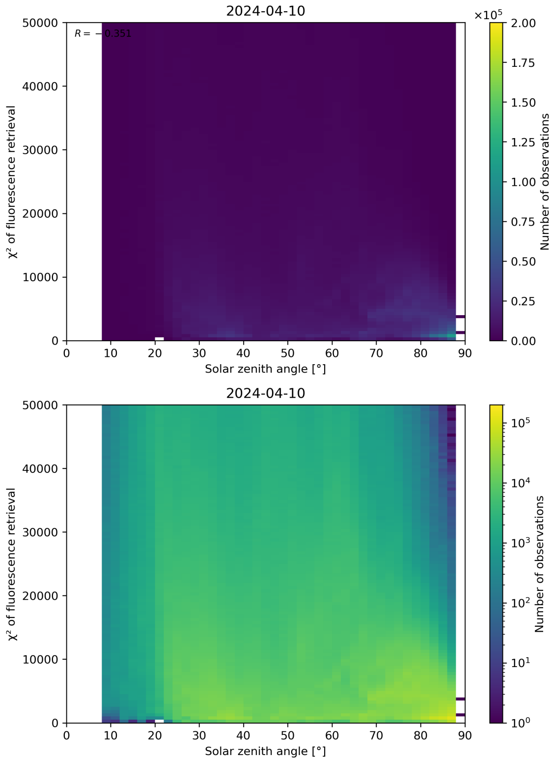
Figure 109: Scatter density plot of “Solar zenith angle” against “ \chi^2 of fluorescence retrieval” for 2024-04-10 to 2024-04-11.
