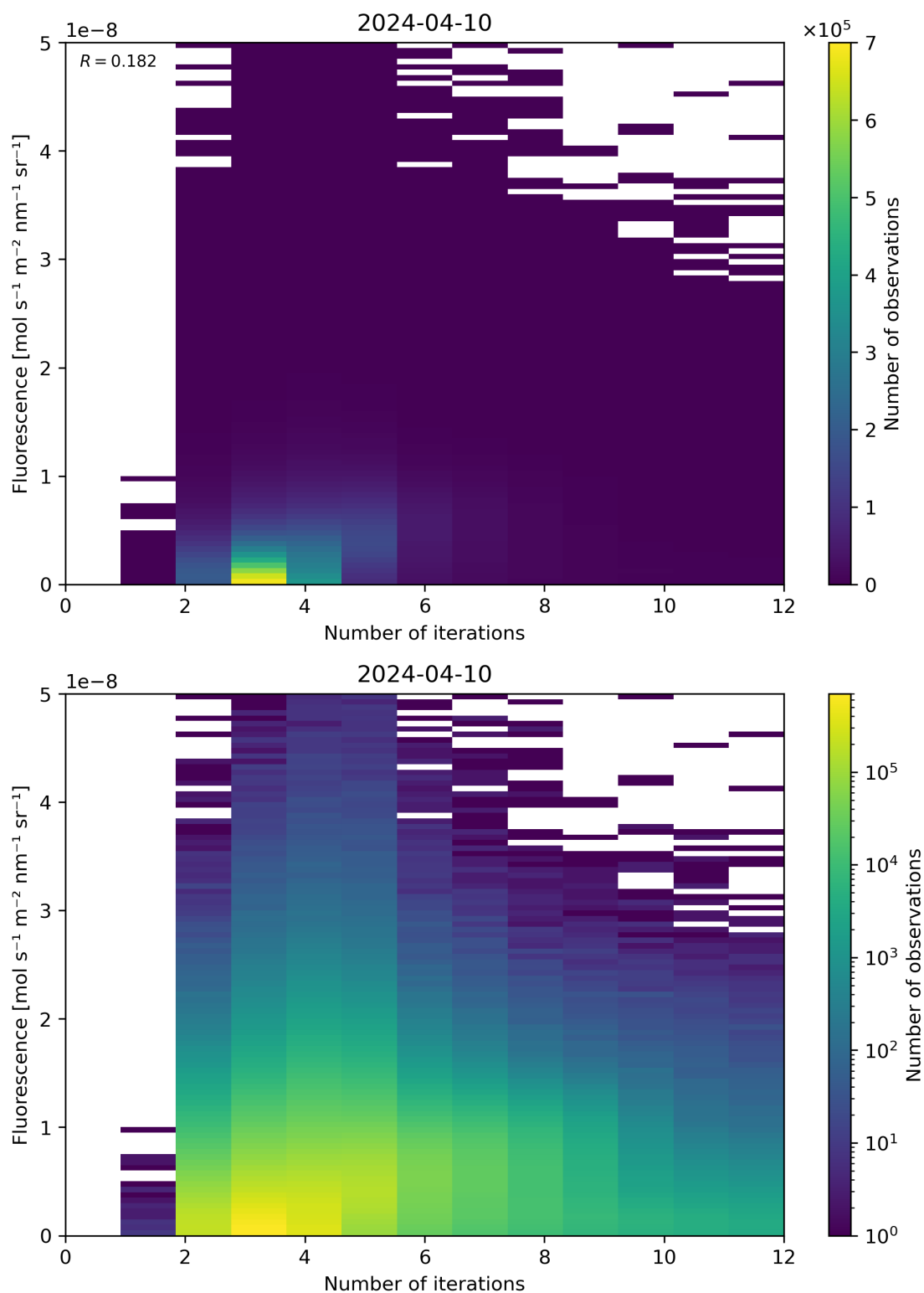
Figure 98: Scatter density plot of “Number of iterations” against “Fluorescence” for 2024-04-10 to 2024-04-11.
