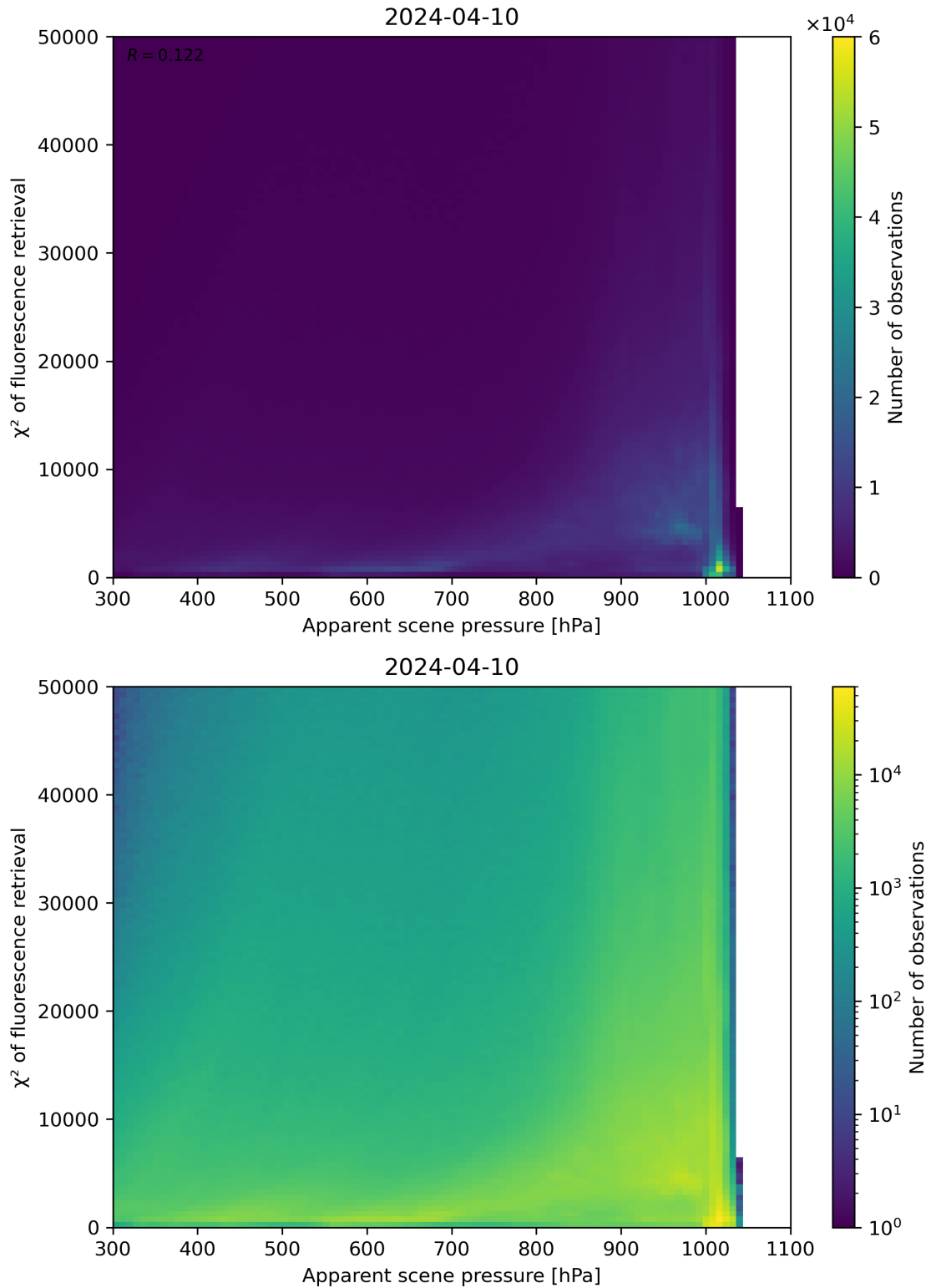
Figure 63: Scatter density plot of “Apparent scene pressure” against “ \chi^2 of fluorescence retrieval” for 2024-04-10 to 2024-04-11.
