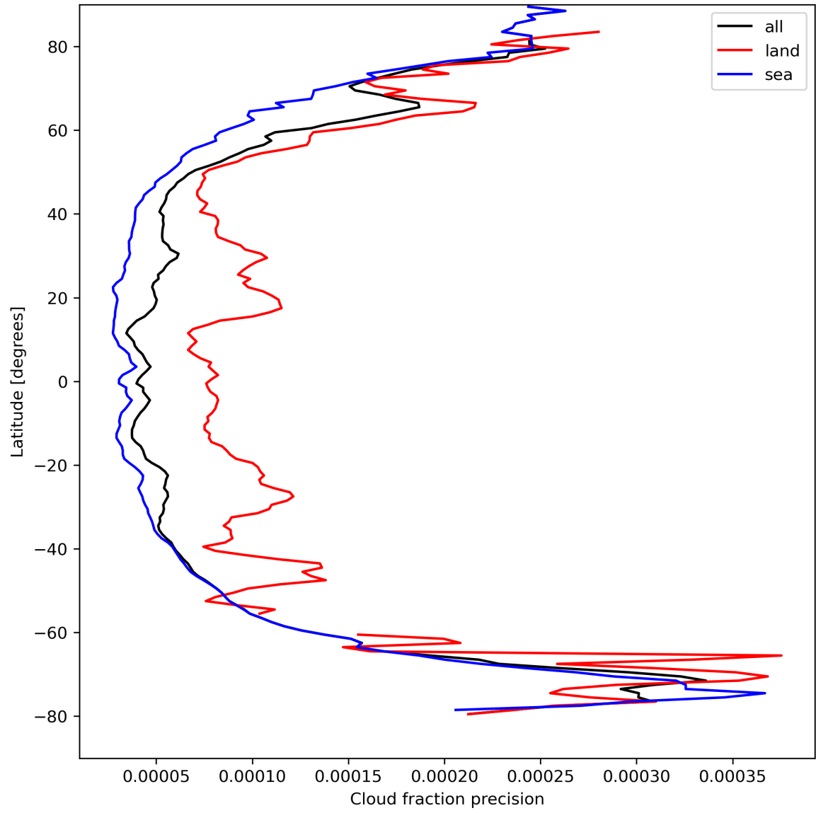
Figure 16: Zonal average of “Cloud fraction precision” for 2024-04-10 to 2024-04-11.
