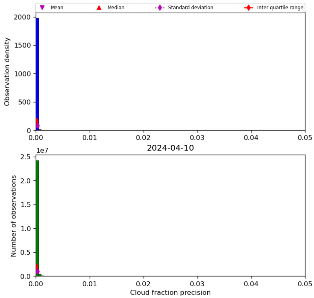
Figure 33: Histogram of “Cloud fraction precision” for 2024-04-10 to 2024-04-11
