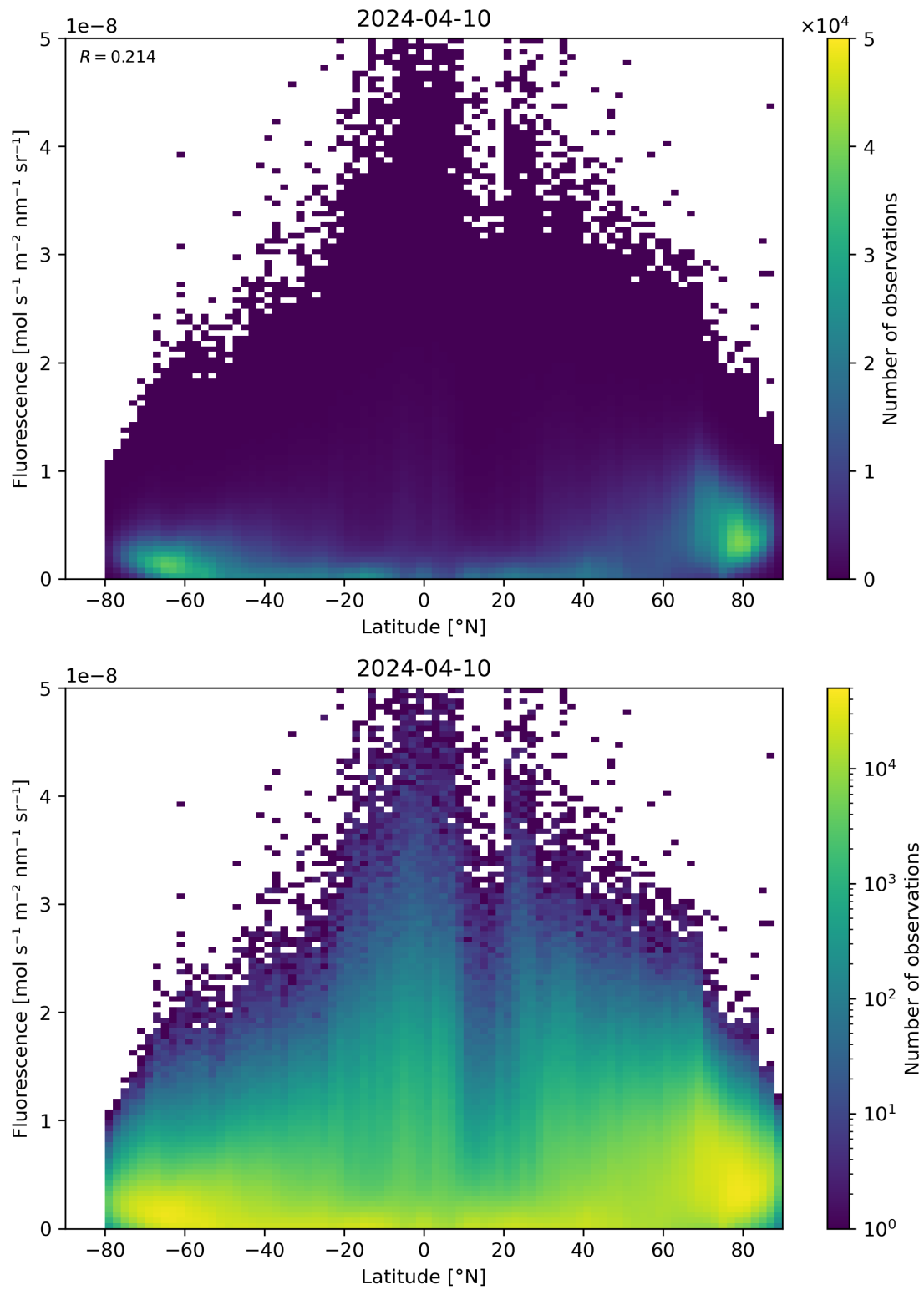
Figure 92: Scatter density plot of “Latitude” against “Fluorescence” for 2024-04-10 to 2024-04-11.
