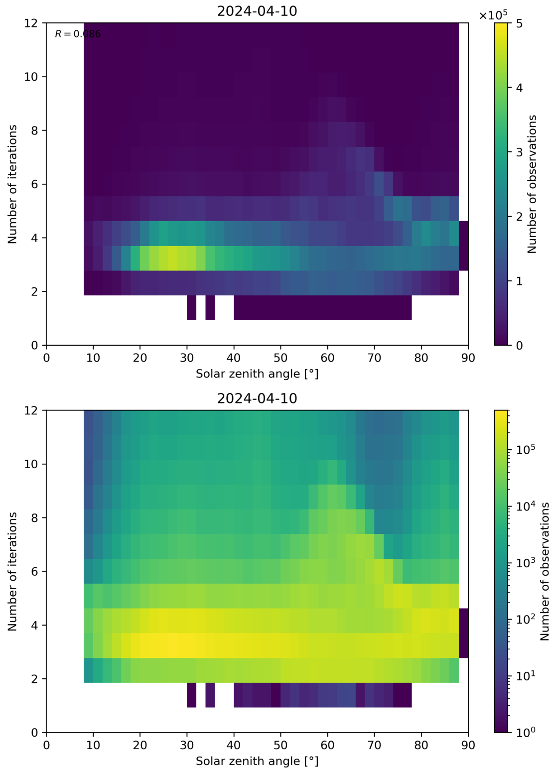
Figure 114: Scatter density plot of “Solar zenith angle” against “Number of iterations” for 2024-04-10 to 2024-04-11.
