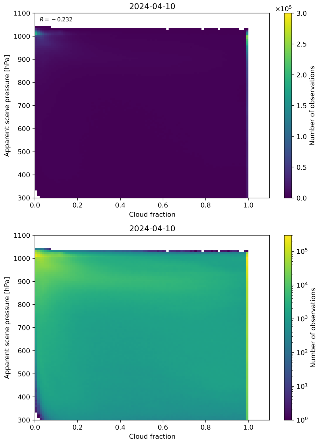
Figure 70: Scatter density plot of “Cloud fraction” against “Apparent scene pressure” for 2024-04-10 to 2024-04-11.
