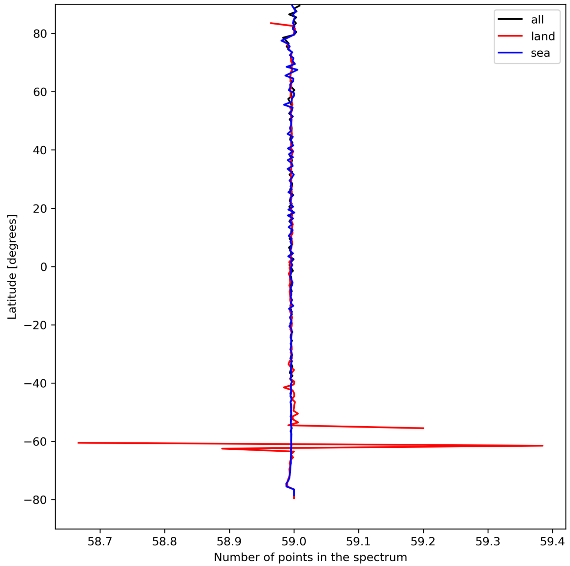
Figure 27: Zonal average of “Number of points in the spectrum” for 2024-04-10 to 2024-04-11.
