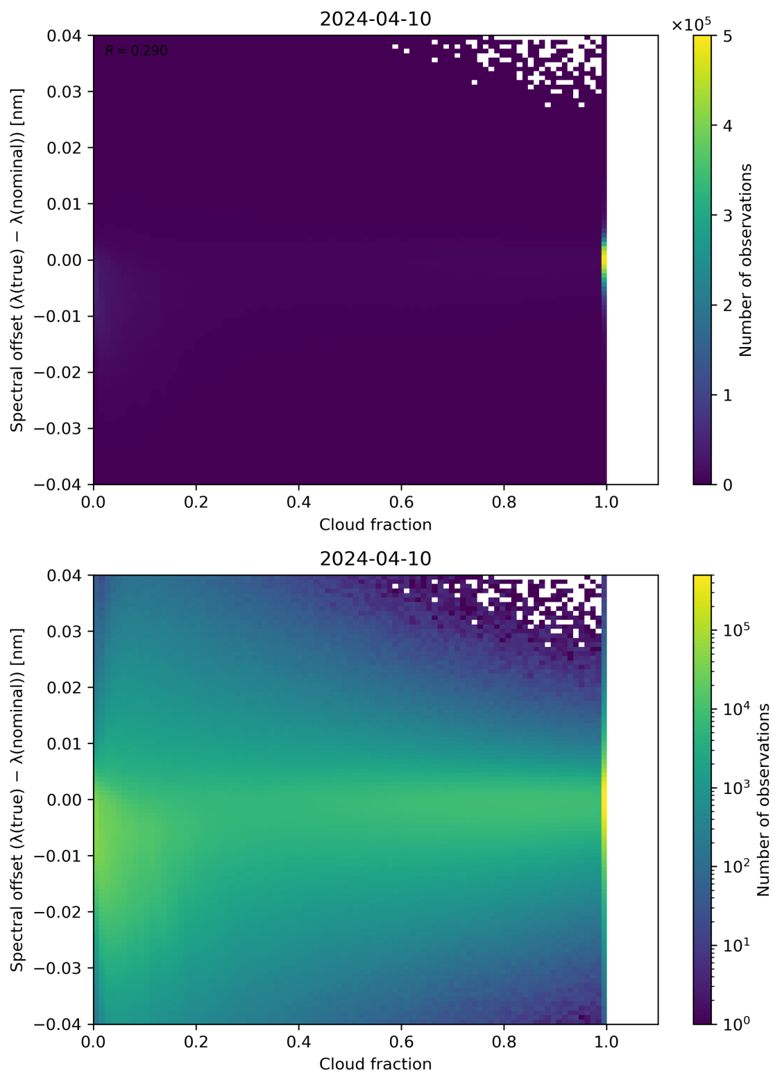
Figure 76: Scatter density plot of “Cloud fraction” against “Spectral offset ( \lambda(\text{true}) - \lambda(\text{nominal}) )” for 2024-04-10 to 2024-04-11.
