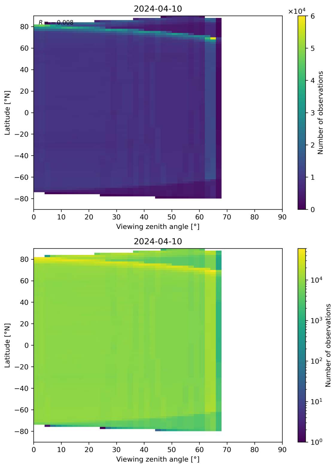
Figure 123: Scatter density plot of “Viewing zenith angle” against “Latitude” for 2024-04-10 to 2024-04-11.
