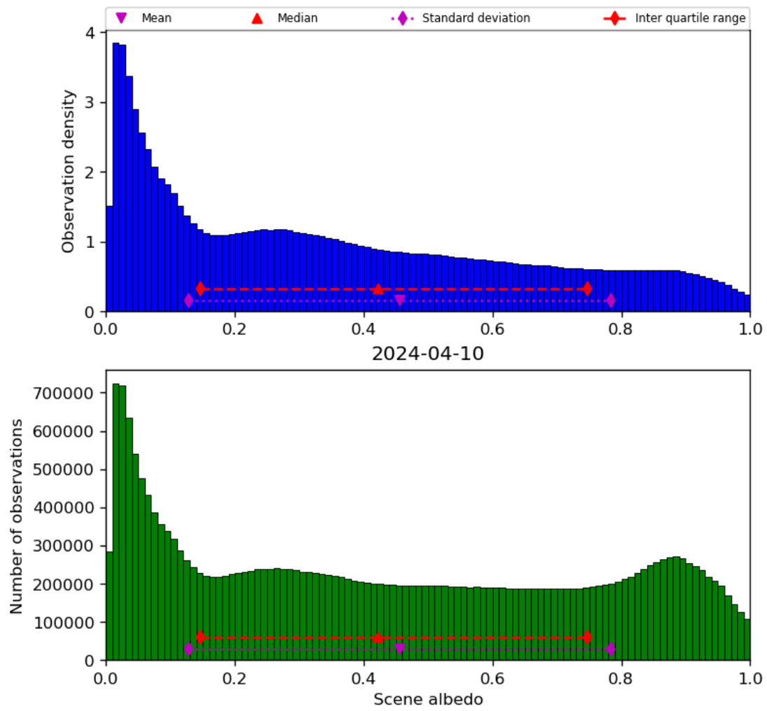
Figure 34: Histogram of “Scene albedo” for 2024-04-10 to 2024-04-11
