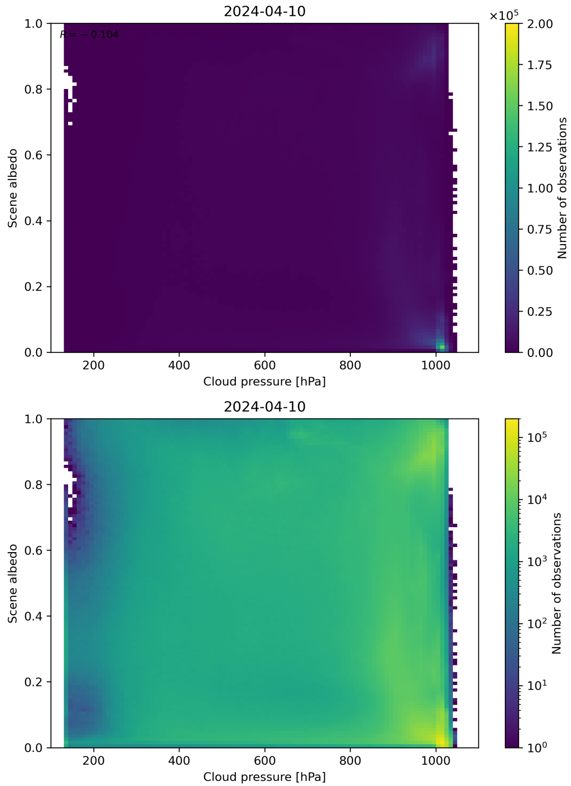
Figure 83: Scatter density plot of “Cloud pressure” against “Scene albedo” for 2024-04-10 to 2024-04-11.
