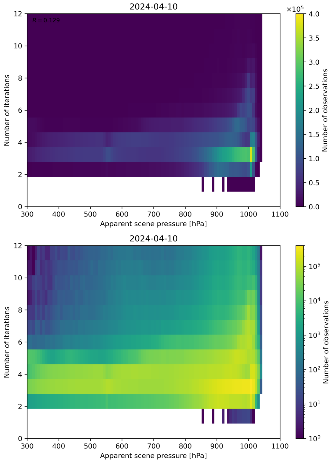
Figure 65: Scatter density plot of “Apparent scene pressure” against “Number of iterations” for 2024-04-10 to 2024-04-11.
