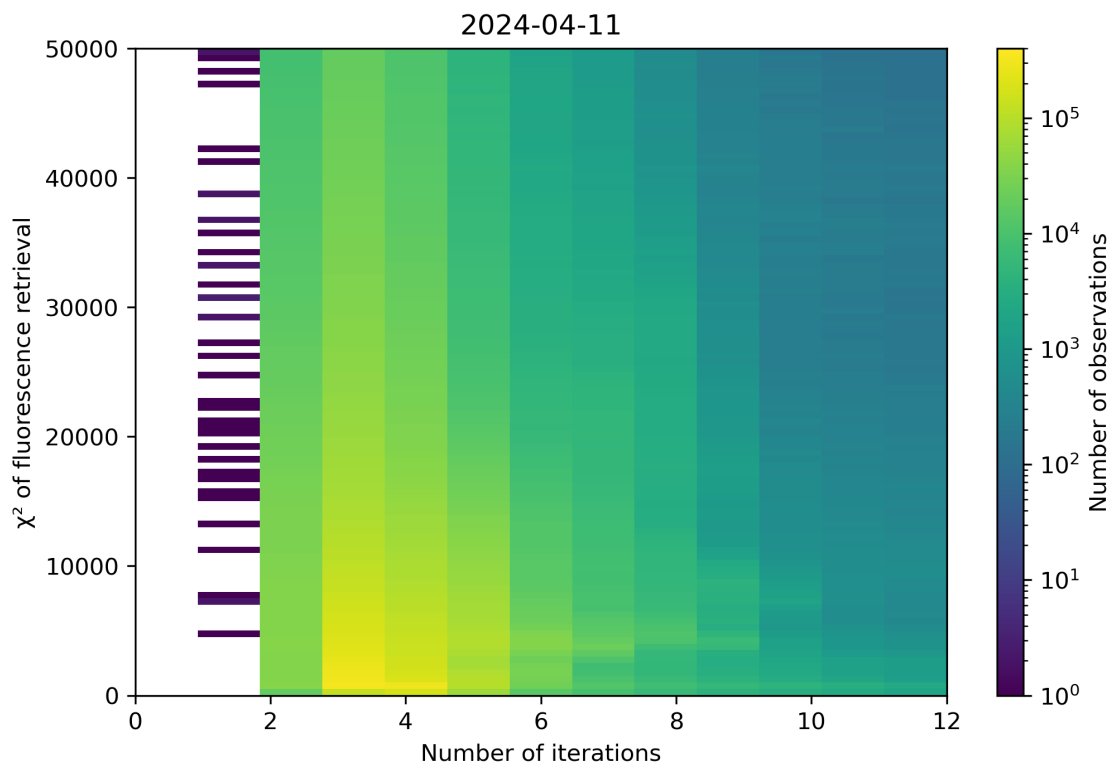
Figure 97: Scatter density plot of “Number of iterations” against “ \chi^2 of fluorescence retrieval” for 2024-04-10 to 2024-04-12.
