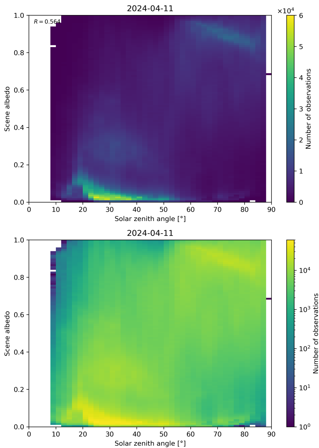
Figure 116: Scatter density plot of “Solar zenith angle” against “Scene albedo” for 2024-04-10 to 2024-04-12.
