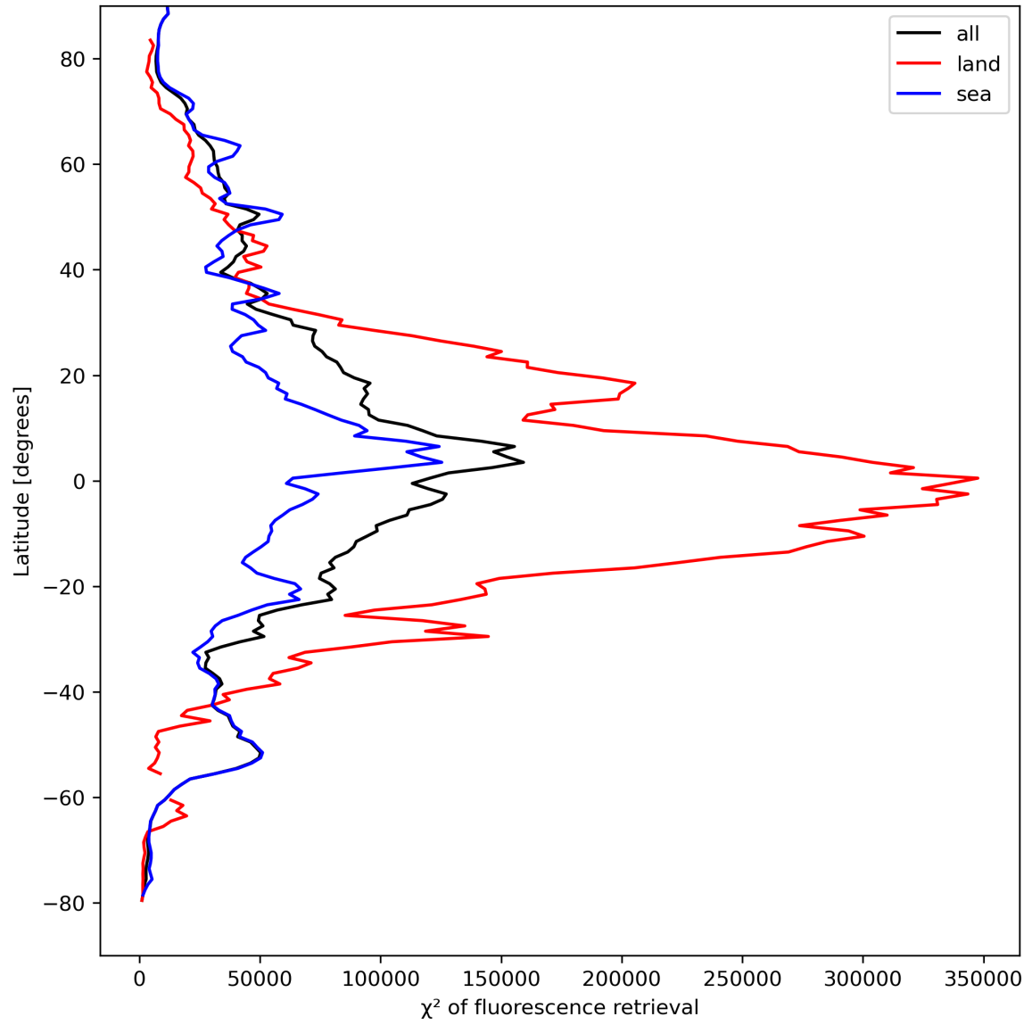
Figure 25: Zonal average of “ \chi^2 of fluorescence retrieval” for 2024-04-10 to 2024-04-12.
