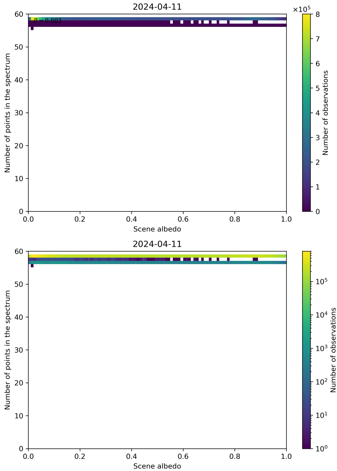
Figure 106: Scatter density plot of “Scene albedo” against “Number of points in the spectrum” for 2024-04-10 to 2024-04-12.
