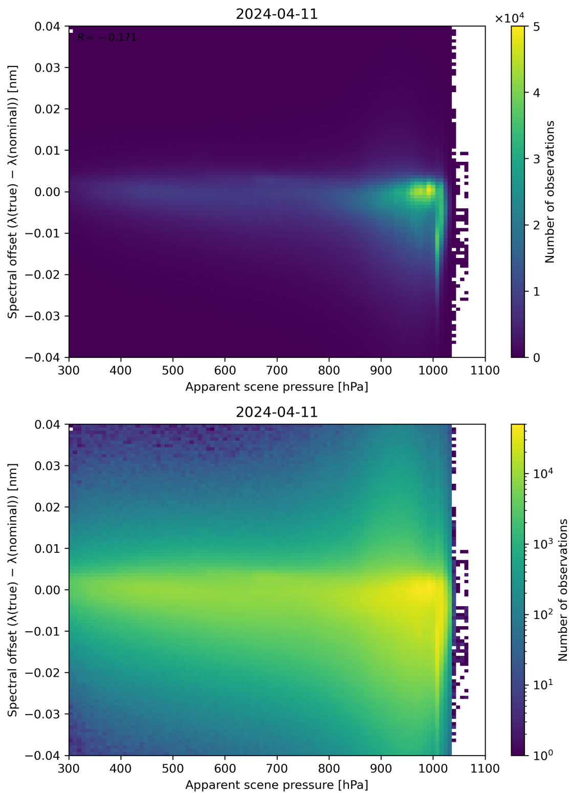
Figure 67: Scatter density plot of “Apparent scene pressure” against “Spectral offset ( \lambda(\text{true}) - \lambda(\text{nominal}) )” for 2024-04-10 to 2024-04-12.
