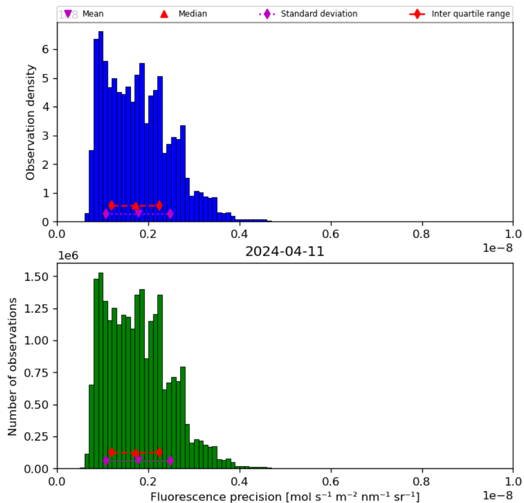
Figure 41: Histogram of “Fluorescence precision” for 2024-04-10 to 2024-04-12
