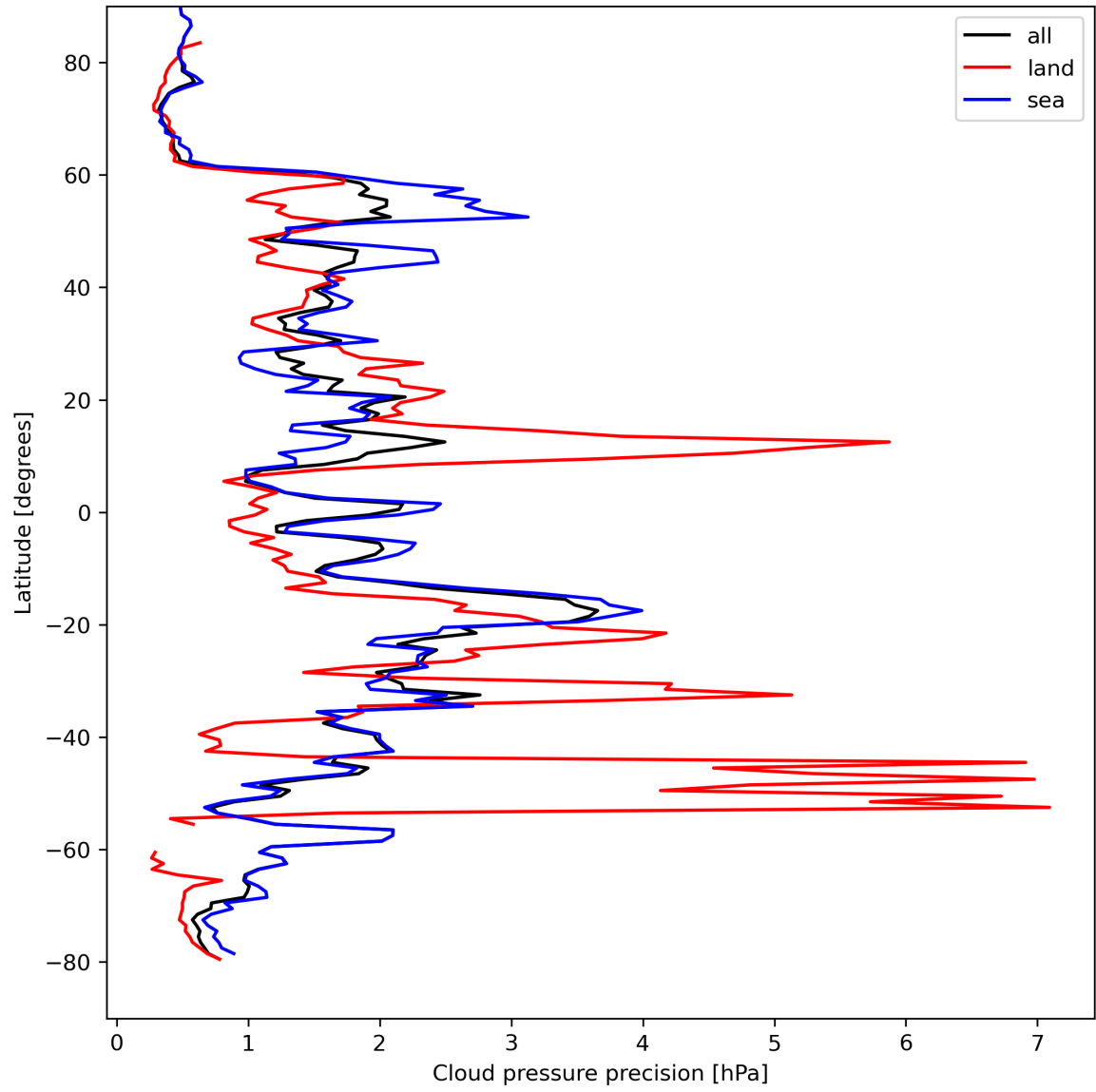
Figure 14: Zonal average of “Cloud pressure precision” for 2024-04-10 to 2024-04-12.
