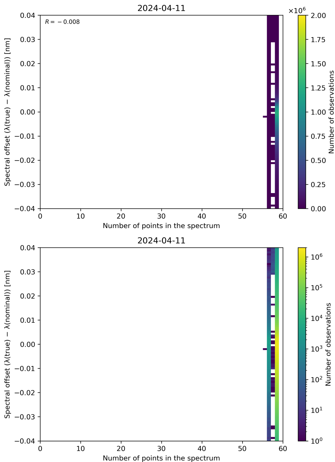
Figure 101: Scatter density plot of “Number of points in the spectrum” against “Spectral offset ( \lambda(\text{true}) - \lambda(\text{nominal}) )” for 2024-04-10 to 2024-04-12.
