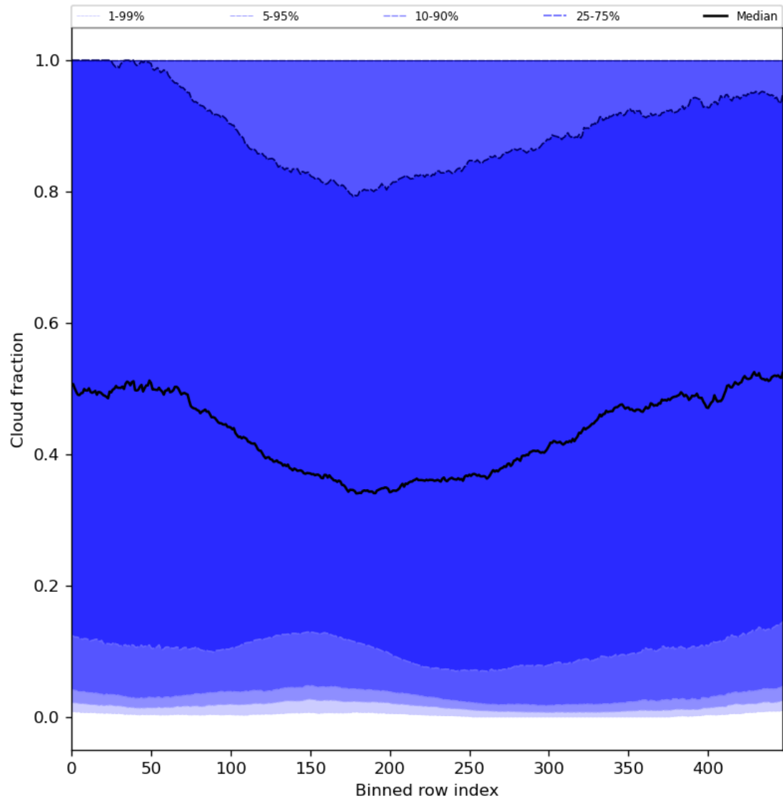
Figure 49: Along track statistics of “Cloud fraction” for 2024-04-10 to 2024-04-12
