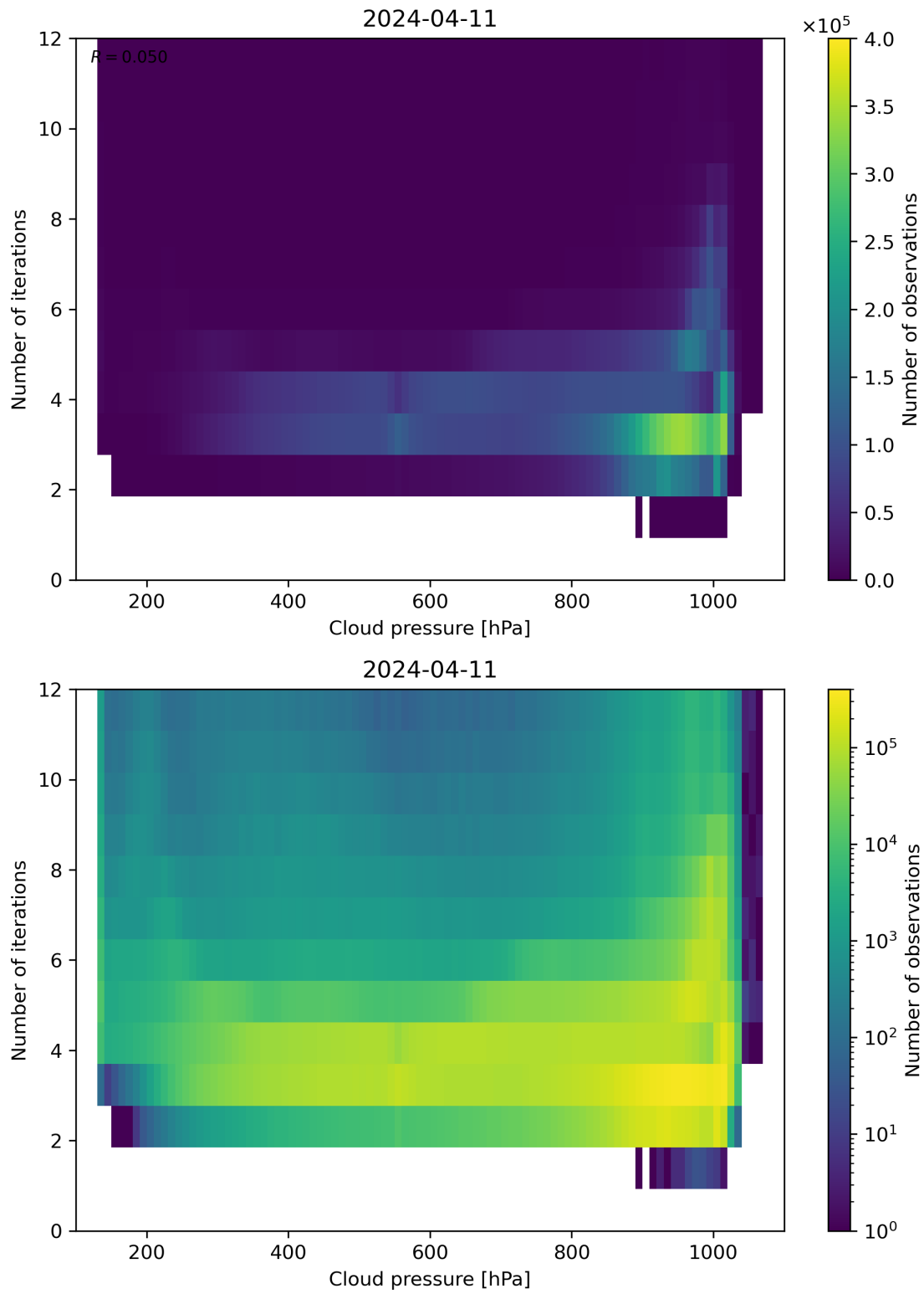
Figure 81: Scatter density plot of “Cloud pressure” against “Number of iterations” for 2024-04-10 to 2024-04-12.
