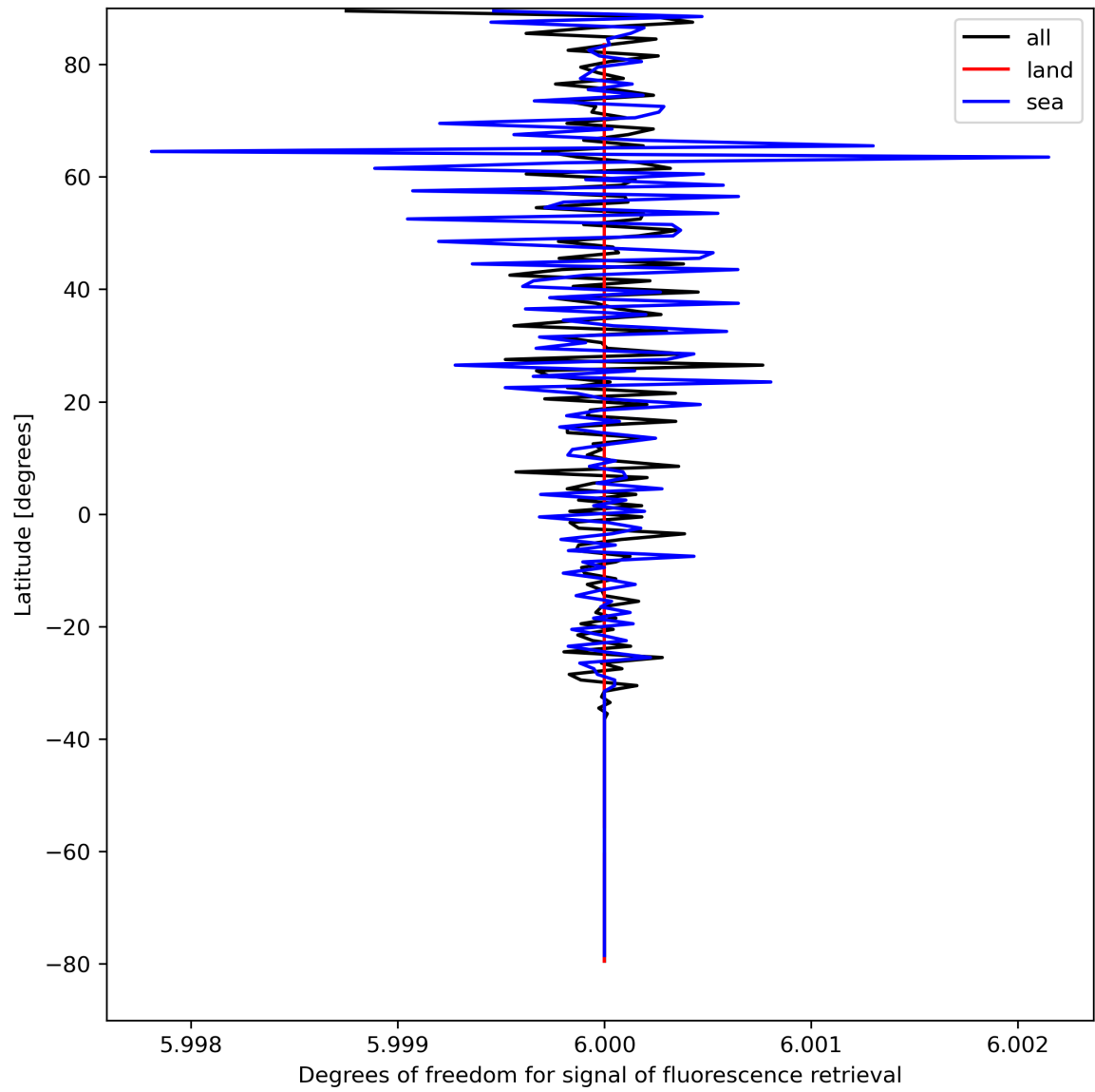
Figure 26: Zonal average of “Degrees of freedom for signal of fluorescence retrieval” for 2024-04-10 to 2024-04-12.
