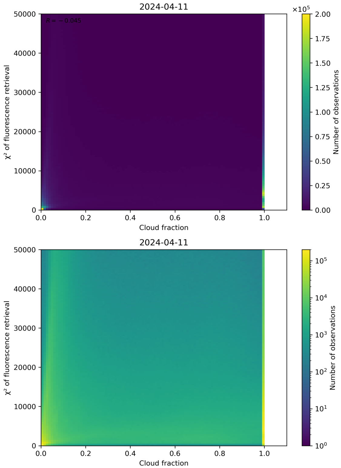
Figure 71: Scatter density plot of “Cloud fraction” against “ \chi^2 of fluorescence retrieval” for 2024-04-10 to 2024-04-12.
