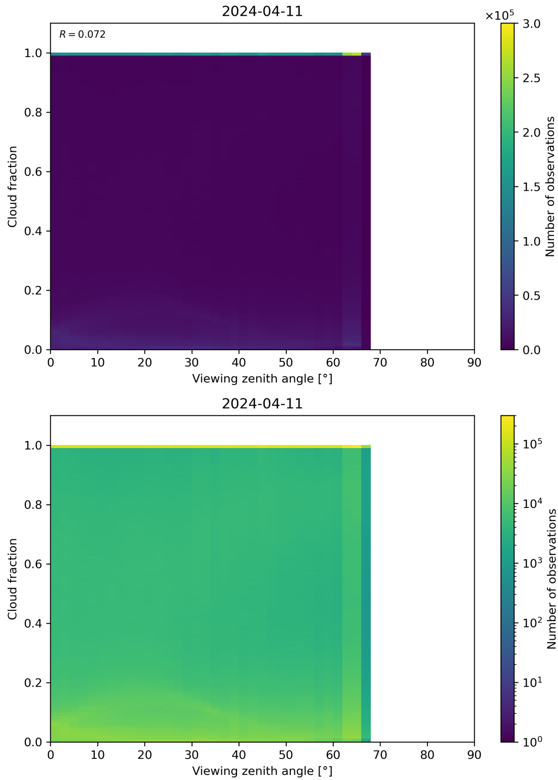
Figure 120: Scatter density plot of “Viewing zenith angle” against “Cloud fraction” for 2024-04-10 to 2024-04-12.
