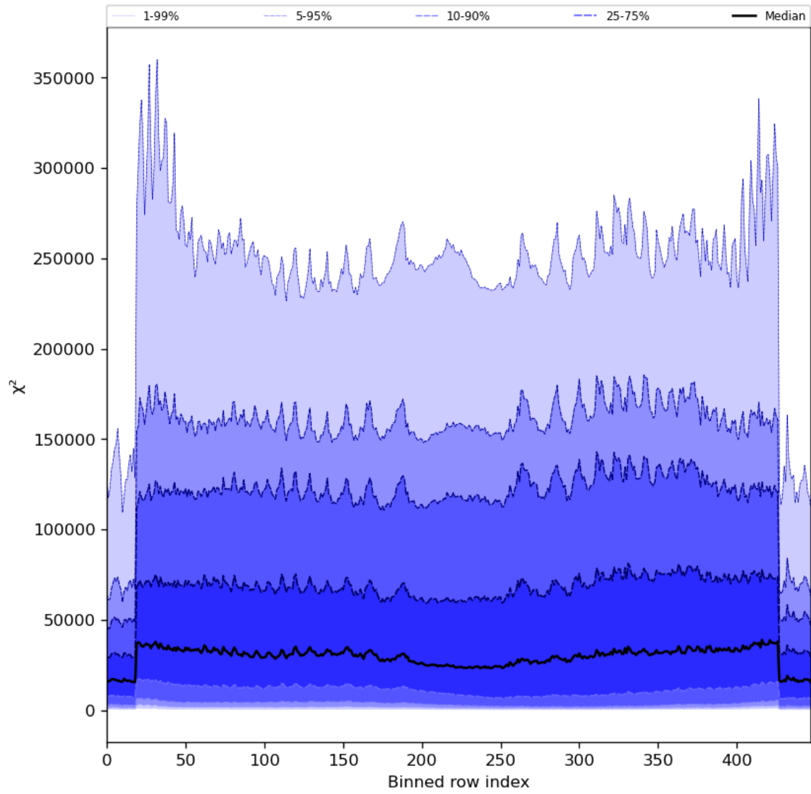
Figure 55: Along track statistics of “ \chi^2 ” for 2024-04-10 to 2024-04-12
