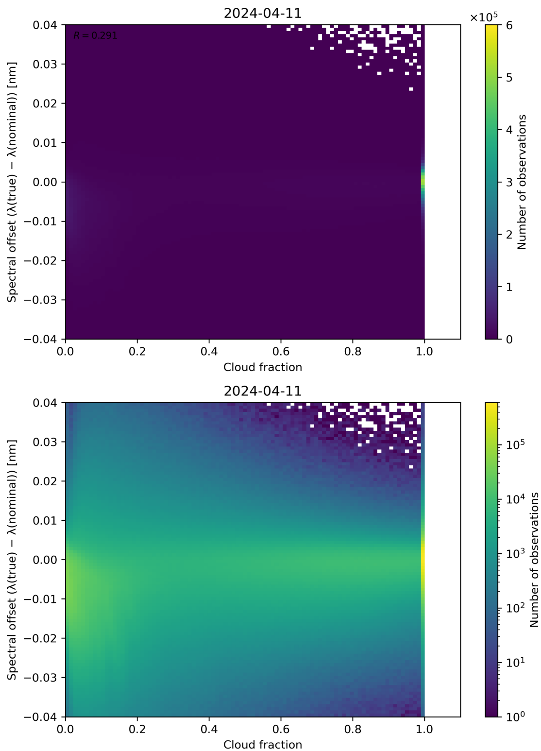
Figure 76: Scatter density plot of “Cloud fraction” against “Spectral offset ( \lambda(\text{true}) - \lambda(\text{nominal}) )” for 2024-04-10 to 2024-04-12.
