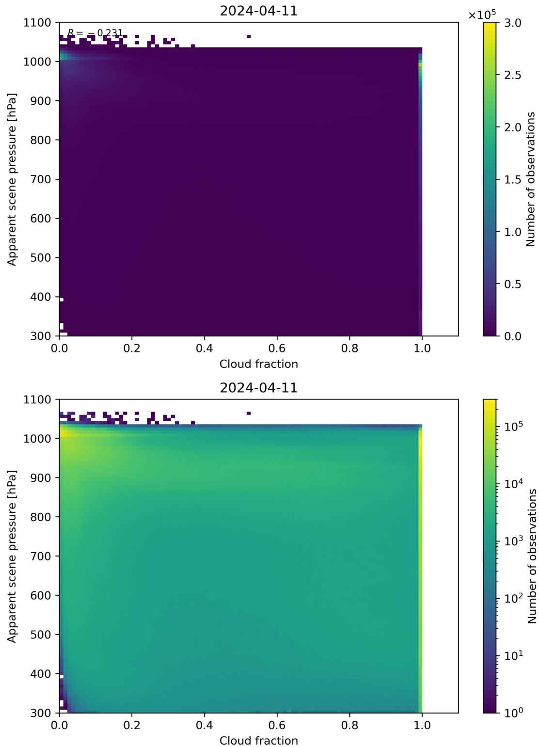
Figure 70: Scatter density plot of “Cloud fraction” against “Apparent scene pressure” for 2024-04-10 to 2024-04-12.
