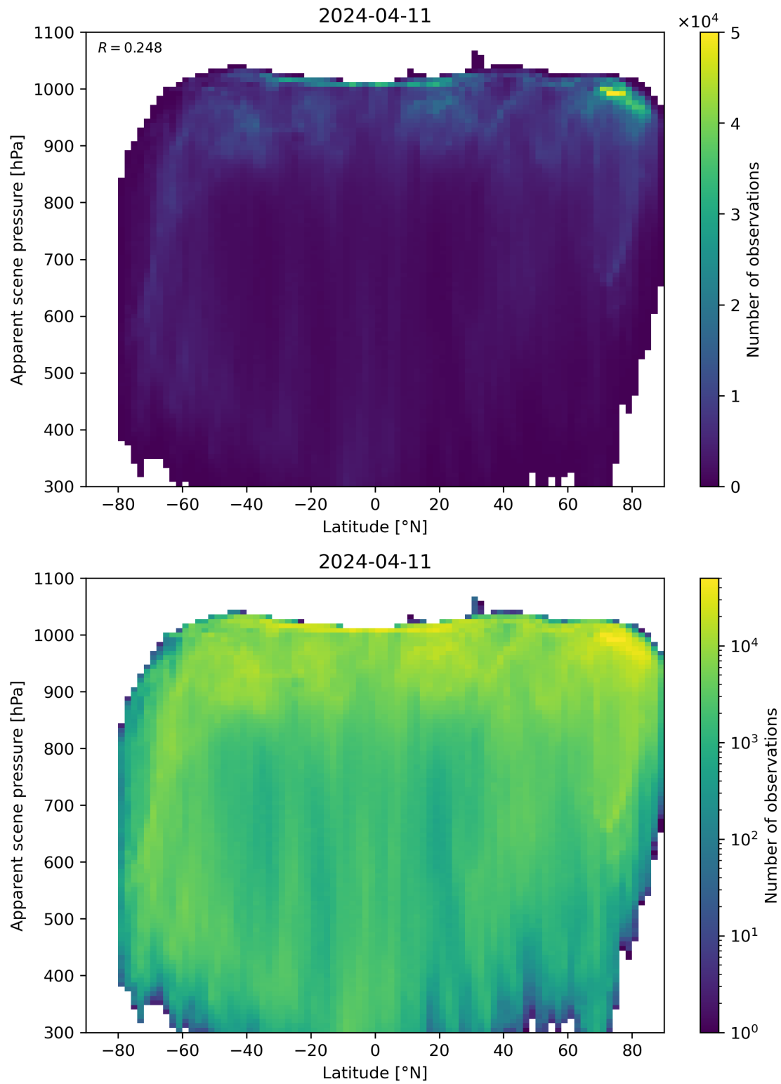
Figure 88: Scatter density plot of “Latitude” against “Apparent scene pressure” for 2024-04-10 to 2024-04-12.
