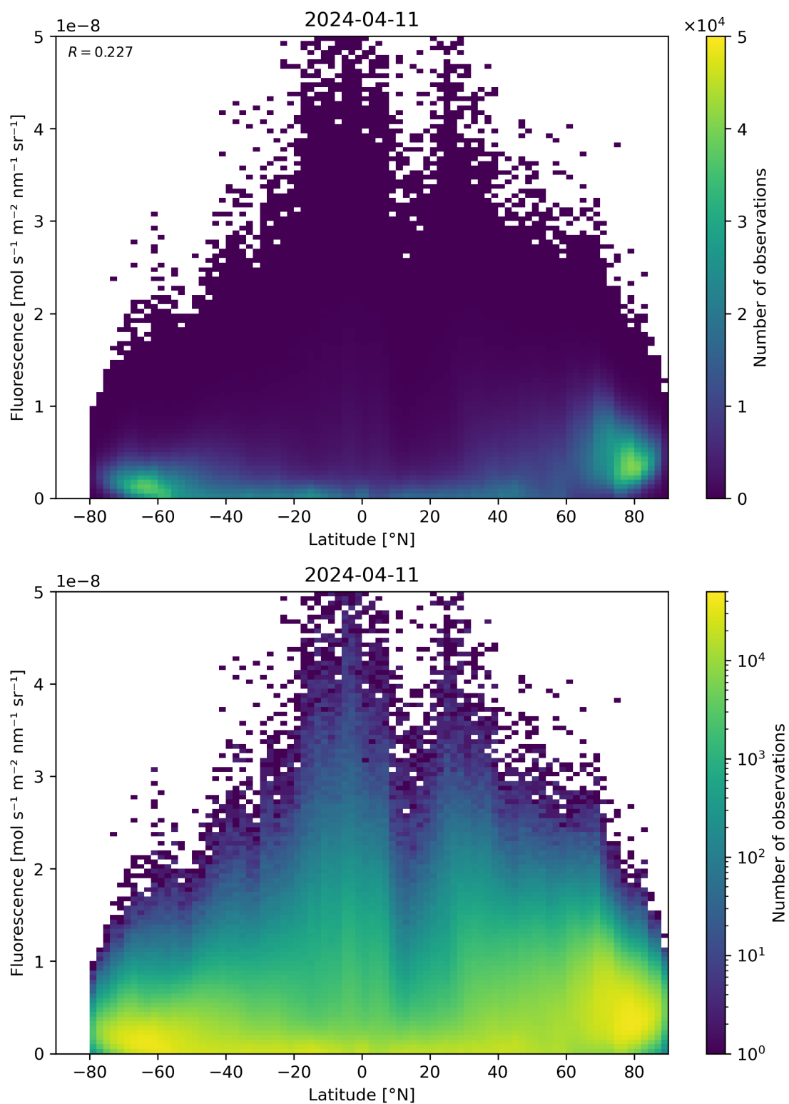
Figure 92: Scatter density plot of “Latitude” against “Fluorescence” for 2024-04-10 to 2024-04-12.
