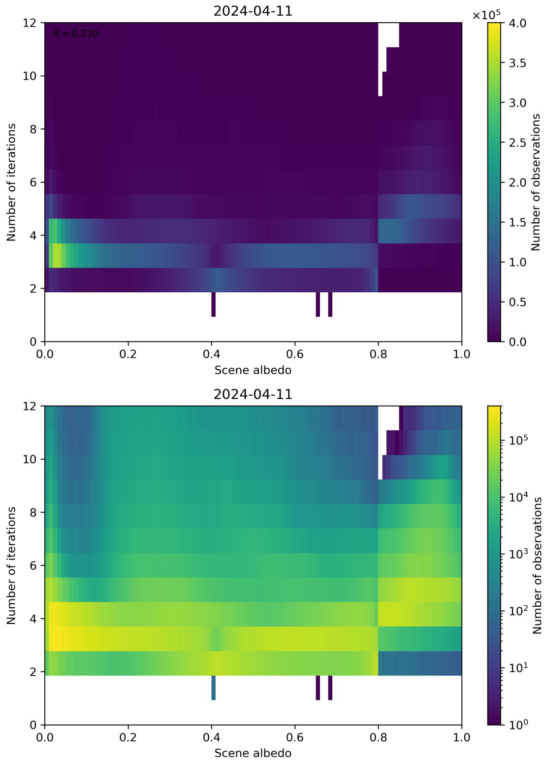
Figure 105: Scatter density plot of “Scene albedo” against “Number of iterations” for 2024-04-10 to 2024-04-12.
