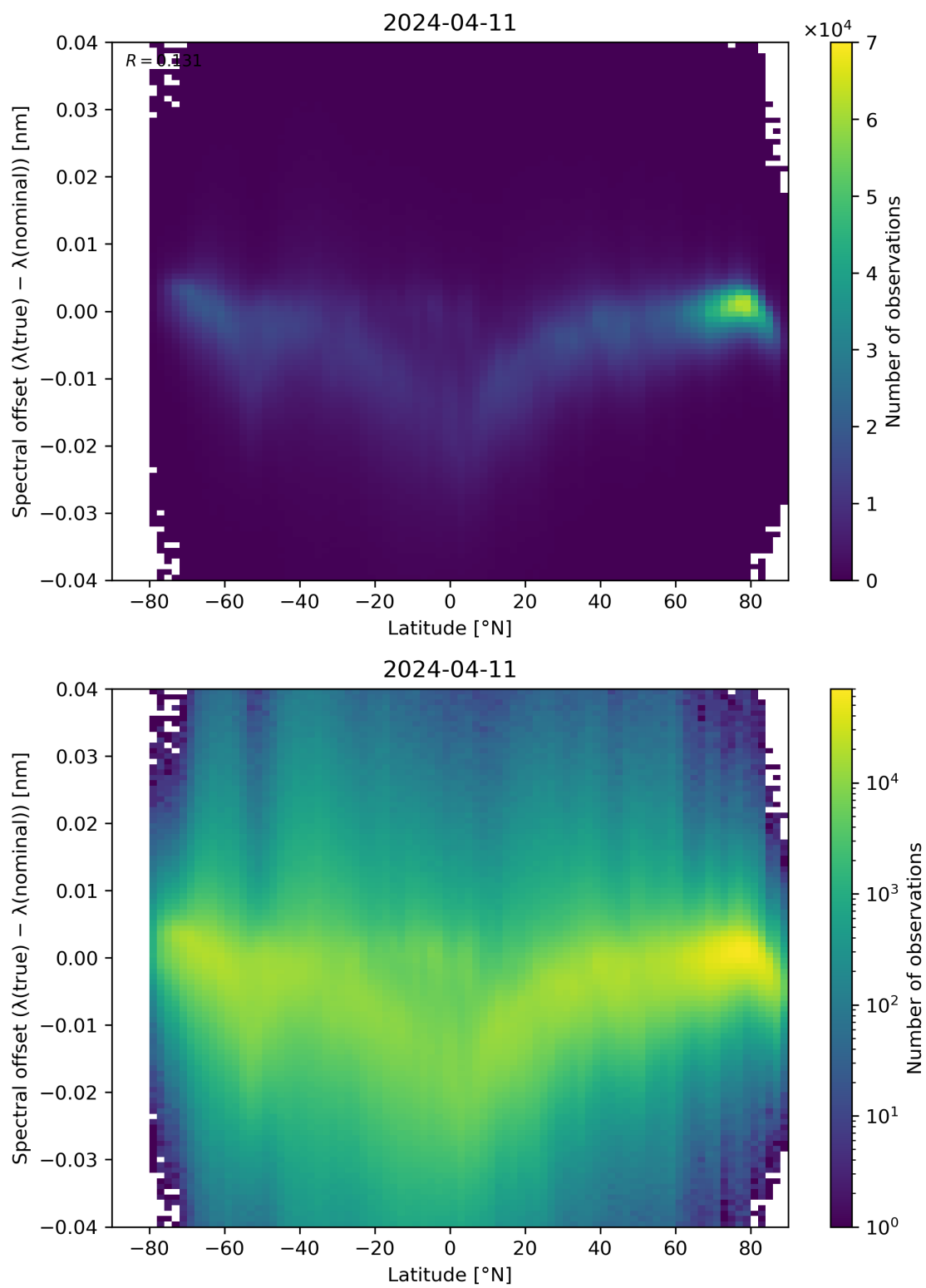
Figure 96: Scatter density plot of “Latitude” against “Spectral offset ( \lambda(\text{true}) - \lambda(\text{nominal}) )” for 2024-04-10 to 2024-04-12.
