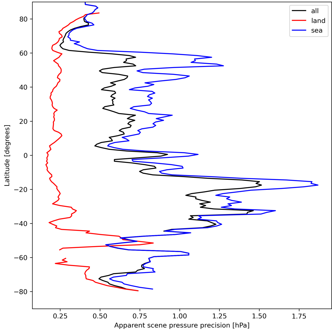
Figure 20: Zonal average of “Apparent scene pressure precision” for 2024-04-10 to 2024-04-12.
