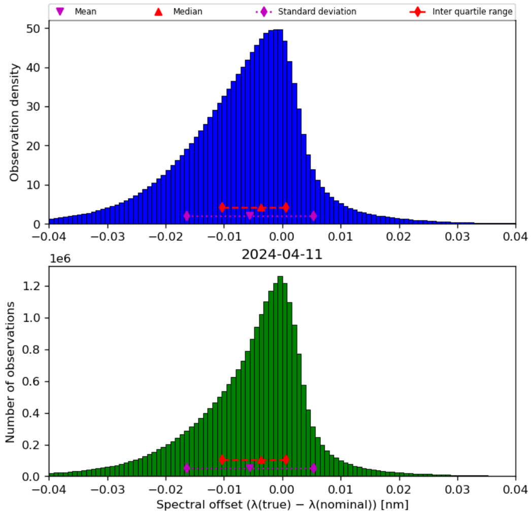
Figure 45: Histogram of “Spectral offset ( \lambda(\text{true}) - \lambda(\text{nominal}) )” for 2024-04-10 to 2024-04-12
