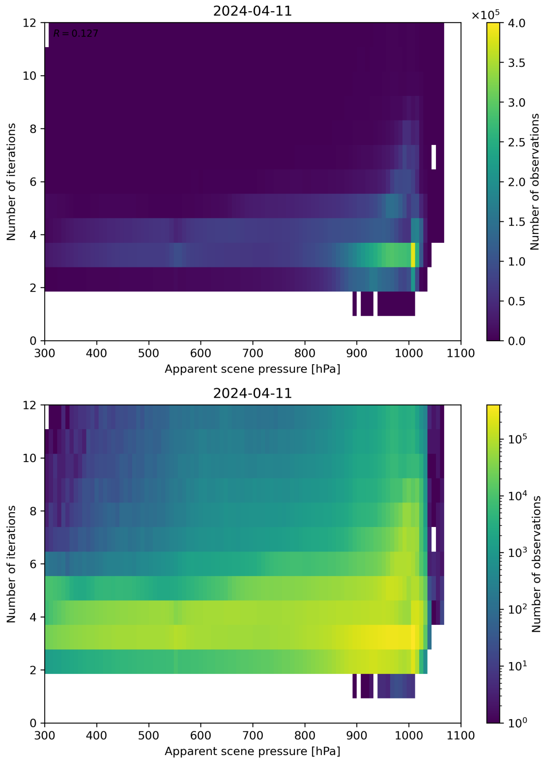
Figure 65: Scatter density plot of “Apparent scene pressure” against “Number of iterations” for 2024-04-10 to 2024-04-12.
