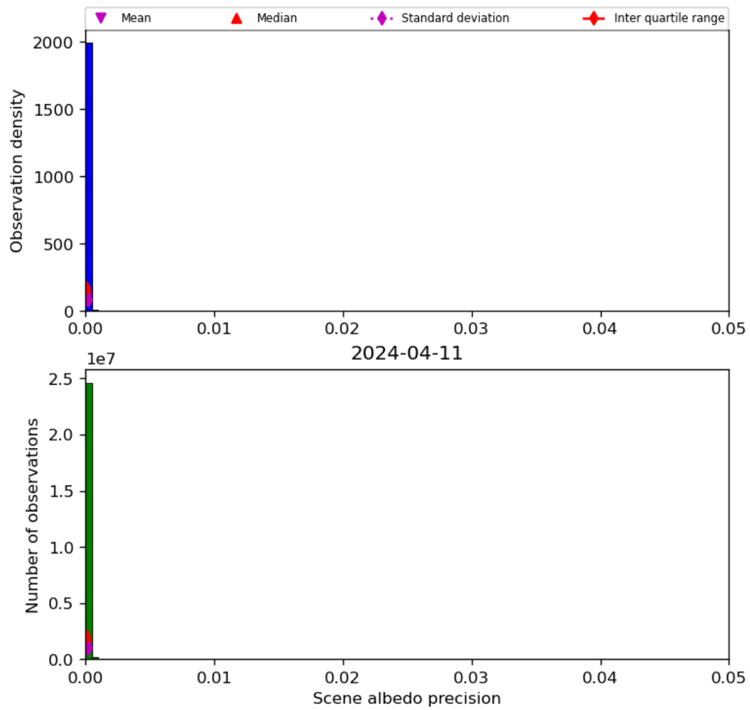
Figure 35: Histogram of “Scene albedo precision” for 2024-04-10 to 2024-04-12
