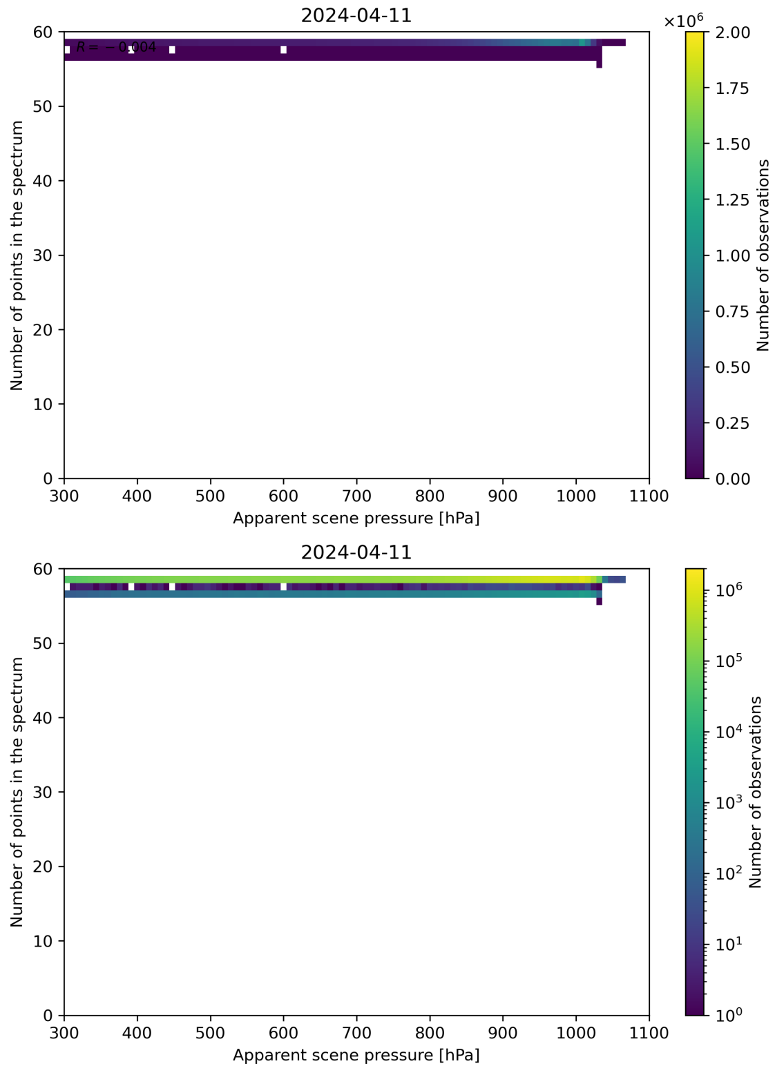
Figure 66: Scatter density plot of “Apparent scene pressure” against “Number of points in the spectrum” for 2024-04-10 to 2024-04-12.
