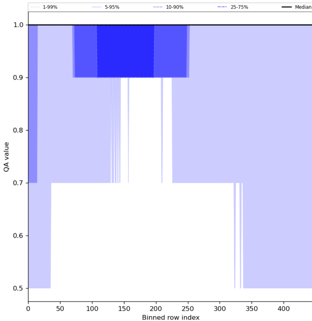
Figure 46: Along track statistics of “QA value” for 2024-04-10 to 2024-04-12
