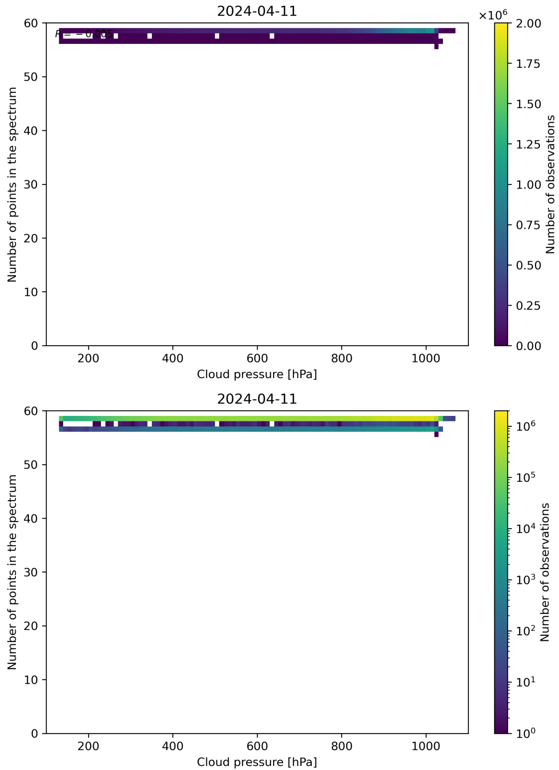
Figure 82: Scatter density plot of “Cloud pressure” against “Number of points in the spectrum” for 2024-04-10 to 2024-04-12.
