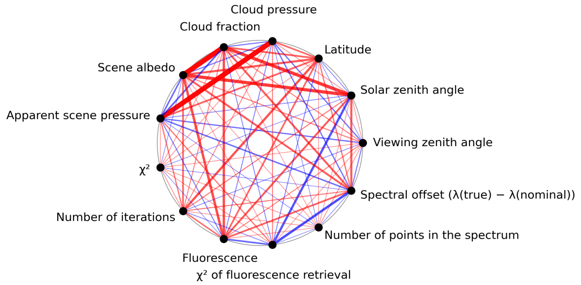
Figure 1: Map of correlation graph for 2024-04-10 to 2024-04-12.
