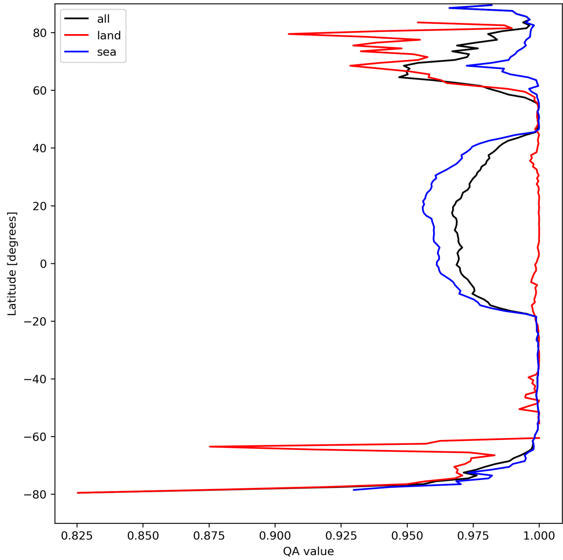
Figure 12: Zonal average of “QA value” for 2024-04-10 to 2024-04-12.
