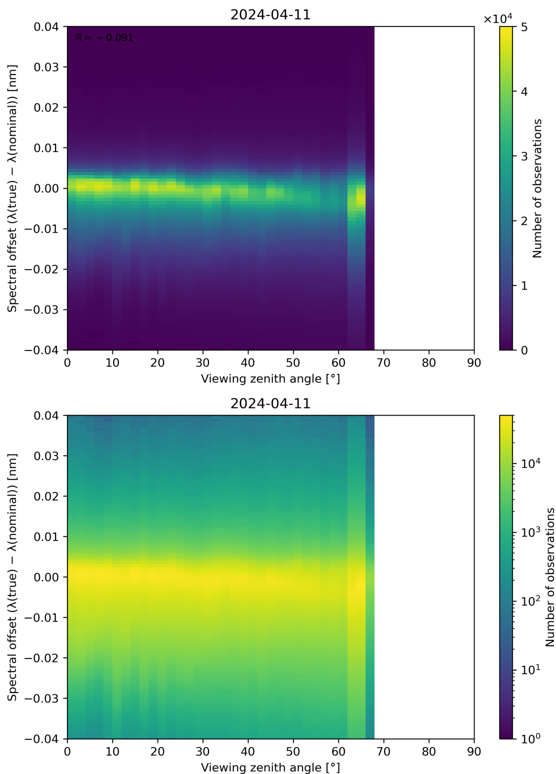
Figure 128: Scatter density plot of “Viewing zenith angle” against “Spectral offset ( \lambda(\text{true}) - \lambda(\text{nominal}) )” for 2024-04-10 to 2024-04-12.
