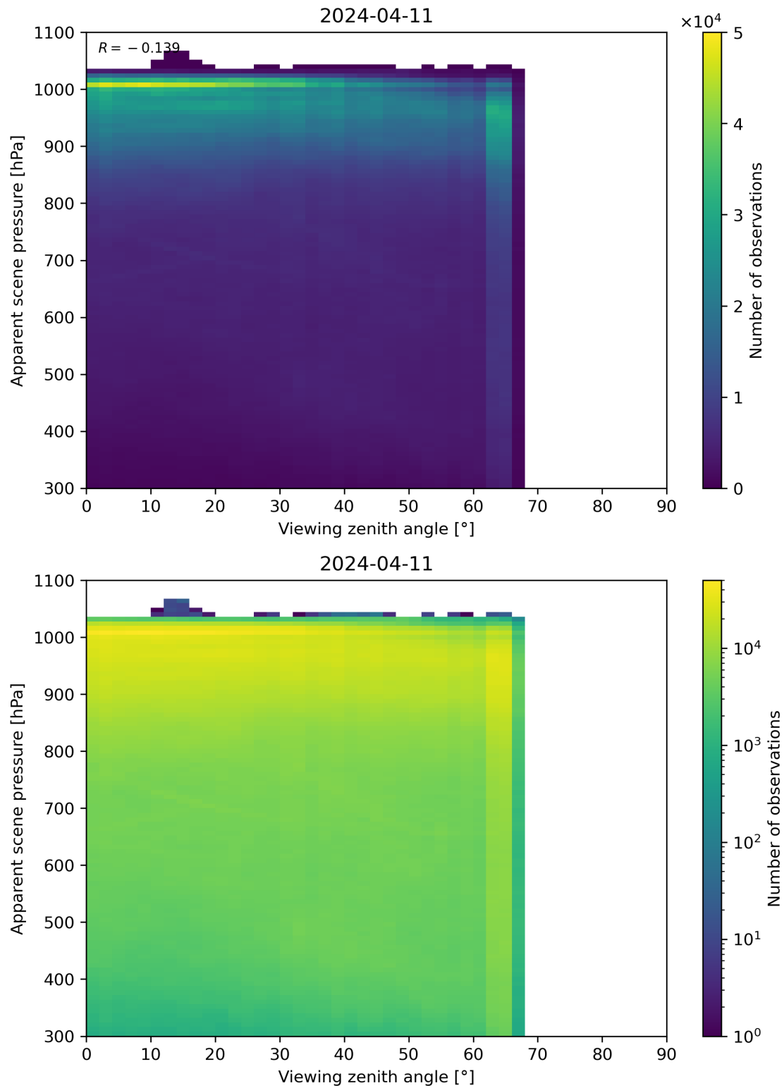
Figure 118: Scatter density plot of “Viewing zenith angle” against “Apparent scene pressure” for 2024-04-10 to 2024-04-12.
