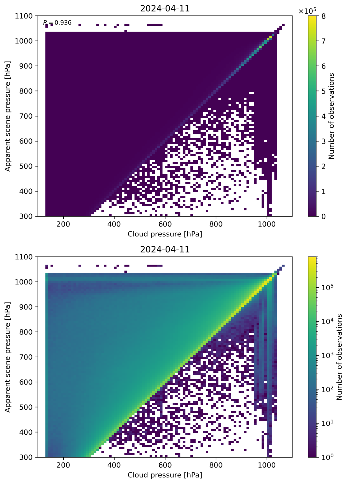
Figure 77: Scatter density plot of “Cloud pressure” against “Apparent scene pressure” for 2024-04-10 to 2024-04-12.
