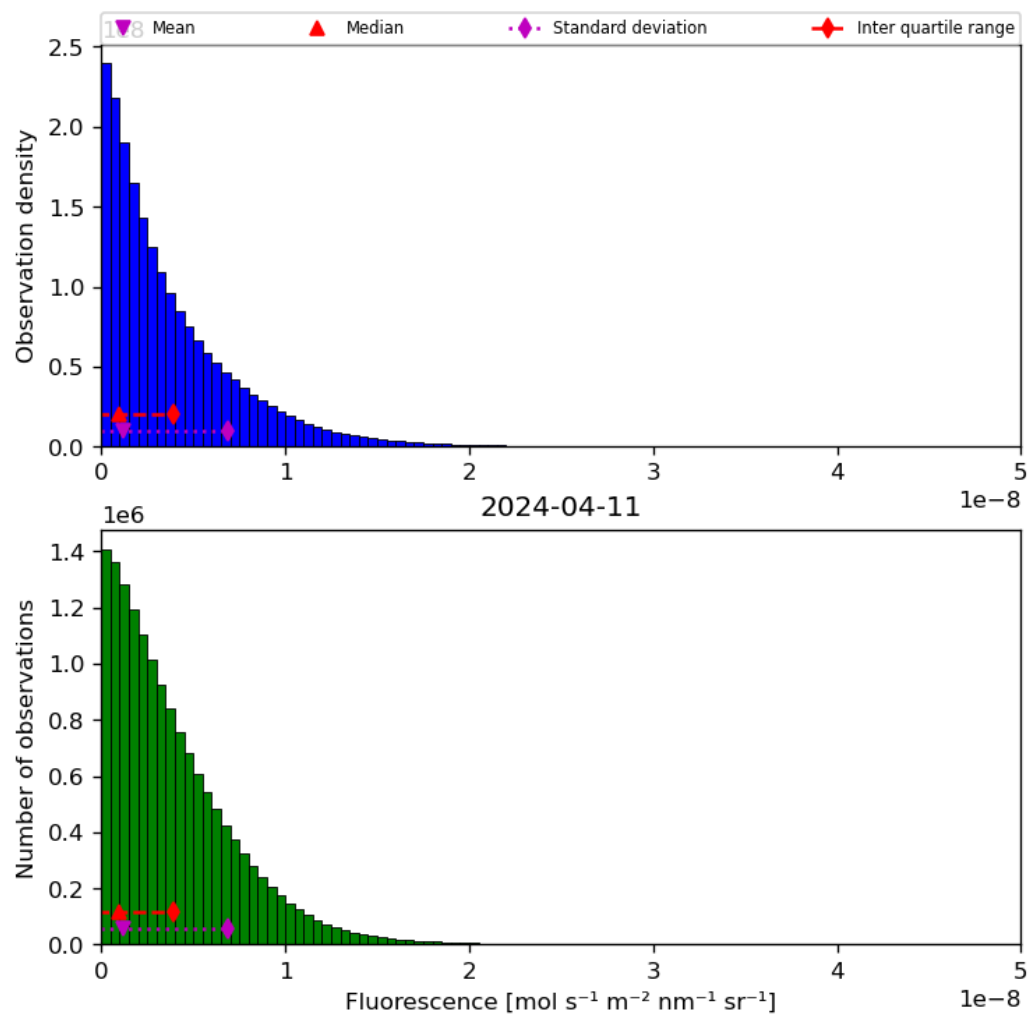
Figure 40: Histogram of “Fluorescence” for 2024-04-10 to 2024-04-12
