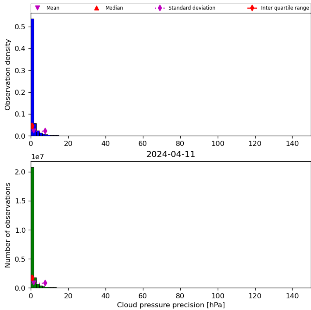
Figure 31: Histogram of “Cloud pressure precision” for 2024-04-10 to 2024-04-12
