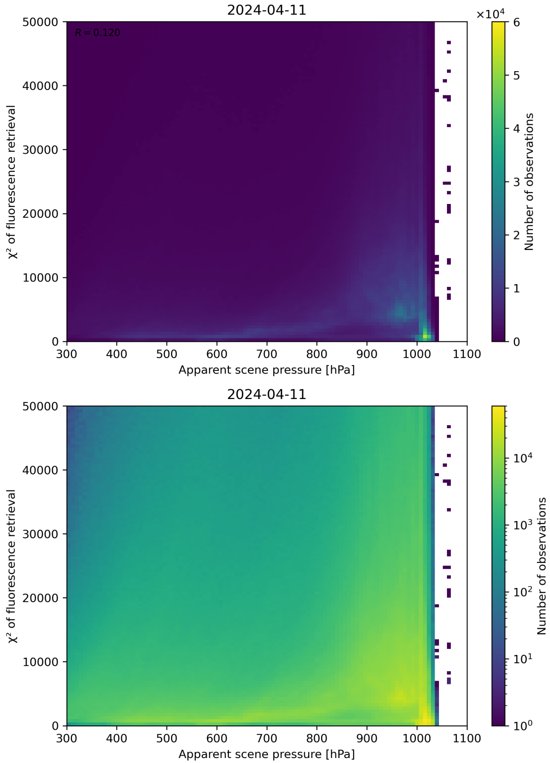
Figure 63: Scatter density plot of “Apparent scene pressure” against “ \chi^2 of fluorescence retrieval” for 2024-04-10 to 2024-04-12.
