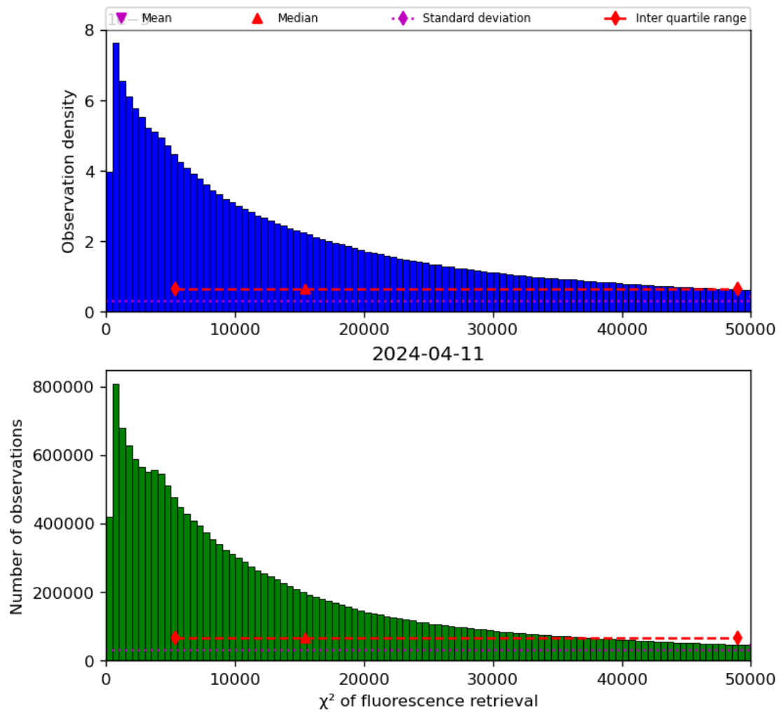
Figure 42: Histogram of “ \chi^2 of fluorescence retrieval” for 2024-04-10 to 2024-04-12
