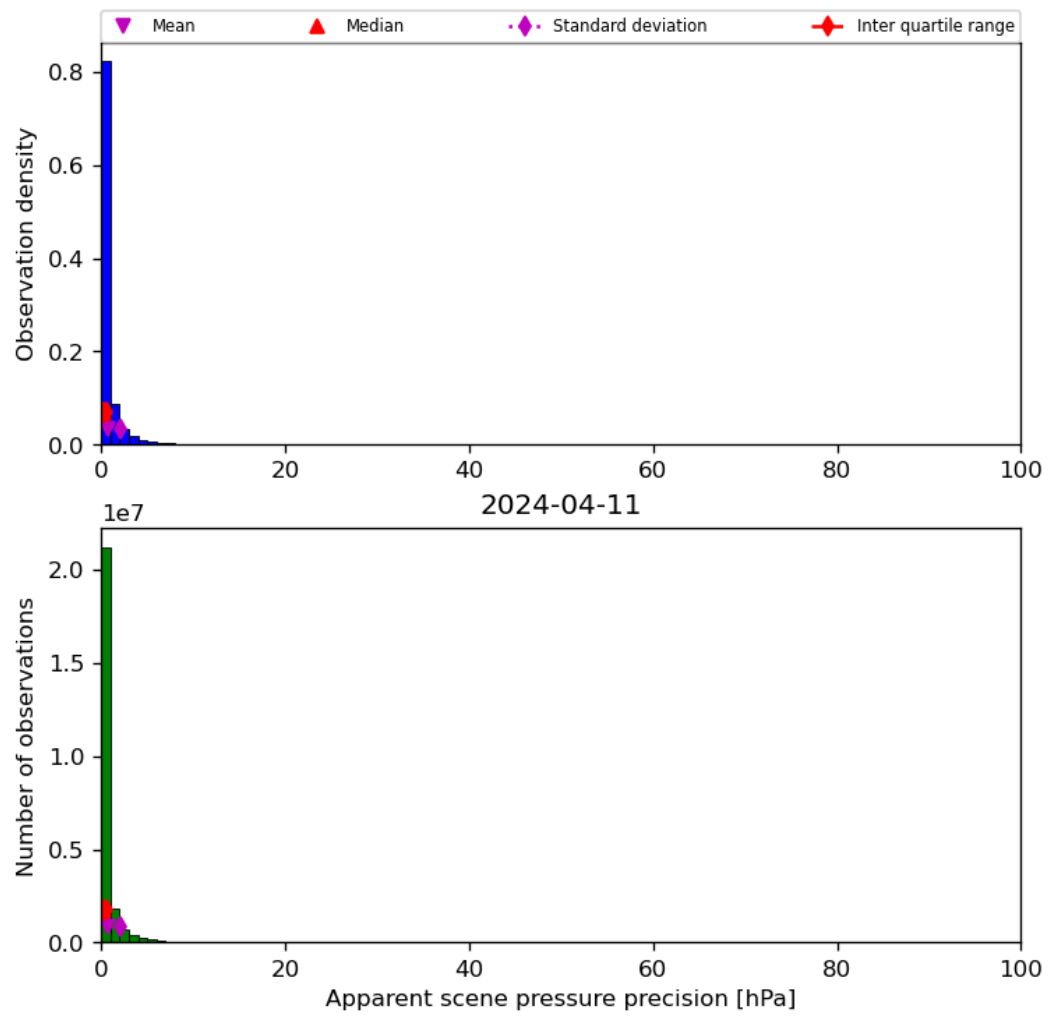
Figure 37: Histogram of “Apparent scene pressure precision” for 2024-04-10 to 2024-04-12
