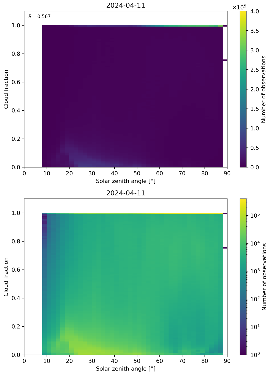
Figure 110: Scatter density plot of “Solar zenith angle” against “Cloud fraction” for 2024-04-10 to 2024-04-12.
