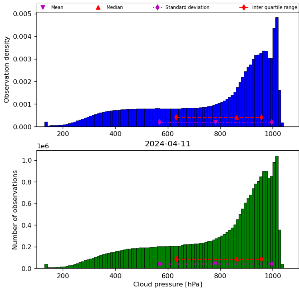
Figure 30: Histogram of “Cloud pressure” for 2024-04-10 to 2024-04-12
