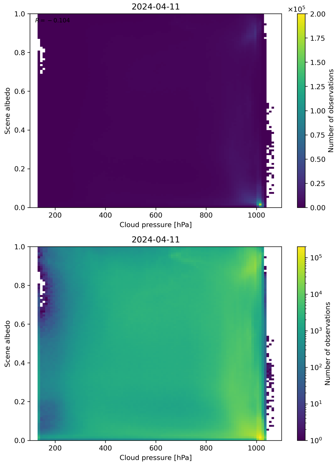
Figure 83: Scatter density plot of “Cloud pressure” against “Scene albedo” for 2024-04-10 to 2024-04-12.
