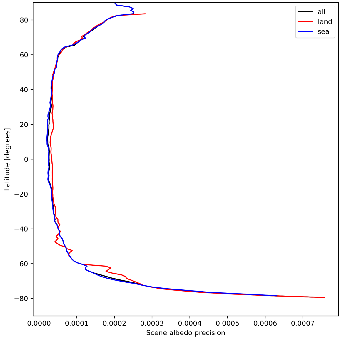
Figure 18: Zonal average of “Scene albedo precision” for 2024-04-10 to 2024-04-12.
