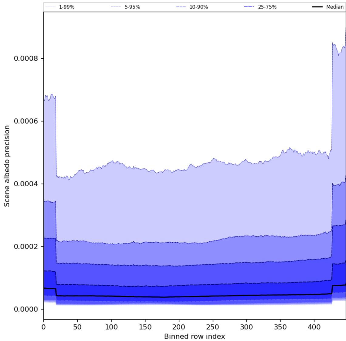
Figure 52: Along track statistics of “Scene albedo precision” for 2024-04-10 to 2024-04-12
