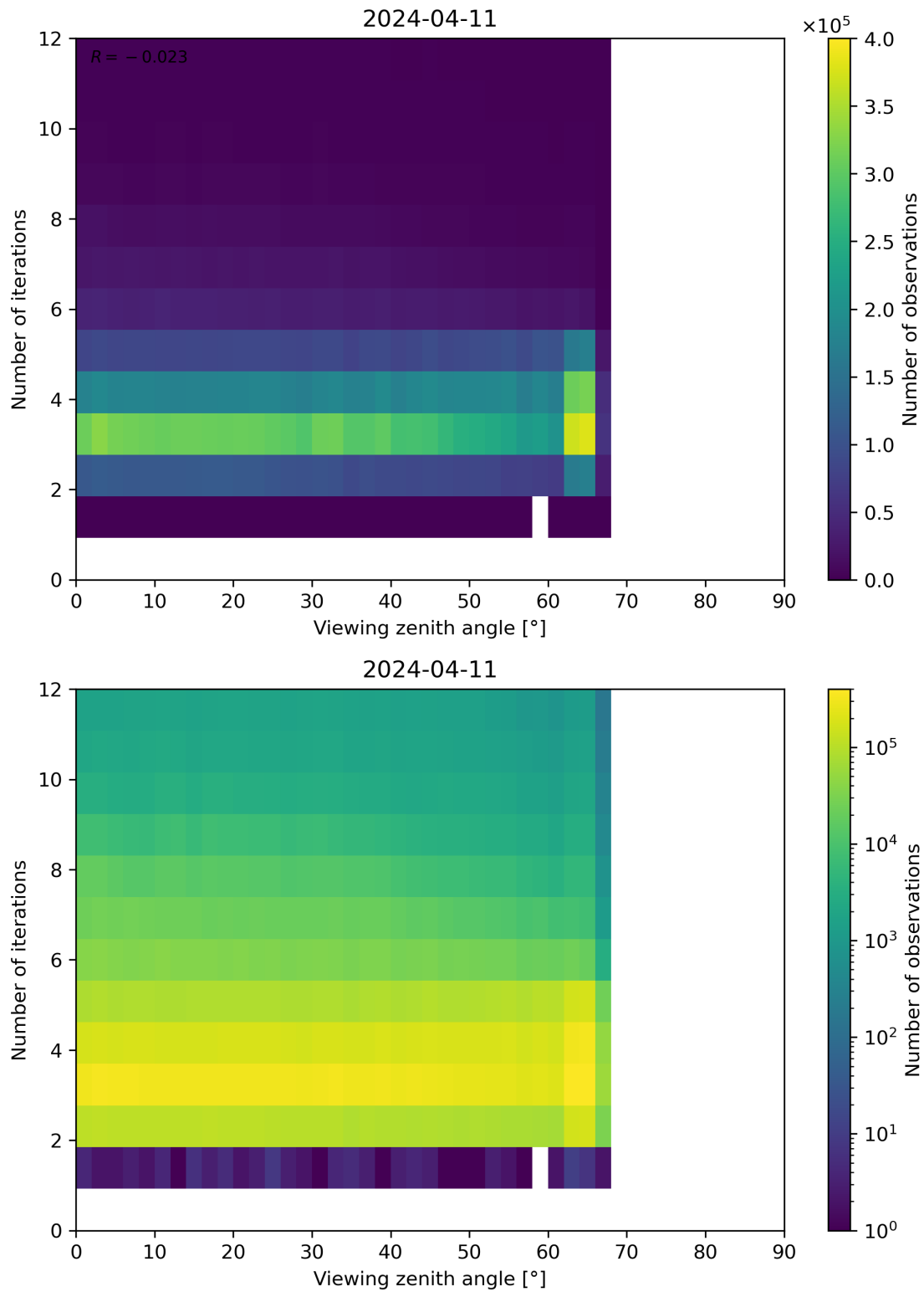
Figure 124: Scatter density plot of “Viewing zenith angle” against “Number of iterations” for 2024-04-10 to 2024-04-12.
