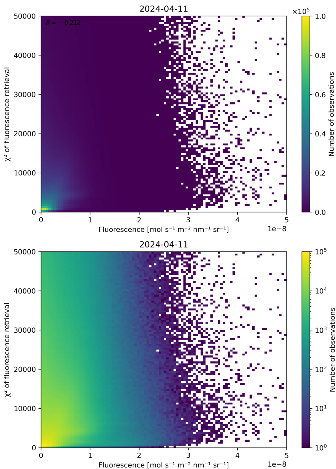
Figure 85: Scatter density plot of “Fluorescence” against “ \chi^2 of fluorescence retrieval” for 2024-04-10 to 2024-04-12.
