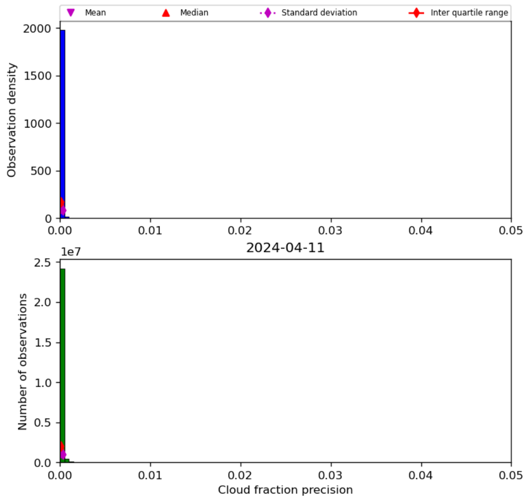
Figure 33: Histogram of “Cloud fraction precision” for 2024-04-10 to 2024-04-12
