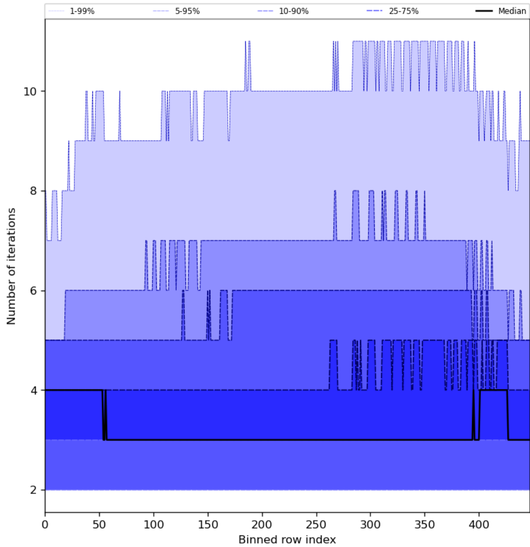
Figure 56: Along track statistics of “Number of iterations” for 2024-04-10 to 2024-04-12
