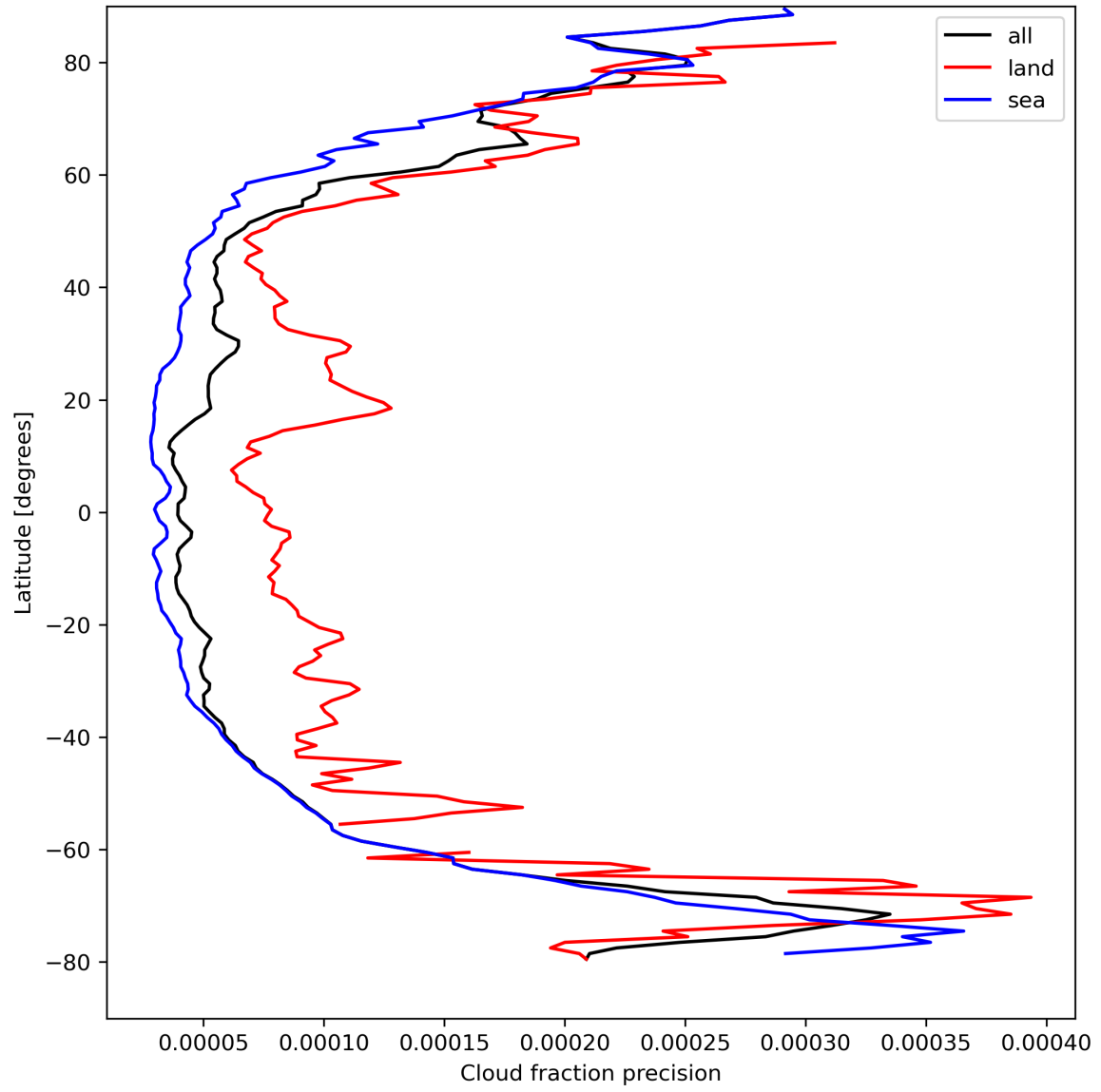
Figure 16: Zonal average of “Cloud fraction precision” for 2024-04-10 to 2024-04-12.
