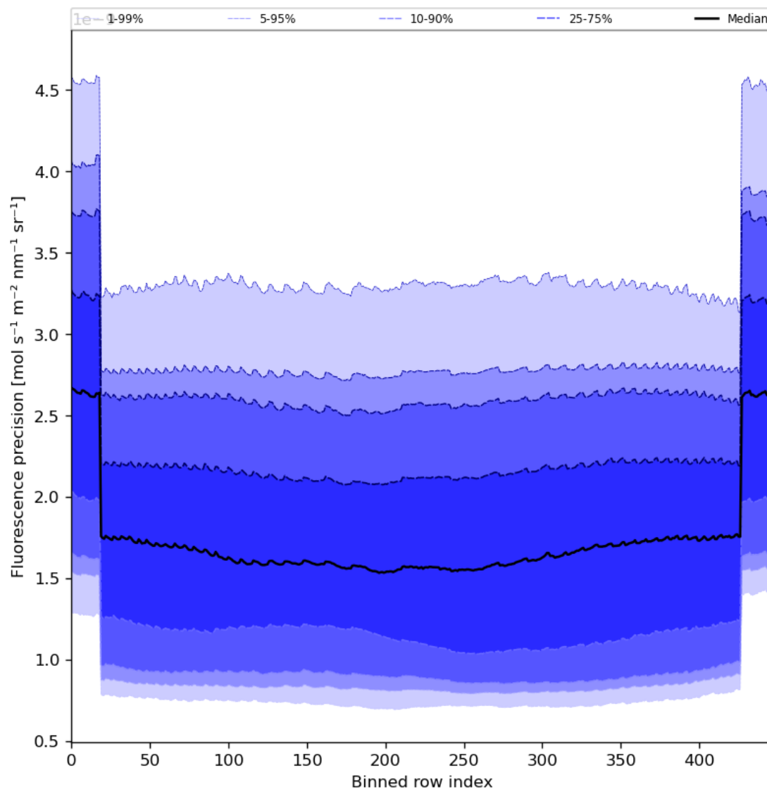
Figure 58: Along track statistics of “Fluorescence precision” for 2024-04-10 to 2024-04-12
