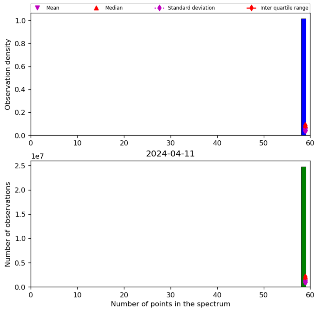
Figure 44: Histogram of "Number of points in the spectrum" for 2024-04-10 to 2024-04-12
