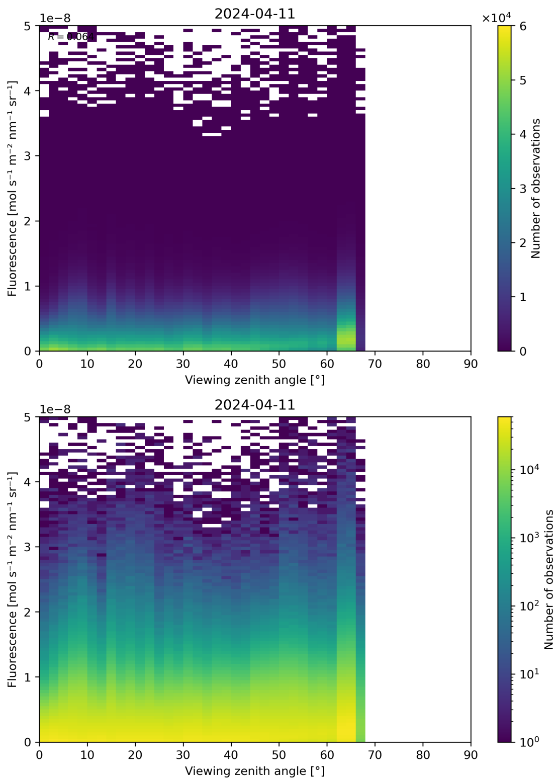
Figure 122: Scatter density plot of “Viewing zenith angle” against “Fluorescence” for 2024-04-10 to 2024-04-12.
