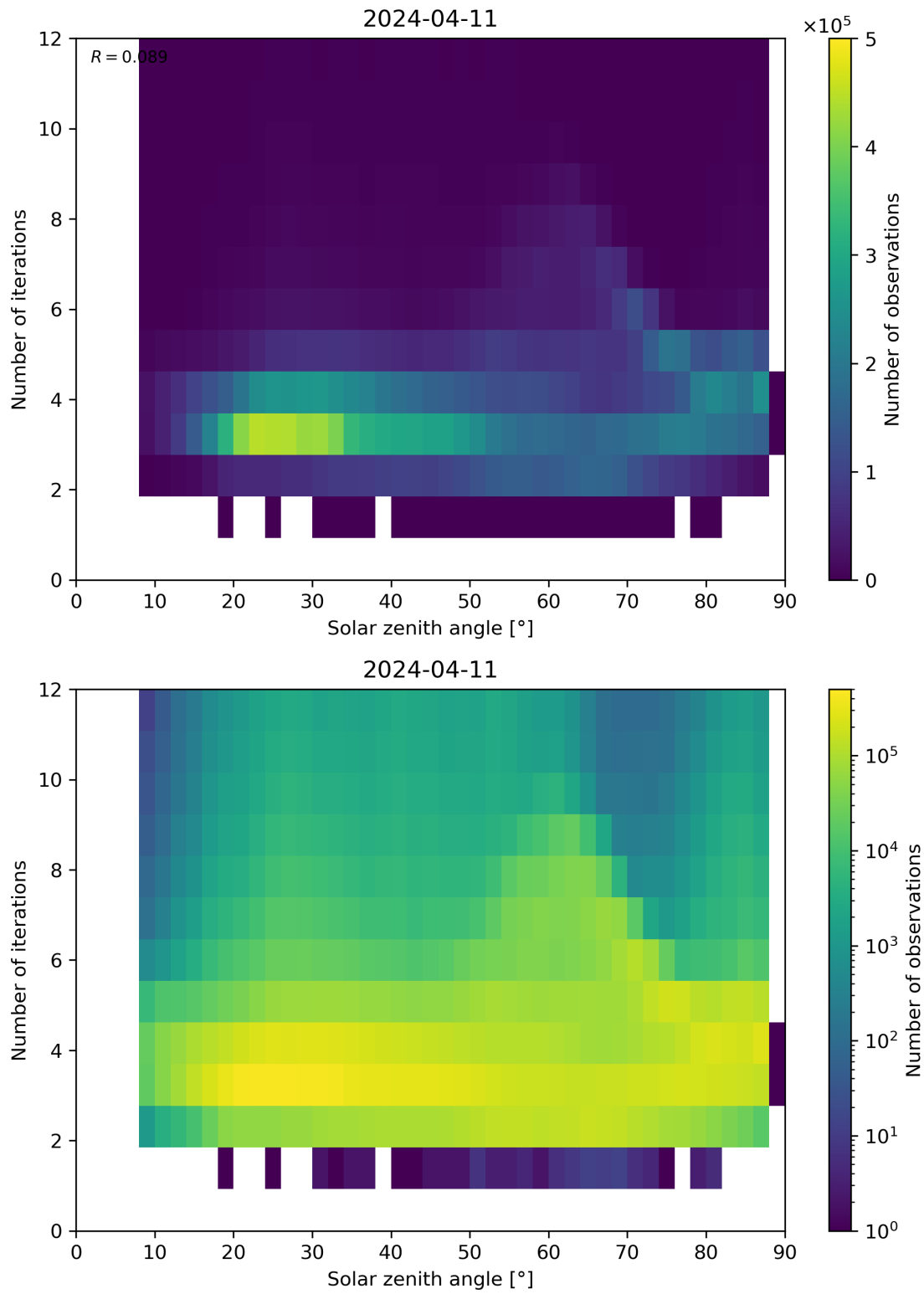
Figure 114: Scatter density plot of “Solar zenith angle” against “Number of iterations” for 2024-04-10 to 2024-04-12.
