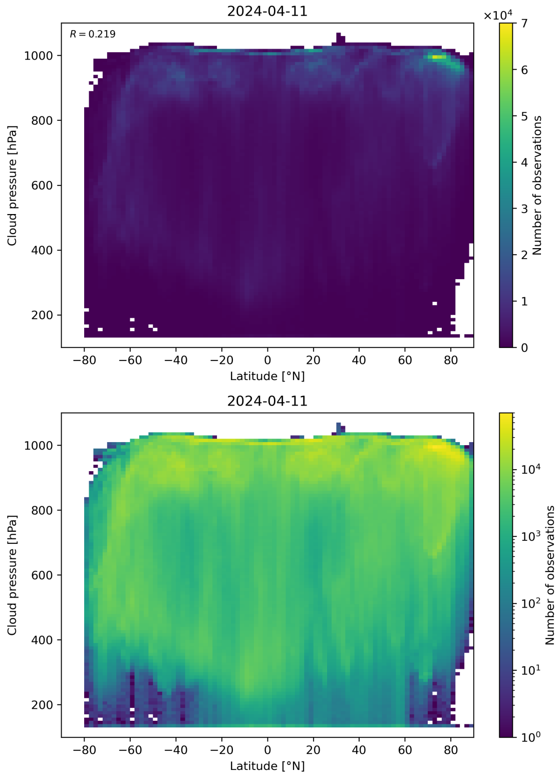
Figure 91: Scatter density plot of “Latitude” against “Cloud pressure” for 2024-04-10 to 2024-04-12.
