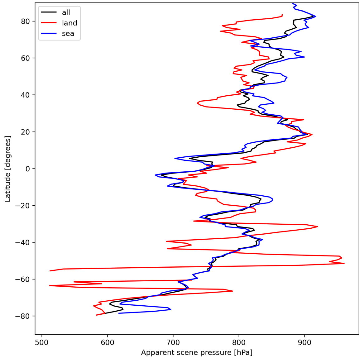
Figure 19: Zonal average of “Apparent scene pressure” for 2024-04-10 to 2024-04-12.
