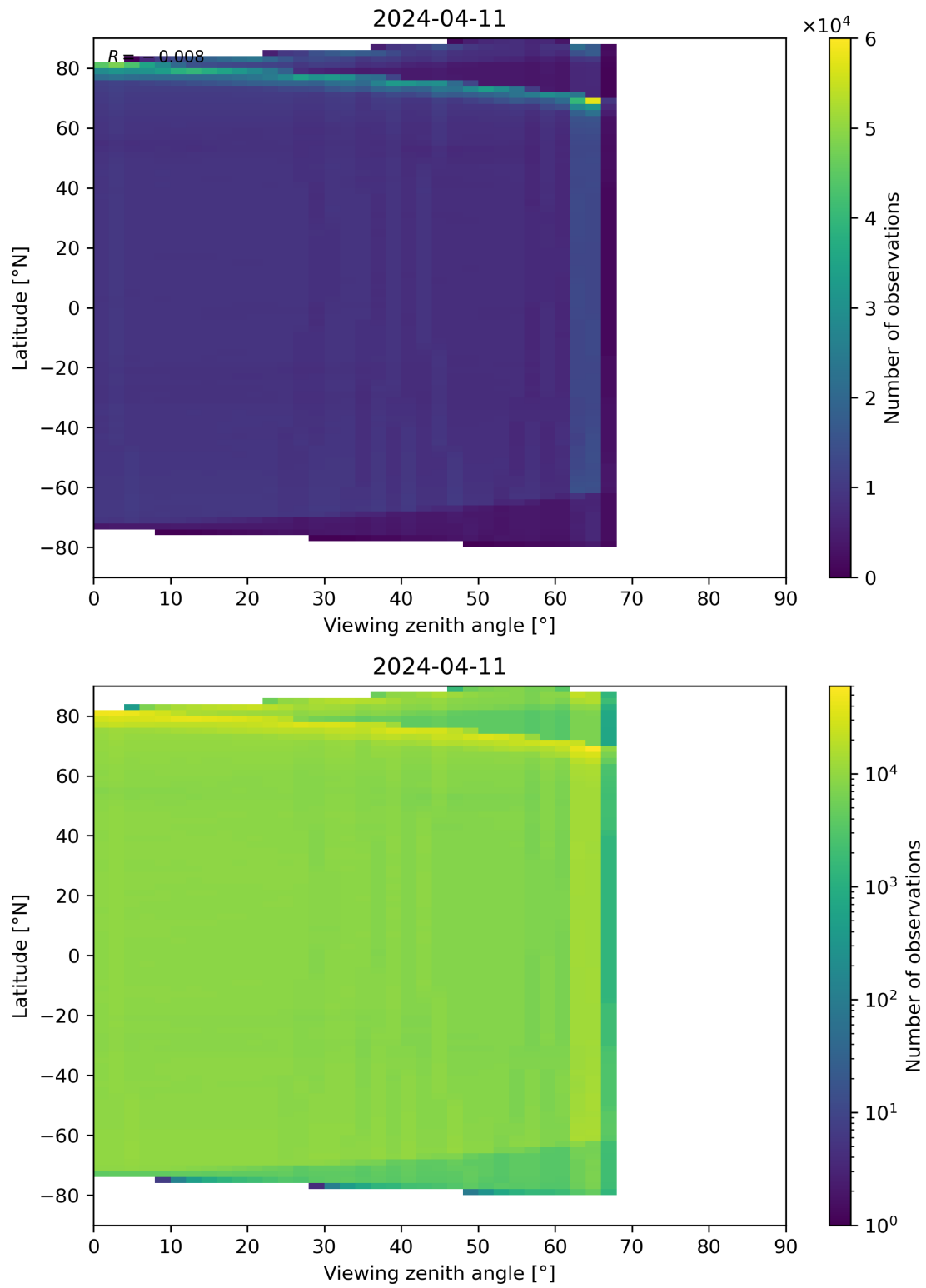
Figure 123: Scatter density plot of “Viewing zenith angle” against “Latitude” for 2024-04-10 to 2024-04-12.
