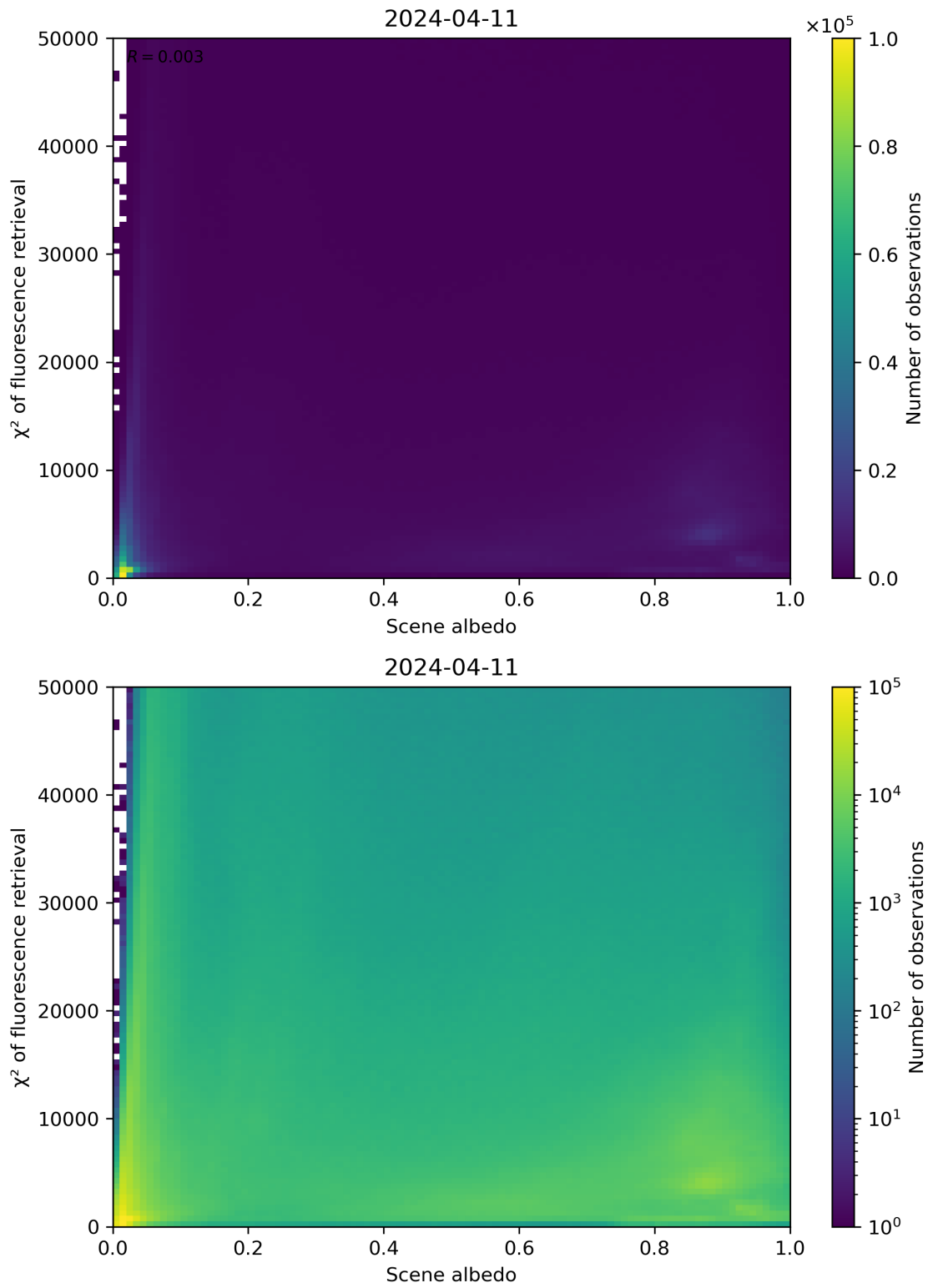
Figure 103: Scatter density plot of “Scene albedo” against “ \chi^2 of fluorescence retrieval” for 2024-04-10 to 2024-04-12.
