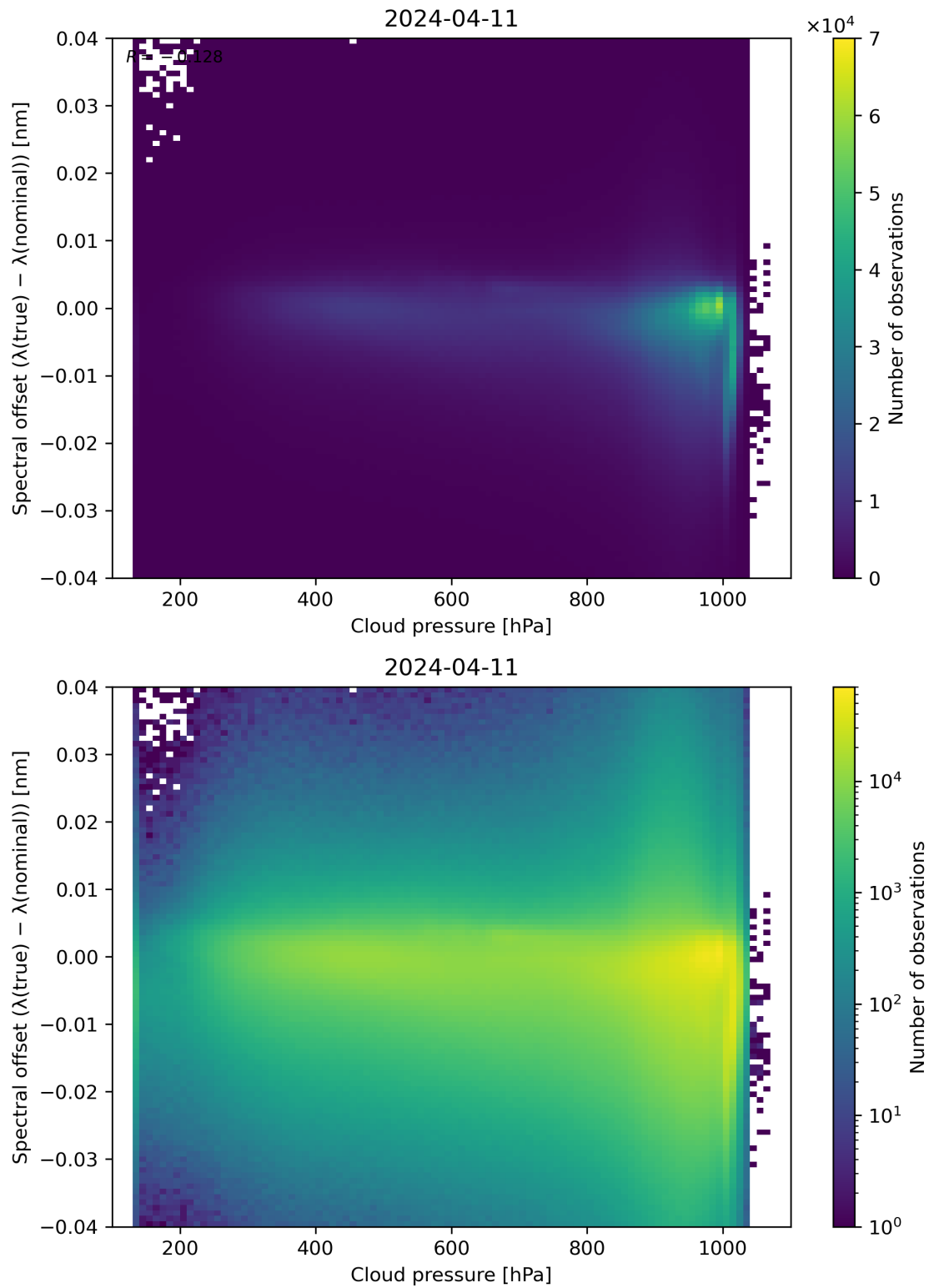
Figure 84: Scatter density plot of “Cloud pressure” against “Spectral offset ( \lambda(\text{true}) - \lambda(\text{nominal}) )” for 2024-04-10 to 2024-04-12.
