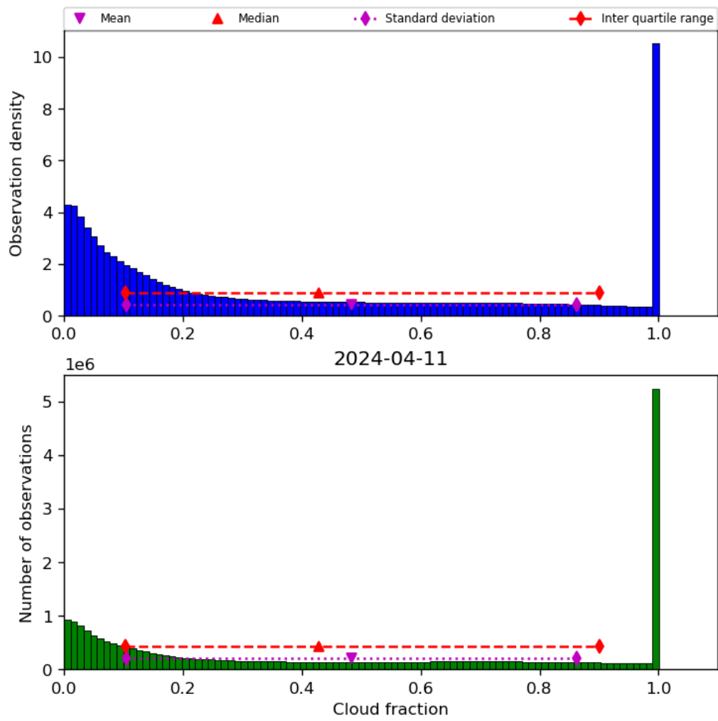
Figure 32: Histogram of “Cloud fraction” for 2024-04-10 to 2024-04-12
