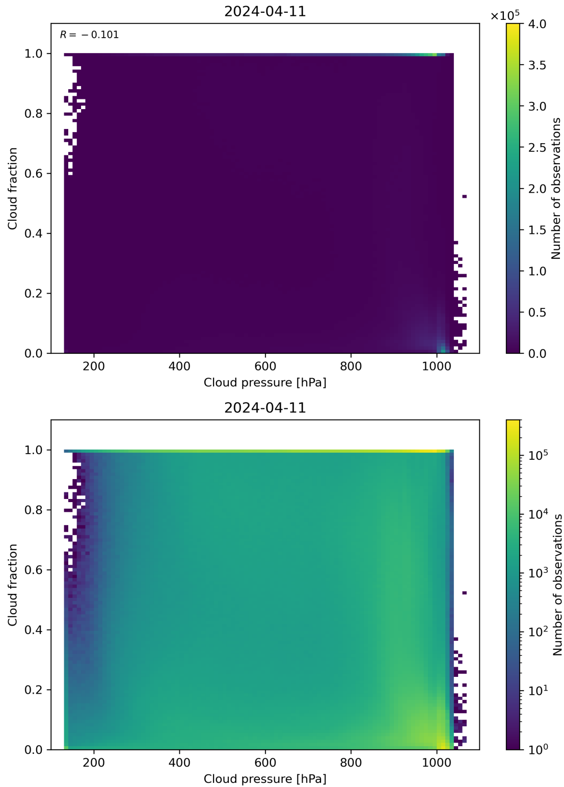
Figure 79: Scatter density plot of “Cloud pressure” against “Cloud fraction” for 2024-04-10 to 2024-04-12.
