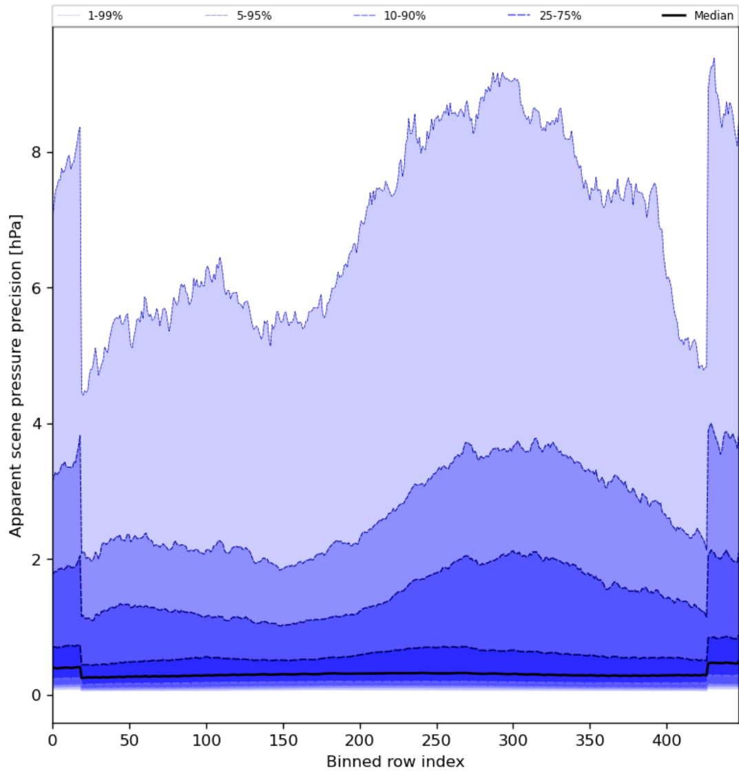
Figure 54: Along track statistics of “Apparent scene pressure precision” for 2024-04-10 to 2024-04-12
