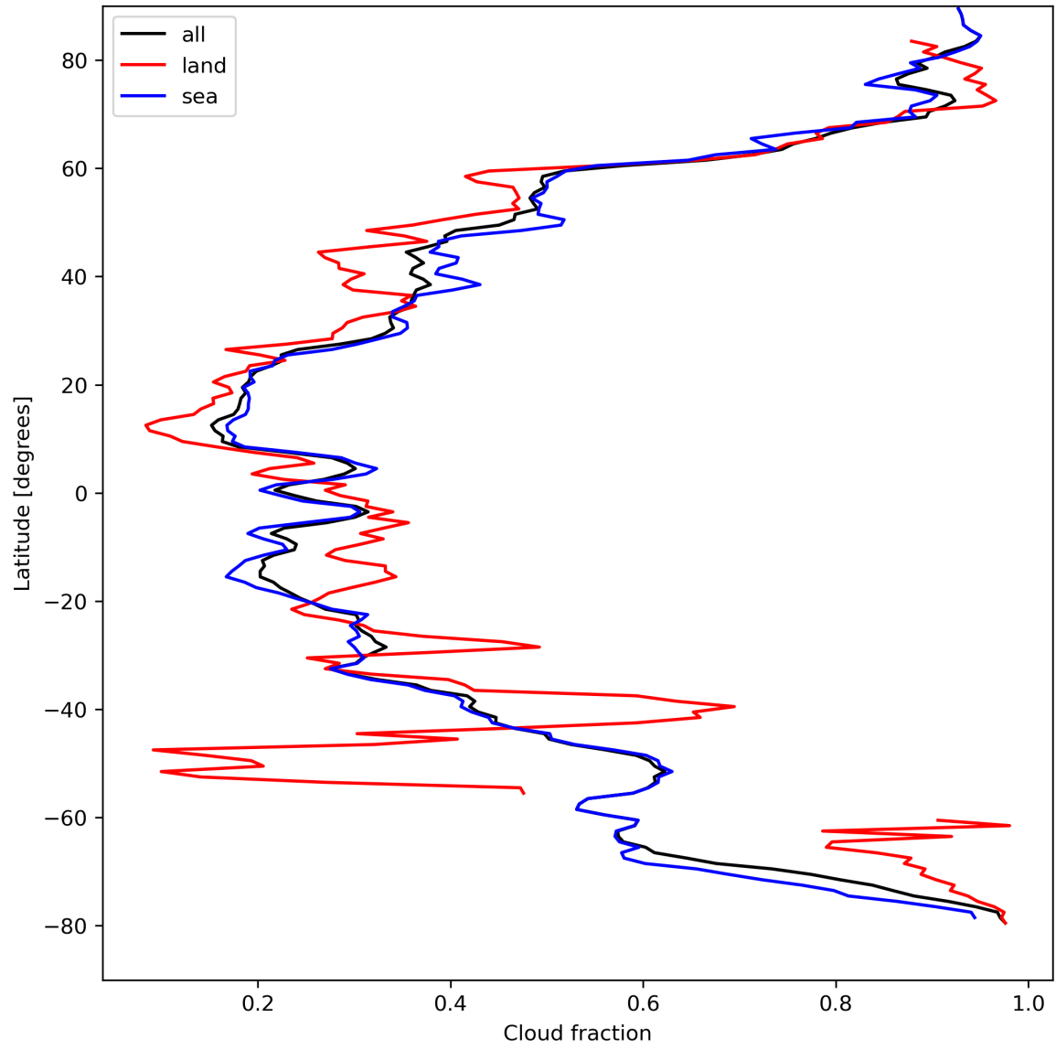
Figure 15: Zonal average of “Cloud fraction” for 2024-04-10 to 2024-04-12.
