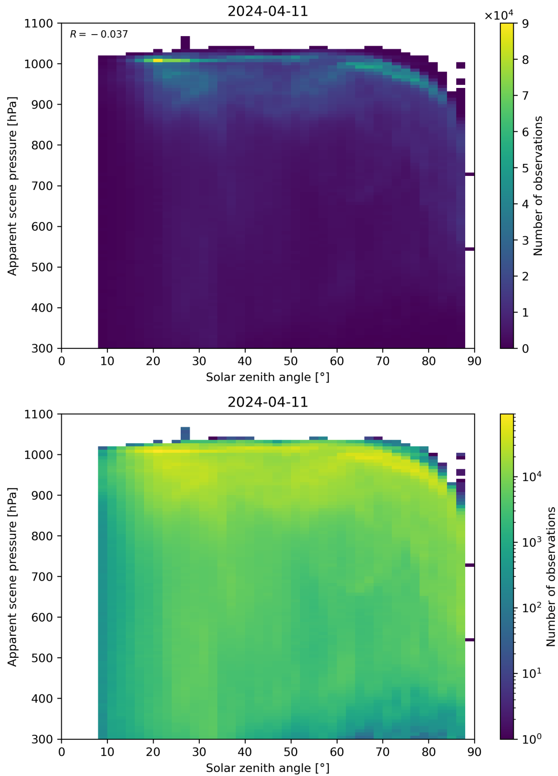
Figure 108: Scatter density plot of “Solar zenith angle” against “Apparent scene pressure” for 2024-04-10 to 2024-04-12.
