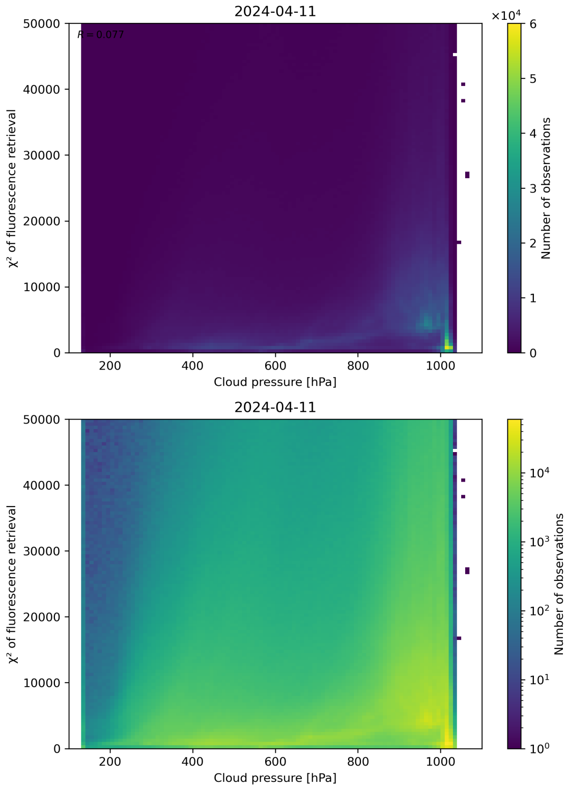
Figure 78: Scatter density plot of “Cloud pressure” against “ \chi^2 of fluorescence retrieval” for 2024-04-10 to 2024-04-12.
