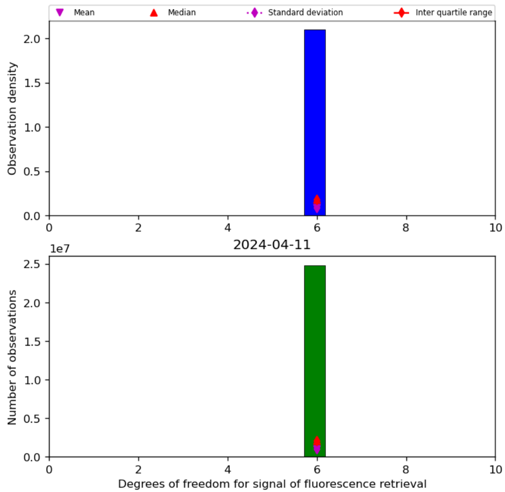
Figure 43: Histogram of “Degrees of freedom for signal of fluorescence retrieval” for 2024-04-10 to 2024-04-12
