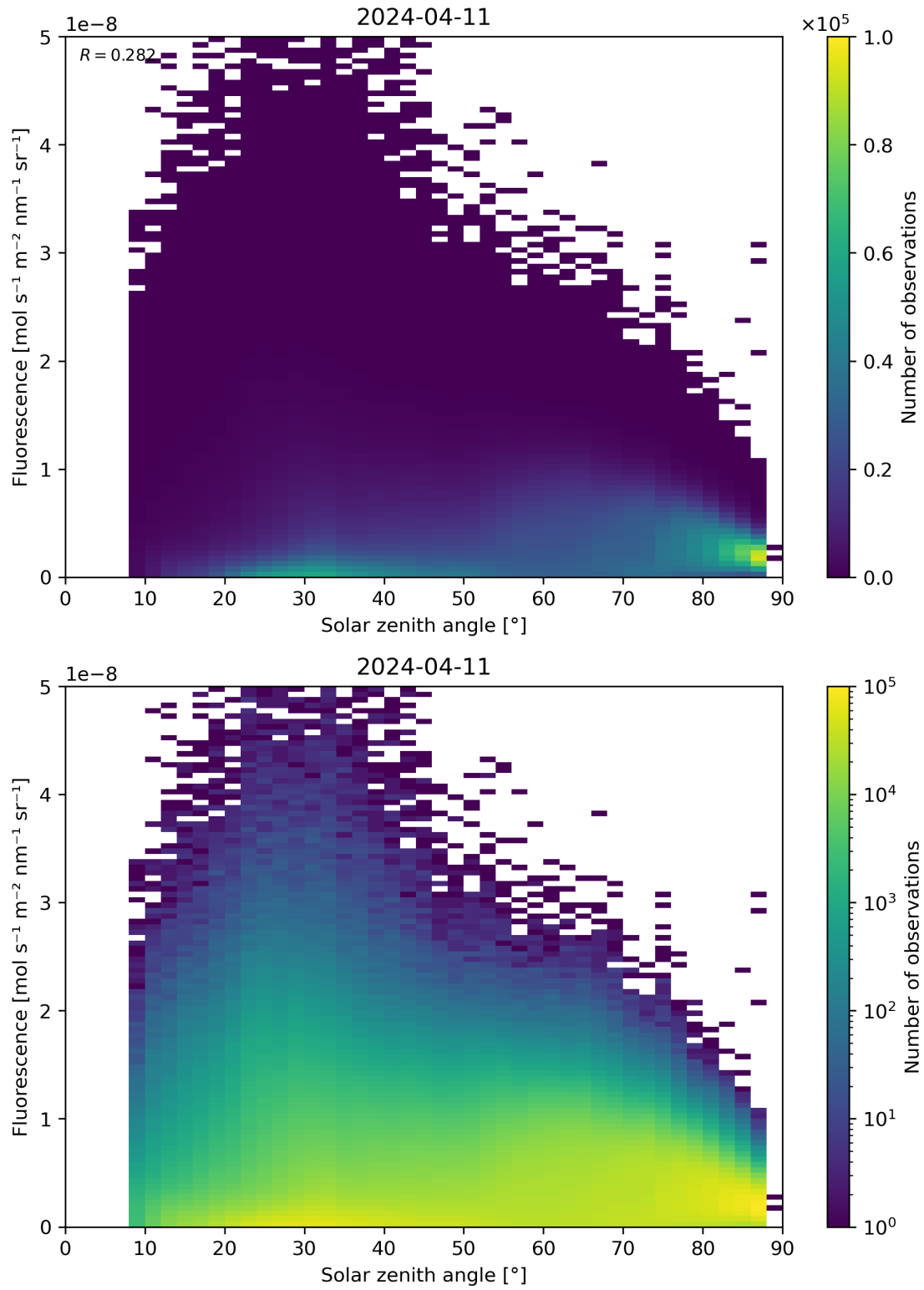
Figure 112: Scatter density plot of “Solar zenith angle” against “Fluorescence” for 2024-04-10 to 2024-04-12.
