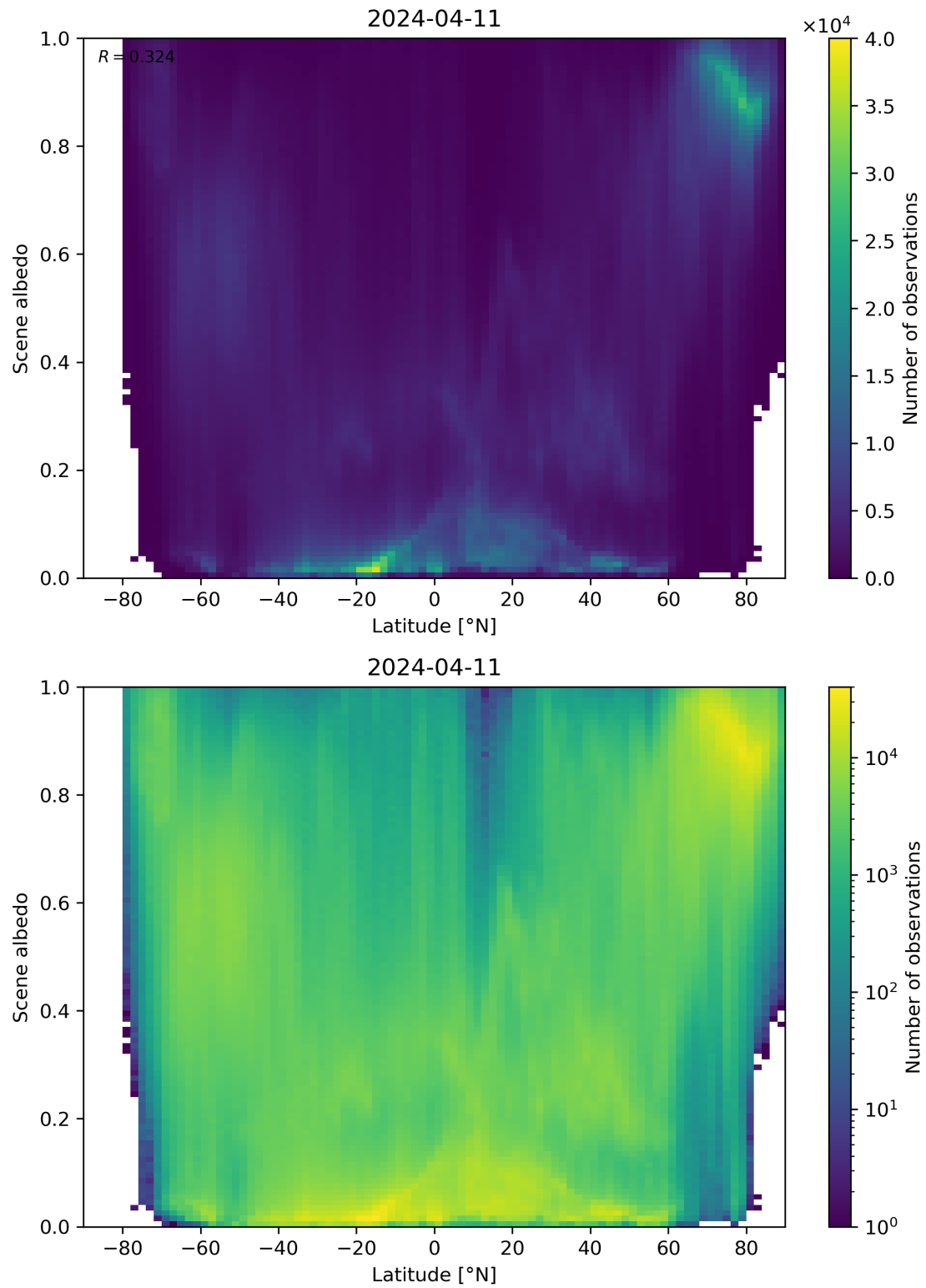
Figure 95: Scatter density plot of “Latitude” against “Scene albedo” for 2024-04-10 to 2024-04-12.
