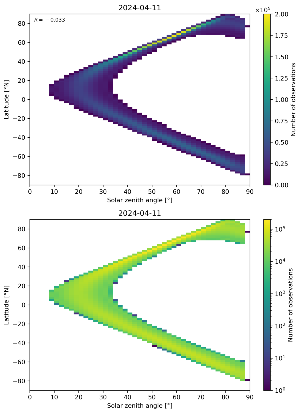
Figure 113: Scatter density plot of “Solar zenith angle” against “Latitude” for 2024-04-10 to 2024-04-12.
