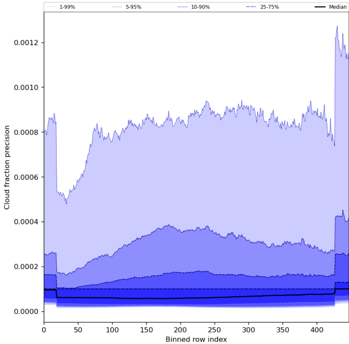
Figure 50: Along track statistics of “Cloud fraction precision” for 2024-04-10 to 2024-04-12
