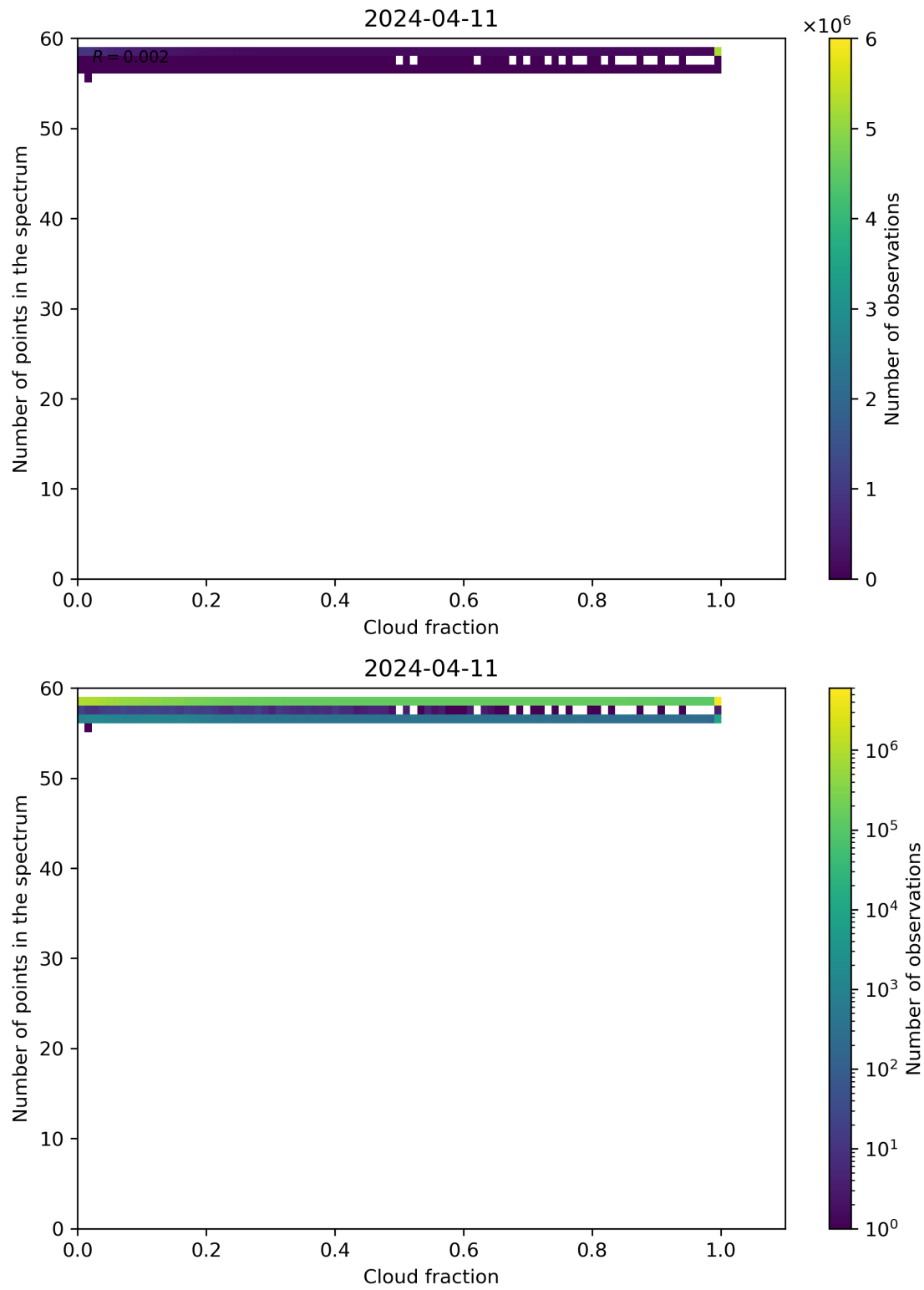
Figure 74: Scatter density plot of “Cloud fraction” against “Number of points in the spectrum” for 2024-04-10 to 2024-04-12.
