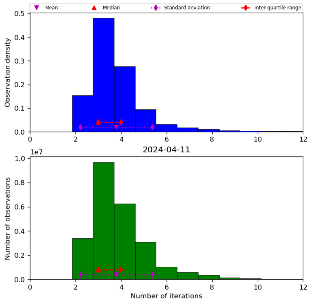
Figure 39: Histogram of “Number of iterations” for 2024-04-10 to 2024-04-12
