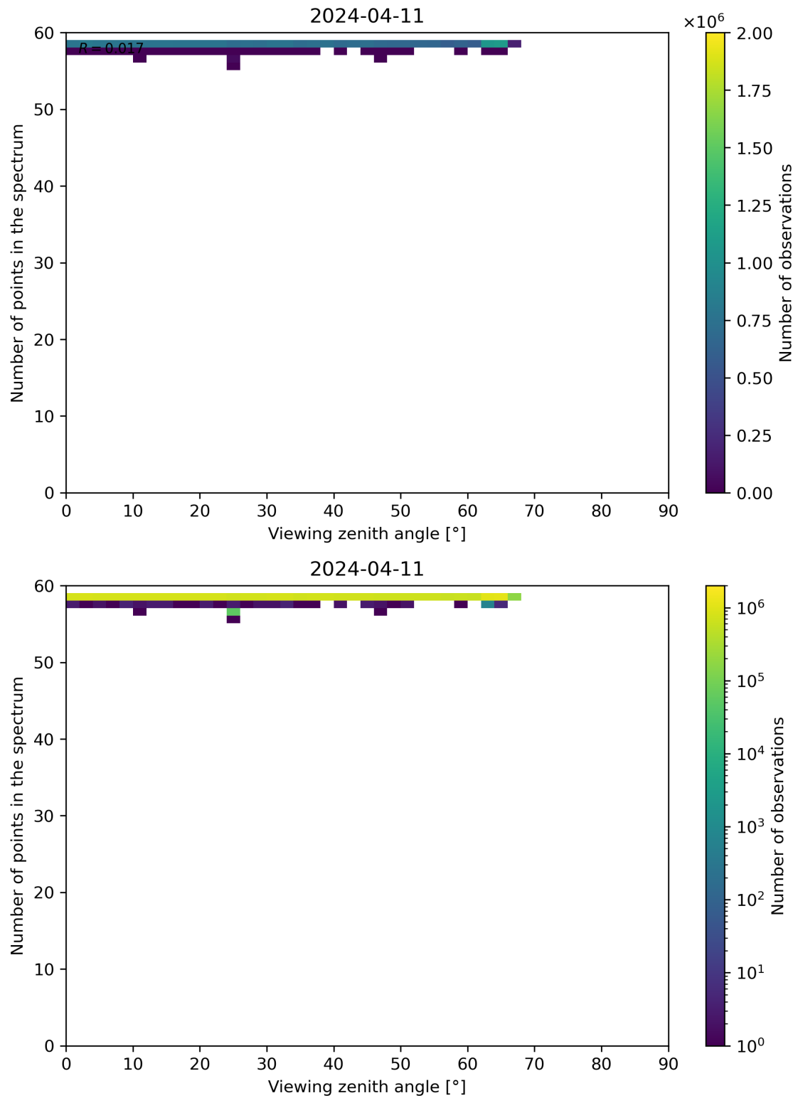
Figure 125: Scatter density plot of “Viewing zenith angle” against “Number of points in the spectrum” for 2024-04-10 to 2024-04-12.
