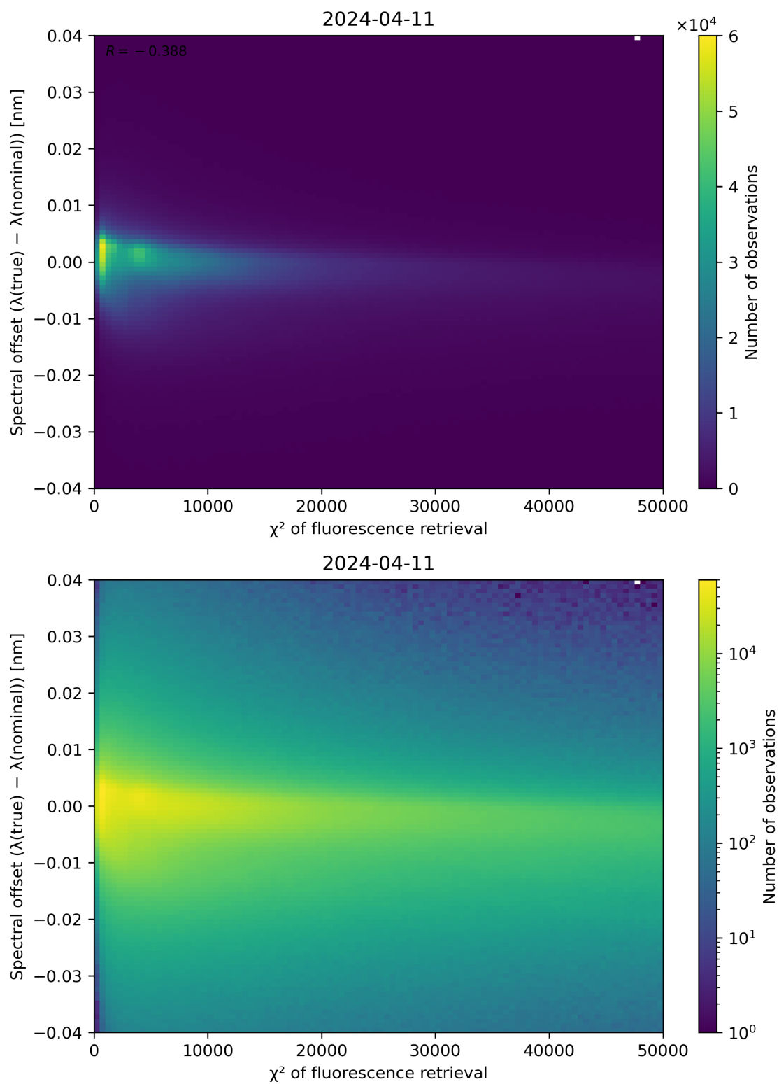
Figure 69: Scatter density plot of " \chi^2 of fluorescence retrieval" against "Spectral offset ( \lambda(\text{true}) - \lambda(\text{nominal}) )" for 2024-04-10 to 2024-04-12.
