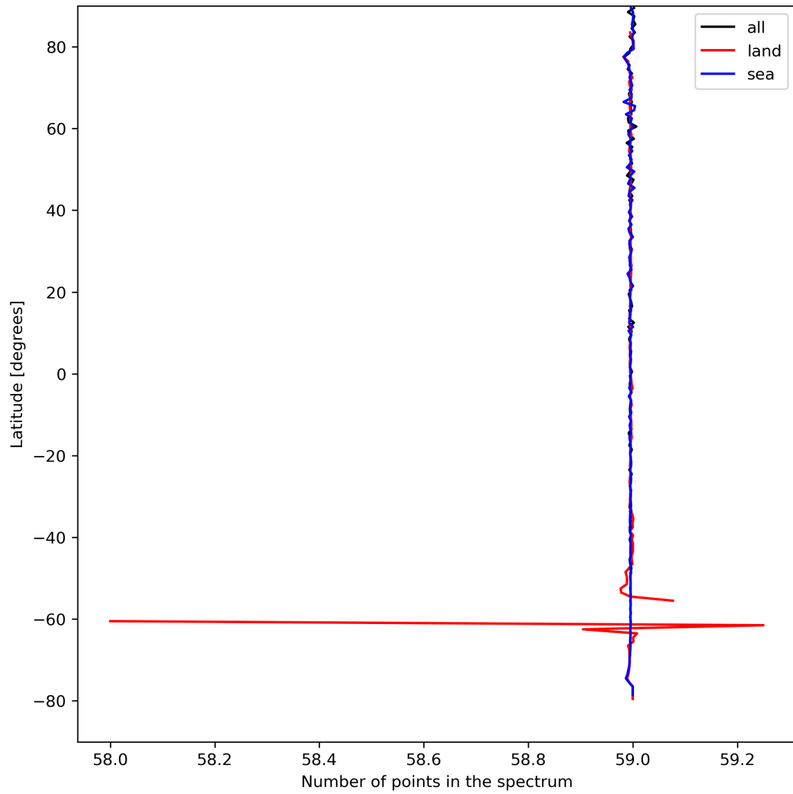
Figure 27: Zonal average of “Number of points in the spectrum” for 2024-04-10 to 2024-04-12.
