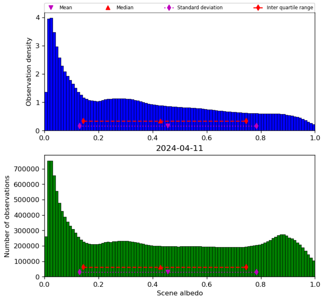
Figure 34: Histogram of “Scene albedo” for 2024-04-10 to 2024-04-12
