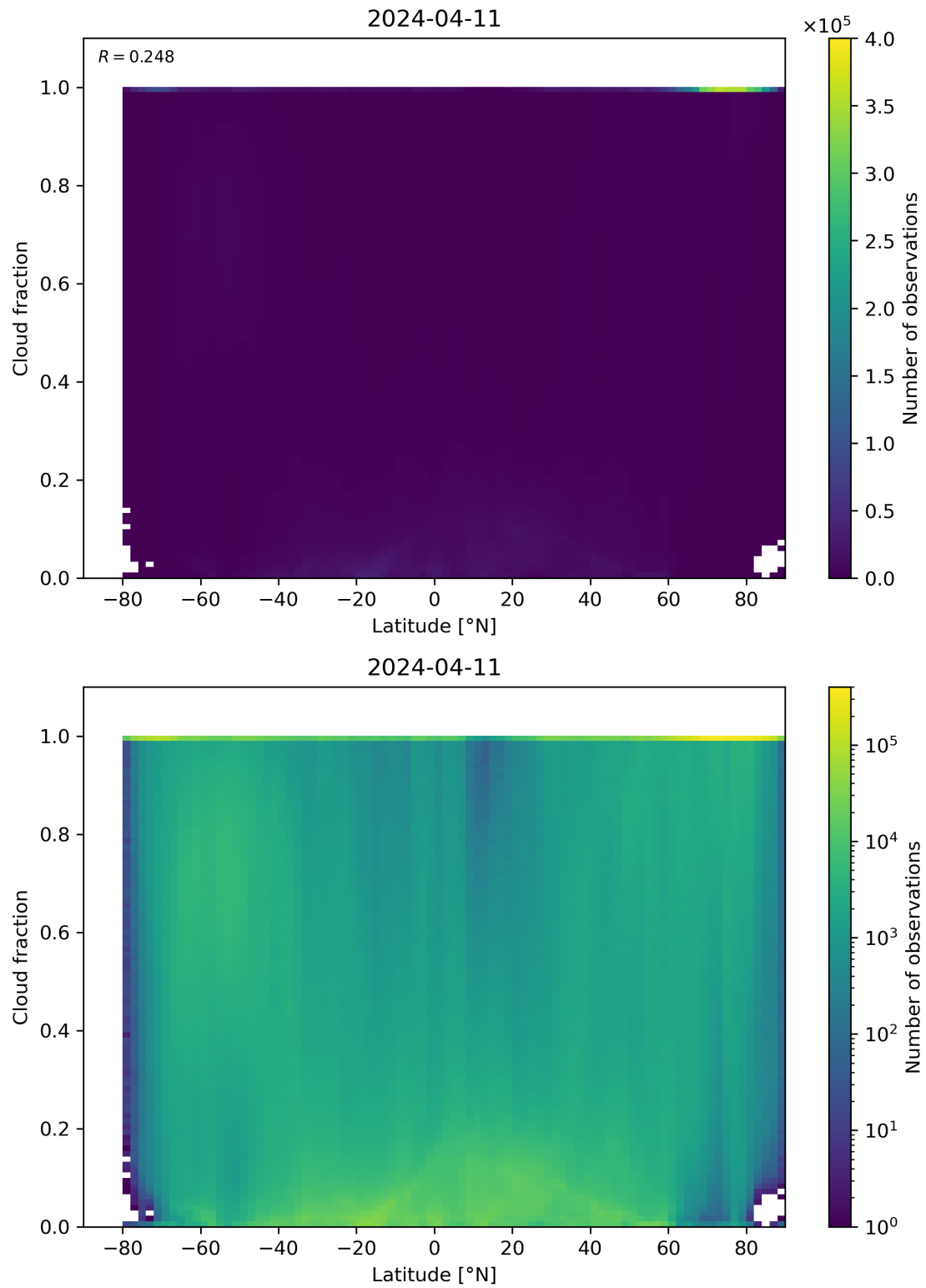
Figure 90: Scatter density plot of “Latitude” against “Cloud fraction” for 2024-04-10 to 2024-04-12.
