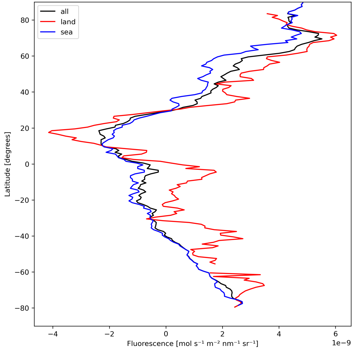
Figure 23: Zonal average of “Fluorescence” for 2024-04-10 to 2024-04-12.
