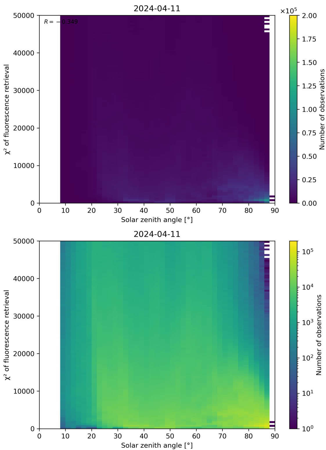
Figure 109: Scatter density plot of “Solar zenith angle” against “ \chi^2 of fluorescence retrieval” for 2024-04-10 to 2024-04-12.
