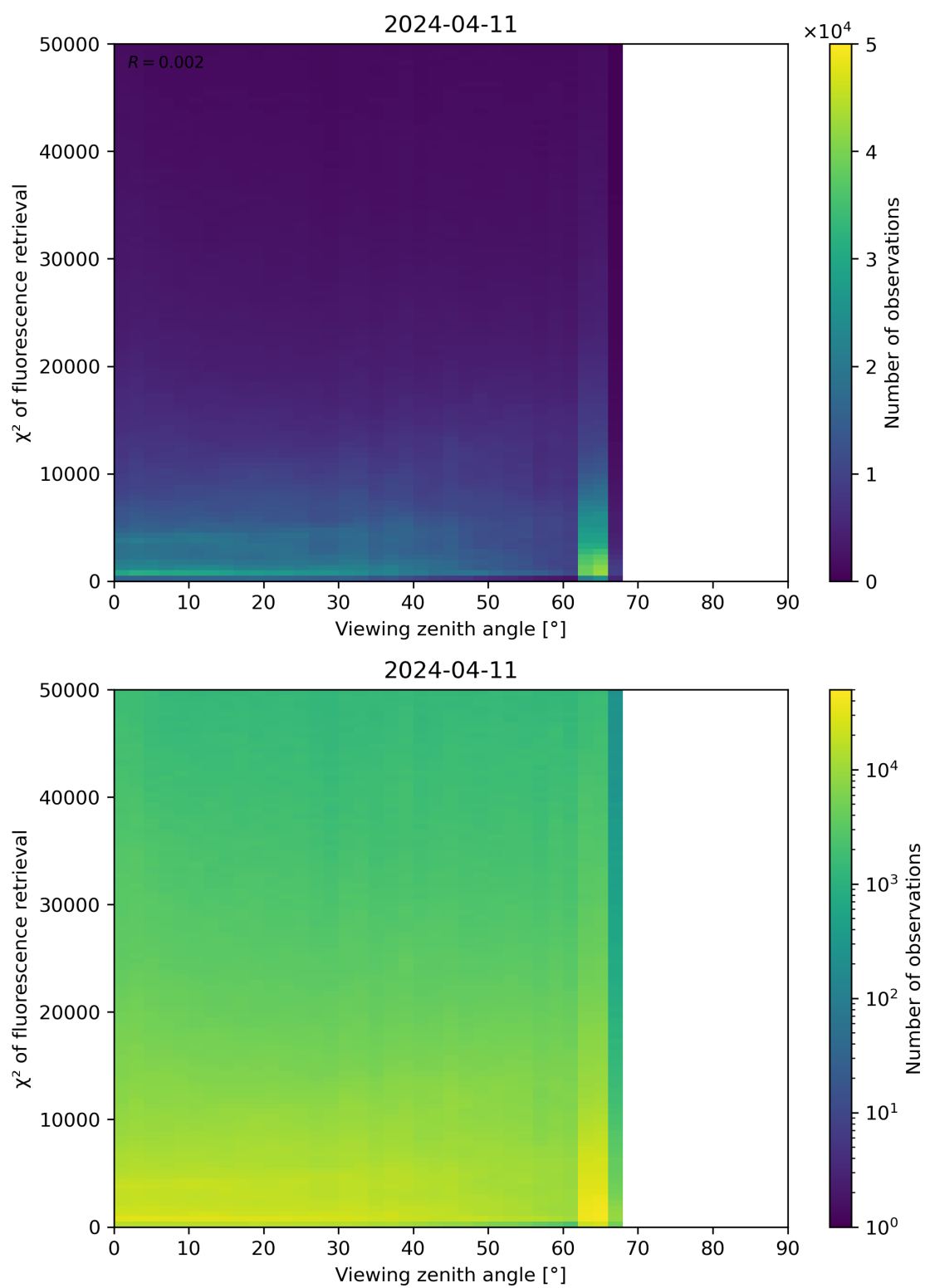
Figure 119: Scatter density plot of “Viewing zenith angle” against “ \chi^2 of fluorescence retrieval” for 2024-04-10 to 2024-04-12.
