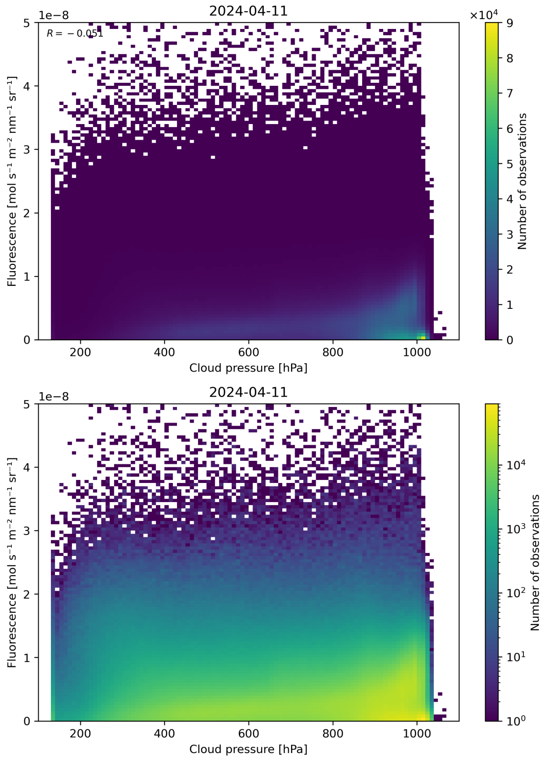
Figure 80: Scatter density plot of “Cloud pressure” against “Fluorescence” for 2024-04-10 to 2024-04-12.
