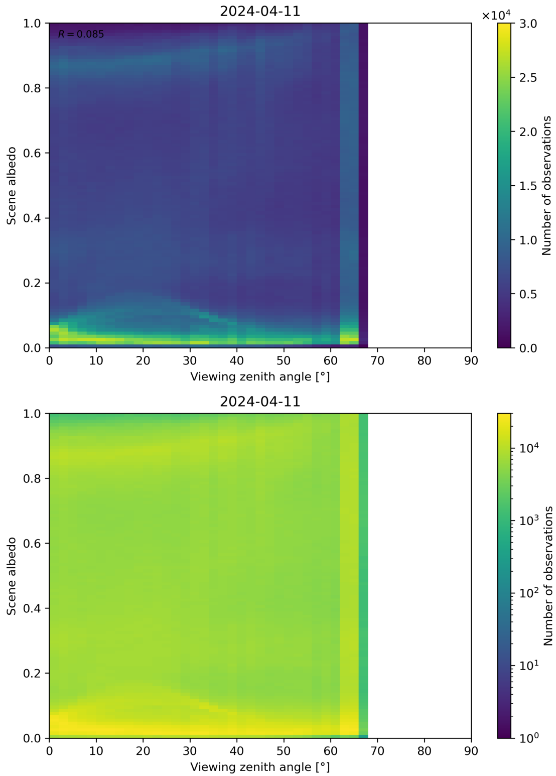
Figure 126: Scatter density plot of “Viewing zenith angle” against “Scene albedo” for 2024-04-10 to 2024-04-12.
