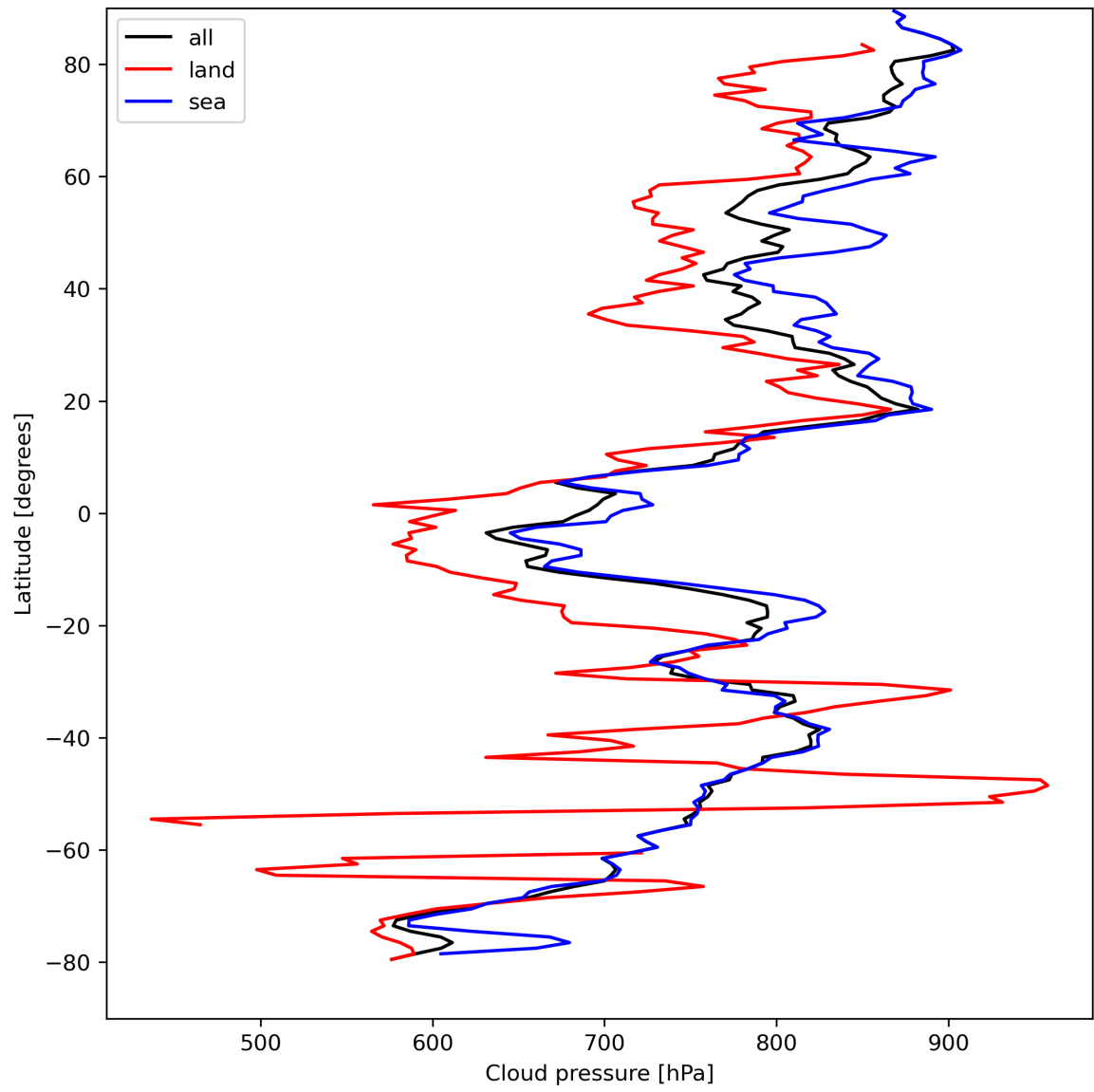
Figure 13: Zonal average of “Cloud pressure” for 2024-04-10 to 2024-04-12.
