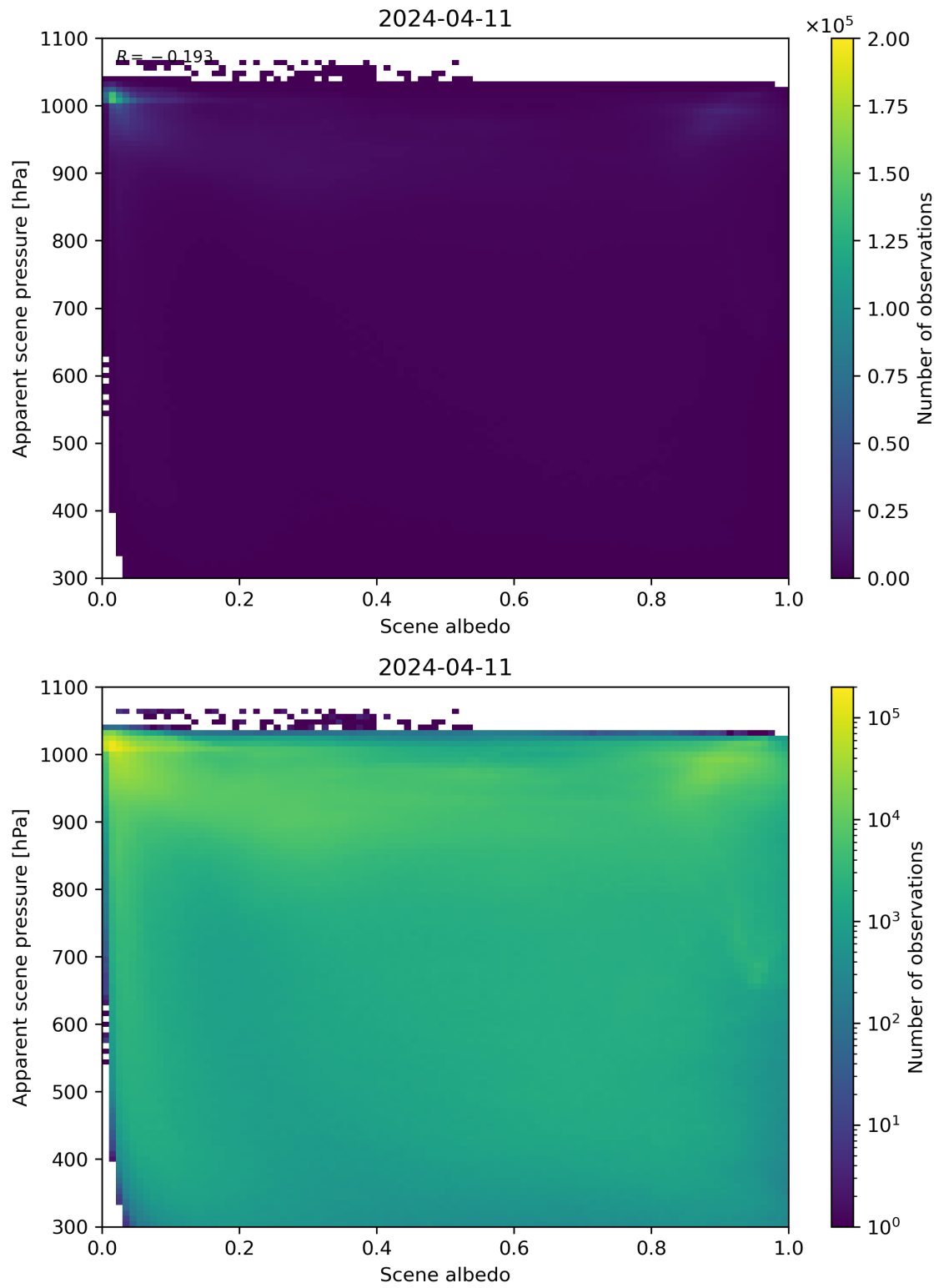
Figure 102: Scatter density plot of “Scene albedo” against “Apparent scene pressure” for 2024-04-10 to 2024-04-12.
