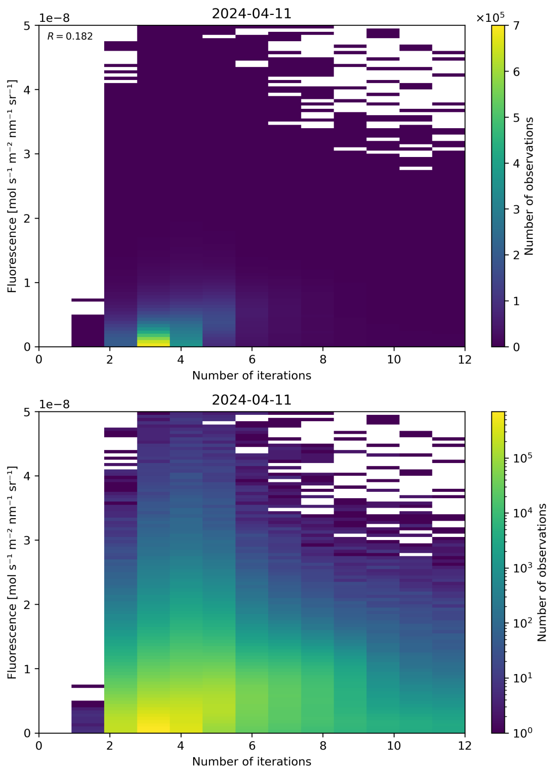
Figure 98: Scatter density plot of “Number of iterations” against “Fluorescence” for 2024-04-10 to 2024-04-12.
