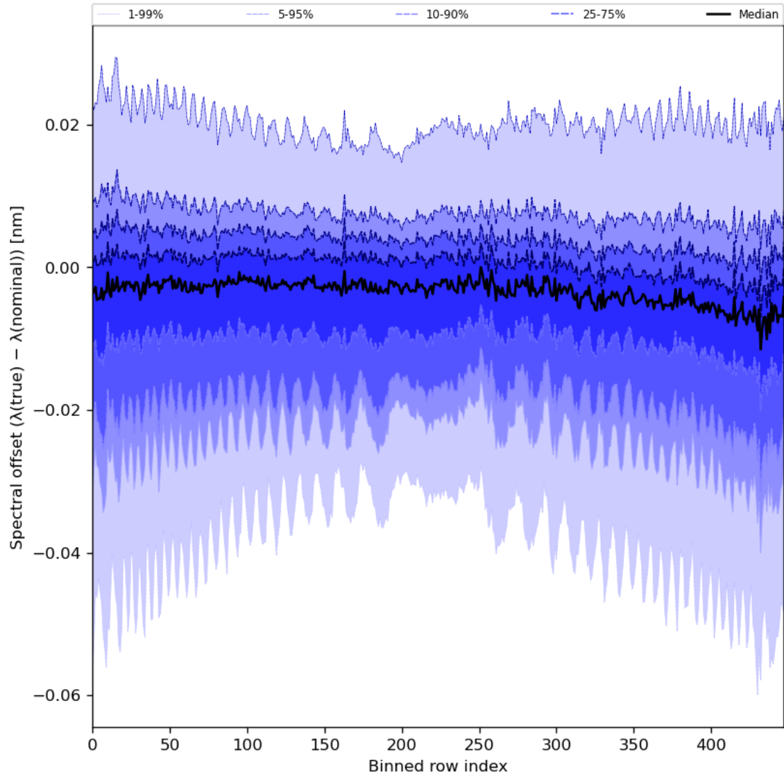
Figure 62: Along track statistics of “Spectral offset ( \lambda(\text{true}) - \lambda(\text{nominal}) )” for 2024-04-10 to 2024-04-12
