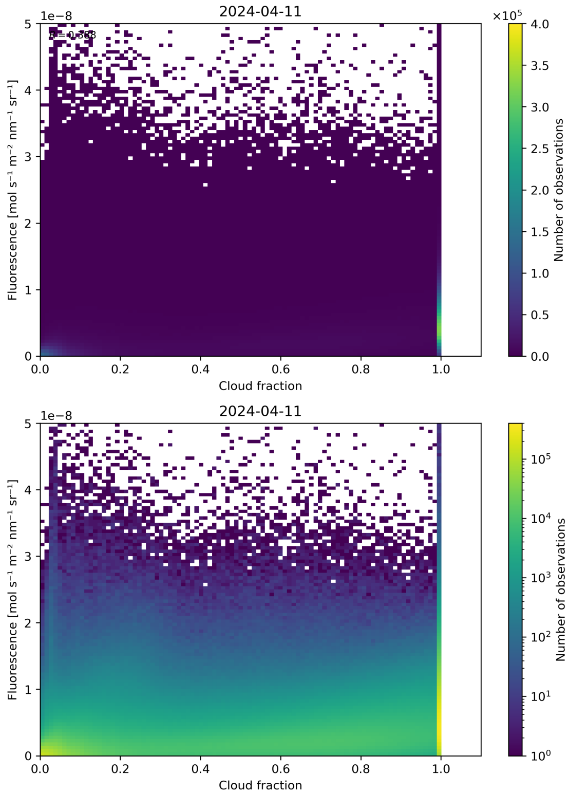
Figure 72: Scatter density plot of “Cloud fraction” against “Fluorescence” for 2024-04-10 to 2024-04-12.
