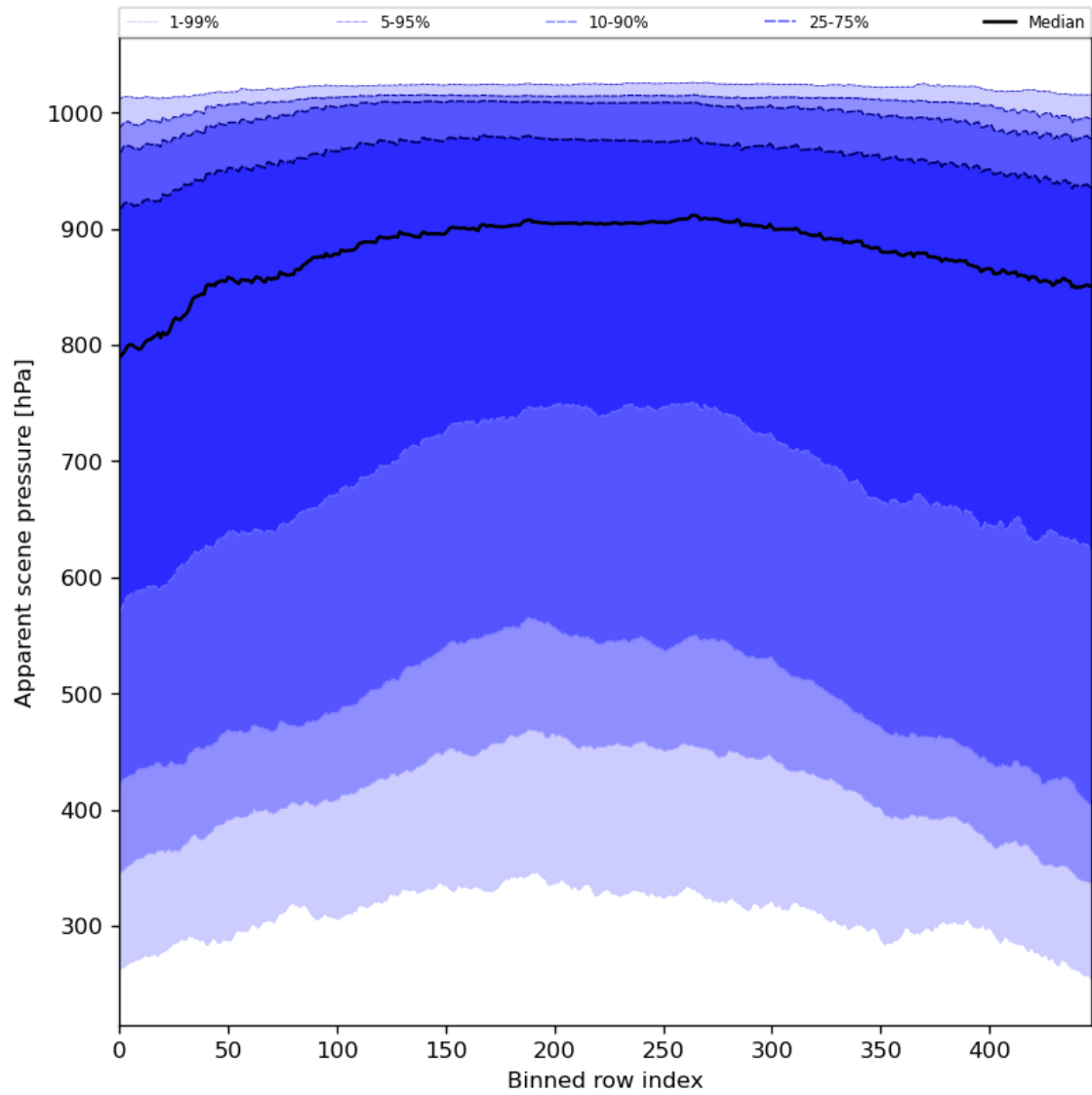
Figure 53: Along track statistics of “Apparent scene pressure” for 2024-04-10 to 2024-04-12
