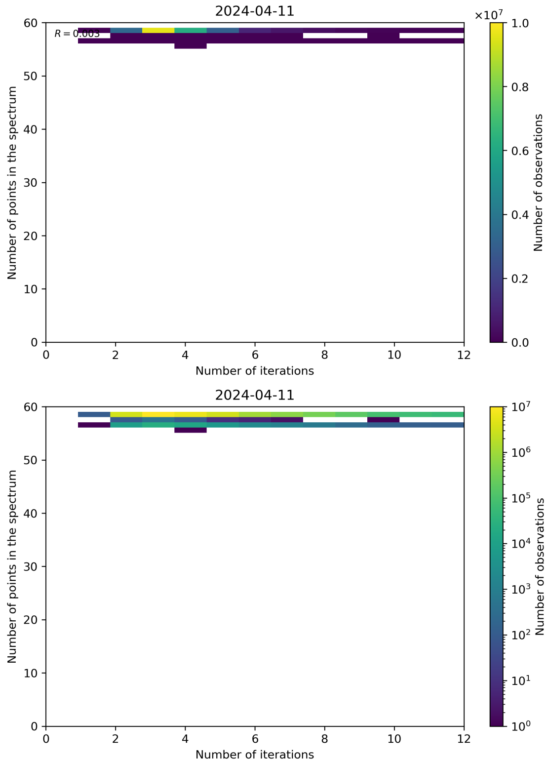
Figure 99: Scatter density plot of “Number of iterations” against “Number of points in the spectrum” for 2024-04-10 to 2024-04-12.
