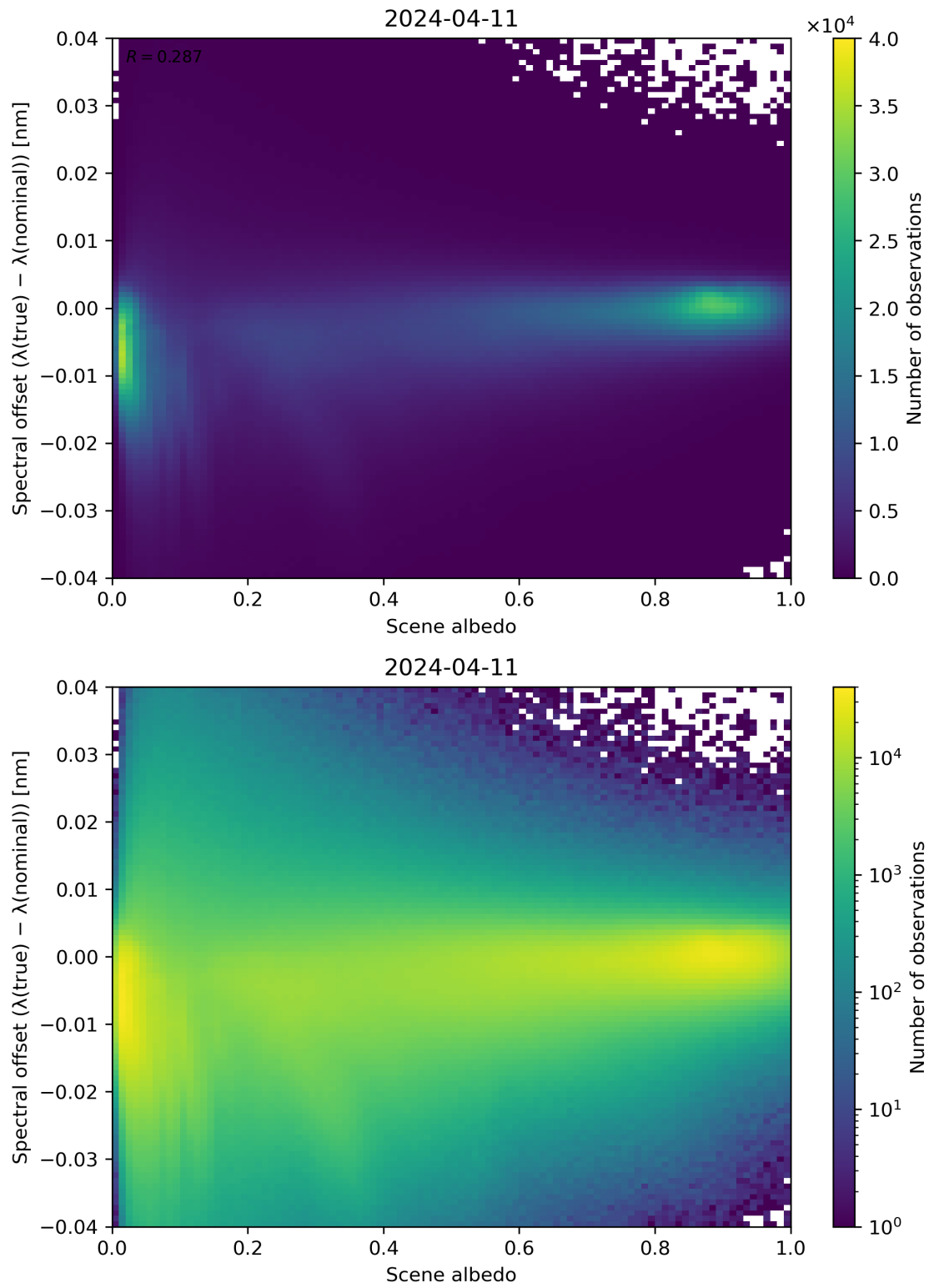
Figure 107: Scatter density plot of “Scene albedo” against “Spectral offset ( \lambda(\text{true}) - \lambda(\text{nominal}) )” for 2024-04-10 to 2024-04-12.
