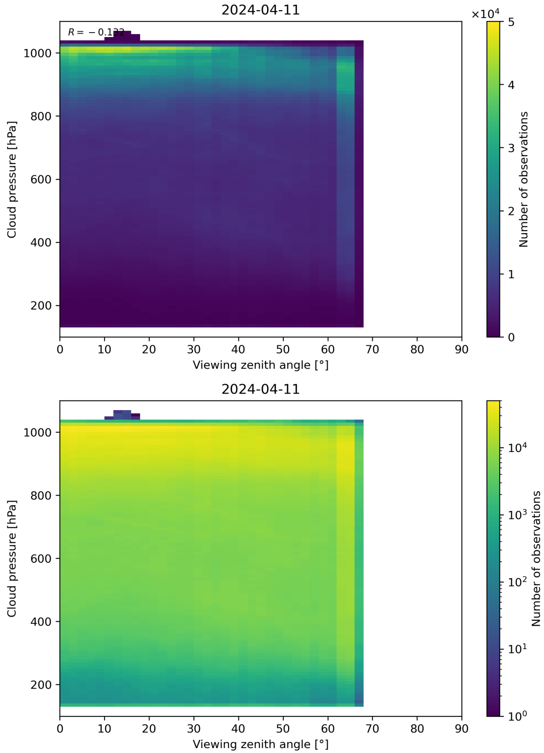
Figure 121: Scatter density plot of “Viewing zenith angle” against “Cloud pressure” for 2024-04-10 to 2024-04-12.
