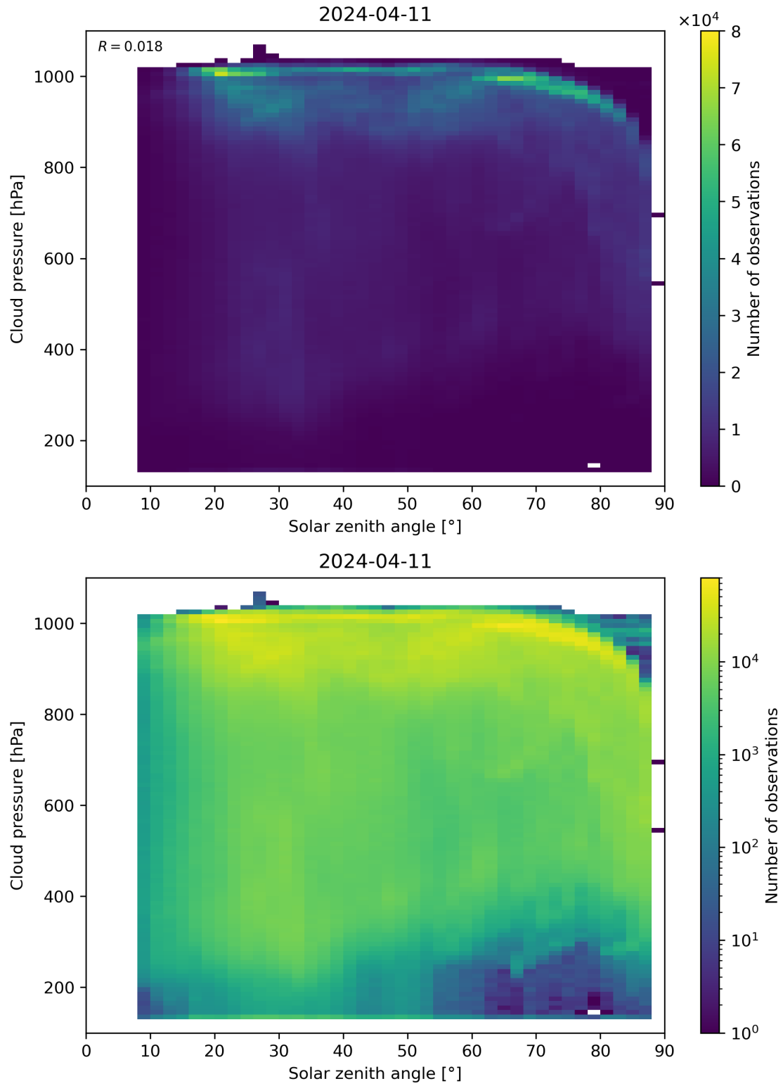
Figure 111: Scatter density plot of “Solar zenith angle” against “Cloud pressure” for 2024-04-10 to 2024-04-12.
