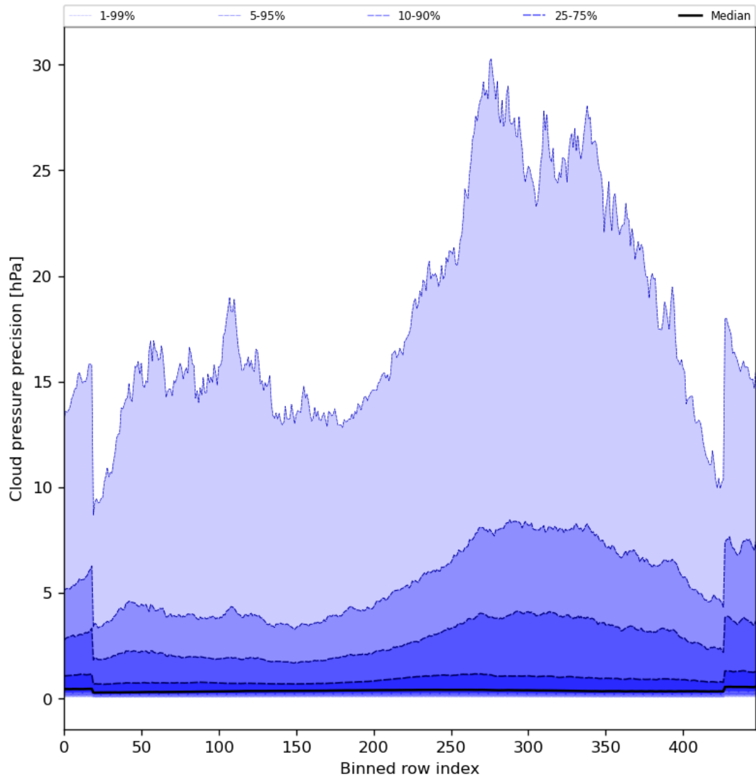
Figure 48: Along track statistics of “Cloud pressure precision” for 2024-04-10 to 2024-04-12
