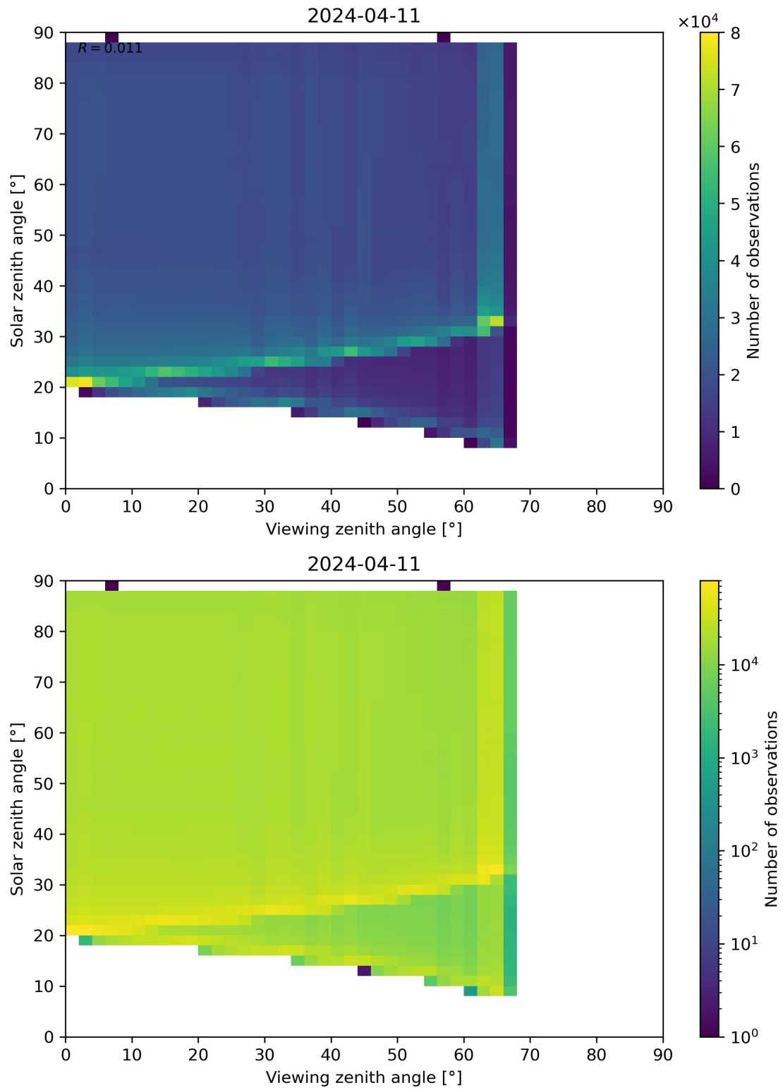
Figure 127: Scatter density plot of “Viewing zenith angle” against “Solar zenith angle” for 2024-04-10 to 2024-04-12.
