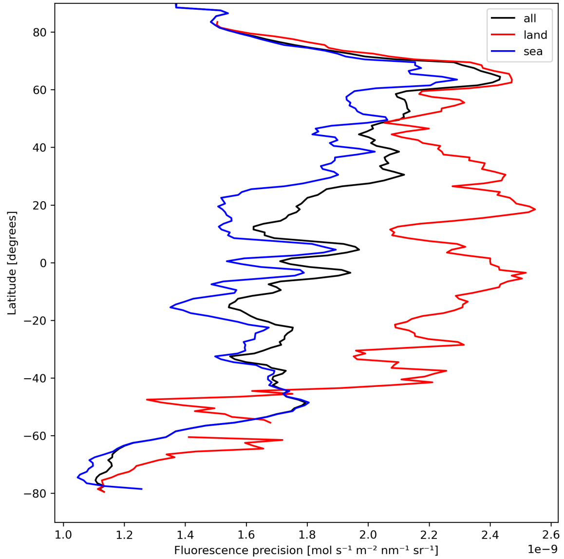
Figure 24: Zonal average of “Fluorescence precision” for 2024-04-10 to 2024-04-12.
