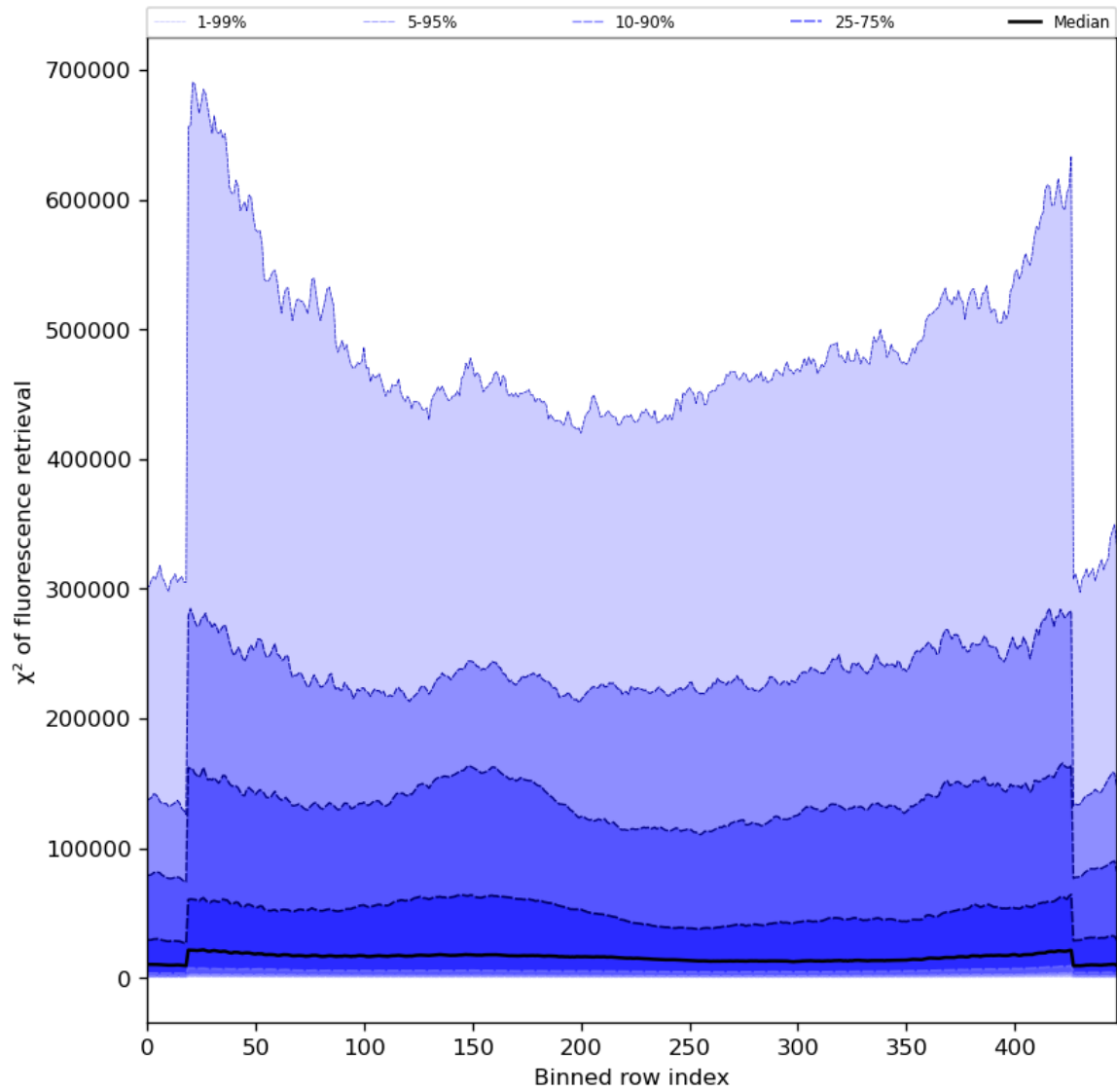
Figure 59: Along track statistics of “ \chi^2 of fluorescence retrieval” for 2024-04-10 to 2024-04-12
