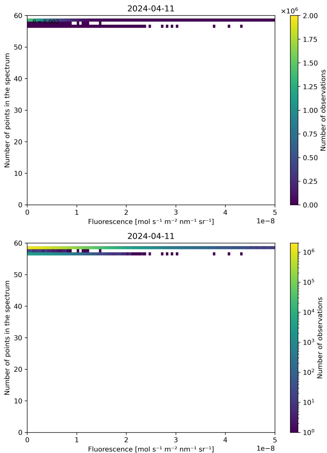
Figure 86: Scatter density plot of “Fluorescence” against “Number of points in the spectrum” for 2024-04-10 to 2024-04-12.
