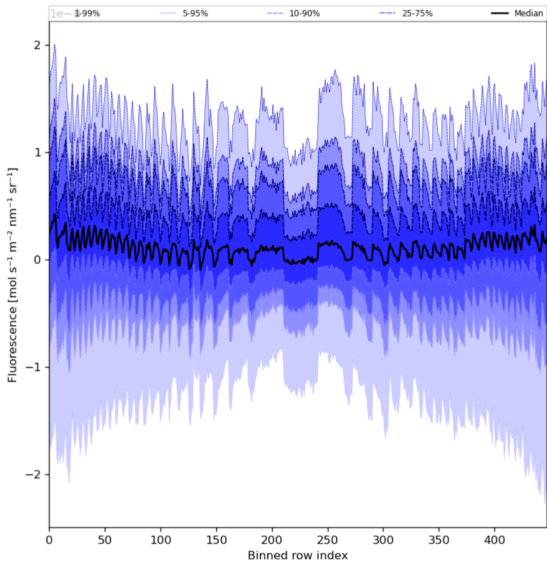
Figure 57: Along track statistics of “Fluorescence” for 2024-04-10 to 2024-04-12
