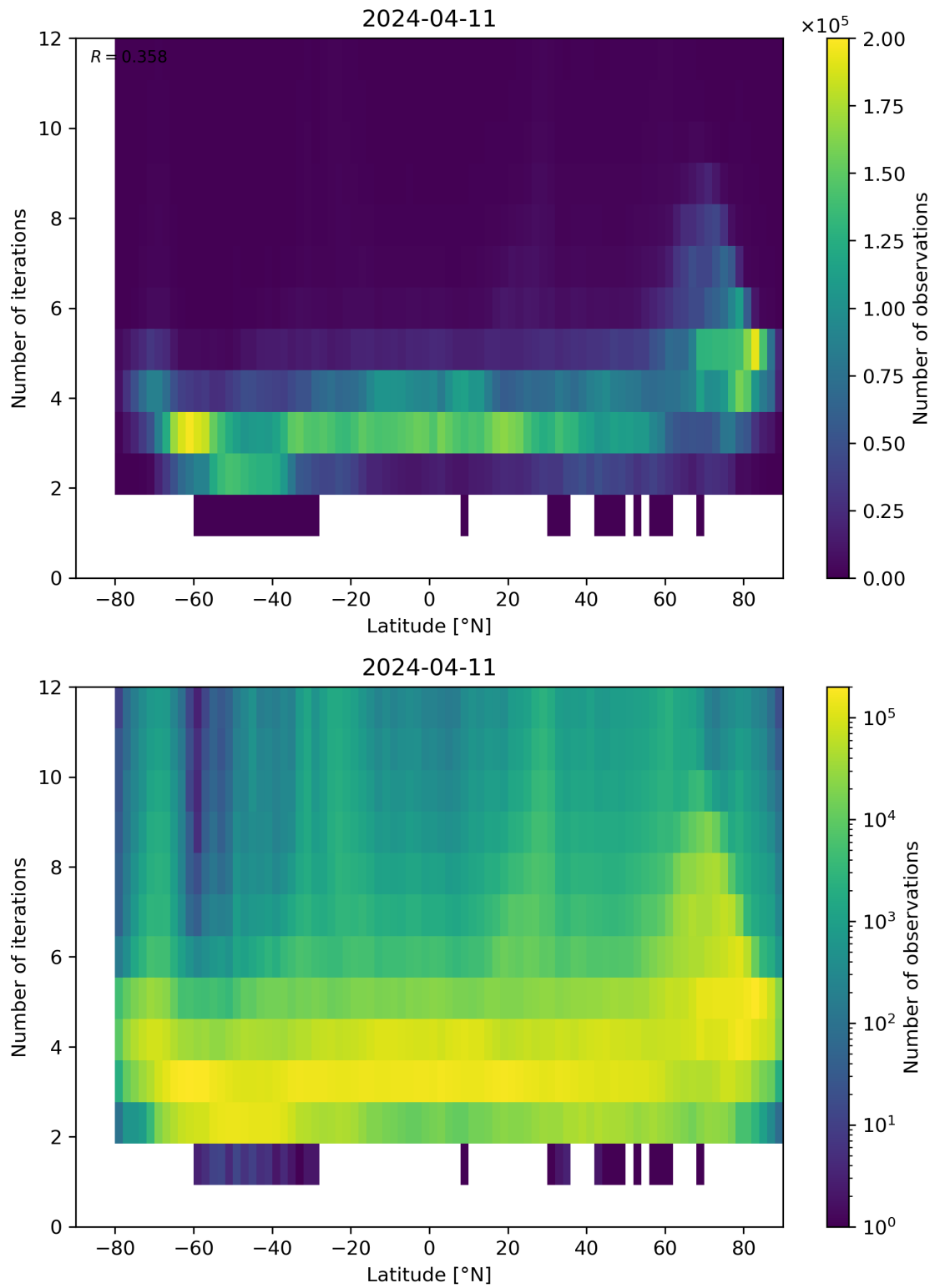
Figure 93: Scatter density plot of “Latitude” against “Number of iterations” for 2024-04-10 to 2024-04-12.
