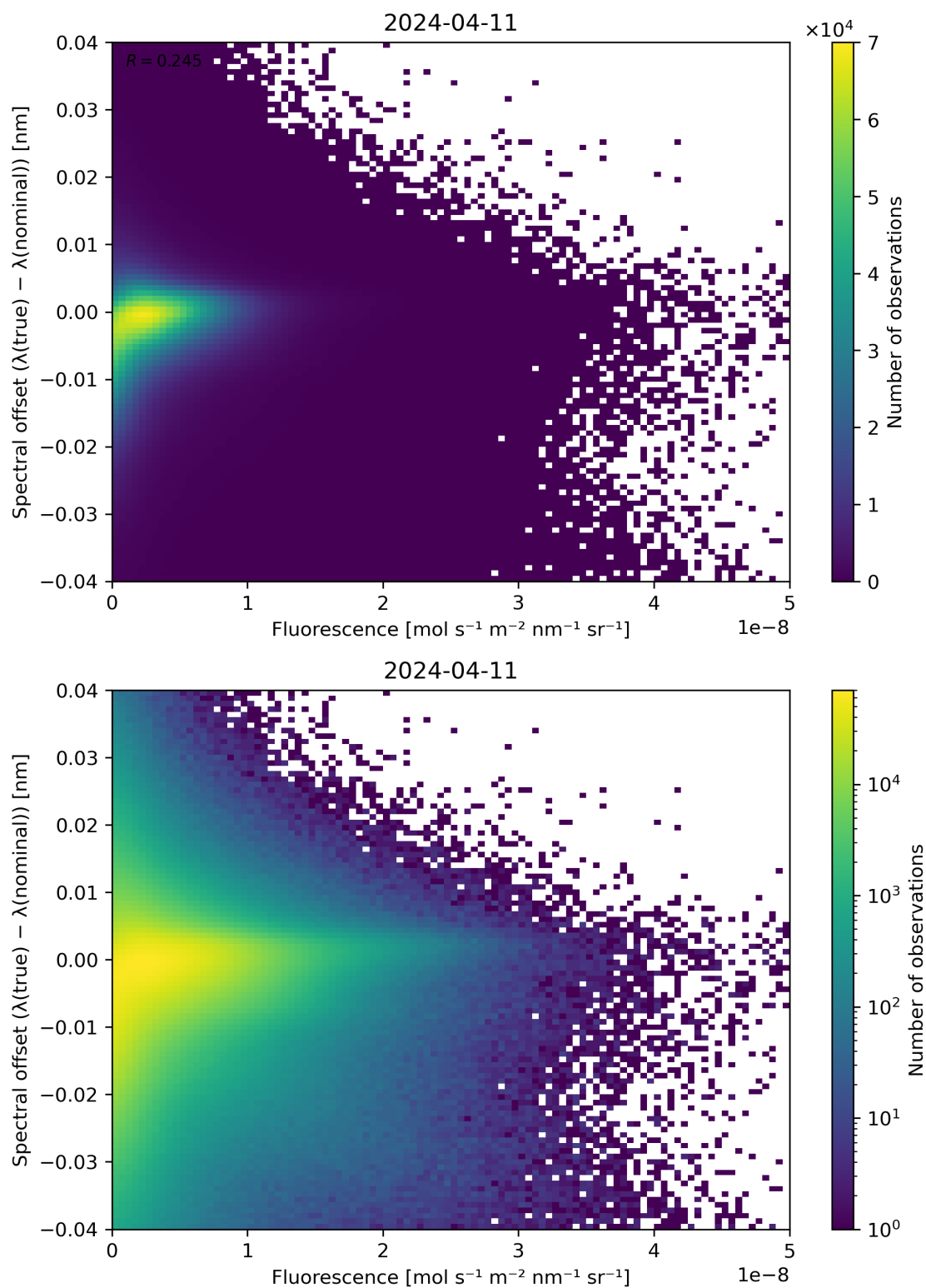
Figure 87: Scatter density plot of “Fluorescence” against “Spectral offset ( \lambda(\text{true}) - \lambda(\text{nominal}) )” for 2024-04-10 to 2024-04-12.
