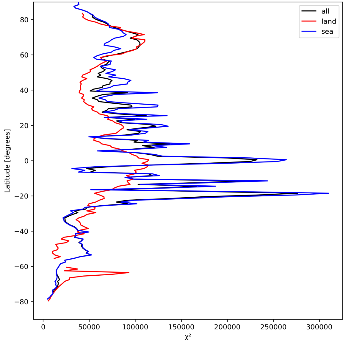
Figure 21: Zonal average of “ \chi^2 ” for 2024-04-10 to 2024-04-12.
