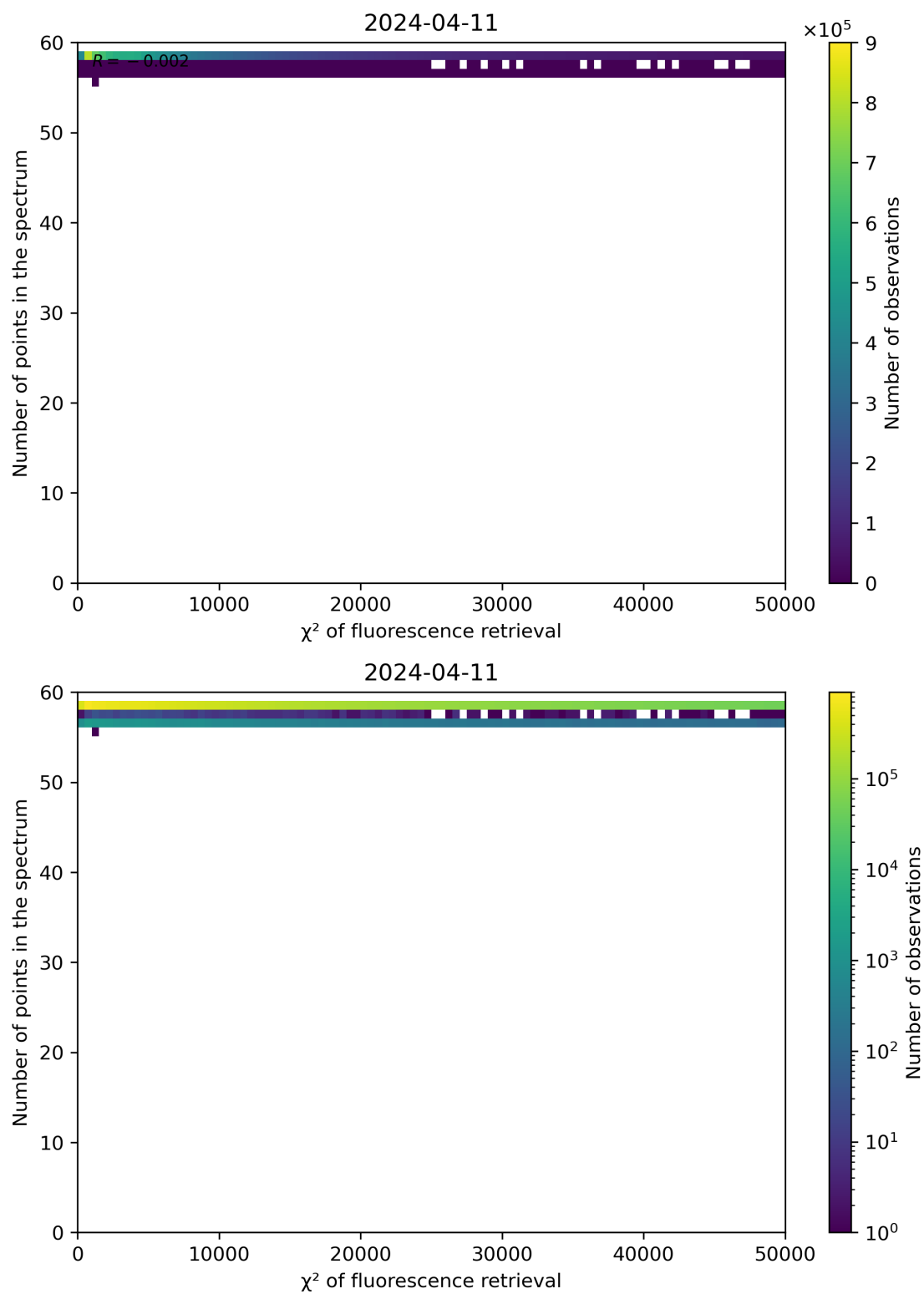
Figure 68: Scatter density plot of " \chi^2 of fluorescence retrieval" against "Number of points in the spectrum" for 2024-04-10 to 2024-04-12.
