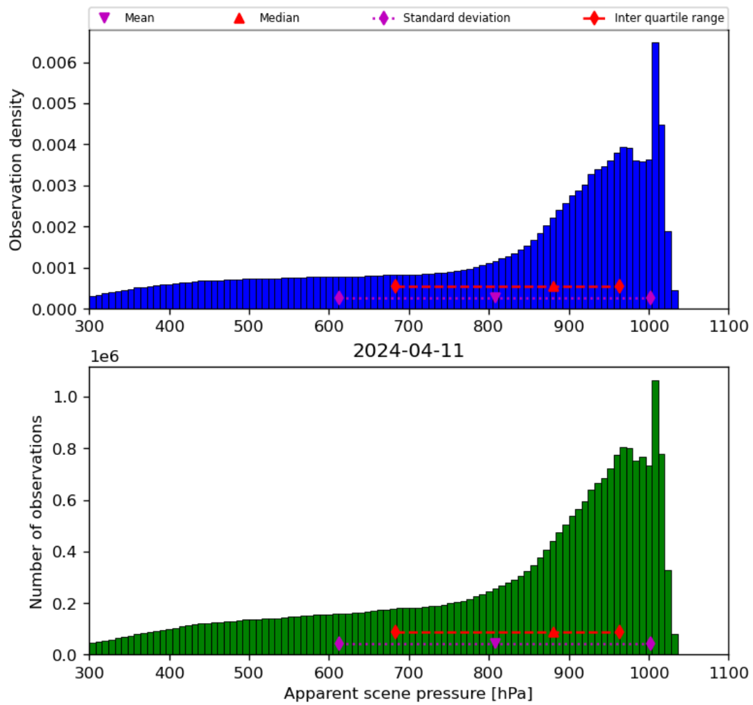
Figure 36: Histogram of “Apparent scene pressure” for 2024-04-10 to 2024-04-12
