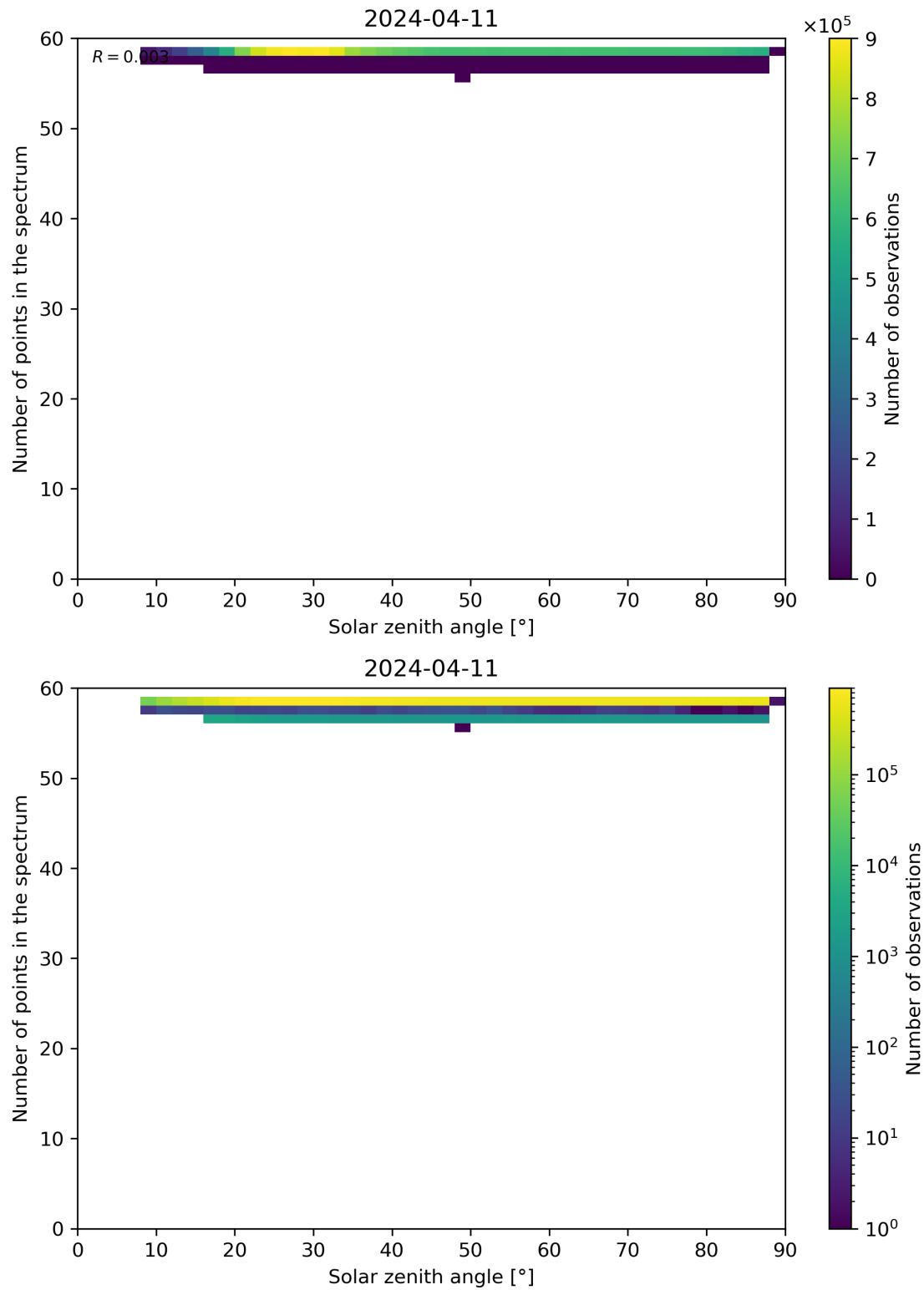
Figure 115: Scatter density plot of “Solar zenith angle” against “Number of points in the spectrum” for 2024-04-10 to 2024-04-12.
