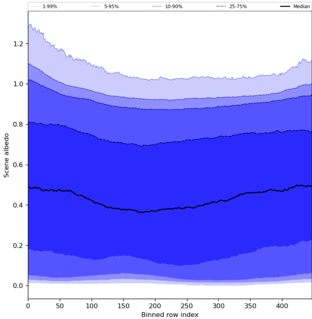
Figure 51: Along track statistics of “Scene albedo” for 2024-04-10 to 2024-04-12
