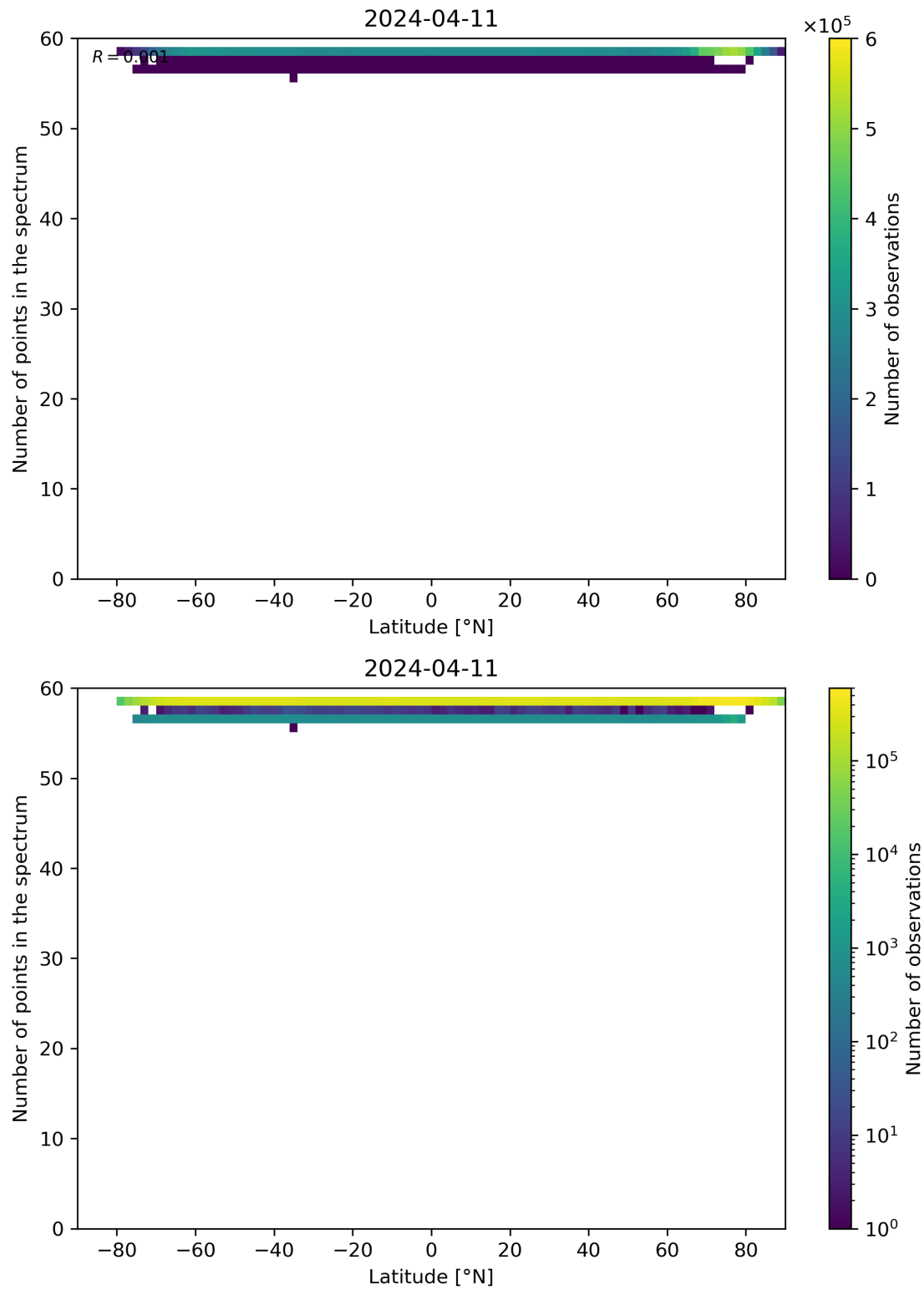
Figure 94: Scatter density plot of “Latitude” against “Number of points in the spectrum” for 2024-04-10 to 2024-04-12.
