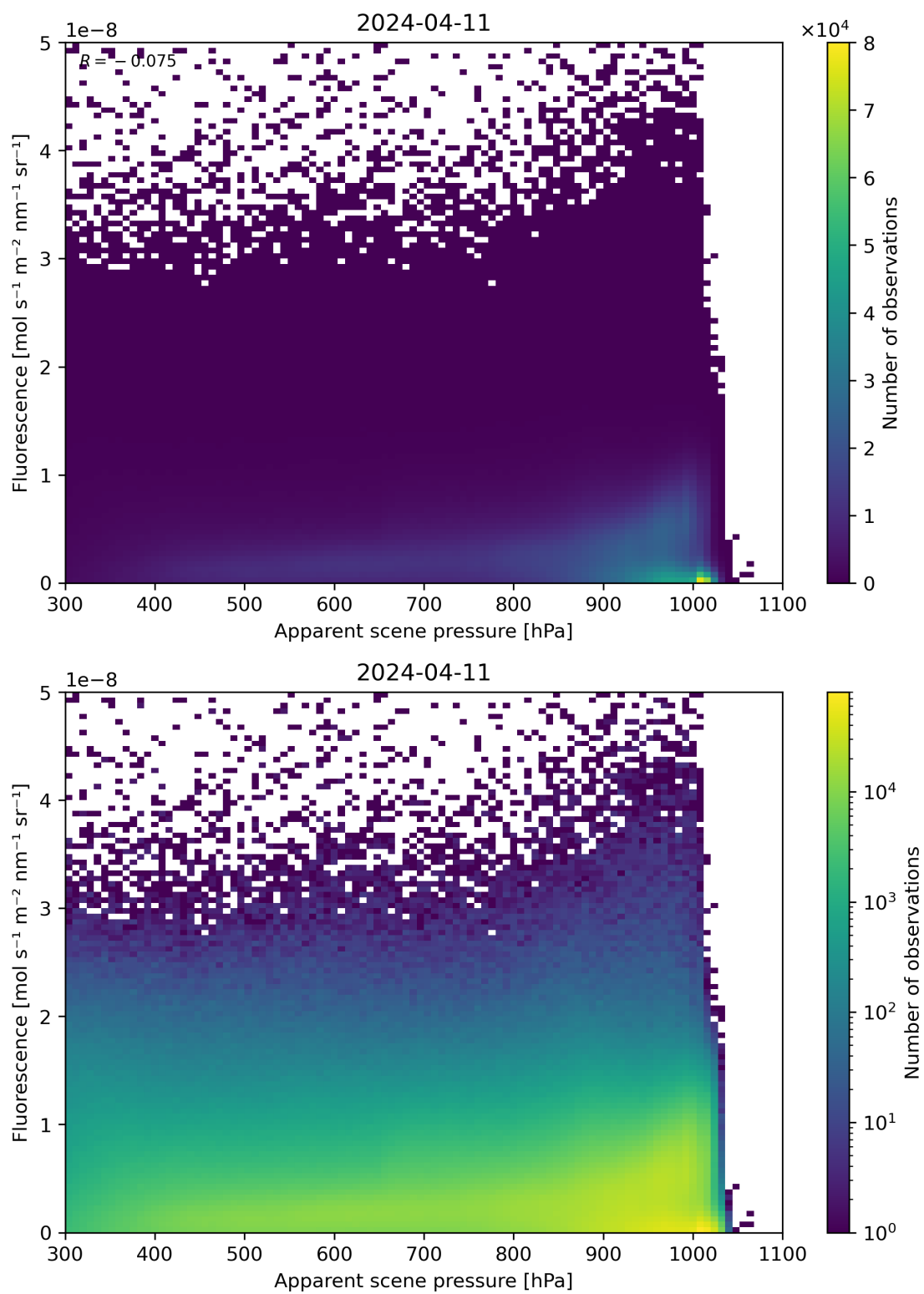
Figure 64: Scatter density plot of “Apparent scene pressure” against “Fluorescence” for 2024-04-10 to 2024-04-12.
