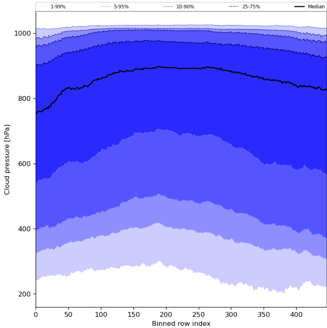
Figure 47: Along track statistics of “Cloud pressure” for 2024-04-10 to 2024-04-12
