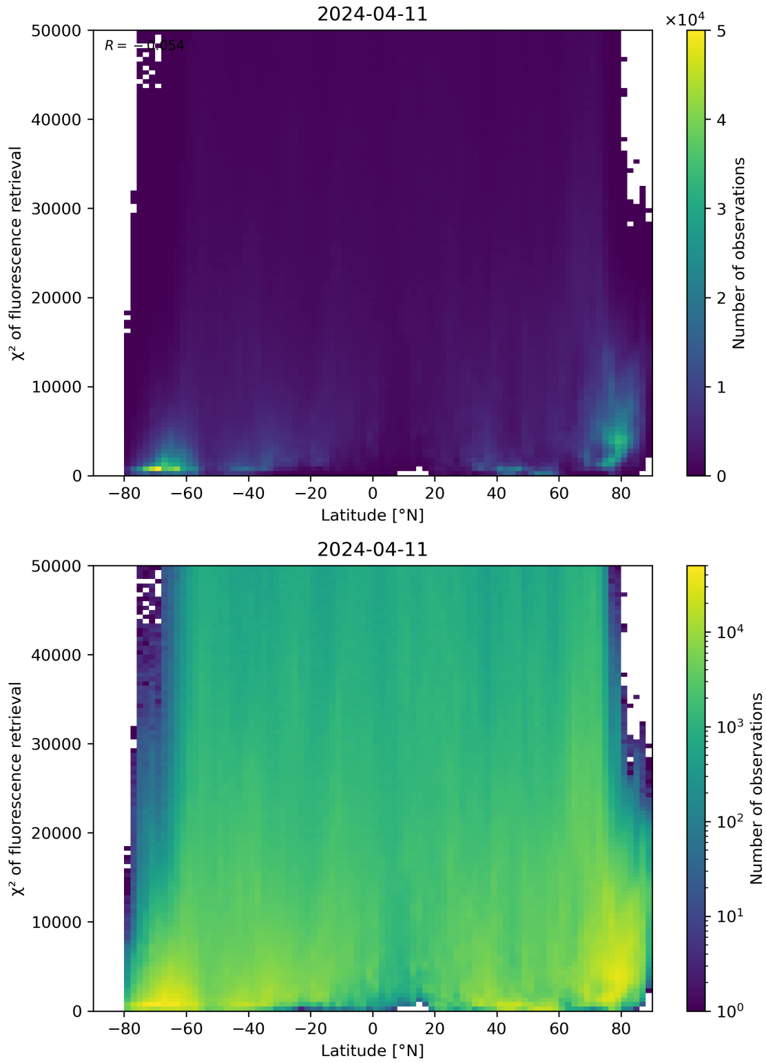
Figure 89: Scatter density plot of “Latitude” against “ \chi^2 of fluorescence retrieval” for 2024-04-10 to 2024-04-12.
