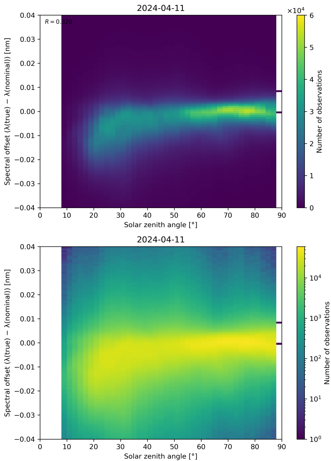
Figure 117: Scatter density plot of “Solar zenith angle” against “Spectral offset ( \lambda(\text{true}) - \lambda(\text{nominal}) )” for 2024-04-10 to 2024-04-12.
