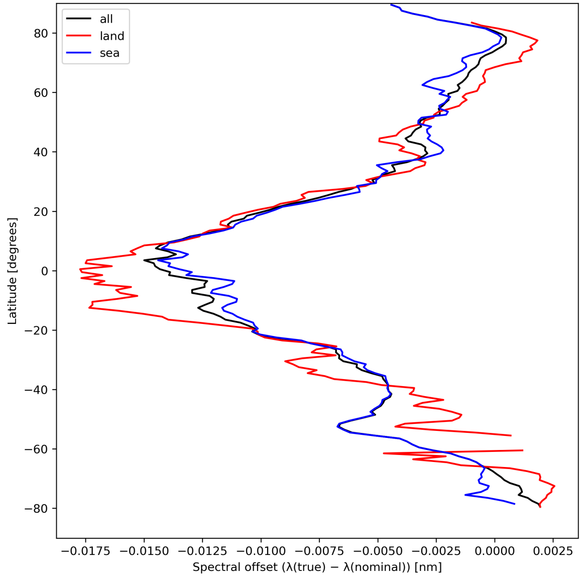
Figure 28: Zonal average of “Spectral offset ( \lambda(\text{true}) - \lambda(\text{nominal}) )” for 2024-04-10 to 2024-04-12.
