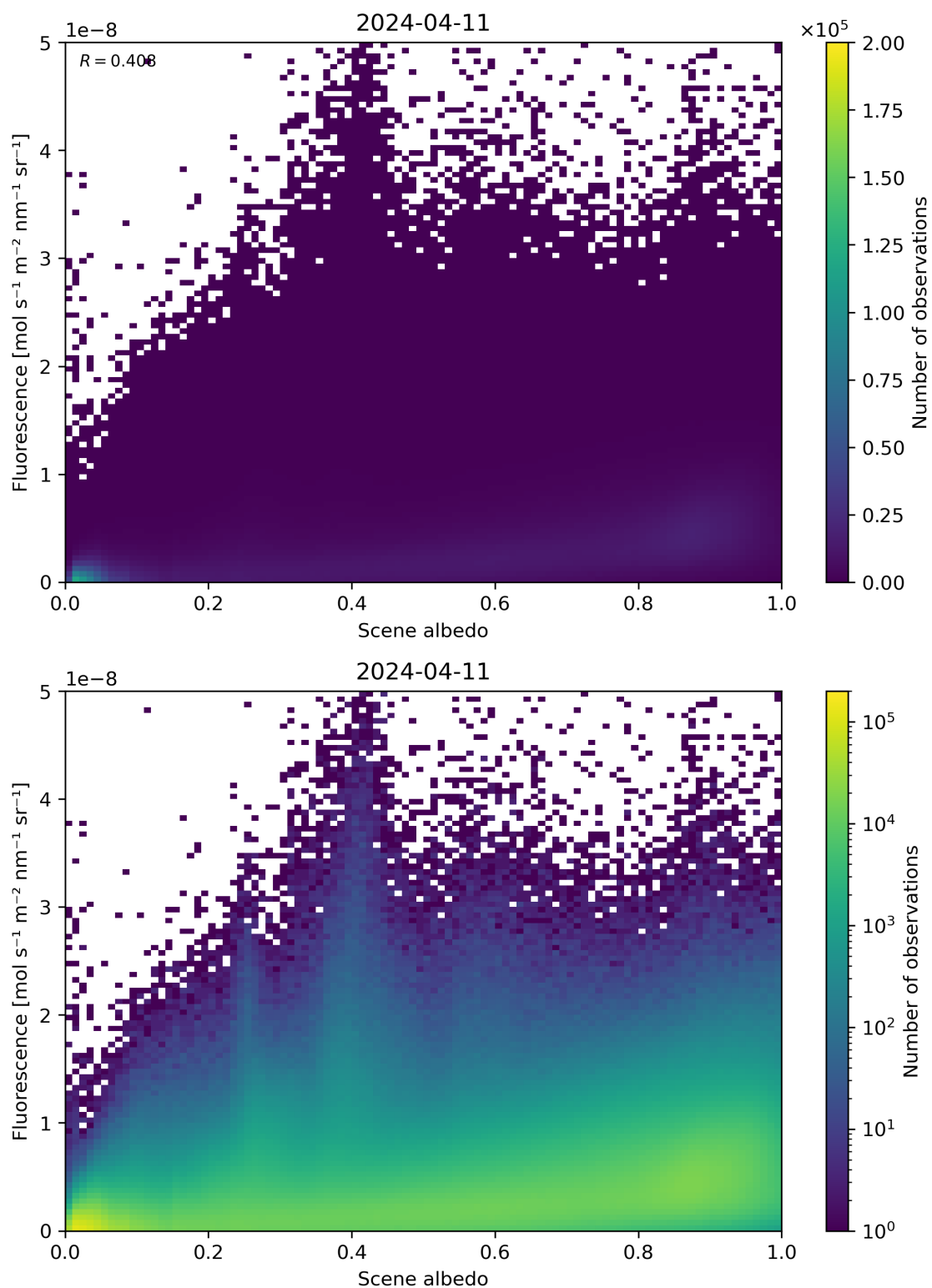
Figure 104: Scatter density plot of “Scene albedo” against “Fluorescence” for 2024-04-10 to 2024-04-12.
