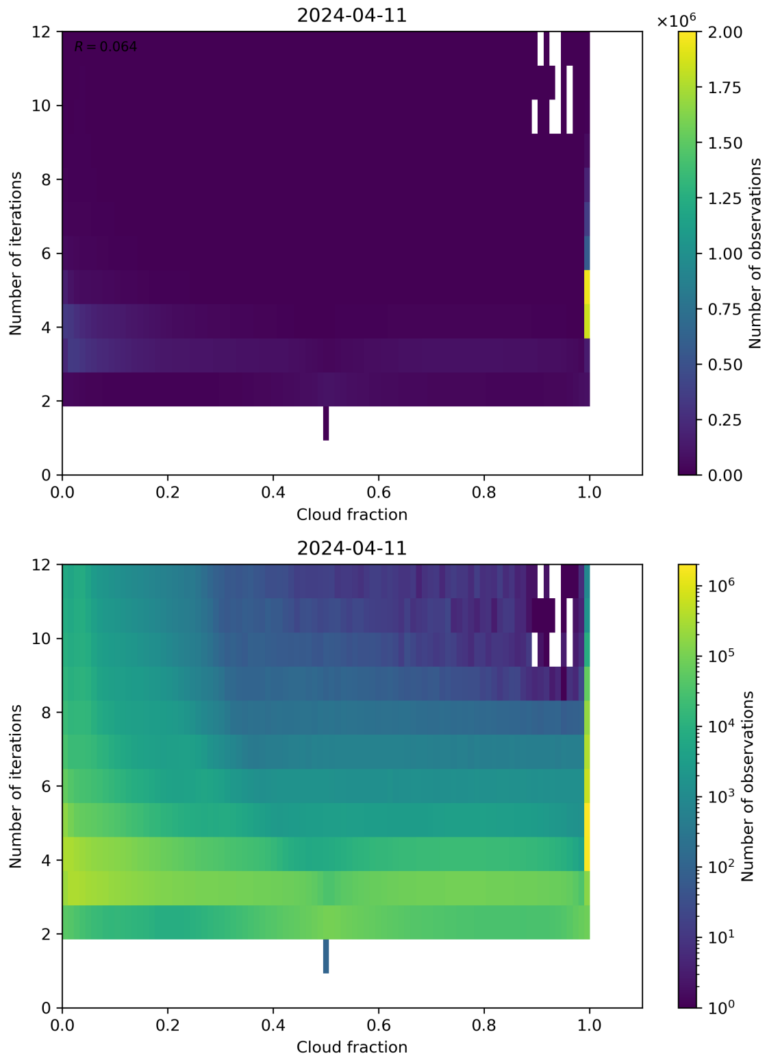
Figure 73: Scatter density plot of “Cloud fraction” against “Number of iterations” for 2024-04-10 to 2024-04-12.
