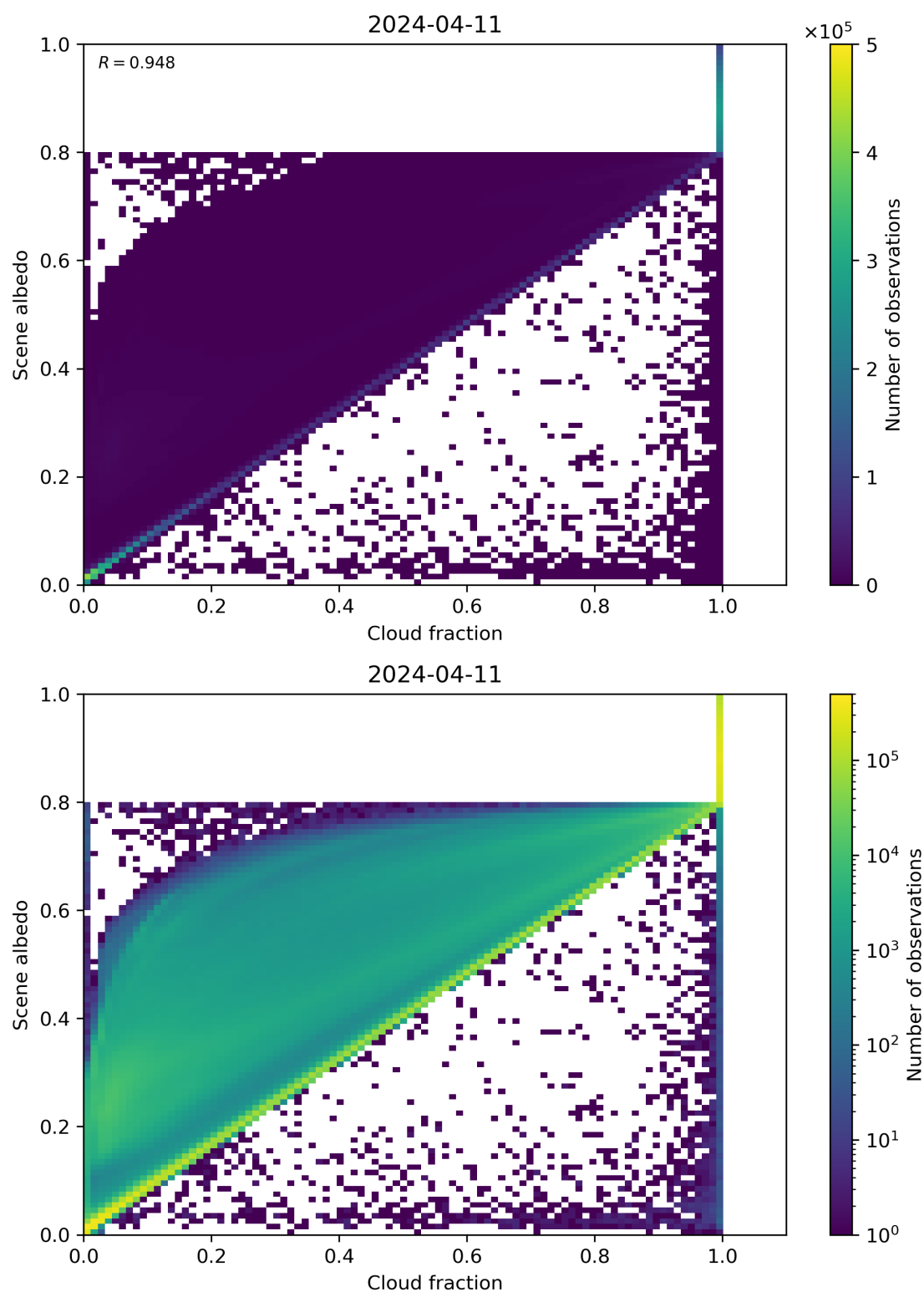
Figure 75: Scatter density plot of “Cloud fraction” against “Scene albedo” for 2024-04-10 to 2024-04-12.
