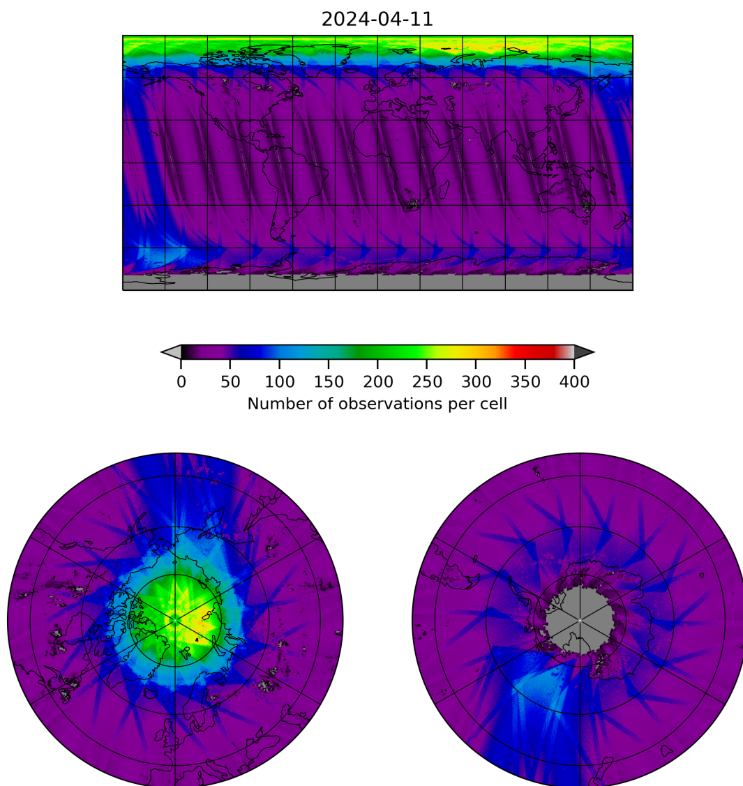
Figure 11: Map of the number of observations for 2024-04-10 to 2024-04-12
