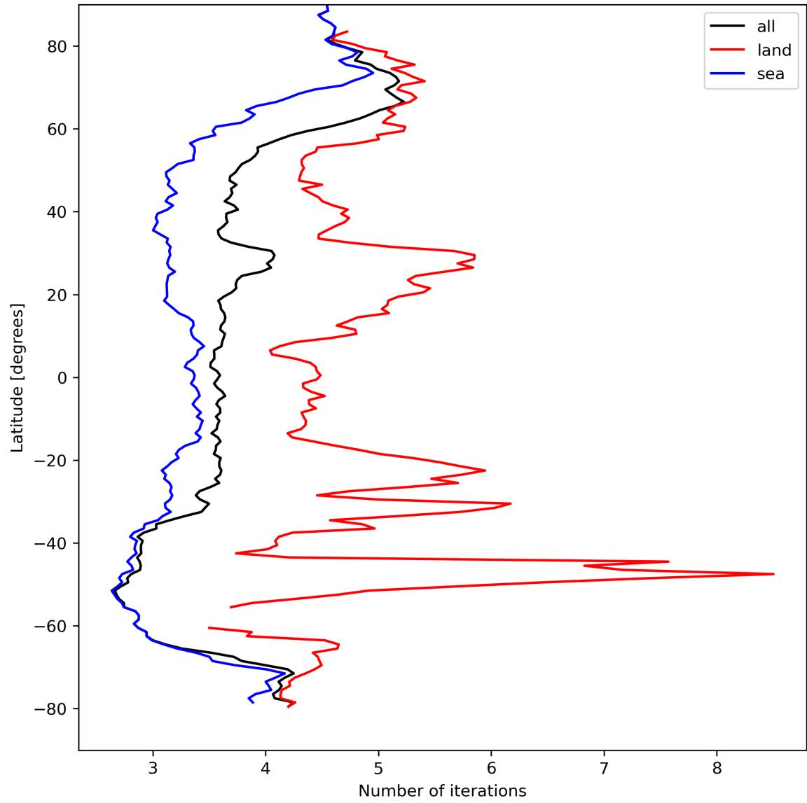
Figure 22: Zonal average of “Number of iterations” for 2024-04-10 to 2024-04-12.
