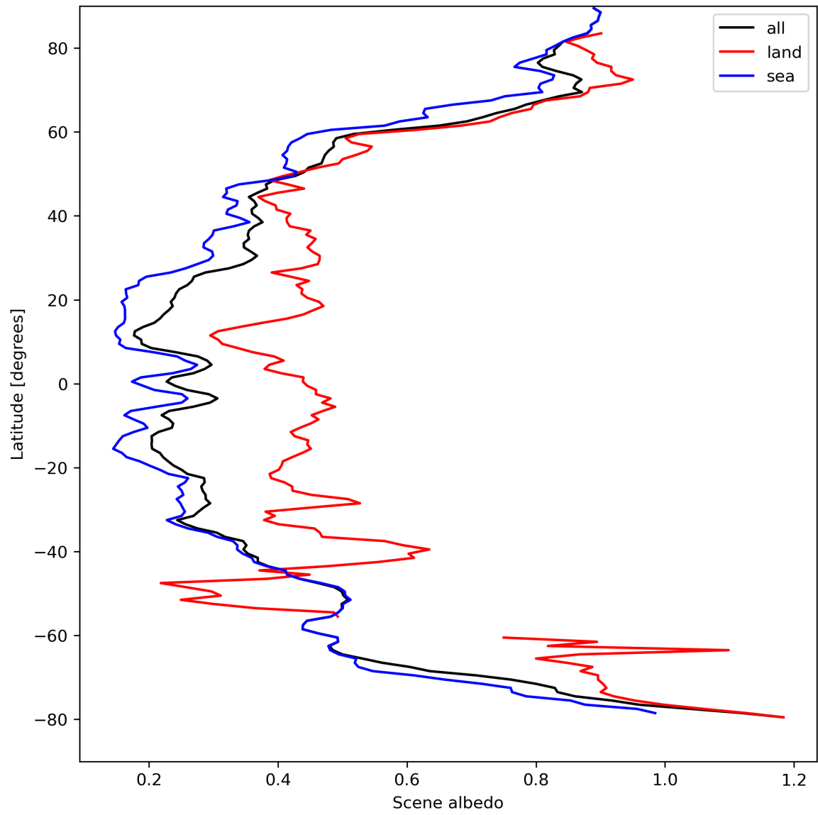
Figure 17: Zonal average of “Scene albedo” for 2024-04-10 to 2024-04-12.
