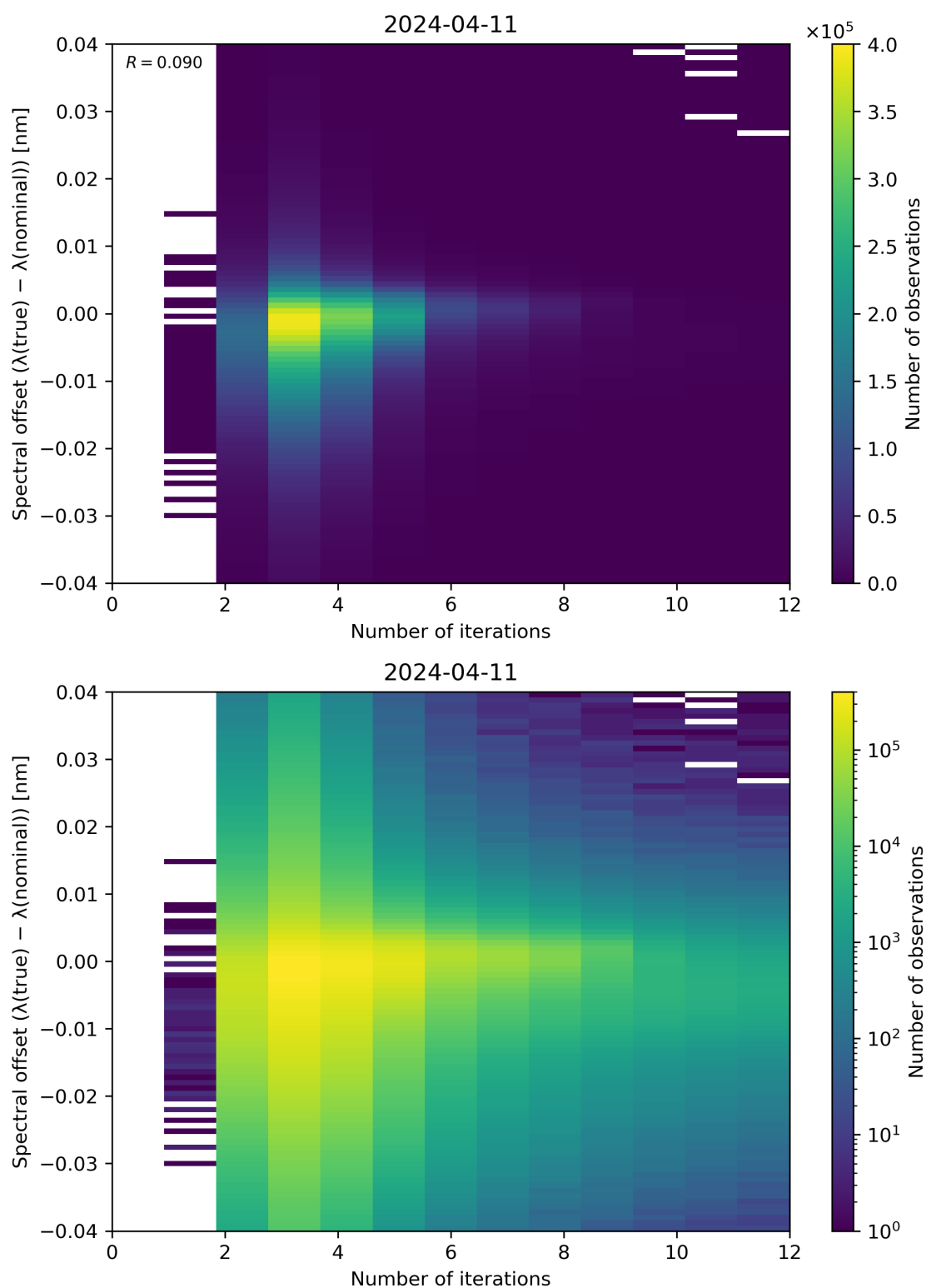
Figure 100: Scatter density plot of “Number of iterations” against “Spectral offset ( \lambda(\text{true}) - \lambda(\text{nominal}) )” for 2024-04-10 to 2024-04-12.
