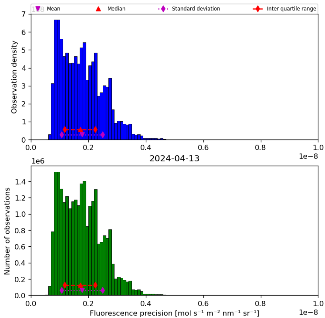
Figure 41: Histogram of “Fluorescence precision” for 2024-04-12 to 2024-04-14
