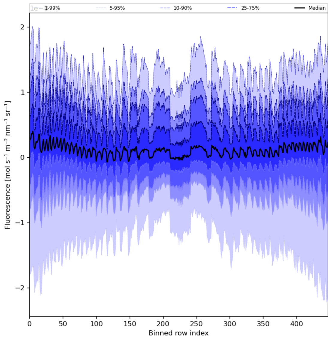
Figure 57: Along track statistics of “Fluorescence” for 2024-04-12 to 2024-04-14
