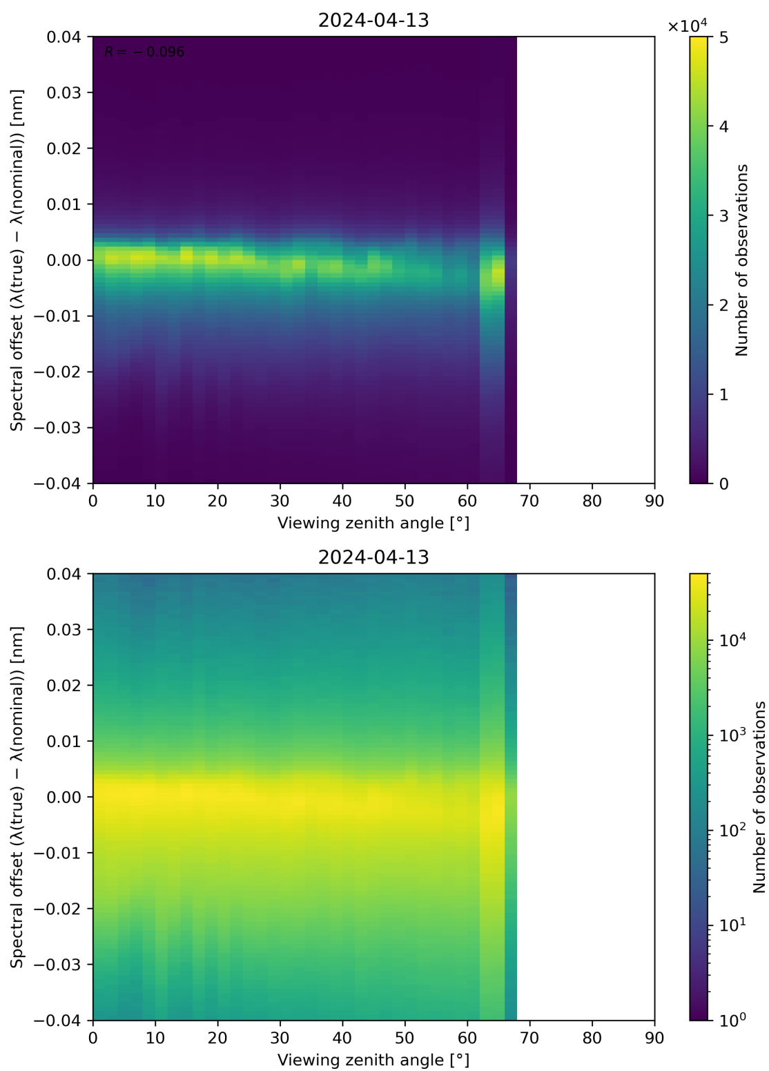
Figure 128: Scatter density plot of “Viewing zenith angle” against “Spectral offset ( \lambda(\text{true}) - \lambda(\text{nominal}) )” for 2024-04-12 to 2024-04-14.
