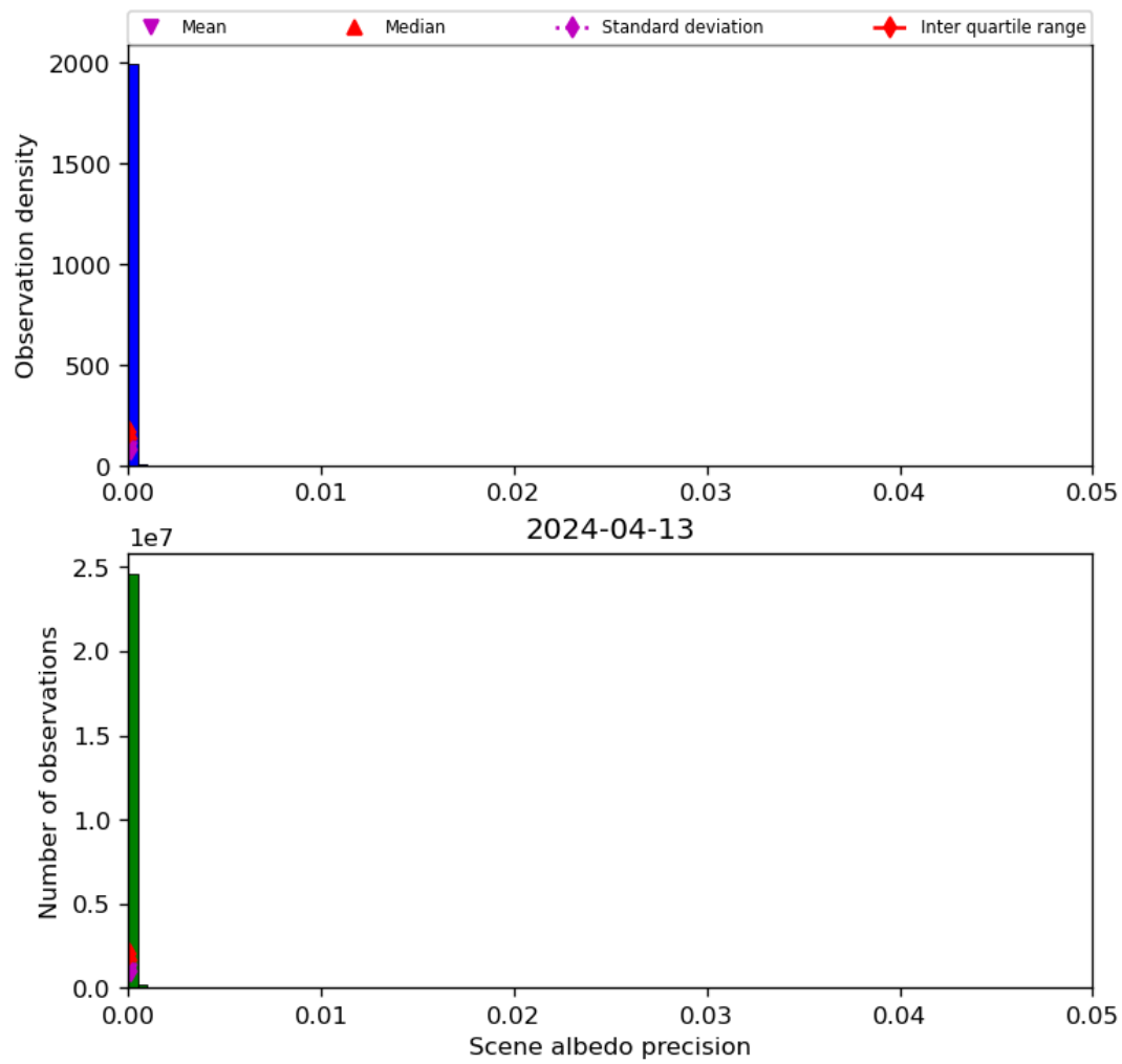
Figure 35: Histogram of “Scene albedo precision” for 2024-04-12 to 2024-04-14
