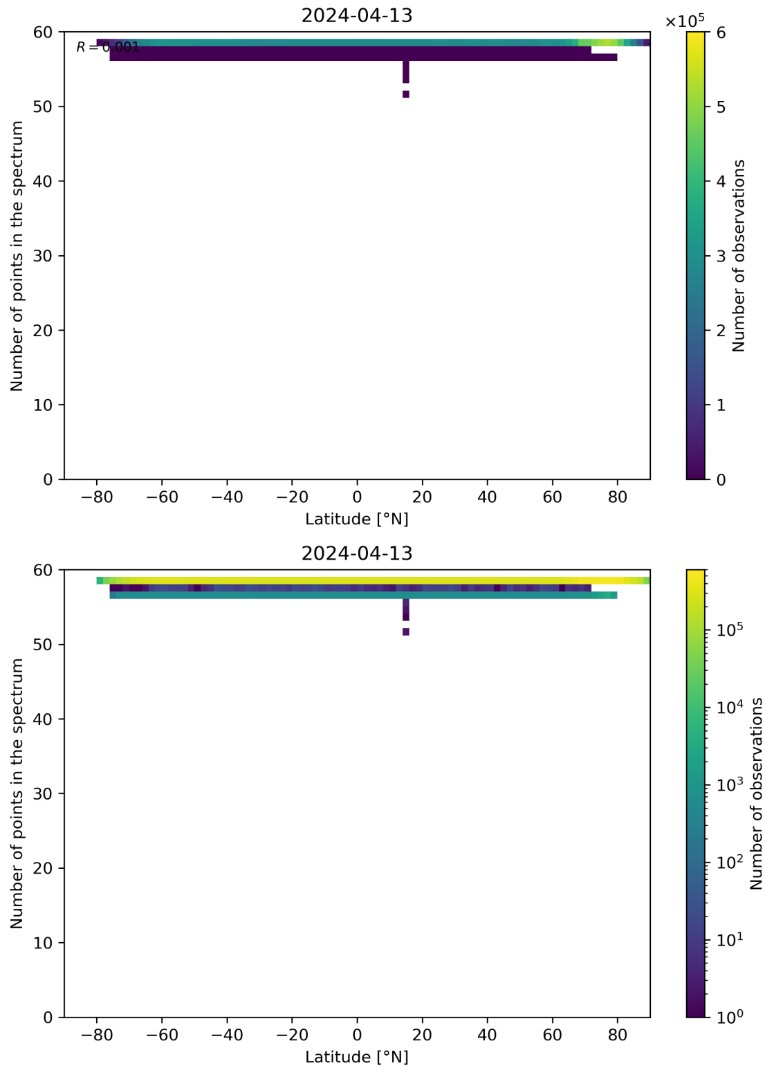
Figure 94: Scatter density plot of “Latitude” against “Number of points in the spectrum” for 2024-04-12 to 2024-04-14.
