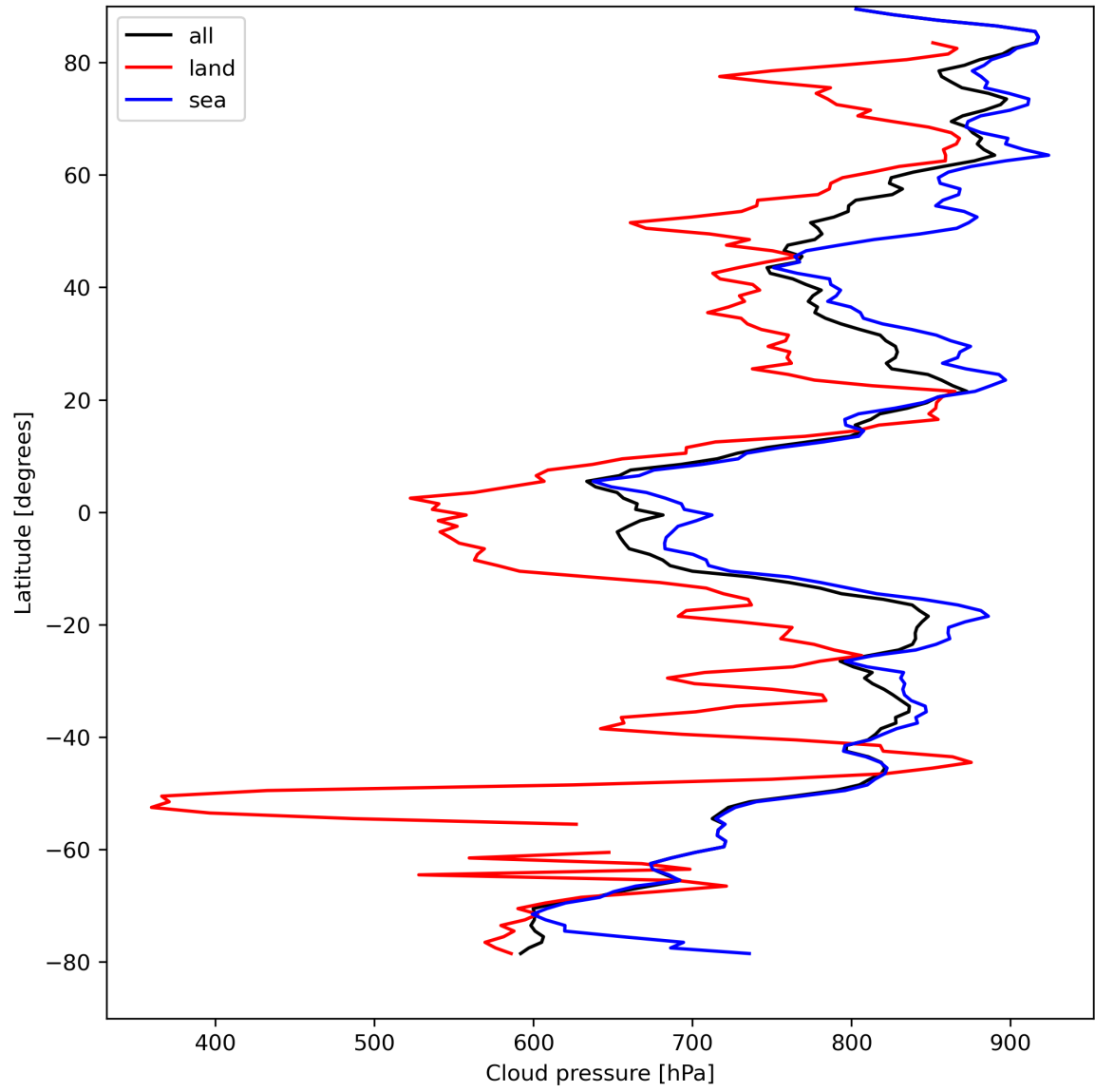
Figure 13: Zonal average of “Cloud pressure” for 2024-04-12 to 2024-04-14.
