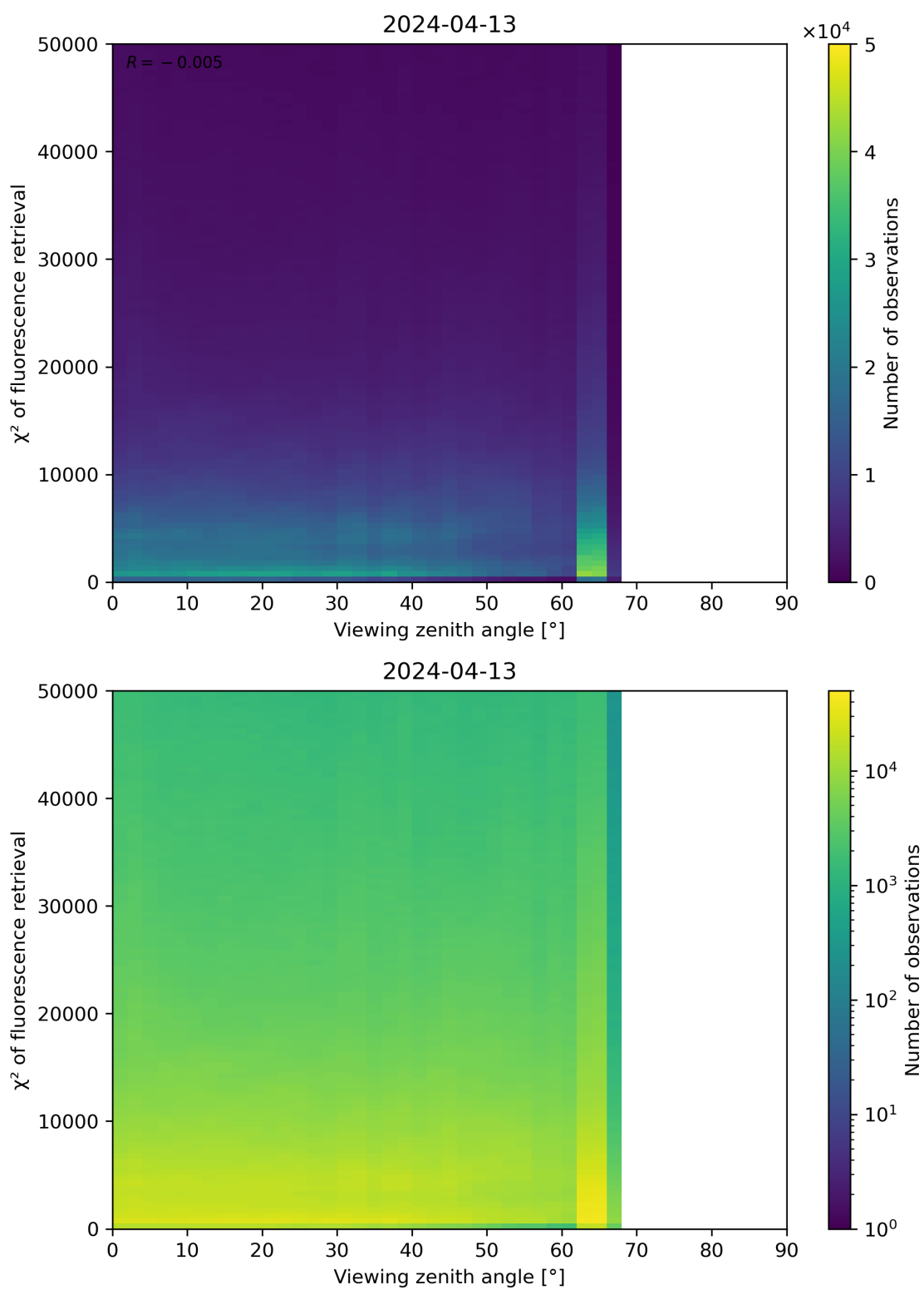
Figure 119: Scatter density plot of “Viewing zenith angle” against “ \chi^2 of fluorescence retrieval” for 2024-04-12 to 2024-04-14.
