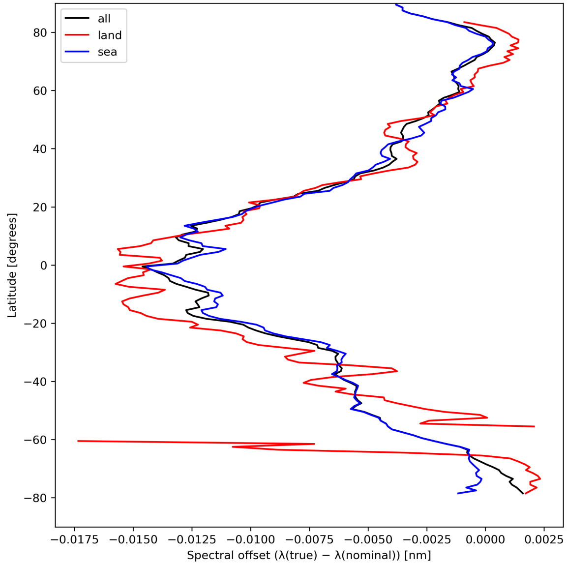
Figure 28: Zonal average of “Spectral offset ( \lambda(\text{true}) - \lambda(\text{nominal}) )” for 2024-04-12 to 2024-04-14.
