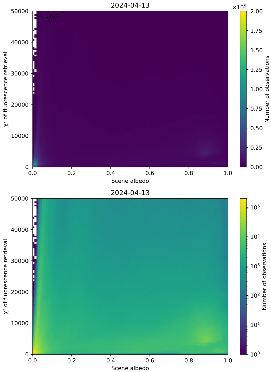
Figure 103: Scatter density plot of “Scene albedo” against “ \chi^2 of fluorescence retrieval” for 2024-04-12 to 2024-04-14.
