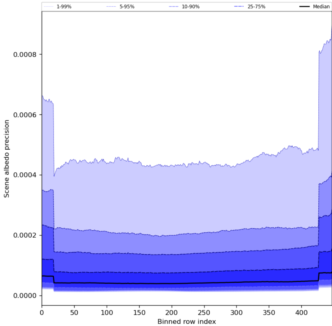
Figure 52: Along track statistics of “Scene albedo precision” for 2024-04-12 to 2024-04-14
