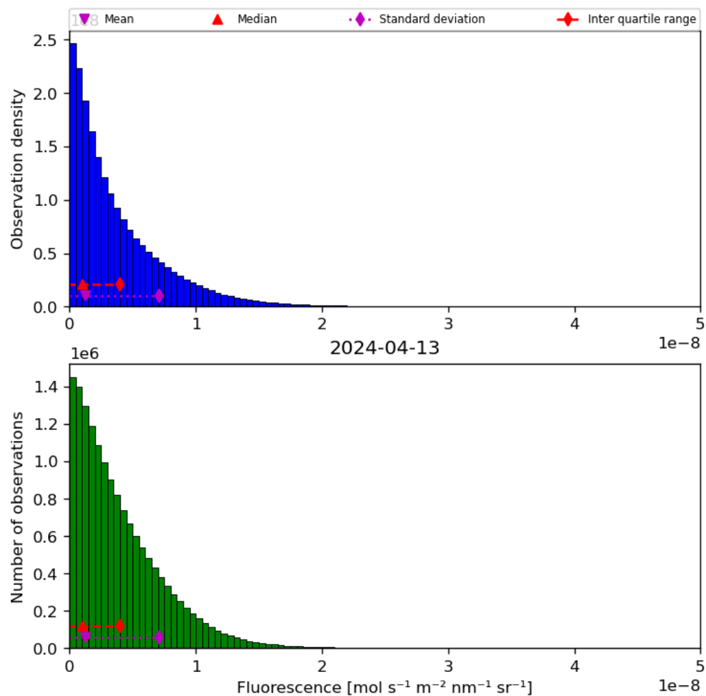
Figure 40: Histogram of “Fluorescence” for 2024-04-12 to 2024-04-14
