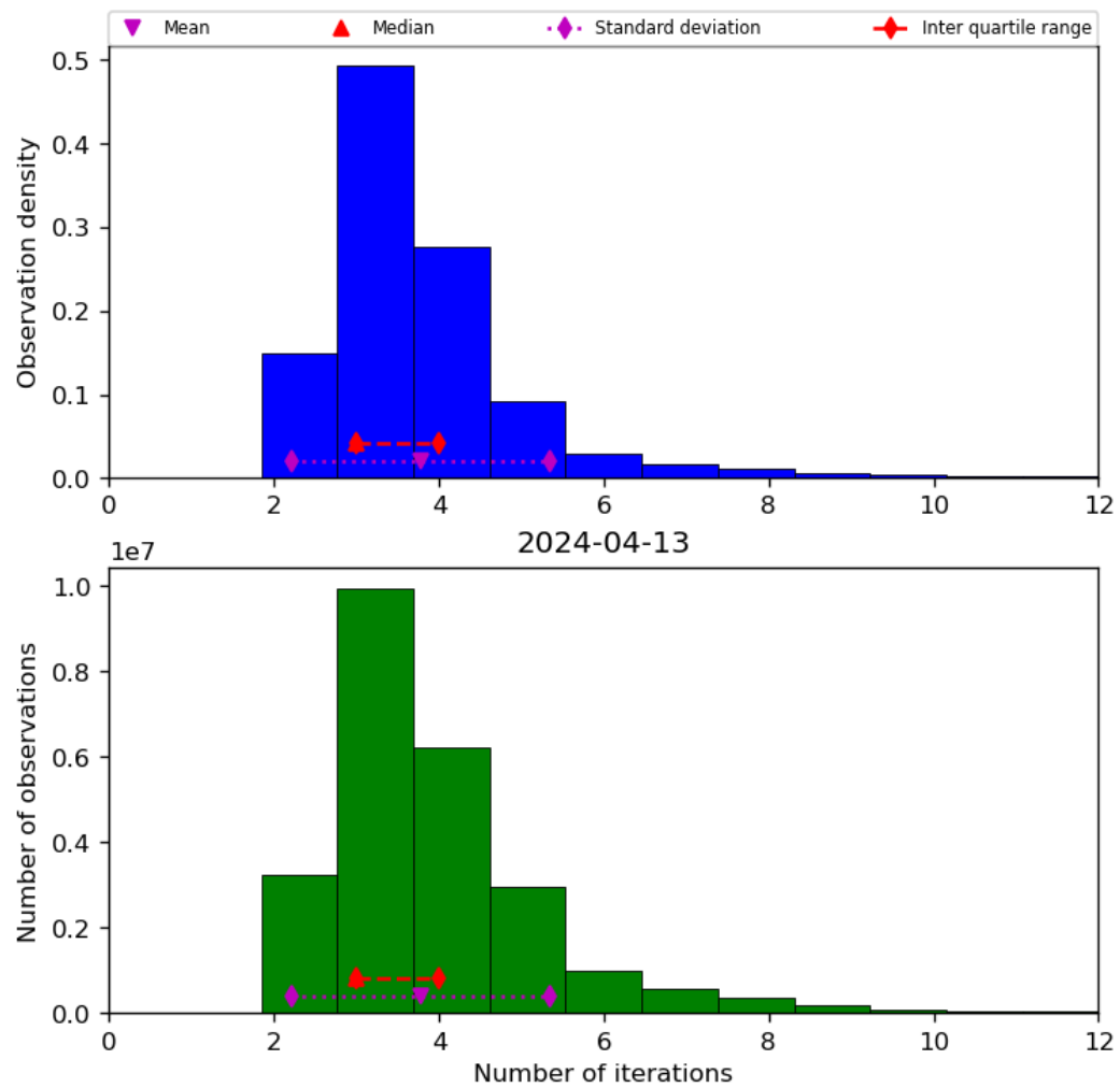
Figure 39: Histogram of “Number of iterations” for 2024-04-12 to 2024-04-14
