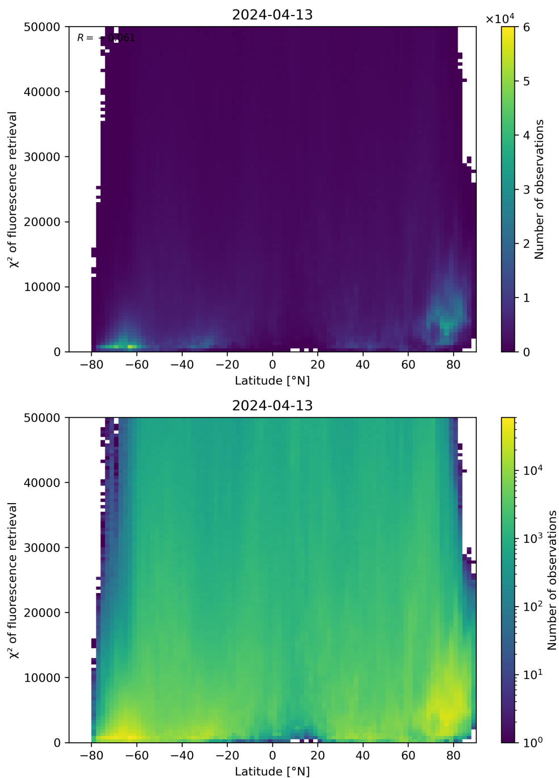
Figure 89: Scatter density plot of “Latitude” against “ \chi^2 of fluorescence retrieval” for 2024-04-12 to 2024-04-14.
