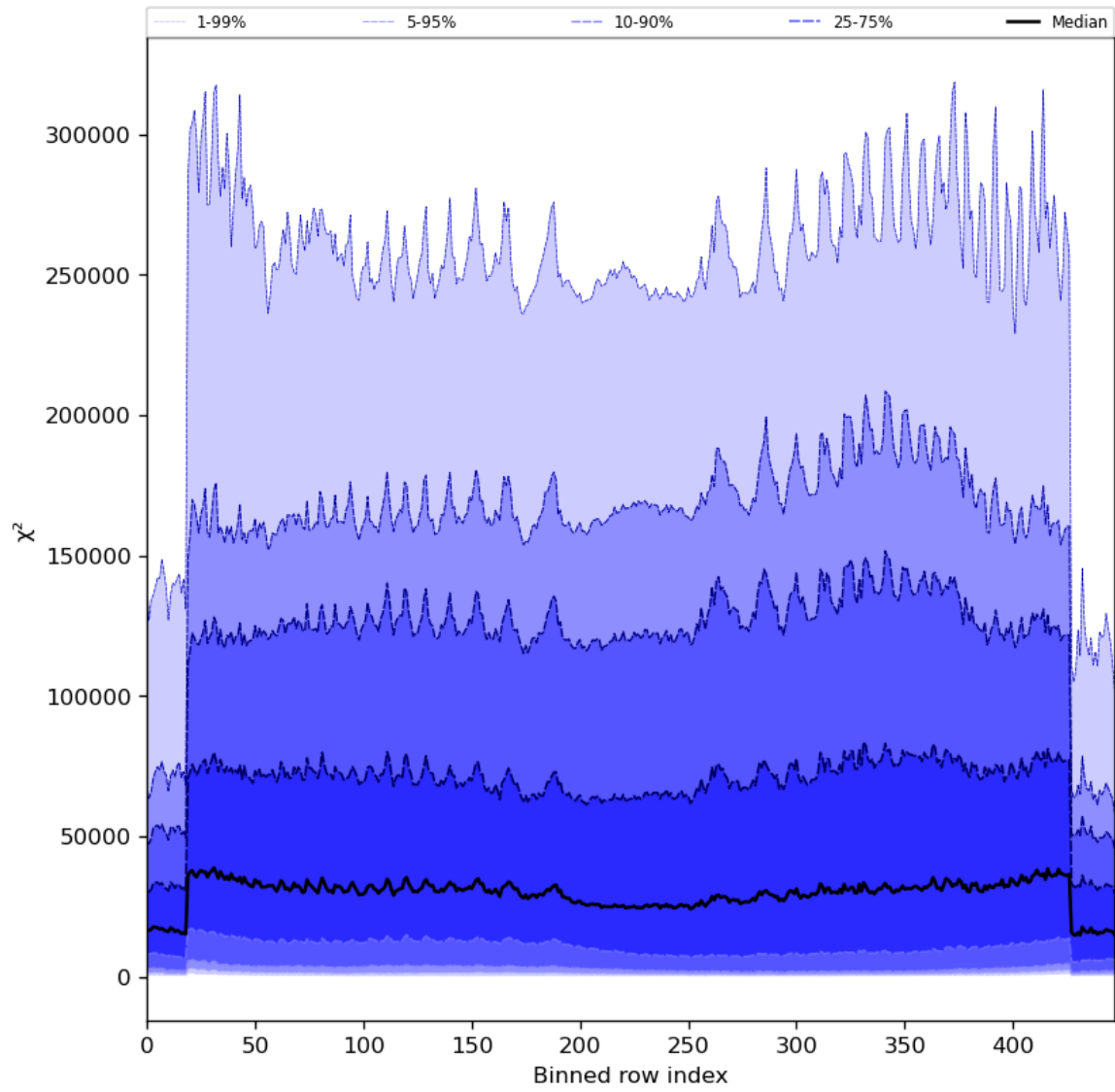
Figure 55: Along track statistics of “ \chi^2 ” for 2024-04-12 to 2024-04-14
