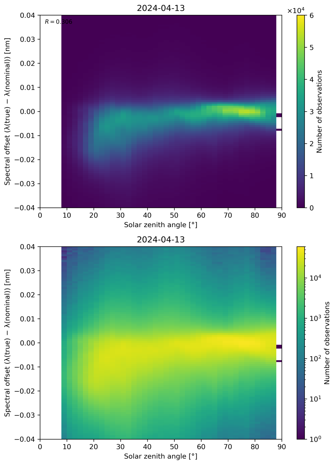
Figure 117: Scatter density plot of “Solar zenith angle” against “Spectral offset ( \lambda(\text{true}) - \lambda(\text{nominal}) )” for 2024-04-12 to 2024-04-14.
