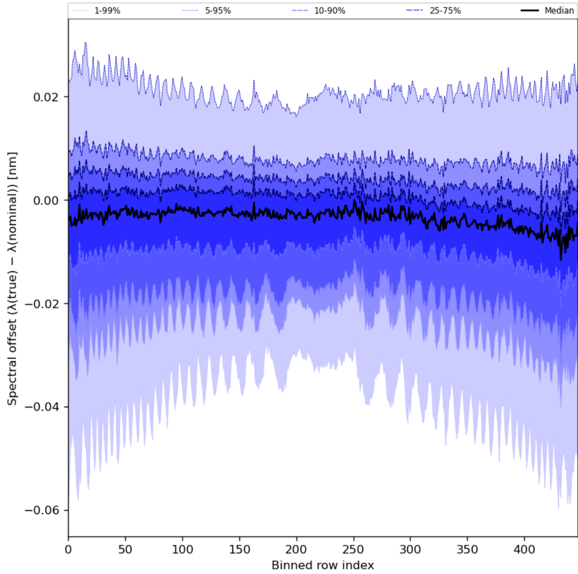
Figure 62: Along track statistics of “Spectral offset ( \lambda(\text{true}) - \lambda(\text{nominal}) )” for 2024-04-12 to 2024-04-14
