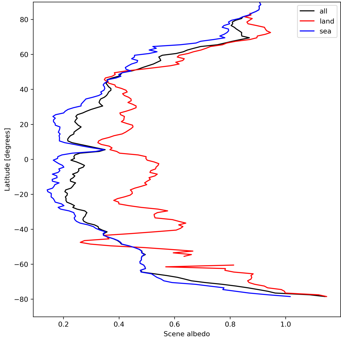
Figure 17: Zonal average of “Scene albedo” for 2024-04-12 to 2024-04-14.
