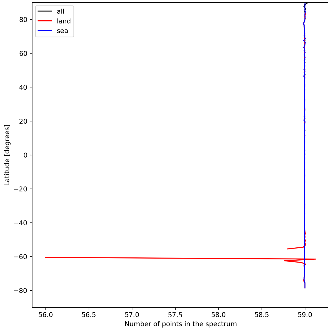
Figure 27: Zonal average of “Number of points in the spectrum” for 2024-04-12 to 2024-04-14.
