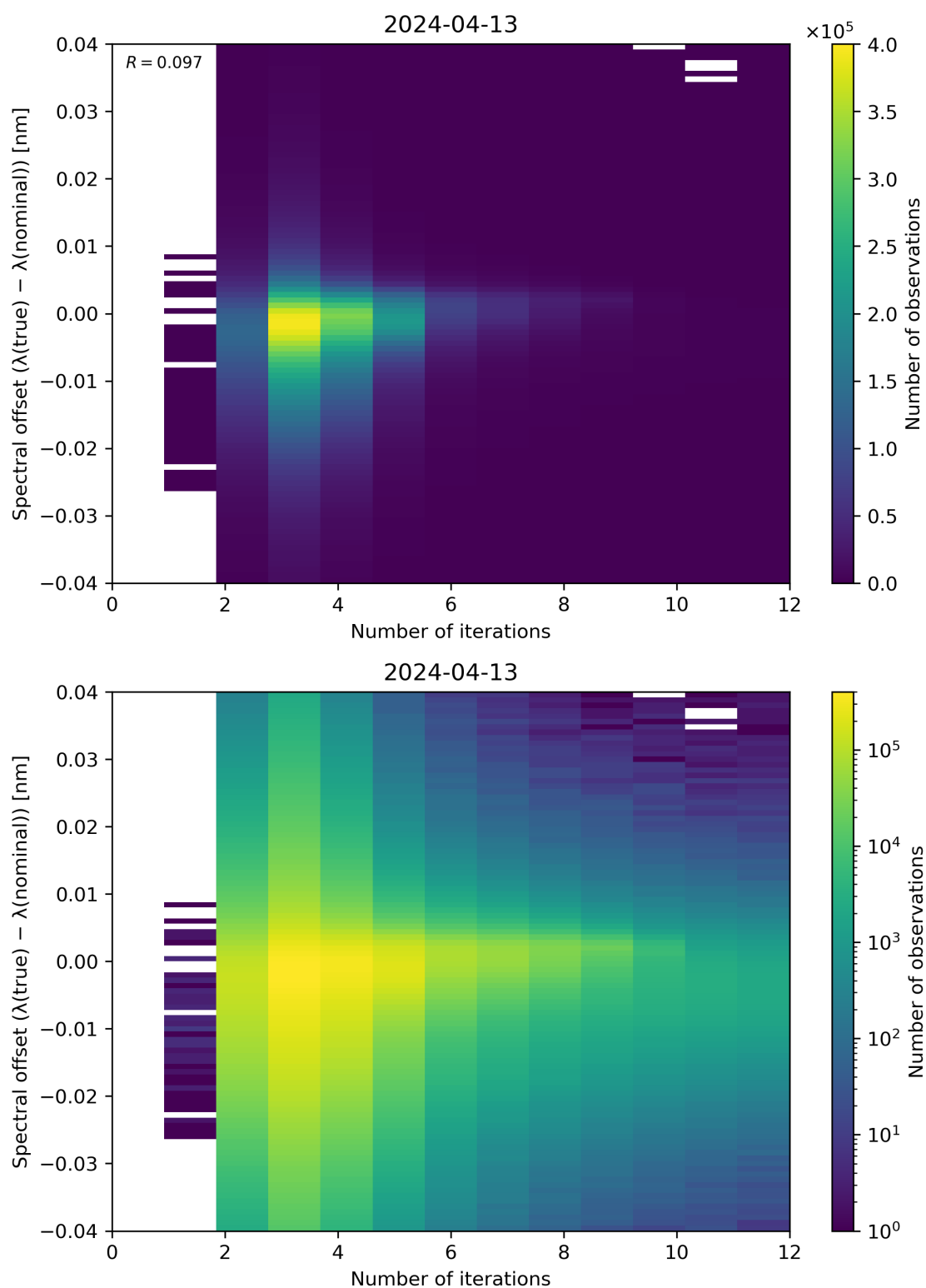
Figure 100: Scatter density plot of “Number of iterations” against “Spectral offset ( \lambda(\text{true}) - \lambda(\text{nominal}) )” for 2024-04-12 to 2024-04-14.
