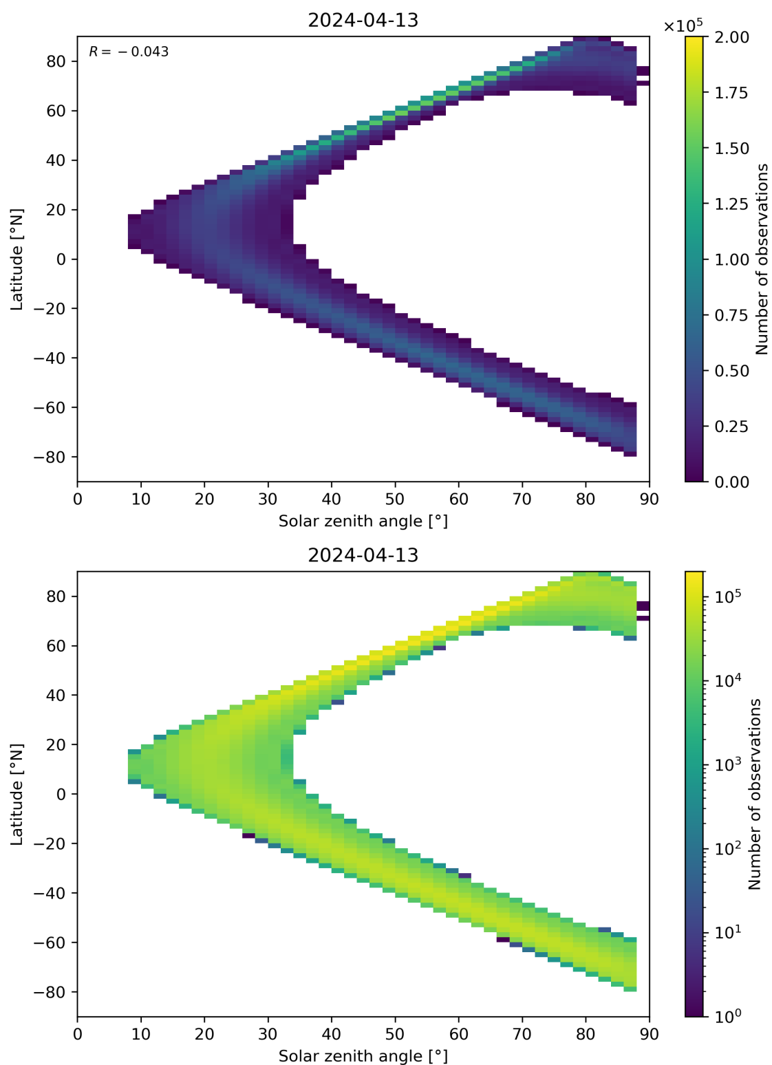
Figure 113: Scatter density plot of “Solar zenith angle” against “Latitude” for 2024-04-12 to 2024-04-14.
