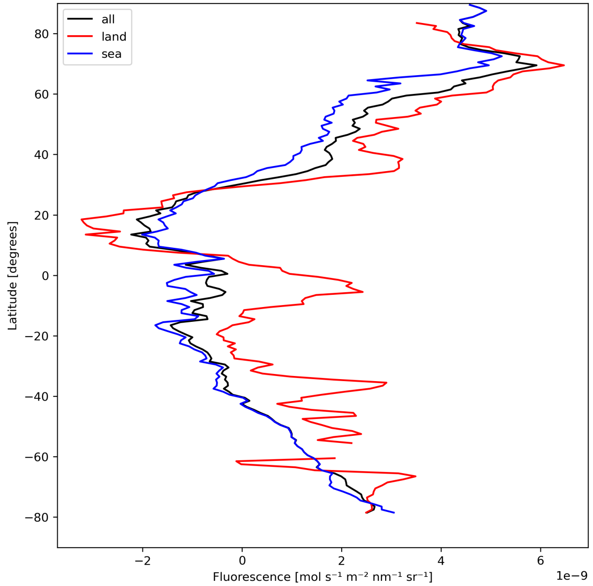
Figure 23: Zonal average of “Fluorescence” for 2024-04-12 to 2024-04-14.
