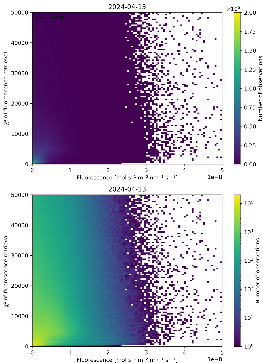
Figure 85: Scatter density plot of “Fluorescence” against “ \chi^2 of fluorescence retrieval” for 2024-04-12 to 2024-04-14.
