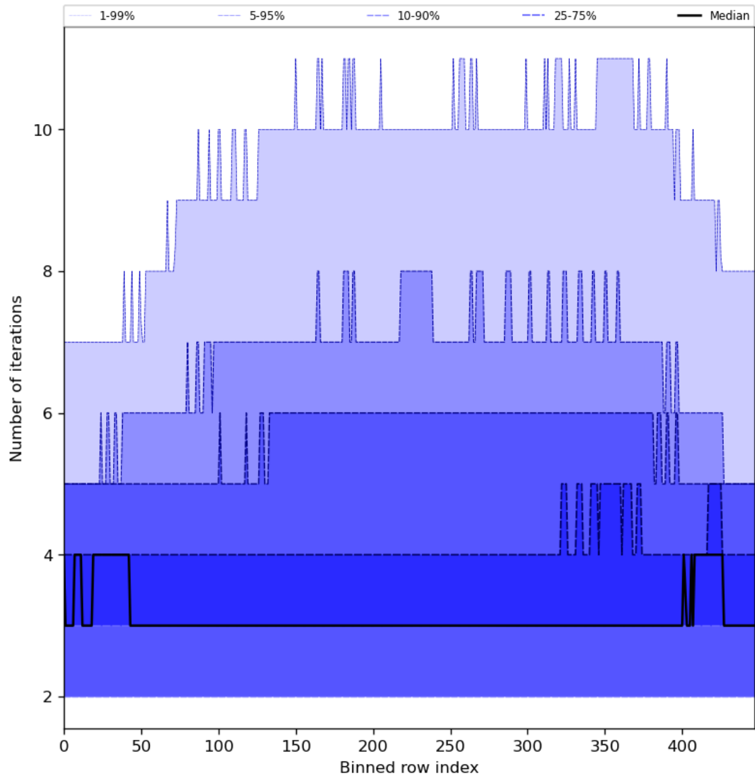
Figure 56: Along track statistics of “Number of iterations” for 2024-04-12 to 2024-04-14
