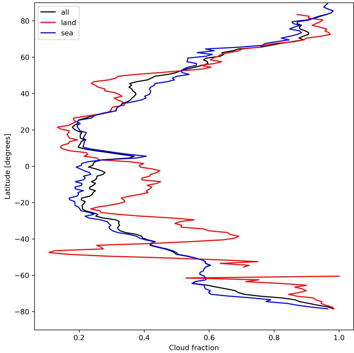
Figure 15: Zonal average of “Cloud fraction” for 2024-04-12 to 2024-04-14.
