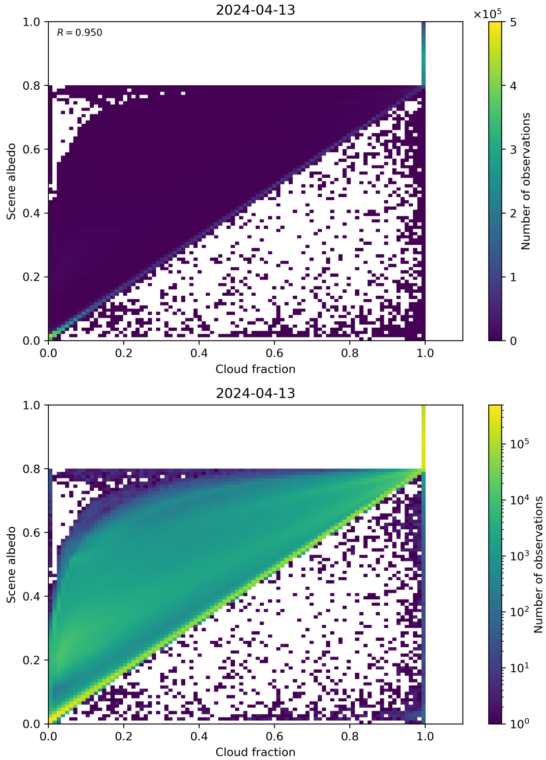
Figure 75: Scatter density plot of “Cloud fraction” against “Scene albedo” for 2024-04-12 to 2024-04-14.
