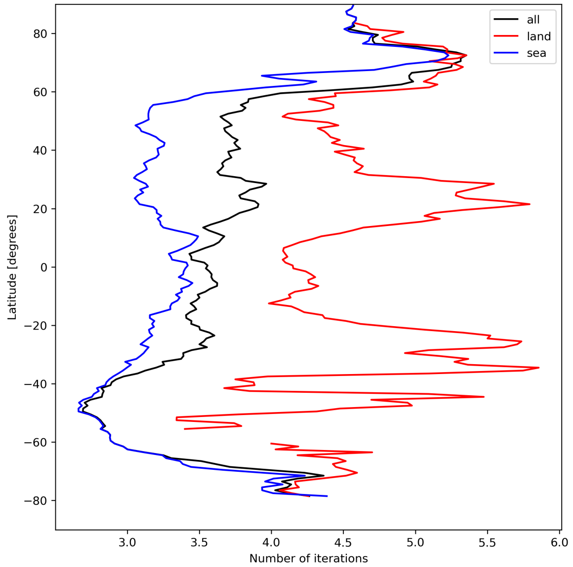
Figure 22: Zonal average of “Number of iterations” for 2024-04-12 to 2024-04-14.
