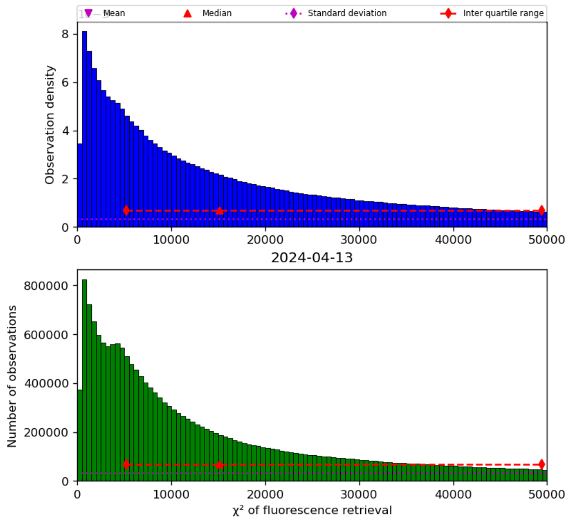
Figure 42: Histogram of “ \chi^2 of fluorescence retrieval” for 2024-04-12 to 2024-04-14
