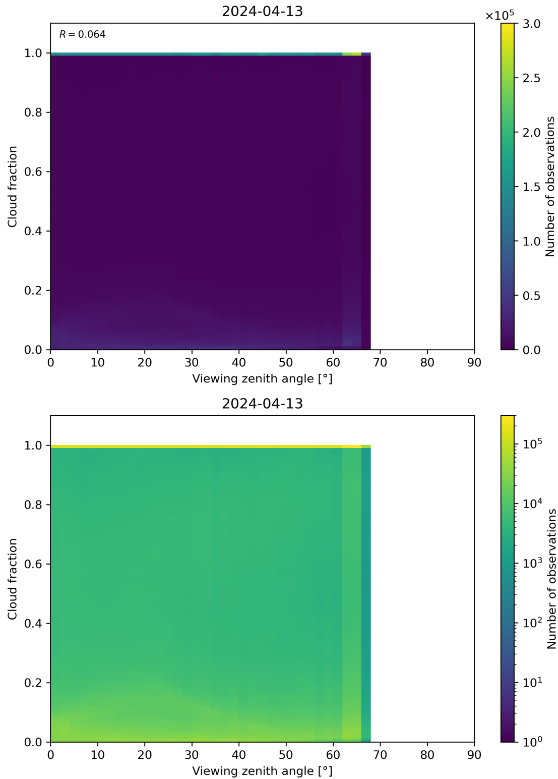
Figure 120: Scatter density plot of “Viewing zenith angle” against “Cloud fraction” for 2024-04-12 to 2024-04-14.
