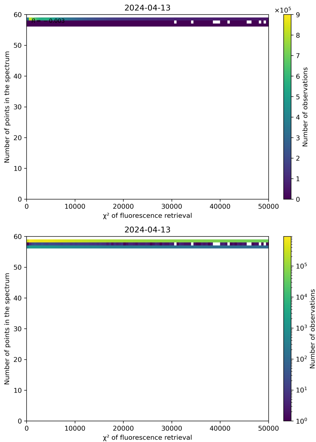
Figure 68: Scatter density plot of " \chi^2 of fluorescence retrieval" against "Number of points in the spectrum" for 2024-04-12 to 2024-04-14.
