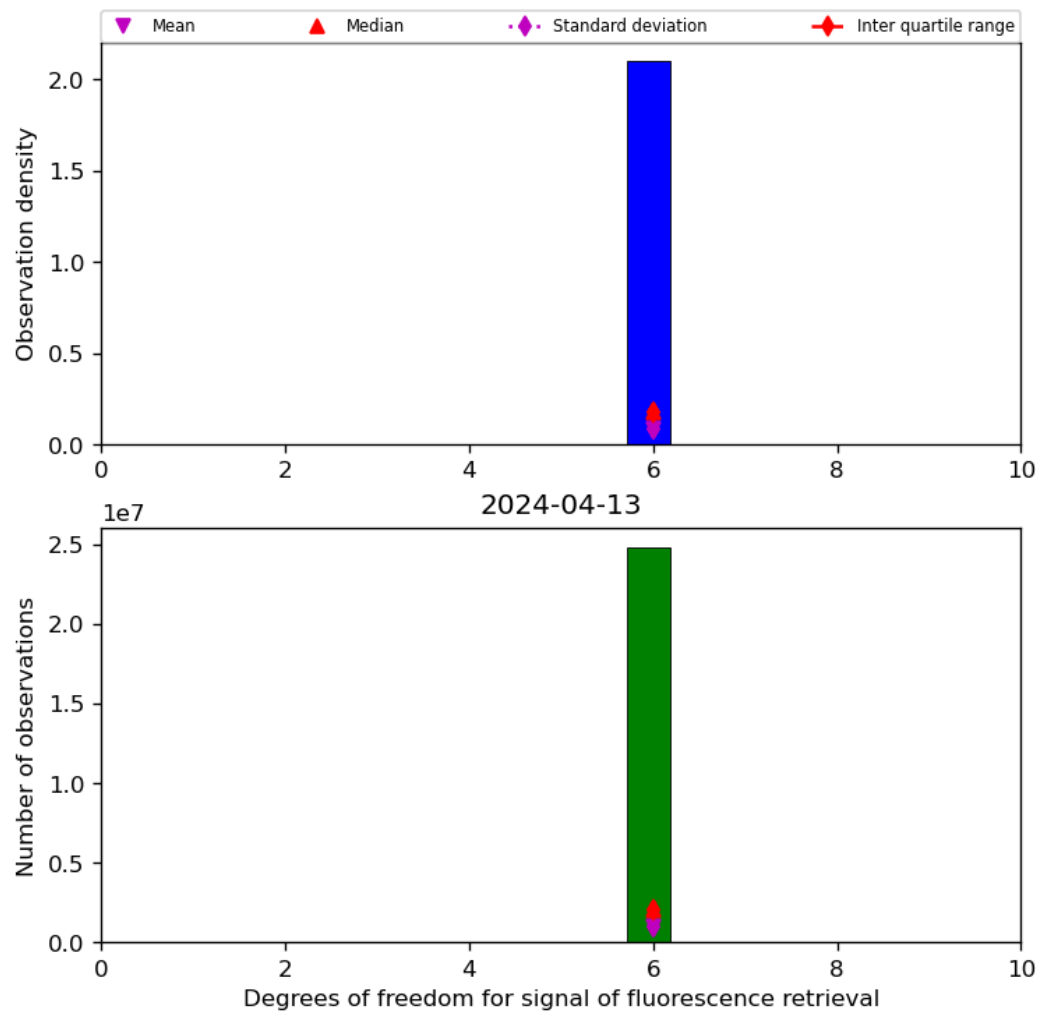
Figure 43: Histogram of “Degrees of freedom for signal of fluorescence retrieval” for 2024-04-12 to 2024-04-14
