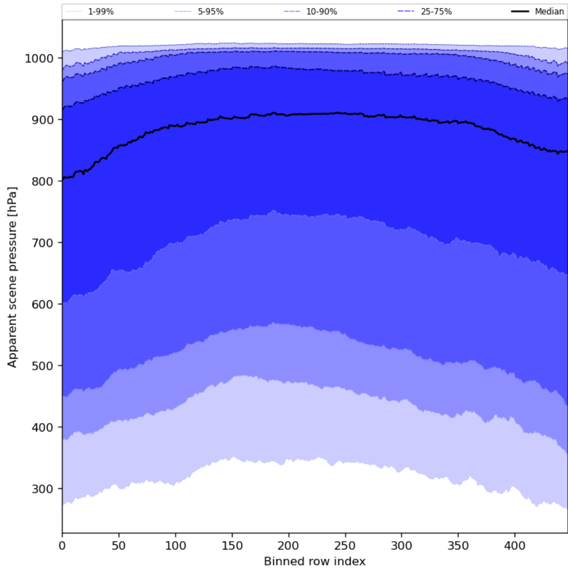
Figure 53: Along track statistics of “Apparent scene pressure” for 2024-04-12 to 2024-04-14
