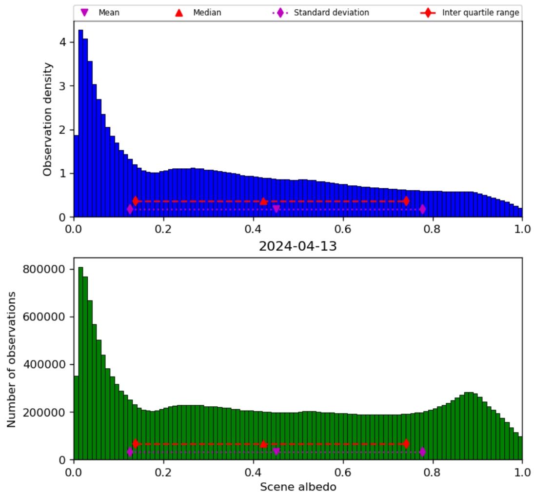
Figure 34: Histogram of “Scene albedo” for 2024-04-12 to 2024-04-14
