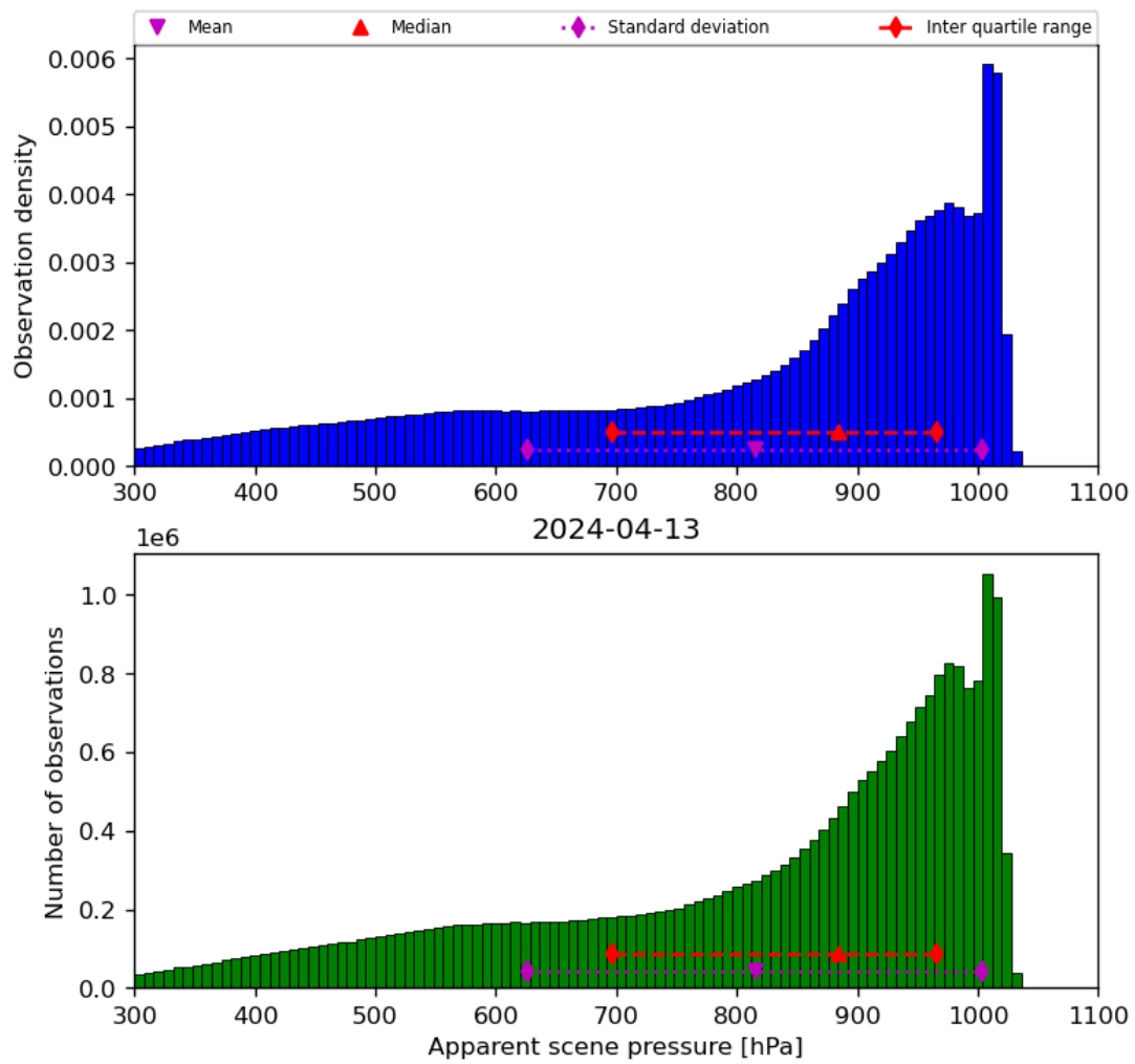
Figure 36: Histogram of “Apparent scene pressure” for 2024-04-12 to 2024-04-14
