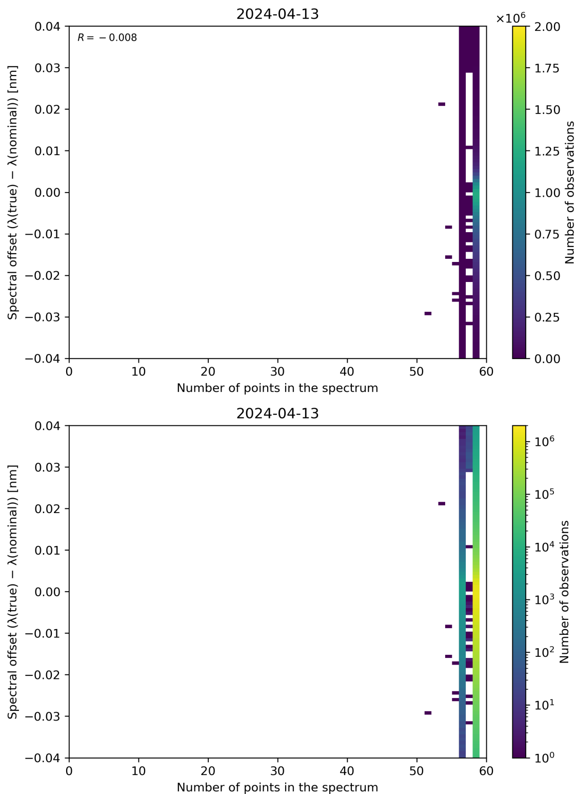
Figure 101: Scatter density plot of “Number of points in the spectrum” against “Spectral offset ( \lambda(\text{true}) - \lambda(\text{nominal}) )” for 2024-04-12 to 2024-04-14.
