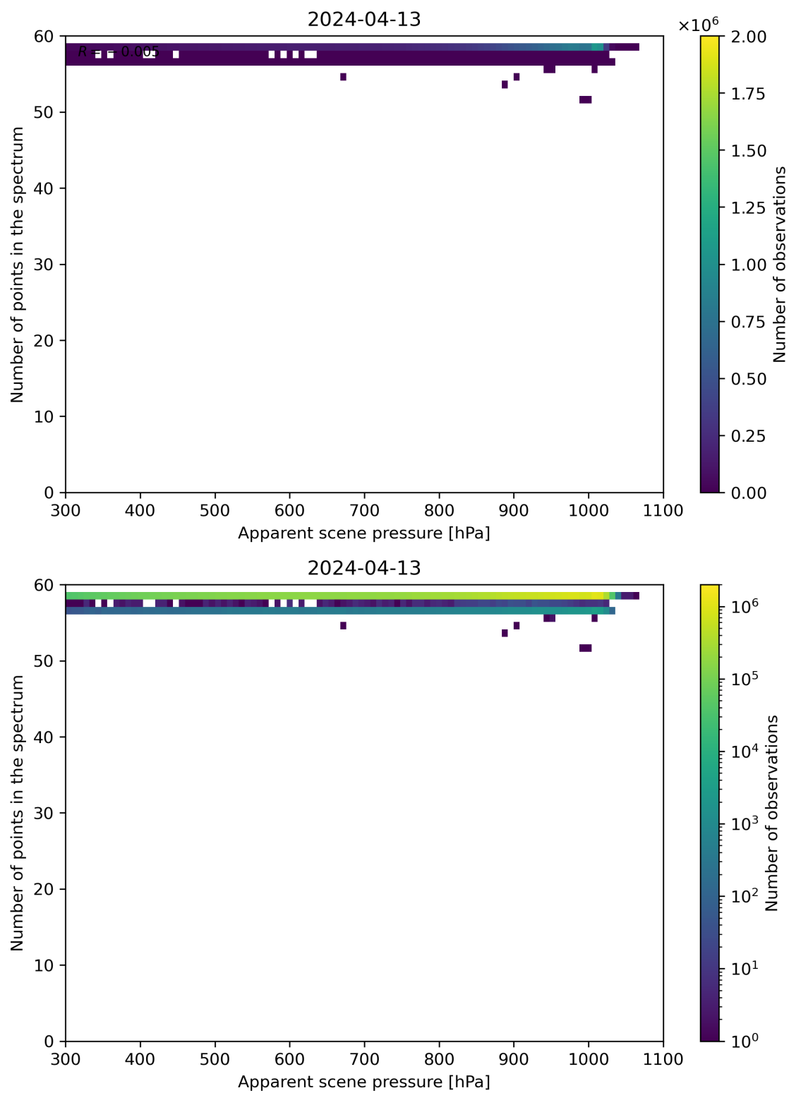
Figure 66: Scatter density plot of “Apparent scene pressure” against “Number of points in the spectrum” for 2024-04-12 to 2024-04-14.
