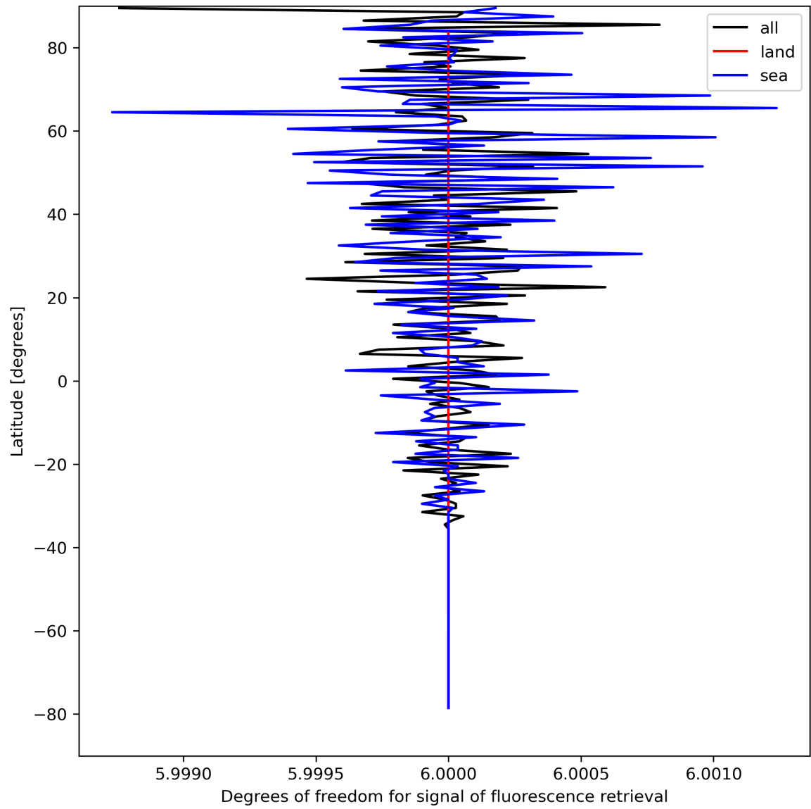
Figure 26: Zonal average of “Degrees of freedom for signal of fluorescence retrieval” for 2024-04-12 to 2024-04-14.
