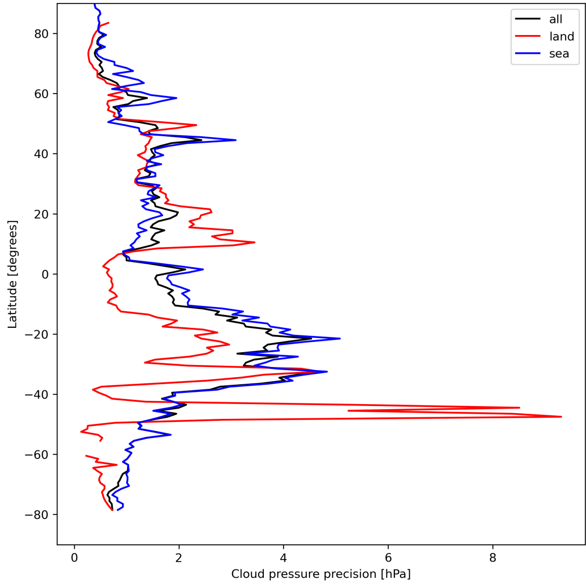
Figure 14: Zonal average of “Cloud pressure precision” for 2024-04-12 to 2024-04-14.
