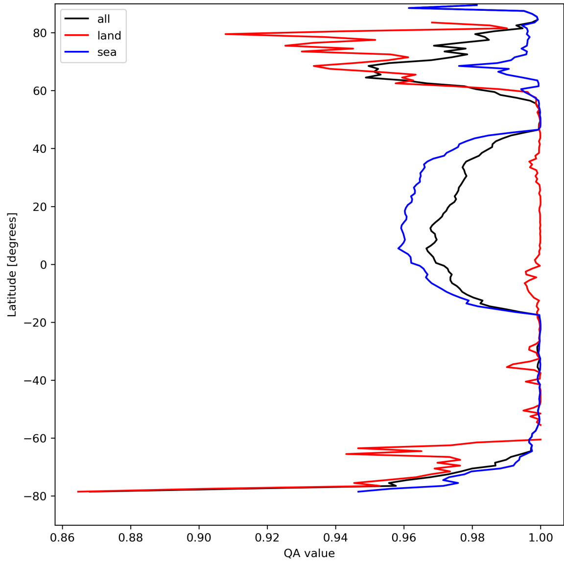
Figure 12: Zonal average of "QA value" for 2024-04-12 to 2024-04-14.
