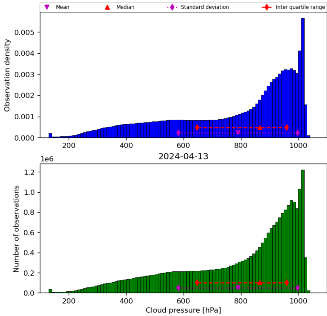
Figure 30: Histogram of “Cloud pressure” for 2024-04-12 to 2024-04-14
