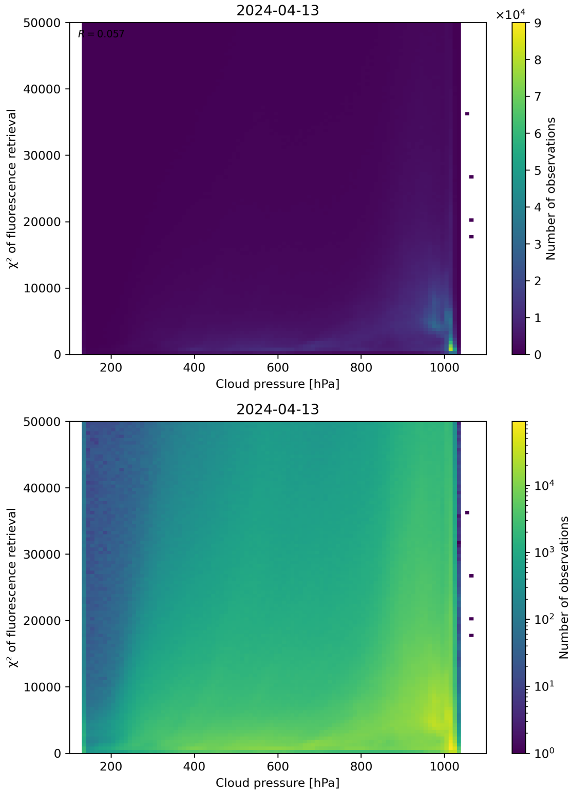
Figure 78: Scatter density plot of “Cloud pressure” against “ \chi^2 of fluorescence retrieval” for 2024-04-12 to 2024-04-14.
