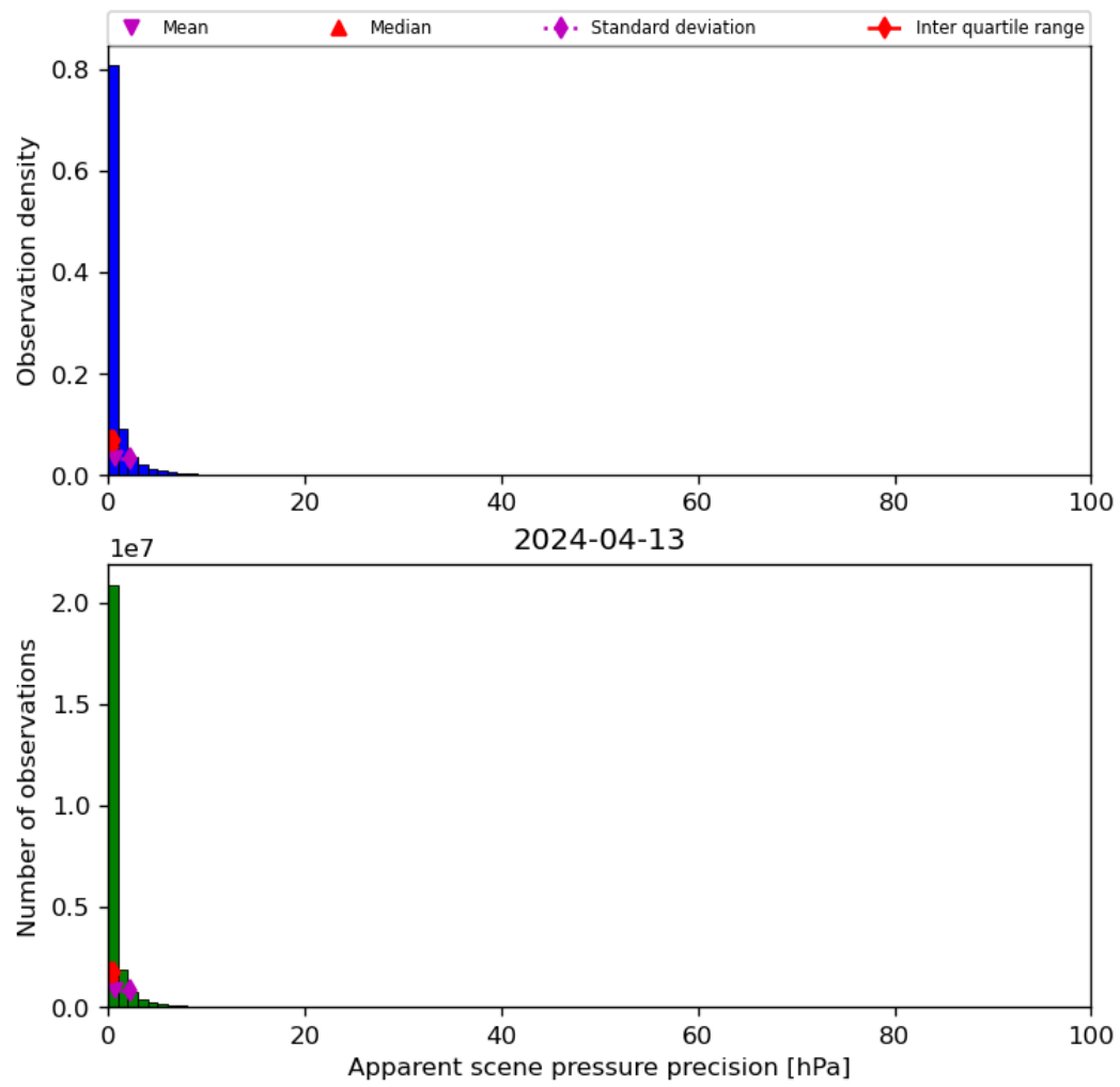
Figure 37: Histogram of “Apparent scene pressure precision” for 2024-04-12 to 2024-04-14
