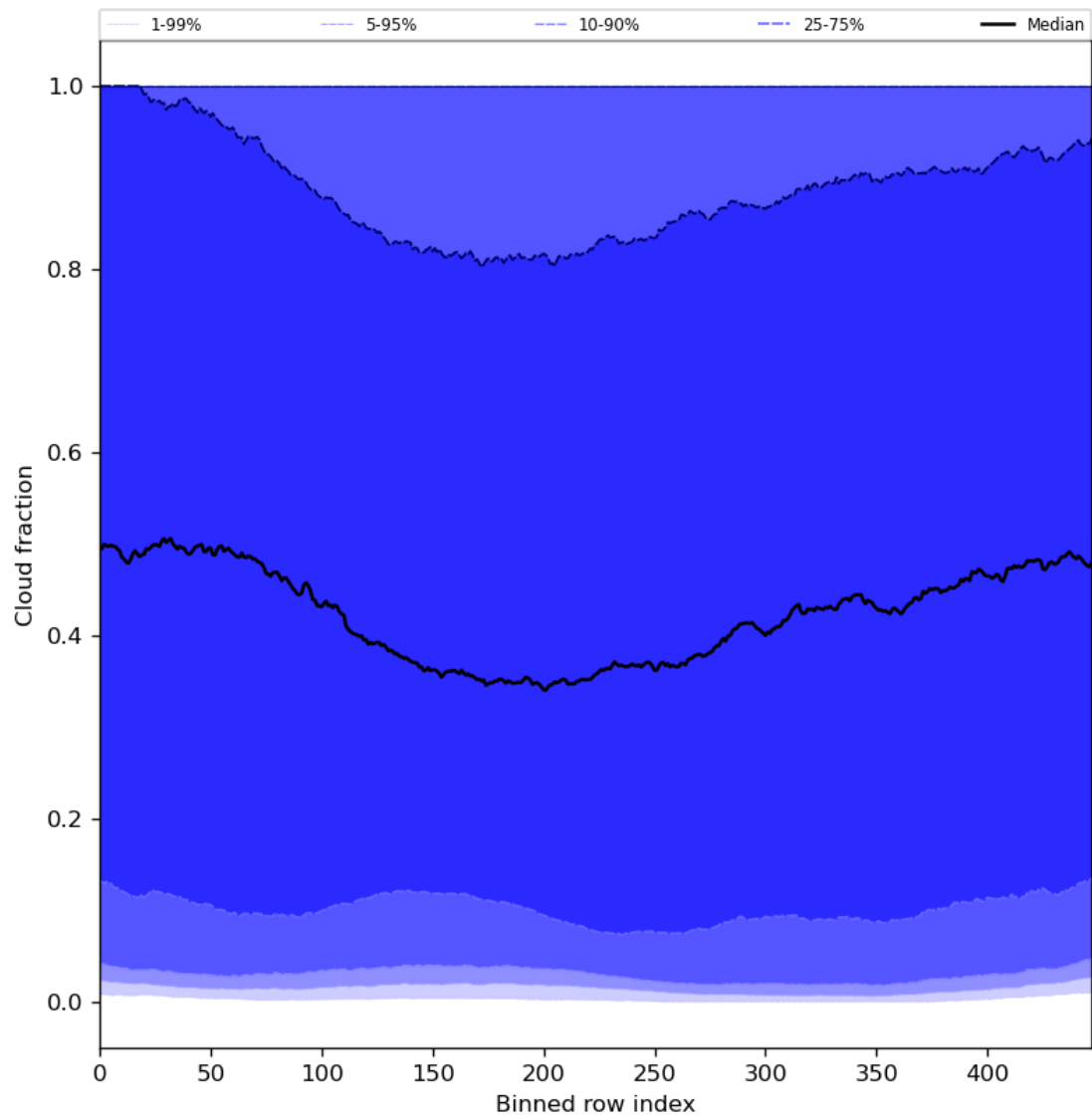
Figure 49: Along track statistics of “Cloud fraction” for 2024-04-12 to 2024-04-14
