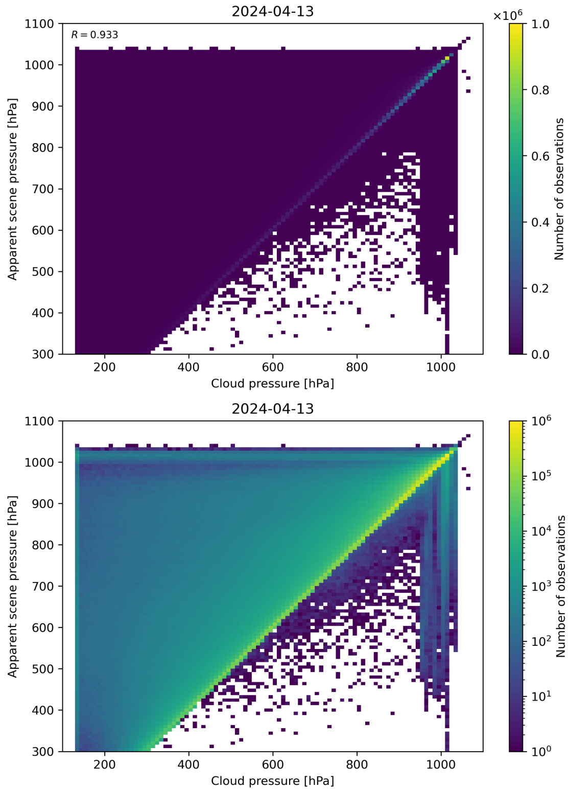
Figure 77: Scatter density plot of “Cloud pressure” against “Apparent scene pressure” for 2024-04-12 to 2024-04-14.
