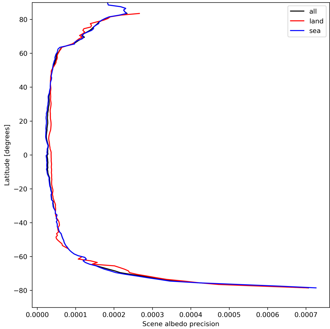
Figure 18: Zonal average of “Scene albedo precision” for 2024-04-12 to 2024-04-14.
