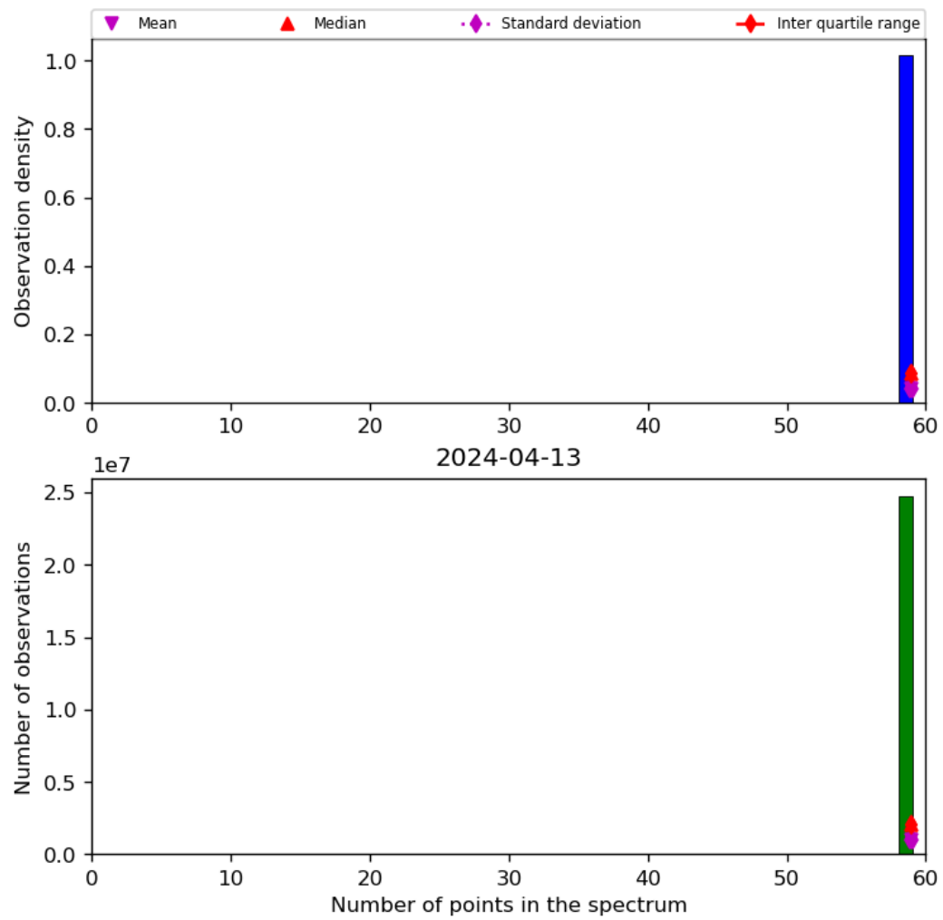
Figure 44: Histogram of “Number of points in the spectrum” for 2024-04-12 to 2024-04-14
