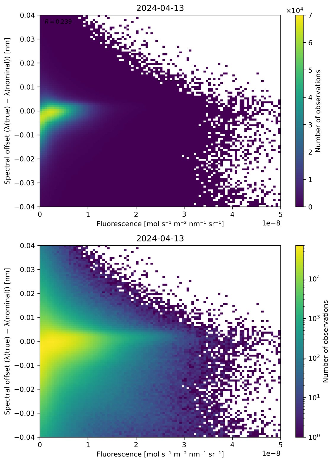
Figure 87: Scatter density plot of “Fluorescence” against “Spectral offset ( \lambda(\text{true}) - \lambda(\text{nominal}) )” for 2024-04-12 to 2024-04-14.
