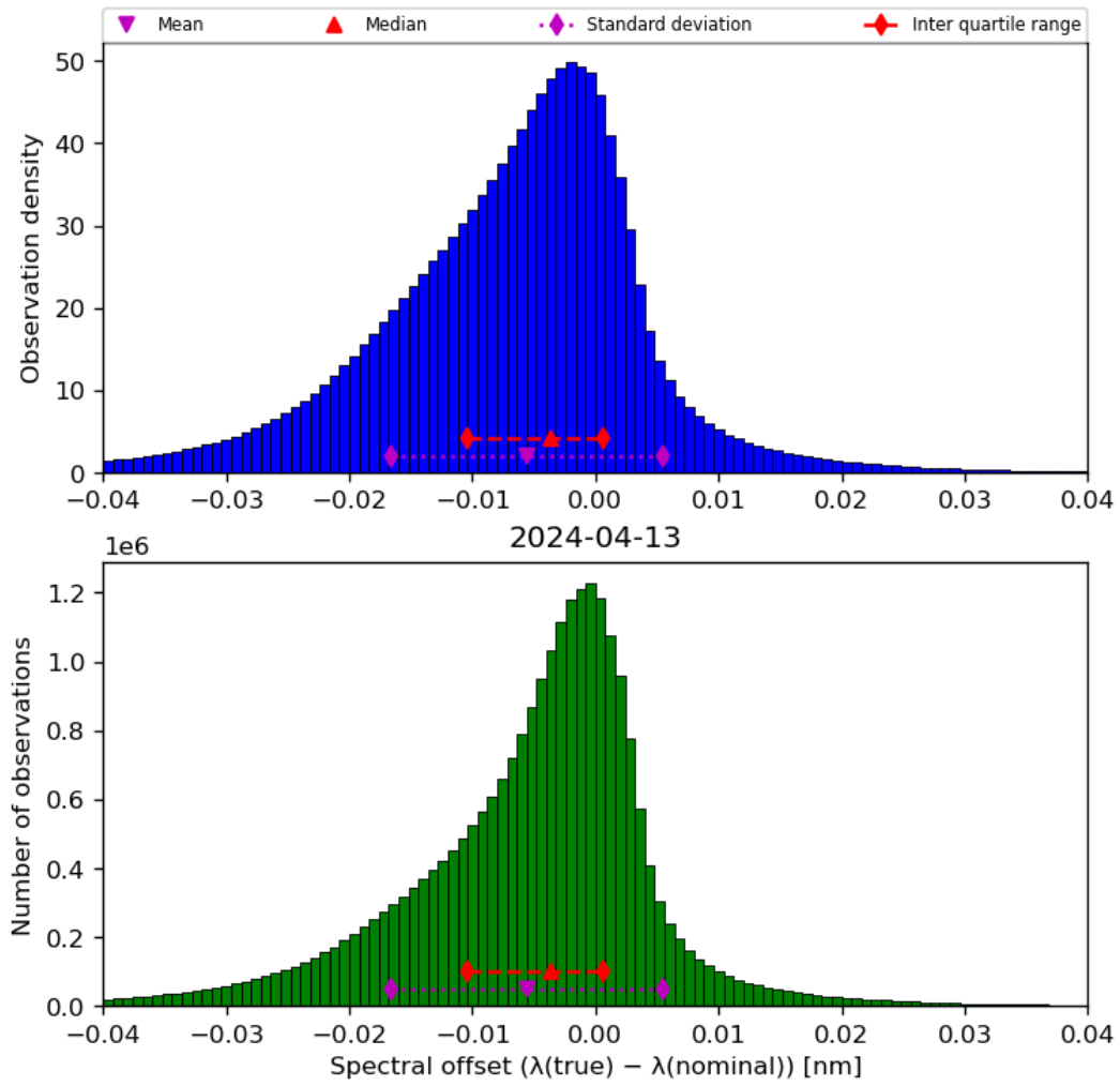
Figure 45: Histogram of “Spectral offset ( \lambda(\text{true}) - \lambda(\text{nominal}) )” for 2024-04-12 to 2024-04-14
