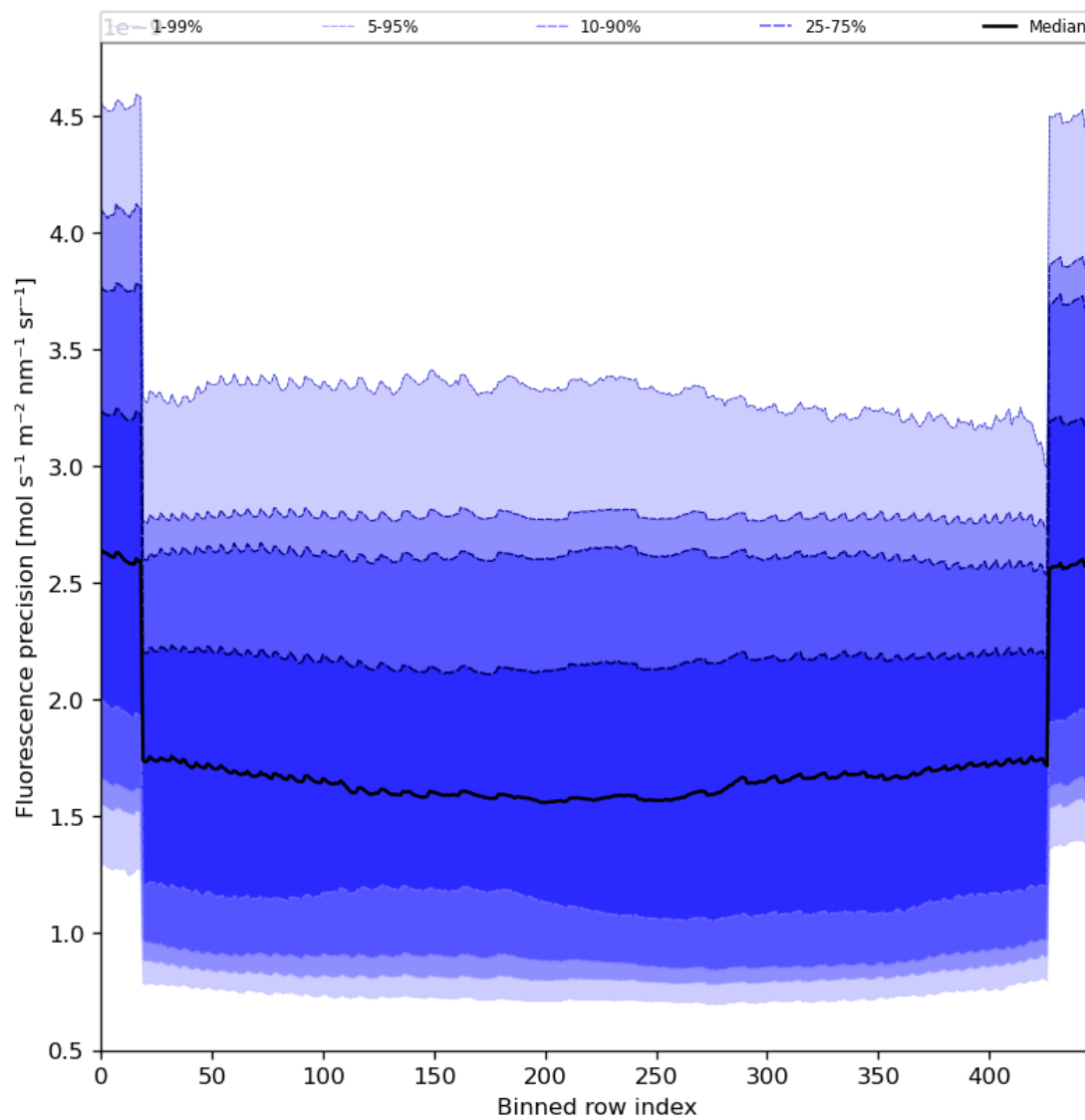
Figure 58: Along track statistics of “Fluorescence precision” for 2024-04-12 to 2024-04-14
