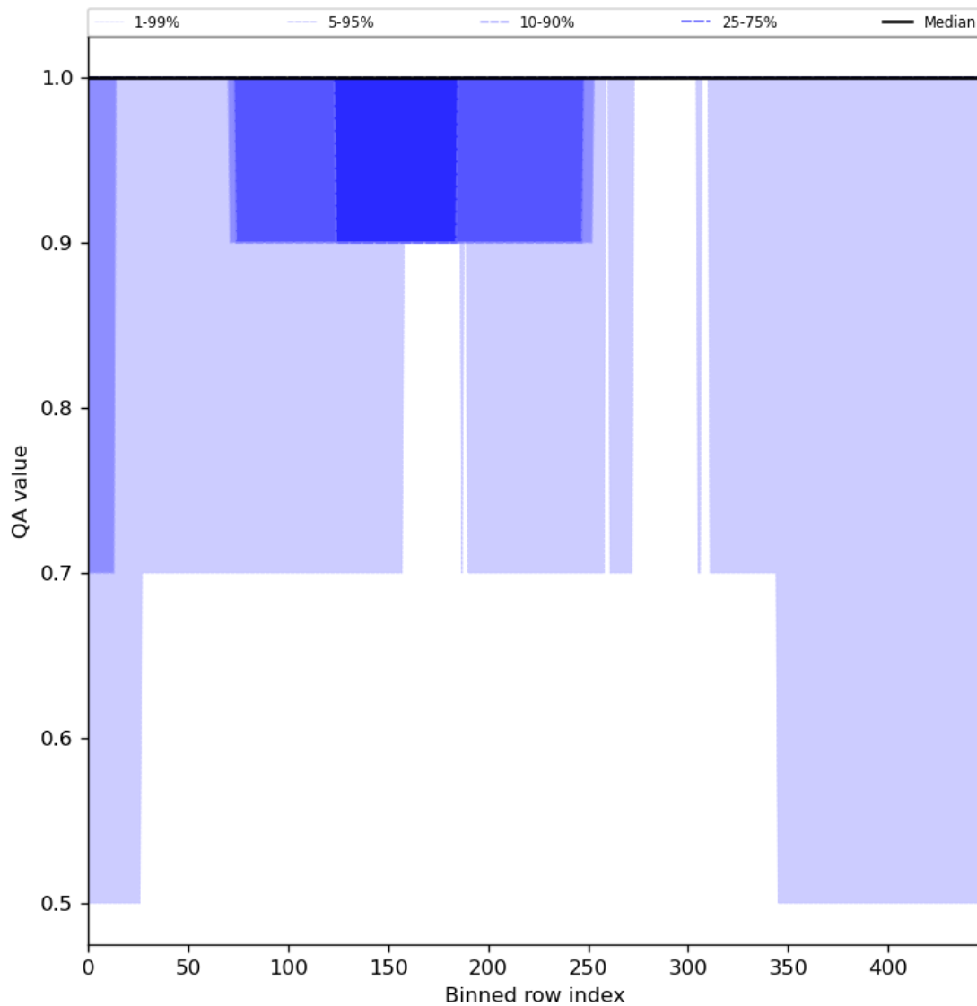
Figure 46: Along track statistics of “QA value” for 2024-04-12 to 2024-04-14
