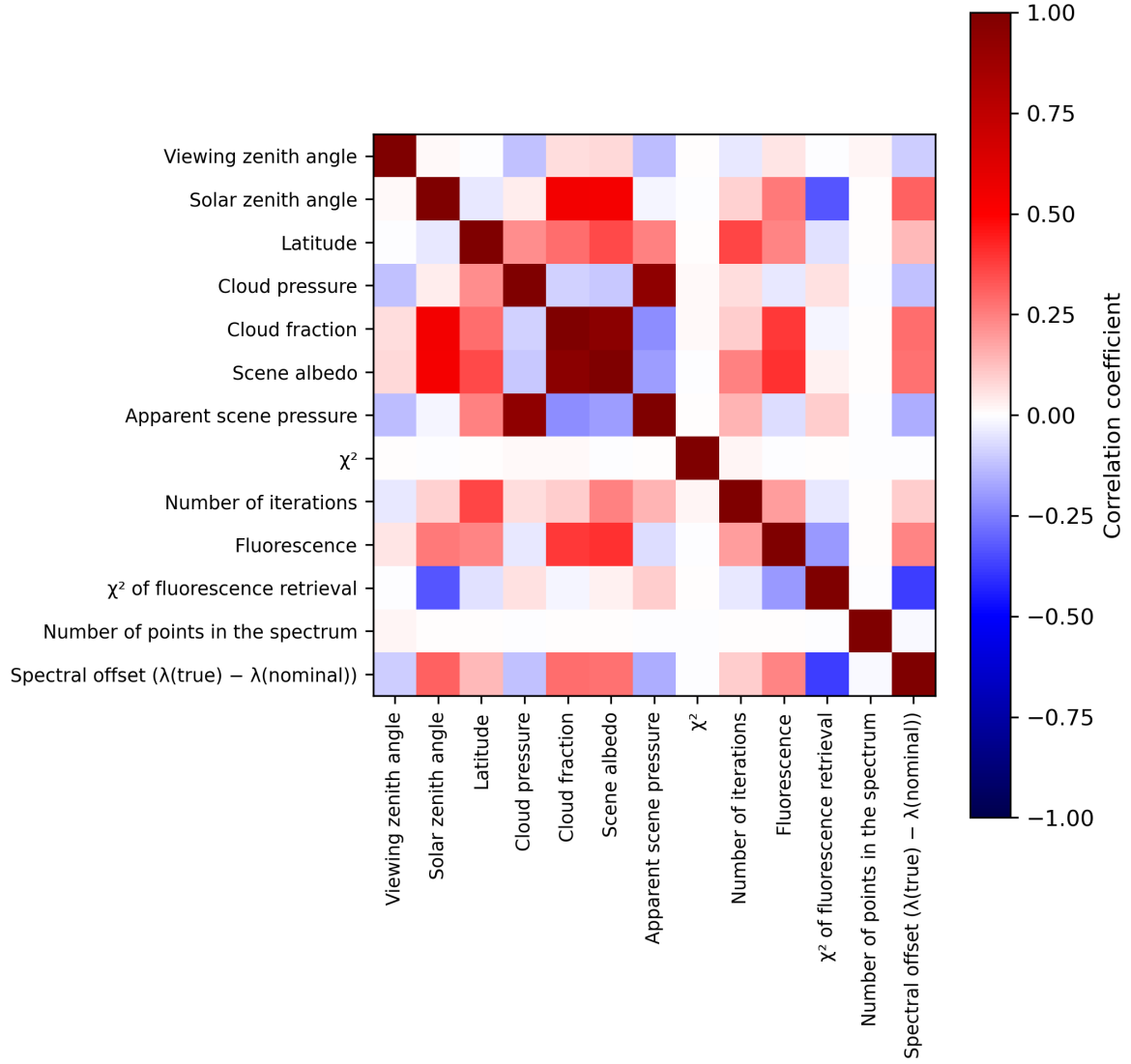
Figure 2: Map of correlation matrix for 2024-04-12 to 2024-04-14.
