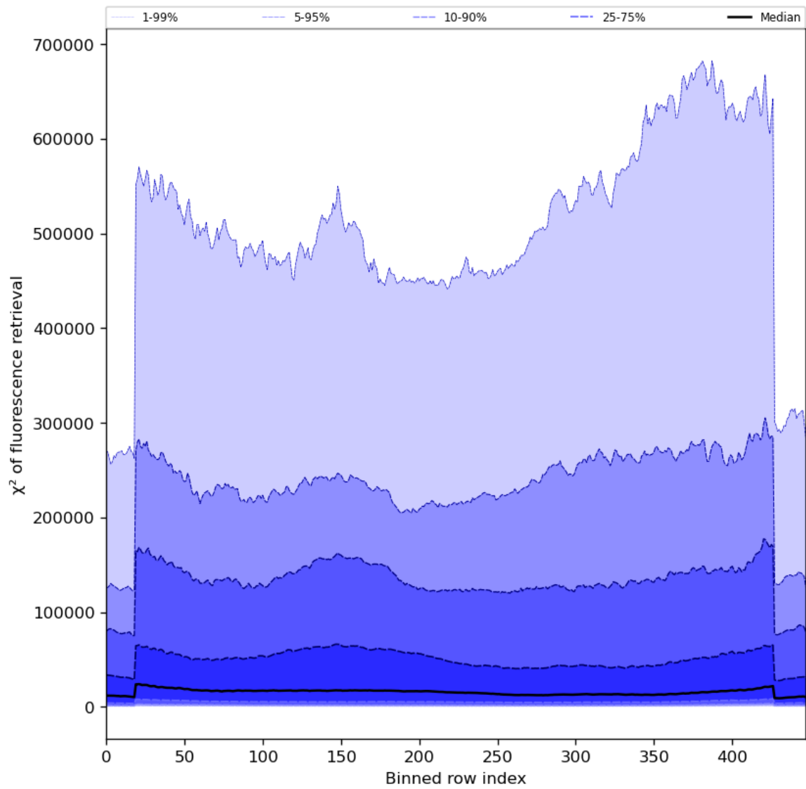
Figure 59: Along track statistics of “ \chi^2 of fluorescence retrieval” for 2024-04-12 to 2024-04-14
