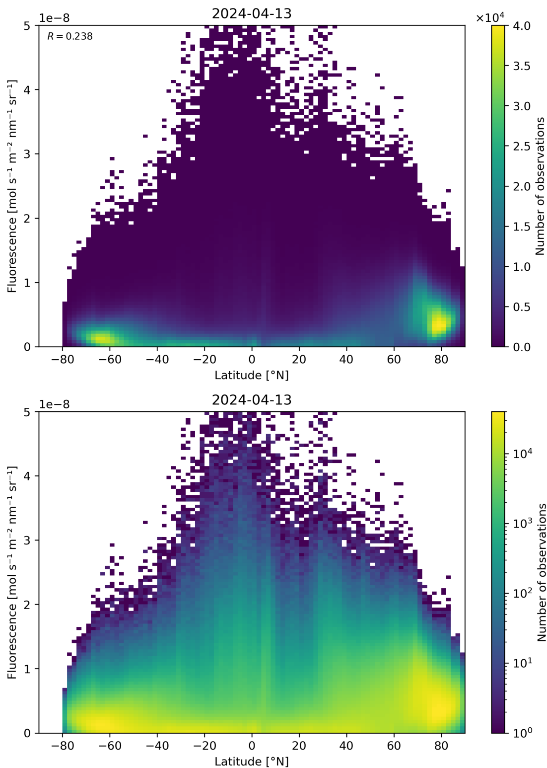
Figure 92: Scatter density plot of “Latitude” against “Fluorescence” for 2024-04-12 to 2024-04-14.
