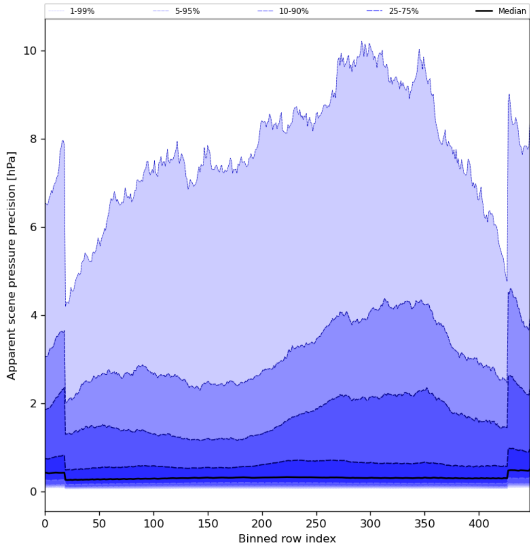
Figure 54: Along track statistics of “Apparent scene pressure precision” for 2024-04-12 to 2024-04-14
