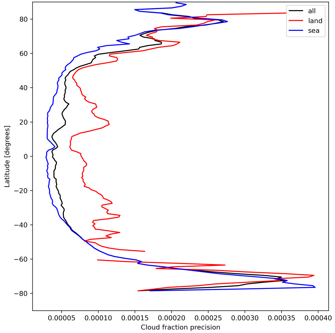
Figure 16: Zonal average of “Cloud fraction precision” for 2024-04-12 to 2024-04-14.
