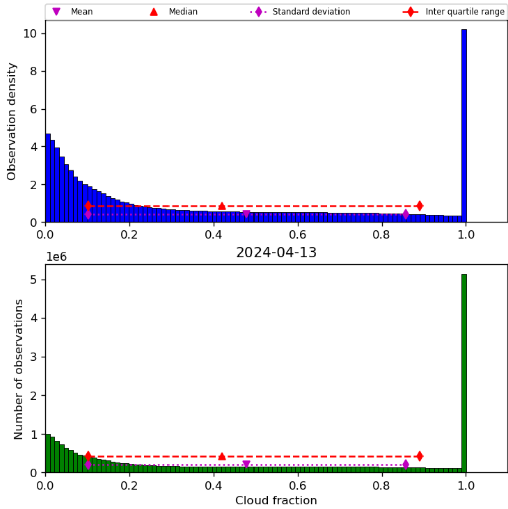
Figure 32: Histogram of “Cloud fraction” for 2024-04-12 to 2024-04-14
