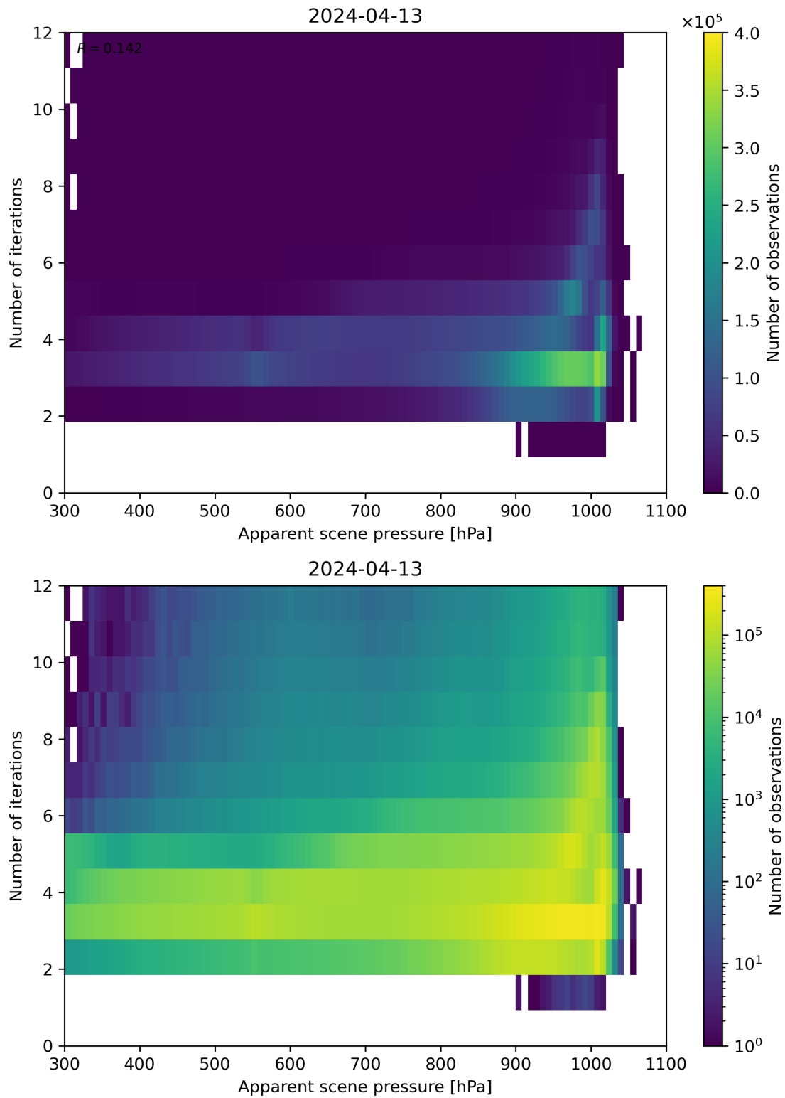
Figure 65: Scatter density plot of “Apparent scene pressure” against “Number of iterations” for 2024-04-12 to 2024-04-14.
