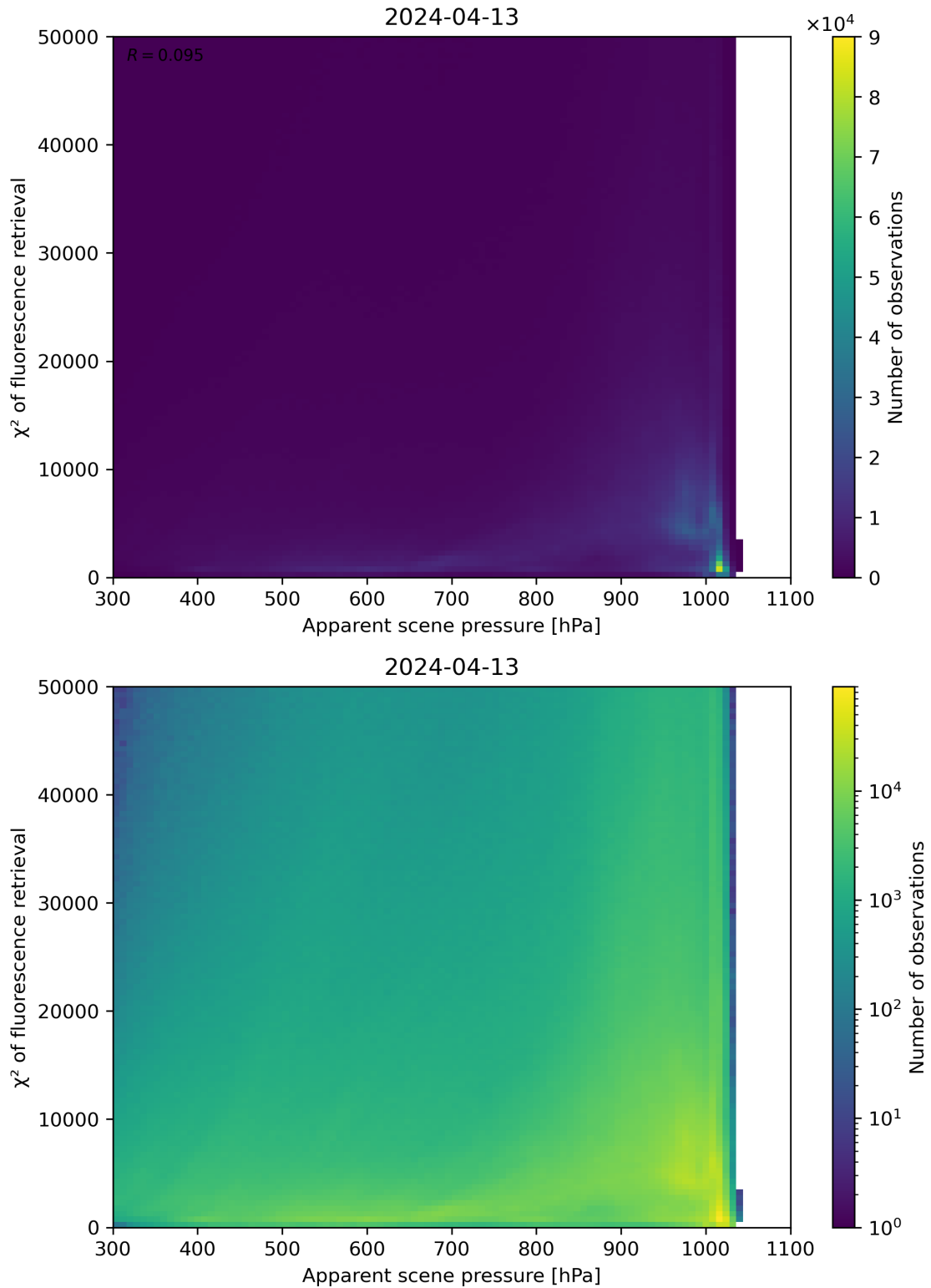
Figure 63: Scatter density plot of “Apparent scene pressure” against “ \chi^2 of fluorescence retrieval” for 2024-04-12 to 2024-04-14.
