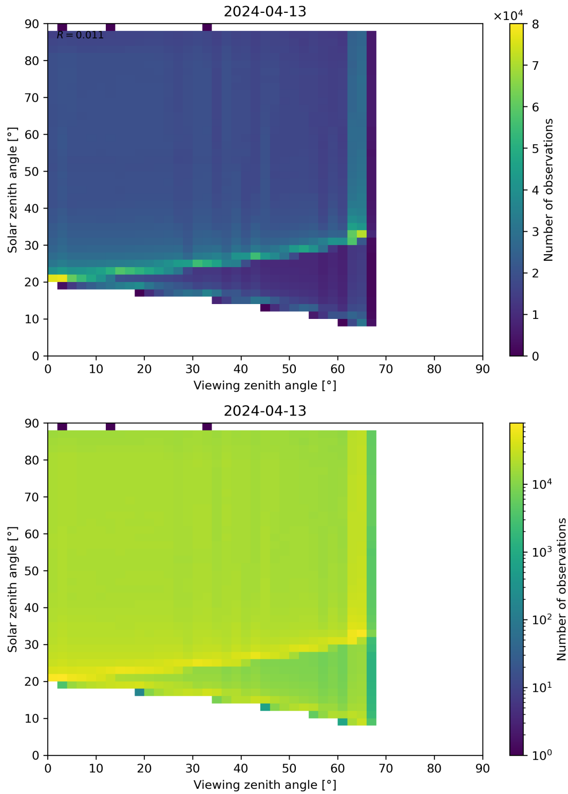
Figure 127: Scatter density plot of “Viewing zenith angle” against “Solar zenith angle” for 2024-04-12 to 2024-04-14.
