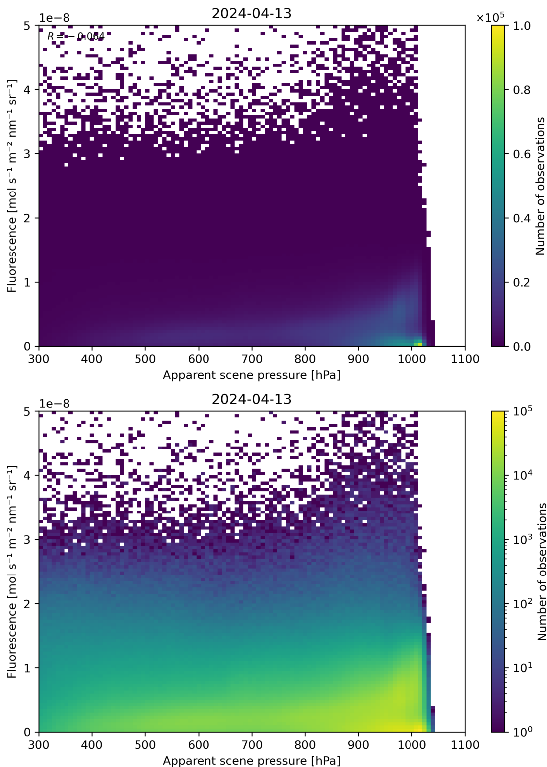
Figure 64: Scatter density plot of “Apparent scene pressure” against “Fluorescence” for 2024-04-12 to 2024-04-14.
