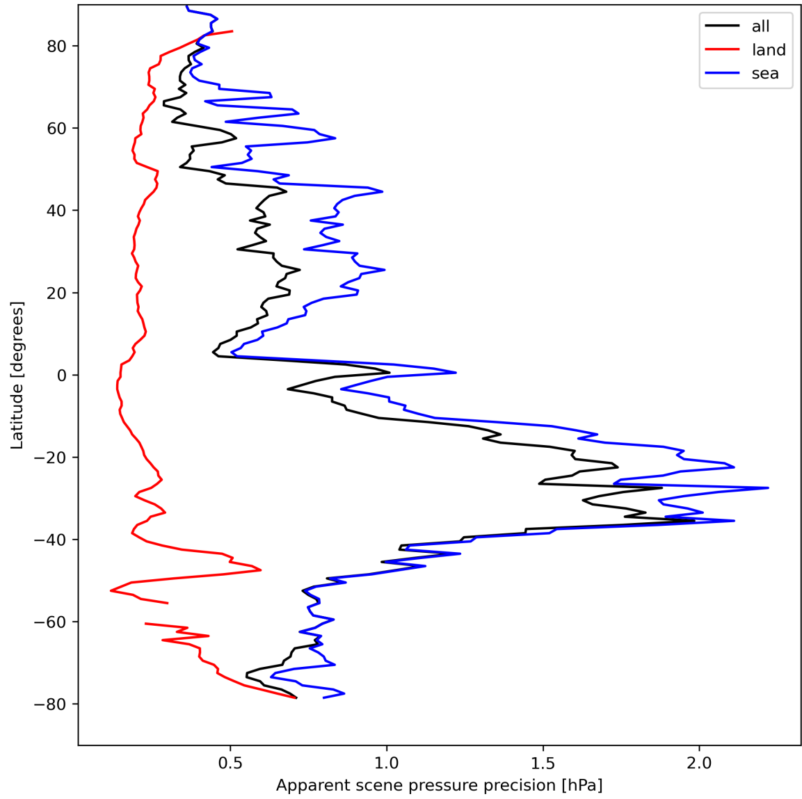
Figure 20: Zonal average of “Apparent scene pressure precision” for 2024-04-12 to 2024-04-14.
