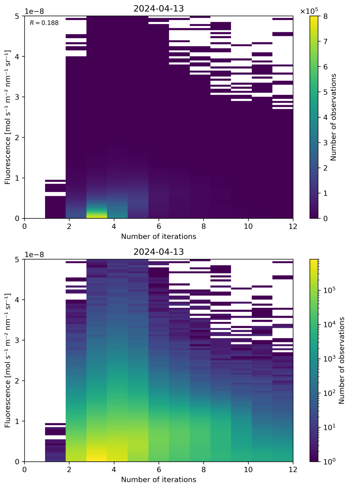
Figure 98: Scatter density plot of “Number of iterations” against “Fluorescence” for 2024-04-12 to 2024-04-14.
