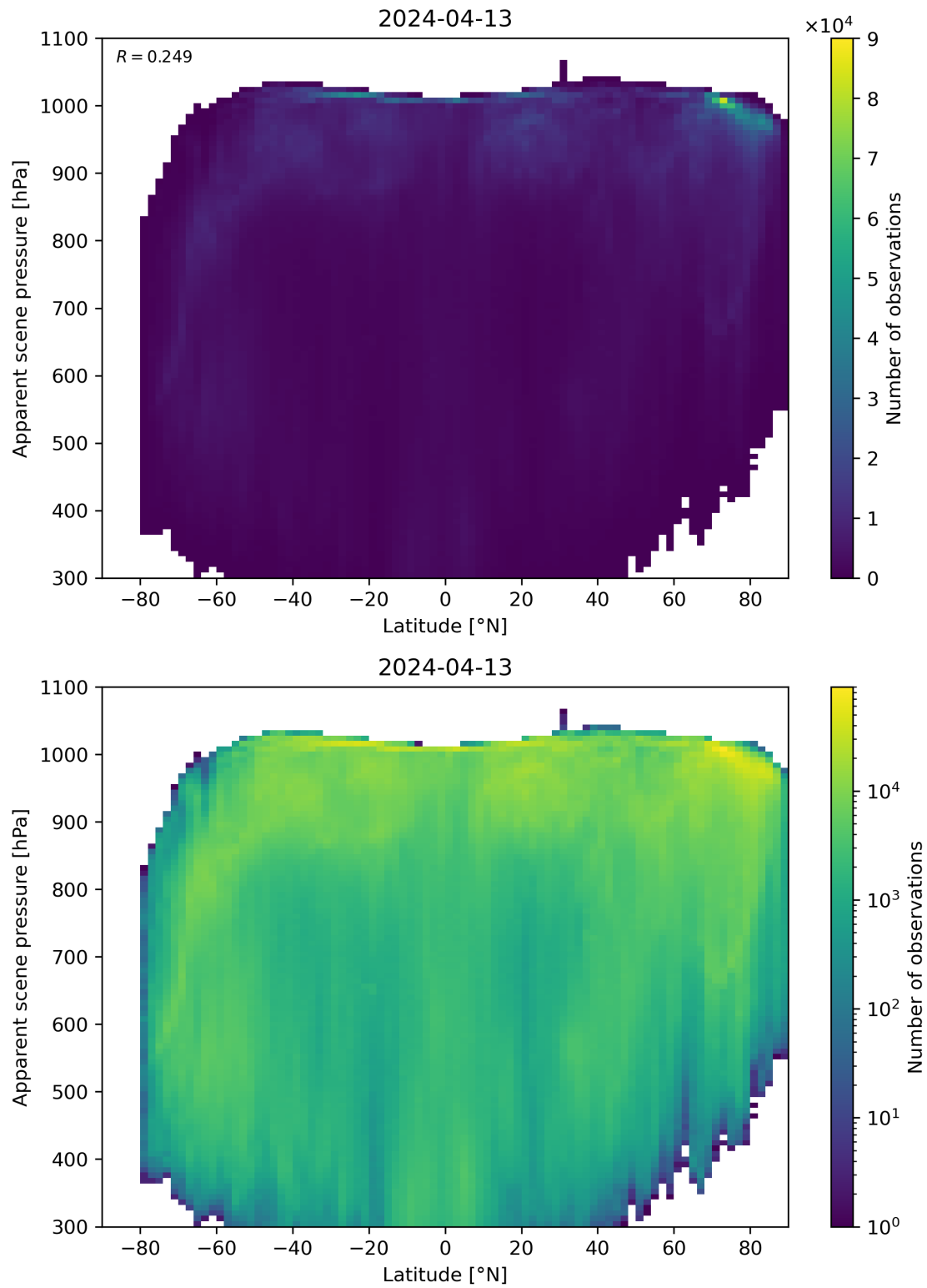
Figure 88: Scatter density plot of “Latitude” against “Apparent scene pressure” for 2024-04-12 to 2024-04-14.
