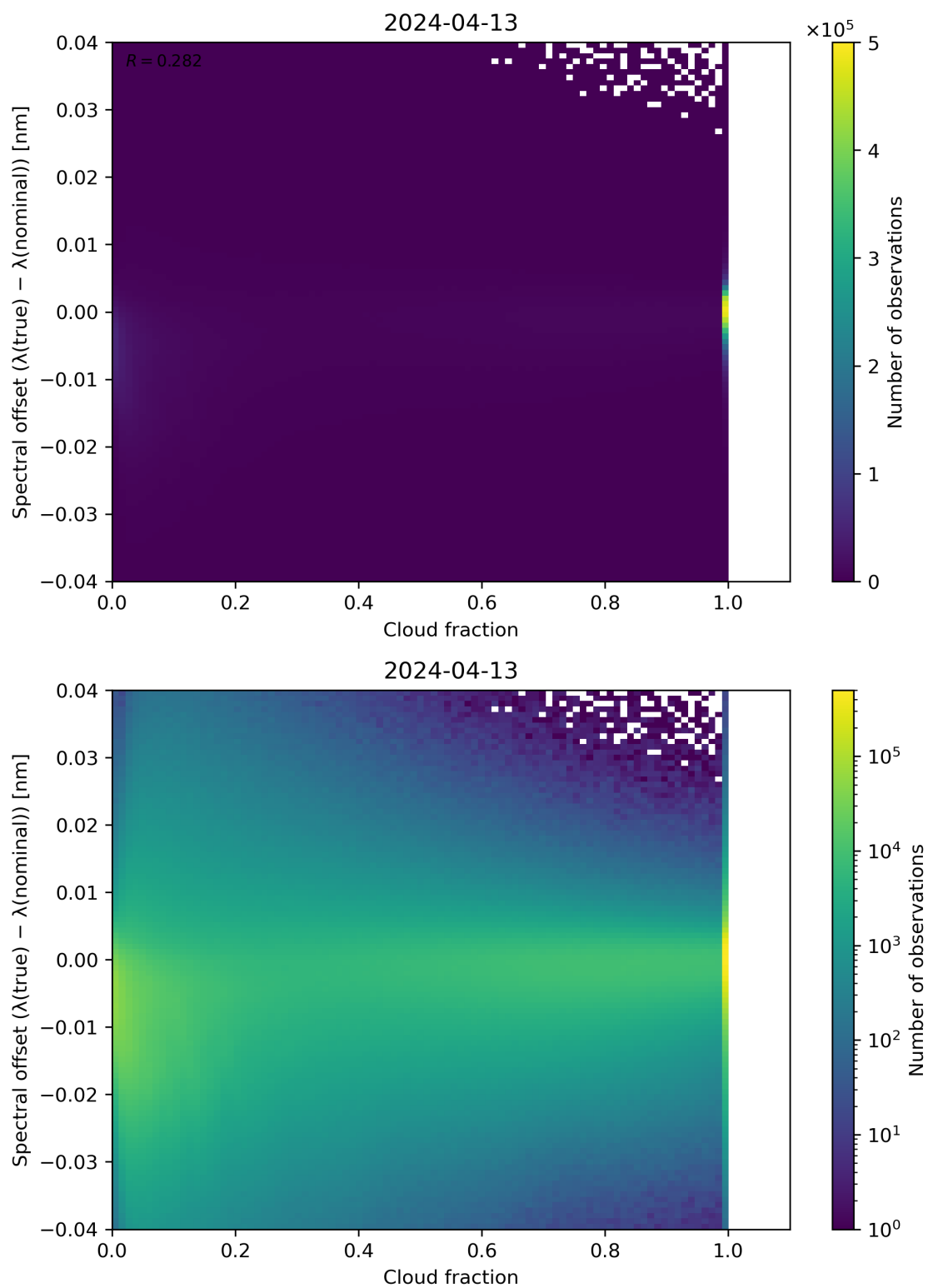
Figure 76: Scatter density plot of “Cloud fraction” against “Spectral offset ( \lambda(\text{true}) - \lambda(\text{nominal}) )” for 2024-04-12 to 2024-04-14.
