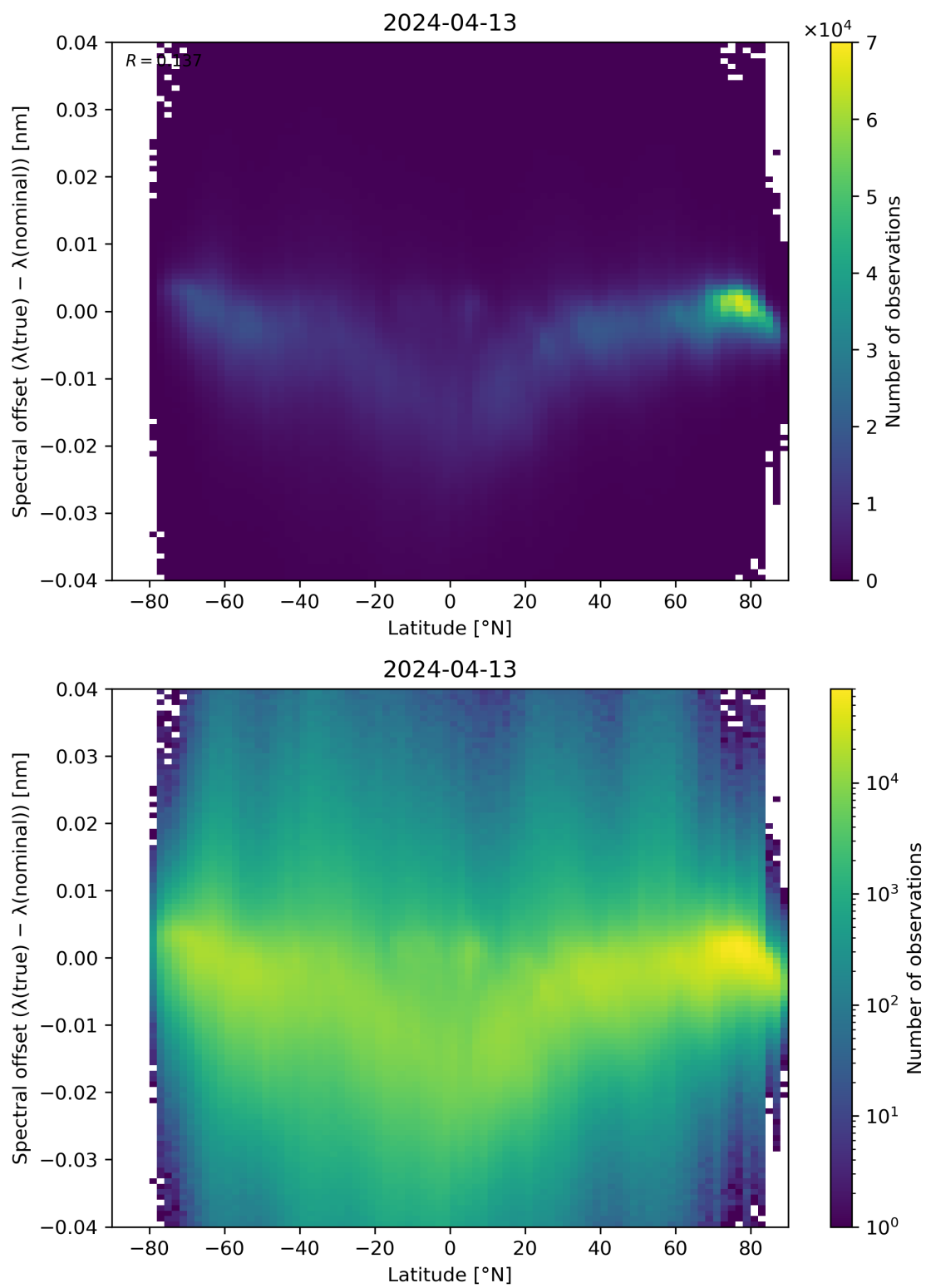
Figure 96: Scatter density plot of “Latitude” against “Spectral offset ( \lambda(\text{true}) - \lambda(\text{nominal}) )” for 2024-04-12 to 2024-04-14.
