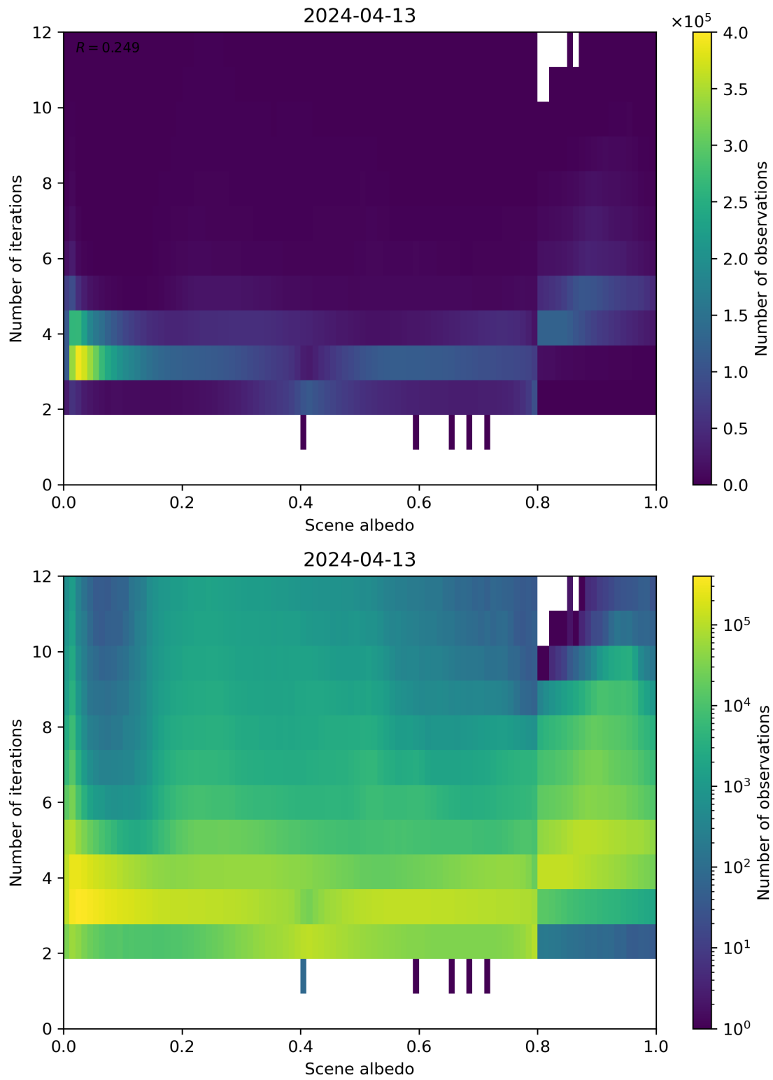
Figure 105: Scatter density plot of “Scene albedo” against “Number of iterations” for 2024-04-12 to 2024-04-14.
