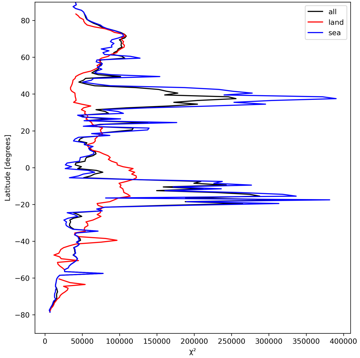
Figure 21: Zonal average of “ \chi^2 ” for 2024-04-12 to 2024-04-14.
