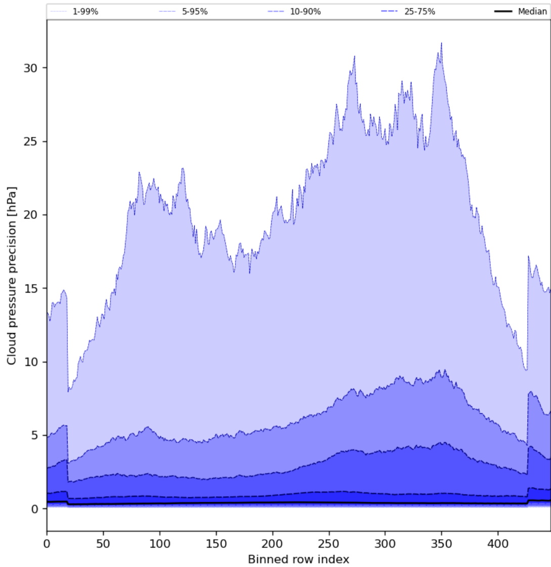
Figure 48: Along track statistics of “Cloud pressure precision” for 2024-04-12 to 2024-04-14
