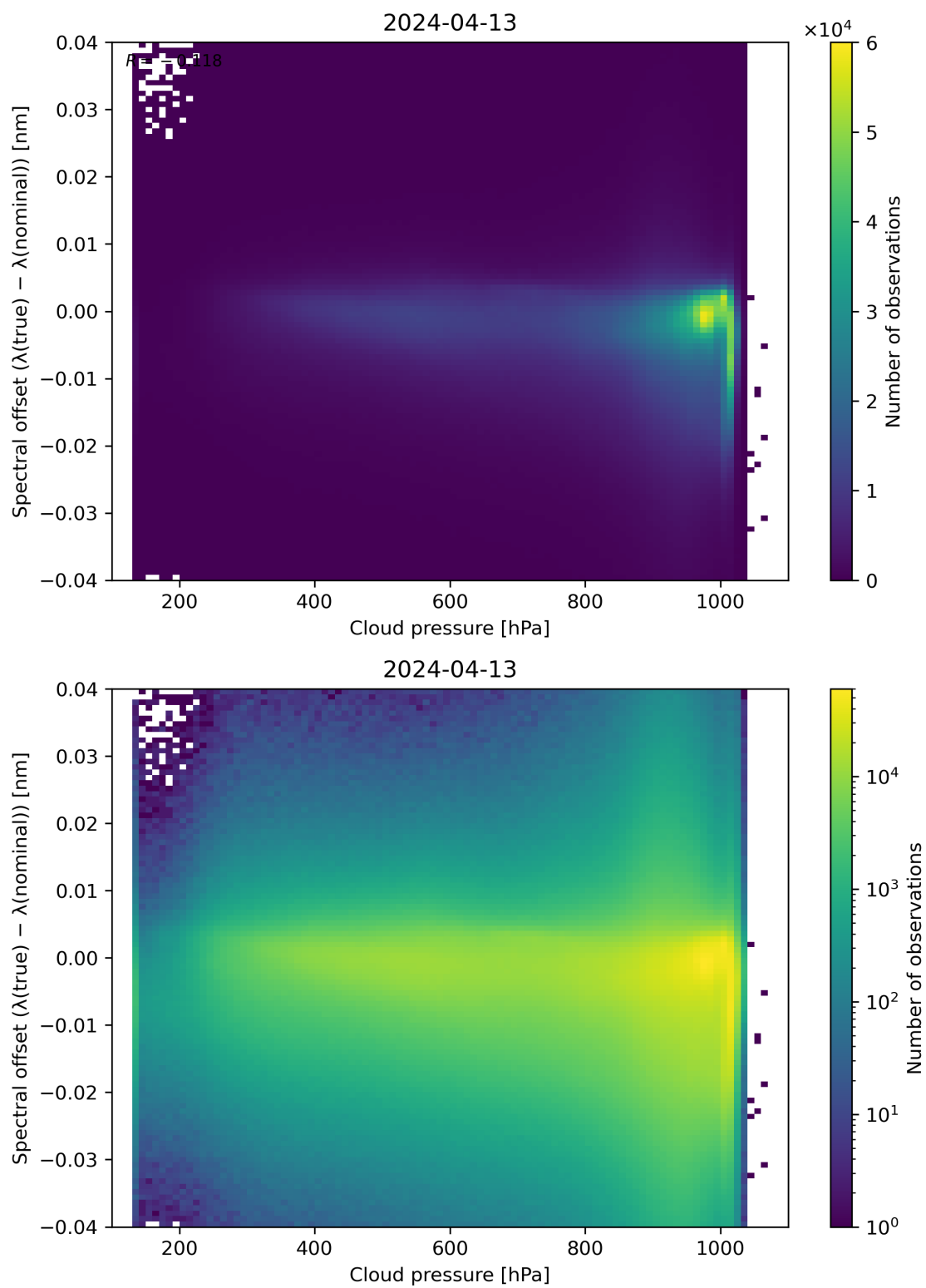
Figure 84: Scatter density plot of “Cloud pressure” against “Spectral offset ( \lambda(\text{true}) - \lambda(\text{nominal}) )” for 2024-04-12 to 2024-04-14.
