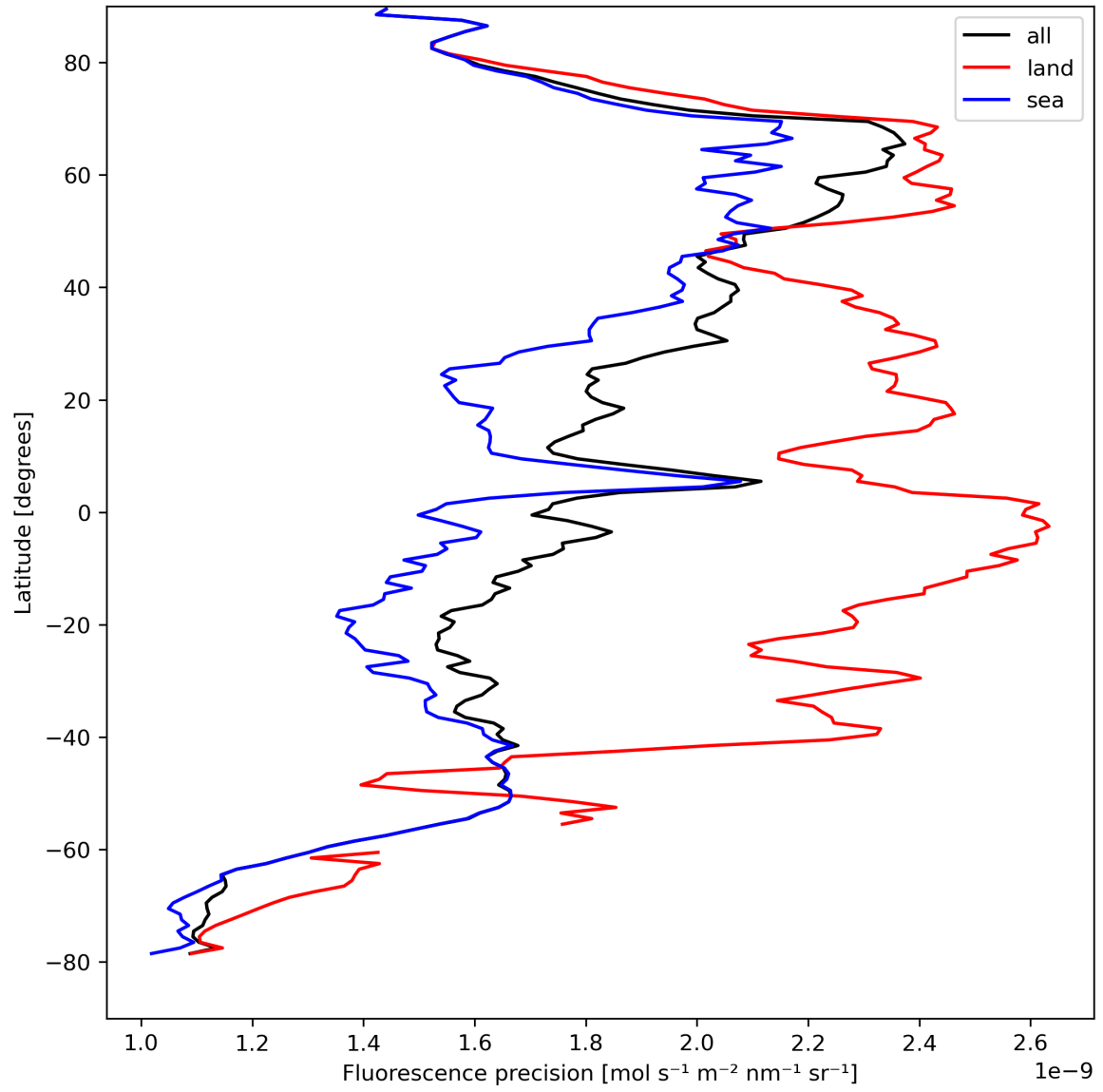
Figure 24: Zonal average of “Fluorescence precision” for 2024-04-12 to 2024-04-14.
