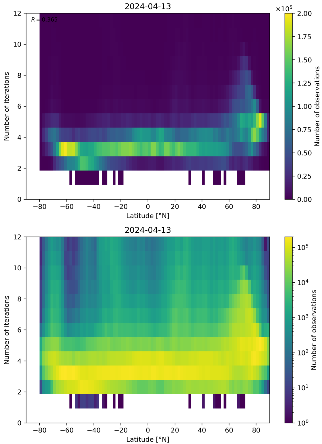
Figure 93: Scatter density plot of “Latitude” against “Number of iterations” for 2024-04-12 to 2024-04-14.
