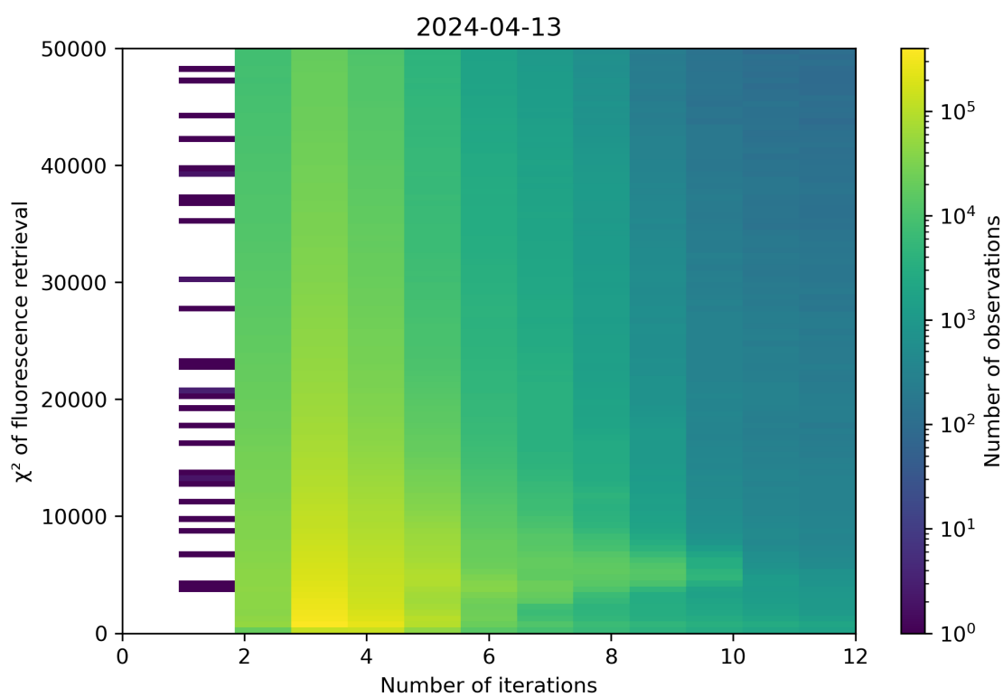
Figure 97: Scatter density plot of “Number of iterations” against “ \chi^2 of fluorescence retrieval” for 2024-04-12 to 2024-04-14.
