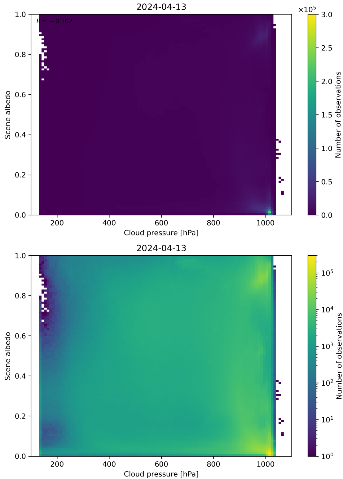
Figure 83: Scatter density plot of “Cloud pressure” against “Scene albedo” for 2024-04-12 to 2024-04-14.
