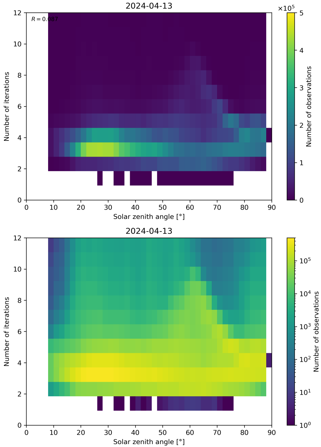
Figure 114: Scatter density plot of “Solar zenith angle” against “Number of iterations” for 2024-04-12 to 2024-04-14.
