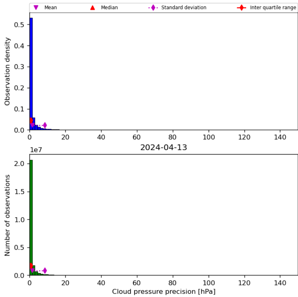
Figure 31: Histogram of “Cloud pressure precision” for 2024-04-12 to 2024-04-14
