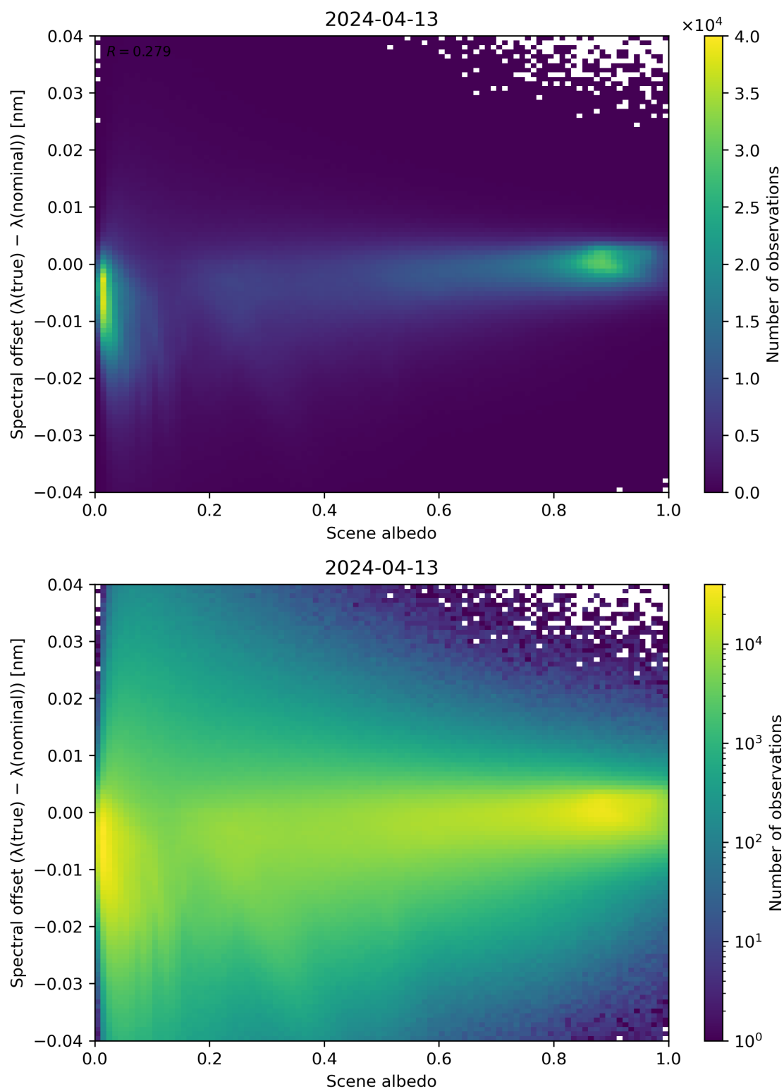
Figure 107: Scatter density plot of “Scene albedo” against “Spectral offset ( \lambda(\text{true}) - \lambda(\text{nominal}) )” for 2024-04-12 to 2024-04-14.
