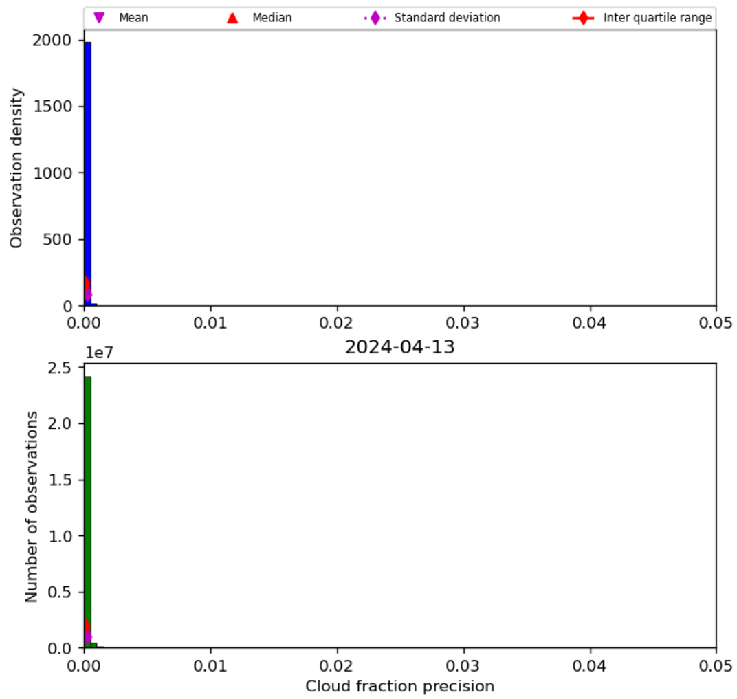
Figure 33: Histogram of “Cloud fraction precision” for 2024-04-12 to 2024-04-14
