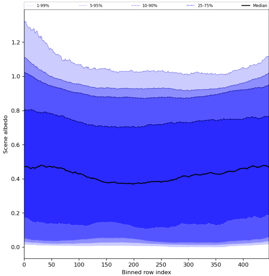
Figure 51: Along track statistics of “Scene albedo” for 2024-04-12 to 2024-04-14
