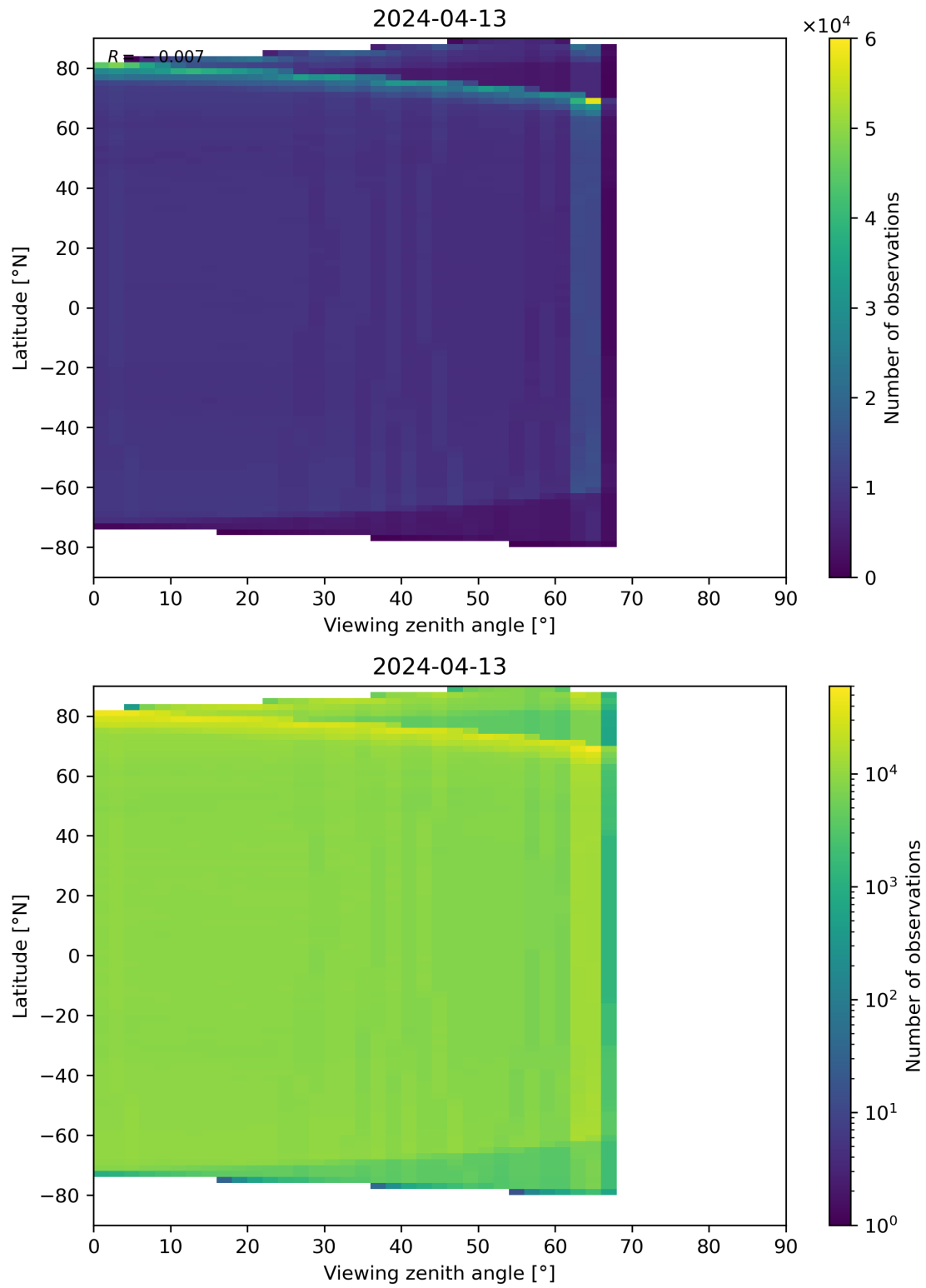
Figure 123: Scatter density plot of “Viewing zenith angle” against “Latitude” for 2024-04-12 to 2024-04-14.
