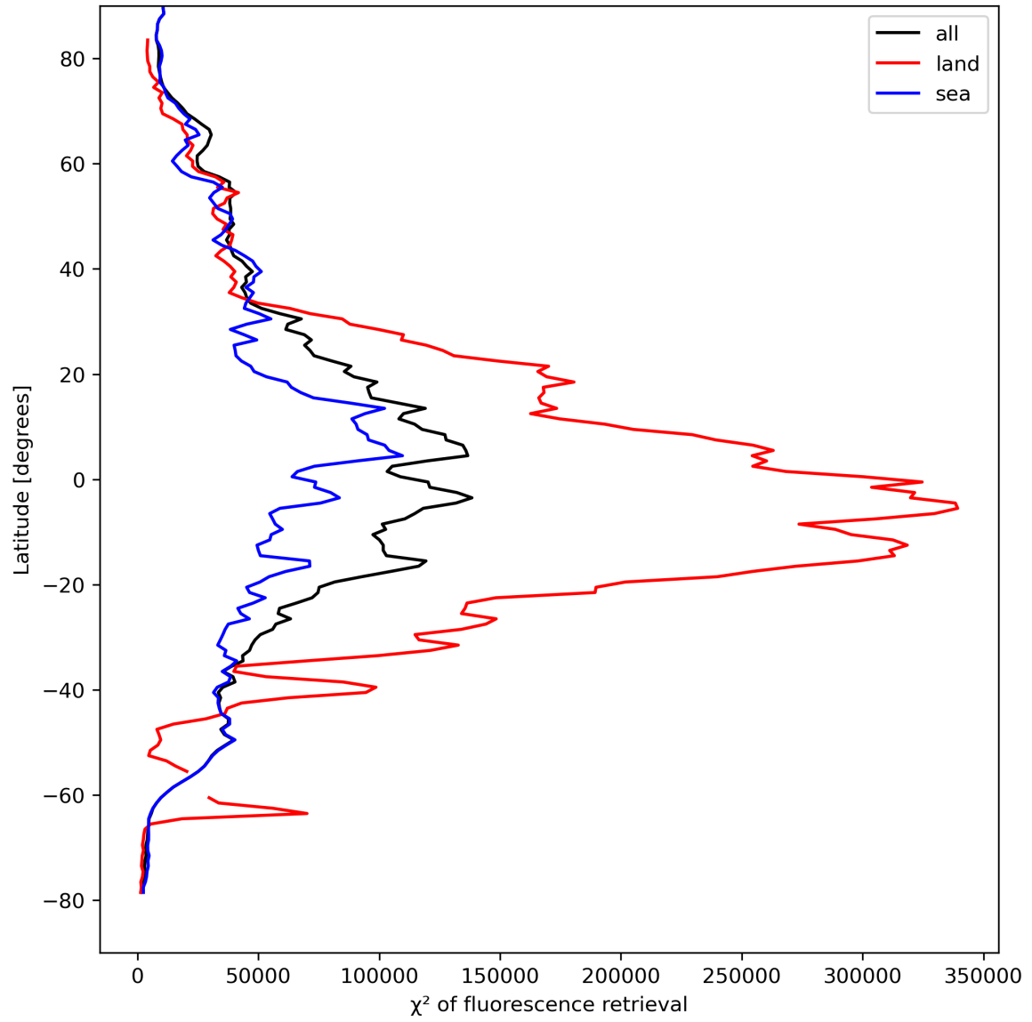
Figure 25: Zonal average of “ \chi^2 of fluorescence retrieval” for 2024-04-12 to 2024-04-14.
