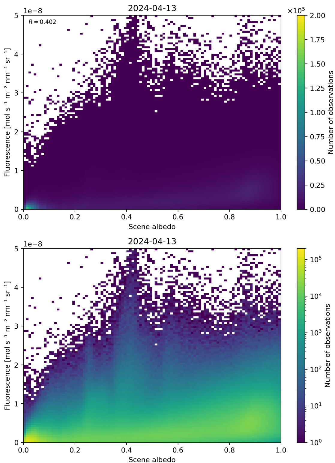
Figure 104: Scatter density plot of “Scene albedo” against “Fluorescence” for 2024-04-12 to 2024-04-14.
