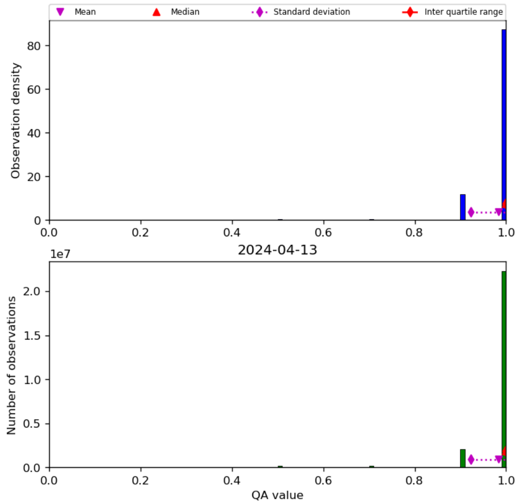
Figure 29: Histogram of “QA value” for 2024-04-12 to 2024-04-14
