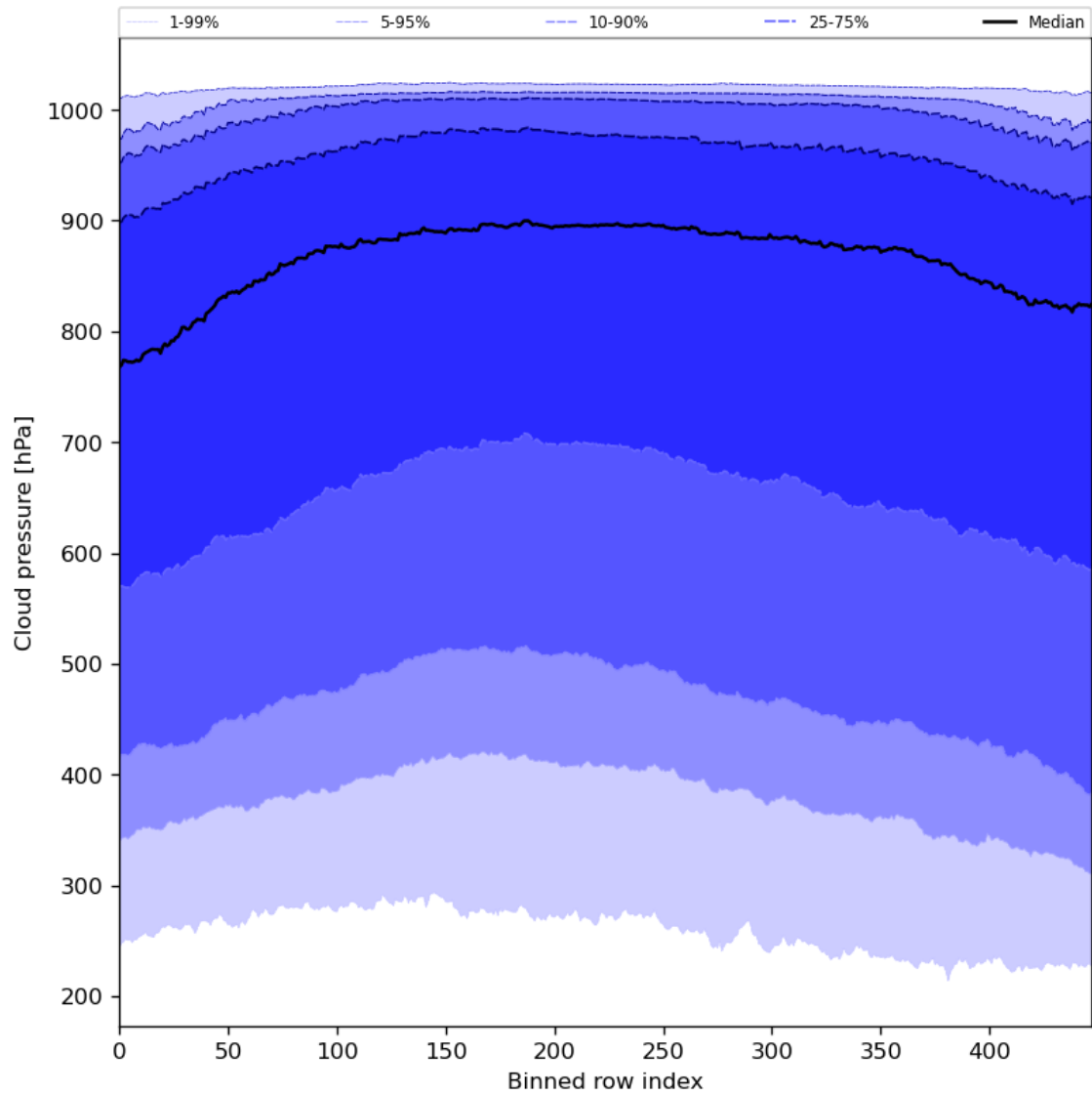
Figure 47: Along track statistics of “Cloud pressure” for 2024-04-12 to 2024-04-14
