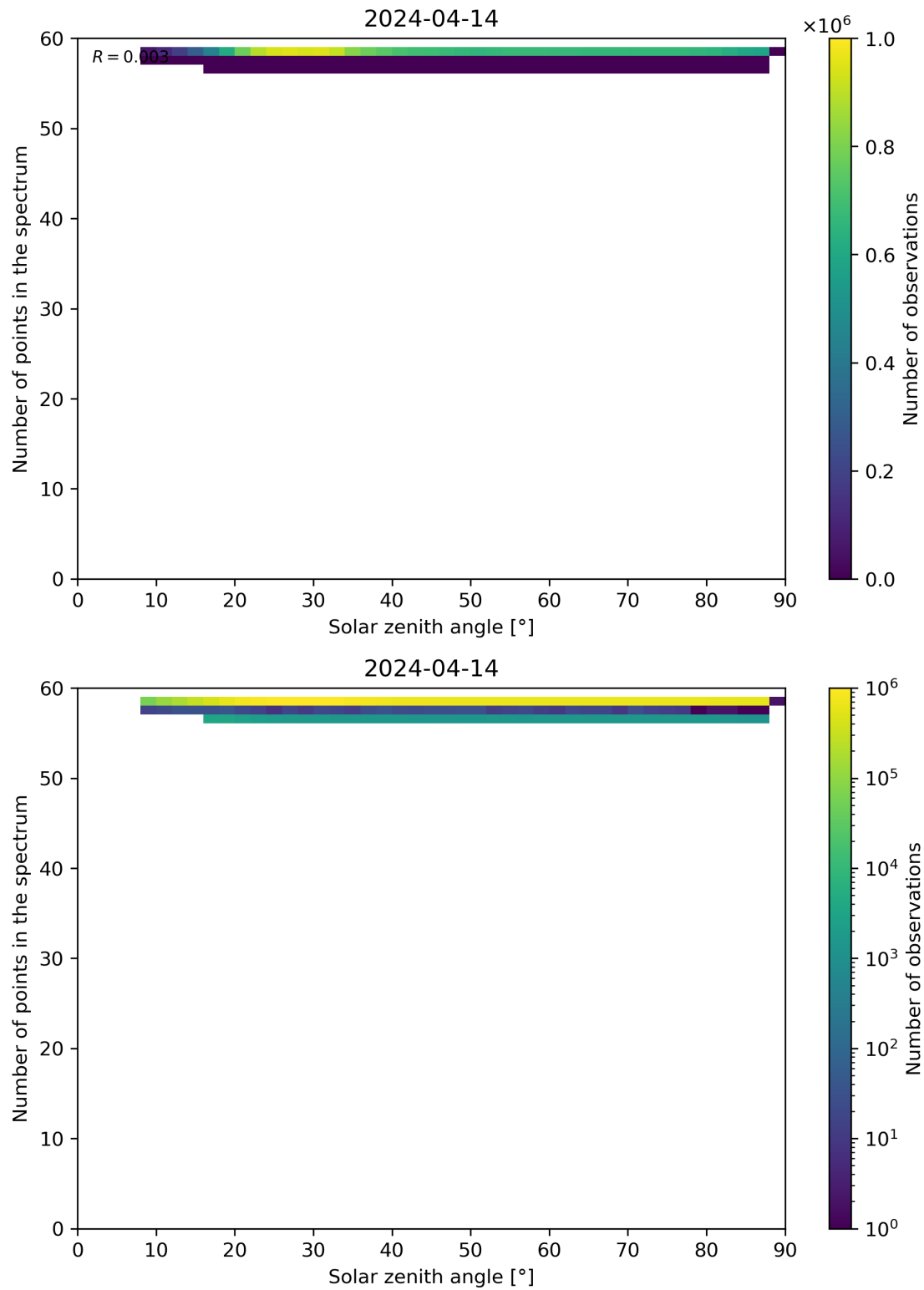
Figure 115: Scatter density plot of “Solar zenith angle” against “Number of points in the spectrum” for 2024-04-13 to 2024-04-15.
