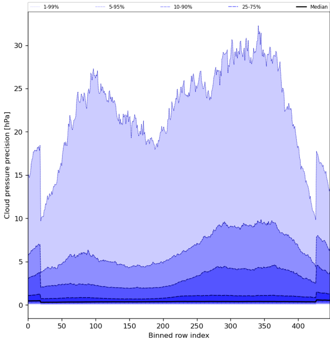
Figure 48: Along track statistics of “Cloud pressure precision” for 2024-04-13 to 2024-04-15
