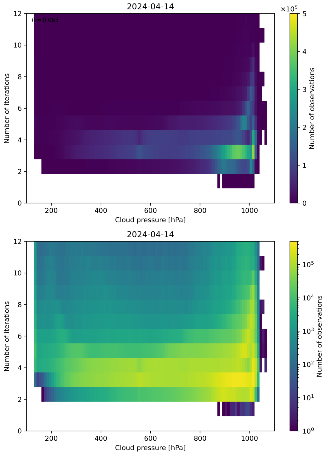
Figure 81: Scatter density plot of “Cloud pressure” against “Number of iterations” for 2024-04-13 to 2024-04-15.
