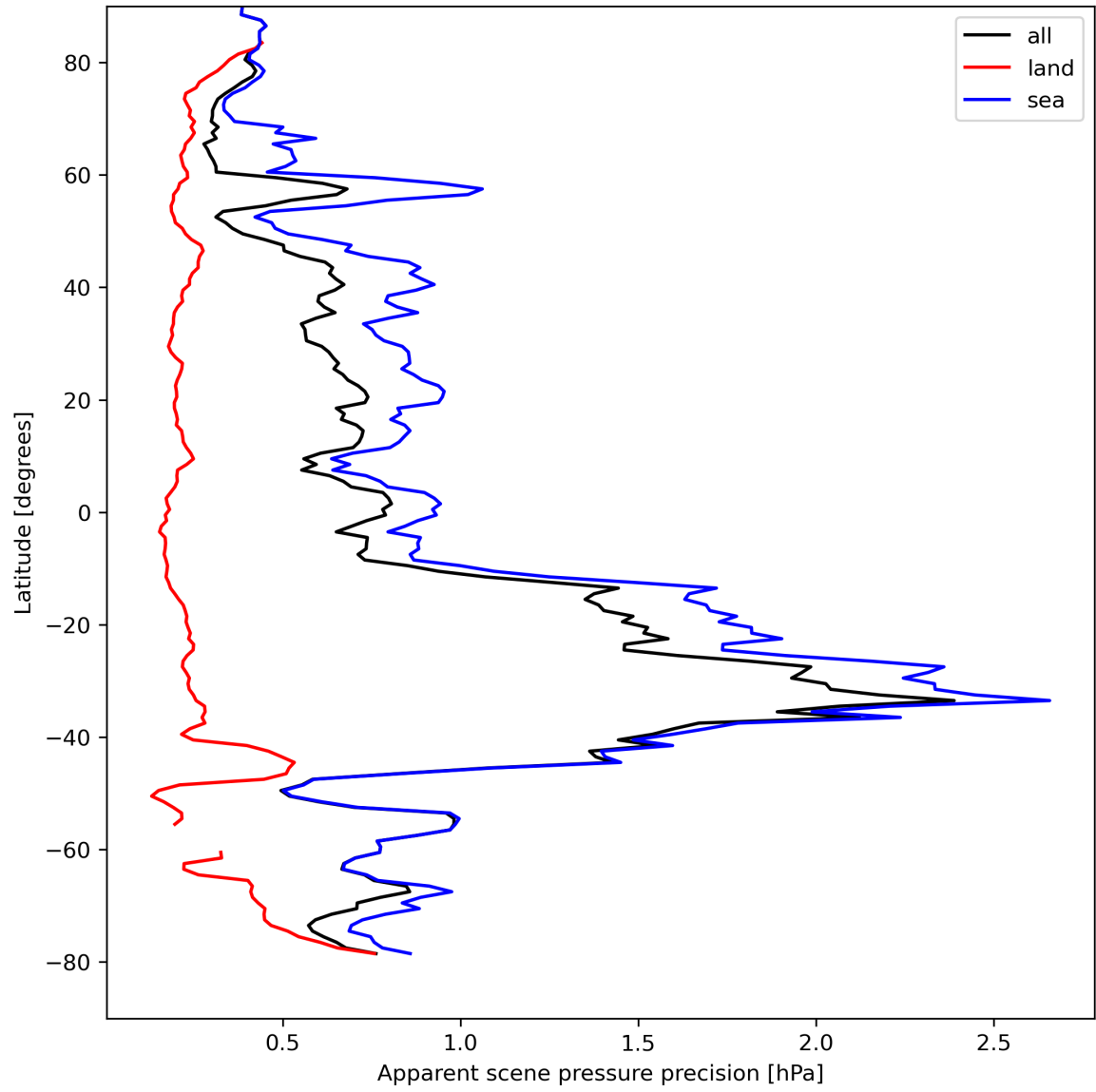
Figure 20: Zonal average of “Apparent scene pressure precision” for 2024-04-13 to 2024-04-15.
