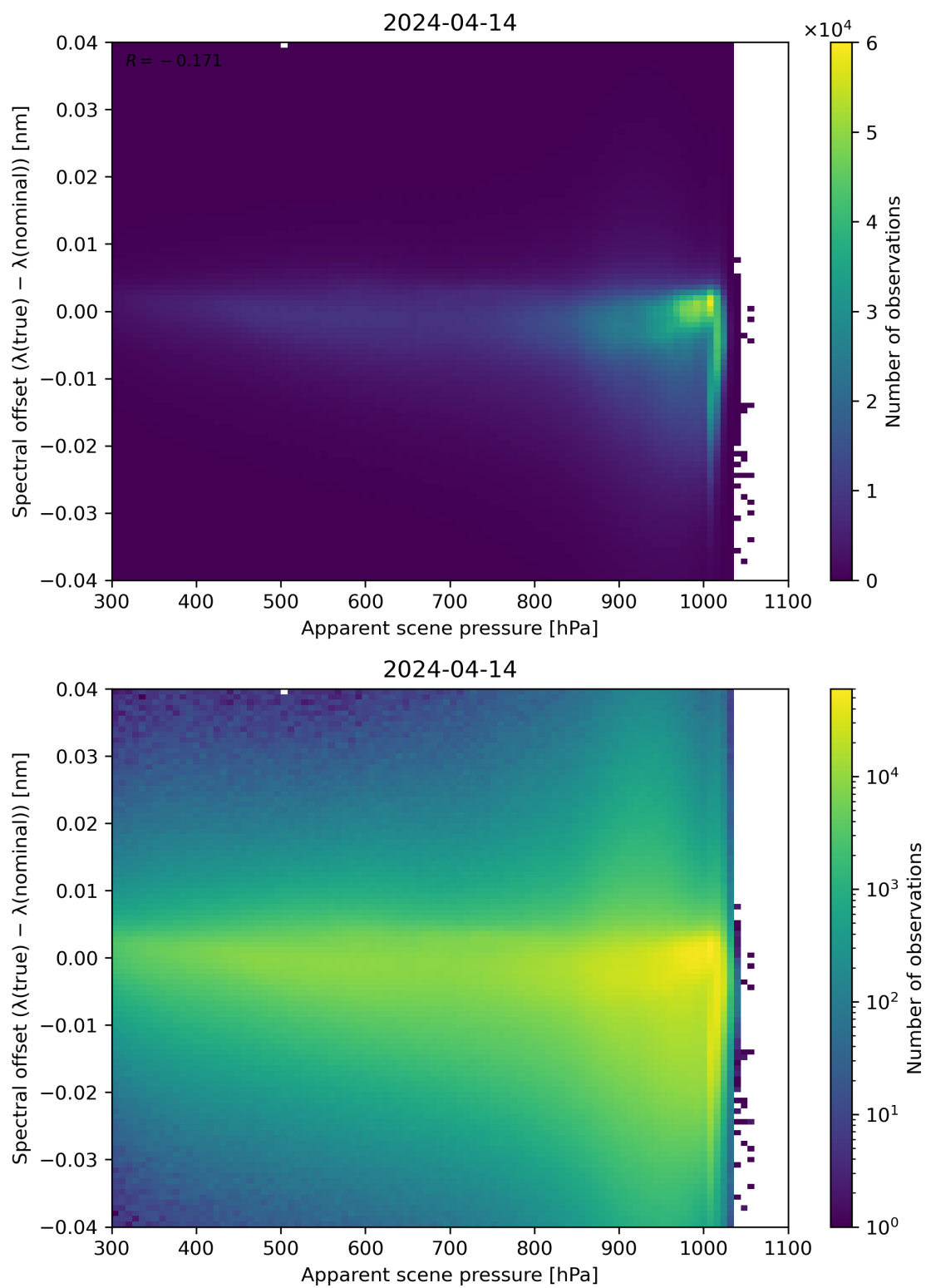
Figure 67: Scatter density plot of “Apparent scene pressure” against “Spectral offset ( \lambda(\text{true}) - \lambda(\text{nominal}) )” for 2024-04-13 to 2024-04-15.
