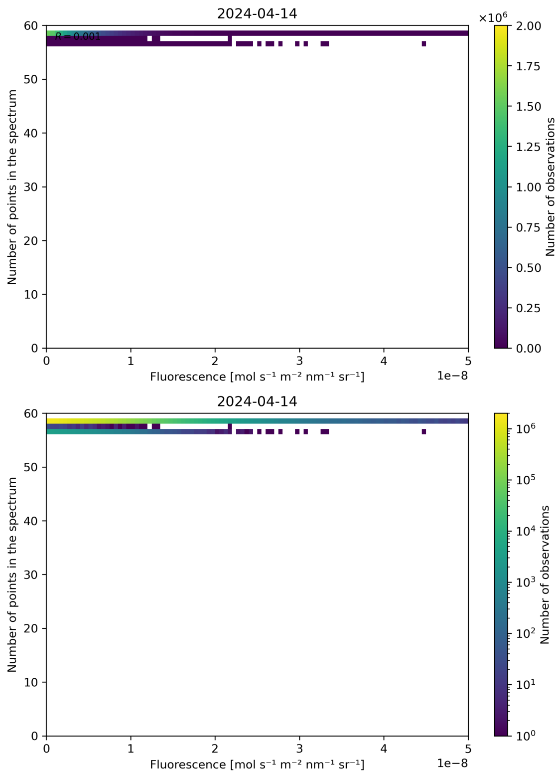
Figure 86: Scatter density plot of “Fluorescence” against “Number of points in the spectrum” for 2024-04-13 to 2024-04-15.
