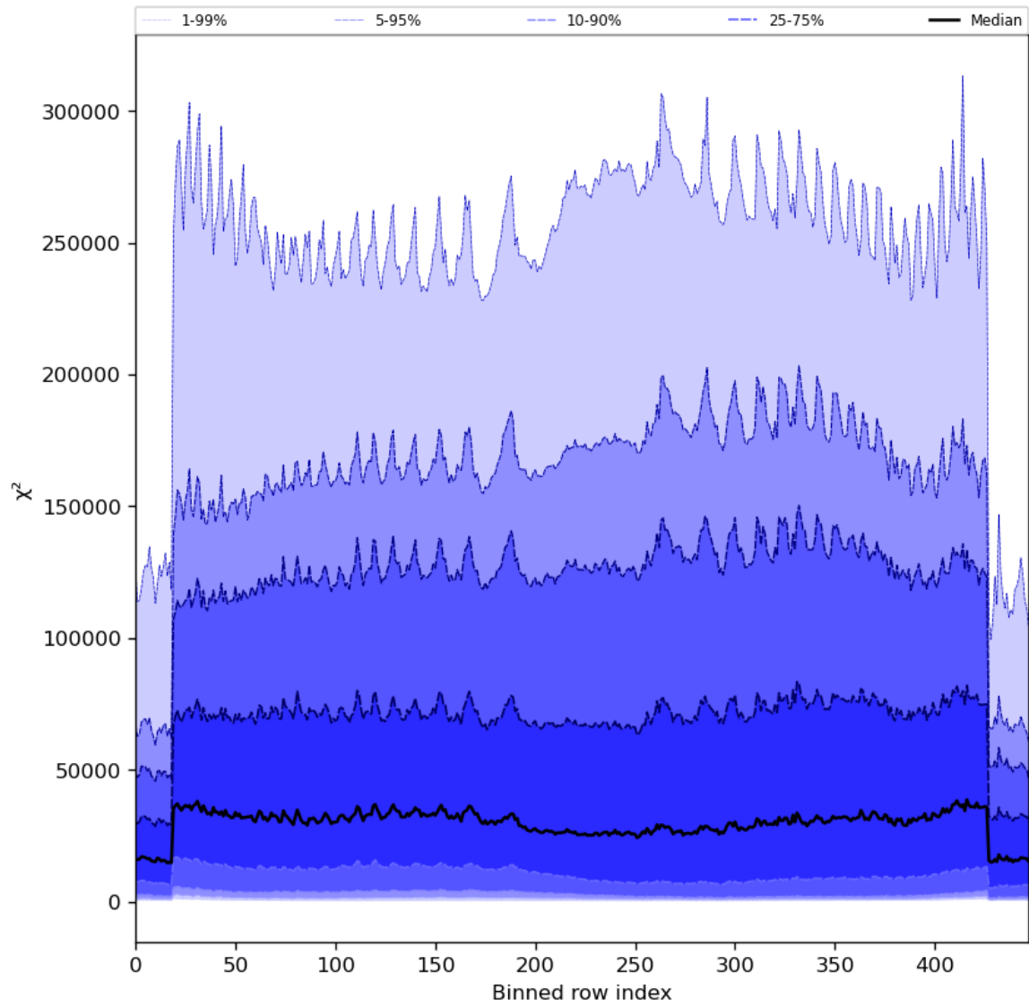
Figure 55: Along track statistics of “ \chi^2 ” for 2024-04-13 to 2024-04-15
