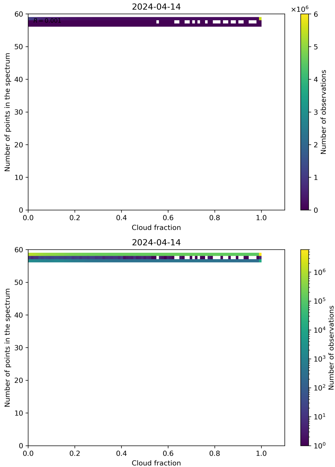
Figure 74: Scatter density plot of “Cloud fraction” against “Number of points in the spectrum” for 2024-04-13 to 2024-04-15.
