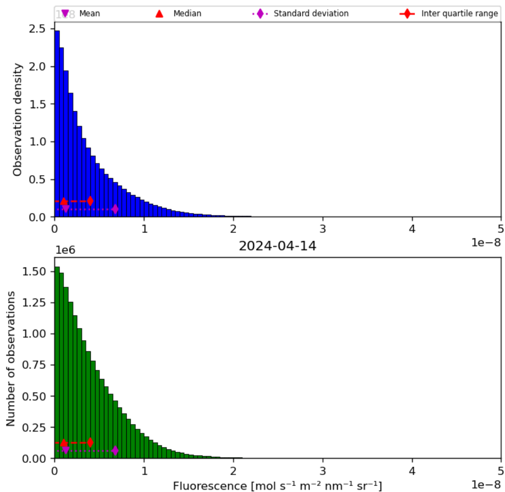
Figure 40: Histogram of “Fluorescence” for 2024-04-13 to 2024-04-15
