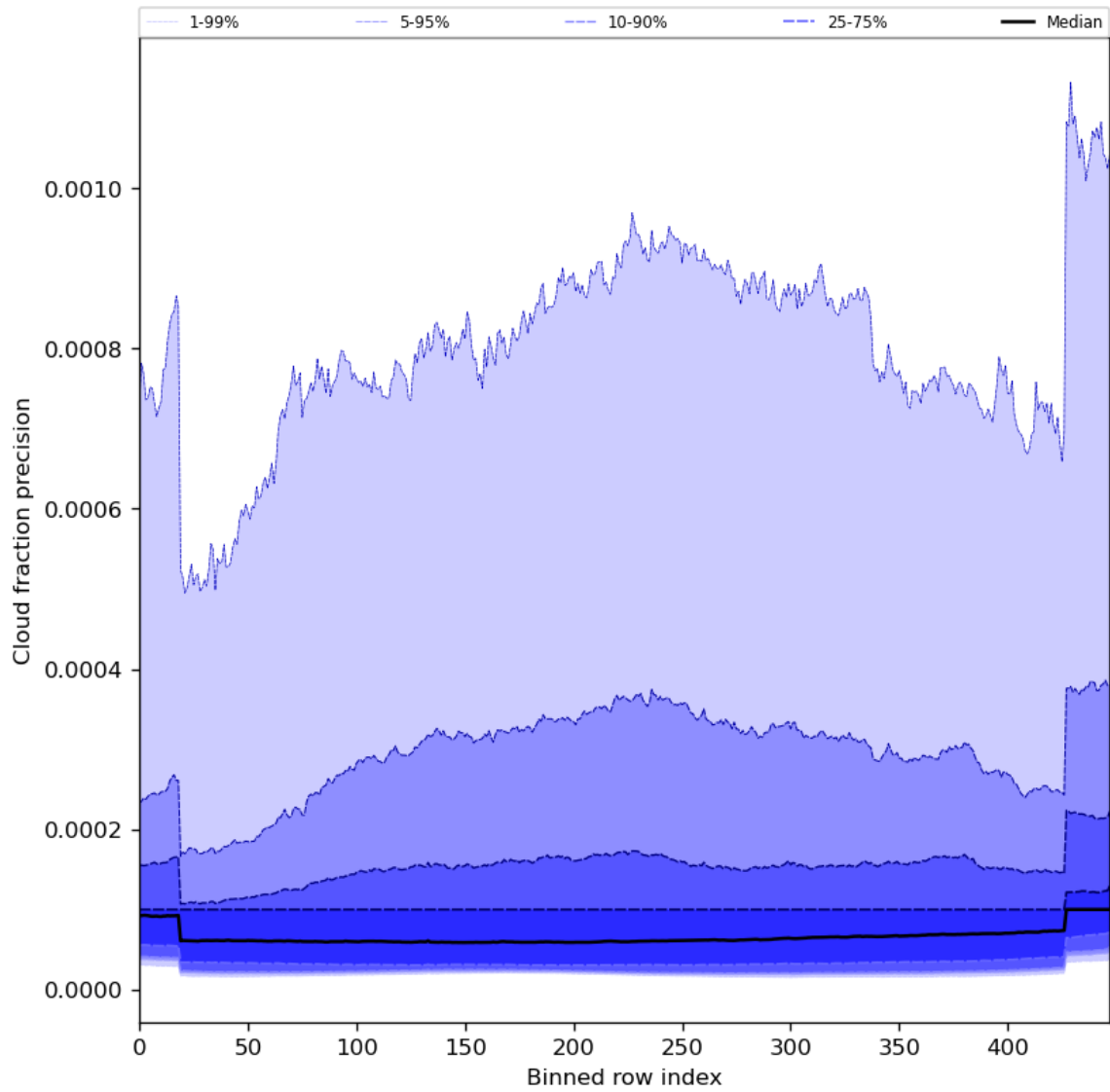
Figure 50: Along track statistics of “Cloud fraction precision” for 2024-04-13 to 2024-04-15
