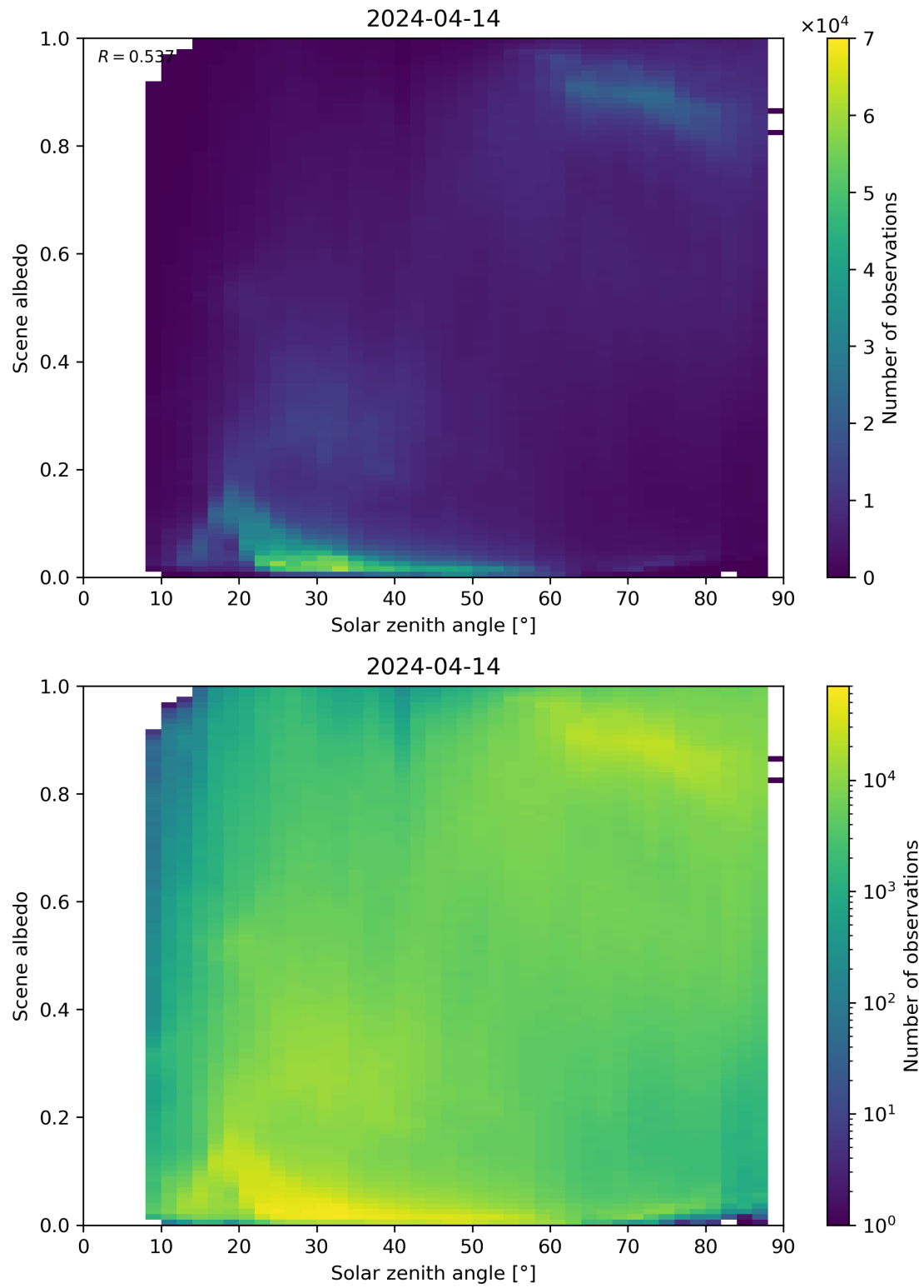
Figure 116: Scatter density plot of “Solar zenith angle” against “Scene albedo” for 2024-04-13 to 2024-04-15.
