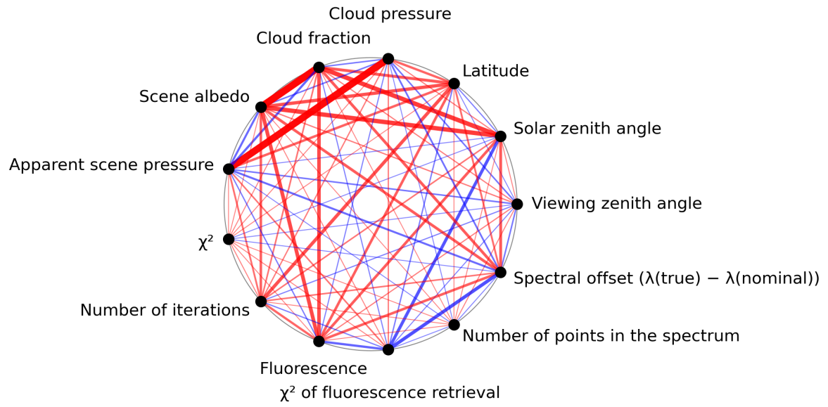
Figure 1: Map of correlation graph for 2024-04-13 to 2024-04-15.
