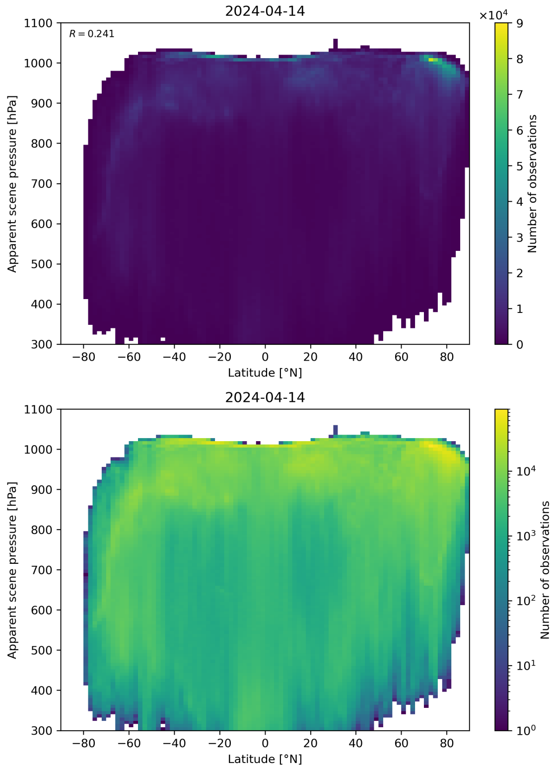
Figure 88: Scatter density plot of “Latitude” against “Apparent scene pressure” for 2024-04-13 to 2024-04-15.
