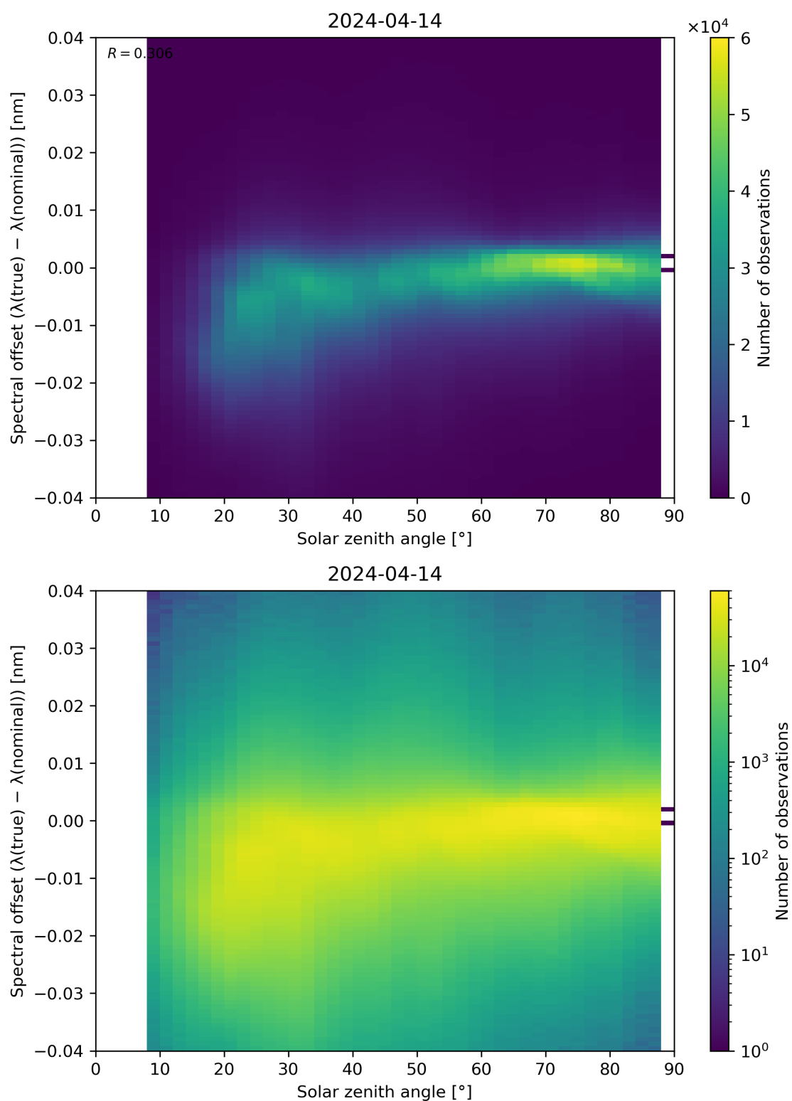
Figure 117: Scatter density plot of “Solar zenith angle” against “Spectral offset ( \lambda(\text{true}) - \lambda(\text{nominal}) )” for 2024-04-13 to 2024-04-15.
