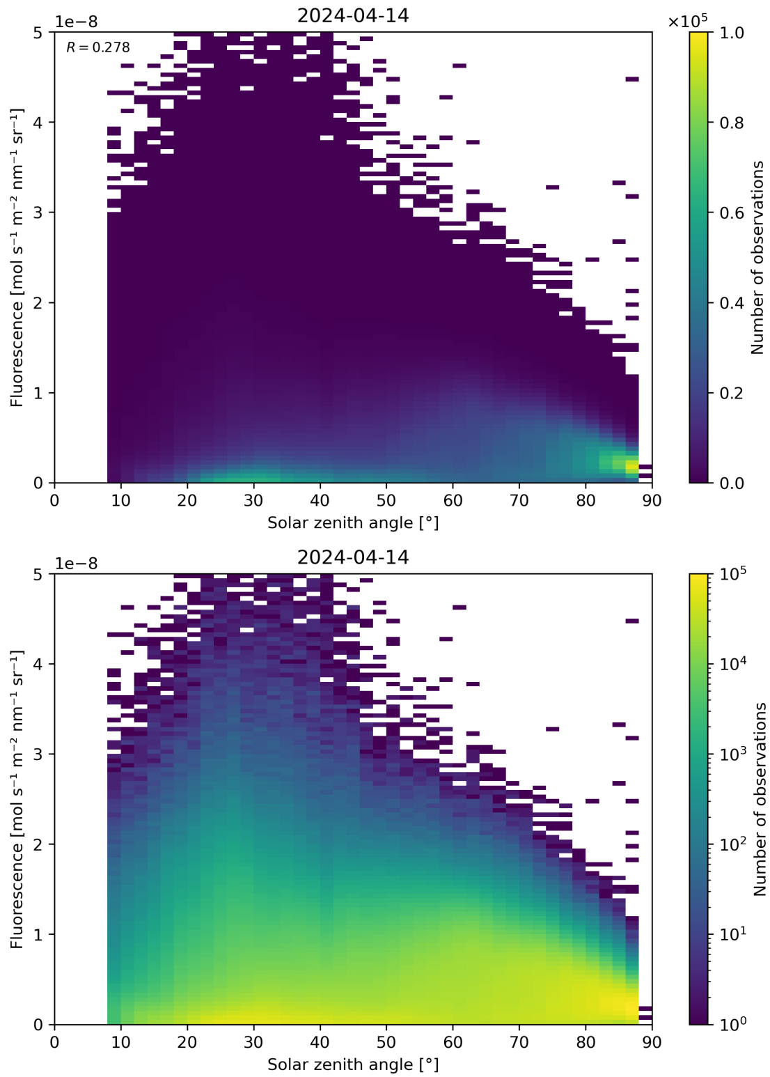
Figure 112: Scatter density plot of “Solar zenith angle” against “Fluorescence” for 2024-04-13 to 2024-04-15.
