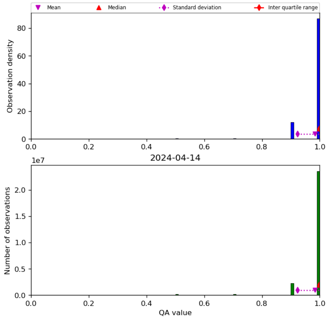
Figure 29: Histogram of “QA value” for 2024-04-13 to 2024-04-15
