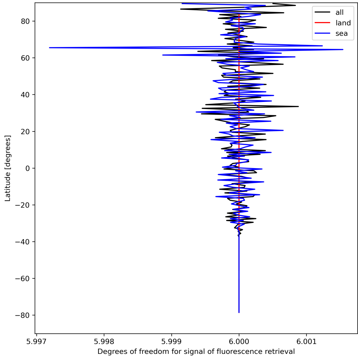
Figure 26: Zonal average of “Degrees of freedom for signal of fluorescence retrieval” for 2024-04-13 to 2024-04-15.
