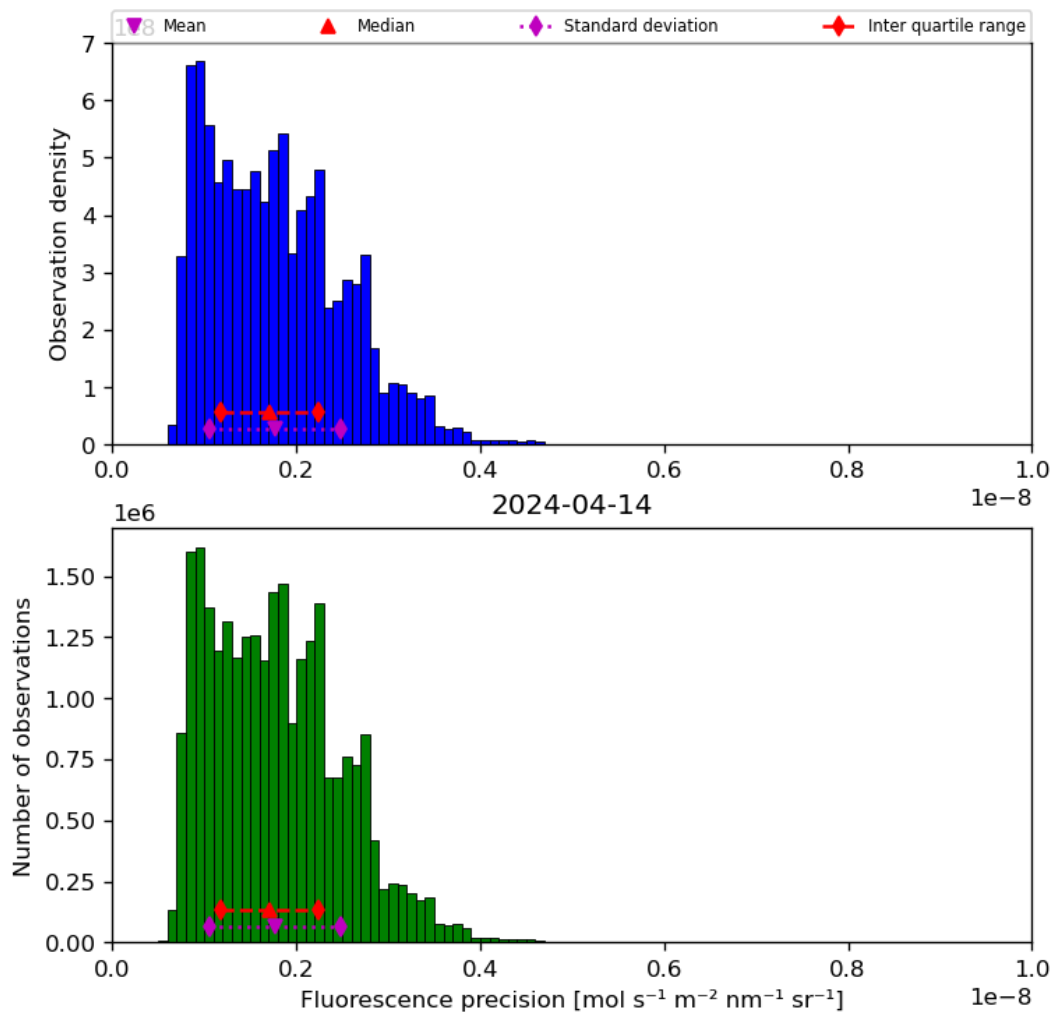
Figure 41: Histogram of “Fluorescence precision” for 2024-04-13 to 2024-04-15
