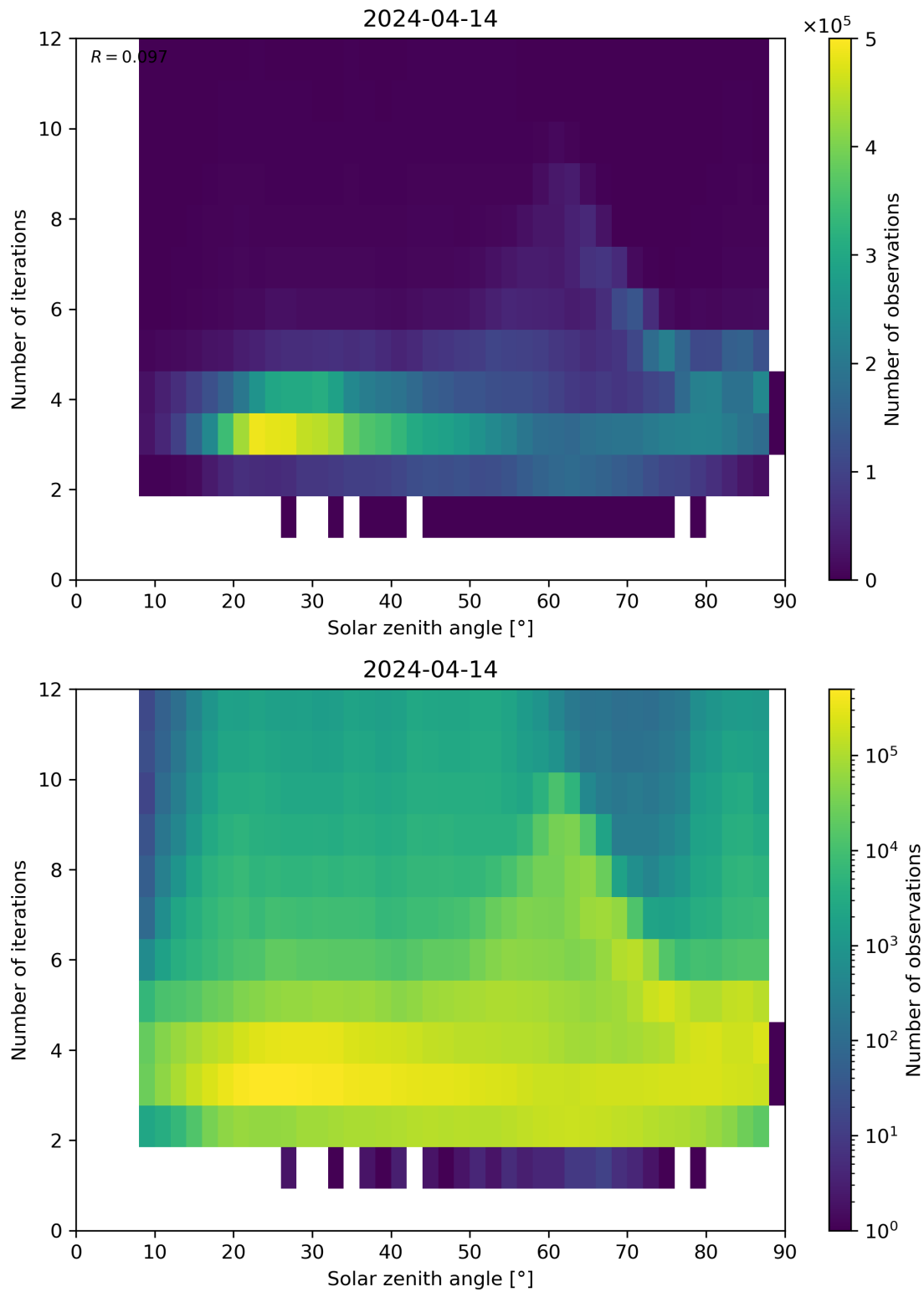
Figure 114: Scatter density plot of “Solar zenith angle” against “Number of iterations” for 2024-04-13 to 2024-04-15.
