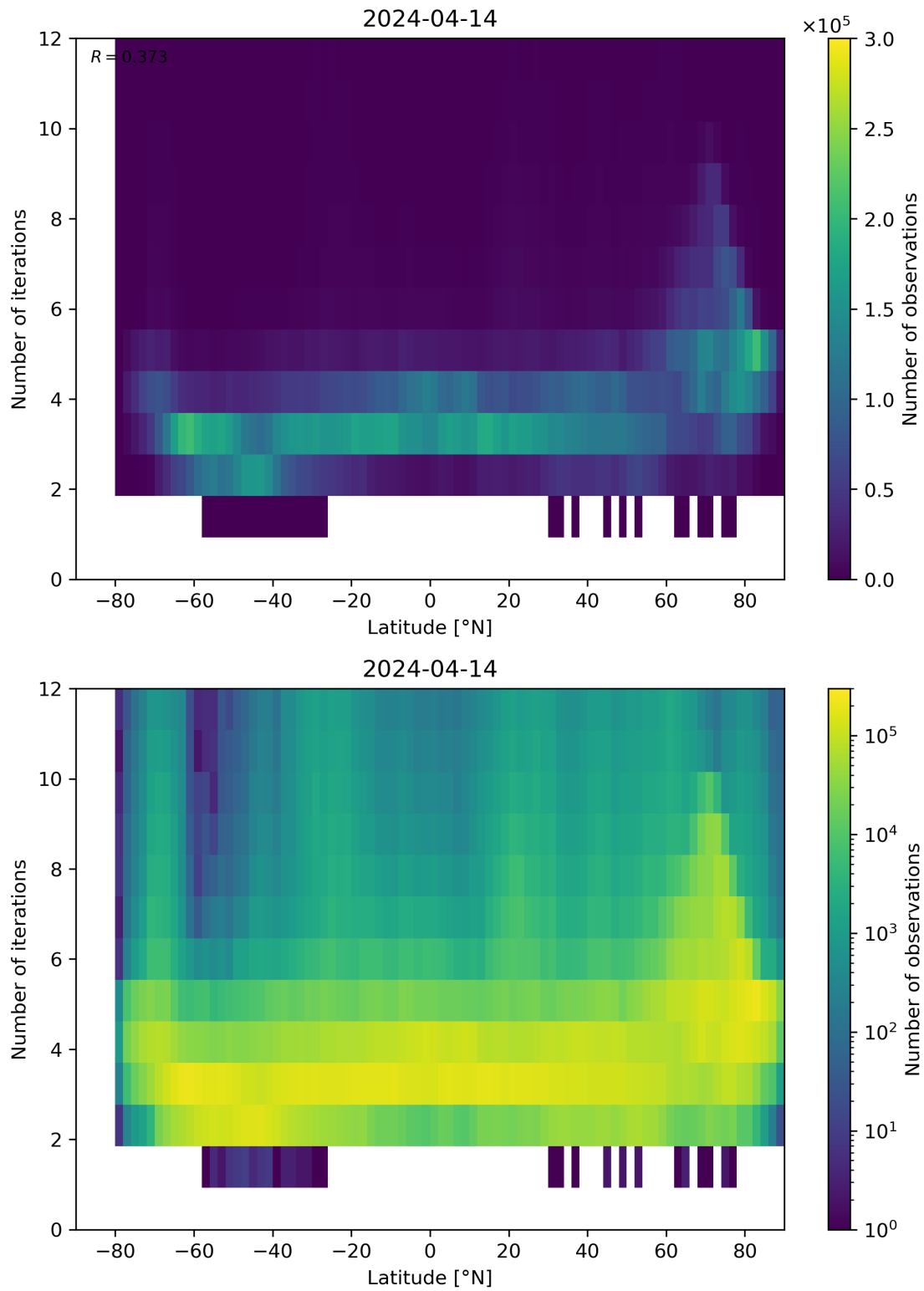
Figure 93: Scatter density plot of “Latitude” against “Number of iterations” for 2024-04-13 to 2024-04-15.
