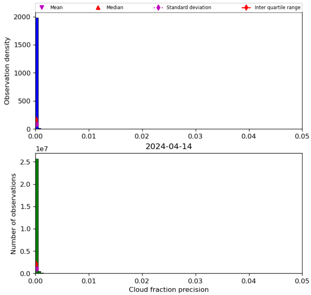
Figure 33: Histogram of “Cloud fraction precision” for 2024-04-13 to 2024-04-15
