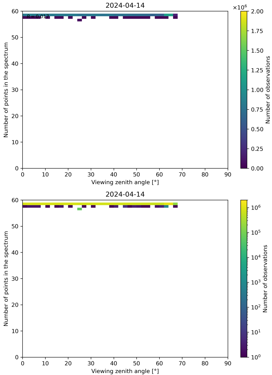
Figure 125: Scatter density plot of “Viewing zenith angle” against “Number of points in the spectrum” for 2024-04-13 to 2024-04-15.
