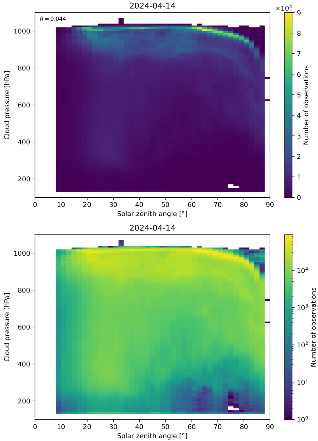
Figure 111: Scatter density plot of “Solar zenith angle” against “Cloud pressure” for 2024-04-13 to 2024-04-15.
