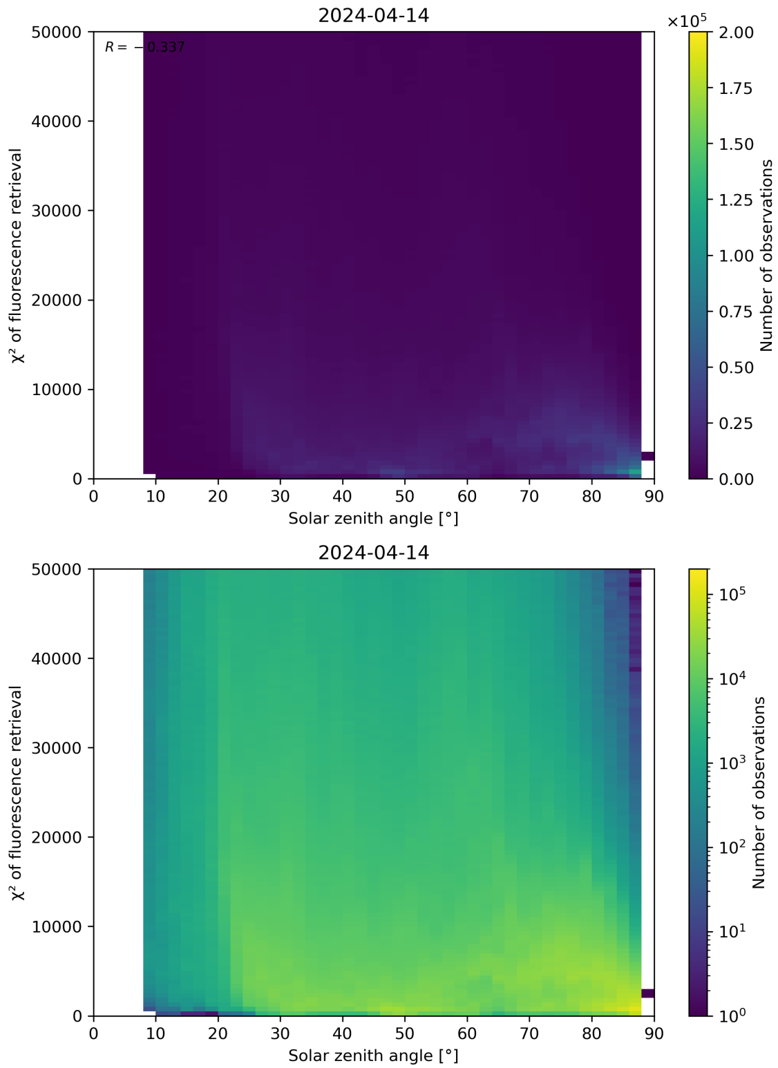
Figure 109: Scatter density plot of “Solar zenith angle” against “ \chi^2 of fluorescence retrieval” for 2024-04-13 to 2024-04-15.
