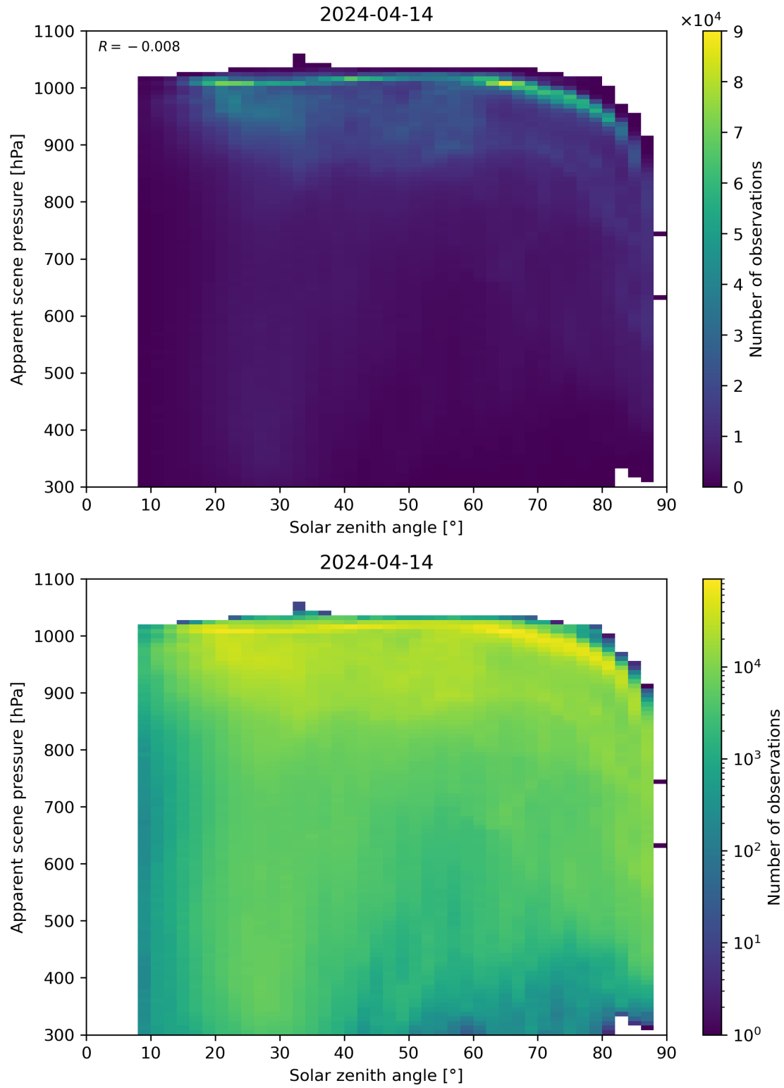
Figure 108: Scatter density plot of “Solar zenith angle” against “Apparent scene pressure” for 2024-04-13 to 2024-04-15.
