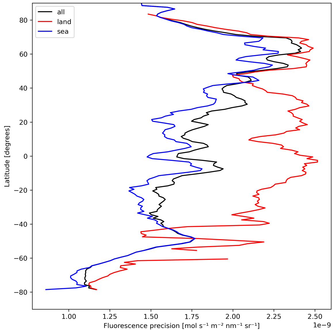
Figure 24: Zonal average of “Fluorescence precision” for 2024-04-13 to 2024-04-15.
