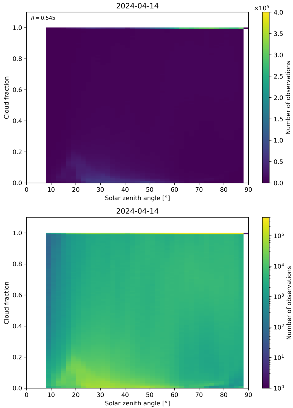
Figure 110: Scatter density plot of “Solar zenith angle” against “Cloud fraction” for 2024-04-13 to 2024-04-15.
