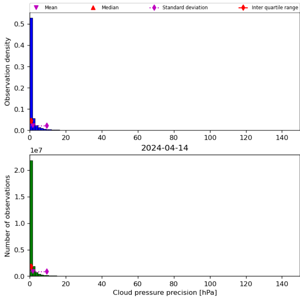
Figure 31: Histogram of “Cloud pressure precision” for 2024-04-13 to 2024-04-15
