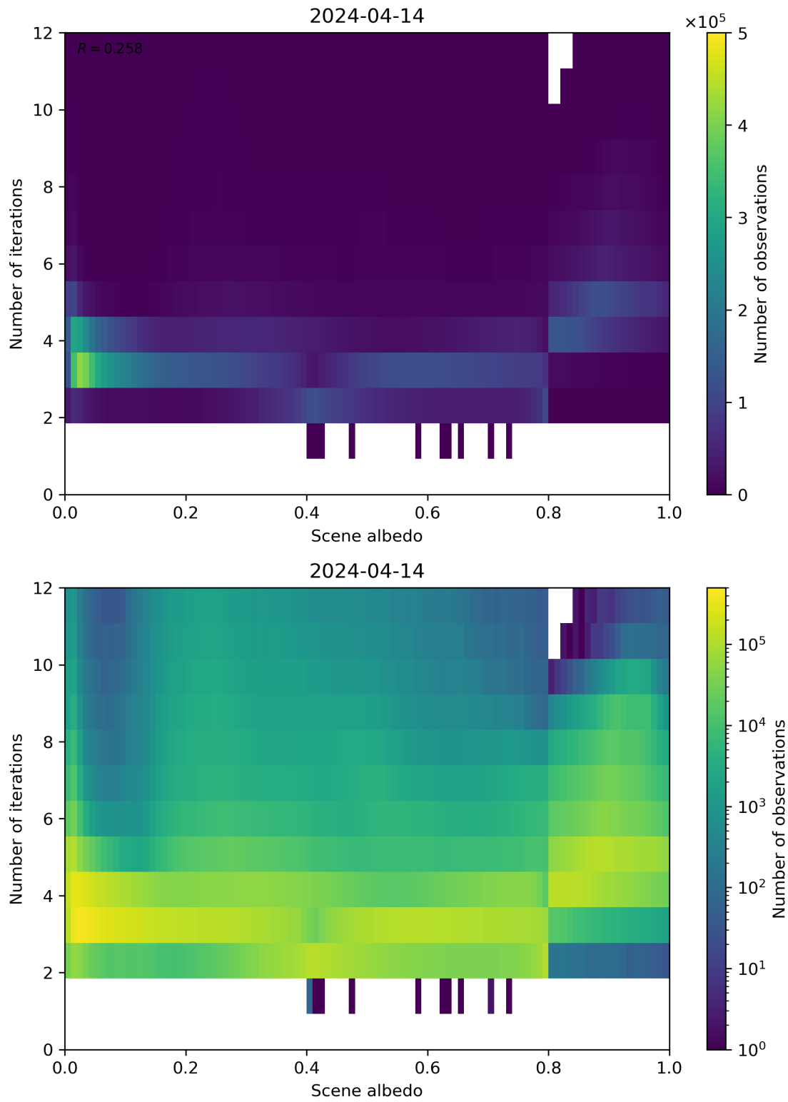
Figure 105: Scatter density plot of “Scene albedo” against “Number of iterations” for 2024-04-13 to 2024-04-15.
