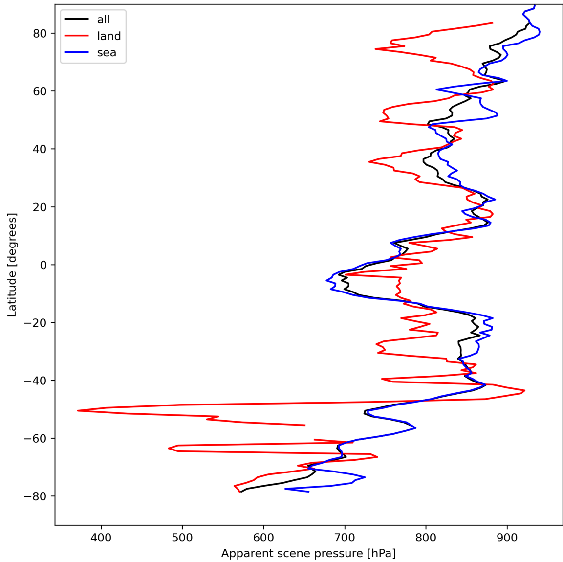
Figure 19: Zonal average of “Apparent scene pressure” for 2024-04-13 to 2024-04-15.
