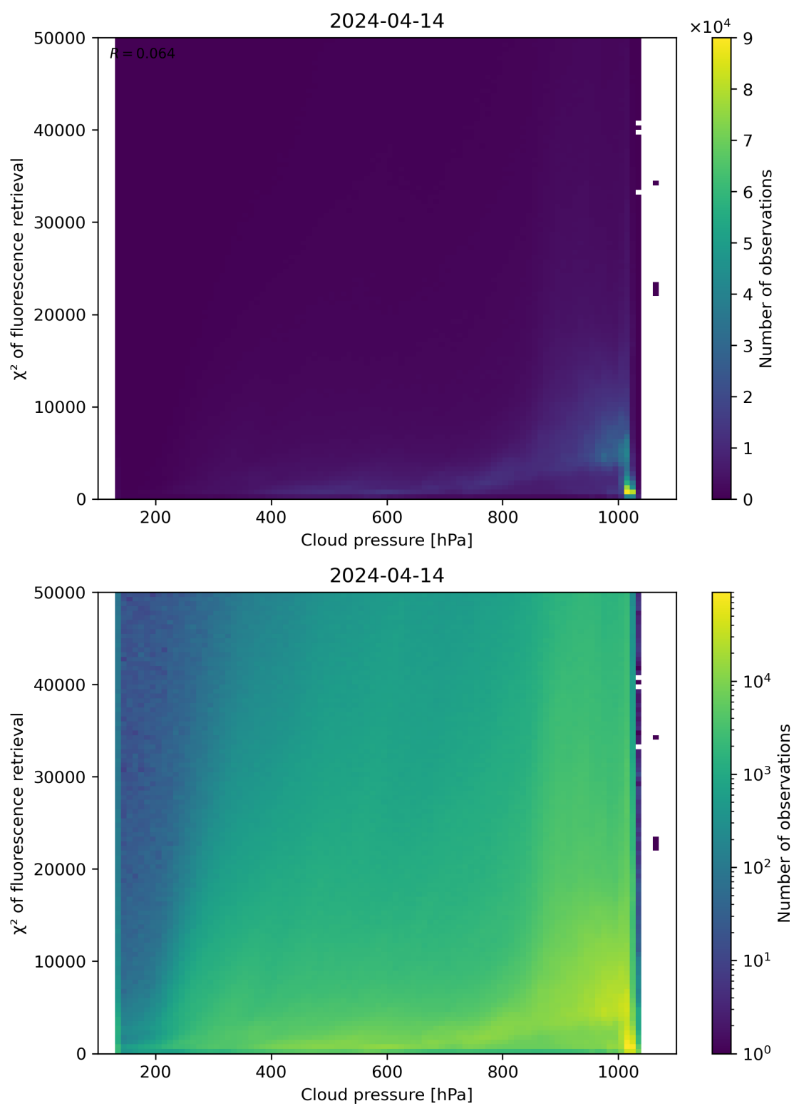
Figure 78: Scatter density plot of “Cloud pressure” against “ \chi^2 of fluorescence retrieval” for 2024-04-13 to 2024-04-15.
