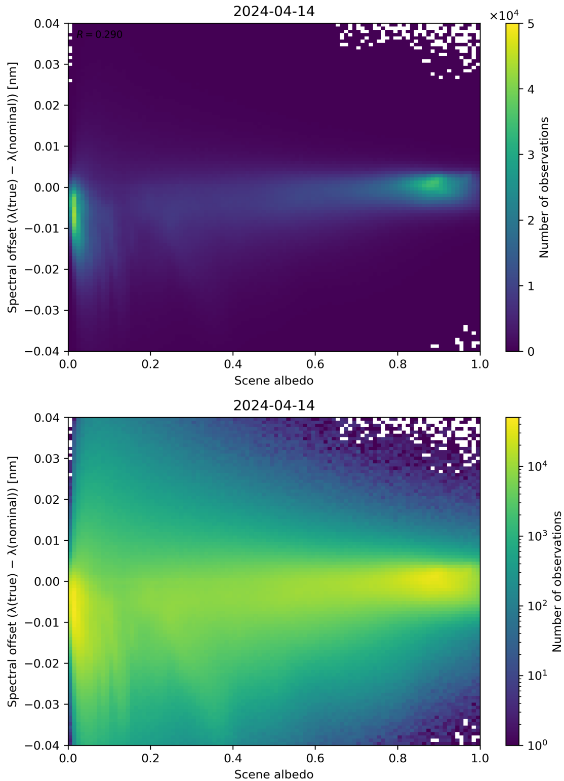
Figure 107: Scatter density plot of “Scene albedo” against “Spectral offset ( \lambda(\text{true}) - \lambda(\text{nominal}) )” for 2024-04-13 to 2024-04-15.
