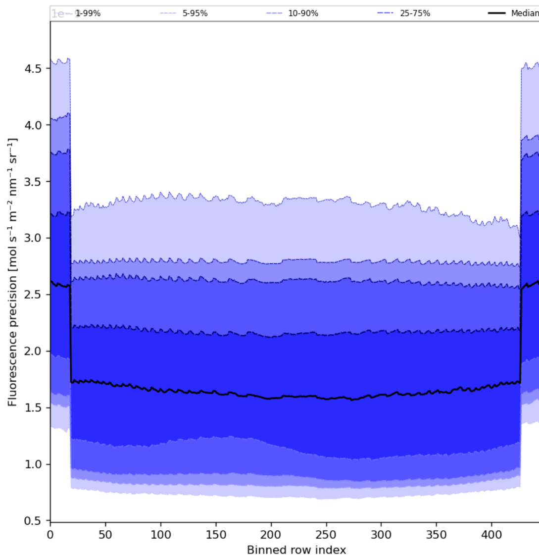
Figure 58: Along track statistics of “Fluorescence precision” for 2024-04-13 to 2024-04-15
