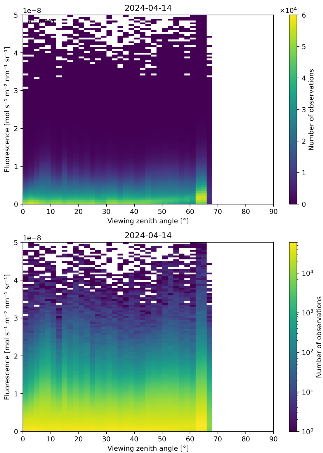
Figure 122: Scatter density plot of “Viewing zenith angle” against “Fluorescence” for 2024-04-13 to 2024-04-15.
