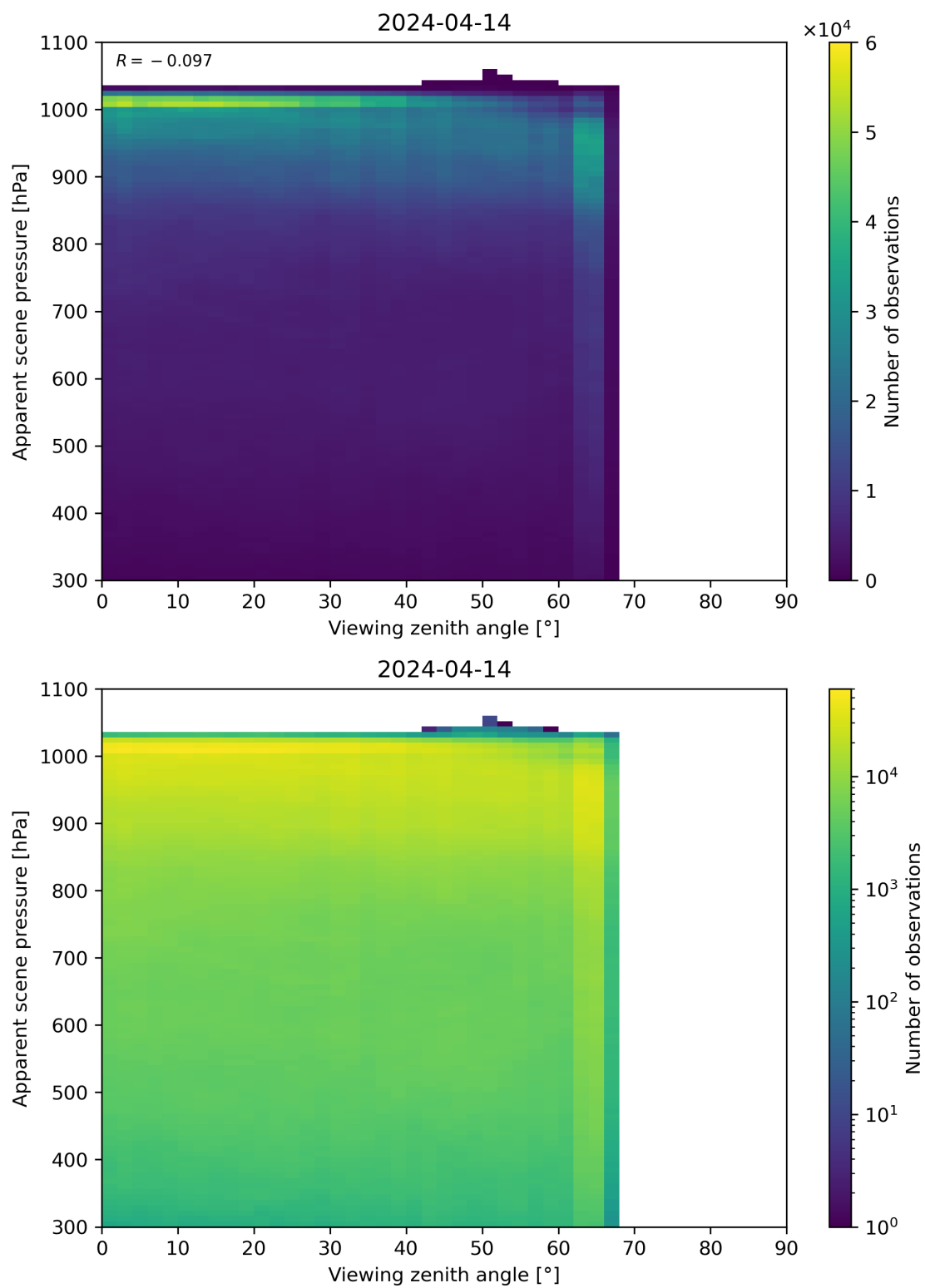
Figure 118: Scatter density plot of “Viewing zenith angle” against “Apparent scene pressure” for 2024-04-13 to 2024-04-15.
