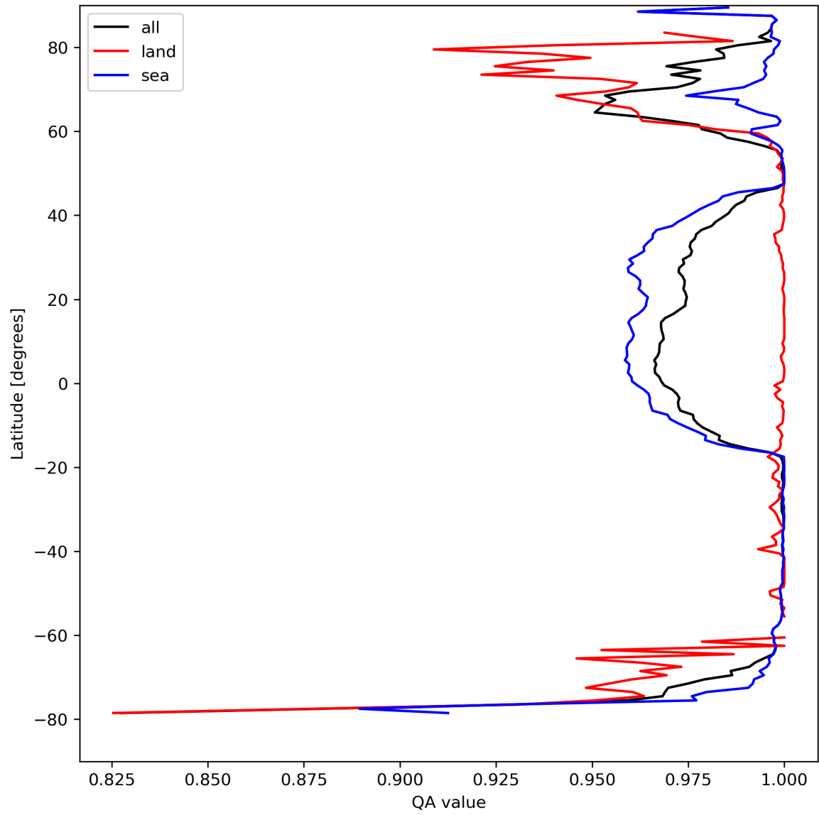
Figure 12: Zonal average of “QA value” for 2024-04-13 to 2024-04-15.
