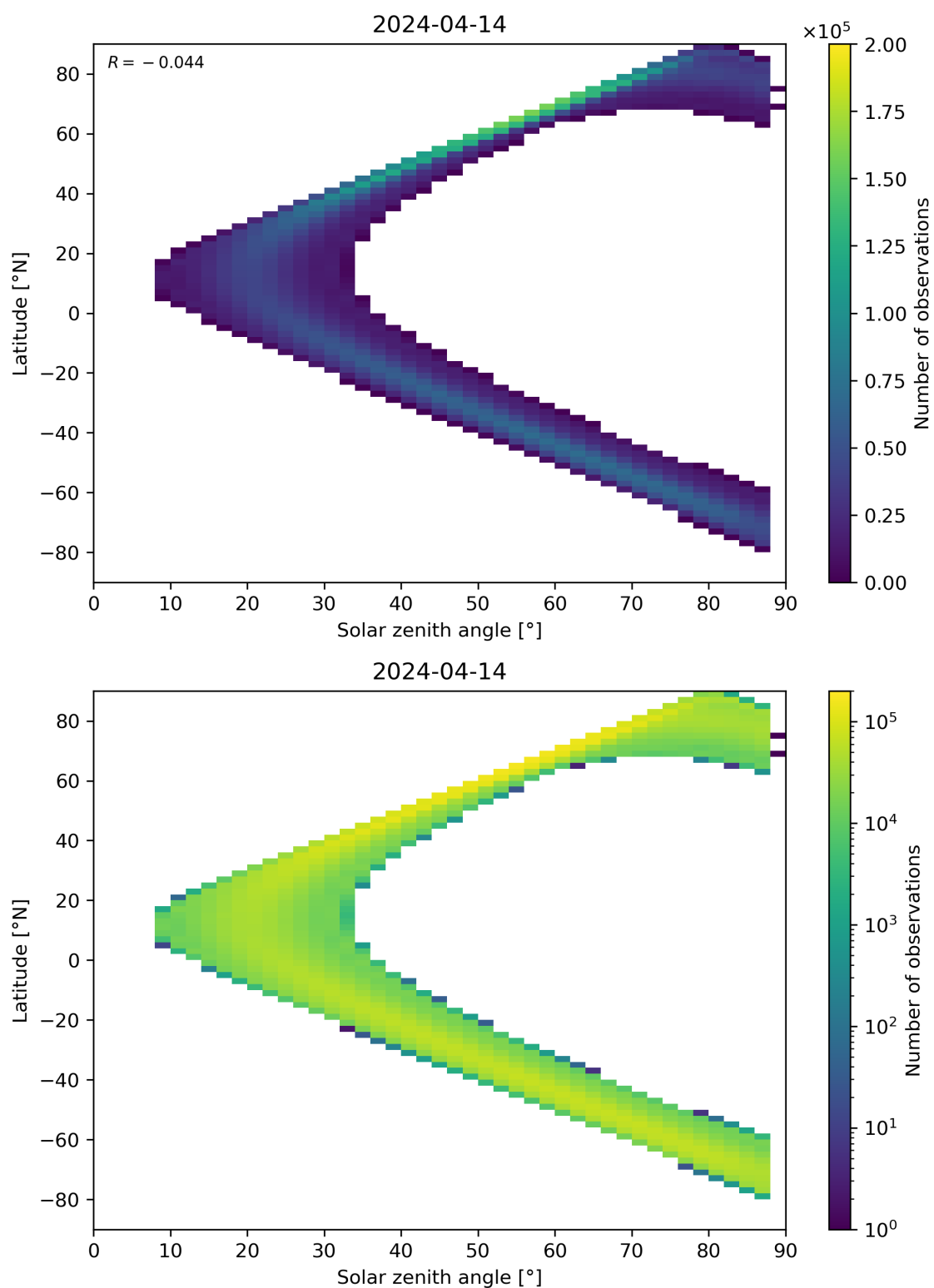
Figure 113: Scatter density plot of “Solar zenith angle” against “Latitude” for 2024-04-13 to 2024-04-15.
