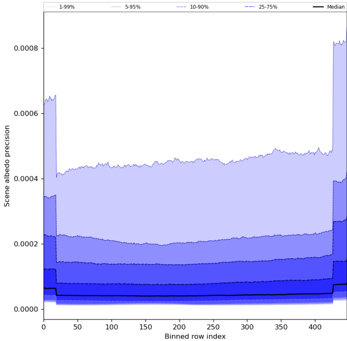
Figure 52: Along track statistics of “Scene albedo precision” for 2024-04-13 to 2024-04-15
