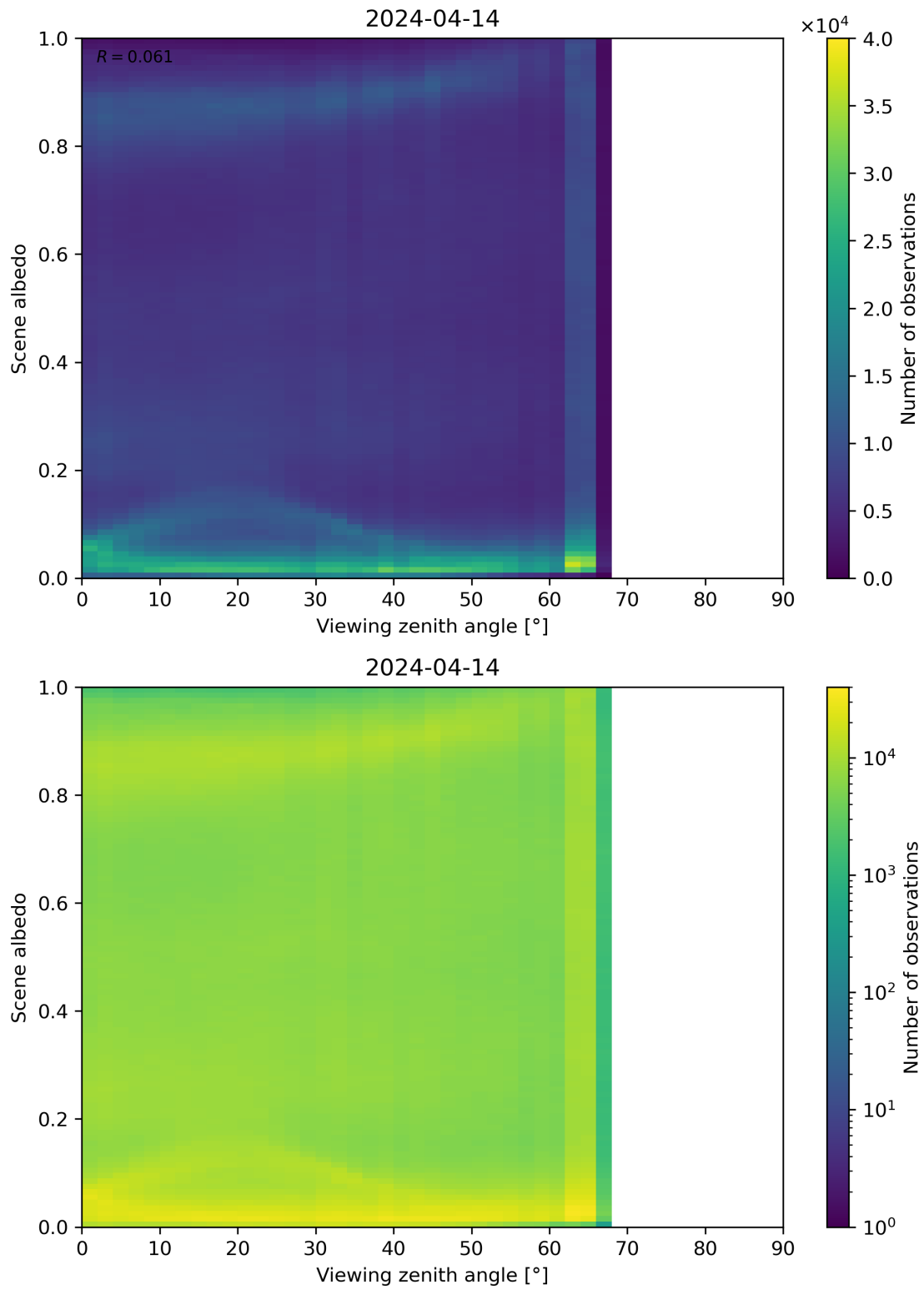
Figure 126: Scatter density plot of “Viewing zenith angle” against “Scene albedo” for 2024-04-13 to 2024-04-15.
