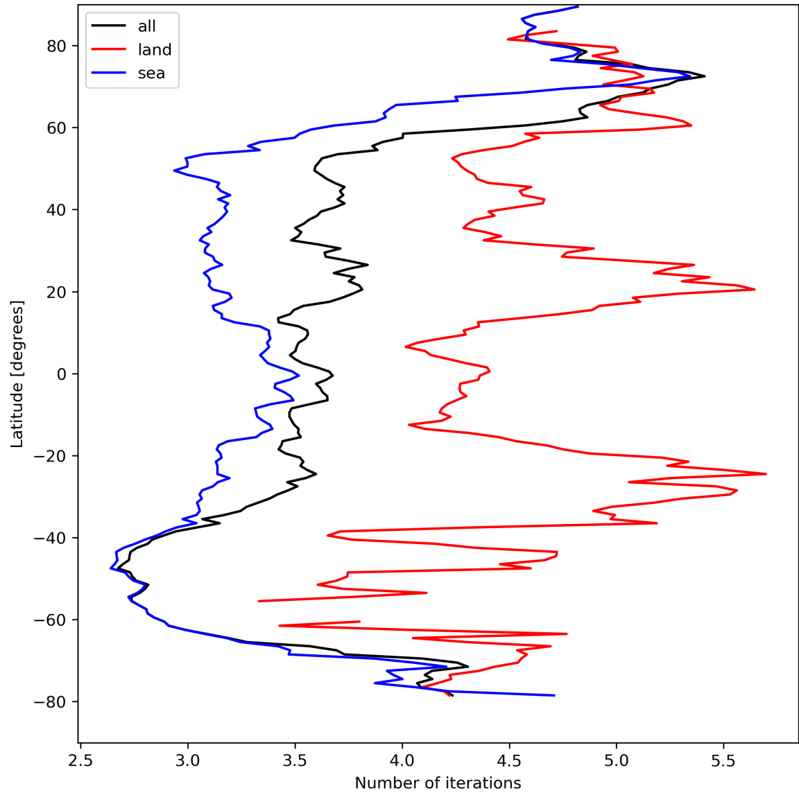
Figure 22: Zonal average of “Number of iterations” for 2024-04-13 to 2024-04-15.
