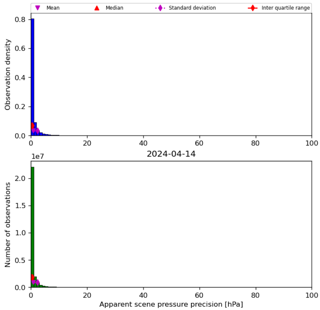
Figure 37: Histogram of “Apparent scene pressure precision” for 2024-04-13 to 2024-04-15
