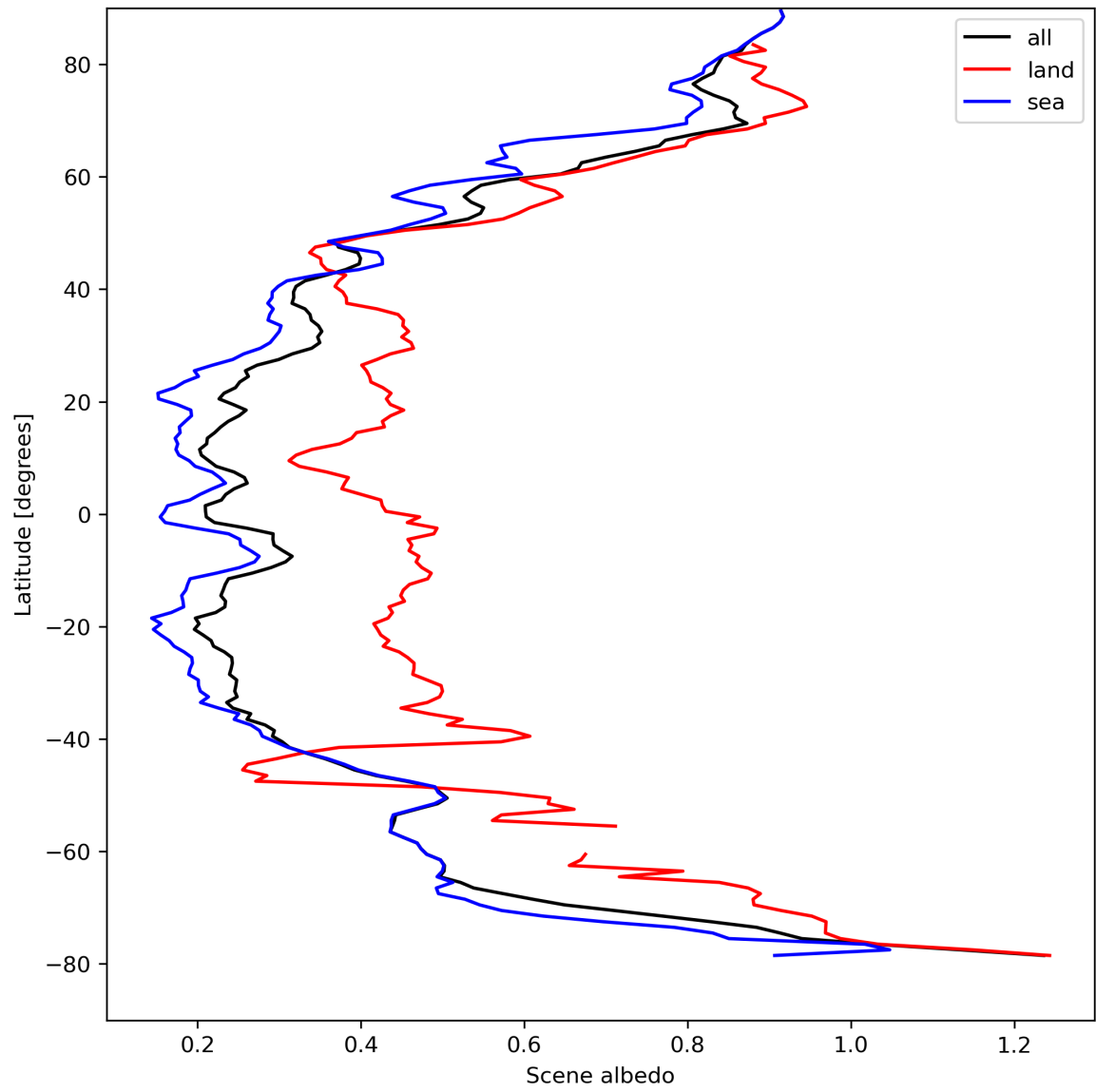
Figure 17: Zonal average of “Scene albedo” for 2024-04-13 to 2024-04-15.
