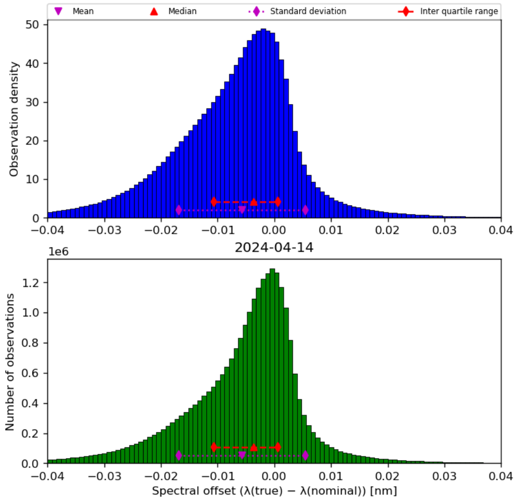
Figure 45: Histogram of “Spectral offset ( \lambda(\text{true}) - \lambda(\text{nominal}) )” for 2024-04-13 to 2024-04-15
