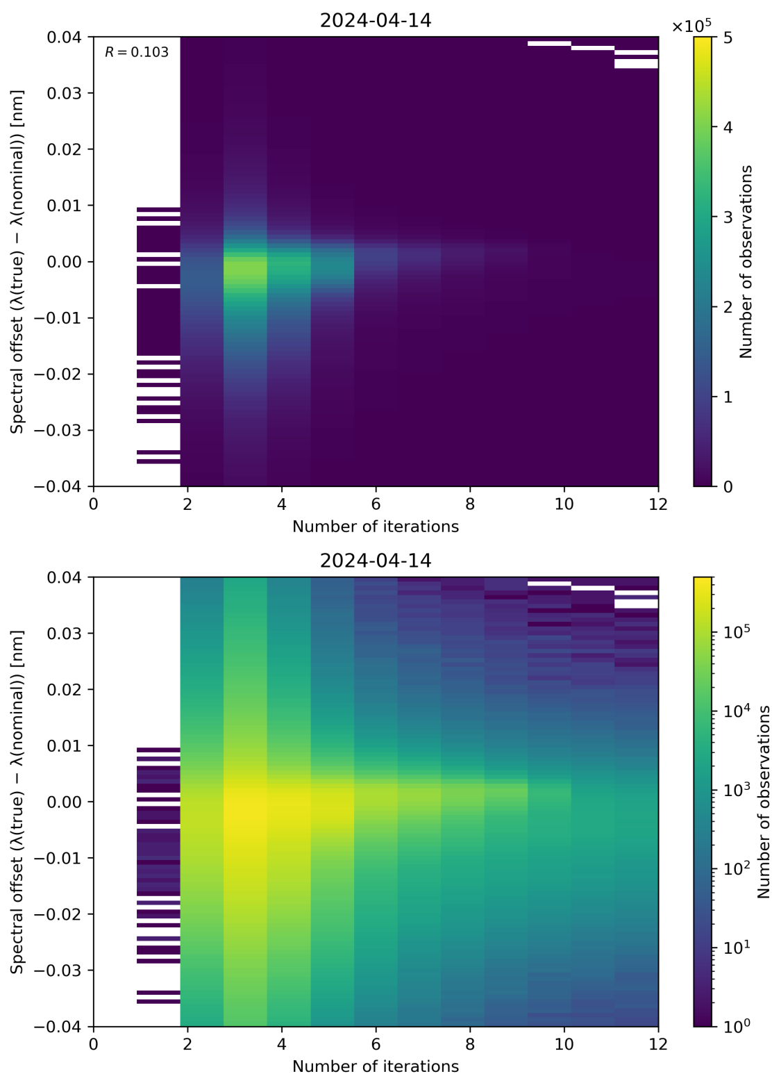
Figure 100: Scatter density plot of “Number of iterations” against “Spectral offset ( \lambda(\text{true}) - \lambda(\text{nominal}) )” for 2024-04-13 to 2024-04-15.
