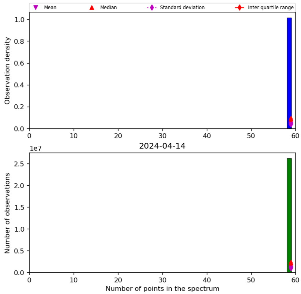
Figure 44: Histogram of “Number of points in the spectrum” for 2024-04-13 to 2024-04-15
