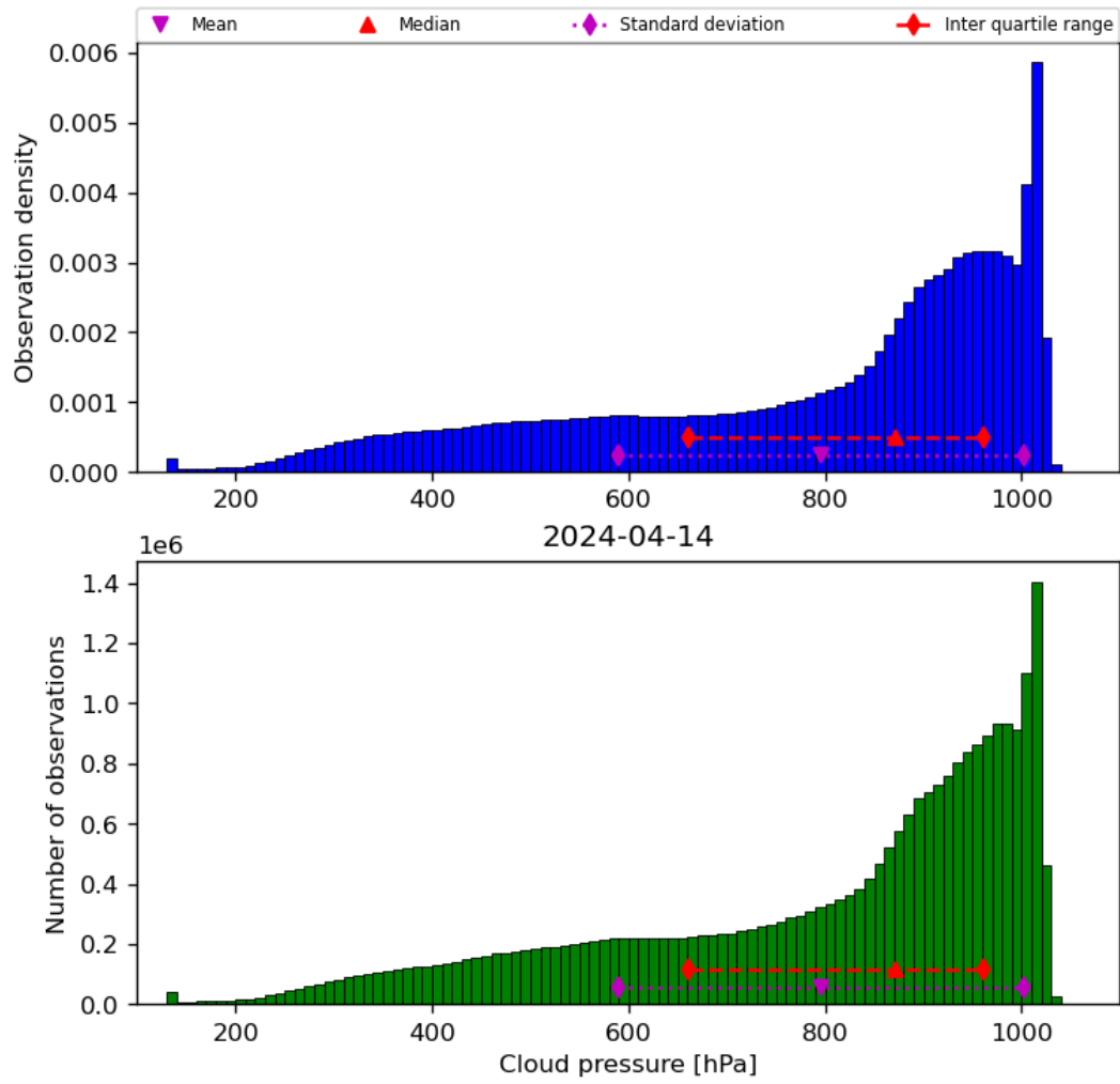
Figure 30: Histogram of “Cloud pressure” for 2024-04-13 to 2024-04-15
