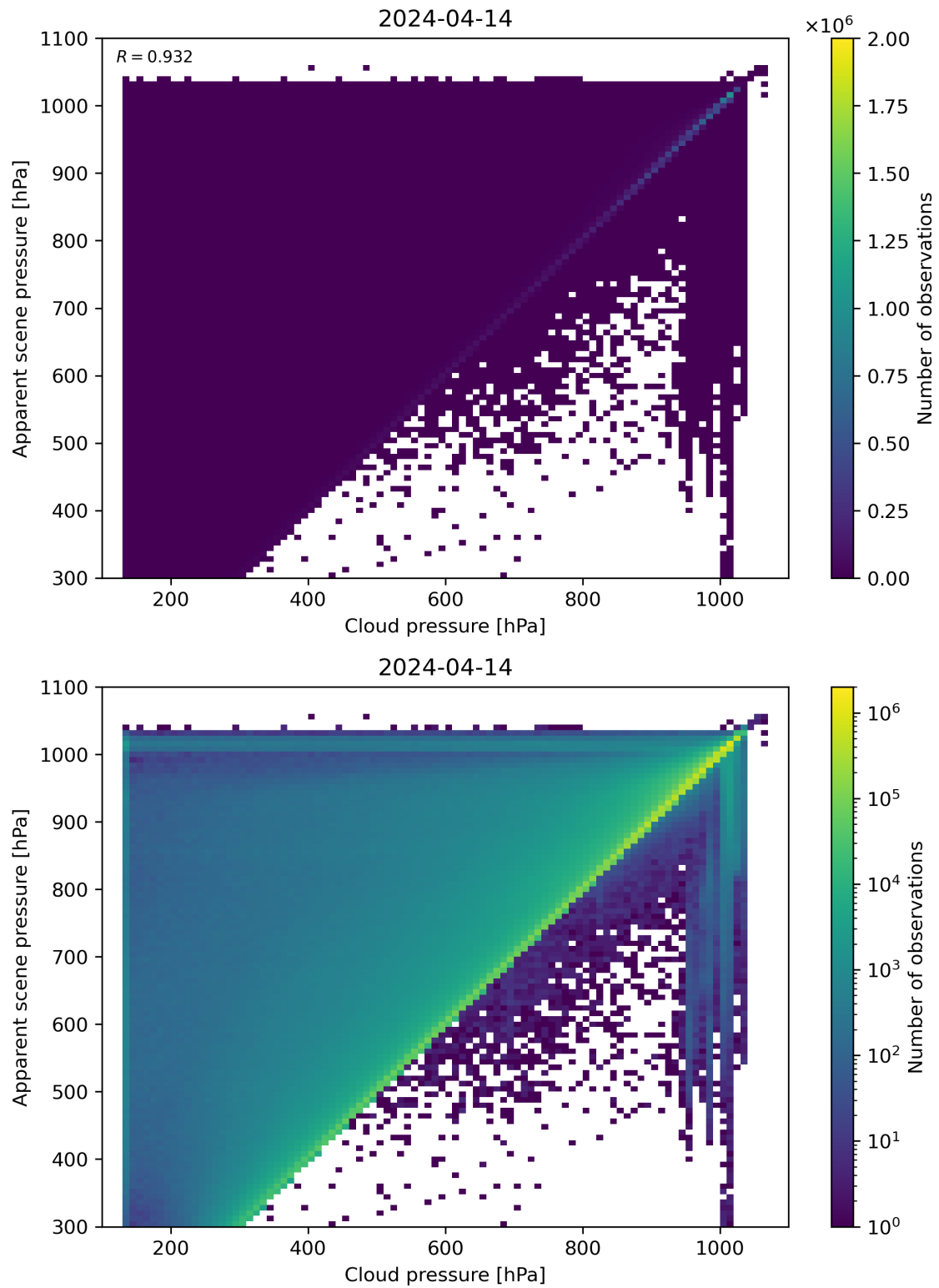
Figure 77: Scatter density plot of “Cloud pressure” against “Apparent scene pressure” for 2024-04-13 to 2024-04-15.
