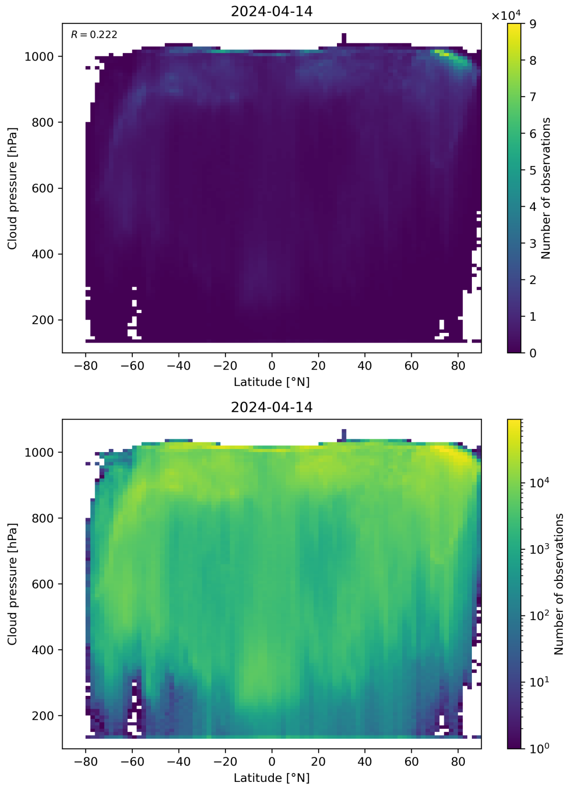
Figure 91: Scatter density plot of “Latitude” against “Cloud pressure” for 2024-04-13 to 2024-04-15.
