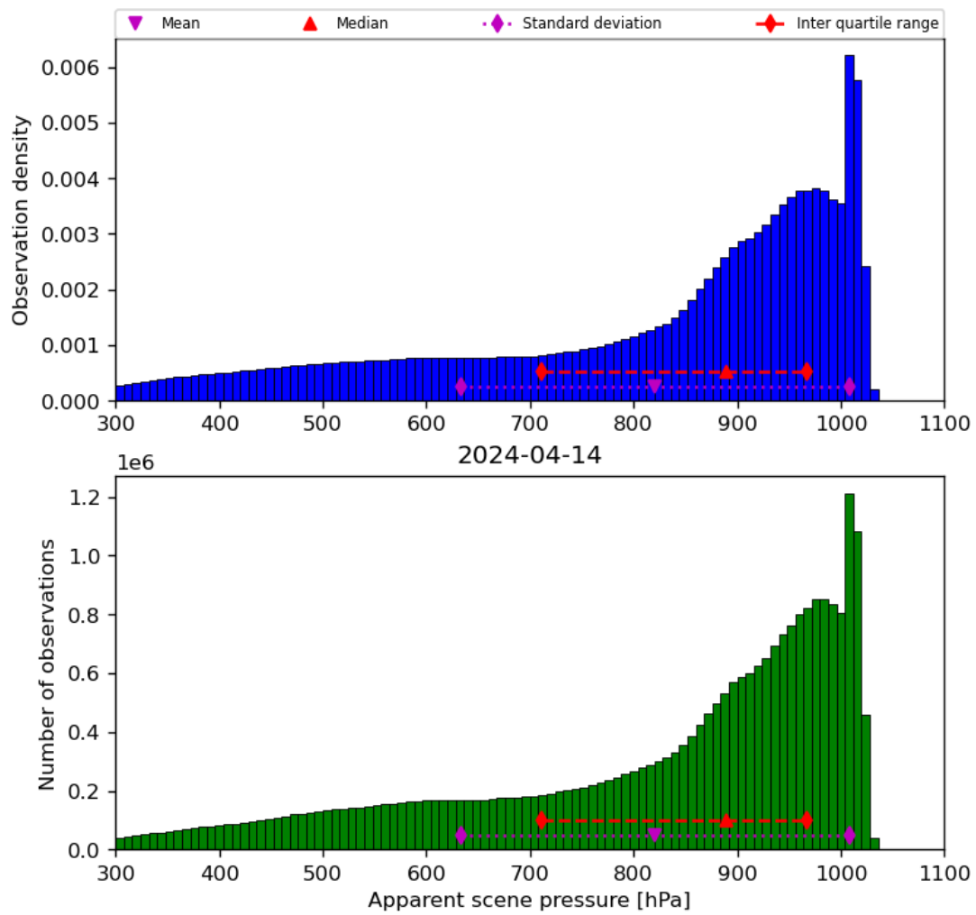
Figure 36: Histogram of “Apparent scene pressure” for 2024-04-13 to 2024-04-15
