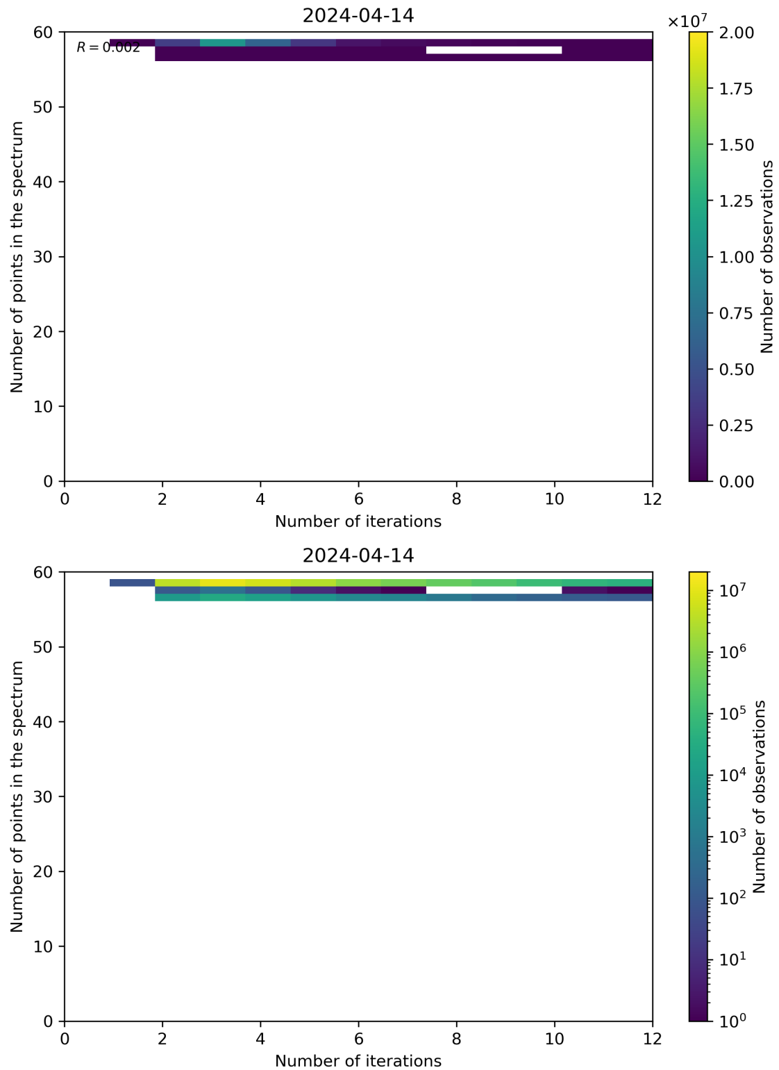
Figure 99: Scatter density plot of “Number of iterations” against “Number of points in the spectrum” for 2024-04-13 to 2024-04-15.
