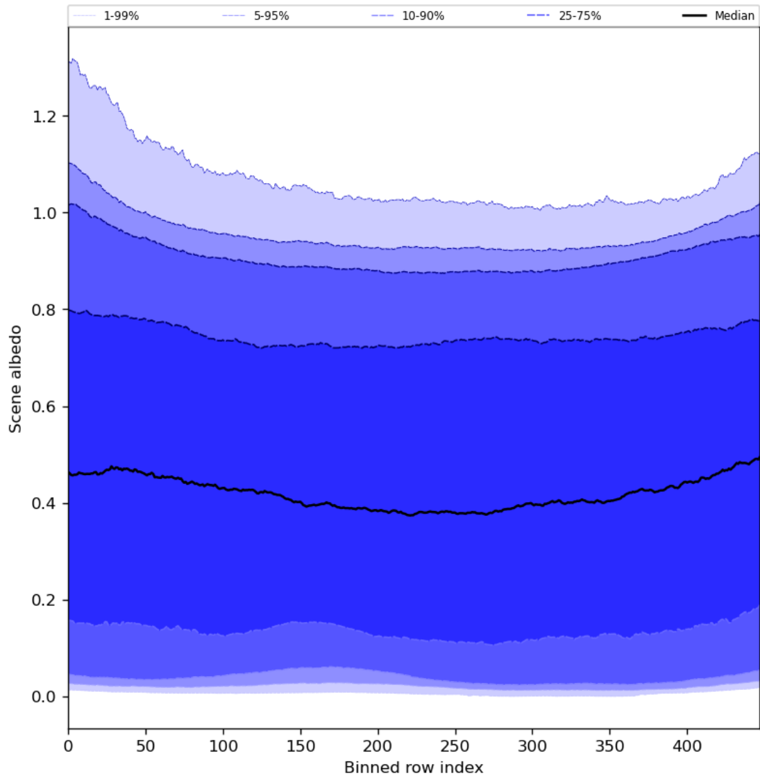
Figure 51: Along track statistics of “Scene albedo” for 2024-04-13 to 2024-04-15
