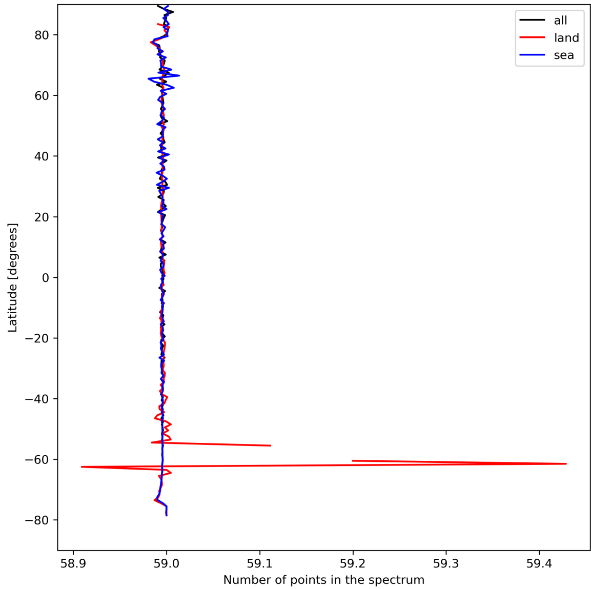
Figure 27: Zonal average of “Number of points in the spectrum” for 2024-04-13 to 2024-04-15.
