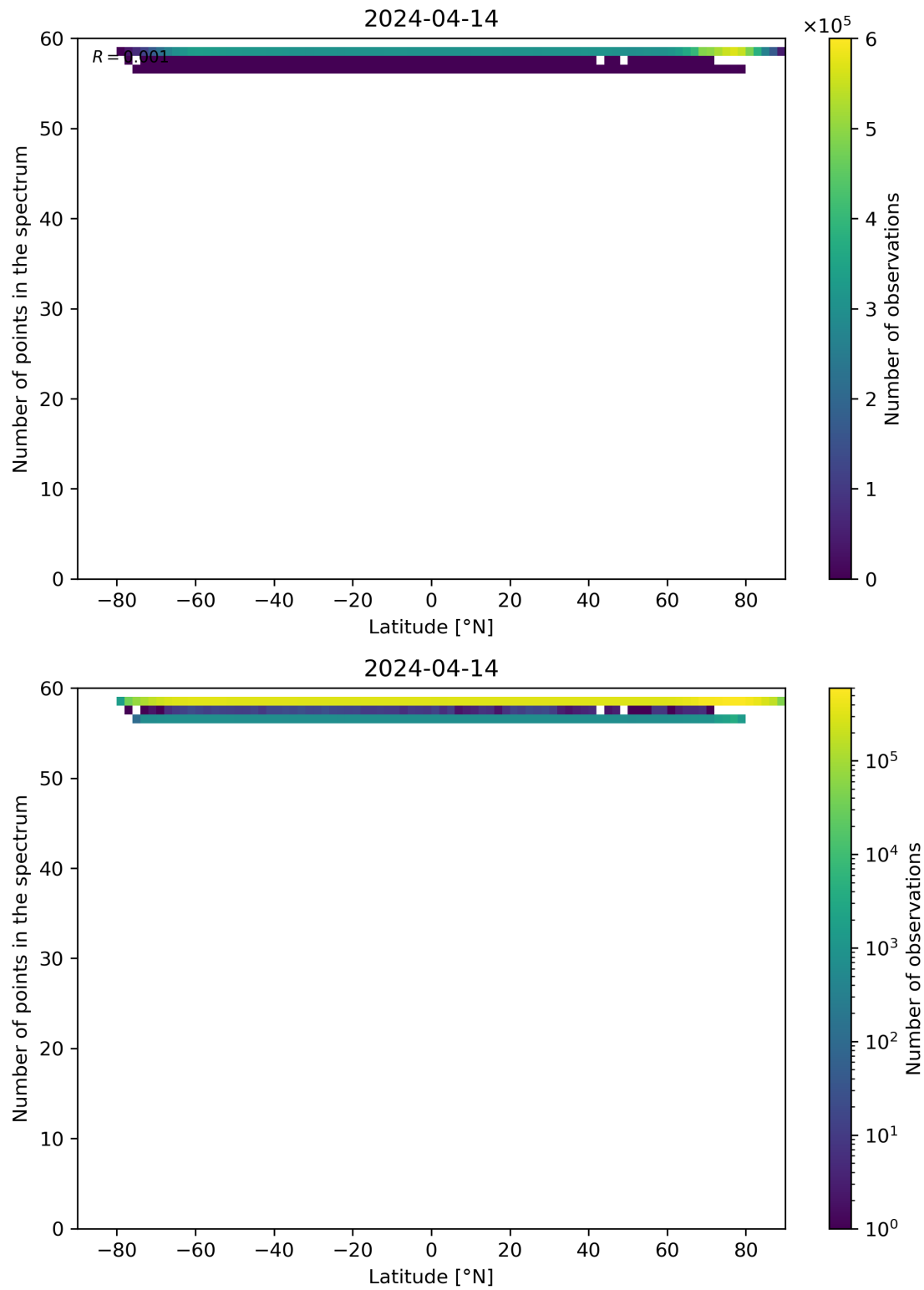
Figure 94: Scatter density plot of “Latitude” against “Number of points in the spectrum” for 2024-04-13 to 2024-04-15.
