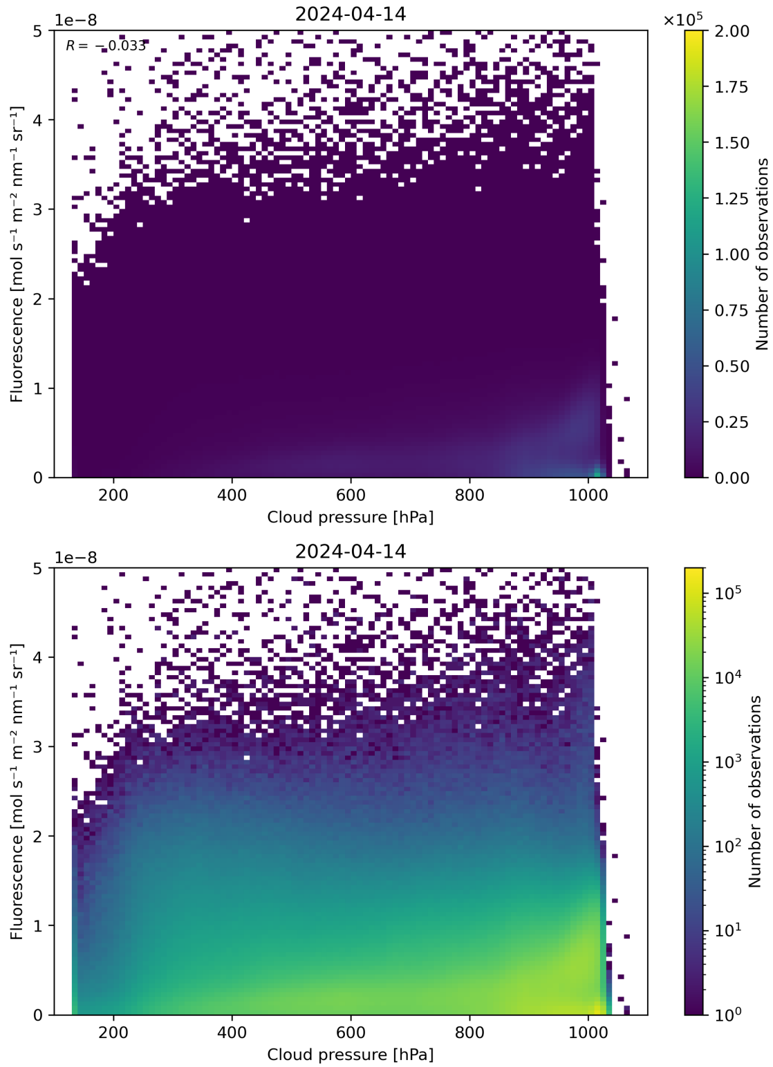
Figure 80: Scatter density plot of “Cloud pressure” against “Fluorescence” for 2024-04-13 to 2024-04-15.
