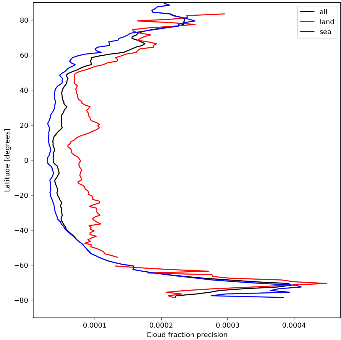
Figure 16: Zonal average of “Cloud fraction precision” for 2024-04-13 to 2024-04-15.
