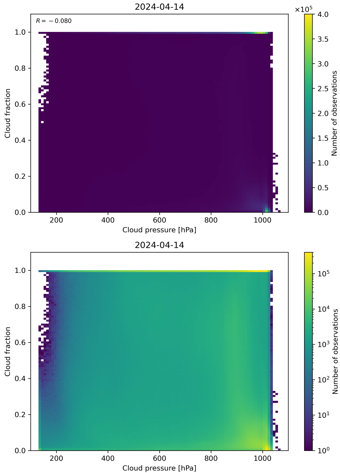
Figure 79: Scatter density plot of “Cloud pressure” against “Cloud fraction” for 2024-04-13 to 2024-04-15.
