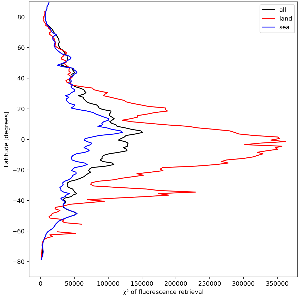
Figure 25: Zonal average of “ \chi^2 of fluorescence retrieval” for 2024-04-13 to 2024-04-15.
