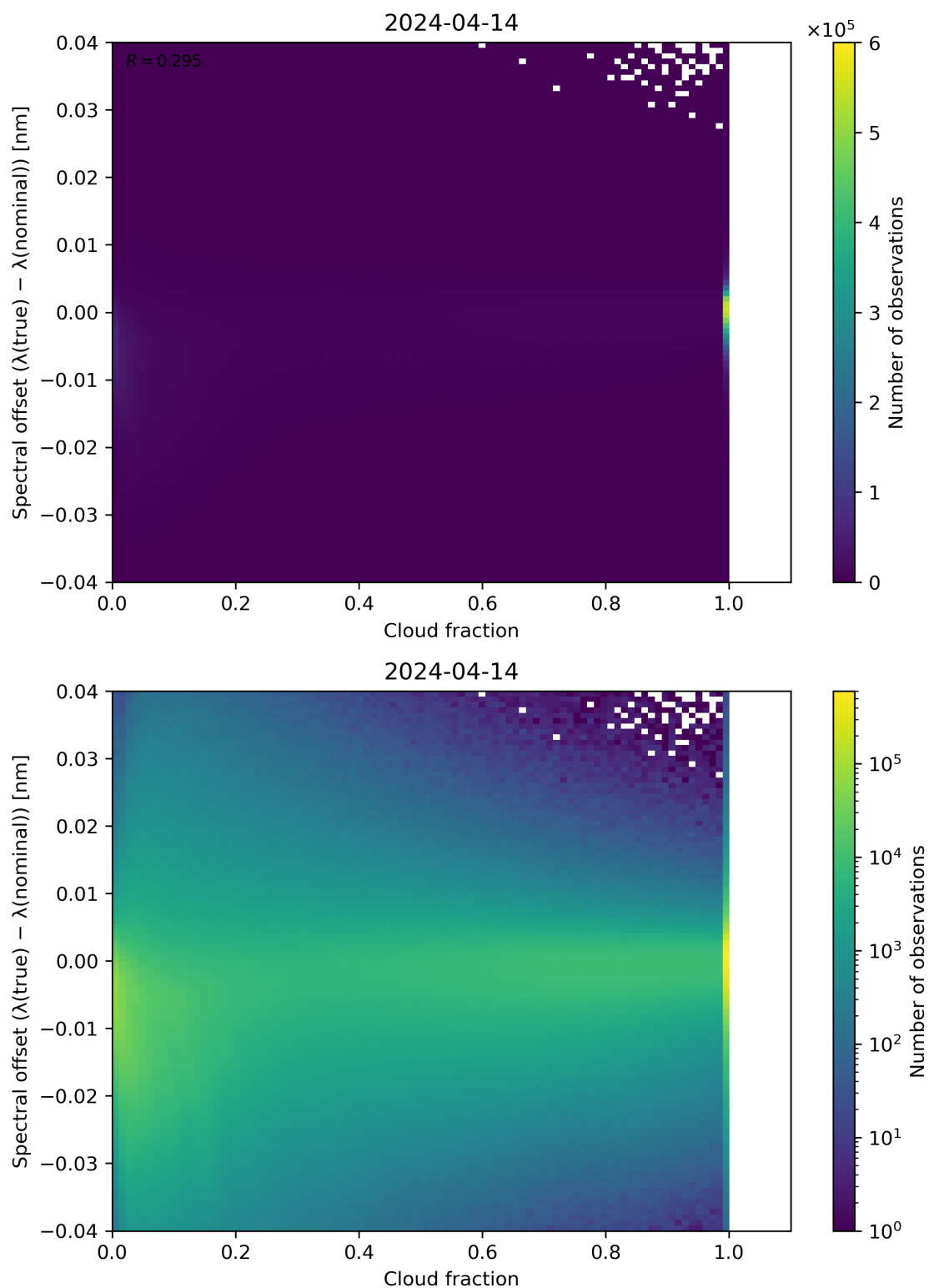
Figure 76: Scatter density plot of “Cloud fraction” against “Spectral offset ( \lambda(\text{true}) - \lambda(\text{nominal}) )” for 2024-04-13 to 2024-04-15.
