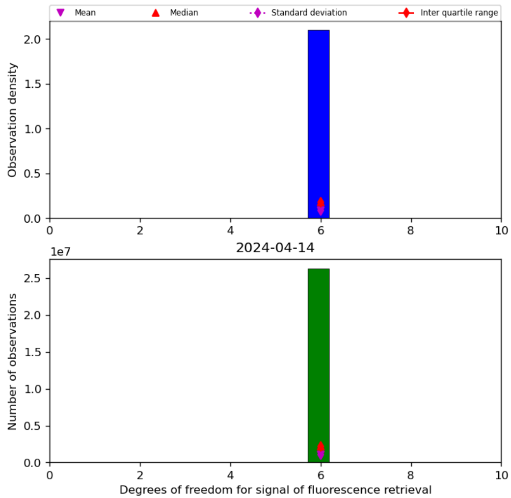
Figure 43: Histogram of “Degrees of freedom for signal of fluorescence retrieval” for 2024-04-13 to 2024-04-15
