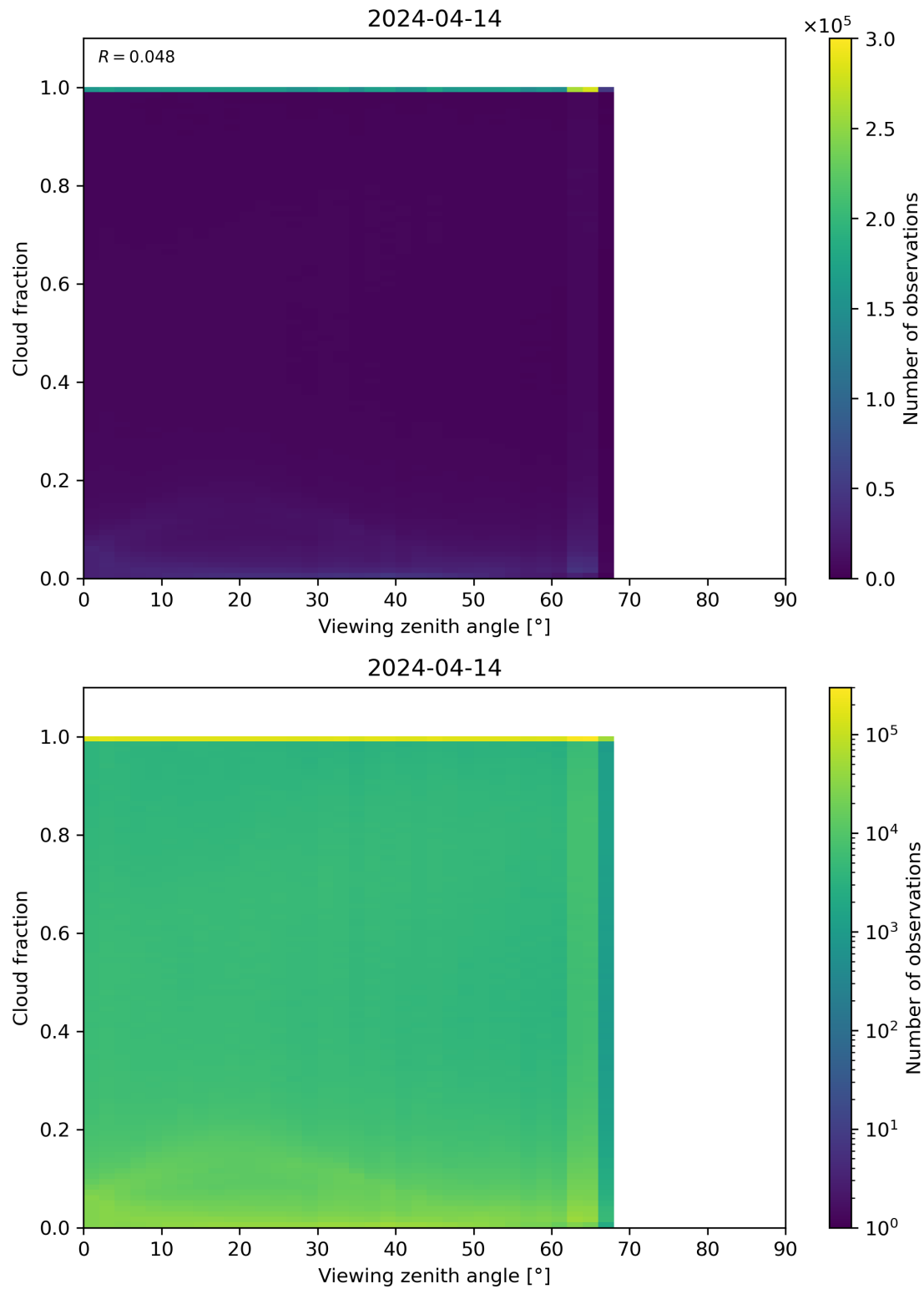
Figure 120: Scatter density plot of “Viewing zenith angle” against “Cloud fraction” for 2024-04-13 to 2024-04-15.
