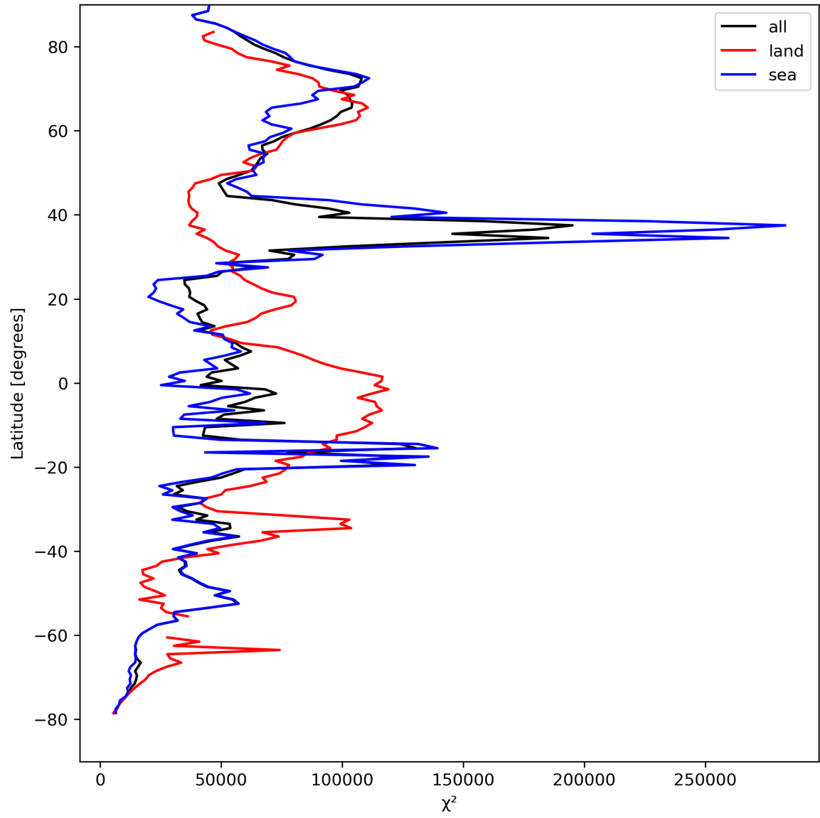
Figure 21: Zonal average of “ \chi^2 ” for 2024-04-13 to 2024-04-15.
