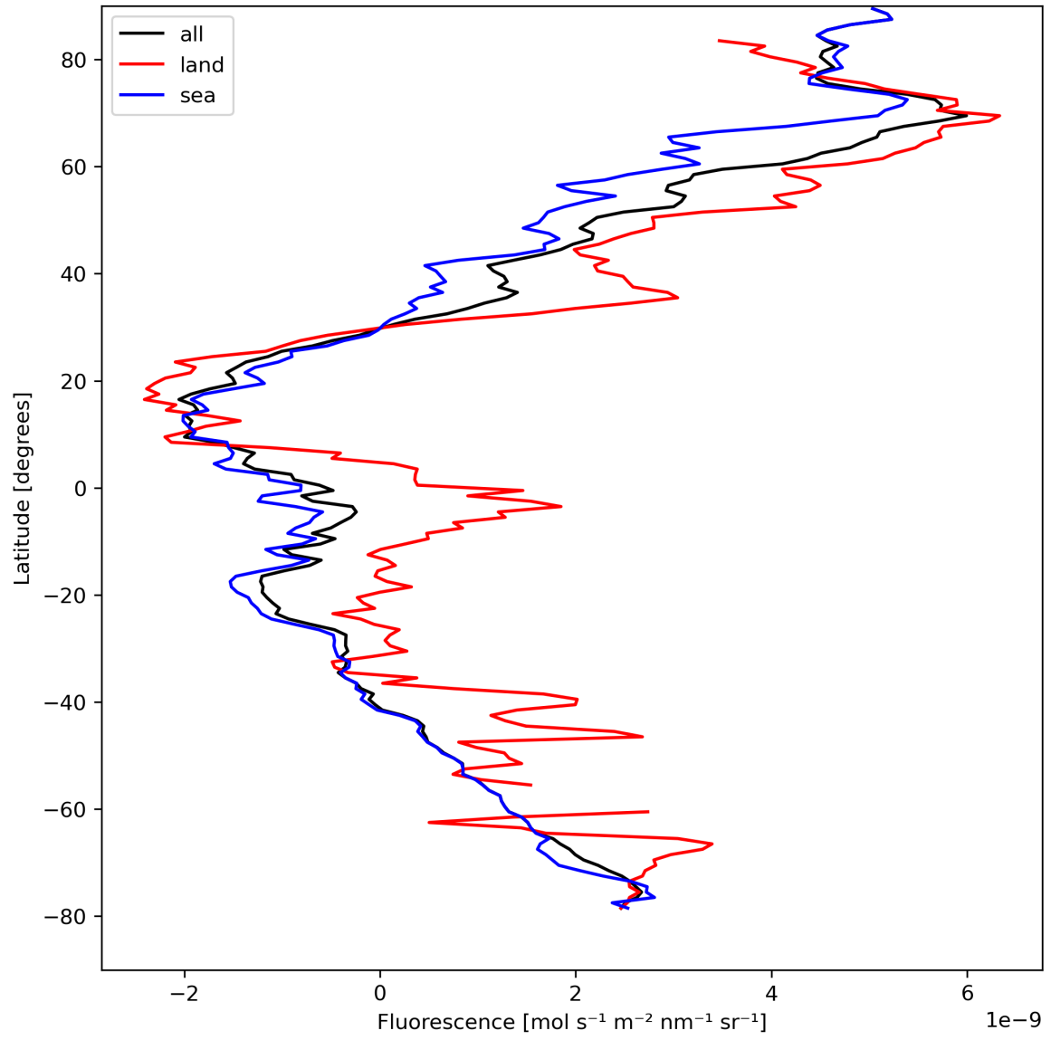
Figure 23: Zonal average of “Fluorescence” for 2024-04-13 to 2024-04-15.
