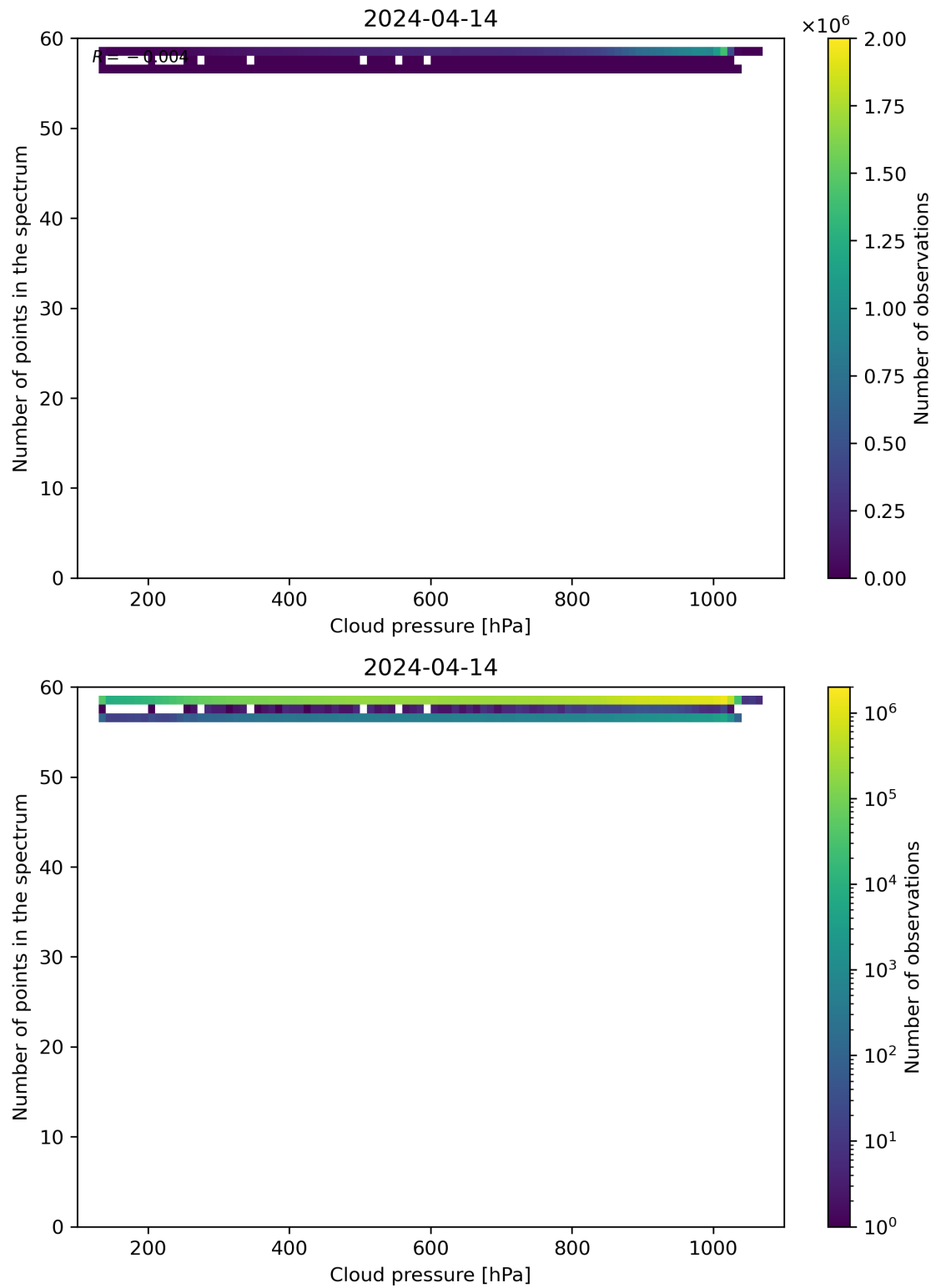
Figure 82: Scatter density plot of “Cloud pressure” against “Number of points in the spectrum” for 2024-04-13 to 2024-04-15.
