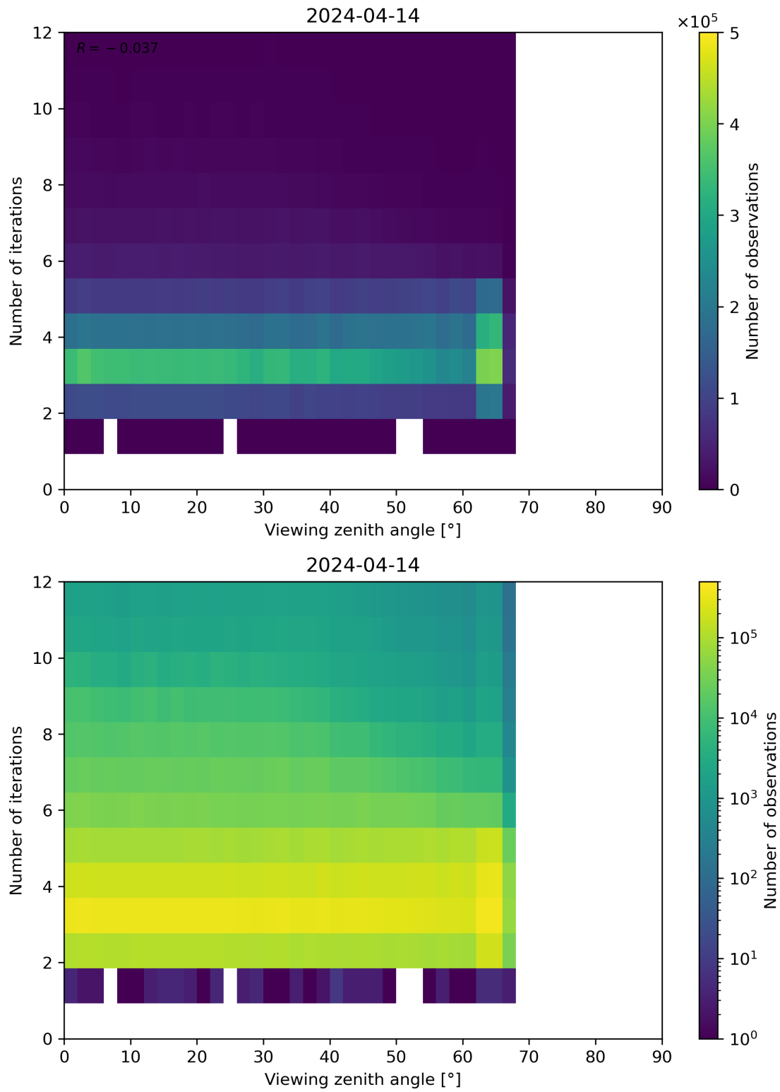
Figure 124: Scatter density plot of “Viewing zenith angle” against “Number of iterations” for 2024-04-13 to 2024-04-15.
