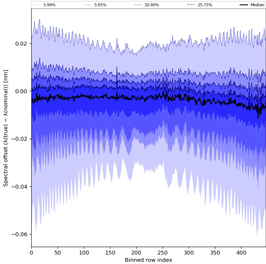
Figure 62: Along track statistics of “Spectral offset ( \lambda(\text{true}) - \lambda(\text{nominal}) )” for 2024-04-13 to 2024-04-15
