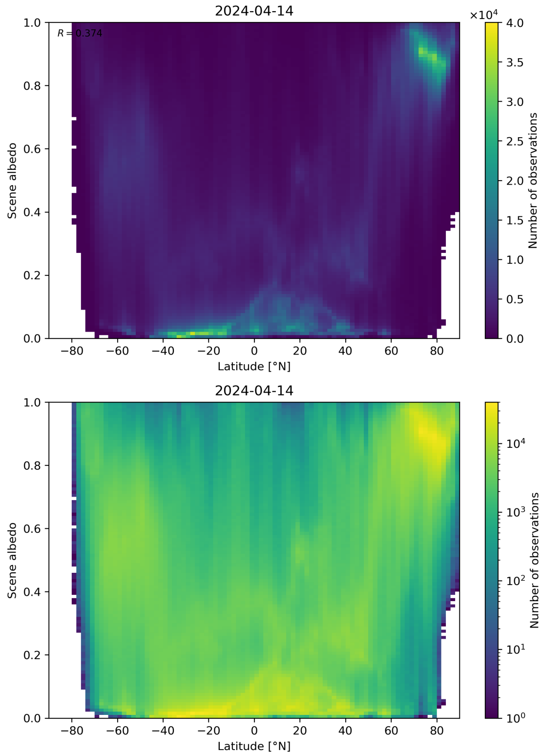
Figure 95: Scatter density plot of “Latitude” against “Scene albedo” for 2024-04-13 to 2024-04-15.
