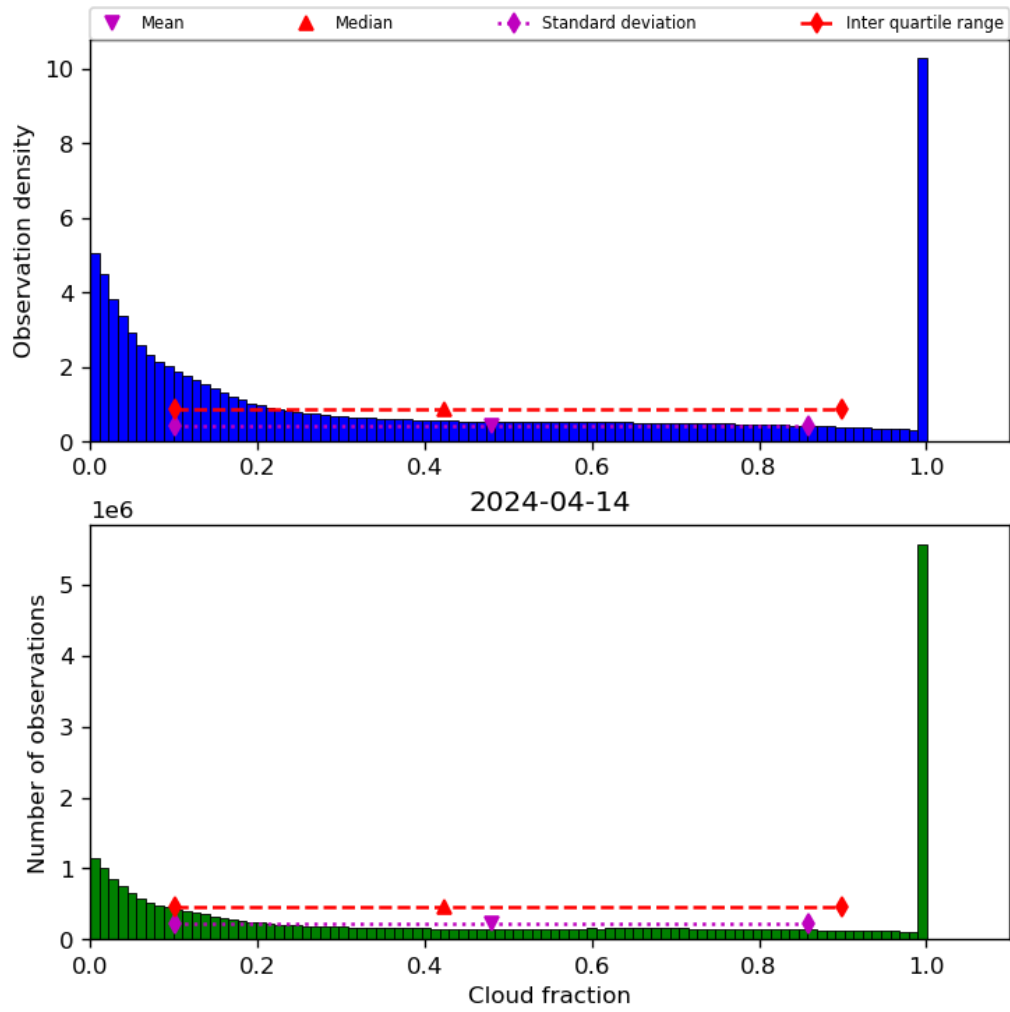
Figure 32: Histogram of “Cloud fraction” for 2024-04-13 to 2024-04-15
