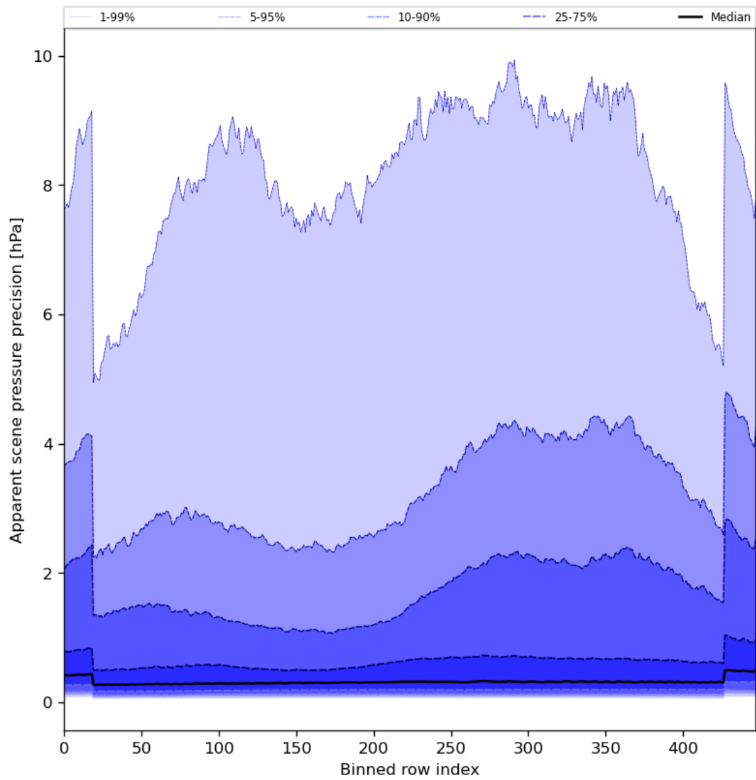
Figure 54: Along track statistics of “Apparent scene pressure precision” for 2024-04-13 to 2024-04-15
