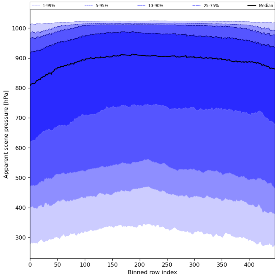
Figure 53: Along track statistics of “Apparent scene pressure” for 2024-04-13 to 2024-04-15
