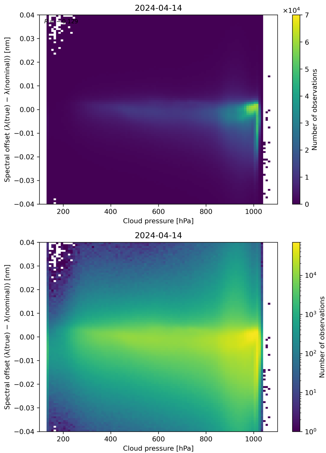
Figure 84: Scatter density plot of “Cloud pressure” against “Spectral offset ( \lambda(\text{true}) - \lambda(\text{nominal}) )” for 2024-04-13 to 2024-04-15.
