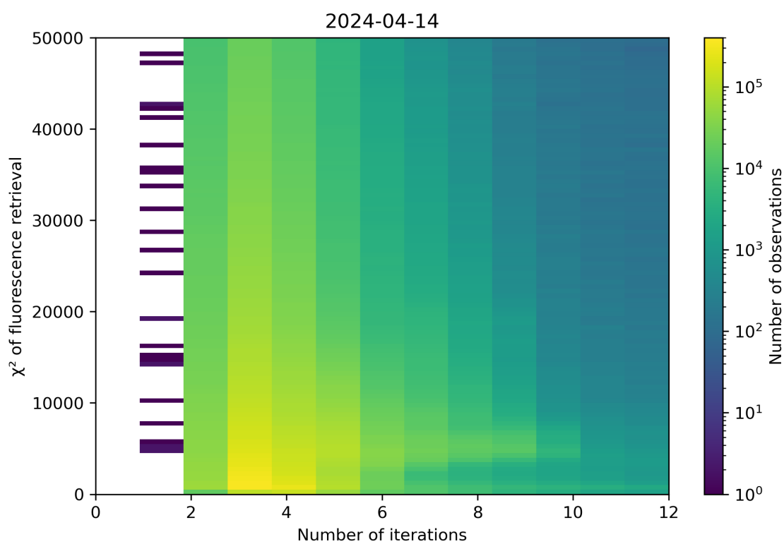
Figure 97: Scatter density plot of “Number of iterations” against “ \chi^2 of fluorescence retrieval” for 2024-04-13 to 2024-04-15.
