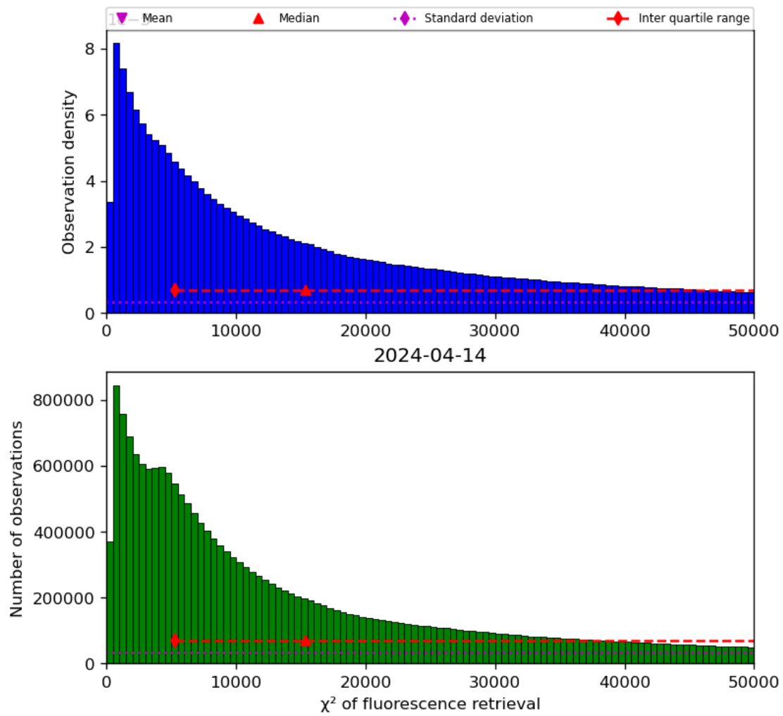
Figure 42: Histogram of “ \chi^2 of fluorescence retrieval” for 2024-04-13 to 2024-04-15
