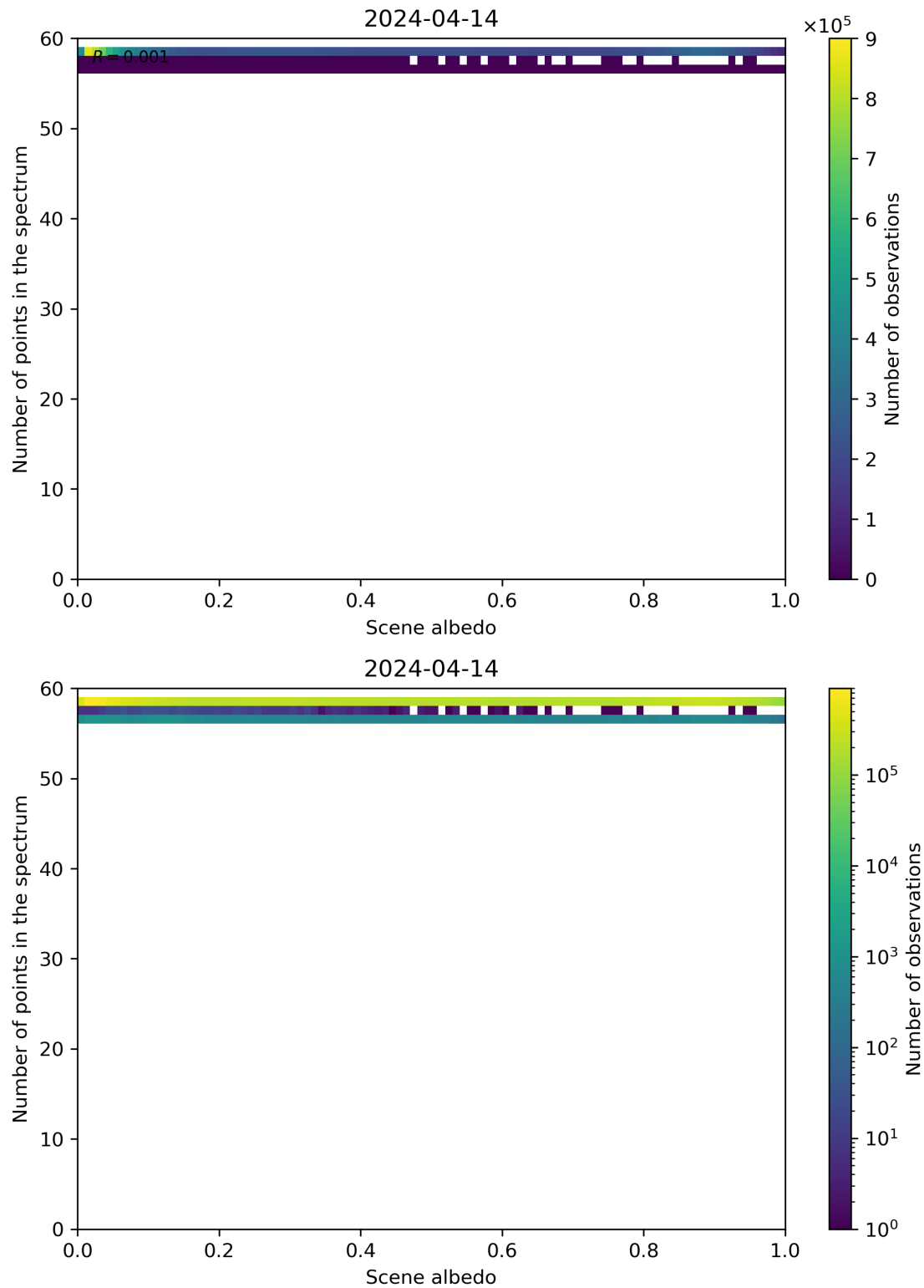
Figure 106: Scatter density plot of “Scene albedo” against “Number of points in the spectrum” for 2024-04-13 to 2024-04-15.
