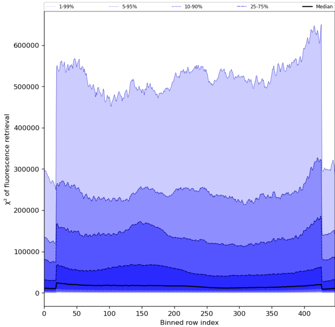
Figure 59: Along track statistics of “ \chi^2 of fluorescence retrieval” for 2024-04-13 to 2024-04-15
