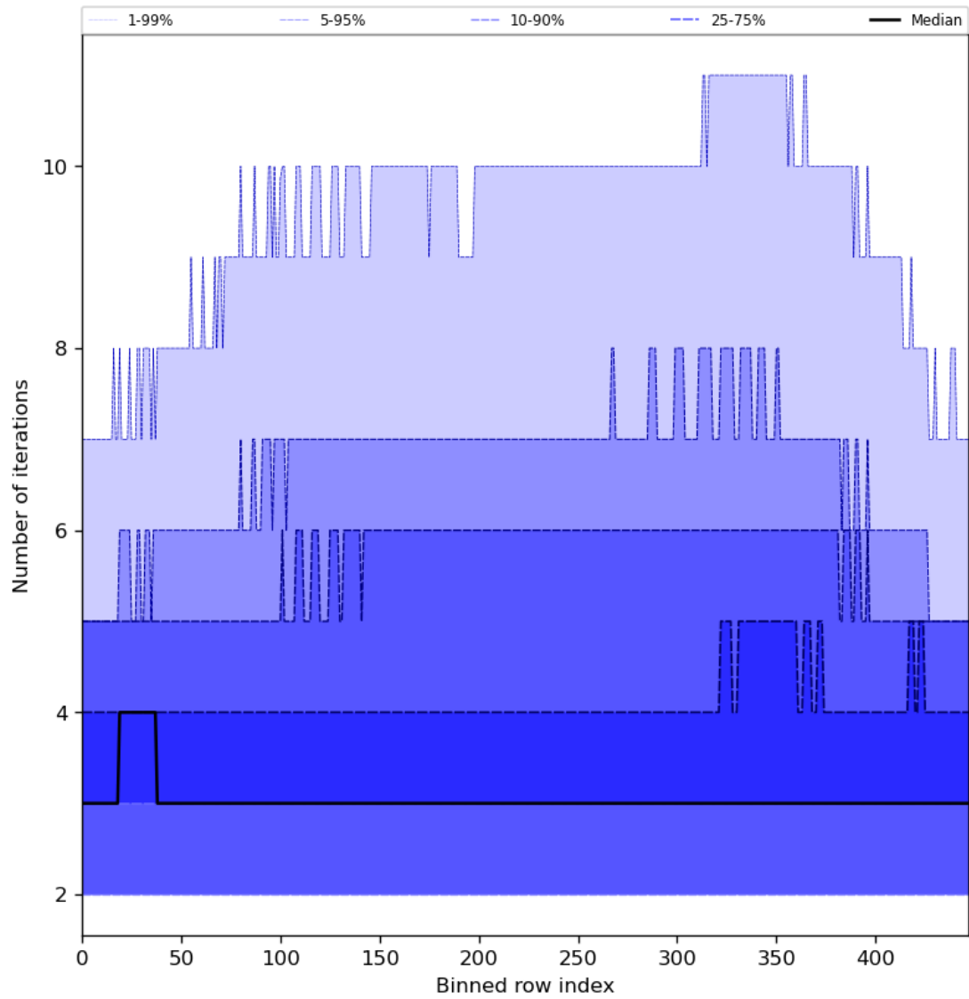
Figure 56: Along track statistics of “Number of iterations” for 2024-04-13 to 2024-04-15
