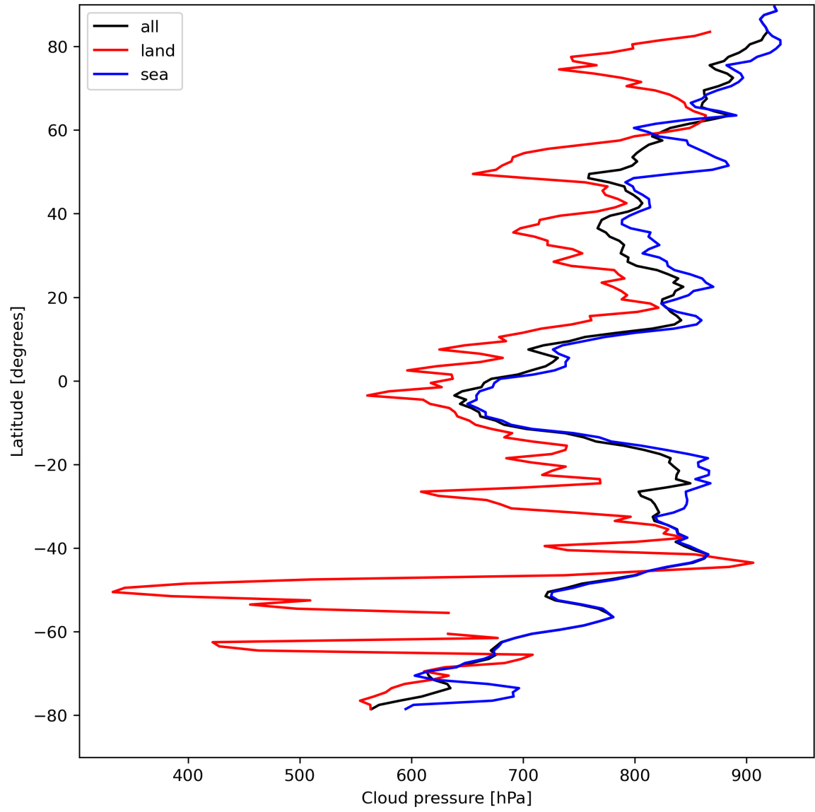
Figure 13: Zonal average of “Cloud pressure” for 2024-04-13 to 2024-04-15.
