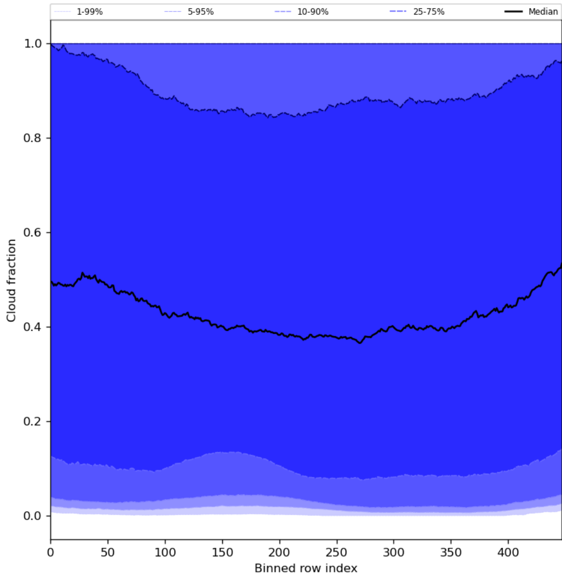
Figure 49: Along track statistics of “Cloud fraction” for 2024-04-13 to 2024-04-15
