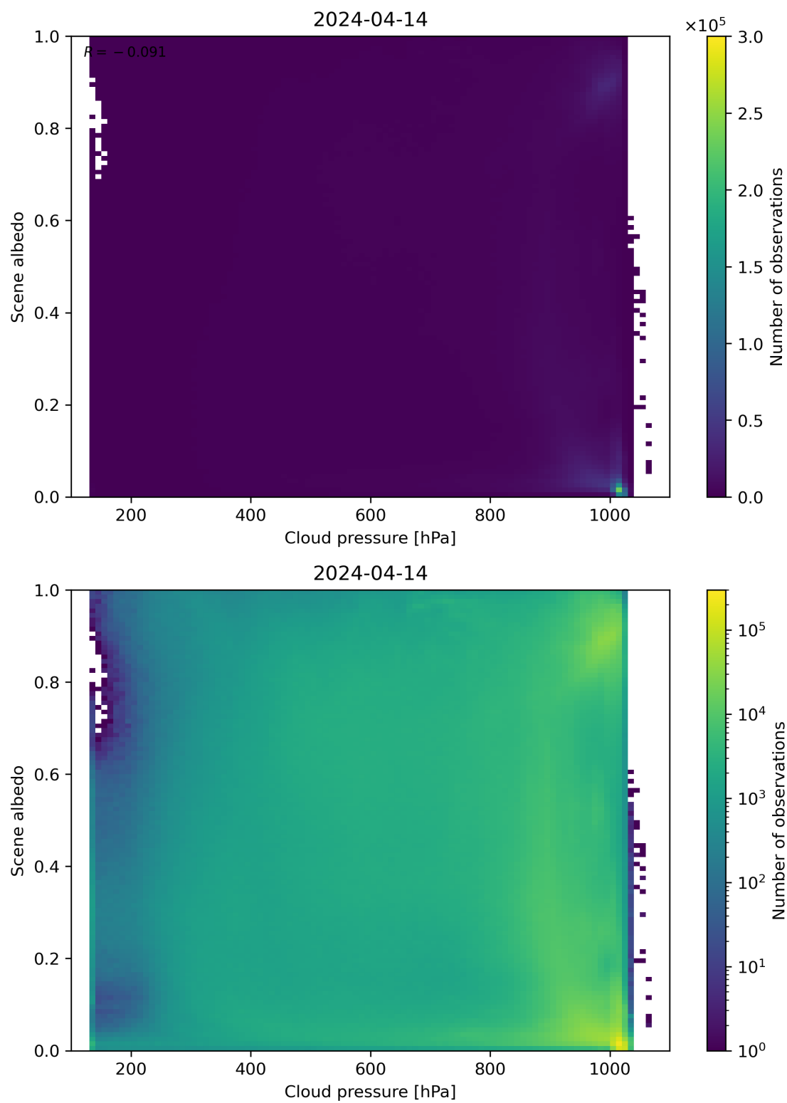
Figure 83: Scatter density plot of “Cloud pressure” against “Scene albedo” for 2024-04-13 to 2024-04-15.
