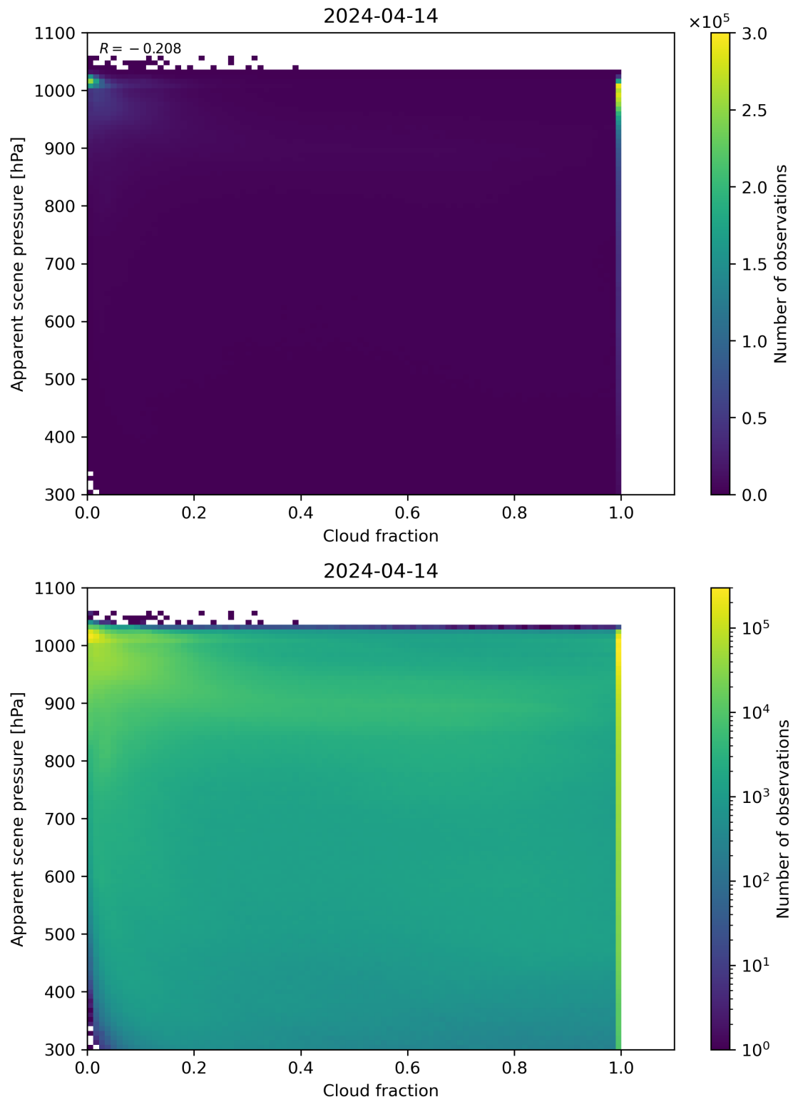
Figure 70: Scatter density plot of “Cloud fraction” against “Apparent scene pressure” for 2024-04-13 to 2024-04-15.
