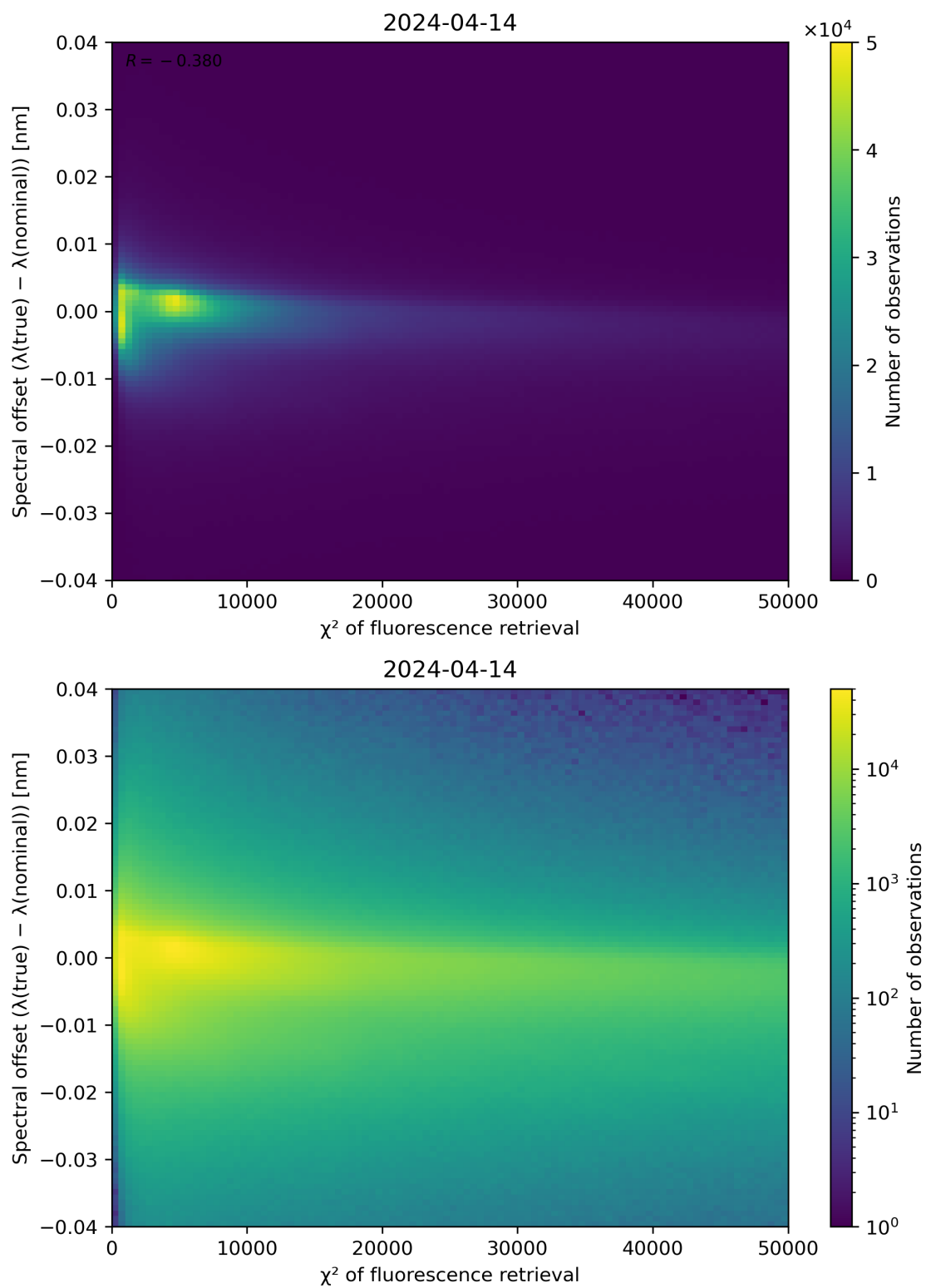
Figure 69: Scatter density plot of " \chi^2 of fluorescence retrieval" against "Spectral offset ( \lambda(\text{true}) - \lambda(\text{nominal}) )" for 2024-04-13 to 2024-04-15.
