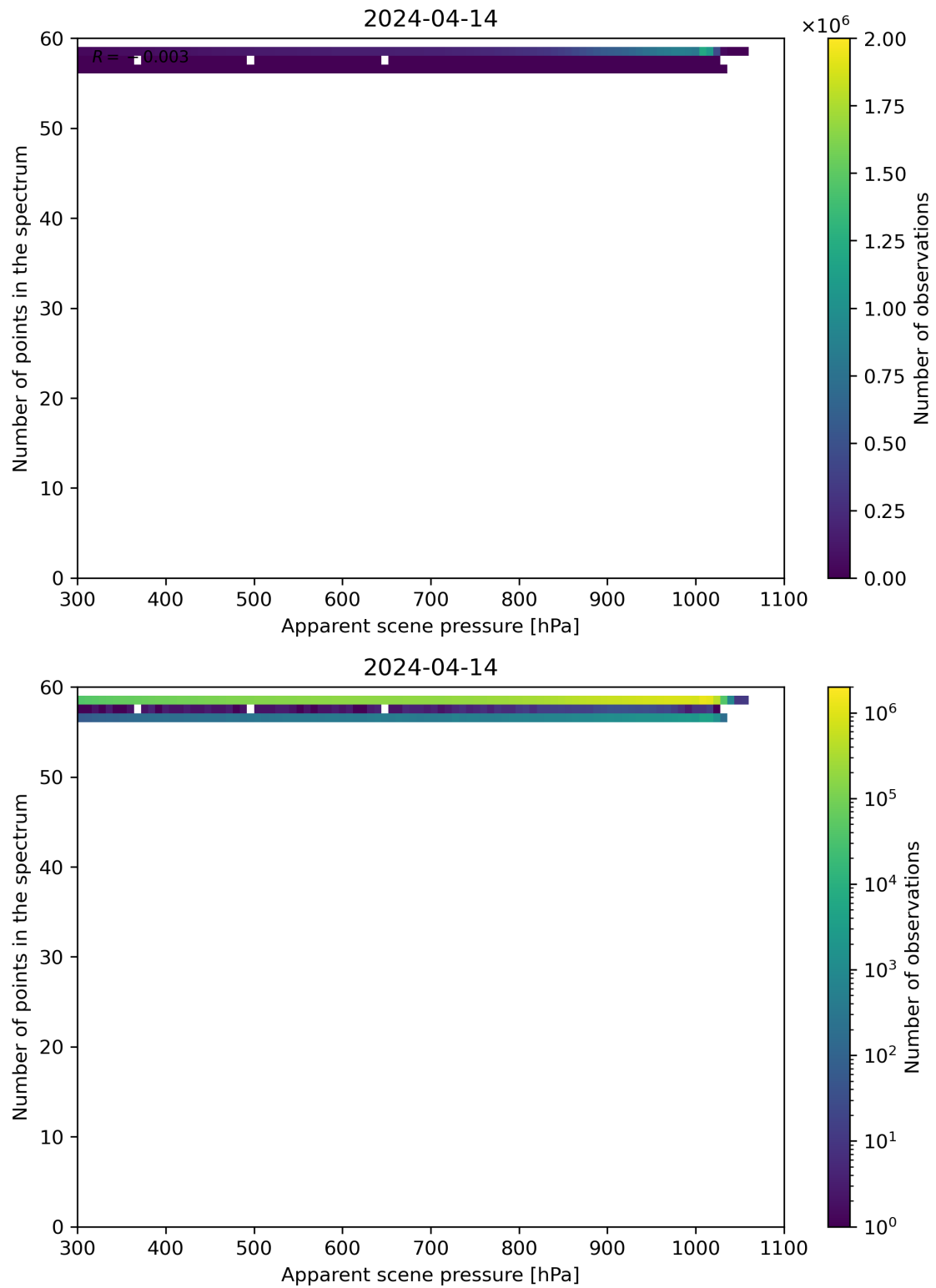
Figure 66: Scatter density plot of “Apparent scene pressure” against “Number of points in the spectrum” for 2024-04-13 to 2024-04-15.
