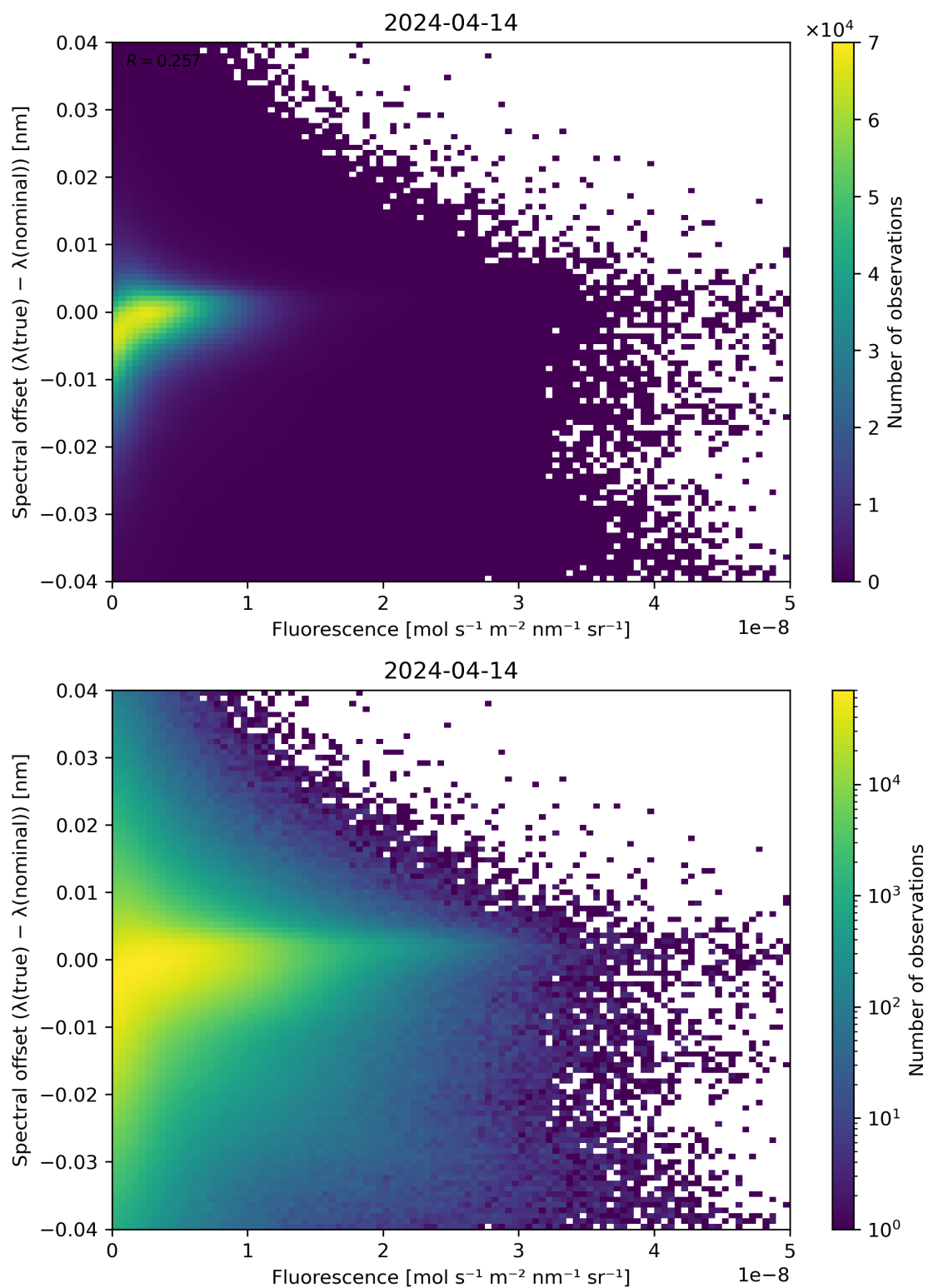
Figure 87: Scatter density plot of “Fluorescence” against “Spectral offset ( \lambda(\text{true}) - \lambda(\text{nominal}) )” for 2024-04-13 to 2024-04-15.
