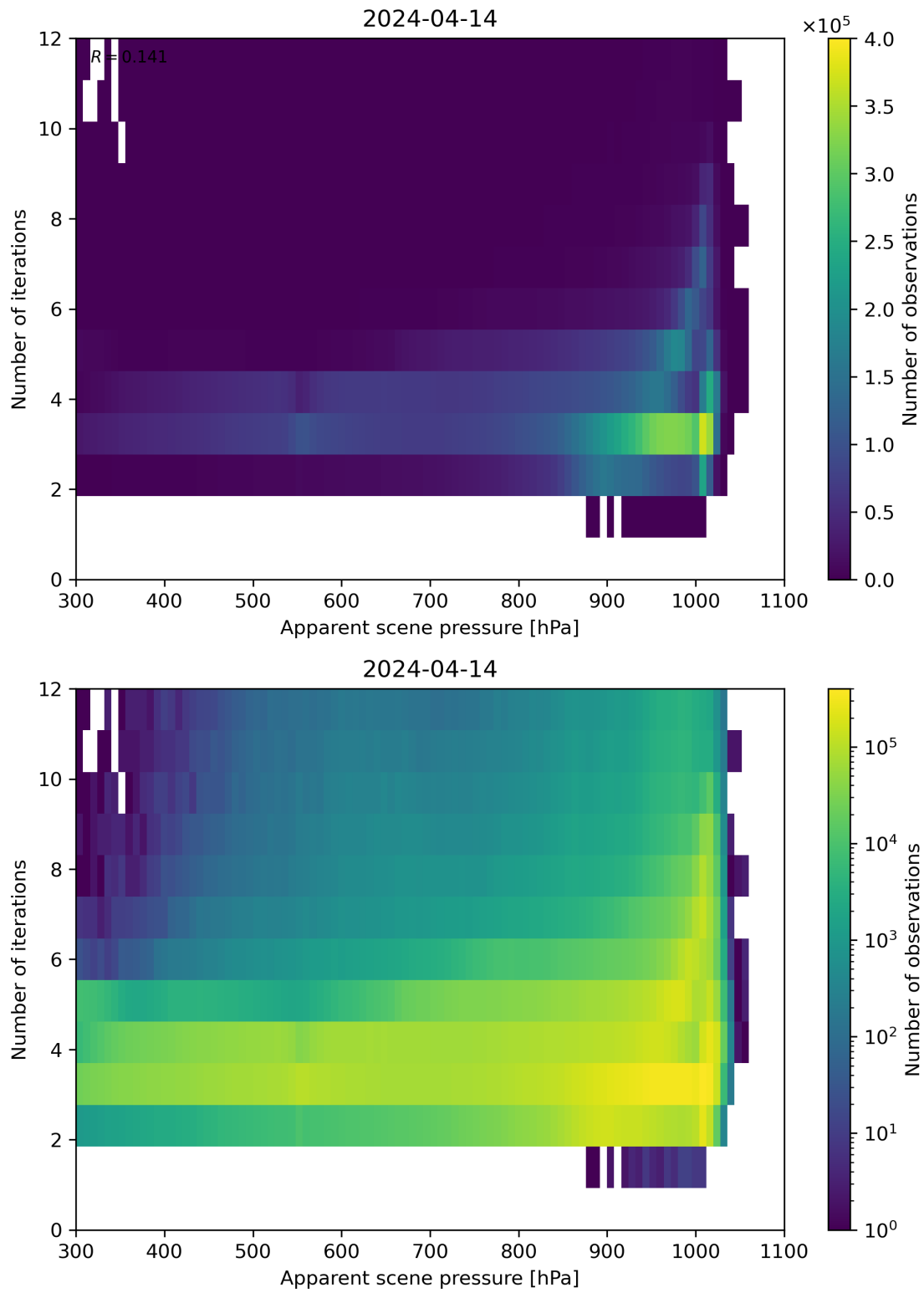
Figure 65: Scatter density plot of “Apparent scene pressure” against “Number of iterations” for 2024-04-13 to 2024-04-15.
