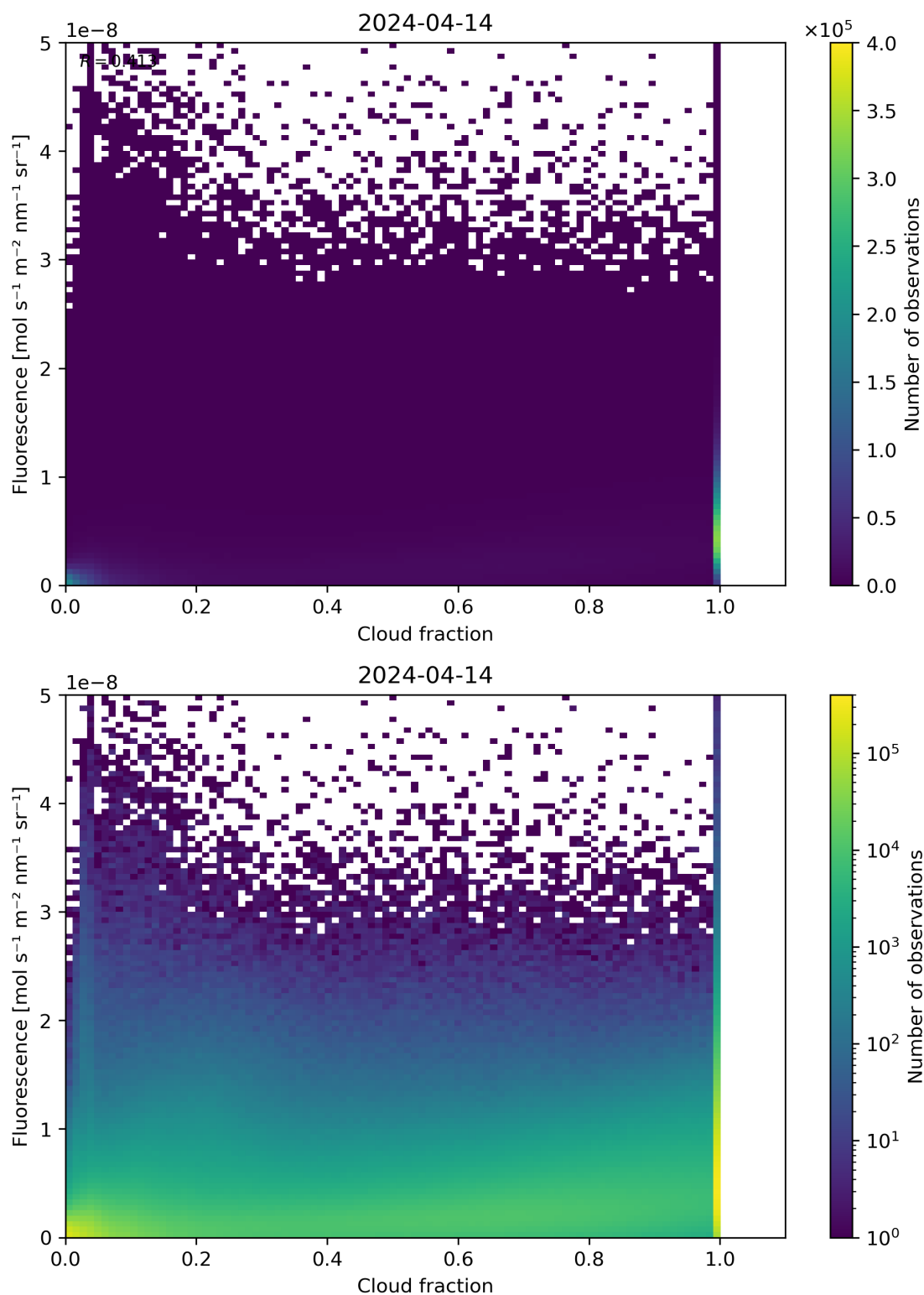
Figure 72: Scatter density plot of “Cloud fraction” against “Fluorescence” for 2024-04-13 to 2024-04-15.
