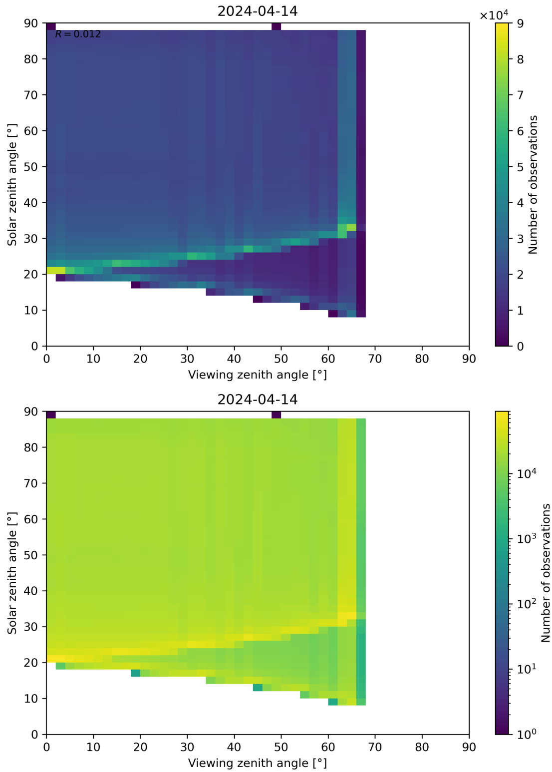
Figure 127: Scatter density plot of “Viewing zenith angle” against “Solar zenith angle” for 2024-04-13 to 2024-04-15.
