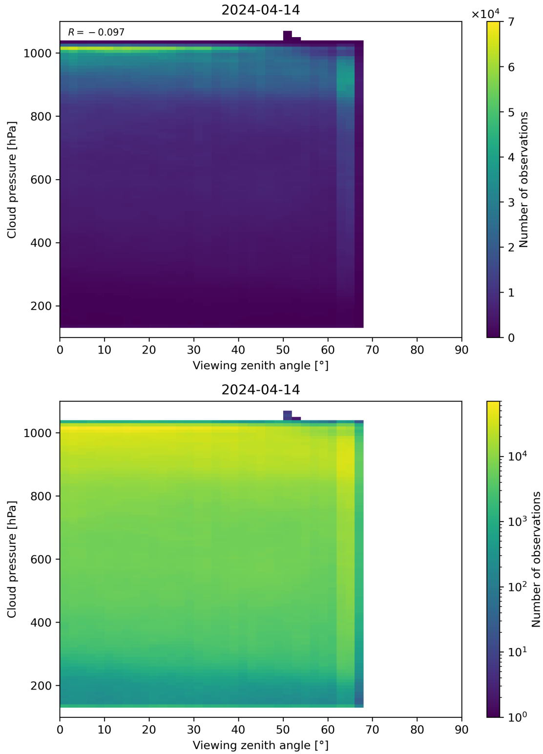
Figure 121: Scatter density plot of “Viewing zenith angle” against “Cloud pressure” for 2024-04-13 to 2024-04-15.
