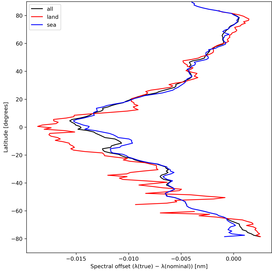
Figure 28: Zonal average of “Spectral offset ( \lambda(\text{true}) - \lambda(\text{nominal}) )” for 2024-04-13 to 2024-04-15.
