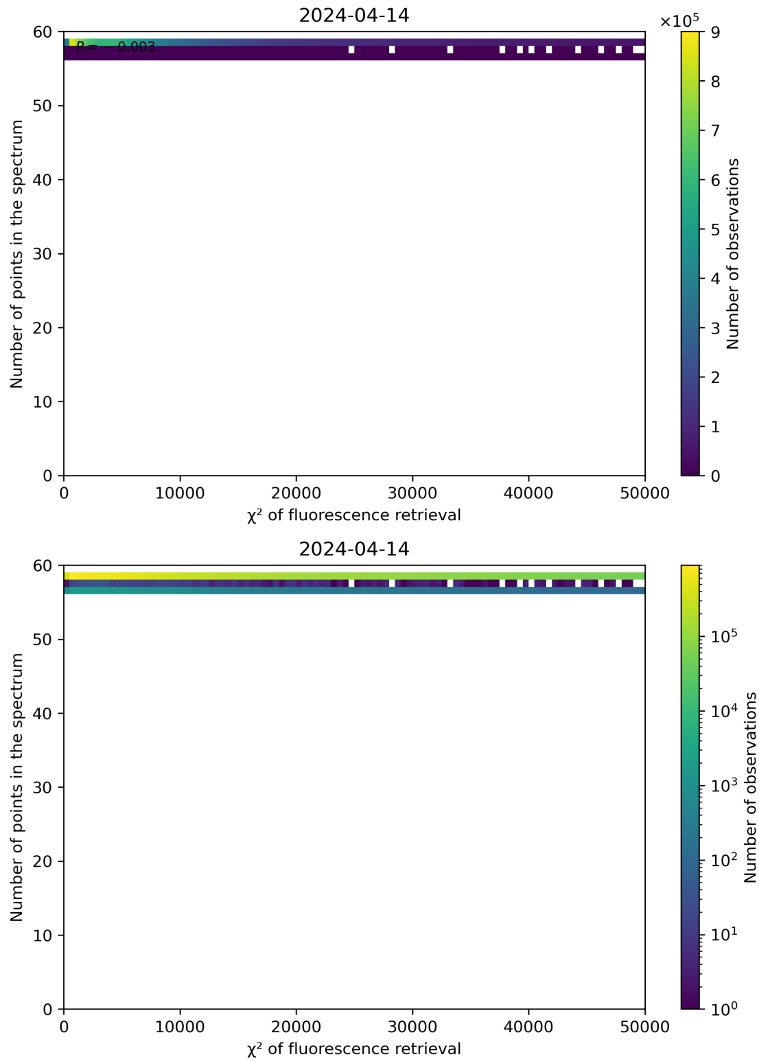
Figure 68: Scatter density plot of " \chi^2 of fluorescence retrieval" against "Number of points in the spectrum" for 2024-04-13 to 2024-04-15.
