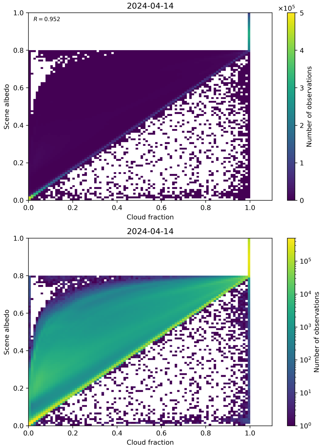
Figure 75: Scatter density plot of “Cloud fraction” against “Scene albedo” for 2024-04-13 to 2024-04-15.
