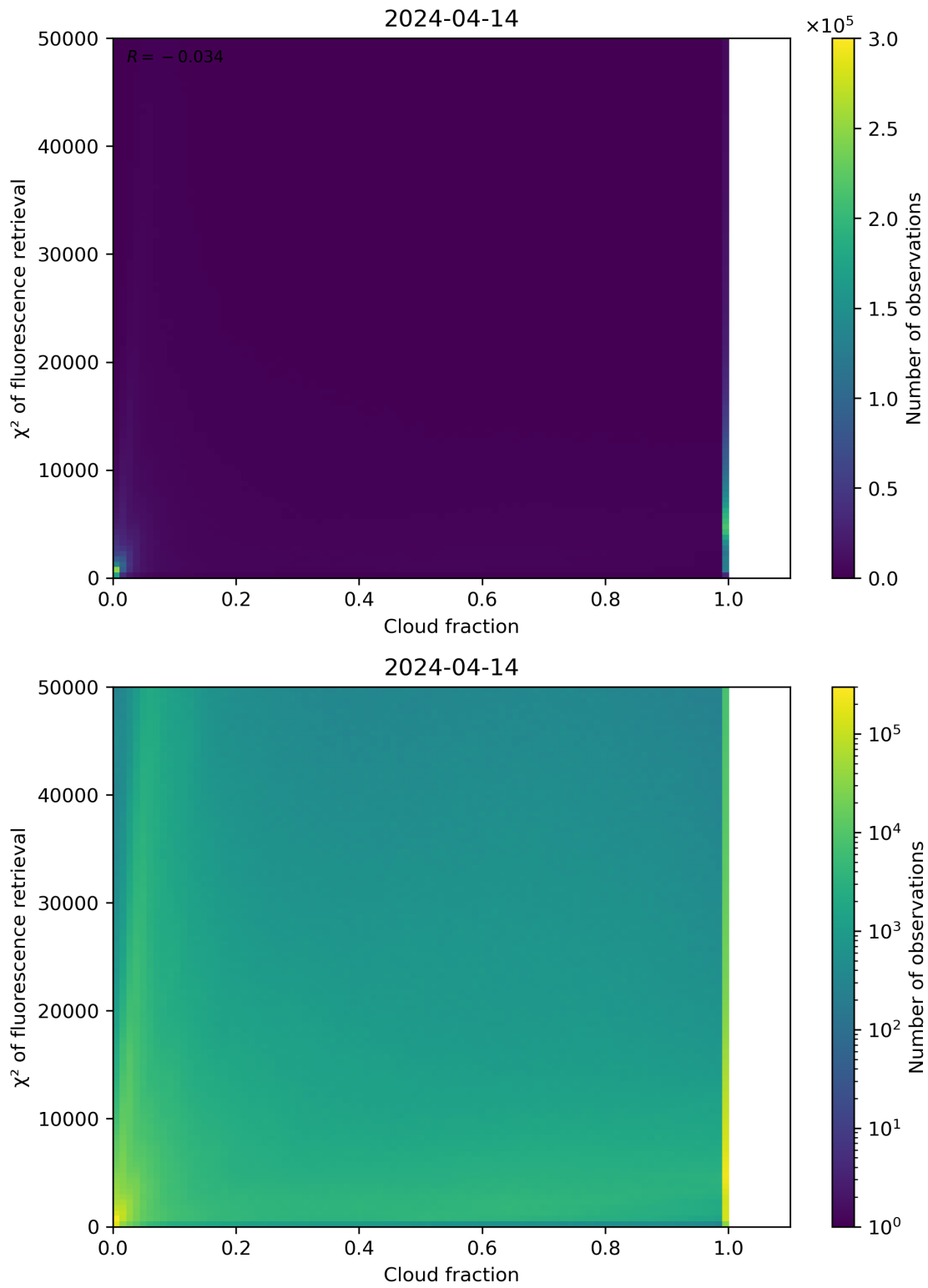
Figure 71: Scatter density plot of “Cloud fraction” against “ \chi^2 of fluorescence retrieval” for 2024-04-13 to 2024-04-15.
