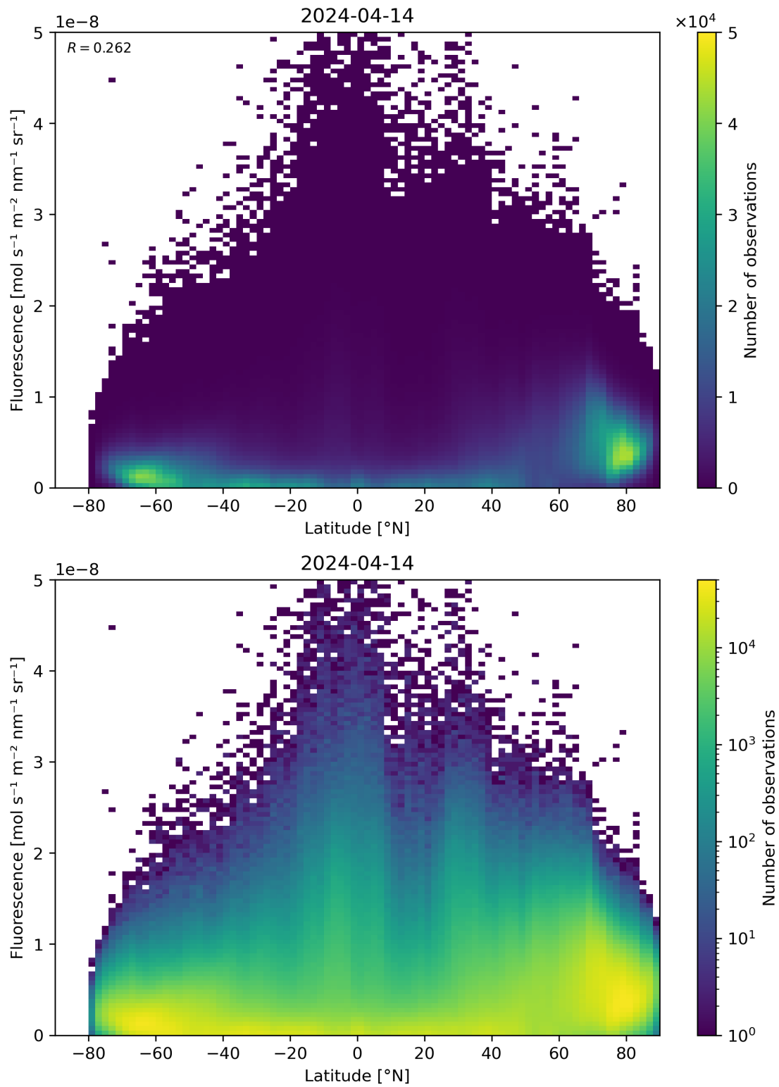
Figure 92: Scatter density plot of “Latitude” against “Fluorescence” for 2024-04-13 to 2024-04-15.
