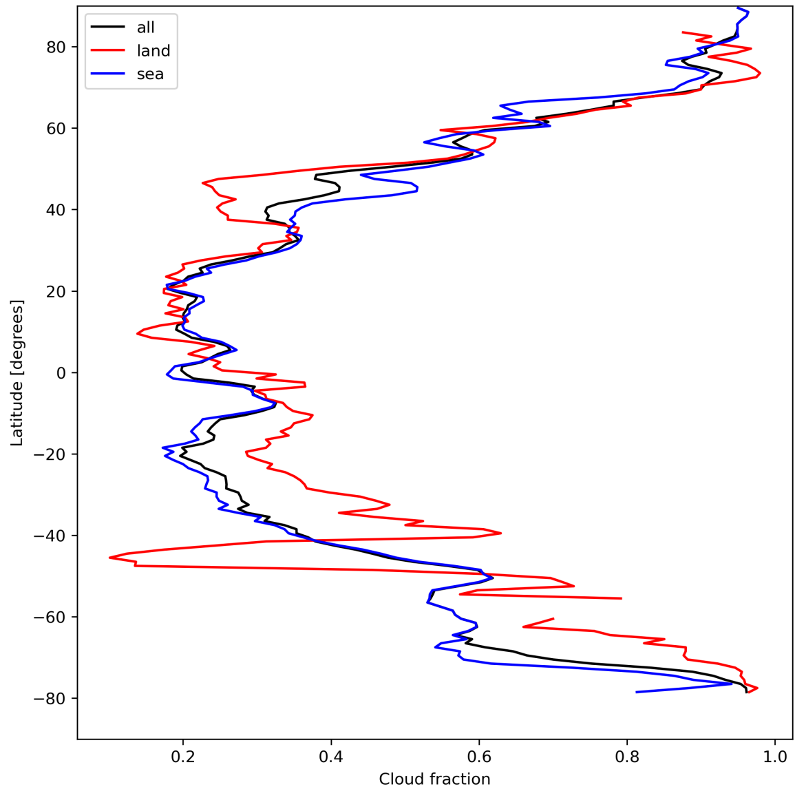
Figure 15: Zonal average of “Cloud fraction” for 2024-04-13 to 2024-04-15.
