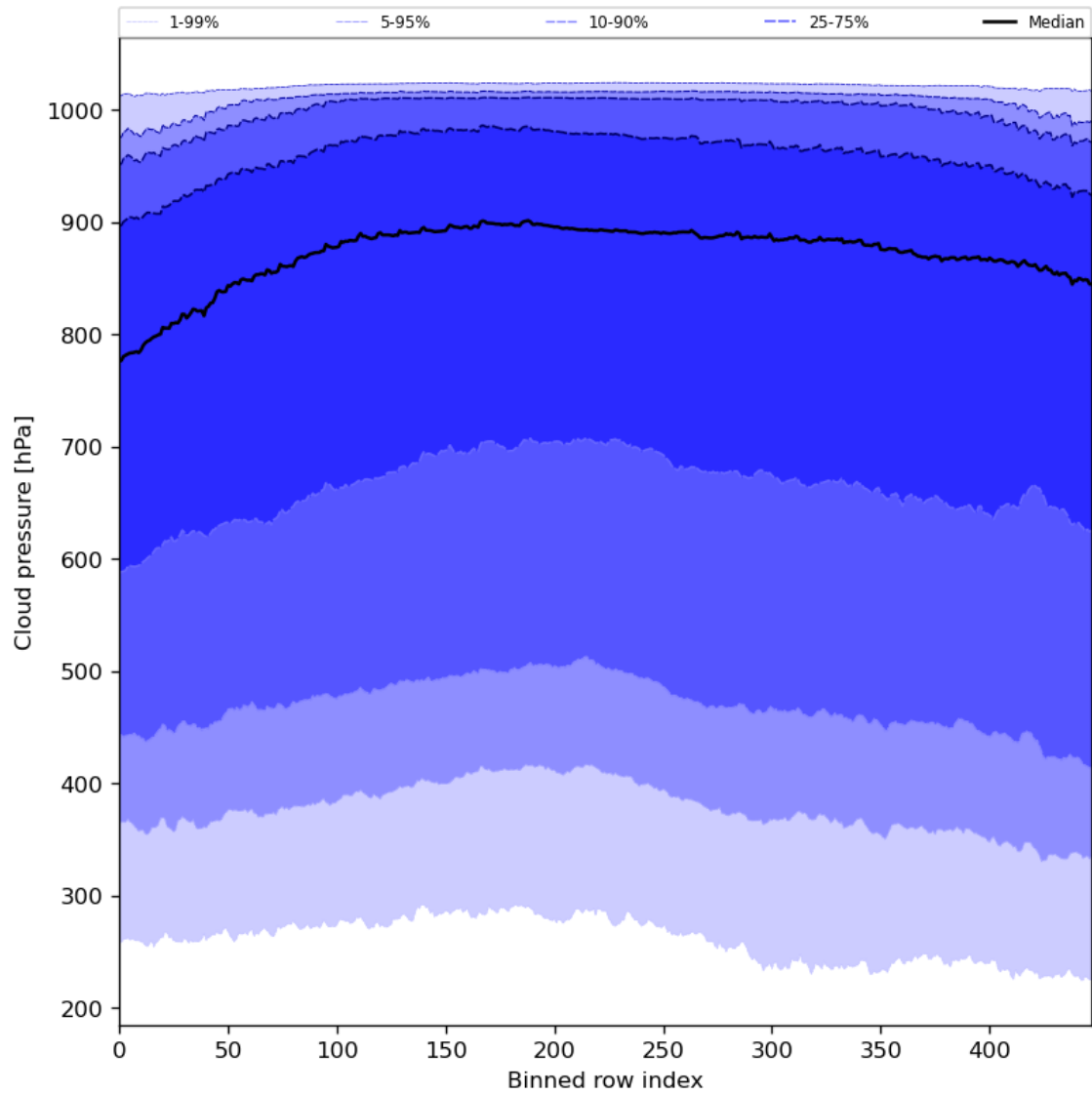
Figure 47: Along track statistics of “Cloud pressure” for 2024-04-13 to 2024-04-15
