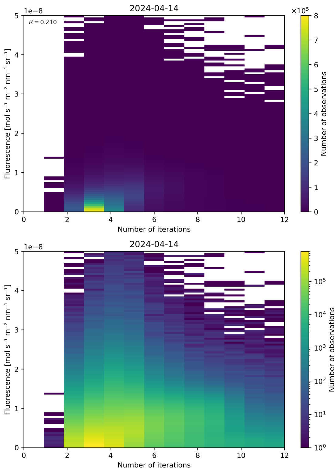
Figure 98: Scatter density plot of “Number of iterations” against “Fluorescence” for 2024-04-13 to 2024-04-15.
