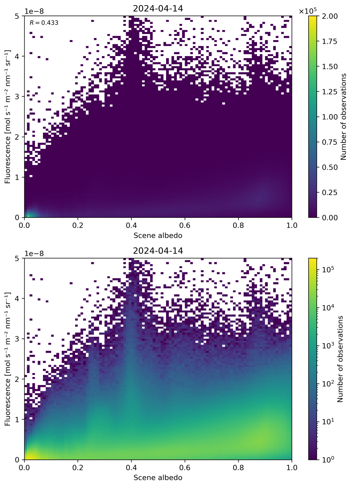
Figure 104: Scatter density plot of “Scene albedo” against “Fluorescence” for 2024-04-13 to 2024-04-15.
