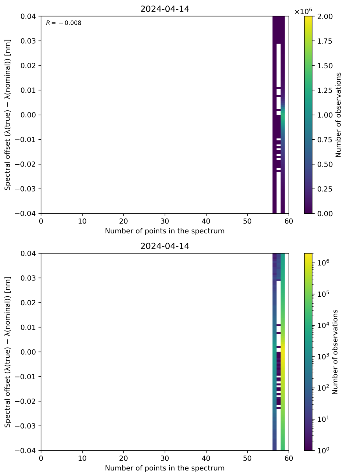
Figure 101: Scatter density plot of “Number of points in the spectrum” against “Spectral offset ( \lambda(\text{true}) - \lambda(\text{nominal}) )” for 2024-04-13 to 2024-04-15.
