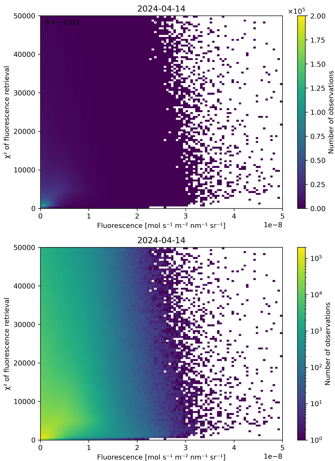
Figure 85: Scatter density plot of “Fluorescence” against “ \chi^2 of fluorescence retrieval” for 2024-04-13 to 2024-04-15.
