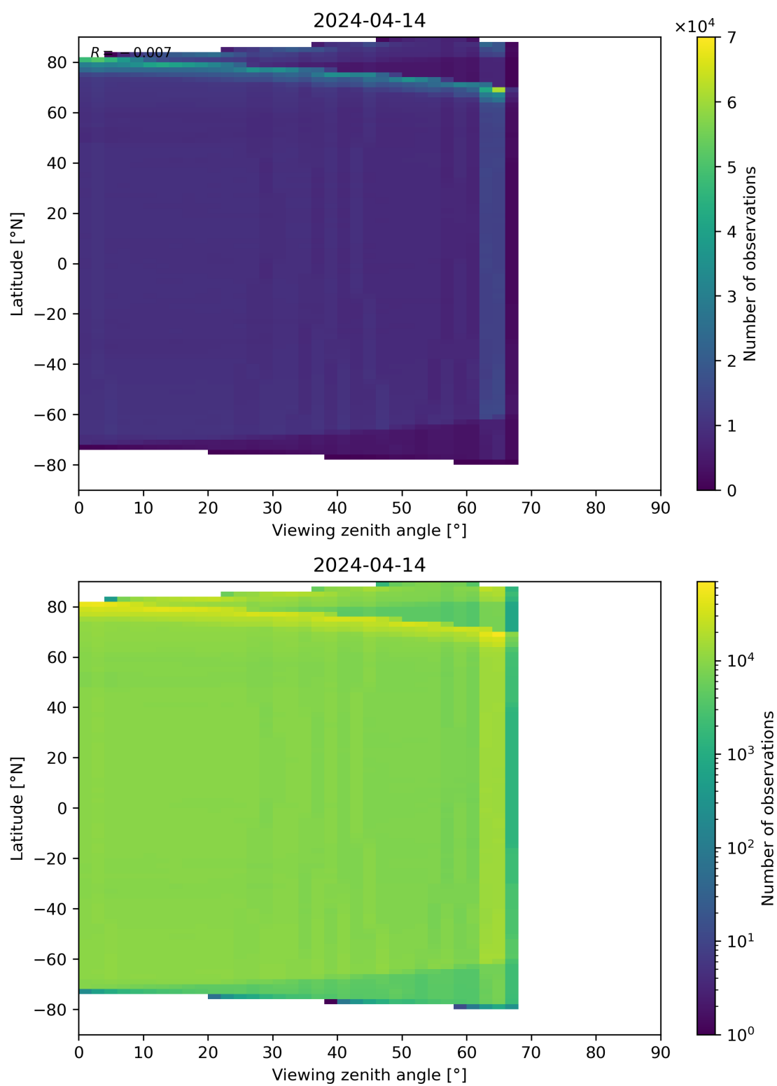
Figure 123: Scatter density plot of “Viewing zenith angle” against “Latitude” for 2024-04-13 to 2024-04-15.
