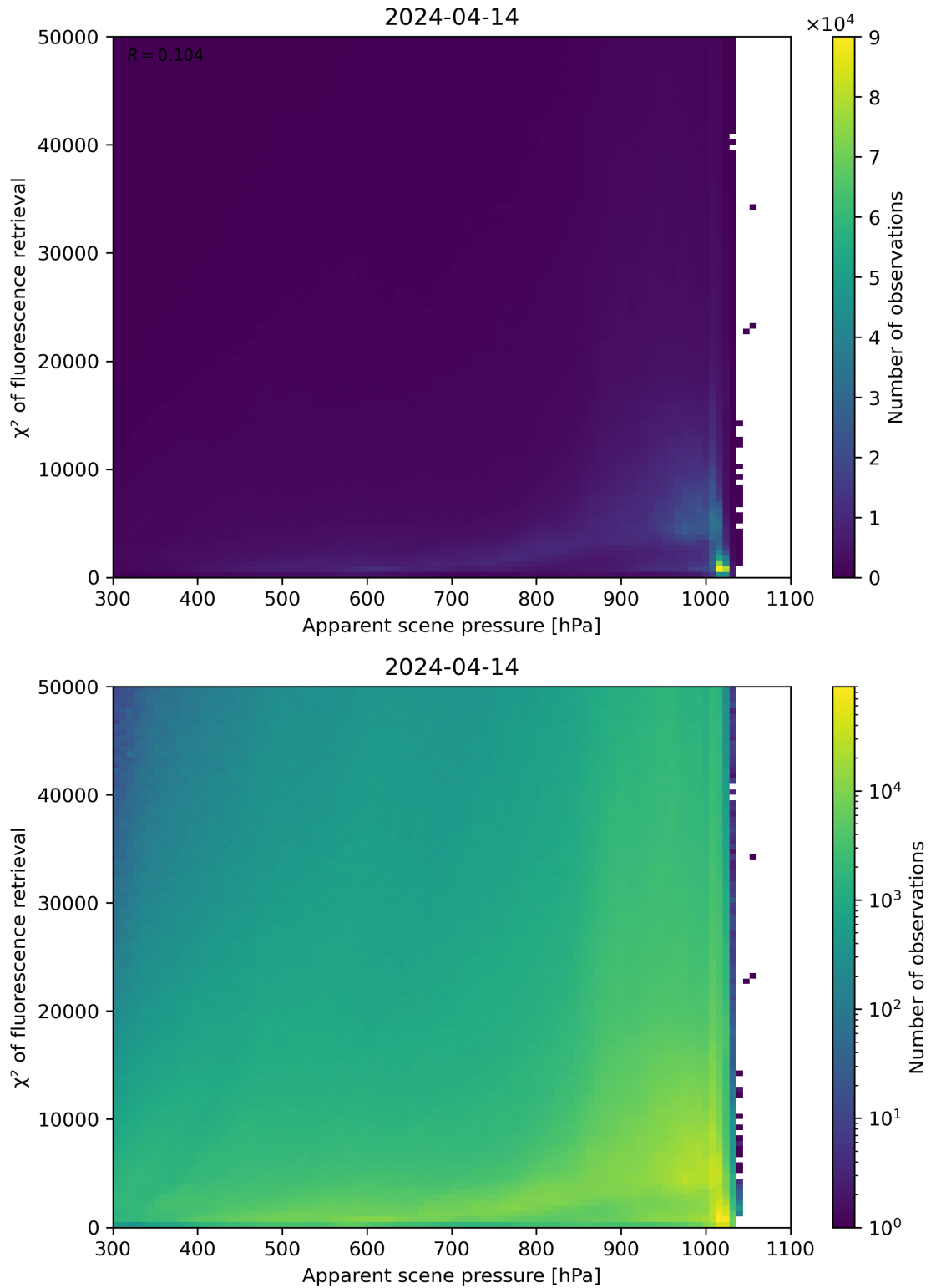
Figure 63: Scatter density plot of “Apparent scene pressure” against “ \chi^2 of fluorescence retrieval” for 2024-04-13 to 2024-04-15.
