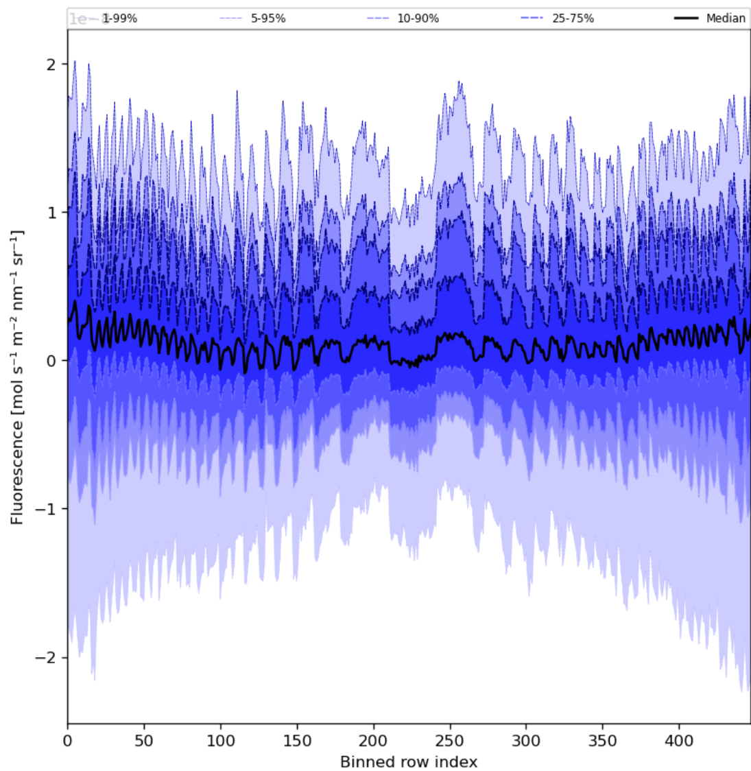
Figure 57: Along track statistics of “Fluorescence” for 2024-04-13 to 2024-04-15
