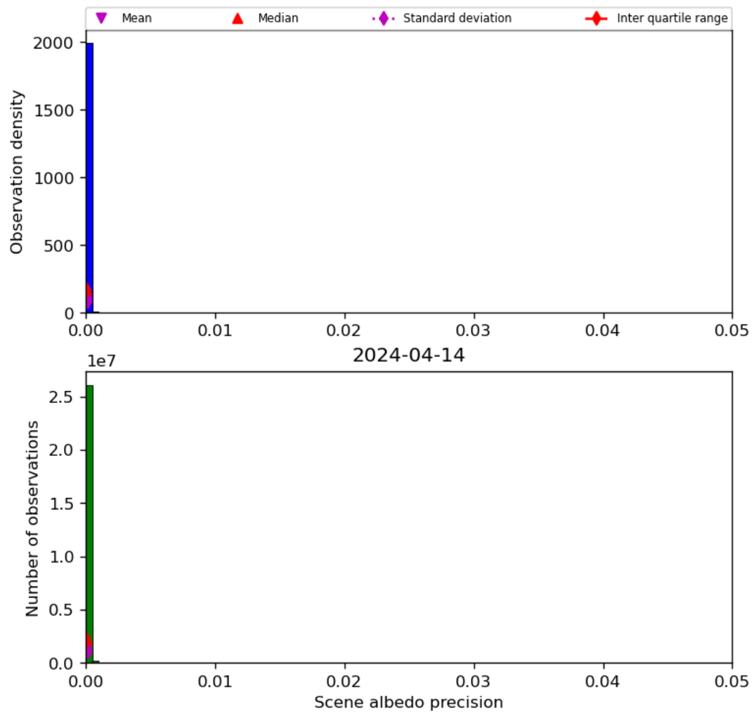
Figure 35: Histogram of “Scene albedo precision” for 2024-04-13 to 2024-04-15
