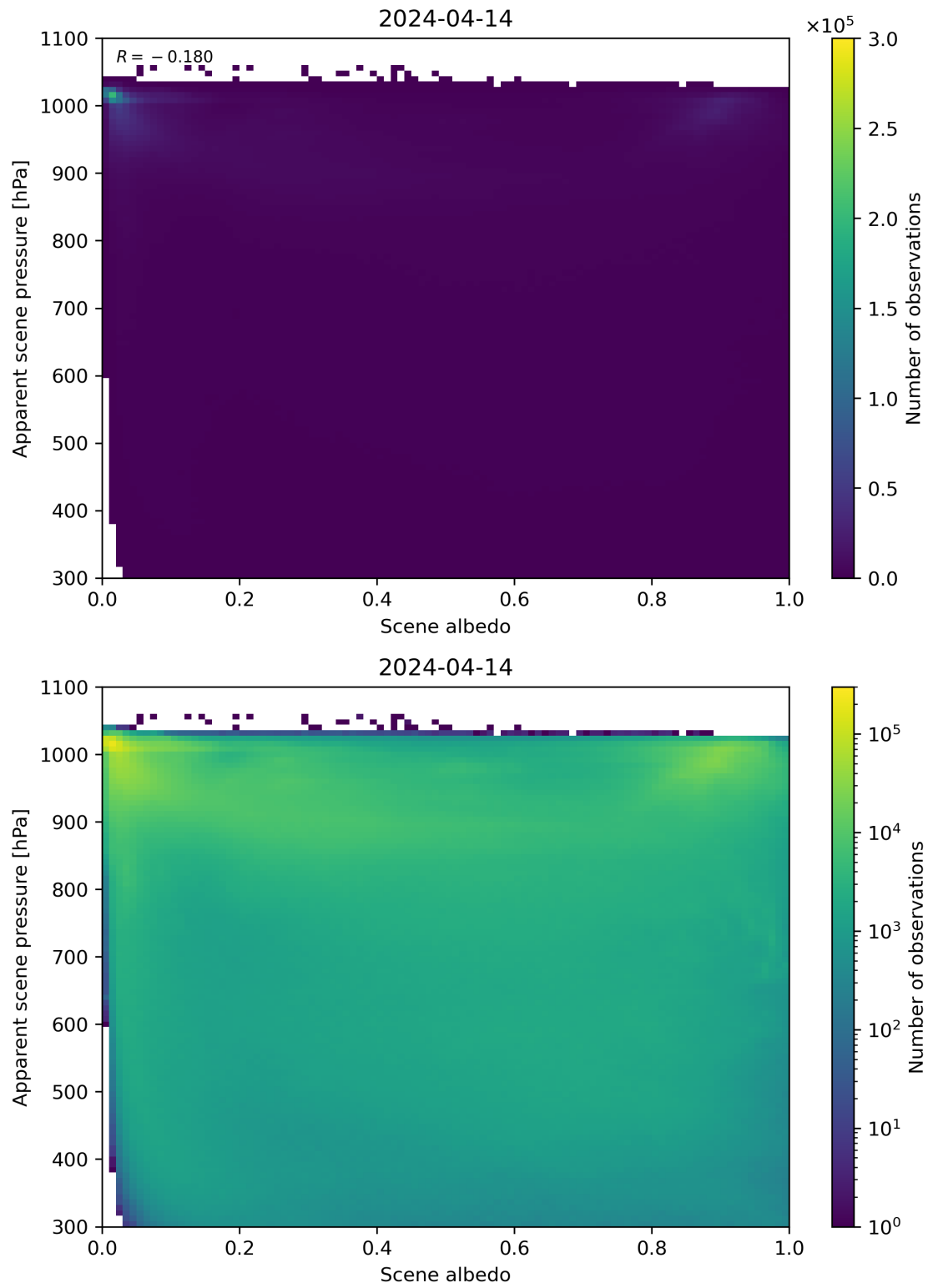
Figure 102: Scatter density plot of “Scene albedo” against “Apparent scene pressure” for 2024-04-13 to 2024-04-15.
