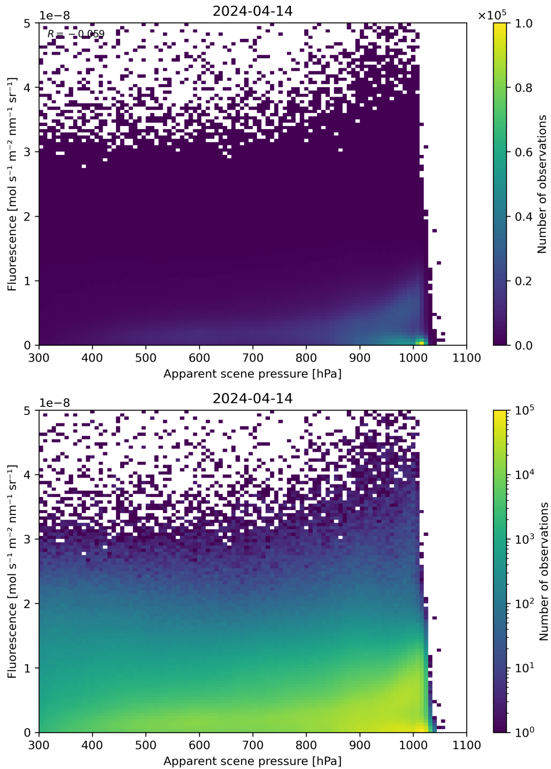
Figure 64: Scatter density plot of “Apparent scene pressure” against “Fluorescence” for 2024-04-13 to 2024-04-15.
