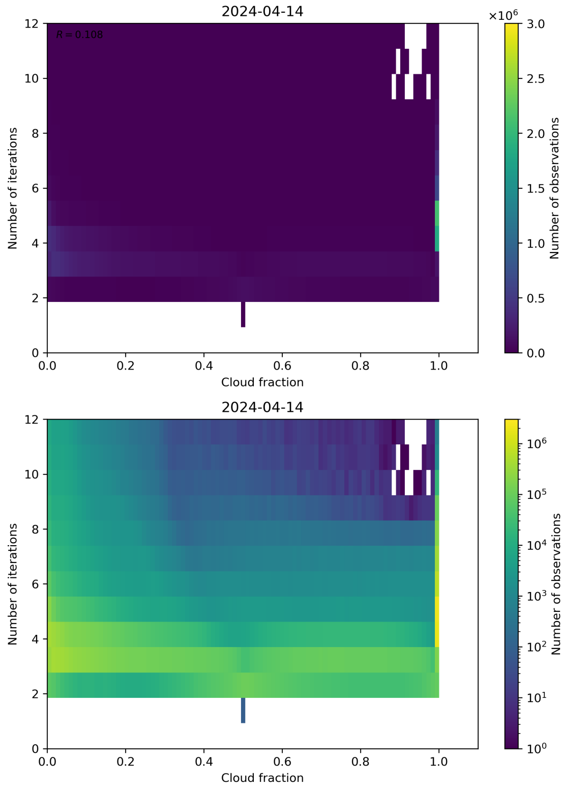
Figure 73: Scatter density plot of “Cloud fraction” against “Number of iterations” for 2024-04-13 to 2024-04-15.
