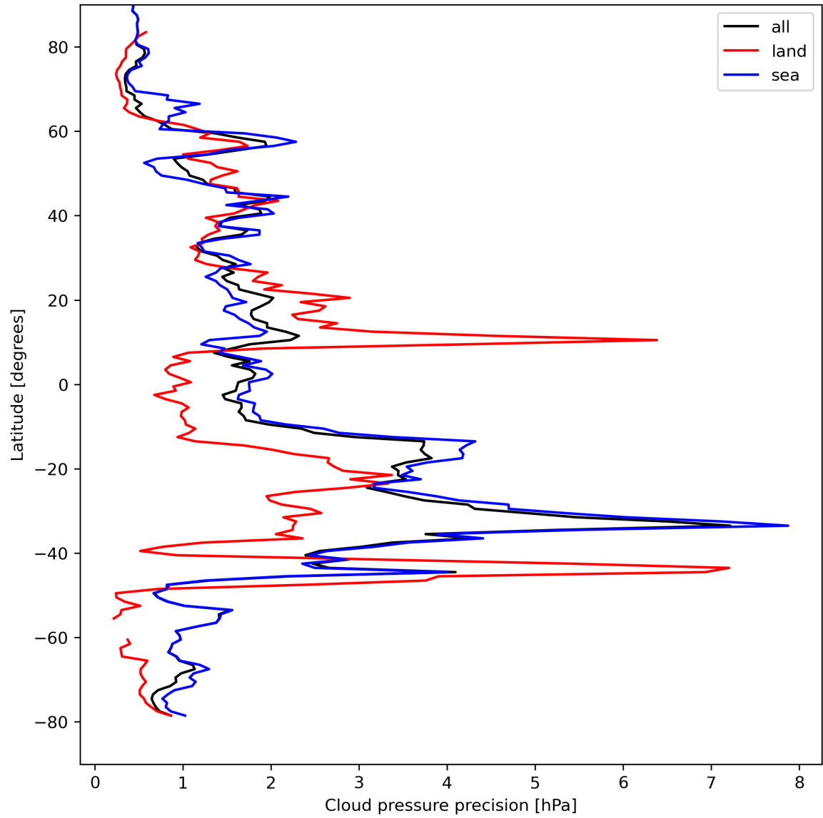
Figure 14: Zonal average of “Cloud pressure precision” for 2024-04-13 to 2024-04-15.
