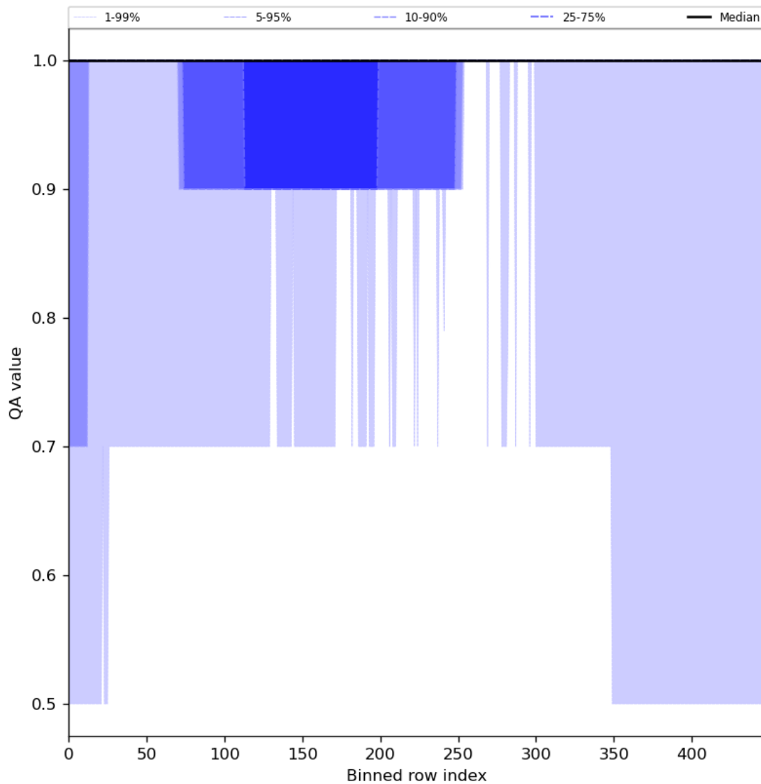
Figure 46: Along track statistics of “QA value” for 2024-04-13 to 2024-04-15
