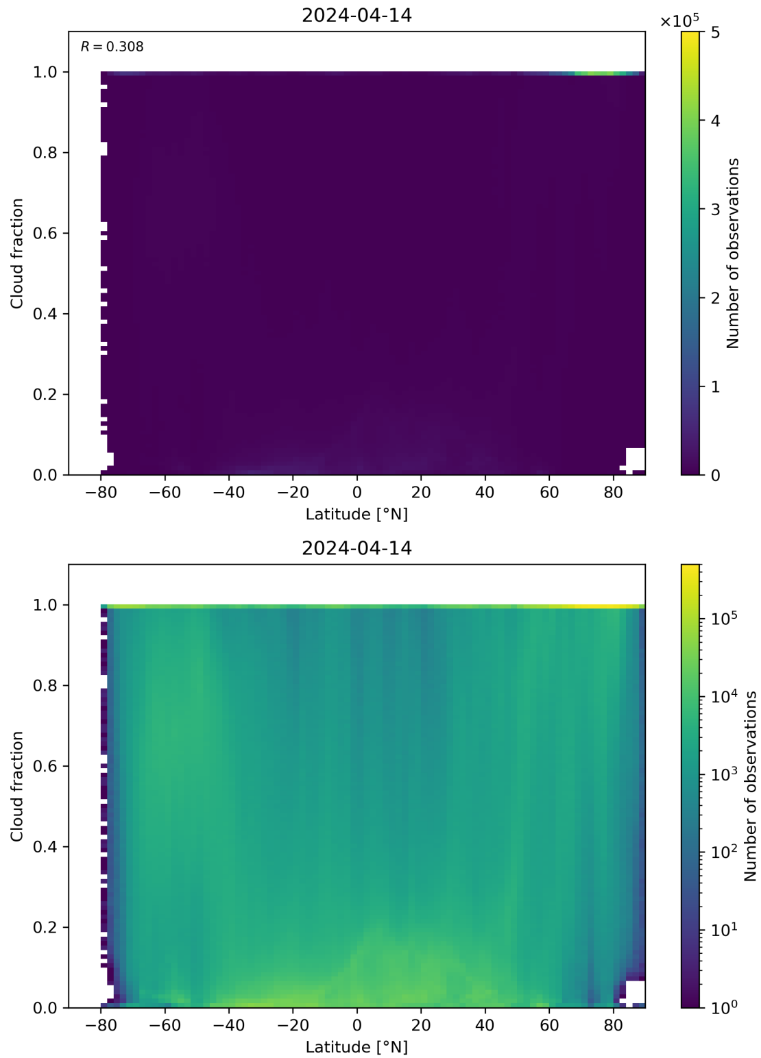
Figure 90: Scatter density plot of “Latitude” against “Cloud fraction” for 2024-04-13 to 2024-04-15.
