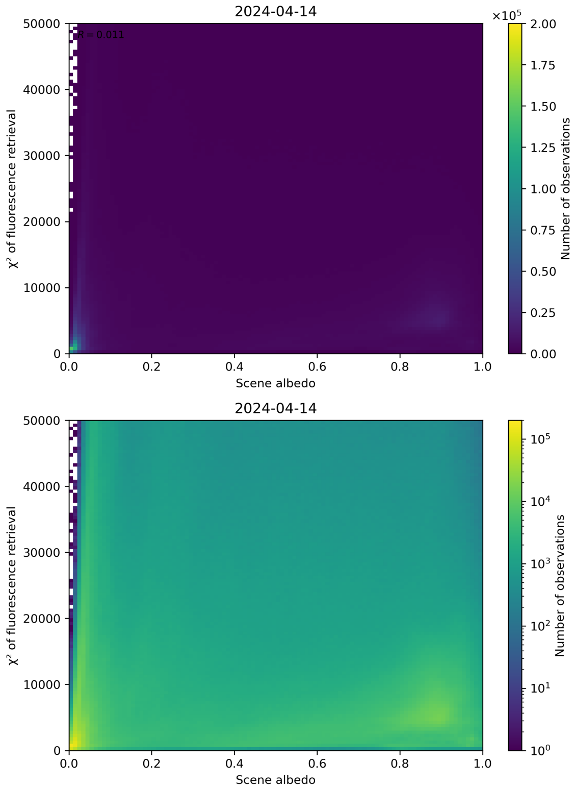
Figure 103: Scatter density plot of “Scene albedo” against “ \chi^2 of fluorescence retrieval” for 2024-04-13 to 2024-04-15.
