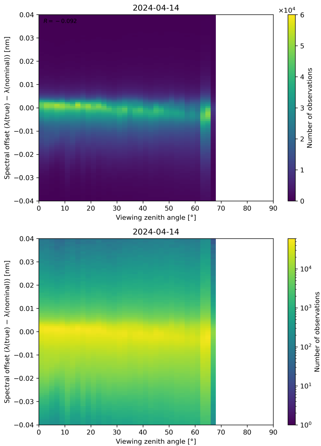
Figure 128: Scatter density plot of “Viewing zenith angle” against “Spectral offset ( \lambda(\text{true}) - \lambda(\text{nominal}) )” for 2024-04-13 to 2024-04-15.
