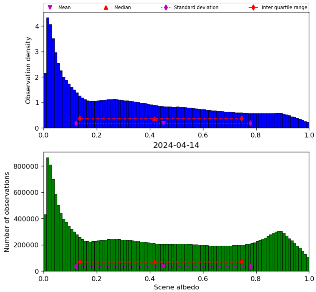
Figure 34: Histogram of “Scene albedo” for 2024-04-13 to 2024-04-15
