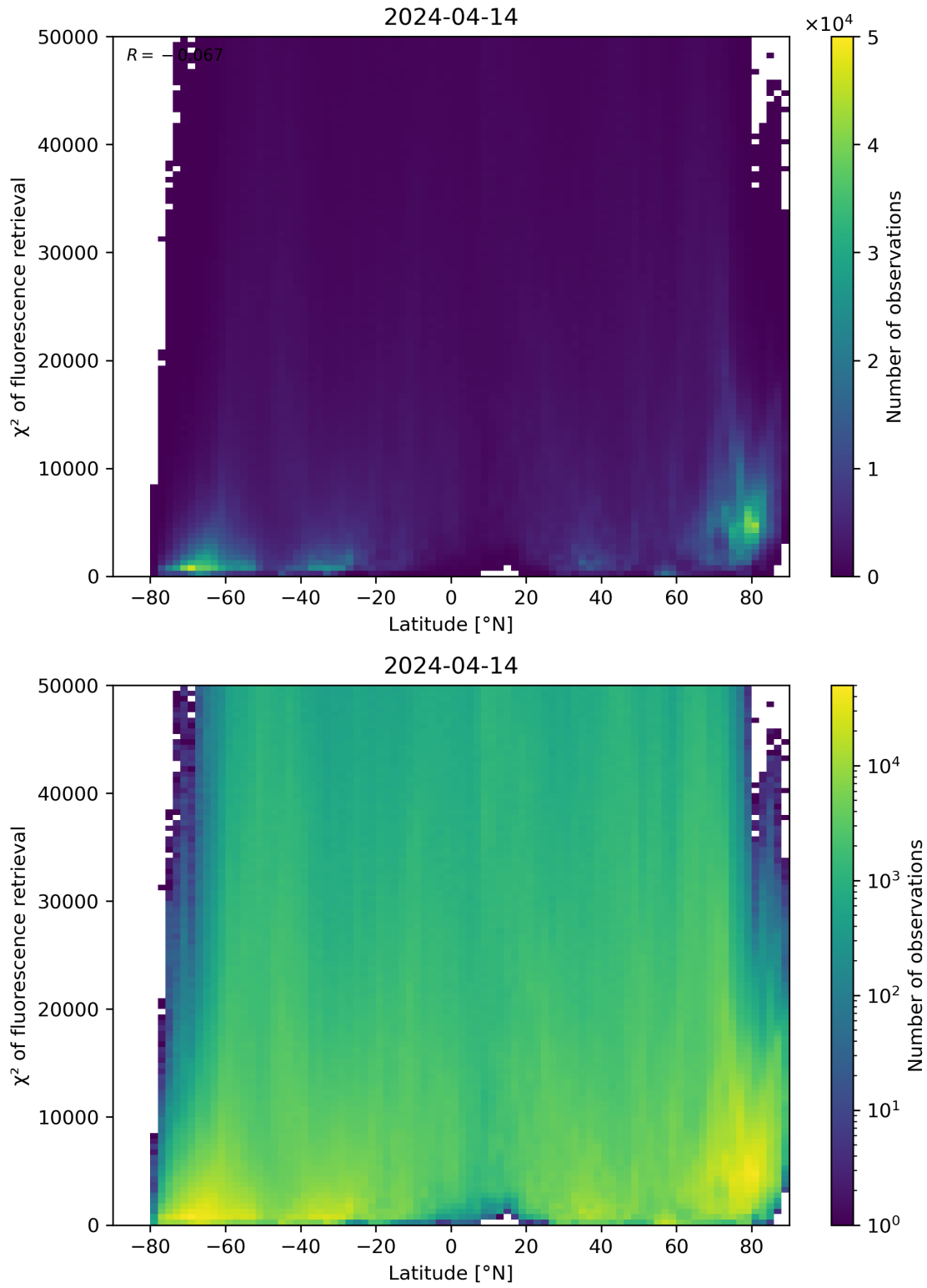
Figure 89: Scatter density plot of “Latitude” against “ \chi^2 of fluorescence retrieval” for 2024-04-13 to 2024-04-15.
