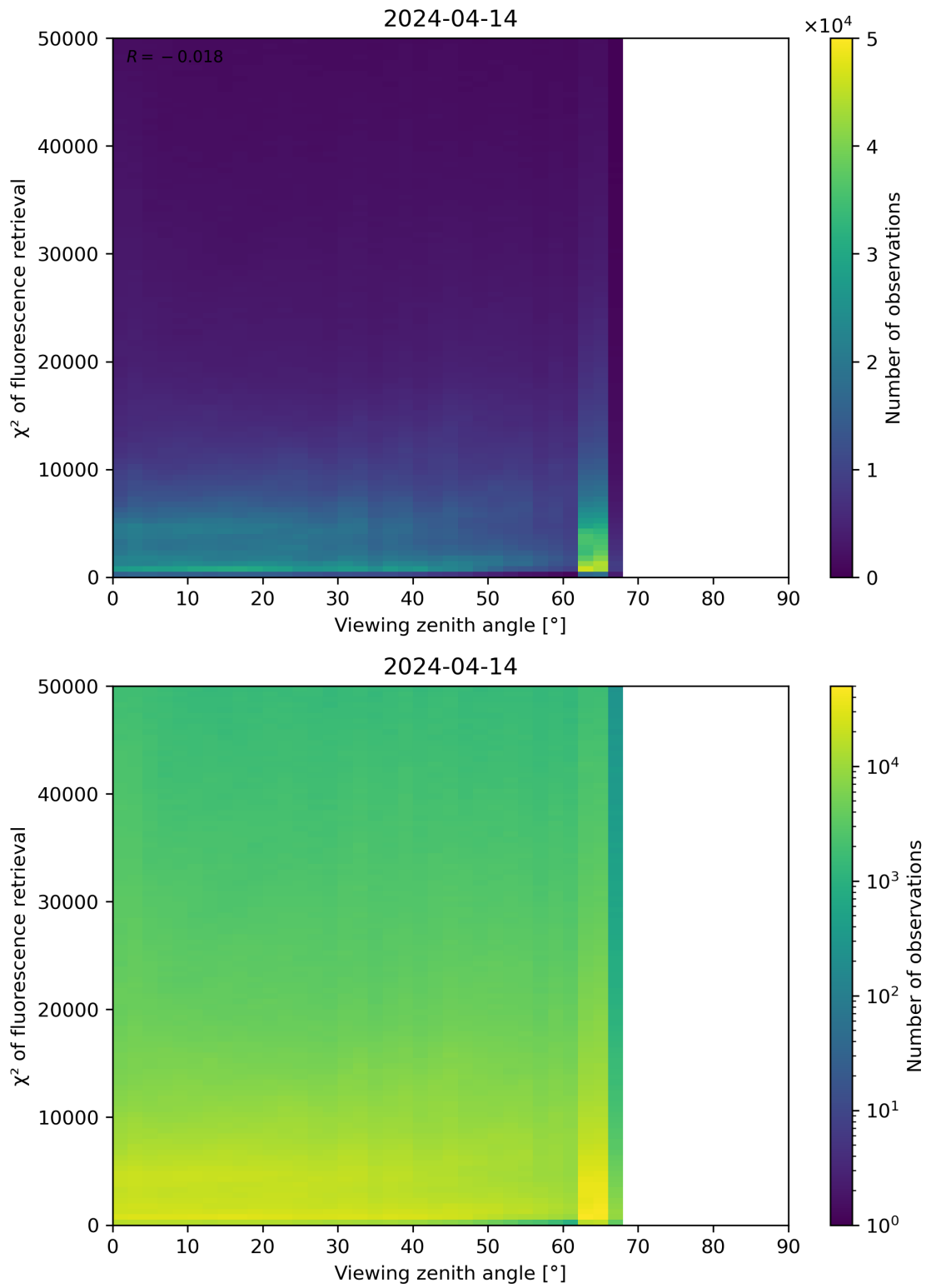
Figure 119: Scatter density plot of “Viewing zenith angle” against “ \chi^2 of fluorescence retrieval” for 2024-04-13 to 2024-04-15.
