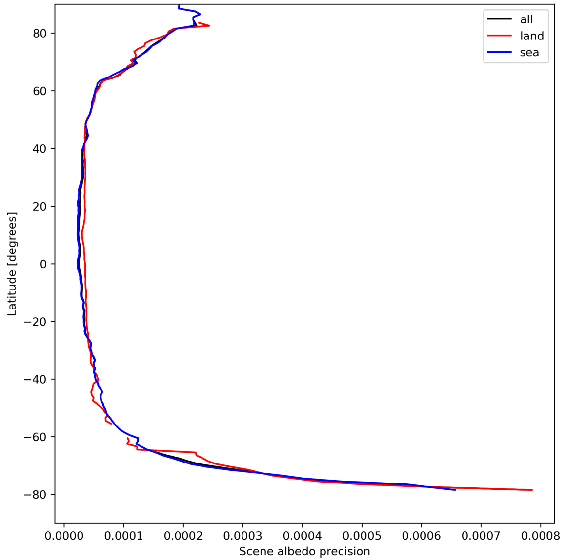
Figure 18: Zonal average of “Scene albedo precision” for 2024-04-13 to 2024-04-15.
