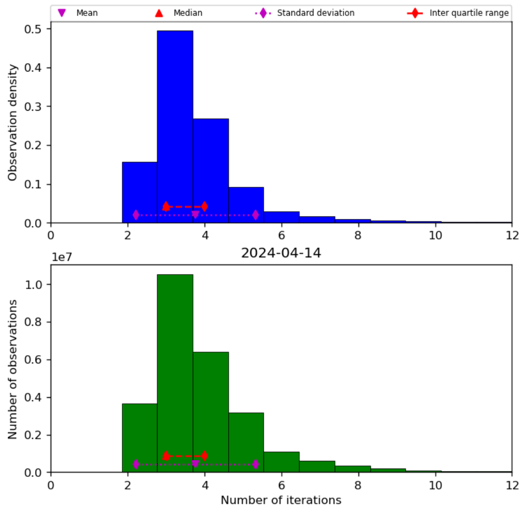
Figure 39: Histogram of “Number of iterations” for 2024-04-13 to 2024-04-15
