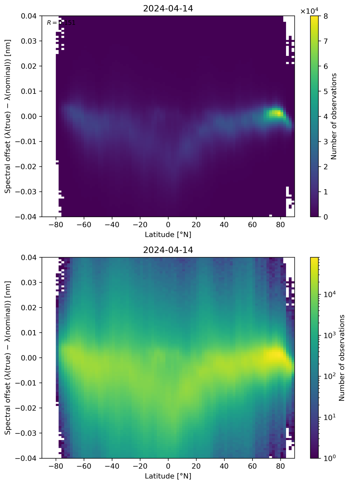
Figure 96: Scatter density plot of “Latitude” against “Spectral offset ( \lambda(\text{true}) - \lambda(\text{nominal}) )” for 2024-04-13 to 2024-04-15.
