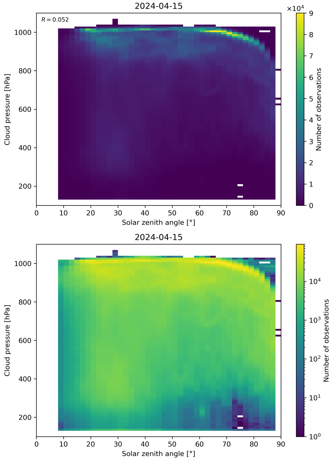
Figure 111: Scatter density plot of “Solar zenith angle” against “Cloud pressure” for 2024-04-15 to 2024-04-16.
