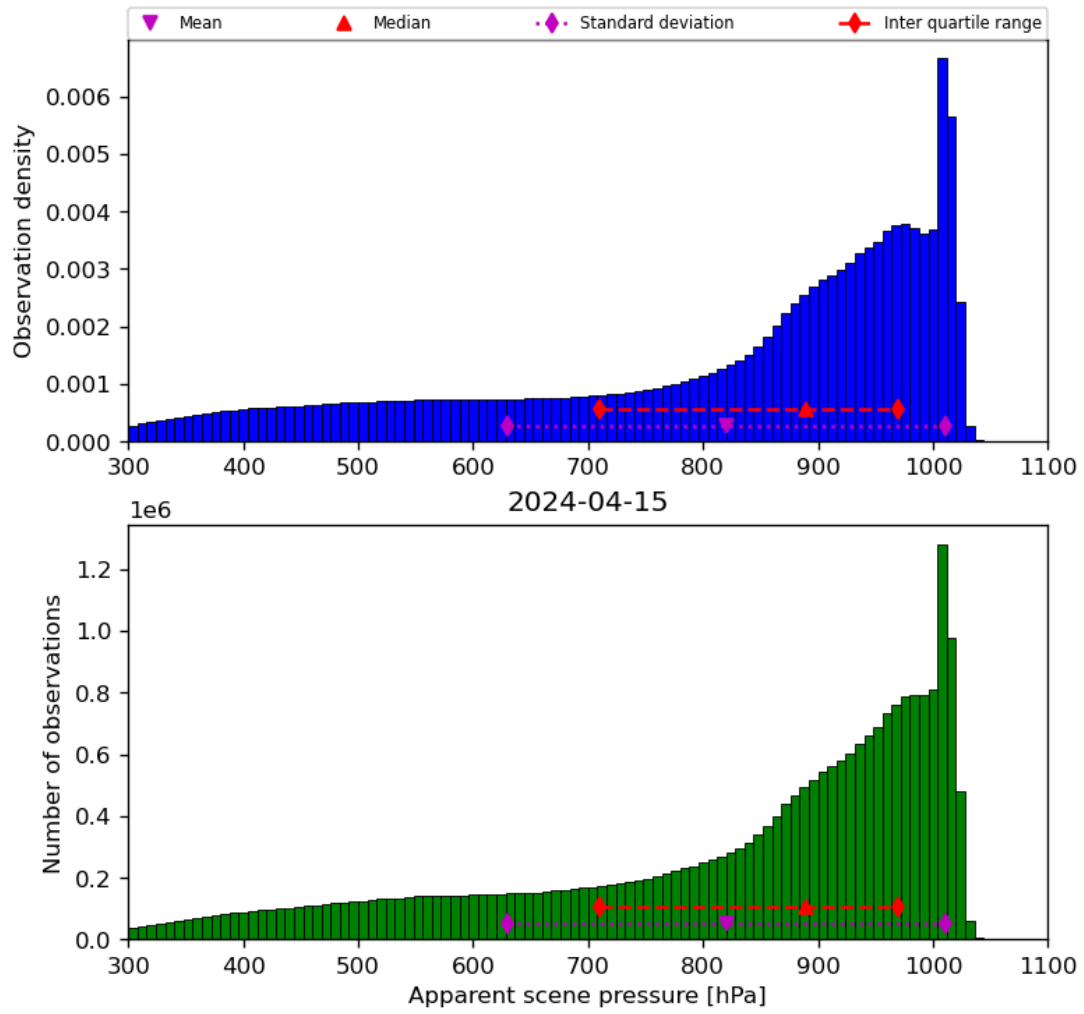
Figure 36: Histogram of “Apparent scene pressure” for 2024-04-15 to 2024-04-16
