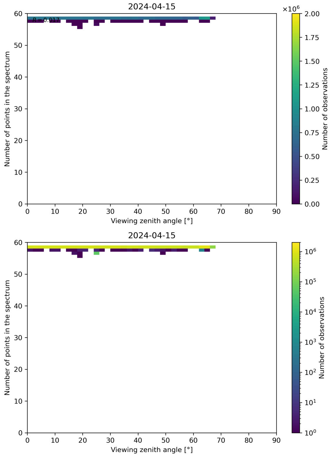
Figure 125: Scatter density plot of “Viewing zenith angle” against “Number of points in the spectrum” for 2024-04-15 to 2024-04-16.
