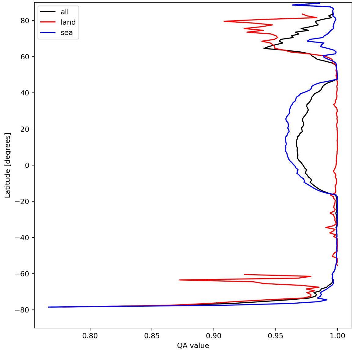
Figure 12: Zonal average of “QA value” for 2024-04-15 to 2024-04-16.
