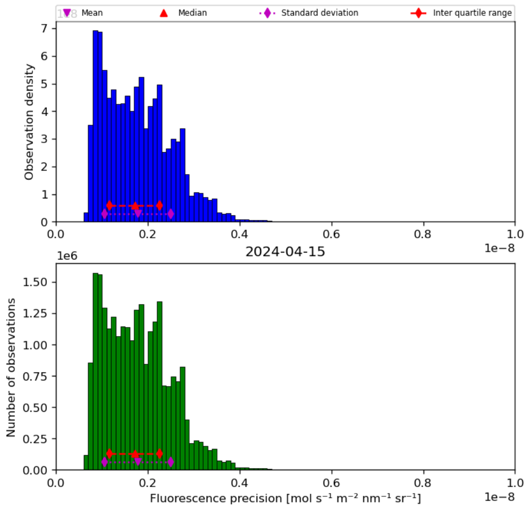
Figure 41: Histogram of “Fluorescence precision” for 2024-04-15 to 2024-04-16
