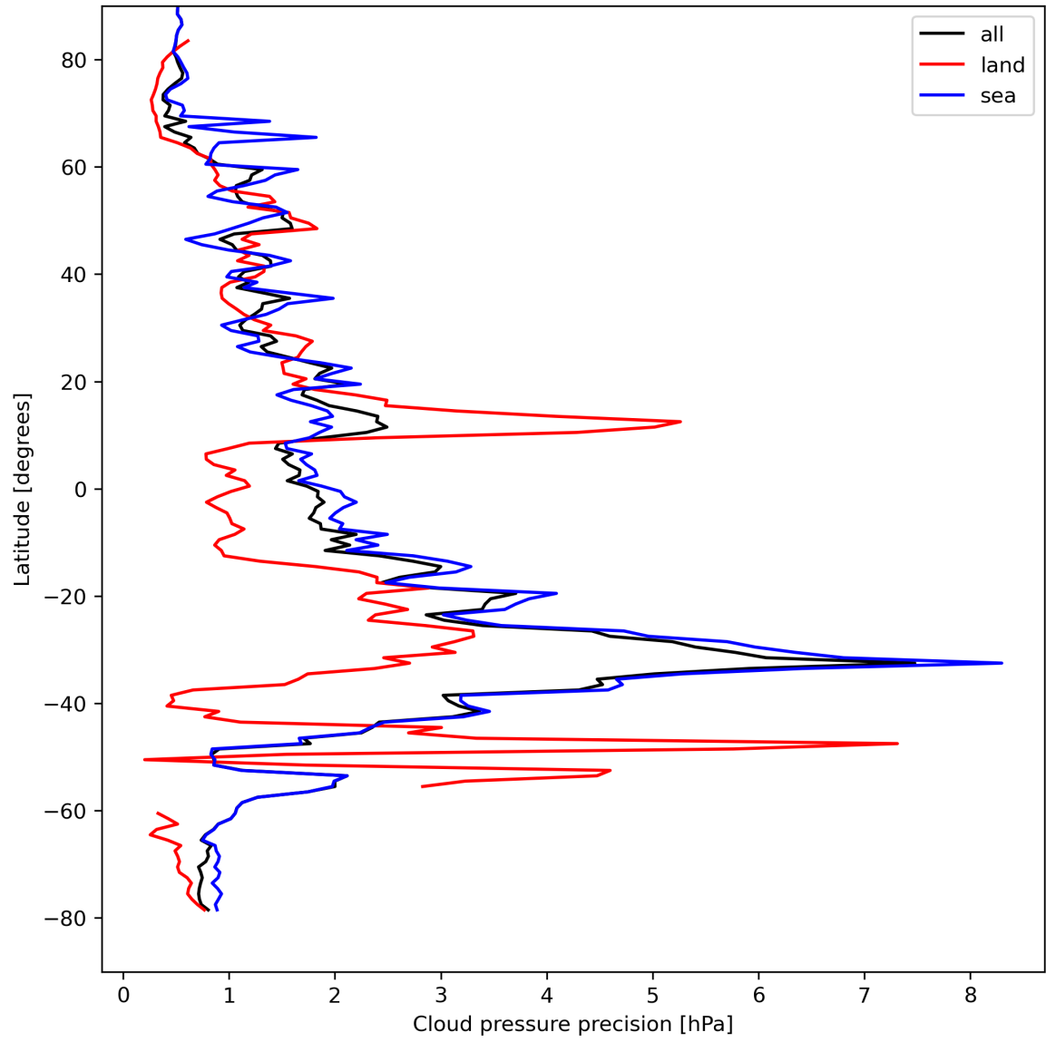
Figure 14: Zonal average of “Cloud pressure precision” for 2024-04-15 to 2024-04-16.
