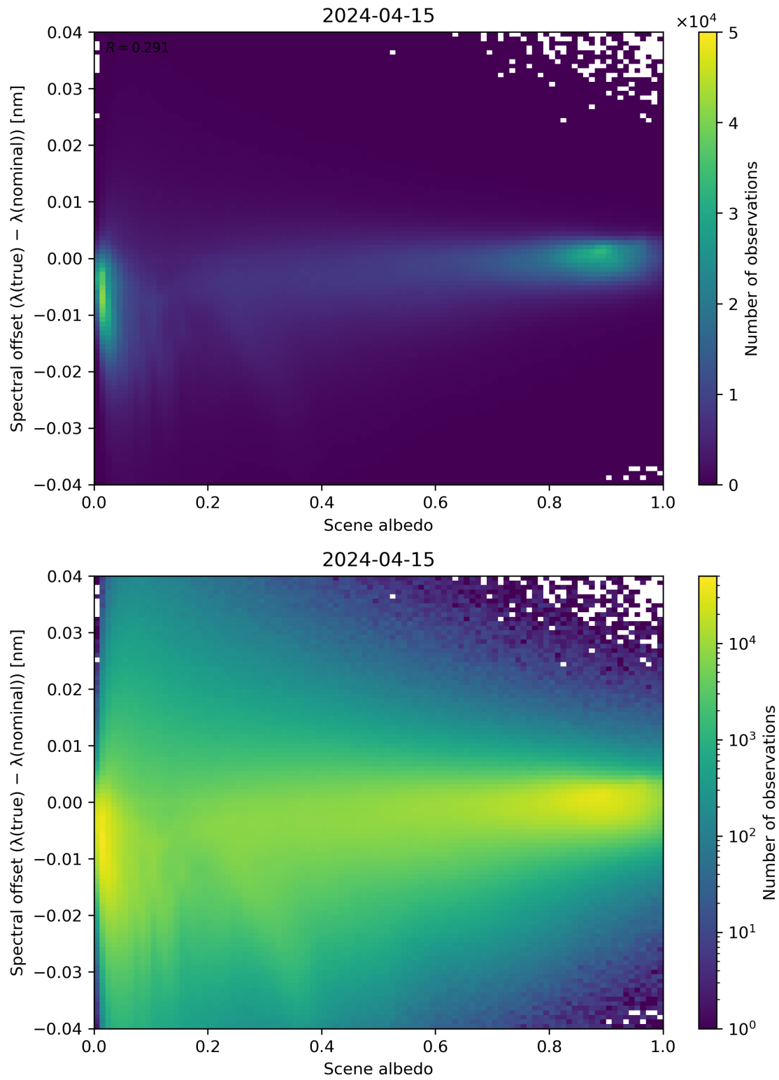
Figure 107: Scatter density plot of “Scene albedo” against “Spectral offset ( \lambda(\text{true}) - \lambda(\text{nominal}) )” for 2024-04-15 to 2024-04-16.
