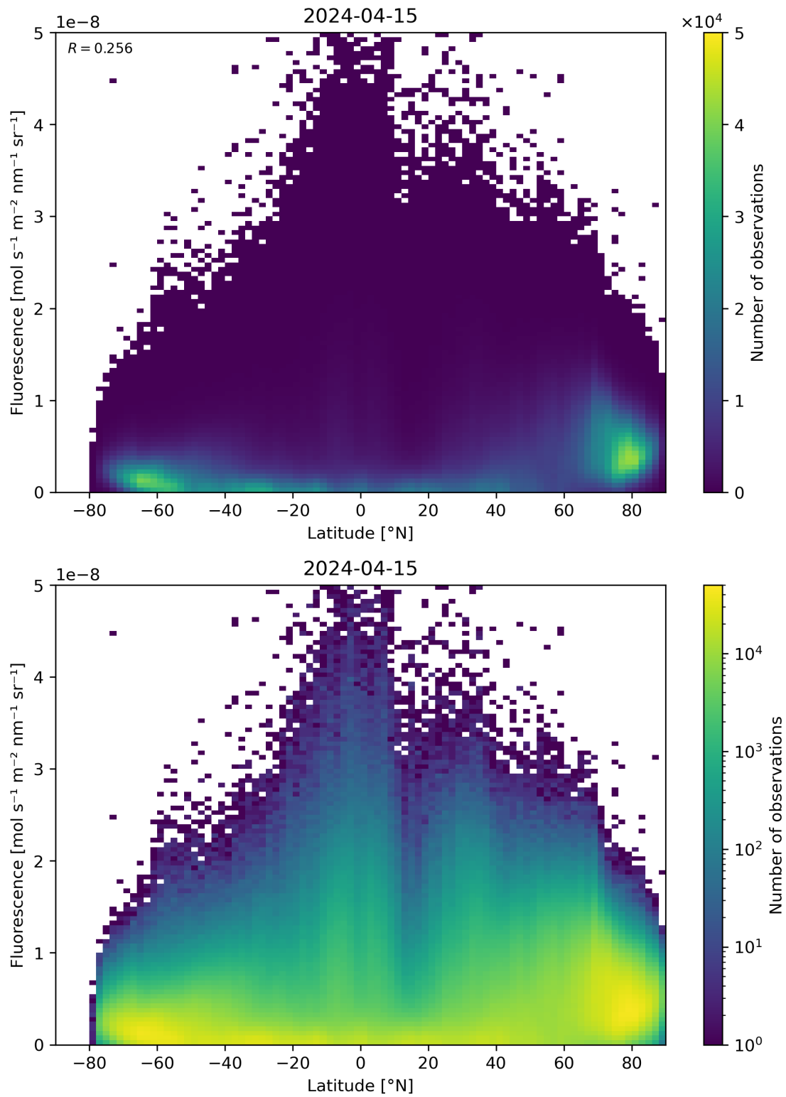
Figure 92: Scatter density plot of “Latitude” against “Fluorescence” for 2024-04-15 to 2024-04-16.
