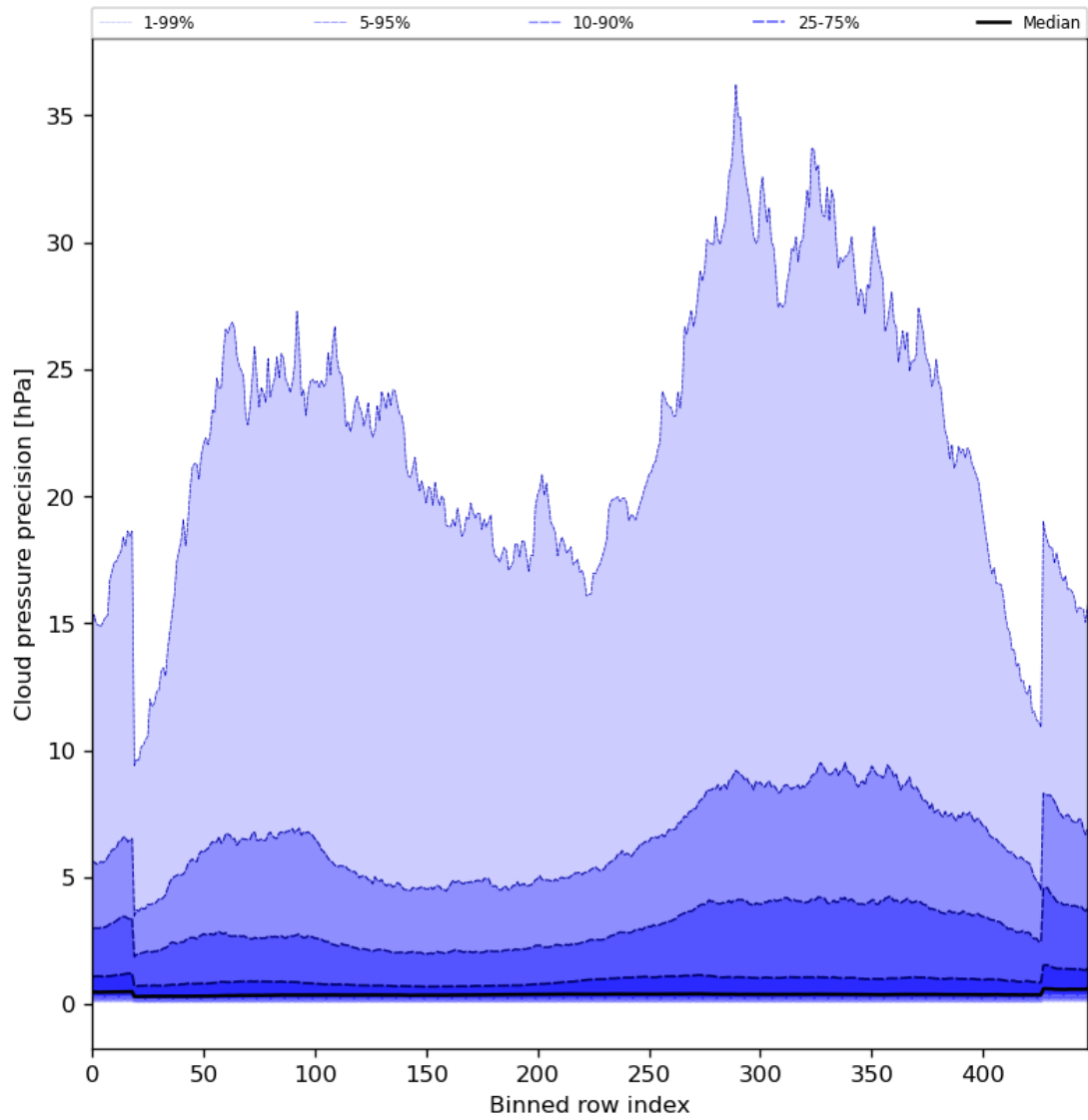
Figure 48: Along track statistics of “Cloud pressure precision” for 2024-04-15 to 2024-04-16
