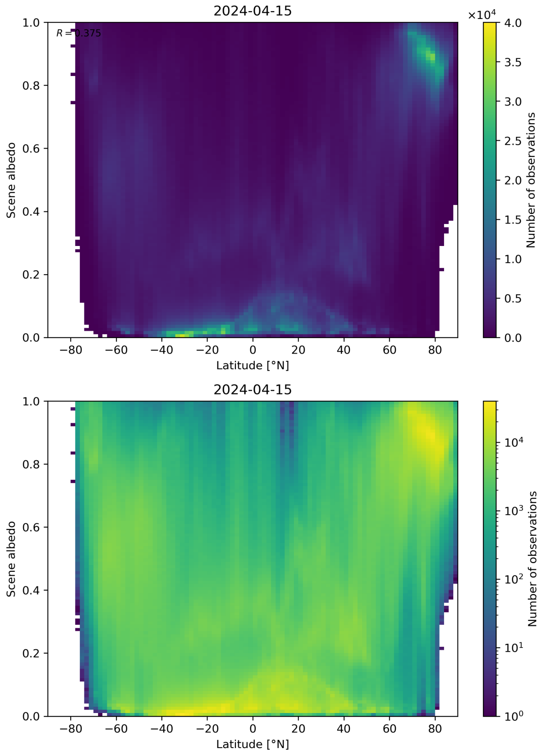
Figure 95: Scatter density plot of “Latitude” against “Scene albedo” for 2024-04-15 to 2024-04-16.
