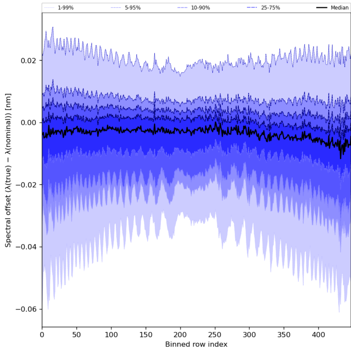
Figure 62: Along track statistics of “Spectral offset ( \lambda(\text{true}) - \lambda(\text{nominal}) )” for 2024-04-15 to 2024-04-16
