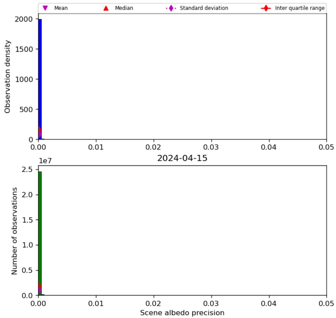
Figure 35: Histogram of “Scene albedo precision” for 2024-04-15 to 2024-04-16
