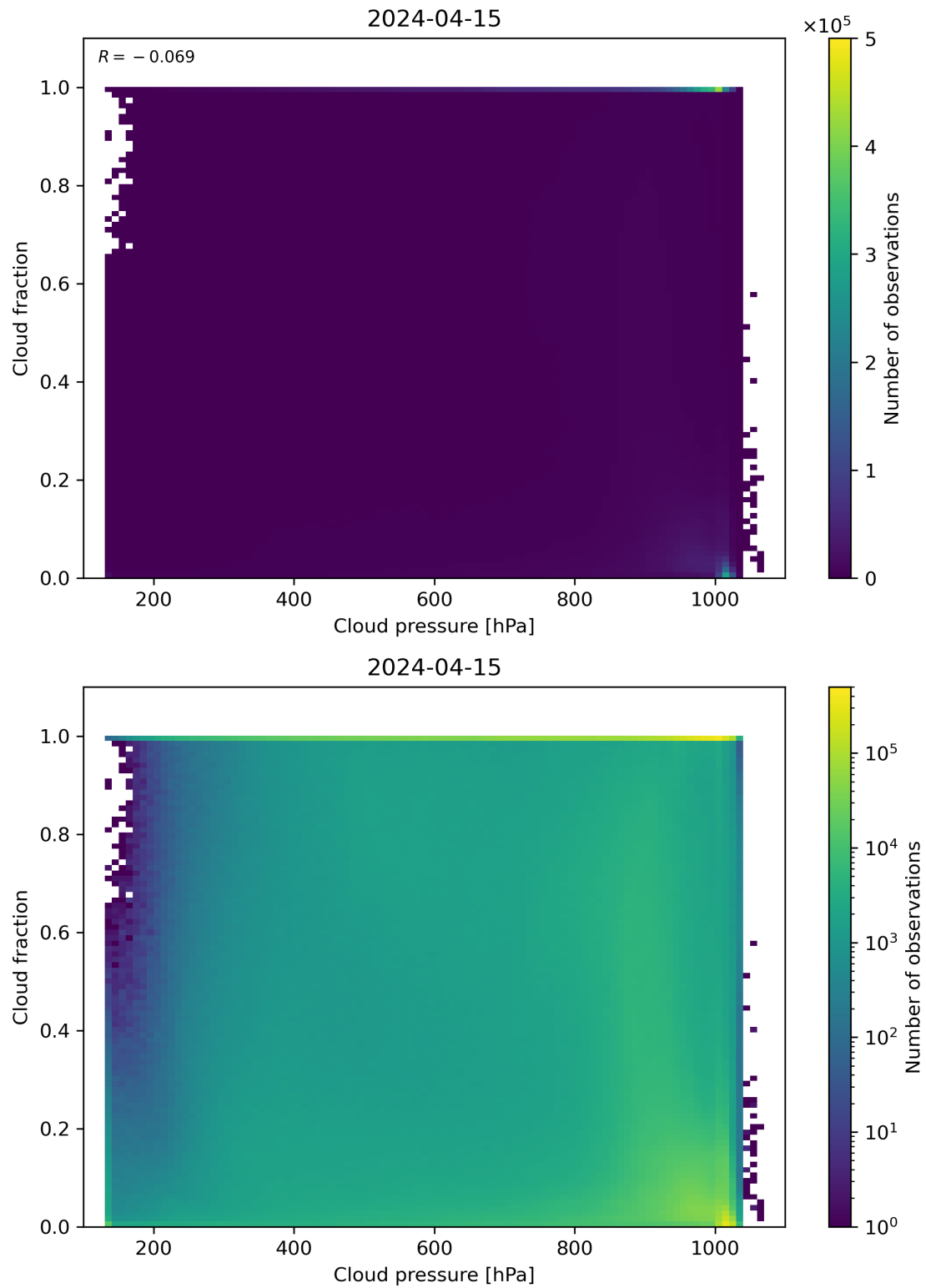
Figure 79: Scatter density plot of “Cloud pressure” against “Cloud fraction” for 2024-04-15 to 2024-04-16.
