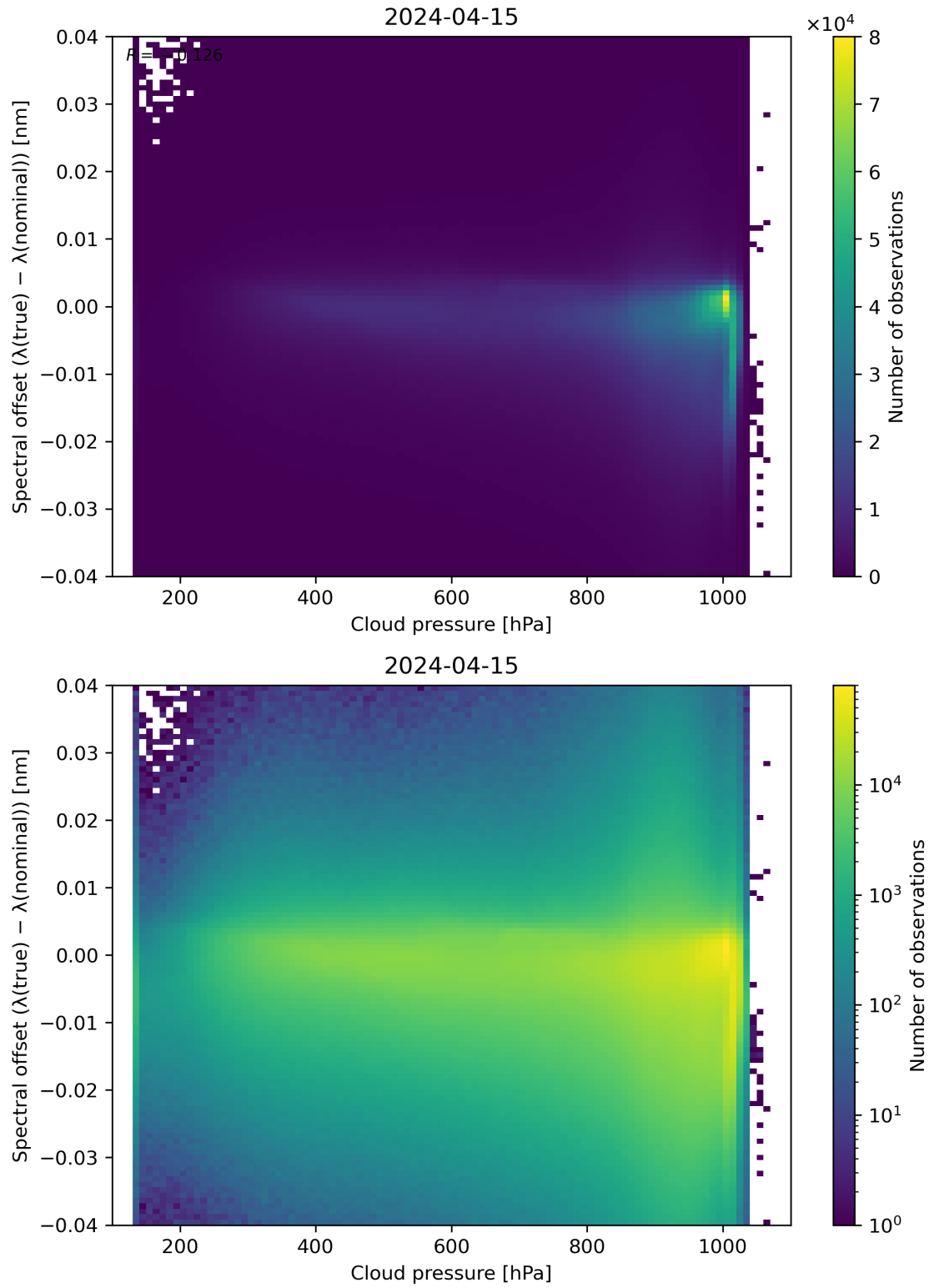
Figure 84: Scatter density plot of “Cloud pressure” against “Spectral offset ( \lambda(\text{true}) - \lambda(\text{nominal}) )” for 2024-04-15 to 2024-04-16.
