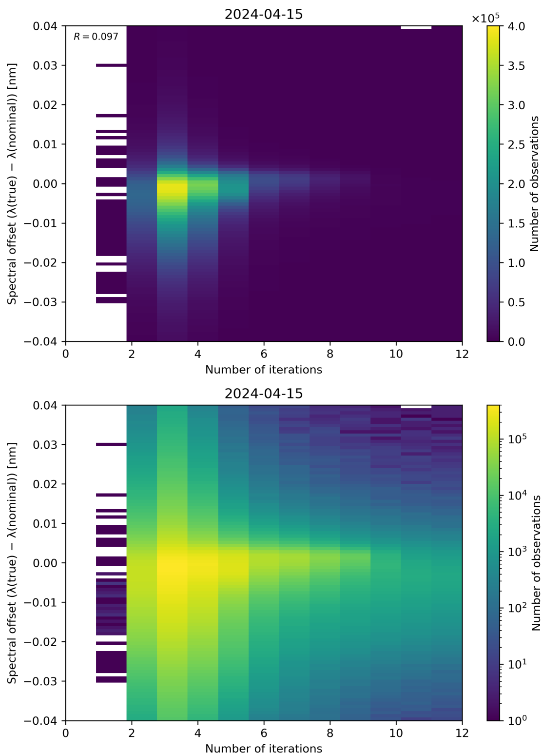
Figure 100: Scatter density plot of “Number of iterations” against “Spectral offset ( \lambda(\text{true}) - \lambda(\text{nominal}) )” for 2024-04-15 to 2024-04-16.
