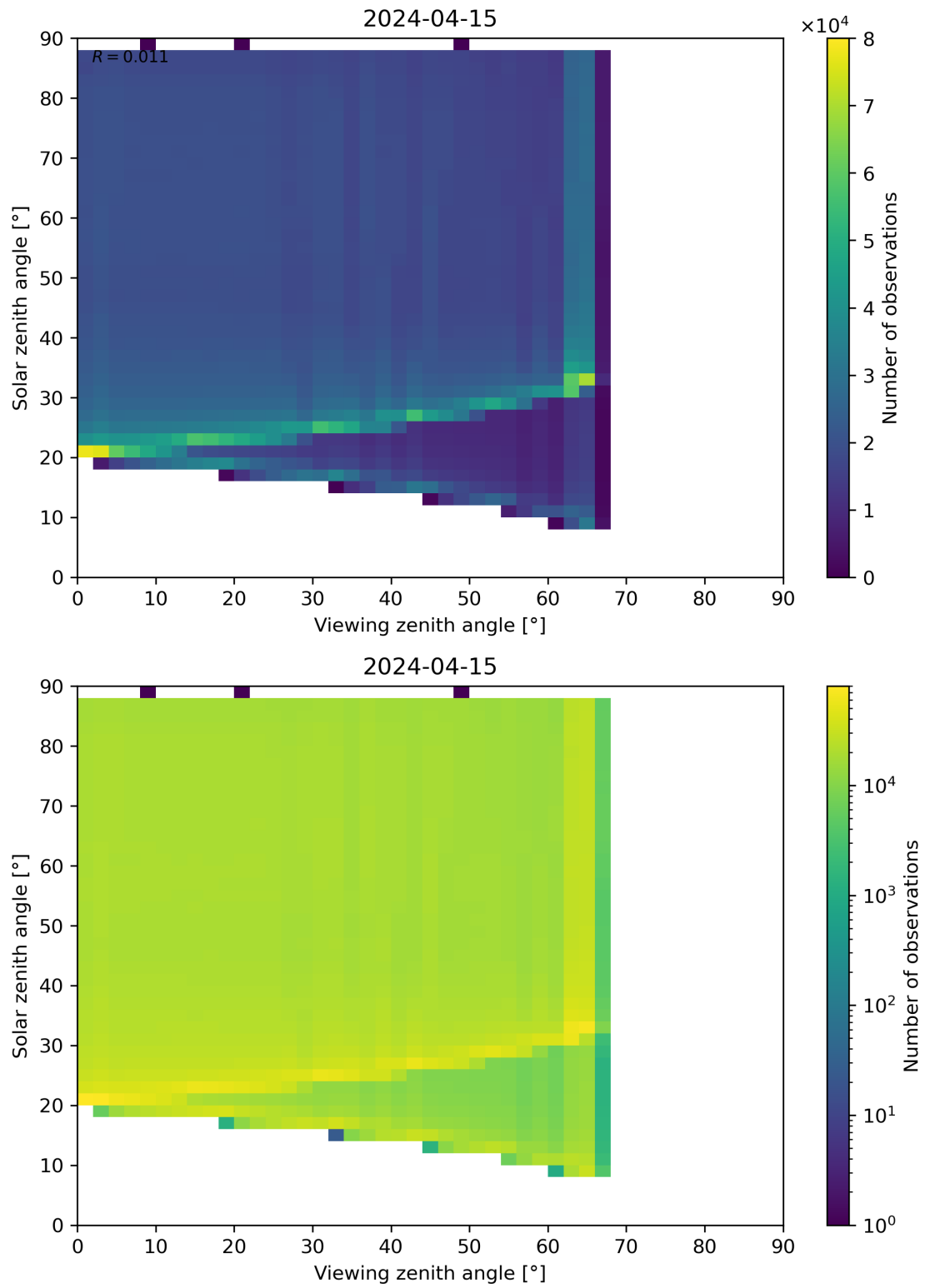
Figure 127: Scatter density plot of “Viewing zenith angle” against “Solar zenith angle” for 2024-04-15 to 2024-04-16.
