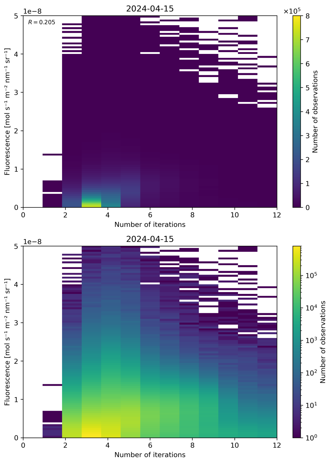
Figure 98: Scatter density plot of “Number of iterations” against “Fluorescence” for 2024-04-15 to 2024-04-16.
