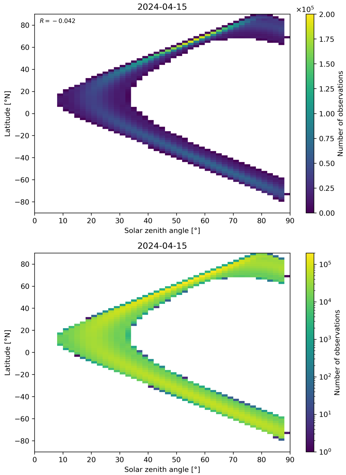
Figure 113: Scatter density plot of “Solar zenith angle” against “Latitude” for 2024-04-15 to 2024-04-16.
