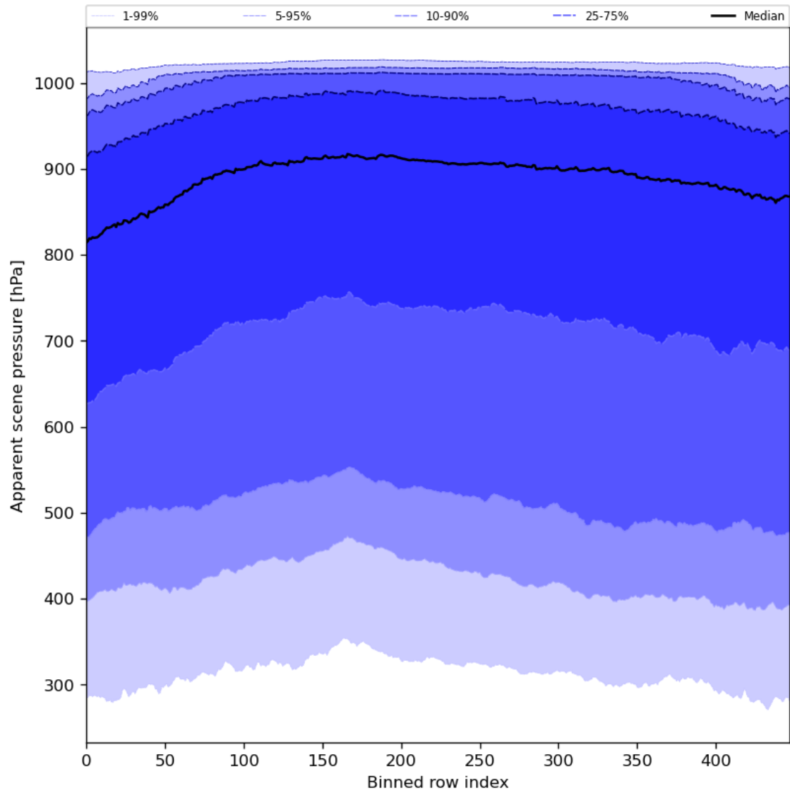
Figure 53: Along track statistics of “Apparent scene pressure” for 2024-04-15 to 2024-04-16
