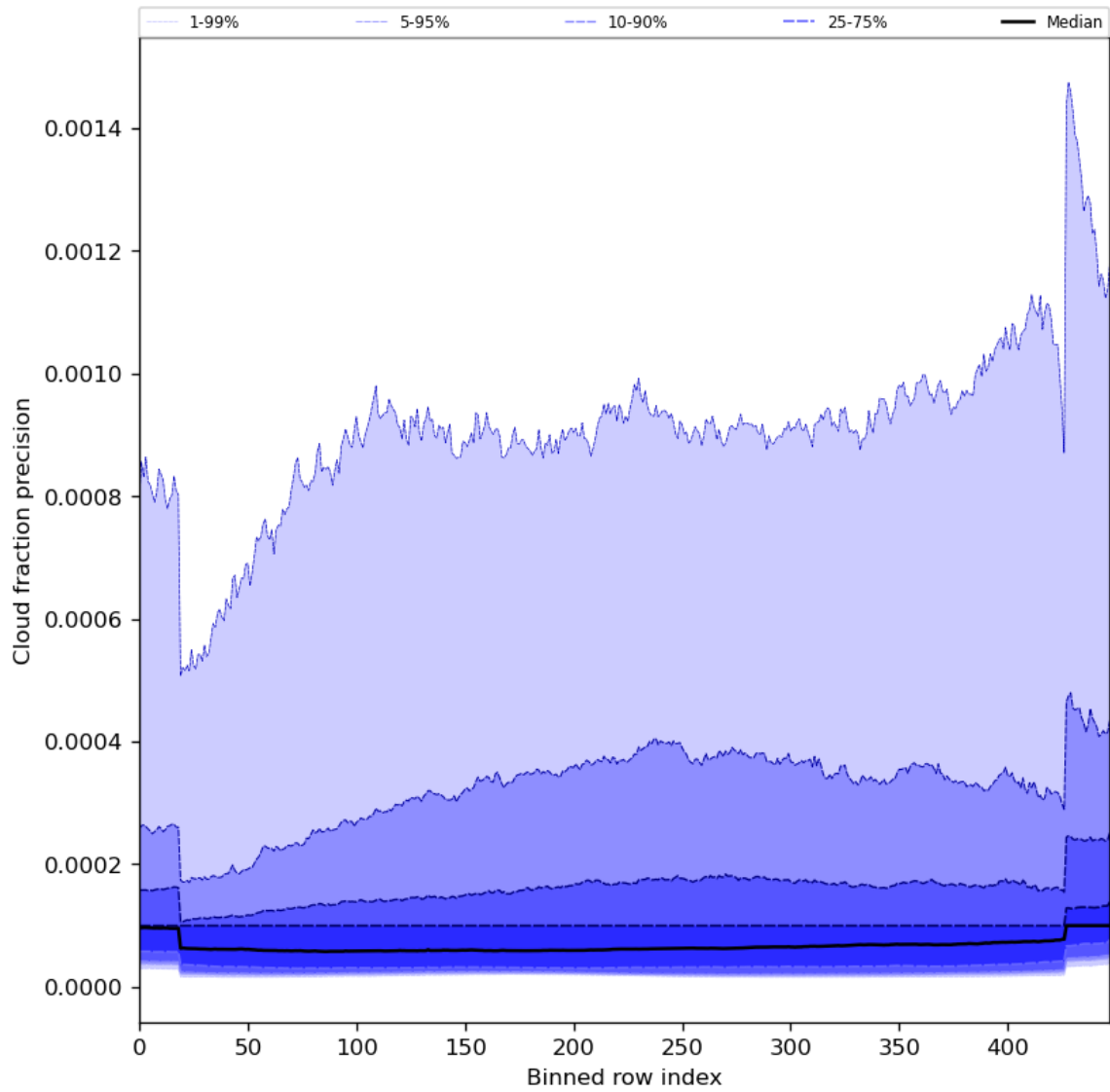
Figure 50: Along track statistics of “Cloud fraction precision” for 2024-04-15 to 2024-04-16
