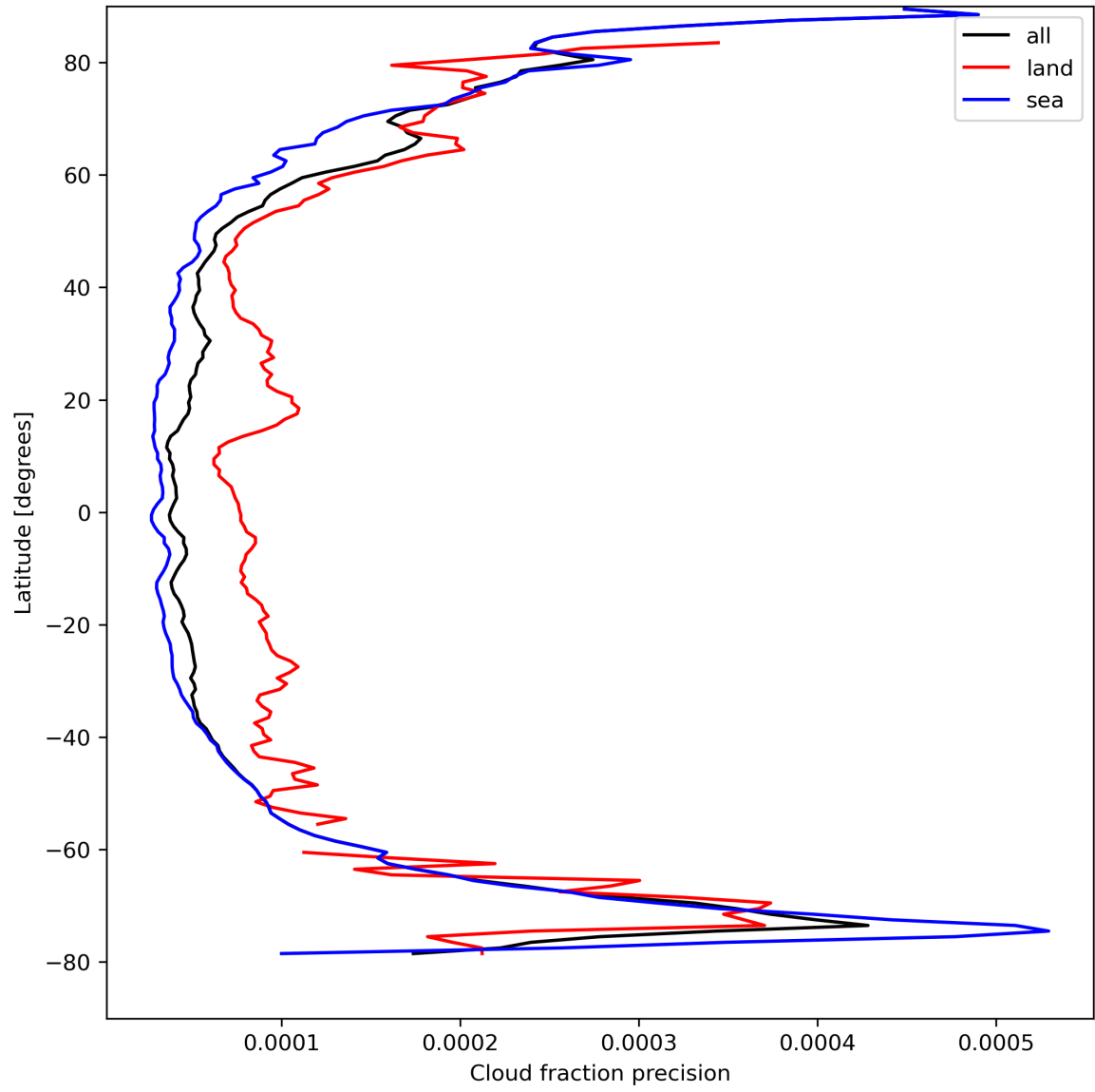
Figure 16: Zonal average of “Cloud fraction precision” for 2024-04-15 to 2024-04-16.
