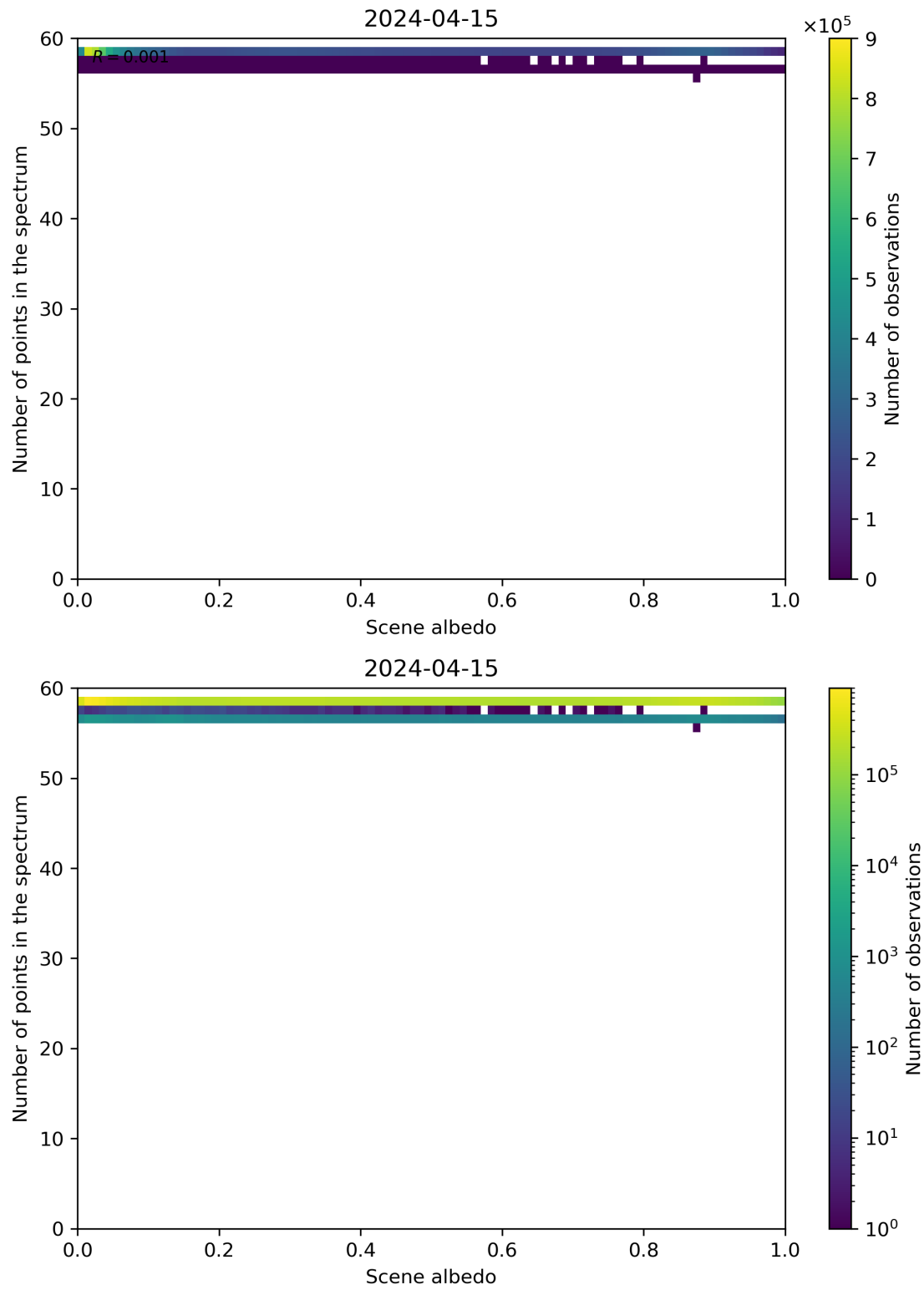
Figure 106: Scatter density plot of “Scene albedo” against “Number of points in the spectrum” for 2024-04-15 to 2024-04-16.
