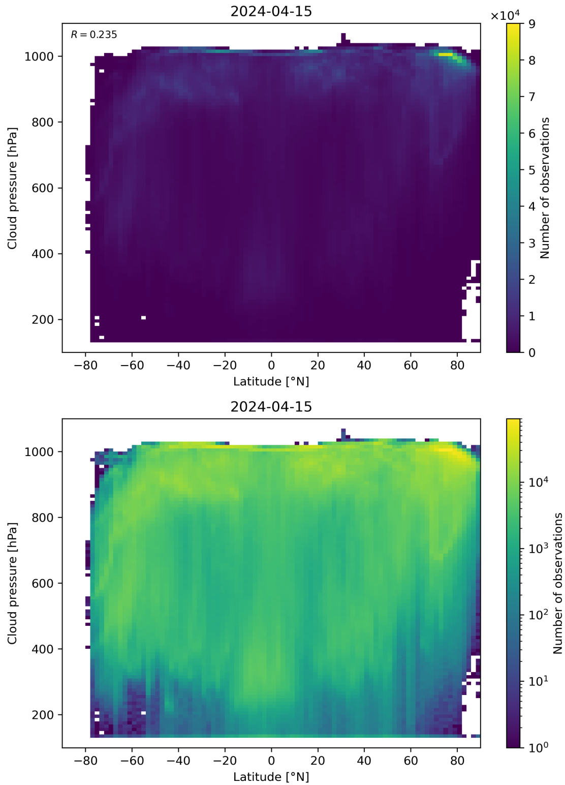
Figure 91: Scatter density plot of “Latitude” against “Cloud pressure” for 2024-04-15 to 2024-04-16.
