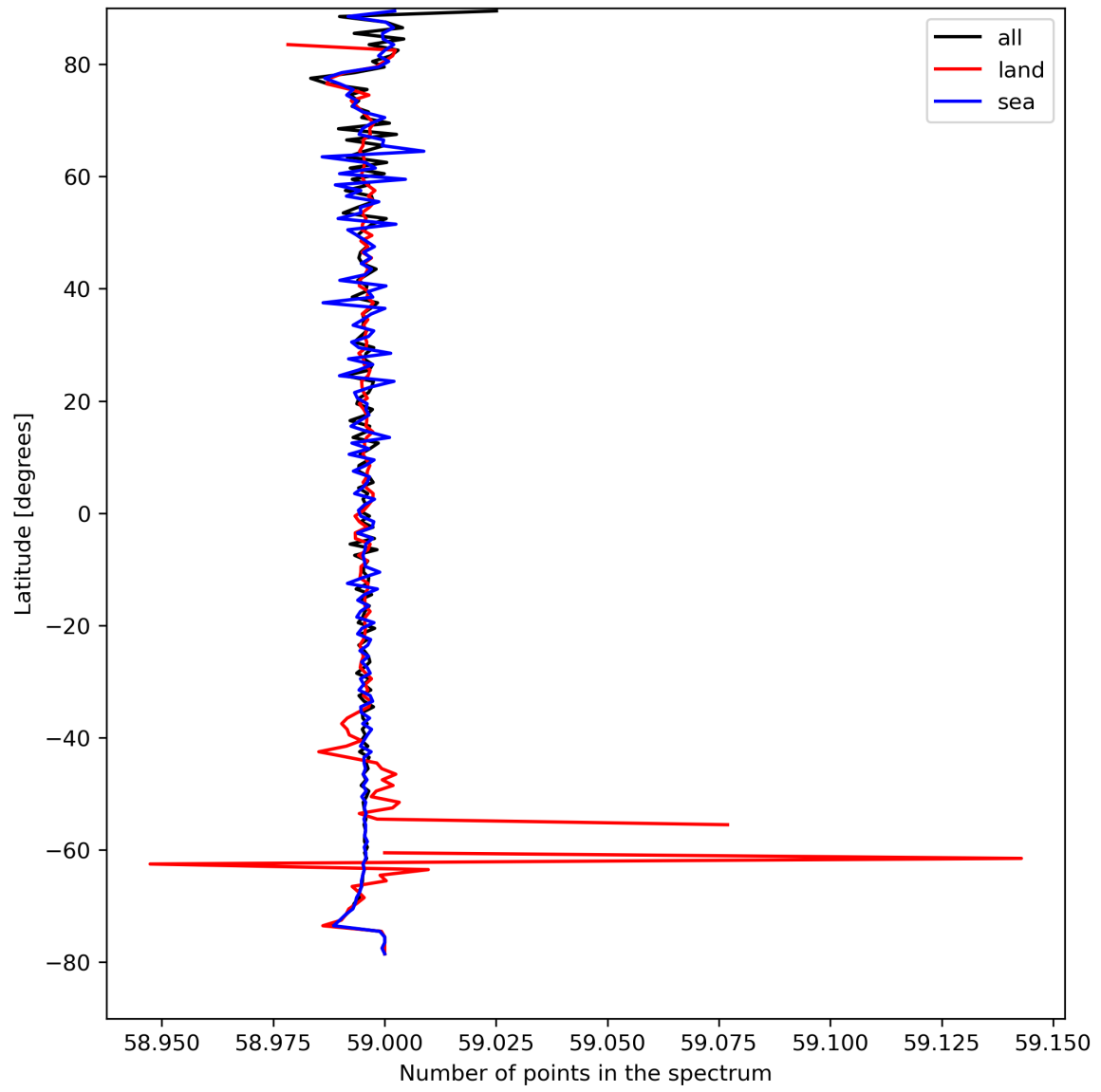
Figure 27: Zonal average of “Number of points in the spectrum” for 2024-04-15 to 2024-04-16.
