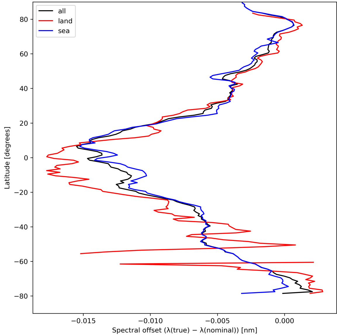
Figure 28: Zonal average of “Spectral offset ( \lambda(\text{true}) - \lambda(\text{nominal}) )” for 2024-04-15 to 2024-04-16.
