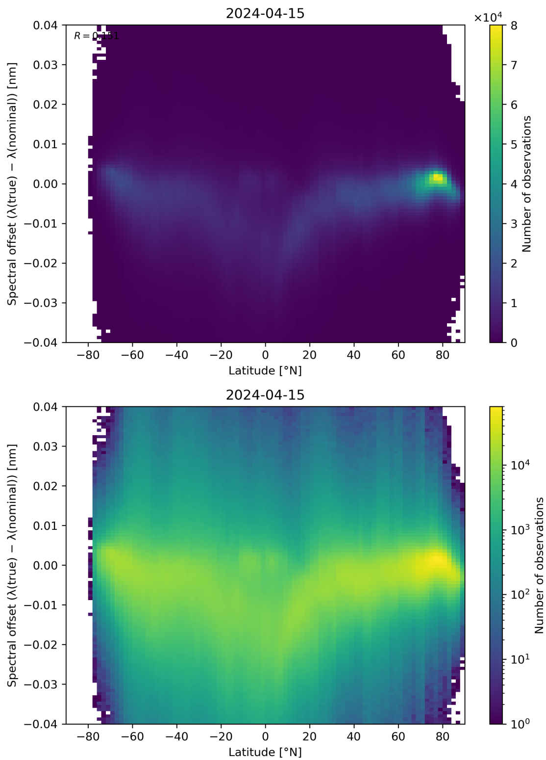
Figure 96: Scatter density plot of “Latitude” against “Spectral offset ( \lambda(\text{true}) - \lambda(\text{nominal}) )” for 2024-04-15 to 2024-04-16.
