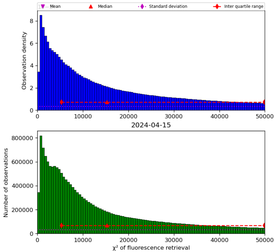
Figure 42: Histogram of “ \chi^2 of fluorescence retrieval” for 2024-04-15 to 2024-04-16
