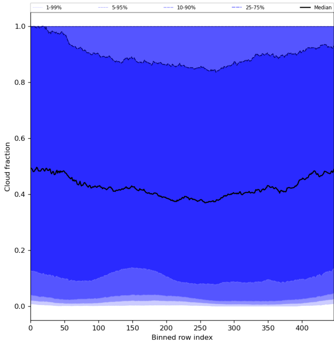
Figure 49: Along track statistics of “Cloud fraction” for 2024-04-15 to 2024-04-16
