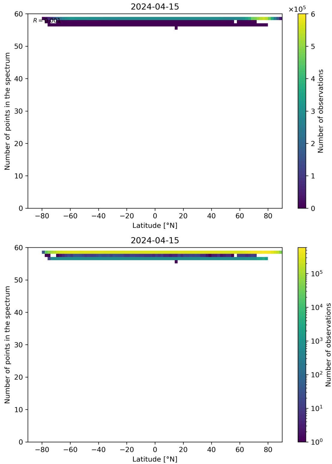
Figure 94: Scatter density plot of “Latitude” against “Number of points in the spectrum” for 2024-04-15 to 2024-04-16.
