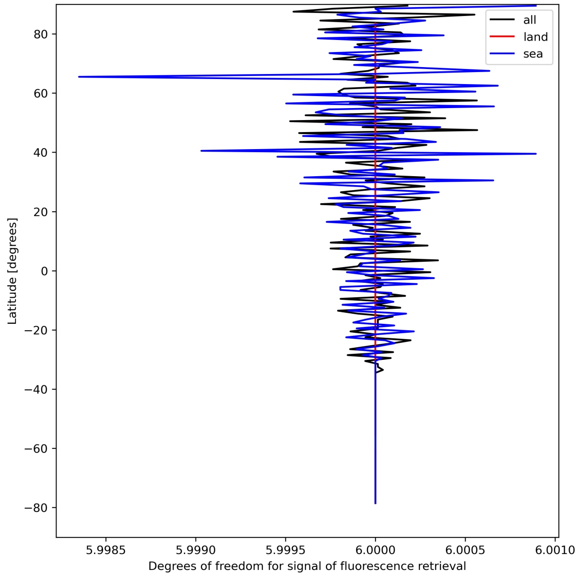
Figure 26: Zonal average of “Degrees of freedom for signal of fluorescence retrieval” for 2024-04-15 to 2024-04-16.
