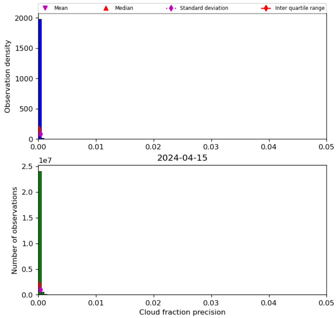
Figure 33: Histogram of “Cloud fraction precision” for 2024-04-15 to 2024-04-16
