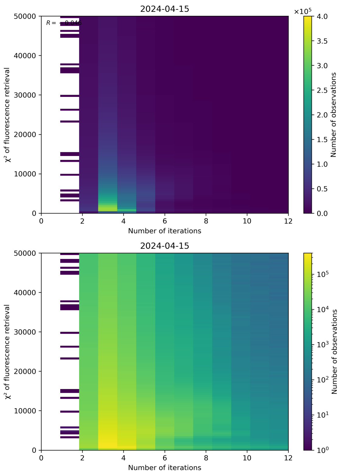
Figure 97: Scatter density plot of “Number of iterations” against “ \chi^2 of fluorescence retrieval” for 2024-04-15 to 2024-04-16.
