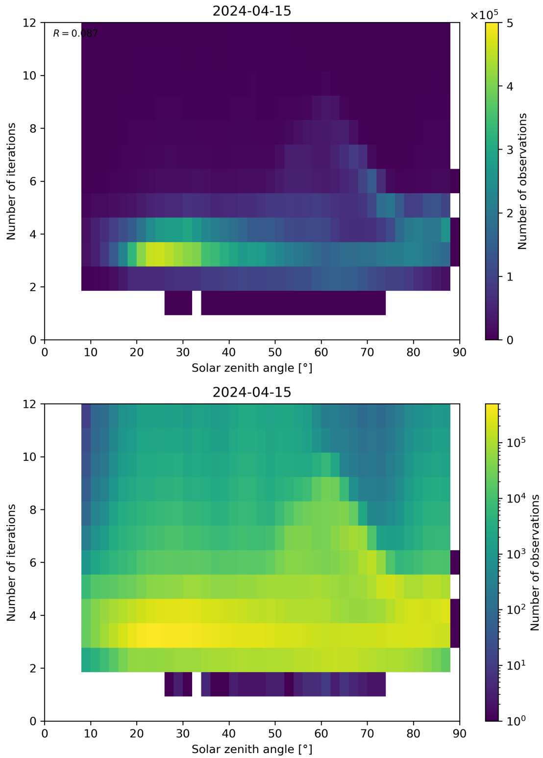
Figure 114: Scatter density plot of “Solar zenith angle” against “Number of iterations” for 2024-04-15 to 2024-04-16.
