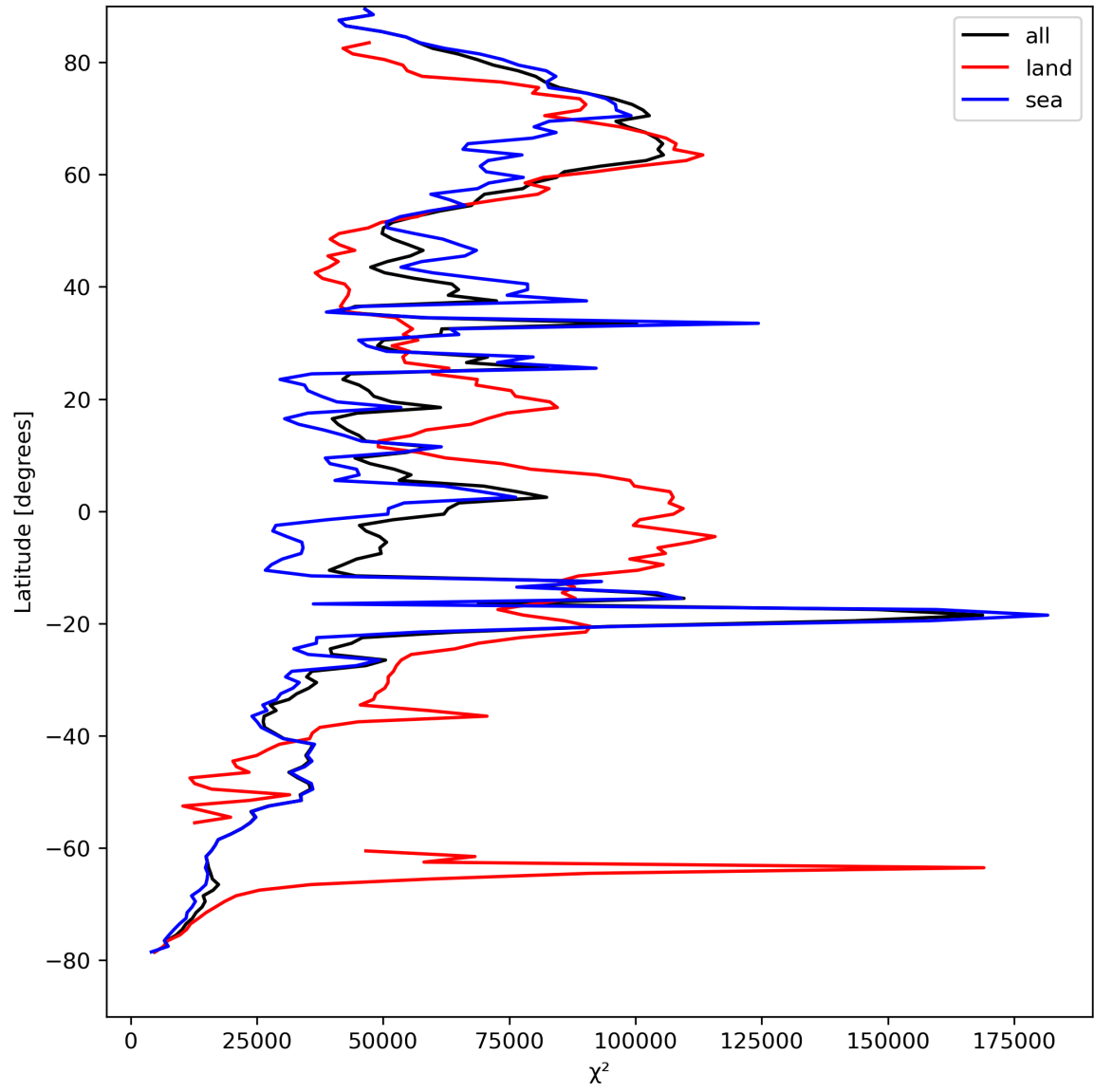
Figure 21: Zonal average of “ \chi^2 ” for 2024-04-15 to 2024-04-16.
