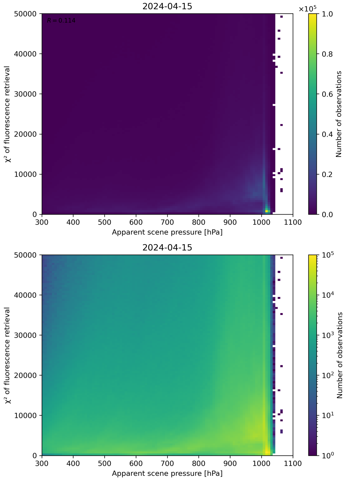
Figure 63: Scatter density plot of “Apparent scene pressure” against “ \chi^2 of fluorescence retrieval” for 2024-04-15 to 2024-04-16.
