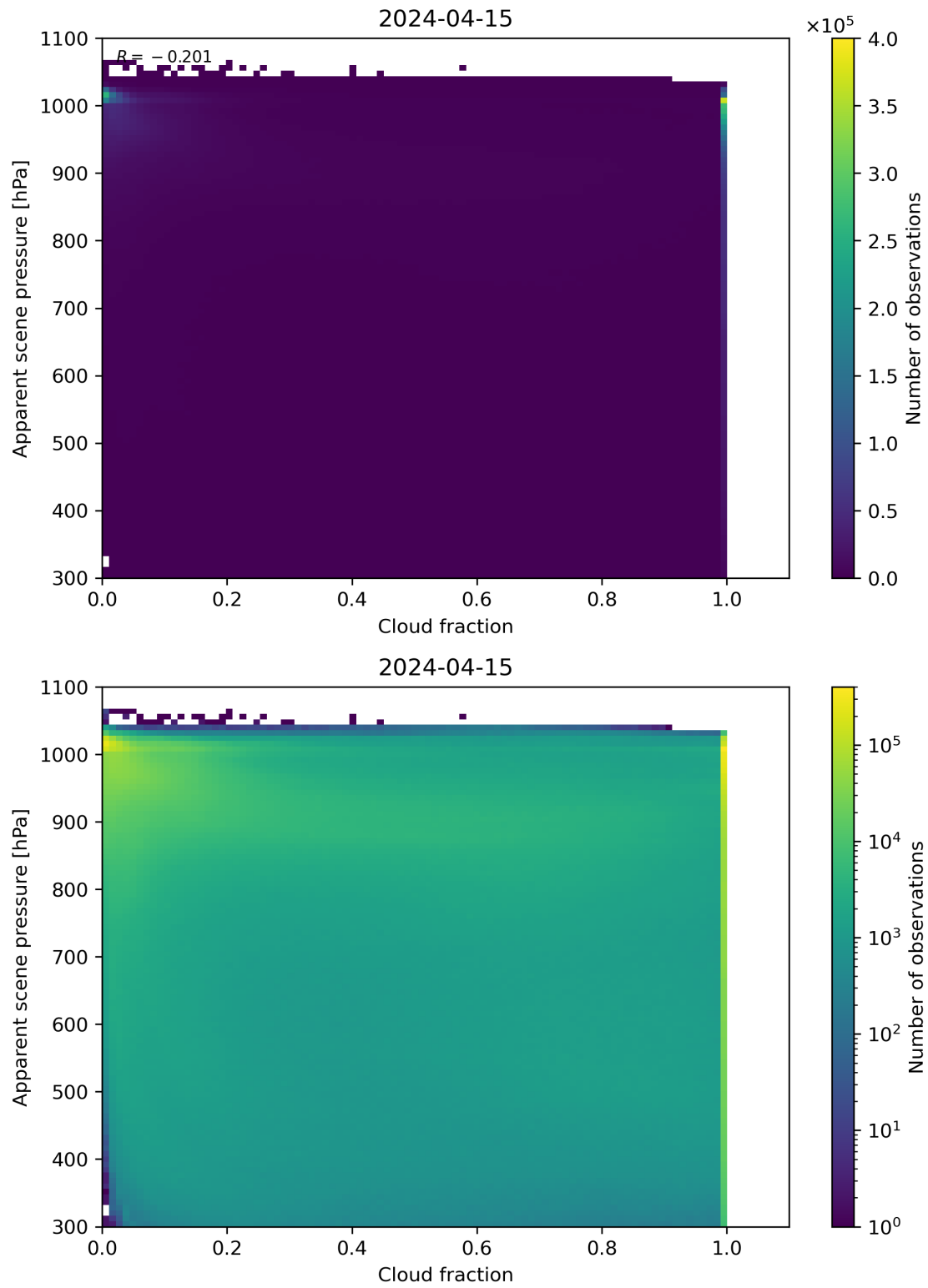
Figure 70: Scatter density plot of “Cloud fraction” against “Apparent scene pressure” for 2024-04-15 to 2024-04-16.
