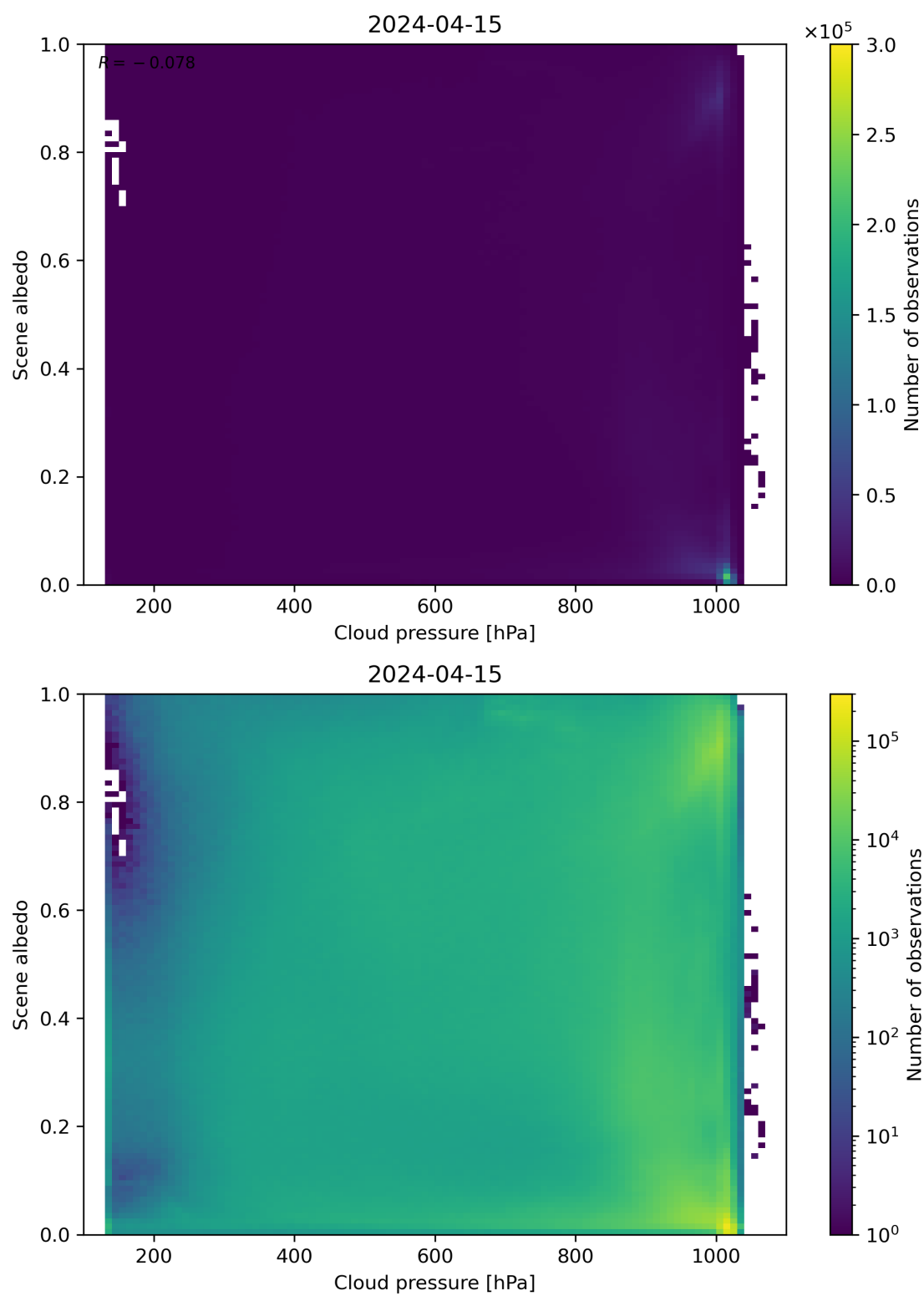
Figure 83: Scatter density plot of “Cloud pressure” against “Scene albedo” for 2024-04-15 to 2024-04-16.
