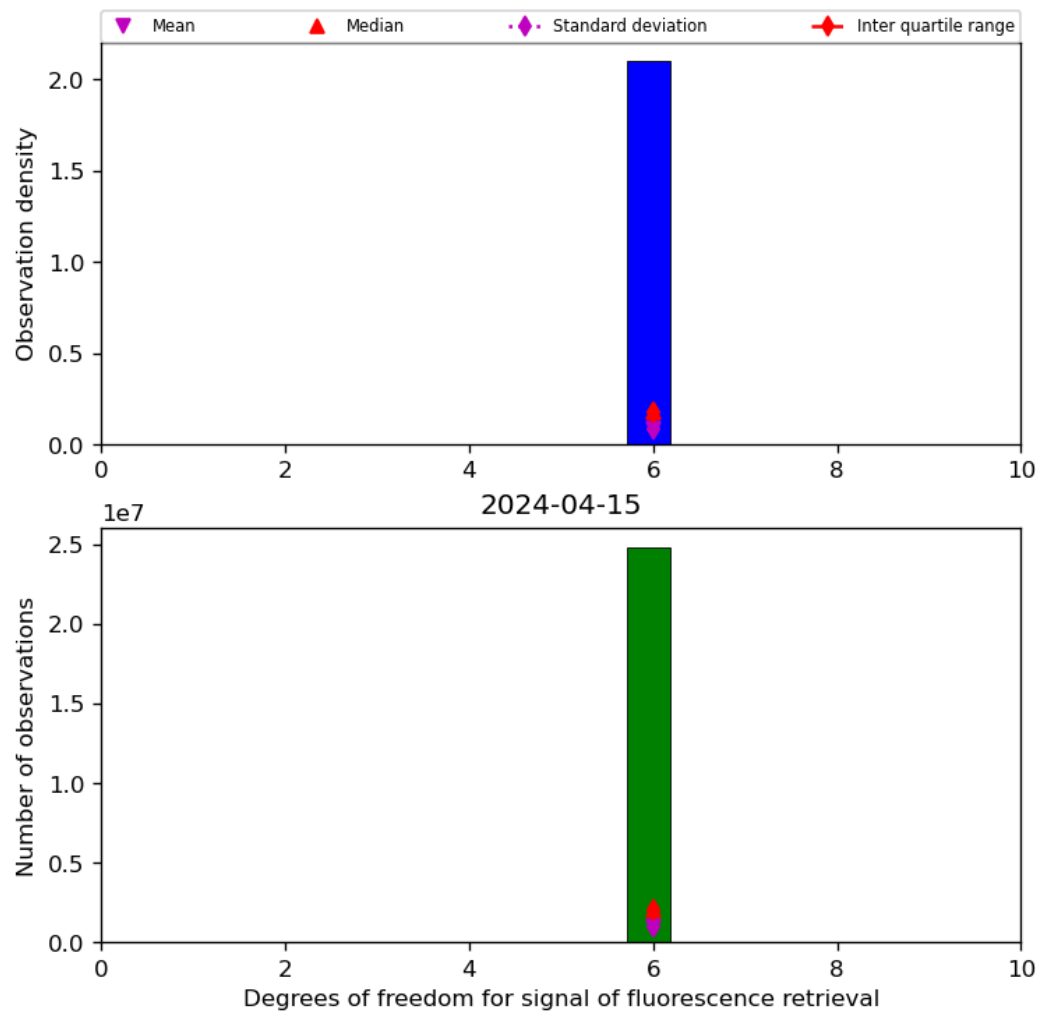
Figure 43: Histogram of “Degrees of freedom for signal of fluorescence retrieval” for 2024-04-15 to 2024-04-16
