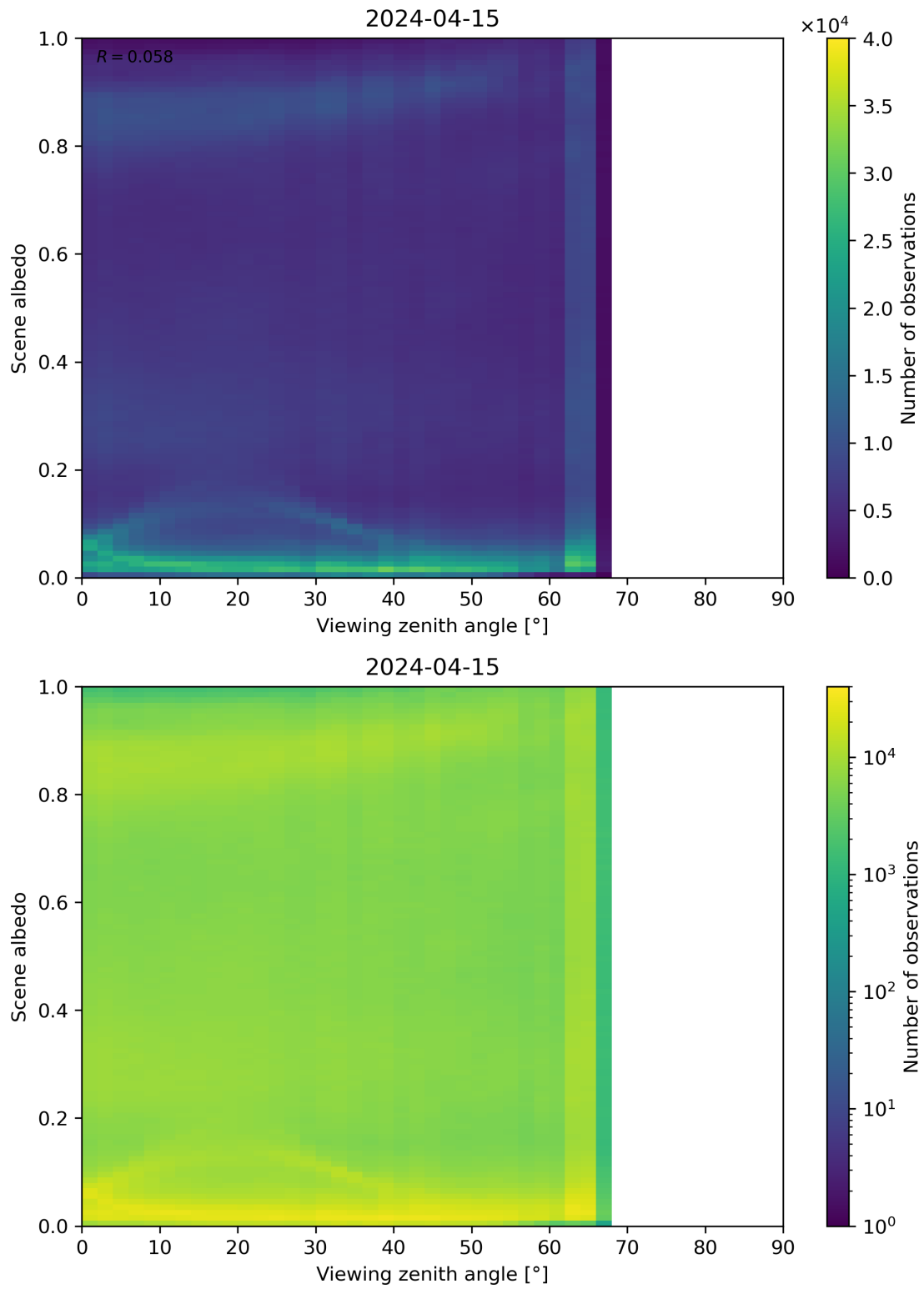
Figure 126: Scatter density plot of “Viewing zenith angle” against “Scene albedo” for 2024-04-15 to 2024-04-16.
