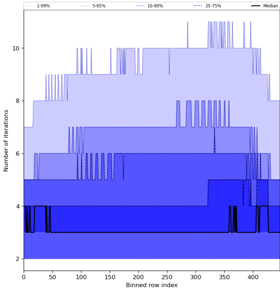
Figure 56: Along track statistics of “Number of iterations” for 2024-04-15 to 2024-04-16
