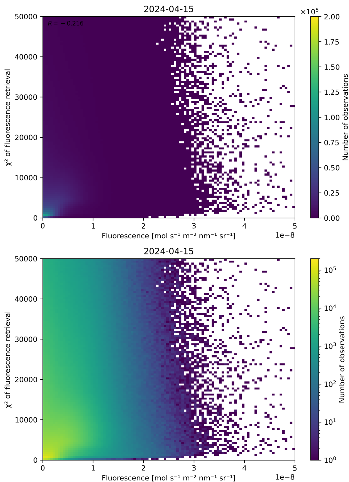
Figure 85: Scatter density plot of “Fluorescence” against “ \chi^2 of fluorescence retrieval” for 2024-04-15 to 2024-04-16.
