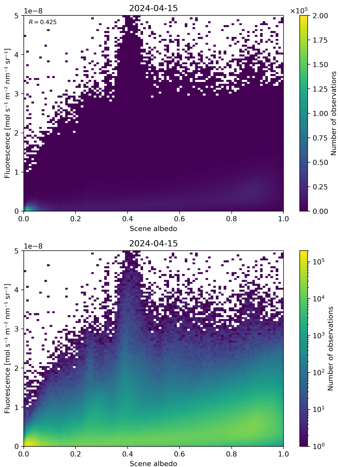
Figure 104: Scatter density plot of “Scene albedo” against “Fluorescence” for 2024-04-15 to 2024-04-16.
