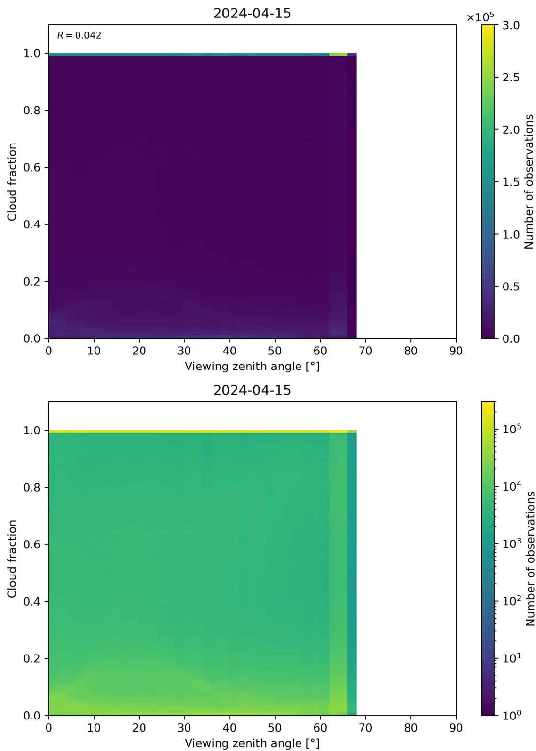
Figure 120: Scatter density plot of “Viewing zenith angle” against “Cloud fraction” for 2024-04-15 to 2024-04-16.
