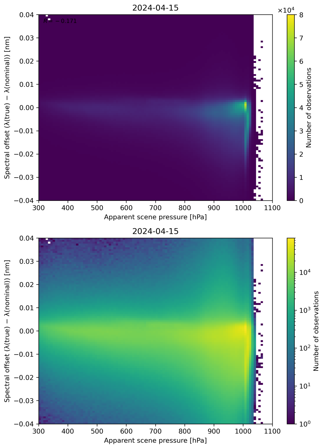
Figure 67: Scatter density plot of “Apparent scene pressure” against “Spectral offset ( \lambda(\text{true}) - \lambda(\text{nominal}) )” for 2024-04-15 to 2024-04-16.
