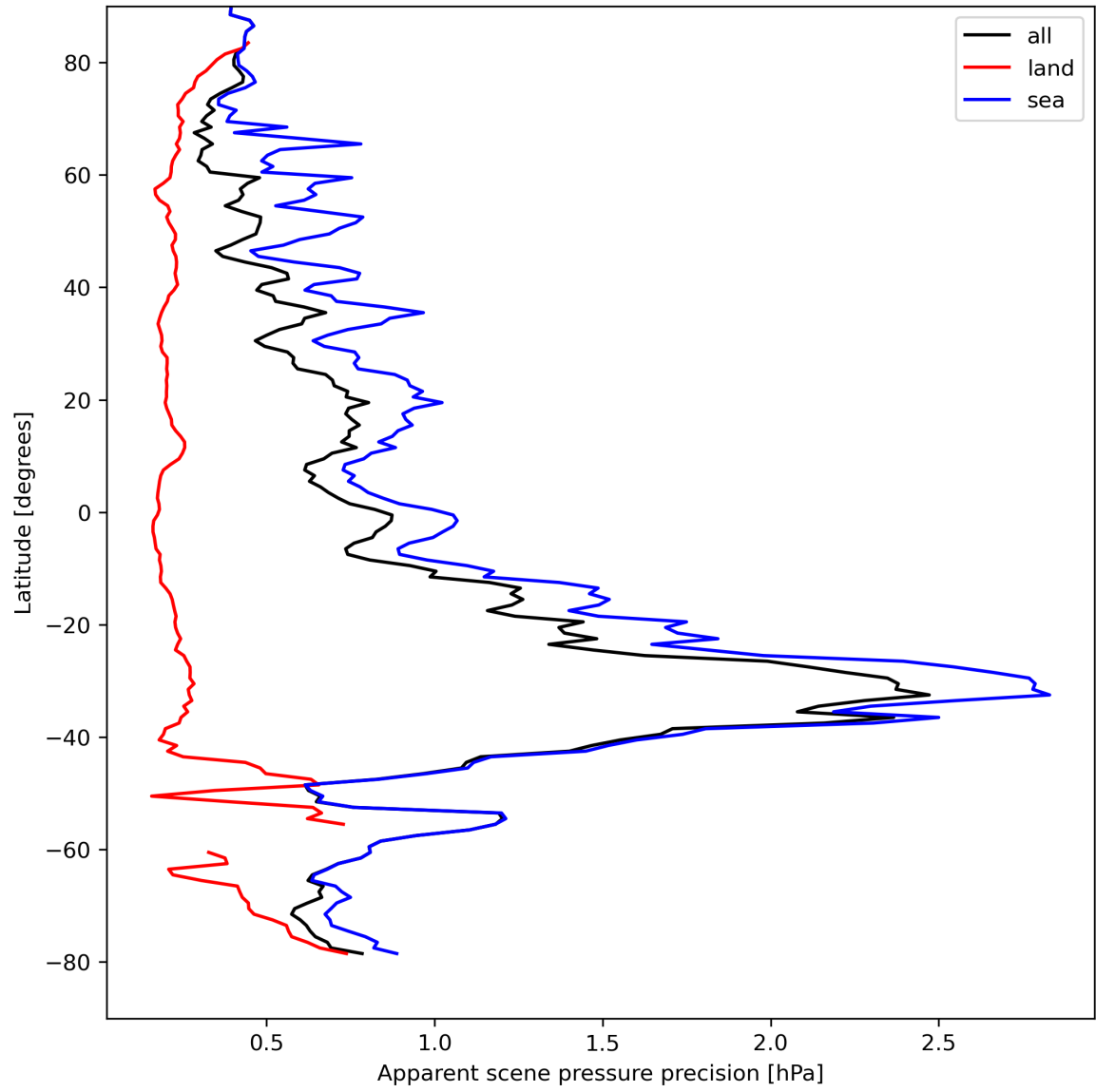
Figure 20: Zonal average of “Apparent scene pressure precision” for 2024-04-15 to 2024-04-16.
