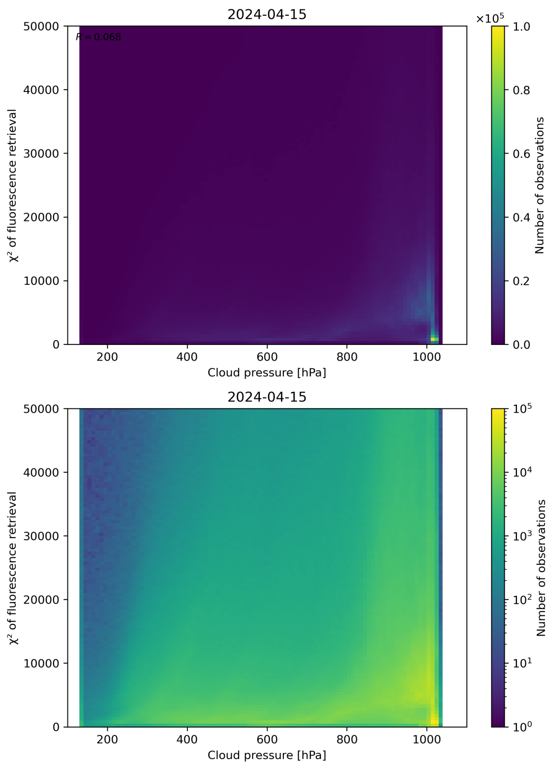
Figure 78: Scatter density plot of “Cloud pressure” against “ \chi^2 of fluorescence retrieval” for 2024-04-15 to 2024-04-16.
