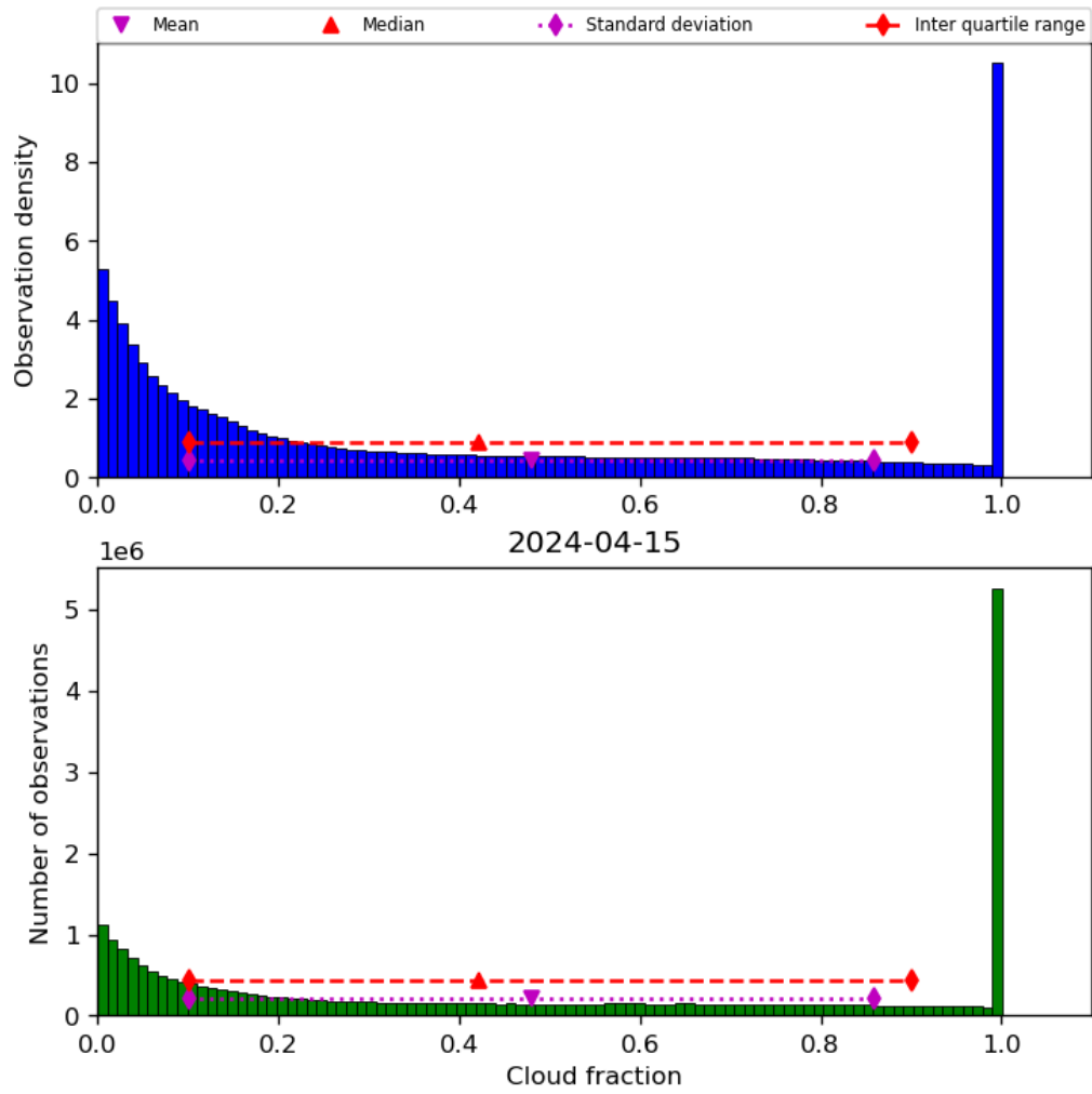
Figure 32: Histogram of “Cloud fraction” for 2024-04-15 to 2024-04-16
