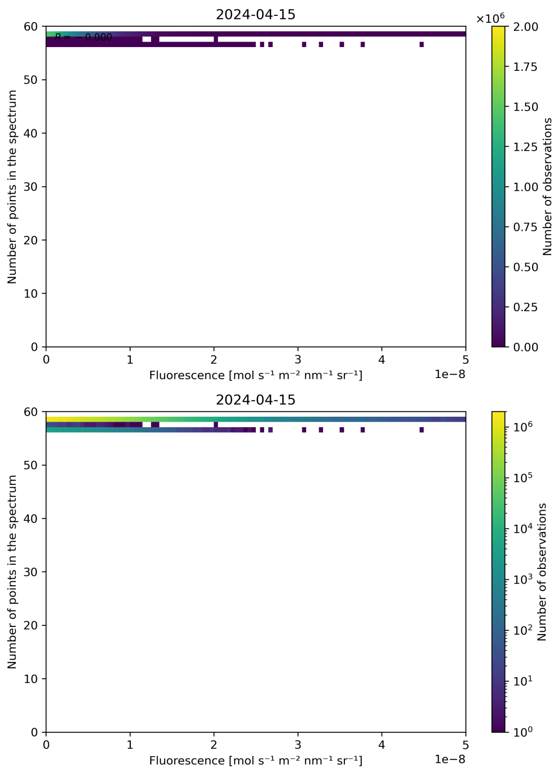
Figure 86: Scatter density plot of “Fluorescence” against “Number of points in the spectrum” for 2024-04-15 to 2024-04-16.
