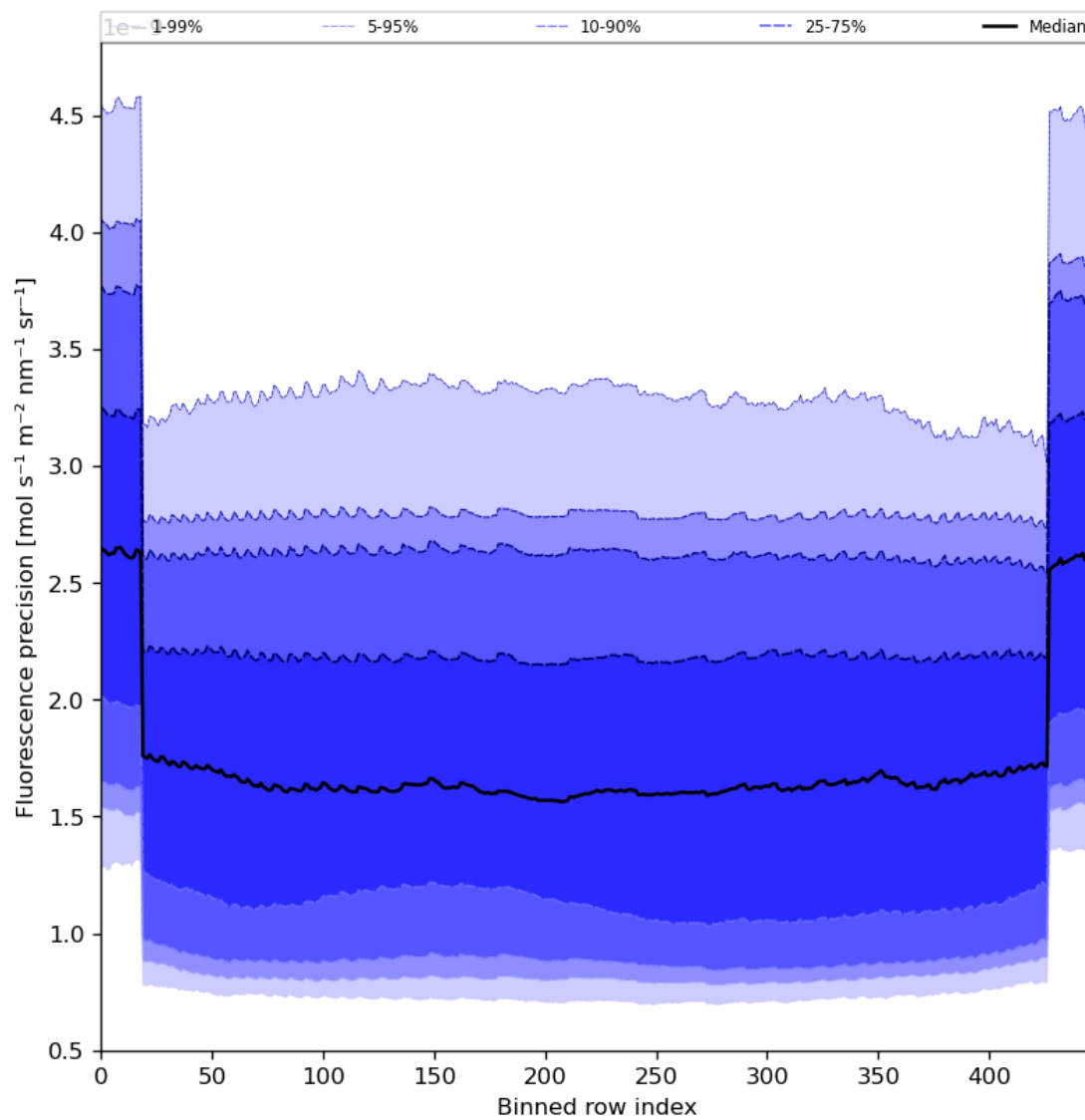
Figure 58: Along track statistics of “Fluorescence precision” for 2024-04-15 to 2024-04-16
