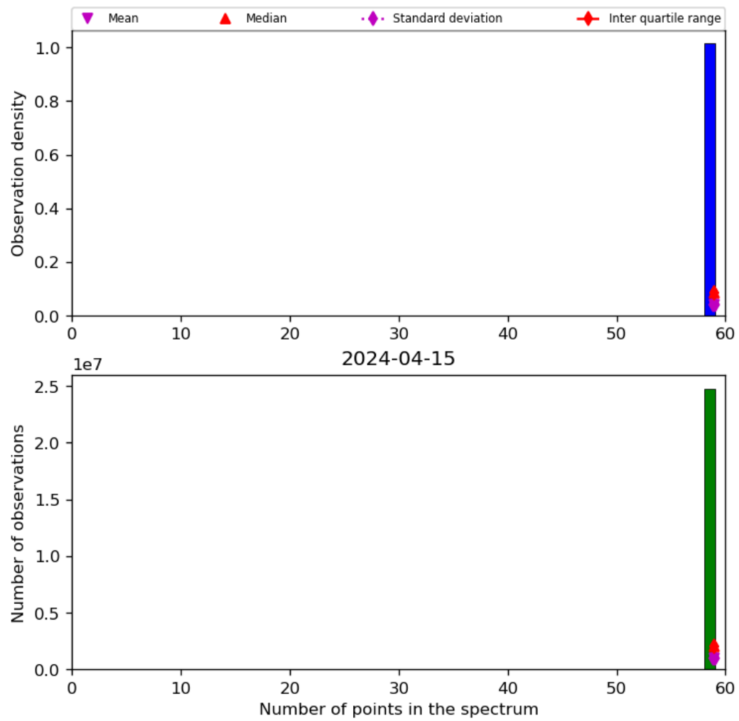
Figure 44: Histogram of “Number of points in the spectrum” for 2024-04-15 to 2024-04-16
