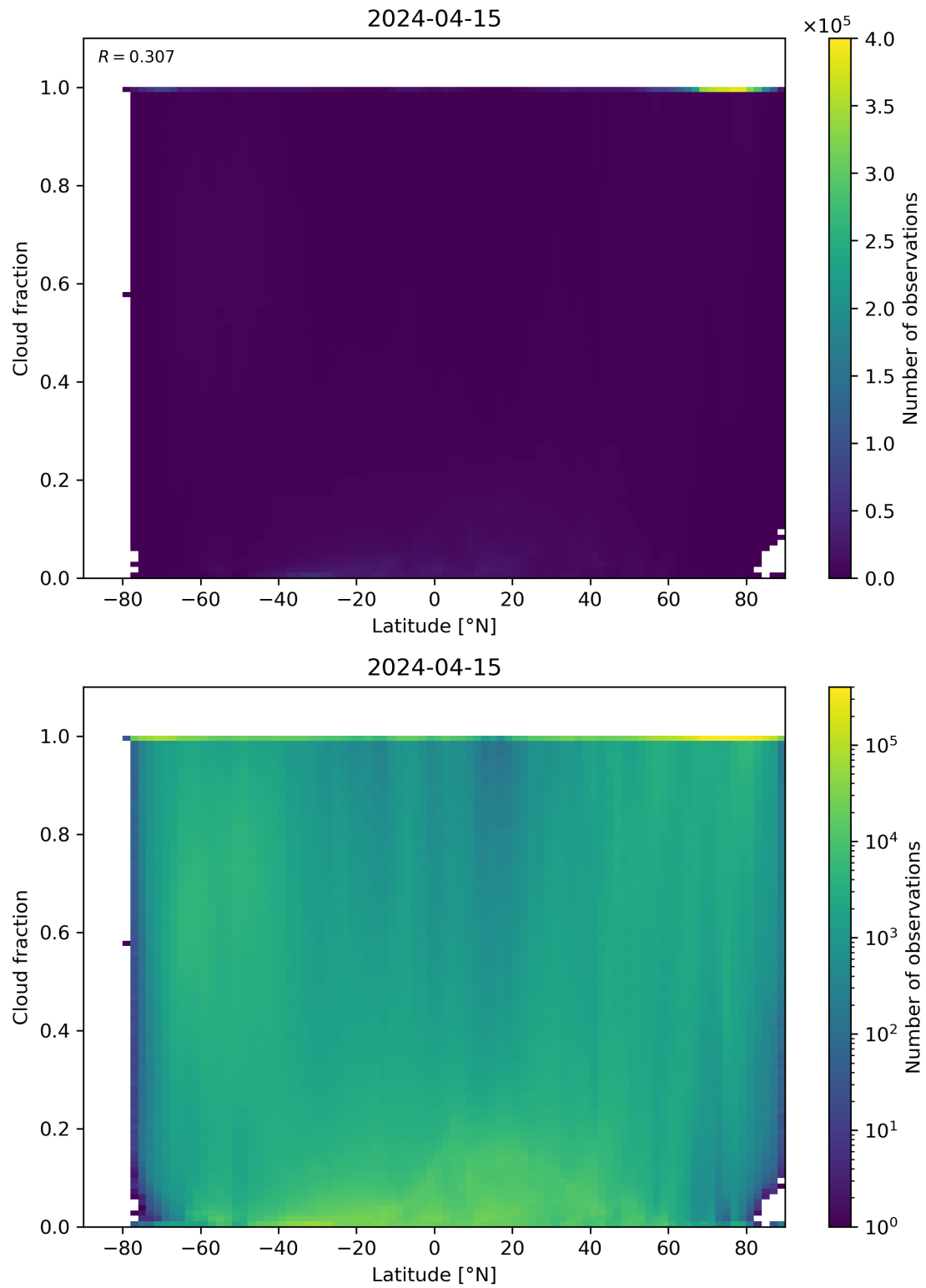
Figure 90: Scatter density plot of “Latitude” against “Cloud fraction” for 2024-04-15 to 2024-04-16.
