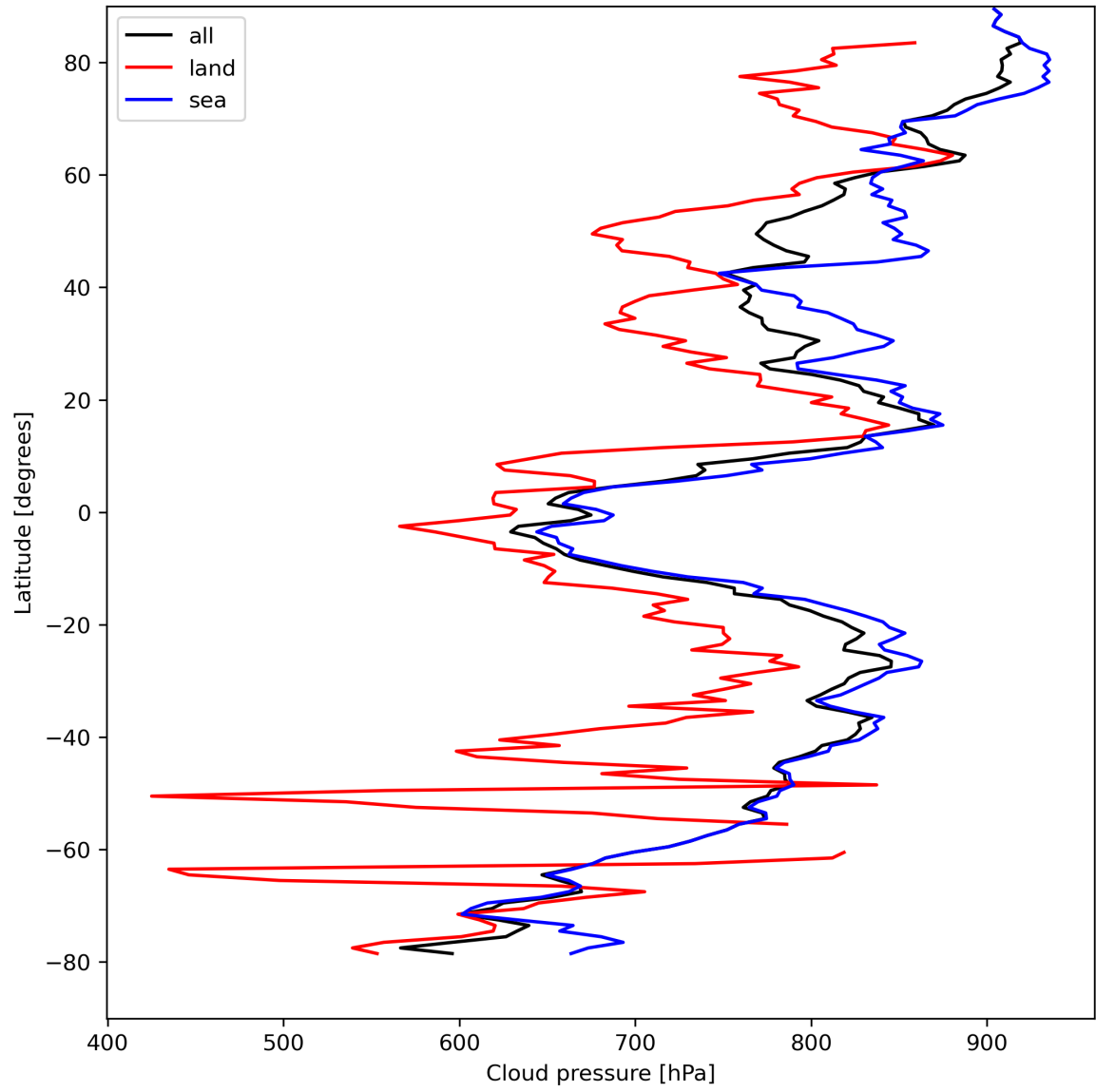
Figure 13: Zonal average of “Cloud pressure” for 2024-04-15 to 2024-04-16.
