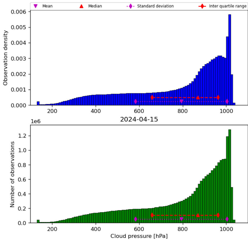
Figure 30: Histogram of “Cloud pressure” for 2024-04-15 to 2024-04-16
