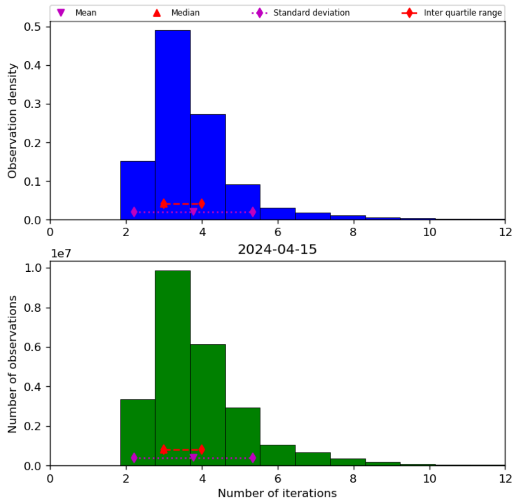
Figure 39: Histogram of “Number of iterations” for 2024-04-15 to 2024-04-16
