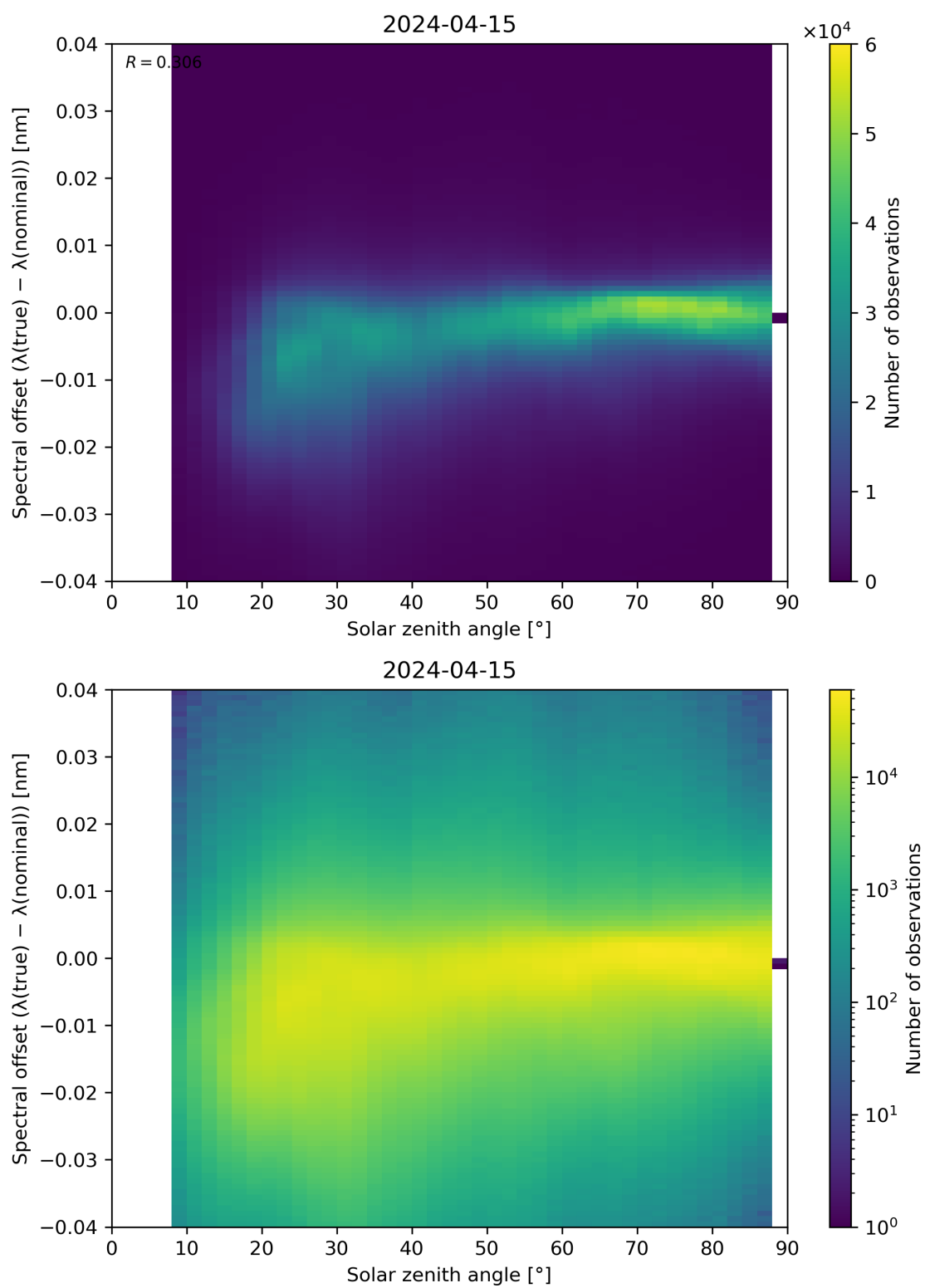
Figure 117: Scatter density plot of “Solar zenith angle” against “Spectral offset ( \lambda(\text{true}) - \lambda(\text{nominal}) )” for 2024-04-15 to 2024-04-16.
