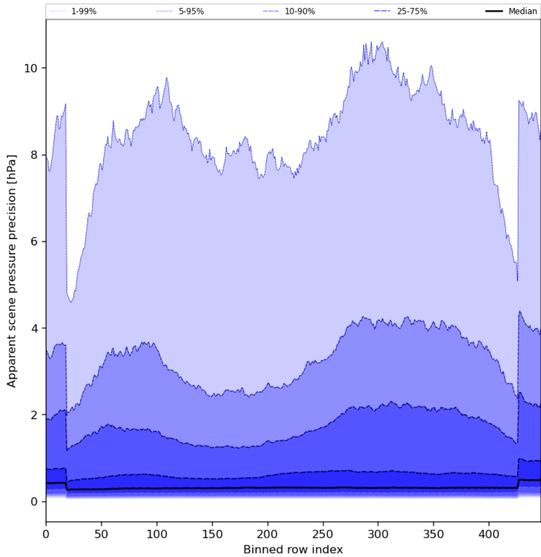
Figure 54: Along track statistics of “Apparent scene pressure precision” for 2024-04-15 to 2024-04-16
