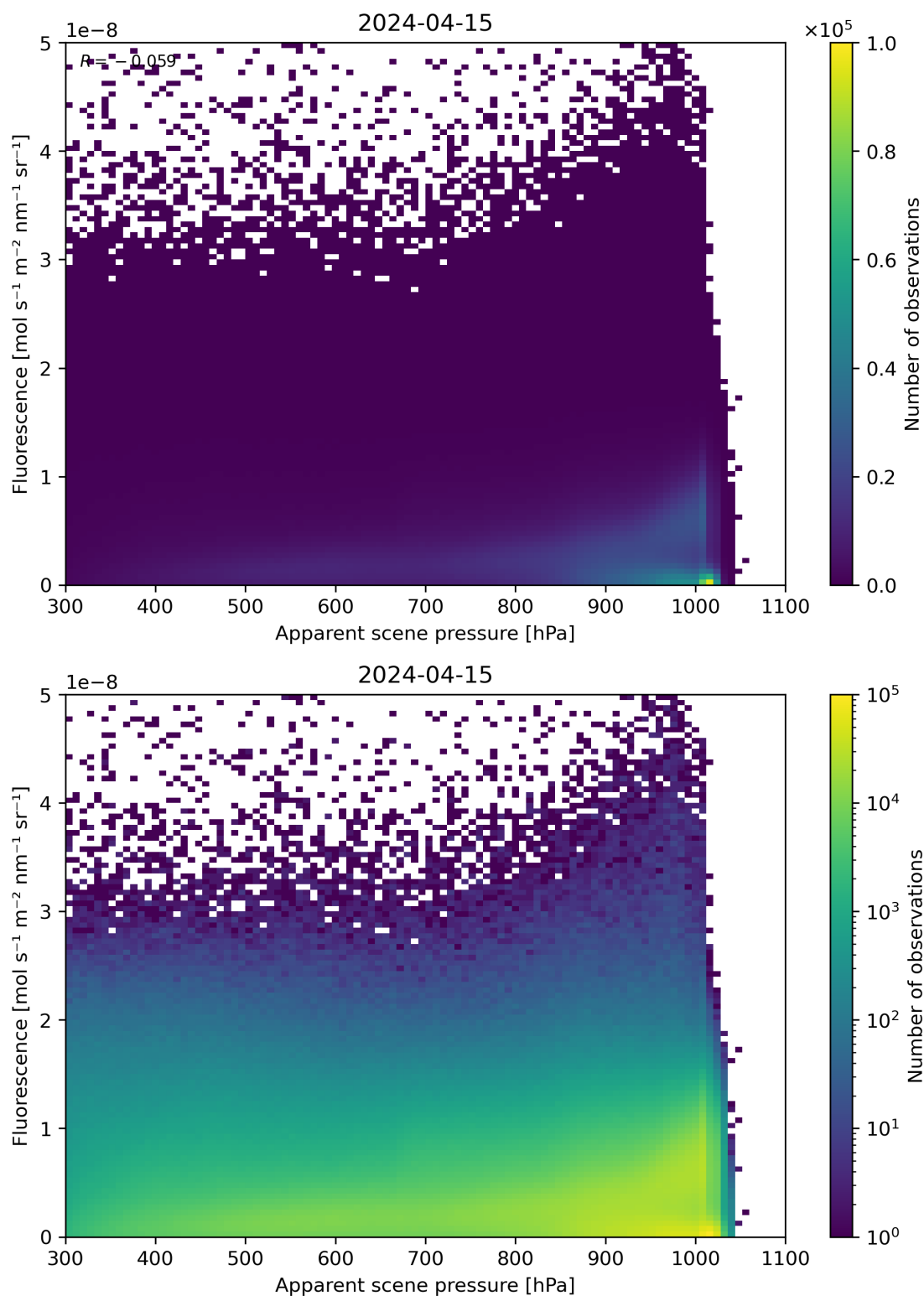
Figure 64: Scatter density plot of “Apparent scene pressure” against “Fluorescence” for 2024-04-15 to 2024-04-16.
