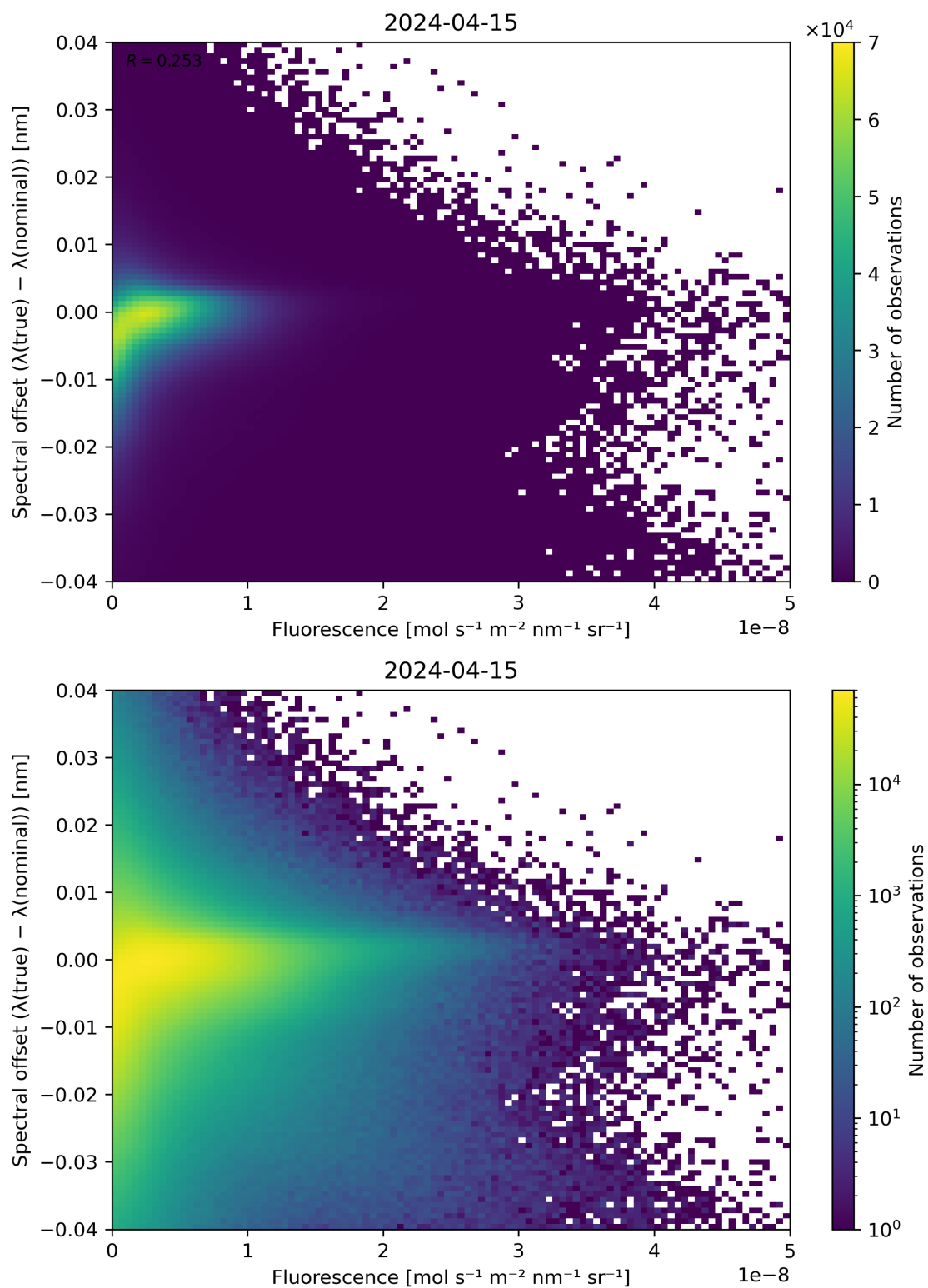
Figure 87: Scatter density plot of “Fluorescence” against “Spectral offset ( \lambda(\text{true}) - \lambda(\text{nominal}) )” for 2024-04-15 to 2024-04-16.
