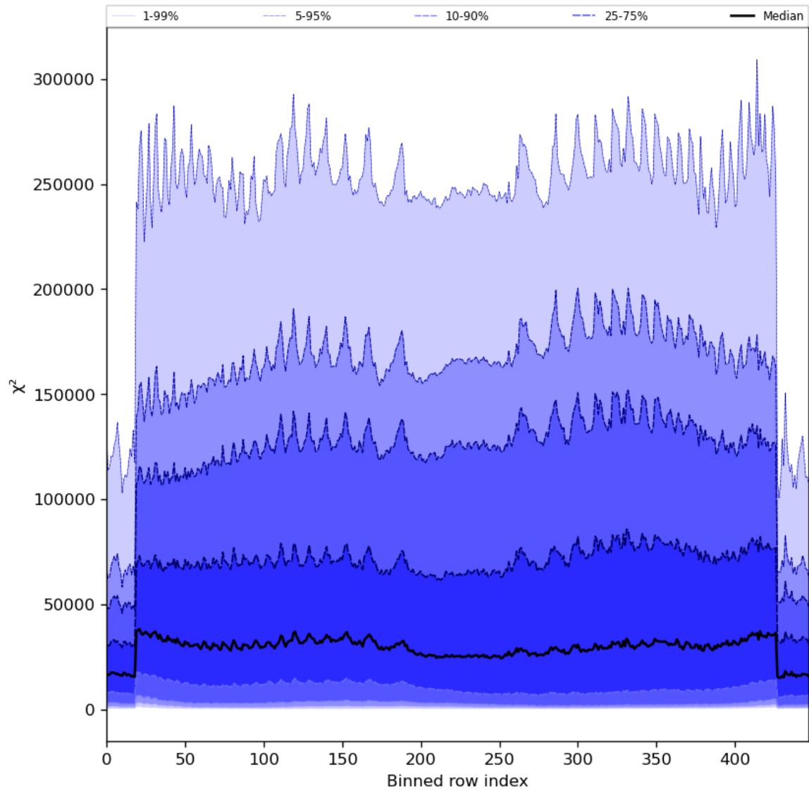
Figure 55: Along track statistics of “ \chi^2 ” for 2024-04-15 to 2024-04-16
