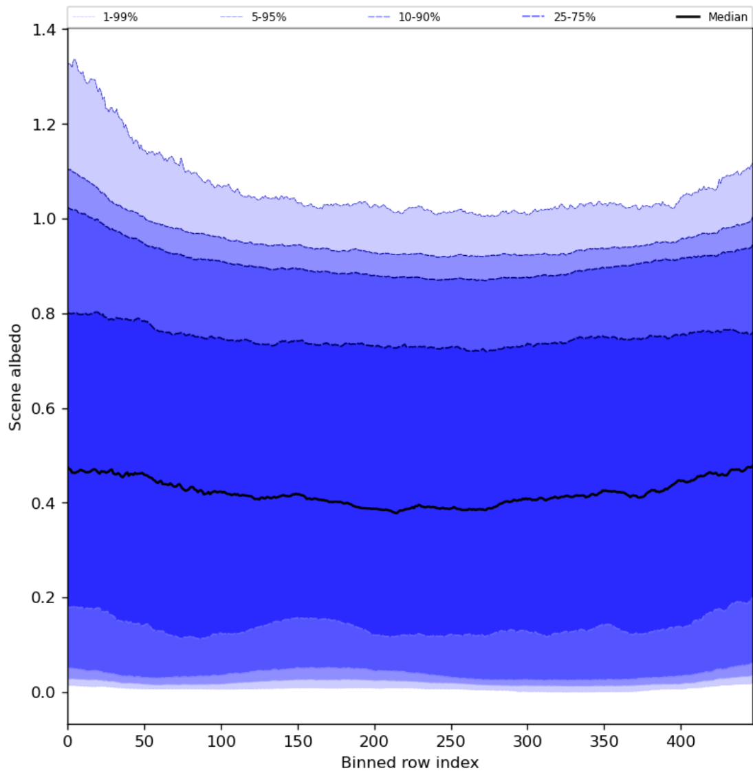
Figure 51: Along track statistics of “Scene albedo” for 2024-04-15 to 2024-04-16
