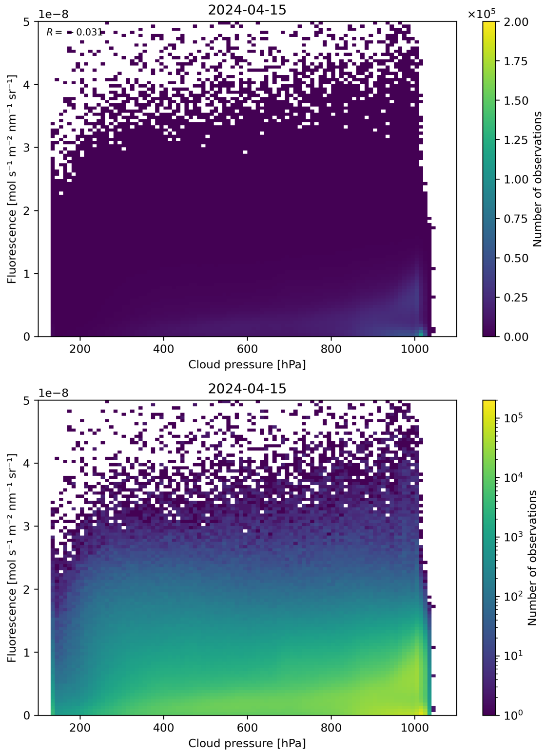
Figure 80: Scatter density plot of “Cloud pressure” against “Fluorescence” for 2024-04-15 to 2024-04-16.
