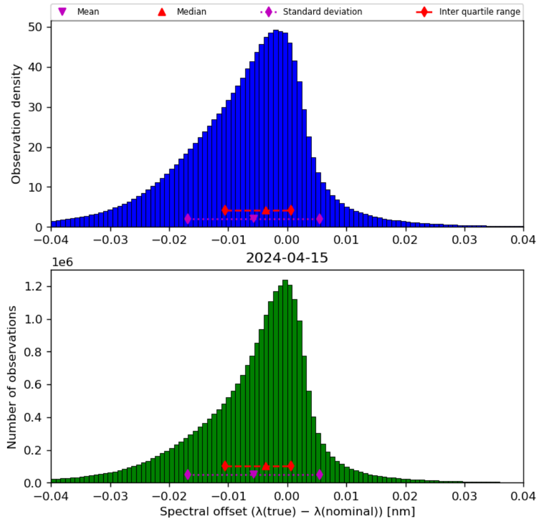
Figure 45: Histogram of “Spectral offset ( \lambda(\text{true}) - \lambda(\text{nominal}) )” for 2024-04-15 to 2024-04-16
