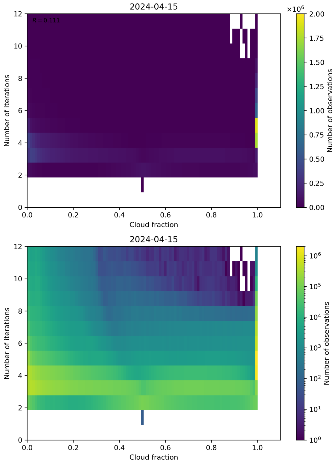
Figure 73: Scatter density plot of “Cloud fraction” against “Number of iterations” for 2024-04-15 to 2024-04-16.
