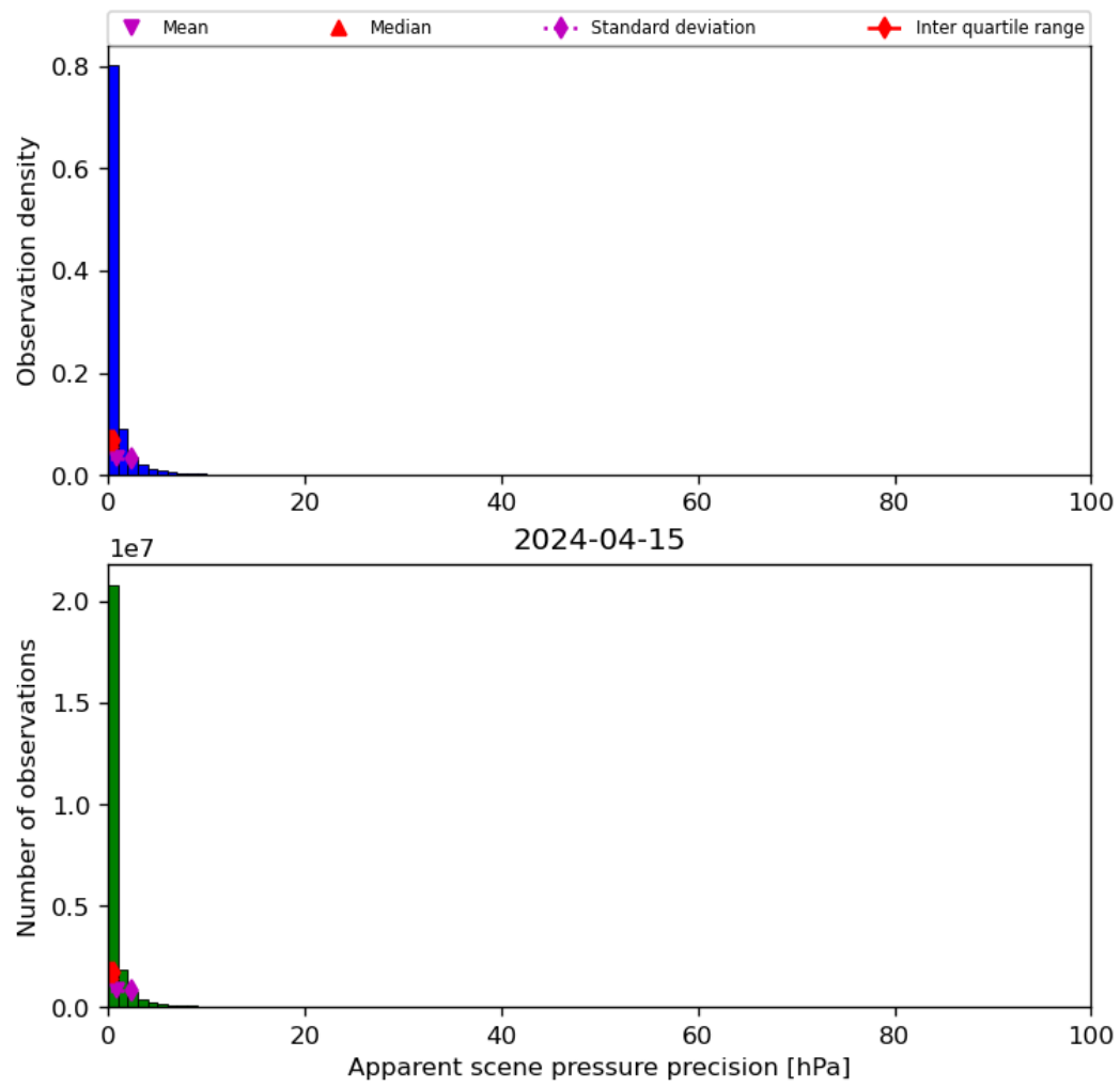
Figure 37: Histogram of “Apparent scene pressure precision” for 2024-04-15 to 2024-04-16
