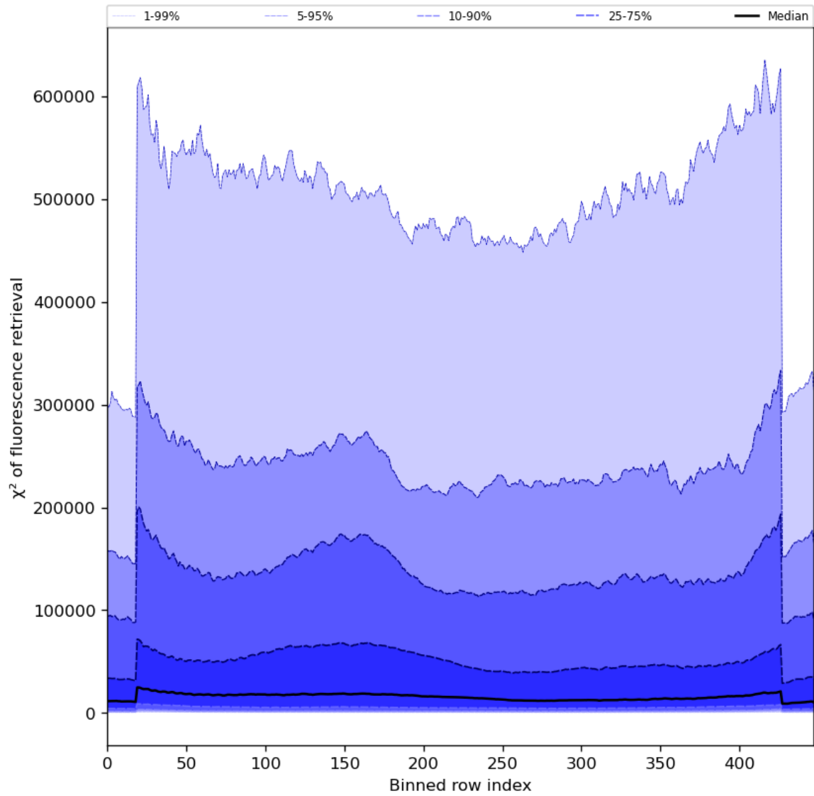
Figure 59: Along track statistics of “ \chi^2 of fluorescence retrieval” for 2024-04-15 to 2024-04-16
