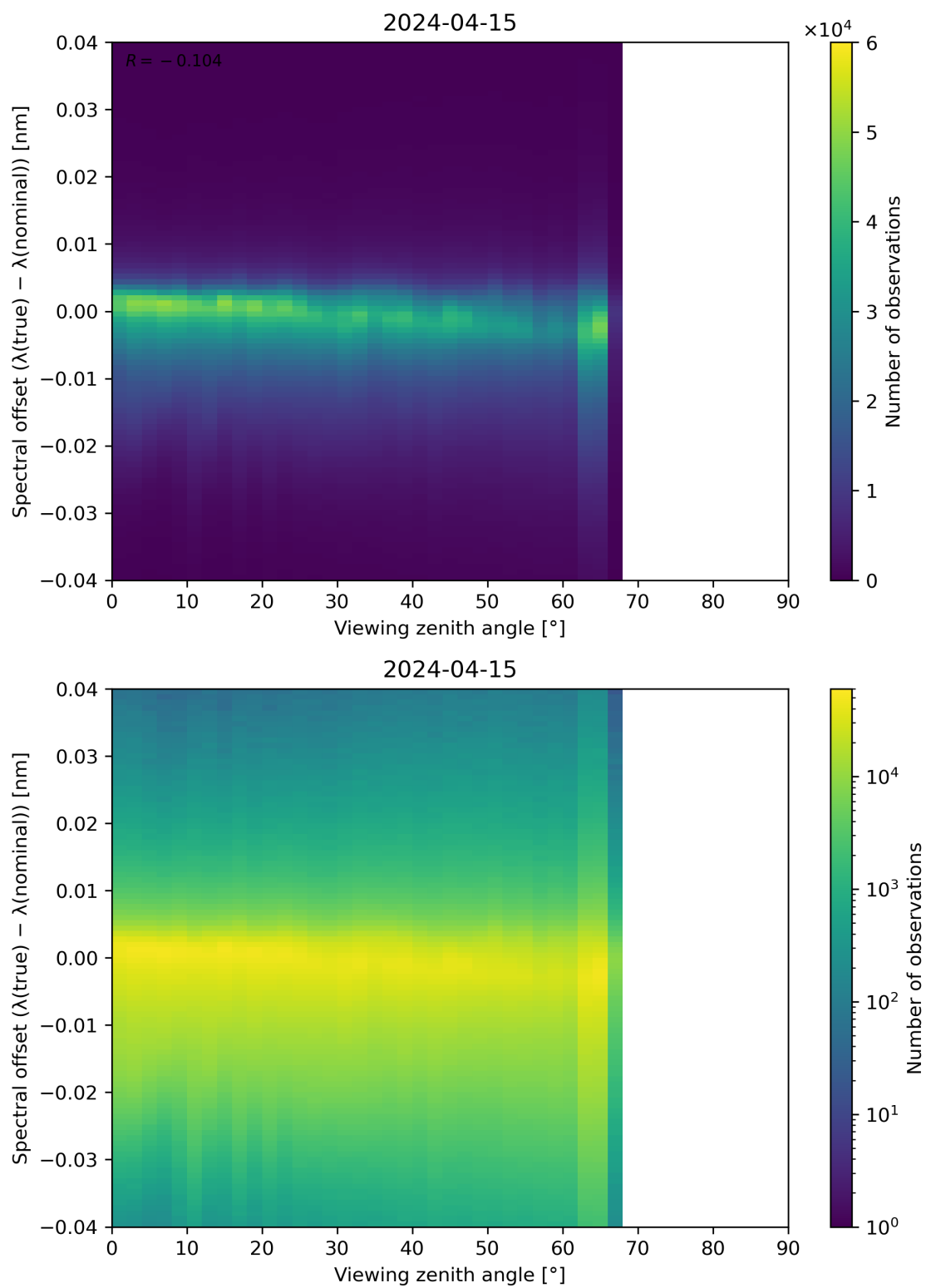
Figure 128: Scatter density plot of “Viewing zenith angle” against “Spectral offset ( \lambda(\text{true}) - \lambda(\text{nominal}) )” for 2024-04-15 to 2024-04-16.
