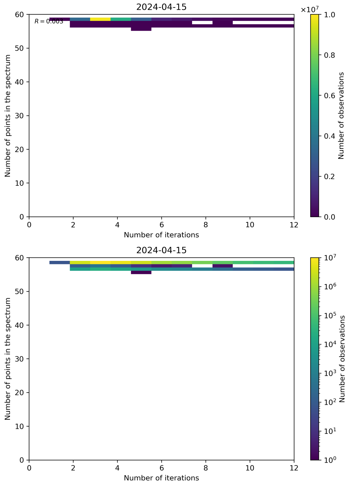
Figure 99: Scatter density plot of “Number of iterations” against “Number of points in the spectrum” for 2024-04-15 to 2024-04-16.
