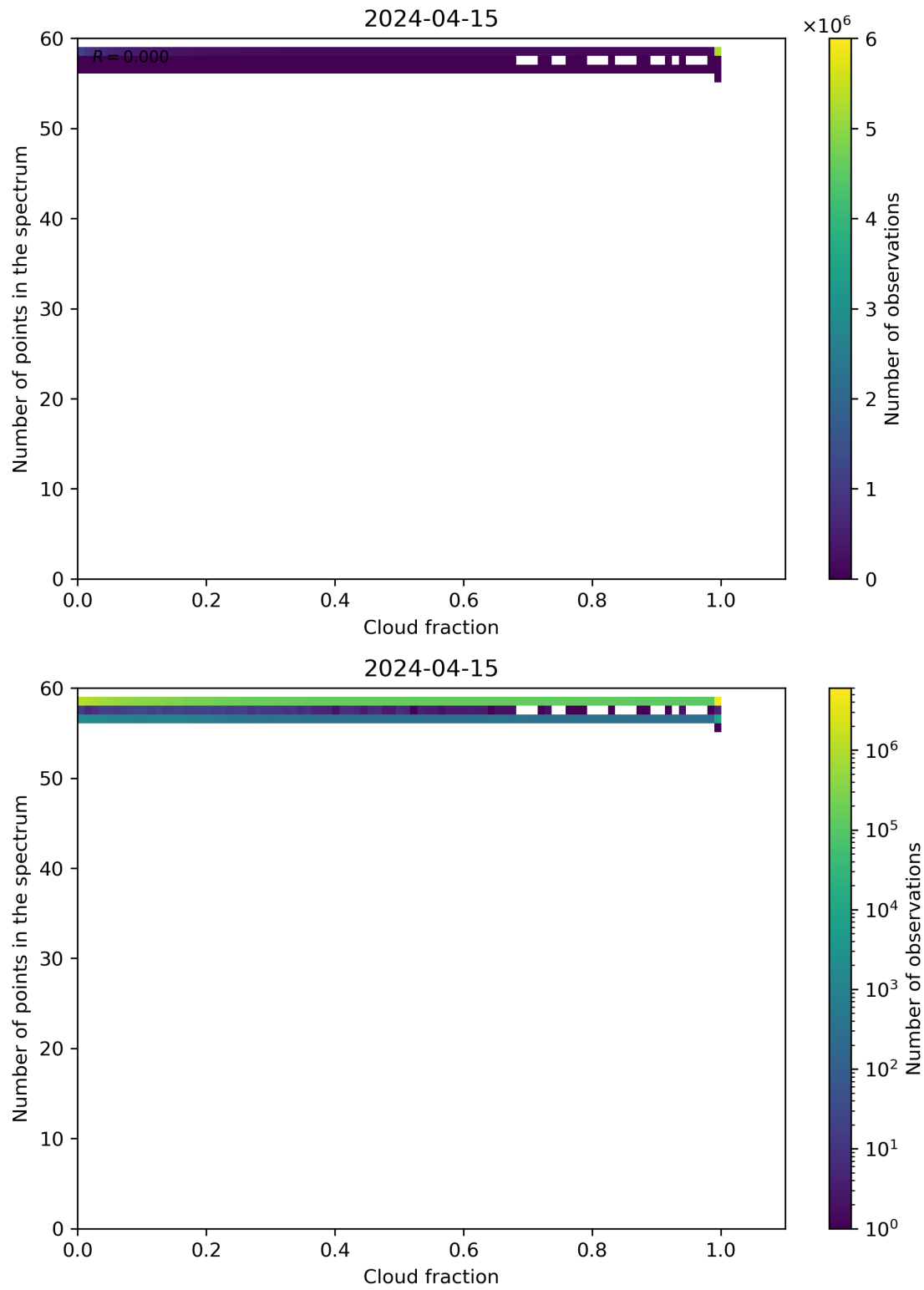
Figure 74: Scatter density plot of “Cloud fraction” against “Number of points in the spectrum” for 2024-04-15 to 2024-04-16.
