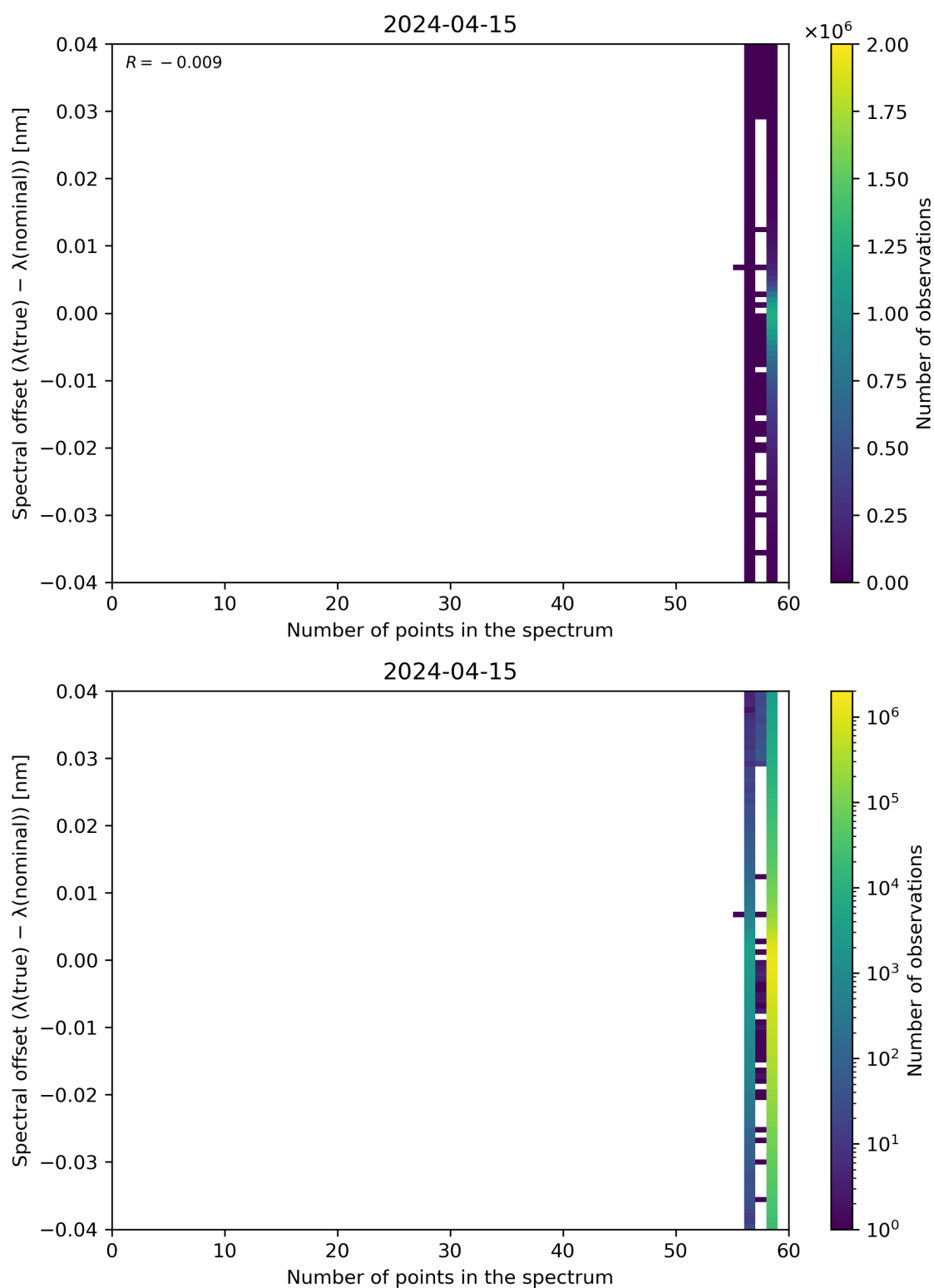
Figure 101: Scatter density plot of “Number of points in the spectrum” against “Spectral offset ( \lambda(\text{true}) - \lambda(\text{nominal}) )” for 2024-04-15 to 2024-04-16.
