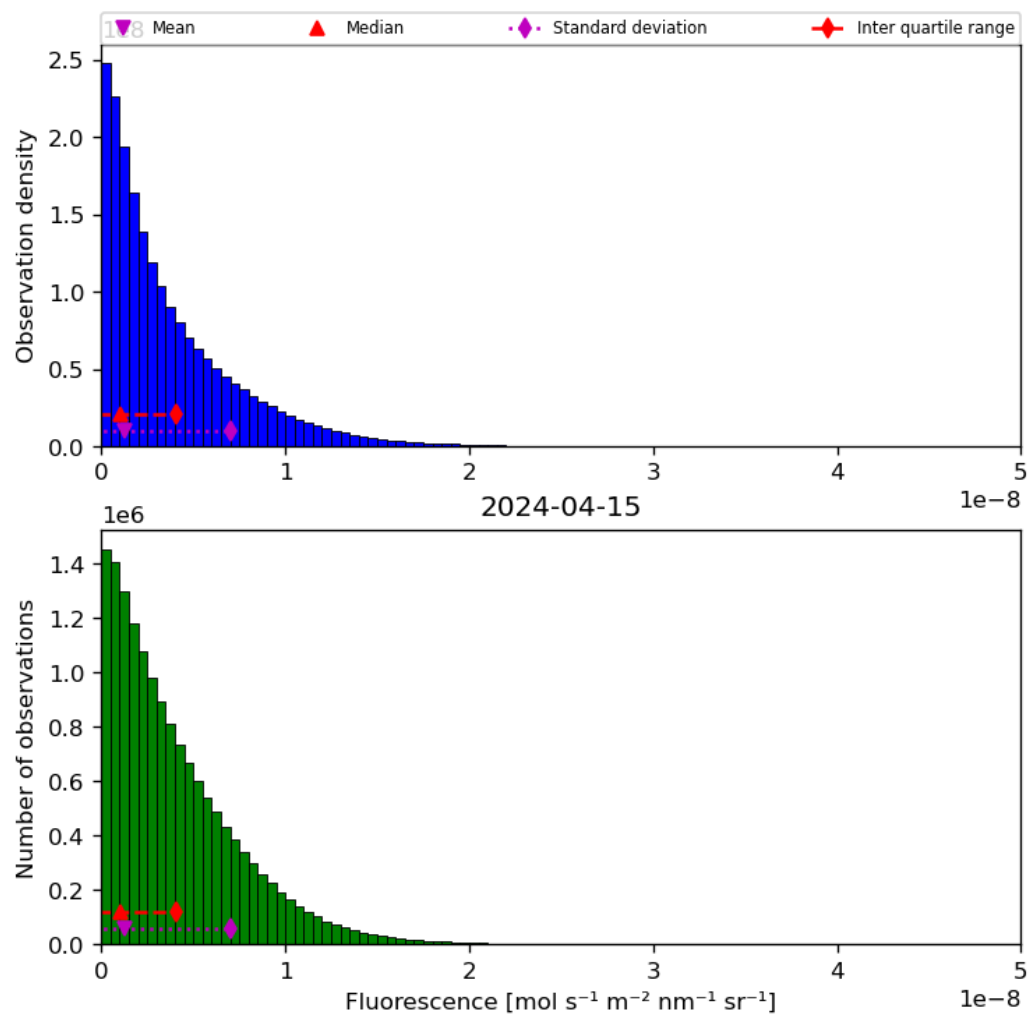
Figure 40: Histogram of “Fluorescence” for 2024-04-15 to 2024-04-16
