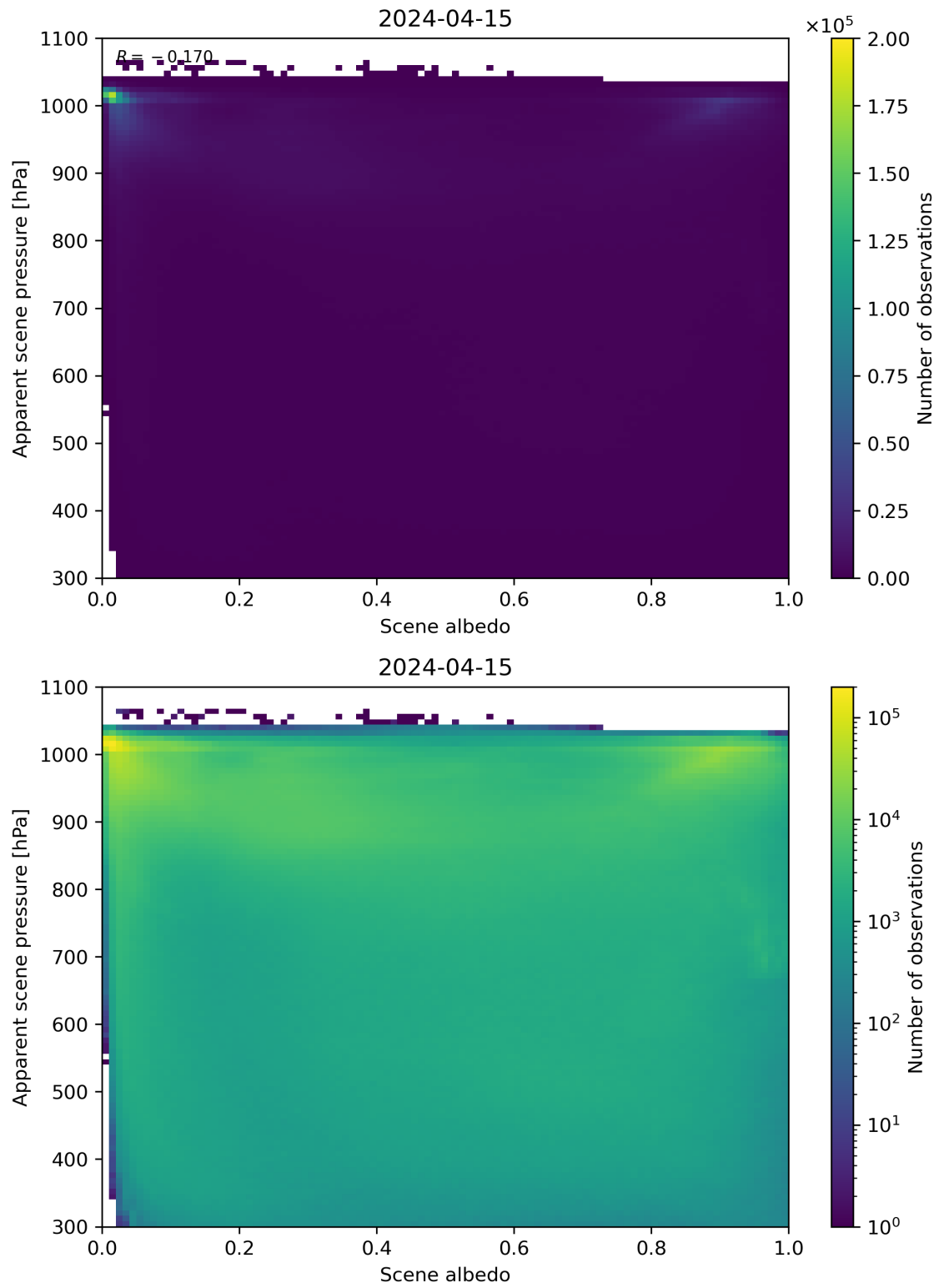
Figure 102: Scatter density plot of “Scene albedo” against “Apparent scene pressure” for 2024-04-15 to 2024-04-16.
