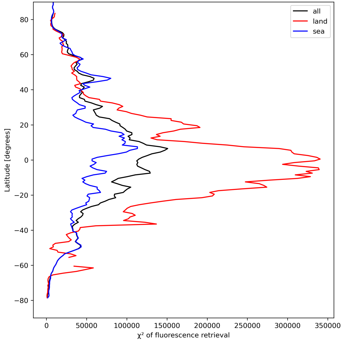
Figure 25: Zonal average of “ \chi^2 of fluorescence retrieval” for 2024-04-15 to 2024-04-16.
