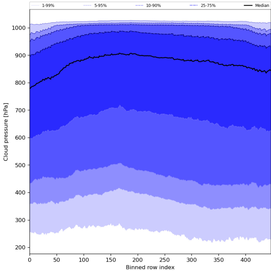
Figure 47: Along track statistics of “Cloud pressure” for 2024-04-15 to 2024-04-16
