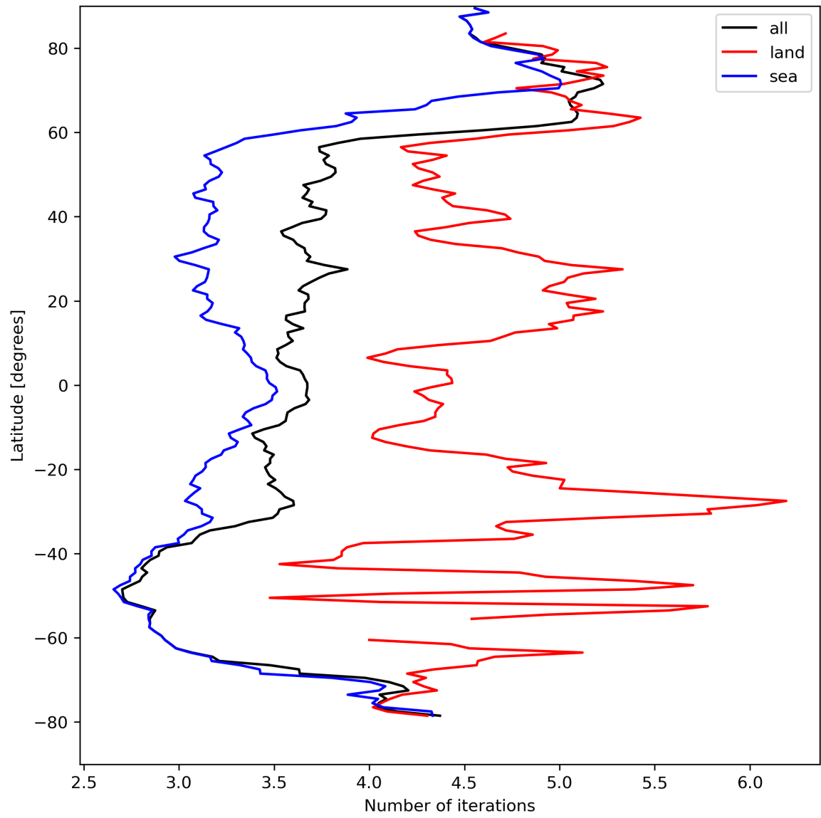
Figure 22: Zonal average of “Number of iterations” for 2024-04-15 to 2024-04-16.
