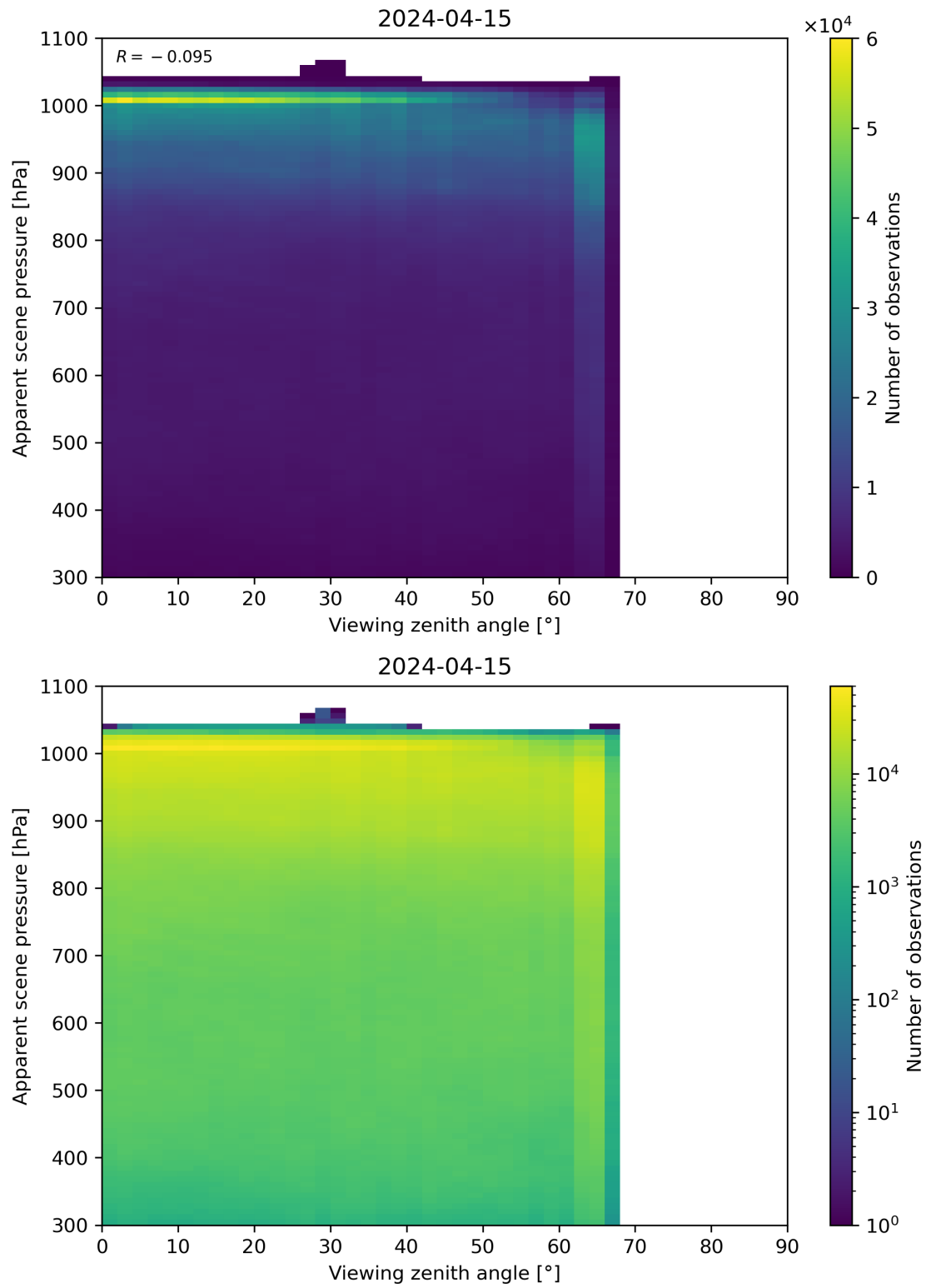
Figure 118: Scatter density plot of “Viewing zenith angle” against “Apparent scene pressure” for 2024-04-15 to 2024-04-16.
