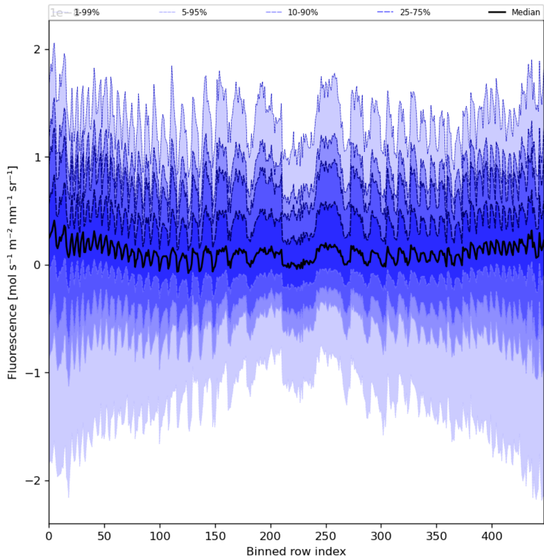
Figure 57: Along track statistics of “Fluorescence” for 2024-04-15 to 2024-04-16
