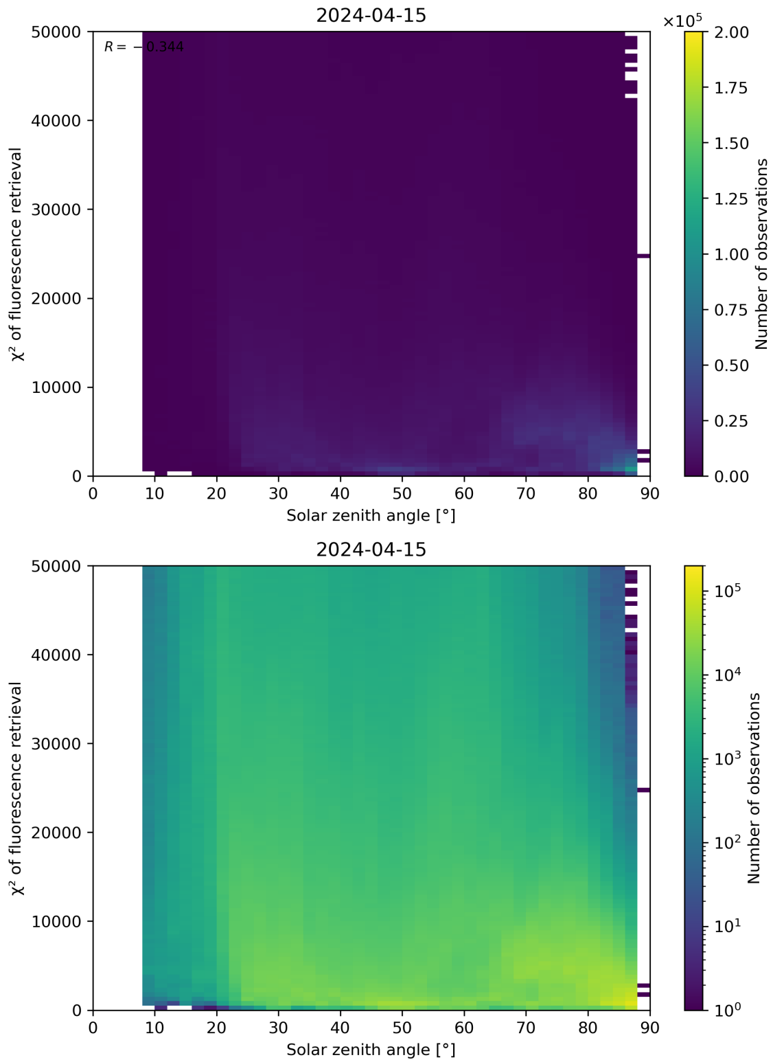
Figure 109: Scatter density plot of “Solar zenith angle” against “ \chi^2 of fluorescence retrieval” for 2024-04-15 to 2024-04-16.
