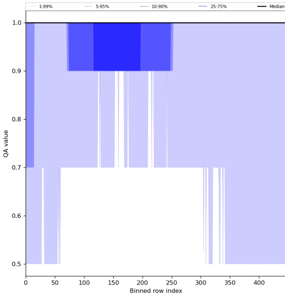
Figure 46: Along track statistics of "QA value" for 2024-04-15 to 2024-04-16
