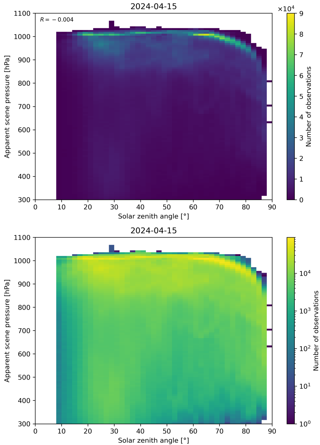
Figure 108: Scatter density plot of “Solar zenith angle” against “Apparent scene pressure” for 2024-04-15 to 2024-04-16.
