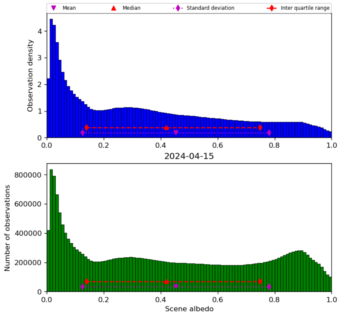
Figure 34: Histogram of “Scene albedo” for 2024-04-15 to 2024-04-16
