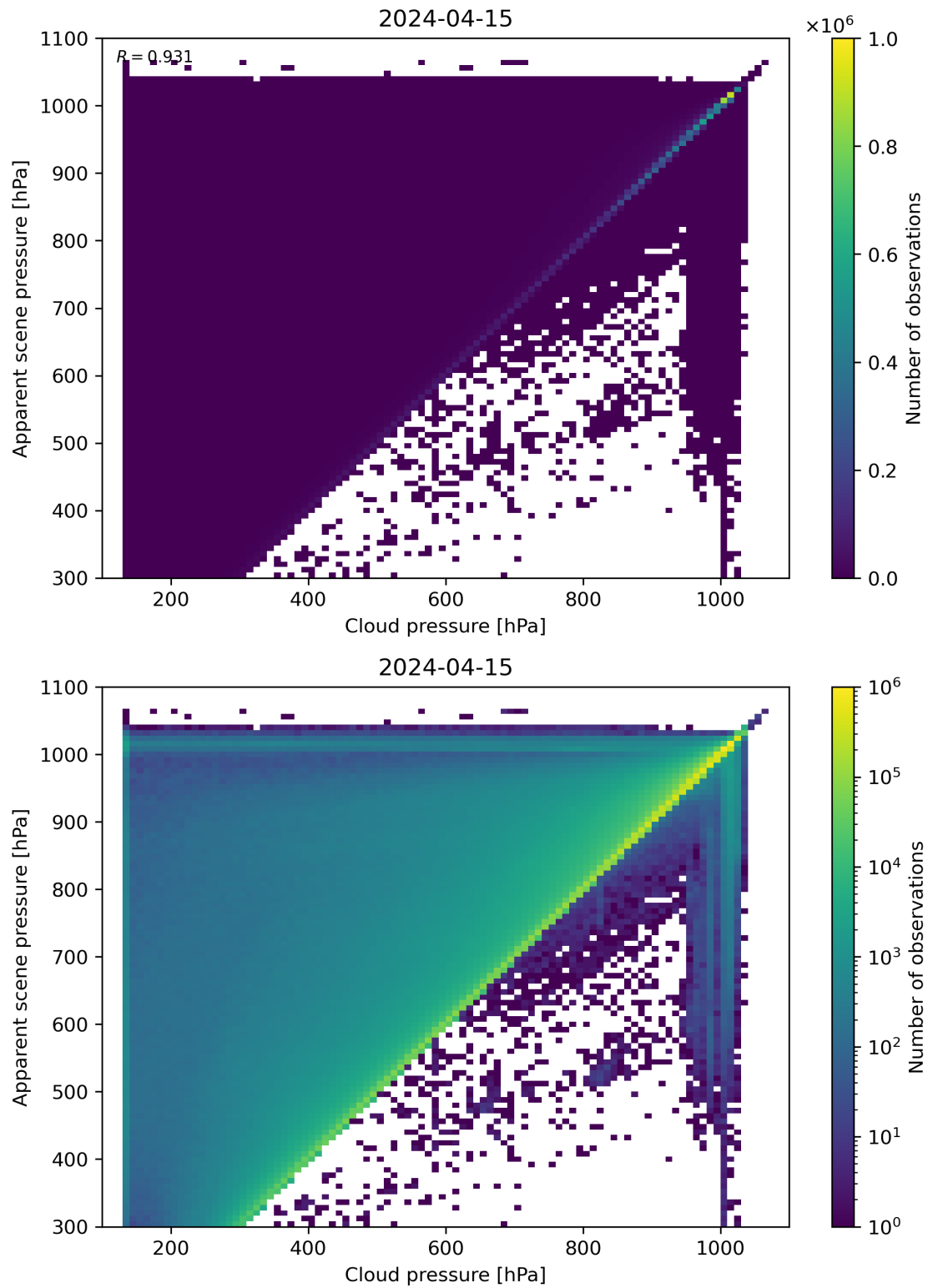
Figure 77: Scatter density plot of “Cloud pressure” against “Apparent scene pressure” for 2024-04-15 to 2024-04-16.
