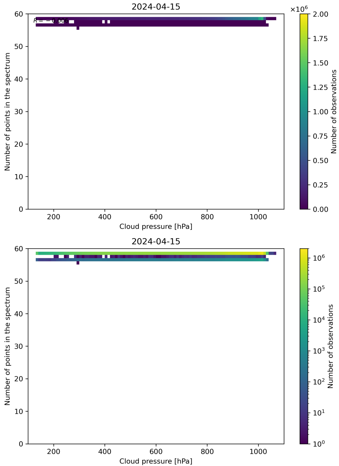
Figure 82: Scatter density plot of “Cloud pressure” against “Number of points in the spectrum” for 2024-04-15 to 2024-04-16.
