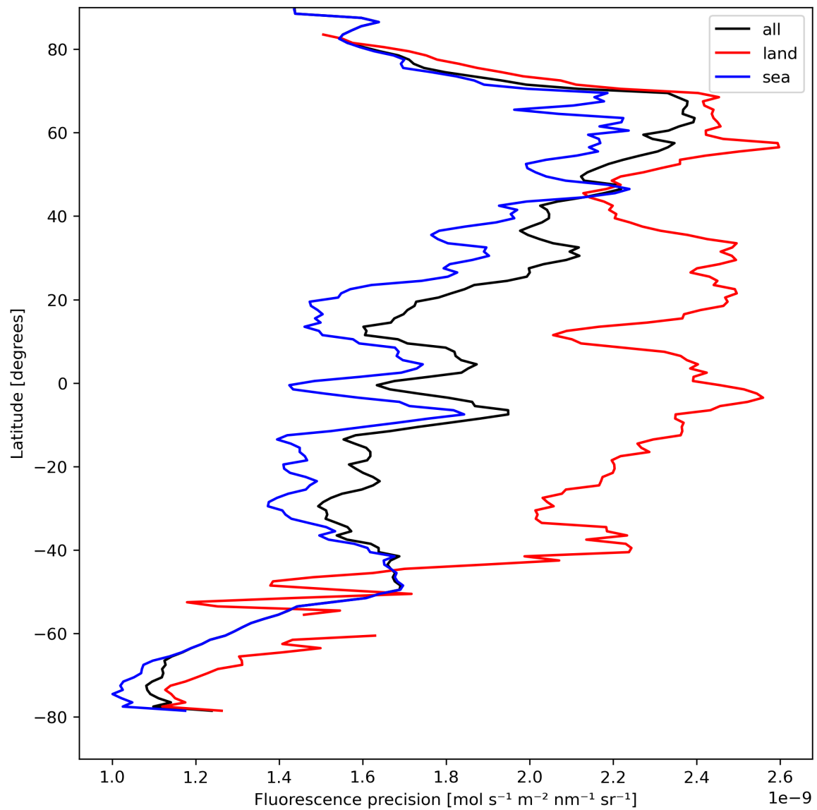
Figure 24: Zonal average of “Fluorescence precision” for 2024-04-15 to 2024-04-16.
