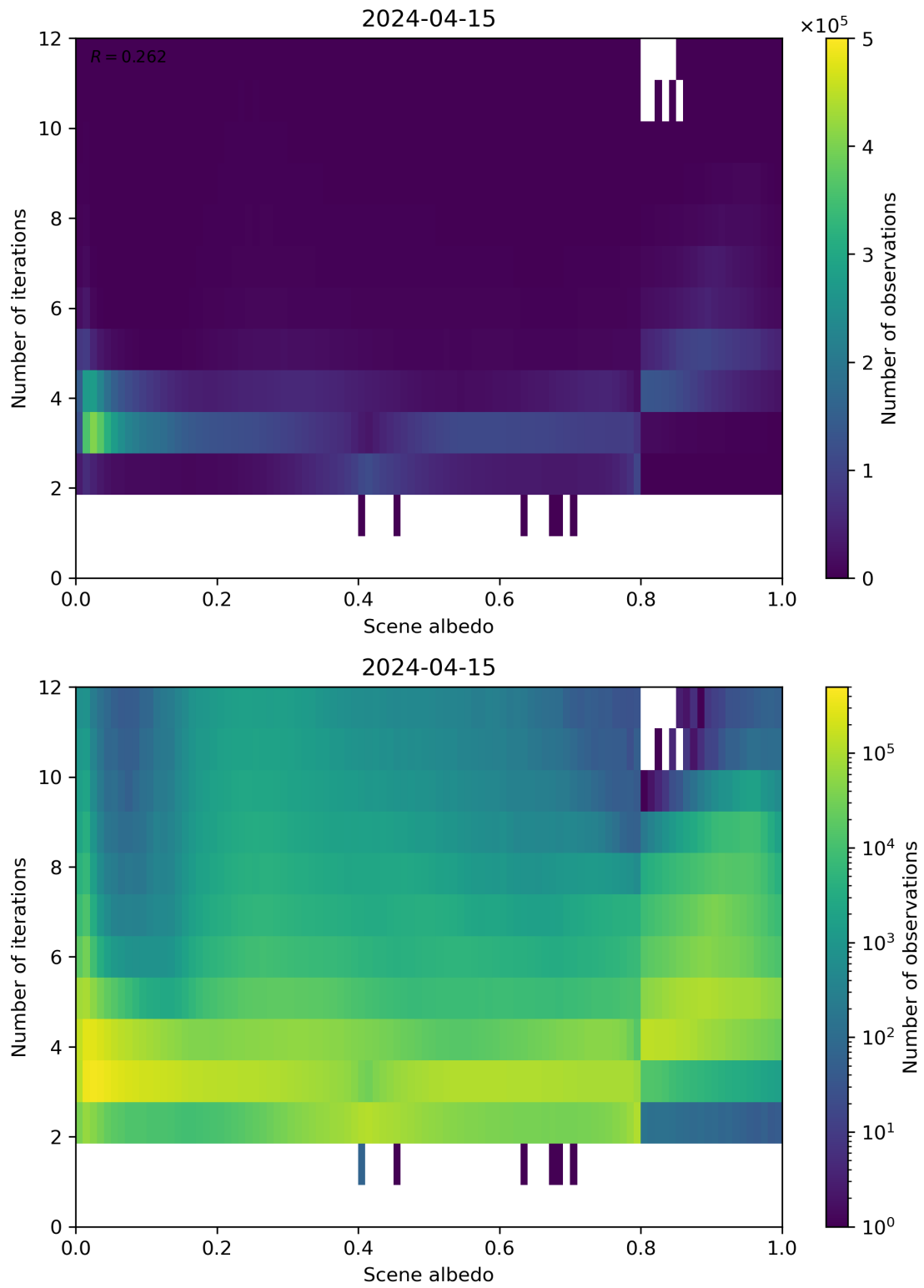
Figure 105: Scatter density plot of “Scene albedo” against “Number of iterations” for 2024-04-15 to 2024-04-16.
