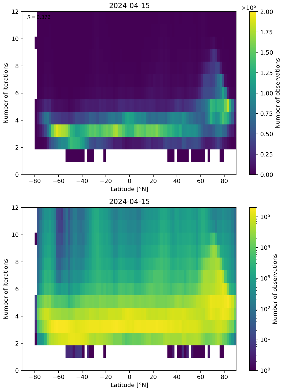
Figure 93: Scatter density plot of “Latitude” against “Number of iterations” for 2024-04-15 to 2024-04-16.
