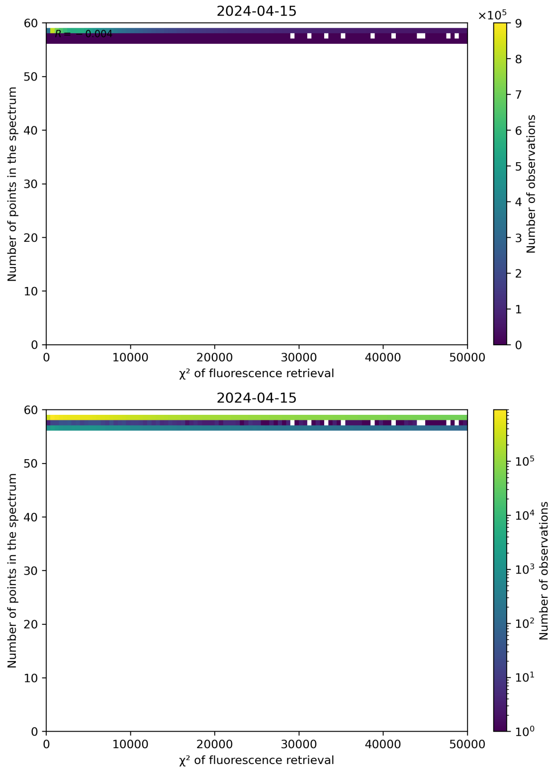
Figure 68: Scatter density plot of " \chi^2 of fluorescence retrieval" against "Number of points in the spectrum" for 2024-04-15 to 2024-04-16.
