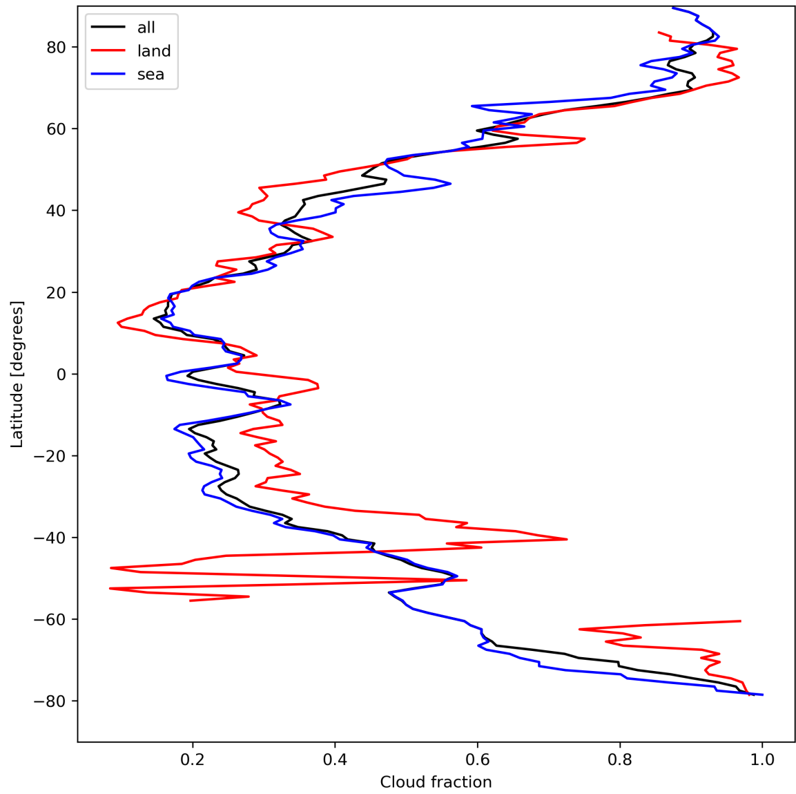
Figure 15: Zonal average of “Cloud fraction” for 2024-04-15 to 2024-04-16.
