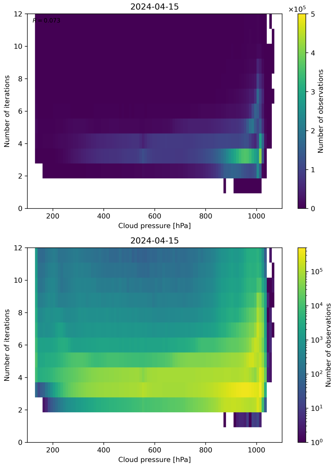
Figure 81: Scatter density plot of “Cloud pressure” against “Number of iterations” for 2024-04-15 to 2024-04-16.
