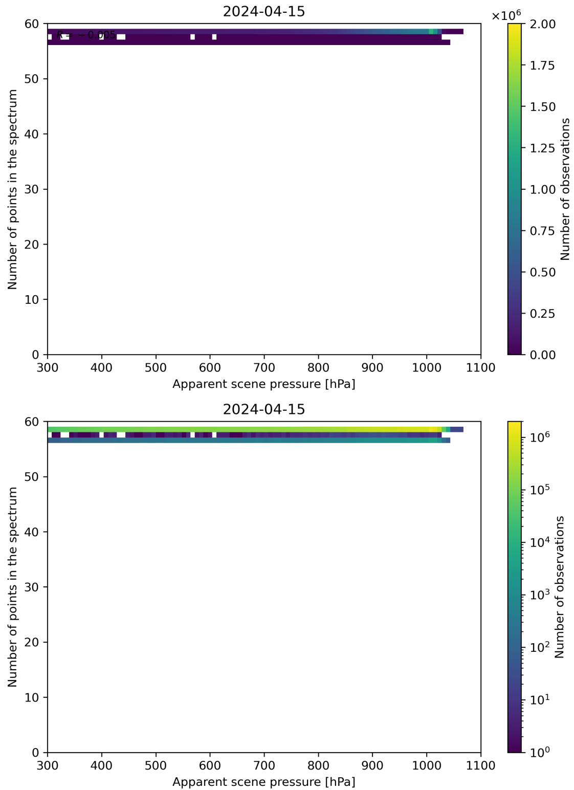
Figure 66: Scatter density plot of “Apparent scene pressure” against “Number of points in the spectrum” for 2024-04-15 to 2024-04-16.
