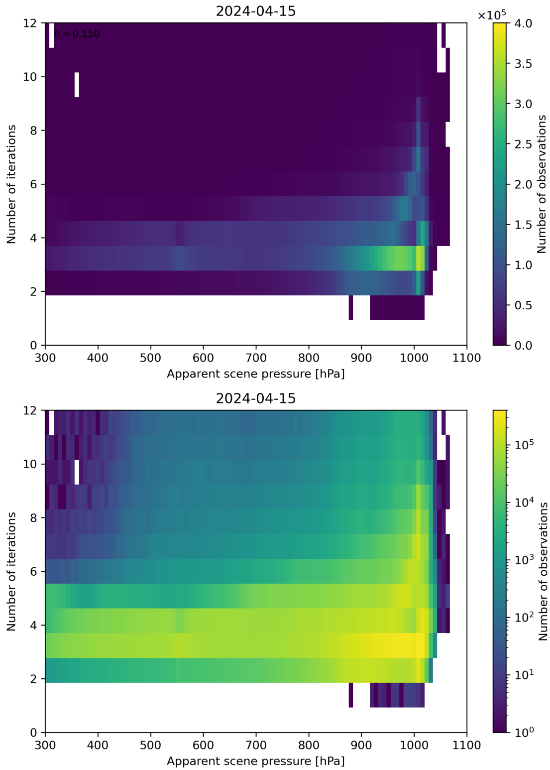
Figure 65: Scatter density plot of “Apparent scene pressure” against “Number of iterations” for 2024-04-15 to 2024-04-16.
