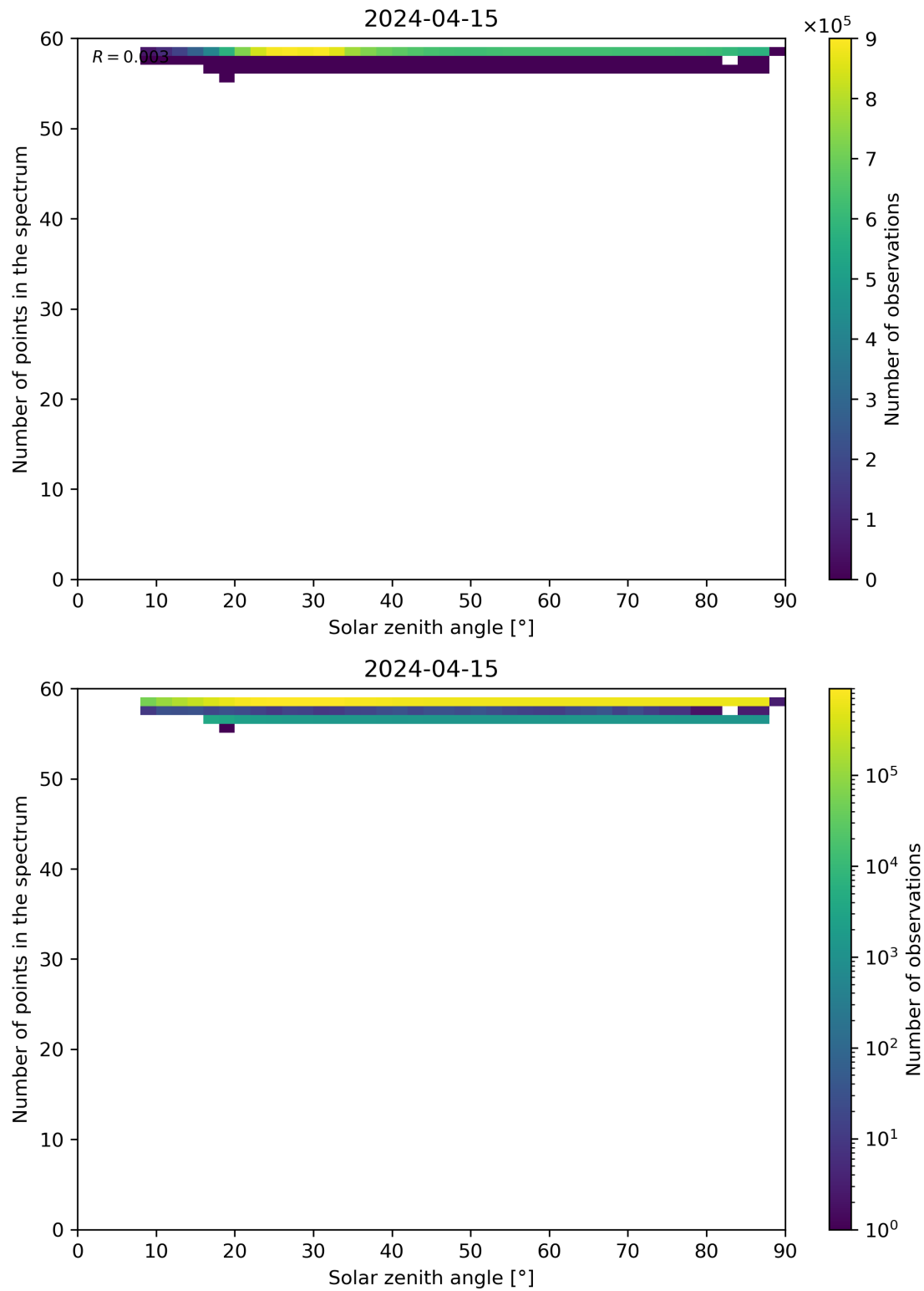
Figure 115: Scatter density plot of “Solar zenith angle” against “Number of points in the spectrum” for 2024-04-15 to 2024-04-16.
