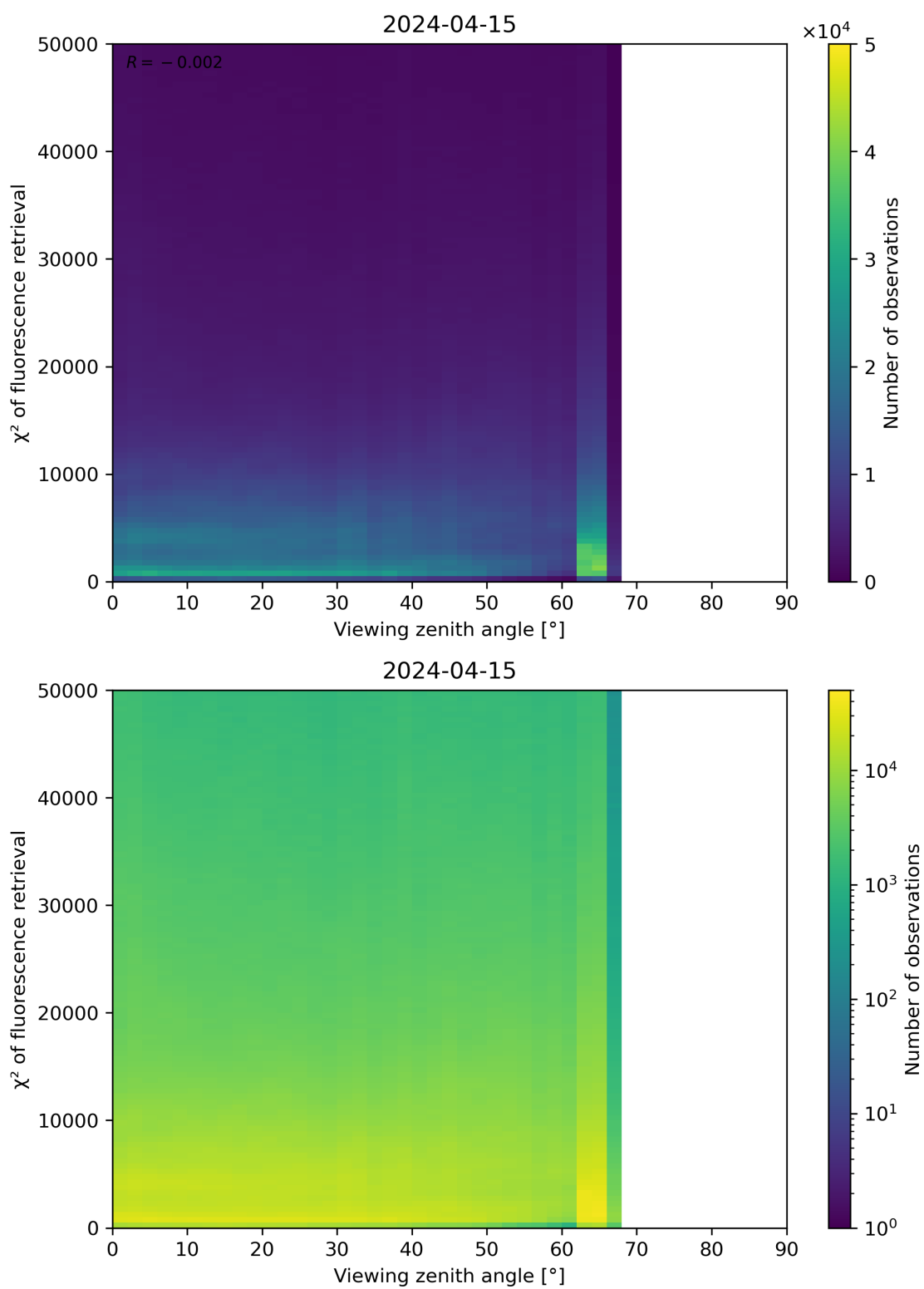
Figure 119: Scatter density plot of “Viewing zenith angle” against “ \chi^2 of fluorescence retrieval” for 2024-04-15 to 2024-04-16.
