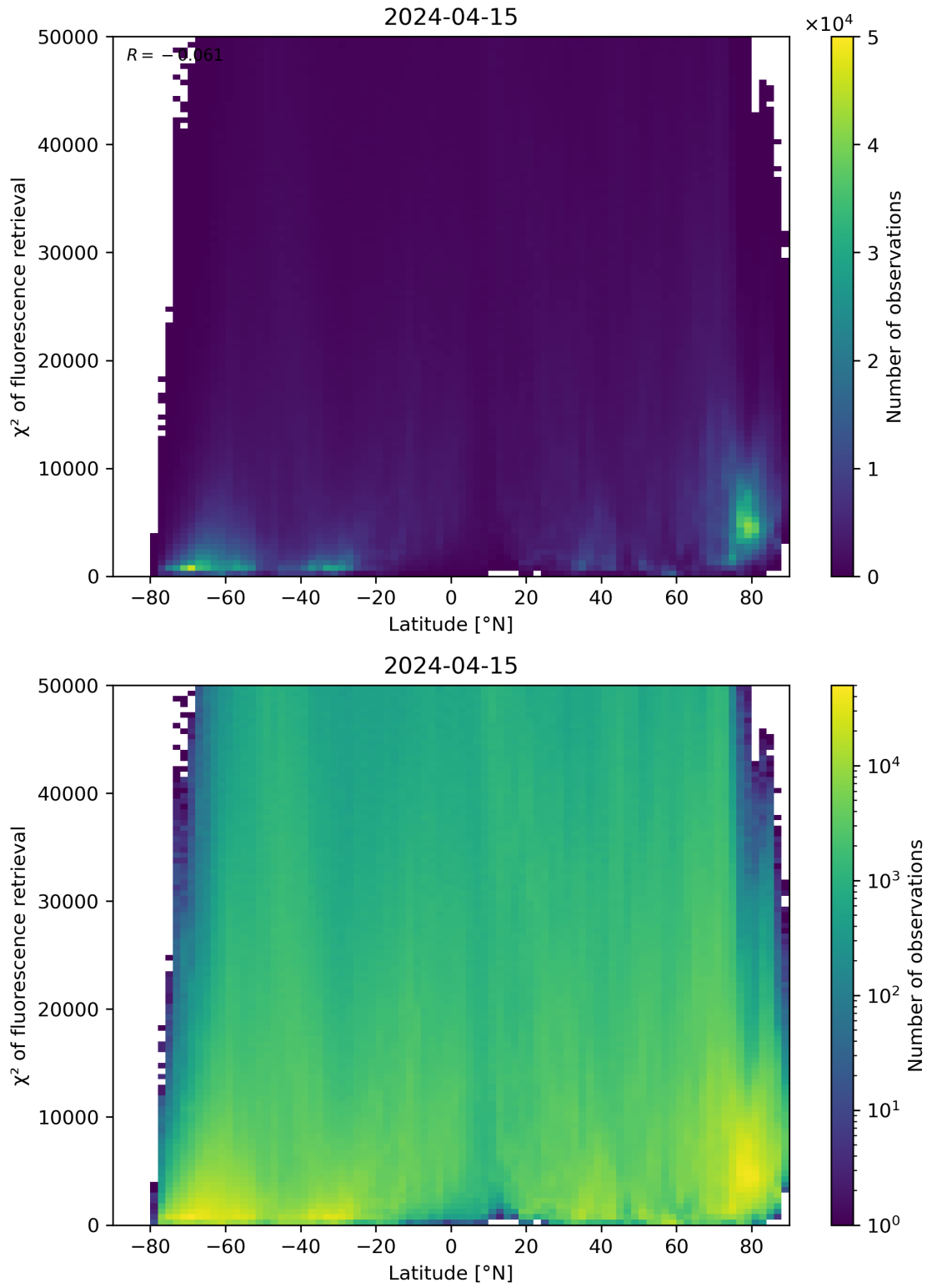
Figure 89: Scatter density plot of “Latitude” against “ \chi^2 of fluorescence retrieval” for 2024-04-15 to 2024-04-16.
