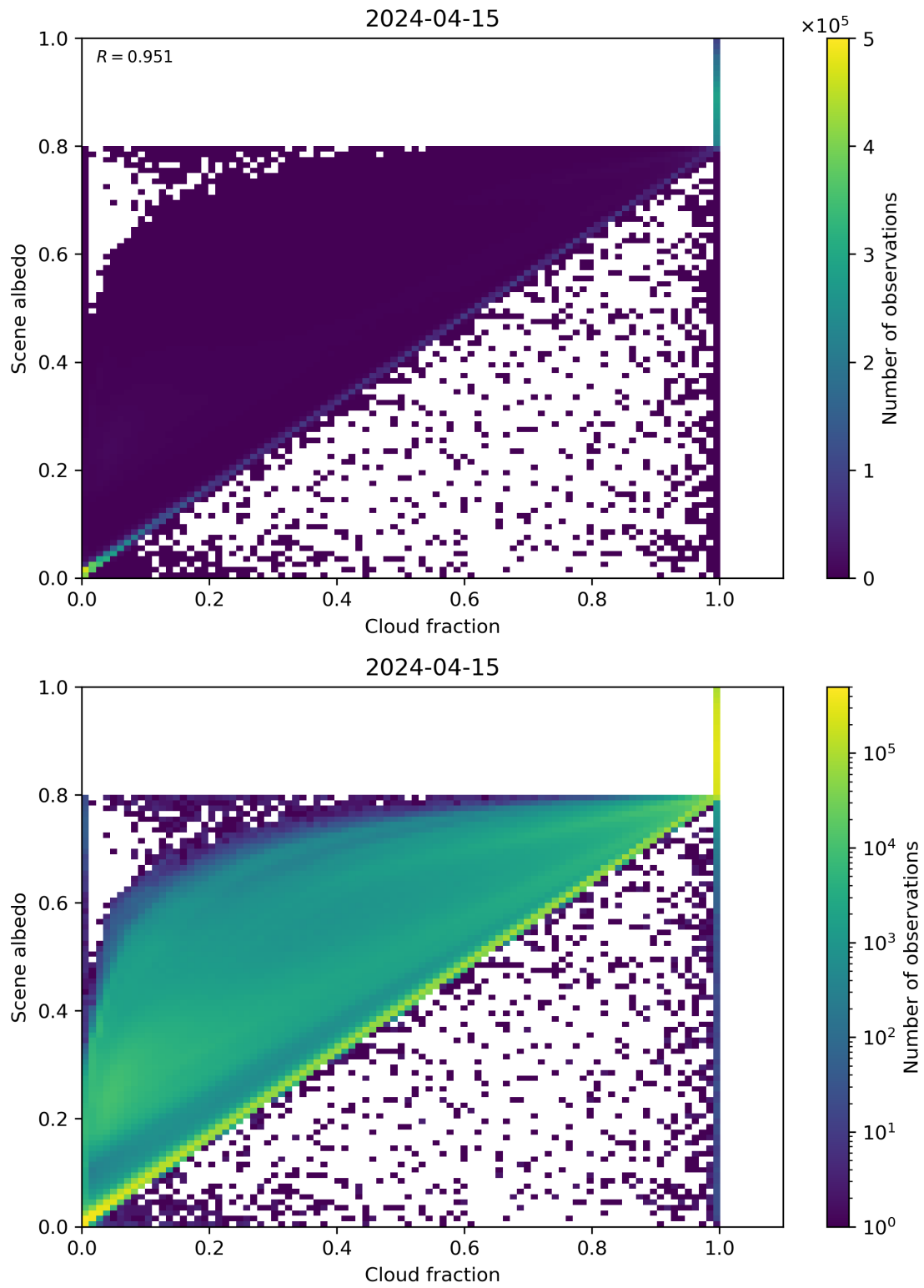
Figure 75: Scatter density plot of “Cloud fraction” against “Scene albedo” for 2024-04-15 to 2024-04-16.
