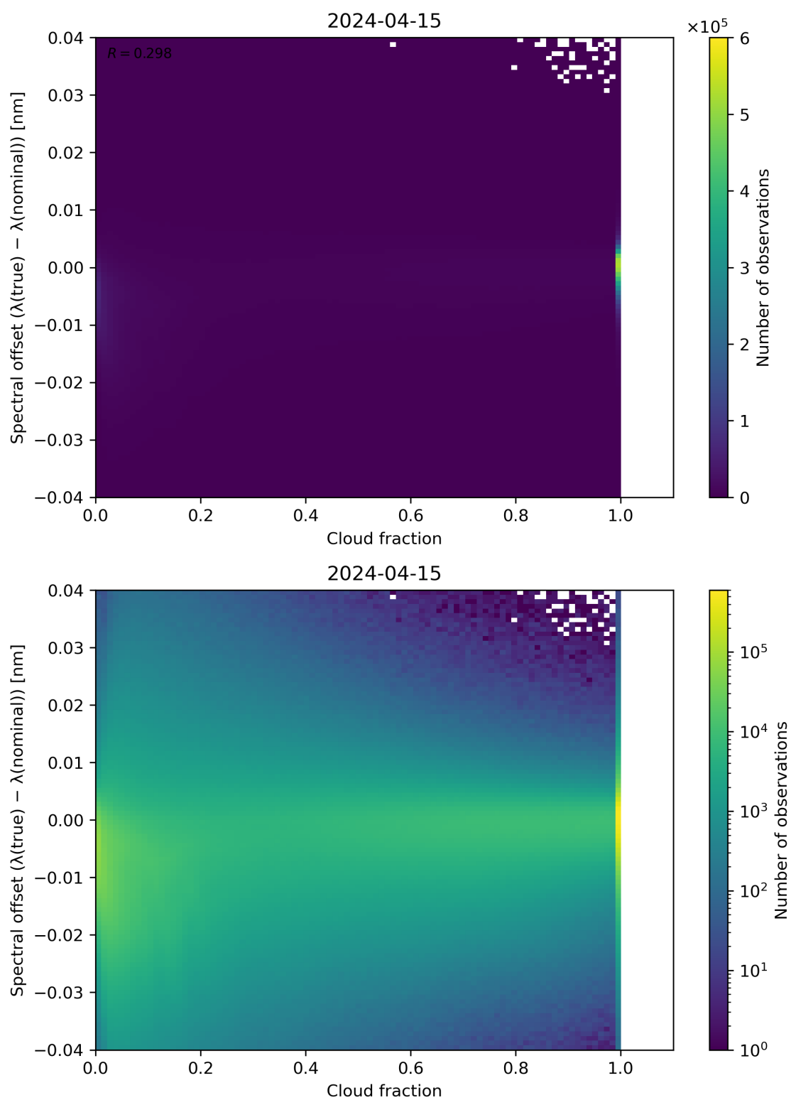
Figure 76: Scatter density plot of “Cloud fraction” against “Spectral offset ( \lambda(\text{true}) - \lambda(\text{nominal}) )” for 2024-04-15 to 2024-04-16.
