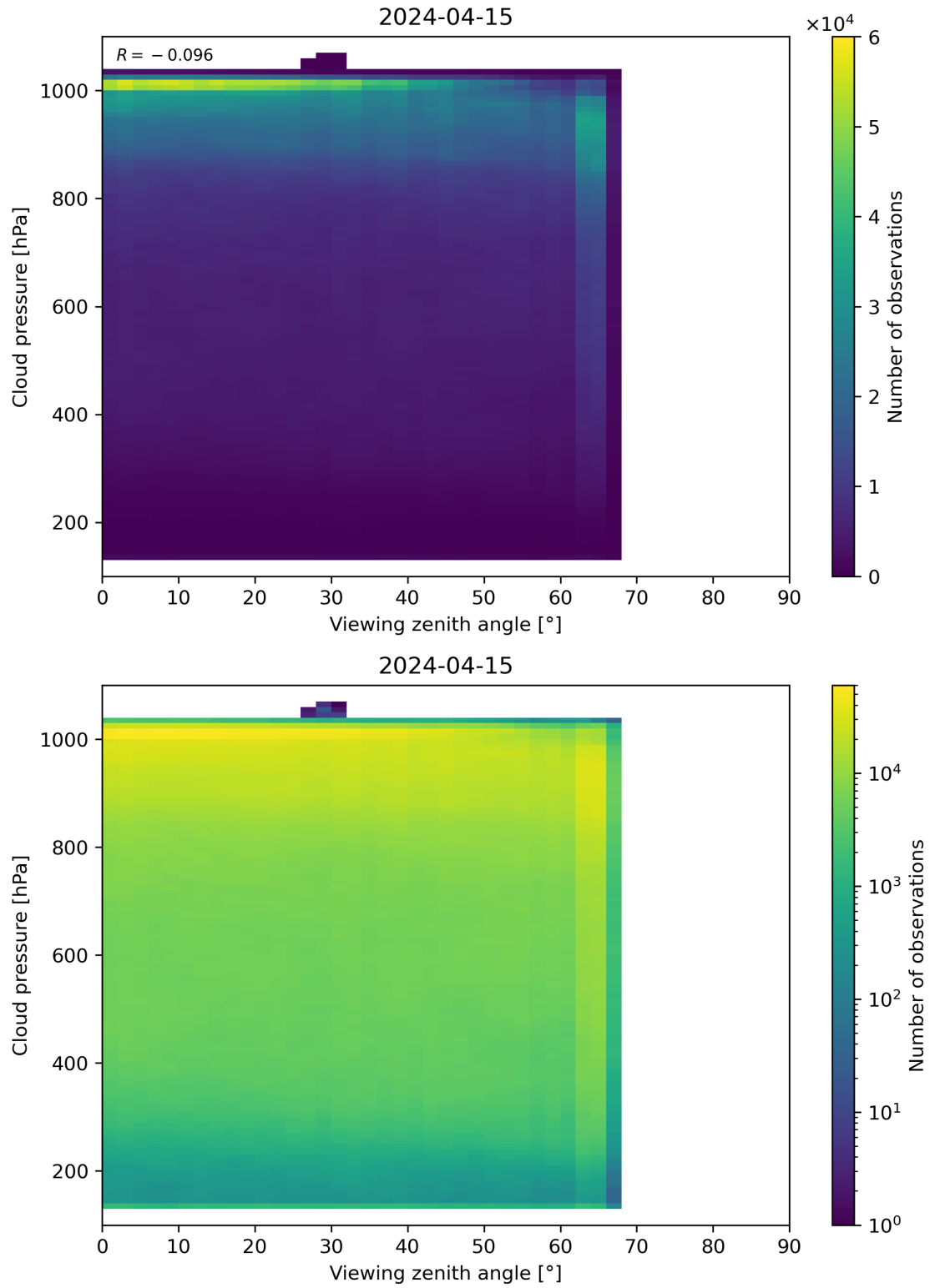
Figure 121: Scatter density plot of “Viewing zenith angle” against “Cloud pressure” for 2024-04-15 to 2024-04-16.
