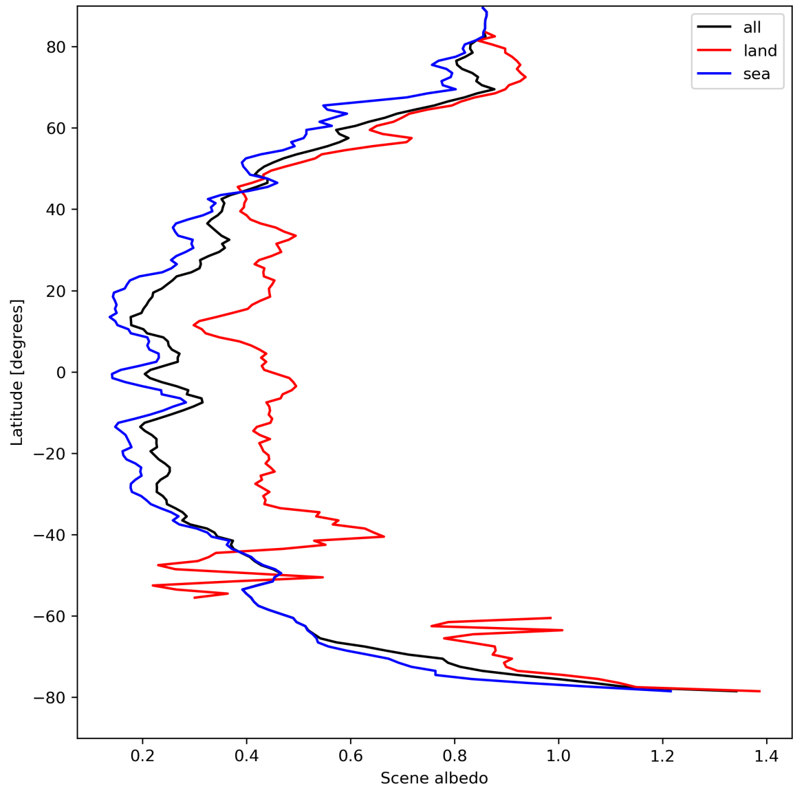
Figure 17: Zonal average of “Scene albedo” for 2024-04-15 to 2024-04-16.
