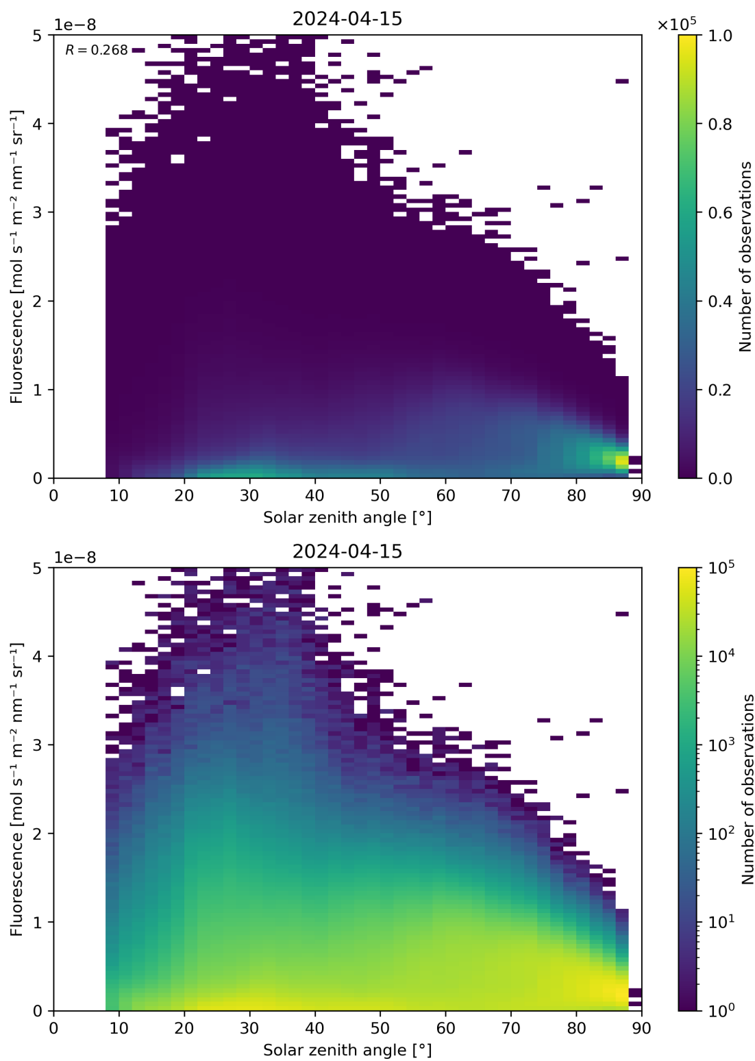
Figure 112: Scatter density plot of “Solar zenith angle” against “Fluorescence” for 2024-04-15 to 2024-04-16.
