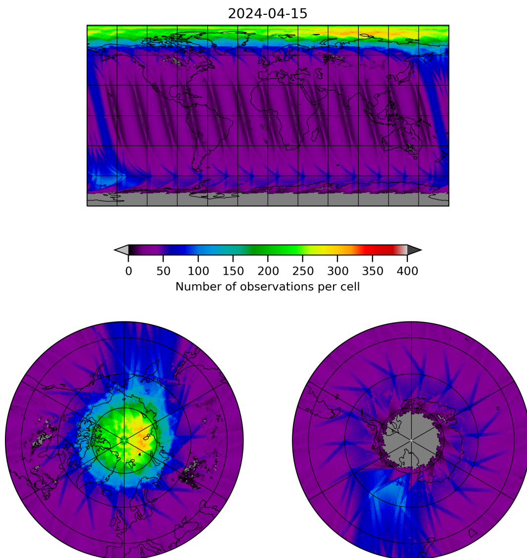
Figure 11: Map of the number of observations for 2024-04-15 to 2024-04-16
