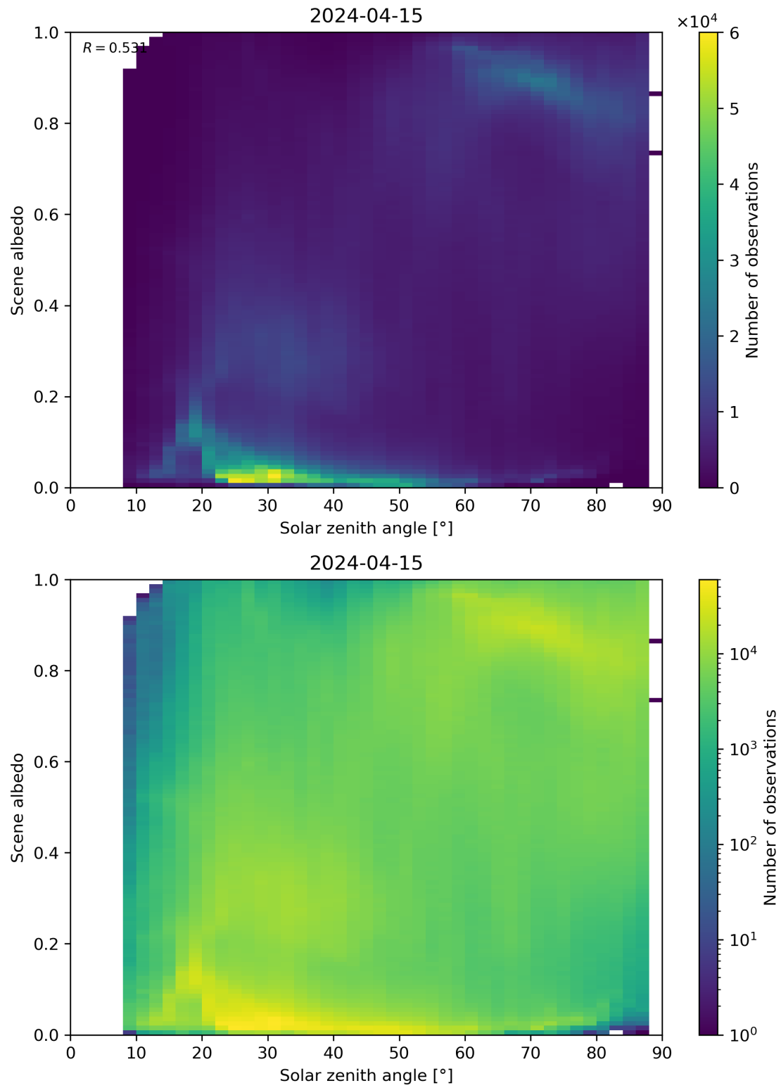
Figure 116: Scatter density plot of “Solar zenith angle” against “Scene albedo” for 2024-04-15 to 2024-04-16.
