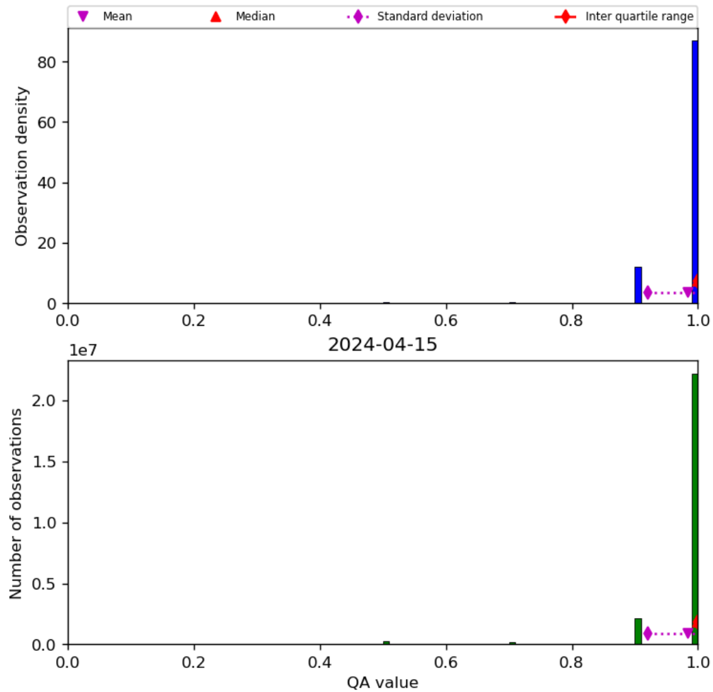
Figure 29: Histogram of “QA value” for 2024-04-15 to 2024-04-16
