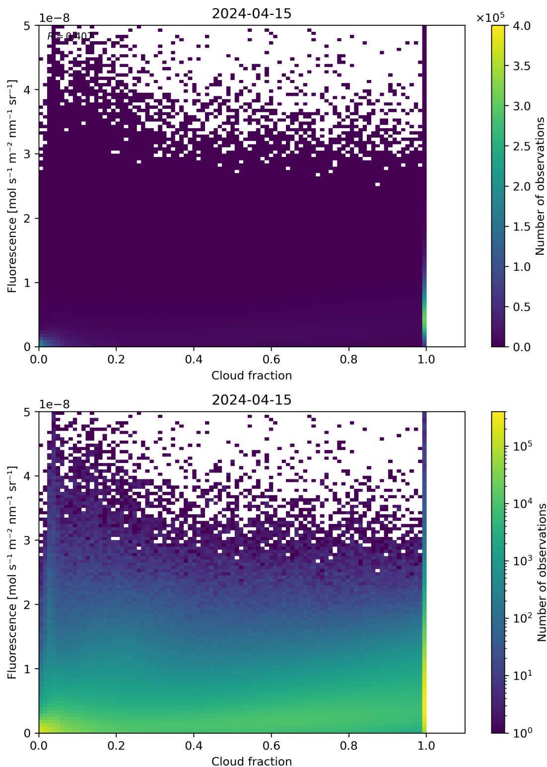
Figure 72: Scatter density plot of “Cloud fraction” against “Fluorescence” for 2024-04-15 to 2024-04-16.
