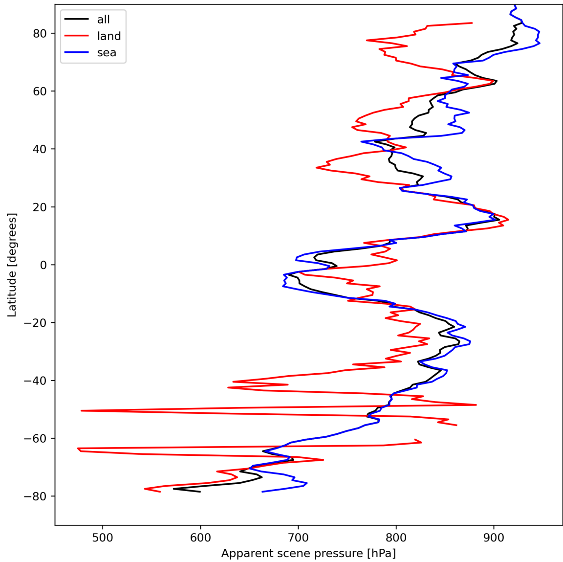
Figure 19: Zonal average of “Apparent scene pressure” for 2024-04-15 to 2024-04-16.
