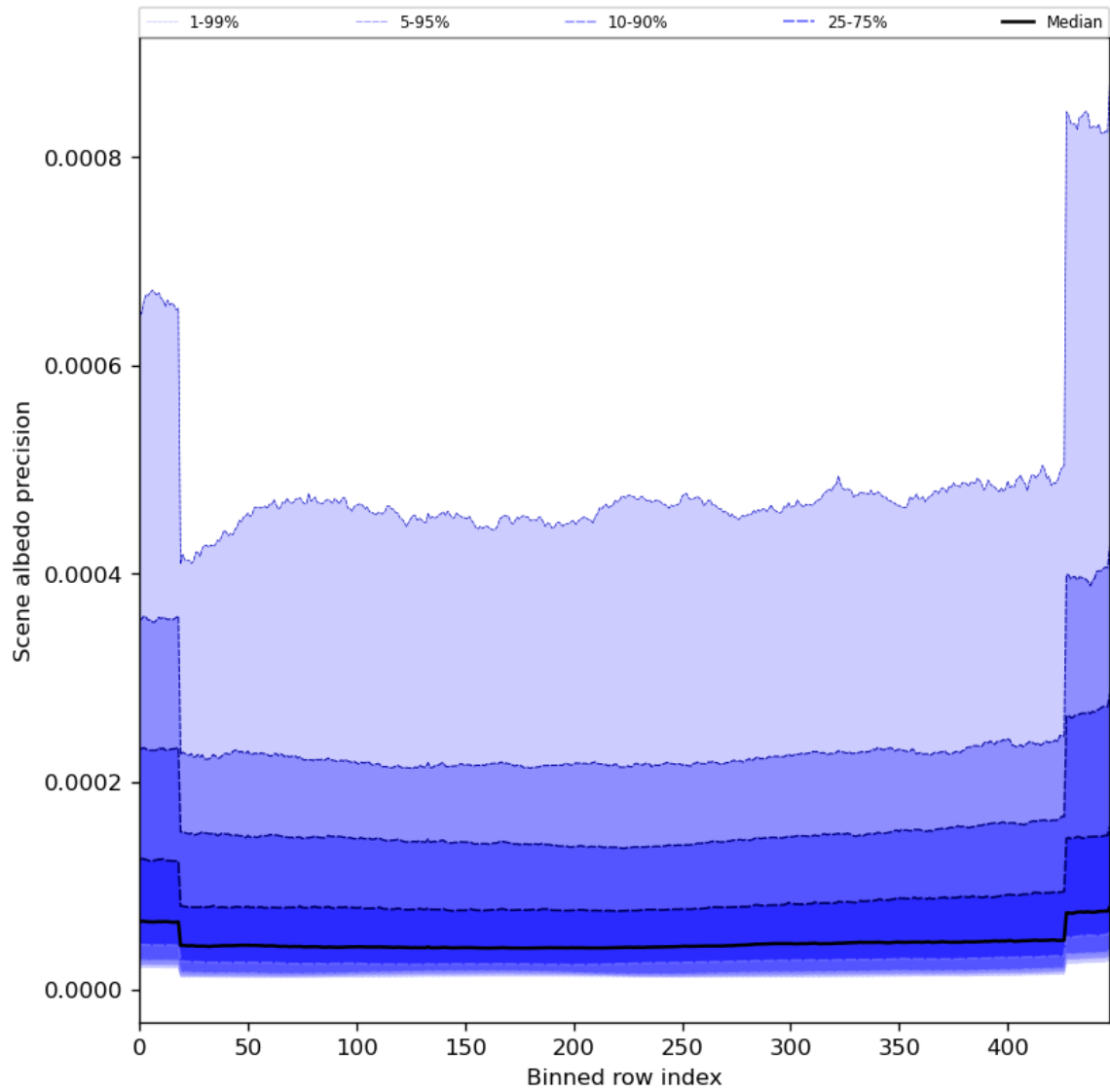
Figure 52: Along track statistics of “Scene albedo precision” for 2024-04-15 to 2024-04-16
