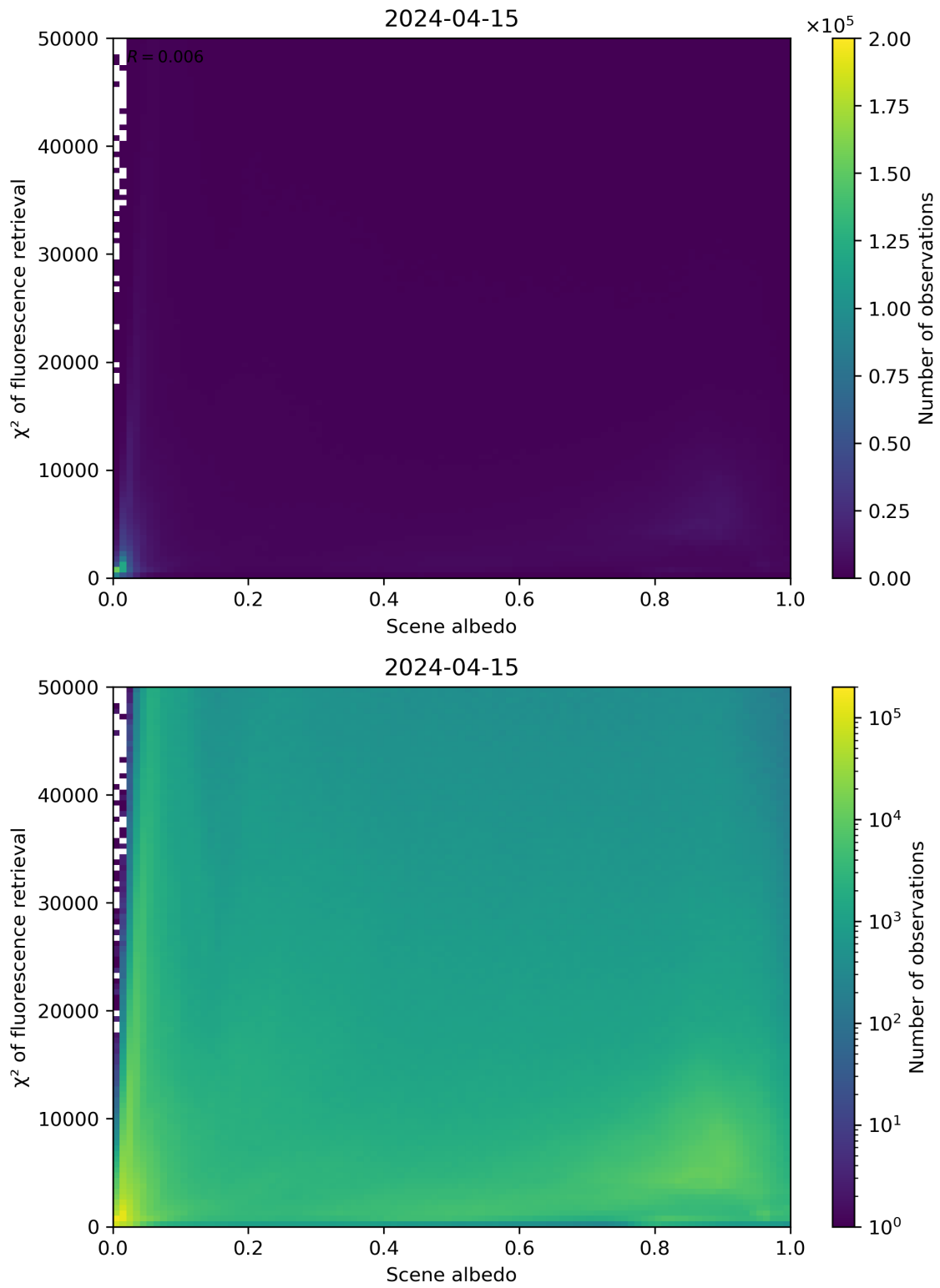
Figure 103: Scatter density plot of “Scene albedo” against “ \chi^2 of fluorescence retrieval” for 2024-04-15 to 2024-04-16.
