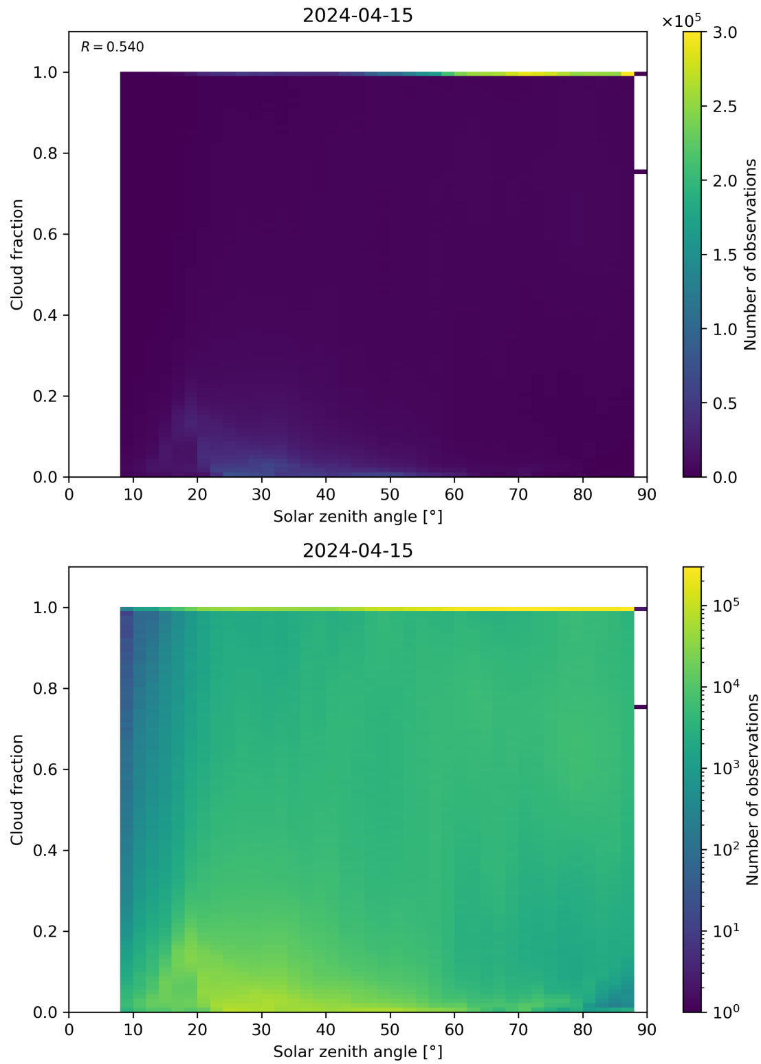
Figure 110: Scatter density plot of “Solar zenith angle” against “Cloud fraction” for 2024-04-15 to 2024-04-16.
