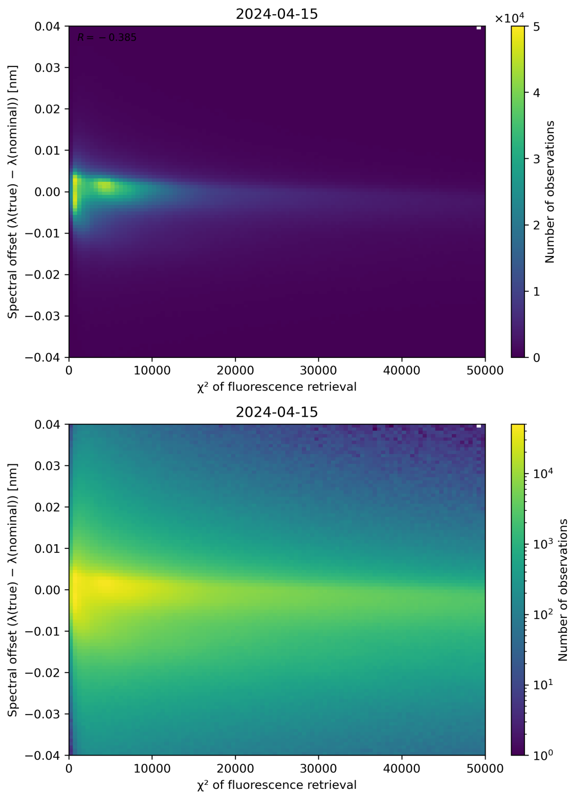
Figure 69: Scatter density plot of " \chi^2 of fluorescence retrieval" against "Spectral offset ( \lambda(\text{true}) - \lambda(\text{nominal}) )" for 2024-04-15 to 2024-04-16.
