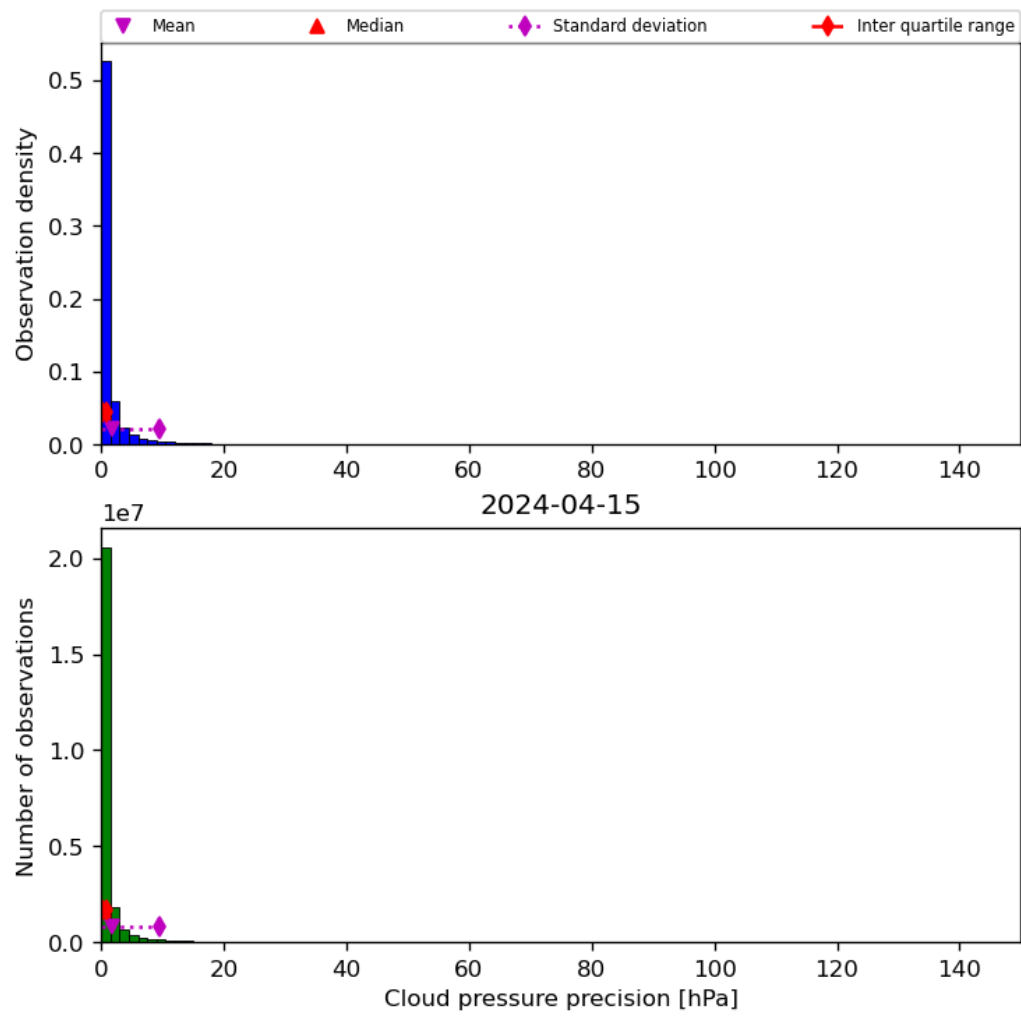
Figure 31: Histogram of “Cloud pressure precision” for 2024-04-15 to 2024-04-16
