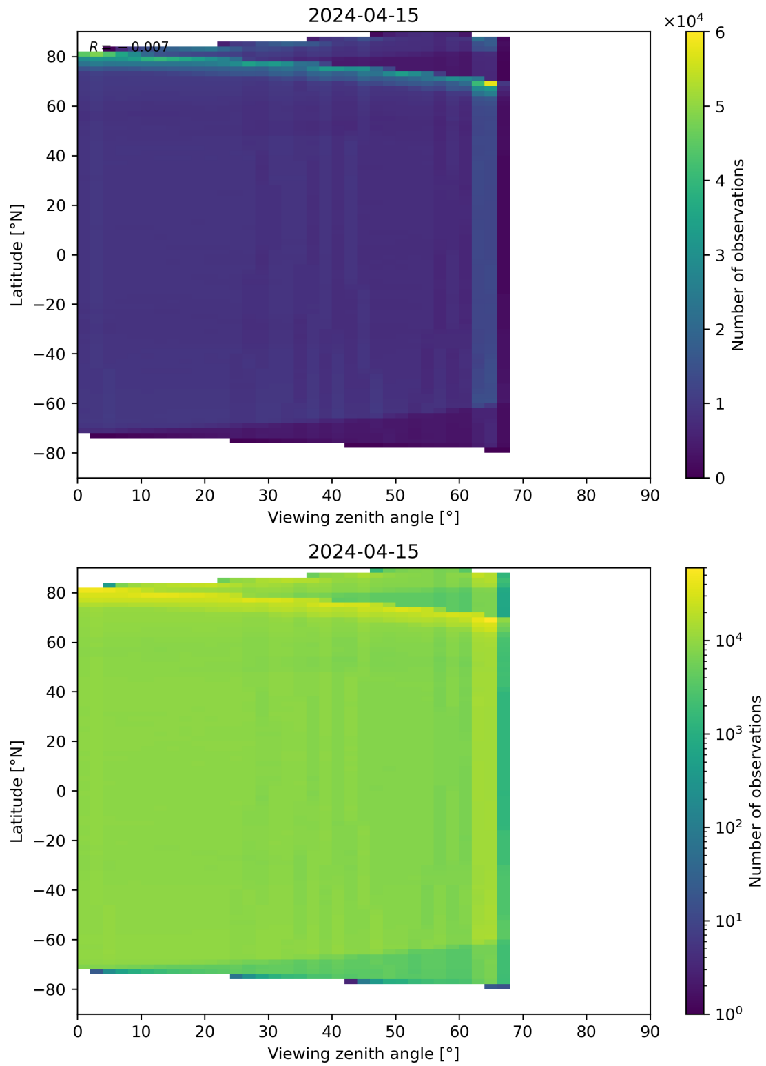
Figure 123: Scatter density plot of “Viewing zenith angle” against “Latitude” for 2024-04-15 to 2024-04-16.
