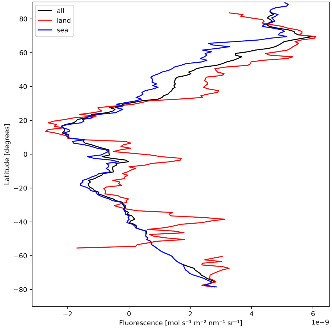
Figure 23: Zonal average of “Fluorescence” for 2024-04-15 to 2024-04-16.
