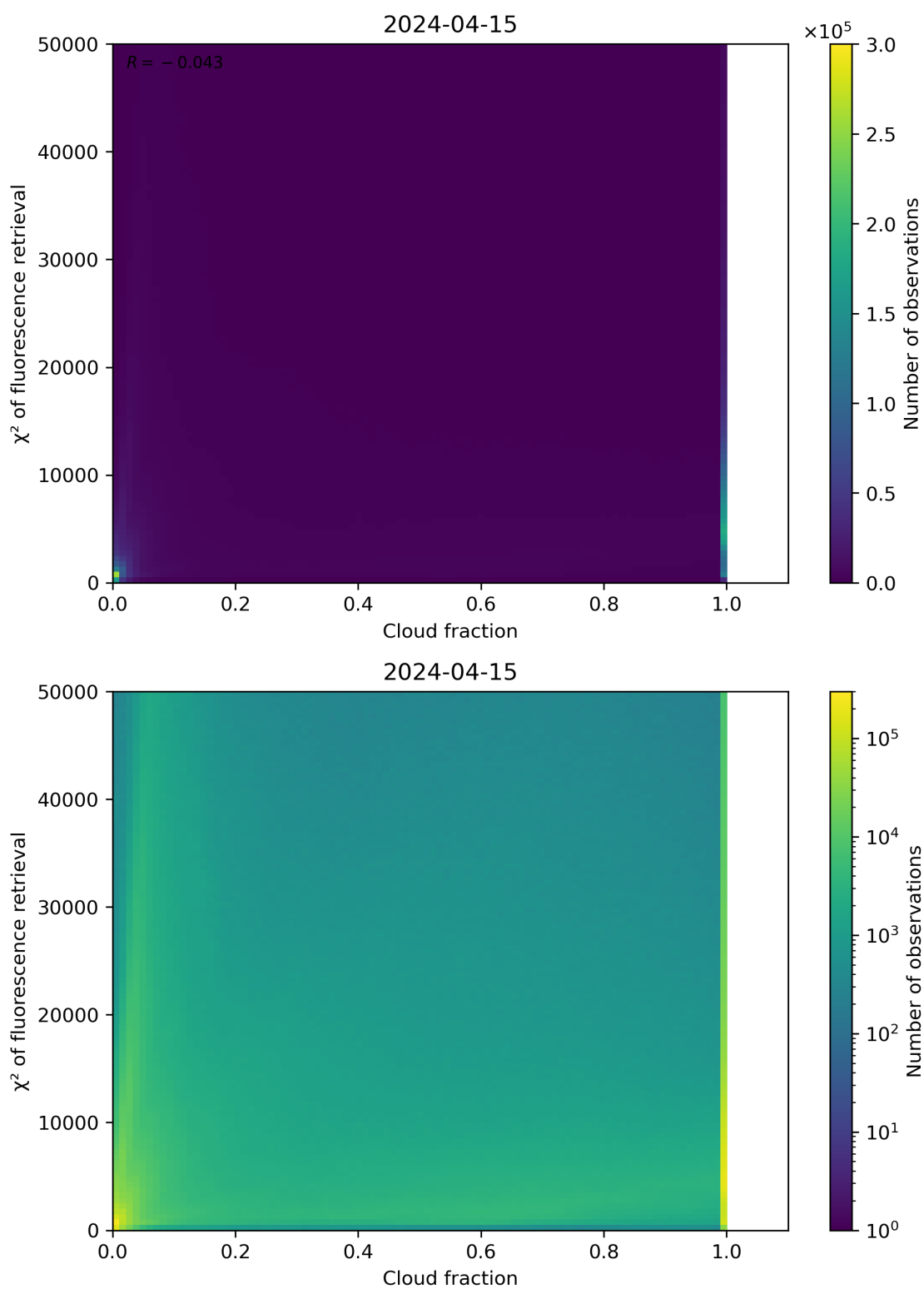
Figure 71: Scatter density plot of “Cloud fraction” against “ \chi^2 of fluorescence retrieval” for 2024-04-15 to 2024-04-16.
