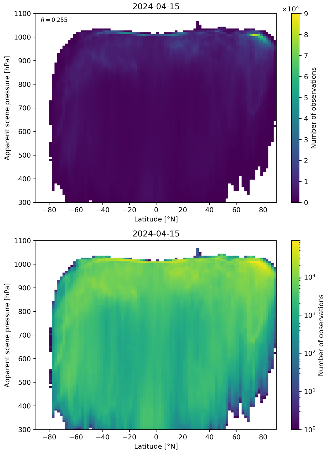
Figure 88: Scatter density plot of “Latitude” against “Apparent scene pressure” for 2024-04-15 to 2024-04-16.
