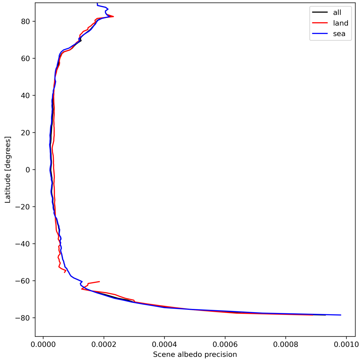
Figure 18: Zonal average of “Scene albedo precision” for 2024-04-15 to 2024-04-16.
