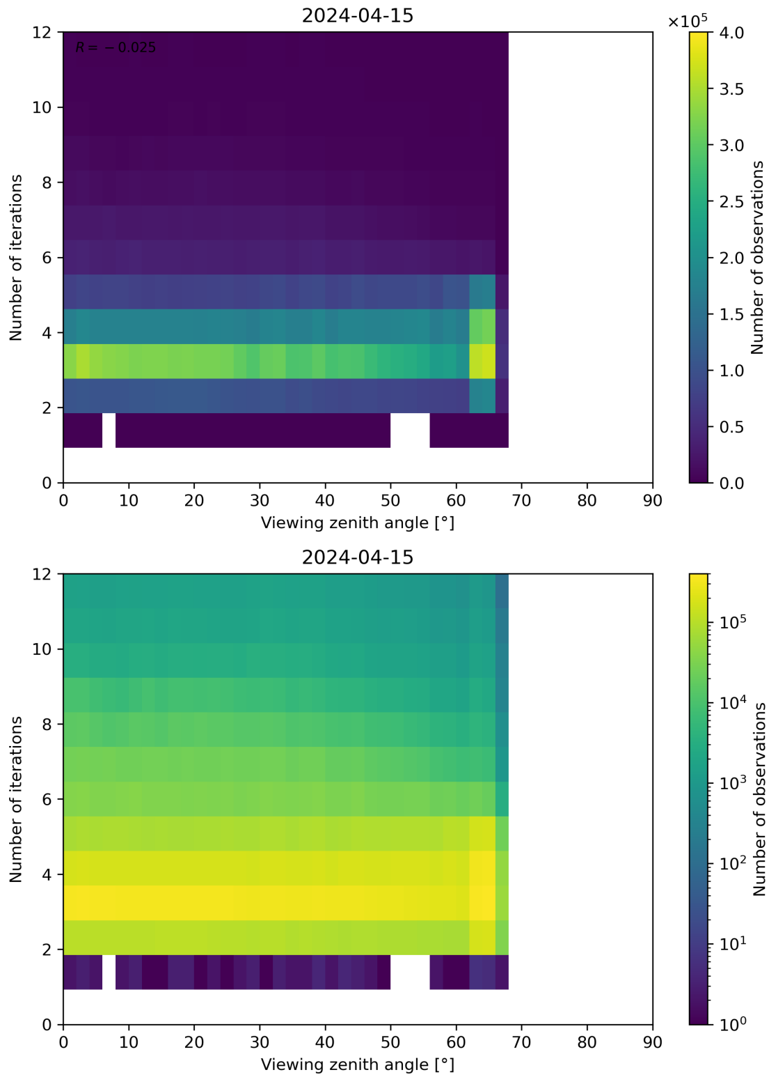
Figure 124: Scatter density plot of “Viewing zenith angle” against “Number of iterations” for 2024-04-15 to 2024-04-16.
