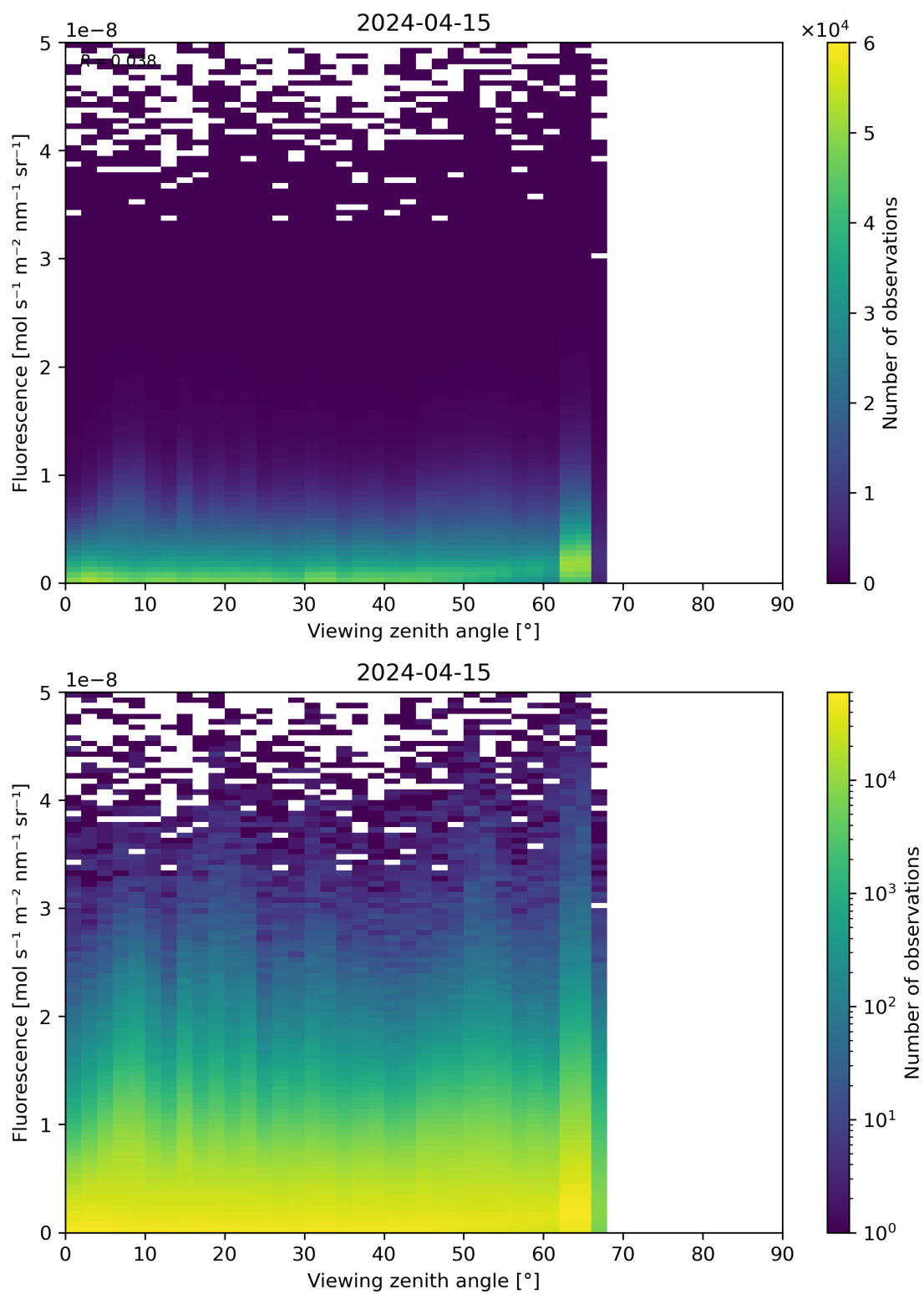
Figure 122: Scatter density plot of “Viewing zenith angle” against “Fluorescence” for 2024-04-15 to 2024-04-16.
