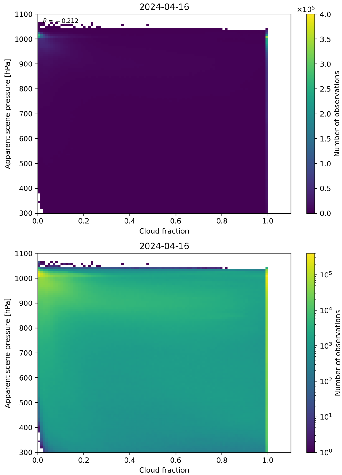
Figure 70: Scatter density plot of “Cloud fraction” against “Apparent scene pressure” for 2024-04-16 to 2024-04-17.
