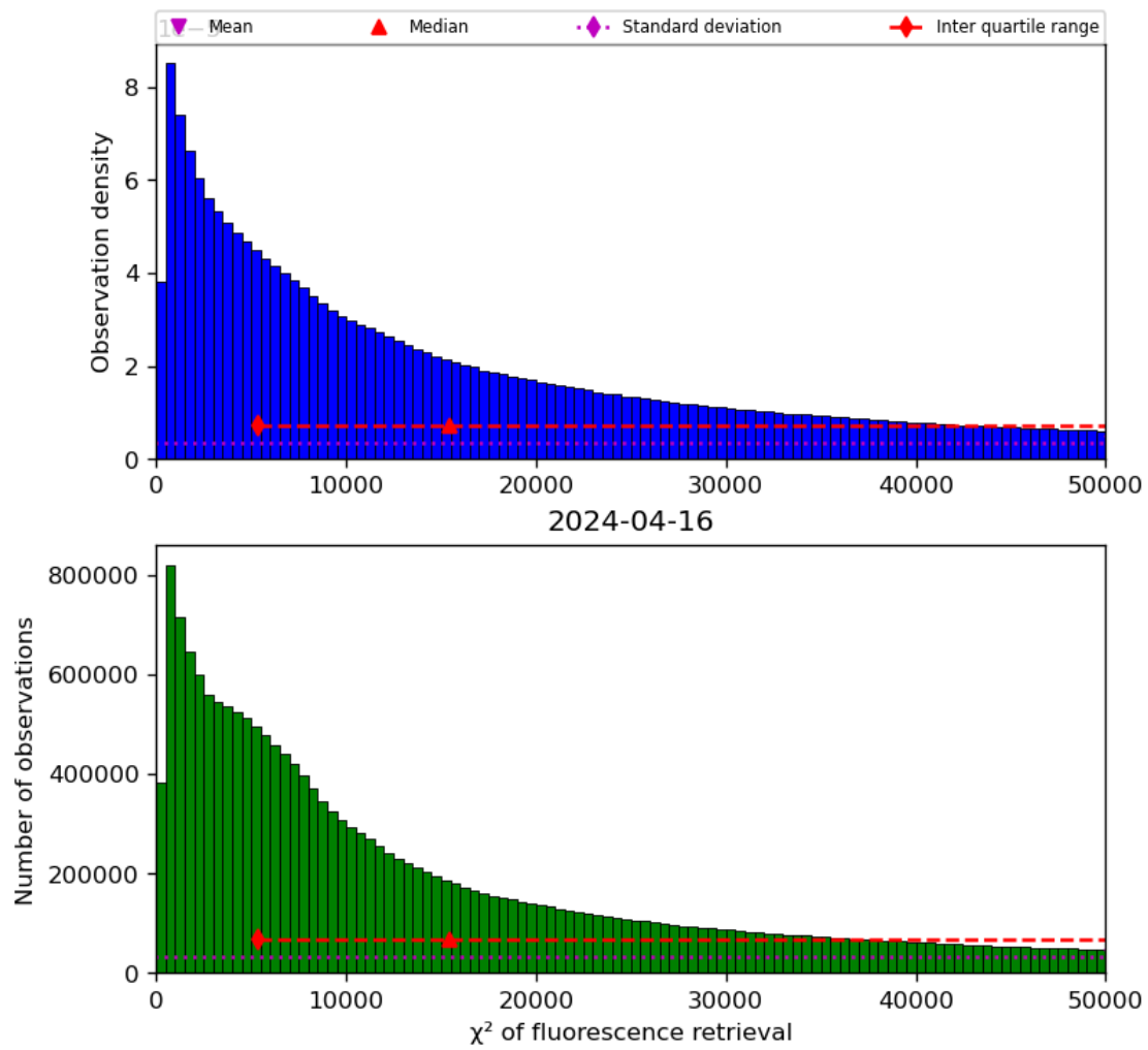
Figure 42: Histogram of “ \chi^2 of fluorescence retrieval” for 2024-04-16 to 2024-04-17
