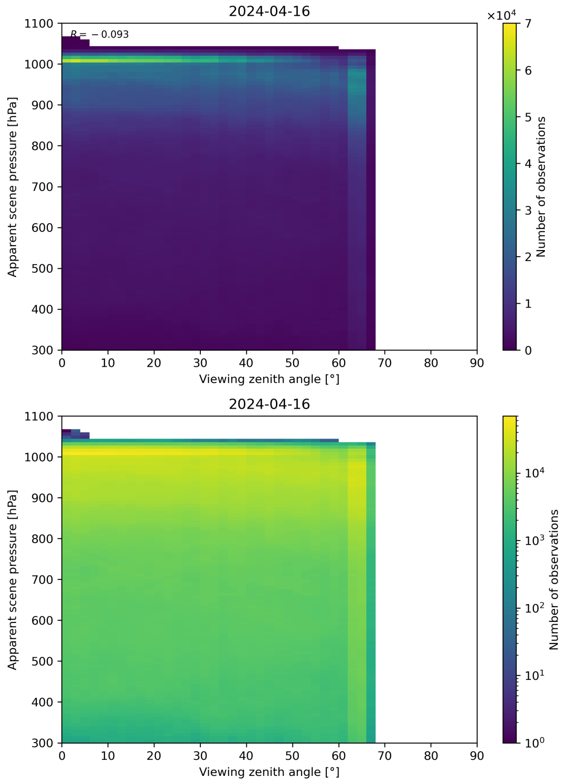
Figure 118: Scatter density plot of “Viewing zenith angle” against “Apparent scene pressure” for 2024-04-16 to 2024-04-17.
