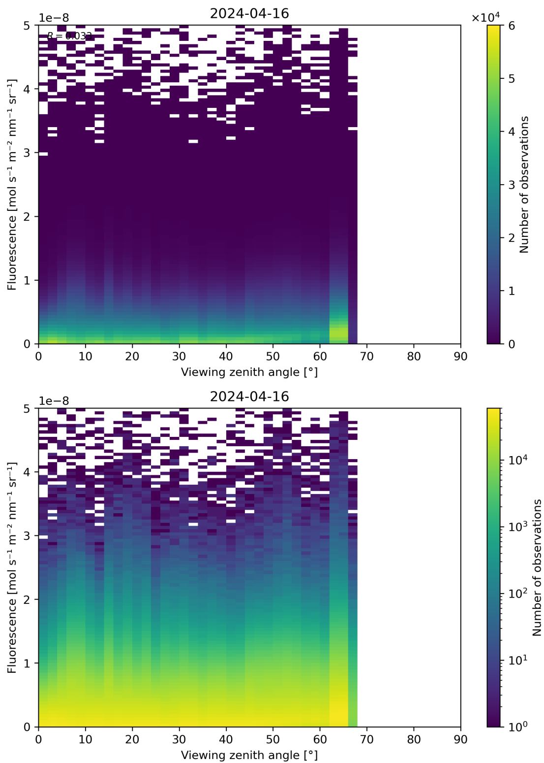
Figure 122: Scatter density plot of “Viewing zenith angle” against “Fluorescence” for 2024-04-16 to 2024-04-17.
