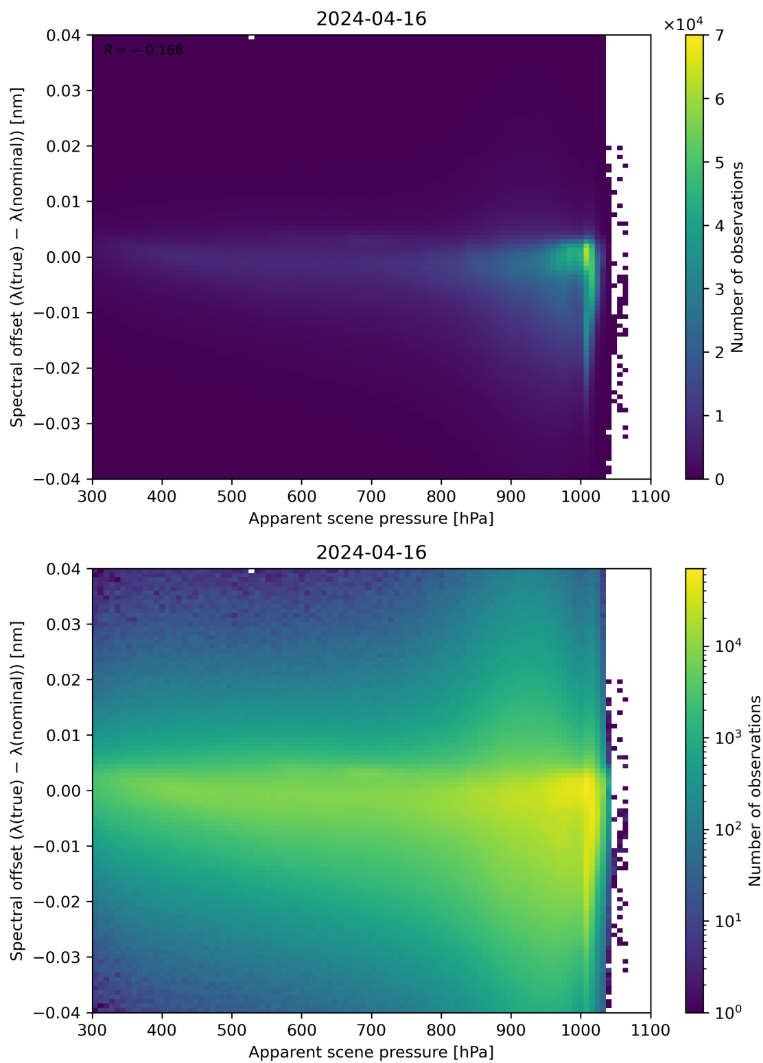
Figure 67: Scatter density plot of “Apparent scene pressure” against “Spectral offset ( \lambda(\text{true}) - \lambda(\text{nominal}) )” for 2024-04-16 to 2024-04-17.
