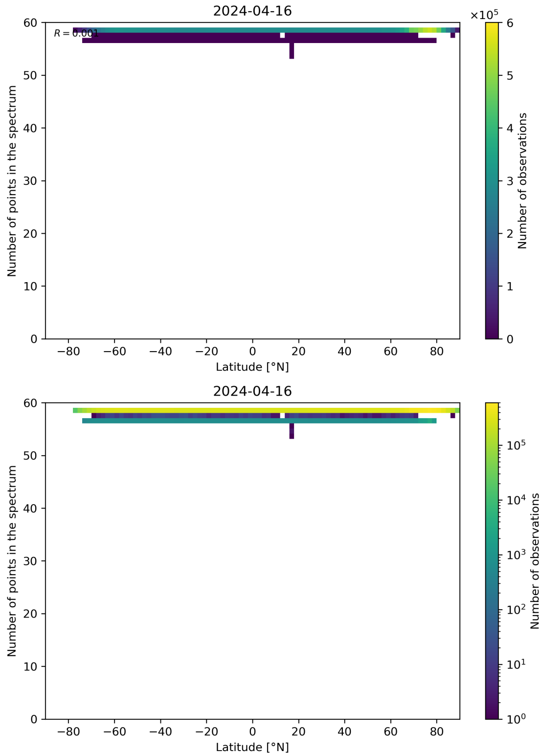
Figure 94: Scatter density plot of “Latitude” against “Number of points in the spectrum” for 2024-04-16 to 2024-04-17.
