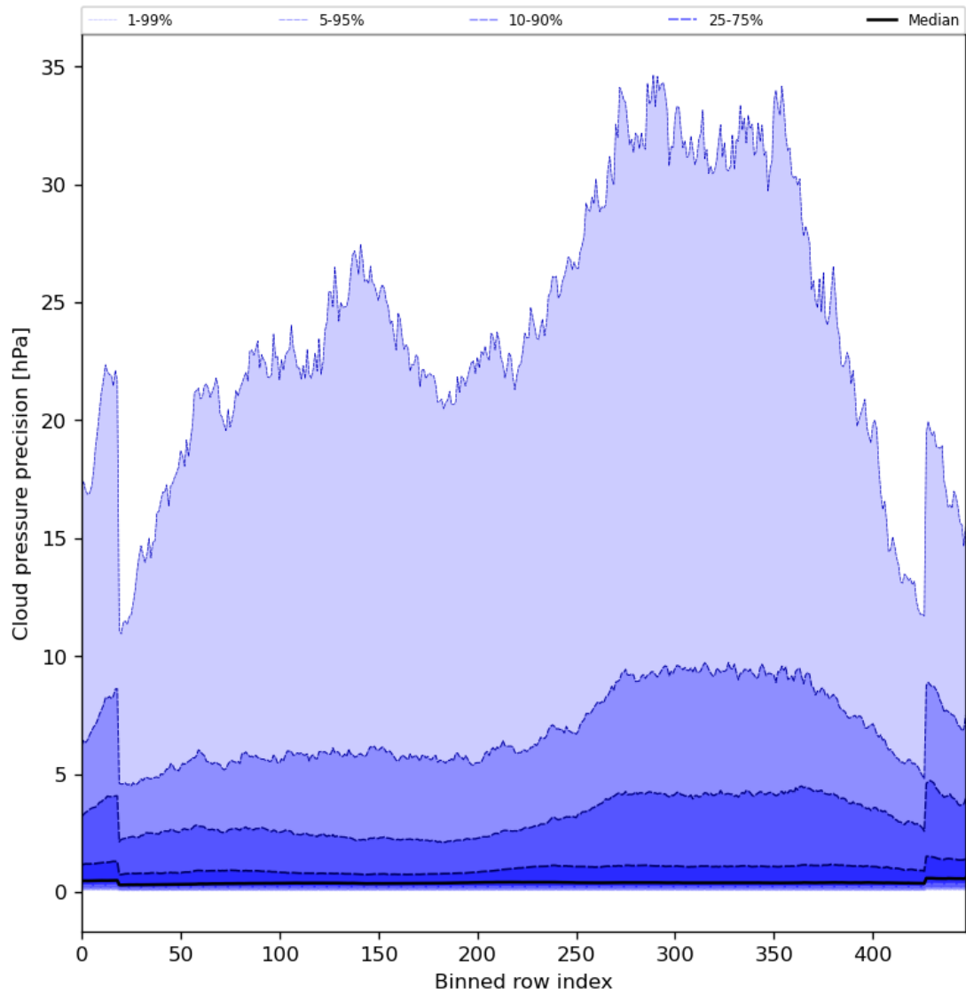
Figure 48: Along track statistics of “Cloud pressure precision” for 2024-04-16 to 2024-04-17
