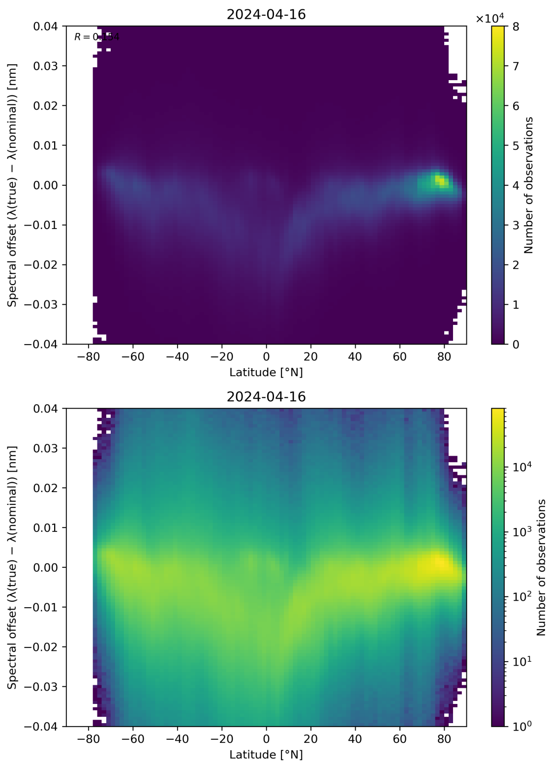
Figure 96: Scatter density plot of “Latitude” against “Spectral offset ( \lambda(\text{true}) - \lambda(\text{nominal}) )” for 2024-04-16 to 2024-04-17.
