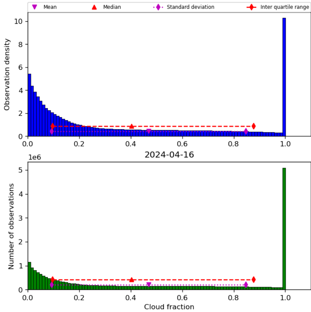
Figure 32: Histogram of “Cloud fraction” for 2024-04-16 to 2024-04-17
