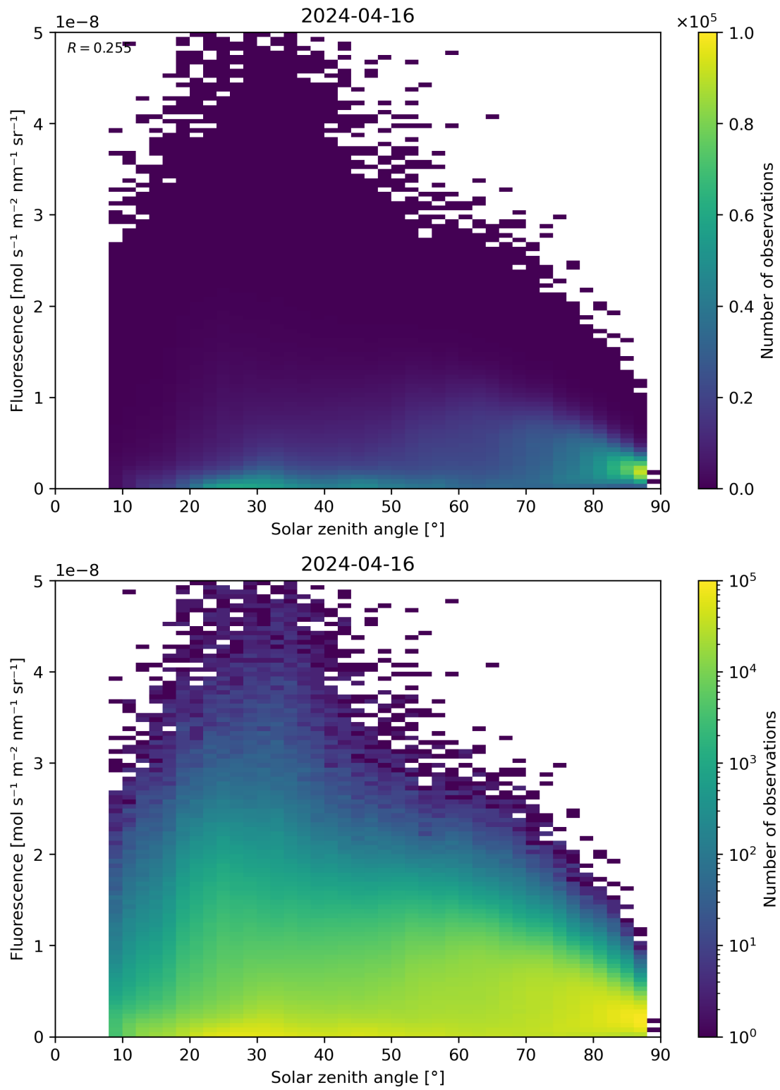
Figure 112: Scatter density plot of “Solar zenith angle” against “Fluorescence” for 2024-04-16 to 2024-04-17.
