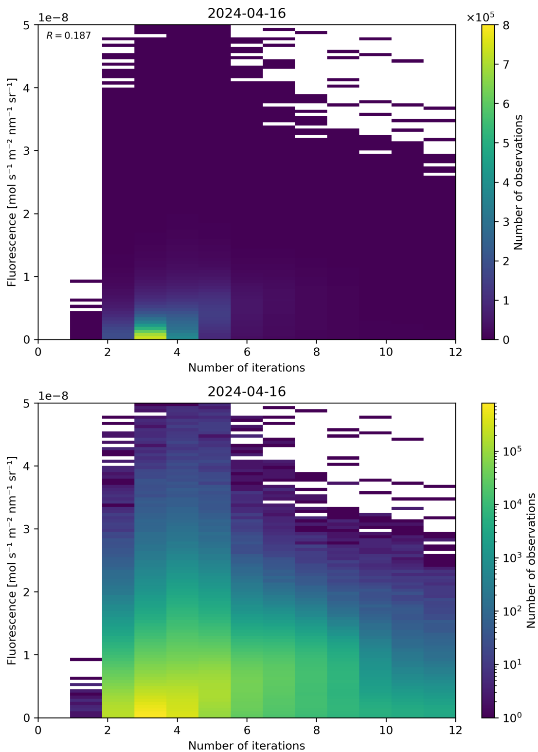
Figure 98: Scatter density plot of “Number of iterations” against “Fluorescence” for 2024-04-16 to 2024-04-17.
