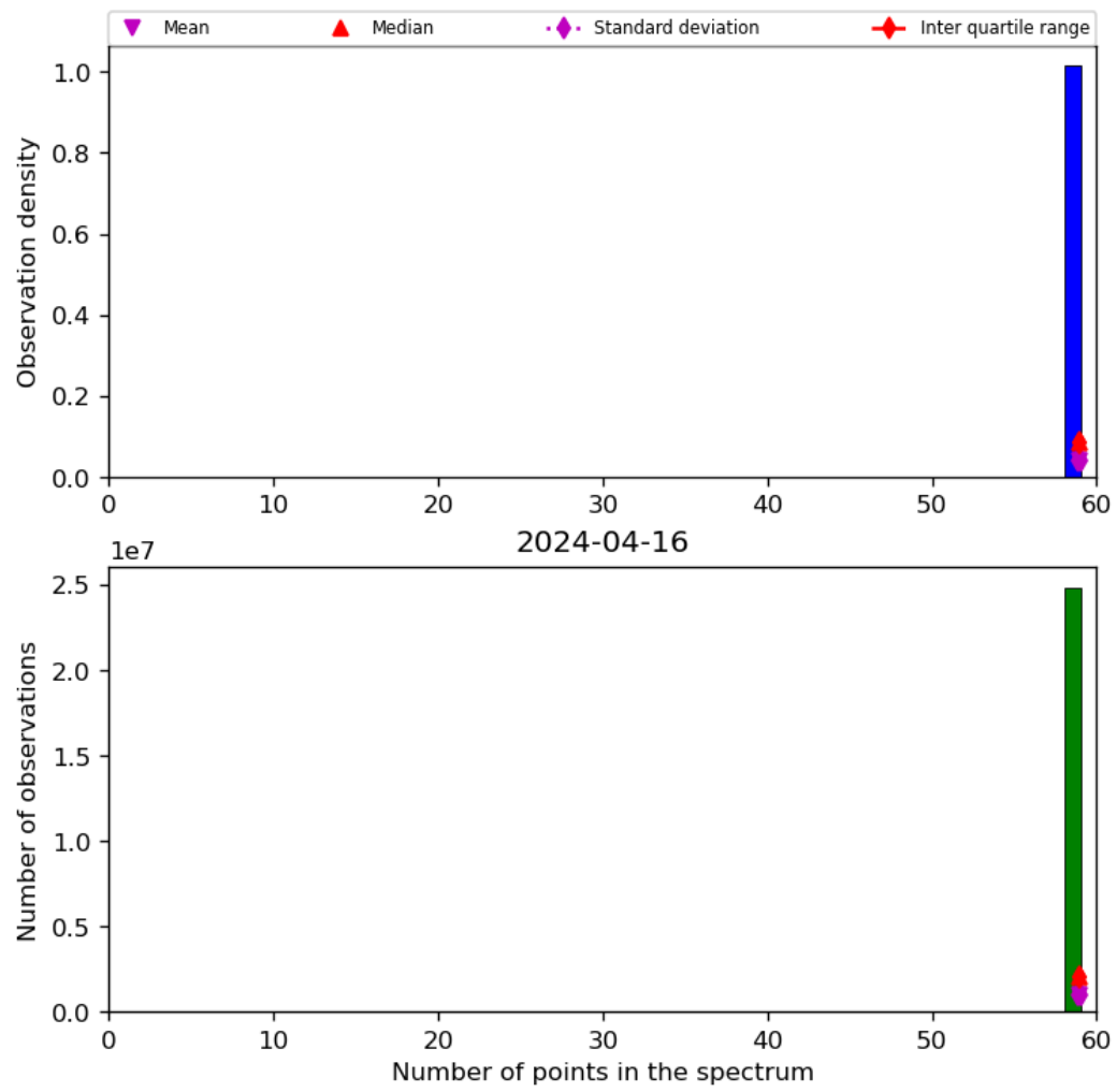
Figure 44: Histogram of “Number of points in the spectrum” for 2024-04-16 to 2024-04-17
