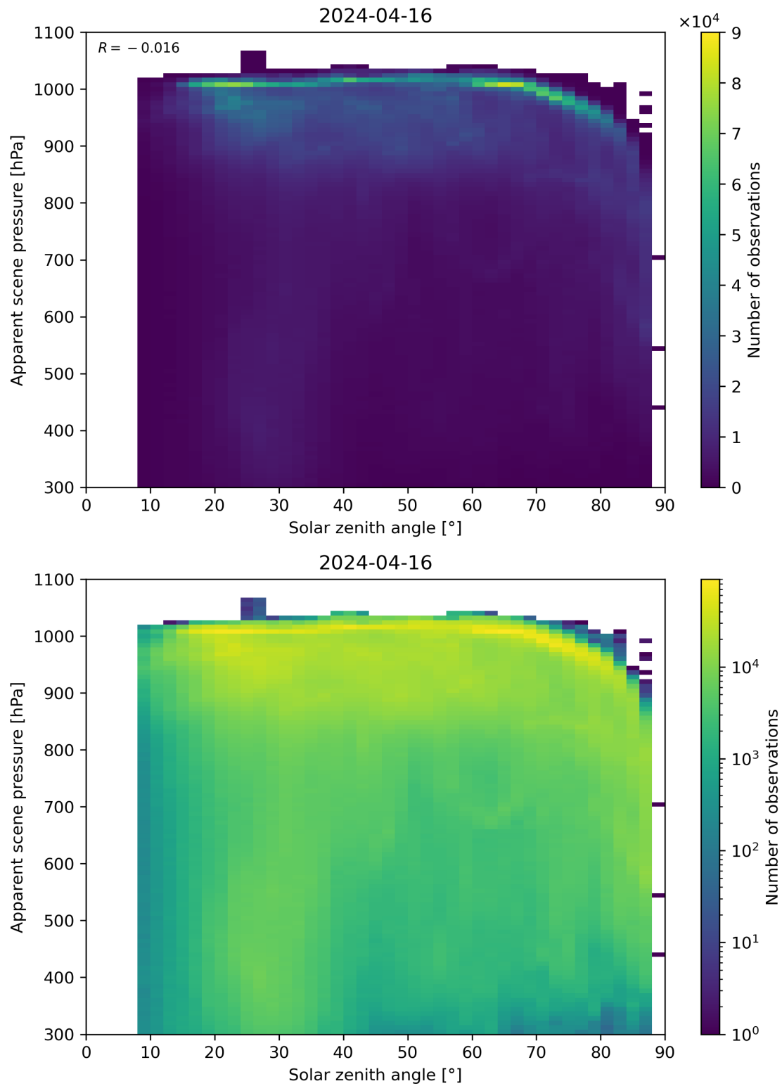
Figure 108: Scatter density plot of “Solar zenith angle” against “Apparent scene pressure” for 2024-04-16 to 2024-04-17.
