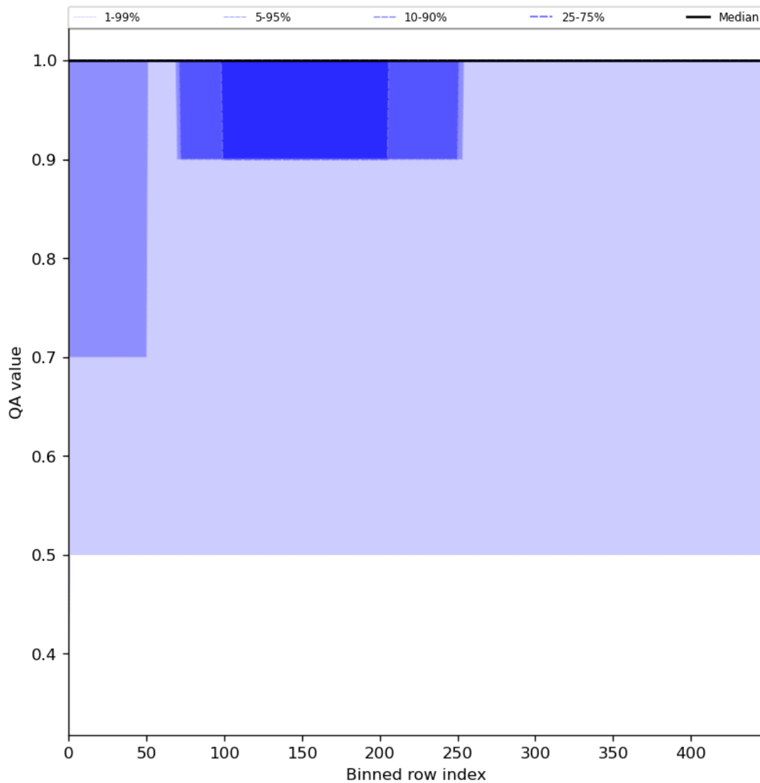
Figure 46: Along track statistics of “QA value” for 2024-04-16 to 2024-04-17
