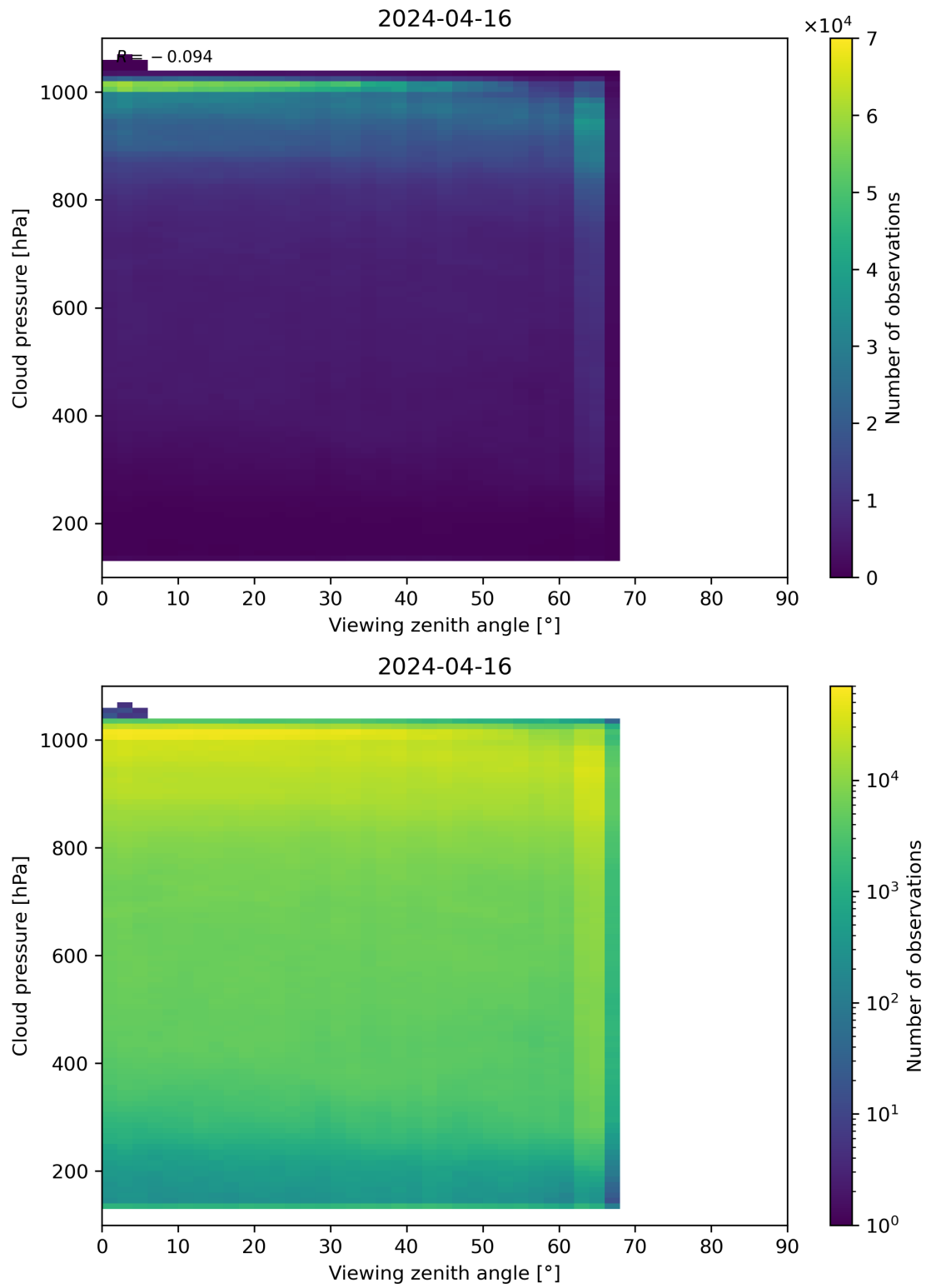
Figure 121: Scatter density plot of “Viewing zenith angle” against “Cloud pressure” for 2024-04-16 to 2024-04-17.
