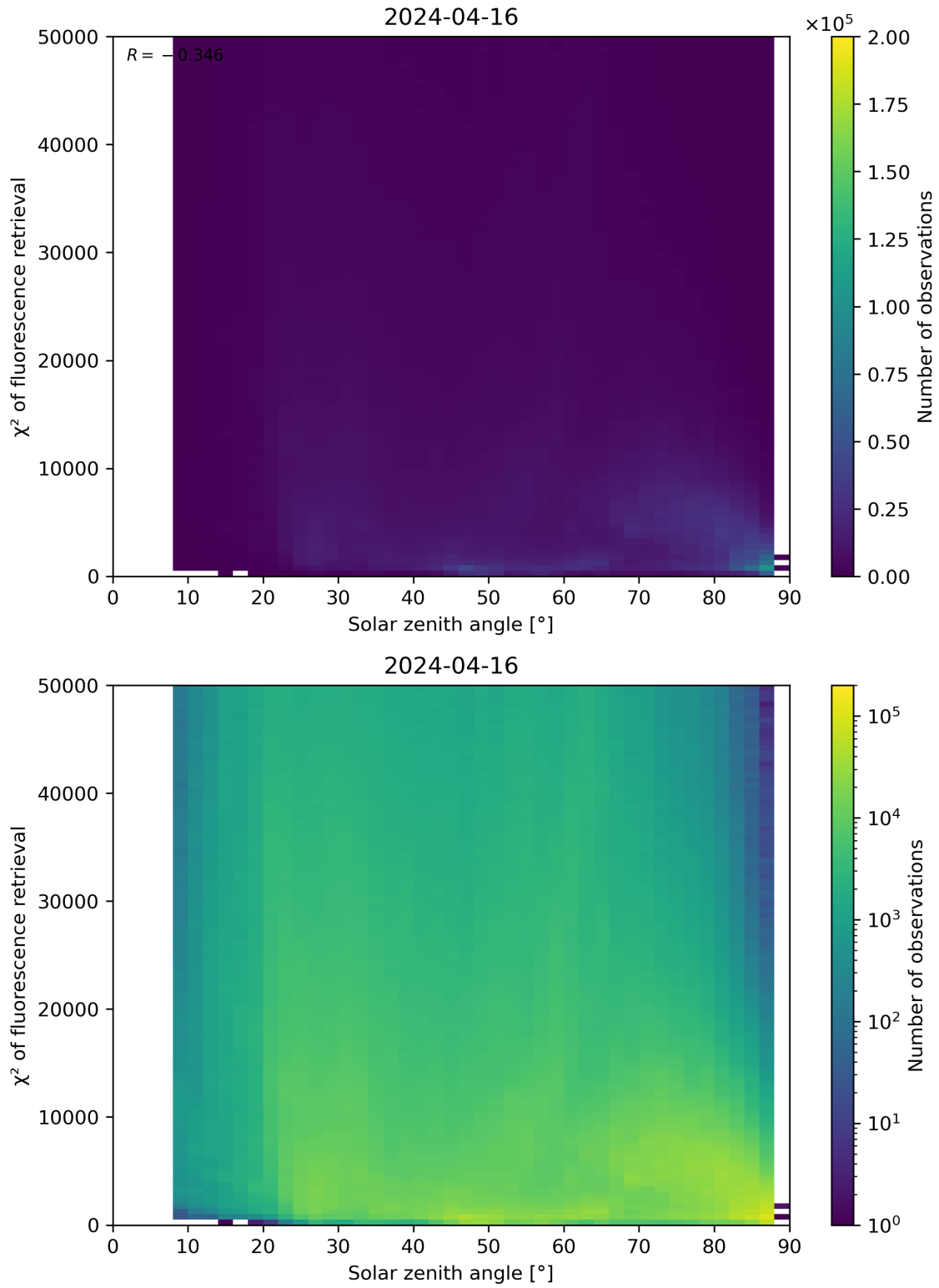
Figure 109: Scatter density plot of “Solar zenith angle” against “ \chi^2 of fluorescence retrieval” for 2024-04-16 to 2024-04-17.
