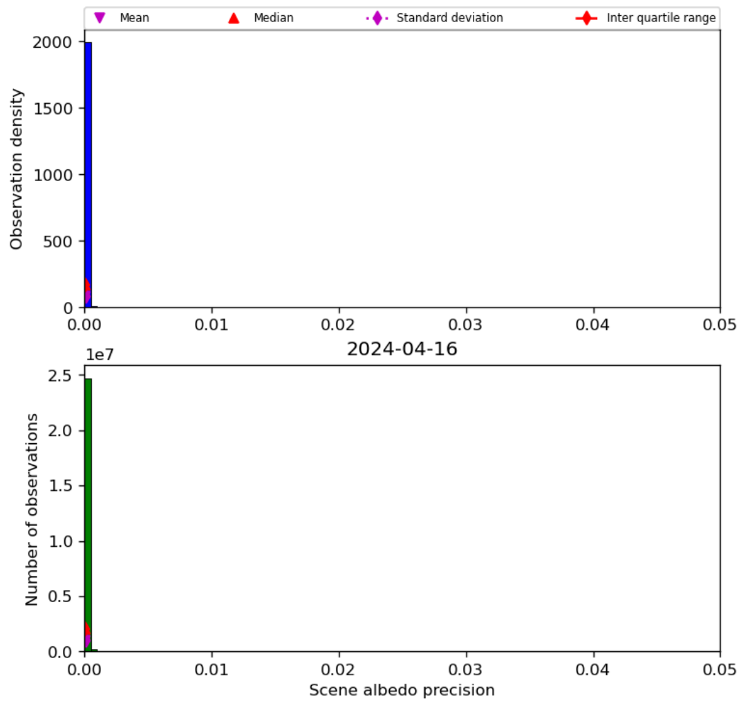
Figure 35: Histogram of “Scene albedo precision” for 2024-04-16 to 2024-04-17
