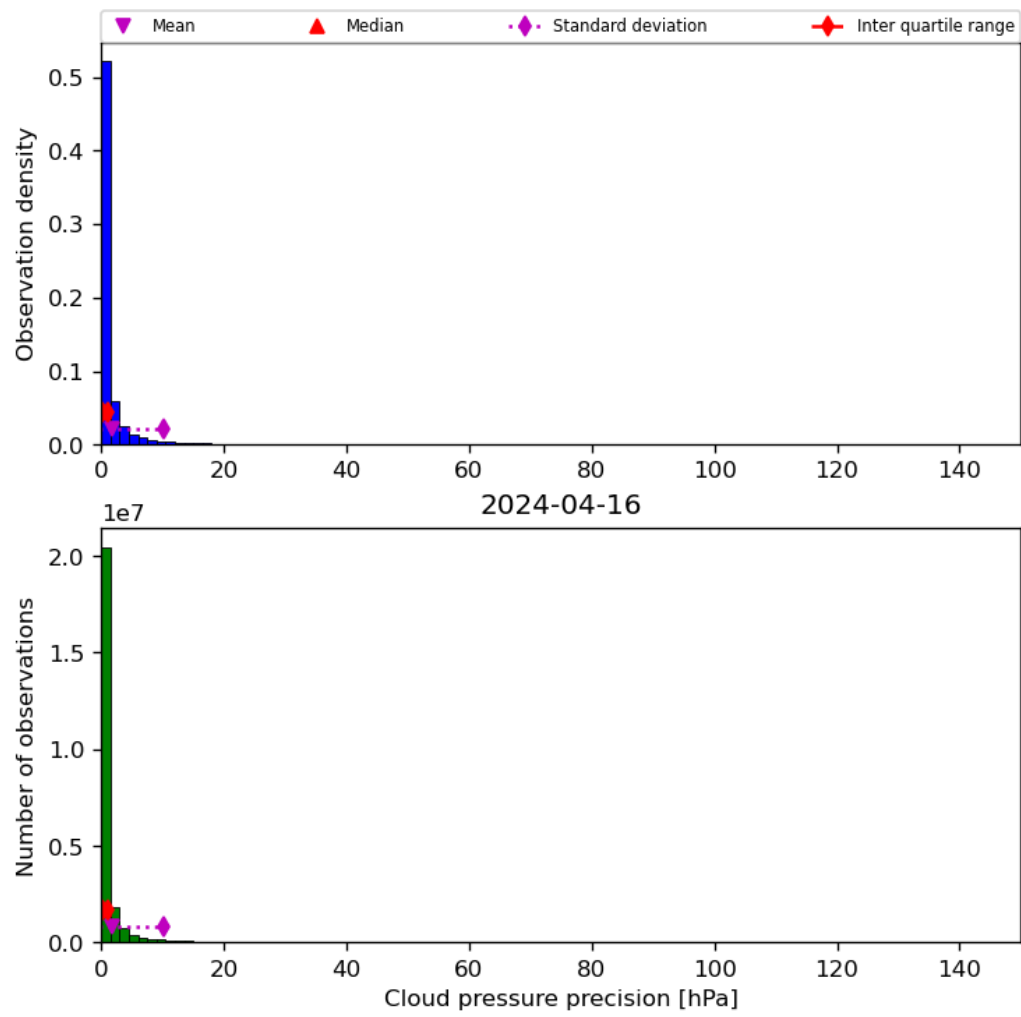
Figure 31: Histogram of “Cloud pressure precision” for 2024-04-16 to 2024-04-17
