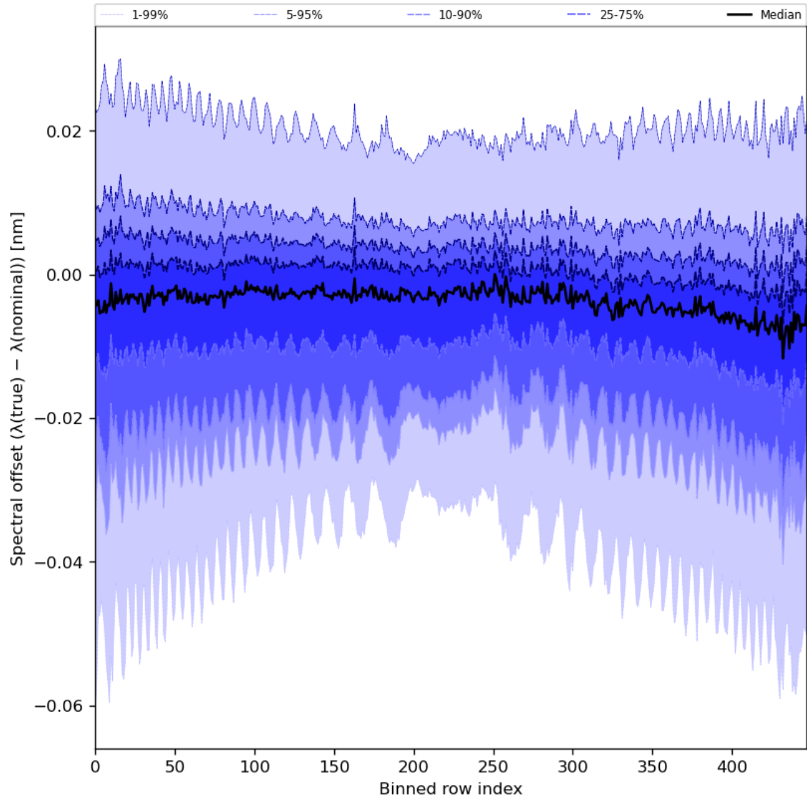
Figure 62: Along track statistics of “Spectral offset ( \lambda(\text{true}) - \lambda(\text{nominal}) )” for 2024-04-16 to 2024-04-17
