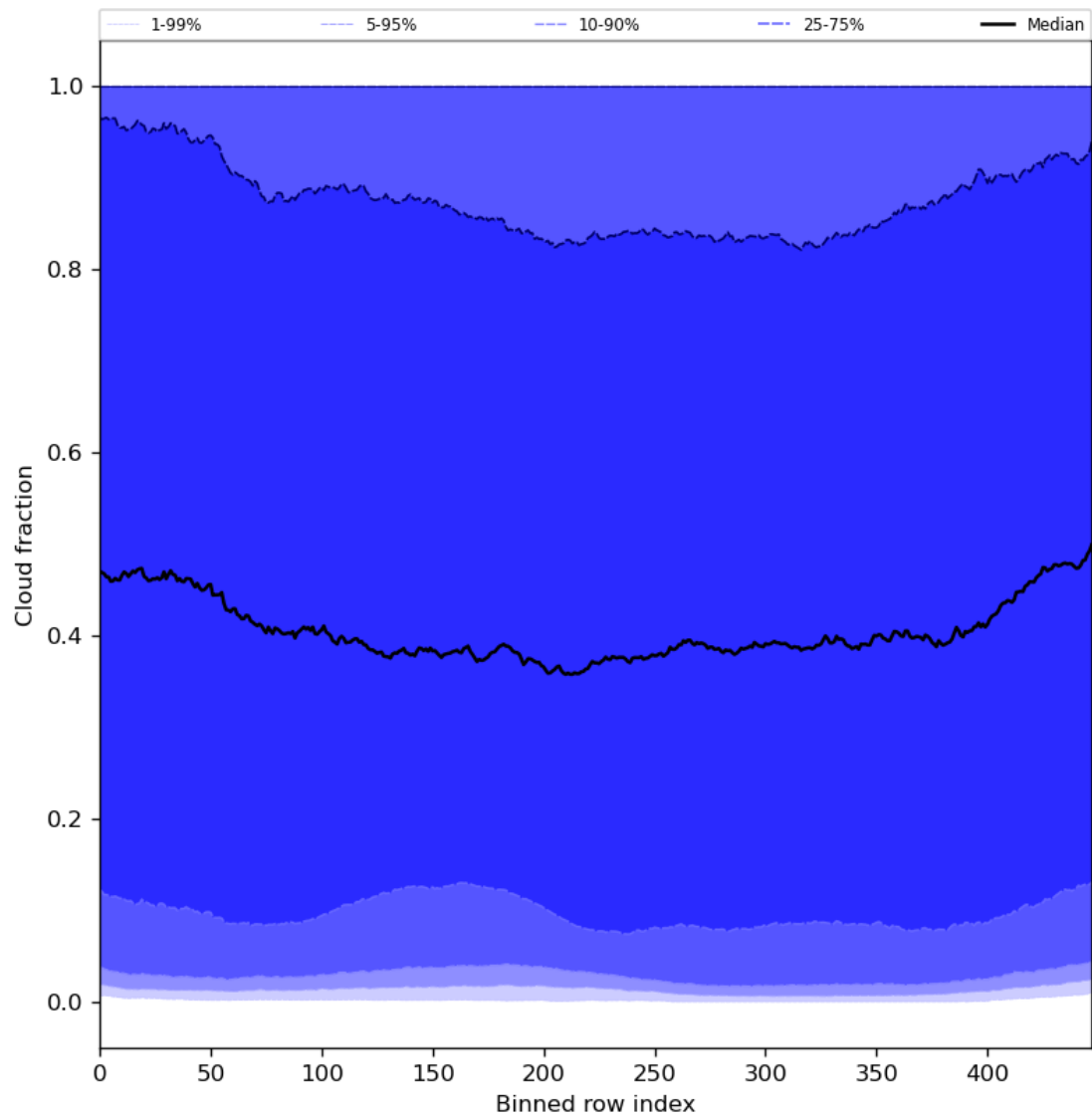
Figure 49: Along track statistics of “Cloud fraction” for 2024-04-16 to 2024-04-17
