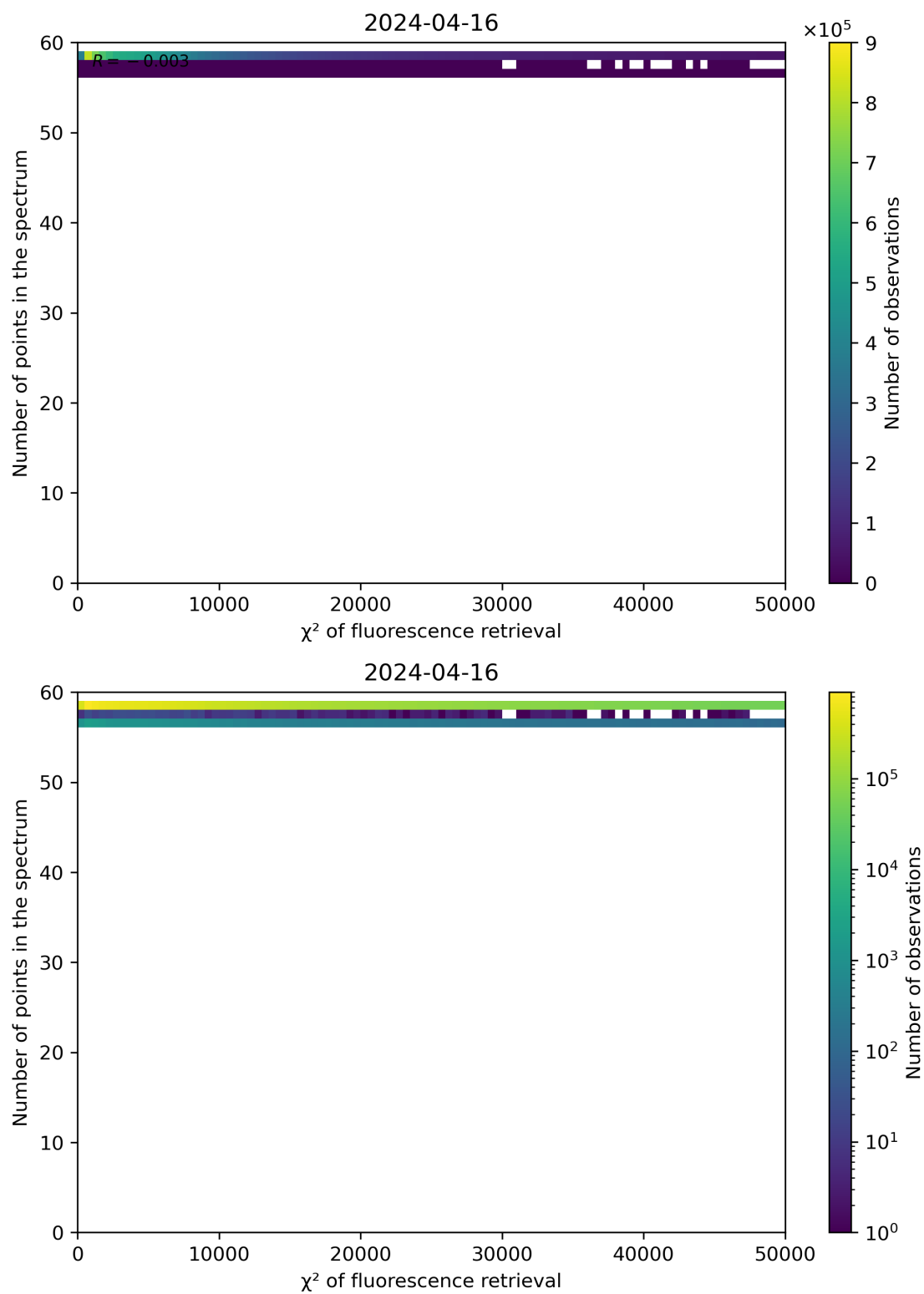
Figure 68: Scatter density plot of “ \chi^2 of fluorescence retrieval” against “Number of points in the spectrum” for 2024-04-16 to 2024-04-17.
