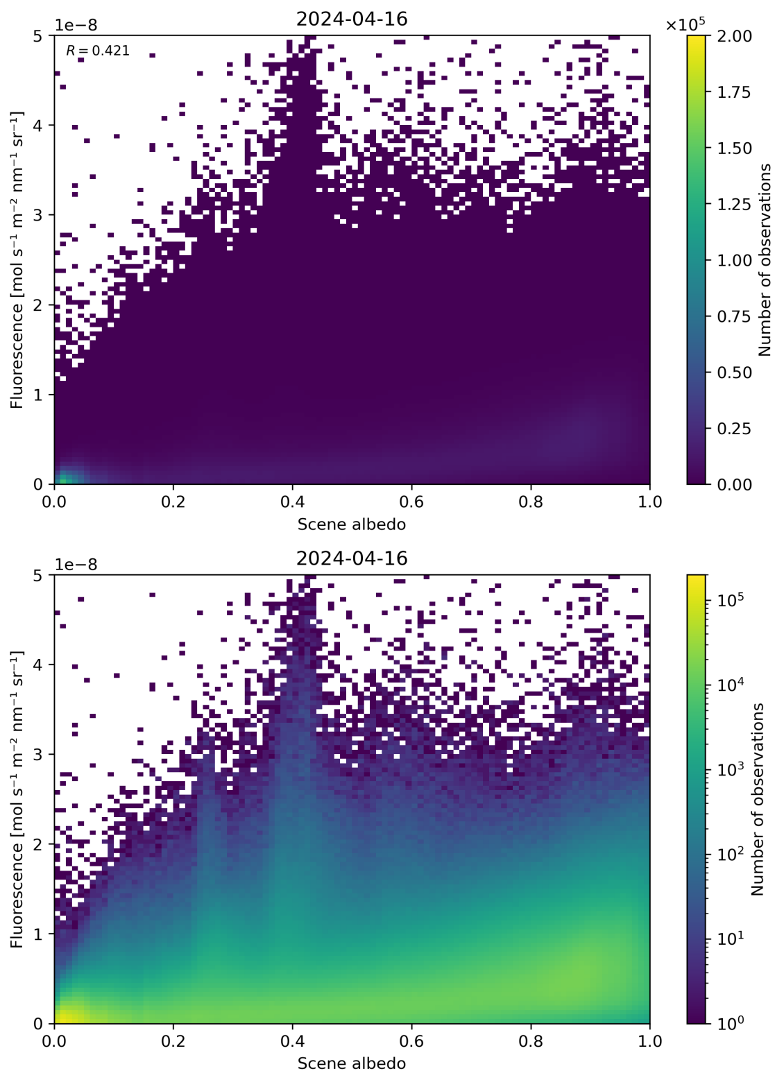
Figure 104: Scatter density plot of “Scene albedo” against “Fluorescence” for 2024-04-16 to 2024-04-17.
