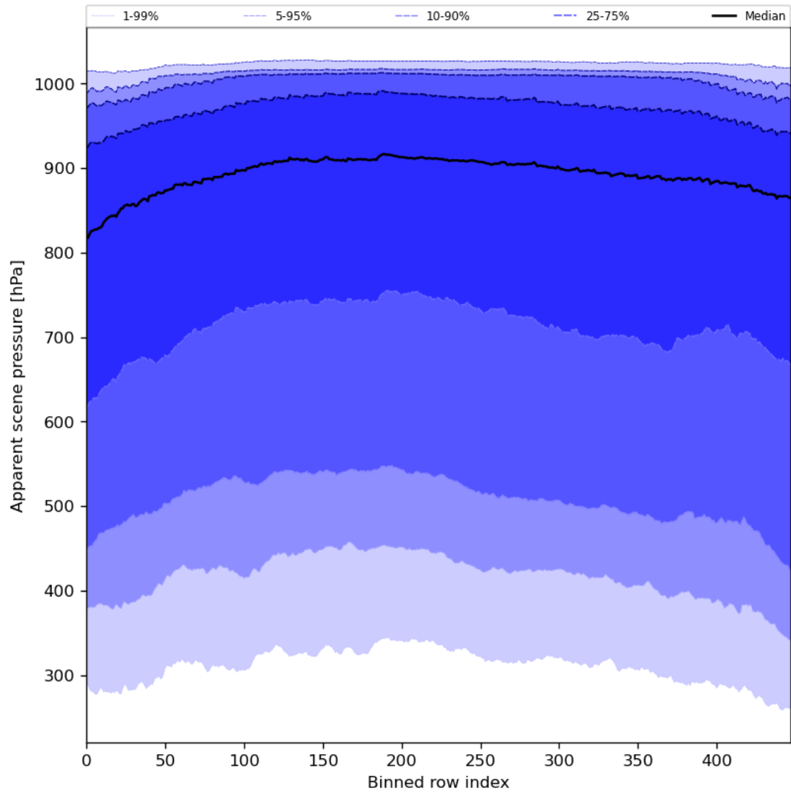
Figure 53: Along track statistics of “Apparent scene pressure” for 2024-04-16 to 2024-04-17
