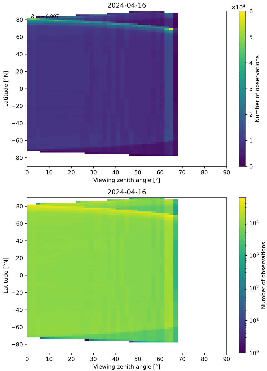
Figure 123: Scatter density plot of “Viewing zenith angle” against “Latitude” for 2024-04-16 to 2024-04-17.
