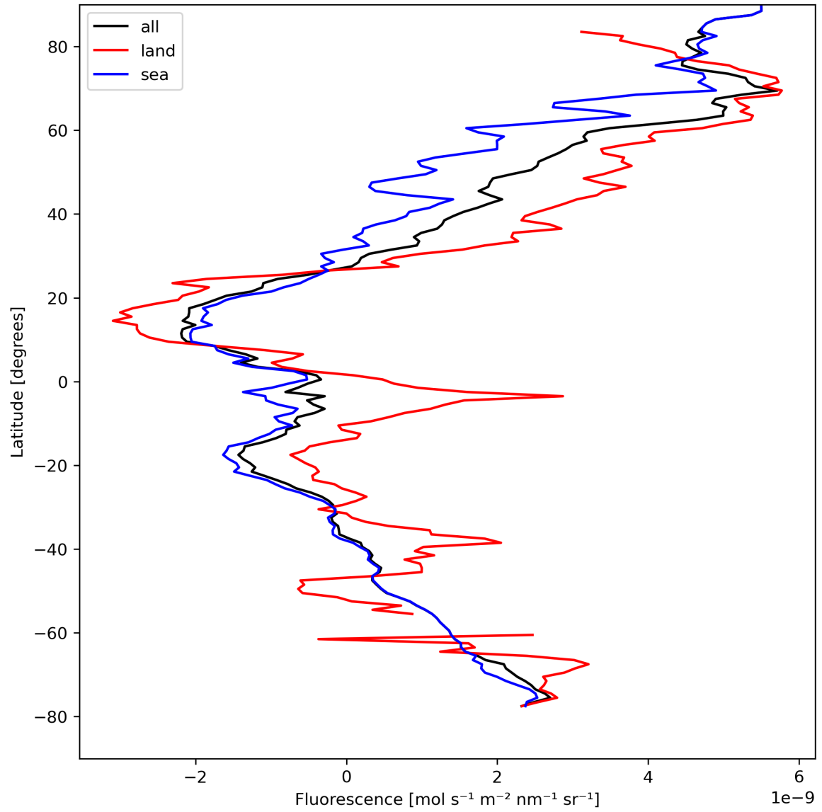
Figure 23: Zonal average of “Fluorescence” for 2024-04-16 to 2024-04-17.
