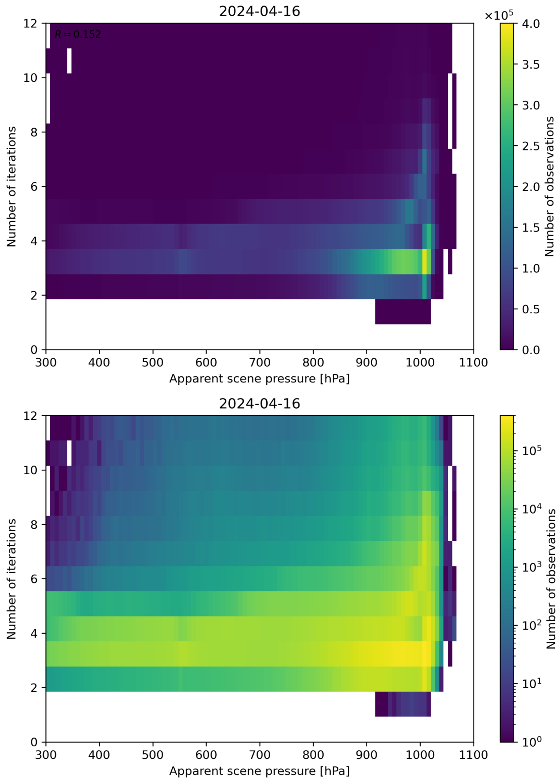
Figure 65: Scatter density plot of “Apparent scene pressure” against “Number of iterations” for 2024-04-16 to 2024-04-17.
