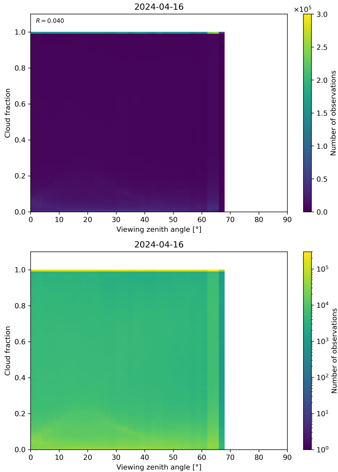
Figure 120: Scatter density plot of “Viewing zenith angle” against “Cloud fraction” for 2024-04-16 to 2024-04-17.
