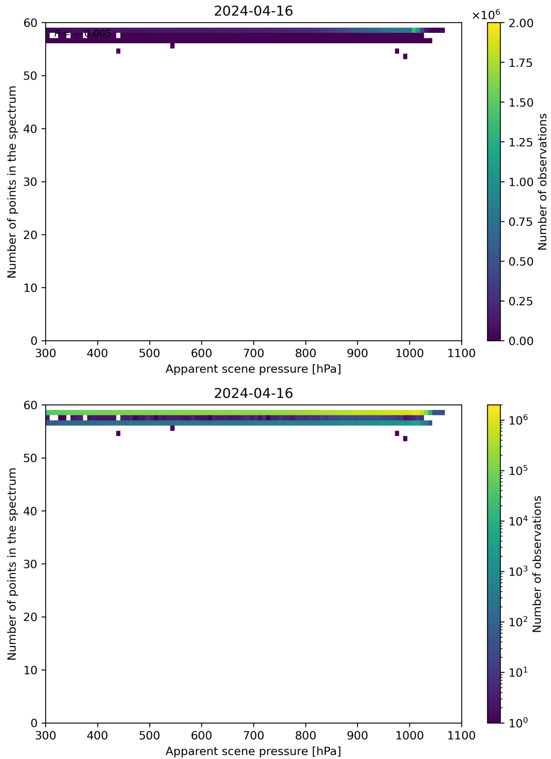
Figure 66: Scatter density plot of “Apparent scene pressure” against “Number of points in the spectrum” for 2024-04-16 to 2024-04-17.
