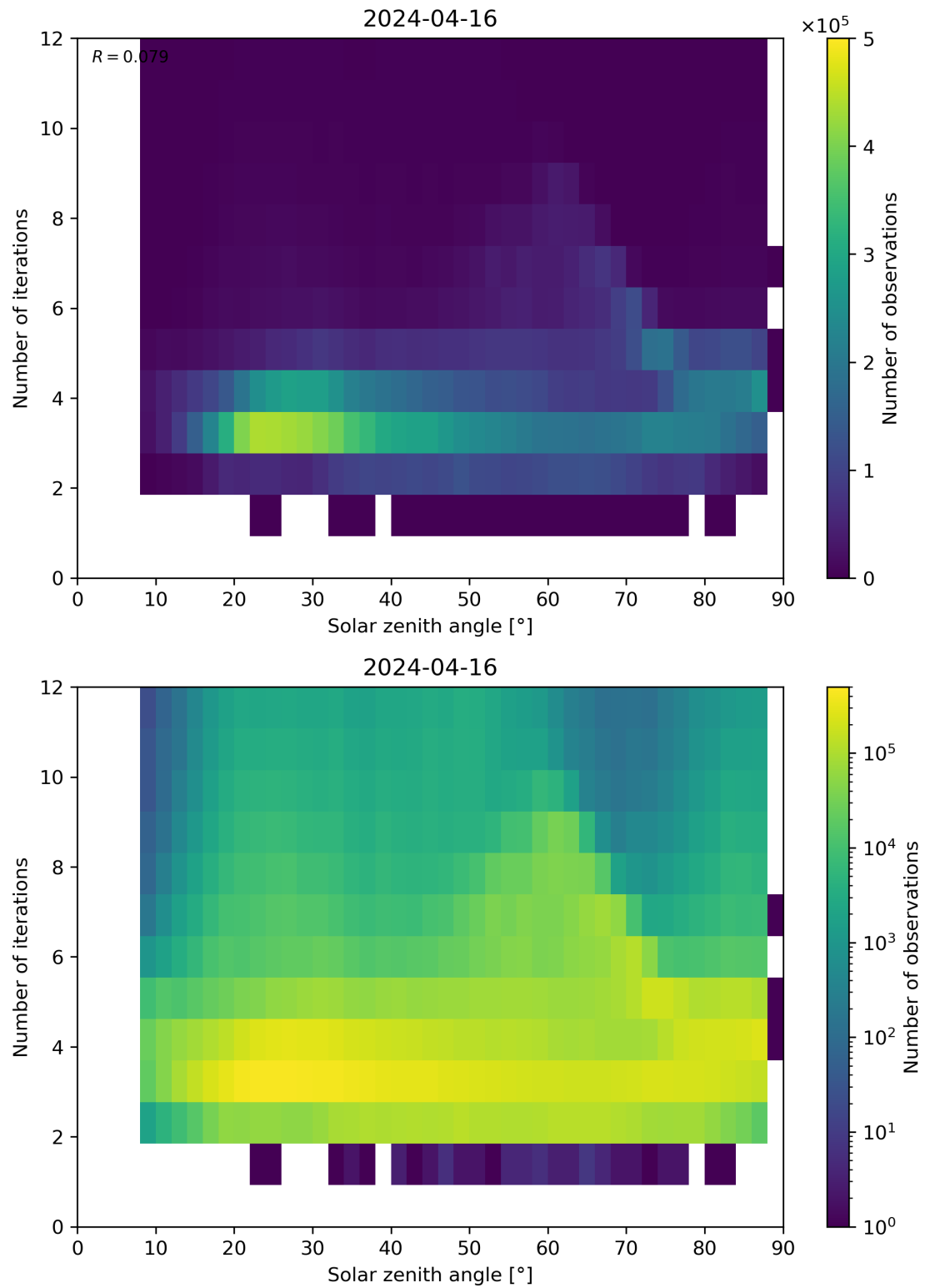
Figure 114: Scatter density plot of “Solar zenith angle” against “Number of iterations” for 2024-04-16 to 2024-04-17.
