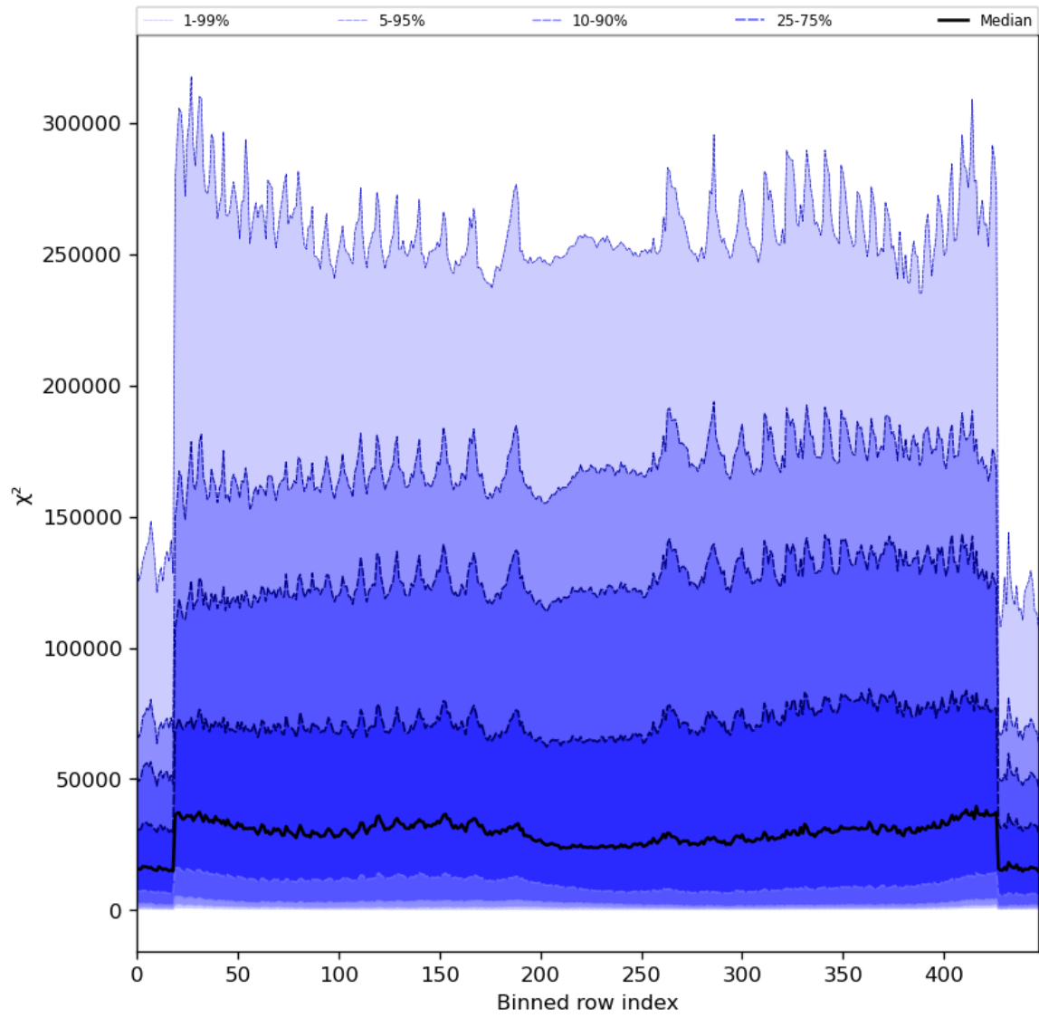
Figure 55: Along track statistics of “ \chi^2 ” for 2024-04-16 to 2024-04-17
