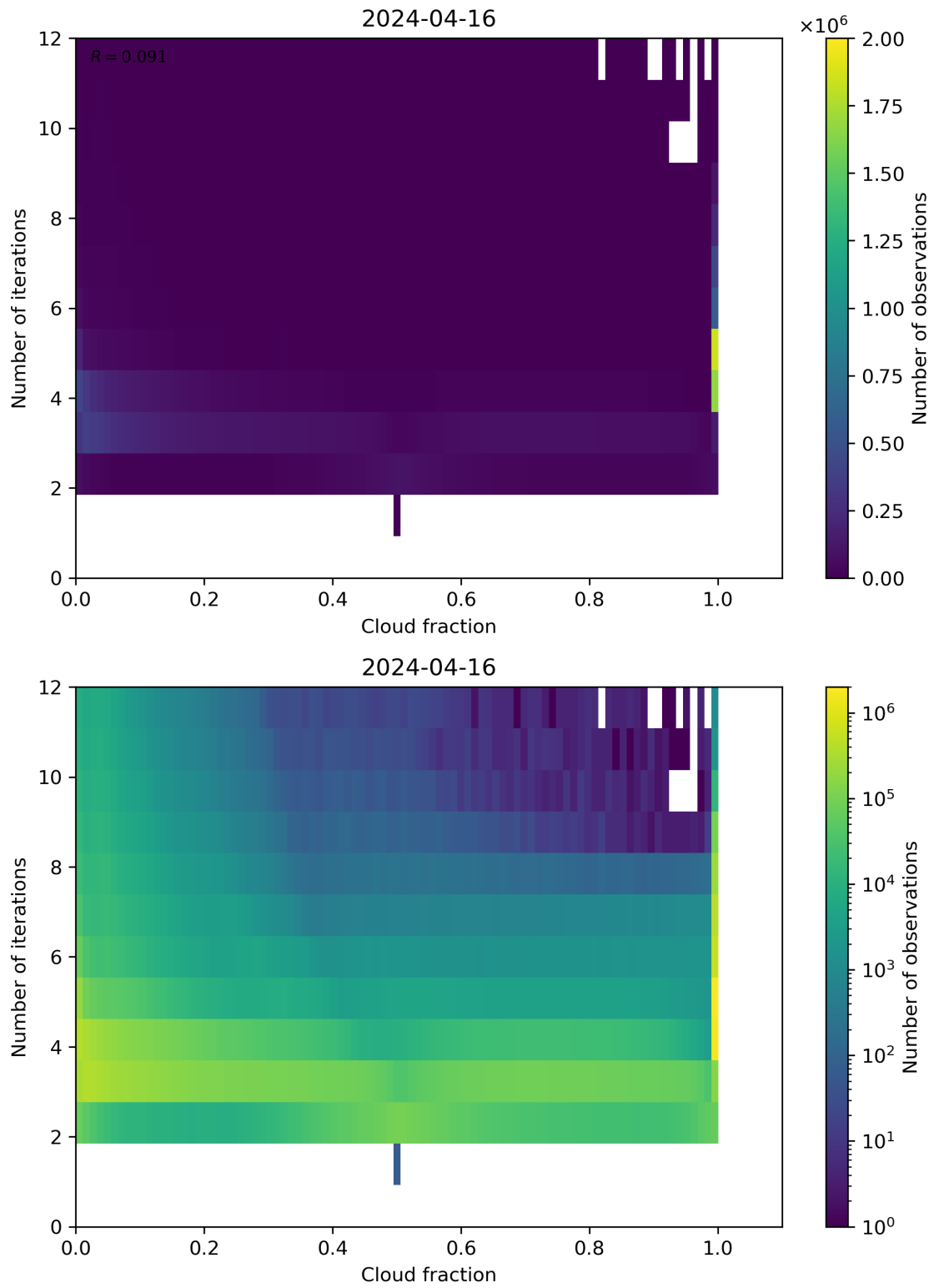
Figure 73: Scatter density plot of “Cloud fraction” against “Number of iterations” for 2024-04-16 to 2024-04-17.
