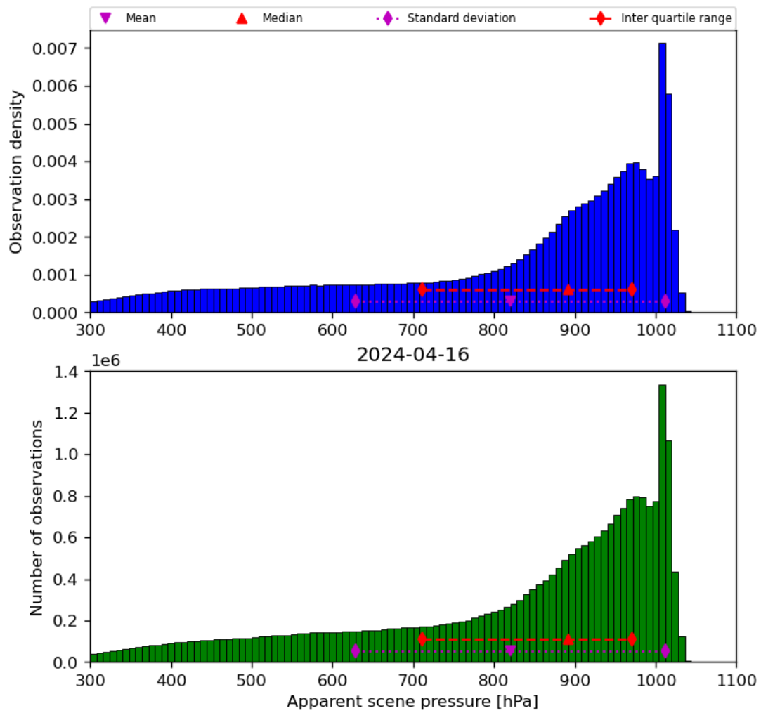
Figure 36: Histogram of “Apparent scene pressure” for 2024-04-16 to 2024-04-17
