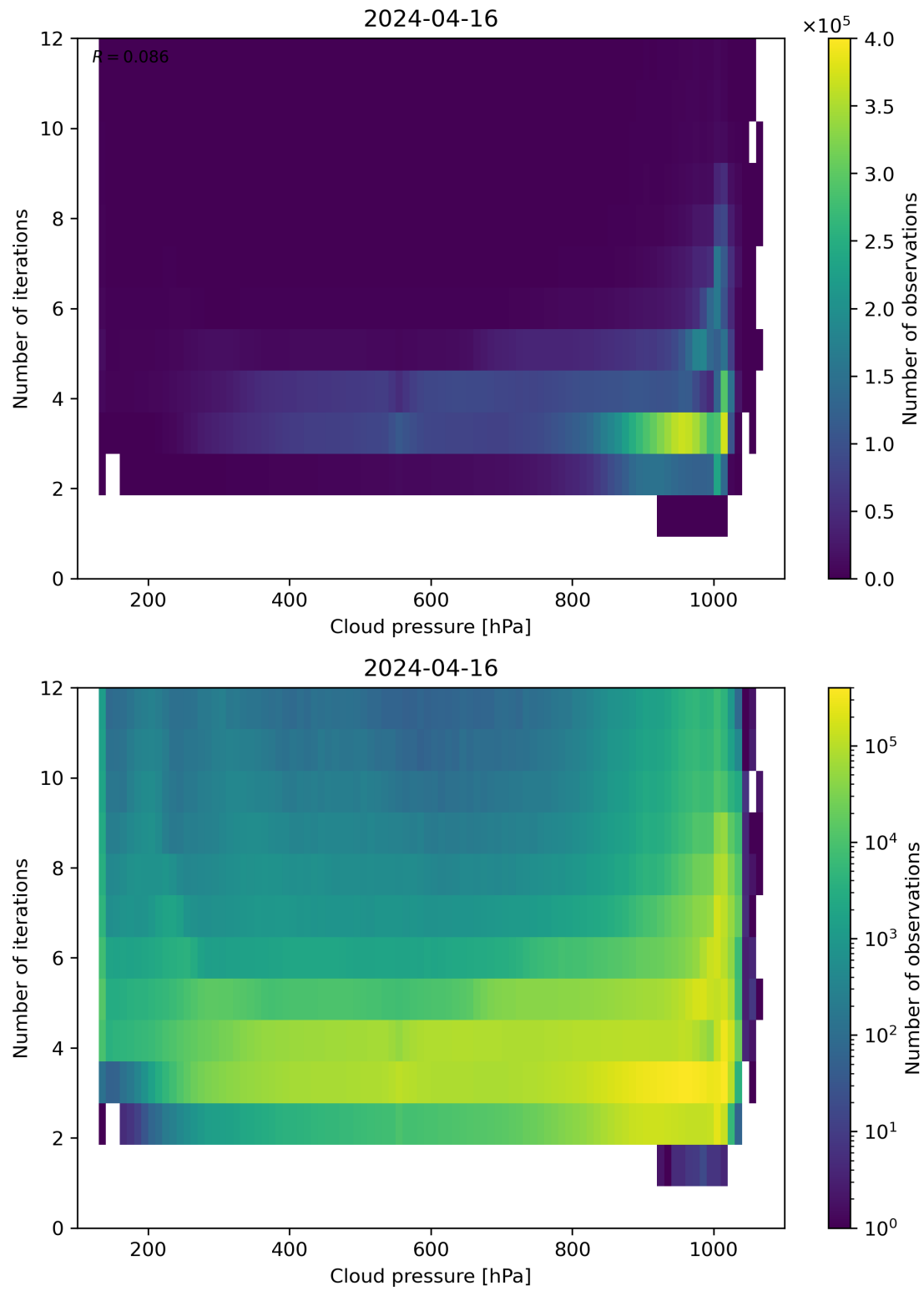
Figure 81: Scatter density plot of “Cloud pressure” against “Number of iterations” for 2024-04-16 to 2024-04-17.
