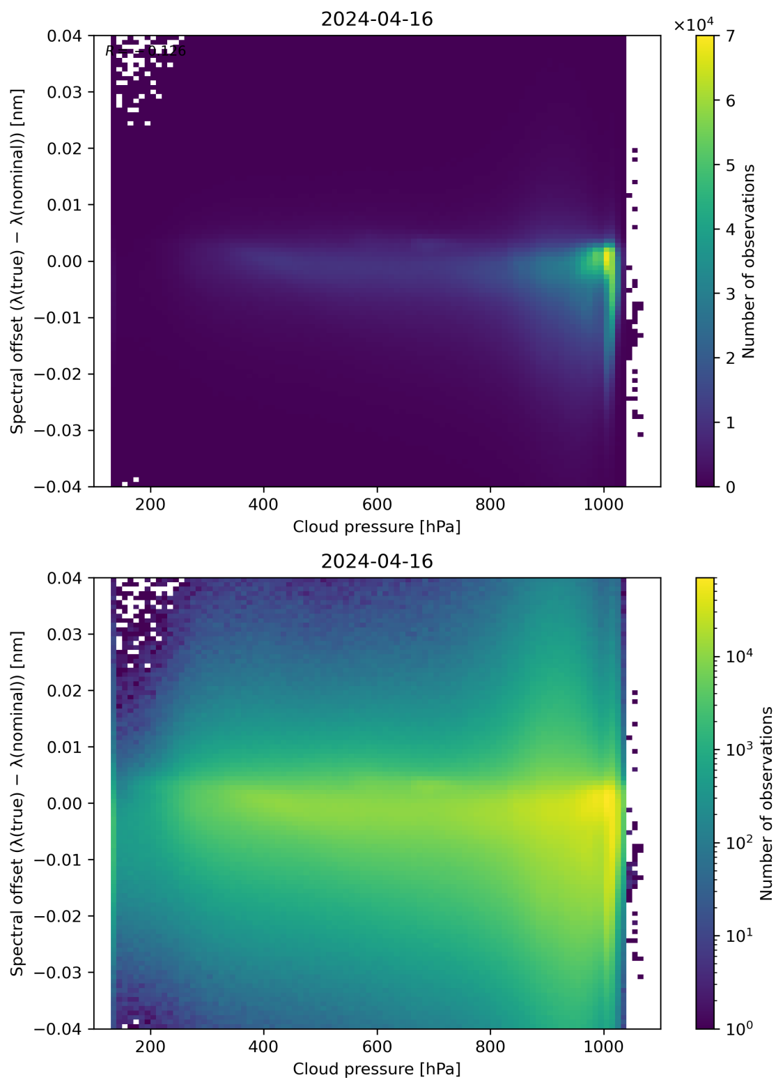
Figure 84: Scatter density plot of “Cloud pressure” against “Spectral offset ( \lambda(\text{true}) - \lambda(\text{nominal}) )” for 2024-04-16 to 2024-04-17.
