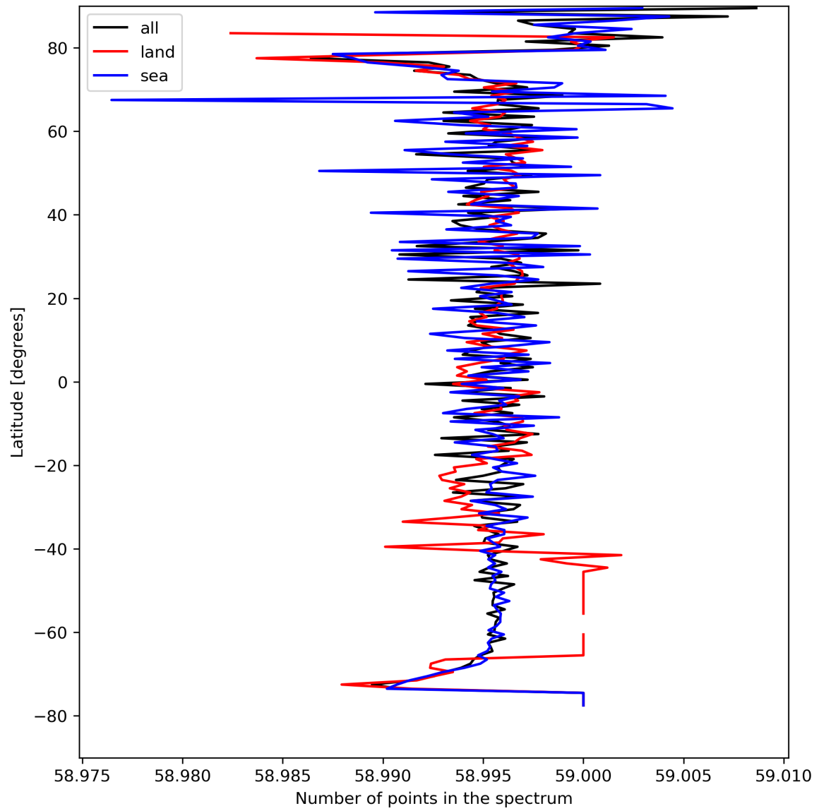
Figure 27: Zonal average of “Number of points in the spectrum” for 2024-04-16 to 2024-04-17.
