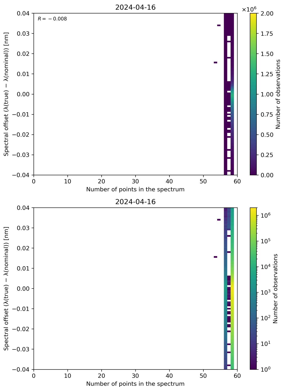
Figure 101: Scatter density plot of “Number of points in the spectrum” against “Spectral offset ( \lambda(\text{true}) - \lambda(\text{nominal}) )” for 2024-04-16 to 2024-04-17.
