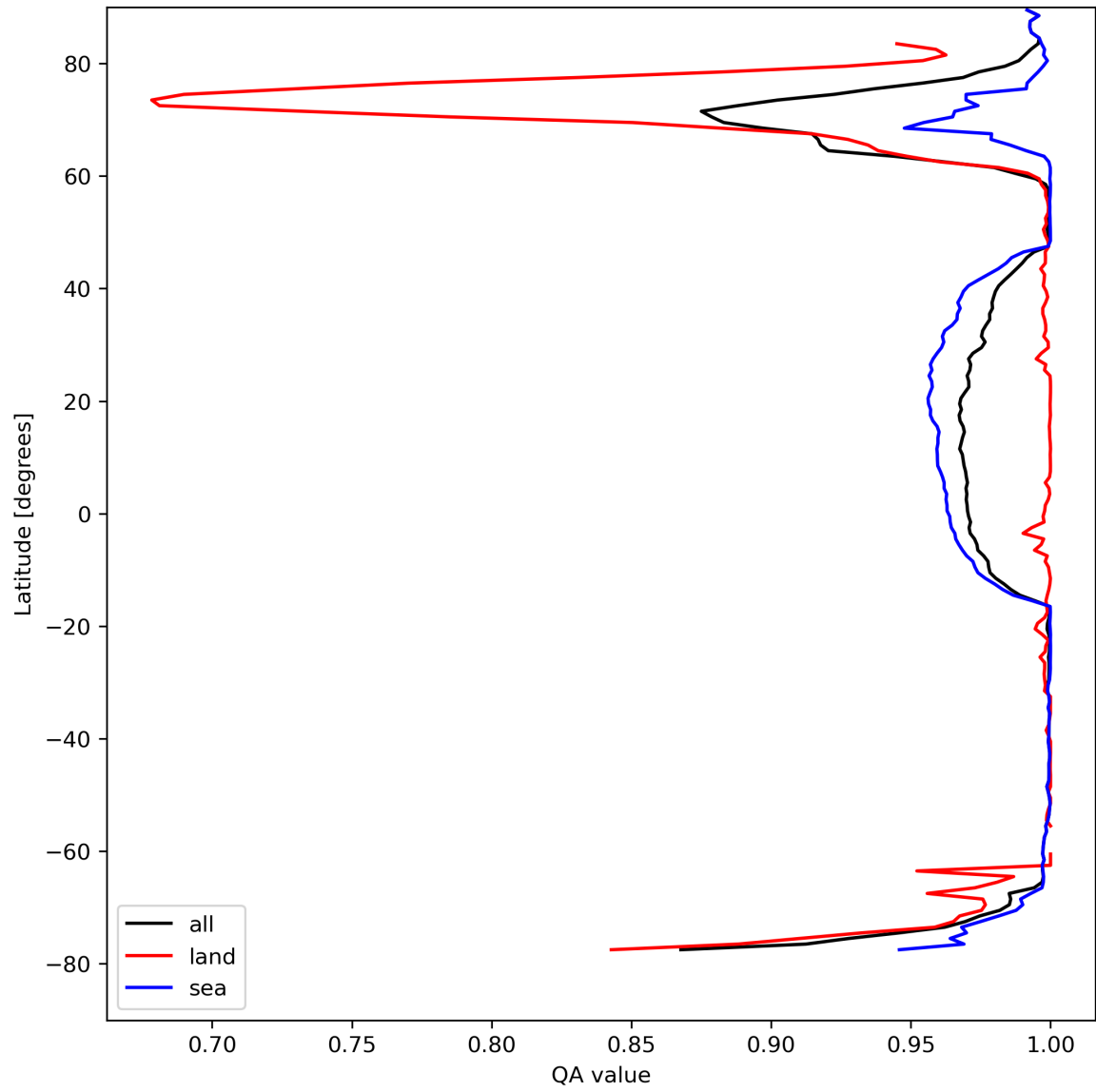
Figure 12: Zonal average of “QA value” for 2024-04-16 to 2024-04-17.
