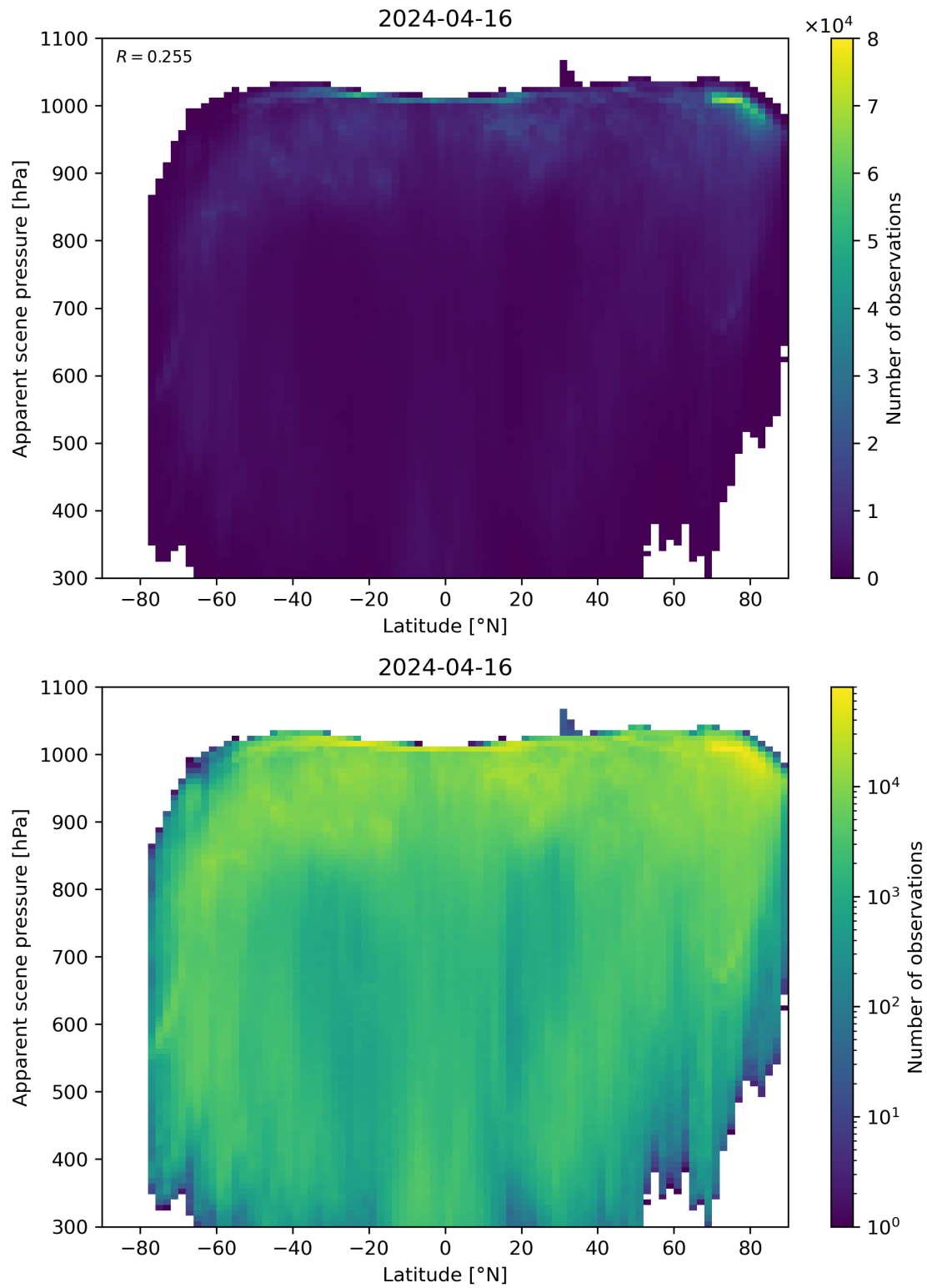
Figure 88: Scatter density plot of “Latitude” against “Apparent scene pressure” for 2024-04-16 to 2024-04-17.
