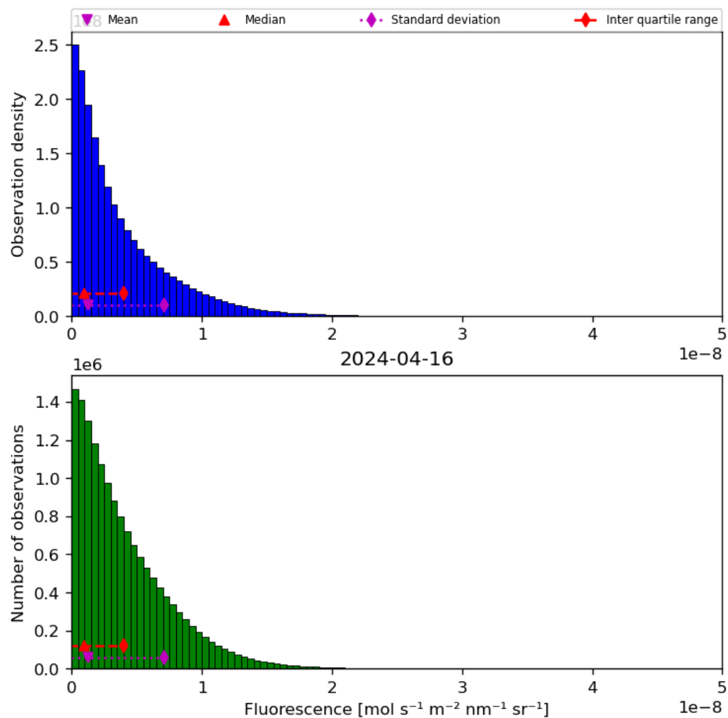
Figure 40: Histogram of “Fluorescence” for 2024-04-16 to 2024-04-17
