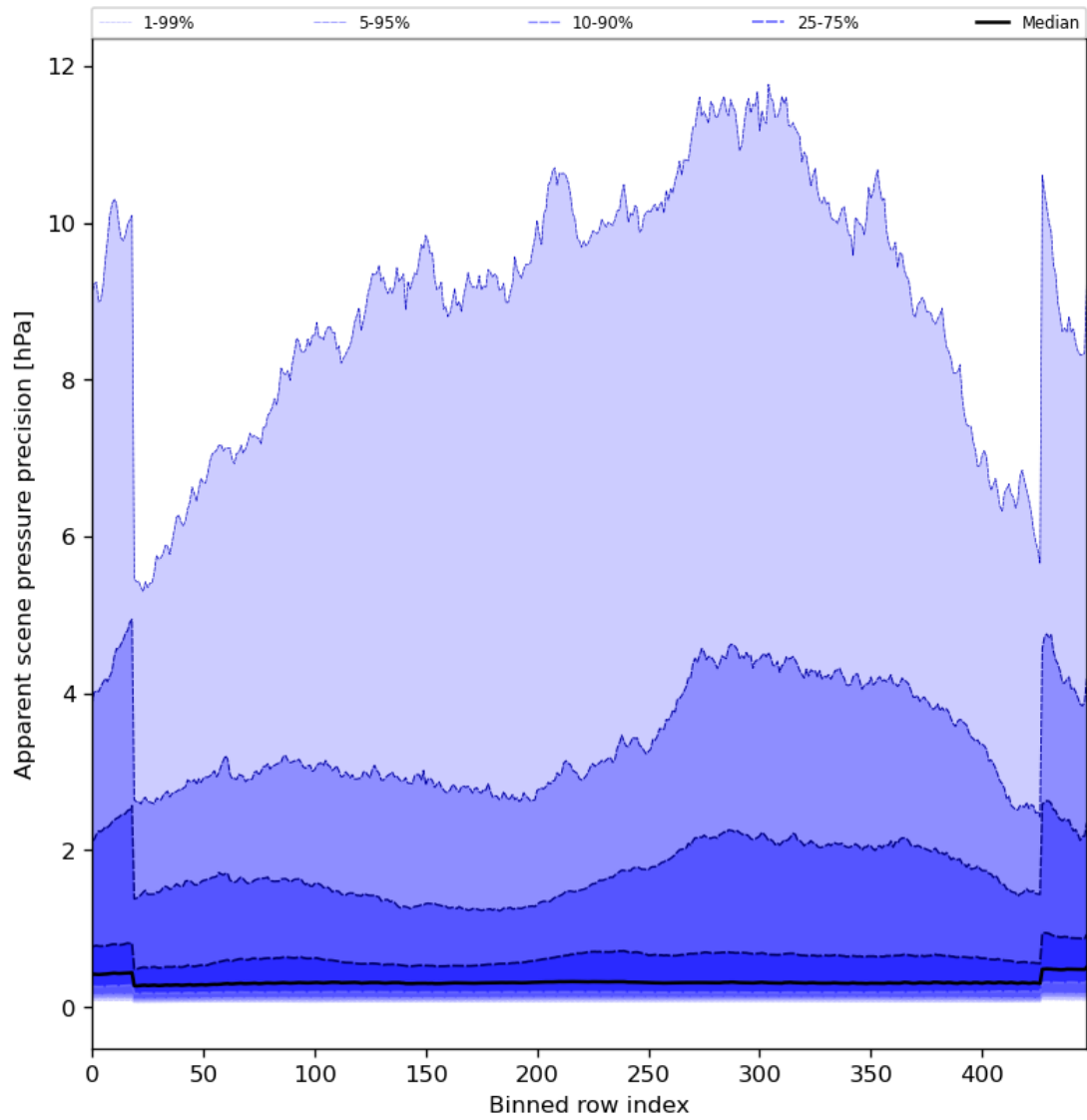
Figure 54: Along track statistics of “Apparent scene pressure precision” for 2024-04-16 to 2024-04-17
