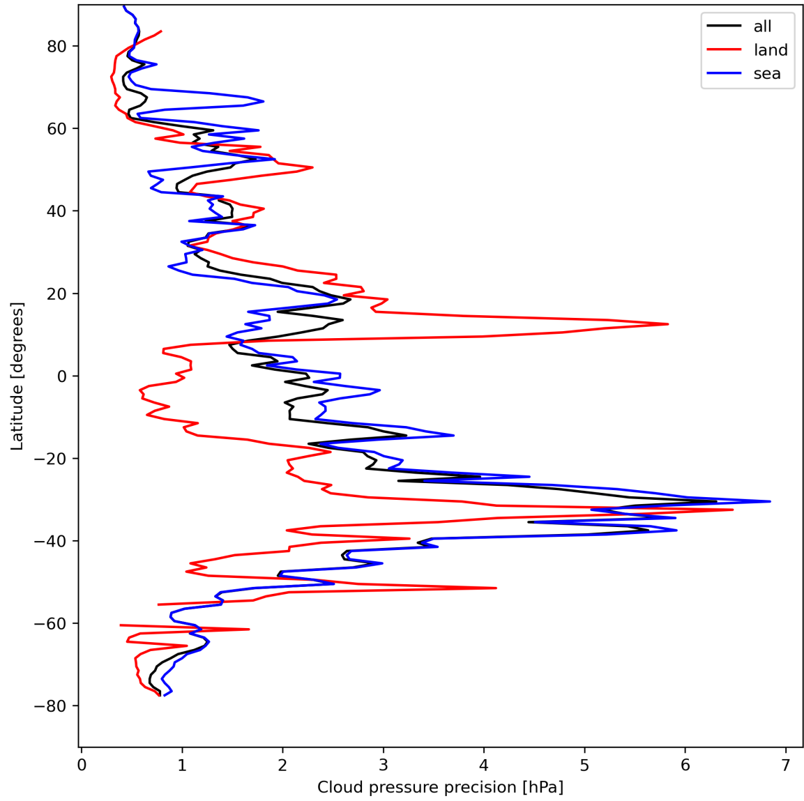
Figure 14: Zonal average of “Cloud pressure precision” for 2024-04-16 to 2024-04-17.
