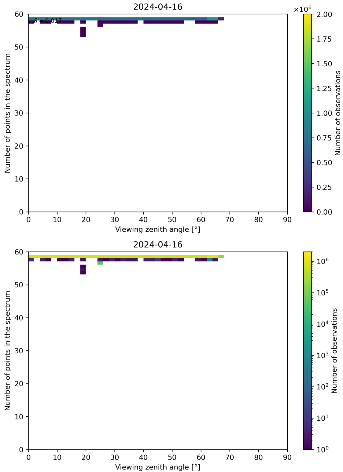
Figure 125: Scatter density plot of “Viewing zenith angle” against “Number of points in the spectrum” for 2024-04-16 to 2024-04-17.
