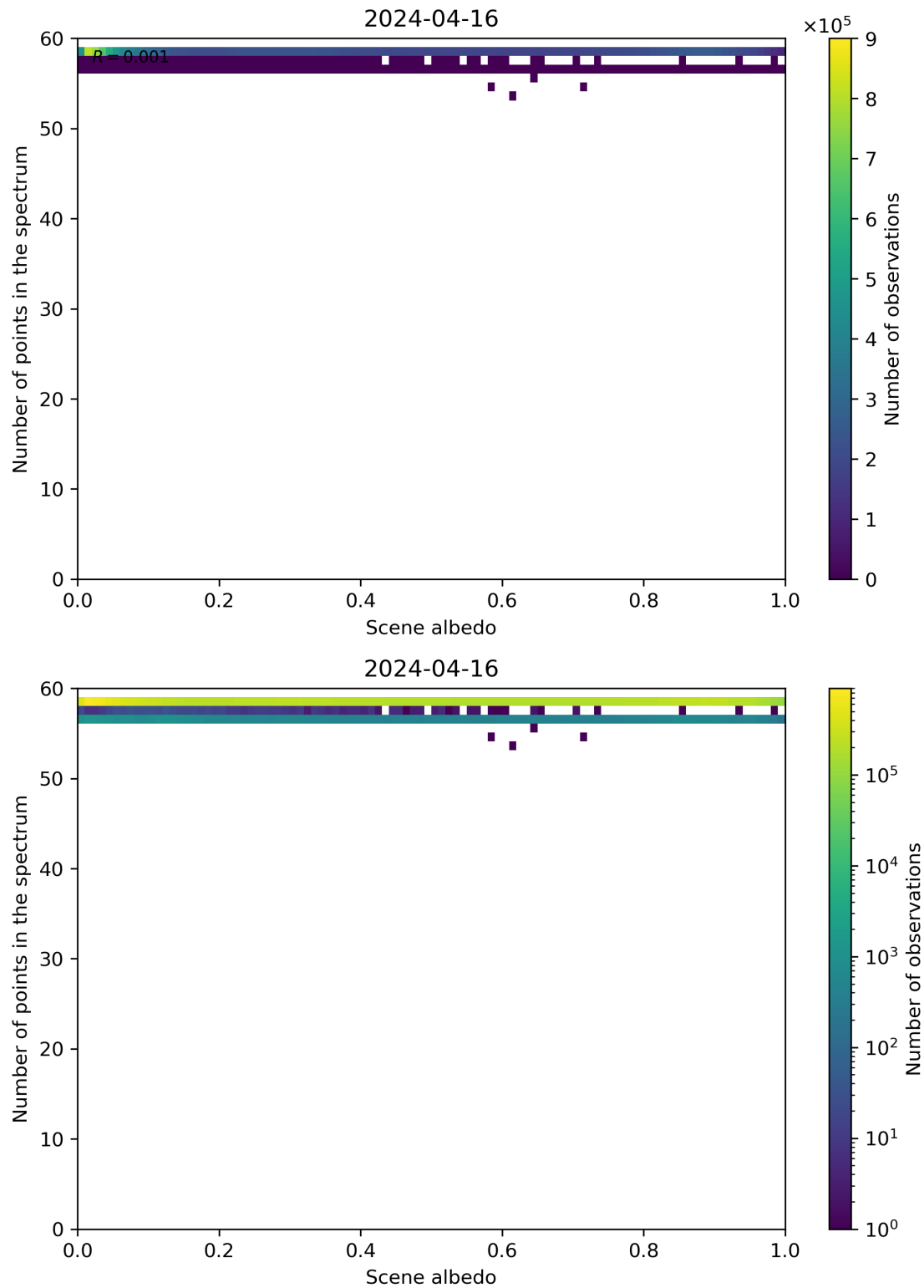
Figure 106: Scatter density plot of “Scene albedo” against “Number of points in the spectrum” for 2024-04-16 to 2024-04-17.
