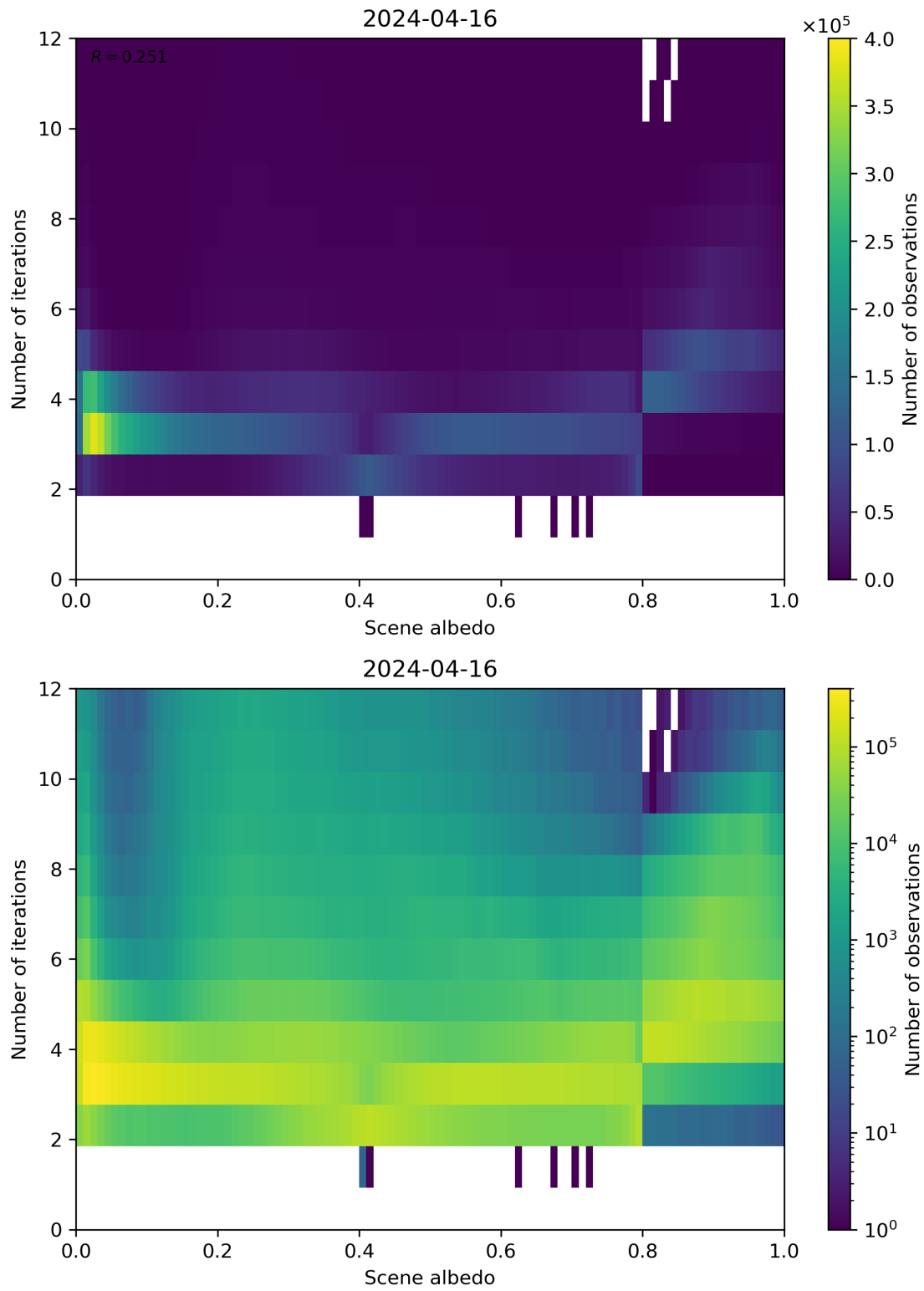
Figure 105: Scatter density plot of “Scene albedo” against “Number of iterations” for 2024-04-16 to 2024-04-17.
