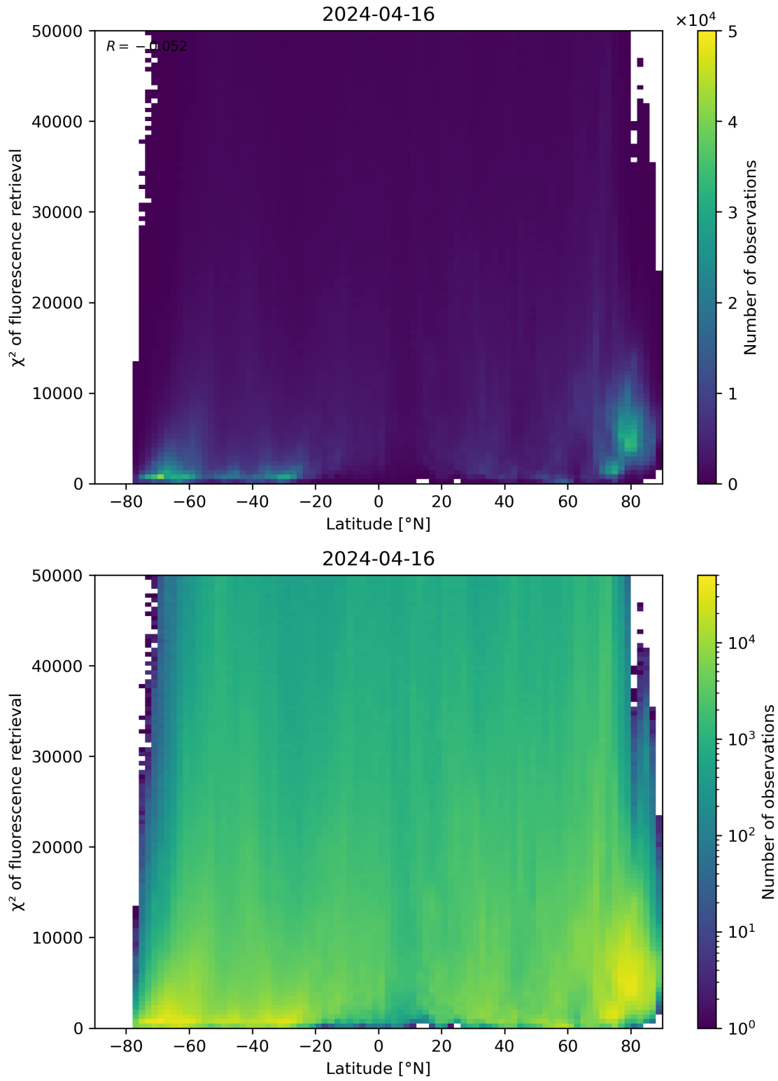
Figure 89: Scatter density plot of “Latitude” against “ \chi^2 of fluorescence retrieval” for 2024-04-16 to 2024-04-17.
