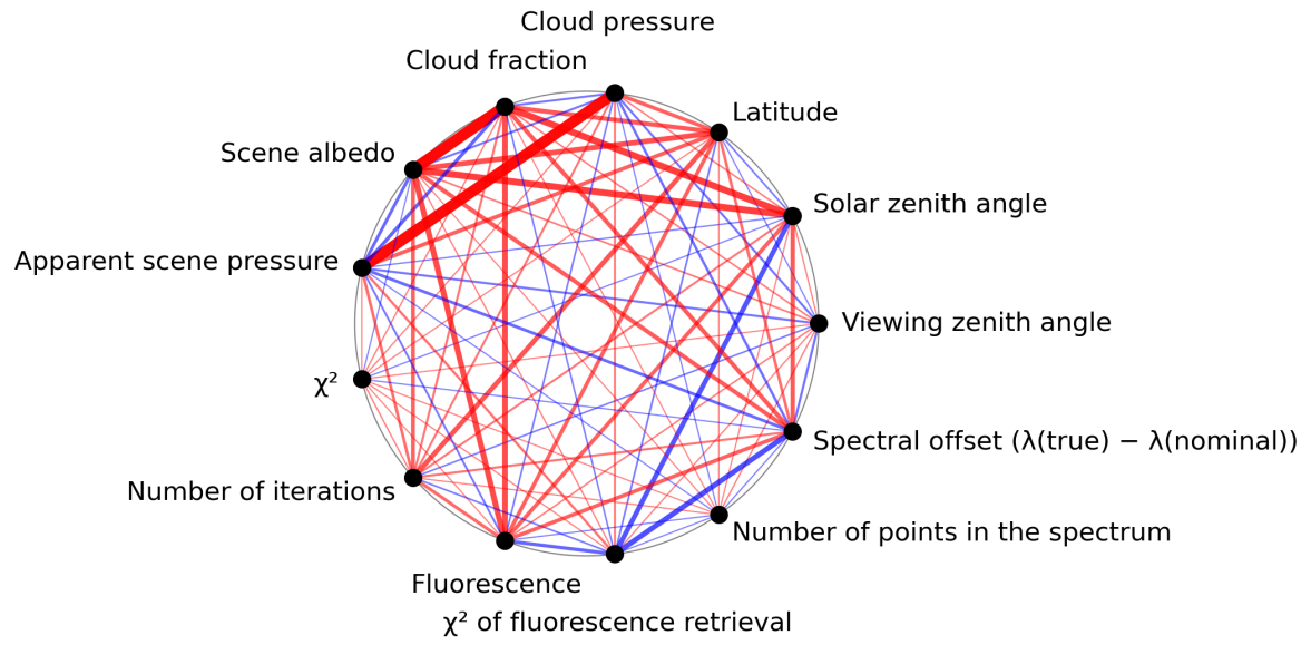
Figure 1: Map of correlation graph for 2024-04-16 to 2024-04-17.
