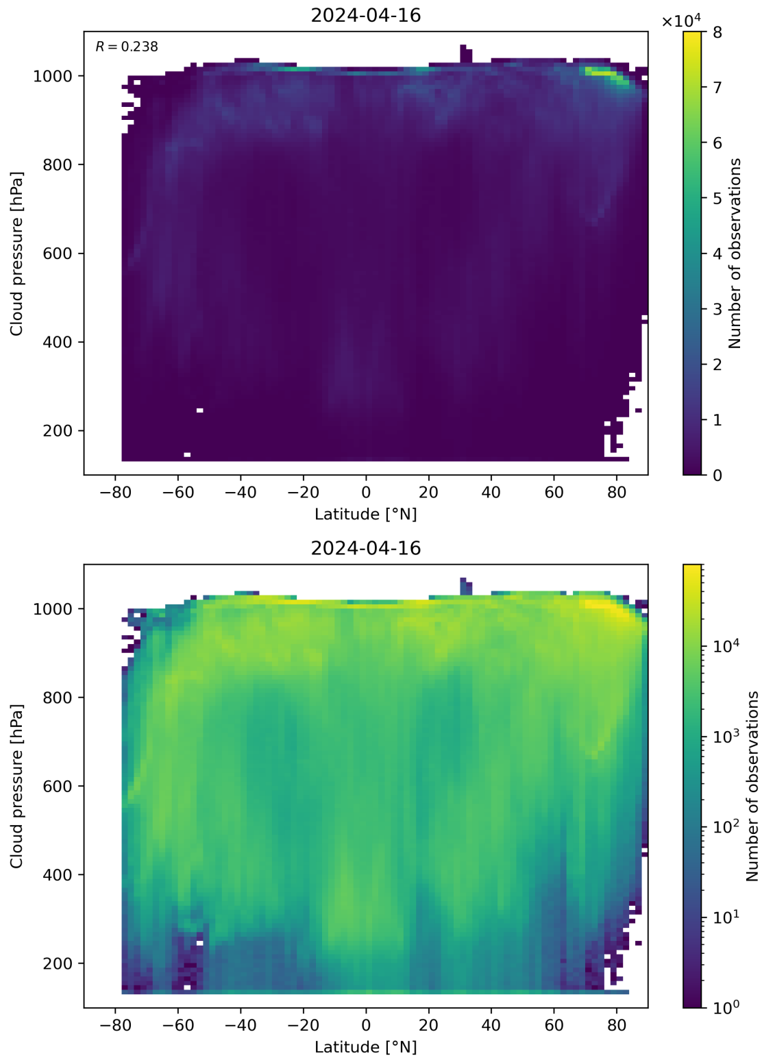
Figure 91: Scatter density plot of “Latitude” against “Cloud pressure” for 2024-04-16 to 2024-04-17.
