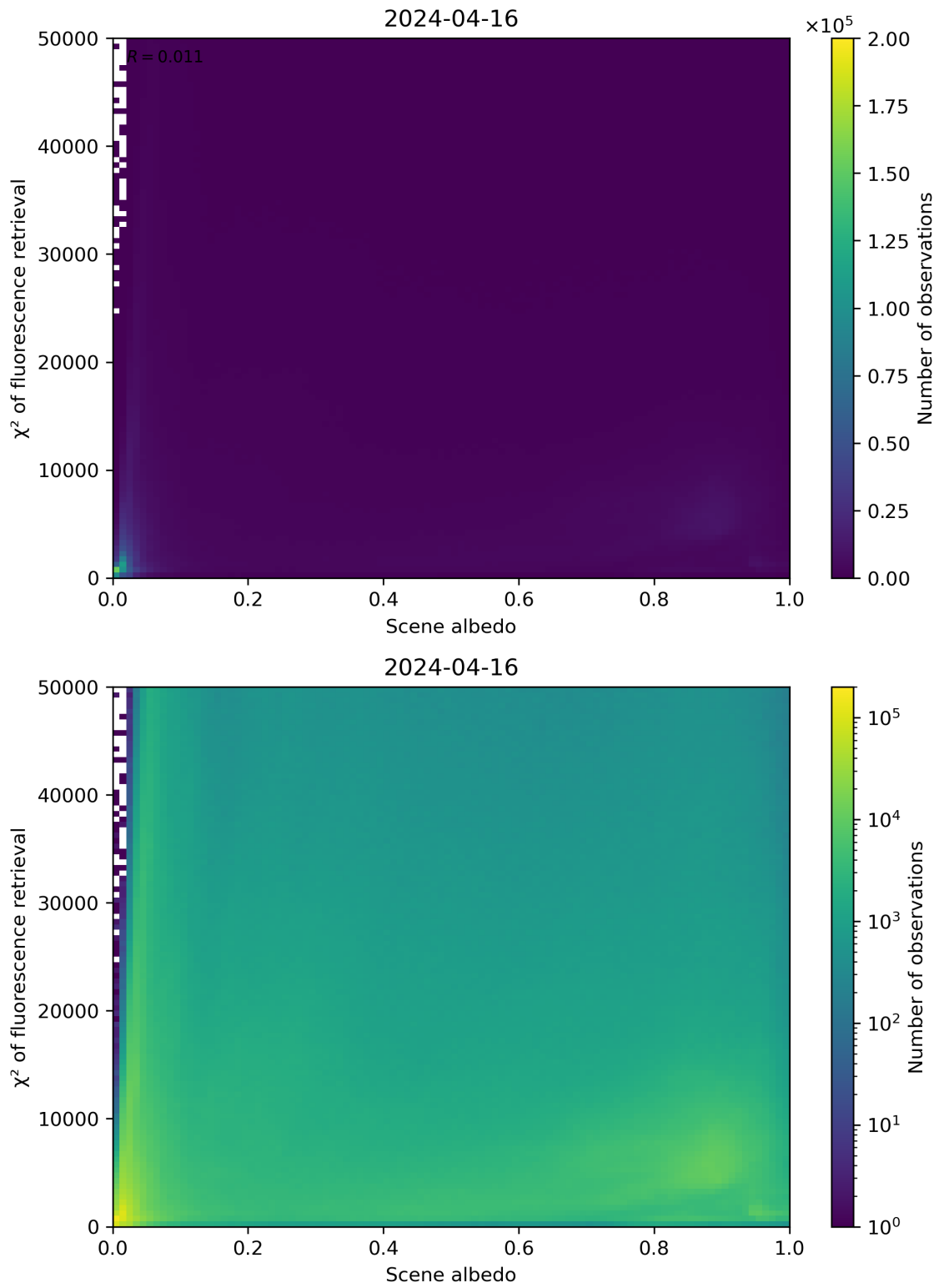
Figure 103: Scatter density plot of “Scene albedo” against “ \chi^2 of fluorescence retrieval” for 2024-04-16 to 2024-04-17.
