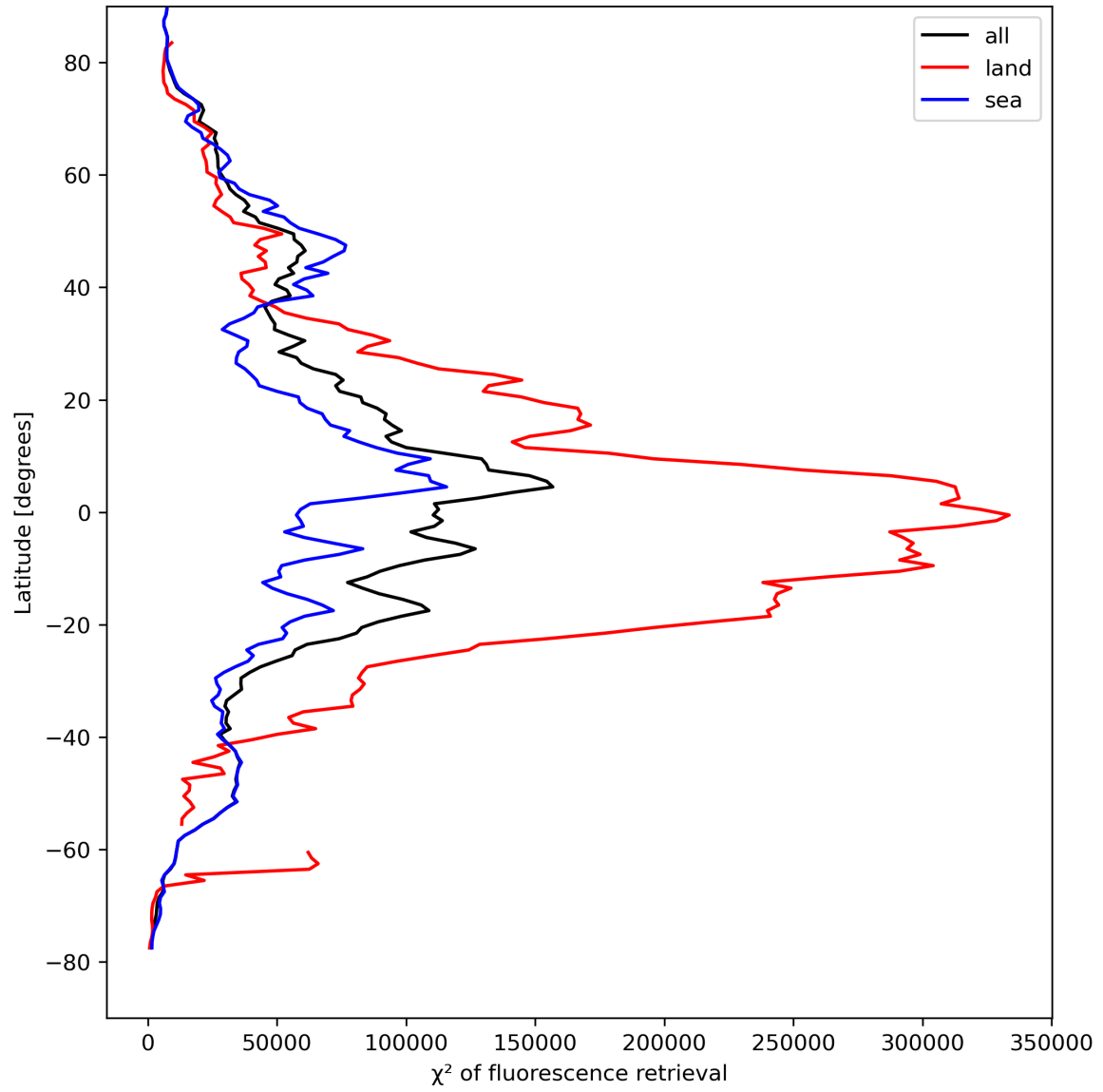
Figure 25: Zonal average of “ \chi^2 of fluorescence retrieval” for 2024-04-16 to 2024-04-17.
