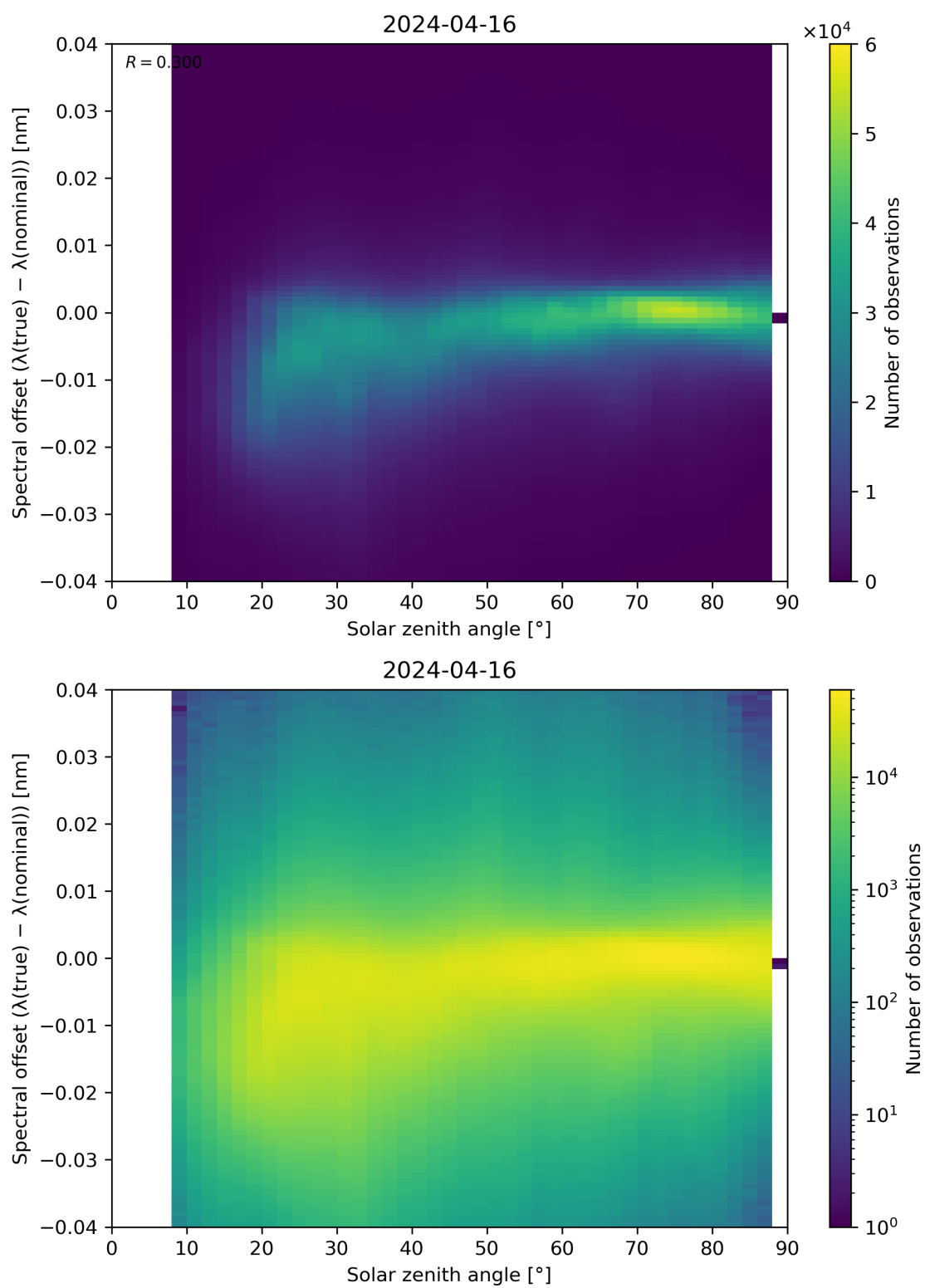
Figure 117: Scatter density plot of “Solar zenith angle” against “Spectral offset ( \lambda(\text{true}) - \lambda(\text{nominal}) )” for 2024-04-16 to 2024-04-17.
