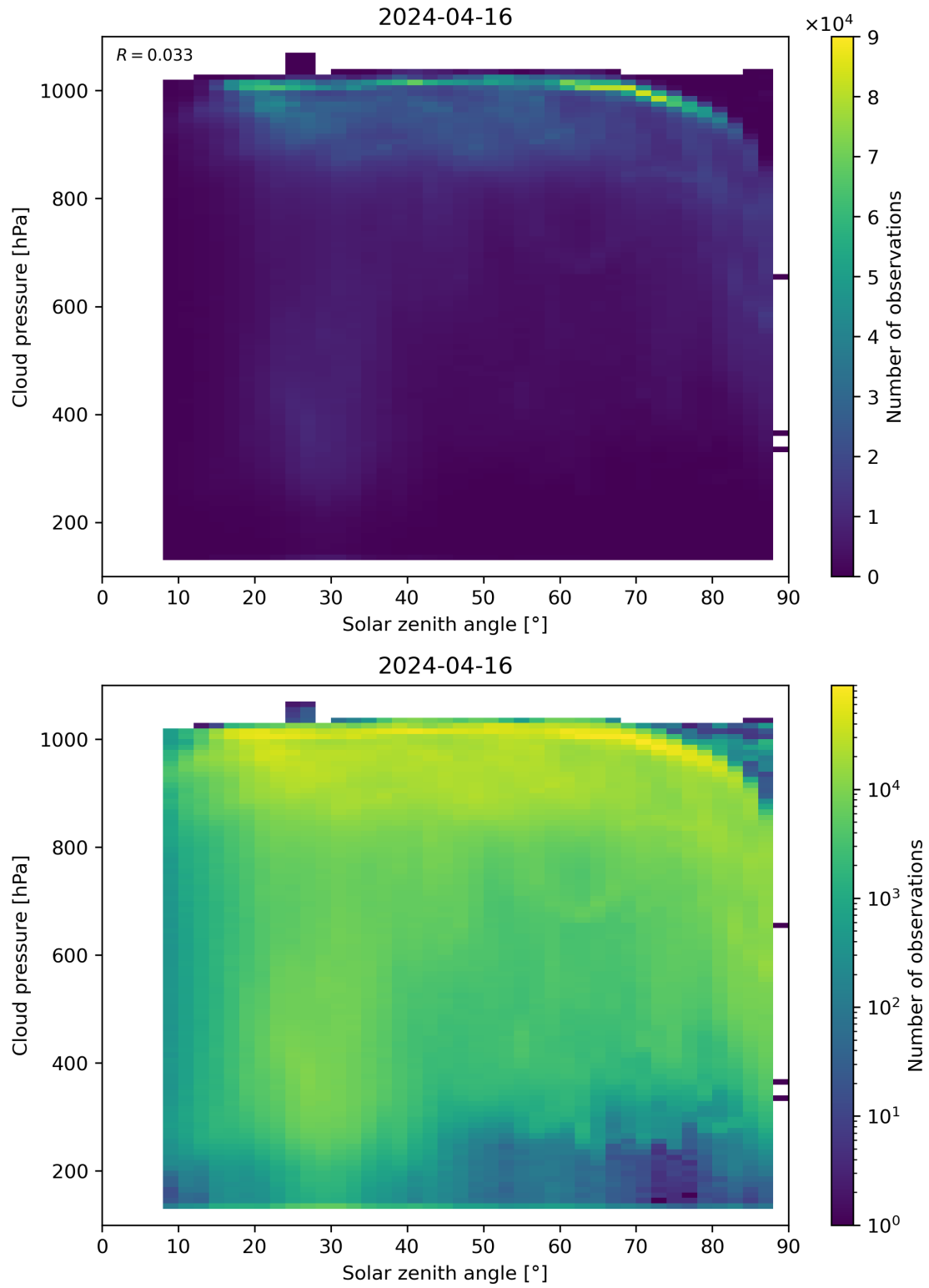
Figure 111: Scatter density plot of “Solar zenith angle” against “Cloud pressure” for 2024-04-16 to 2024-04-17.
