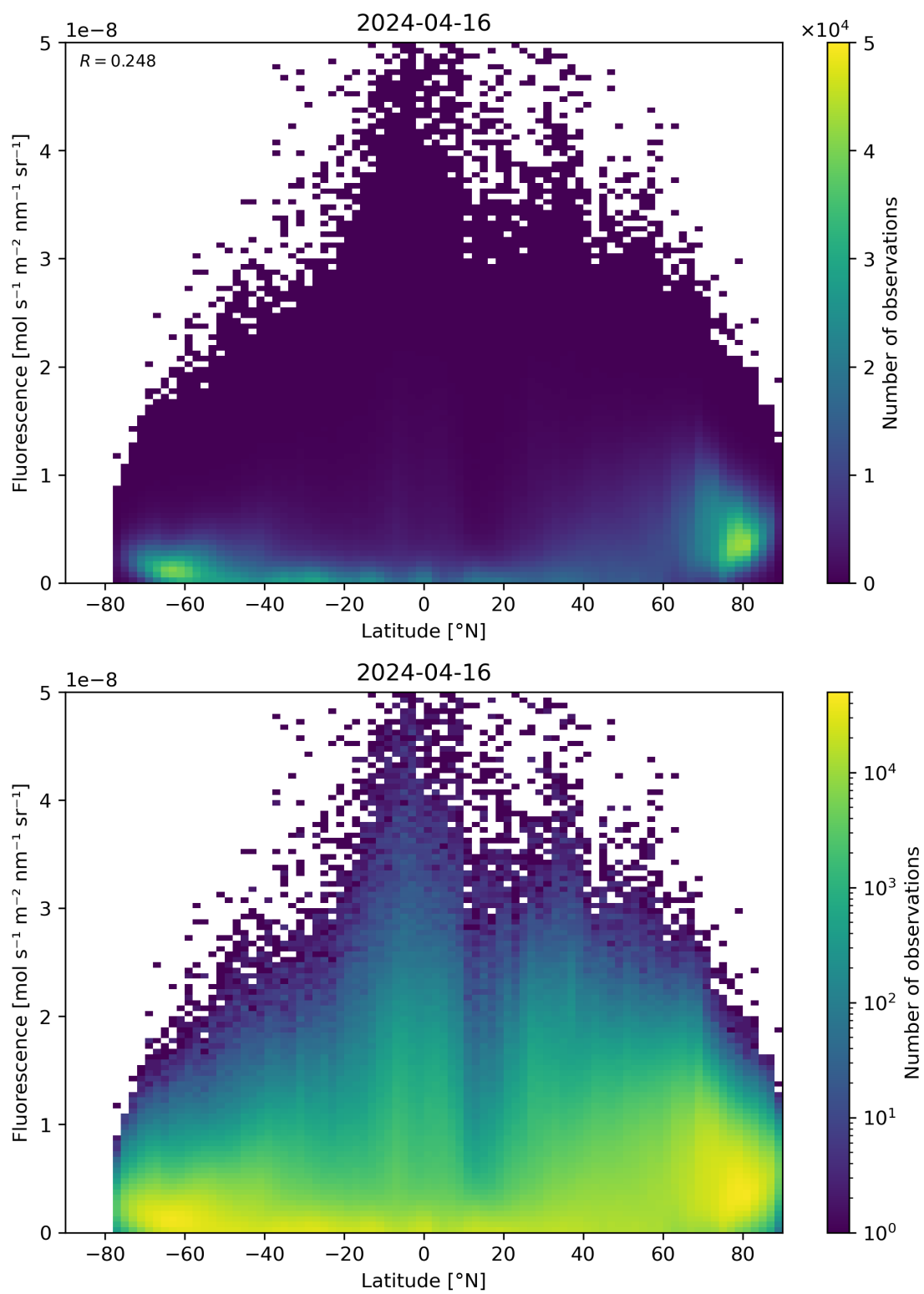
Figure 92: Scatter density plot of “Latitude” against “Fluorescence” for 2024-04-16 to 2024-04-17.
