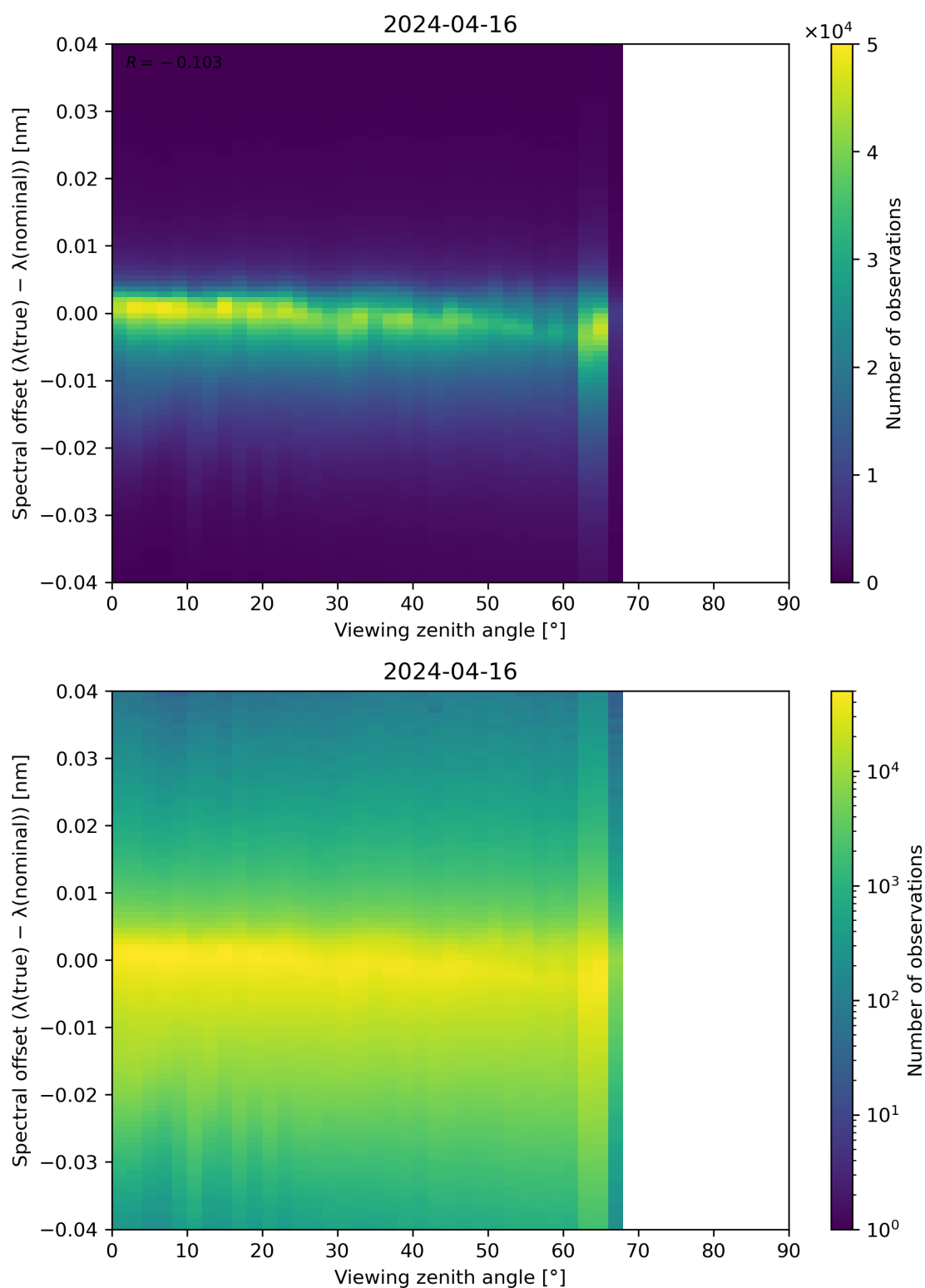
Figure 128: Scatter density plot of “Viewing zenith angle” against “Spectral offset ( \lambda(\text{true}) - \lambda(\text{nominal}) )” for 2024-04-16 to 2024-04-17.
