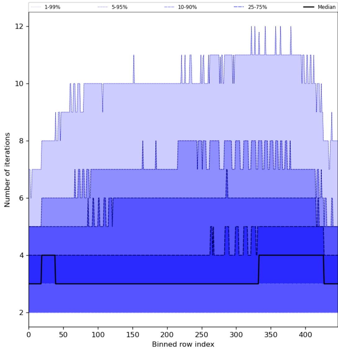
Figure 56: Along track statistics of “Number of iterations” for 2024-04-16 to 2024-04-17
