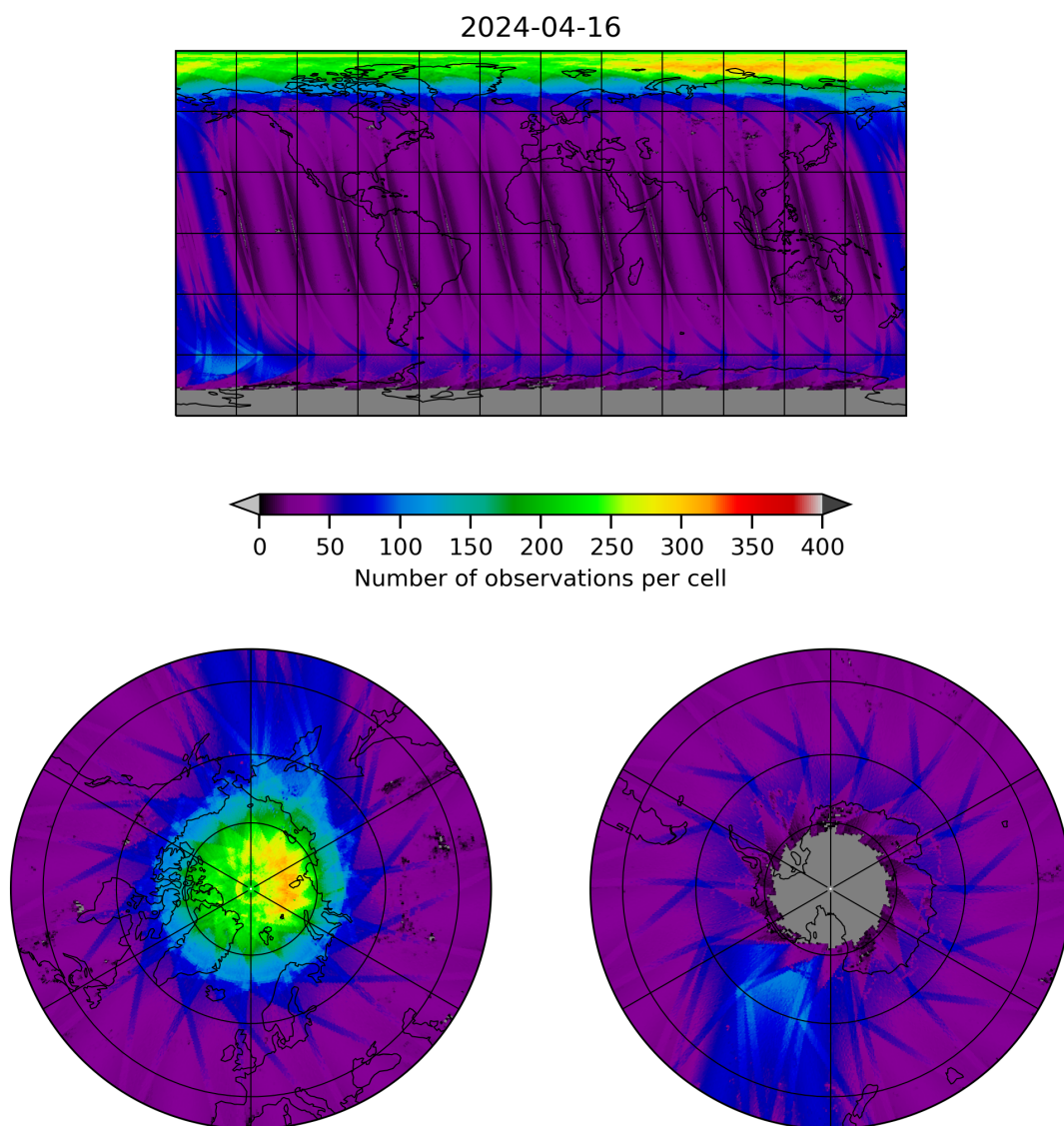
Figure 11: Map of the number of observations for 2024-04-16 to 2024-04-17
