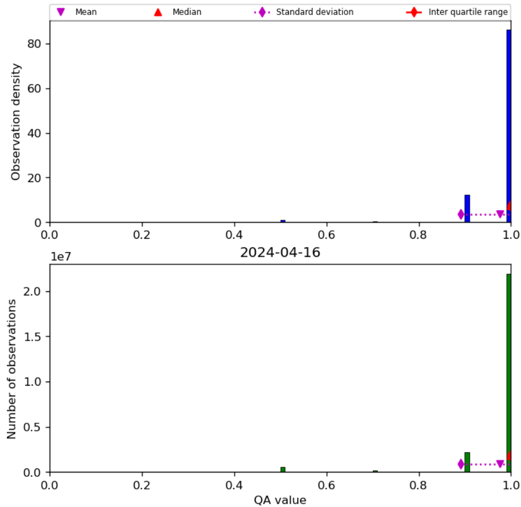
Figure 29: Histogram of “QA value” for 2024-04-16 to 2024-04-17
