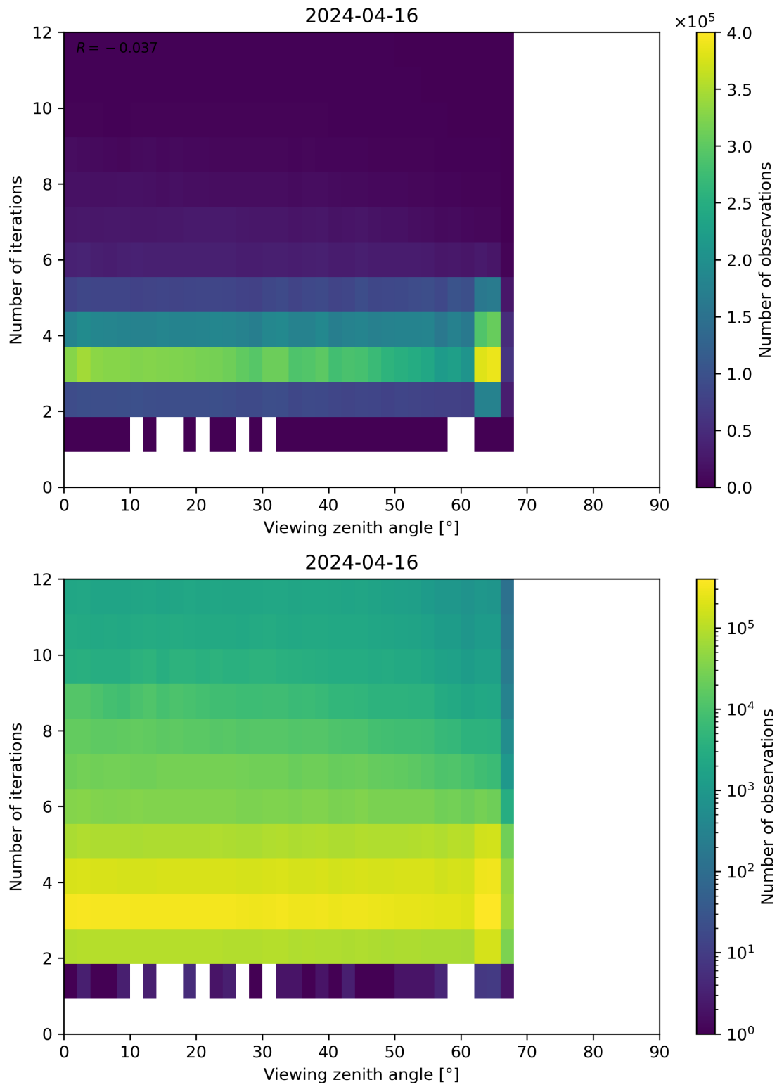
Figure 124: Scatter density plot of “Viewing zenith angle” against “Number of iterations” for 2024-04-16 to 2024-04-17.
