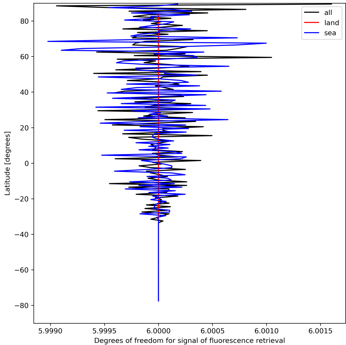
Figure 26: Zonal average of “Degrees of freedom for signal of fluorescence retrieval” for 2024-04-16 to 2024-04-17.
