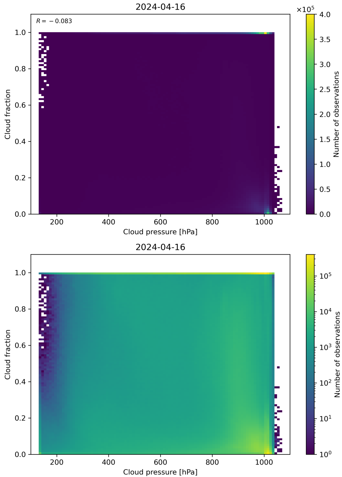
Figure 79: Scatter density plot of “Cloud pressure” against “Cloud fraction” for 2024-04-16 to 2024-04-17.
