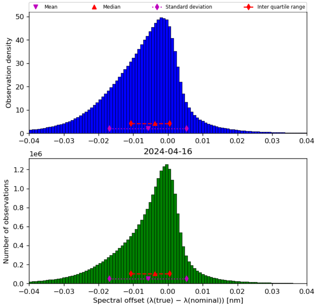
Figure 45: Histogram of “Spectral offset ( \lambda(\text{true}) - \lambda(\text{nominal}) )” for 2024-04-16 to 2024-04-17
