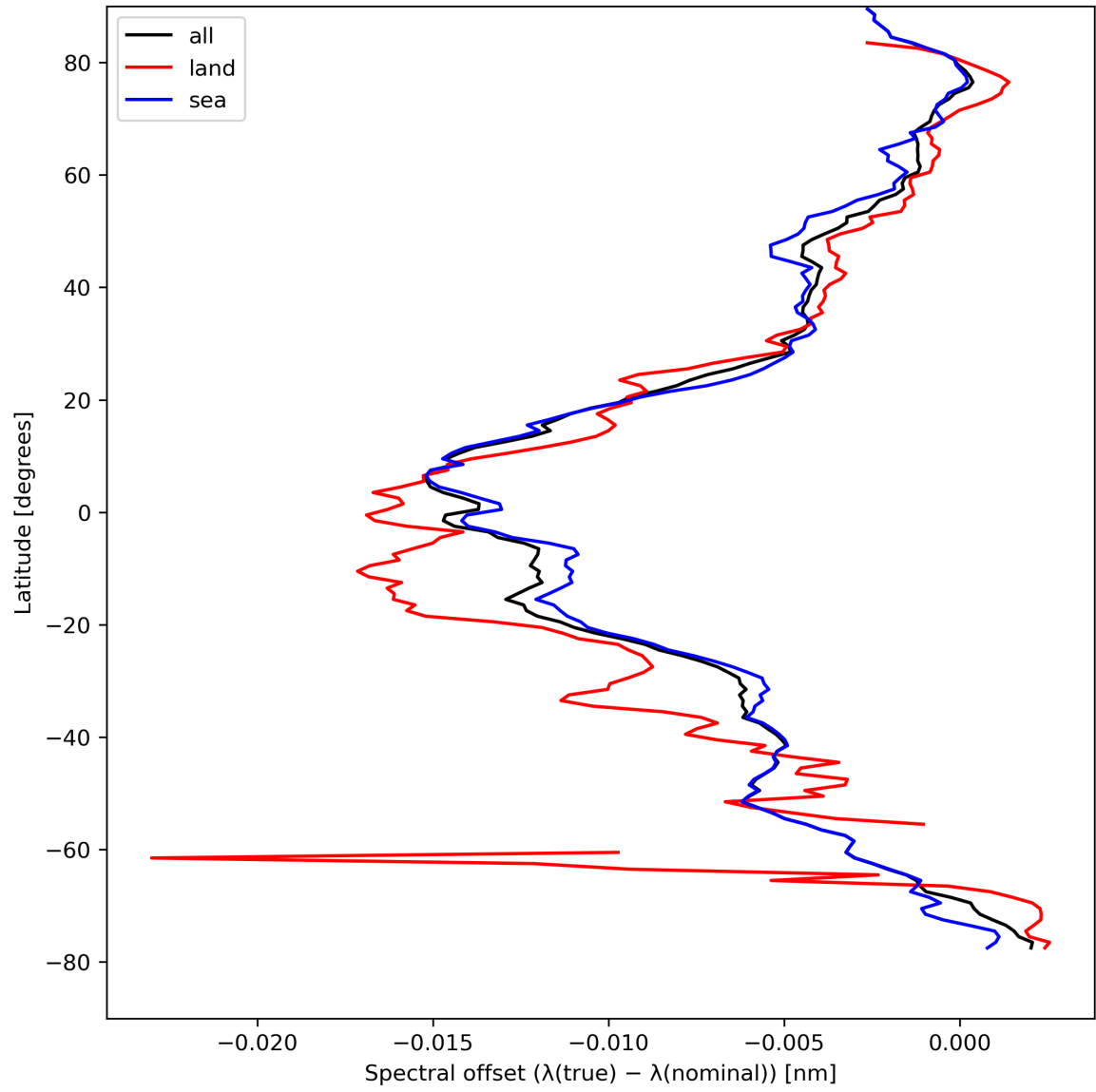
Figure 28: Zonal average of “Spectral offset ( \lambda(\text{true}) - \lambda(\text{nominal}) )” for 2024-04-16 to 2024-04-17.
