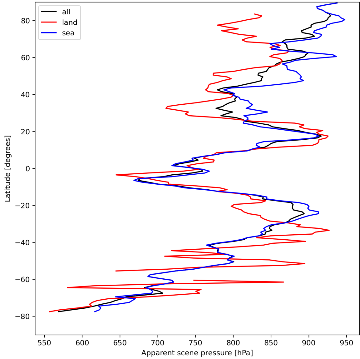
Figure 19: Zonal average of “Apparent scene pressure” for 2024-04-16 to 2024-04-17.
