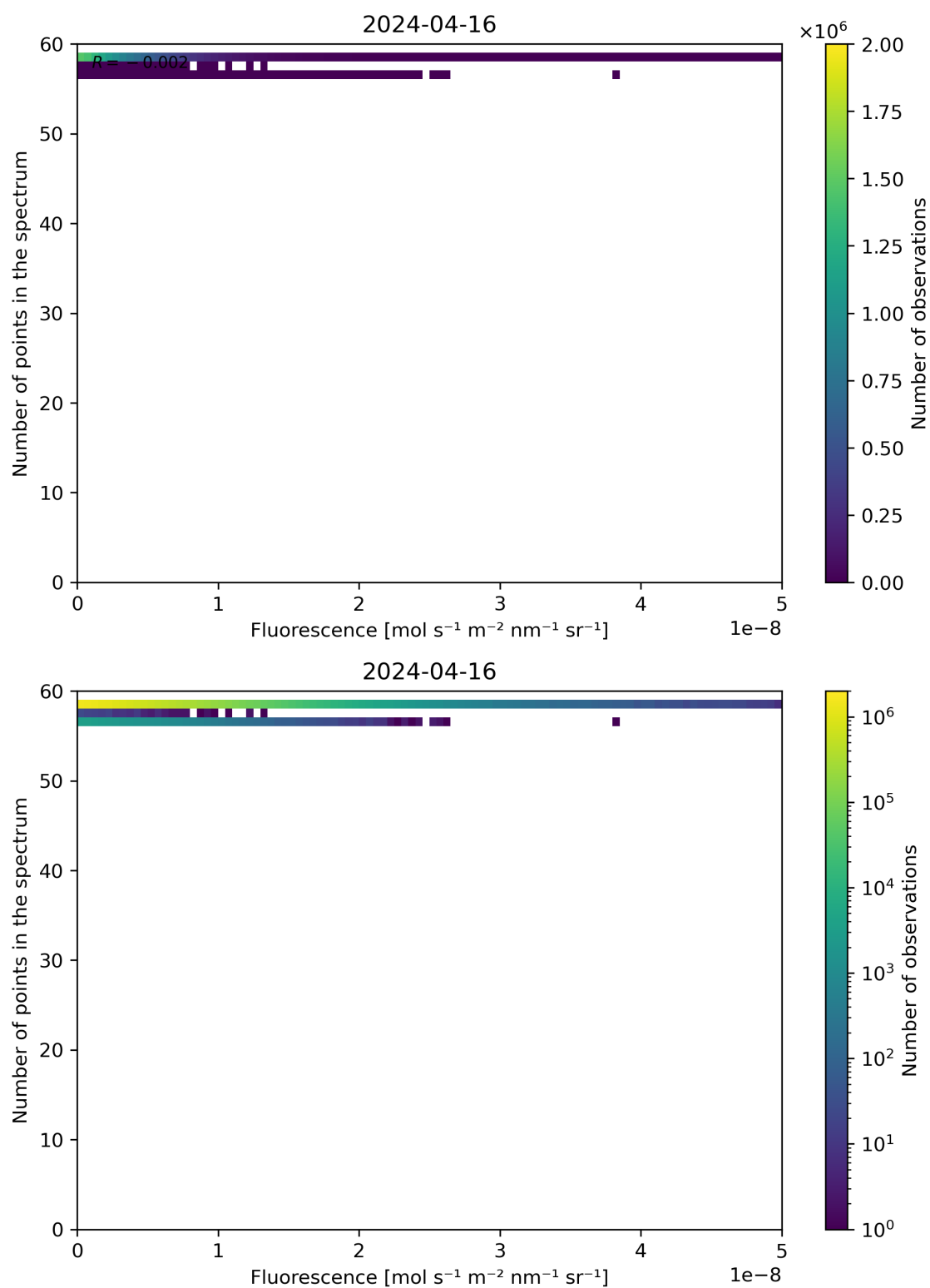
Figure 86: Scatter density plot of “Fluorescence” against “Number of points in the spectrum” for 2024-04-16 to 2024-04-17.
