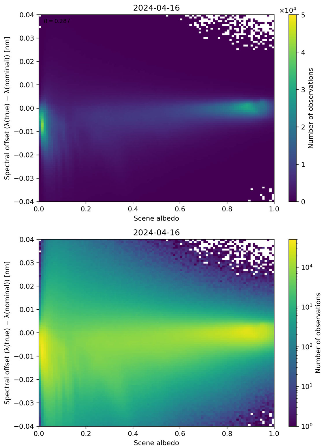
Figure 107: Scatter density plot of “Scene albedo” against “Spectral offset ( \lambda(\text{true}) - \lambda(\text{nominal}) )” for 2024-04-16 to 2024-04-17.
