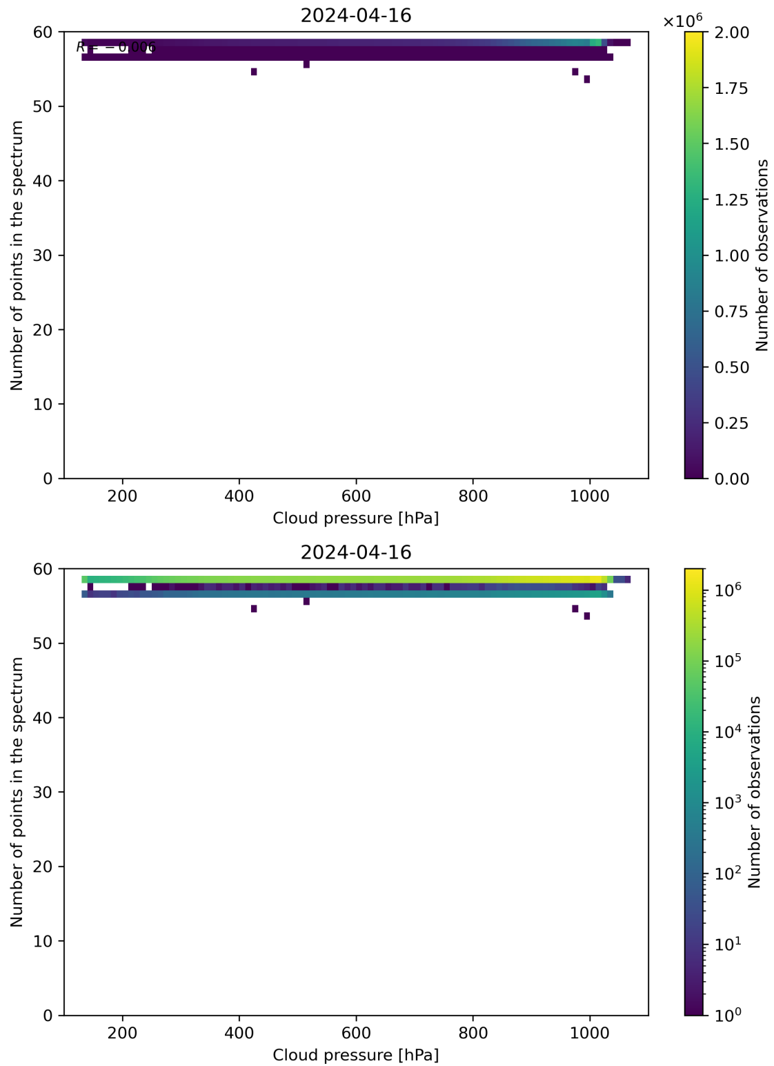
Figure 82: Scatter density plot of “Cloud pressure” against “Number of points in the spectrum” for 2024-04-16 to 2024-04-17.
