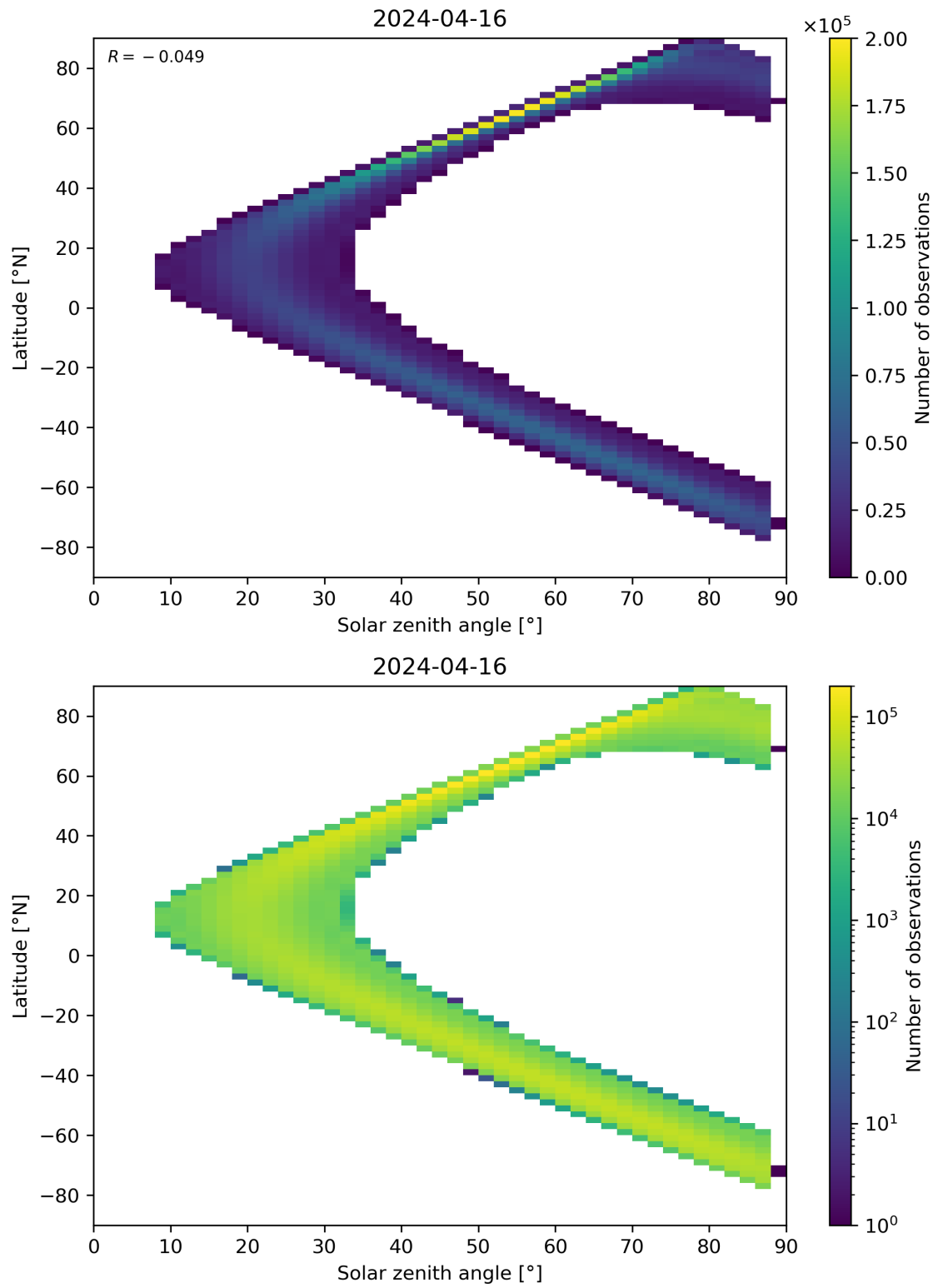
Figure 113: Scatter density plot of “Solar zenith angle” against “Latitude” for 2024-04-16 to 2024-04-17.
