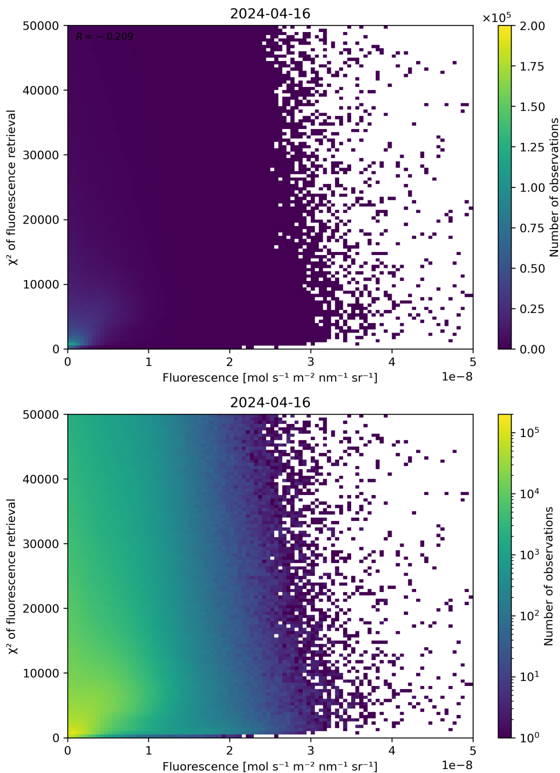
Figure 85: Scatter density plot of “Fluorescence” against “ \chi^2 of fluorescence retrieval” for 2024-04-16 to 2024-04-17.
