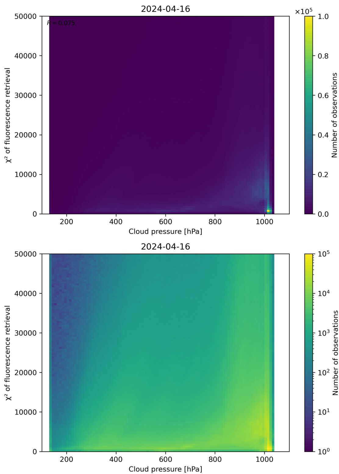
Figure 78: Scatter density plot of “Cloud pressure” against “ \chi^2 of fluorescence retrieval” for 2024-04-16 to 2024-04-17.
