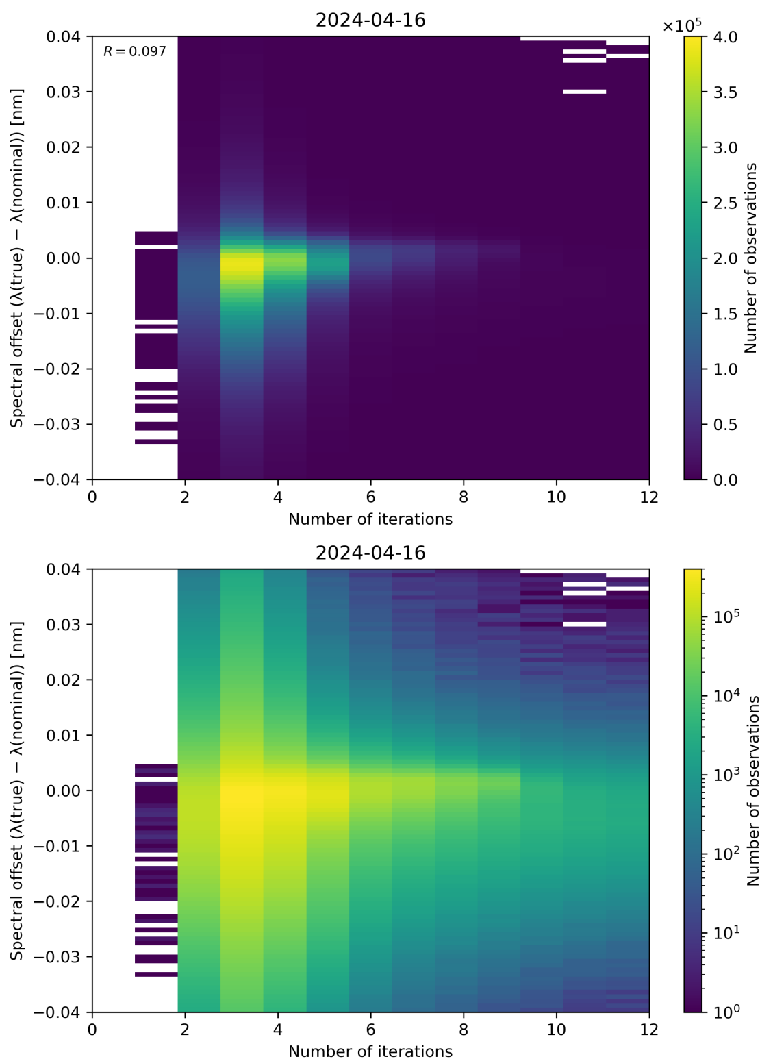
Figure 100: Scatter density plot of “Number of iterations” against “Spectral offset ( \lambda(\text{true}) - \lambda(\text{nominal}) )” for 2024-04-16 to 2024-04-17.
