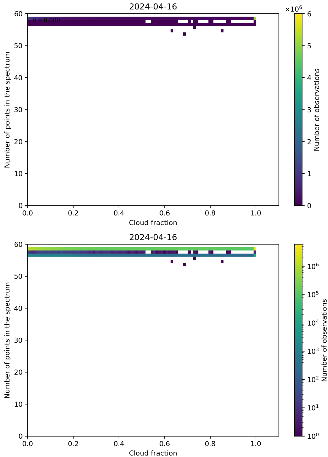
Figure 74: Scatter density plot of “Cloud fraction” against “Number of points in the spectrum” for 2024-04-16 to 2024-04-17.
