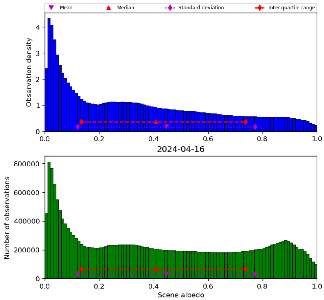
Figure 34: Histogram of “Scene albedo” for 2024-04-16 to 2024-04-17
