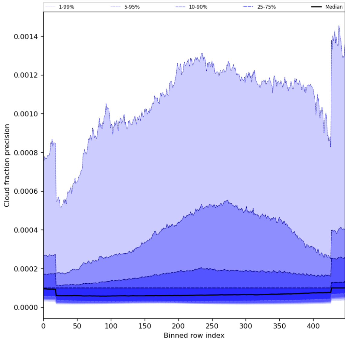
Figure 50: Along track statistics of “Cloud fraction precision” for 2024-04-16 to 2024-04-17
