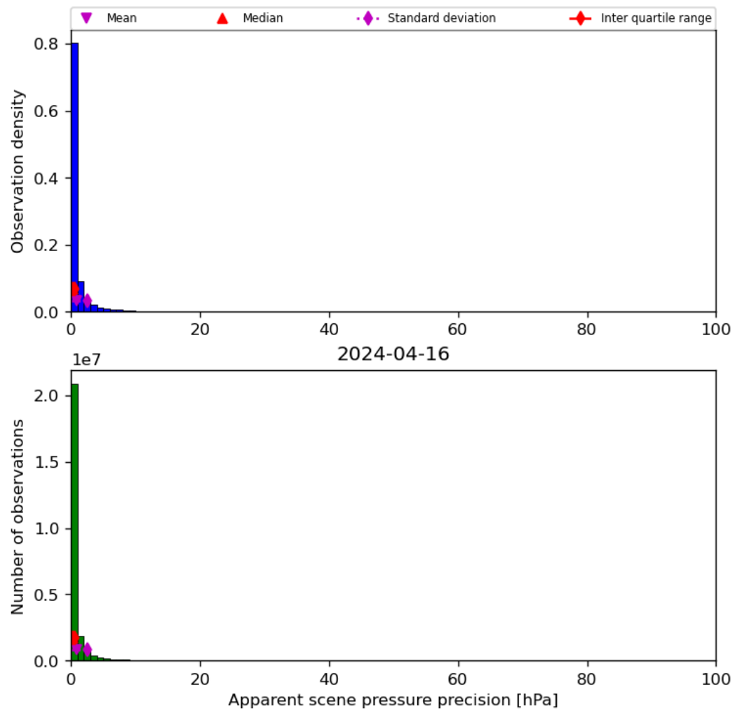
Figure 37: Histogram of “Apparent scene pressure precision” for 2024-04-16 to 2024-04-17
