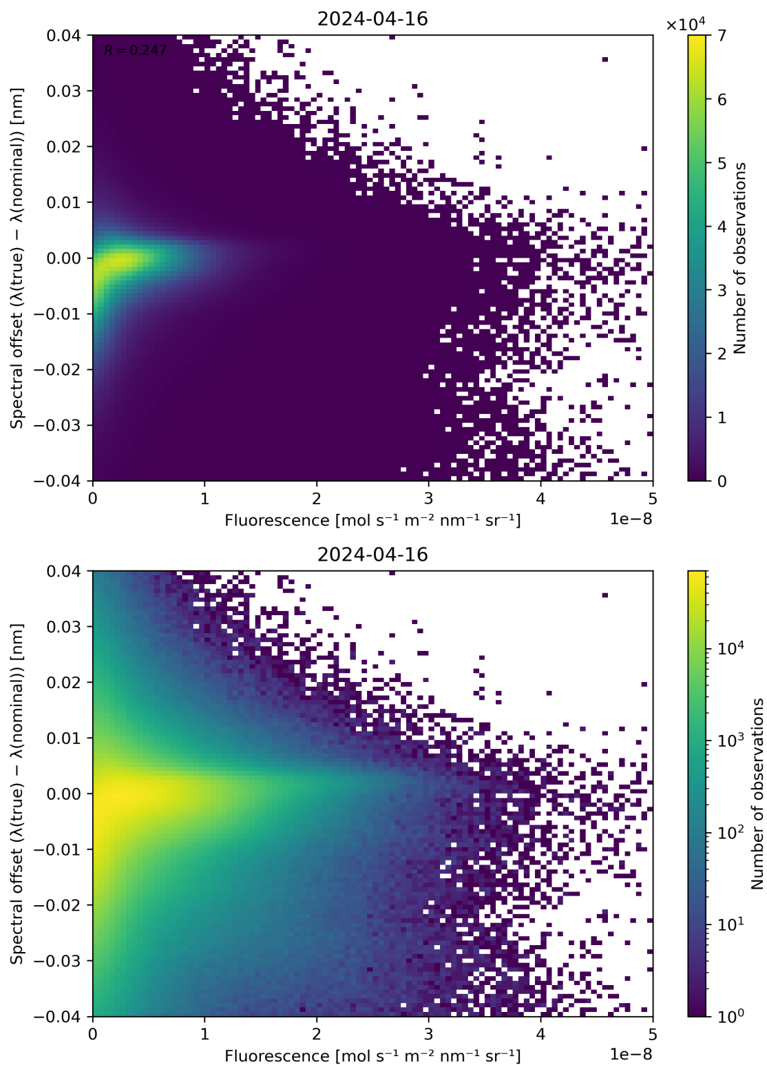
Figure 87: Scatter density plot of “Fluorescence” against “Spectral offset ( \lambda(\text{true}) - \lambda(\text{nominal}) )” for 2024-04-16 to 2024-04-17.
