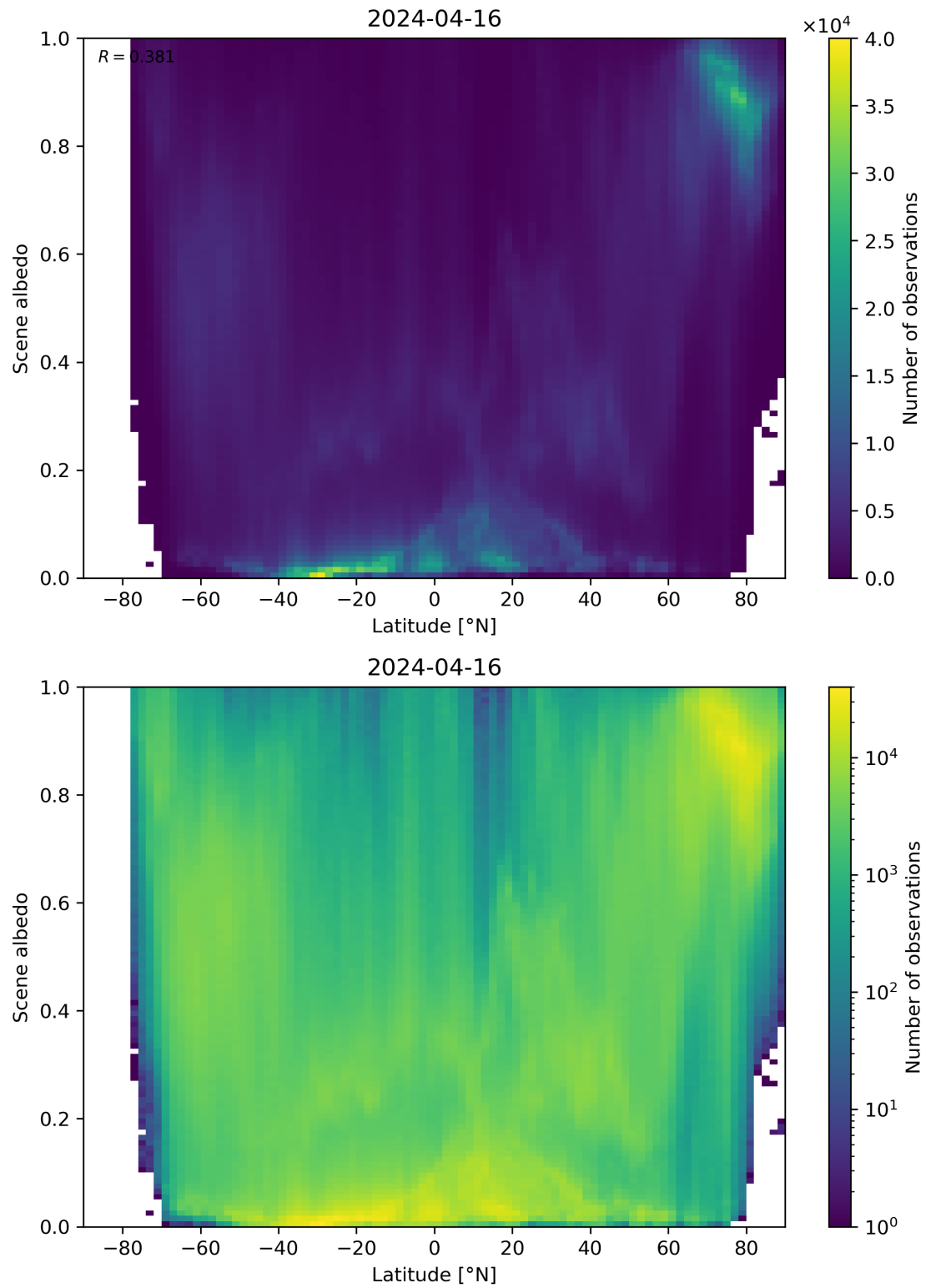
Figure 95: Scatter density plot of “Latitude” against “Scene albedo” for 2024-04-16 to 2024-04-17.
