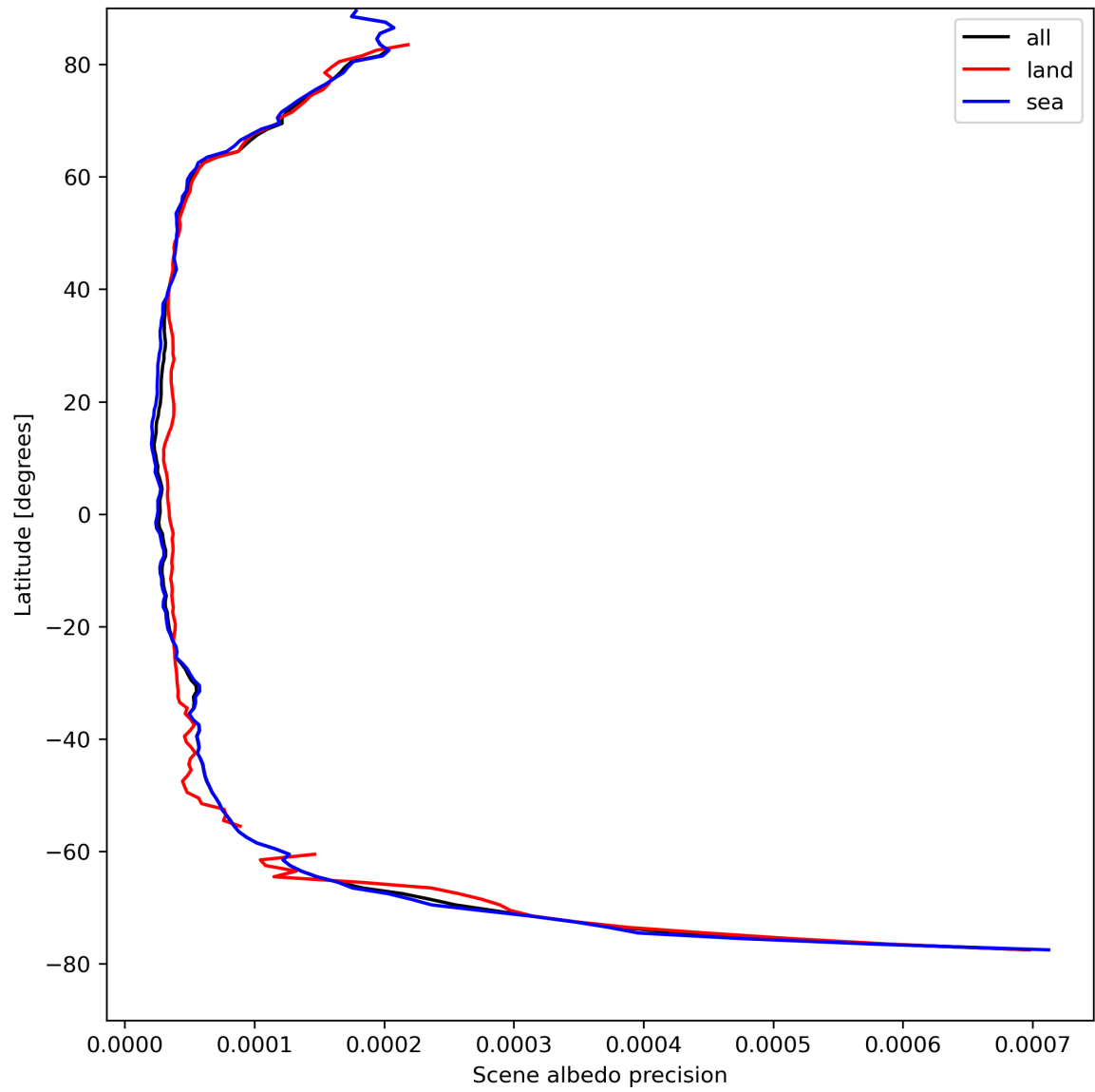
Figure 18: Zonal average of “Scene albedo precision” for 2024-04-16 to 2024-04-17.
