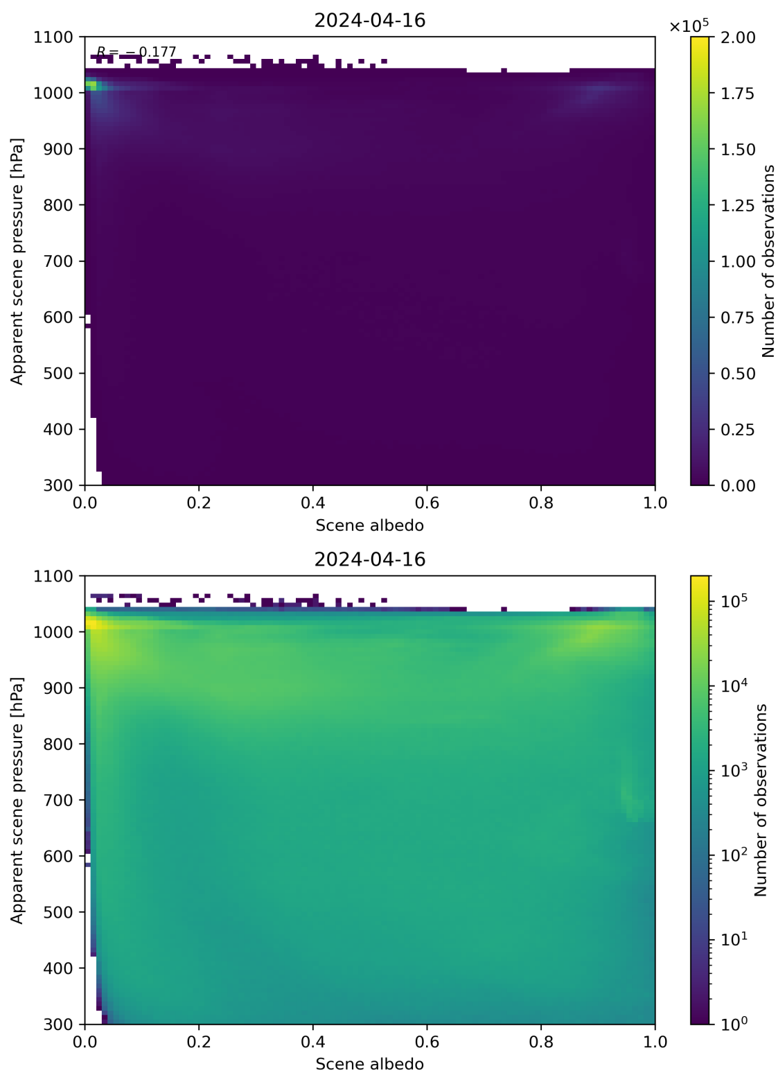
Figure 102: Scatter density plot of “Scene albedo” against “Apparent scene pressure” for 2024-04-16 to 2024-04-17.
