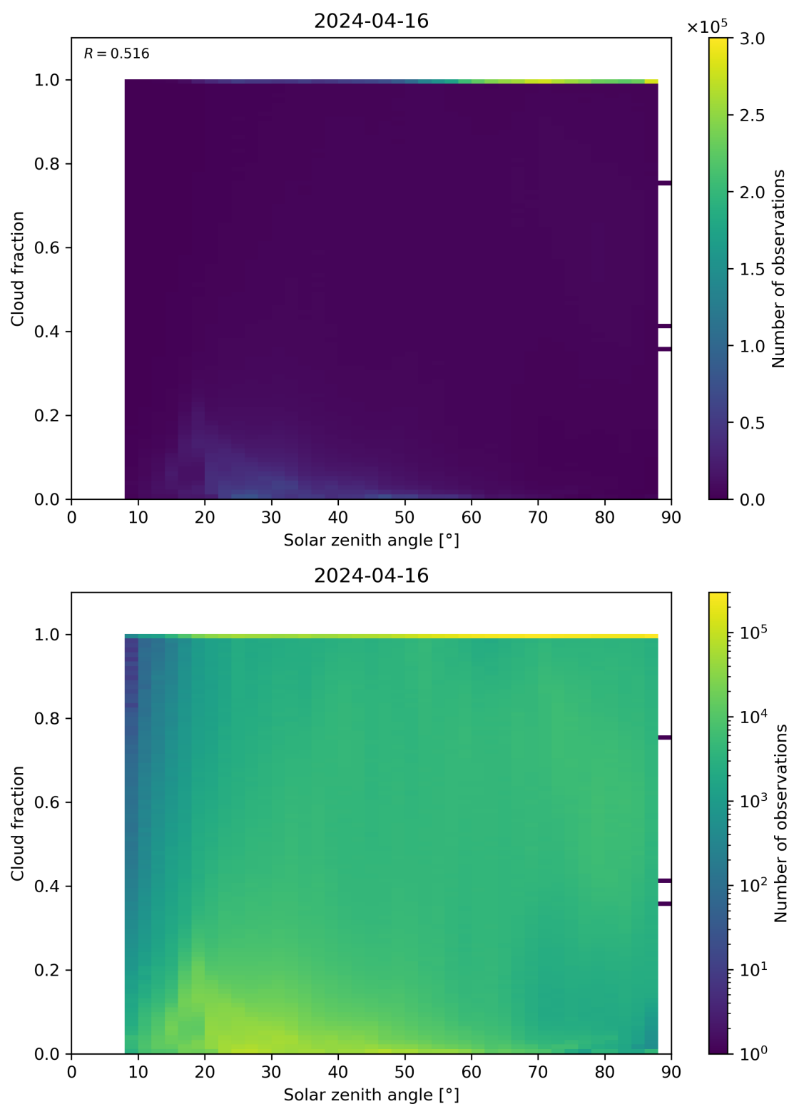
Figure 110: Scatter density plot of “Solar zenith angle” against “Cloud fraction” for 2024-04-16 to 2024-04-17.
