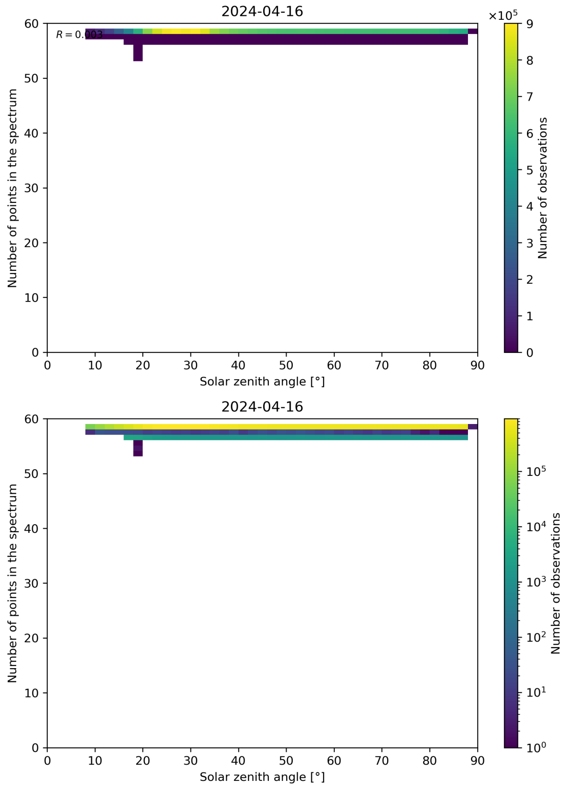
Figure 115: Scatter density plot of “Solar zenith angle” against “Number of points in the spectrum” for 2024-04-16 to 2024-04-17.
