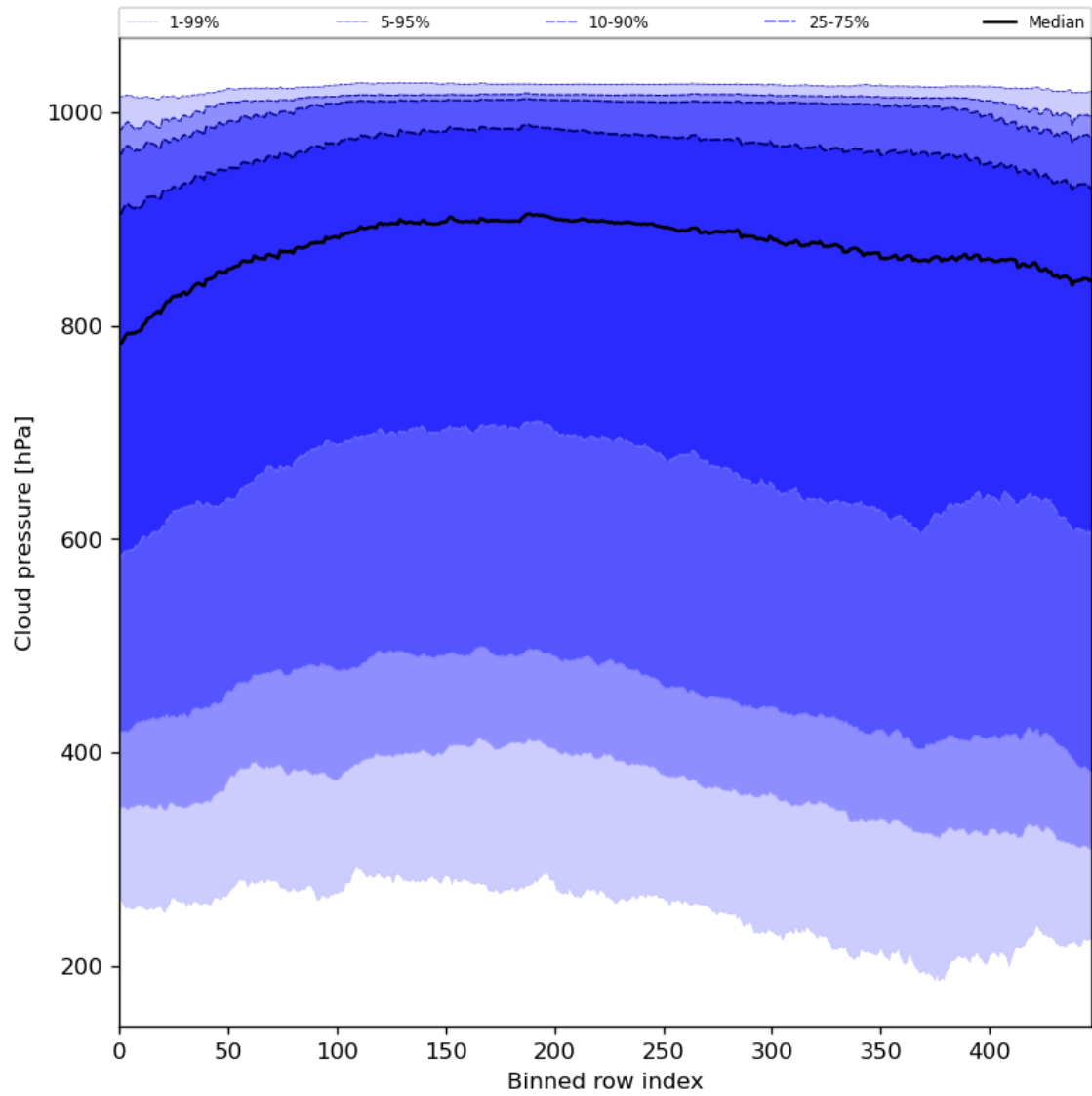
Figure 47: Along track statistics of “Cloud pressure” for 2024-04-16 to 2024-04-17
