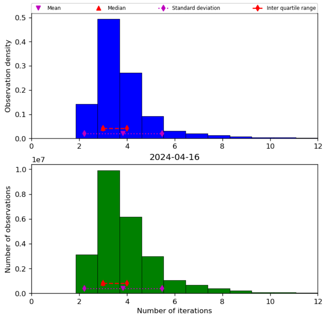
Figure 39: Histogram of “Number of iterations” for 2024-04-16 to 2024-04-17
