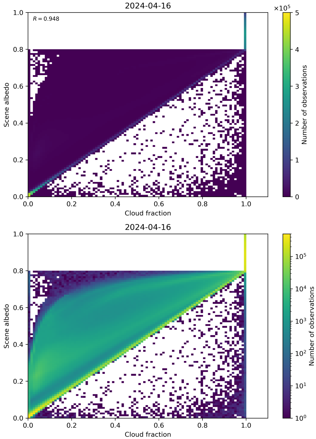
Figure 75: Scatter density plot of “Cloud fraction” against “Scene albedo” for 2024-04-16 to 2024-04-17.
