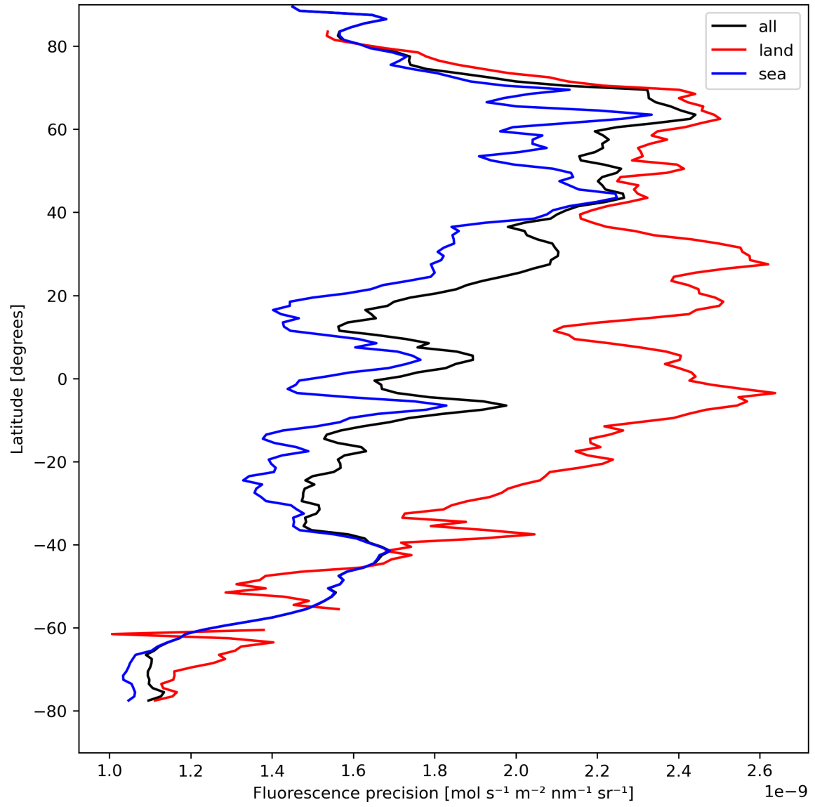
Figure 24: Zonal average of “Fluorescence precision” for 2024-04-16 to 2024-04-17.
