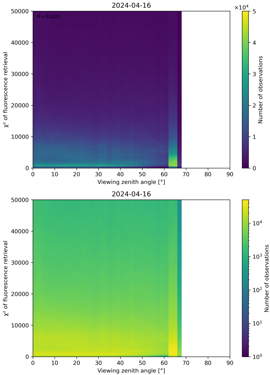
Figure 119: Scatter density plot of “Viewing zenith angle” against “ \chi^2 of fluorescence retrieval” for 2024-04-16 to 2024-04-17.
