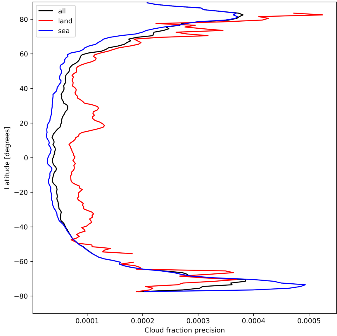
Figure 16: Zonal average of “Cloud fraction precision” for 2024-04-16 to 2024-04-17.
