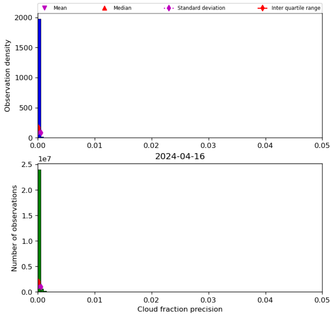
Figure 33: Histogram of “Cloud fraction precision” for 2024-04-16 to 2024-04-17
