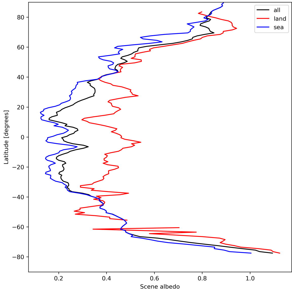
Figure 17: Zonal average of “Scene albedo” for 2024-04-16 to 2024-04-17.
