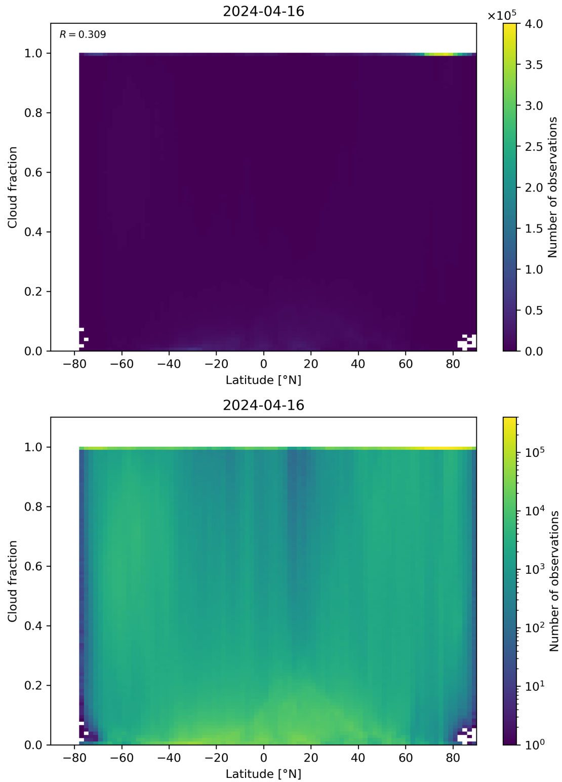
Figure 90: Scatter density plot of “Latitude” against “Cloud fraction” for 2024-04-16 to 2024-04-17.
