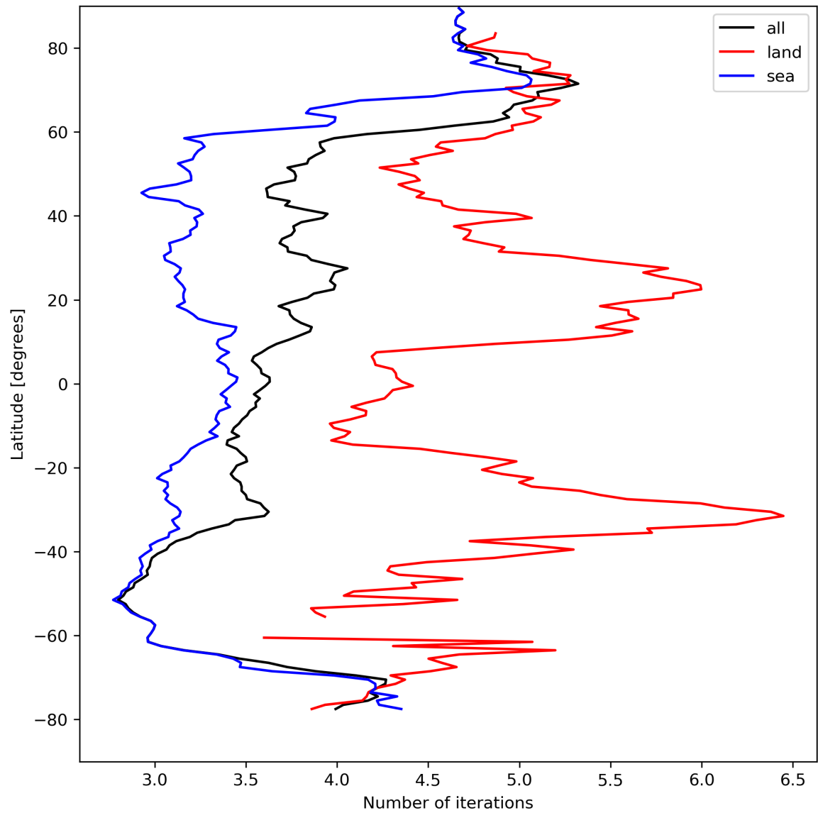
Figure 22: Zonal average of “Number of iterations” for 2024-04-16 to 2024-04-17.
