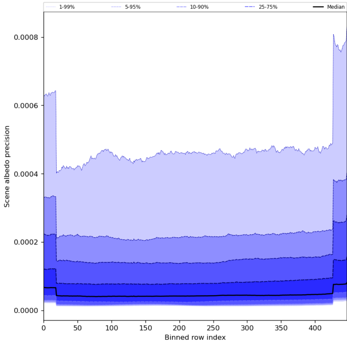
Figure 52: Along track statistics of “Scene albedo precision” for 2024-04-16 to 2024-04-17
