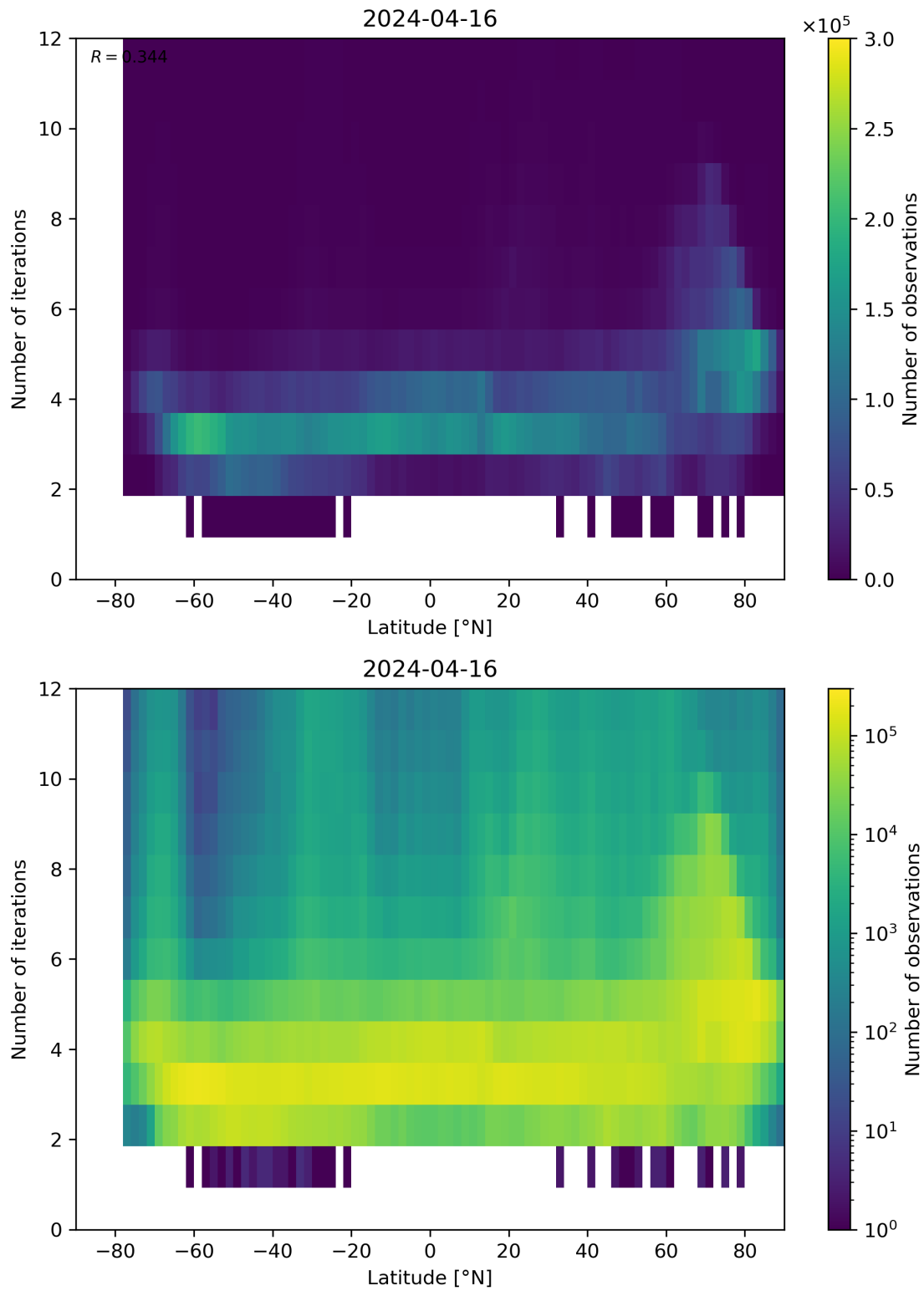
Figure 93: Scatter density plot of “Latitude” against “Number of iterations” for 2024-04-16 to 2024-04-17.
