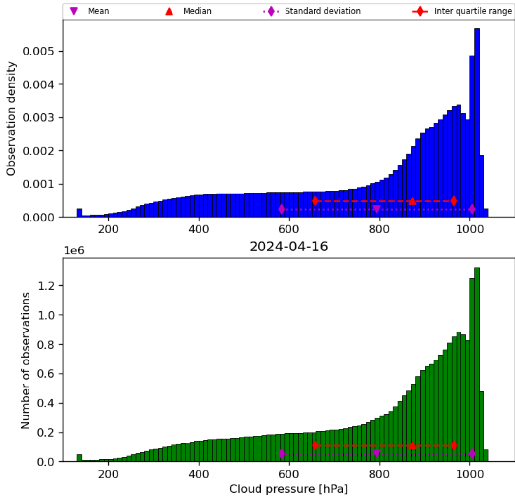
Figure 30: Histogram of “Cloud pressure” for 2024-04-16 to 2024-04-17
