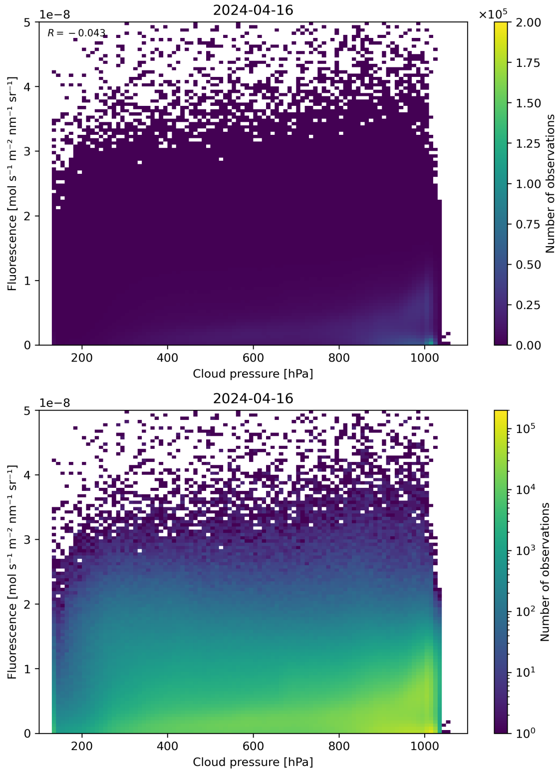
Figure 80: Scatter density plot of “Cloud pressure” against “Fluorescence” for 2024-04-16 to 2024-04-17.
