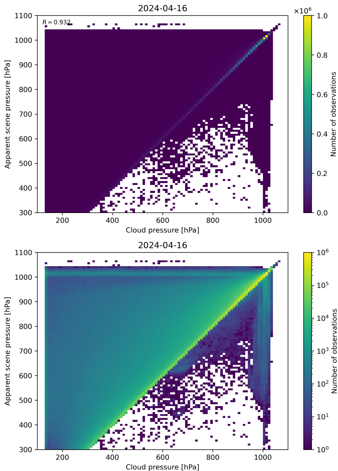
Figure 77: Scatter density plot of “Cloud pressure” against “Apparent scene pressure” for 2024-04-16 to 2024-04-17.
