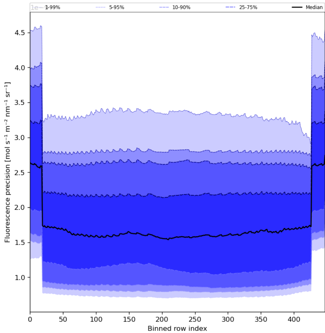
Figure 58: Along track statistics of “Fluorescence precision” for 2024-04-16 to 2024-04-17
