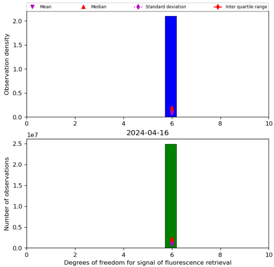
Figure 43: Histogram of “Degrees of freedom for signal of fluorescence retrieval” for 2024-04-16 to 2024-04-17
