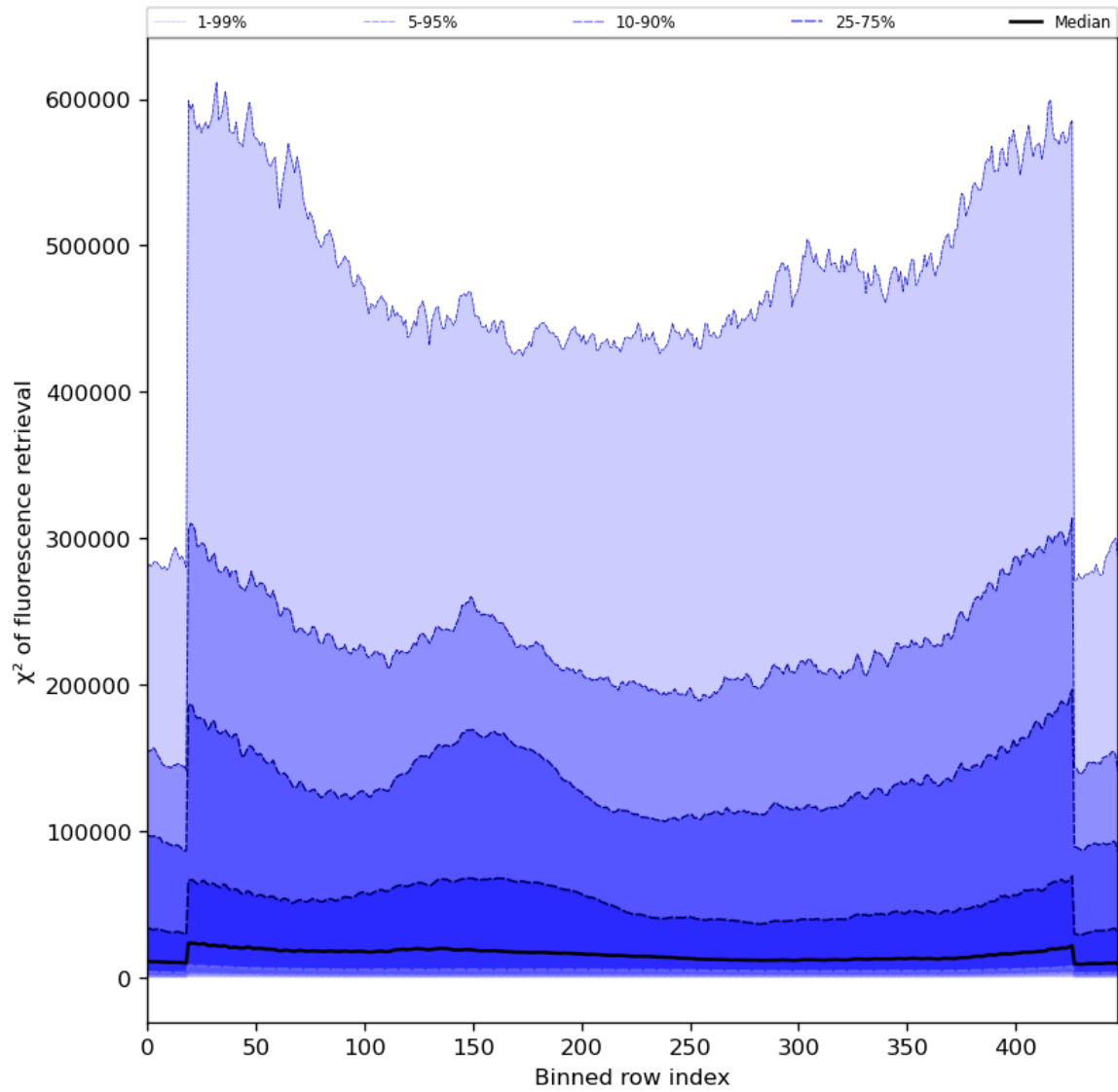
Figure 59: Along track statistics of “ \chi^2 of fluorescence retrieval” for 2024-04-16 to 2024-04-17
