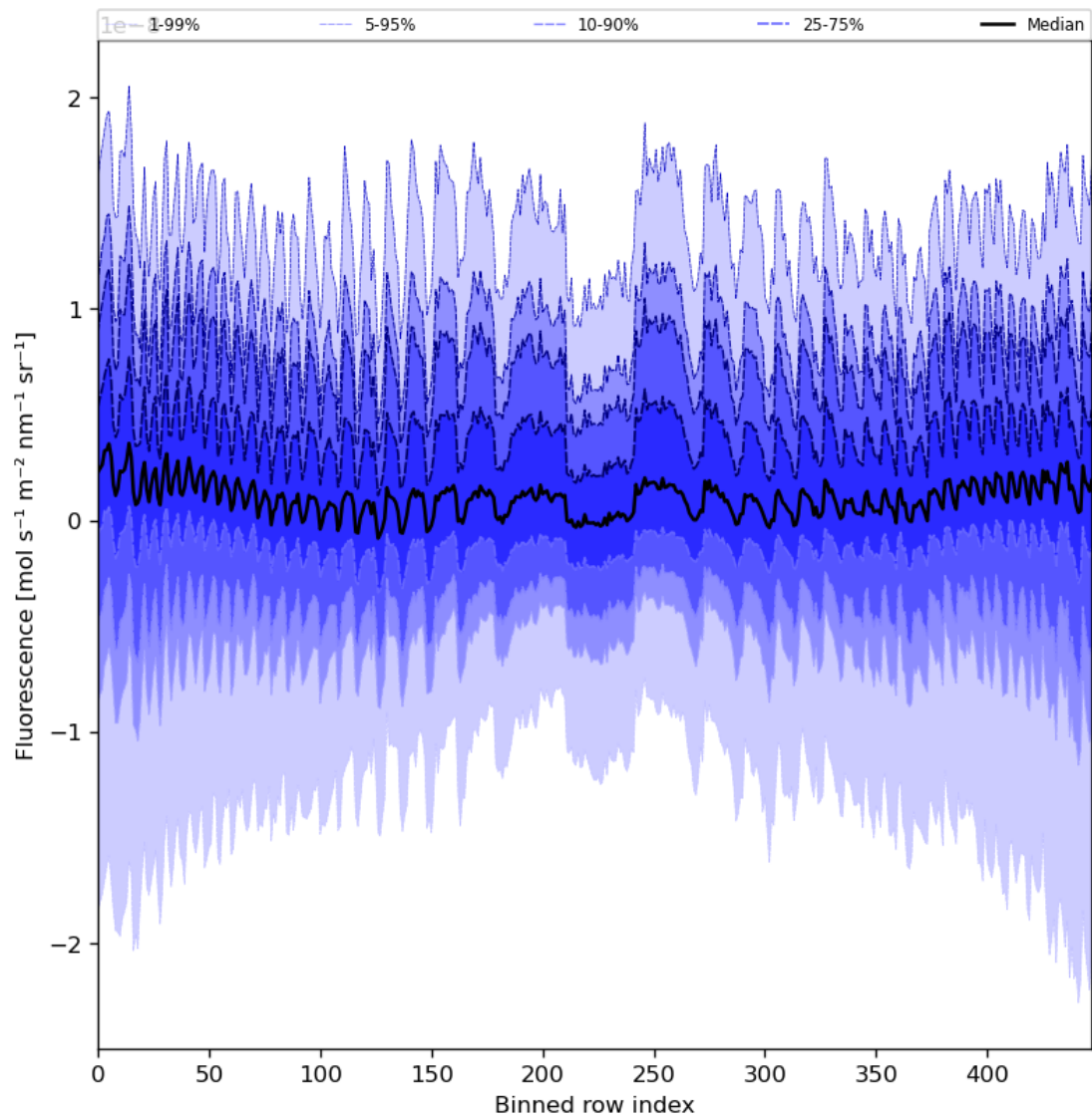
Figure 57: Along track statistics of “Fluorescence” for 2024-04-16 to 2024-04-17
