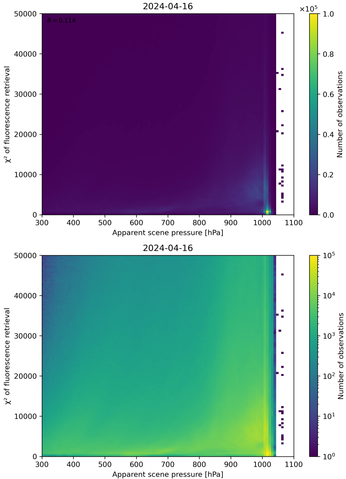
Figure 63: Scatter density plot of “Apparent scene pressure” against “ \chi^2 of fluorescence retrieval” for 2024-04-16 to 2024-04-17.
