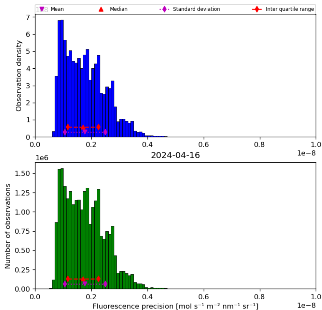
Figure 41: Histogram of “Fluorescence precision” for 2024-04-16 to 2024-04-17
