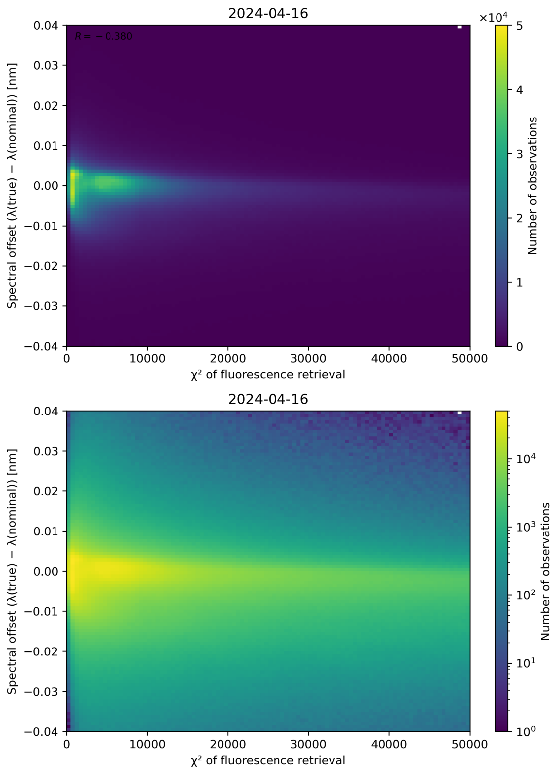
Figure 69: Scatter density plot of " \chi^2 of fluorescence retrieval" against "Spectral offset ( \lambda(\text{true}) - \lambda(\text{nominal}) )" for 2024-04-16 to 2024-04-17.
