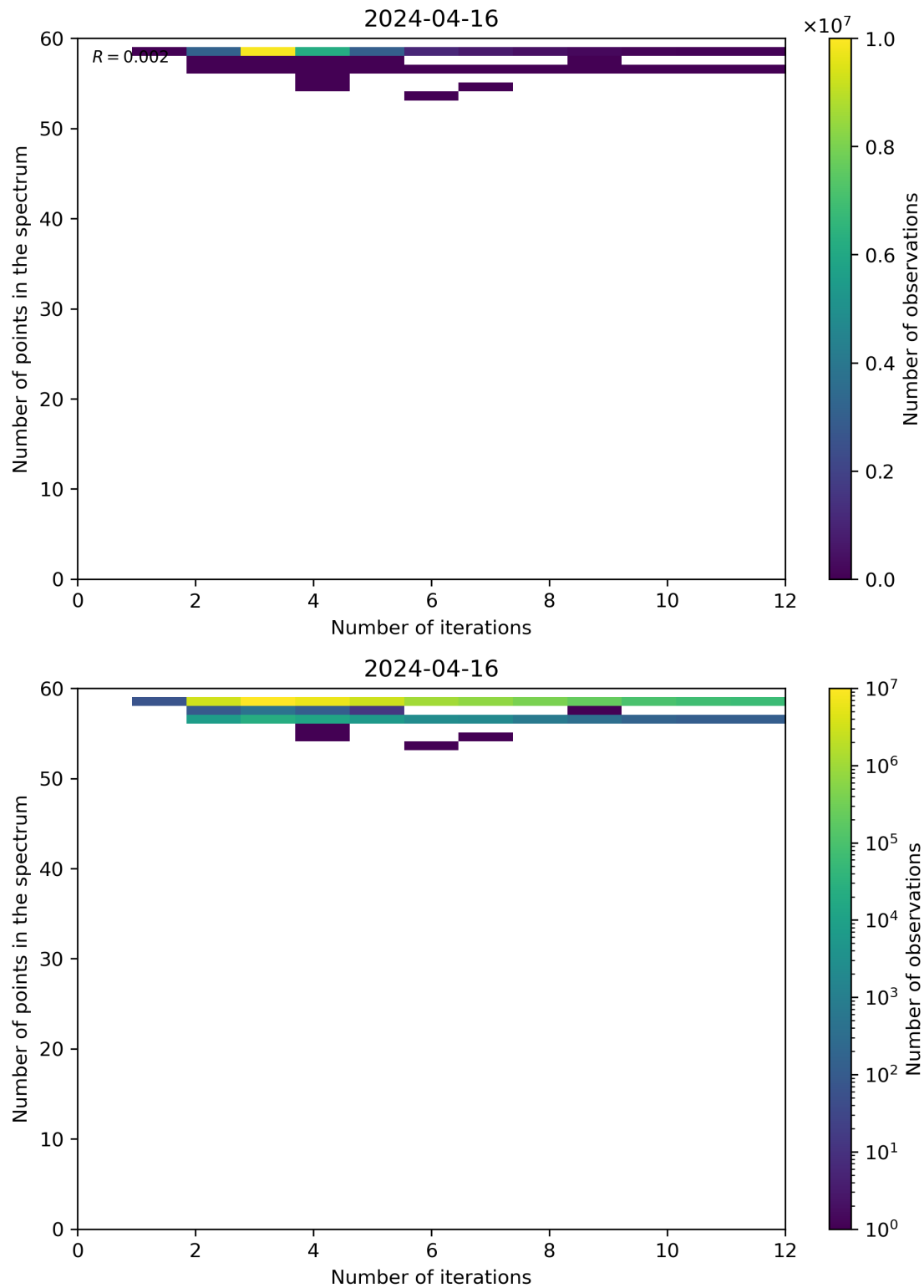
Figure 99: Scatter density plot of “Number of iterations” against “Number of points in the spectrum” for 2024-04-16 to 2024-04-17.
