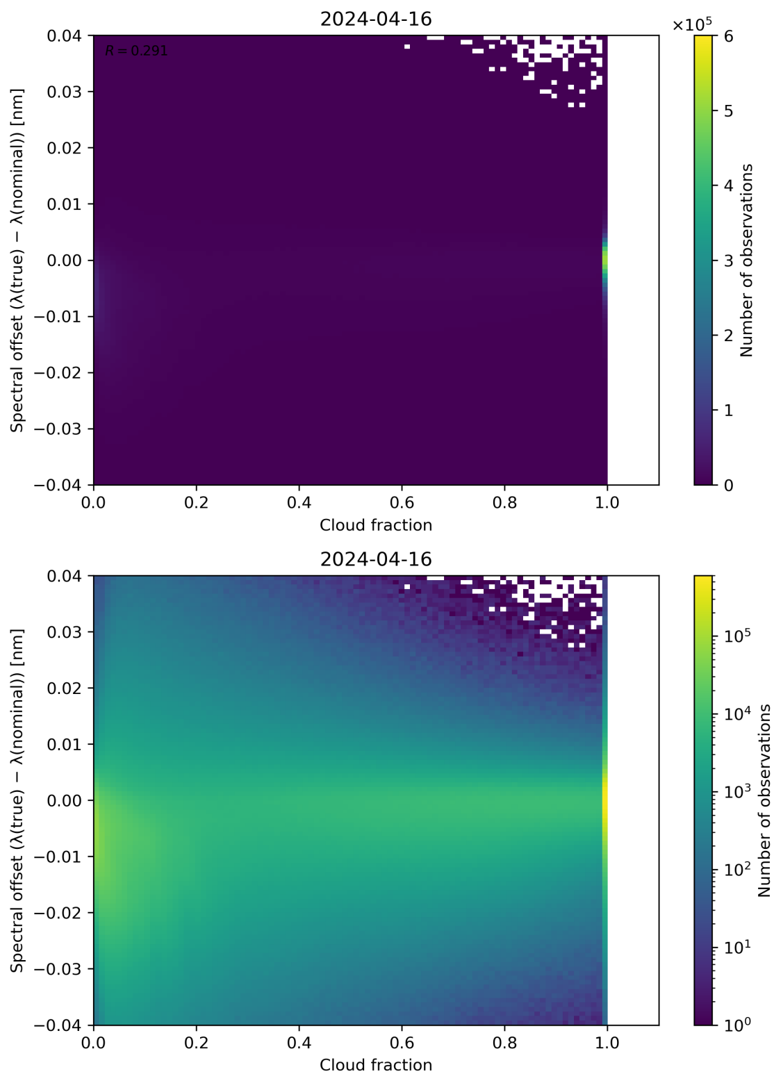
Figure 76: Scatter density plot of “Cloud fraction” against “Spectral offset ( \lambda(\text{true}) - \lambda(\text{nominal}) )” for 2024-04-16 to 2024-04-17.
