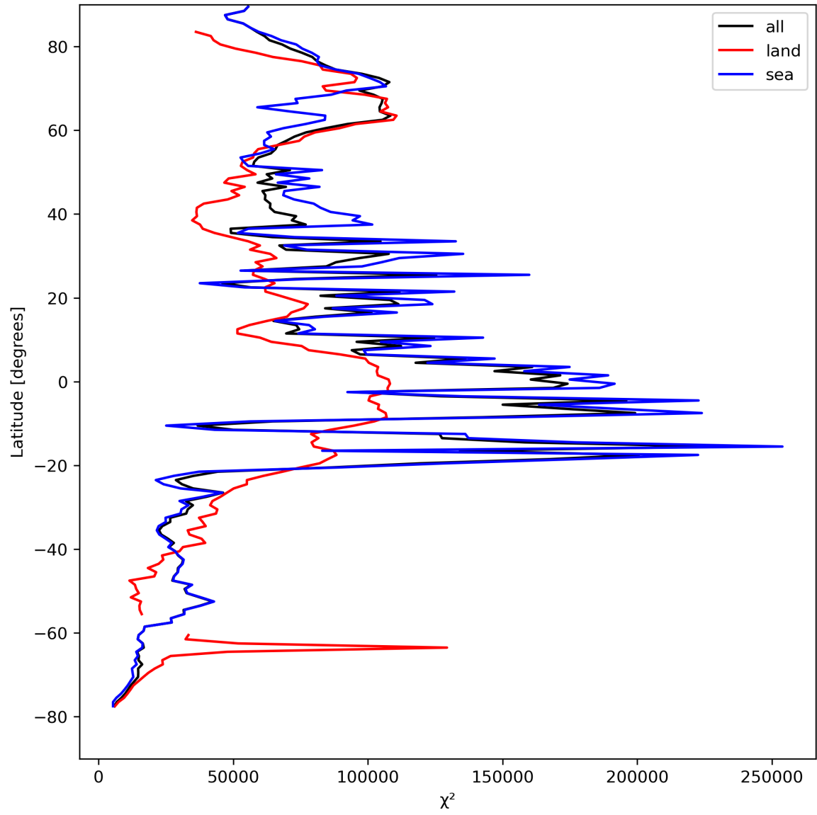
Figure 21: Zonal average of “ \chi^2 ” for 2024-04-16 to 2024-04-17.
