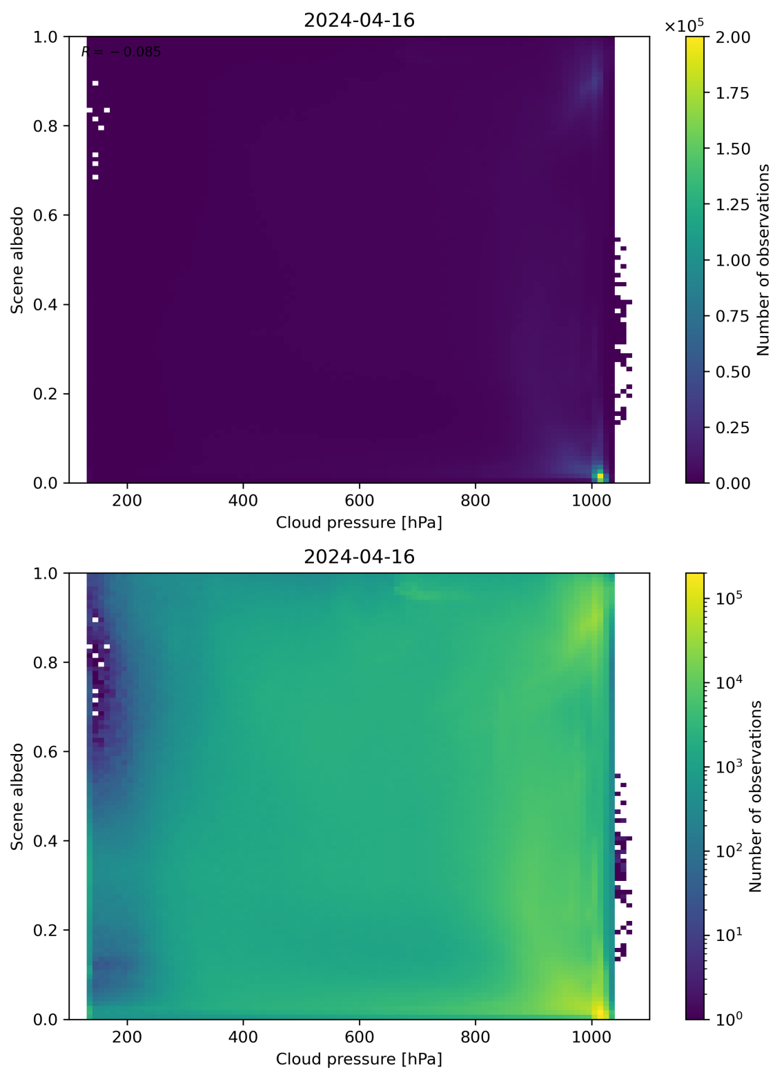
Figure 83: Scatter density plot of “Cloud pressure” against “Scene albedo” for 2024-04-16 to 2024-04-17.
