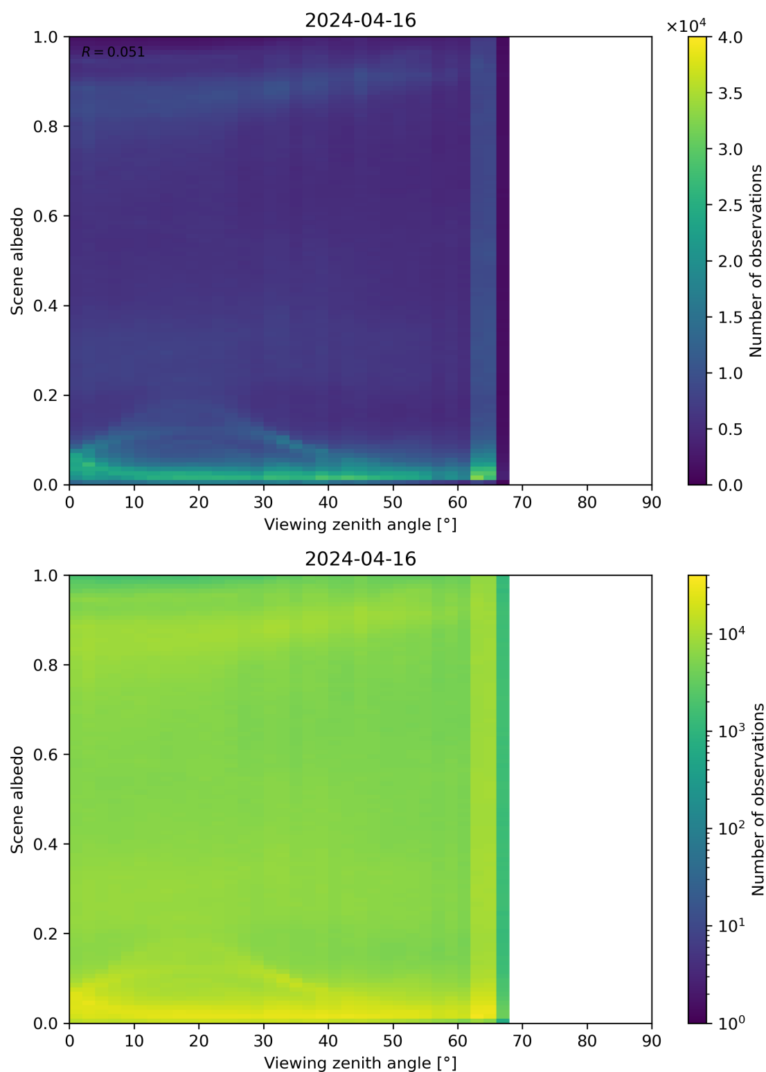
Figure 126: Scatter density plot of “Viewing zenith angle” against “Scene albedo” for 2024-04-16 to 2024-04-17.
