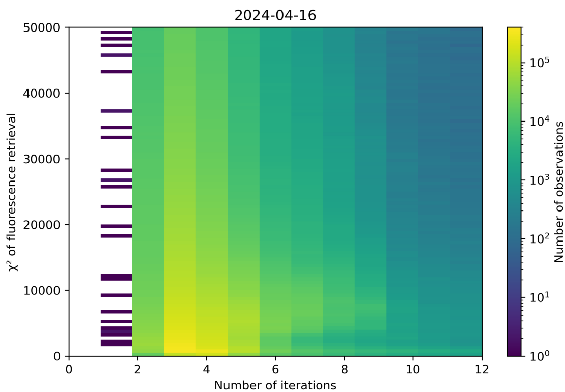
Figure 97: Scatter density plot of “Number of iterations” against “ \chi^2 of fluorescence retrieval” for 2024-04-16 to 2024-04-17.
