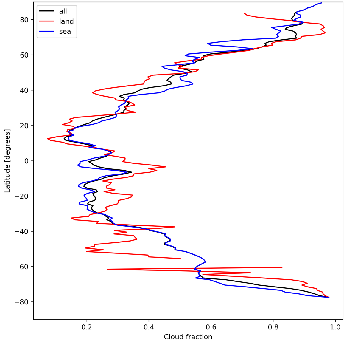
Figure 15: Zonal average of “Cloud fraction” for 2024-04-16 to 2024-04-17.
