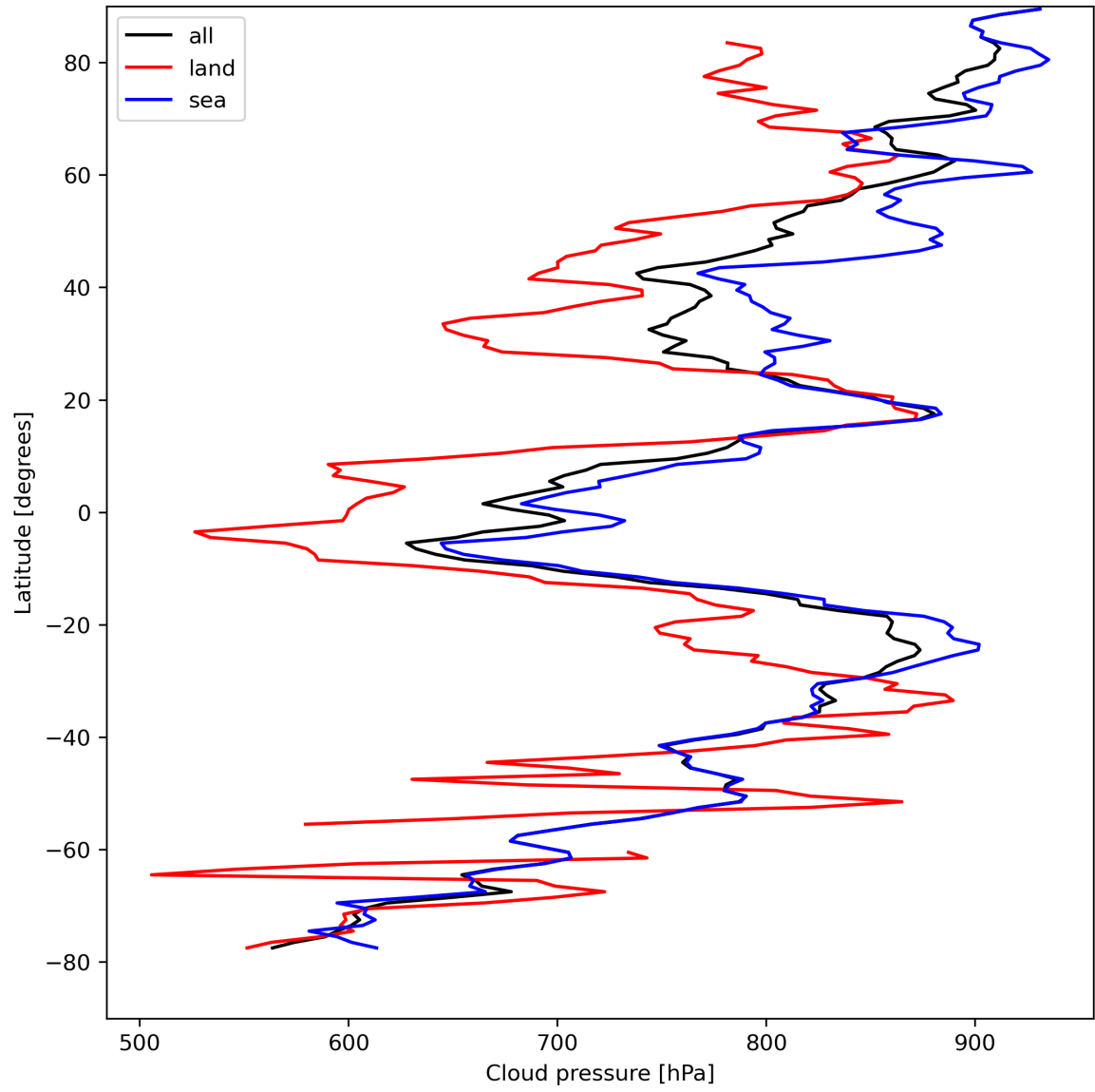
Figure 13: Zonal average of “Cloud pressure” for 2024-04-16 to 2024-04-17.
