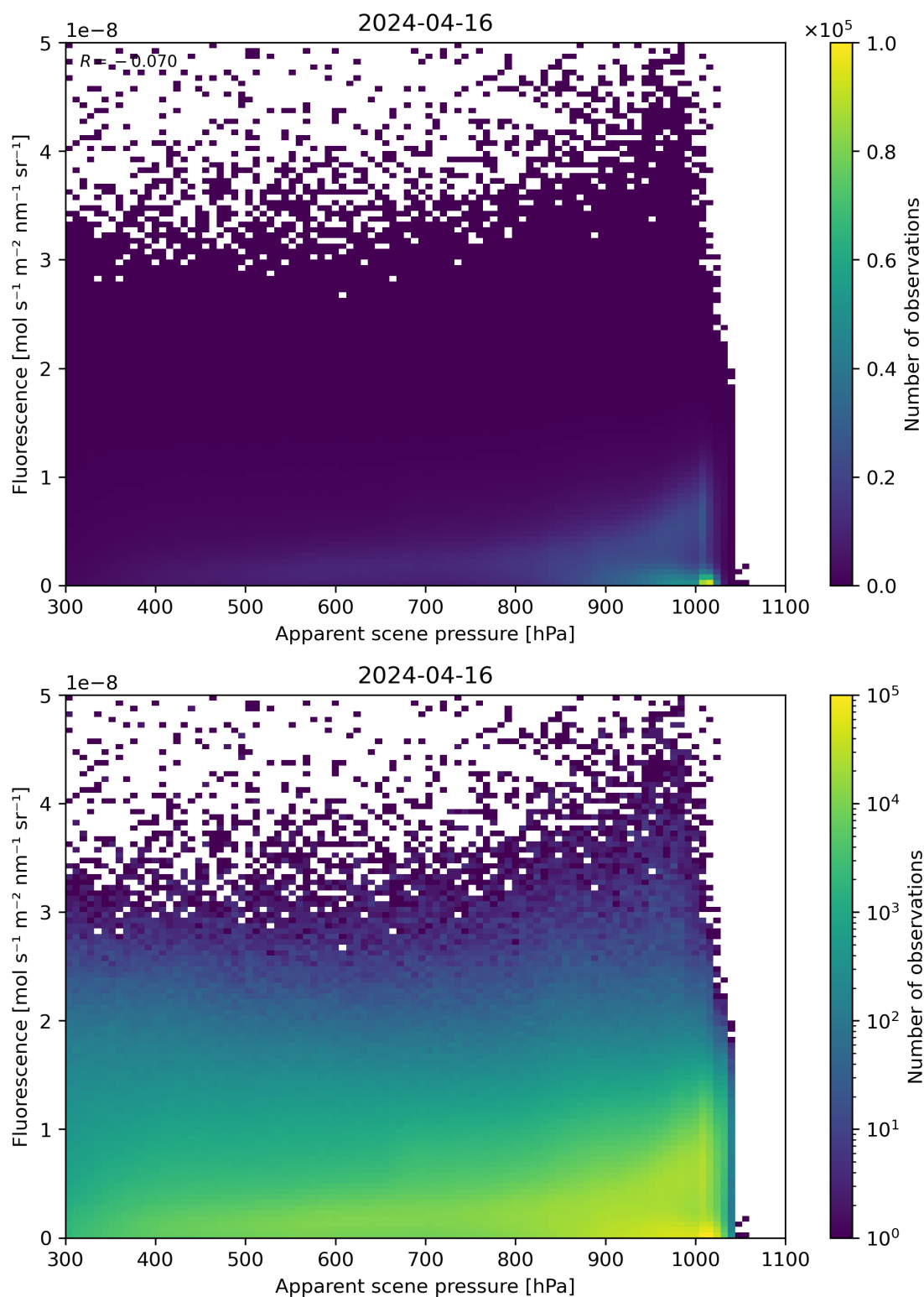
Figure 64: Scatter density plot of “Apparent scene pressure” against “Fluorescence” for 2024-04-16 to 2024-04-17.
