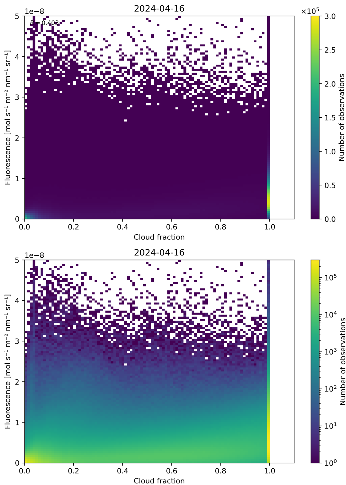
Figure 72: Scatter density plot of “Cloud fraction” against “Fluorescence” for 2024-04-16 to 2024-04-17.
