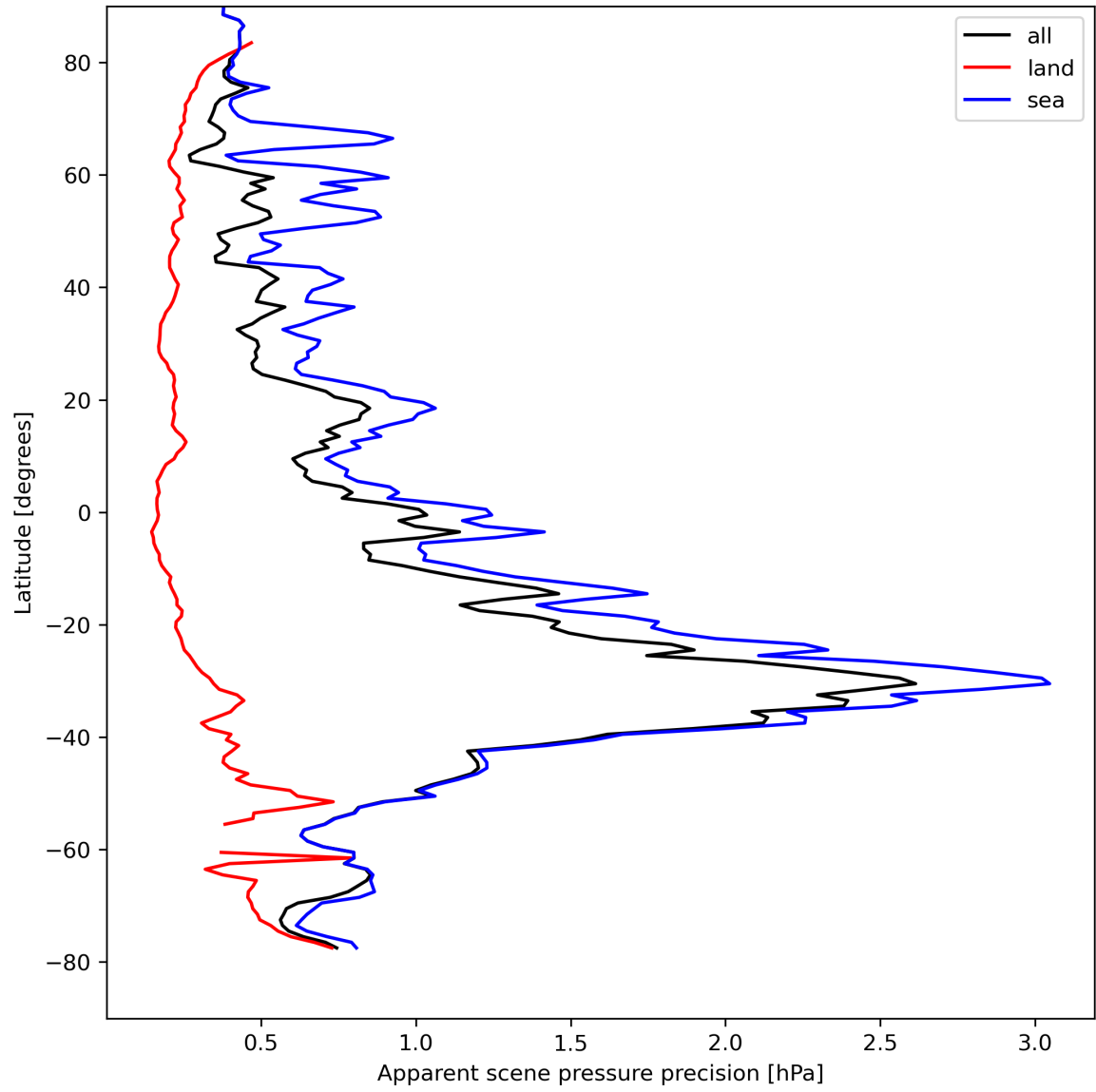
Figure 20: Zonal average of “Apparent scene pressure precision” for 2024-04-16 to 2024-04-17.
