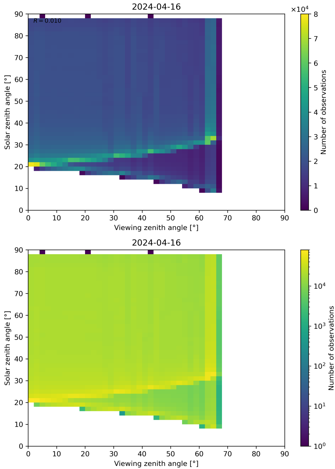
Figure 127: Scatter density plot of “Viewing zenith angle” against “Solar zenith angle” for 2024-04-16 to 2024-04-17.
