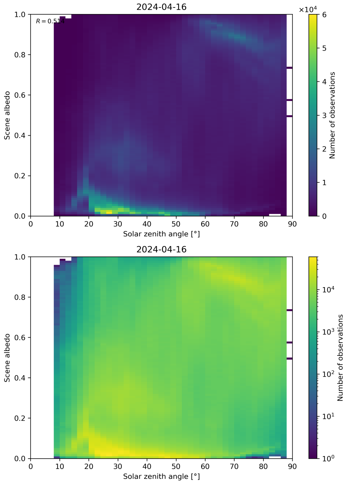
Figure 116: Scatter density plot of “Solar zenith angle” against “Scene albedo” for 2024-04-16 to 2024-04-17.
