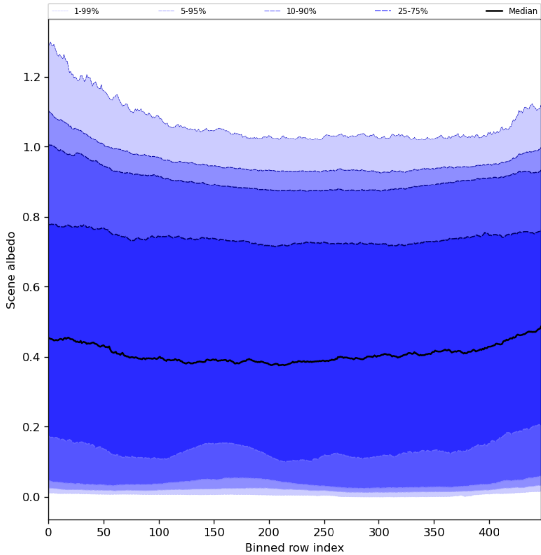
Figure 51: Along track statistics of “Scene albedo” for 2024-04-16 to 2024-04-17
