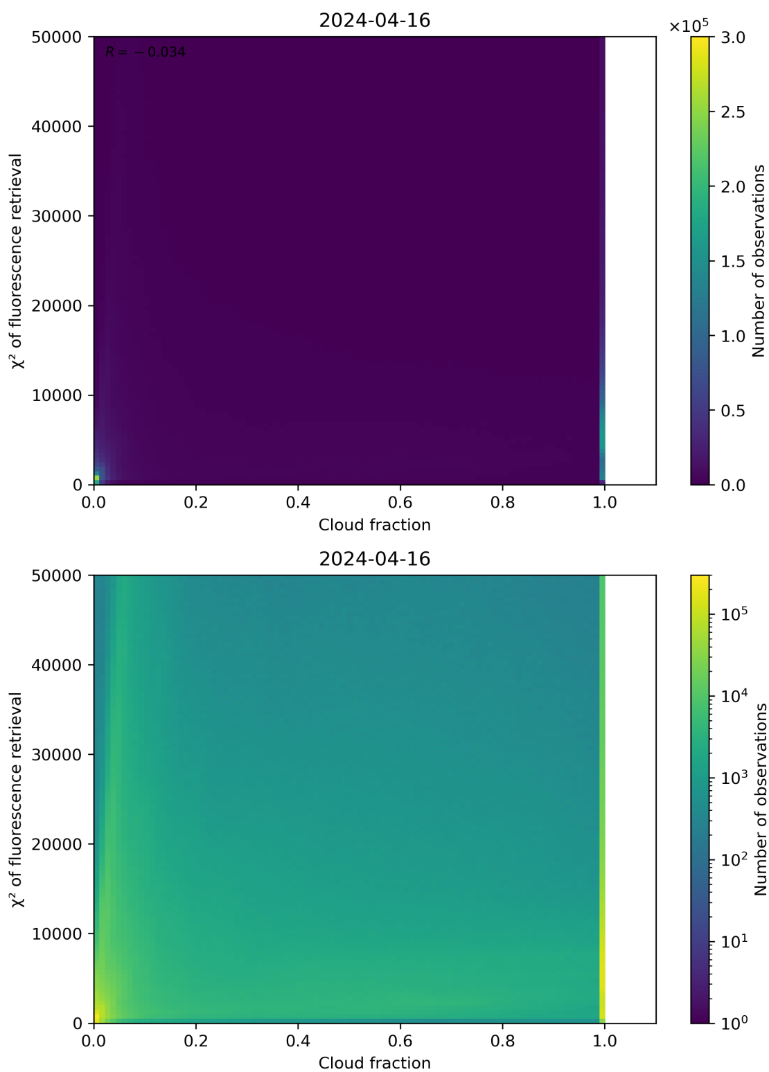
Figure 71: Scatter density plot of “Cloud fraction” against “ \chi^2 of fluorescence retrieval” for 2024-04-16 to 2024-04-17.
