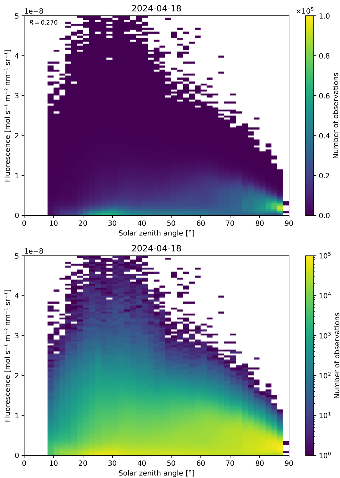
Figure 112: Scatter density plot of “Solar zenith angle” against “Fluorescence” for 2024-04-17 to 2024-04-19.
