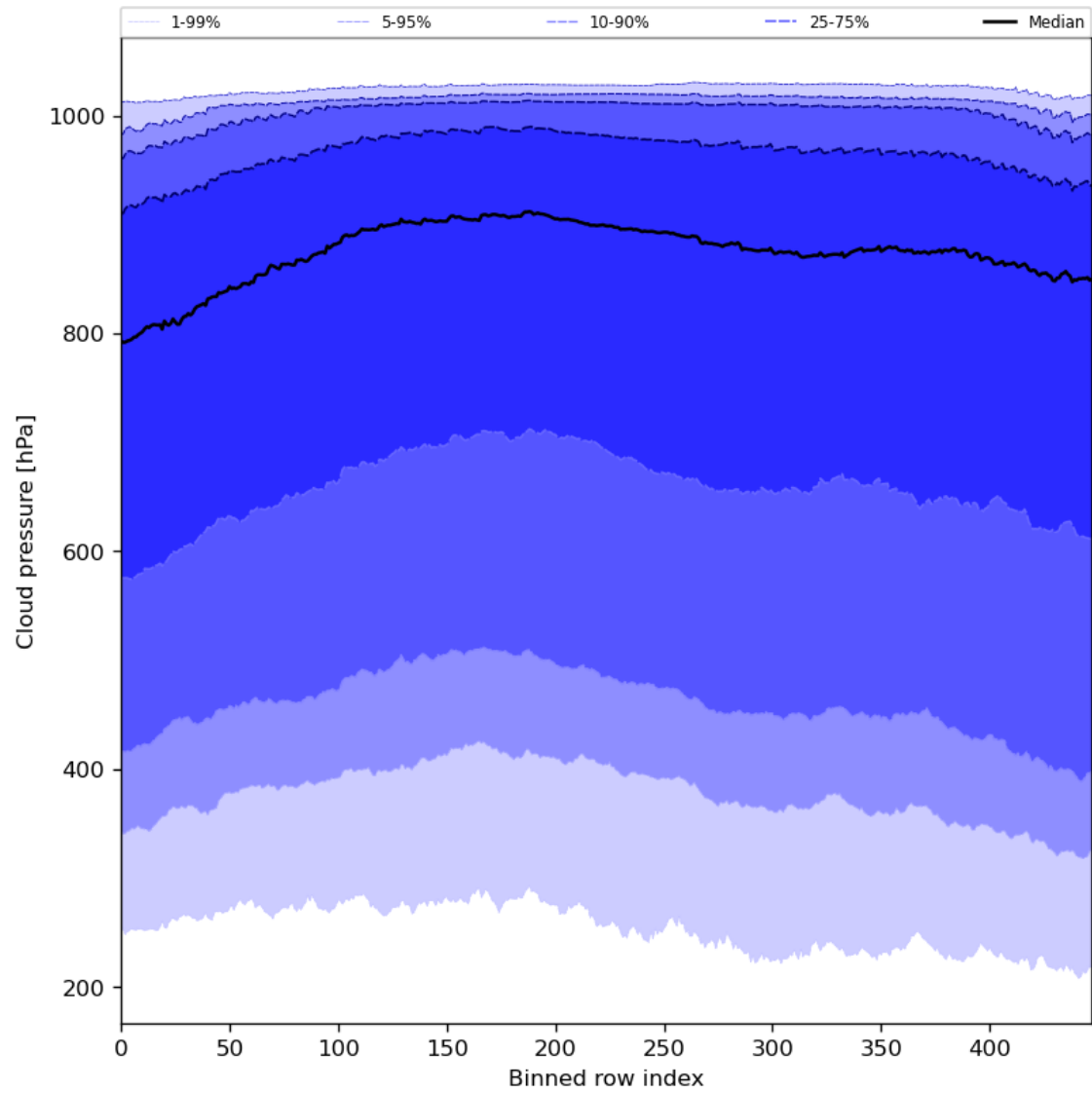
Figure 47: Along track statistics of “Cloud pressure” for 2024-04-17 to 2024-04-19
