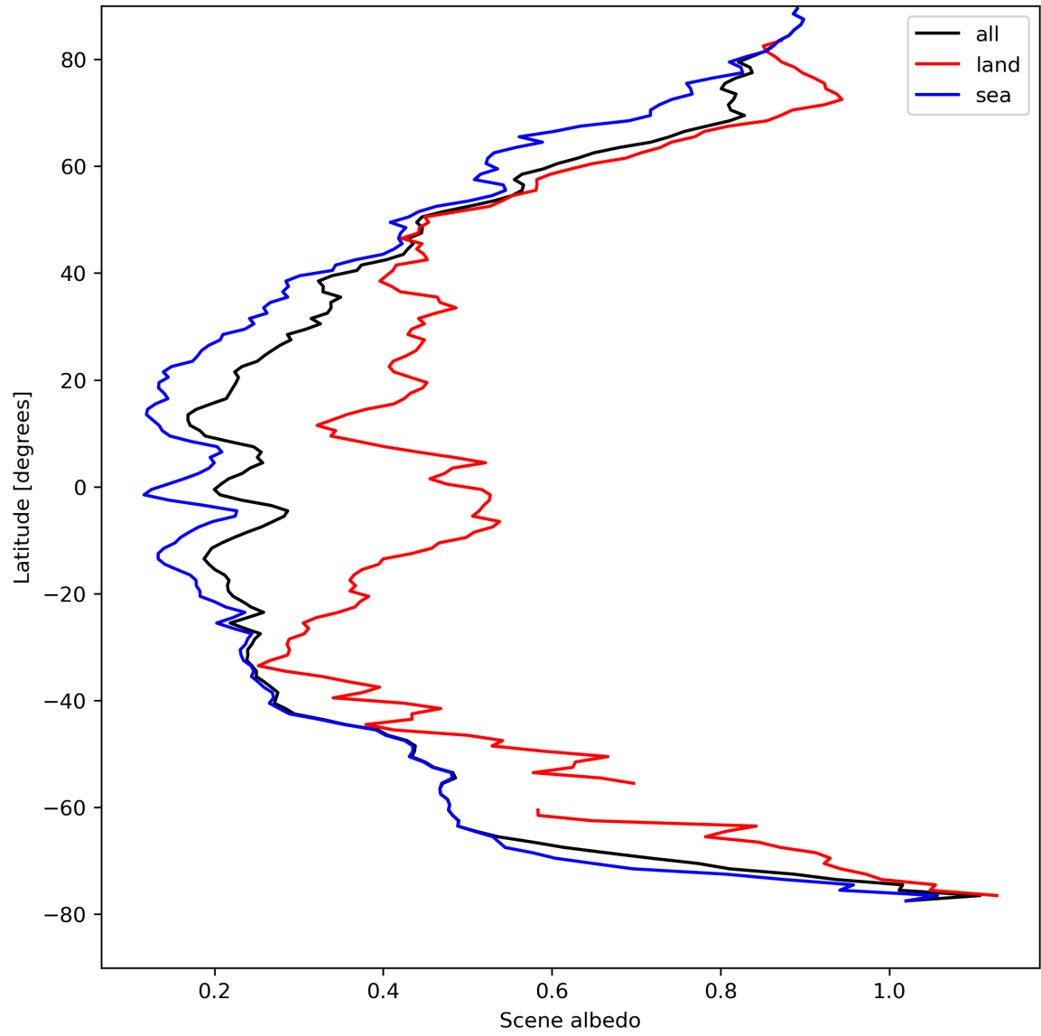
Figure 17: Zonal average of “Scene albedo” for 2024-04-17 to 2024-04-19.
