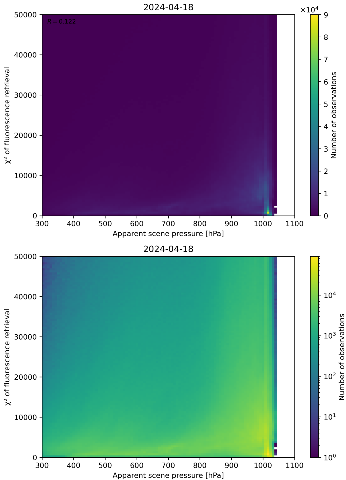
Figure 63: Scatter density plot of “Apparent scene pressure” against “ \chi^2 of fluorescence retrieval” for 2024-04-17 to 2024-04-19.
