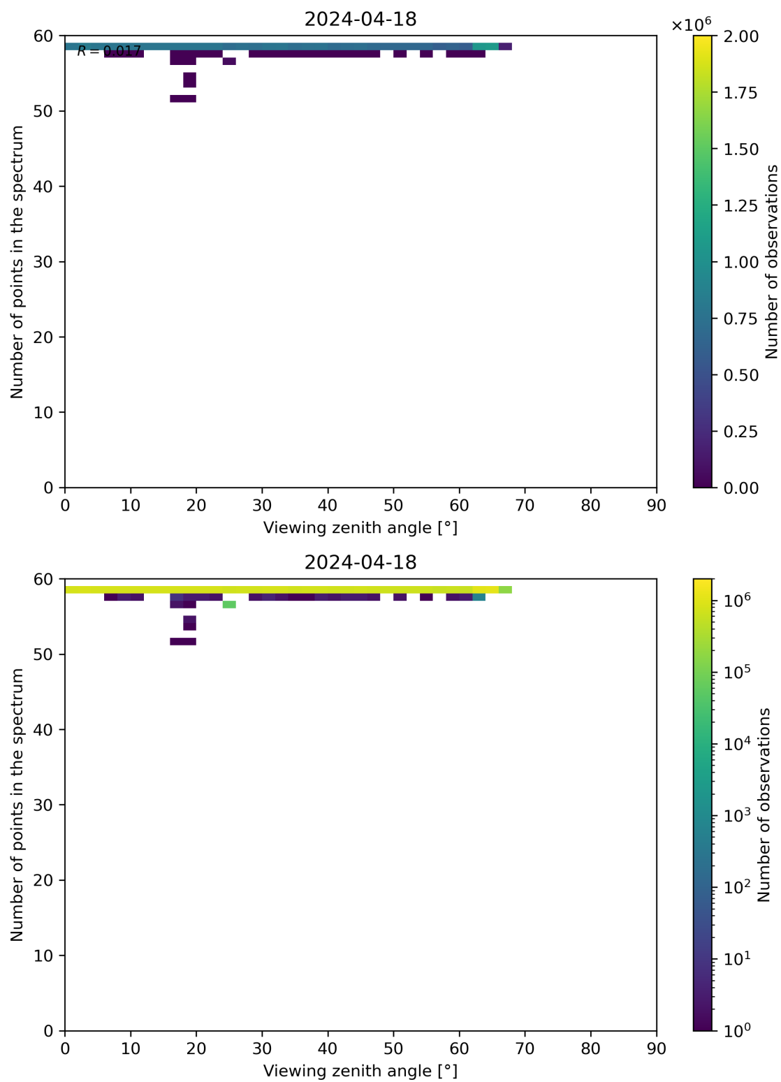
Figure 125: Scatter density plot of “Viewing zenith angle” against “Number of points in the spectrum” for 2024-04-17 to 2024-04-19.
