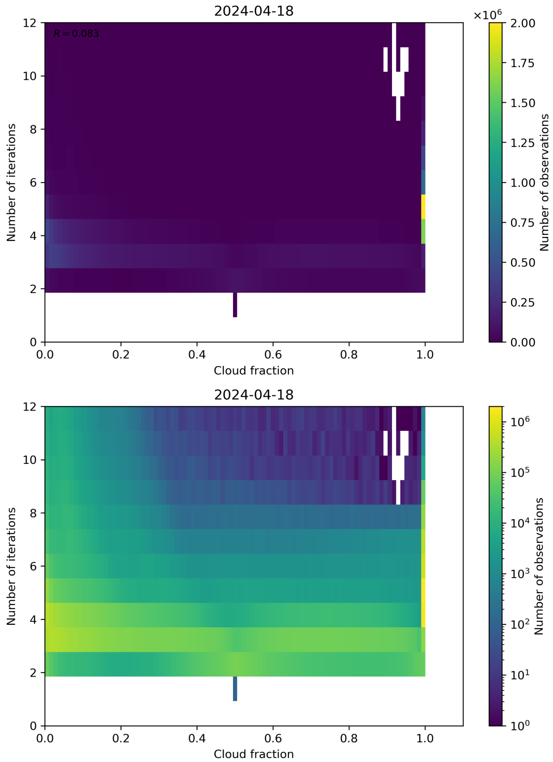
Figure 73: Scatter density plot of “Cloud fraction” against “Number of iterations” for 2024-04-17 to 2024-04-19.
