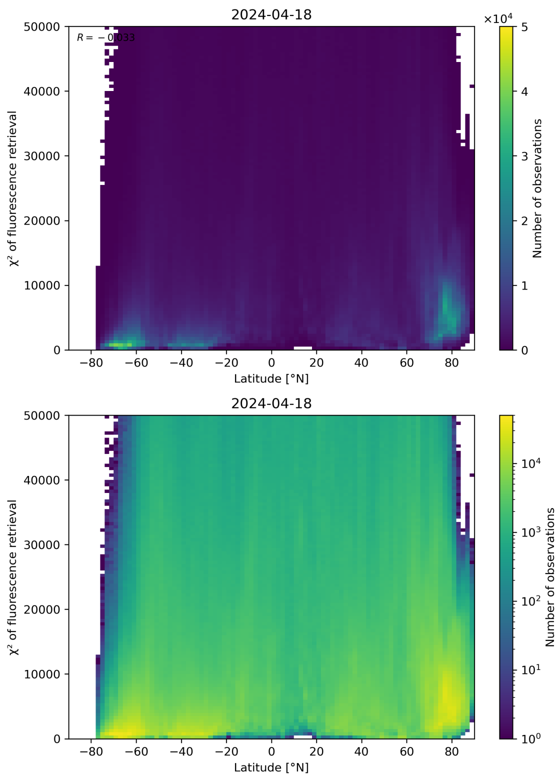
Figure 89: Scatter density plot of “Latitude” against “ \chi^2 of fluorescence retrieval” for 2024-04-17 to 2024-04-19.
