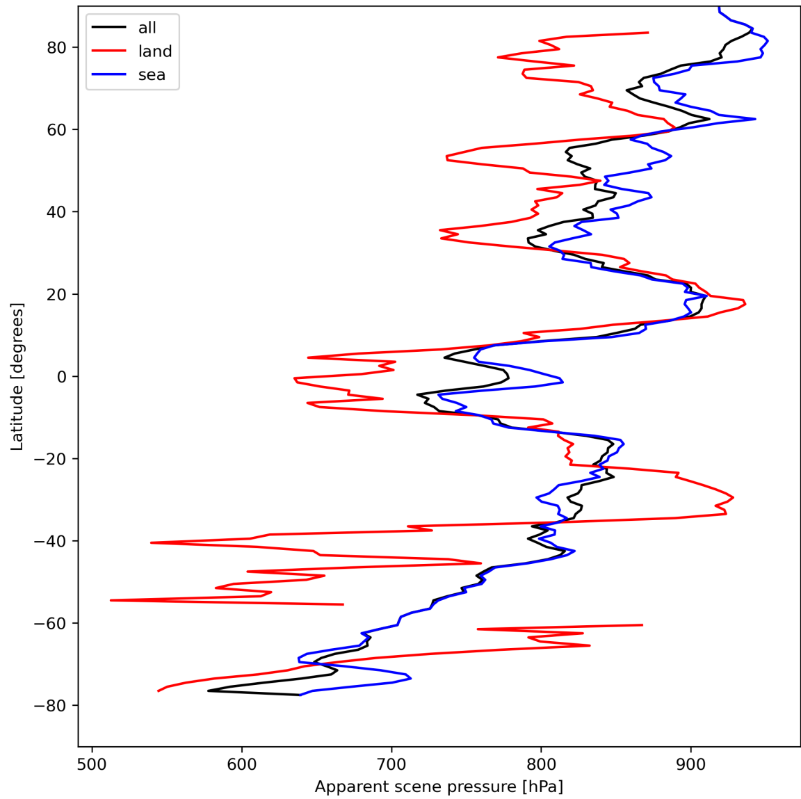
Figure 19: Zonal average of “Apparent scene pressure” for 2024-04-17 to 2024-04-19.
