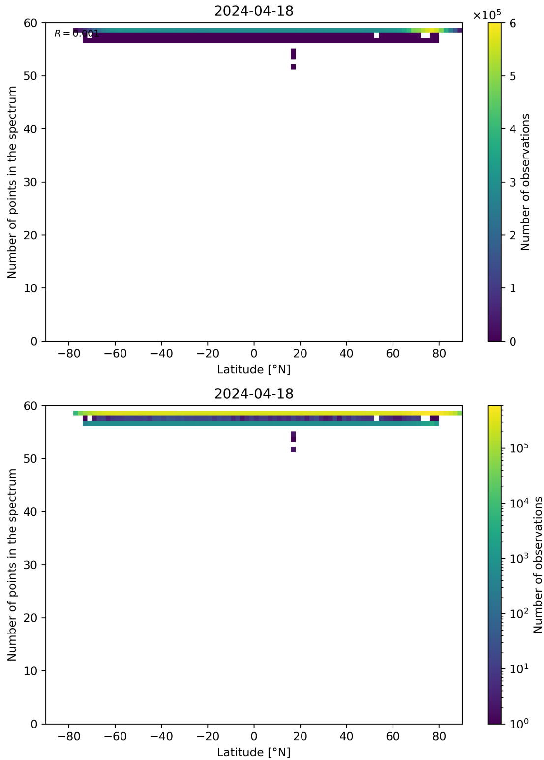
Figure 94: Scatter density plot of “Latitude” against “Number of points in the spectrum” for 2024-04-17 to 2024-04-19.
