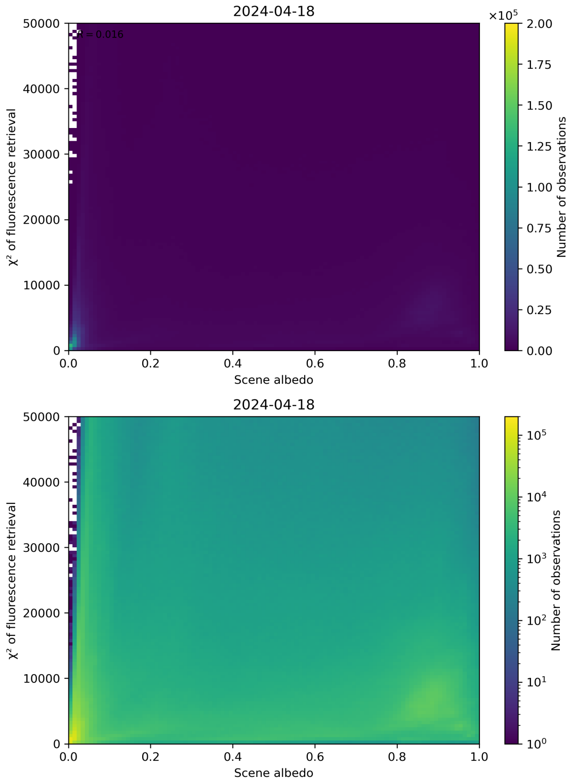
Figure 103: Scatter density plot of “Scene albedo” against “ \chi^2 of fluorescence retrieval” for 2024-04-17 to 2024-04-19.
