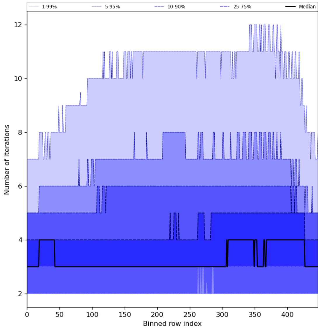
Figure 56: Along track statistics of “Number of iterations” for 2024-04-17 to 2024-04-19
