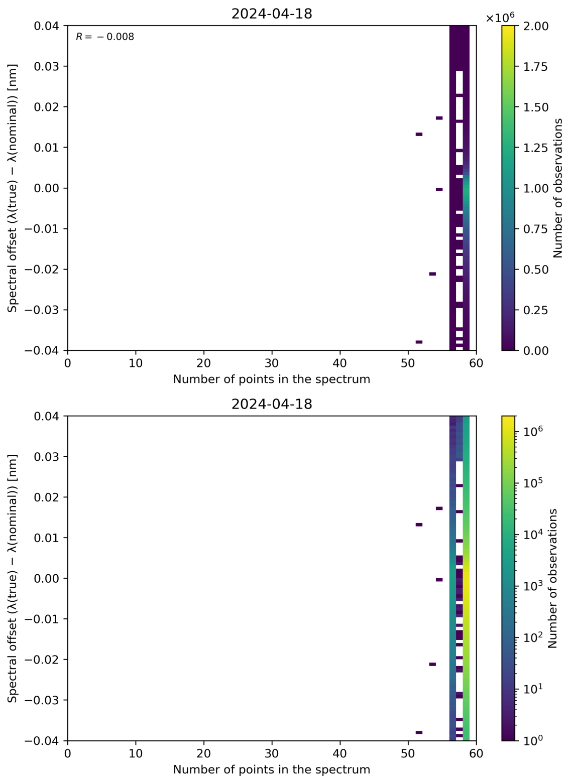
Figure 101: Scatter density plot of “Number of points in the spectrum” against “Spectral offset ( \lambda(\text{true}) - \lambda(\text{nominal}) )” for 2024-04-17 to 2024-04-19.
