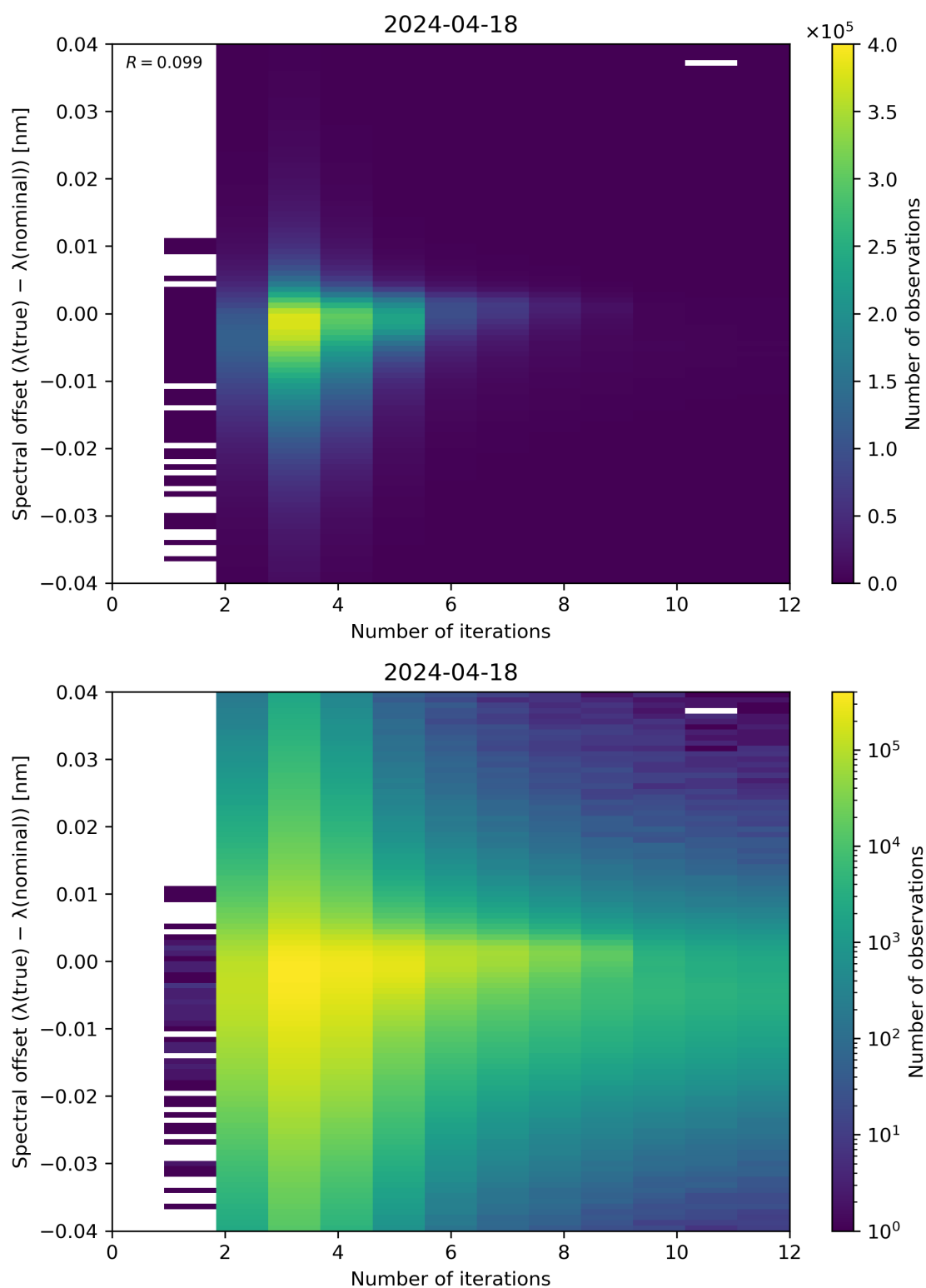
Figure 100: Scatter density plot of “Number of iterations” against “Spectral offset ( \lambda(\text{true}) - \lambda(\text{nominal}) )” for 2024-04-17 to 2024-04-19.
