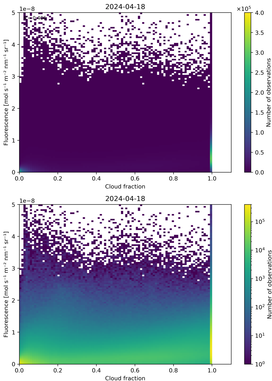
Figure 72: Scatter density plot of “Cloud fraction” against “Fluorescence” for 2024-04-17 to 2024-04-19.
