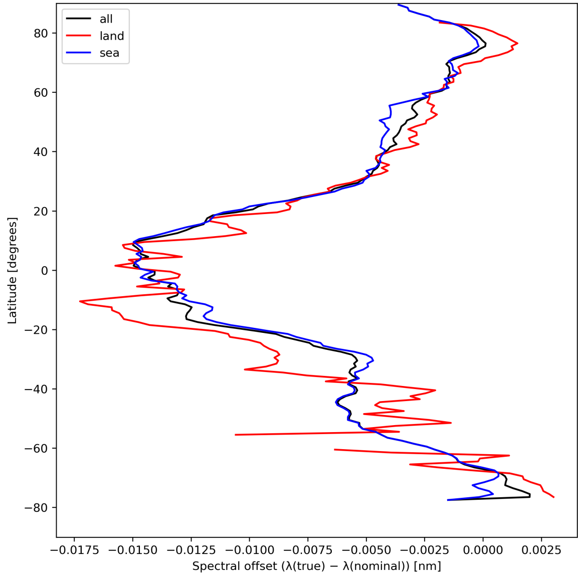
Figure 28: Zonal average of “Spectral offset ( \lambda(\text{true}) - \lambda(\text{nominal}) )” for 2024-04-17 to 2024-04-19.
