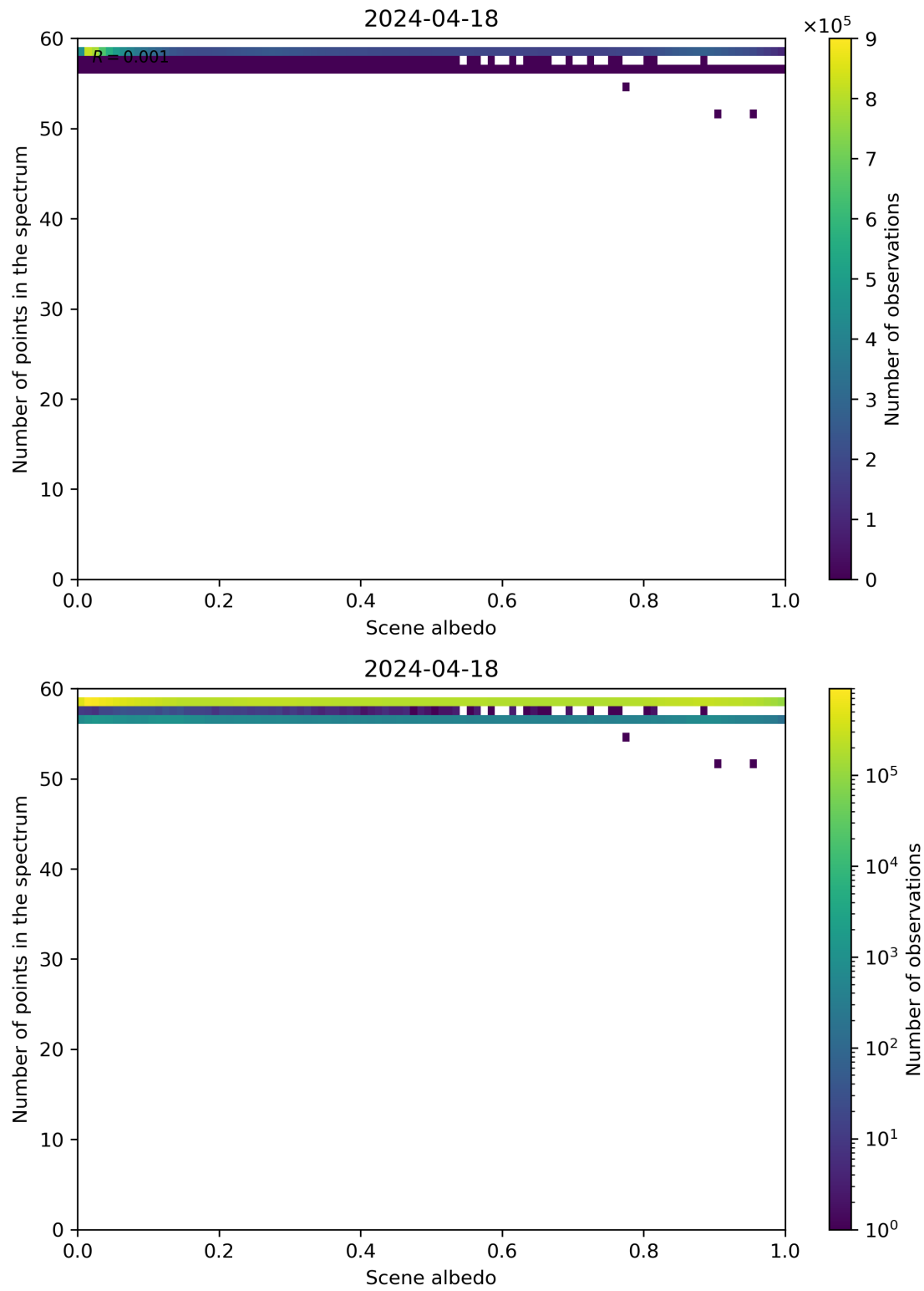
Figure 106: Scatter density plot of “Scene albedo” against “Number of points in the spectrum” for 2024-04-17 to 2024-04-19.
