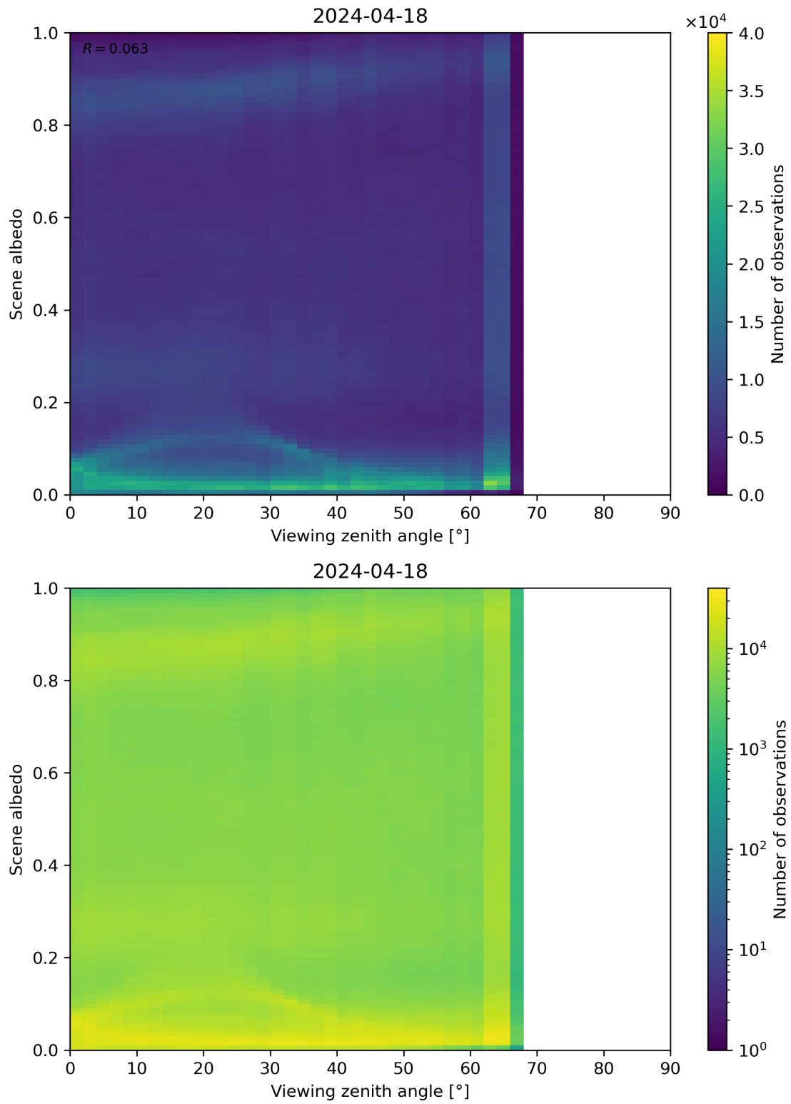
Figure 126: Scatter density plot of “Viewing zenith angle” against “Scene albedo” for 2024-04-17 to 2024-04-19.
