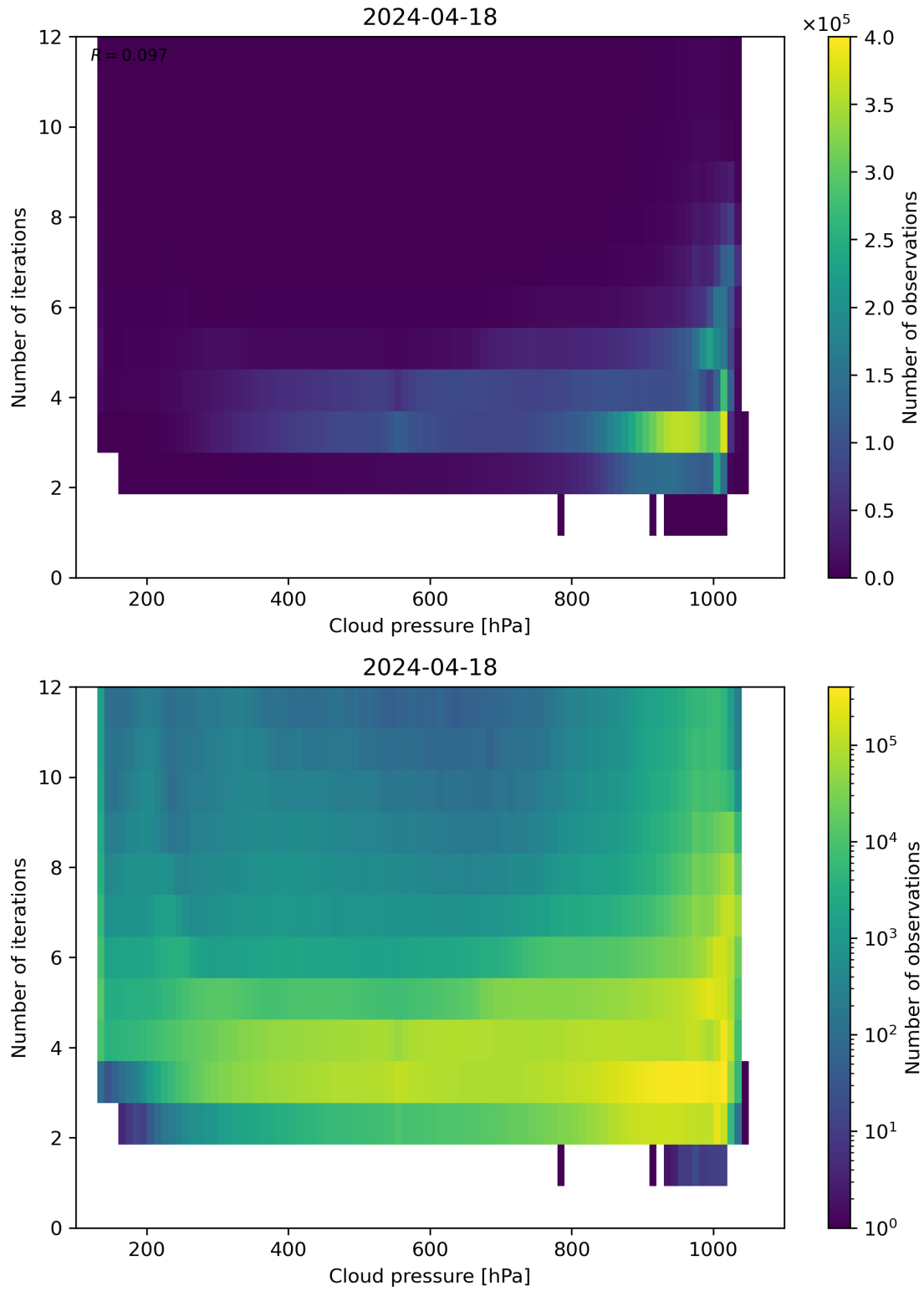
Figure 81: Scatter density plot of “Cloud pressure” against “Number of iterations” for 2024-04-17 to 2024-04-19.
