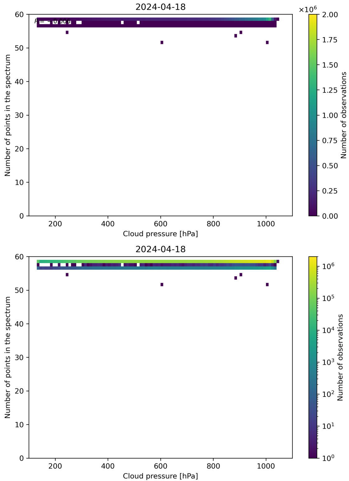
Figure 82: Scatter density plot of “Cloud pressure” against “Number of points in the spectrum” for 2024-04-17 to 2024-04-19.
