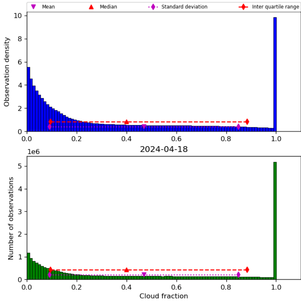
Figure 32: Histogram of “Cloud fraction” for 2024-04-17 to 2024-04-19
