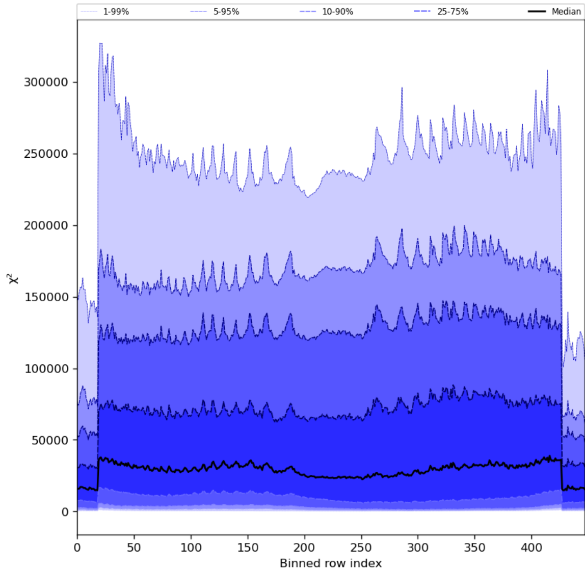
Figure 55: Along track statistics of “ \chi^2 ” for 2024-04-17 to 2024-04-19
