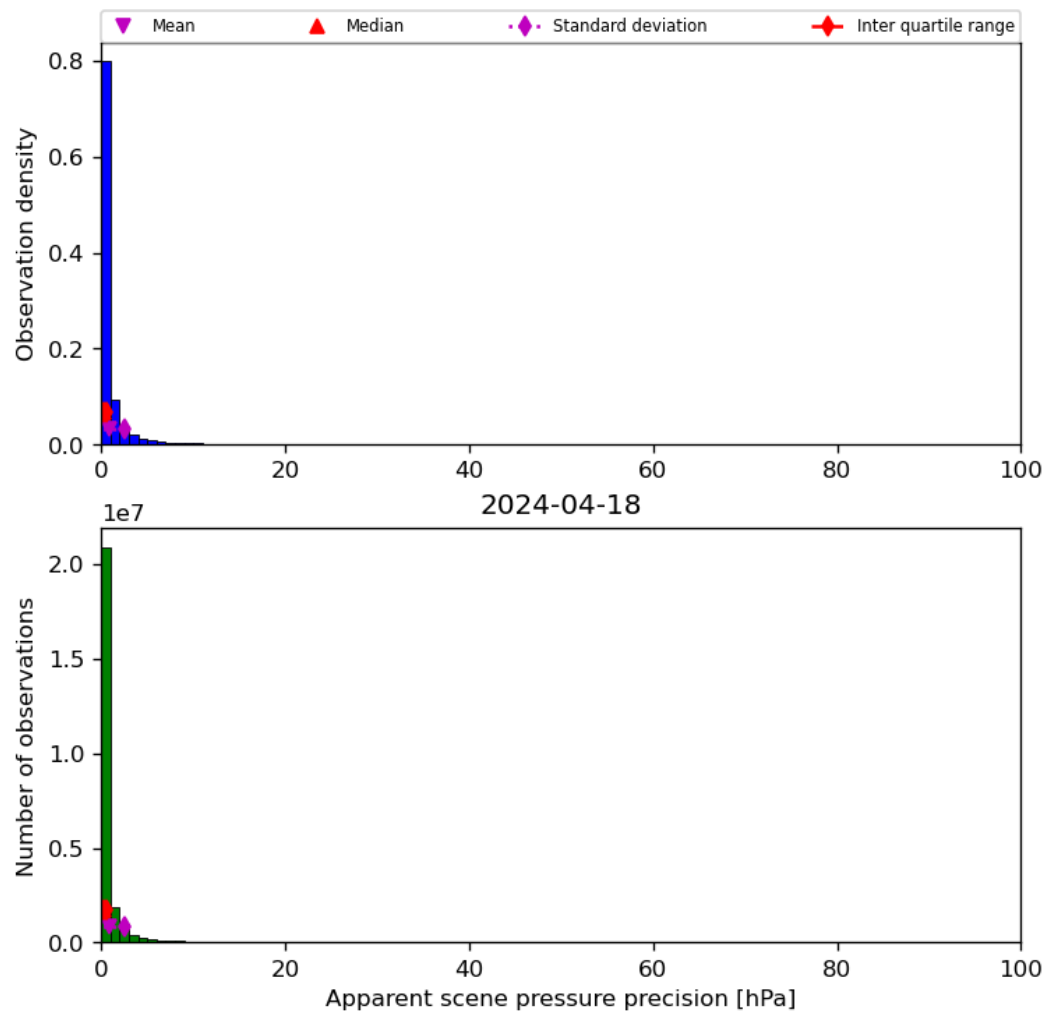
Figure 37: Histogram of “Apparent scene pressure precision” for 2024-04-17 to 2024-04-19
