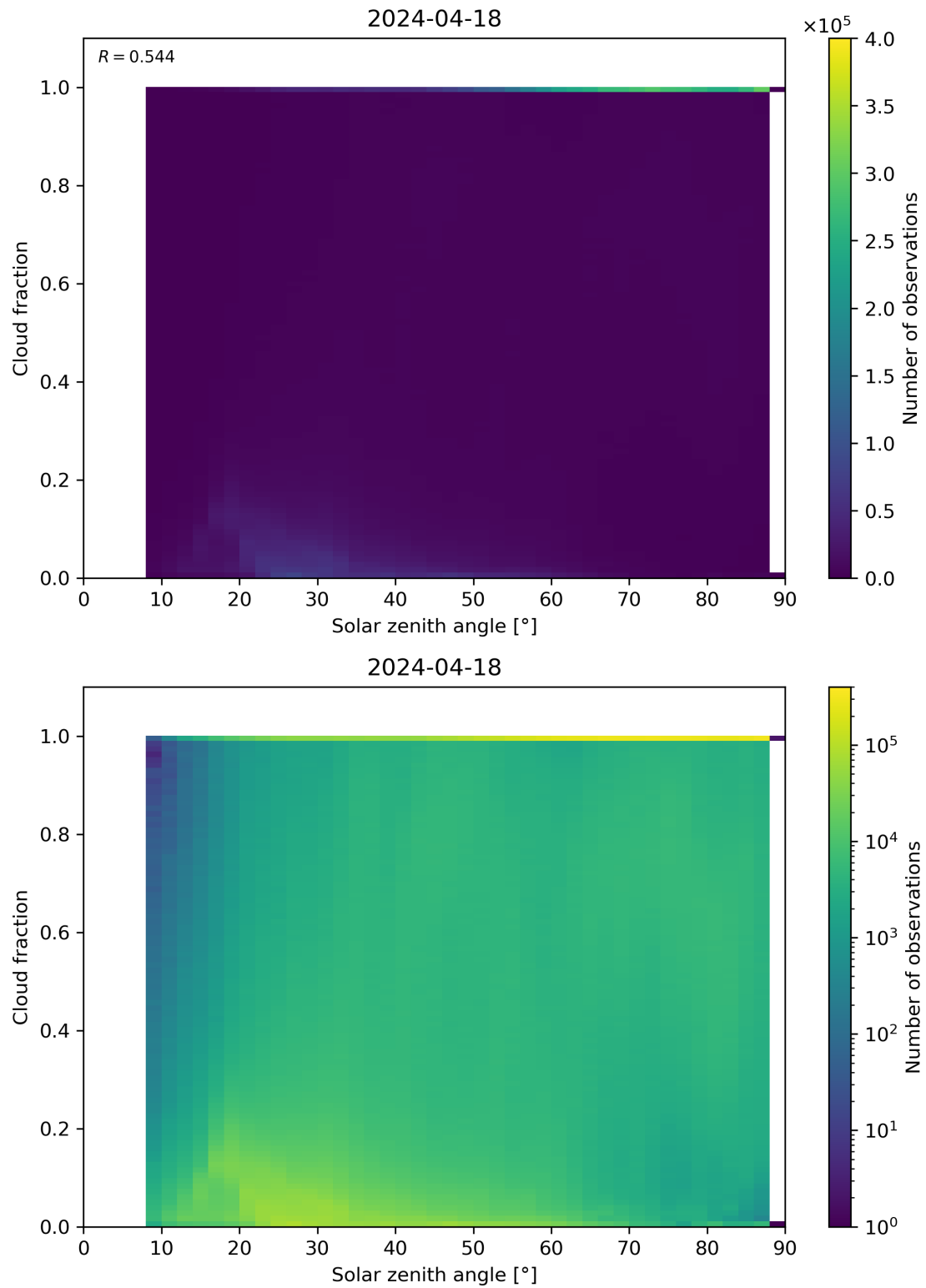
Figure 110: Scatter density plot of “Solar zenith angle” against “Cloud fraction” for 2024-04-17 to 2024-04-19.
