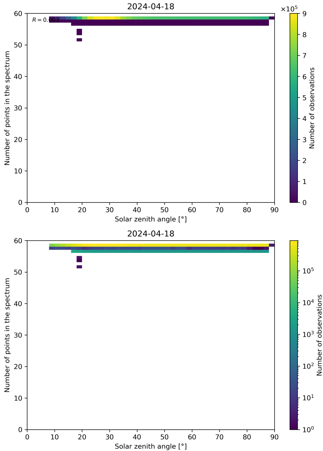
Figure 115: Scatter density plot of “Solar zenith angle” against “Number of points in the spectrum” for 2024-04-17 to 2024-04-19.
