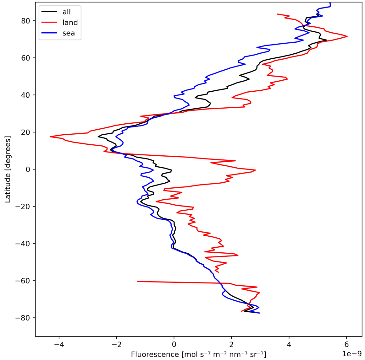
Figure 23: Zonal average of “Fluorescence” for 2024-04-17 to 2024-04-19.
