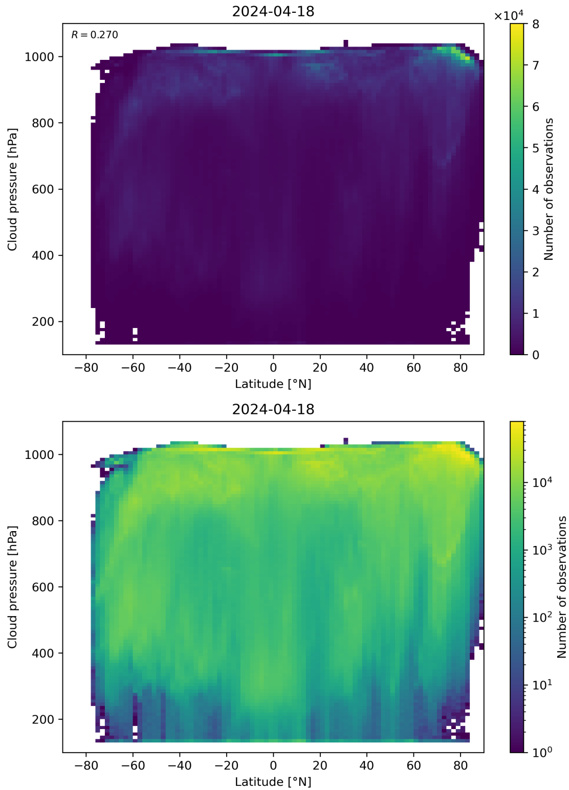
Figure 91: Scatter density plot of “Latitude” against “Cloud pressure” for 2024-04-17 to 2024-04-19.
