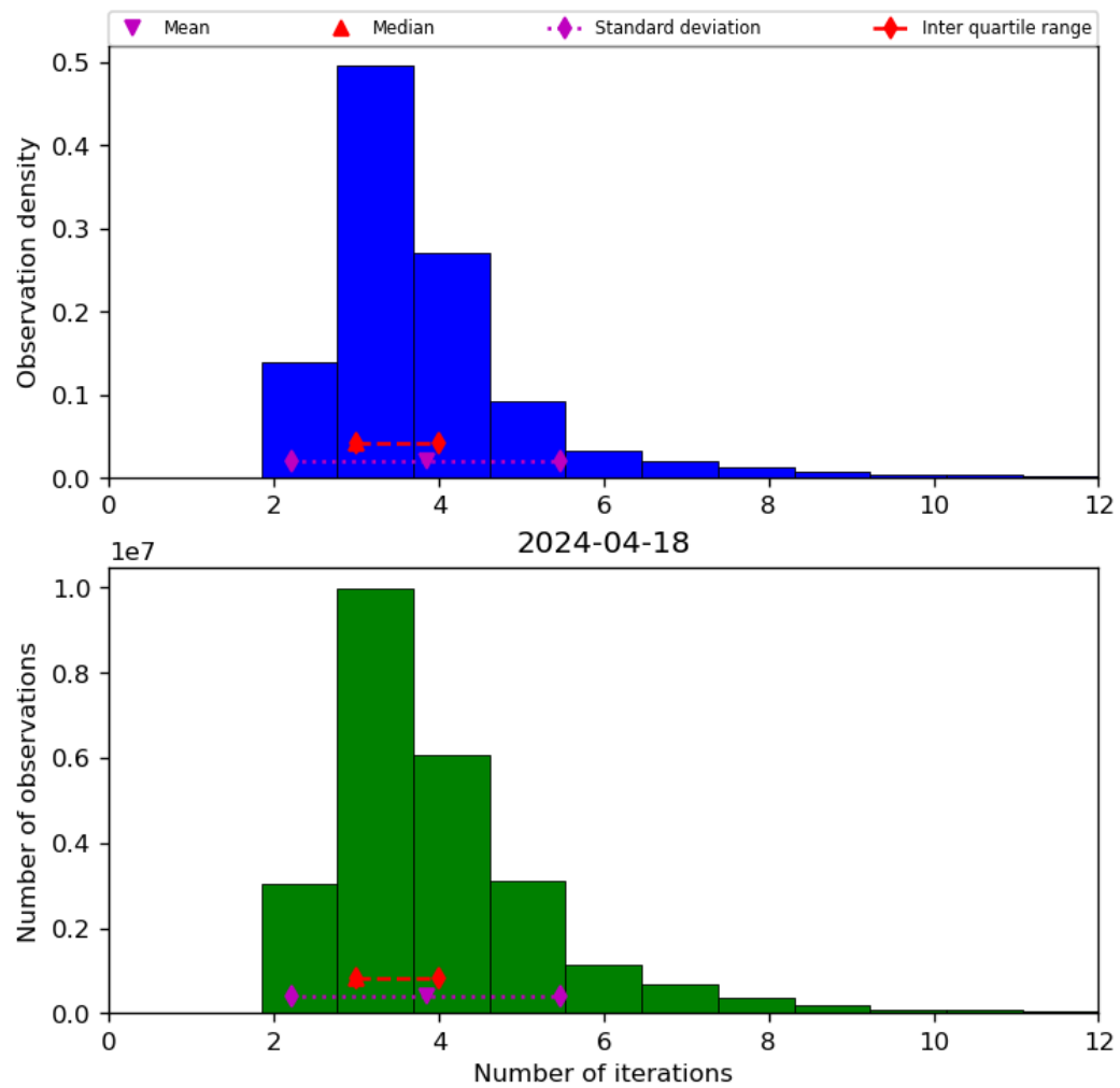
Figure 39: Histogram of “Number of iterations” for 2024-04-17 to 2024-04-19
