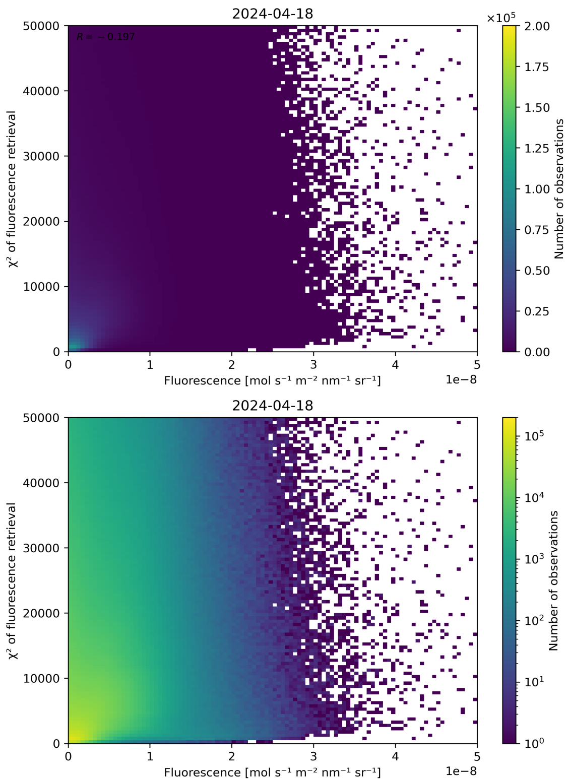
Figure 85: Scatter density plot of “Fluorescence” against “ \chi^2 of fluorescence retrieval” for 2024-04-17 to 2024-04-19.
