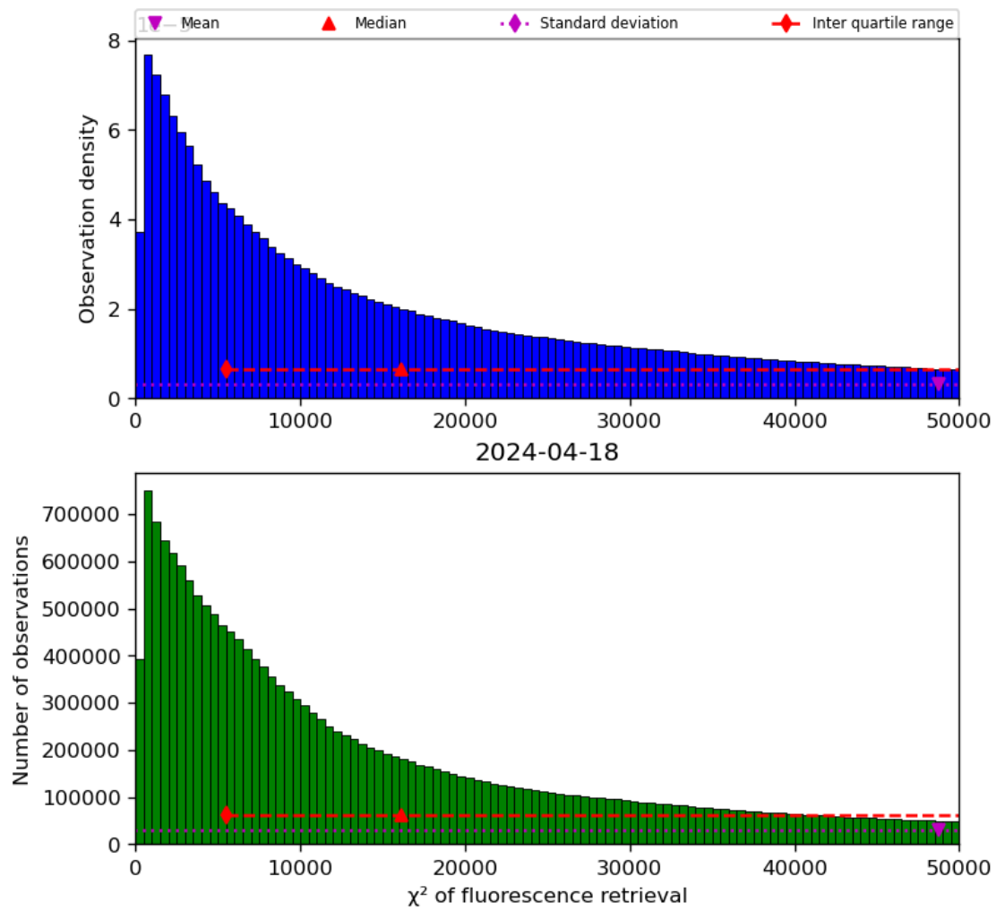
Figure 42: Histogram of “ \chi^2 of fluorescence retrieval” for 2024-04-17 to 2024-04-19
