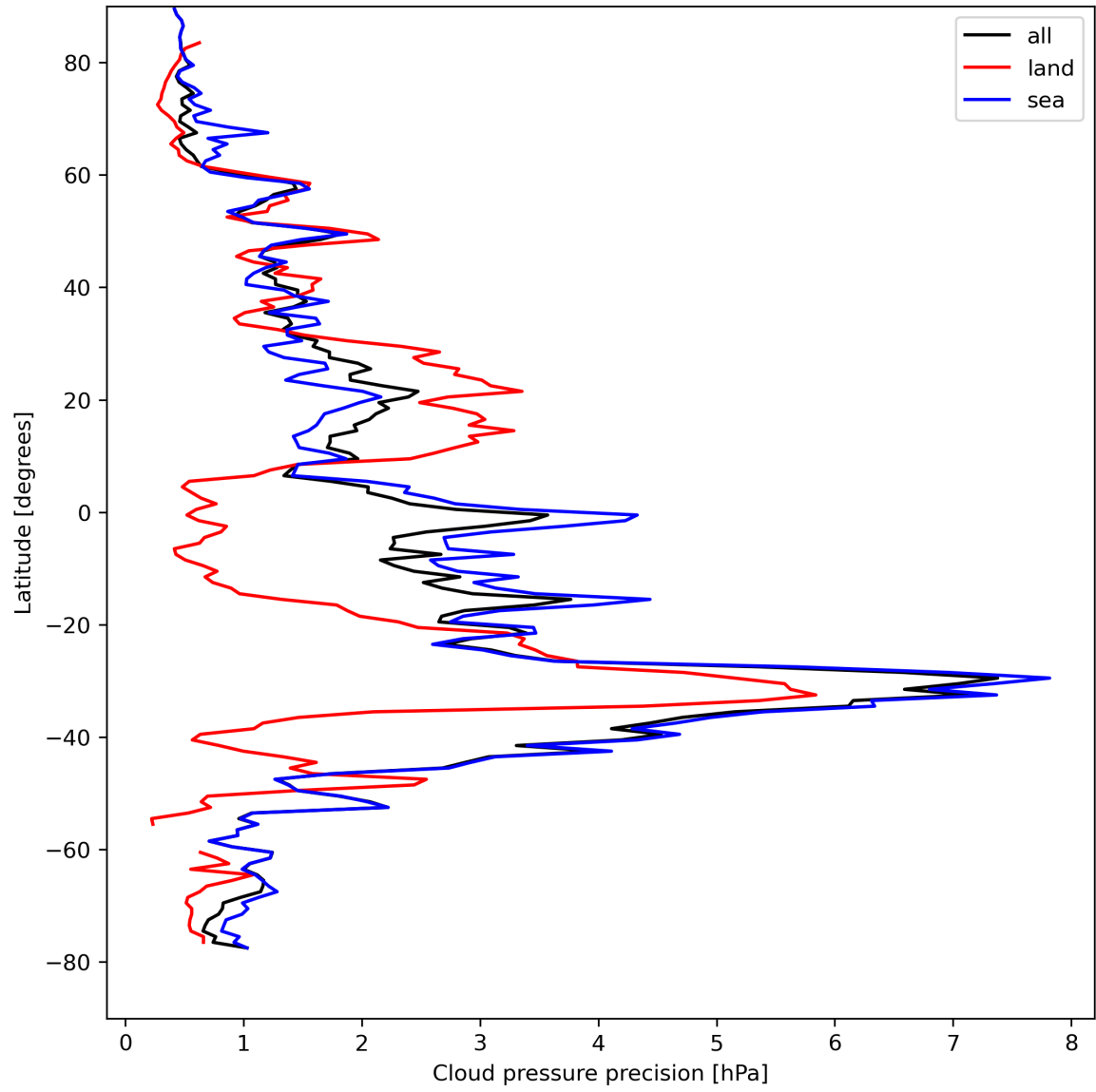
Figure 14: Zonal average of “Cloud pressure precision” for 2024-04-17 to 2024-04-19.
