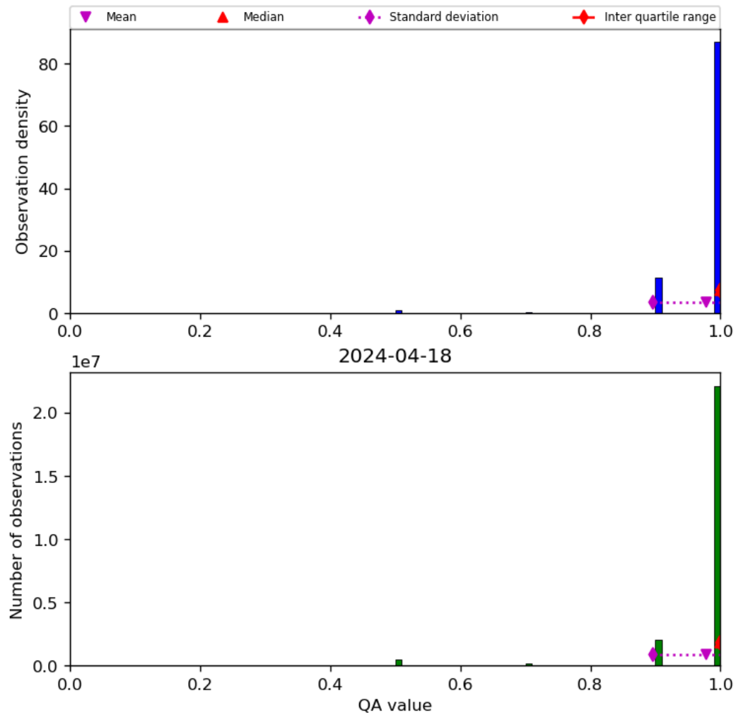
Figure 29: Histogram of “QA value” for 2024-04-17 to 2024-04-19
