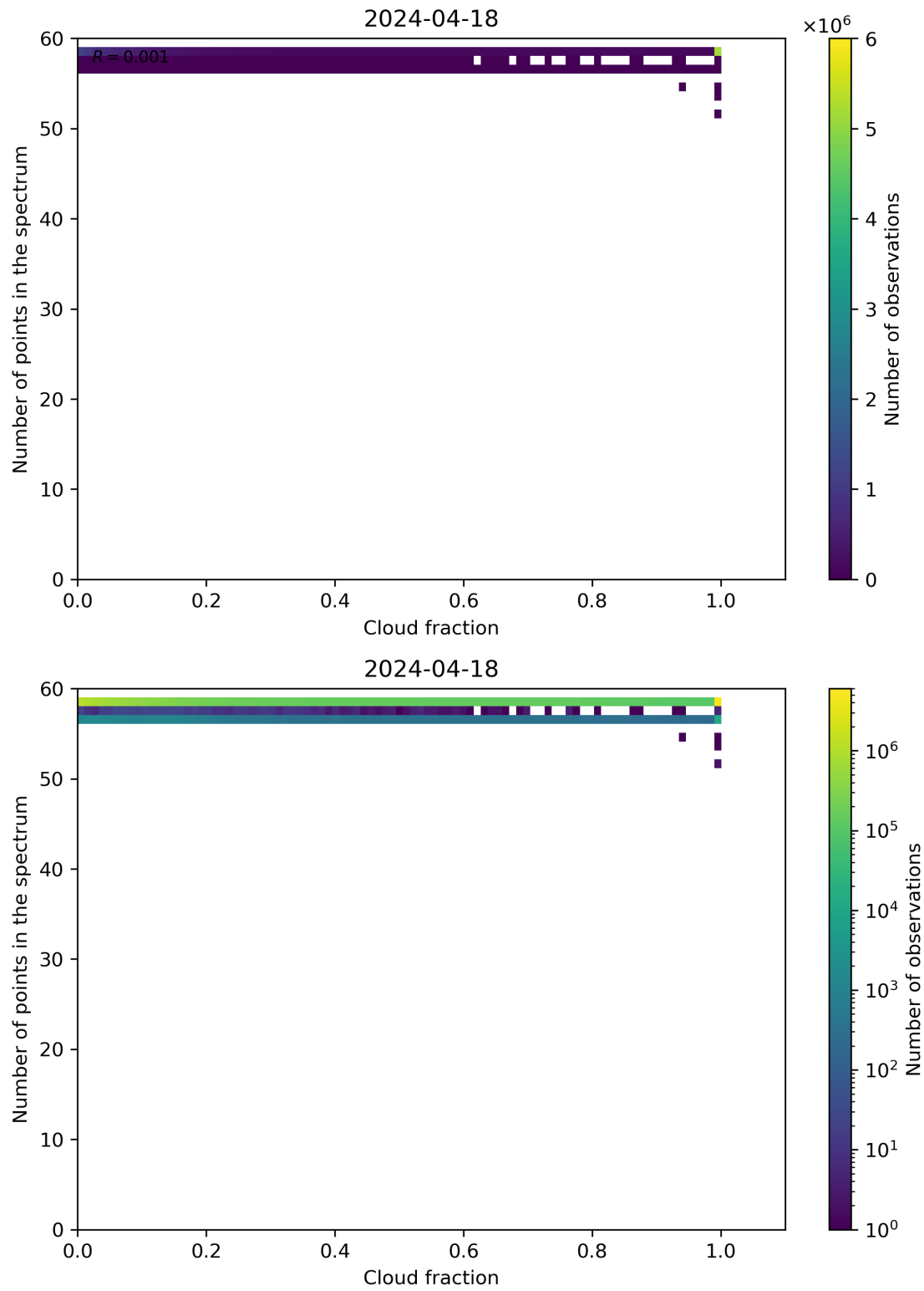
Figure 74: Scatter density plot of “Cloud fraction” against “Number of points in the spectrum” for 2024-04-17 to 2024-04-19.
