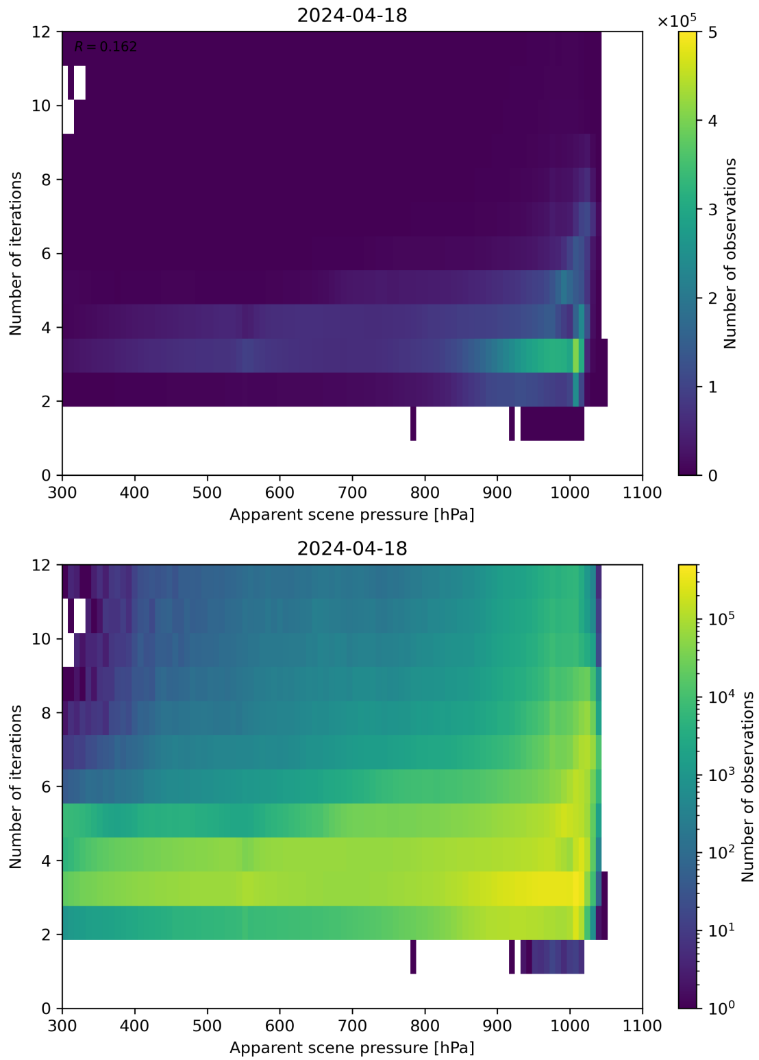
Figure 65: Scatter density plot of “Apparent scene pressure” against “Number of iterations” for 2024-04-17 to 2024-04-19.
