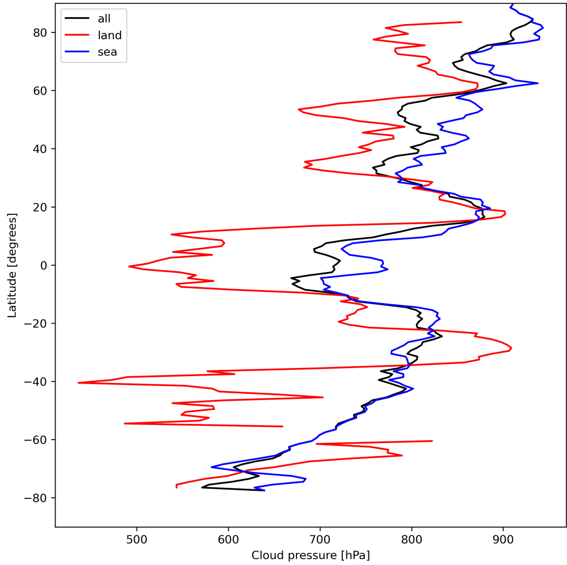
Figure 13: Zonal average of “Cloud pressure” for 2024-04-17 to 2024-04-19.
