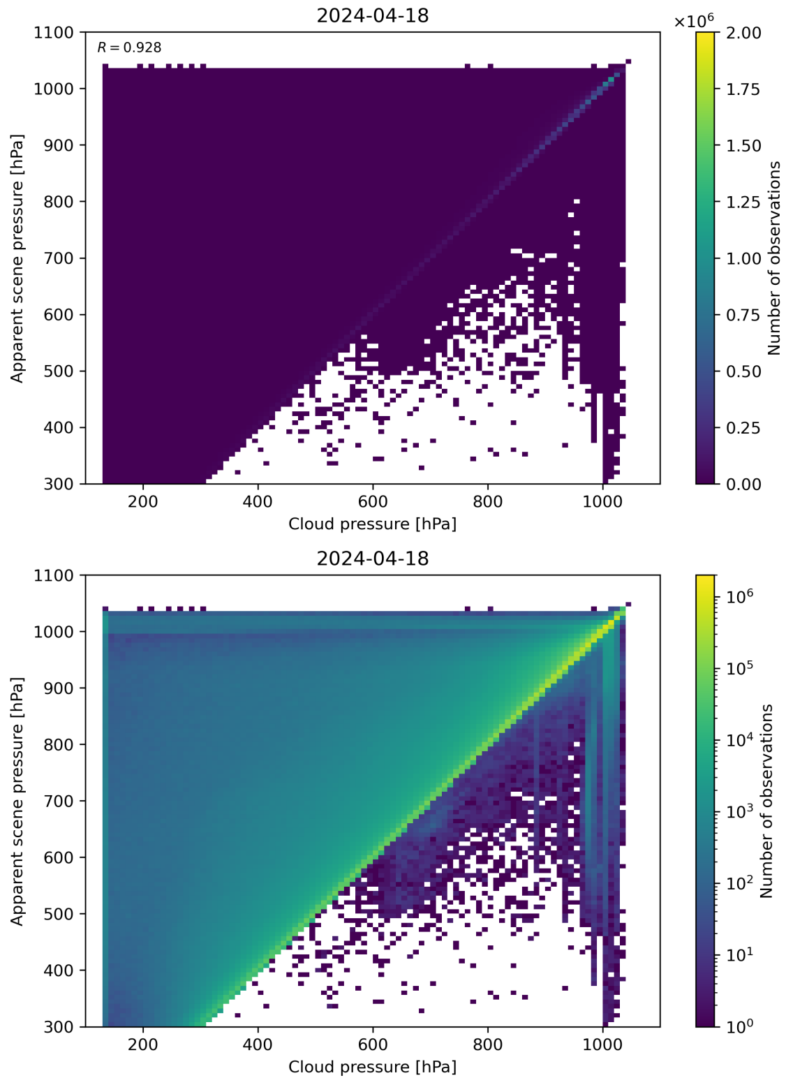
Figure 77: Scatter density plot of “Cloud pressure” against “Apparent scene pressure” for 2024-04-17 to 2024-04-19.
