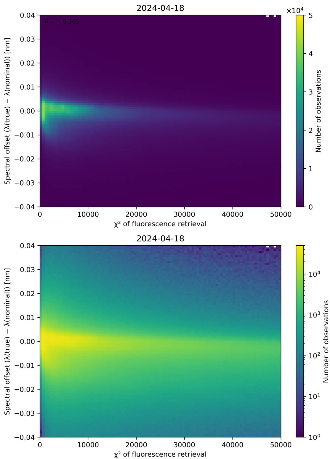
Figure 69: Scatter density plot of " \chi^2 of fluorescence retrieval" against "Spectral offset ( \lambda(\text{true}) - \lambda(\text{nominal})) " for 2024-04-17 to 2024-04-19.
