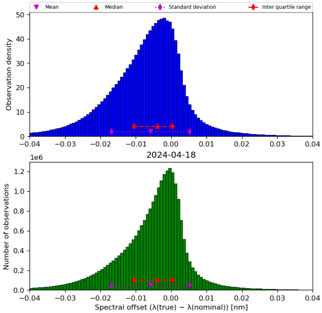
Figure 45: Histogram of “Spectral offset ( \lambda(\text{true}) - \lambda(\text{nominal}) )” for 2024-04-17 to 2024-04-19
