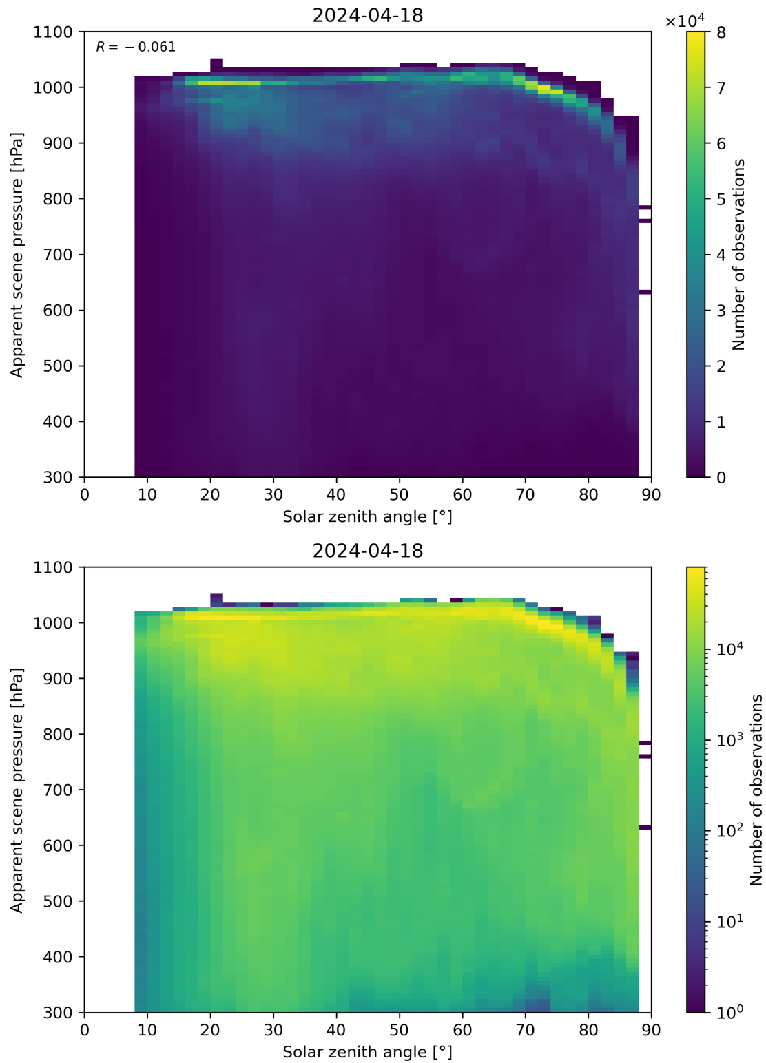
Figure 108: Scatter density plot of “Solar zenith angle” against “Apparent scene pressure” for 2024-04-17 to 2024-04-19.
