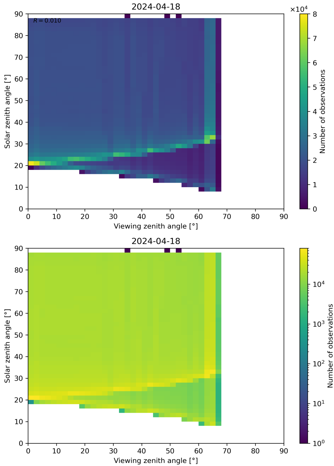
Figure 127: Scatter density plot of “Viewing zenith angle” against “Solar zenith angle” for 2024-04-17 to 2024-04-19.
