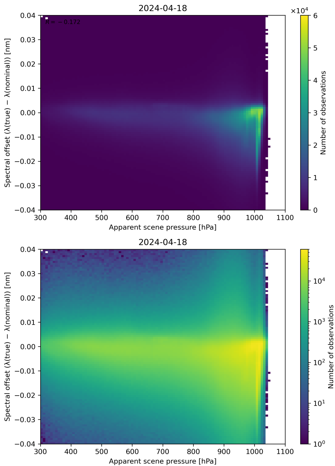
Figure 67: Scatter density plot of “Apparent scene pressure” against “Spectral offset ( \lambda(\text{true}) - \lambda(\text{nominal}) )” for 2024-04-17 to 2024-04-19.
