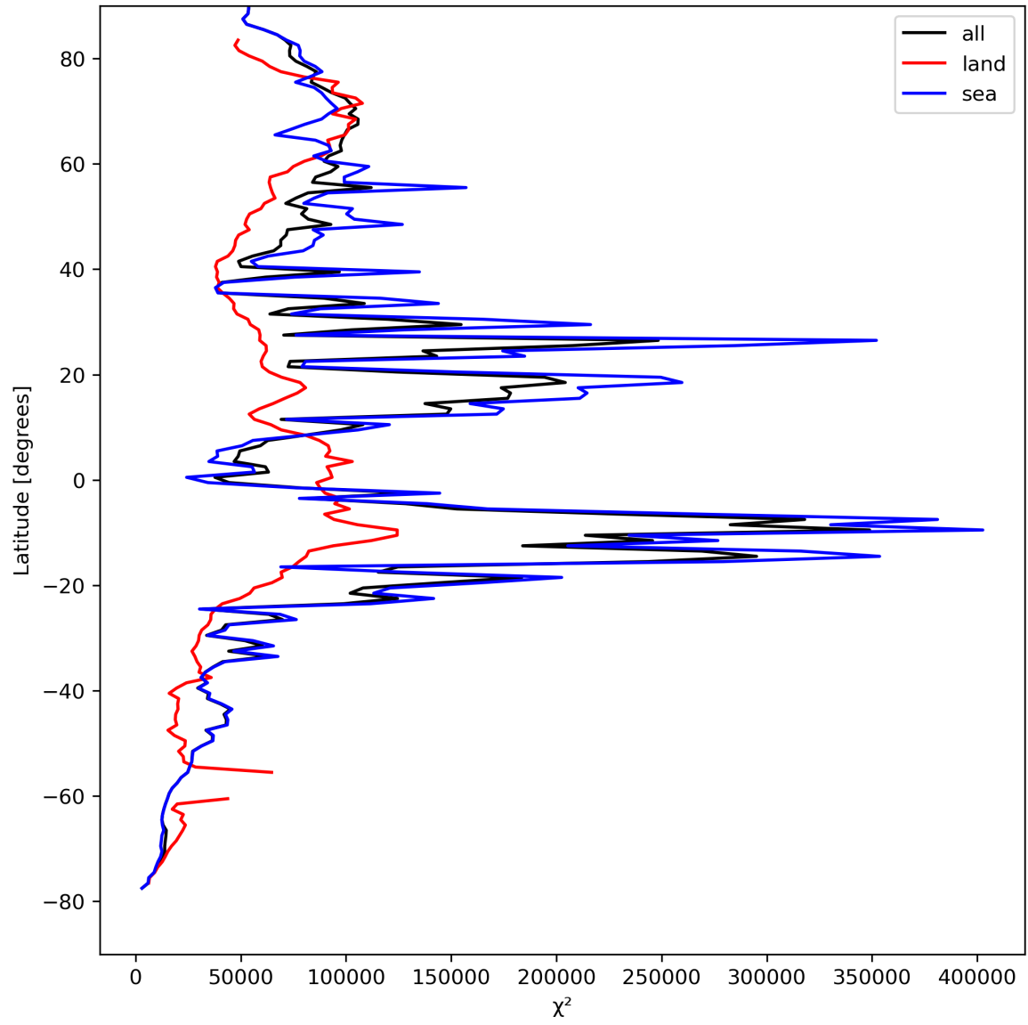
Figure 21: Zonal average of “ \chi^2 ” for 2024-04-17 to 2024-04-19.
