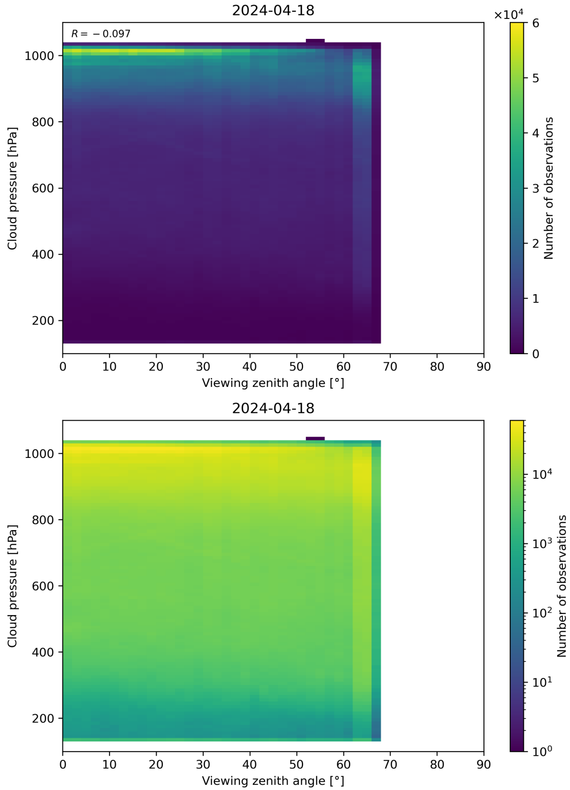
Figure 121: Scatter density plot of “Viewing zenith angle” against “Cloud pressure” for 2024-04-17 to 2024-04-19.
