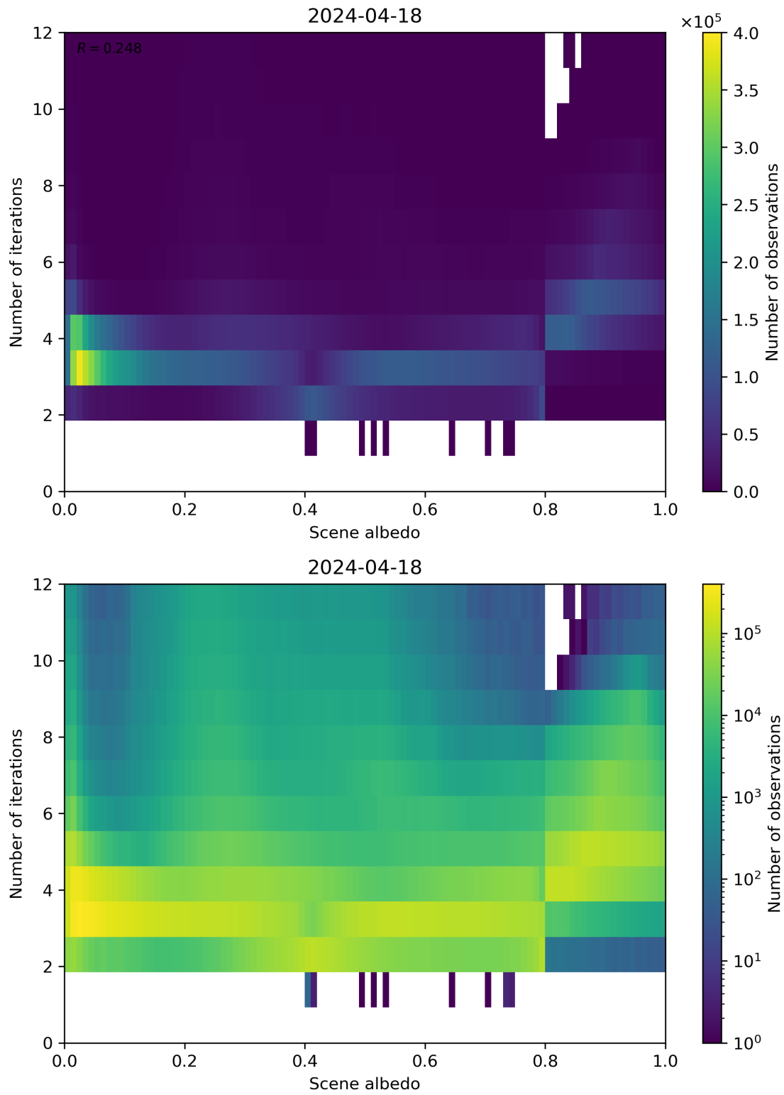
Figure 105: Scatter density plot of “Scene albedo” against “Number of iterations” for 2024-04-17 to 2024-04-19.
