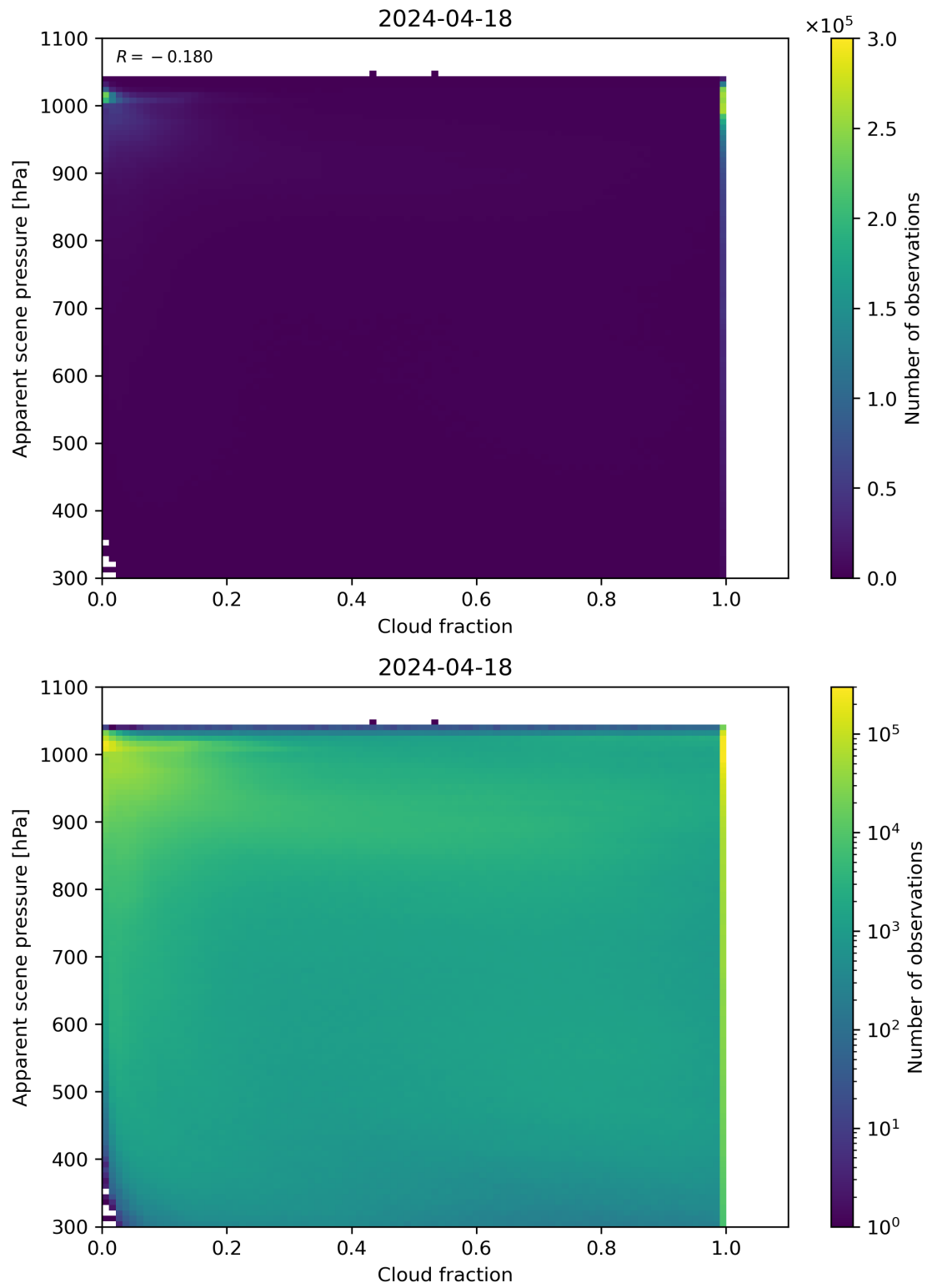
Figure 70: Scatter density plot of “Cloud fraction” against “Apparent scene pressure” for 2024-04-17 to 2024-04-19.
