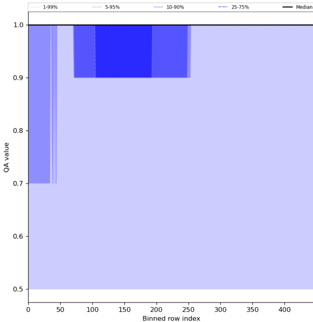
Figure 46: Along track statistics of “QA value” for 2024-04-17 to 2024-04-19
