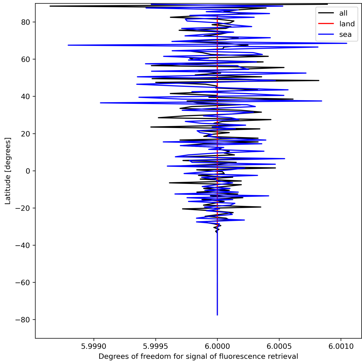
Figure 26: Zonal average of “Degrees of freedom for signal of fluorescence retrieval” for 2024-04-17 to 2024-04-19.
