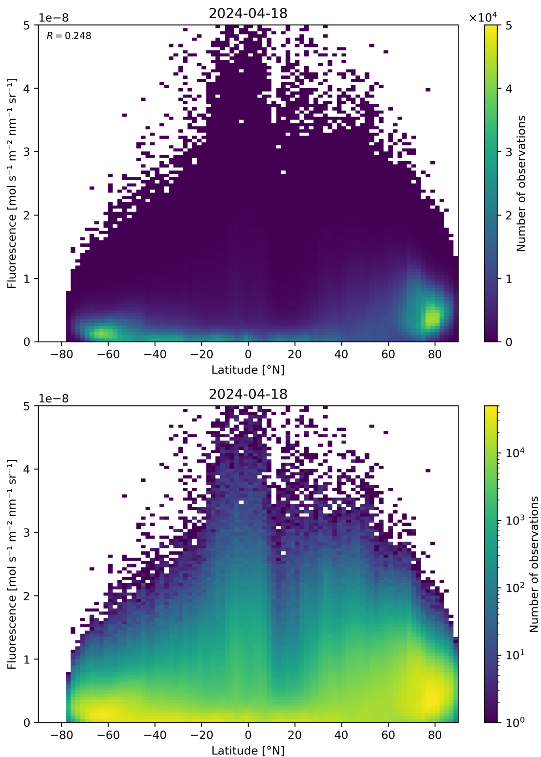
Figure 92: Scatter density plot of “Latitude” against “Fluorescence” for 2024-04-17 to 2024-04-19.
