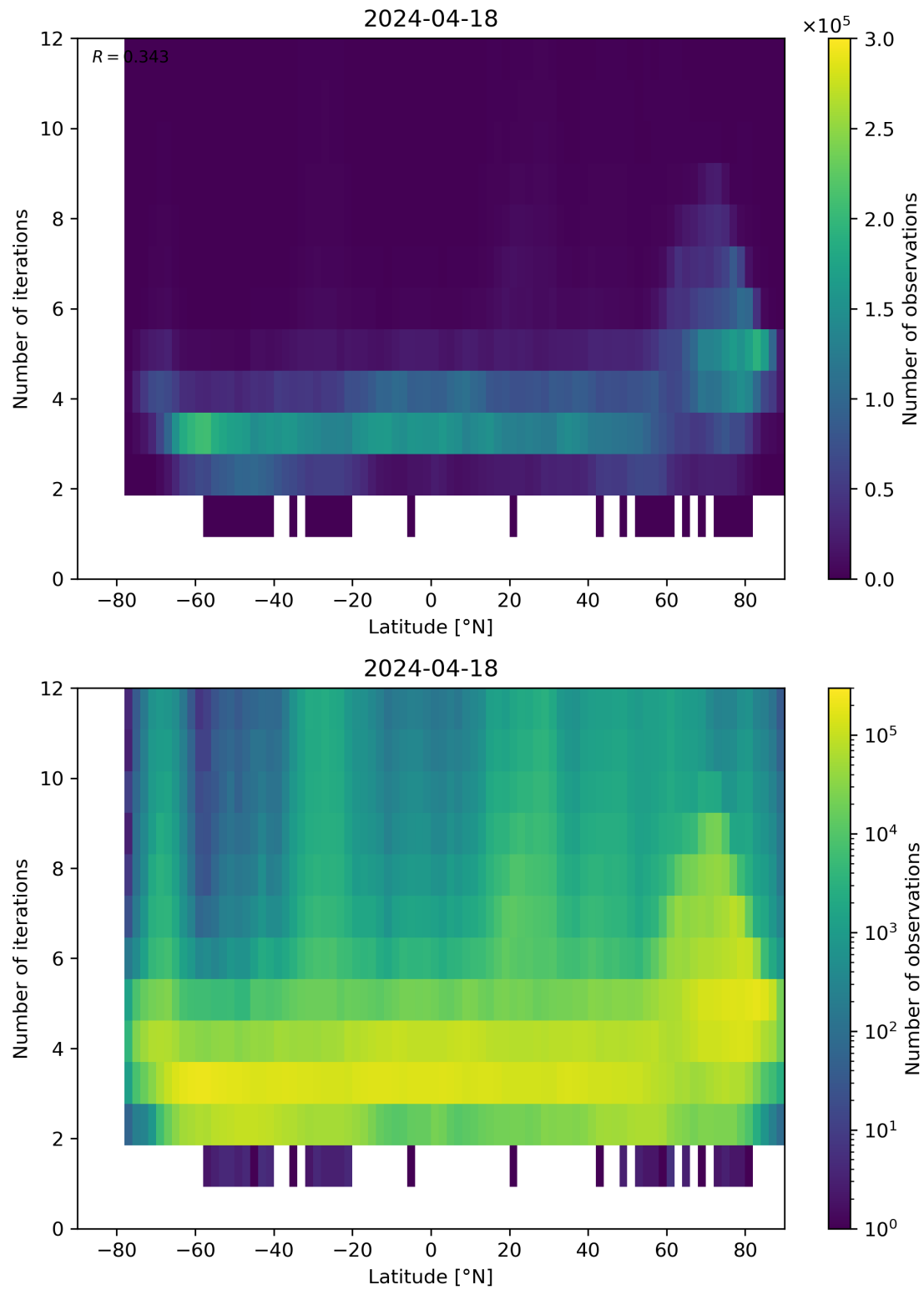
Figure 93: Scatter density plot of “Latitude” against “Number of iterations” for 2024-04-17 to 2024-04-19.
