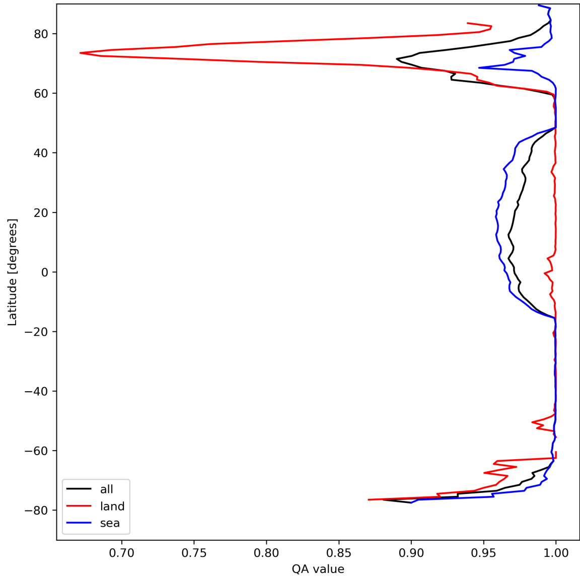
Figure 12: Zonal average of “QA value” for 2024-04-17 to 2024-04-19.
