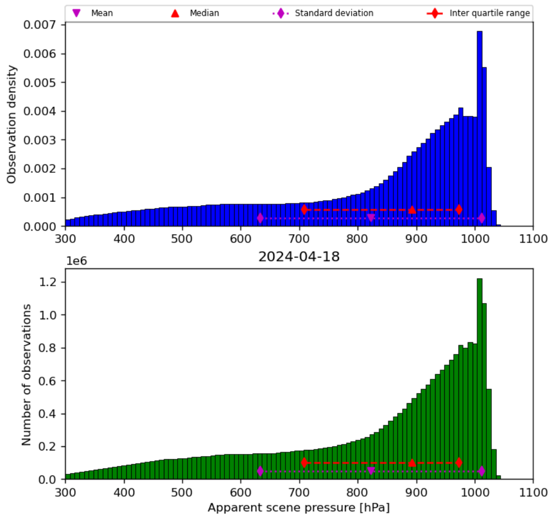
Figure 36: Histogram of “Apparent scene pressure” for 2024-04-17 to 2024-04-19
