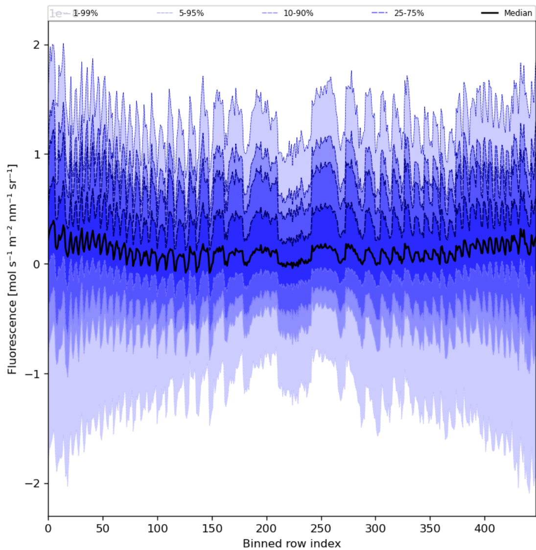
Figure 57: Along track statistics of “Fluorescence” for 2024-04-17 to 2024-04-19
