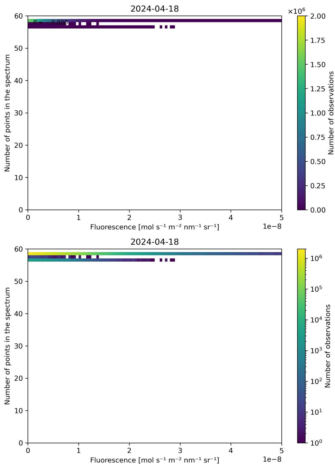
Figure 86: Scatter density plot of “Fluorescence” against “Number of points in the spectrum” for 2024-04-17 to 2024-04-19.
