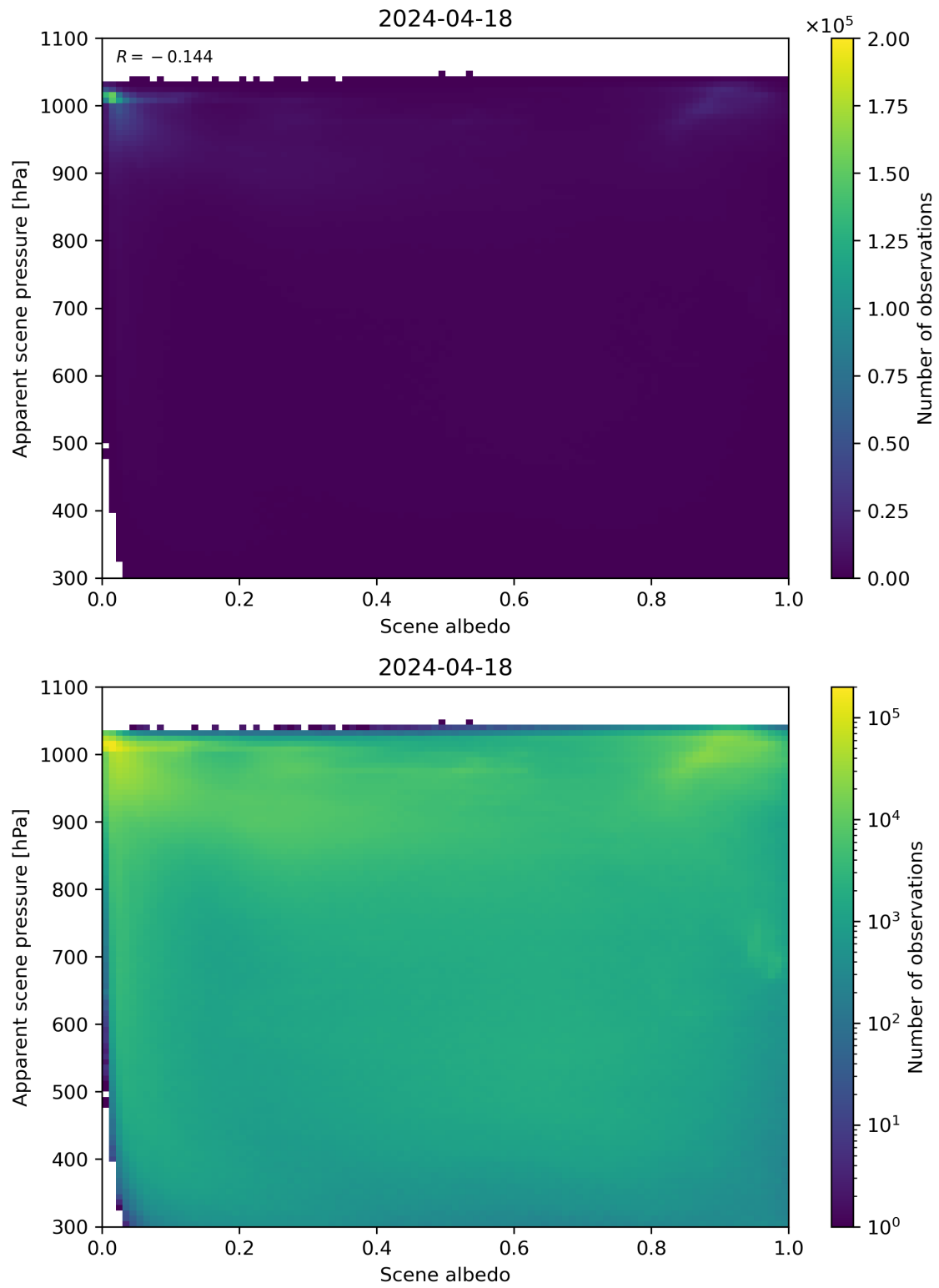
Figure 102: Scatter density plot of “Scene albedo” against “Apparent scene pressure” for 2024-04-17 to 2024-04-19.
