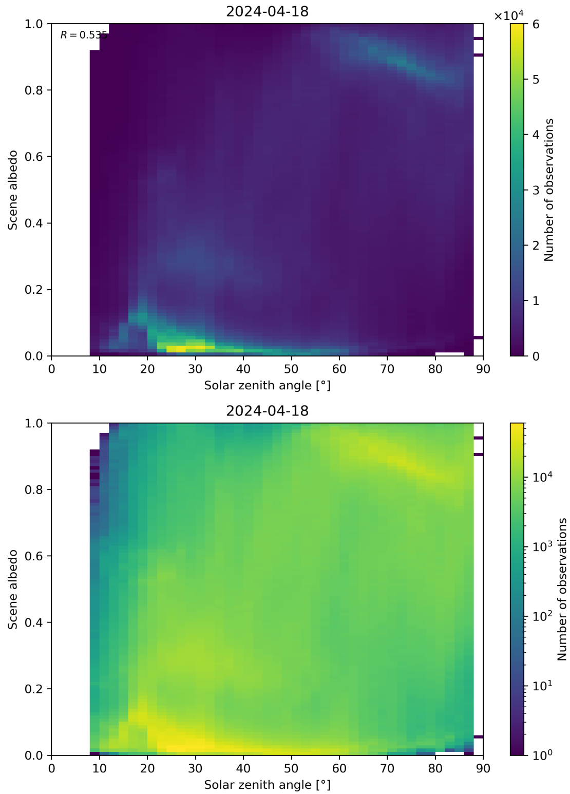
Figure 116: Scatter density plot of “Solar zenith angle” against “Scene albedo” for 2024-04-17 to 2024-04-19.
