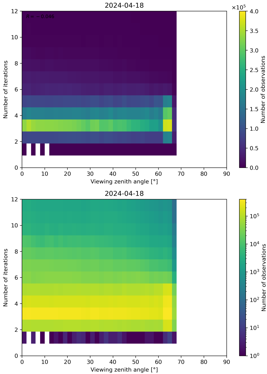
Figure 124: Scatter density plot of “Viewing zenith angle” against “Number of iterations” for 2024-04-17 to 2024-04-19.
