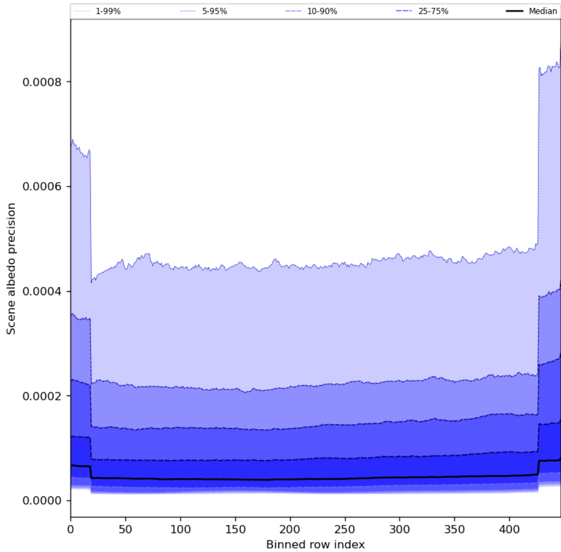
Figure 52: Along track statistics of “Scene albedo precision” for 2024-04-17 to 2024-04-19
