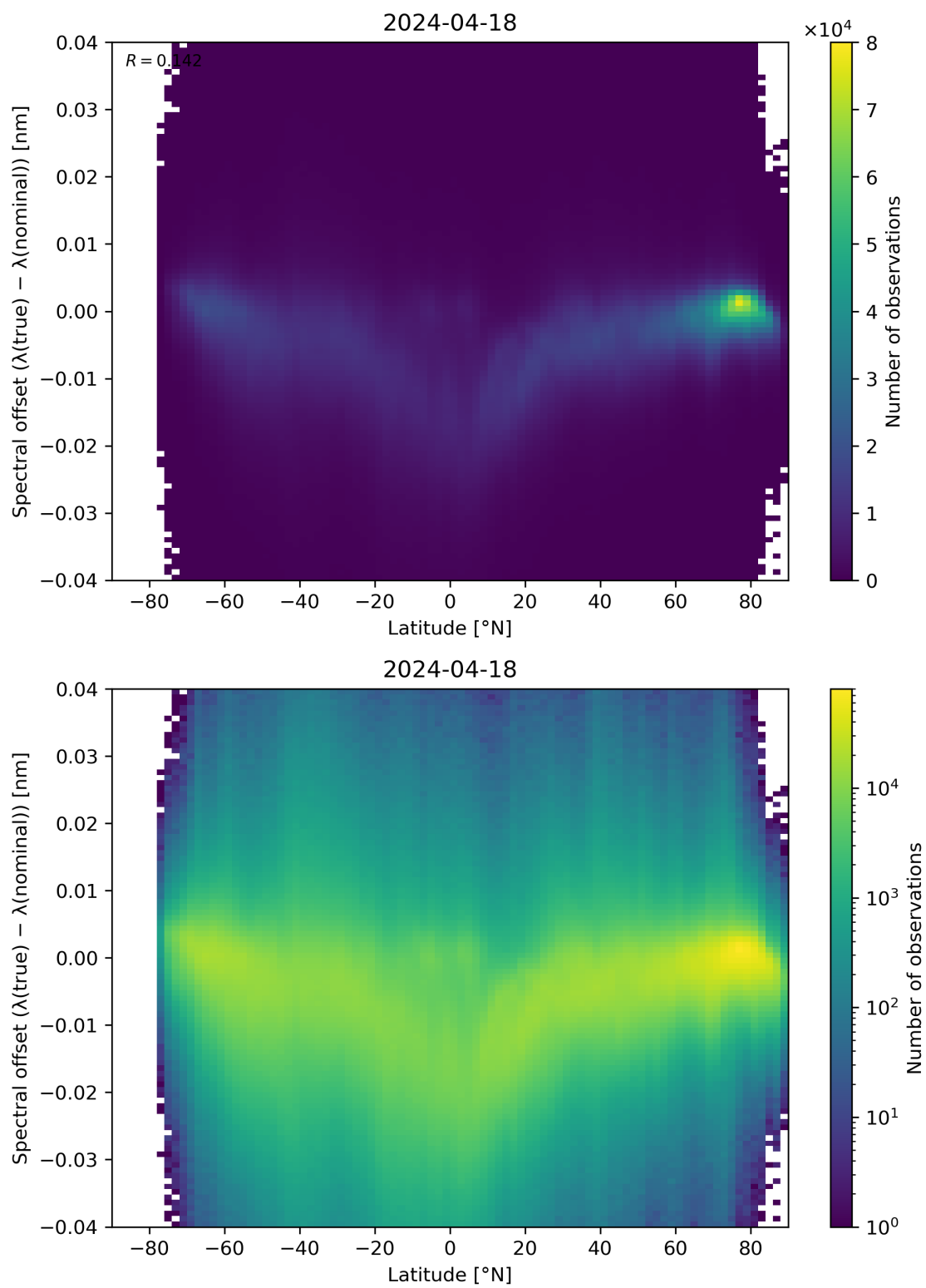
Figure 96: Scatter density plot of “Latitude” against “Spectral offset ( \lambda(\text{true}) - \lambda(\text{nominal}) )” for 2024-04-17 to 2024-04-19.
