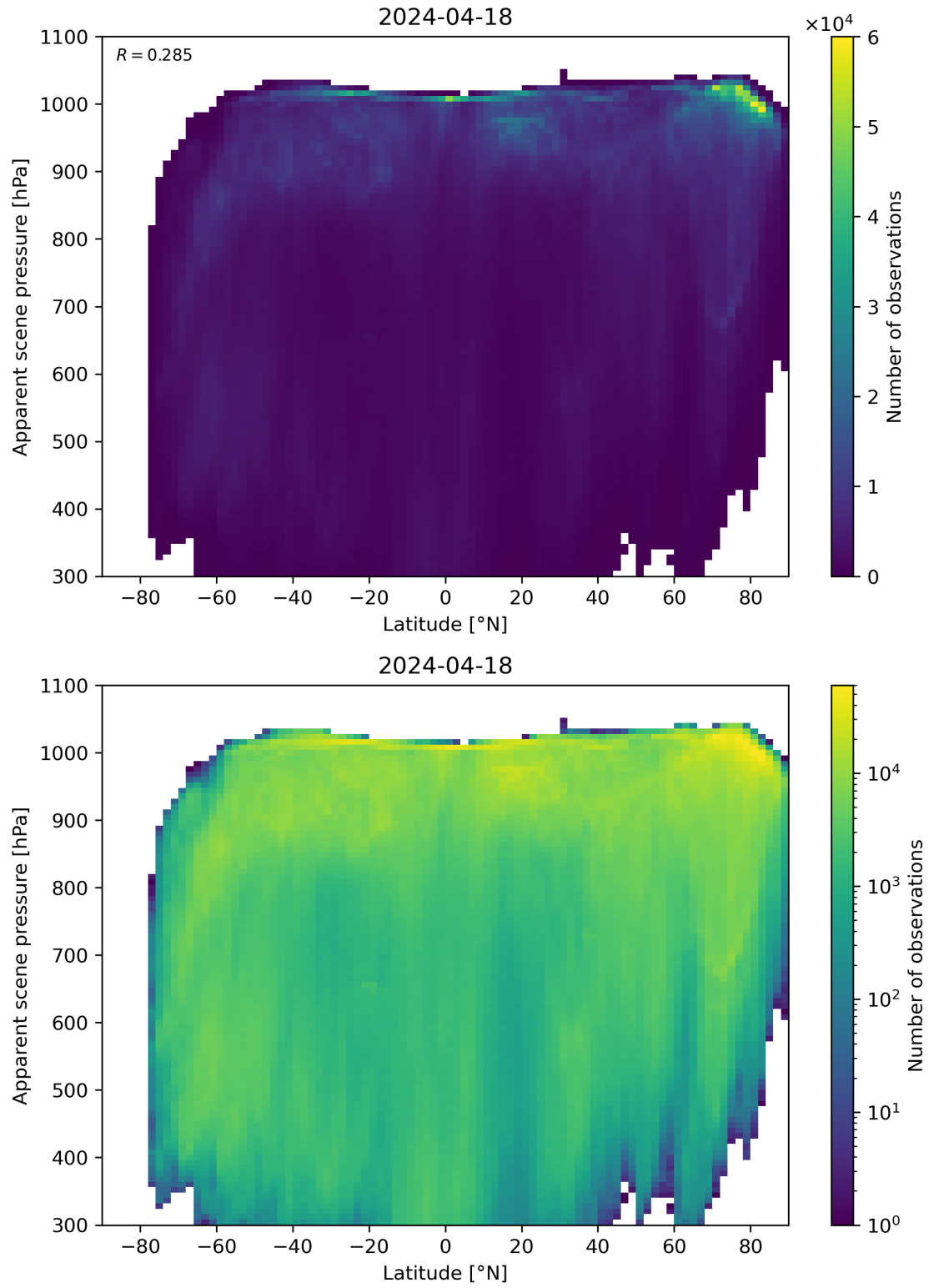
Figure 88: Scatter density plot of “Latitude” against “Apparent scene pressure” for 2024-04-17 to 2024-04-19.
