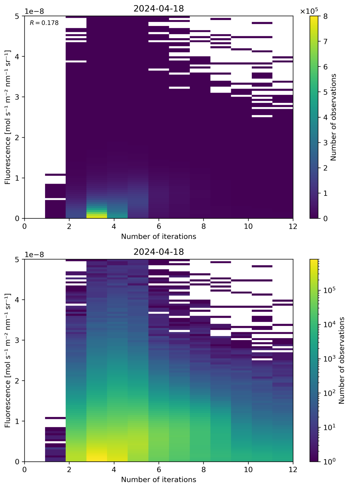
Figure 98: Scatter density plot of “Number of iterations” against “Fluorescence” for 2024-04-17 to 2024-04-19.
