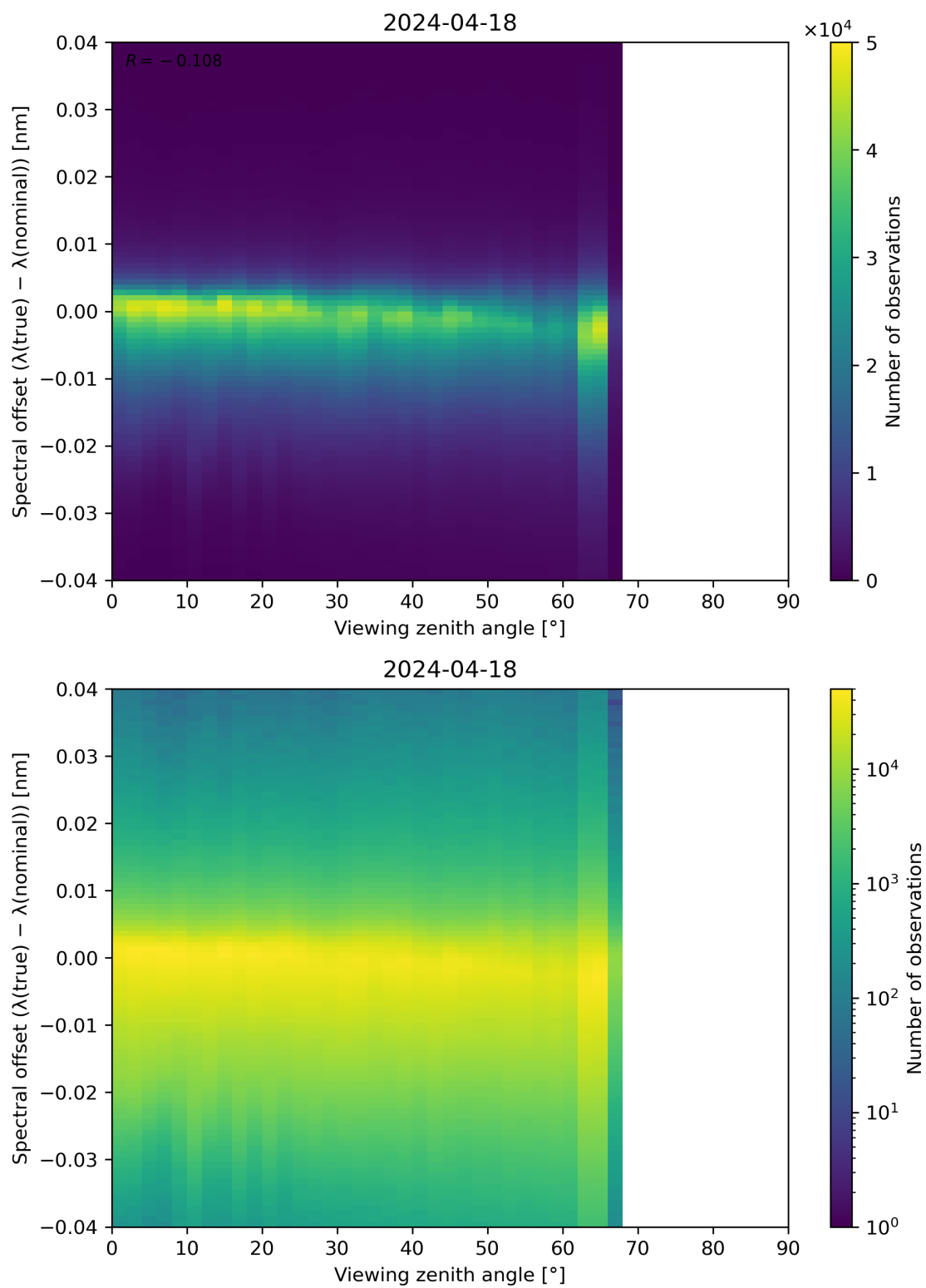
Figure 128: Scatter density plot of “Viewing zenith angle” against “Spectral offset ( \lambda(\text{true}) - \lambda(\text{nominal}) )” for 2024-04-17 to 2024-04-19.
