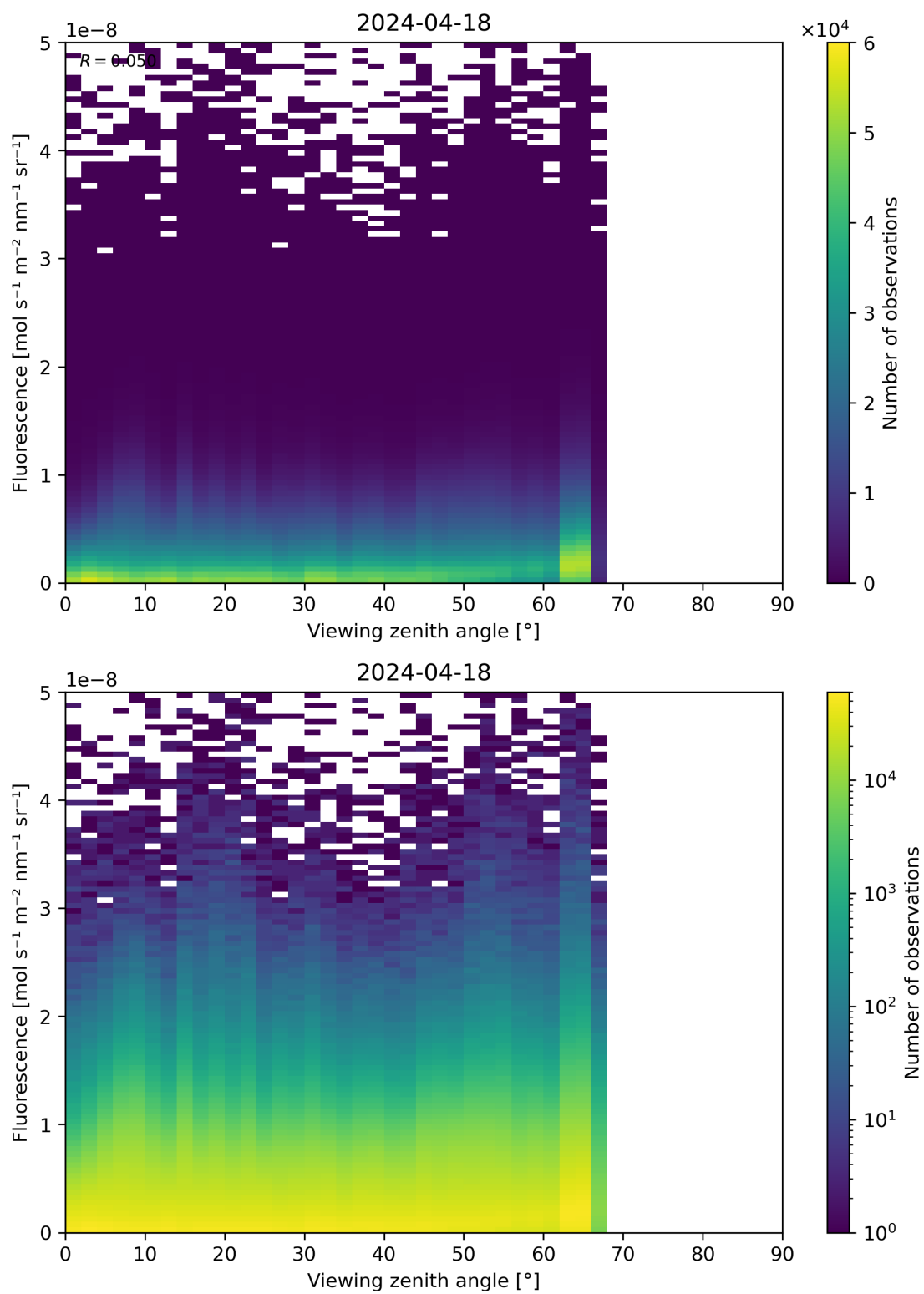
Figure 122: Scatter density plot of “Viewing zenith angle” against “Fluorescence” for 2024-04-17 to 2024-04-19.
