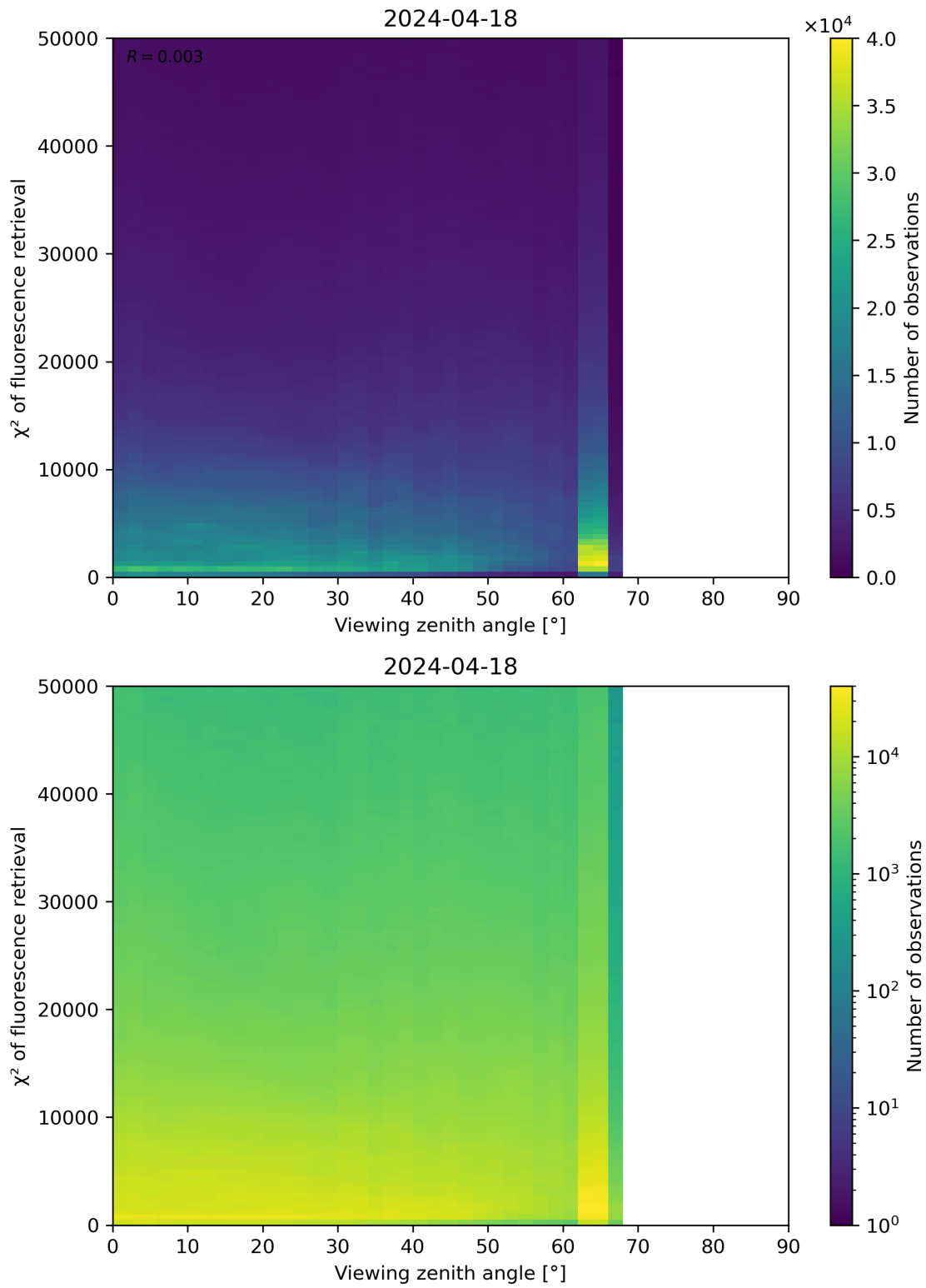
Figure 119: Scatter density plot of “Viewing zenith angle” against “ \chi^2 of fluorescence retrieval” for 2024-04-17 to 2024-04-19.
