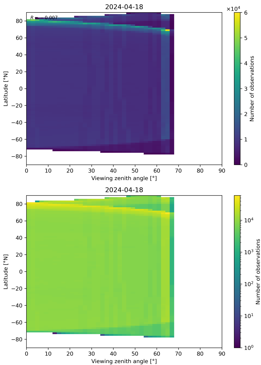
Figure 123: Scatter density plot of “Viewing zenith angle” against “Latitude” for 2024-04-17 to 2024-04-19.
