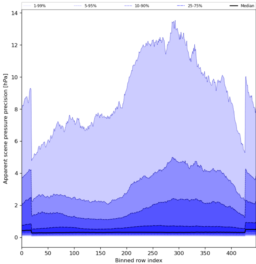
Figure 54: Along track statistics of “Apparent scene pressure precision” for 2024-04-17 to 2024-04-19
