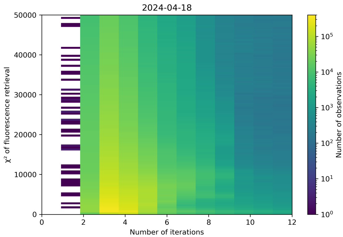
Figure 97: Scatter density plot of “Number of iterations” against “ \chi^2 of fluorescence retrieval” for 2024-04-17 to 2024-04-19.
