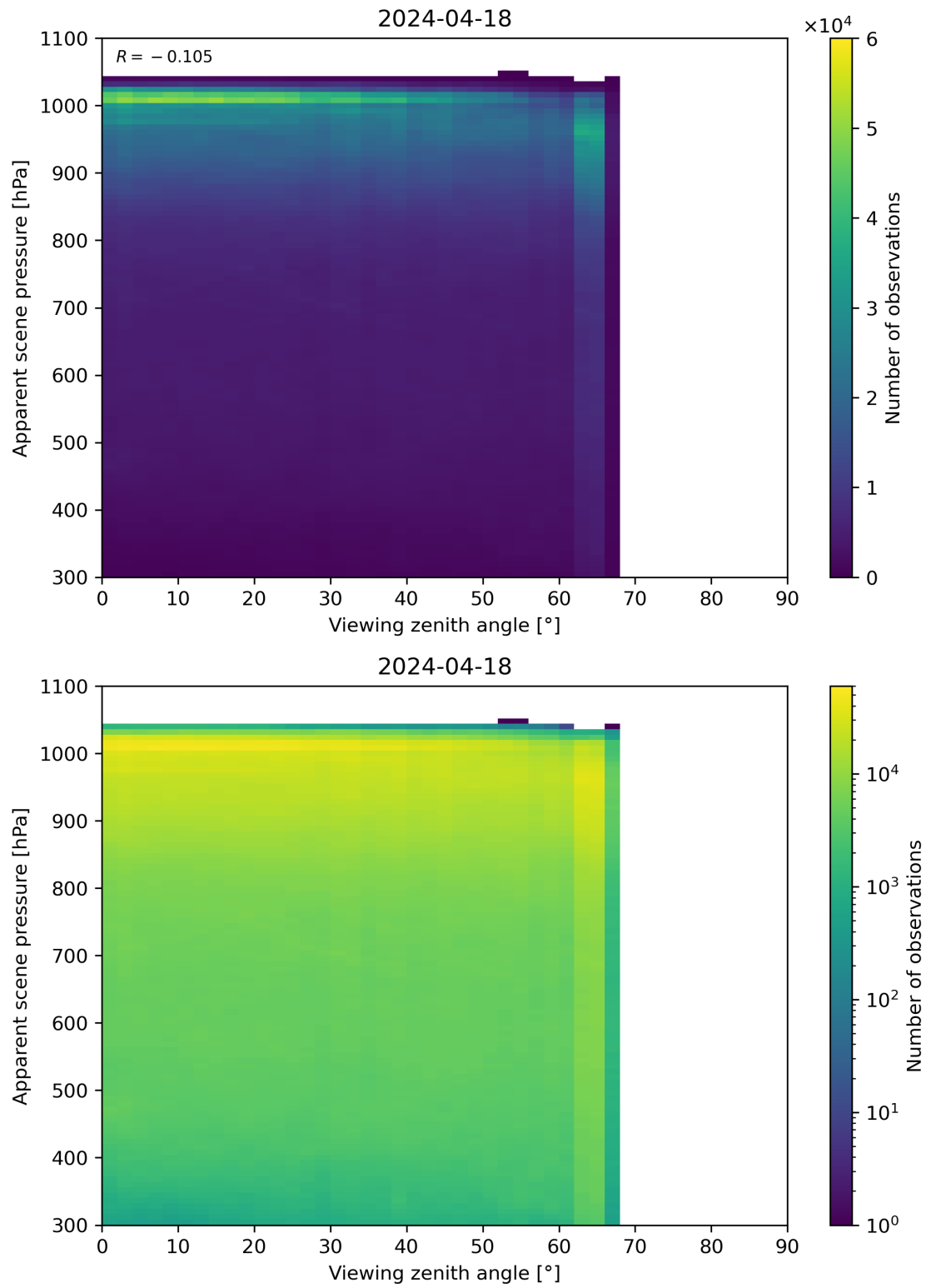
Figure 118: Scatter density plot of “Viewing zenith angle” against “Apparent scene pressure” for 2024-04-17 to 2024-04-19.
