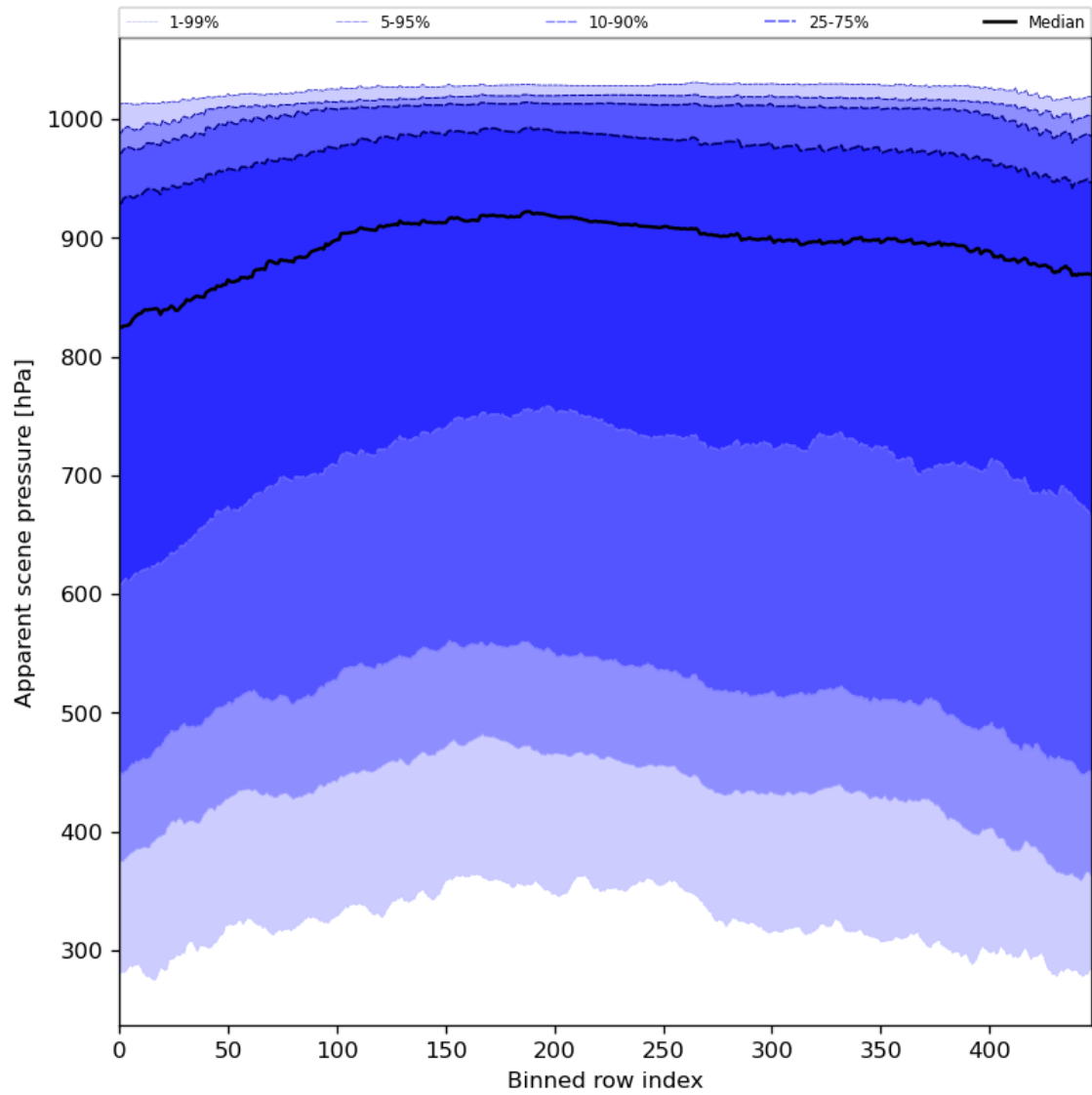
Figure 53: Along track statistics of “Apparent scene pressure” for 2024-04-17 to 2024-04-19
