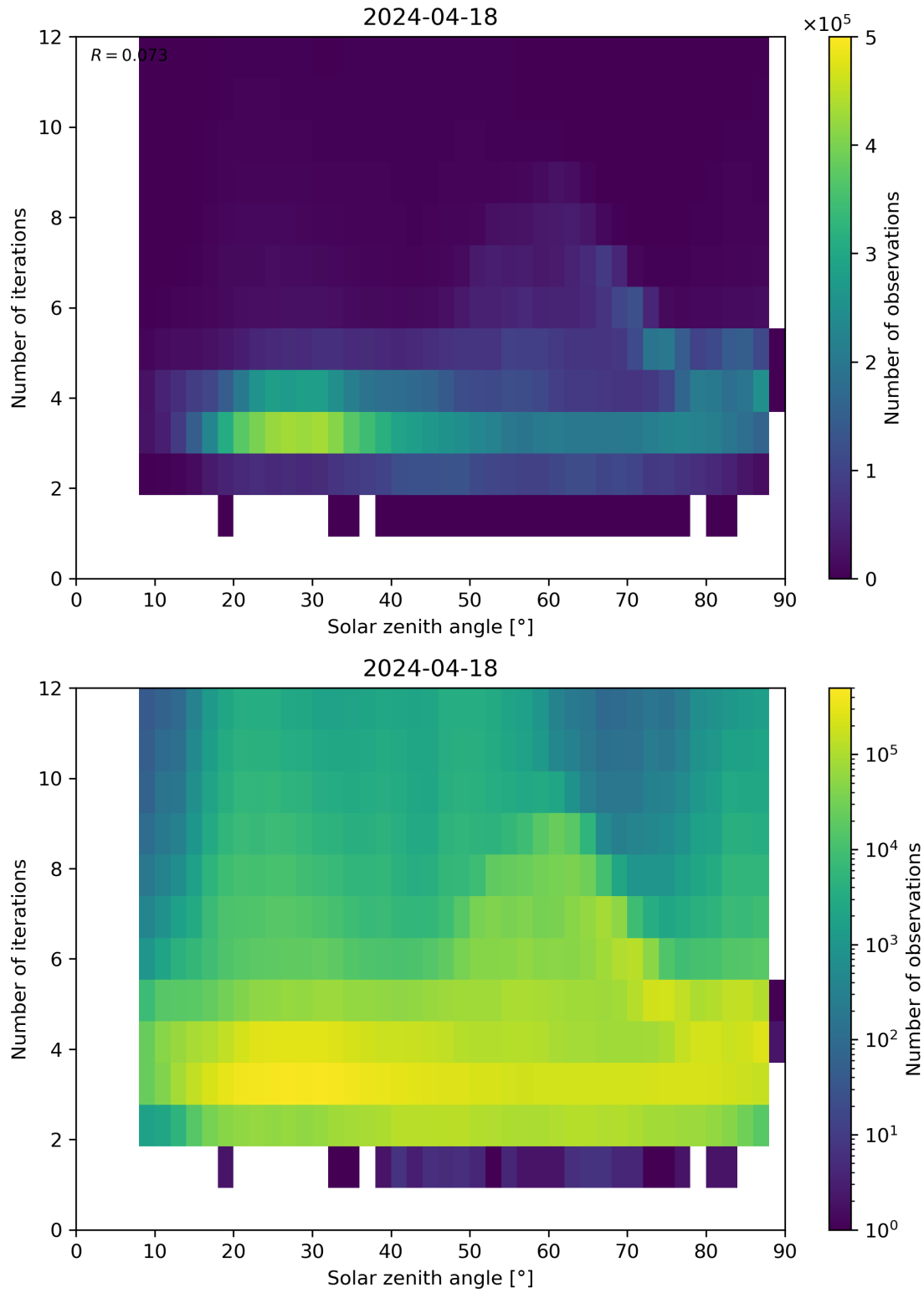
Figure 114: Scatter density plot of “Solar zenith angle” against “Number of iterations” for 2024-04-17 to 2024-04-19.
