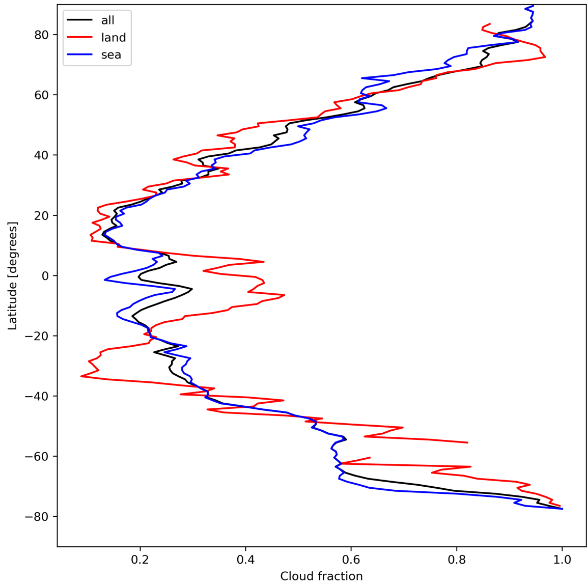
Figure 15: Zonal average of “Cloud fraction” for 2024-04-17 to 2024-04-19.
