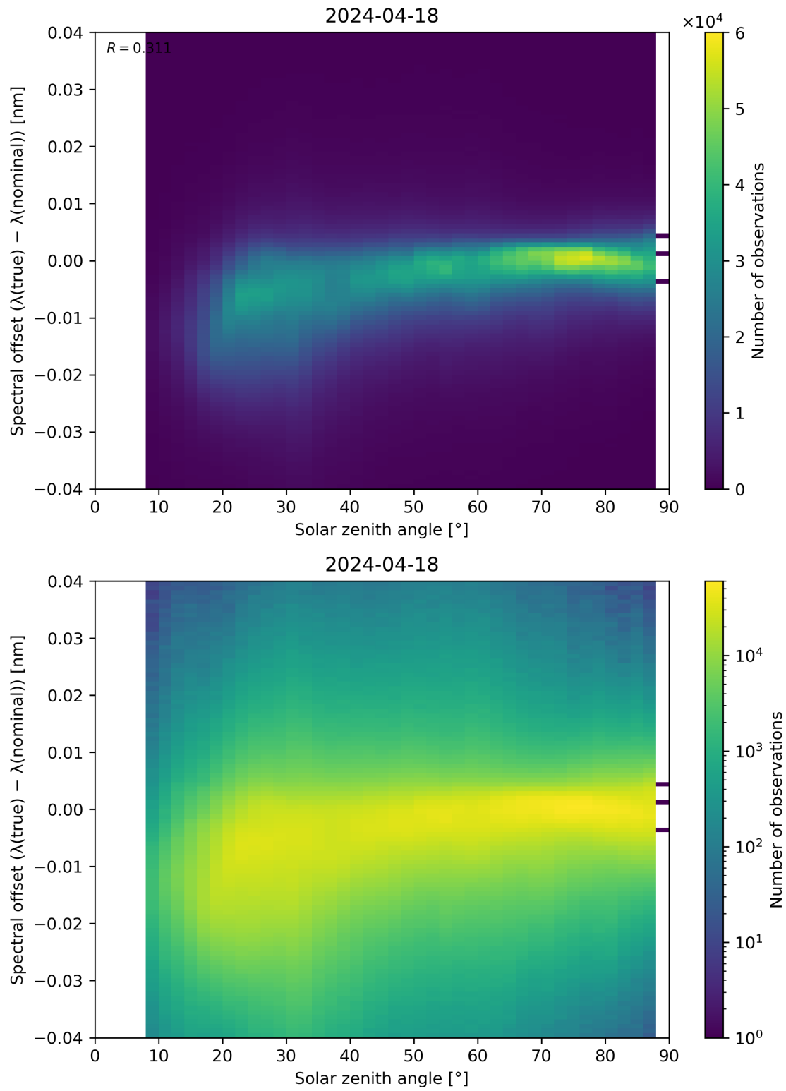
Figure 117: Scatter density plot of “Solar zenith angle” against “Spectral offset ( \lambda(\text{true}) - \lambda(\text{nominal}) )” for 2024-04-17 to 2024-04-19.
