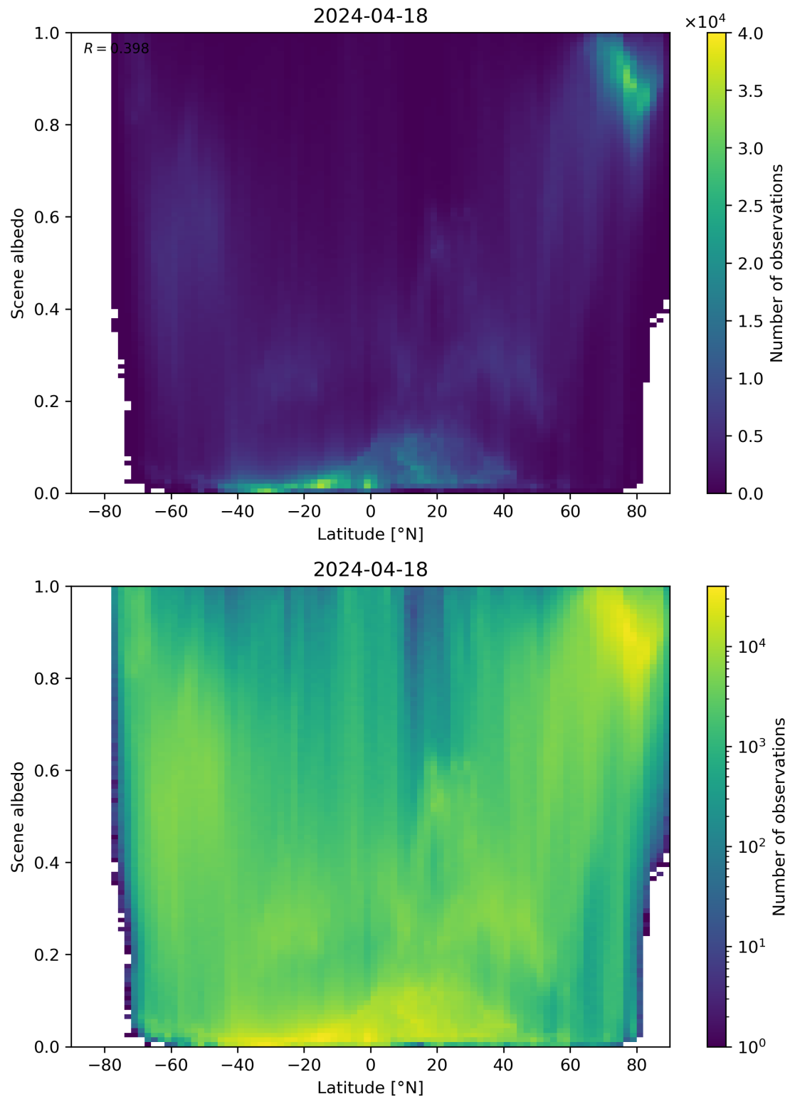
Figure 95: Scatter density plot of “Latitude” against “Scene albedo” for 2024-04-17 to 2024-04-19.
