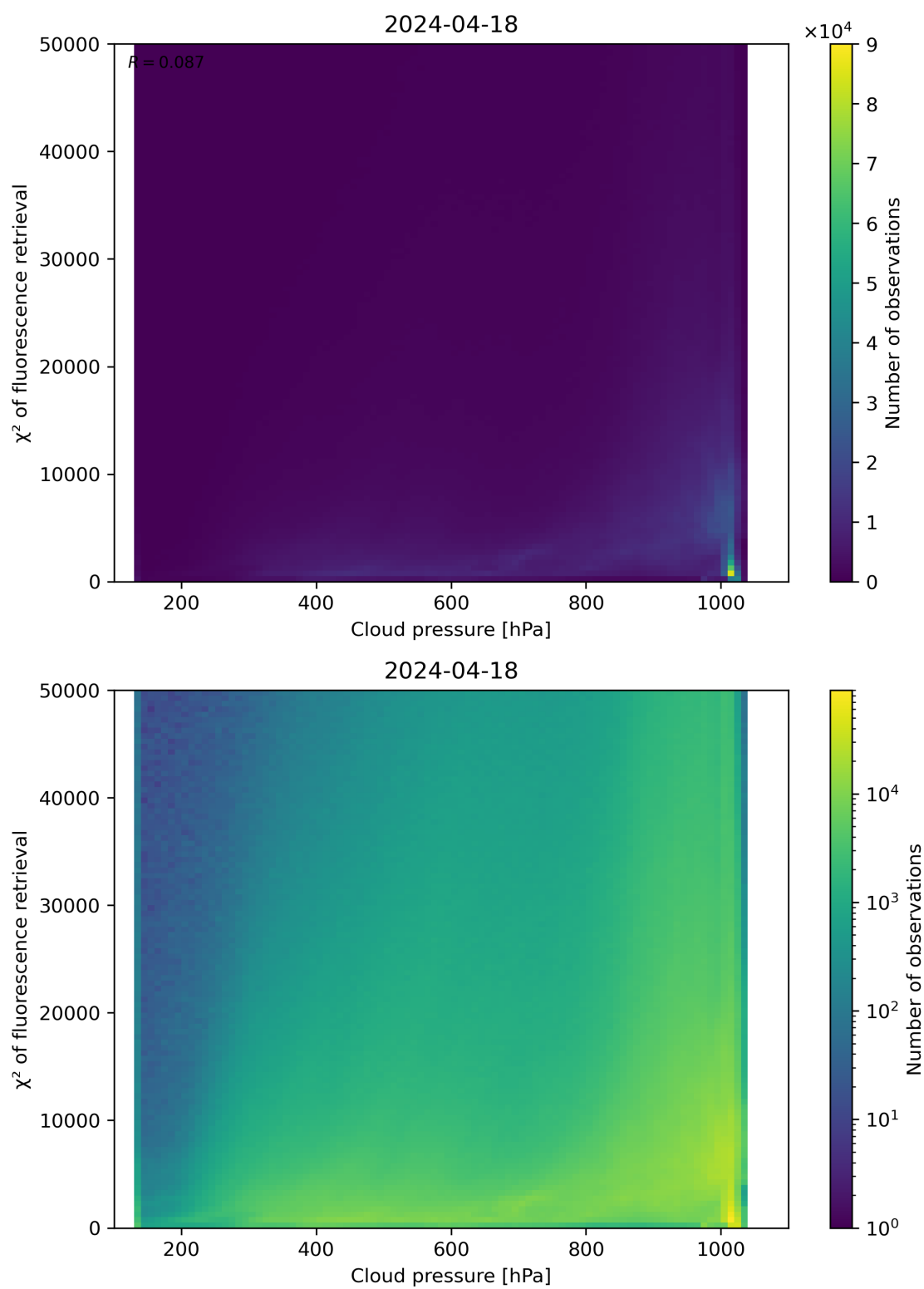
Figure 78: Scatter density plot of “Cloud pressure” against “ \chi^2 of fluorescence retrieval” for 2024-04-17 to 2024-04-19.
