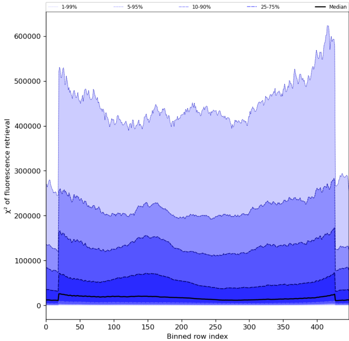
Figure 59: Along track statistics of “ \chi^2 of fluorescence retrieval” for 2024-04-17 to 2024-04-19
