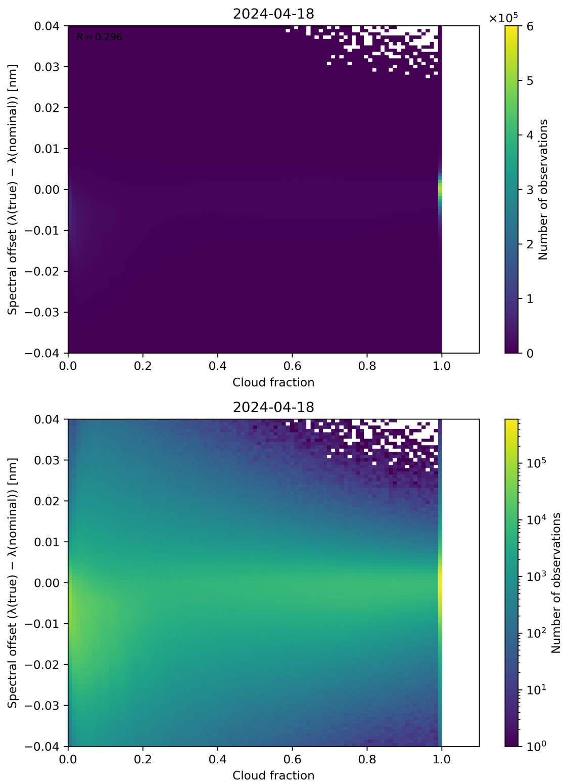
Figure 76: Scatter density plot of “Cloud fraction” against “Spectral offset ( \lambda(\text{true}) - \lambda(\text{nominal}) )” for 2024-04-17 to 2024-04-19.
