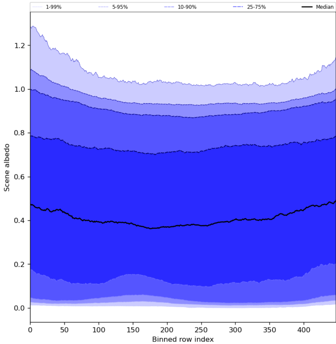
Figure 51: Along track statistics of “Scene albedo” for 2024-04-17 to 2024-04-19
