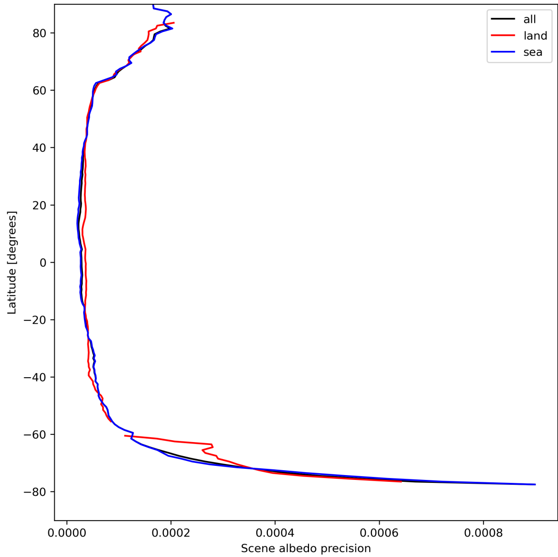
Figure 18: Zonal average of “Scene albedo precision” for 2024-04-17 to 2024-04-19.
