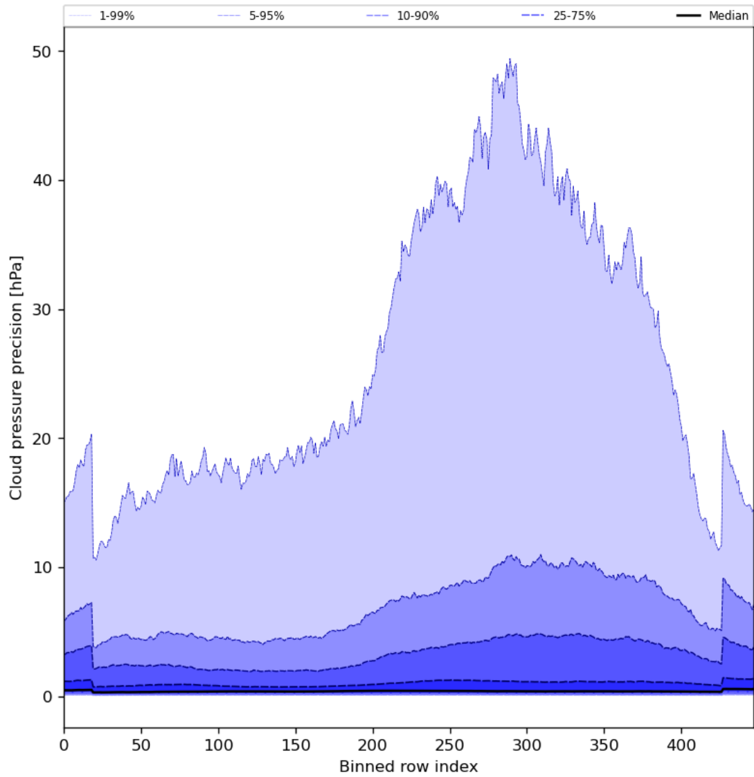
Figure 48: Along track statistics of “Cloud pressure precision” for 2024-04-17 to 2024-04-19
