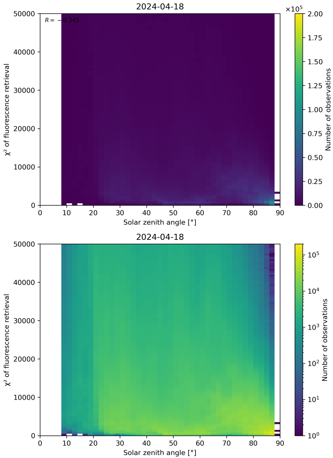
Figure 109: Scatter density plot of “Solar zenith angle” against “ \chi^2 of fluorescence retrieval” for 2024-04-17 to 2024-04-19.
