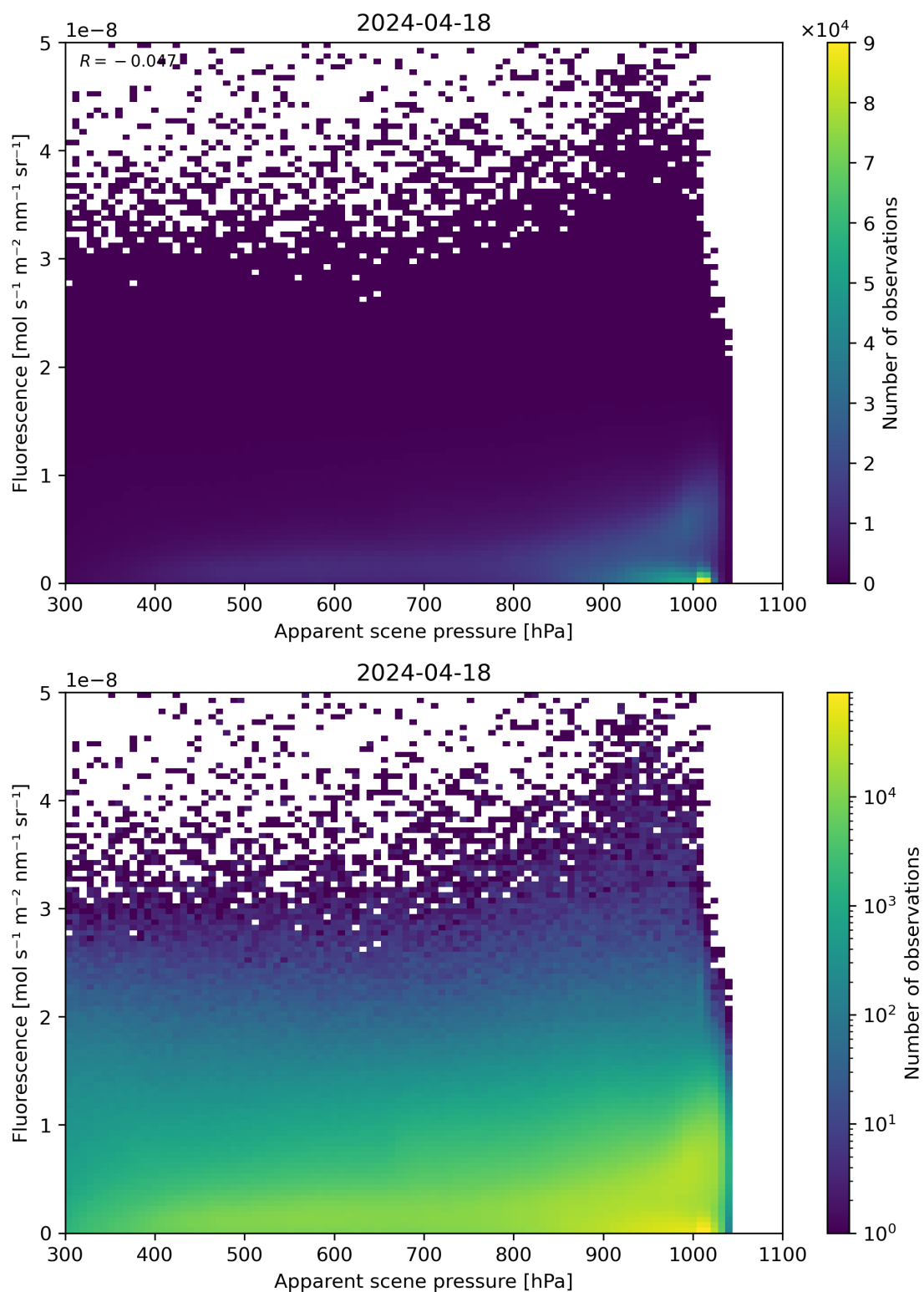
Figure 64: Scatter density plot of “Apparent scene pressure” against “Fluorescence” for 2024-04-17 to 2024-04-19.
