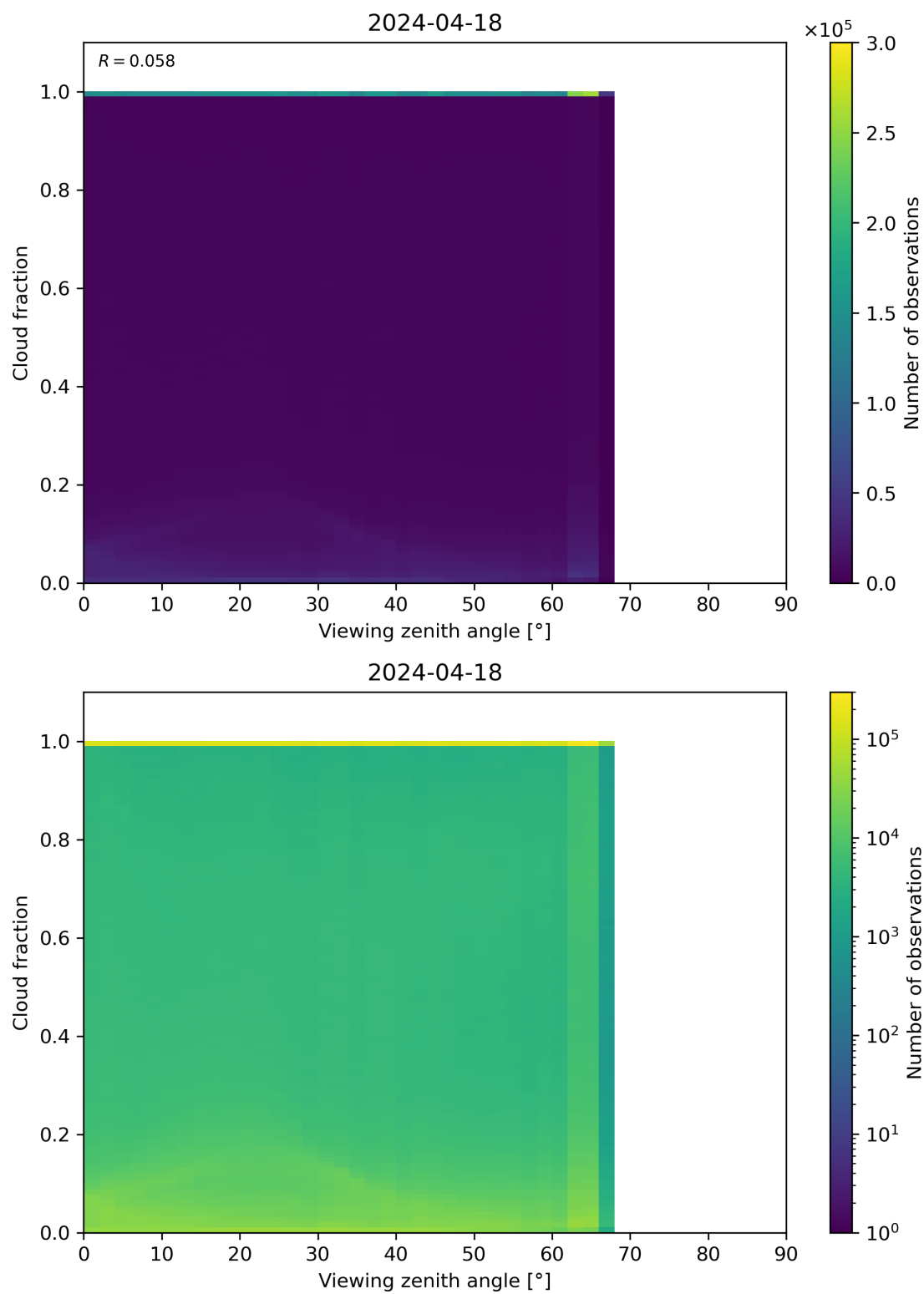
Figure 120: Scatter density plot of “Viewing zenith angle” against “Cloud fraction” for 2024-04-17 to 2024-04-19.
