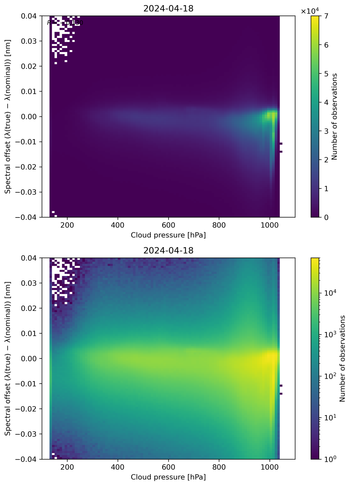
Figure 84: Scatter density plot of “Cloud pressure” against “Spectral offset ( \lambda(\text{true}) - \lambda(\text{nominal}) )” for 2024-04-17 to 2024-04-19.
