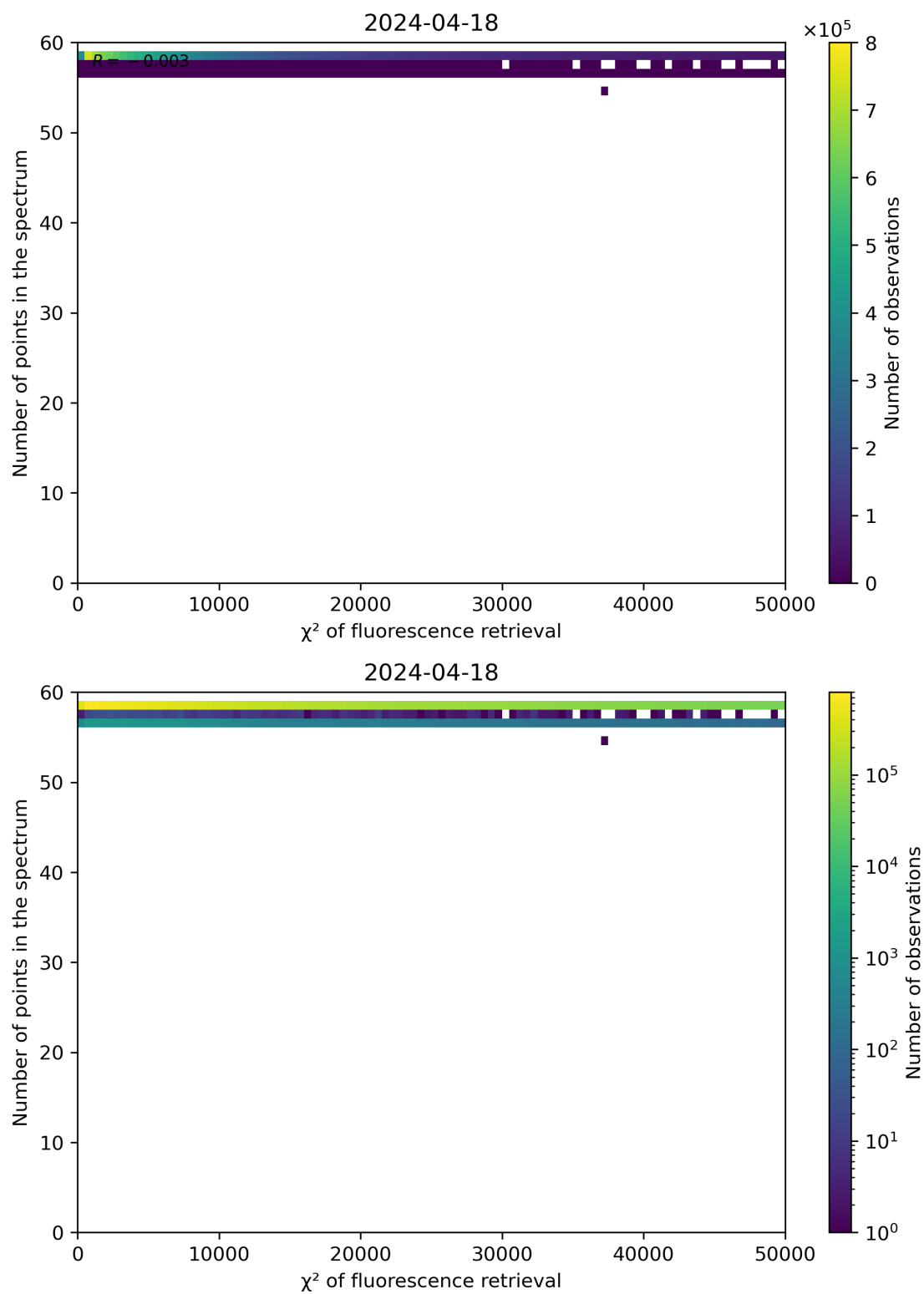
Figure 68: Scatter density plot of “ \chi^2 of fluorescence retrieval” against “Number of points in the spectrum” for 2024-04-17 to 2024-04-19.
