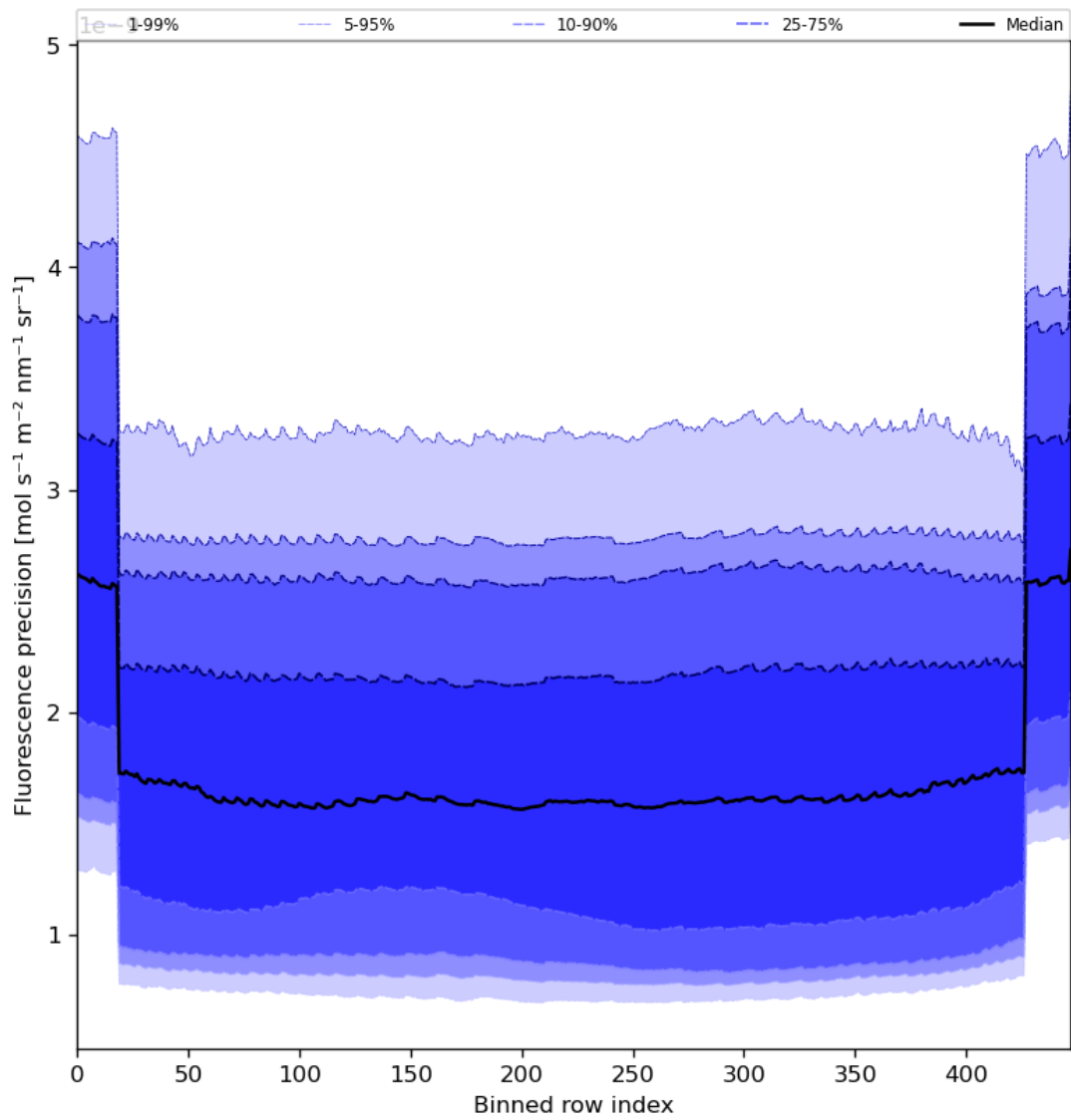
Figure 58: Along track statistics of “Fluorescence precision” for 2024-04-17 to 2024-04-19
