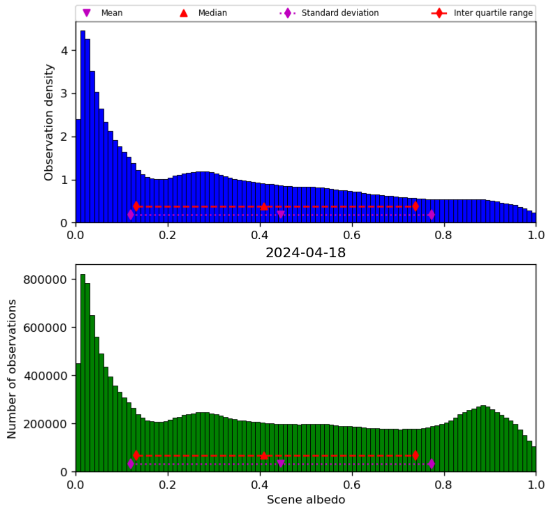
Figure 34: Histogram of “Scene albedo” for 2024-04-17 to 2024-04-19
