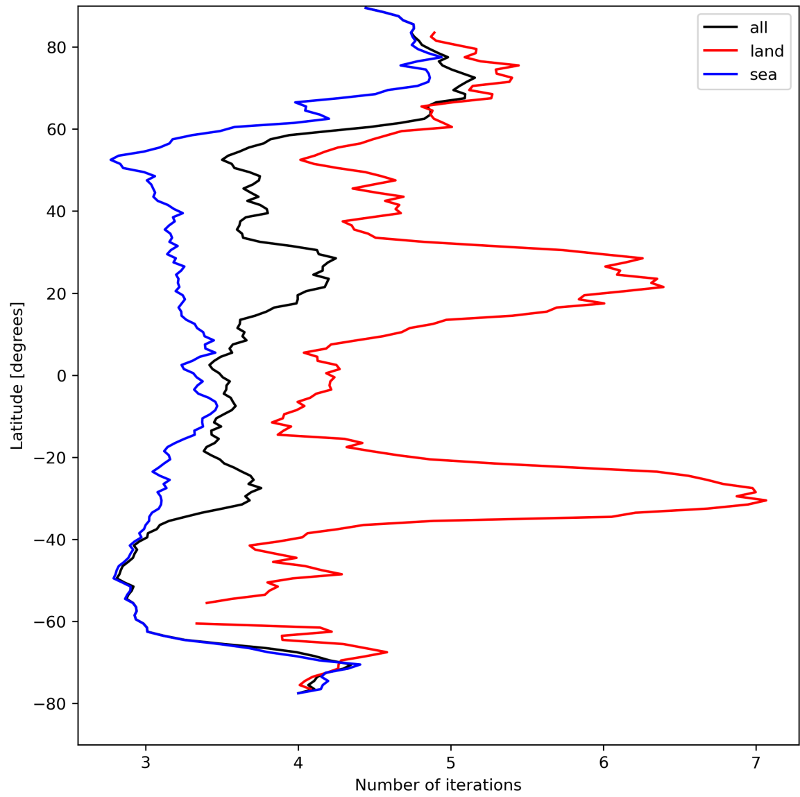
Figure 22: Zonal average of “Number of iterations” for 2024-04-17 to 2024-04-19.
