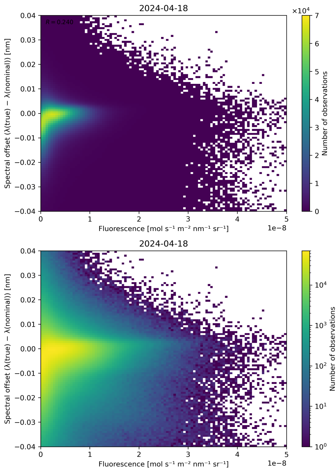
Figure 87: Scatter density plot of “Fluorescence” against “Spectral offset ( \lambda(\text{true}) - \lambda(\text{nominal}) )” for 2024-04-17 to 2024-04-19.
