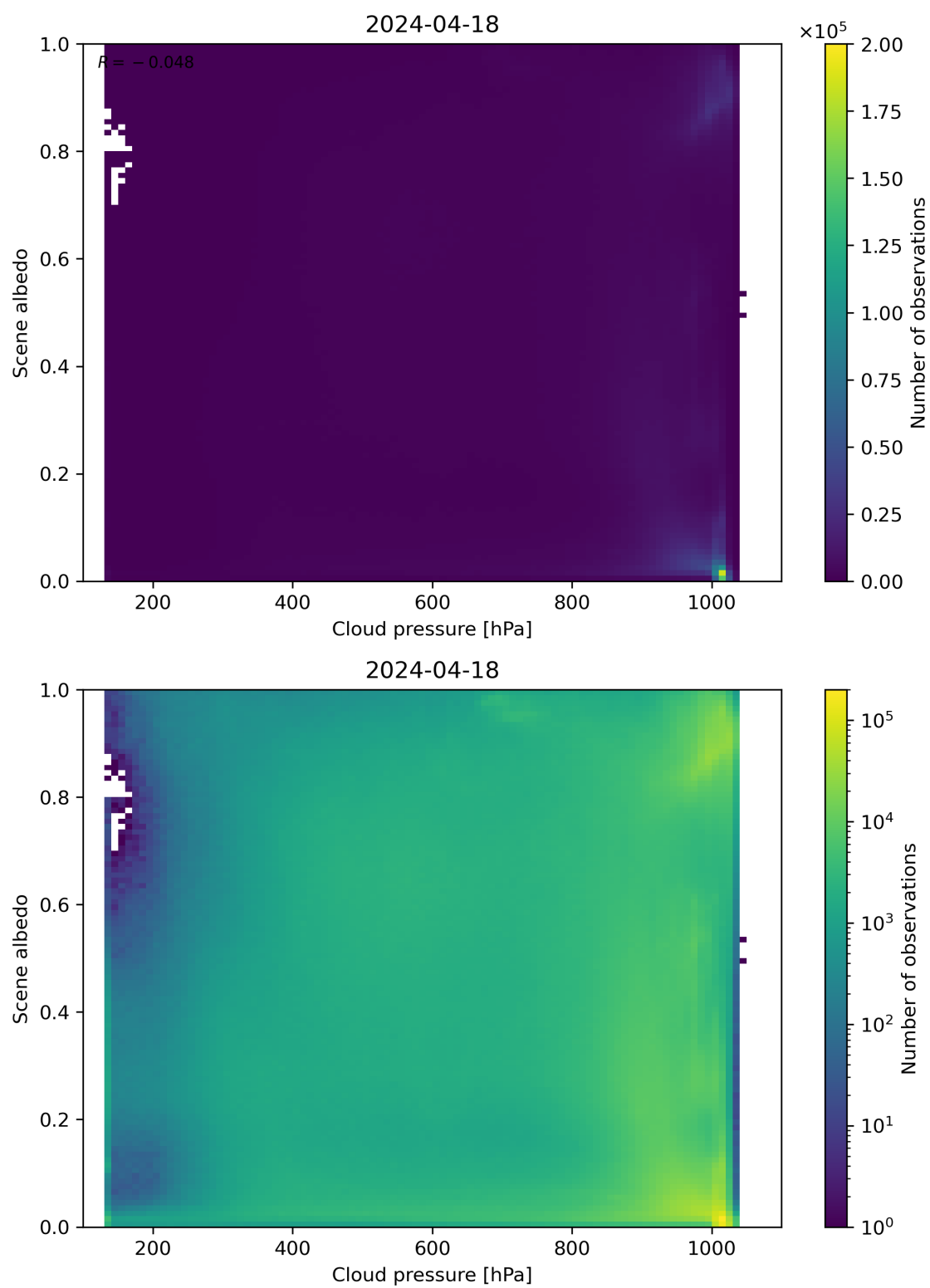
Figure 83: Scatter density plot of “Cloud pressure” against “Scene albedo” for 2024-04-17 to 2024-04-19.
