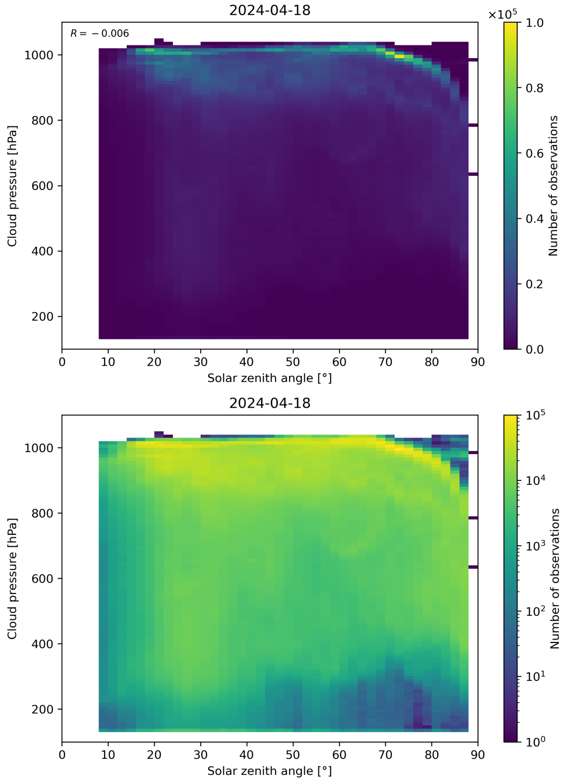
Figure 111: Scatter density plot of “Solar zenith angle” against “Cloud pressure” for 2024-04-17 to 2024-04-19.
