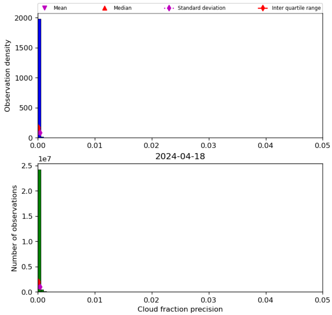
Figure 33: Histogram of “Cloud fraction precision” for 2024-04-17 to 2024-04-19
