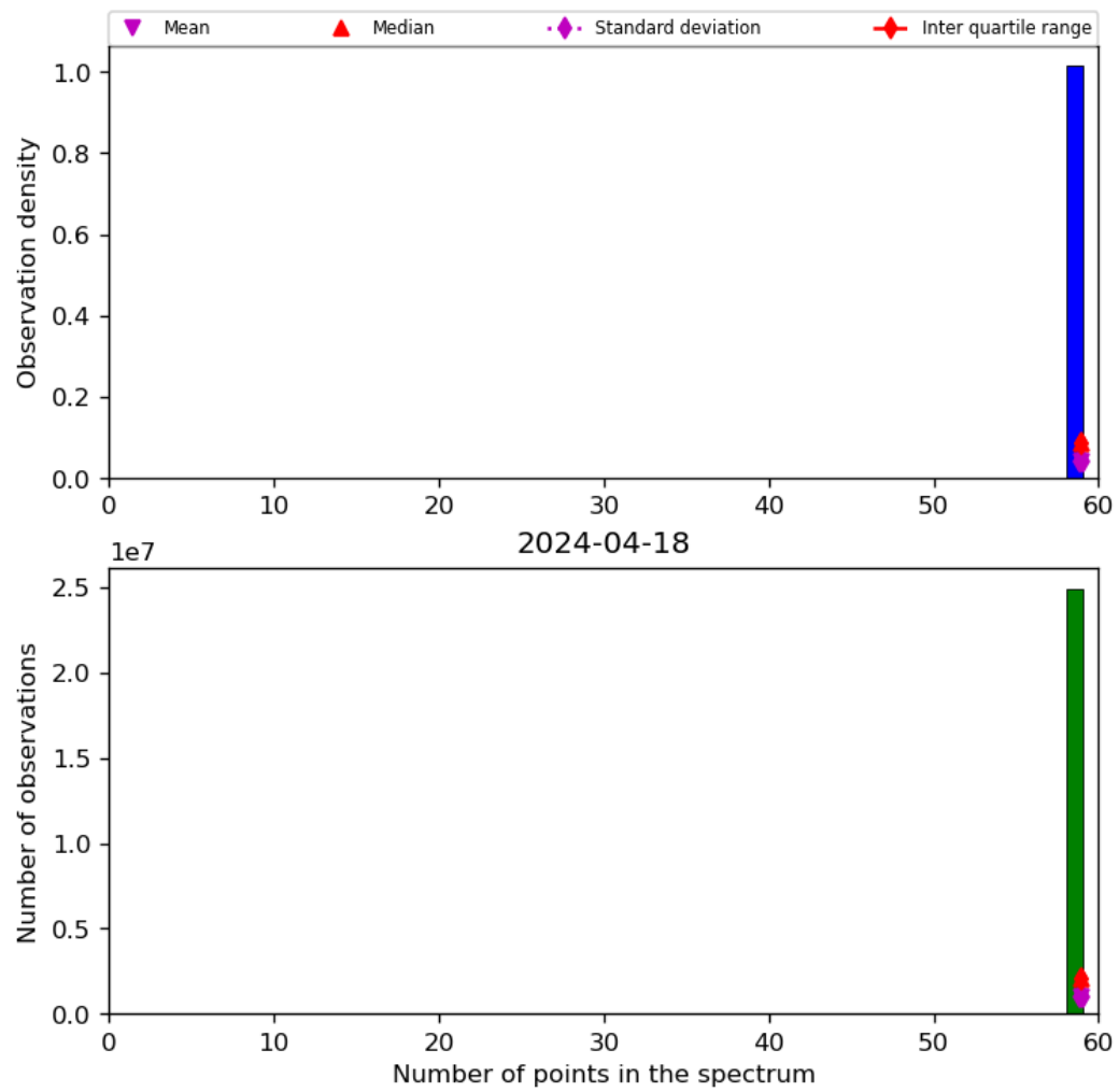
Figure 44: Histogram of “Number of points in the spectrum” for 2024-04-17 to 2024-04-19
