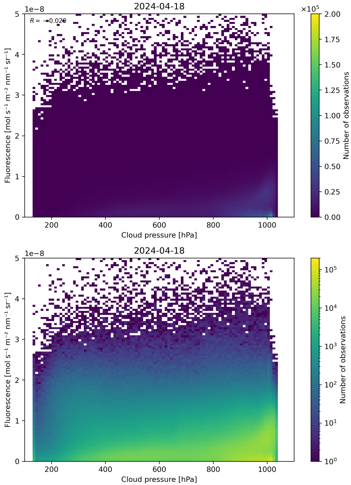
Figure 80: Scatter density plot of “Cloud pressure” against “Fluorescence” for 2024-04-17 to 2024-04-19.
