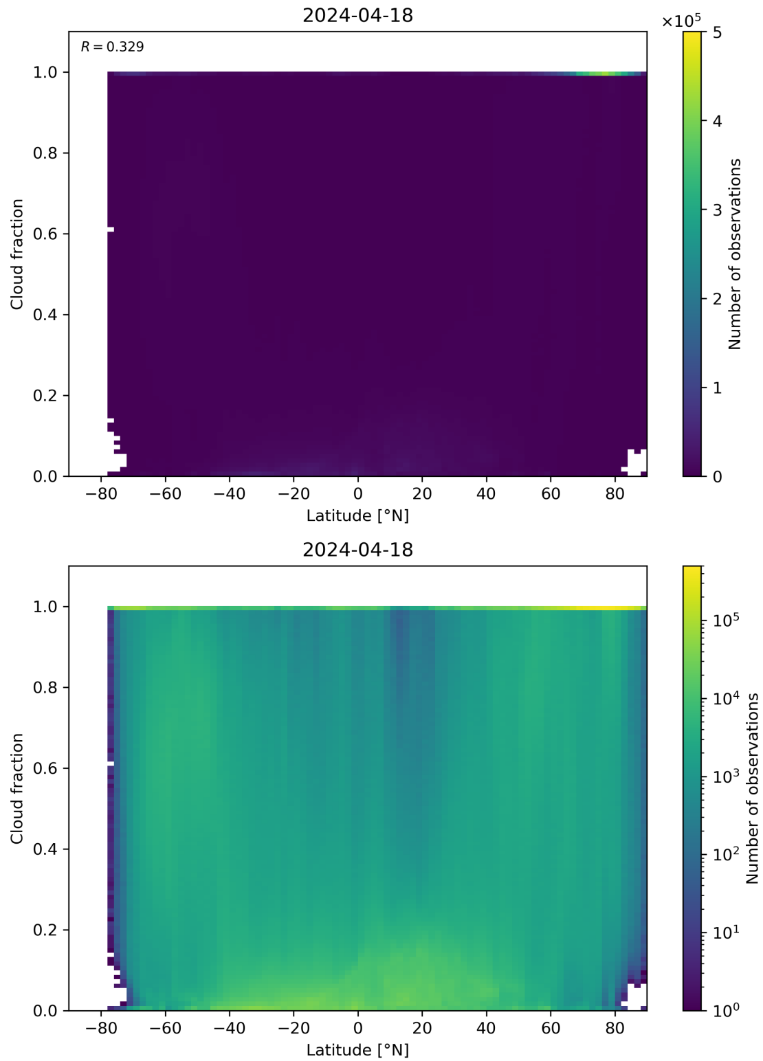
Figure 90: Scatter density plot of “Latitude” against “Cloud fraction” for 2024-04-17 to 2024-04-19.
