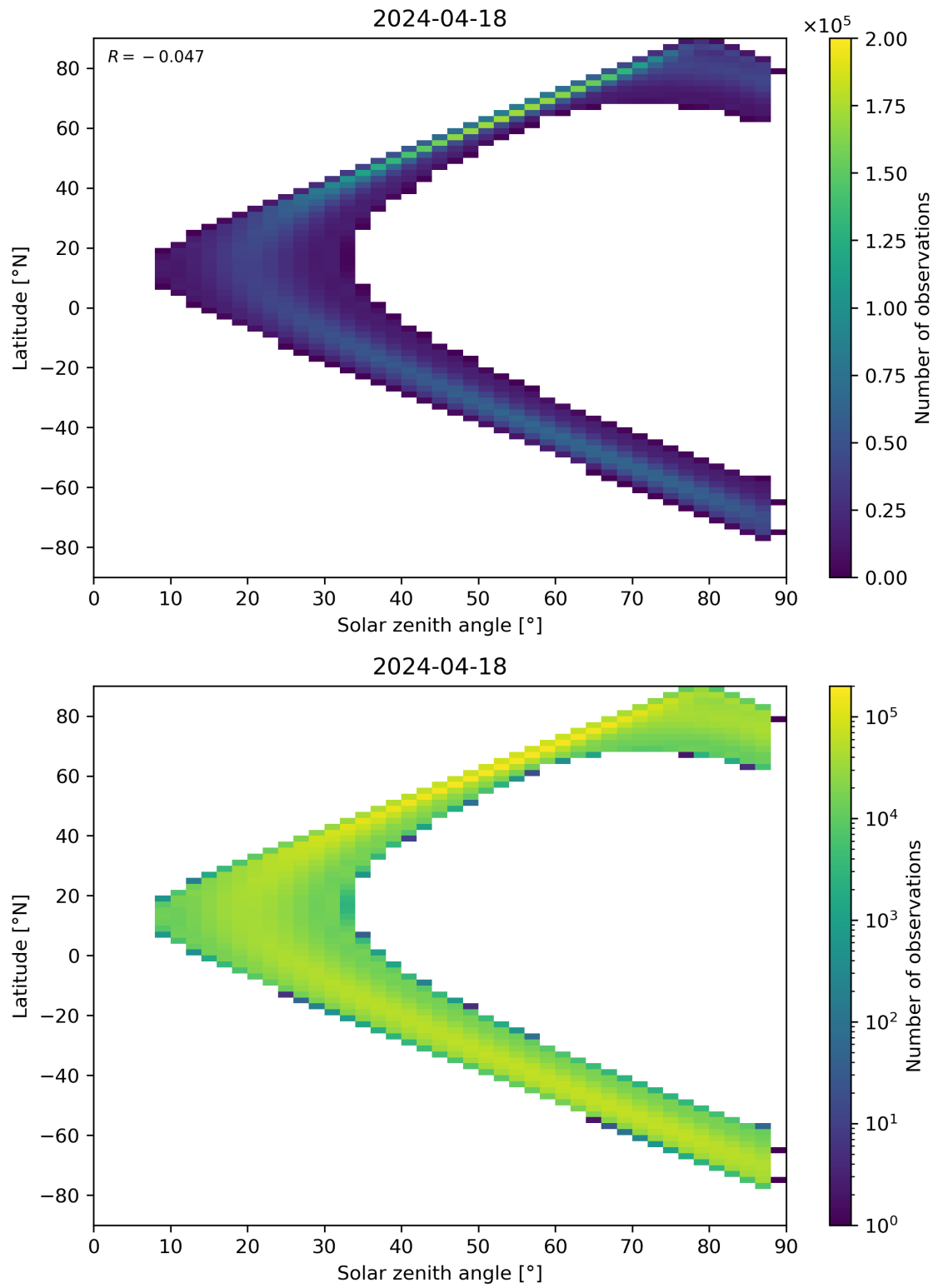
Figure 113: Scatter density plot of “Solar zenith angle” against “Latitude” for 2024-04-17 to 2024-04-19.
