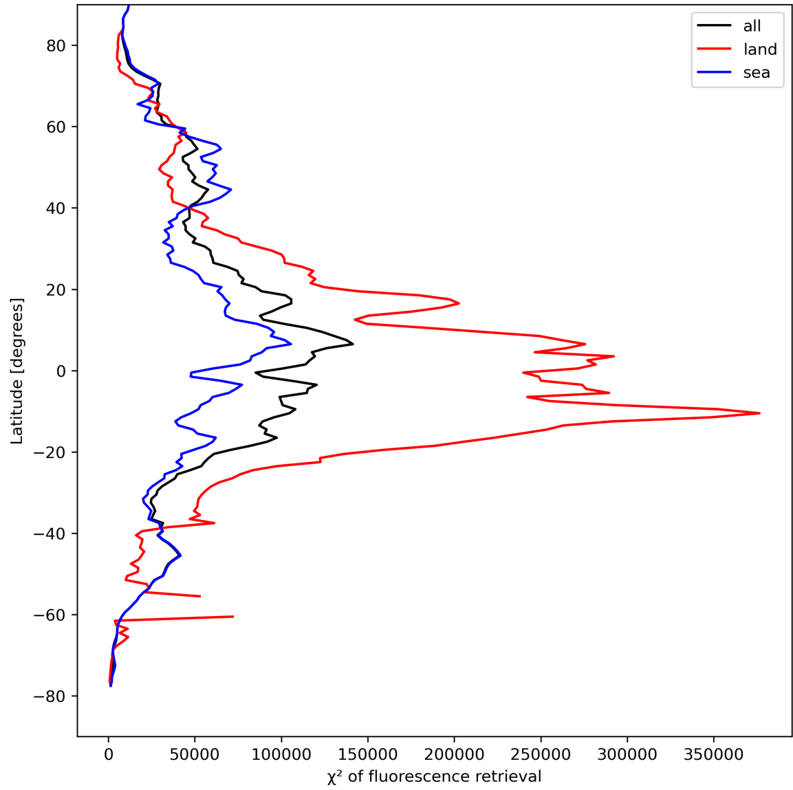
Figure 25: Zonal average of “ \chi^2 of fluorescence retrieval” for 2024-04-17 to 2024-04-19.
