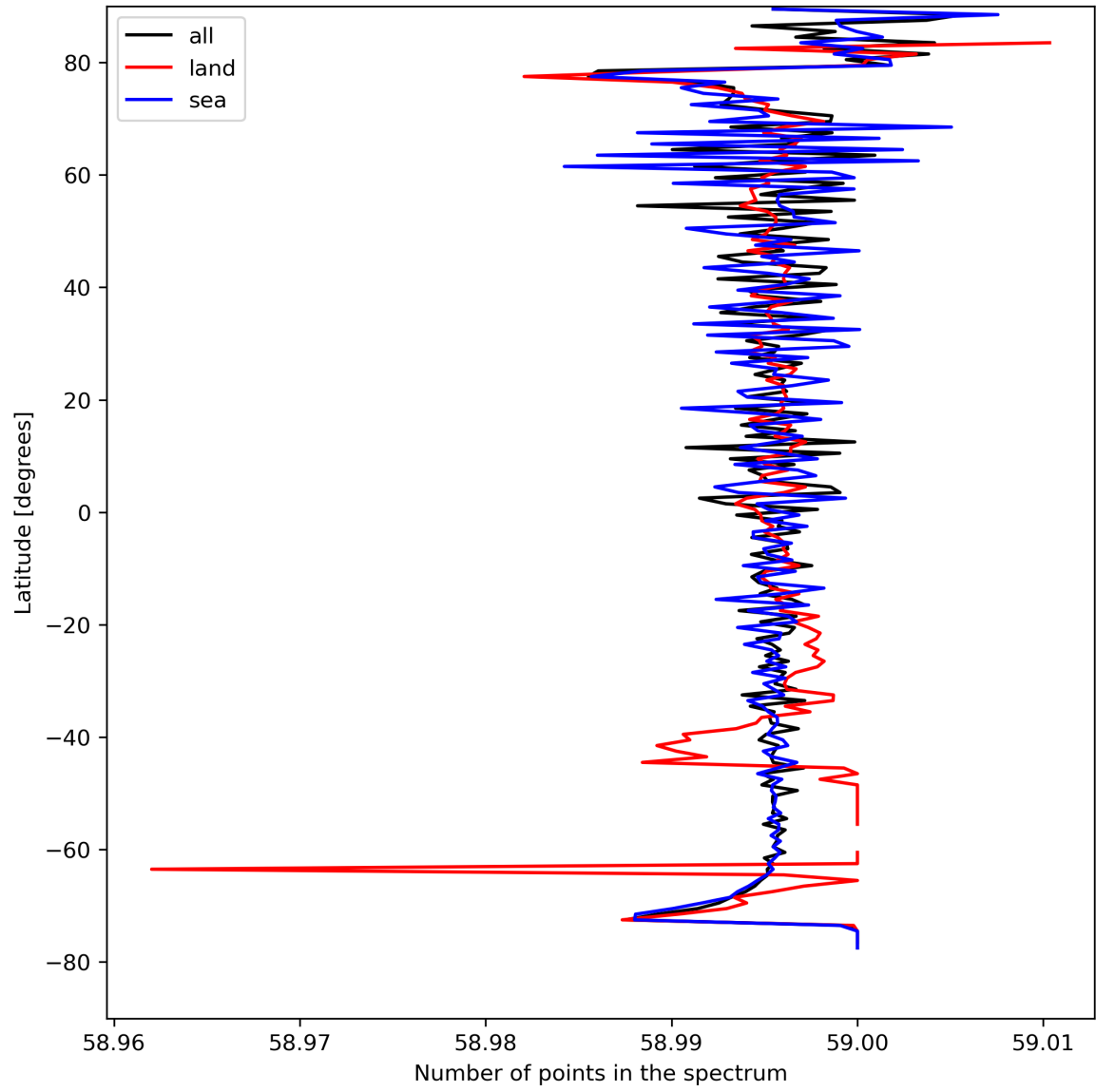
Figure 27: Zonal average of “Number of points in the spectrum” for 2024-04-17 to 2024-04-19.
