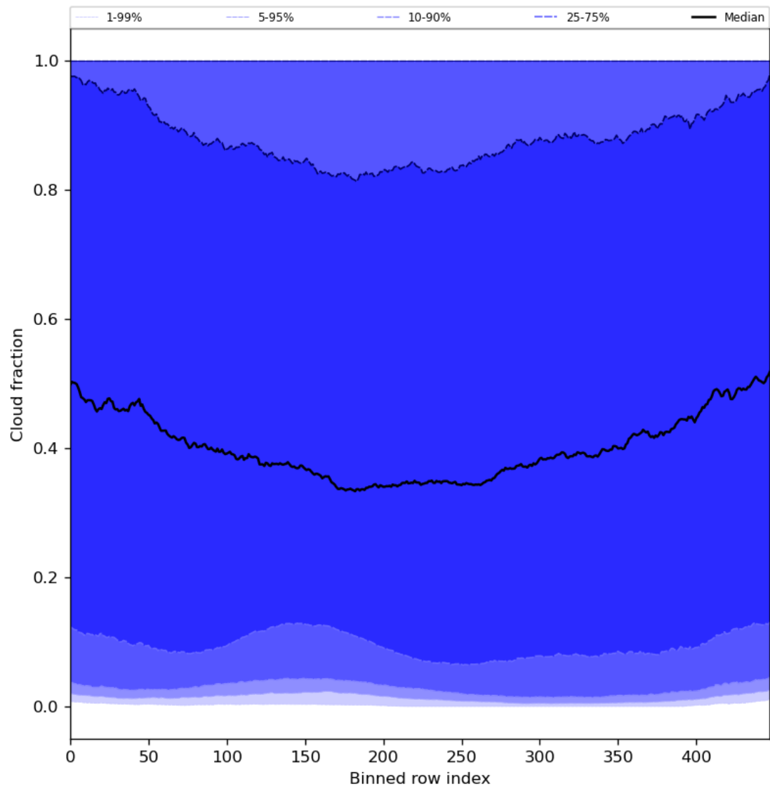
Figure 49: Along track statistics of “Cloud fraction” for 2024-04-17 to 2024-04-19
