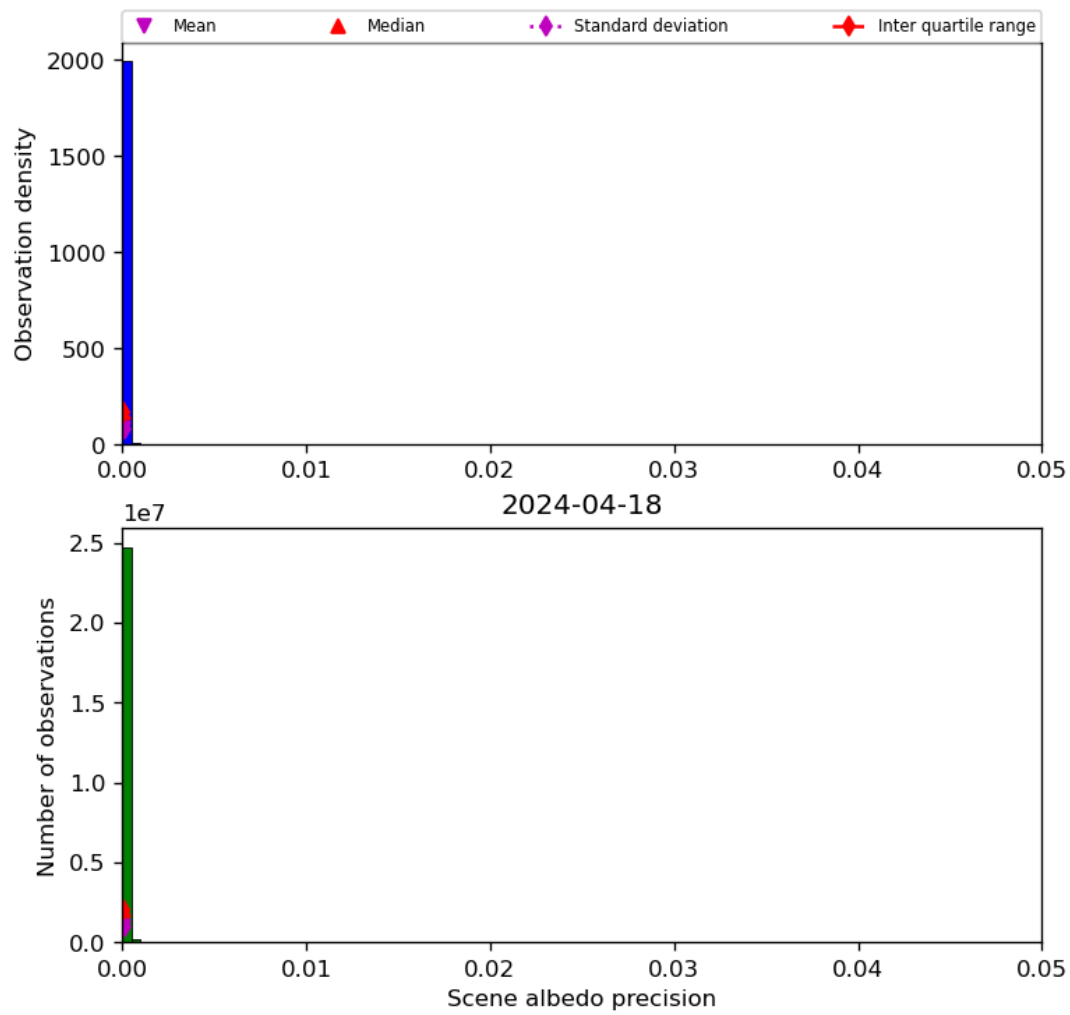
Figure 35: Histogram of “Scene albedo precision” for 2024-04-17 to 2024-04-19
