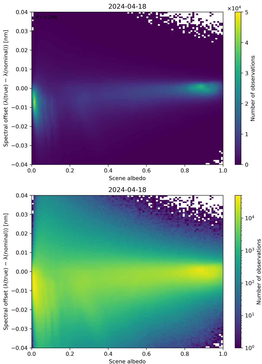
Figure 107: Scatter density plot of “Scene albedo” against “Spectral offset ( \lambda(\text{true}) - \lambda(\text{nominal}) )” for 2024-04-17 to 2024-04-19.
