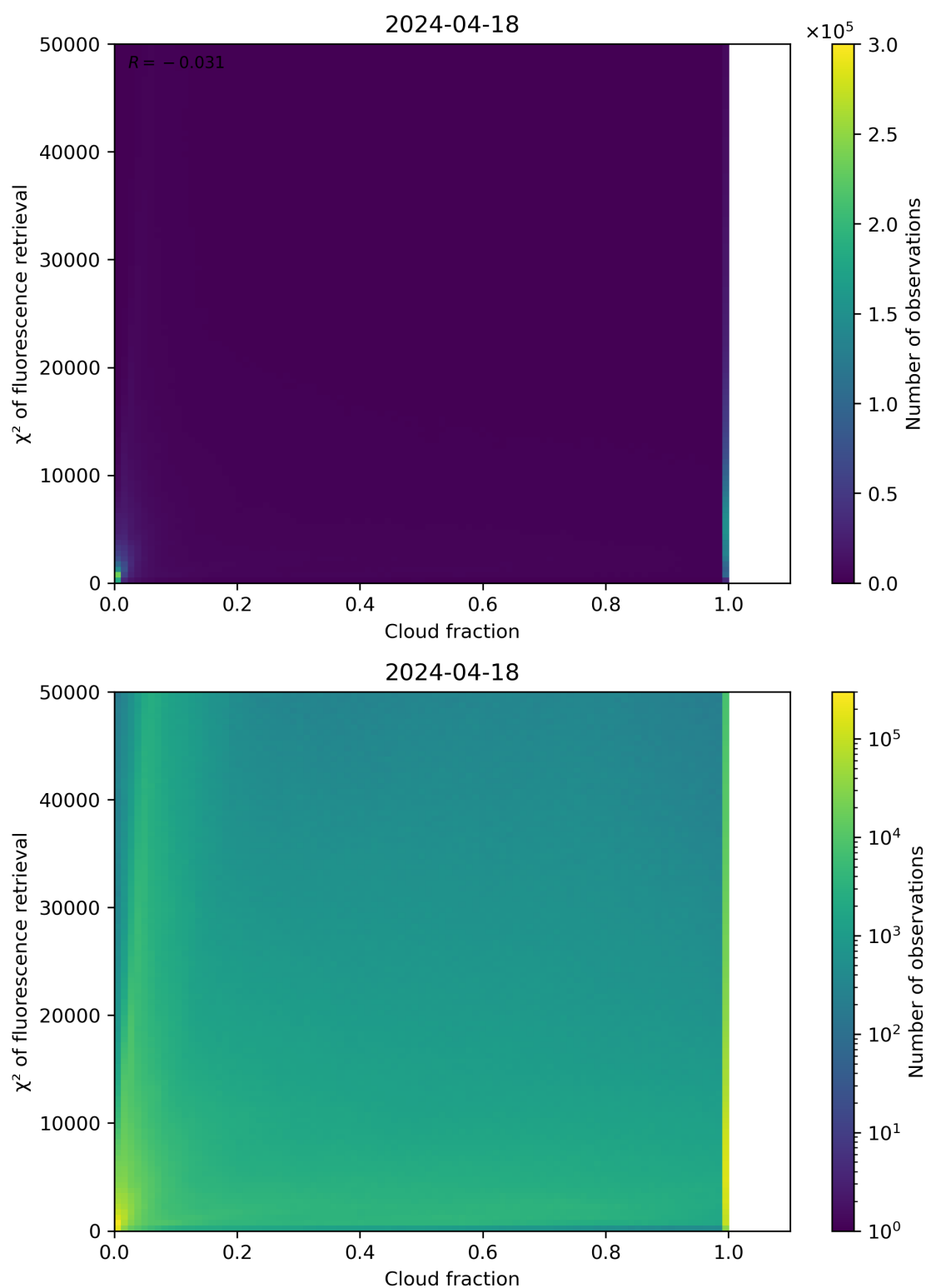
Figure 71: Scatter density plot of “Cloud fraction” against “ \chi^2 of fluorescence retrieval” for 2024-04-17 to 2024-04-19.
