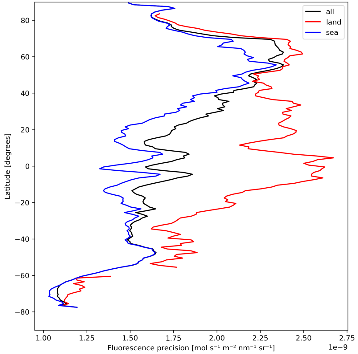
Figure 24: Zonal average of “Fluorescence precision” for 2024-04-17 to 2024-04-19.
