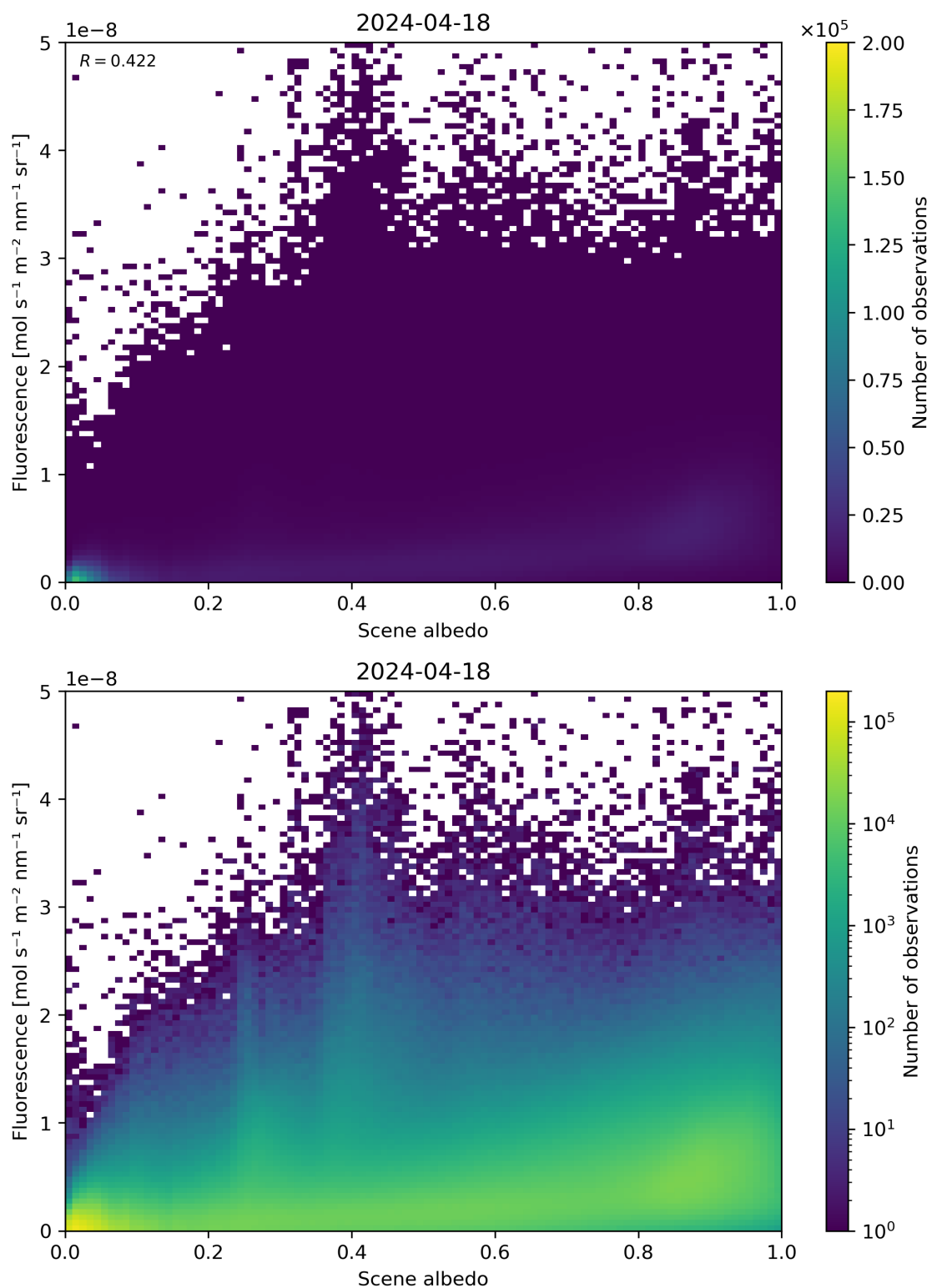
Figure 104: Scatter density plot of “Scene albedo” against “Fluorescence” for 2024-04-17 to 2024-04-19.
