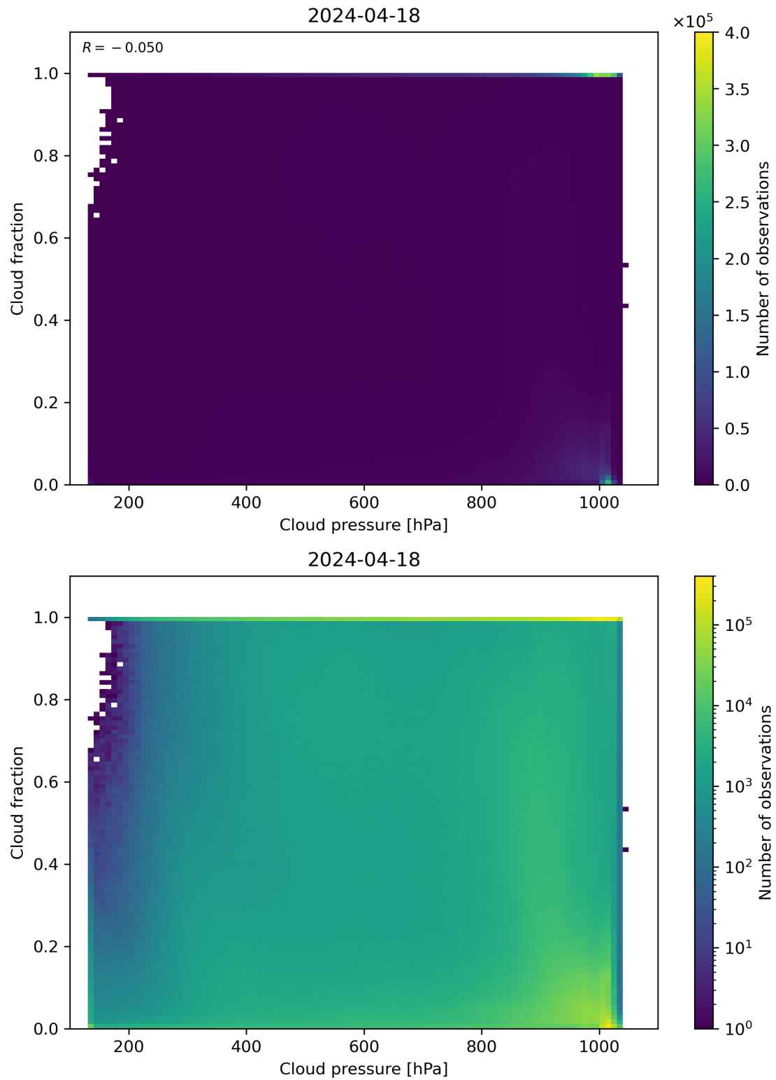
Figure 79: Scatter density plot of “Cloud pressure” against “Cloud fraction” for 2024-04-17 to 2024-04-19.
