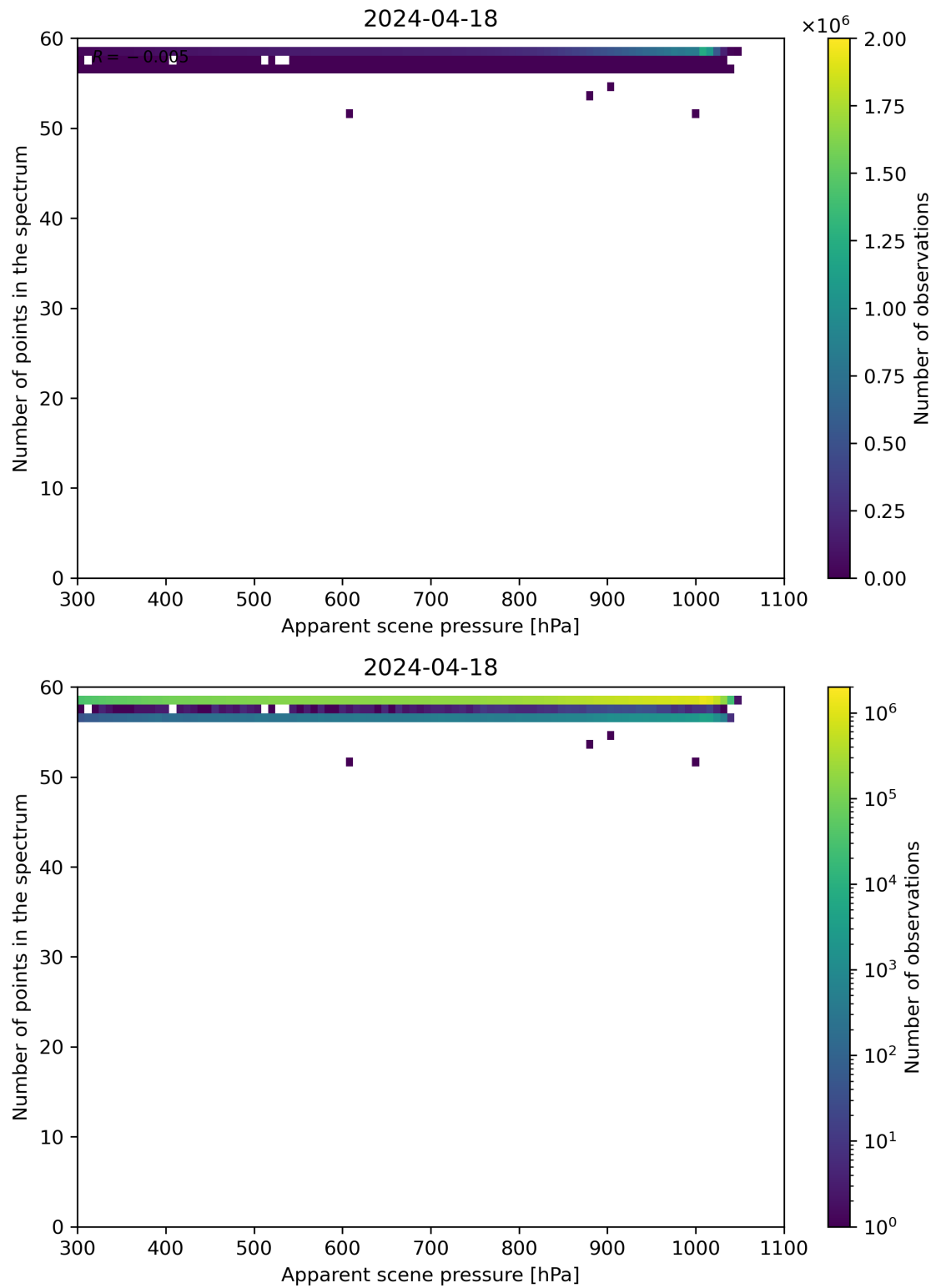
Figure 66: Scatter density plot of “Apparent scene pressure” against “Number of points in the spectrum” for 2024-04-17 to 2024-04-19.
