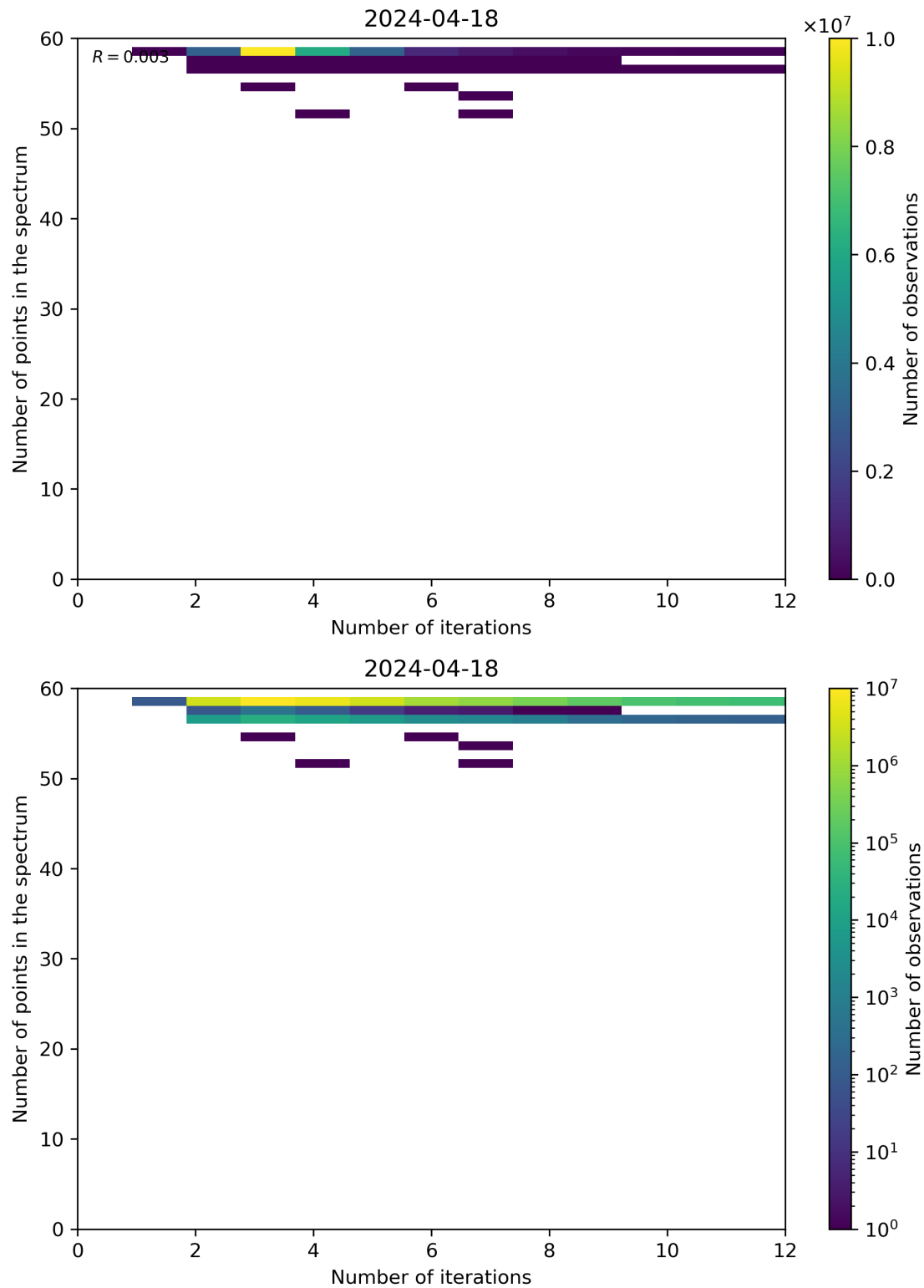
Figure 99: Scatter density plot of “Number of iterations” against “Number of points in the spectrum” for 2024-04-17 to 2024-04-19.
