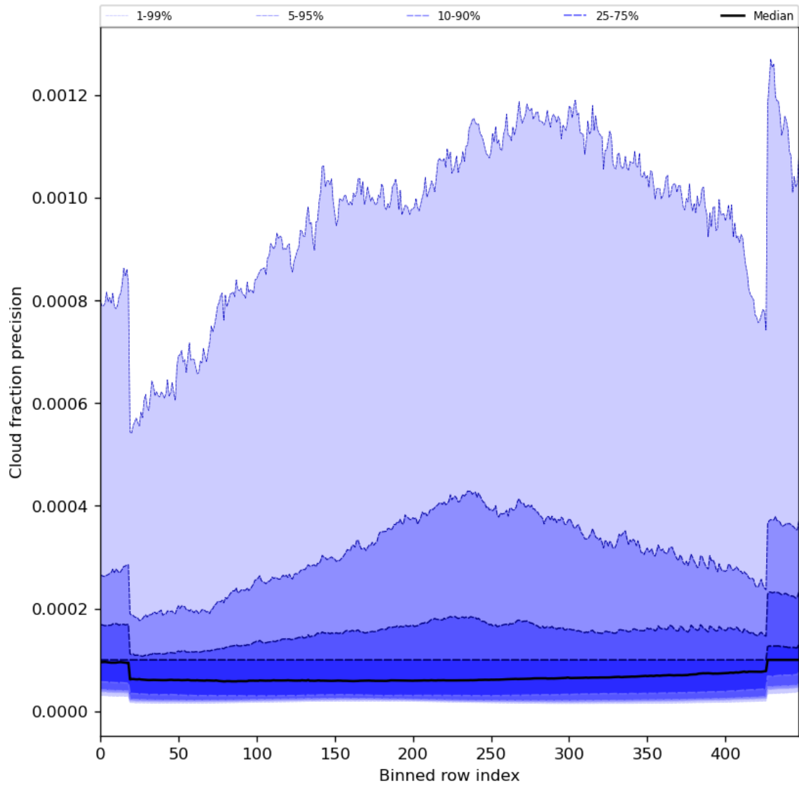
Figure 50: Along track statistics of “Cloud fraction precision” for 2024-04-17 to 2024-04-19
