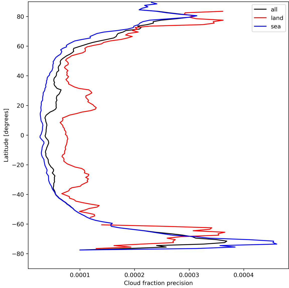
Figure 16: Zonal average of “Cloud fraction precision” for 2024-04-17 to 2024-04-19.
