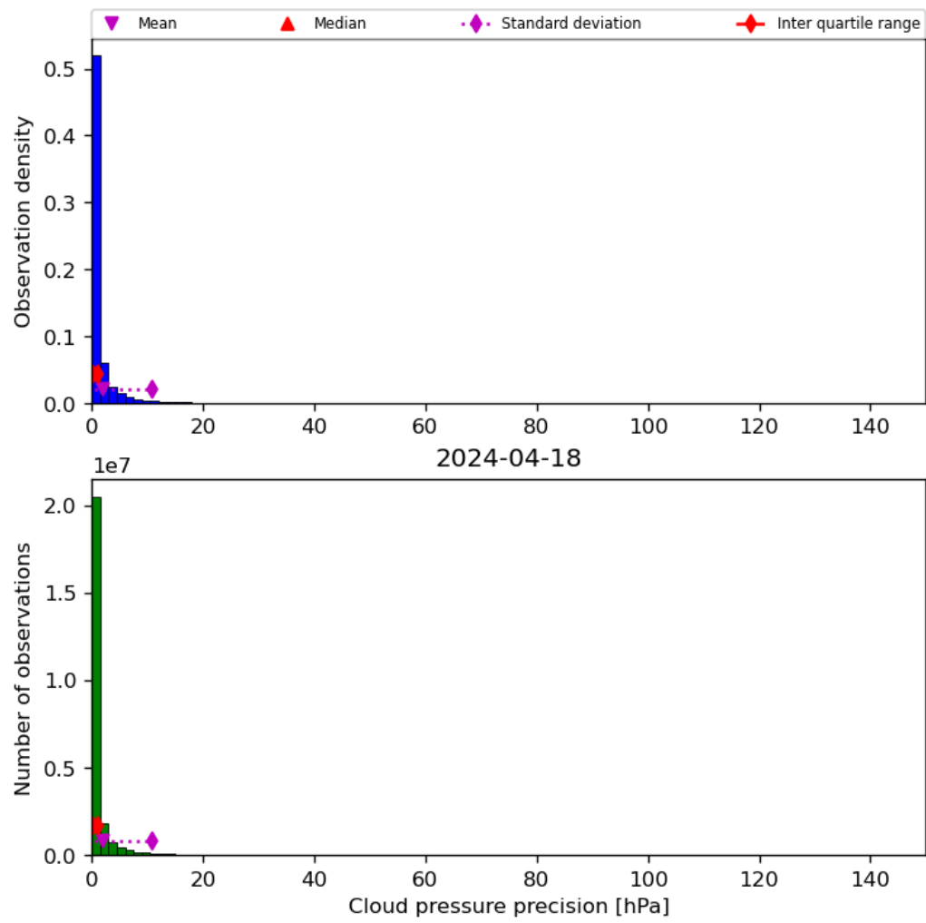
Figure 31: Histogram of “Cloud pressure precision” for 2024-04-17 to 2024-04-19
