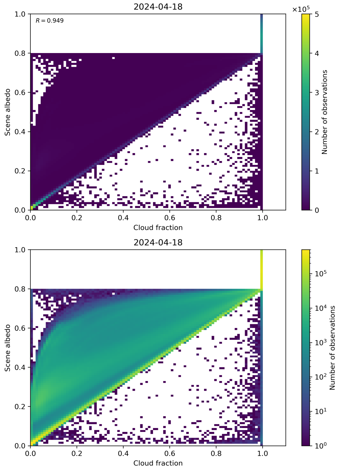
Figure 75: Scatter density plot of “Cloud fraction” against “Scene albedo” for 2024-04-17 to 2024-04-19.
