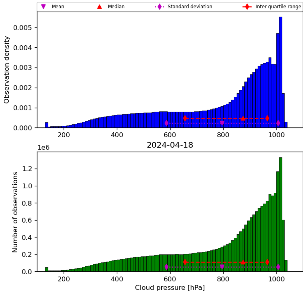
Figure 30: Histogram of “Cloud pressure” for 2024-04-17 to 2024-04-19
