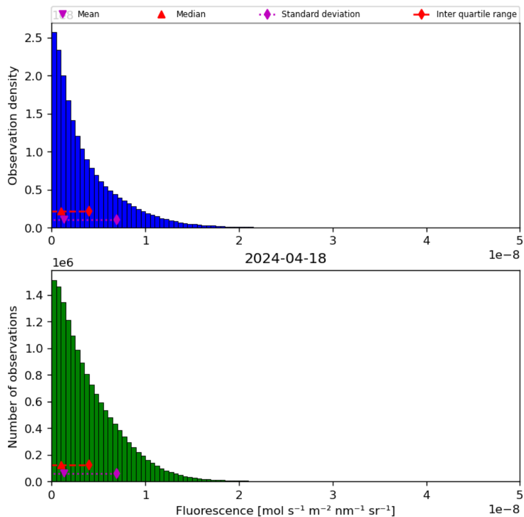
Figure 40: Histogram of “Fluorescence” for 2024-04-17 to 2024-04-19
