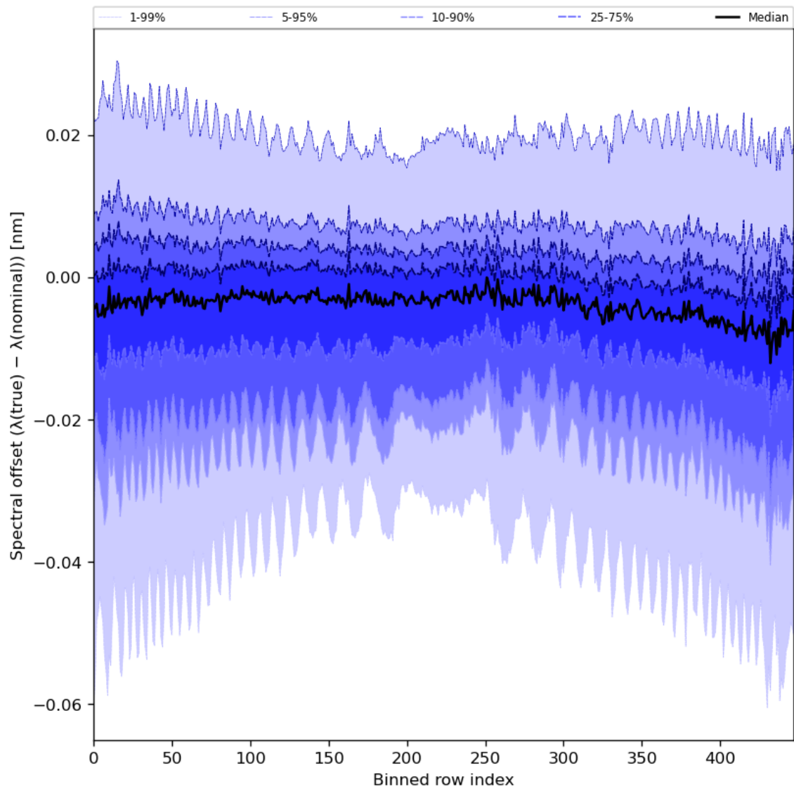
Figure 62: Along track statistics of “Spectral offset ( \lambda(\text{true}) - \lambda(\text{nominal}) )” for 2024-04-17 to 2024-04-19
