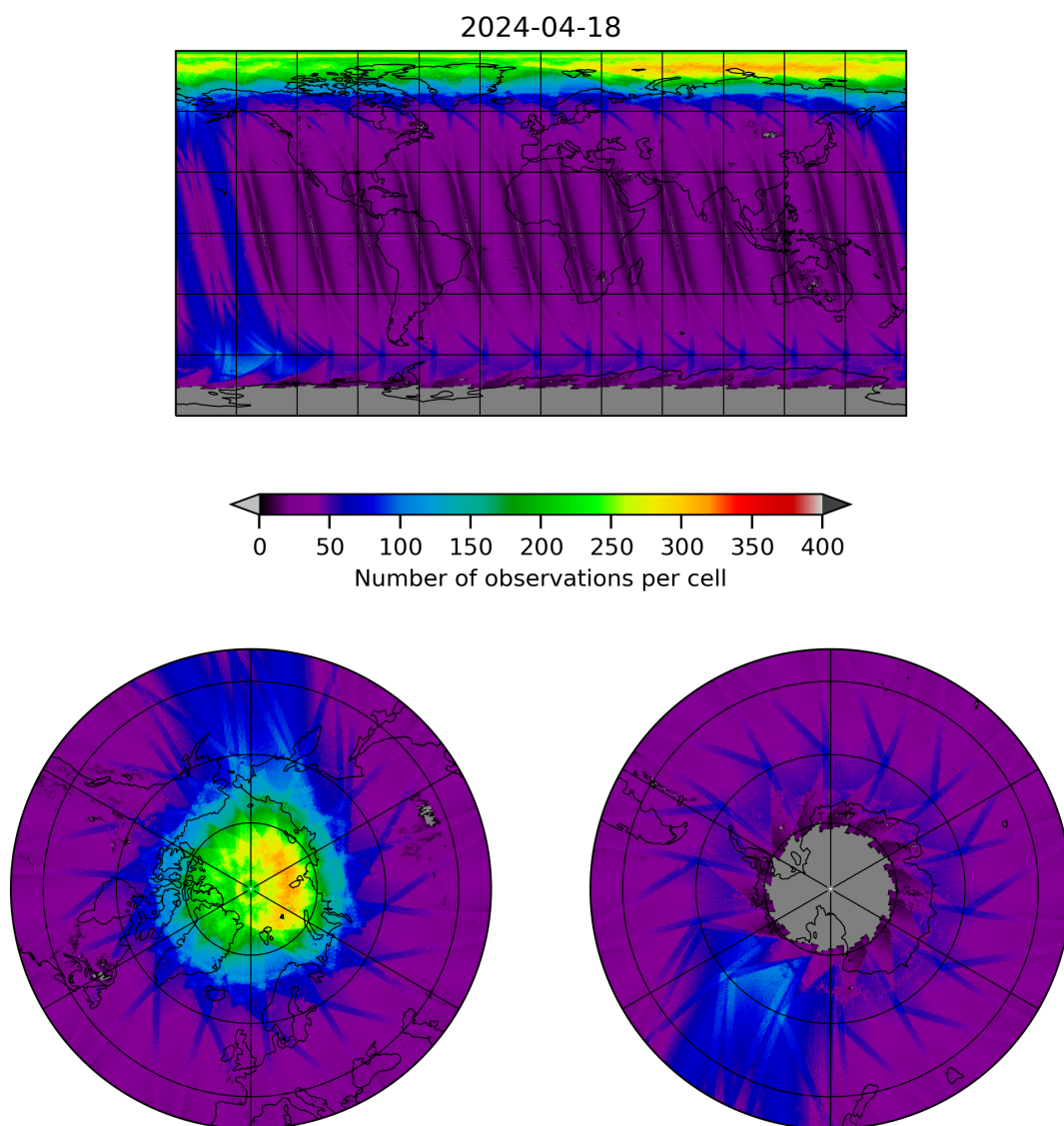
Figure 11: Map of the number of observations for 2024-04-17 to 2024-04-19
