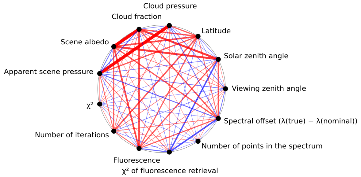
Figure 1: Map of correlation graph for 2024-04-17 to 2024-04-19.
