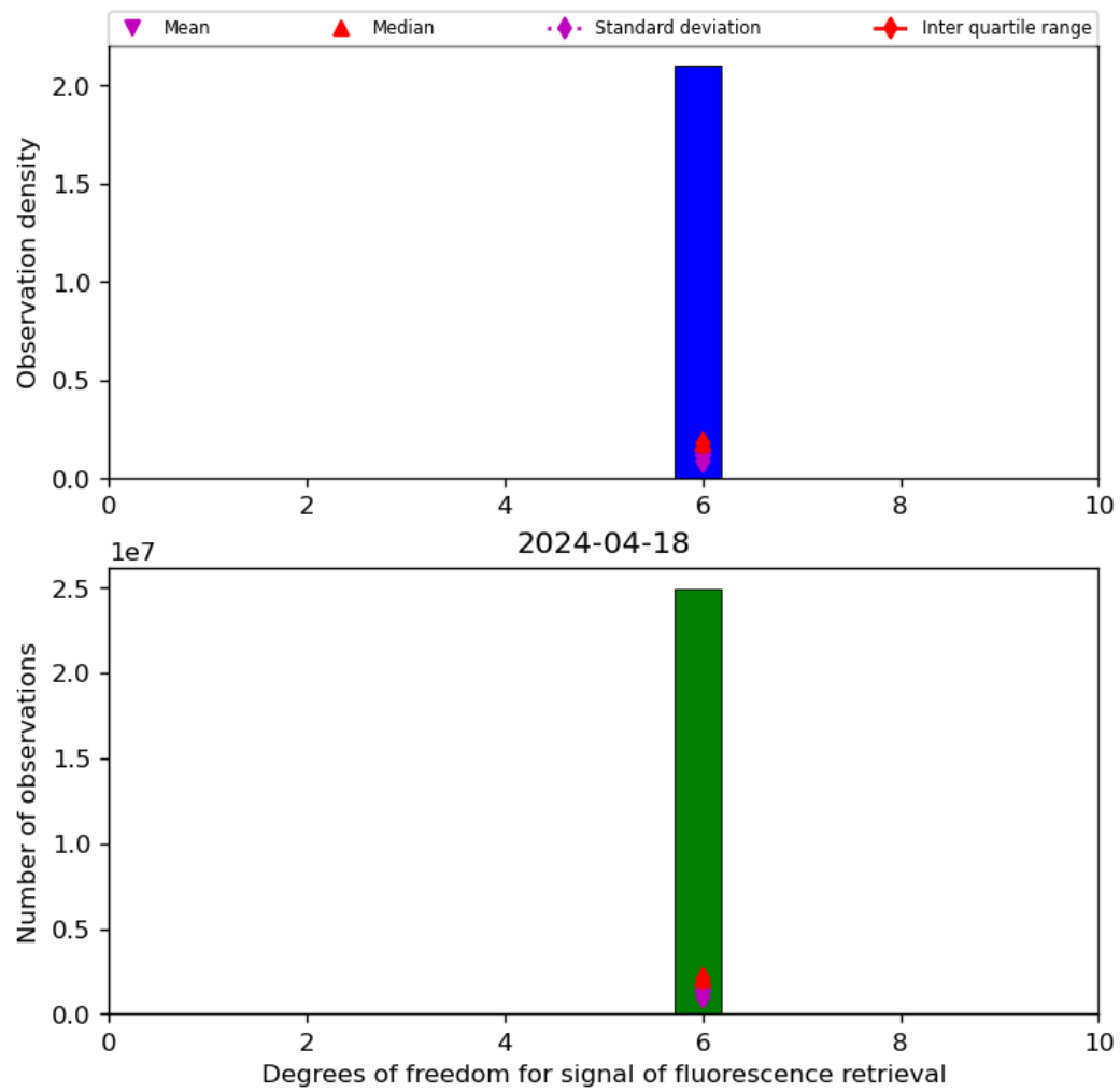
Figure 43: Histogram of "Degrees of freedom for signal of fluorescence retrieval" for 2024-04-17 to 2024-04-19
