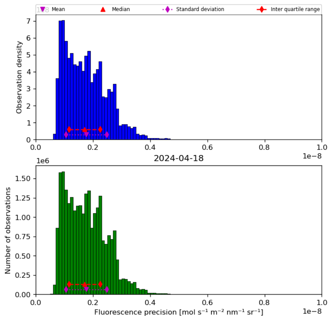
Figure 41: Histogram of “Fluorescence precision” for 2024-04-17 to 2024-04-19
