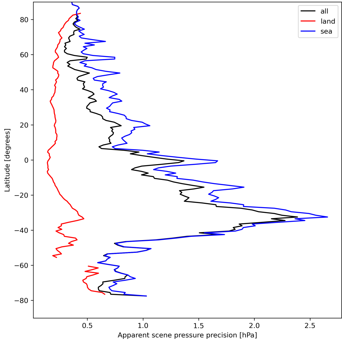
Figure 20: Zonal average of “Apparent scene pressure precision” for 2024-04-17 to 2024-04-19.
