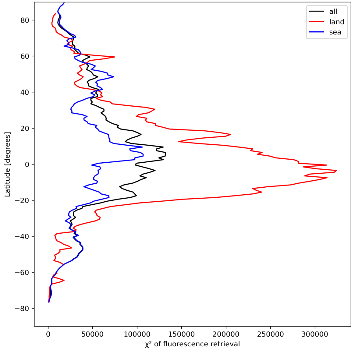
Figure 25: Zonal average of “ \chi^2 of fluorescence retrieval” for 2024-04-18 to 2024-04-20.
