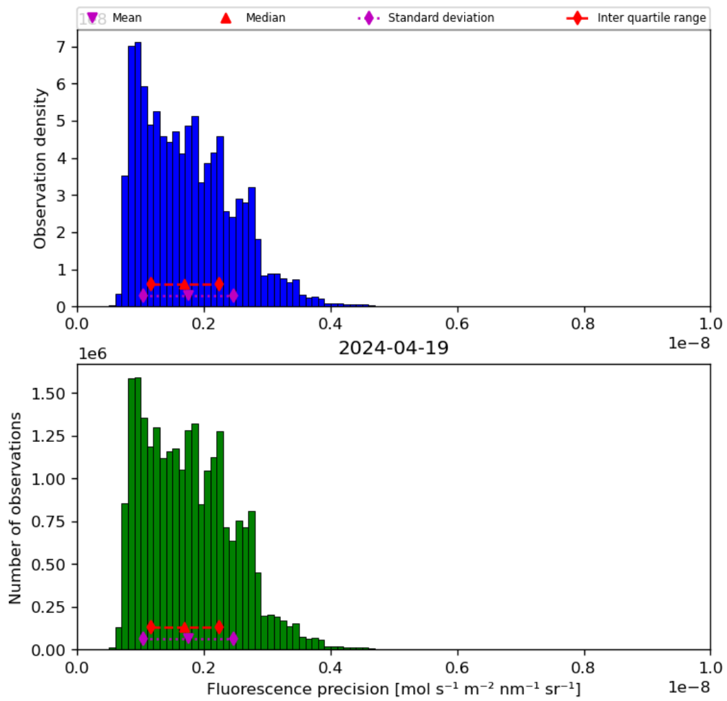
Figure 41: Histogram of “Fluorescence precision” for 2024-04-18 to 2024-04-20
