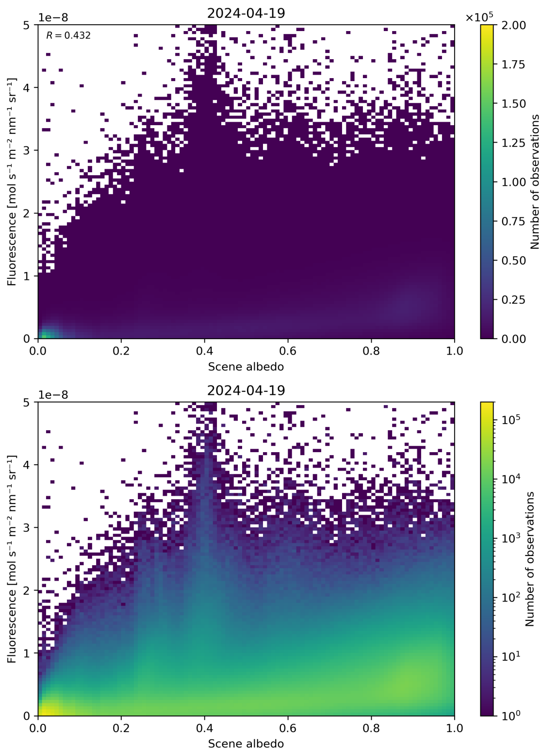
Figure 104: Scatter density plot of “Scene albedo” against “Fluorescence” for 2024-04-18 to 2024-04-20.
