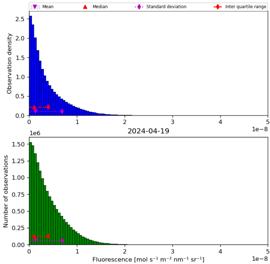
Figure 40: Histogram of “Fluorescence” for 2024-04-18 to 2024-04-20
