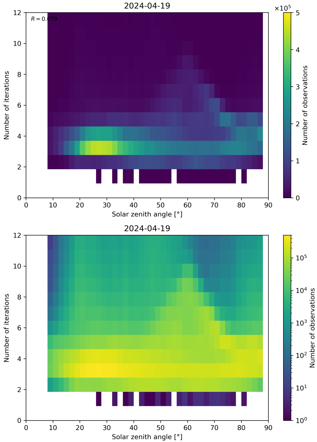
Figure 114: Scatter density plot of “Solar zenith angle” against “Number of iterations” for 2024-04-18 to 2024-04-20.
