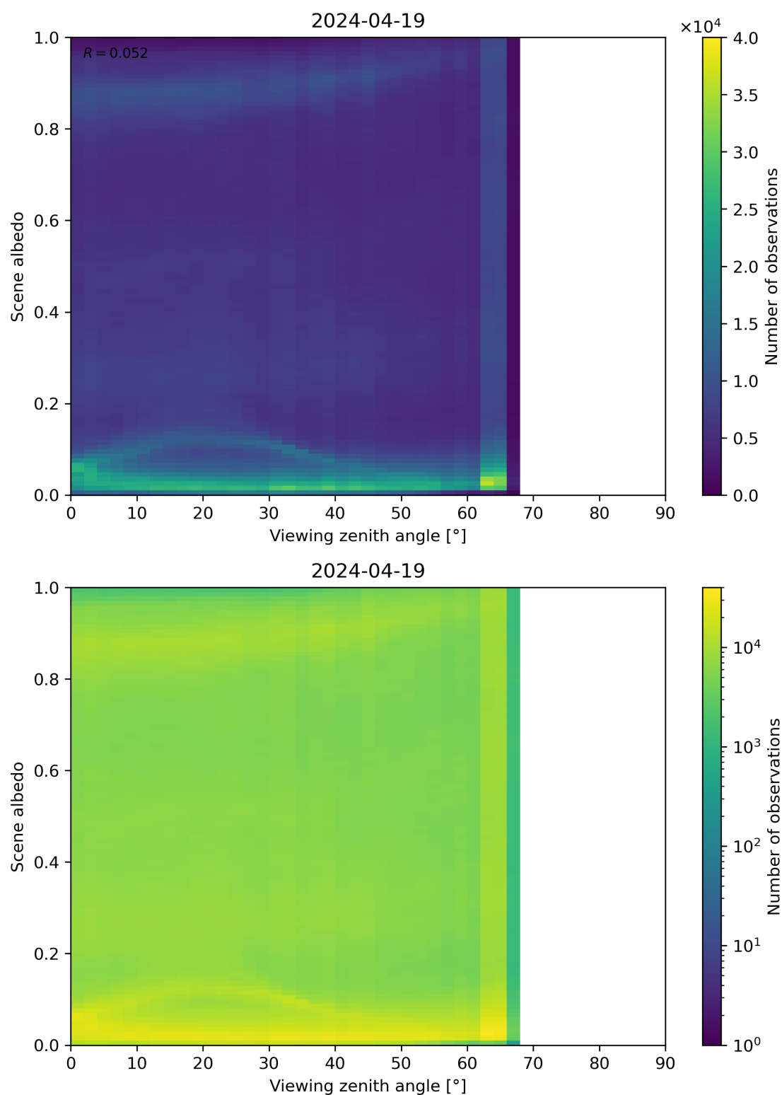
Figure 126: Scatter density plot of “Viewing zenith angle” against “Scene albedo” for 2024-04-18 to 2024-04-20.
