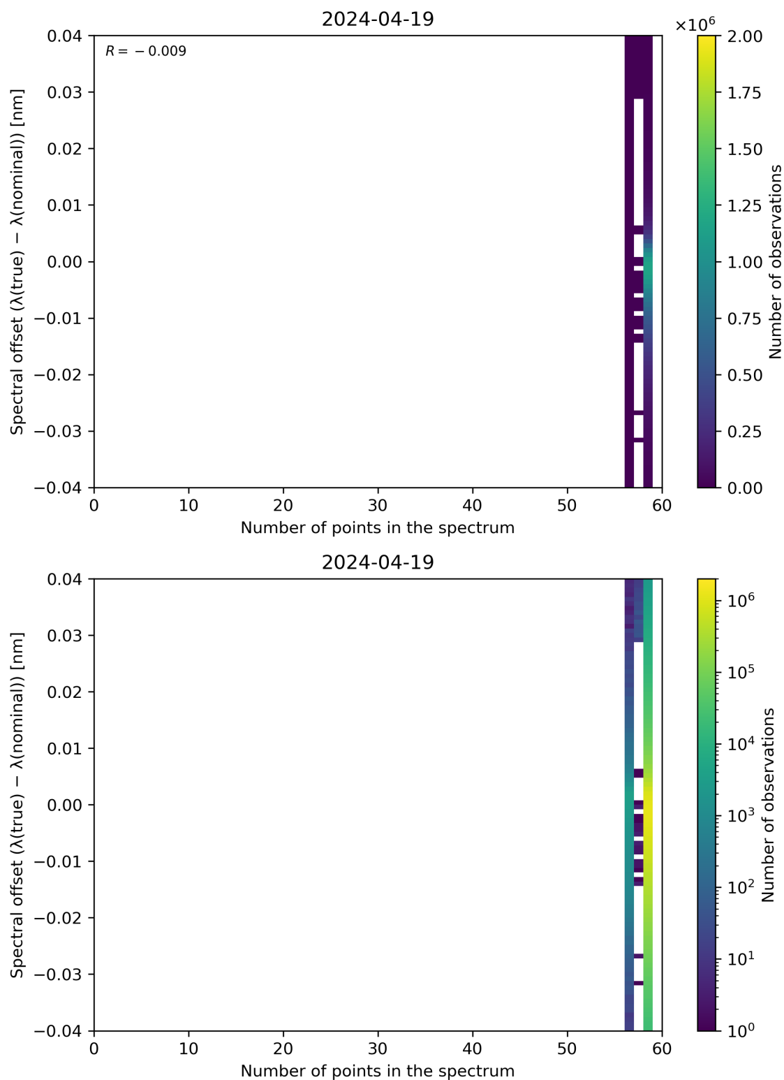
Figure 101: Scatter density plot of “Number of points in the spectrum” against “Spectral offset ( \lambda(\text{true}) - \lambda(\text{nominal}) )” for 2024-04-18 to 2024-04-20.
