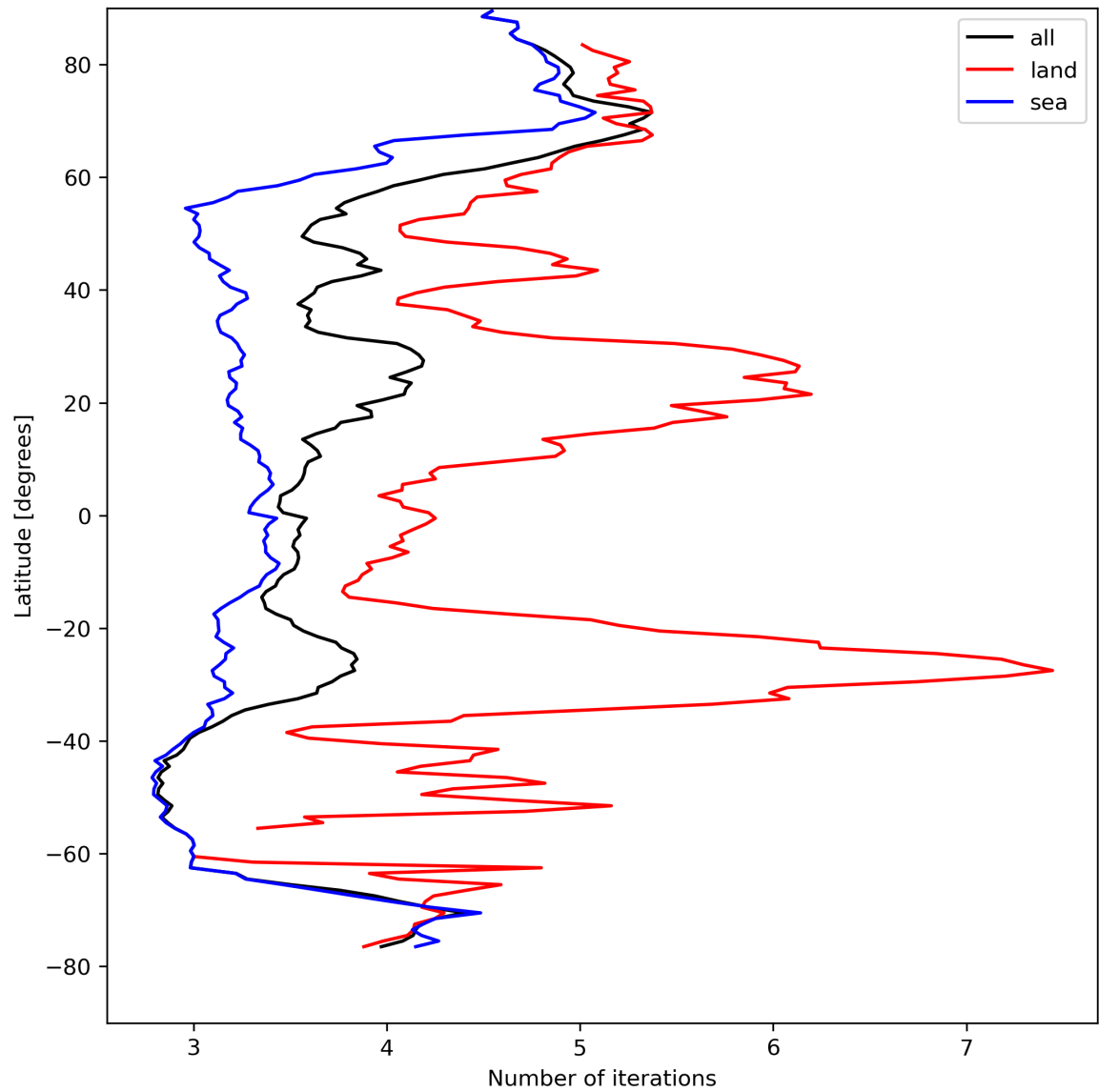
Figure 22: Zonal average of “Number of iterations” for 2024-04-18 to 2024-04-20.
