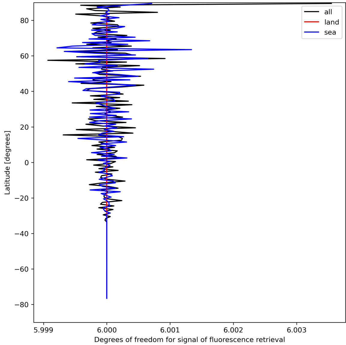
Figure 26: Zonal average of “Degrees of freedom for signal of fluorescence retrieval” for 2024-04-18 to 2024-04-20.
