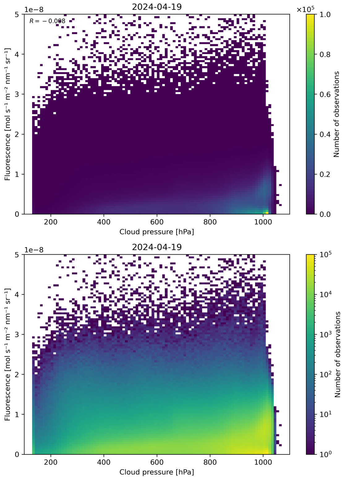
Figure 80: Scatter density plot of “Cloud pressure” against “Fluorescence” for 2024-04-18 to 2024-04-20.
