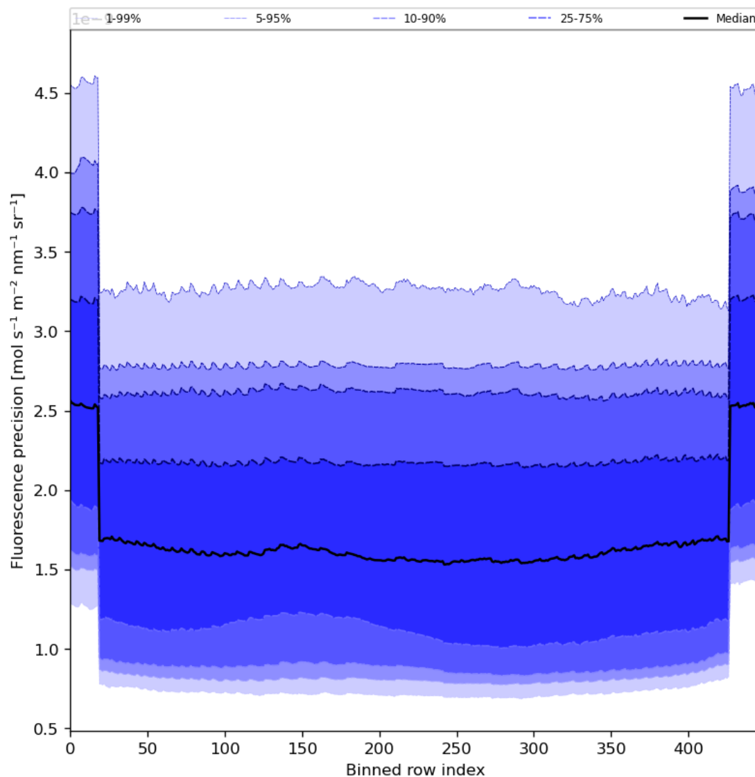
Figure 58: Along track statistics of “Fluorescence precision” for 2024-04-18 to 2024-04-20
