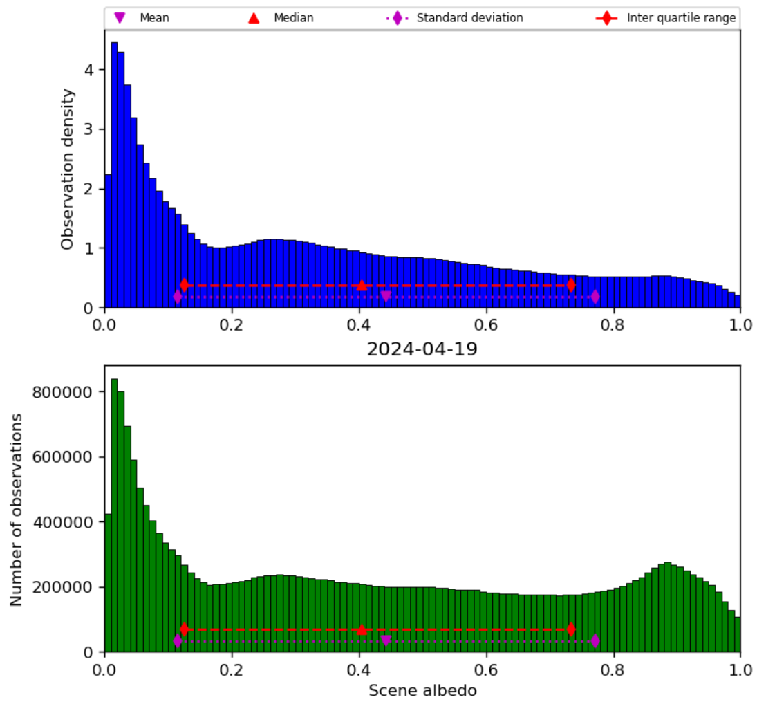
Figure 34: Histogram of “Scene albedo” for 2024-04-18 to 2024-04-20
