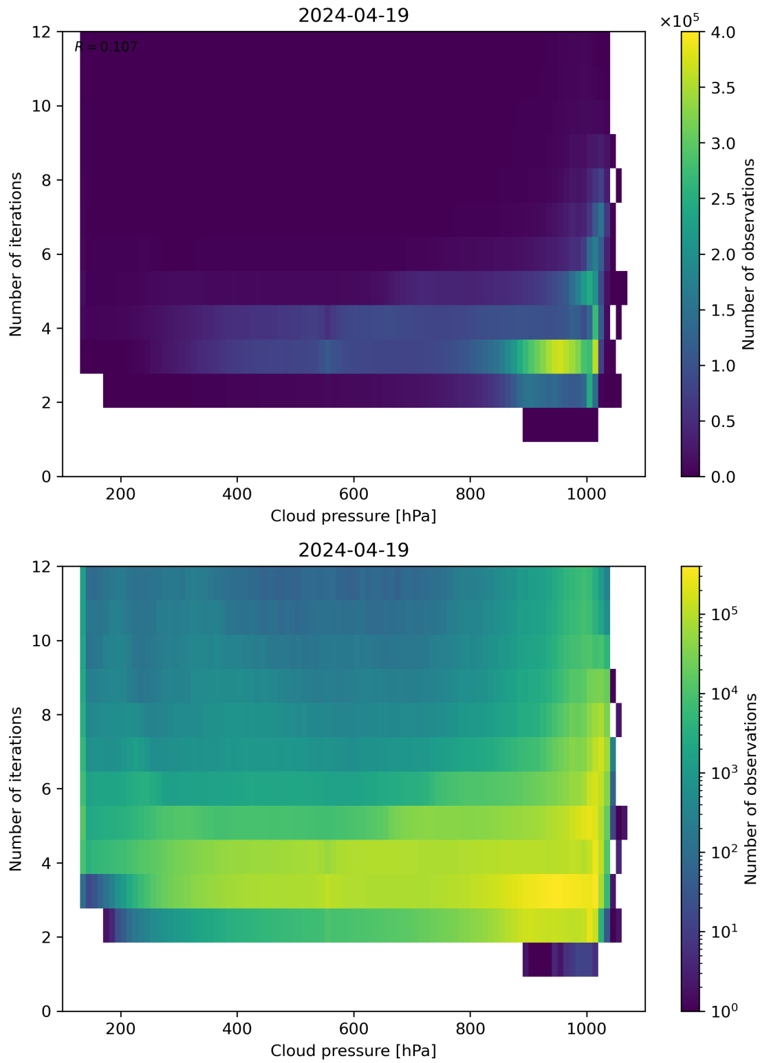
Figure 81: Scatter density plot of “Cloud pressure” against “Number of iterations” for 2024-04-18 to 2024-04-20.
