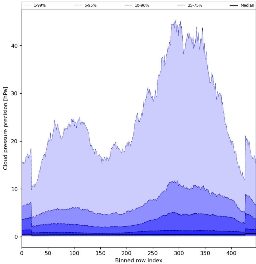
Figure 48: Along track statistics of “Cloud pressure precision” for 2024-04-18 to 2024-04-20
