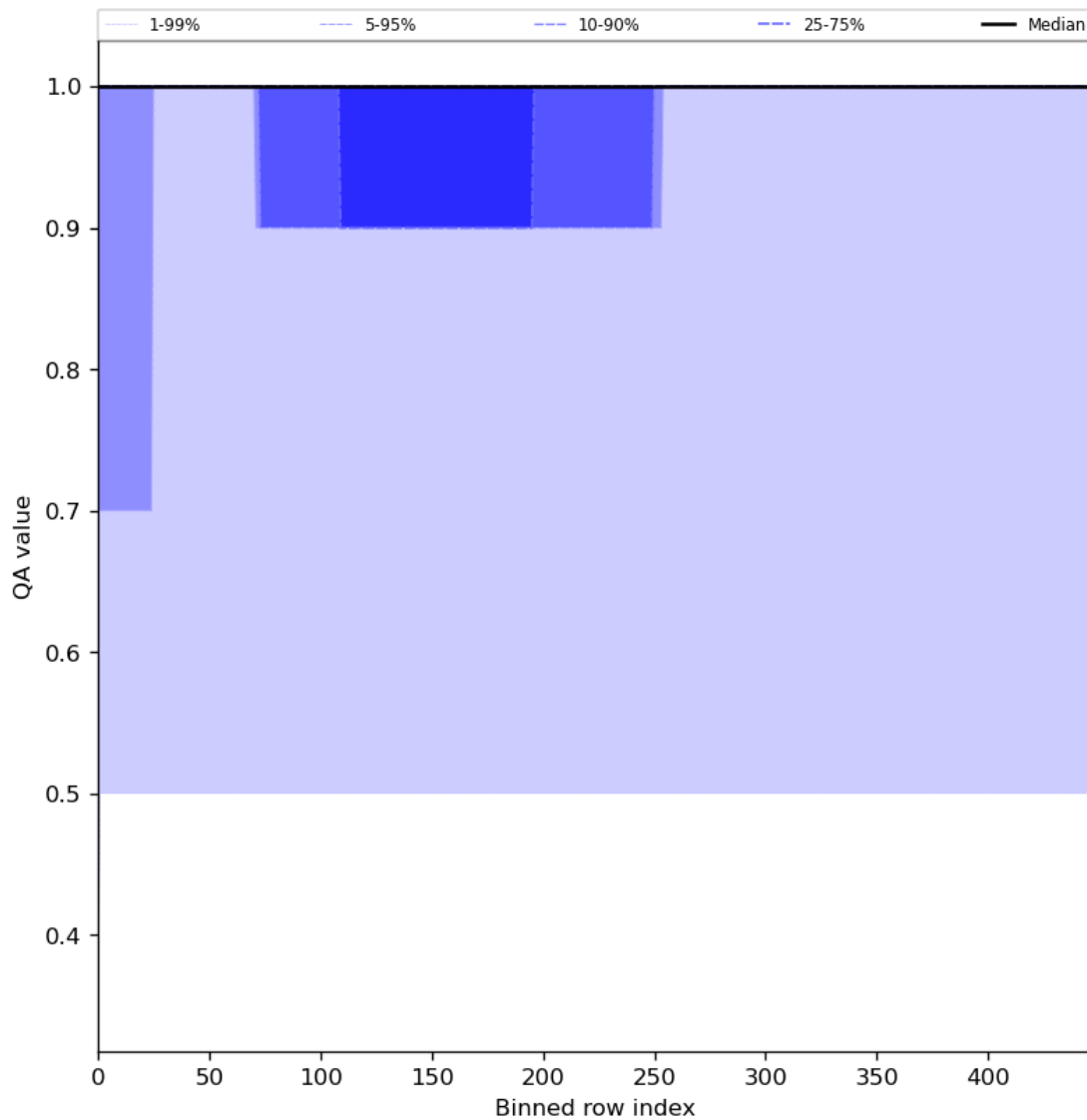
Figure 46: Along track statistics of “QA value” for 2024-04-18 to 2024-04-20
