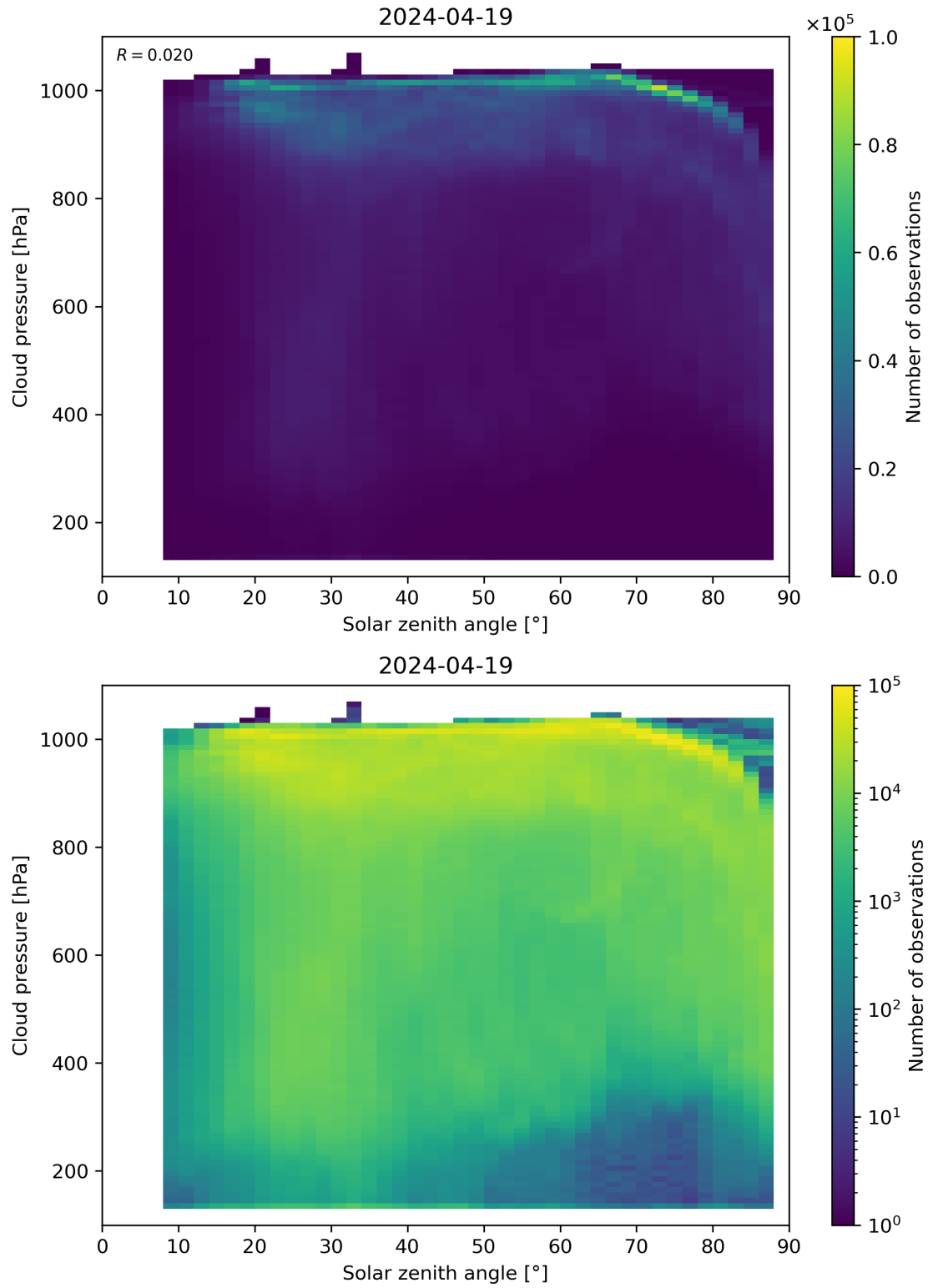
Figure 111: Scatter density plot of “Solar zenith angle” against “Cloud pressure” for 2024-04-18 to 2024-04-20.
