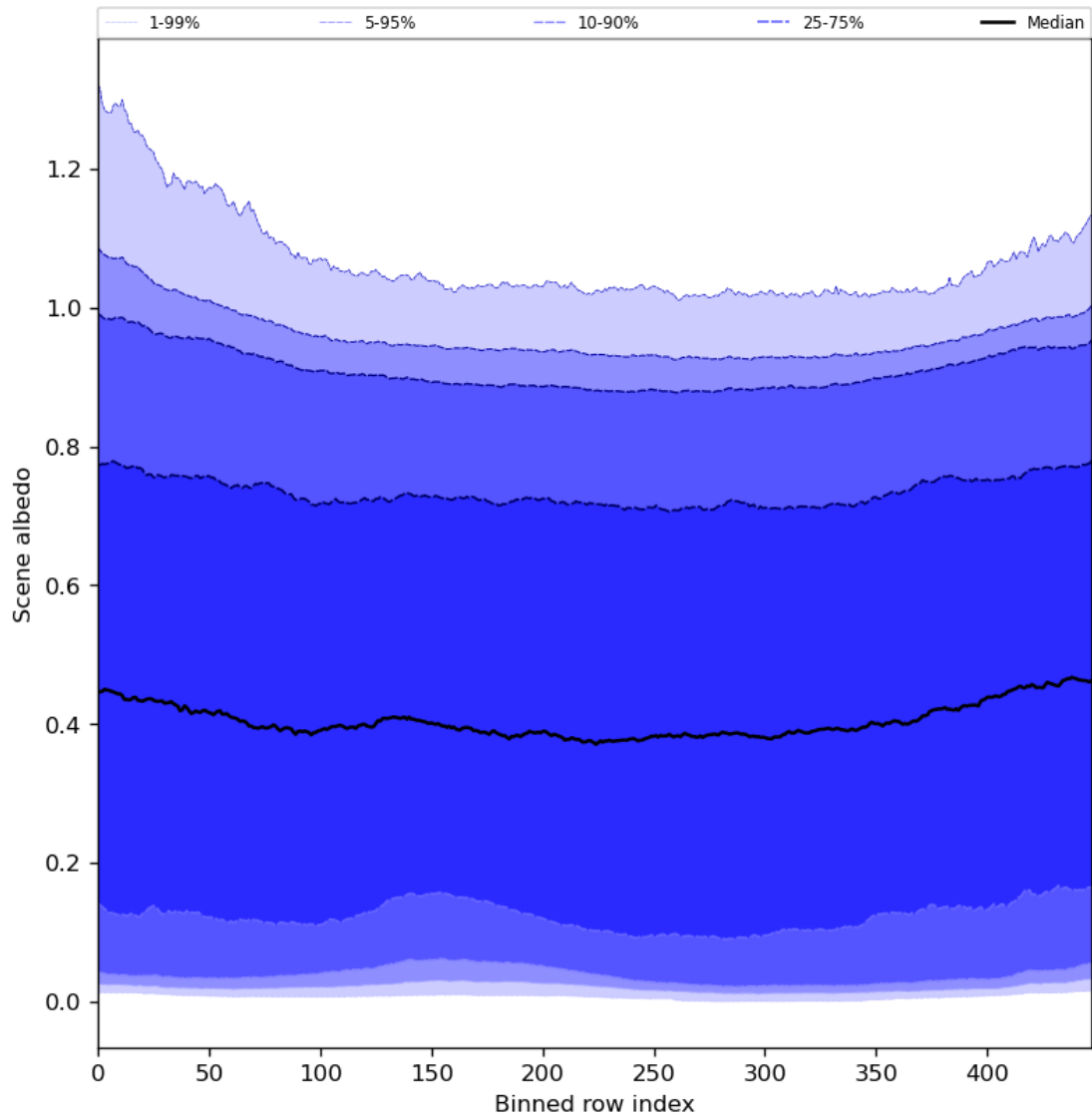
Figure 51: Along track statistics of “Scene albedo” for 2024-04-18 to 2024-04-20
