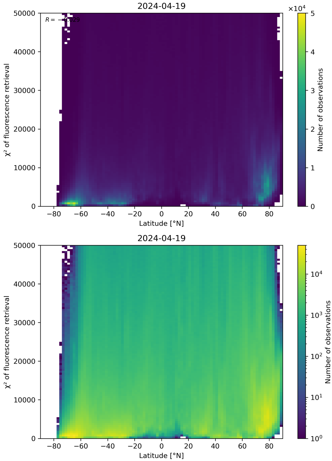
Figure 89: Scatter density plot of “Latitude” against “ \chi^2 of fluorescence retrieval” for 2024-04-18 to 2024-04-20.
