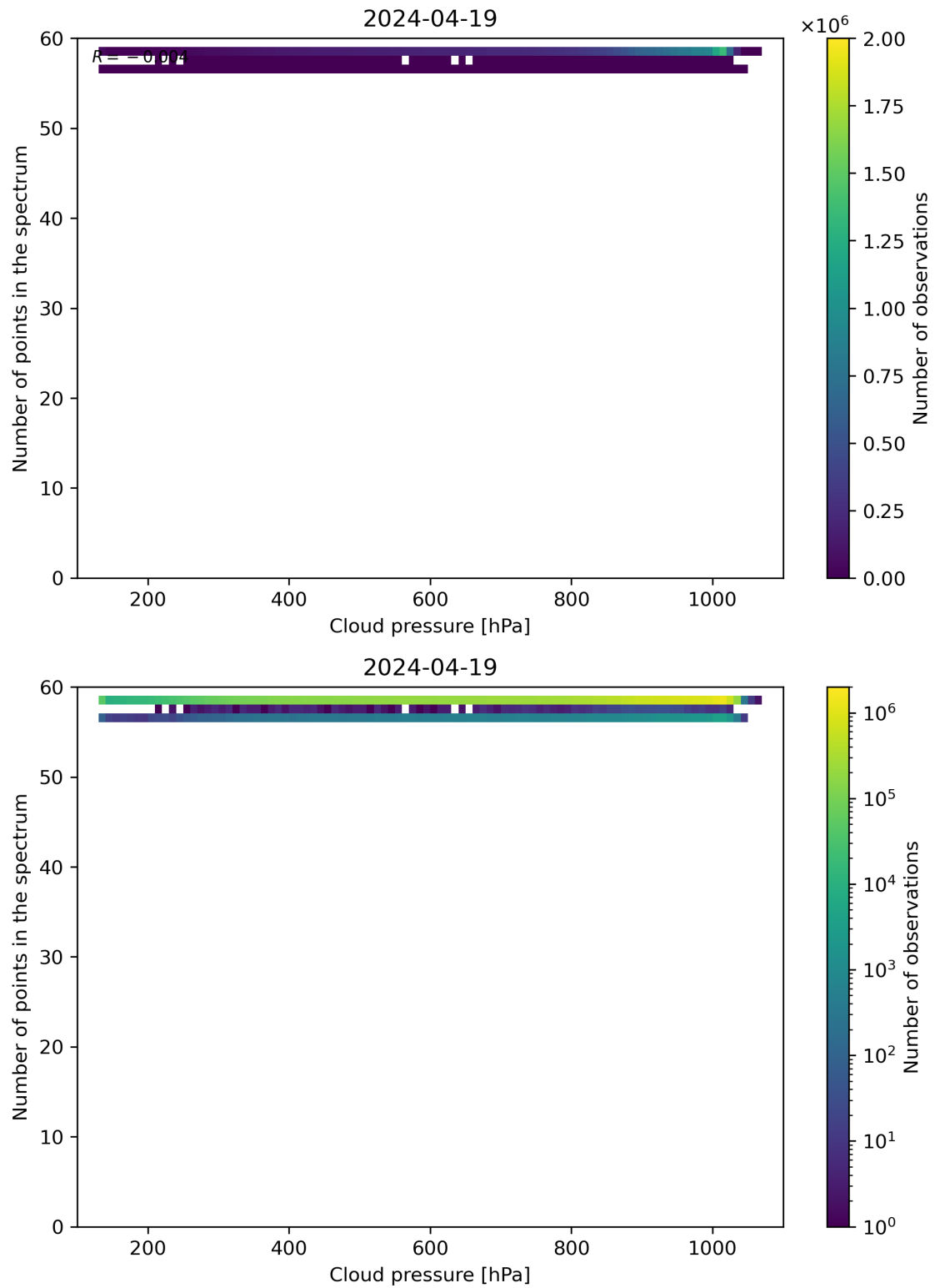
Figure 82: Scatter density plot of “Cloud pressure” against “Number of points in the spectrum” for 2024-04-18 to 2024-04-20.
