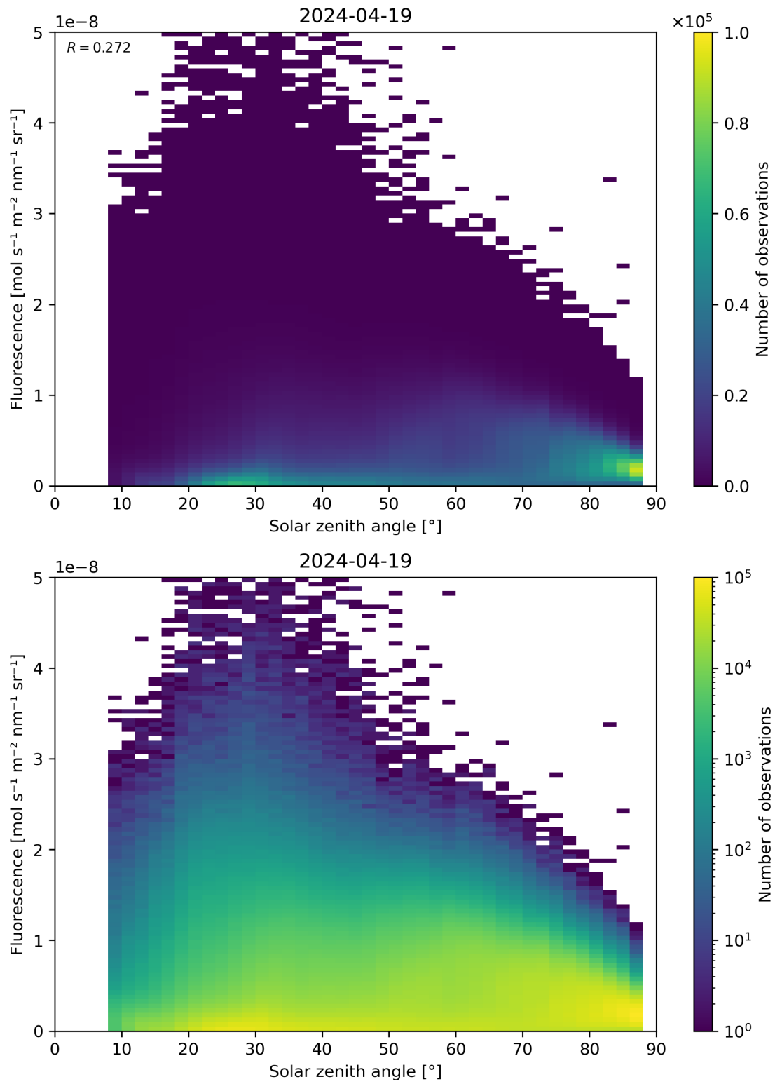
Figure 112: Scatter density plot of “Solar zenith angle” against “Fluorescence” for 2024-04-18 to 2024-04-20.
