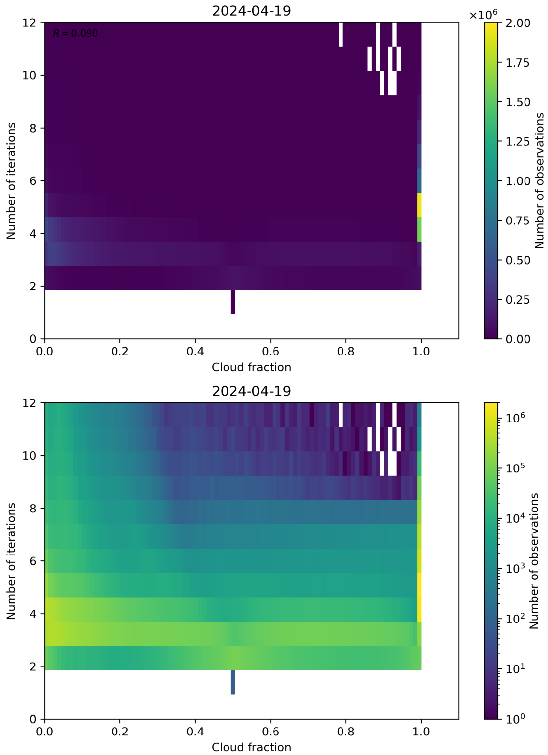
Figure 73: Scatter density plot of “Cloud fraction” against “Number of iterations” for 2024-04-18 to 2024-04-20.
