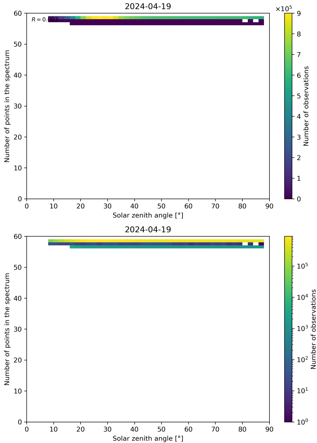
Figure 115: Scatter density plot of “Solar zenith angle” against “Number of points in the spectrum” for 2024-04-18 to 2024-04-20.
