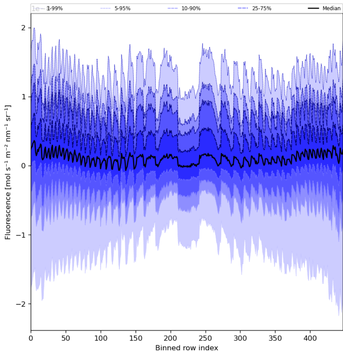
Figure 57: Along track statistics of “Fluorescence” for 2024-04-18 to 2024-04-20
