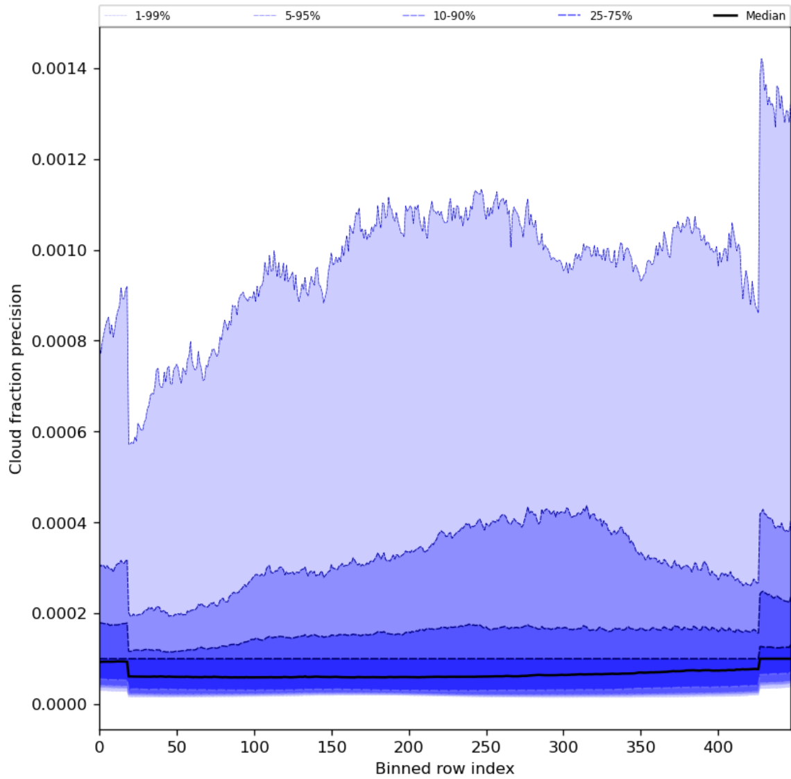
Figure 50: Along track statistics of “Cloud fraction precision” for 2024-04-18 to 2024-04-20
