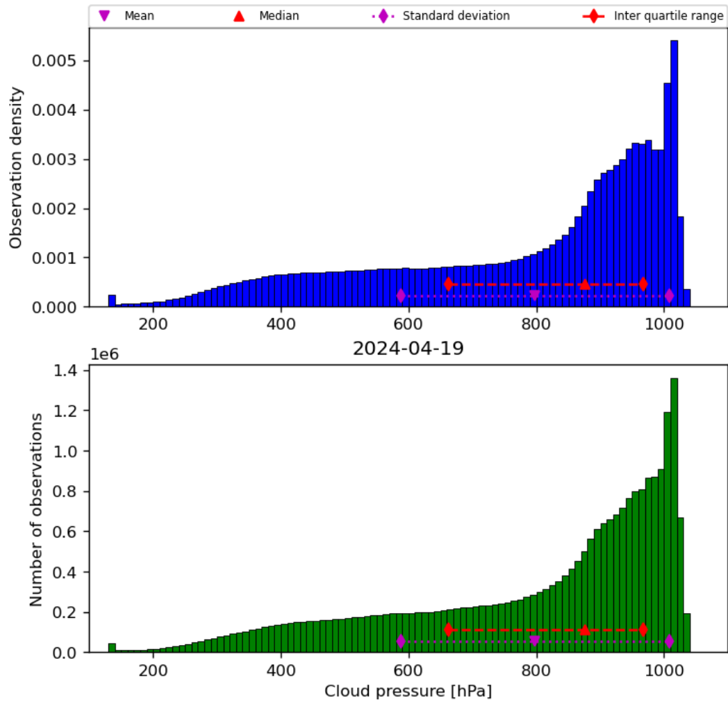
Figure 30: Histogram of “Cloud pressure” for 2024-04-18 to 2024-04-20
