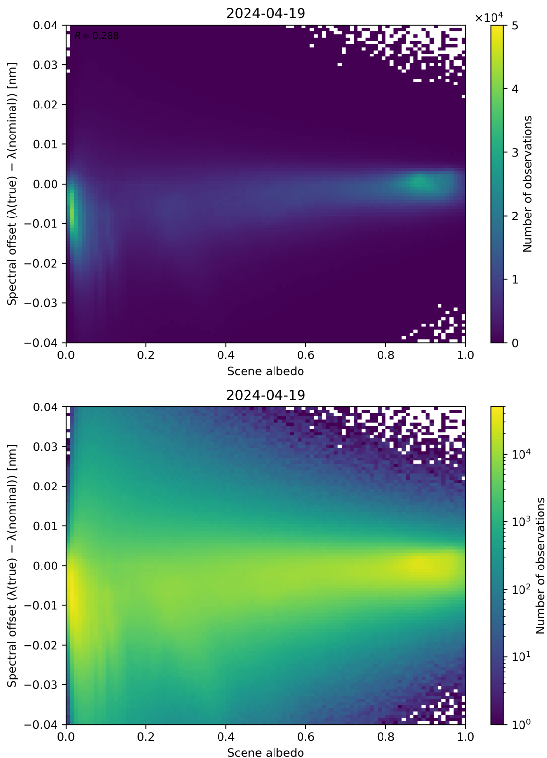
Figure 107: Scatter density plot of “Scene albedo” against “Spectral offset ( \lambda(\text{true}) - \lambda(\text{nominal}) )” for 2024-04-18 to 2024-04-20.
