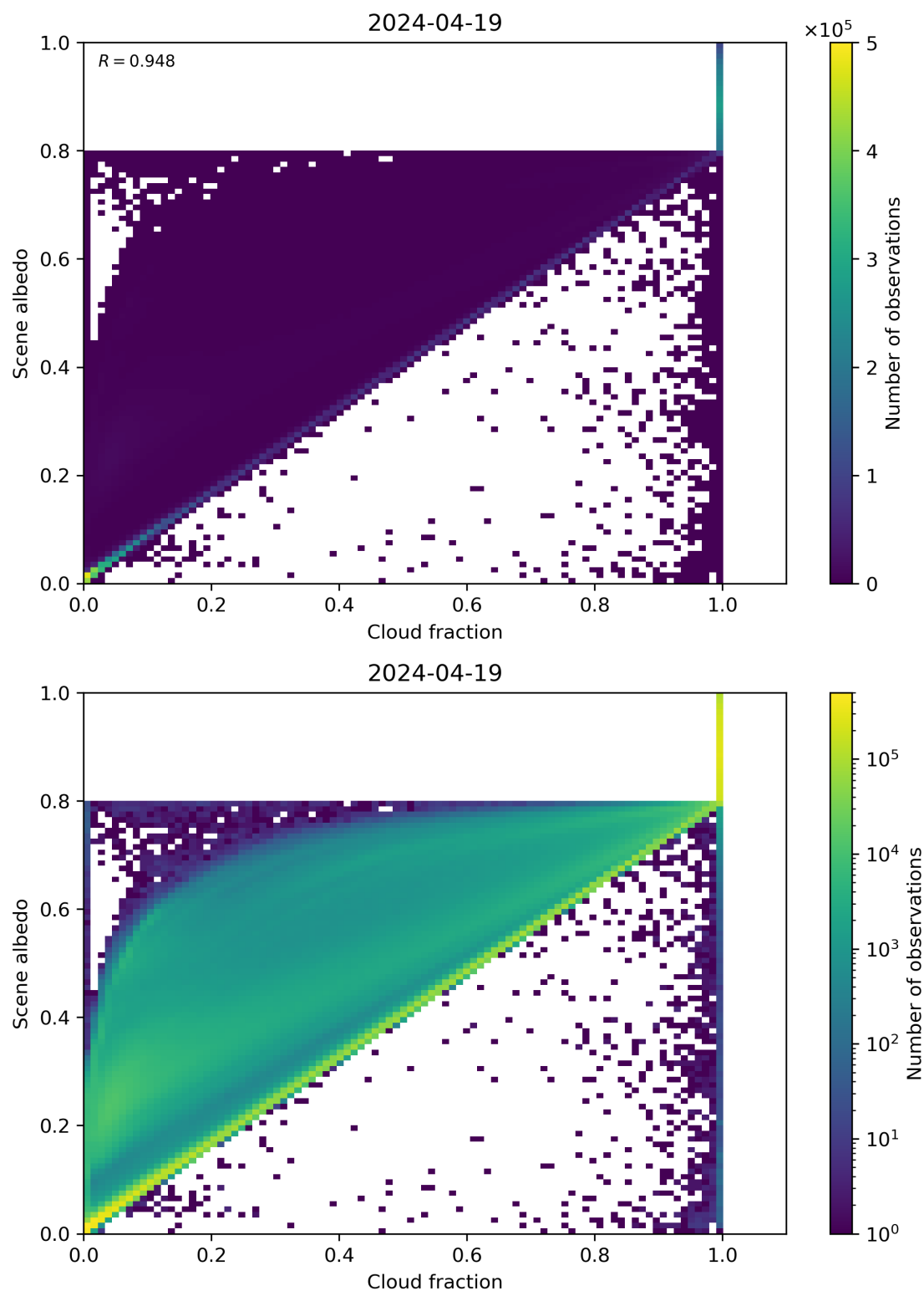
Figure 75: Scatter density plot of “Cloud fraction” against “Scene albedo” for 2024-04-18 to 2024-04-20.
