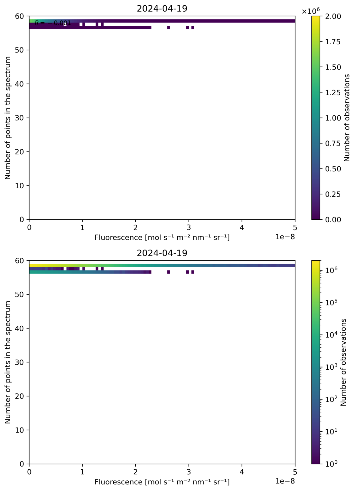
Figure 86: Scatter density plot of “Fluorescence” against “Number of points in the spectrum” for 2024-04-18 to 2024-04-20.
