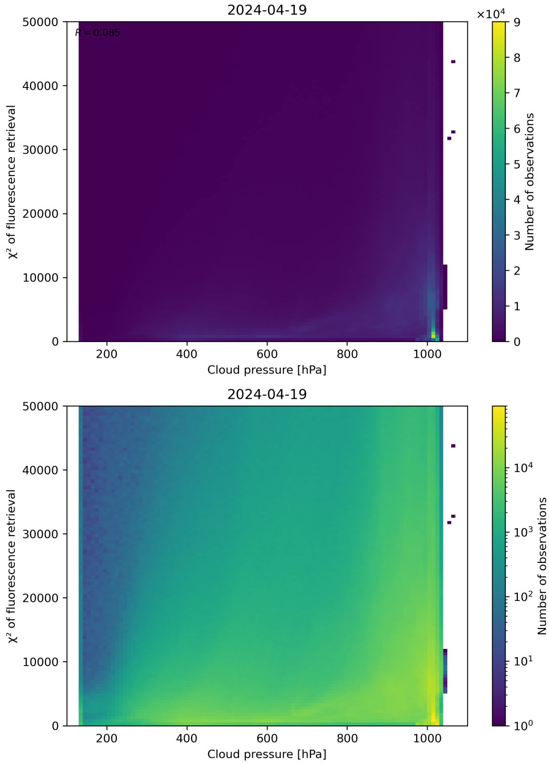
Figure 78: Scatter density plot of “Cloud pressure” against “ \chi^2 of fluorescence retrieval” for 2024-04-18 to 2024-04-20.
