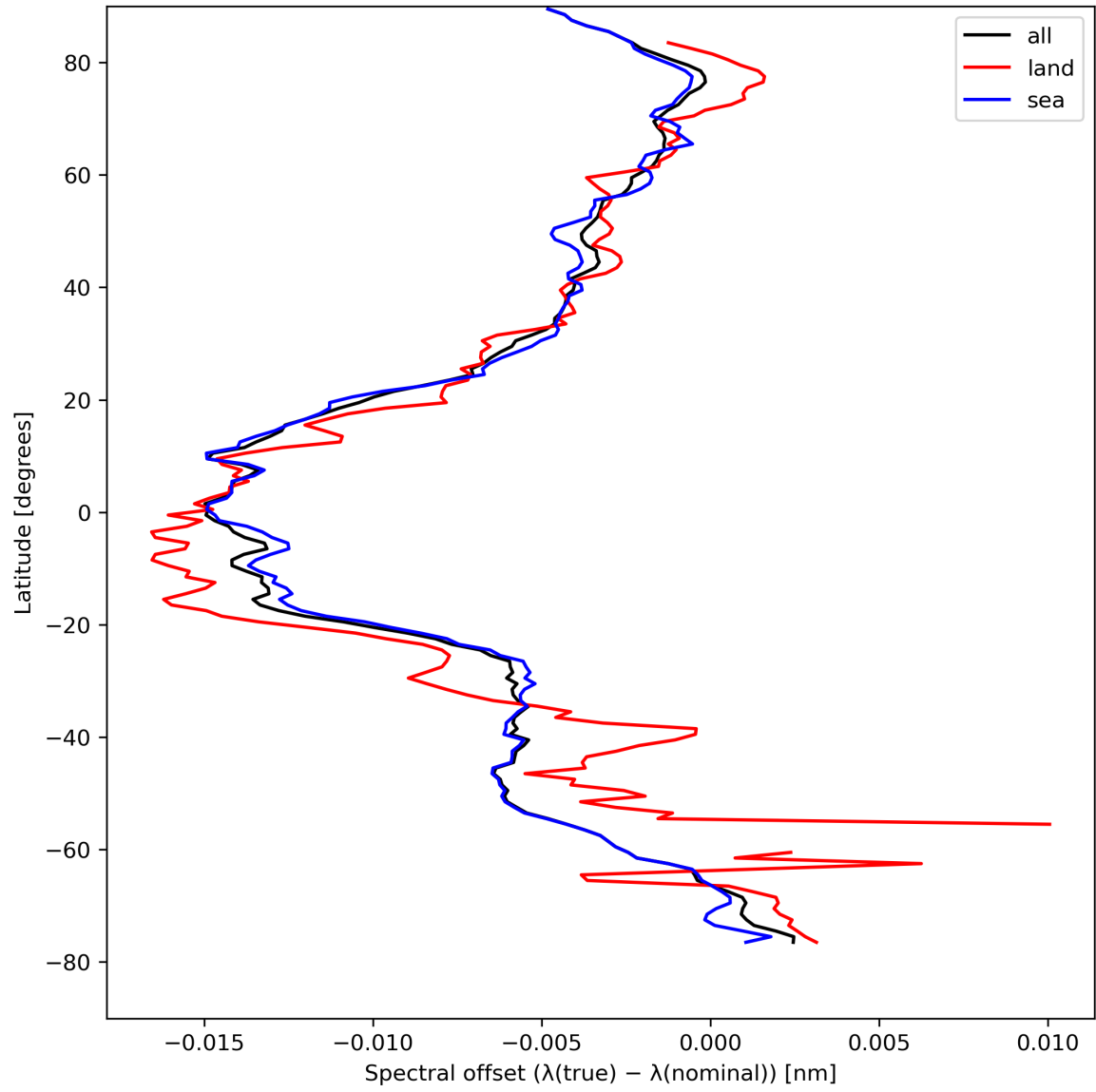
Figure 28: Zonal average of “Spectral offset ( \lambda(\text{true}) - \lambda(\text{nominal}) )” for 2024-04-18 to 2024-04-20.
