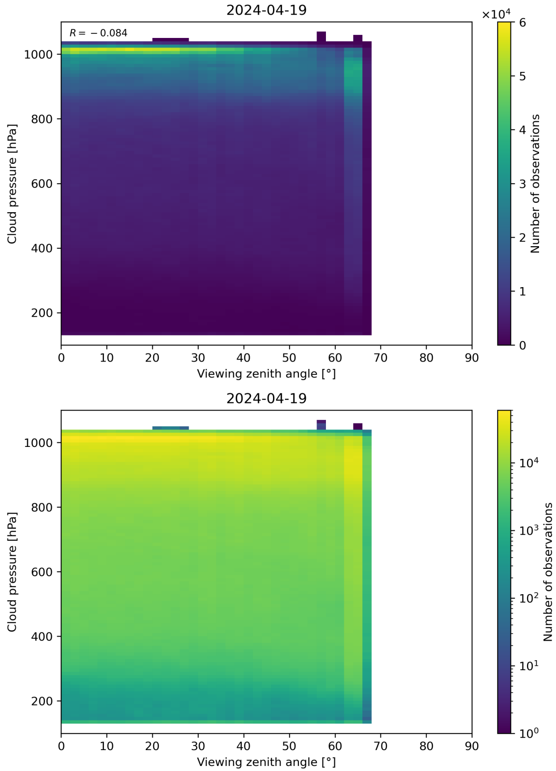
Figure 121: Scatter density plot of “Viewing zenith angle” against “Cloud pressure” for 2024-04-18 to 2024-04-20.
