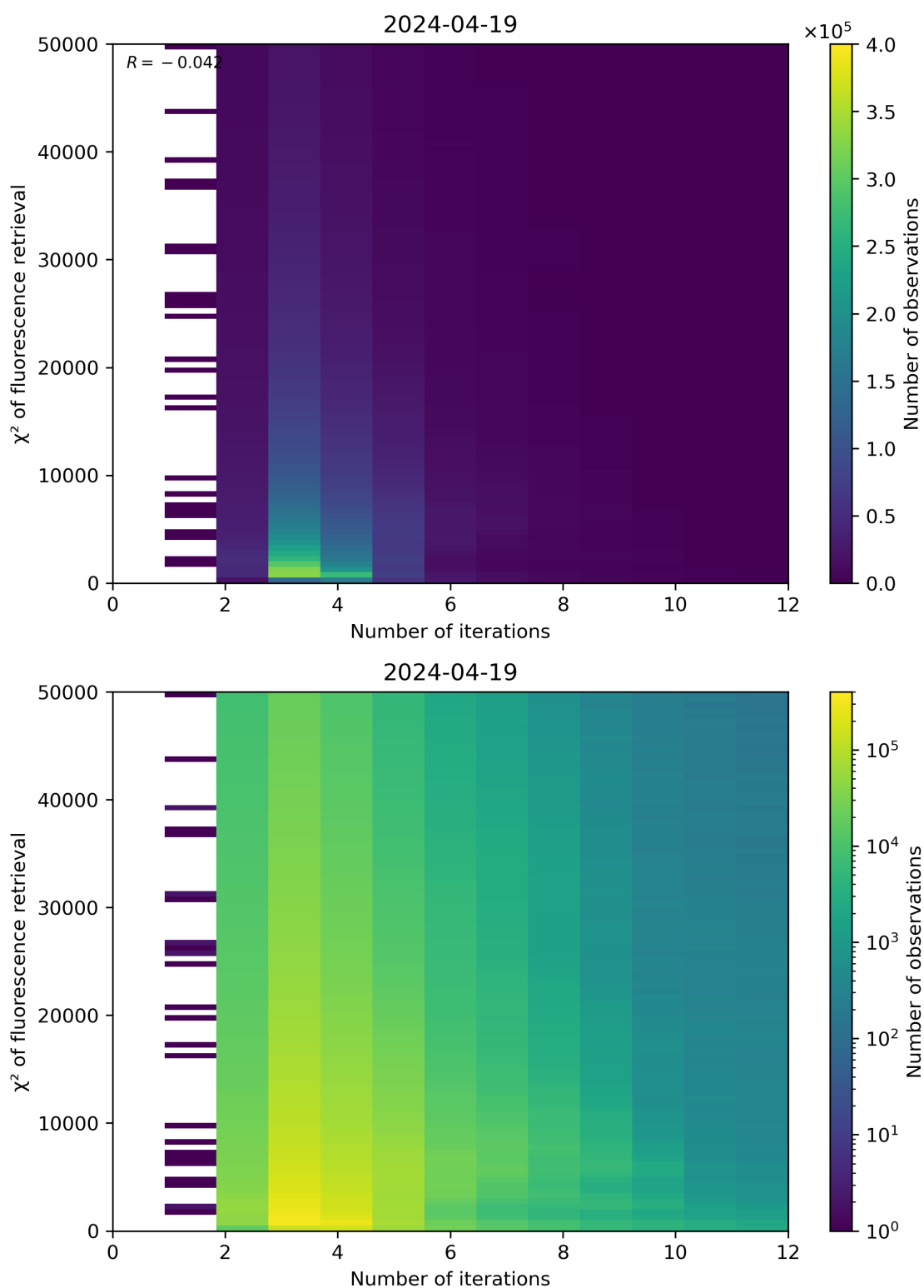
Figure 97: Scatter density plot of “Number of iterations” against “ \chi^2 of fluorescence retrieval” for 2024-04-18 to 2024-04-20.
