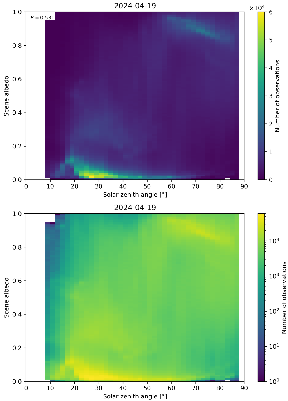
Figure 116: Scatter density plot of “Solar zenith angle” against “Scene albedo” for 2024-04-18 to 2024-04-20.
