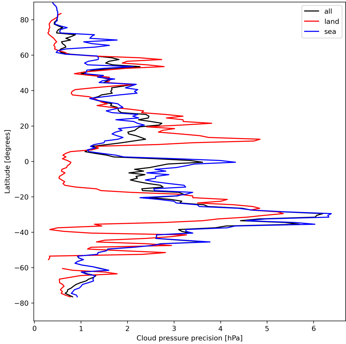
Figure 14: Zonal average of “Cloud pressure precision” for 2024-04-18 to 2024-04-20.
