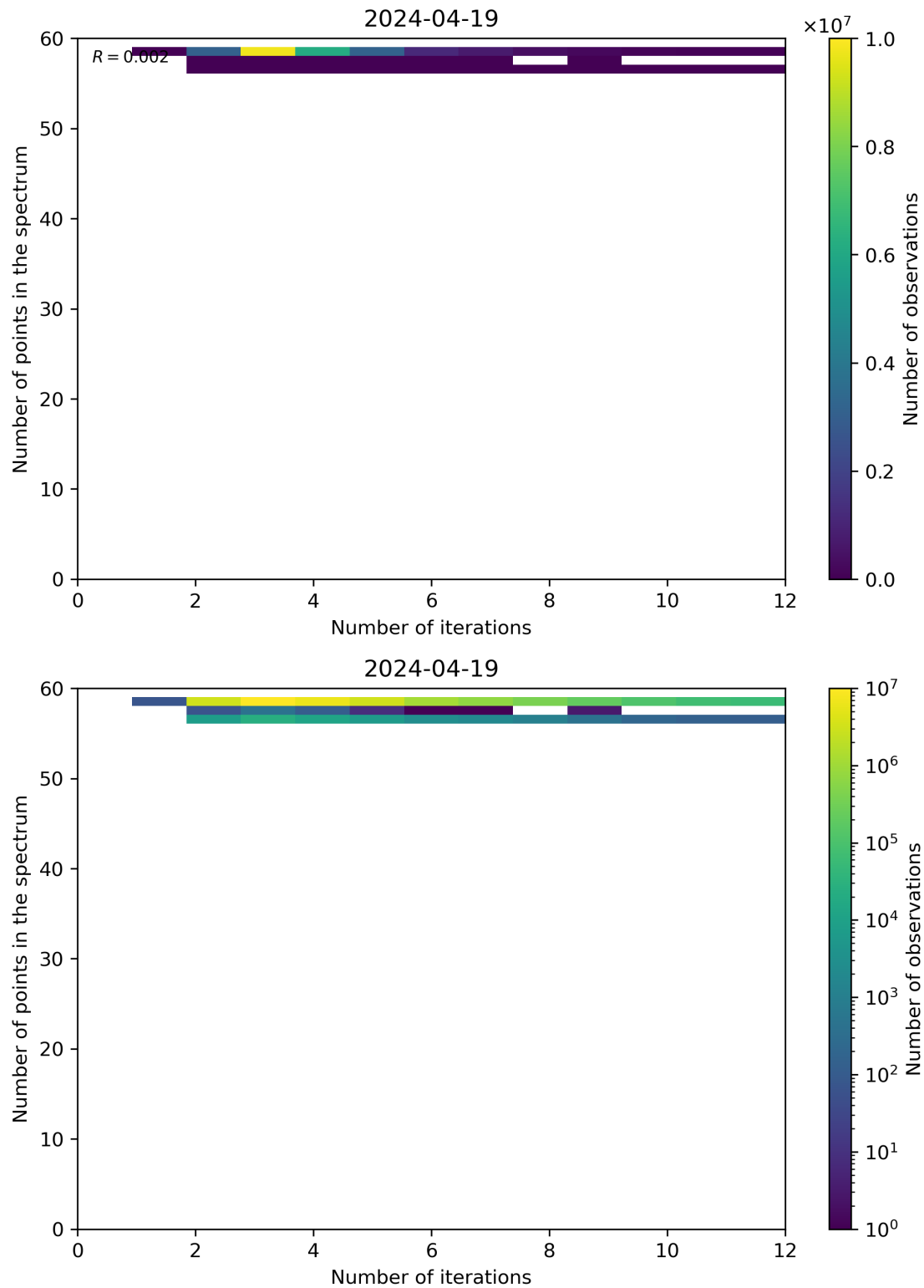
Figure 99: Scatter density plot of “Number of iterations” against “Number of points in the spectrum” for 2024-04-18 to 2024-04-20.
