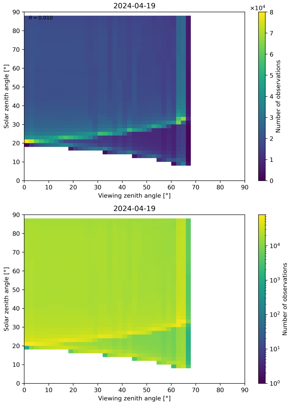
Figure 127: Scatter density plot of “Viewing zenith angle” against “Solar zenith angle” for 2024-04-18 to 2024-04-20.
