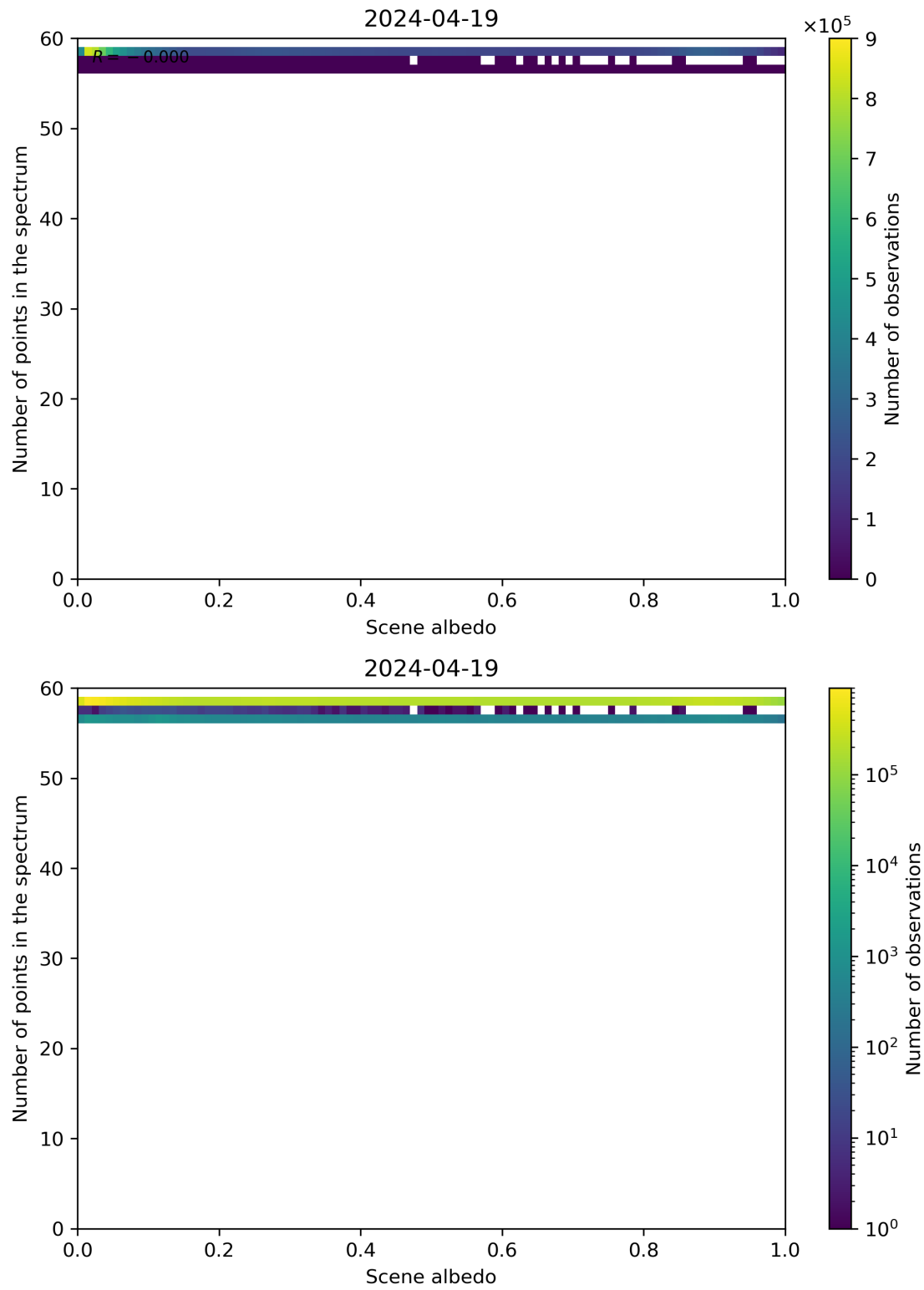
Figure 106: Scatter density plot of “Scene albedo” against “Number of points in the spectrum” for 2024-04-18 to 2024-04-20.
