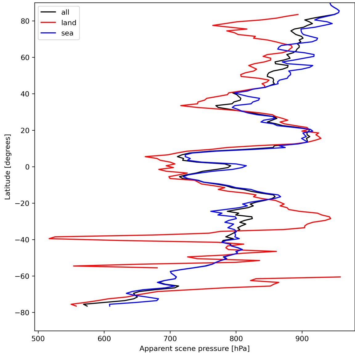
Figure 19: Zonal average of “Apparent scene pressure” for 2024-04-18 to 2024-04-20.
