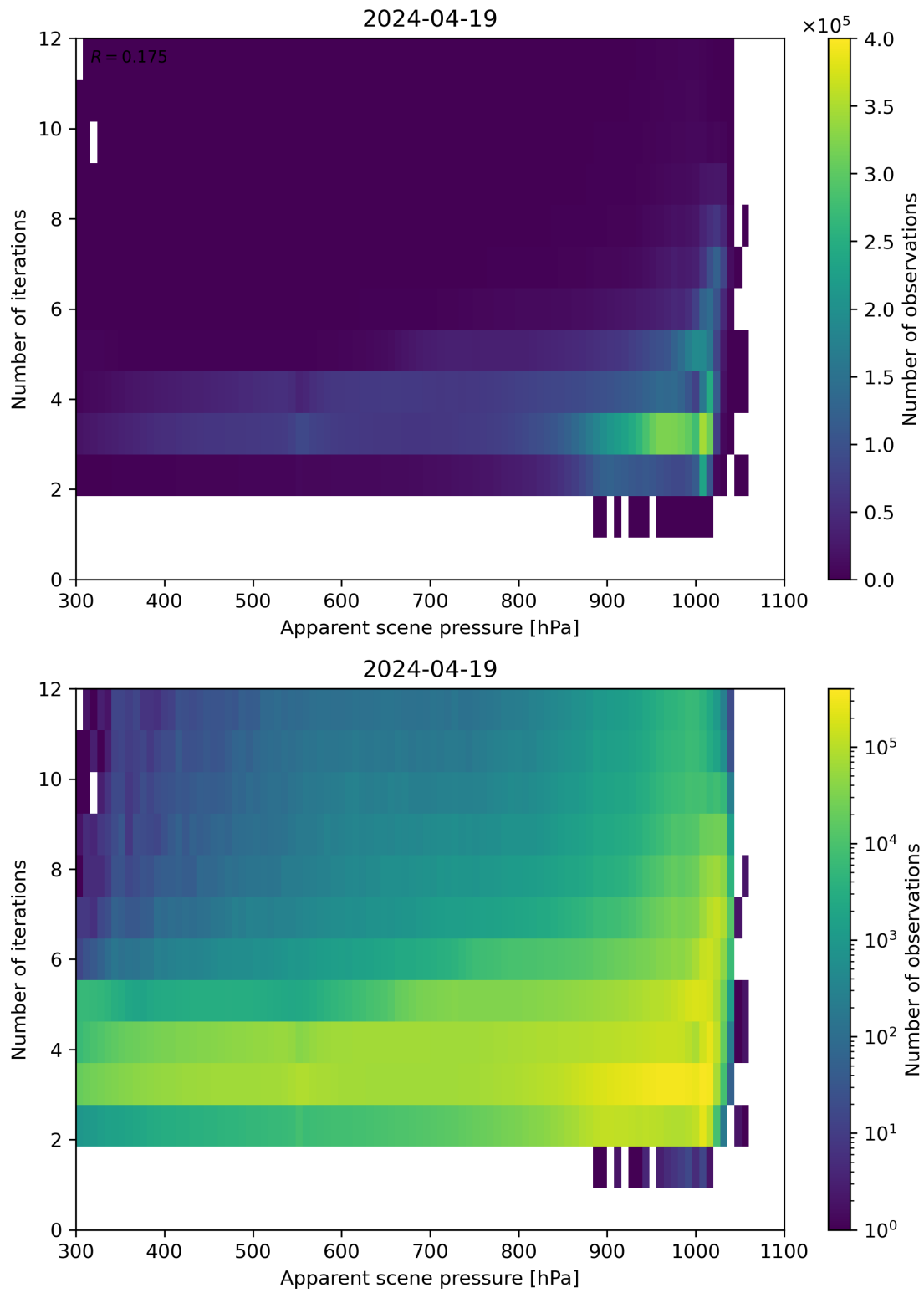
Figure 65: Scatter density plot of “Apparent scene pressure” against “Number of iterations” for 2024-04-18 to 2024-04-20.
