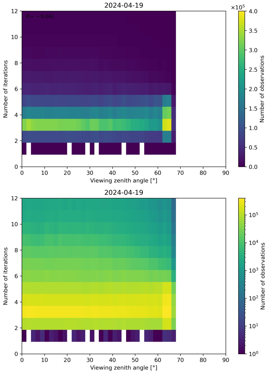
Figure 124: Scatter density plot of “Viewing zenith angle” against “Number of iterations” for 2024-04-18 to 2024-04-20.
