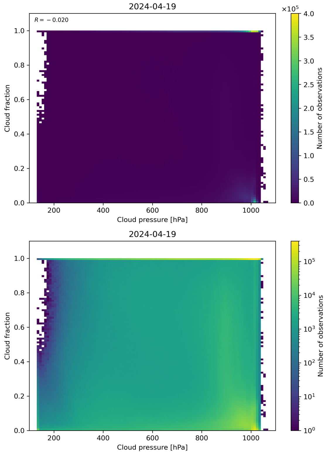
Figure 79: Scatter density plot of “Cloud pressure” against “Cloud fraction” for 2024-04-18 to 2024-04-20.
