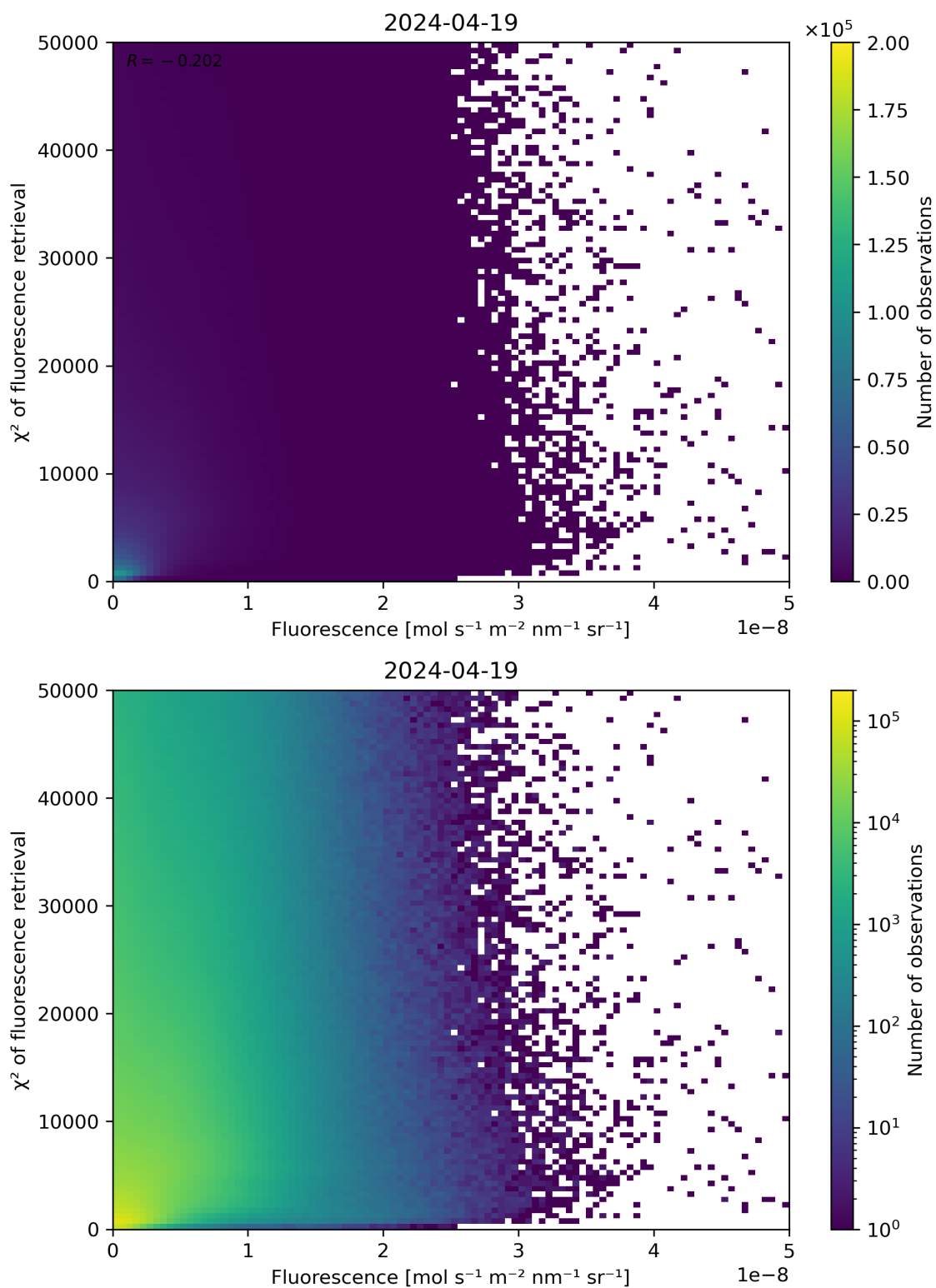
Figure 85: Scatter density plot of “Fluorescence” against “ \chi^2 of fluorescence retrieval” for 2024-04-18 to 2024-04-20.
