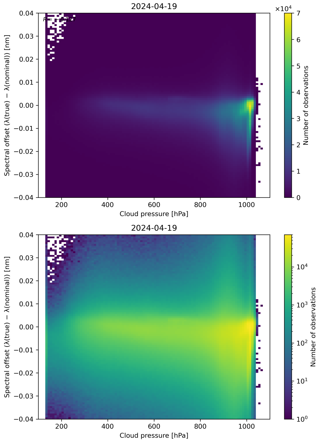
Figure 84: Scatter density plot of “Cloud pressure” against “Spectral offset ( \lambda(\text{true}) - \lambda(\text{nominal}) )” for 2024-04-18 to 2024-04-20.
