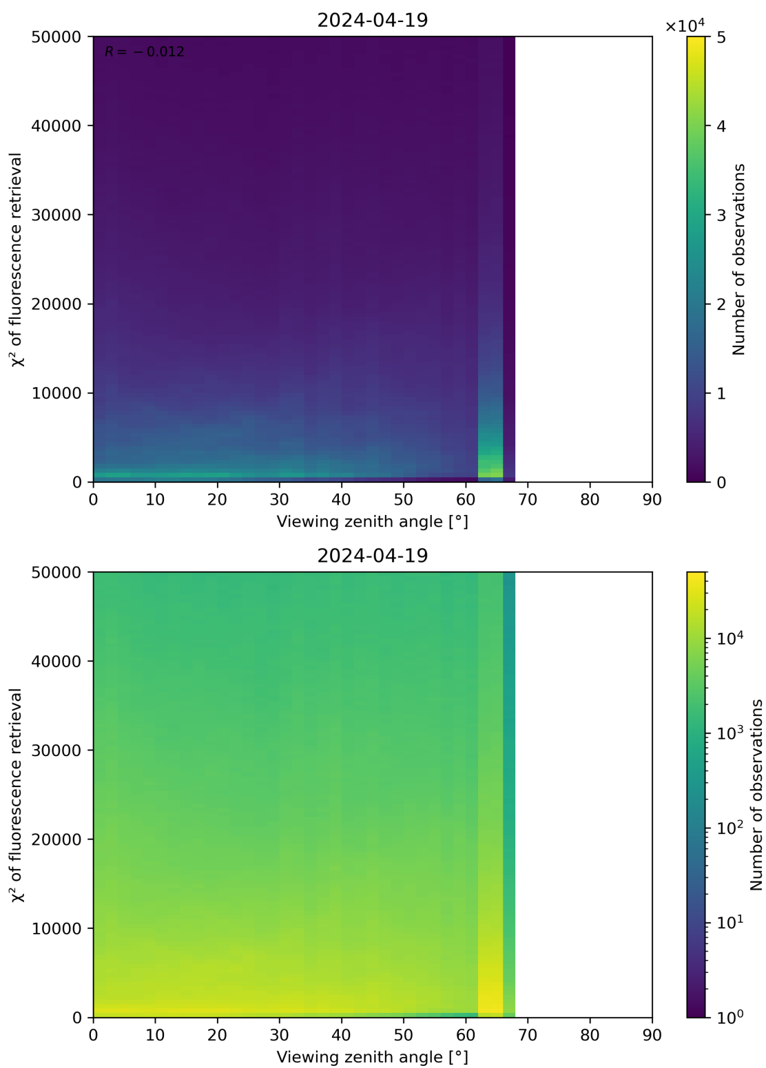
Figure 119: Scatter density plot of “Viewing zenith angle” against “ \chi^2 of fluorescence retrieval” for 2024-04-18 to 2024-04-20.
