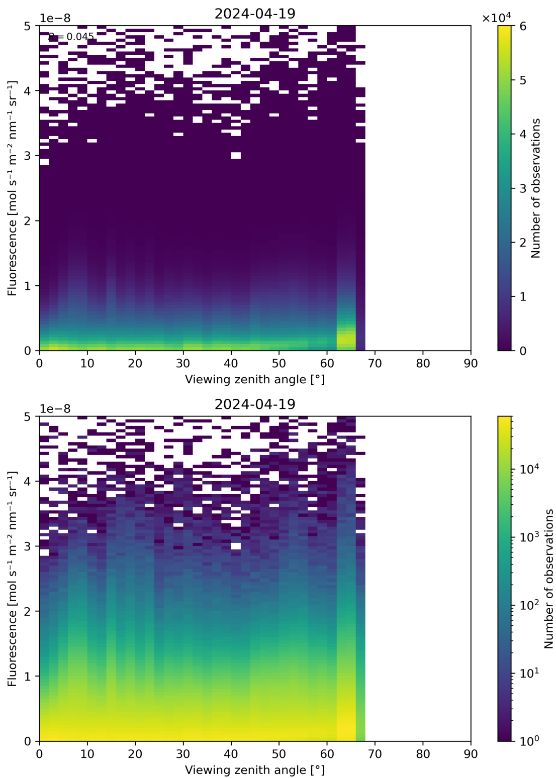
Figure 122: Scatter density plot of “Viewing zenith angle” against “Fluorescence” for 2024-04-18 to 2024-04-20.
