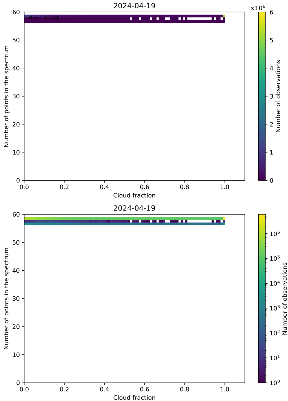
Figure 74: Scatter density plot of “Cloud fraction” against “Number of points in the spectrum” for 2024-04-18 to 2024-04-20.
