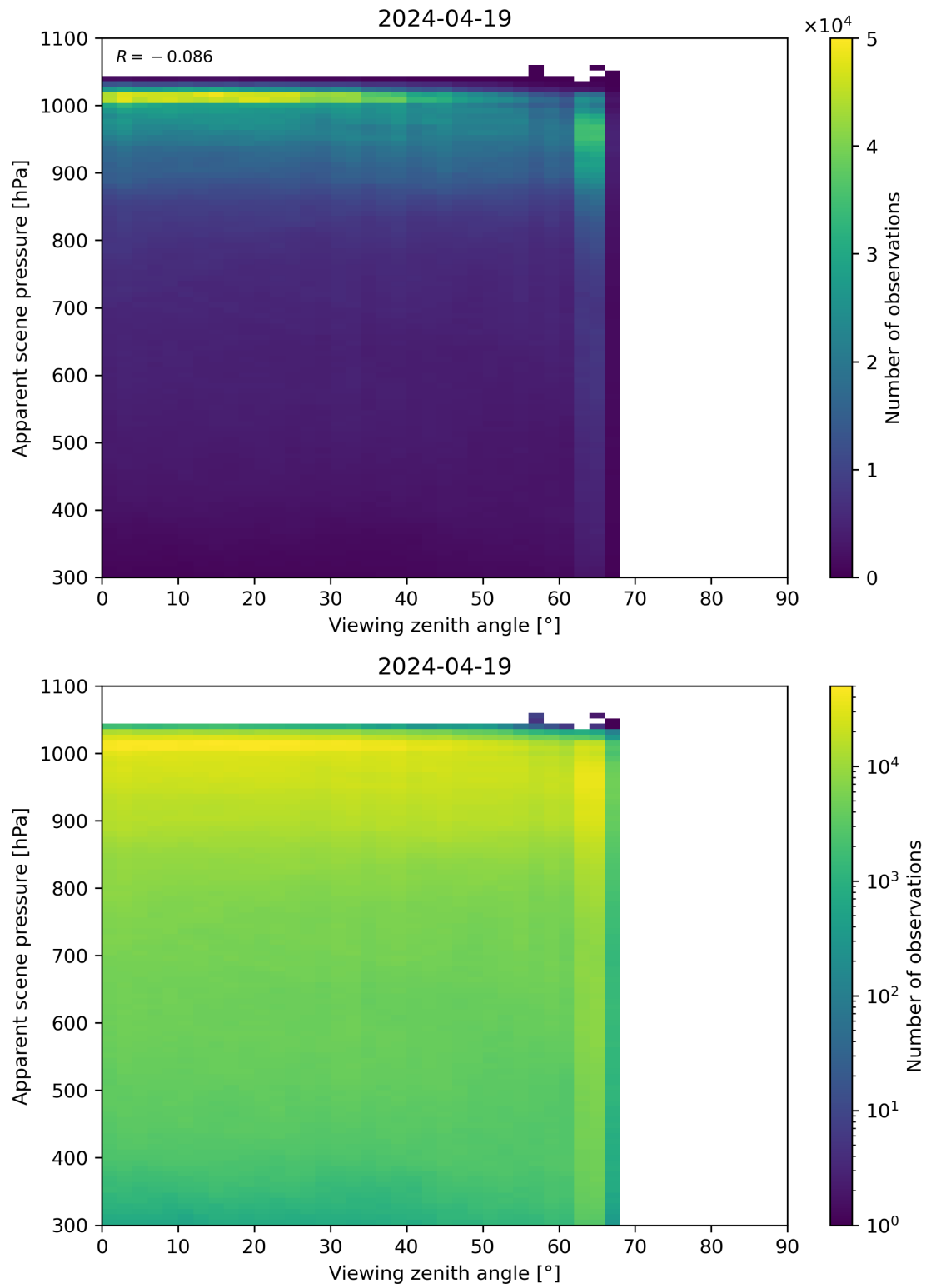
Figure 118: Scatter density plot of “Viewing zenith angle” against “Apparent scene pressure” for 2024-04-18 to 2024-04-20.
