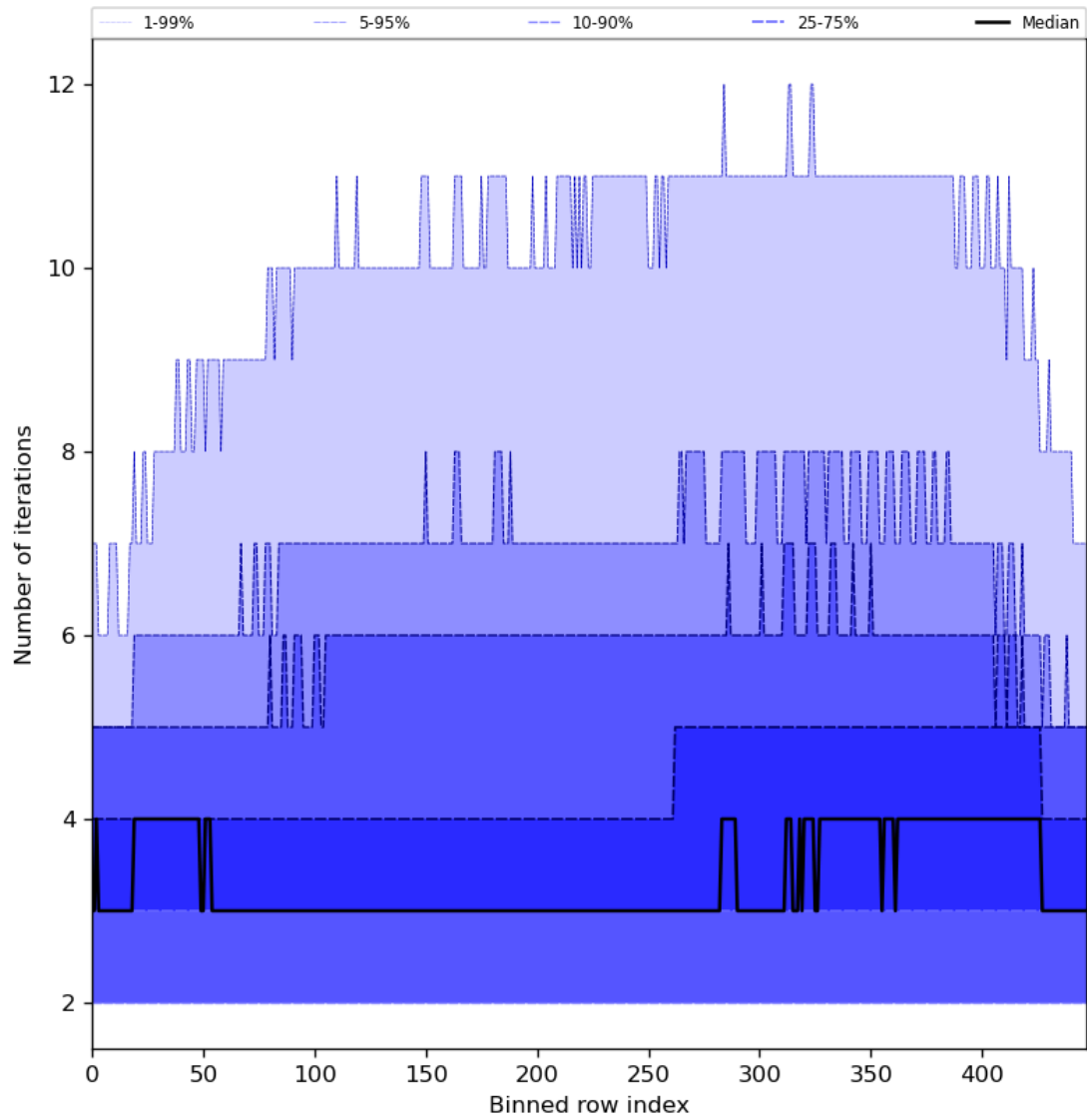
Figure 56: Along track statistics of “Number of iterations” for 2024-04-18 to 2024-04-20
