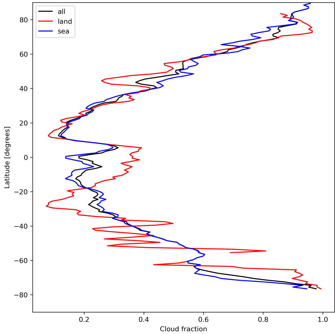
Figure 15: Zonal average of “Cloud fraction” for 2024-04-18 to 2024-04-20.
