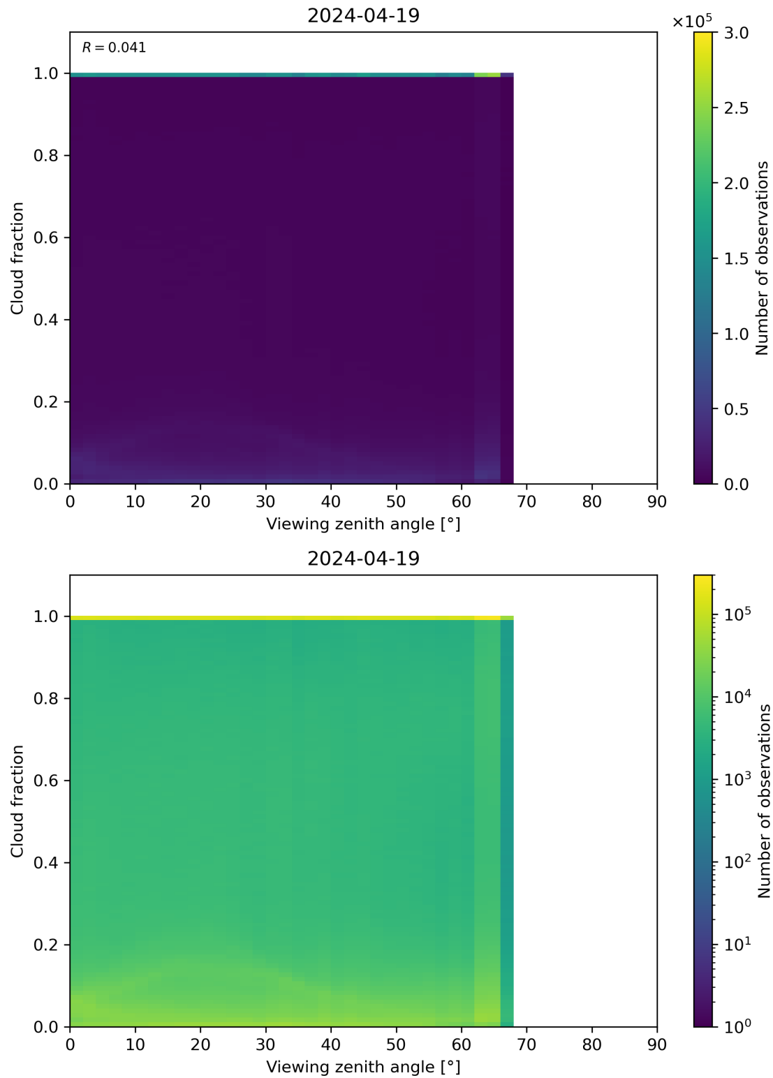
Figure 120: Scatter density plot of “Viewing zenith angle” against “Cloud fraction” for 2024-04-18 to 2024-04-20.
