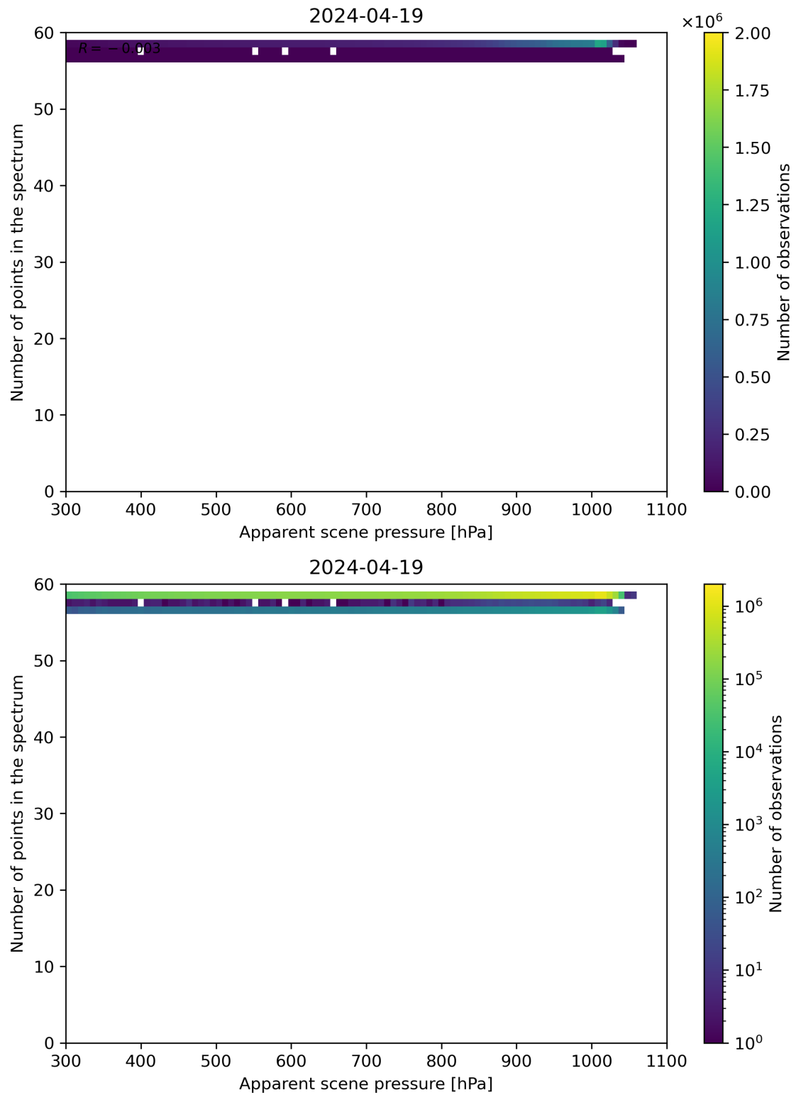
Figure 66: Scatter density plot of “Apparent scene pressure” against “Number of points in the spectrum” for 2024-04-18 to 2024-04-20.
