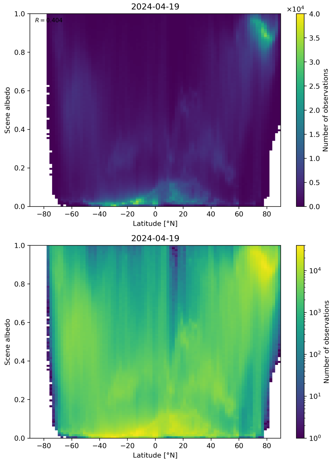
Figure 95: Scatter density plot of “Latitude” against “Scene albedo” for 2024-04-18 to 2024-04-20.
