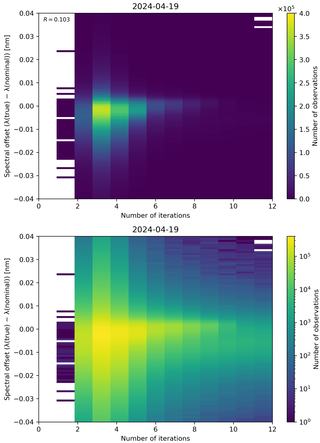
Figure 100: Scatter density plot of “Number of iterations” against “Spectral offset ( \lambda(\text{true}) - \lambda(\text{nominal}) )” for 2024-04-18 to 2024-04-20.
