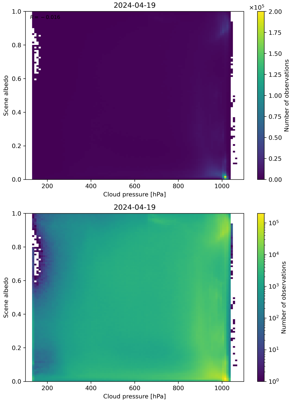
Figure 83: Scatter density plot of “Cloud pressure” against “Scene albedo” for 2024-04-18 to 2024-04-20.
