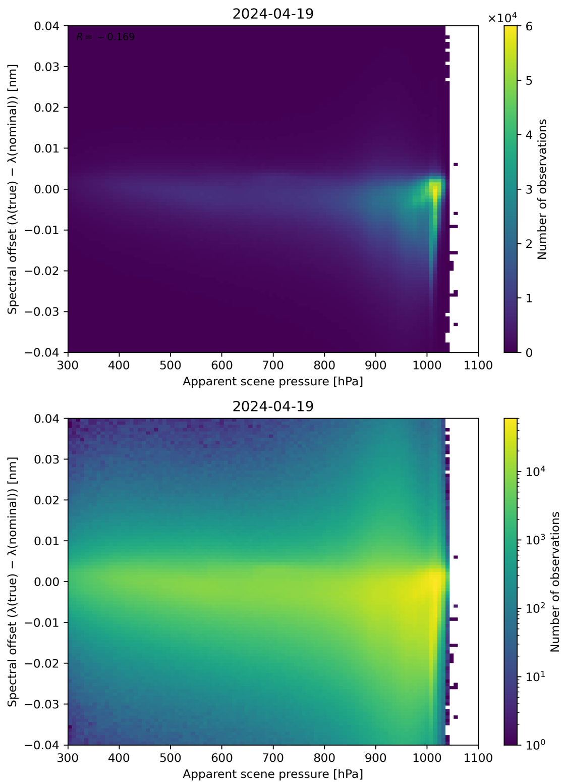
Figure 67: Scatter density plot of “Apparent scene pressure” against “Spectral offset ( \lambda(\text{true}) - \lambda(\text{nominal}) )” for 2024-04-18 to 2024-04-20.
