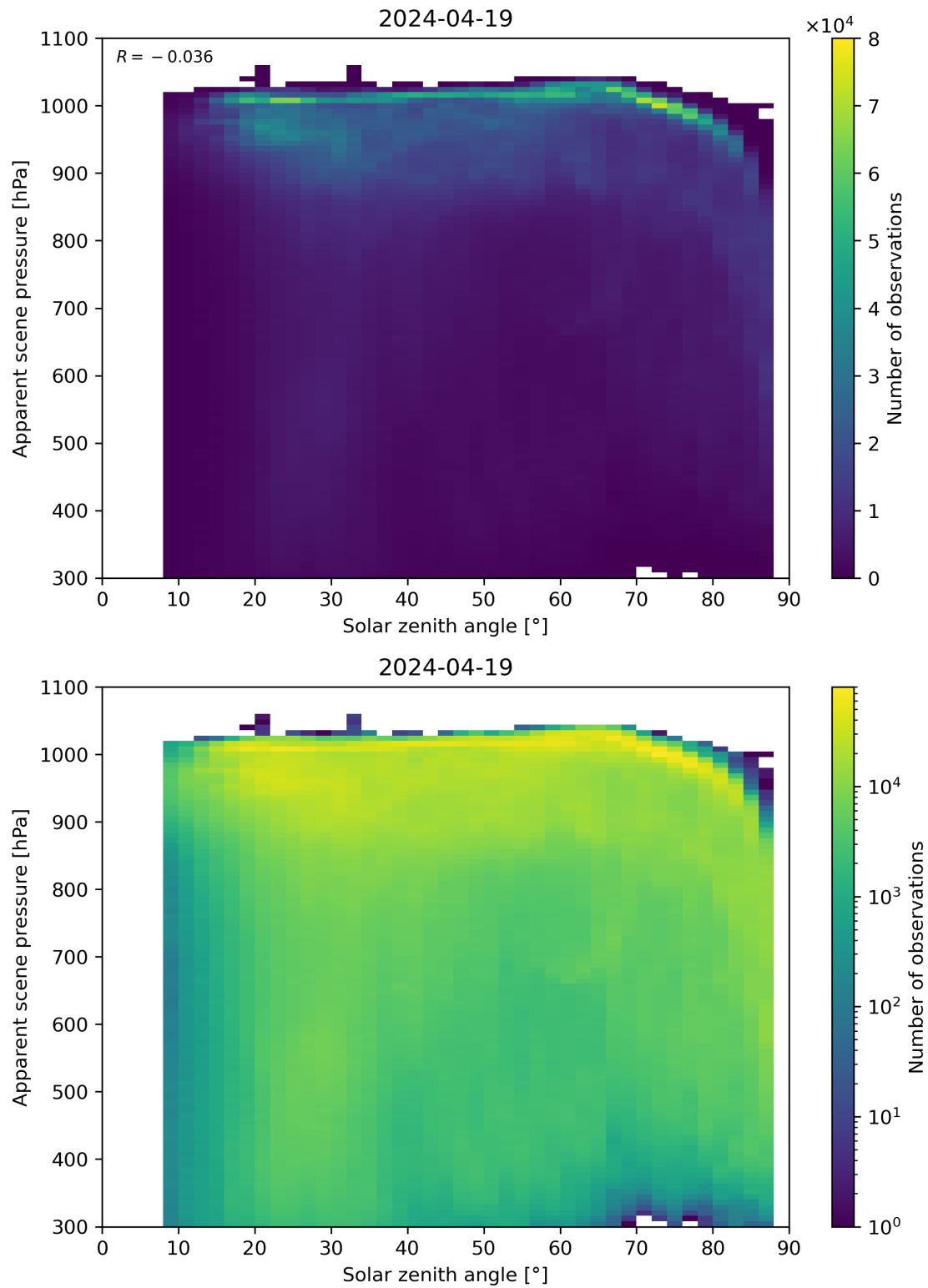
Figure 108: Scatter density plot of “Solar zenith angle” against “Apparent scene pressure” for 2024-04-18 to 2024-04-20.
