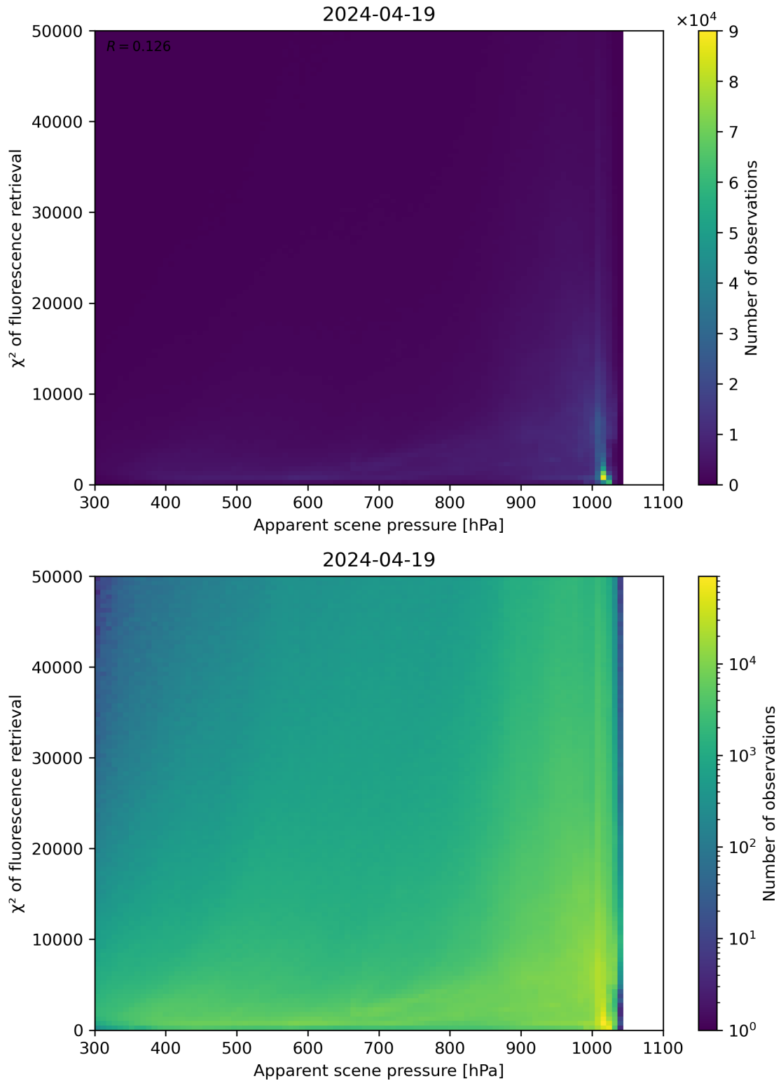
Figure 63: Scatter density plot of “Apparent scene pressure” against “ \chi^2 of fluorescence retrieval” for 2024-04-18 to 2024-04-20.
