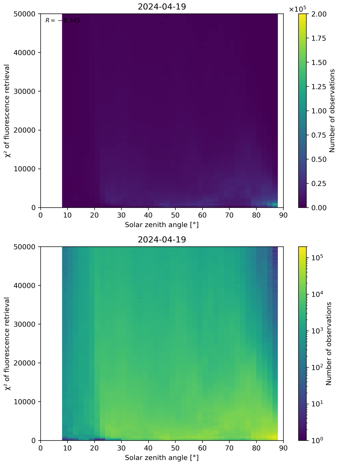
Figure 109: Scatter density plot of “Solar zenith angle” against “ \chi^2 of fluorescence retrieval” for 2024-04-18 to 2024-04-20.
