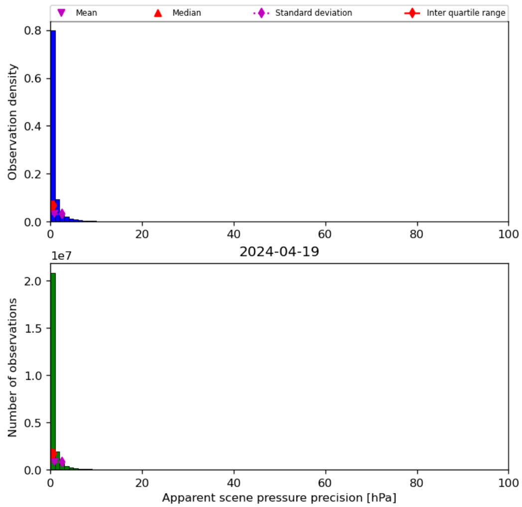
Figure 37: Histogram of “Apparent scene pressure precision” for 2024-04-18 to 2024-04-20
