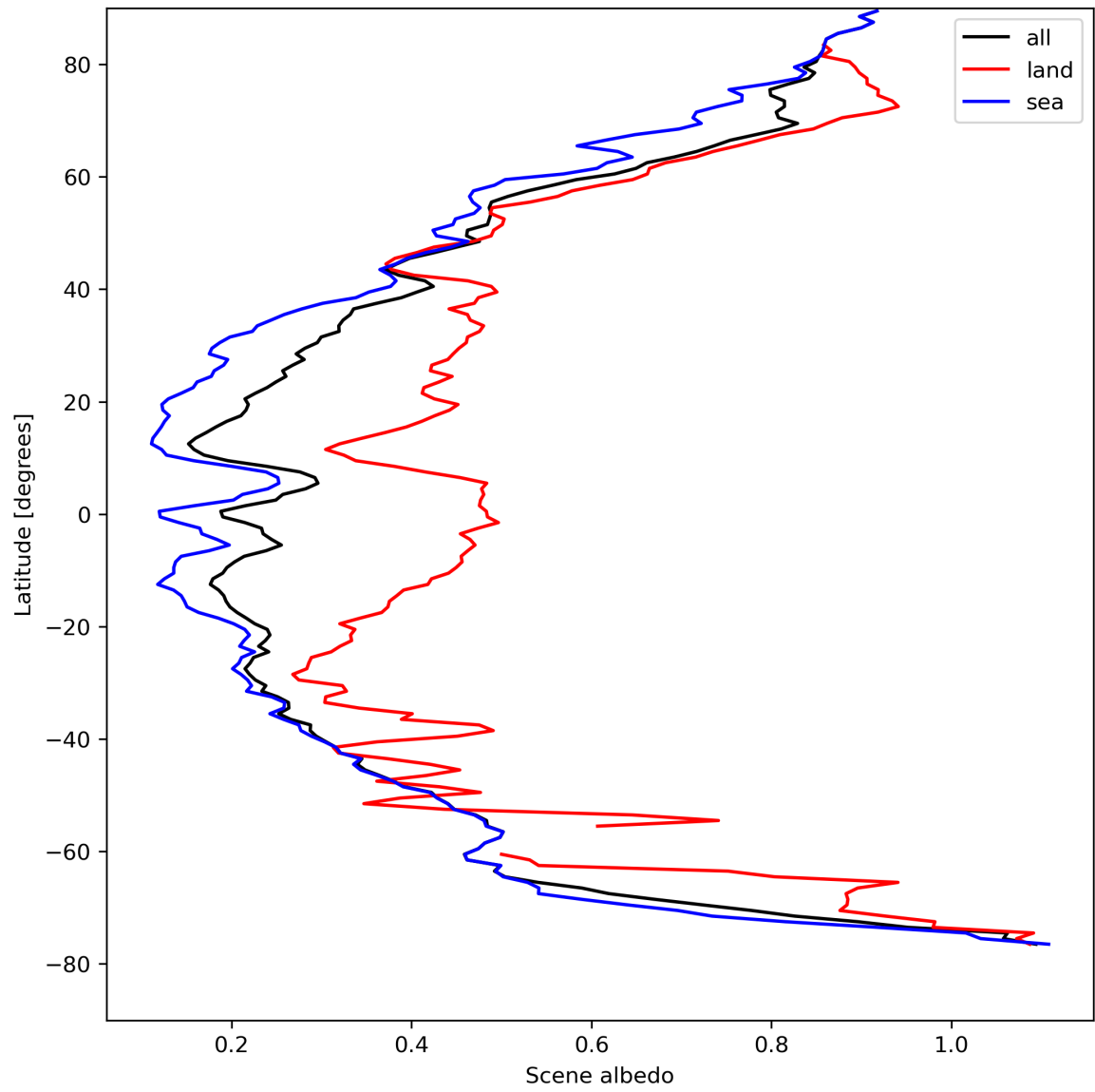
Figure 17: Zonal average of “Scene albedo” for 2024-04-18 to 2024-04-20.
