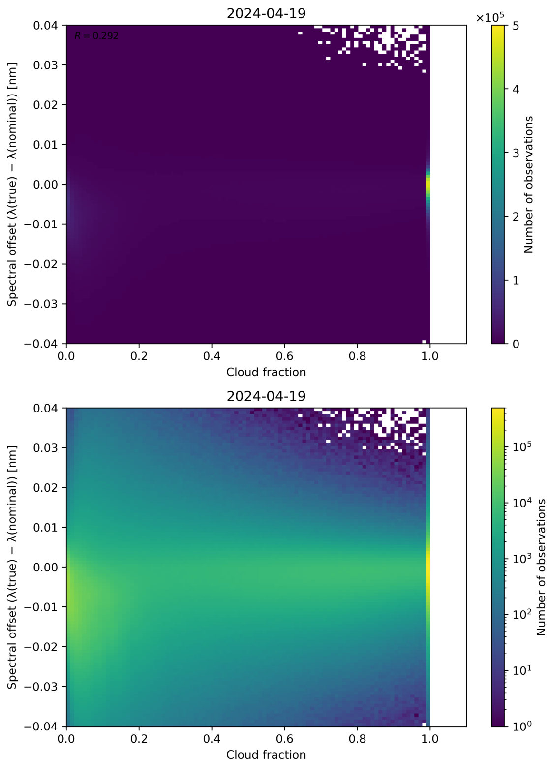
Figure 76: Scatter density plot of “Cloud fraction” against “Spectral offset ( \lambda(\text{true}) - \lambda(\text{nominal}) )” for 2024-04-18 to 2024-04-20.
