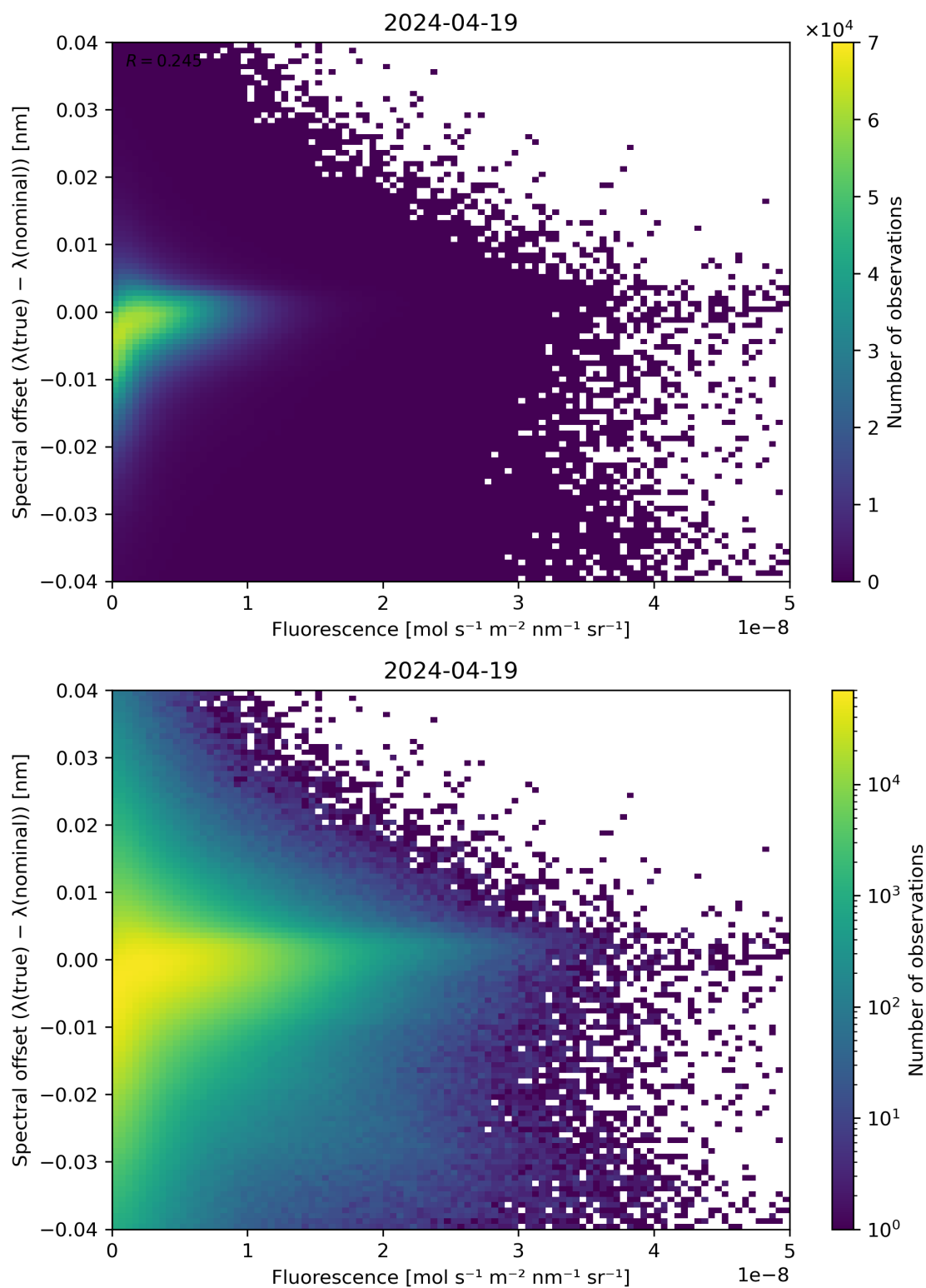
Figure 87: Scatter density plot of “Fluorescence” against “Spectral offset ( \lambda(\text{true}) - \lambda(\text{nominal}) )” for 2024-04-18 to 2024-04-20.
