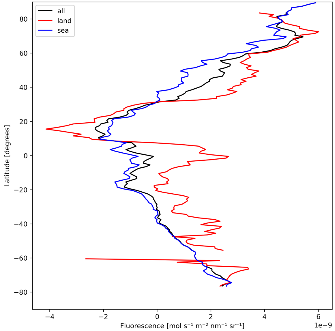
Figure 23: Zonal average of “Fluorescence” for 2024-04-18 to 2024-04-20.
