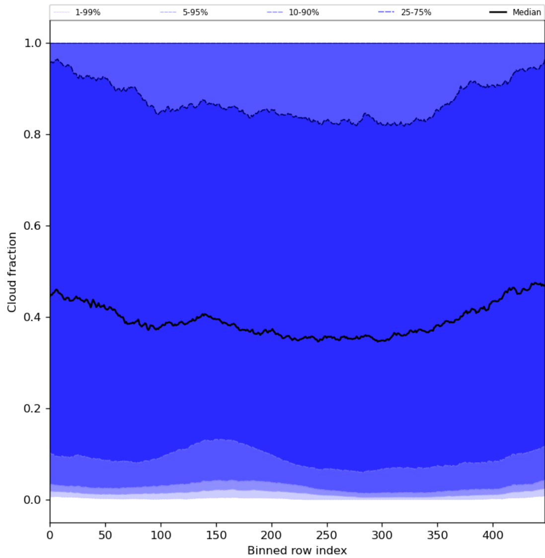
Figure 49: Along track statistics of “Cloud fraction” for 2024-04-18 to 2024-04-20
