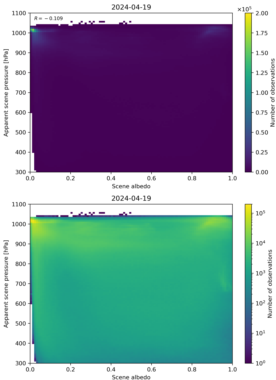
Figure 102: Scatter density plot of “Scene albedo” against “Apparent scene pressure” for 2024-04-18 to 2024-04-20.
