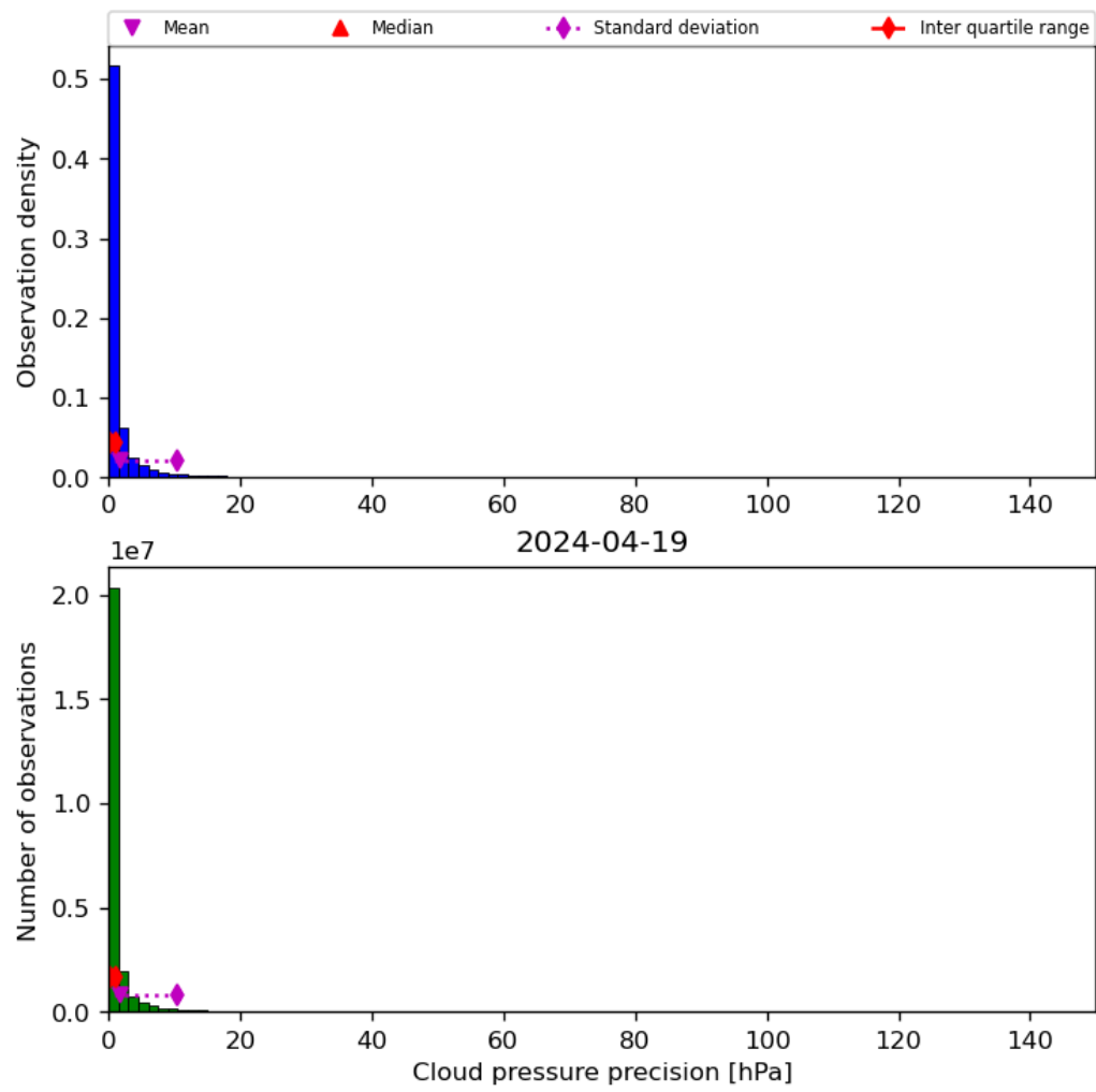
Figure 31: Histogram of “Cloud pressure precision” for 2024-04-18 to 2024-04-20
