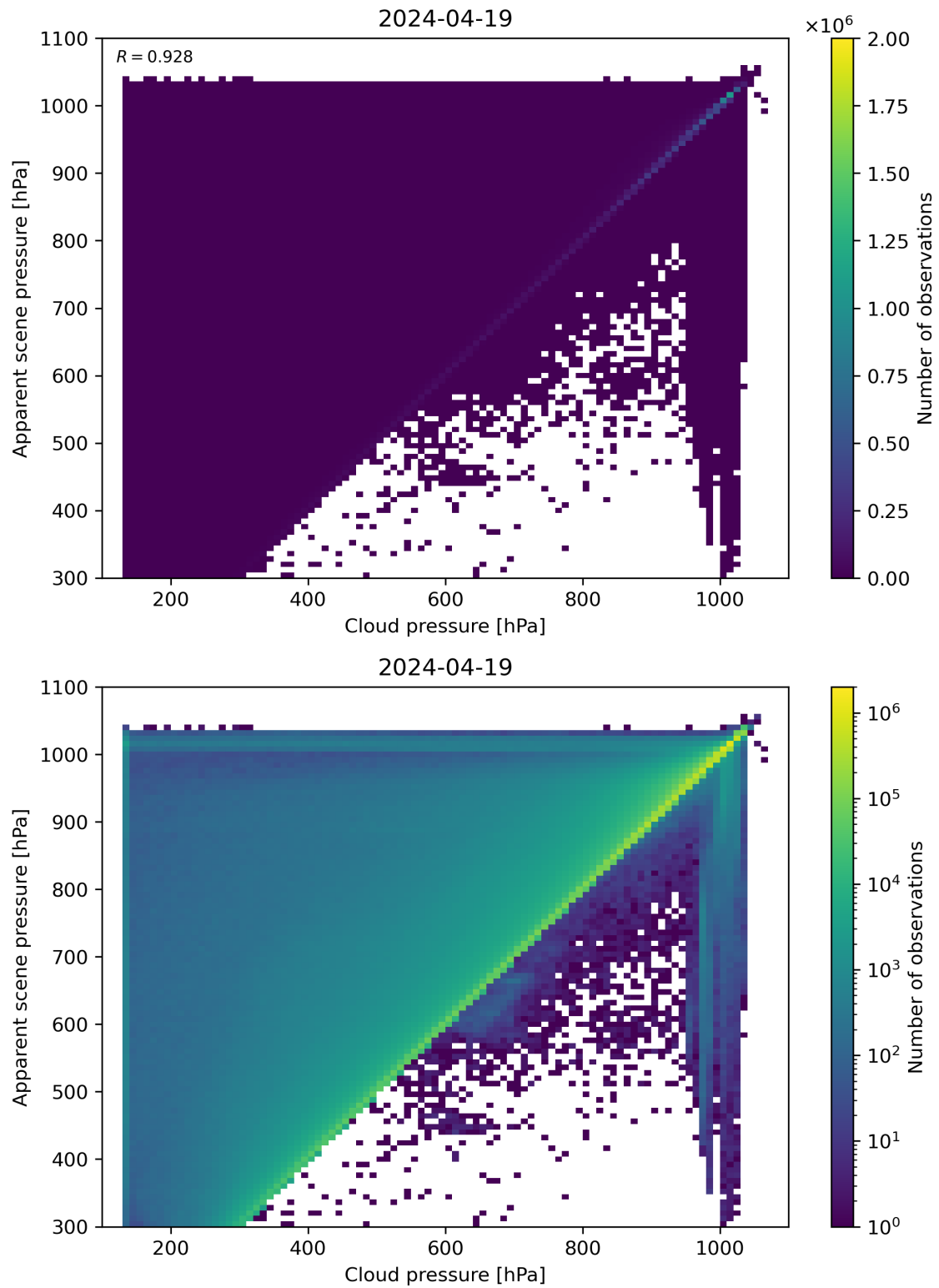
Figure 77: Scatter density plot of “Cloud pressure” against “Apparent scene pressure” for 2024-04-18 to 2024-04-20.
