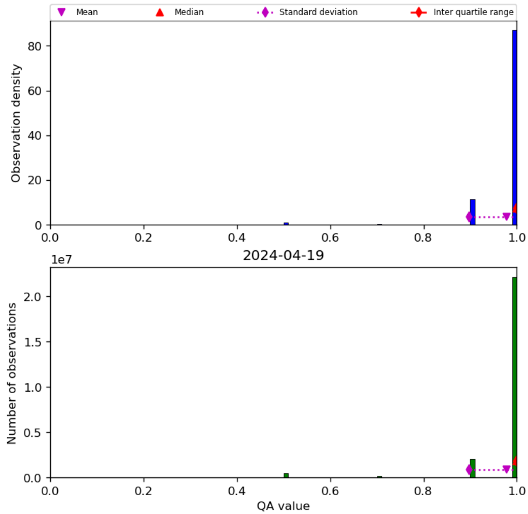
Figure 29: Histogram of “QA value” for 2024-04-18 to 2024-04-20
