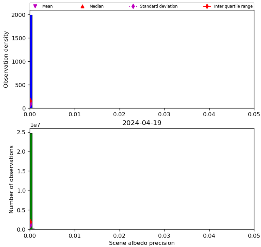
Figure 35: Histogram of “Scene albedo precision” for 2024-04-18 to 2024-04-20
