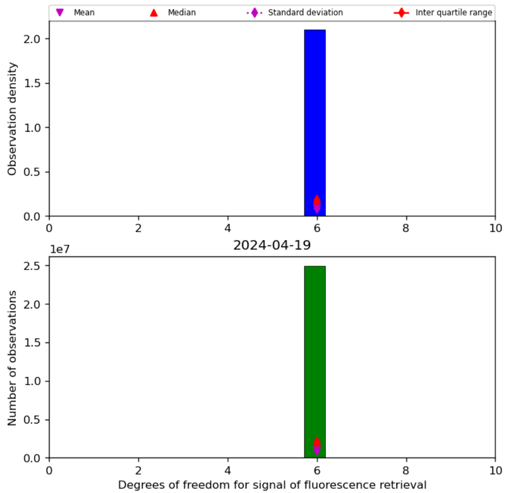
Figure 43: Histogram of “Degrees of freedom for signal of fluorescence retrieval” for 2024-04-18 to 2024-04-20
