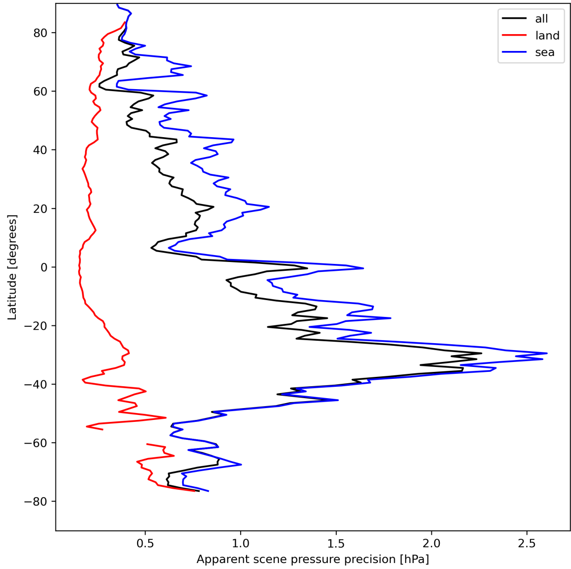
Figure 20: Zonal average of “Apparent scene pressure precision” for 2024-04-18 to 2024-04-20.
