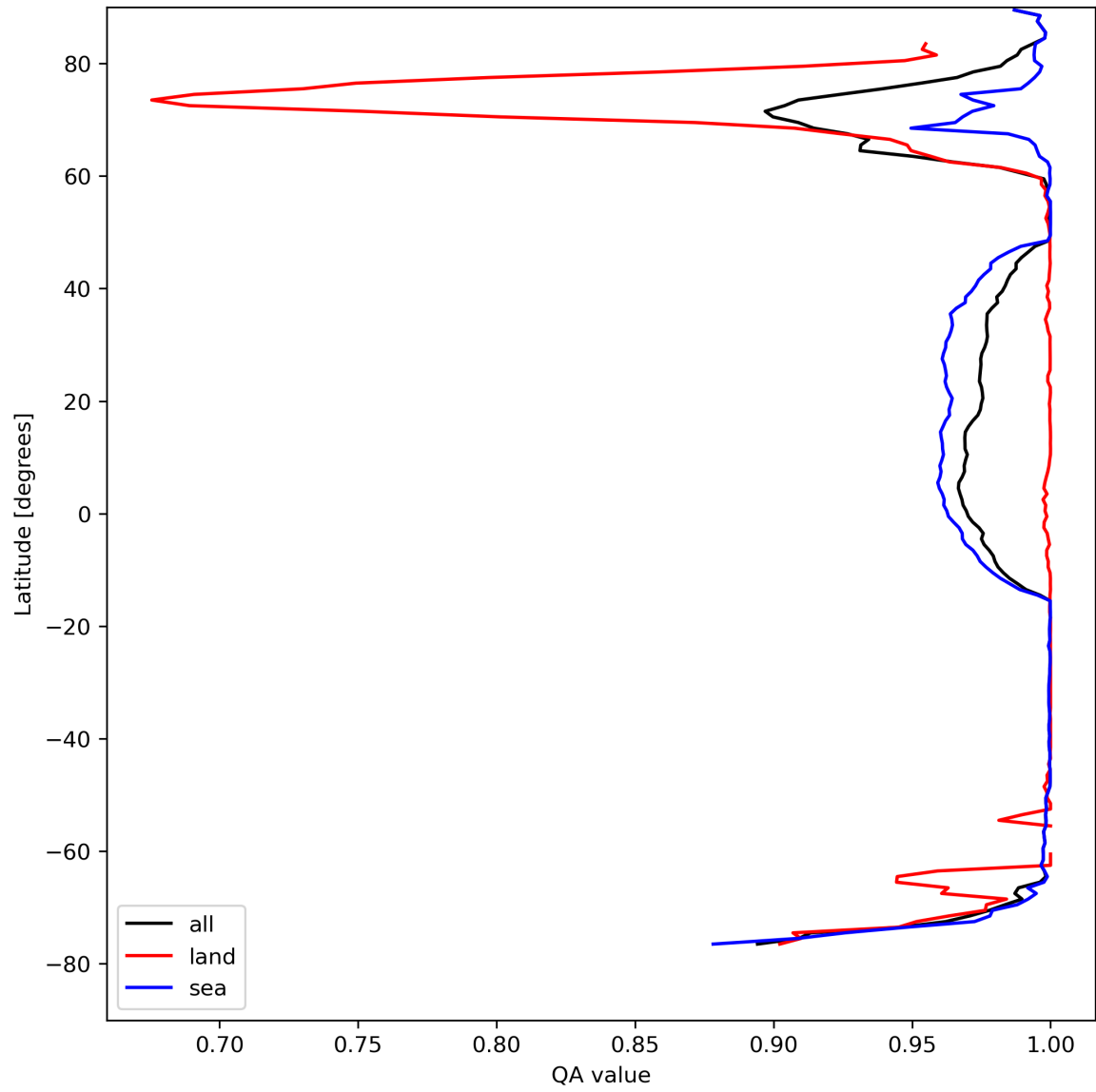
Figure 12: Zonal average of “QA value” for 2024-04-18 to 2024-04-20.
