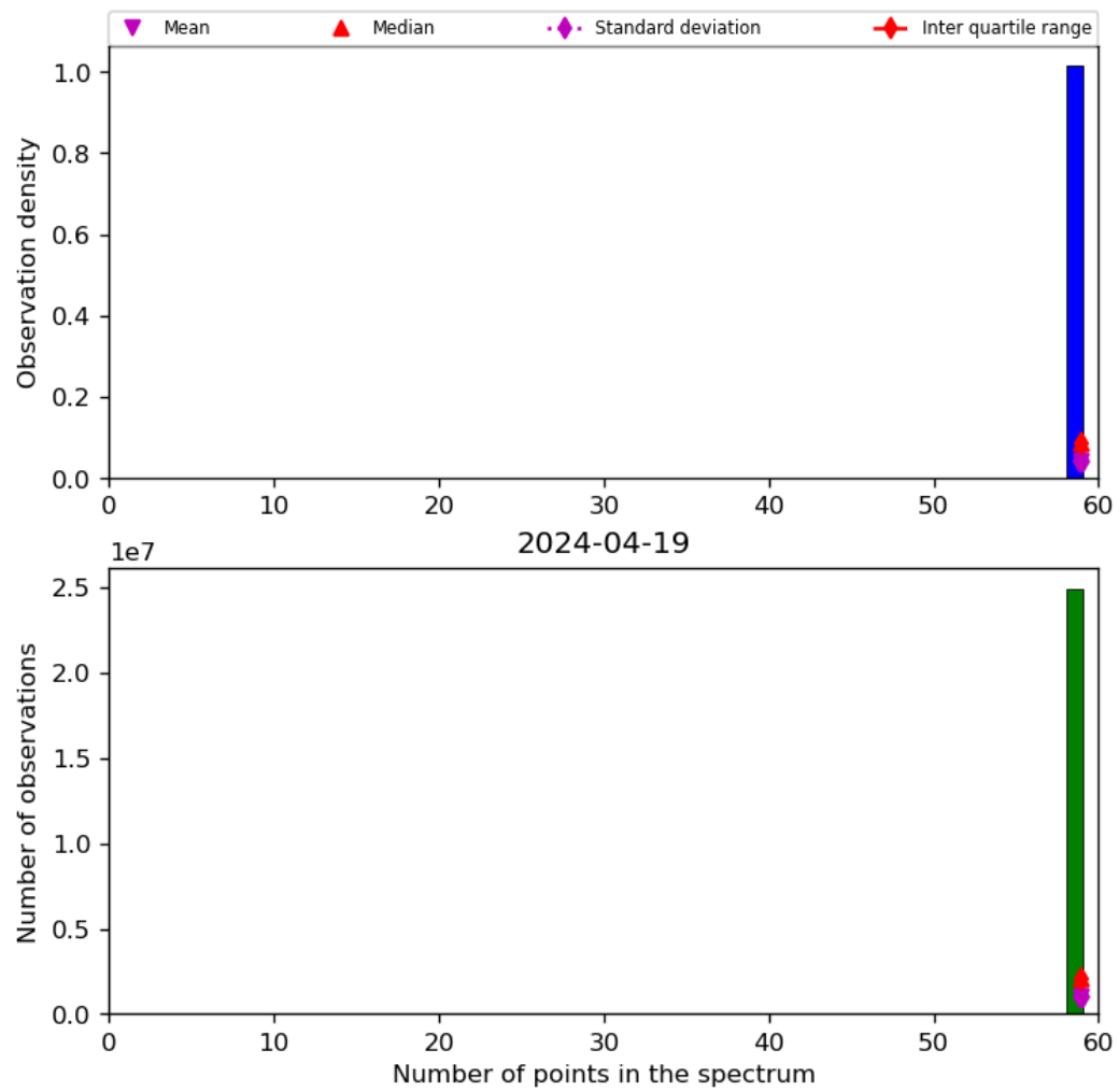
Figure 44: Histogram of “Number of points in the spectrum” for 2024-04-18 to 2024-04-20
