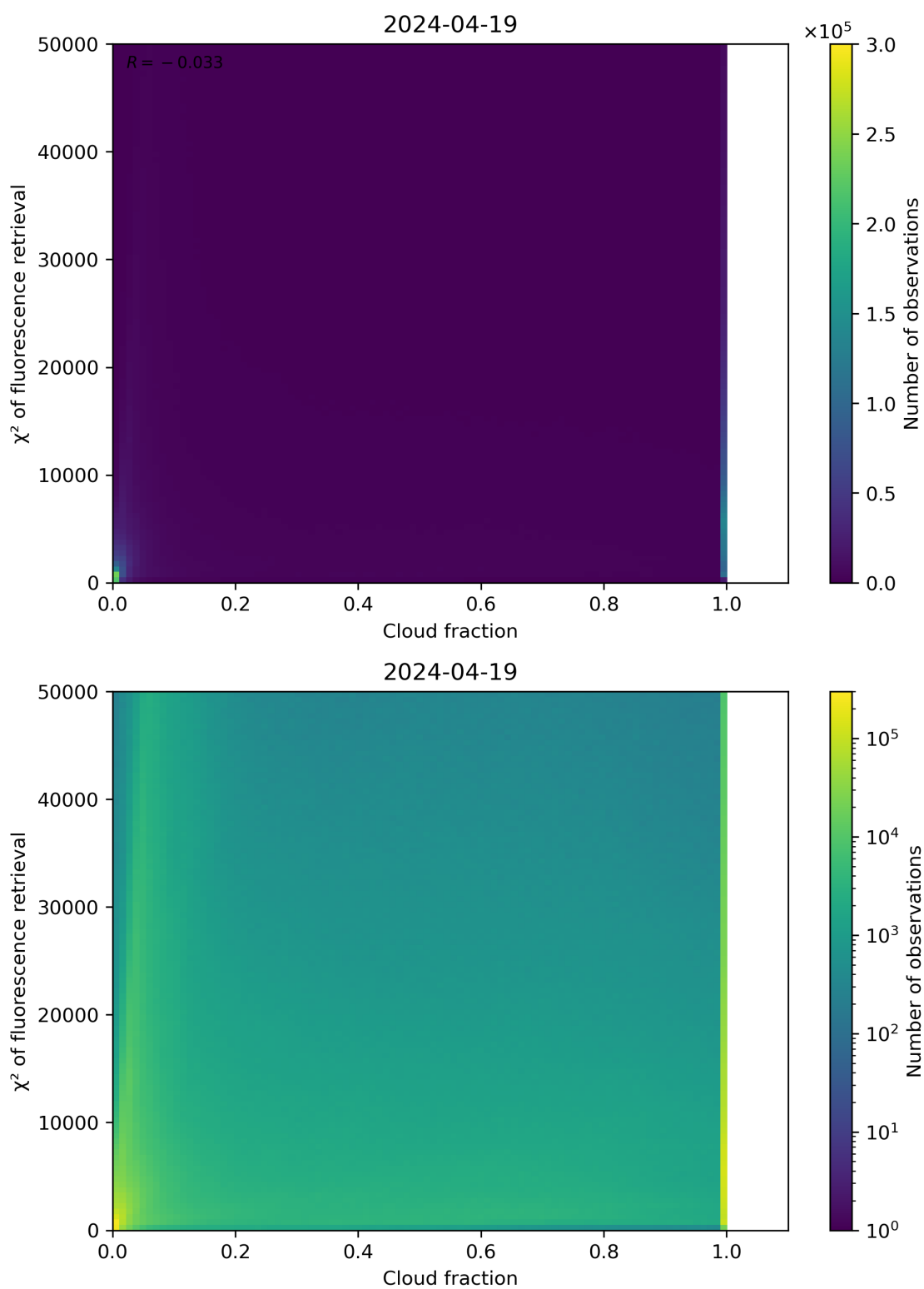
Figure 71: Scatter density plot of “Cloud fraction” against “ \chi^2 of fluorescence retrieval” for 2024-04-18 to 2024-04-20.
