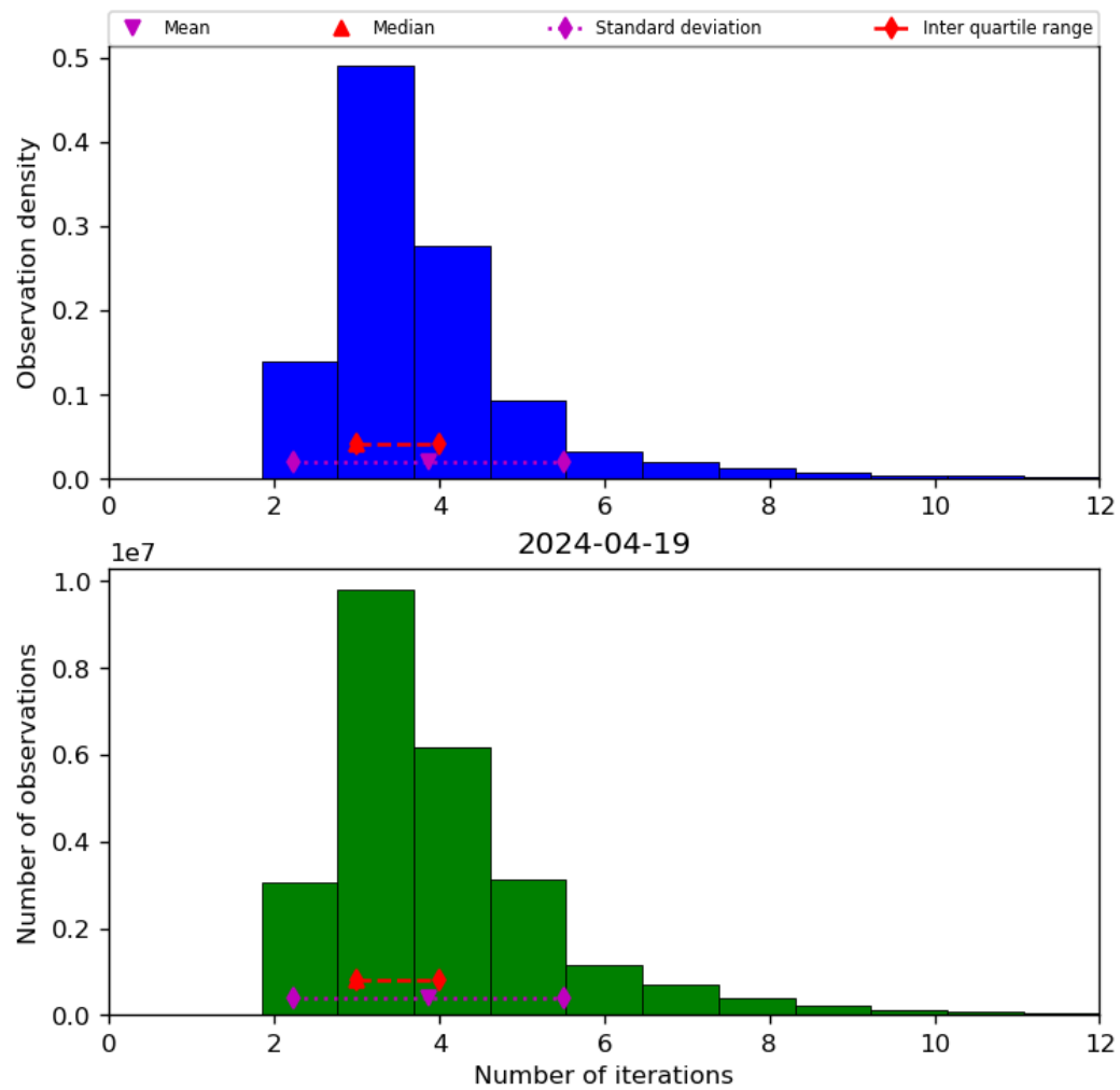
Figure 39: Histogram of “Number of iterations” for 2024-04-18 to 2024-04-20
