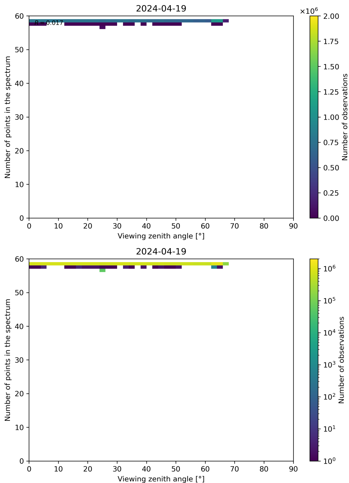
Figure 125: Scatter density plot of “Viewing zenith angle” against “Number of points in the spectrum” for 2024-04-18 to 2024-04-20.
