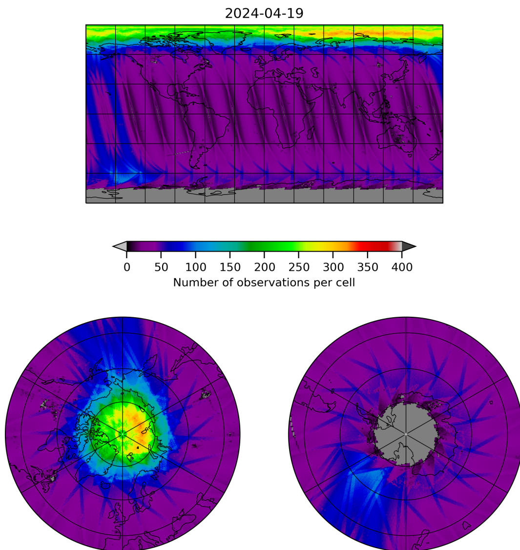
Figure 11: Map of the number of observations for 2024-04-18 to 2024-04-20
