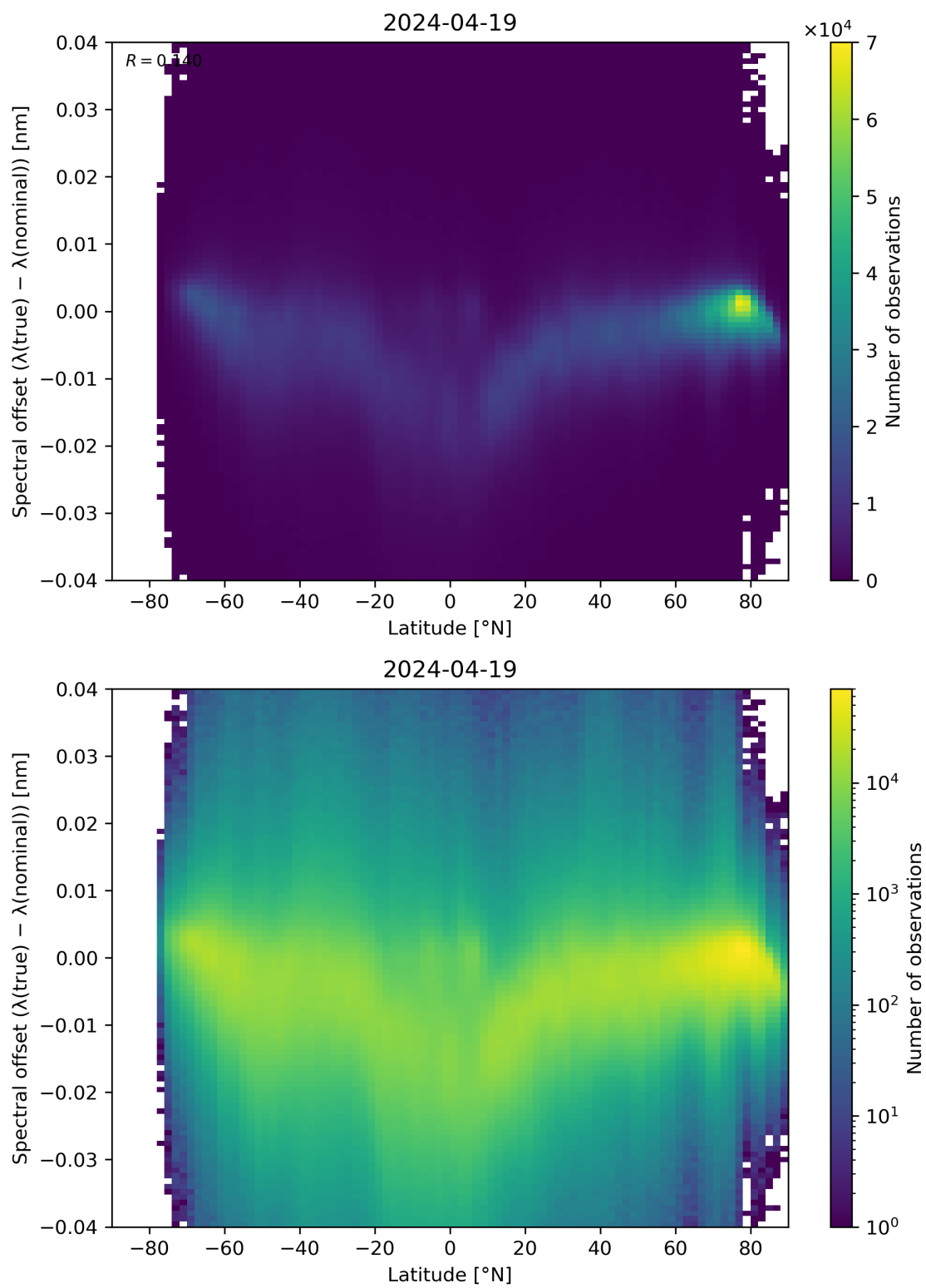
Figure 96: Scatter density plot of “Latitude” against “Spectral offset ( \lambda(\text{true}) - \lambda(\text{nominal}) )” for 2024-04-18 to 2024-04-20.
