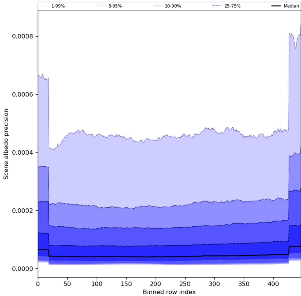
Figure 52: Along track statistics of “Scene albedo precision” for 2024-04-18 to 2024-04-20
