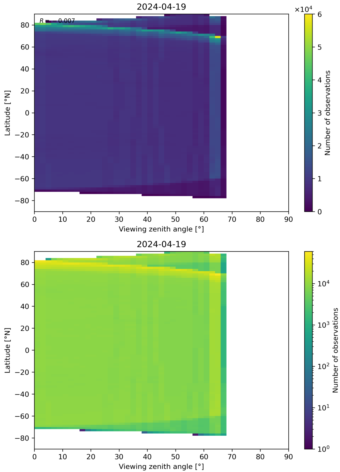
Figure 123: Scatter density plot of “Viewing zenith angle” against “Latitude” for 2024-04-18 to 2024-04-20.
