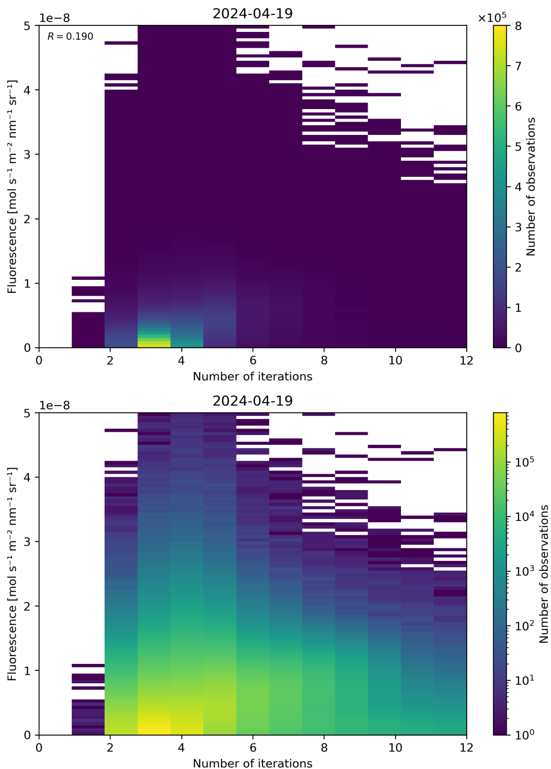
Figure 98: Scatter density plot of “Number of iterations” against “Fluorescence” for 2024-04-18 to 2024-04-20.
