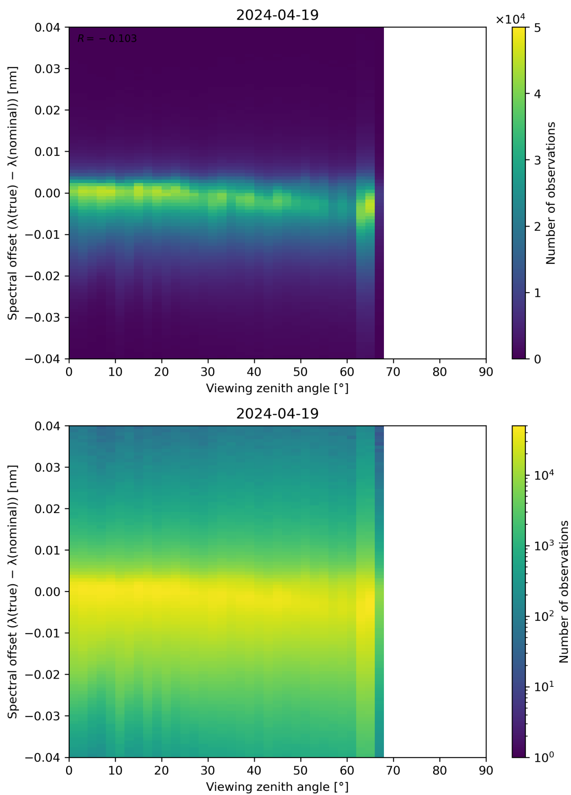
Figure 128: Scatter density plot of “Viewing zenith angle” against “Spectral offset ( \lambda(\text{true}) - \lambda(\text{nominal}) )” for 2024-04-18 to 2024-04-20.
