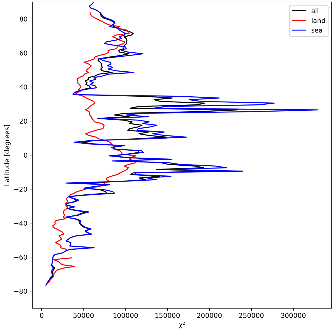
Figure 21: Zonal average of “ \chi^2 ” for 2024-04-18 to 2024-04-20.
