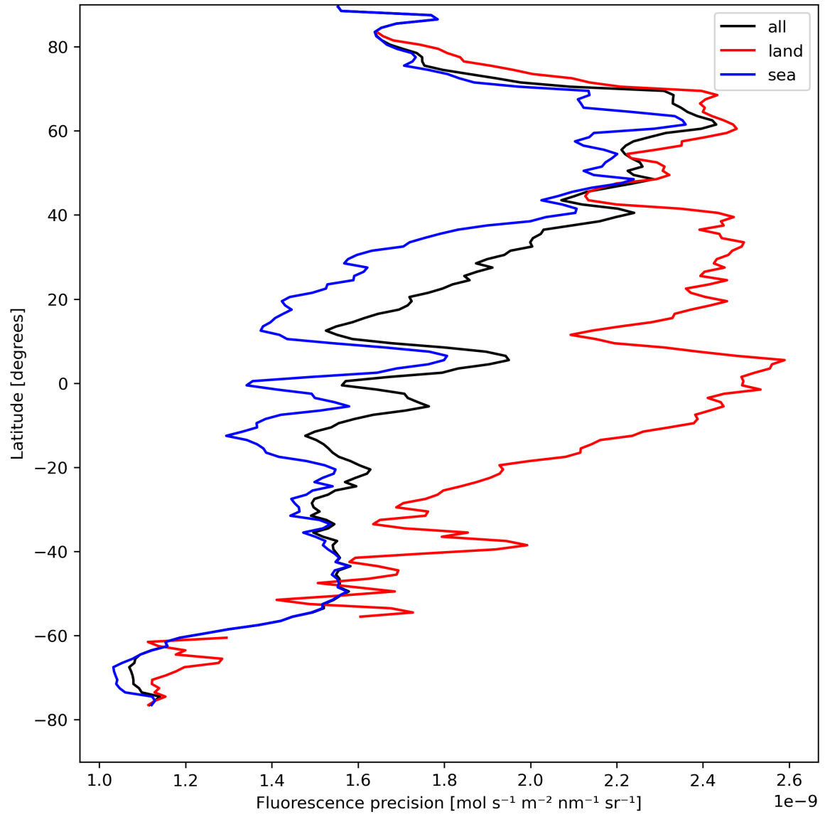
Figure 24: Zonal average of “Fluorescence precision” for 2024-04-18 to 2024-04-20.
