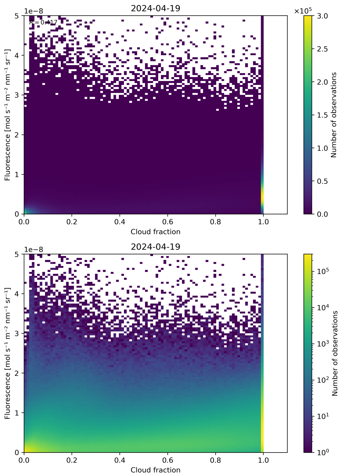
Figure 72: Scatter density plot of “Cloud fraction” against “Fluorescence” for 2024-04-18 to 2024-04-20.
