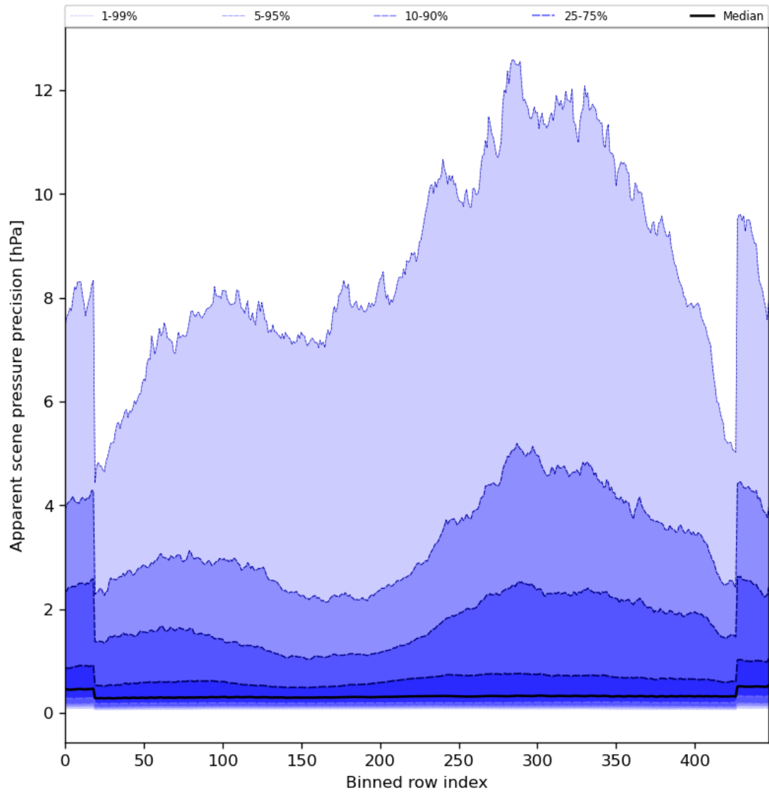
Figure 54: Along track statistics of “Apparent scene pressure precision” for 2024-04-18 to 2024-04-20
