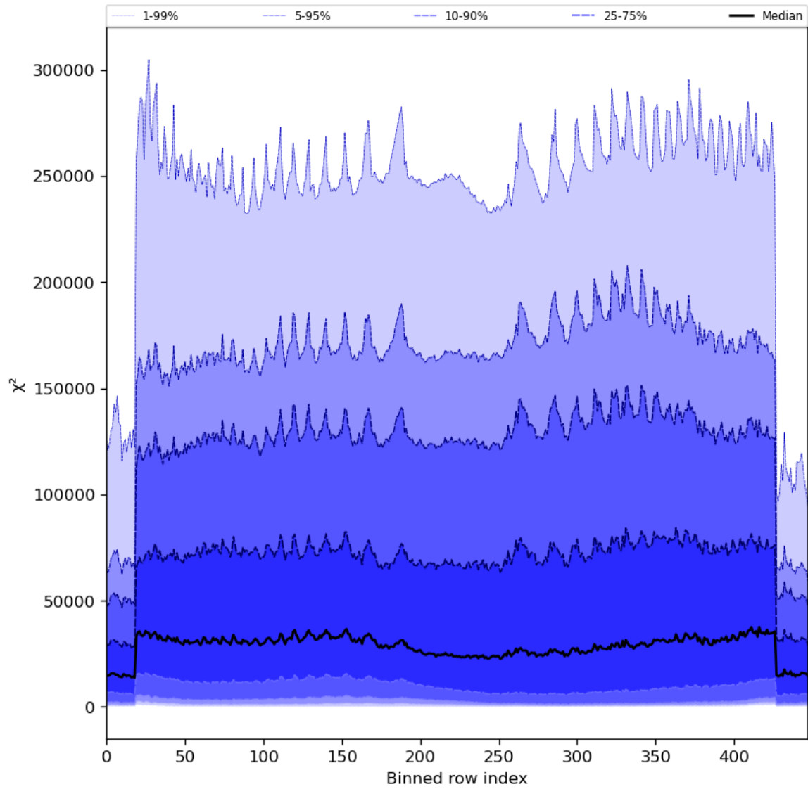
Figure 55: Along track statistics of “ \chi^2 ” for 2024-04-18 to 2024-04-20
