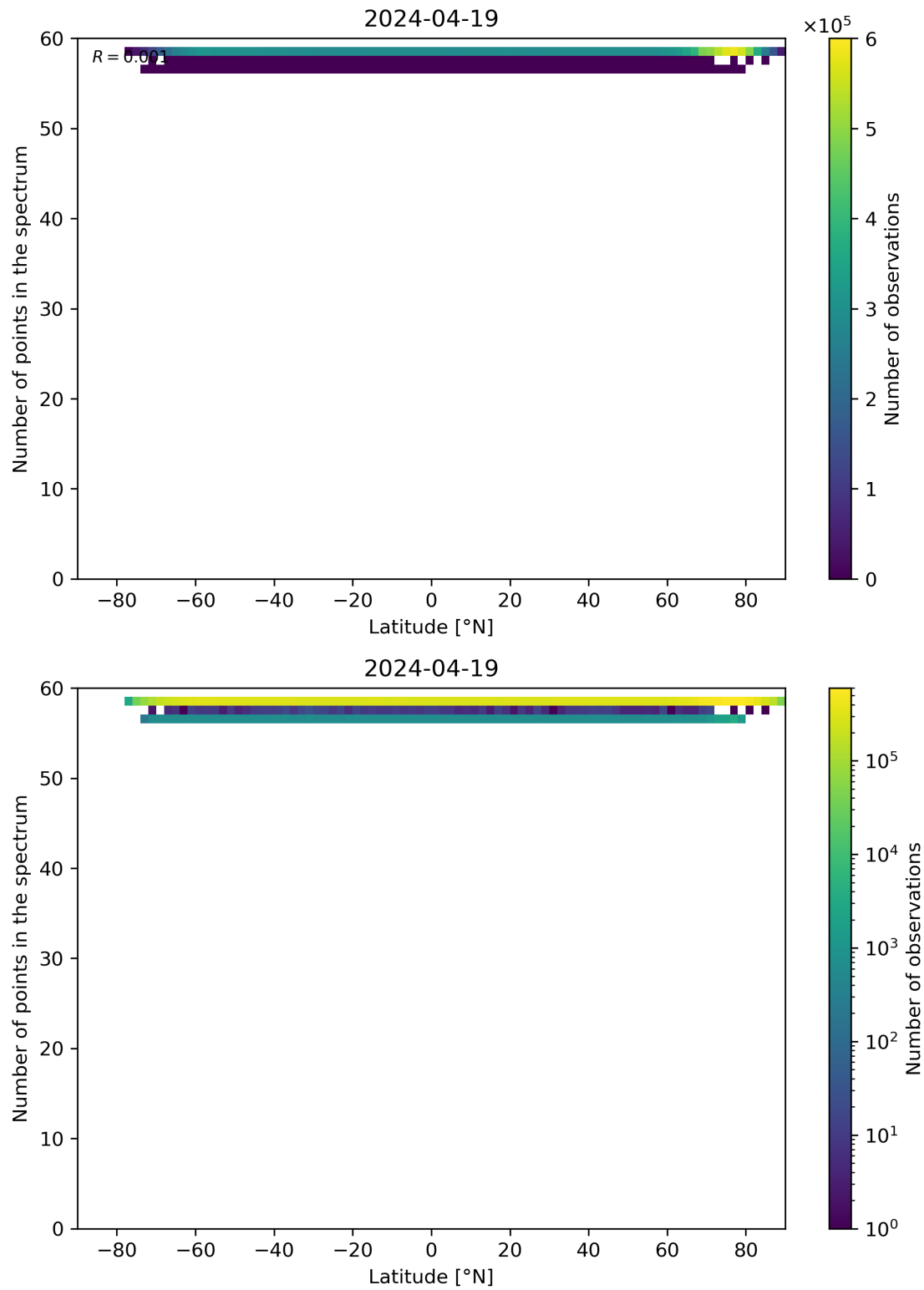
Figure 94: Scatter density plot of “Latitude” against “Number of points in the spectrum” for 2024-04-18 to 2024-04-20.
