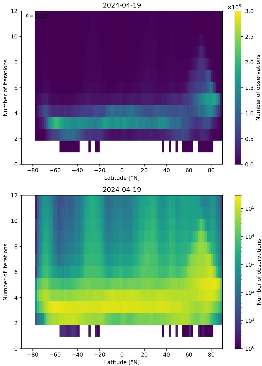
Figure 93: Scatter density plot of “Latitude” against “Number of iterations” for 2024-04-18 to 2024-04-20.
