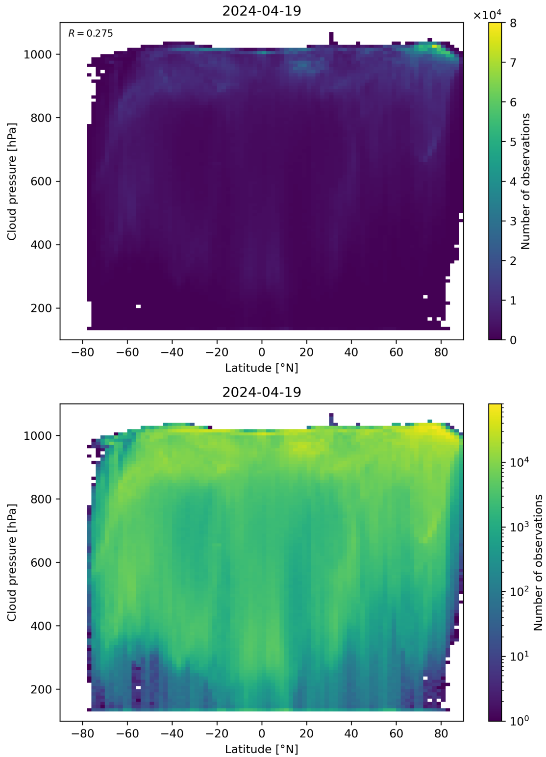
Figure 91: Scatter density plot of “Latitude” against “Cloud pressure” for 2024-04-18 to 2024-04-20.
