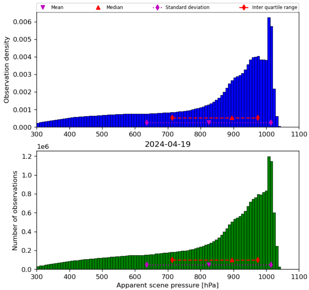
Figure 36: Histogram of “Apparent scene pressure” for 2024-04-18 to 2024-04-20
