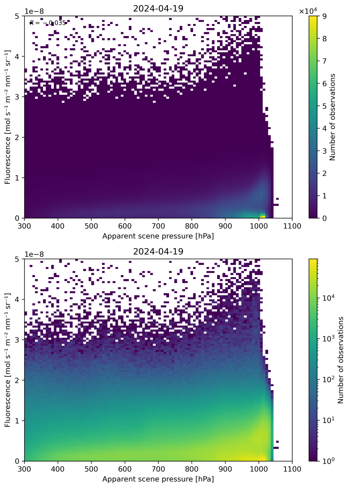
Figure 64: Scatter density plot of “Apparent scene pressure” against “Fluorescence” for 2024-04-18 to 2024-04-20.
