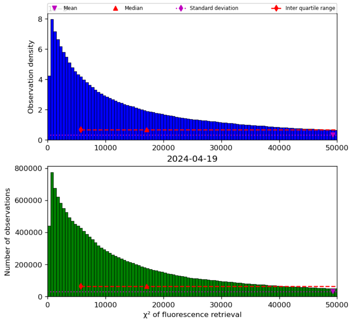
Figure 42: Histogram of “ \chi^2 of fluorescence retrieval” for 2024-04-18 to 2024-04-20
