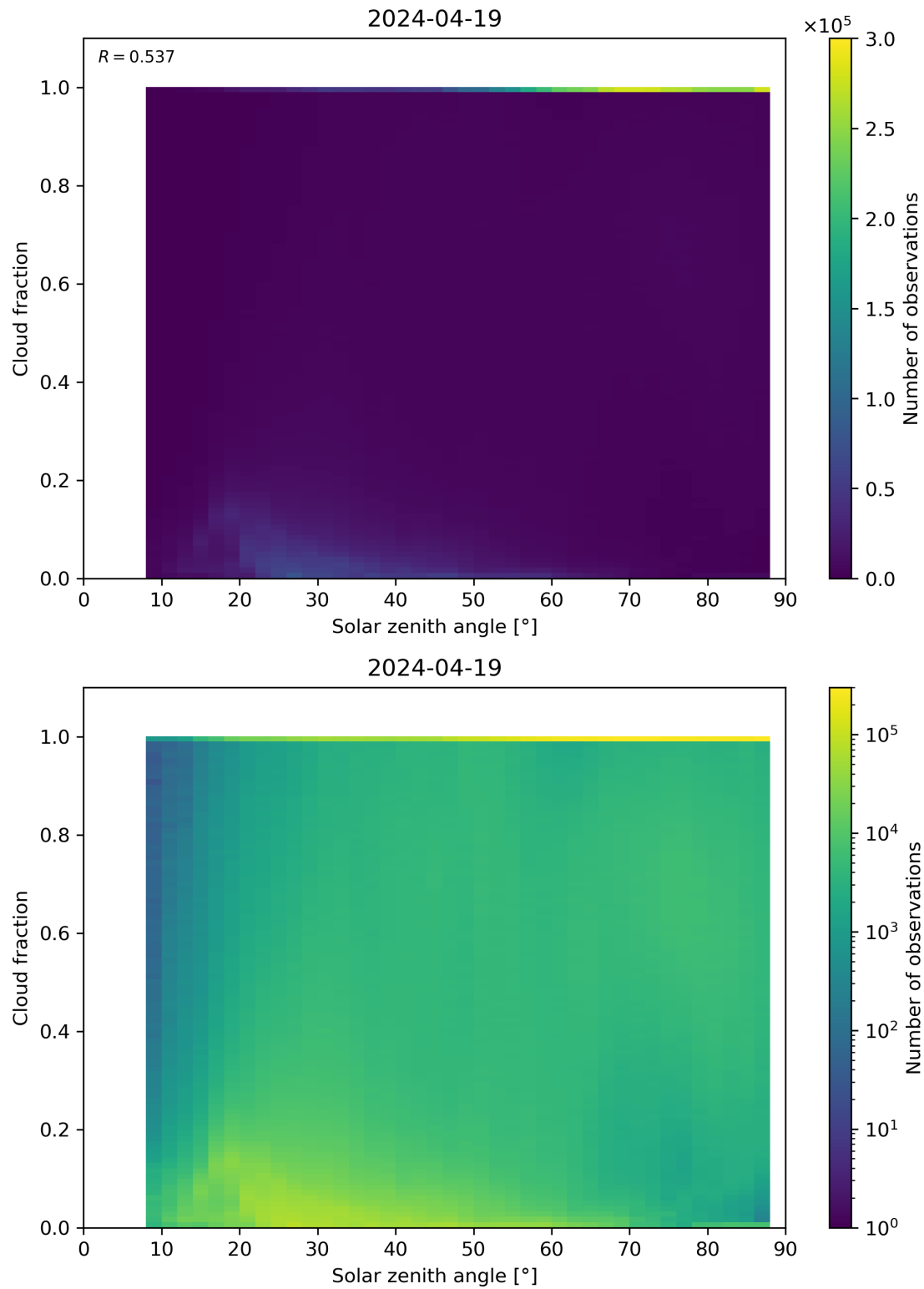
Figure 110: Scatter density plot of “Solar zenith angle” against “Cloud fraction” for 2024-04-18 to 2024-04-20.
