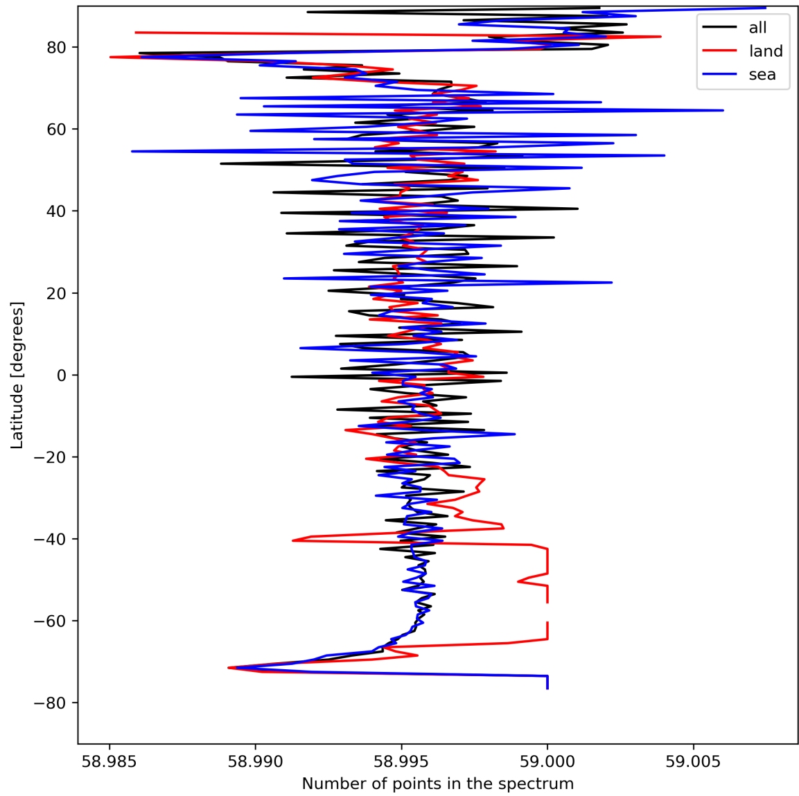
Figure 27: Zonal average of “Number of points in the spectrum” for 2024-04-18 to 2024-04-20.
