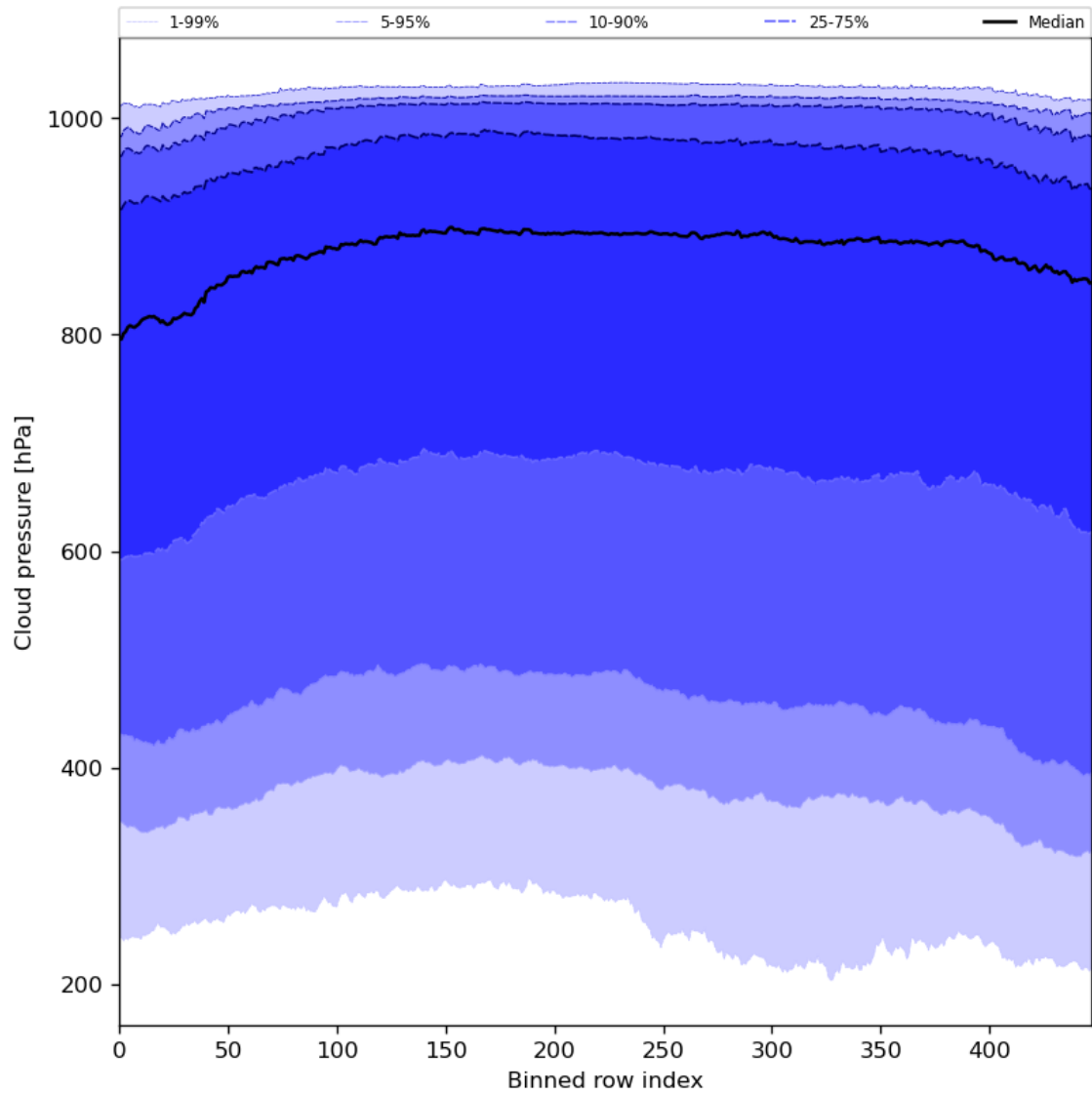
Figure 47: Along track statistics of “Cloud pressure” for 2024-04-18 to 2024-04-20
