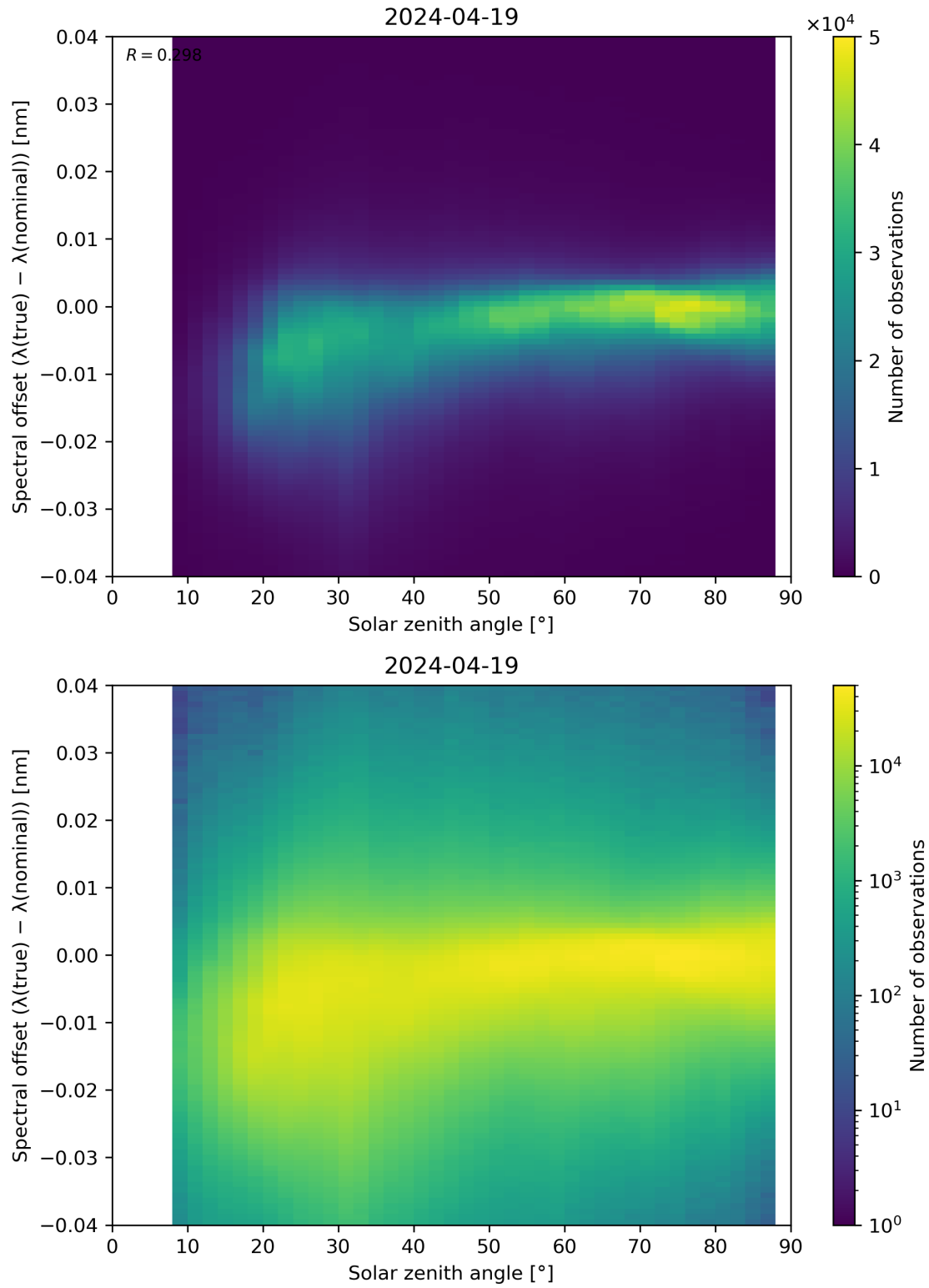
Figure 117: Scatter density plot of “Solar zenith angle” against “Spectral offset ( \lambda(\text{true}) - \lambda(\text{nominal}) )” for 2024-04-18 to 2024-04-20.
