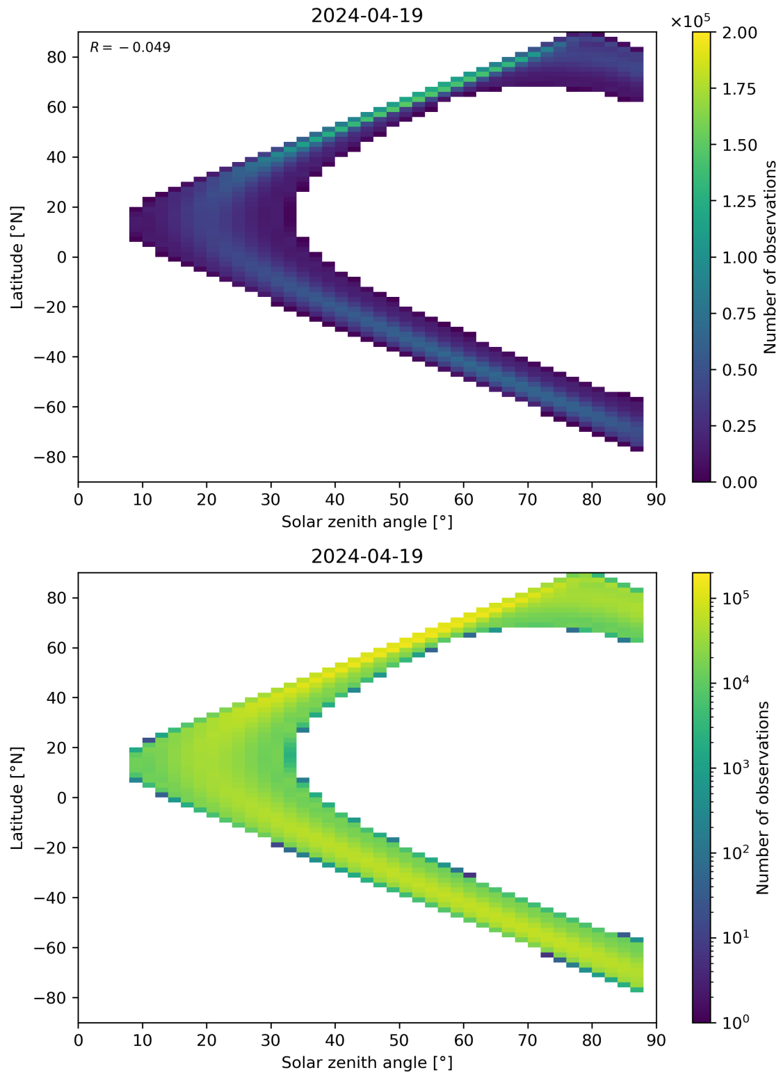
Figure 113: Scatter density plot of “Solar zenith angle” against “Latitude” for 2024-04-18 to 2024-04-20.
