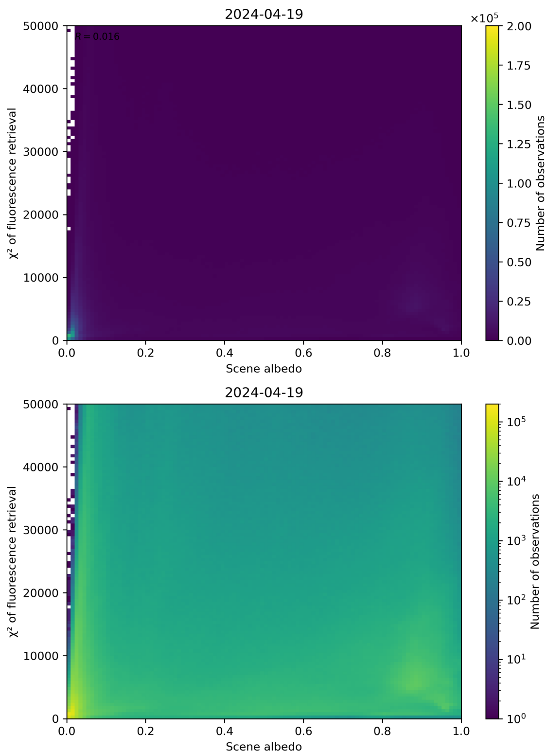
Figure 103: Scatter density plot of “Scene albedo” against “ \chi^2 of fluorescence retrieval” for 2024-04-18 to 2024-04-20.
