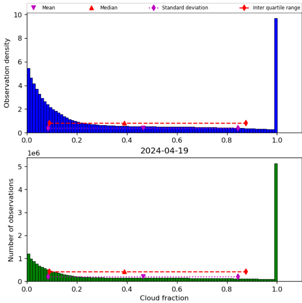
Figure 32: Histogram of “Cloud fraction” for 2024-04-18 to 2024-04-20
