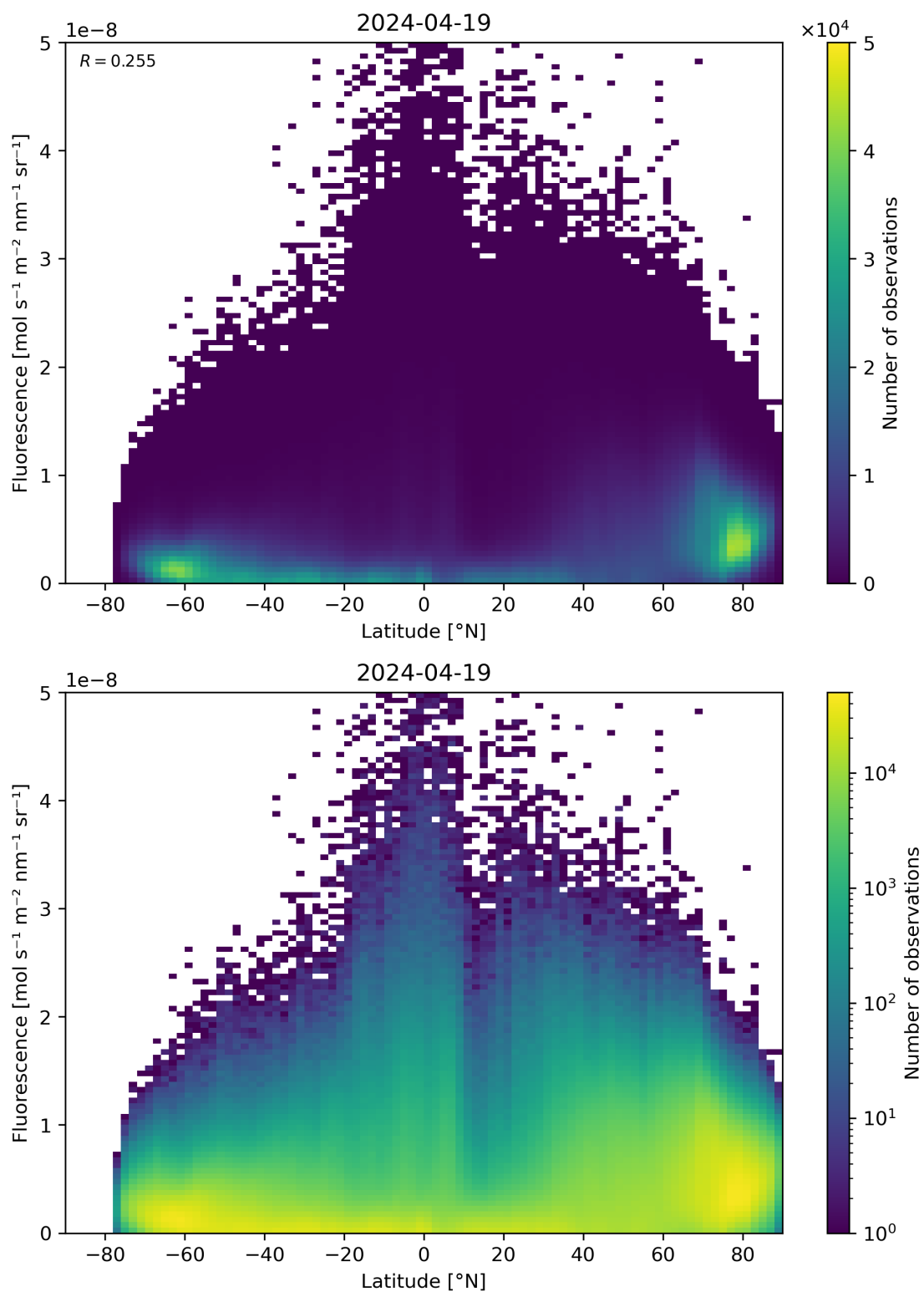
Figure 92: Scatter density plot of “Latitude” against “Fluorescence” for 2024-04-18 to 2024-04-20.
