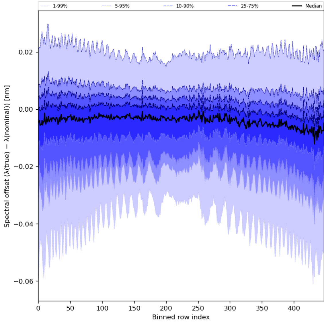
Figure 62: Along track statistics of “Spectral offset ( \lambda(\text{true}) - \lambda(\text{nominal}) )” for 2024-04-18 to 2024-04-20
