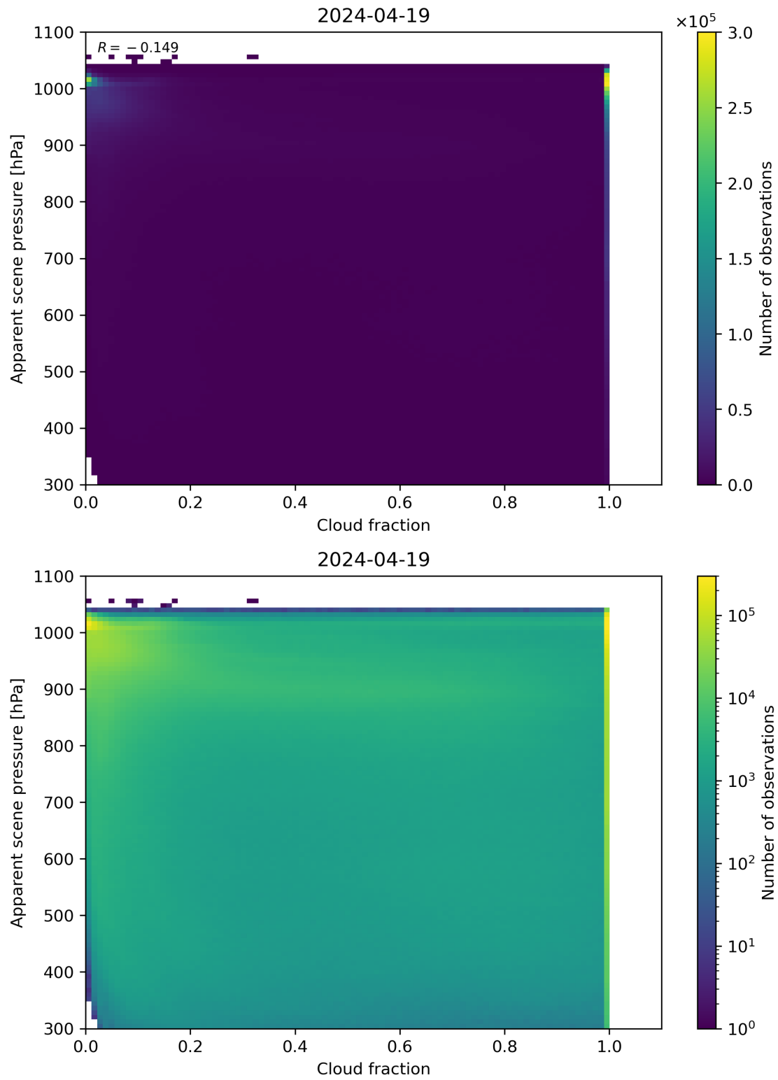
Figure 70: Scatter density plot of “Cloud fraction” against “Apparent scene pressure” for 2024-04-18 to 2024-04-20.
