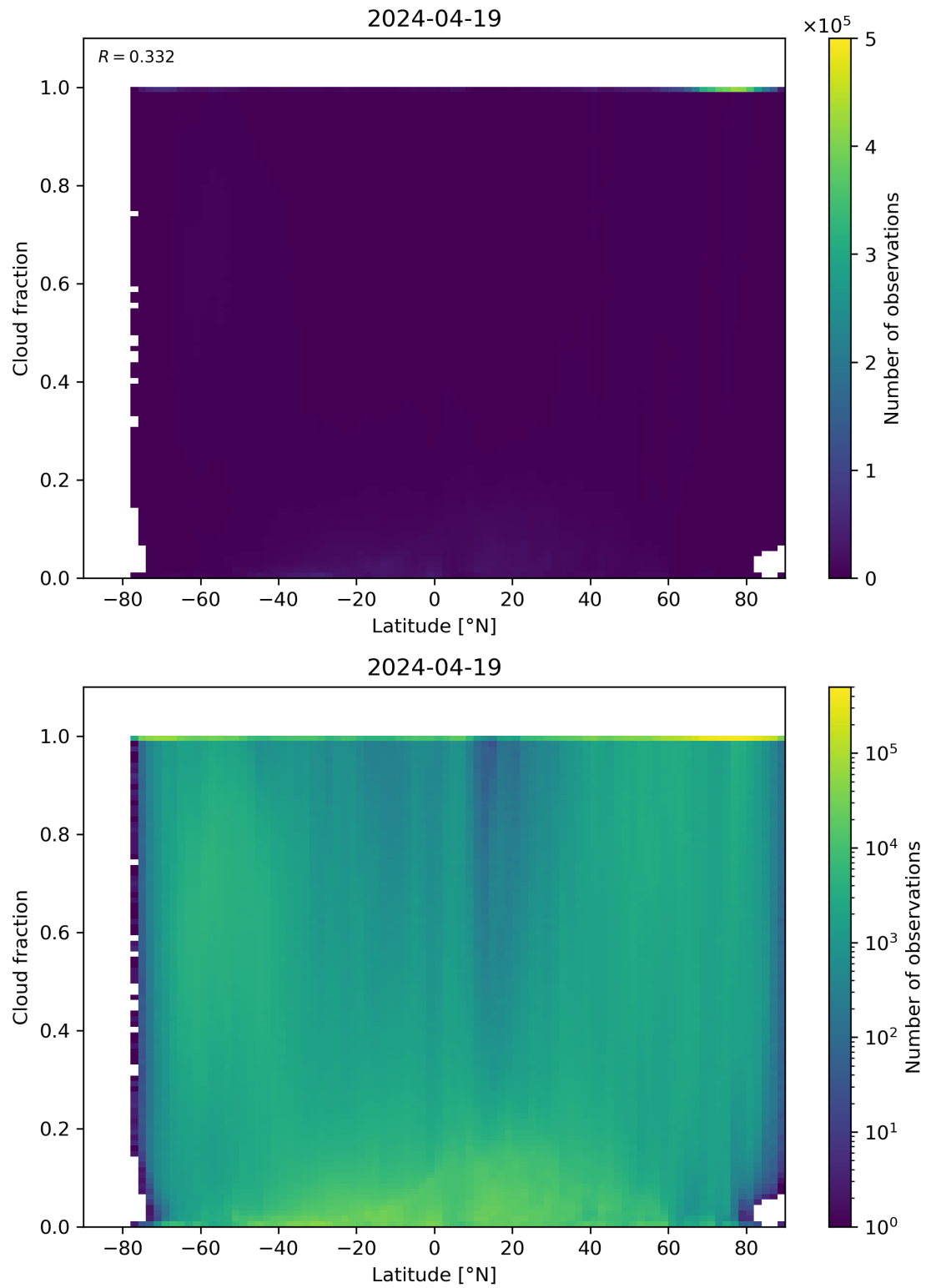
Figure 90: Scatter density plot of “Latitude” against “Cloud fraction” for 2024-04-18 to 2024-04-20.
