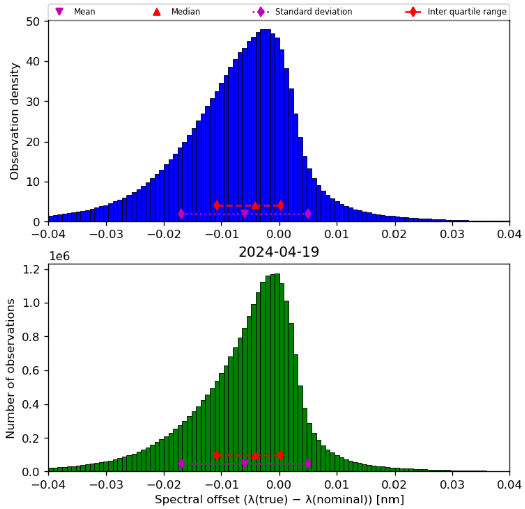
Figure 45: Histogram of “Spectral offset ( \lambda(\text{true}) - \lambda(\text{nominal}) )” for 2024-04-18 to 2024-04-20
