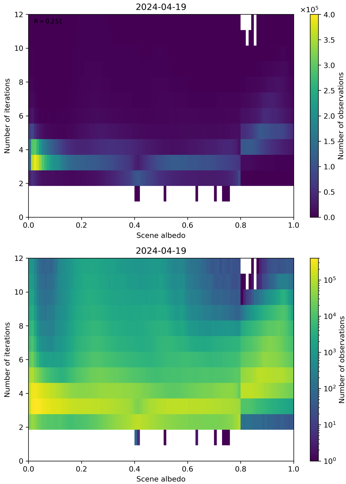
Figure 105: Scatter density plot of “Scene albedo” against “Number of iterations” for 2024-04-18 to 2024-04-20.
