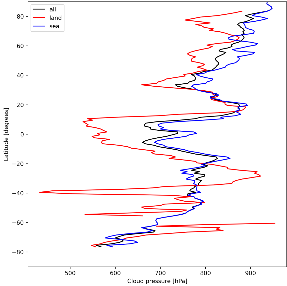
Figure 13: Zonal average of “Cloud pressure” for 2024-04-18 to 2024-04-20.
