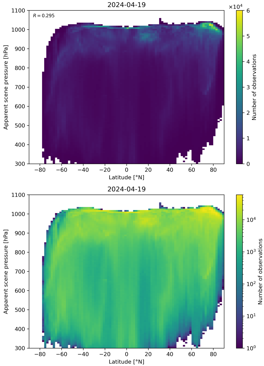
Figure 88: Scatter density plot of “Latitude” against “Apparent scene pressure” for 2024-04-18 to 2024-04-20.
