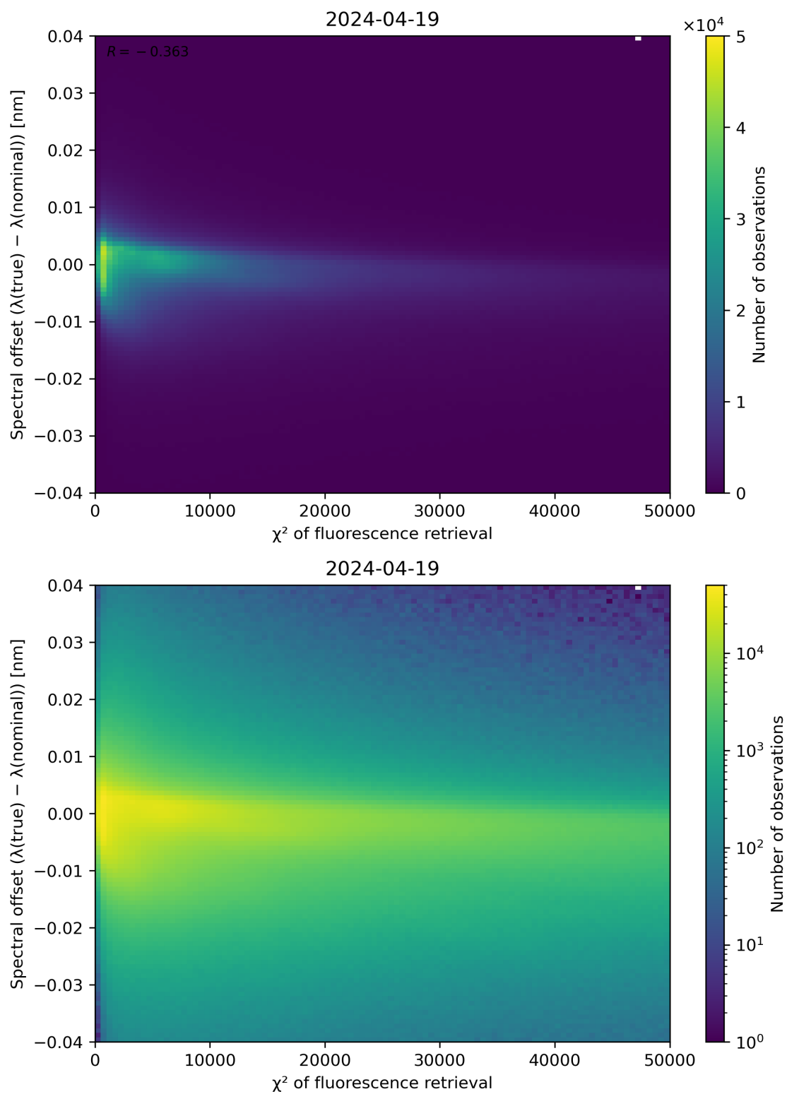
Figure 69: Scatter density plot of " \chi^2 of fluorescence retrieval" against "Spectral offset ( \lambda(\text{true}) - \lambda(\text{nominal})) " for 2024-04-18 to 2024-04-20.
