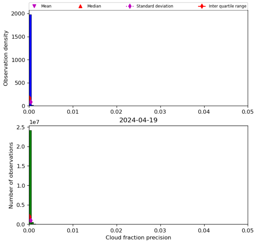
Figure 33: Histogram of “Cloud fraction precision” for 2024-04-18 to 2024-04-20
