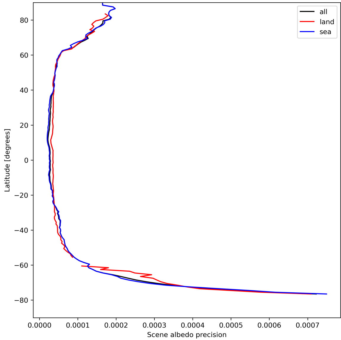
Figure 18: Zonal average of “Scene albedo precision” for 2024-04-18 to 2024-04-20.
