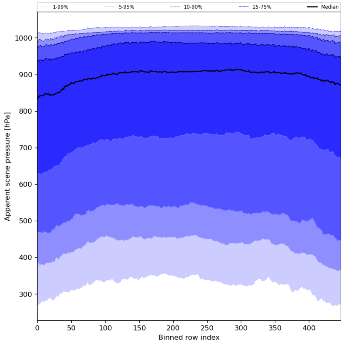
Figure 53: Along track statistics of “Apparent scene pressure” for 2024-04-18 to 2024-04-20
