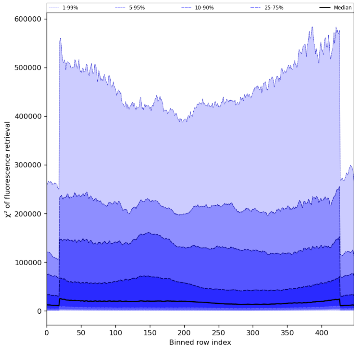
Figure 59: Along track statistics of “ \chi^2 of fluorescence retrieval” for 2024-04-18 to 2024-04-20
