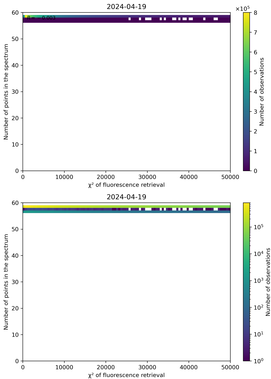
Figure 68: Scatter density plot of " \chi^2 of fluorescence retrieval" against "Number of points in the spectrum" for 2024-04-18 to 2024-04-20.
