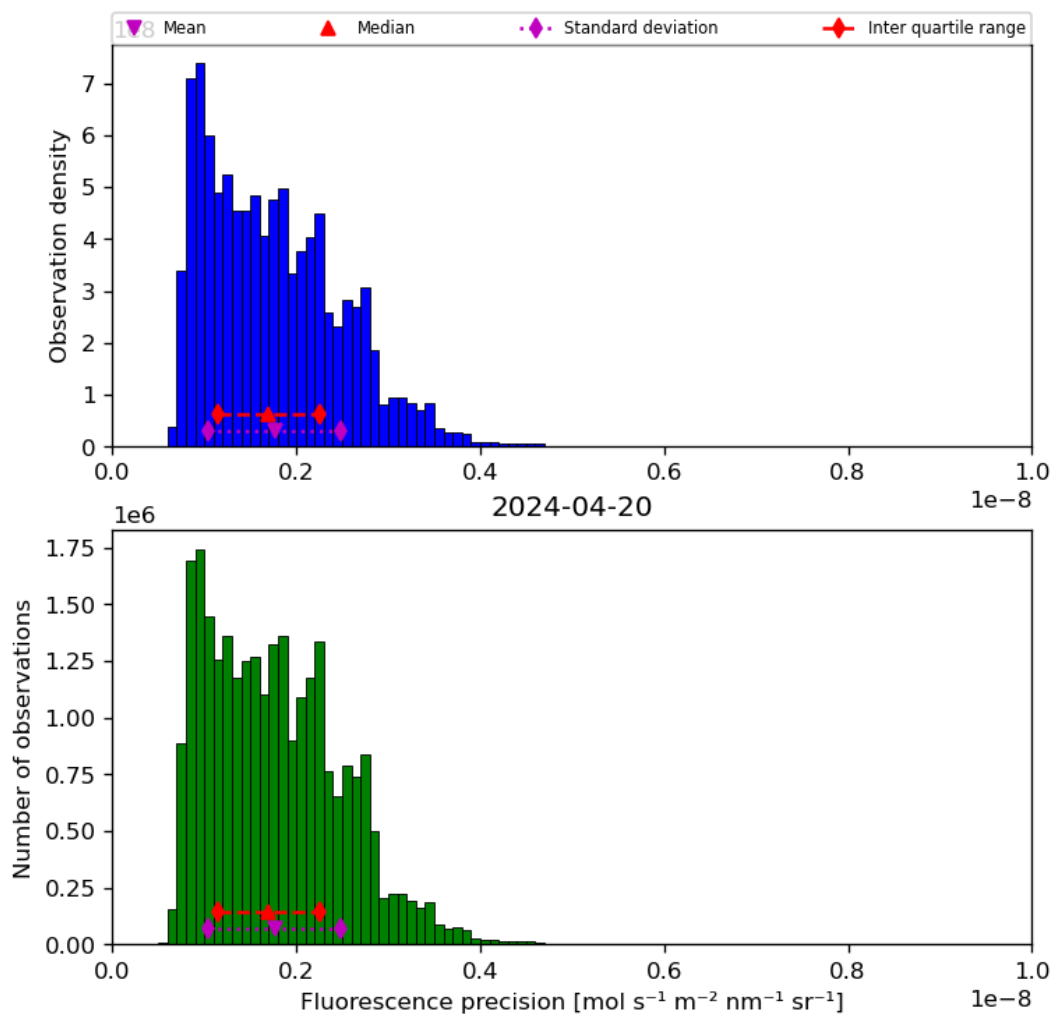
Figure 41: Histogram of “Fluorescence precision” for 2024-04-19 to 2024-04-21
