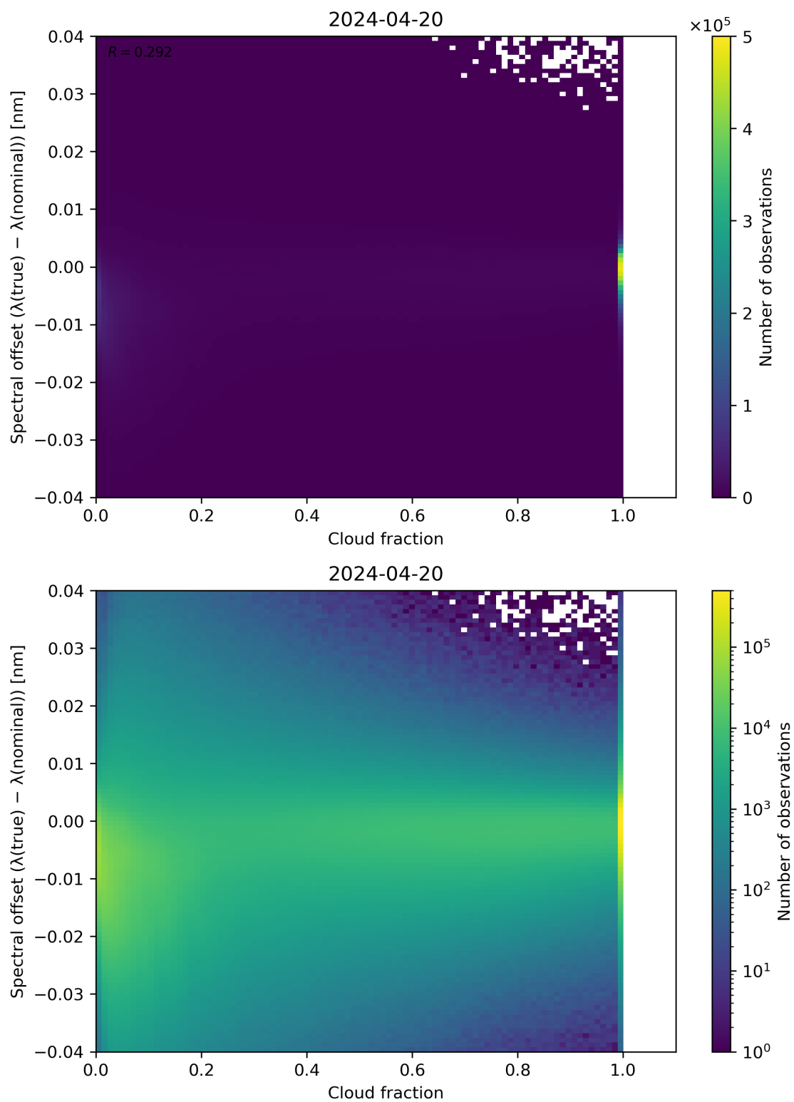
Figure 76: Scatter density plot of “Cloud fraction” against “Spectral offset ( \lambda(\text{true}) - \lambda(\text{nominal}) )” for 2024-04-19 to 2024-04-21.
