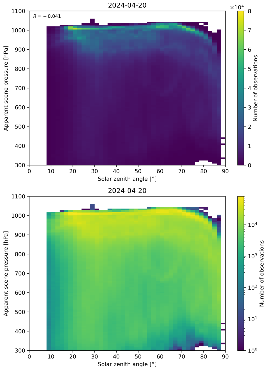
Figure 108: Scatter density plot of “Solar zenith angle” against “Apparent scene pressure” for 2024-04-19 to 2024-04-21.
