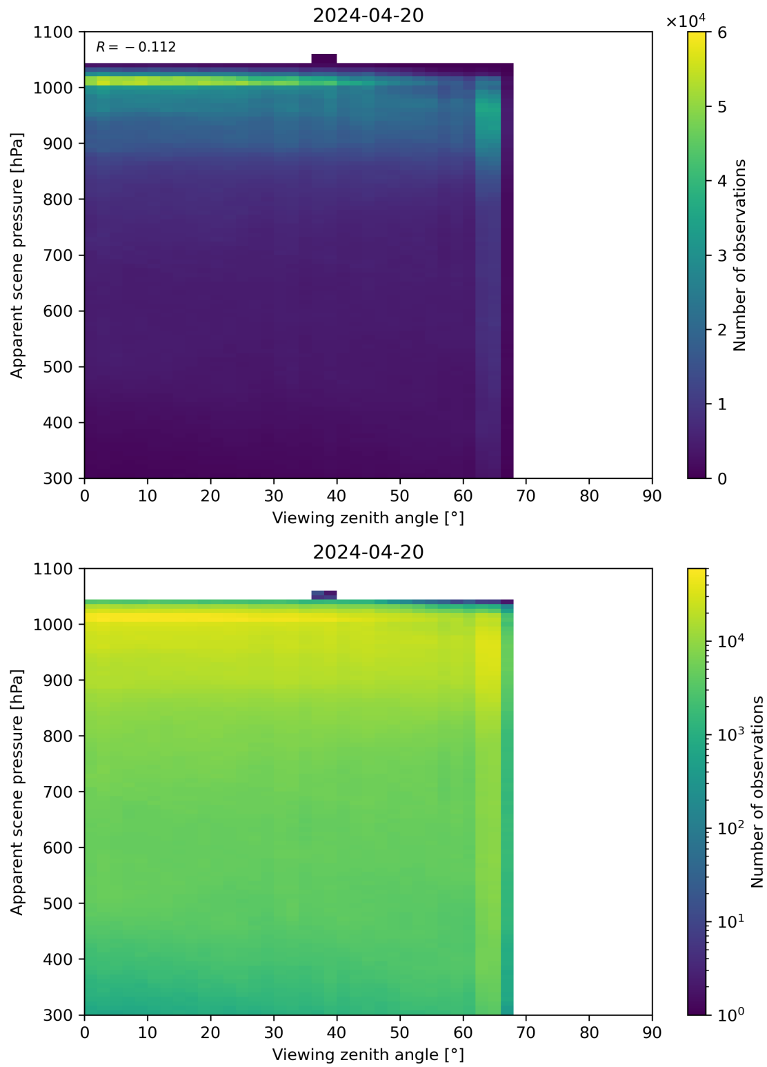
Figure 118: Scatter density plot of “Viewing zenith angle” against “Apparent scene pressure” for 2024-04-19 to 2024-04-21.
