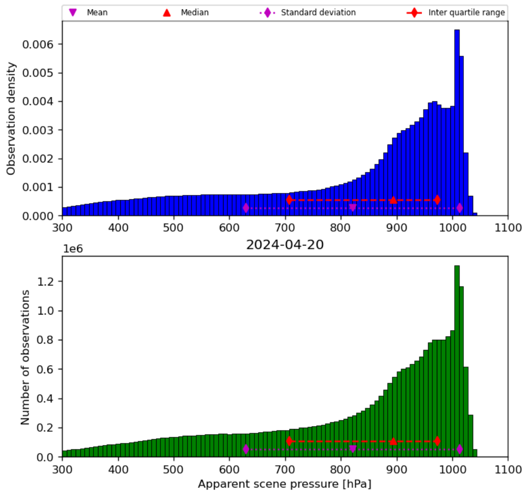
Figure 36: Histogram of “Apparent scene pressure” for 2024-04-19 to 2024-04-21
