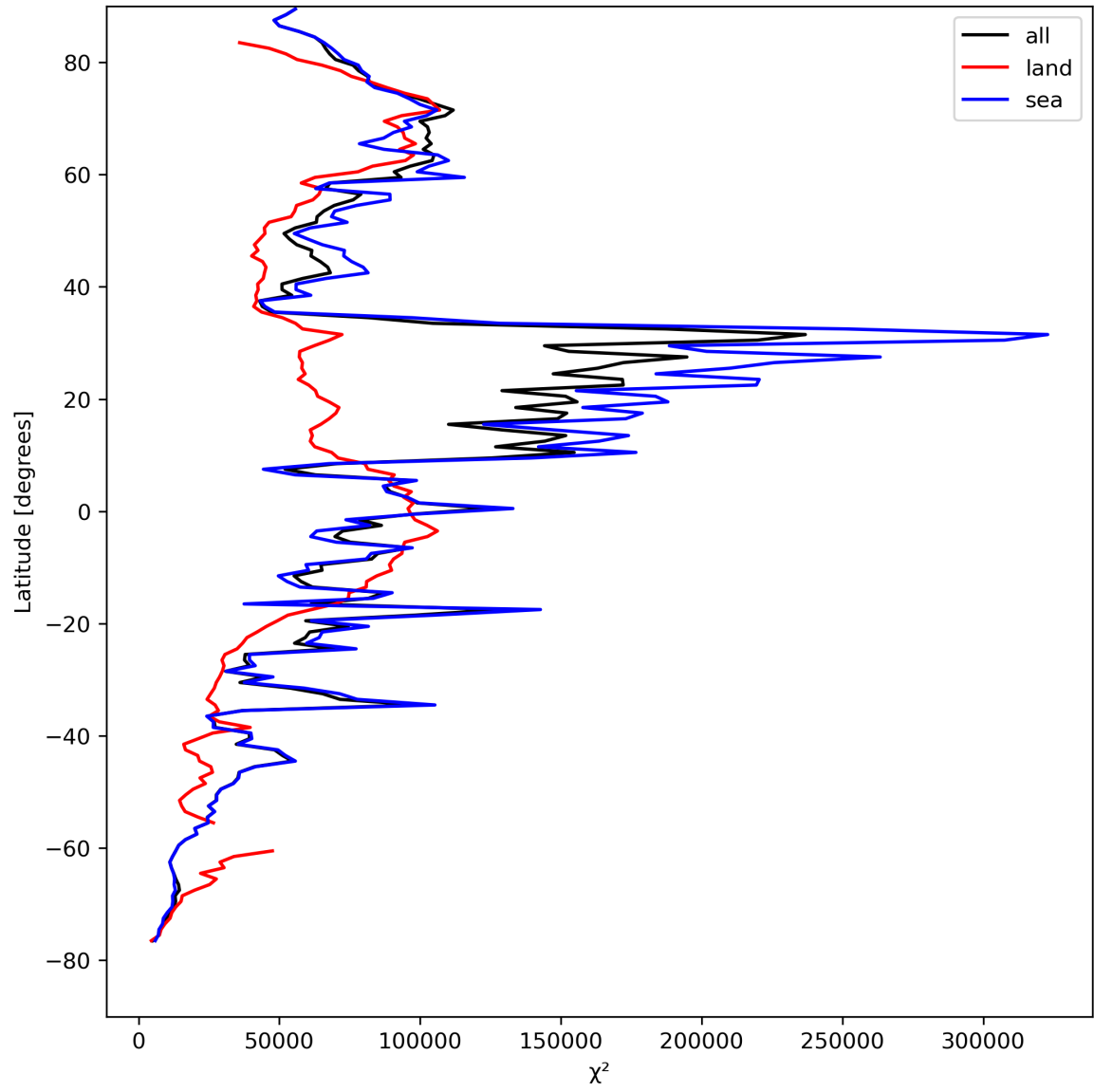
Figure 21: Zonal average of “ \chi^2 ” for 2024-04-19 to 2024-04-21.
