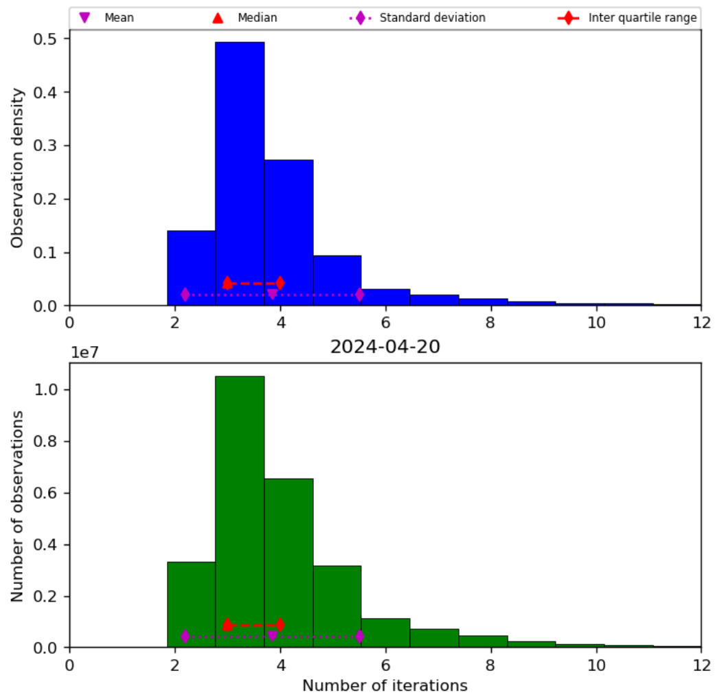
Figure 39: Histogram of “Number of iterations” for 2024-04-19 to 2024-04-21
