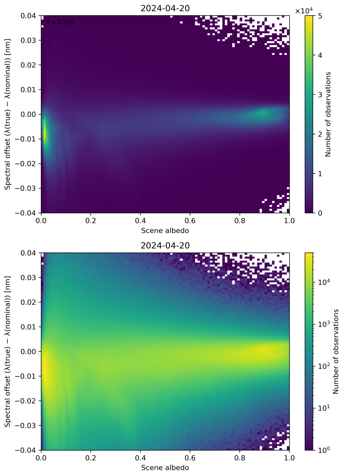
Figure 107: Scatter density plot of “Scene albedo” against “Spectral offset ( \lambda(\text{true}) - \lambda(\text{nominal}) )” for 2024-04-19 to 2024-04-21.
