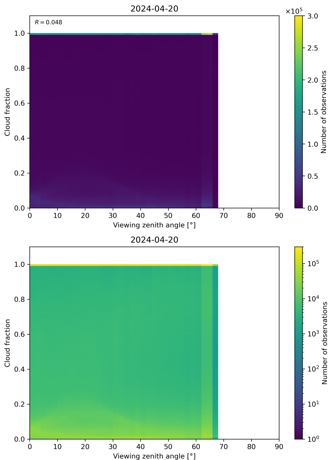
Figure 120: Scatter density plot of “Viewing zenith angle” against “Cloud fraction” for 2024-04-19 to 2024-04-21.
