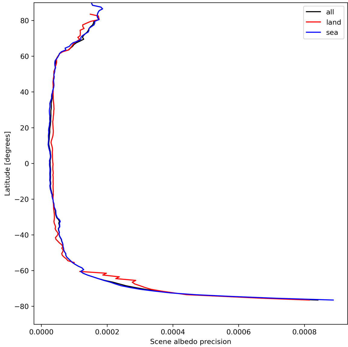
Figure 18: Zonal average of “Scene albedo precision” for 2024-04-19 to 2024-04-21.
