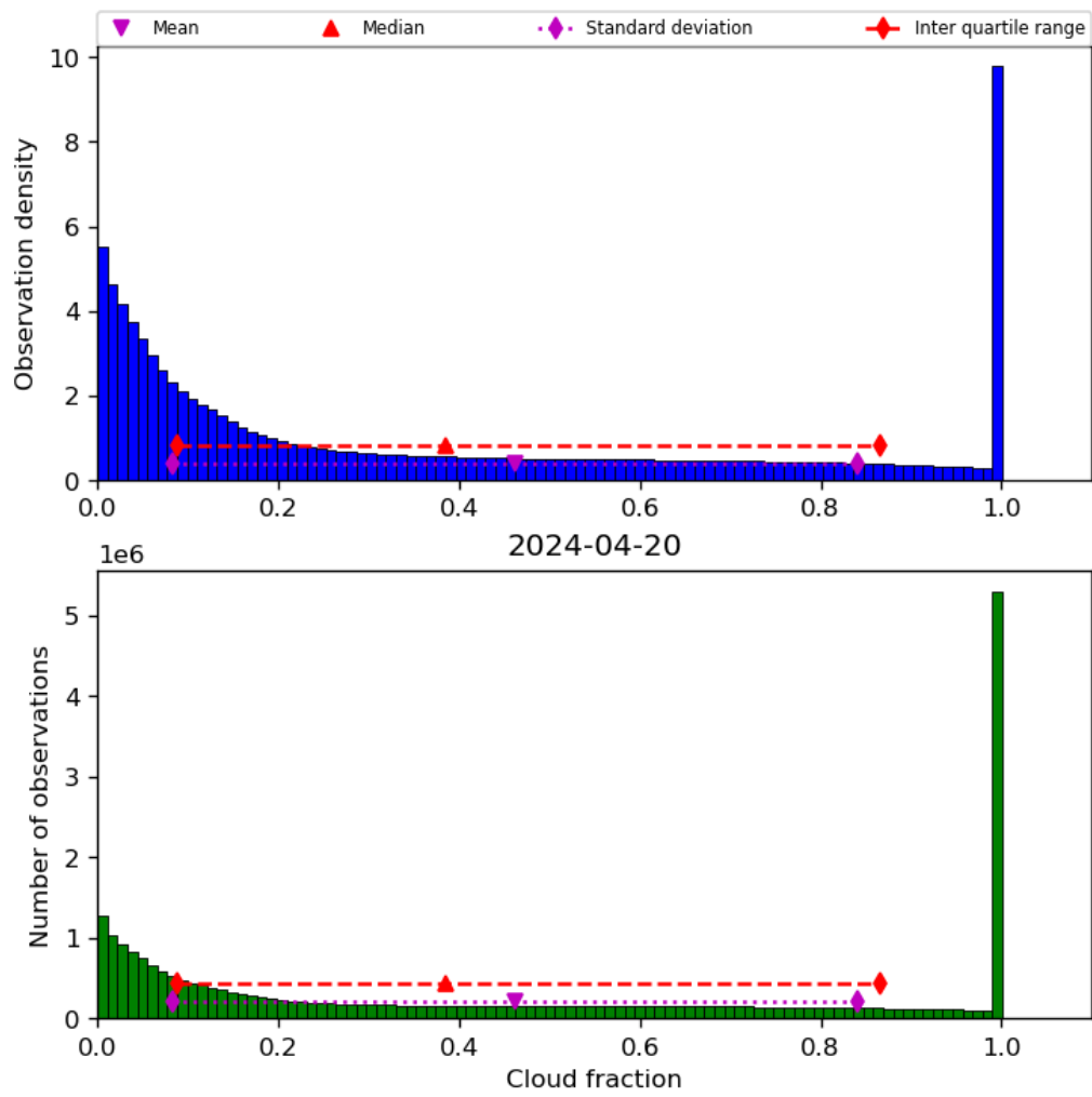
Figure 32: Histogram of “Cloud fraction” for 2024-04-19 to 2024-04-21
