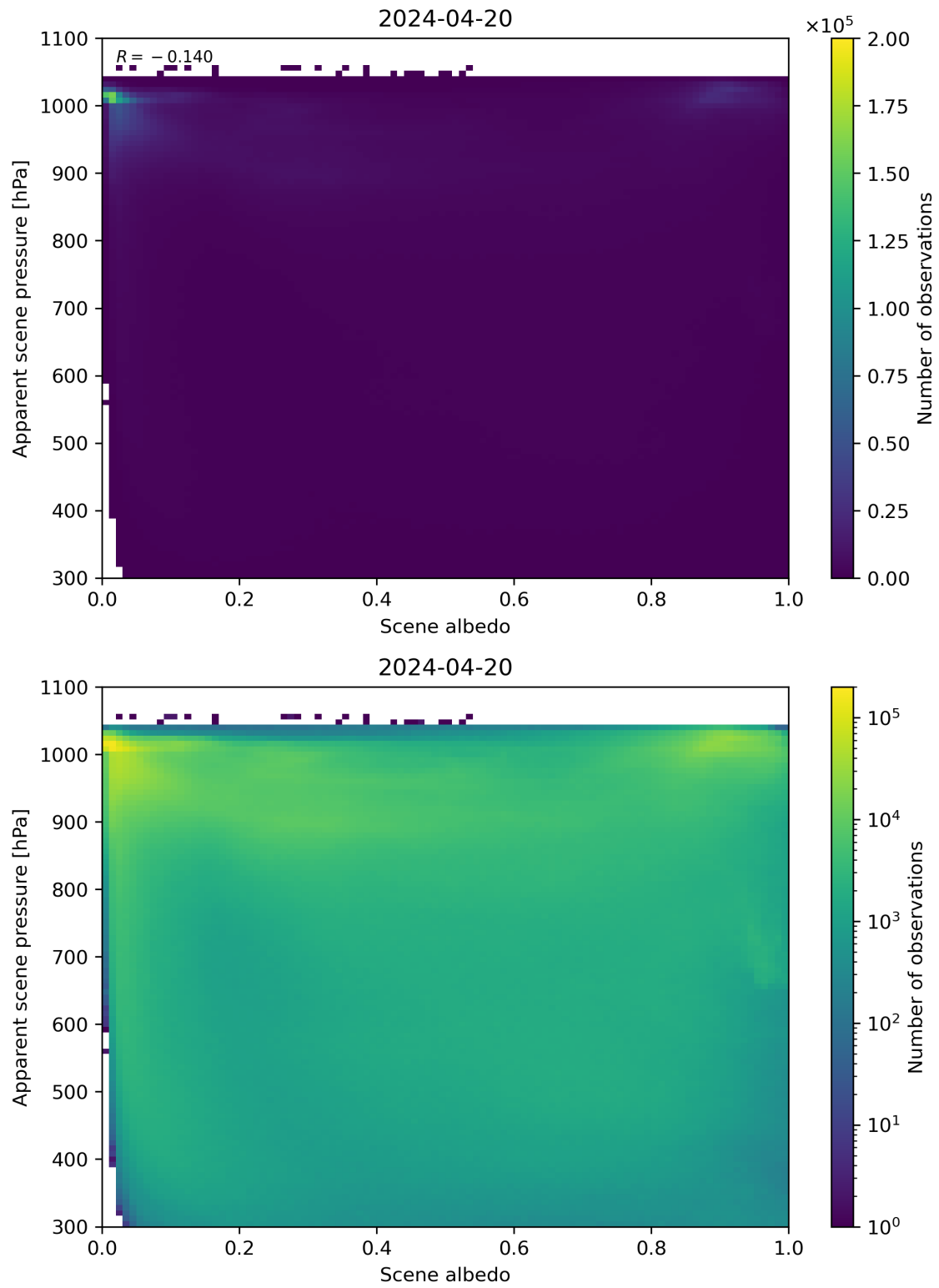
Figure 102: Scatter density plot of “Scene albedo” against “Apparent scene pressure” for 2024-04-19 to 2024-04-21.
