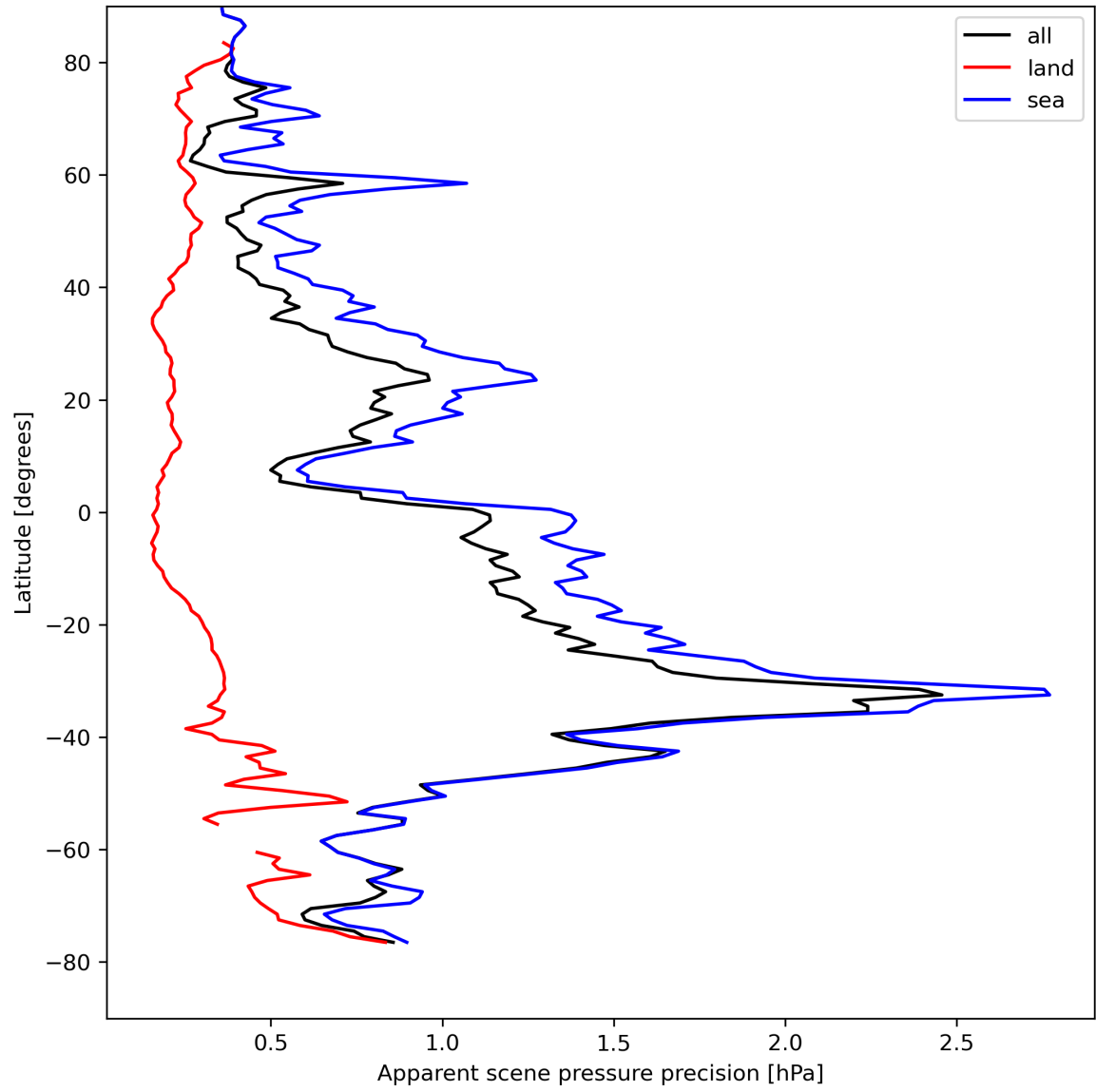
Figure 20: Zonal average of “Apparent scene pressure precision” for 2024-04-19 to 2024-04-21.
