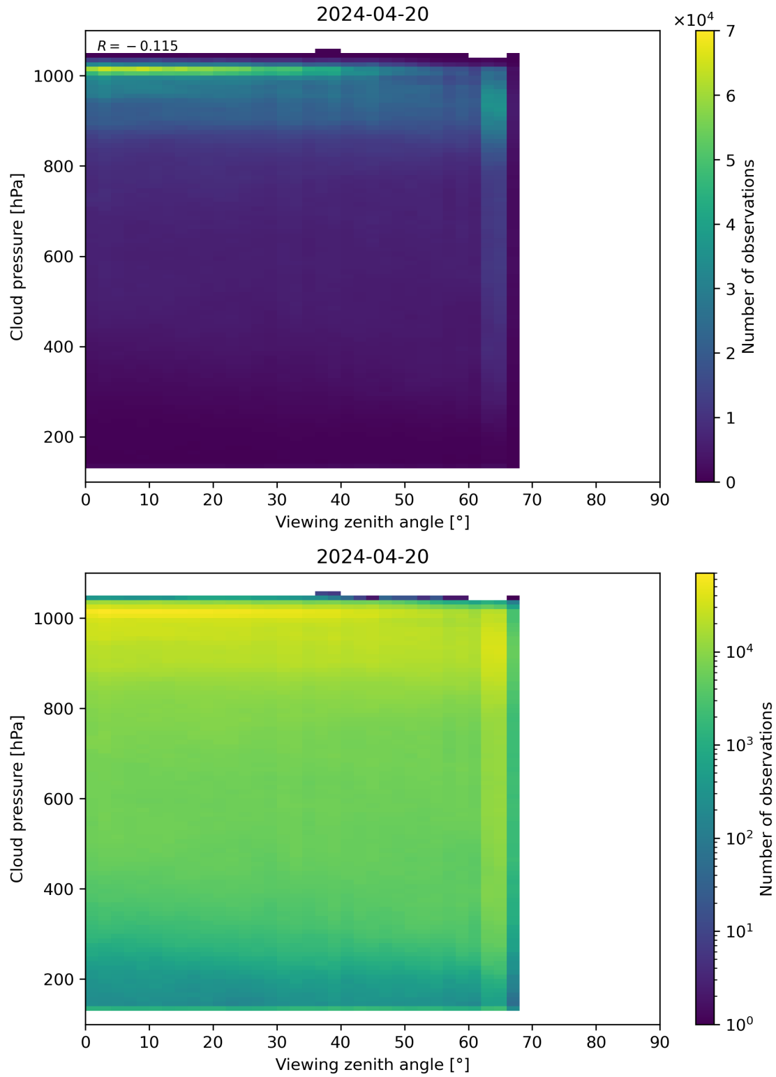
Figure 121: Scatter density plot of “Viewing zenith angle” against “Cloud pressure” for 2024-04-19 to 2024-04-21.
