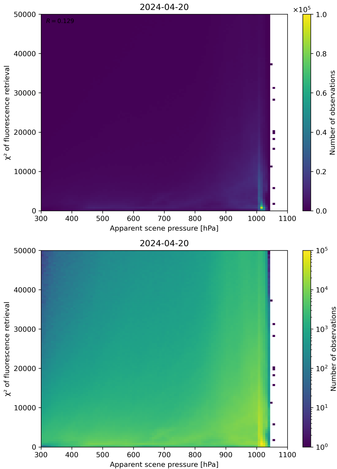
Figure 63: Scatter density plot of “Apparent scene pressure” against “ \chi^2 of fluorescence retrieval” for 2024-04-19 to 2024-04-21.
