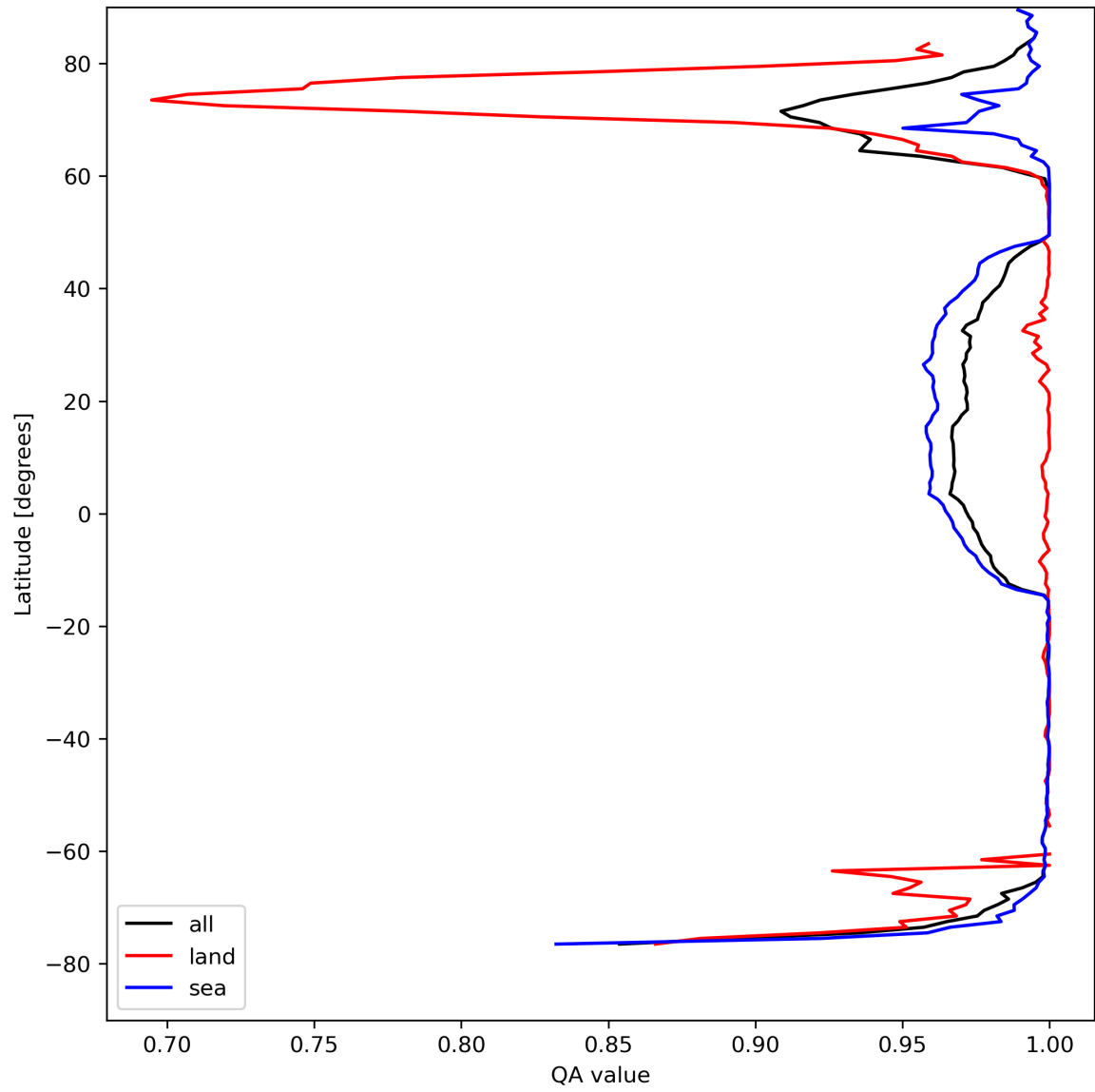
Figure 12: Zonal average of “QA value” for 2024-04-19 to 2024-04-21.
