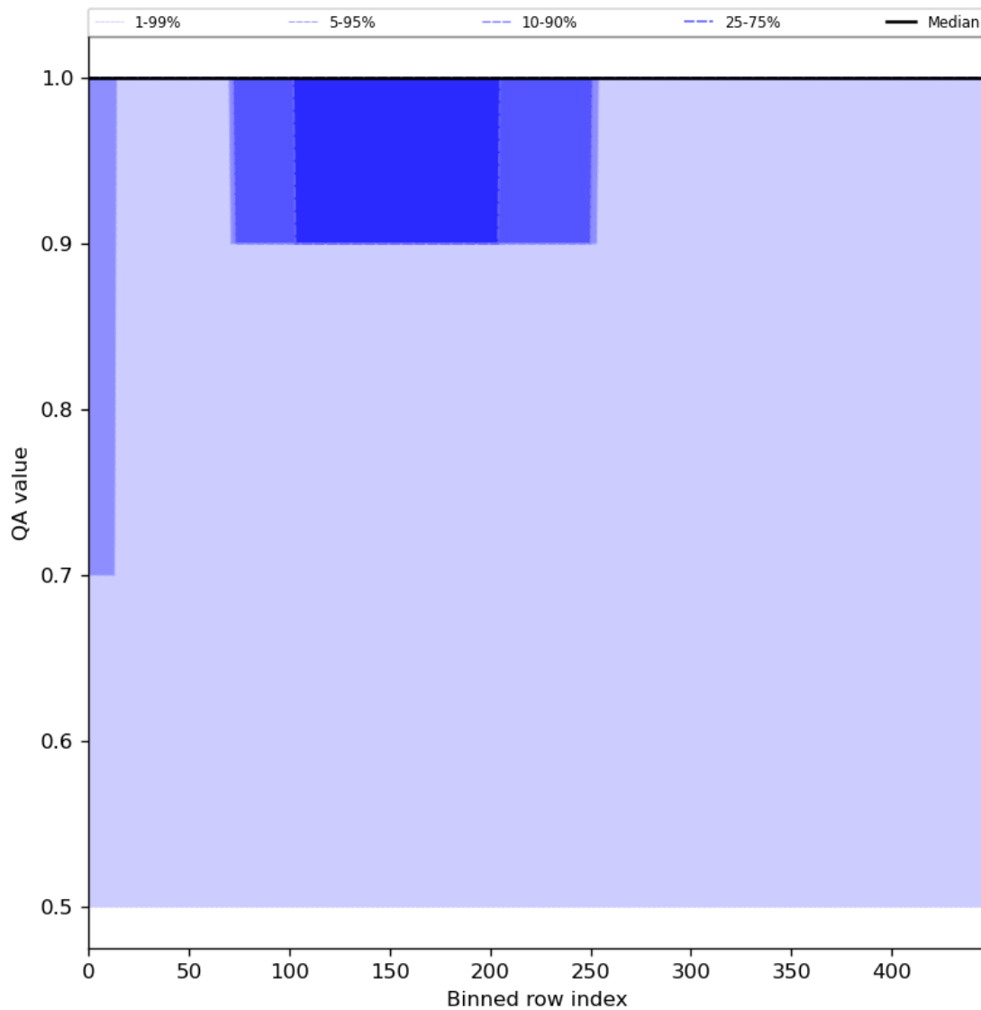
Figure 46: Along track statistics of “QA value” for 2024-04-19 to 2024-04-21
