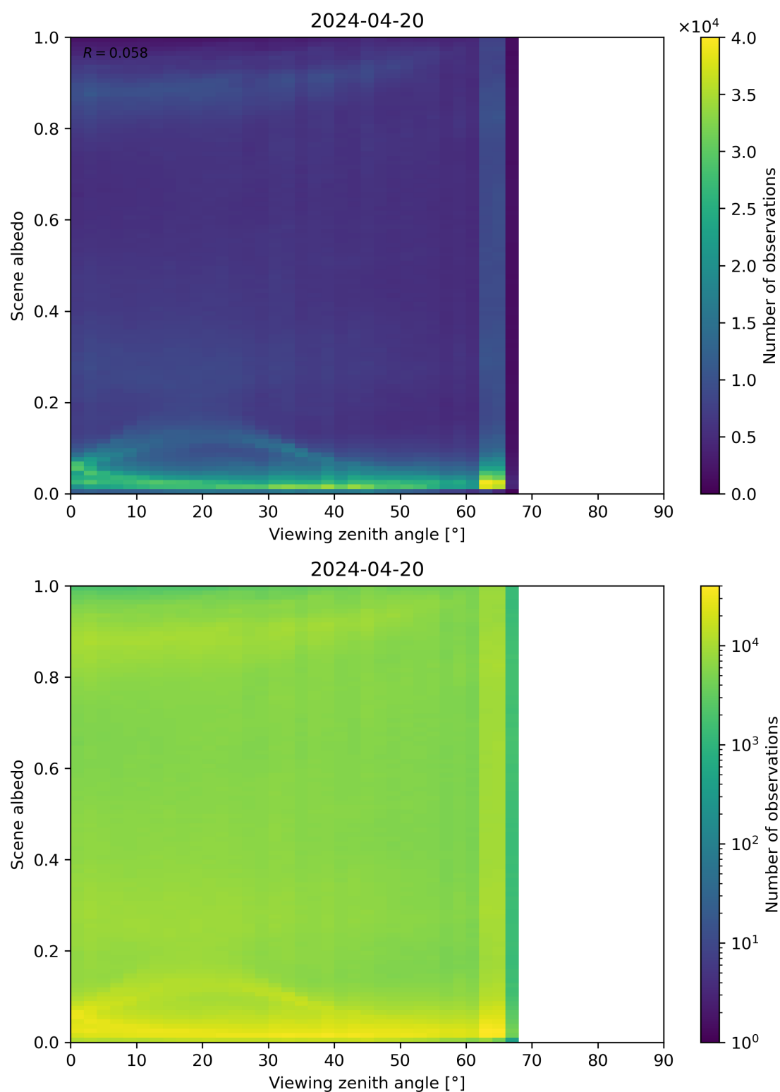
Figure 126: Scatter density plot of “Viewing zenith angle” against “Scene albedo” for 2024-04-19 to 2024-04-21.
