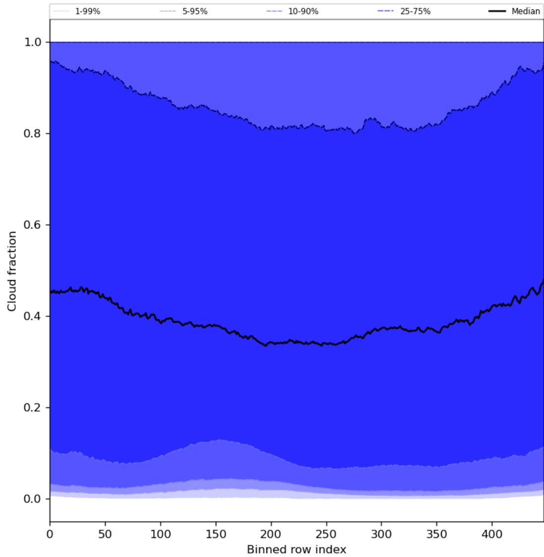
Figure 49: Along track statistics of “Cloud fraction” for 2024-04-19 to 2024-04-21
