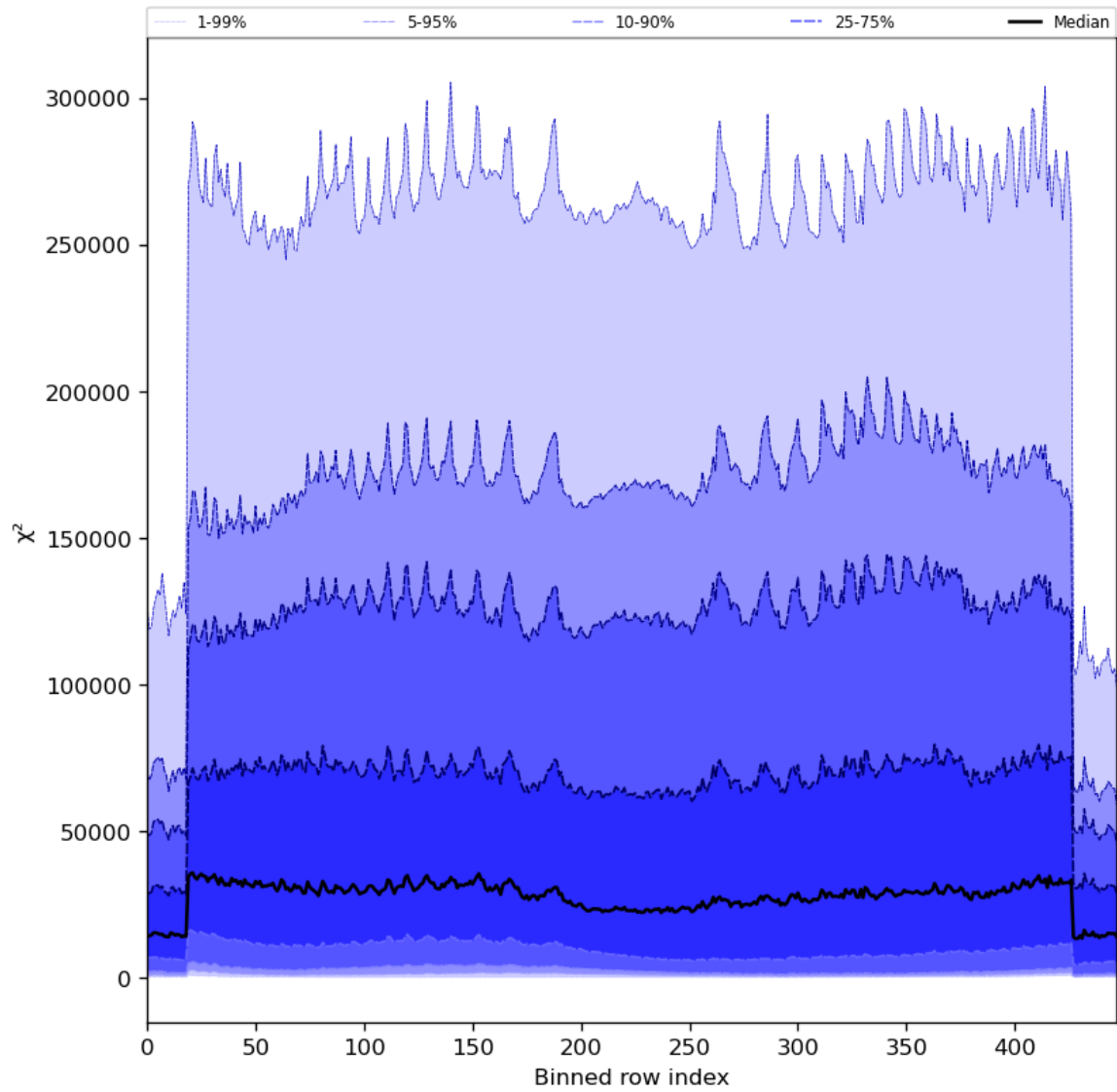
Figure 55: Along track statistics of “ \chi^2 ” for 2024-04-19 to 2024-04-21
