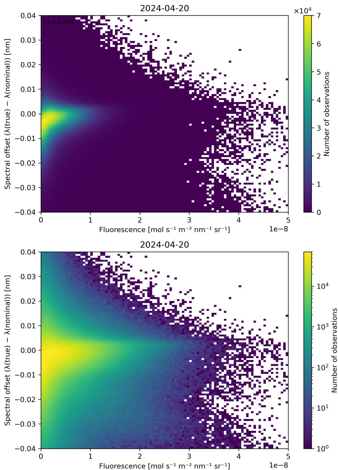
Figure 87: Scatter density plot of “Fluorescence” against “Spectral offset ( \lambda(\text{true}) - \lambda(\text{nominal}) )” for 2024-04-19 to 2024-04-21.
