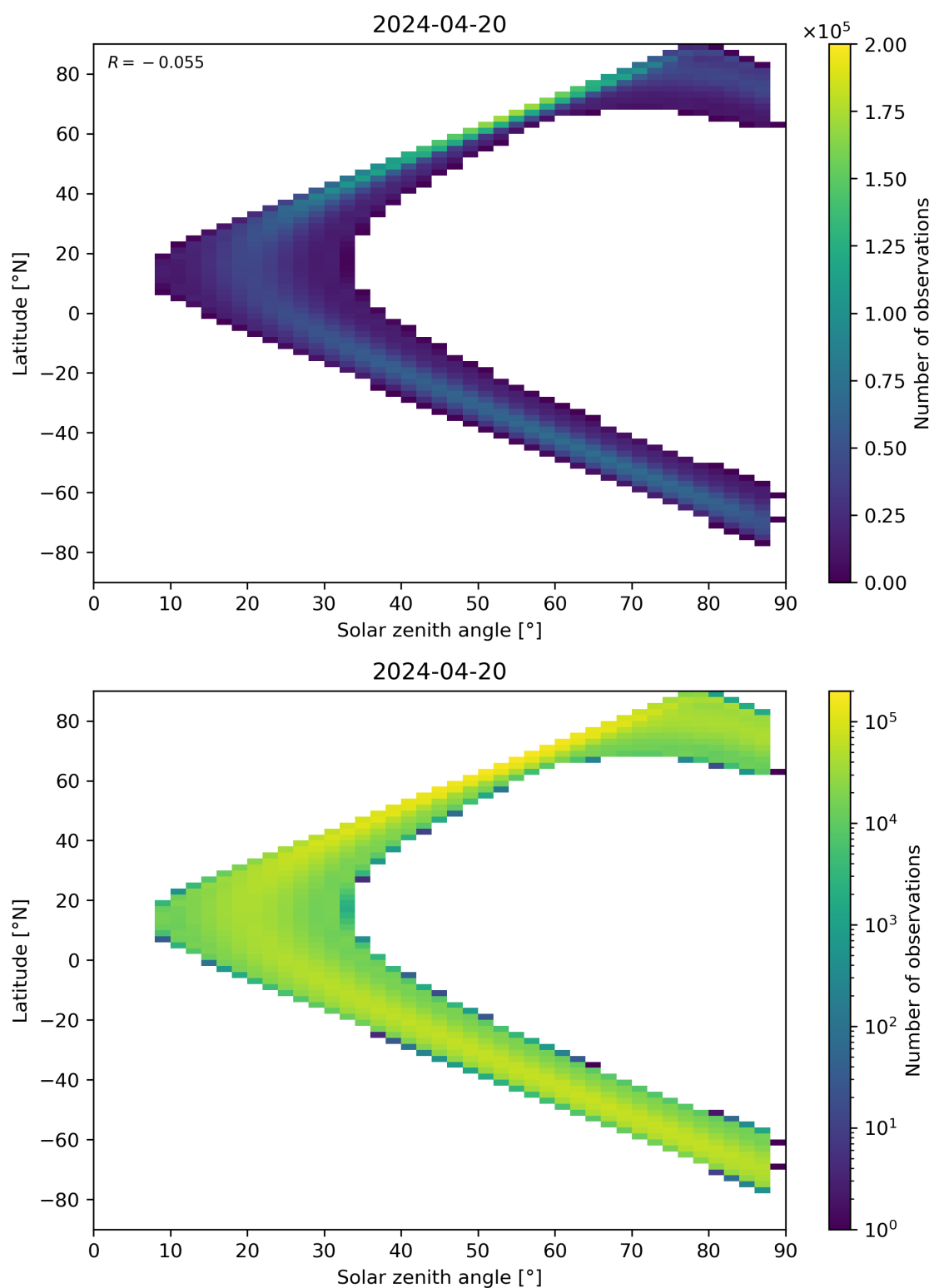
Figure 113: Scatter density plot of “Solar zenith angle” against “Latitude” for 2024-04-19 to 2024-04-21.
