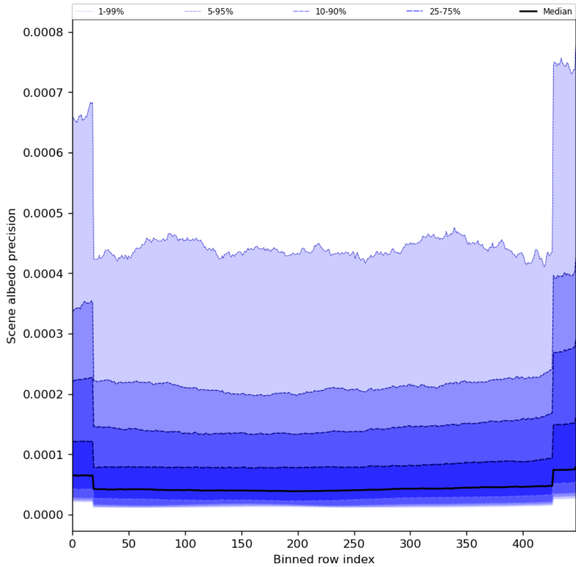
Figure 52: Along track statistics of “Scene albedo precision” for 2024-04-19 to 2024-04-21
