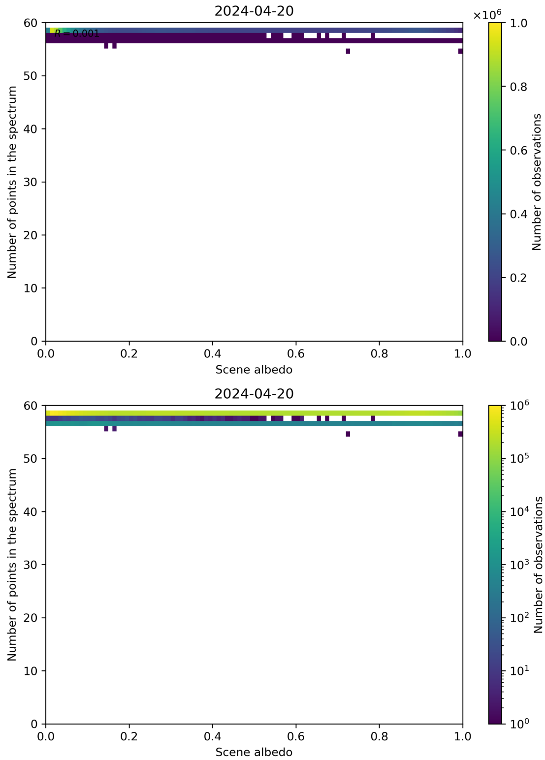
Figure 106: Scatter density plot of “Scene albedo” against “Number of points in the spectrum” for 2024-04-19 to 2024-04-21.
