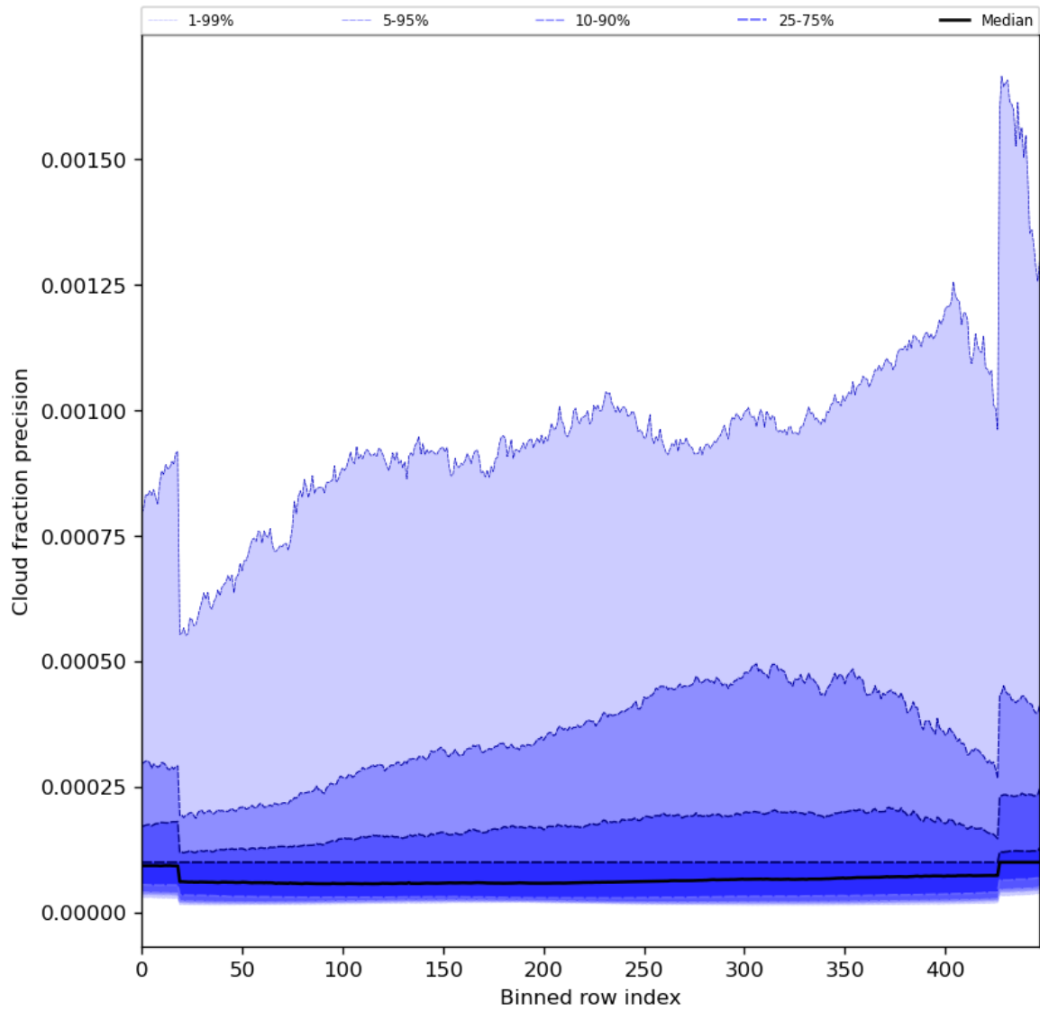
Figure 50: Along track statistics of “Cloud fraction precision” for 2024-04-19 to 2024-04-21
