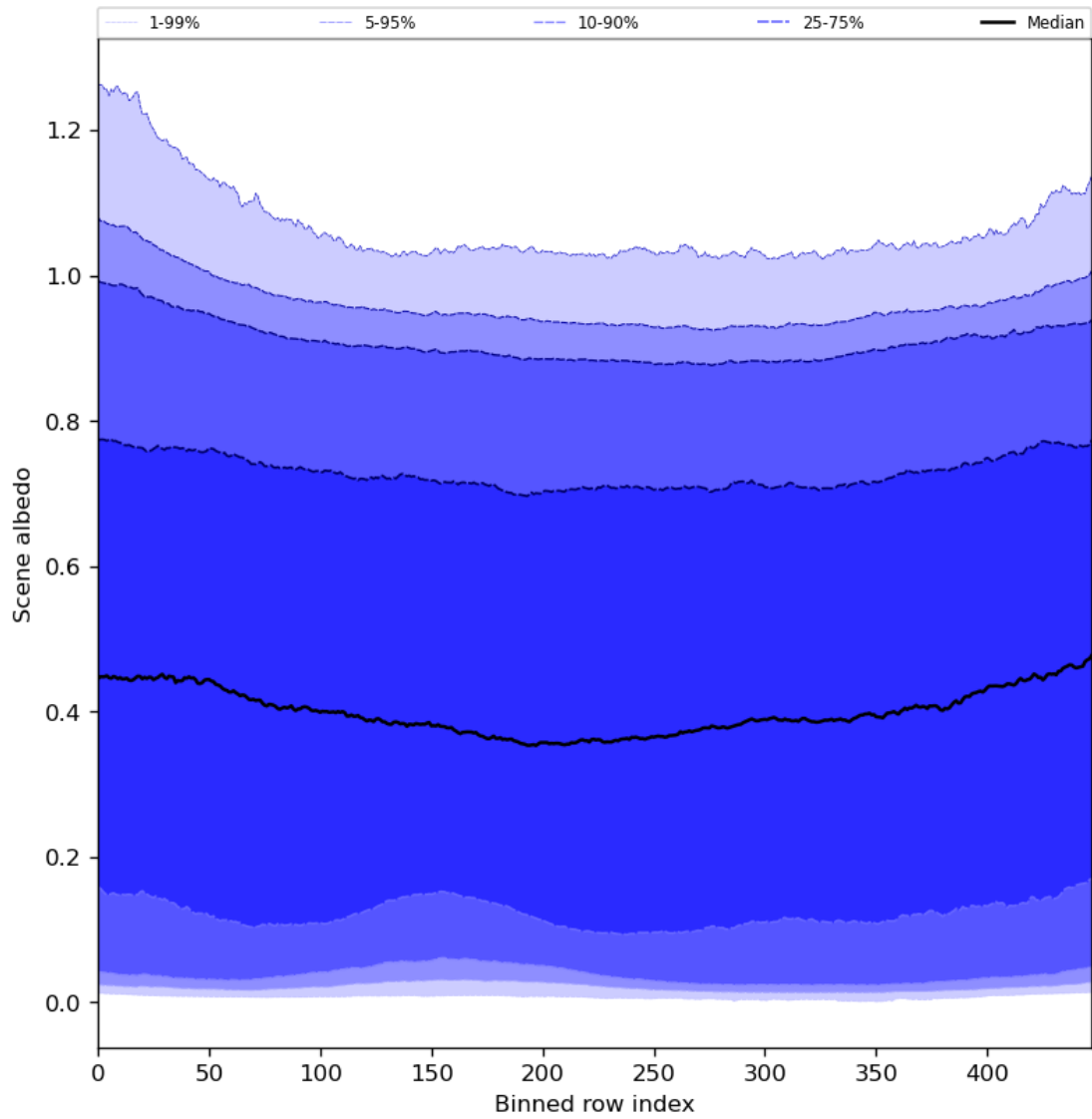
Figure 51: Along track statistics of "Scene albedo" for 2024-04-19 to 2024-04-21
