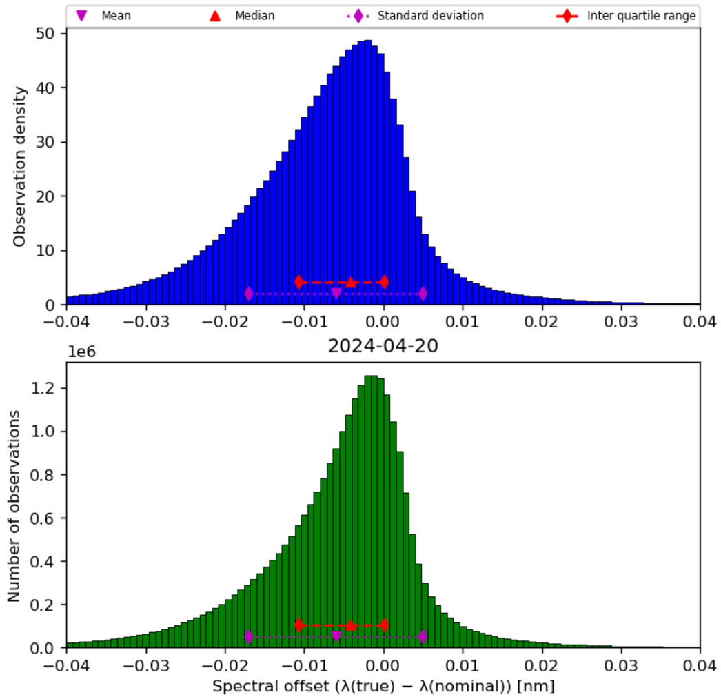
Figure 45: Histogram of “Spectral offset ( \lambda(\text{true}) - \lambda(\text{nominal}) )” for 2024-04-19 to 2024-04-21
