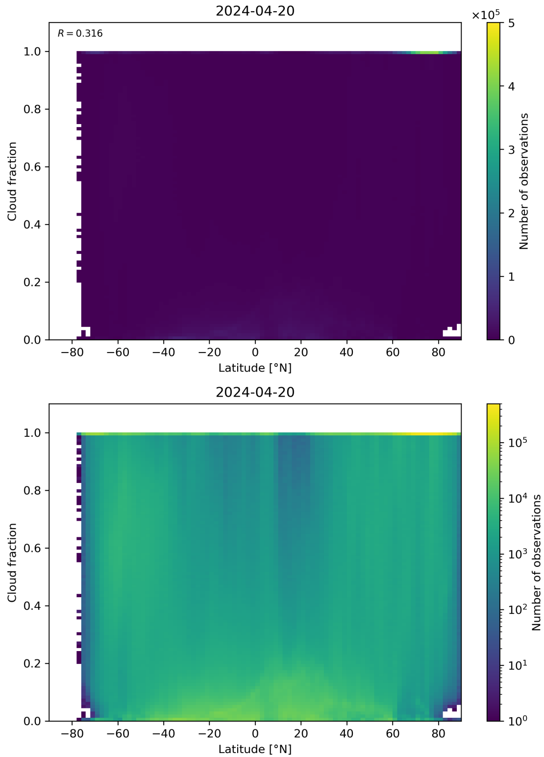
Figure 90: Scatter density plot of “Latitude” against “Cloud fraction” for 2024-04-19 to 2024-04-21.
