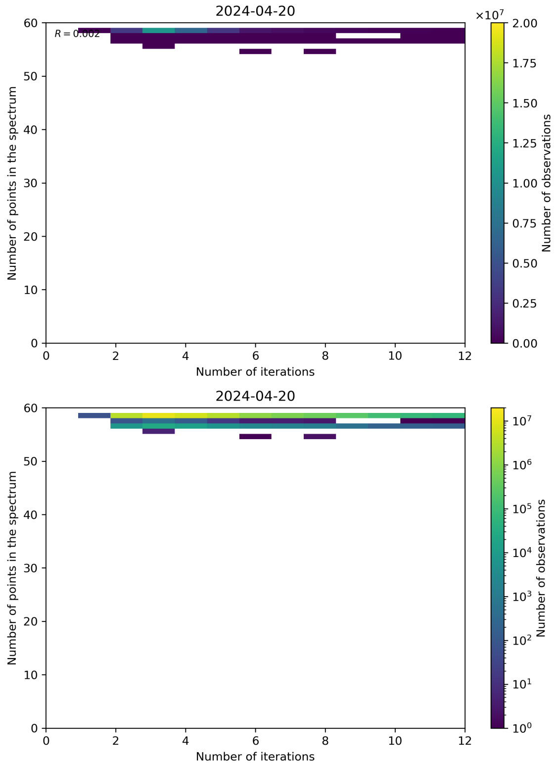
Figure 99: Scatter density plot of “Number of iterations” against “Number of points in the spectrum” for 2024-04-19 to 2024-04-21.
