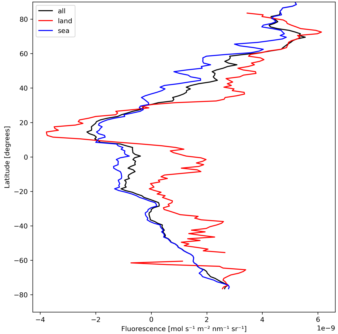
Figure 23: Zonal average of “Fluorescence” for 2024-04-19 to 2024-04-21.
