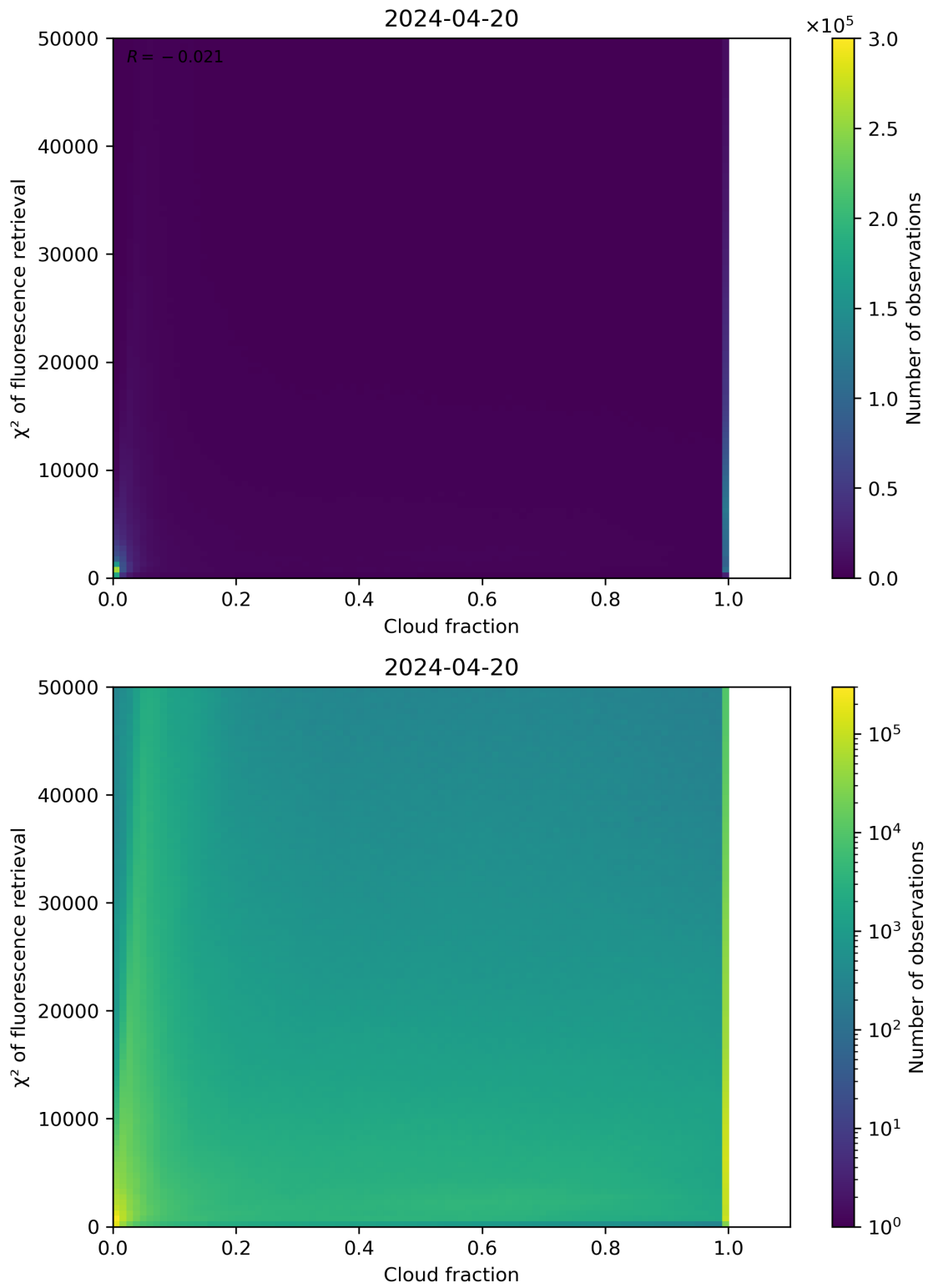
Figure 71: Scatter density plot of “Cloud fraction” against “ \chi^2 of fluorescence retrieval” for 2024-04-19 to 2024-04-21.
