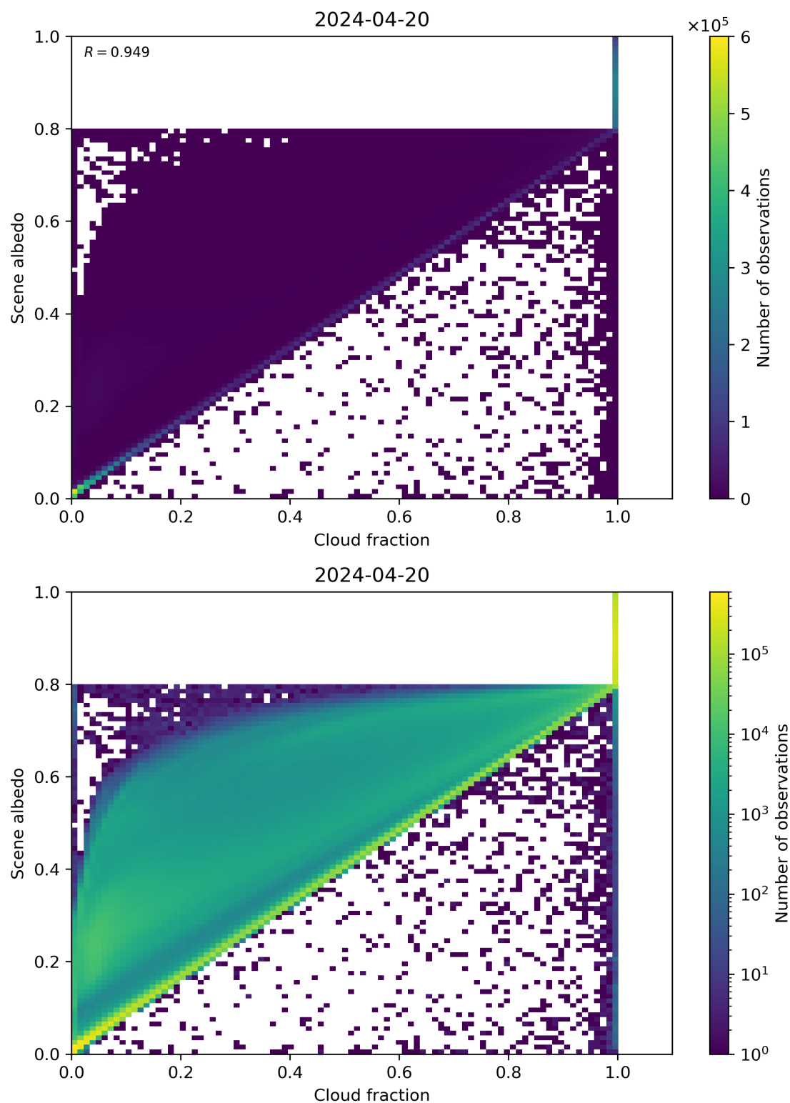
Figure 75: Scatter density plot of “Cloud fraction” against “Scene albedo” for 2024-04-19 to 2024-04-21.
