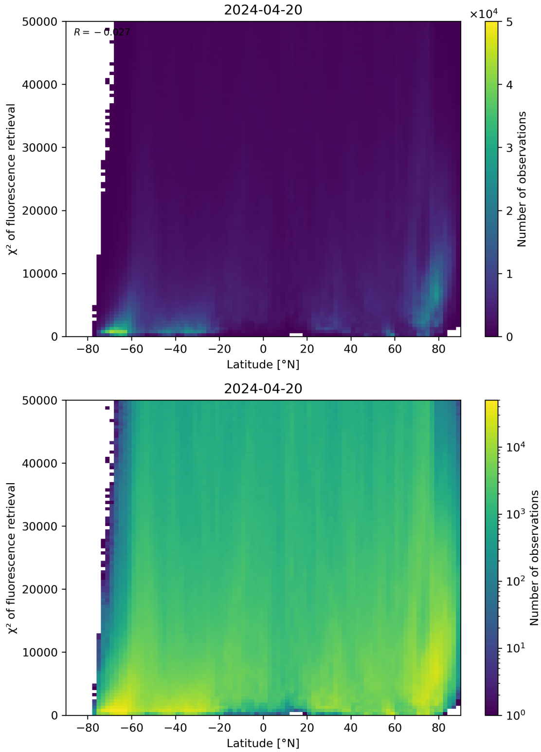
Figure 89: Scatter density plot of “Latitude” against “ \chi^2 of fluorescence retrieval” for 2024-04-19 to 2024-04-21.
