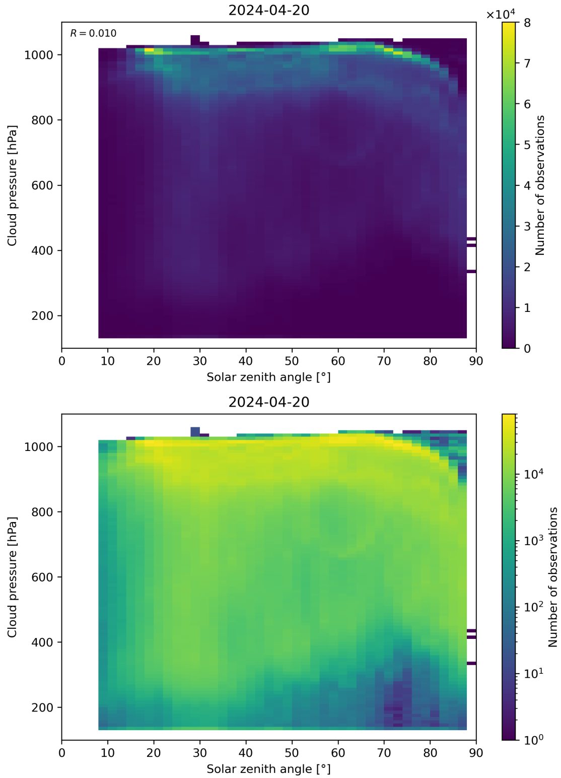
Figure 111: Scatter density plot of “Solar zenith angle” against “Cloud pressure” for 2024-04-19 to 2024-04-21.
