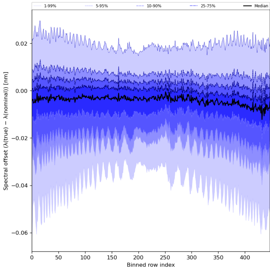
Figure 62: Along track statistics of “Spectral offset ( \lambda(\text{true}) - \lambda(\text{nominal}) )” for 2024-04-19 to 2024-04-21
