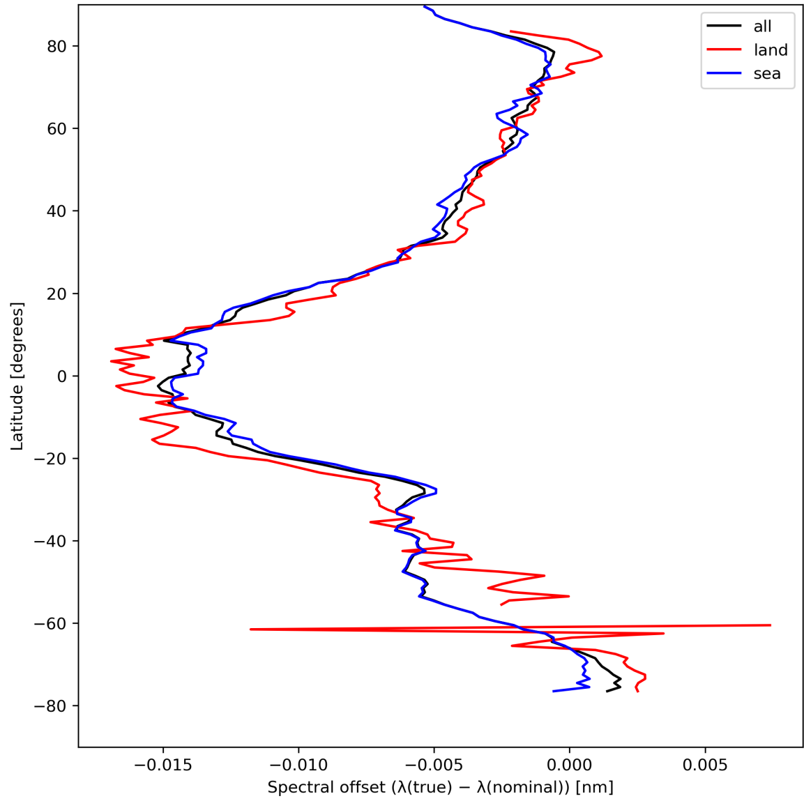
Figure 28: Zonal average of “Spectral offset ( \lambda(\text{true}) - \lambda(\text{nominal}) )” for 2024-04-19 to 2024-04-21.
