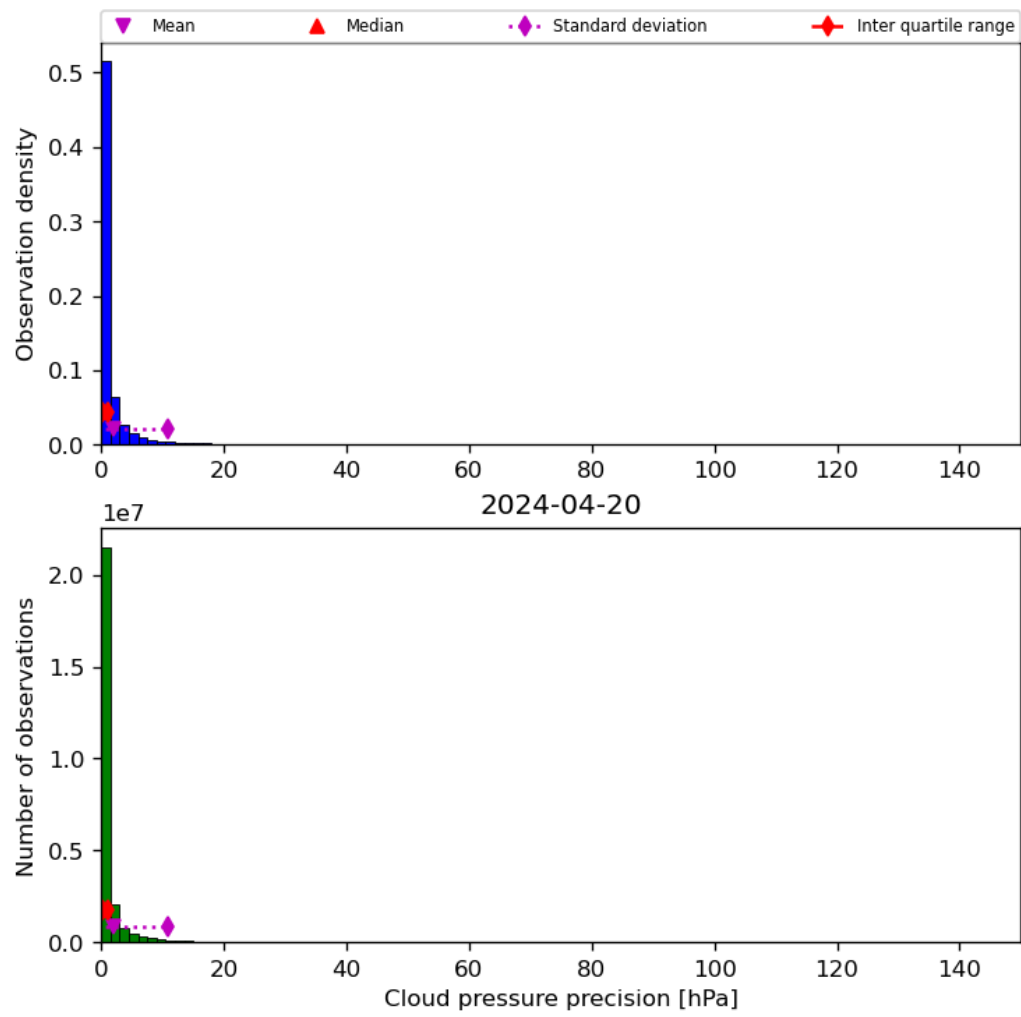
Figure 31: Histogram of “Cloud pressure precision” for 2024-04-19 to 2024-04-21
