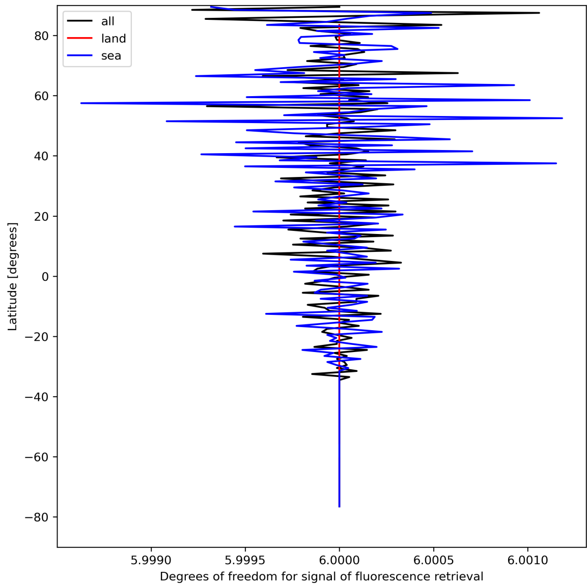
Figure 26: Zonal average of “Degrees of freedom for signal of fluorescence retrieval” for 2024-04-19 to 2024-04-21.
