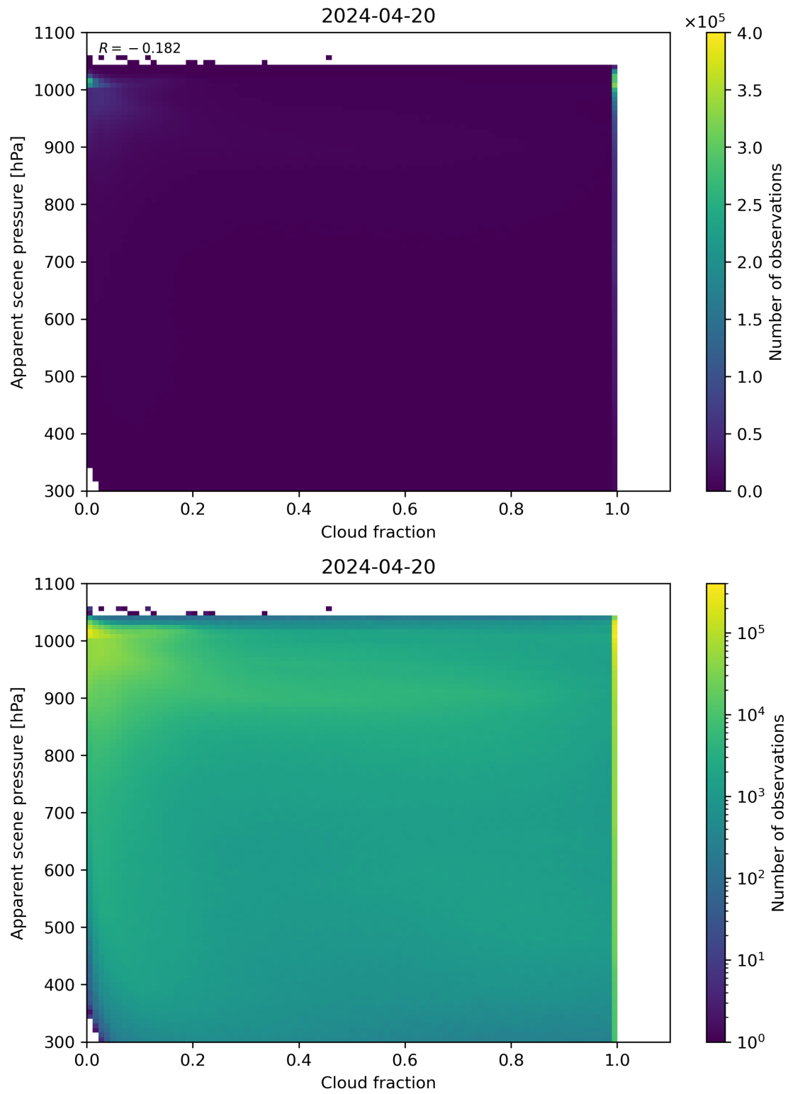
Figure 70: Scatter density plot of “Cloud fraction” against “Apparent scene pressure” for 2024-04-19 to 2024-04-21.
