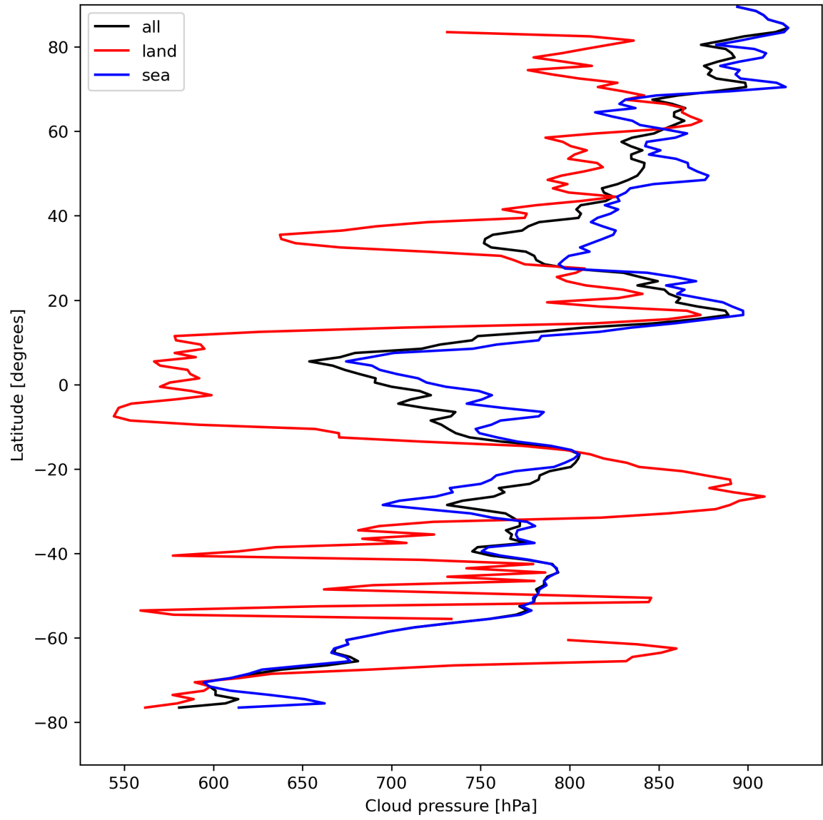
Figure 13: Zonal average of “Cloud pressure” for 2024-04-19 to 2024-04-21.
