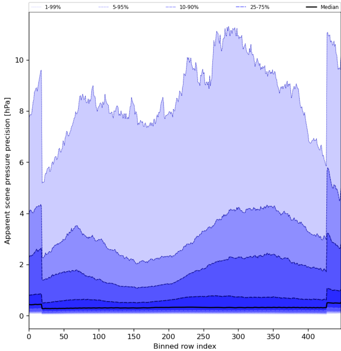
Figure 54: Along track statistics of “Apparent scene pressure precision” for 2024-04-19 to 2024-04-21
