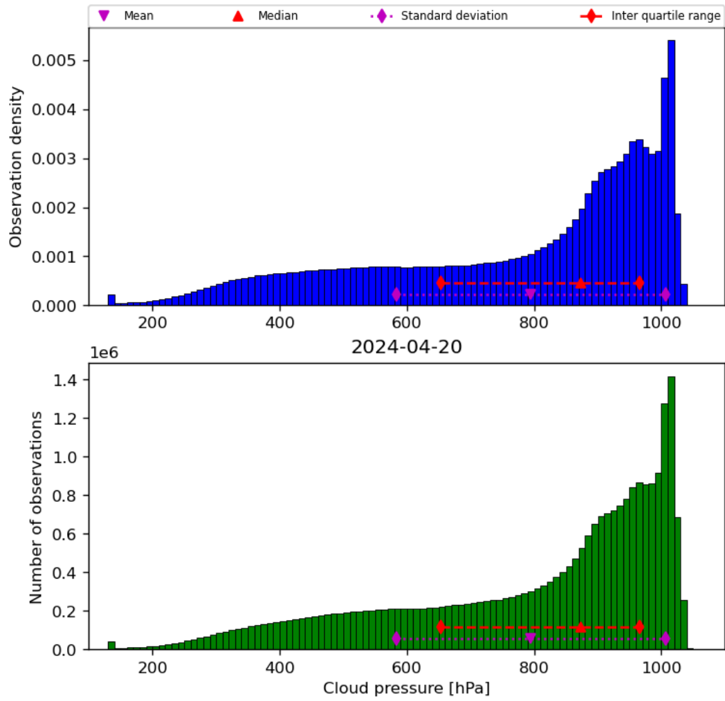
Figure 30: Histogram of “Cloud pressure” for 2024-04-19 to 2024-04-21
