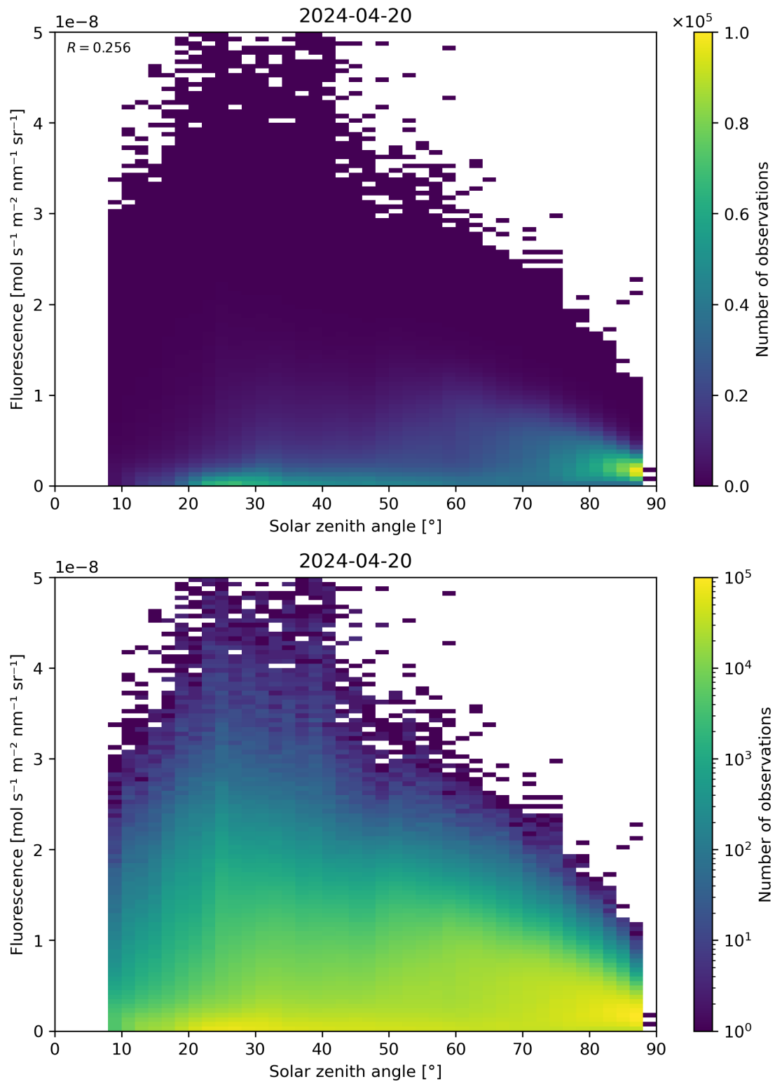
Figure 112: Scatter density plot of “Solar zenith angle” against “Fluorescence” for 2024-04-19 to 2024-04-21.
