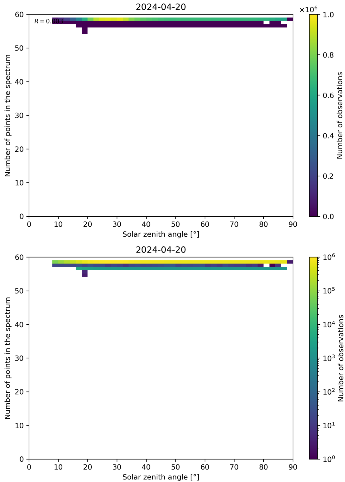
Figure 115: Scatter density plot of “Solar zenith angle” against “Number of points in the spectrum” for 2024-04-19 to 2024-04-21.
