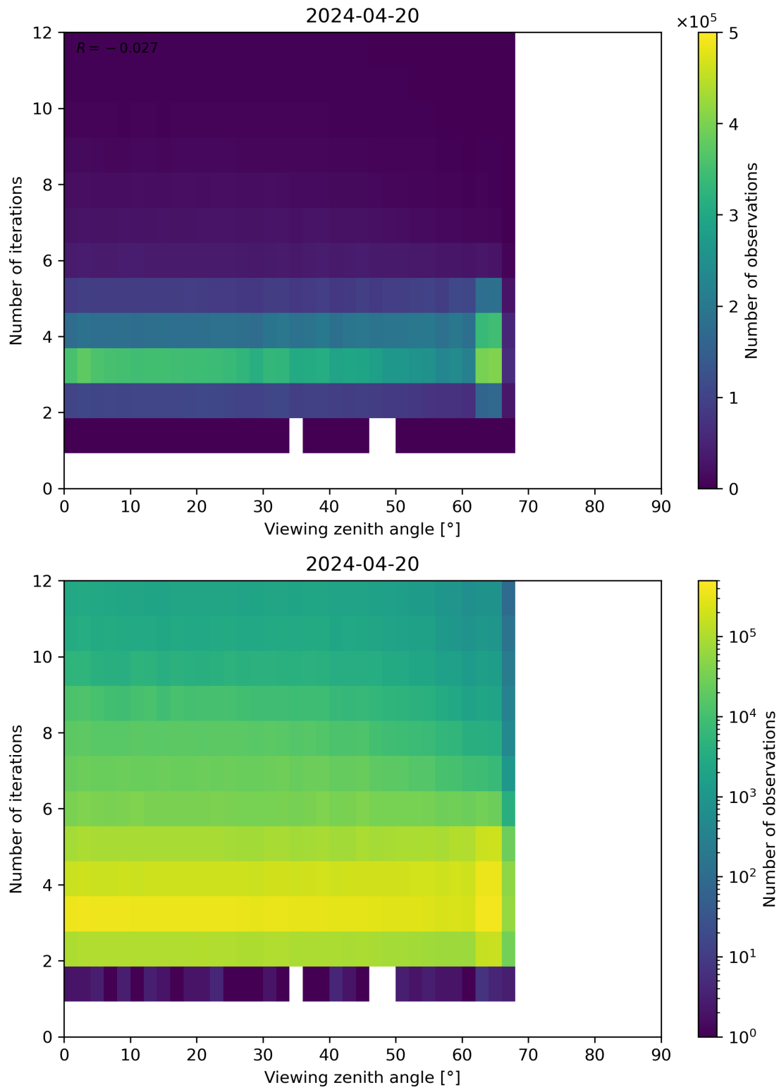
Figure 124: Scatter density plot of “Viewing zenith angle” against “Number of iterations” for 2024-04-19 to 2024-04-21.
