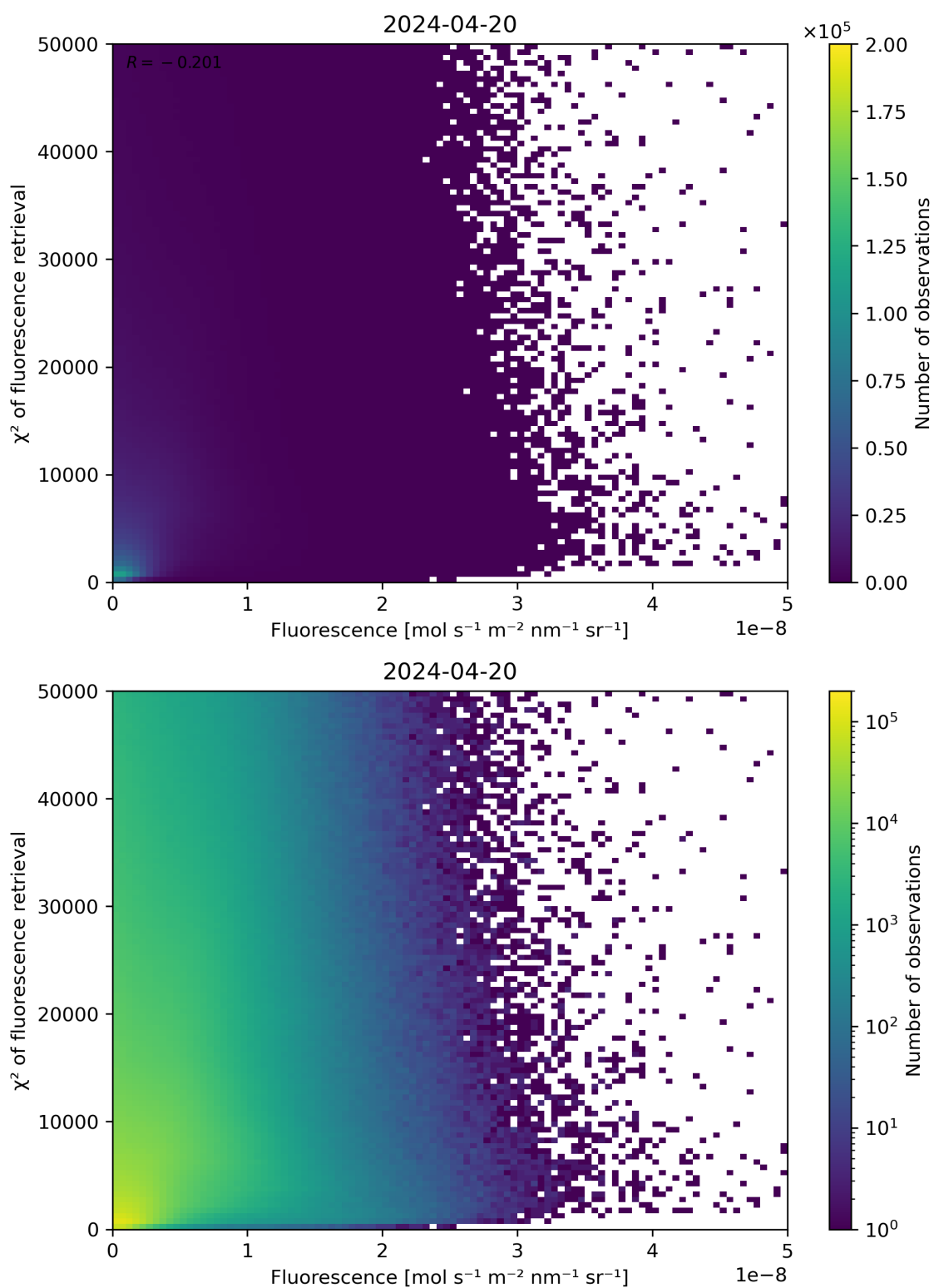
Figure 85: Scatter density plot of “Fluorescence” against “ \chi^2 of fluorescence retrieval” for 2024-04-19 to 2024-04-21.
