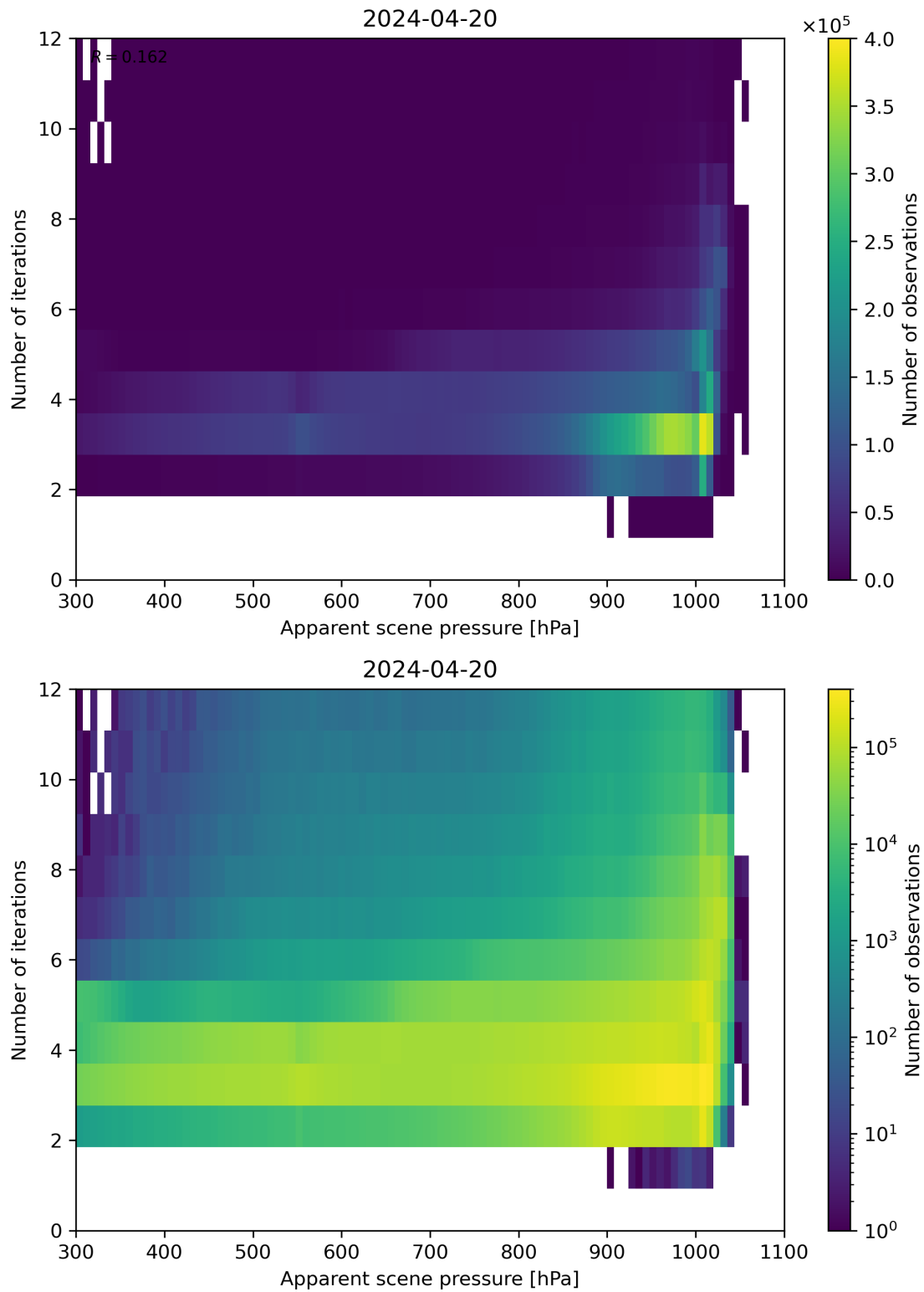
Figure 65: Scatter density plot of “Apparent scene pressure” against “Number of iterations” for 2024-04-19 to 2024-04-21.
