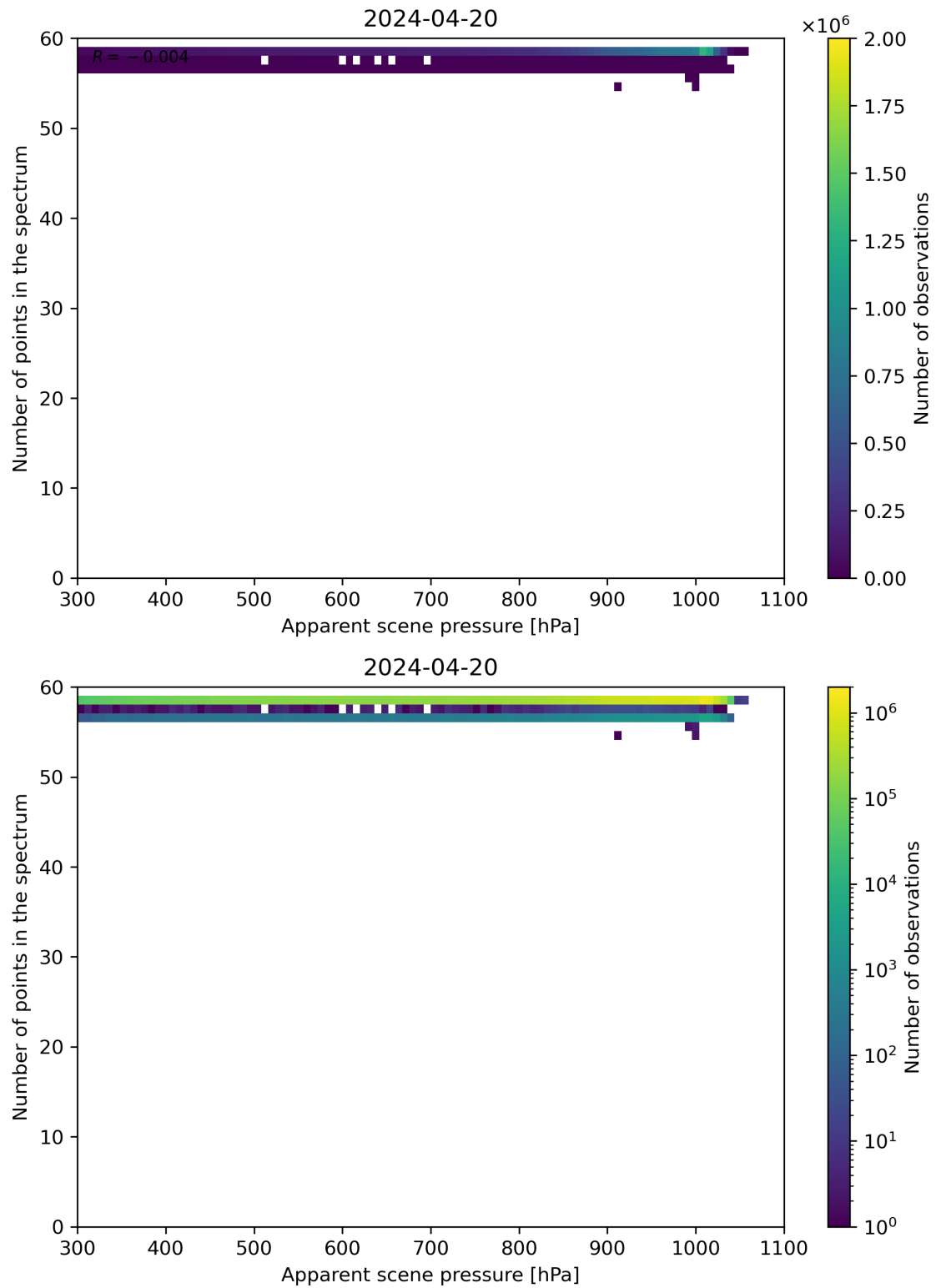
Figure 66: Scatter density plot of “Apparent scene pressure” against “Number of points in the spectrum” for 2024-04-19 to 2024-04-21.
