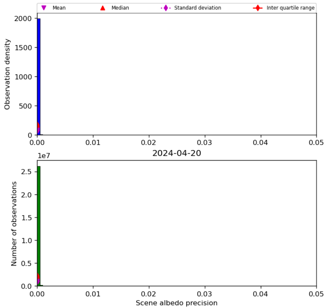
Figure 35: Histogram of “Scene albedo precision” for 2024-04-19 to 2024-04-21
