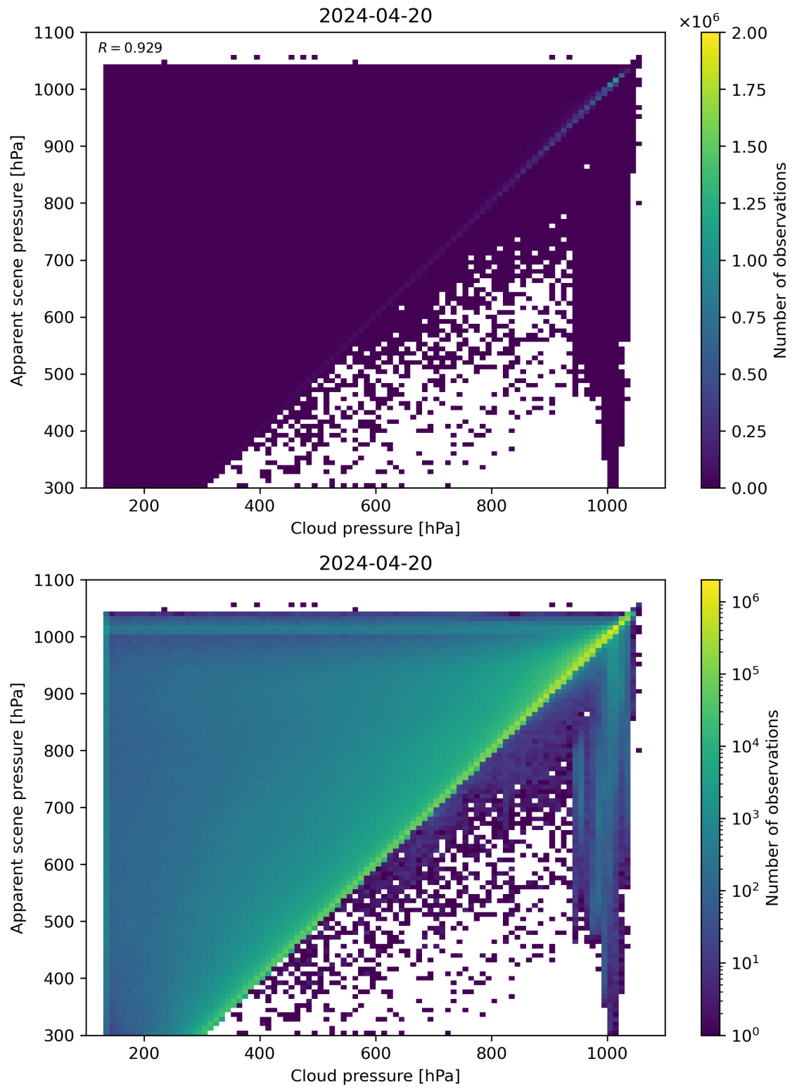
Figure 77: Scatter density plot of “Cloud pressure” against “Apparent scene pressure” for 2024-04-19 to 2024-04-21.
