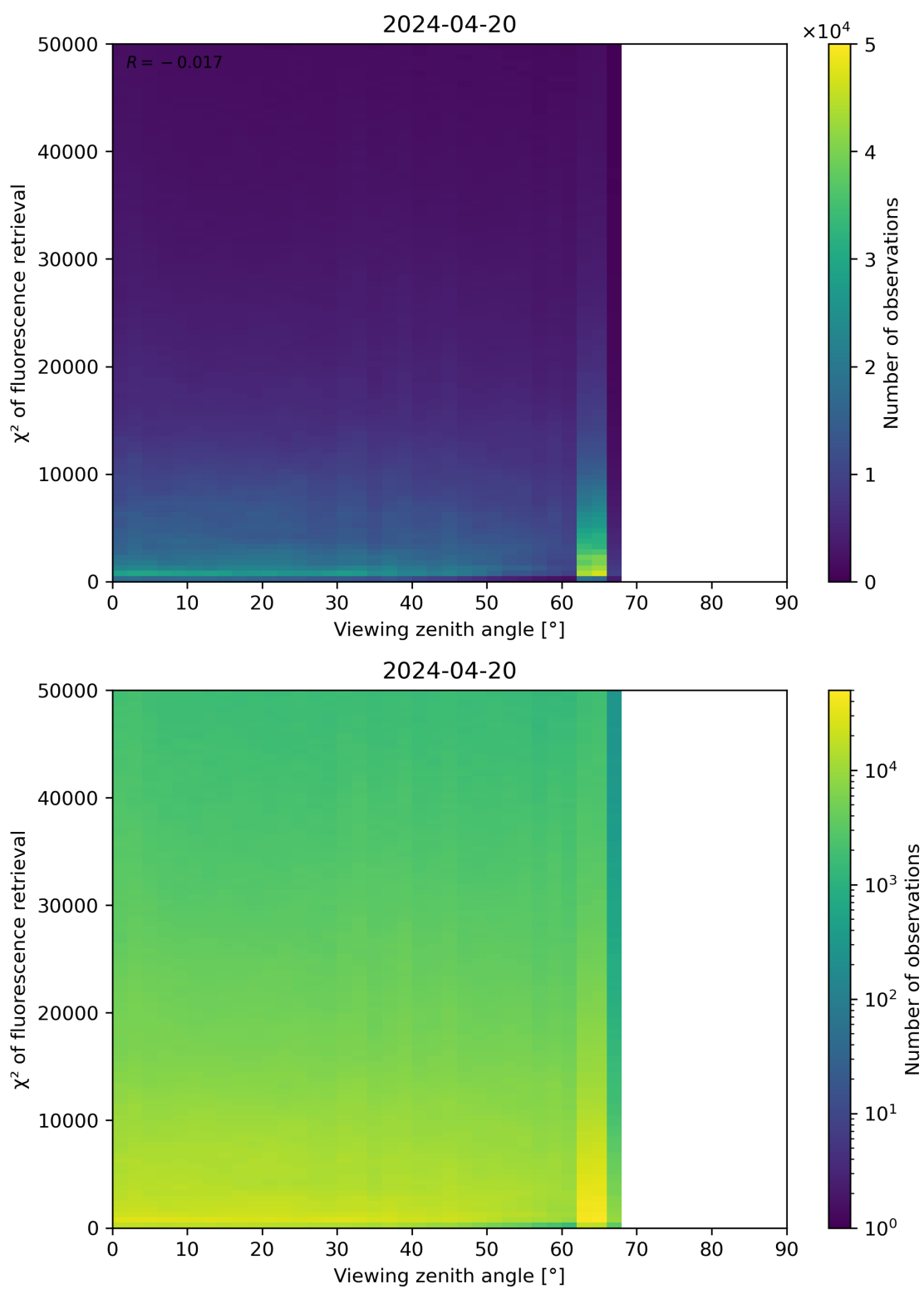
Figure 119: Scatter density plot of “Viewing zenith angle” against “ \chi^2 of fluorescence retrieval” for 2024-04-19 to 2024-04-21.
