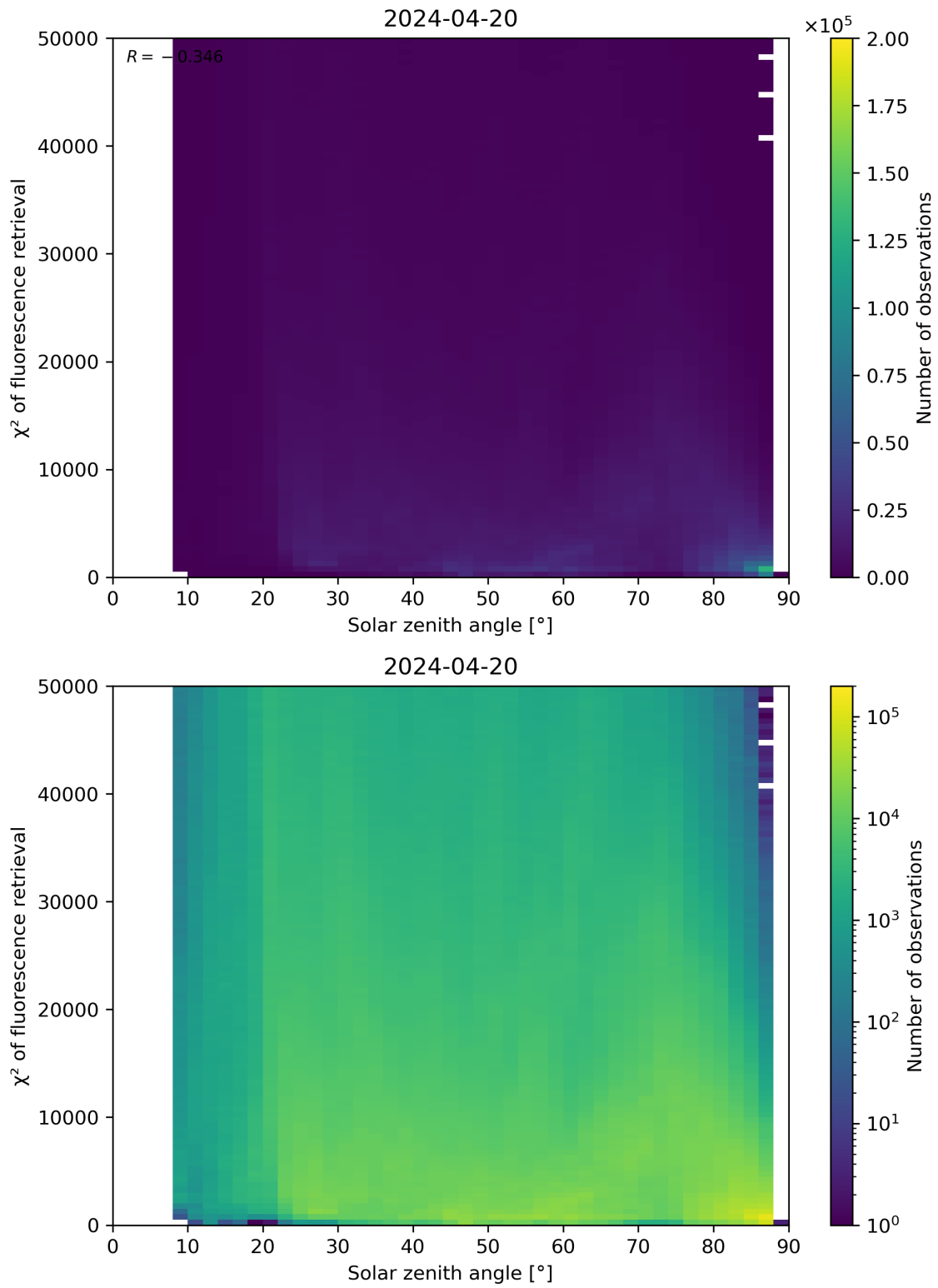
Figure 109: Scatter density plot of “Solar zenith angle” against “ \chi^2 of fluorescence retrieval” for 2024-04-19 to 2024-04-21.
