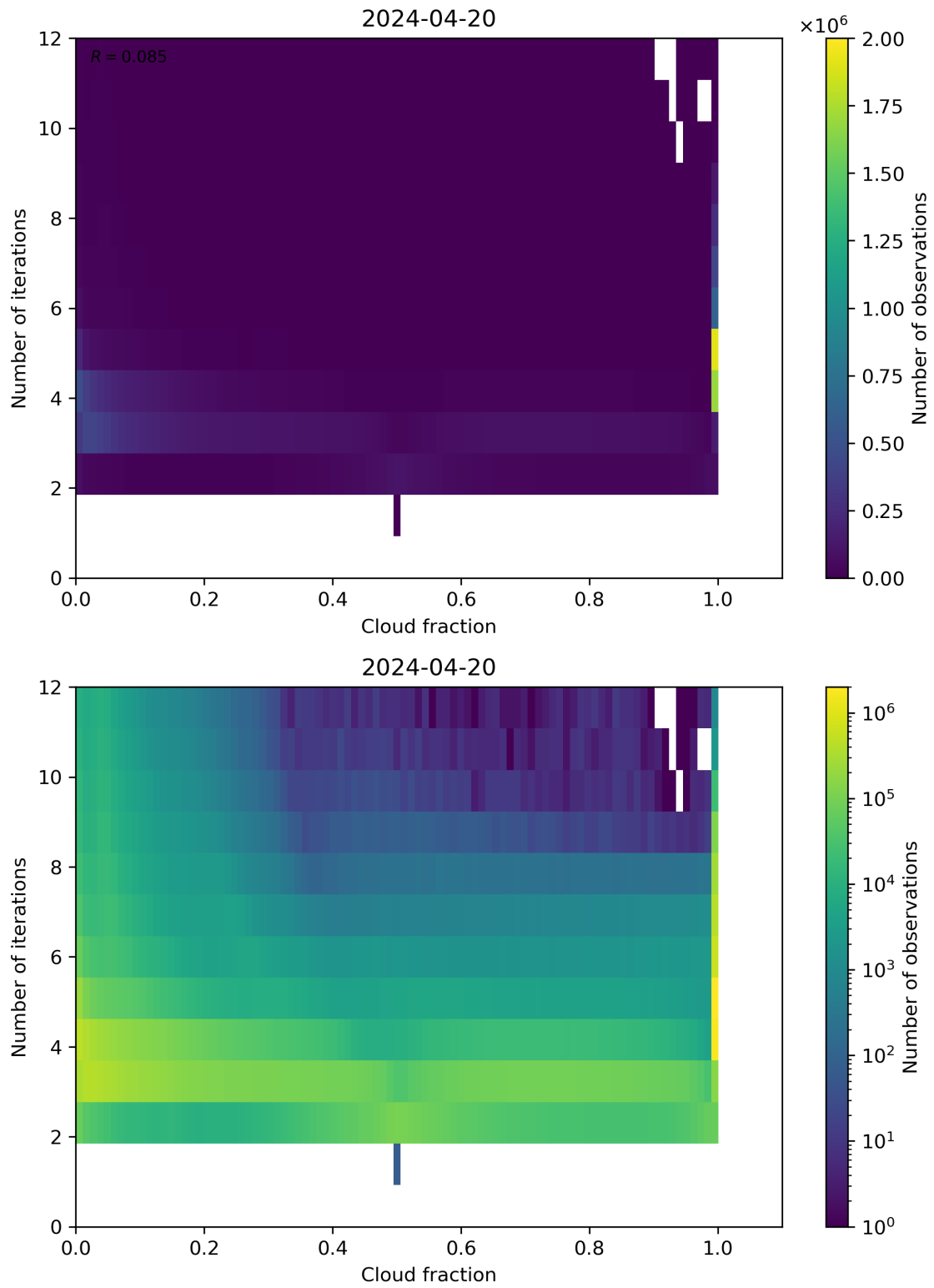
Figure 73: Scatter density plot of “Cloud fraction” against “Number of iterations” for 2024-04-19 to 2024-04-21.
