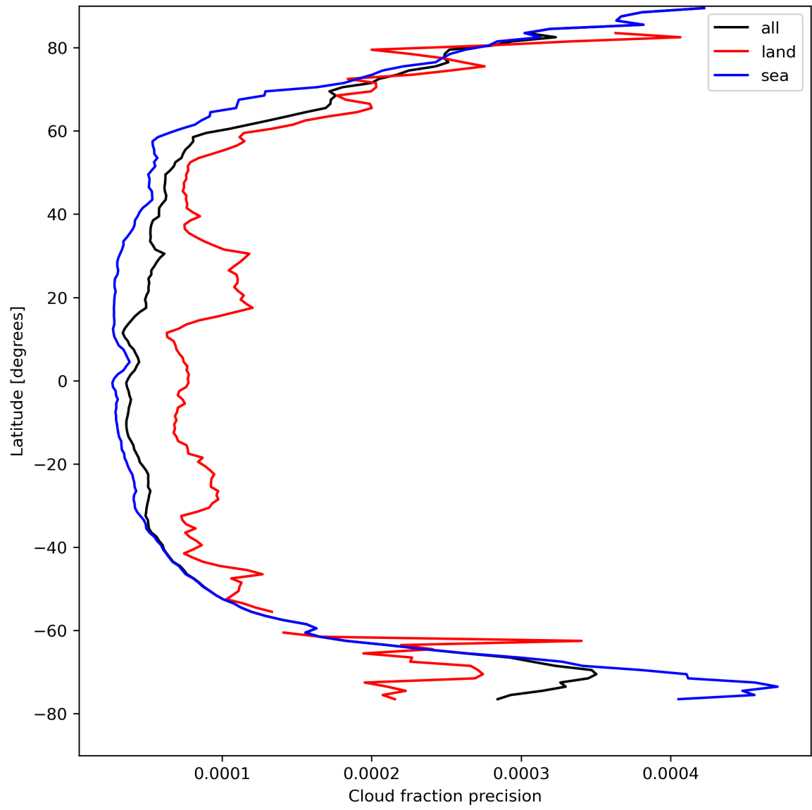
Figure 16: Zonal average of “Cloud fraction precision” for 2024-04-19 to 2024-04-21.
