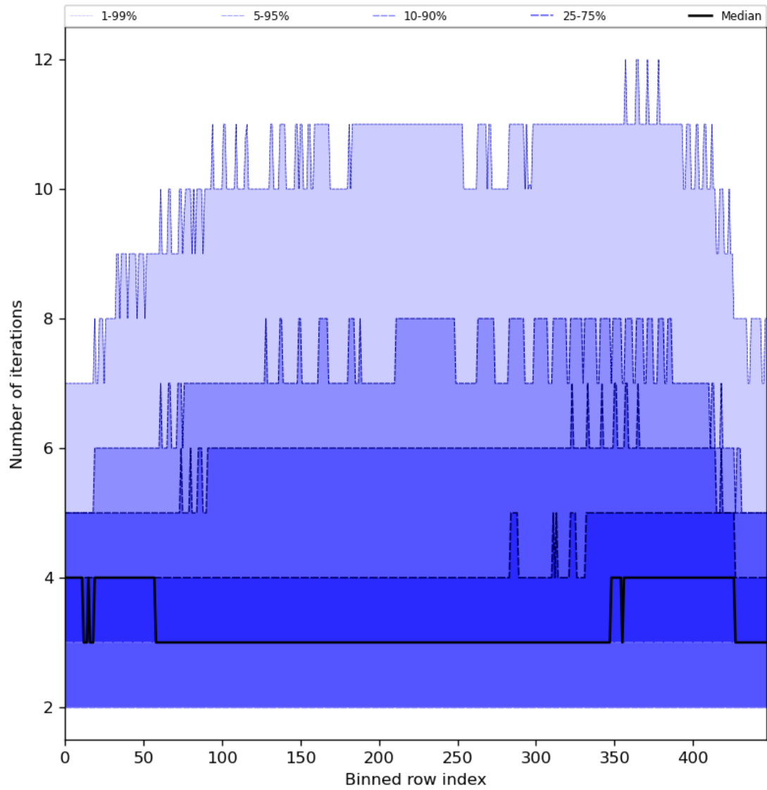
Figure 56: Along track statistics of “Number of iterations” for 2024-04-19 to 2024-04-21
