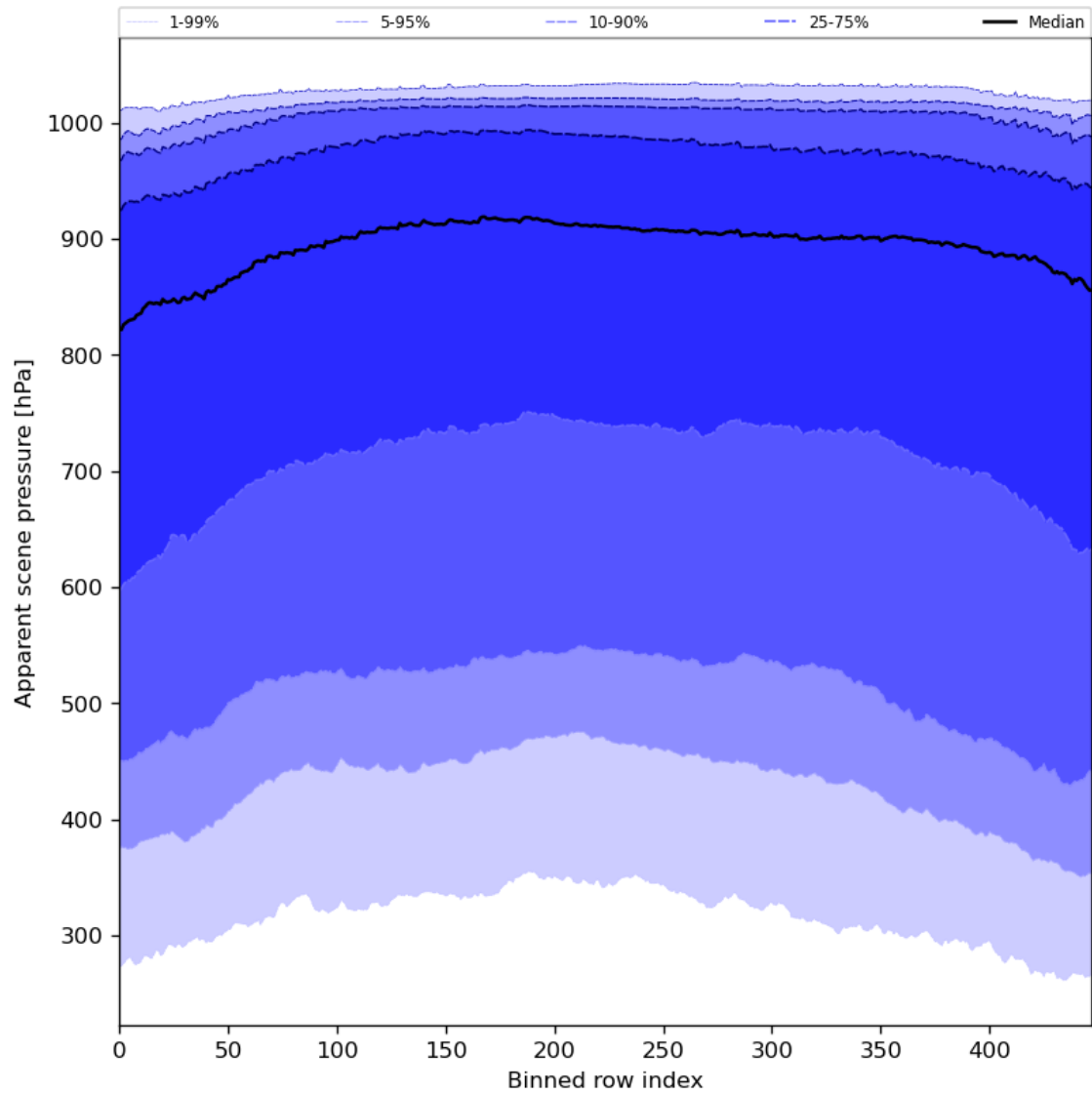
Figure 53: Along track statistics of “Apparent scene pressure” for 2024-04-19 to 2024-04-21
