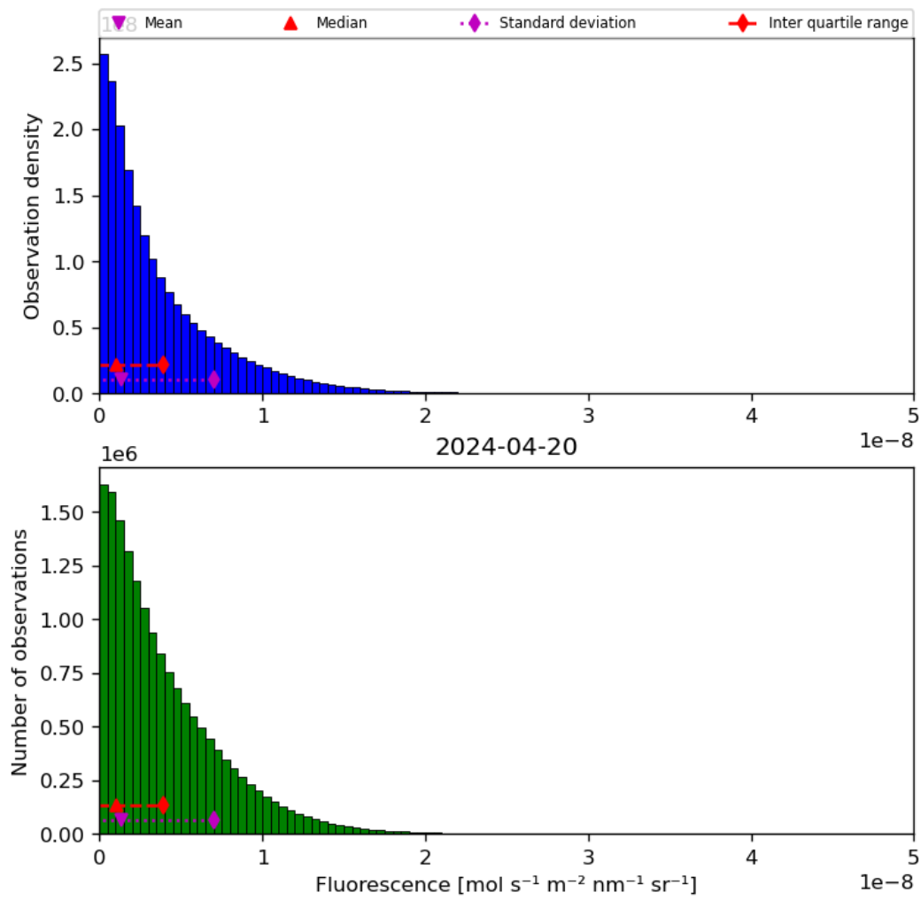
Figure 40: Histogram of “Fluorescence” for 2024-04-19 to 2024-04-21
