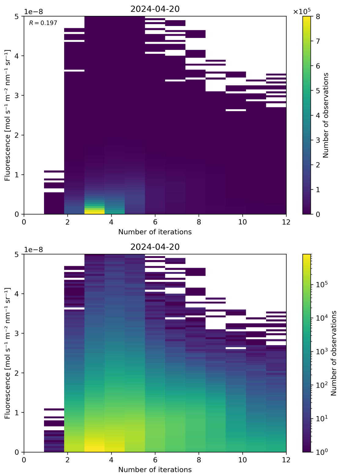
Figure 98: Scatter density plot of “Number of iterations” against “Fluorescence” for 2024-04-19 to 2024-04-21.
