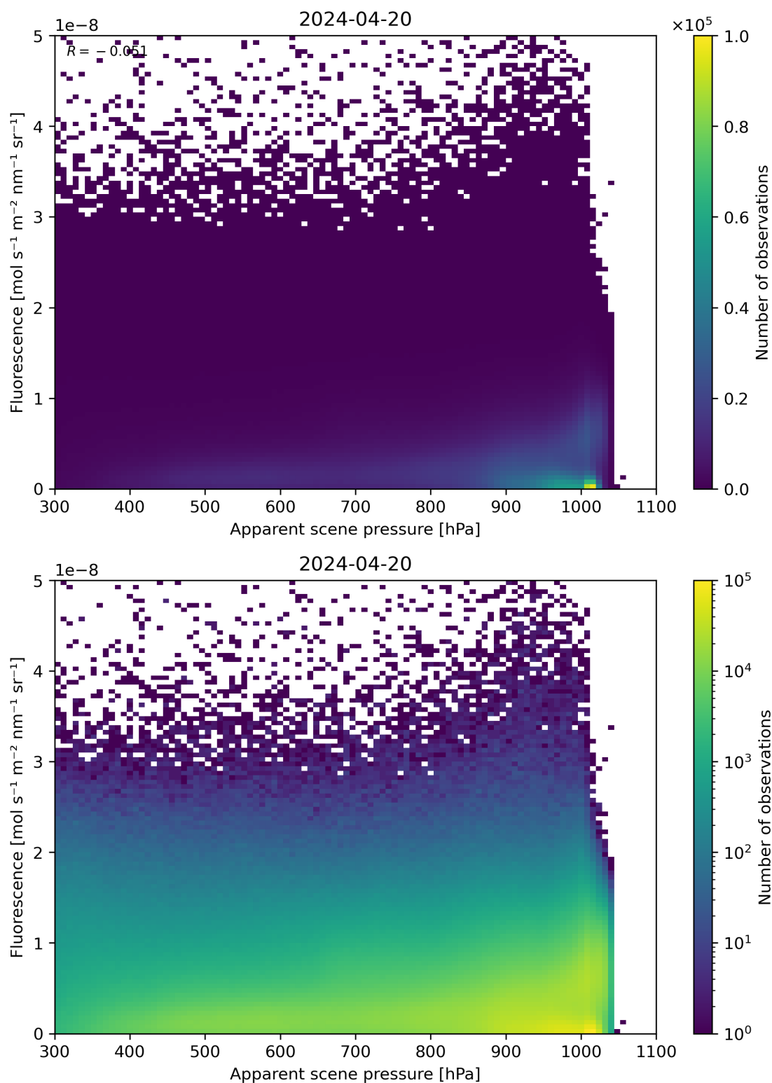
Figure 64: Scatter density plot of “Apparent scene pressure” against “Fluorescence” for 2024-04-19 to 2024-04-21.
