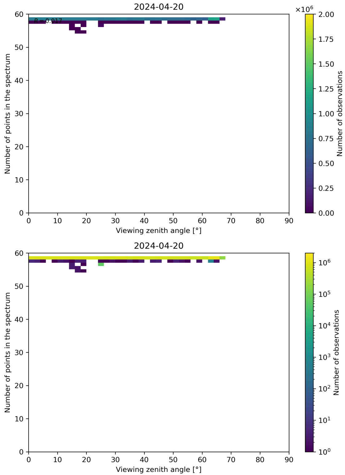
Figure 125: Scatter density plot of “Viewing zenith angle” against “Number of points in the spectrum” for 2024-04-19 to 2024-04-21.
