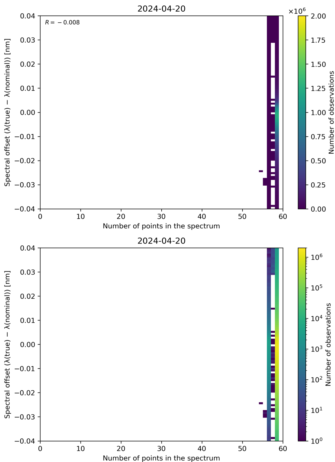
Figure 101: Scatter density plot of “Number of points in the spectrum” against “Spectral offset ( \lambda(\text{true}) - \lambda(\text{nominal}) )” for 2024-04-19 to 2024-04-21.
