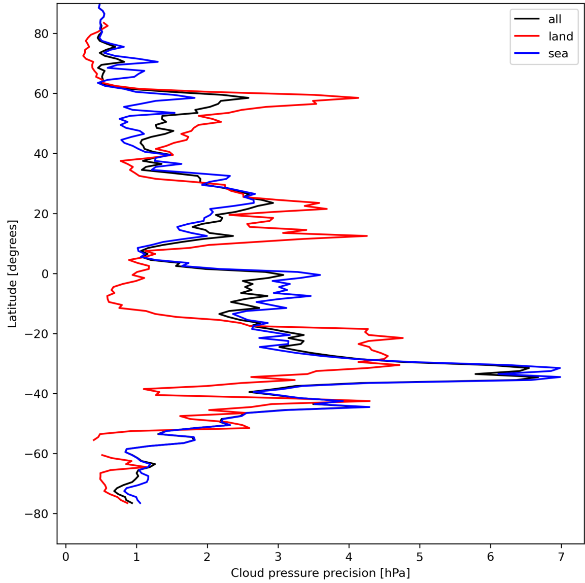
Figure 14: Zonal average of “Cloud pressure precision” for 2024-04-19 to 2024-04-21.
