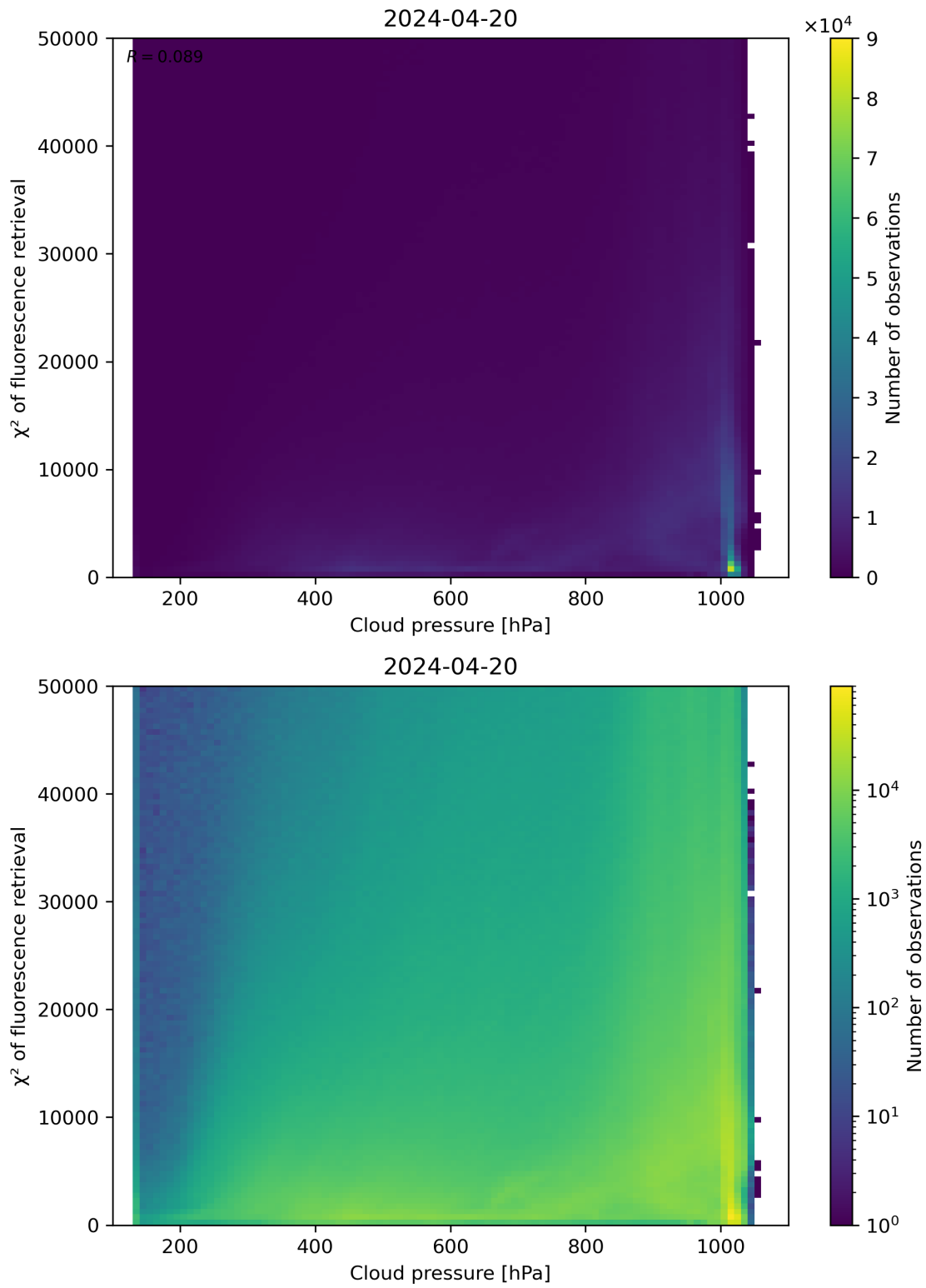
Figure 78: Scatter density plot of “Cloud pressure” against “ \chi^2 of fluorescence retrieval” for 2024-04-19 to 2024-04-21.
