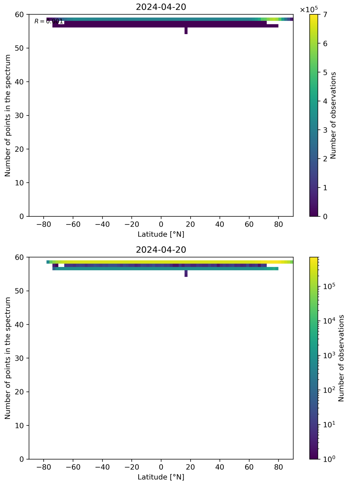
Figure 94: Scatter density plot of “Latitude” against “Number of points in the spectrum” for 2024-04-19 to 2024-04-21.
