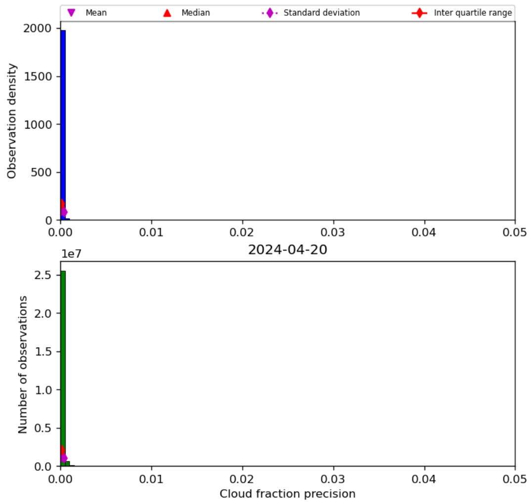
Figure 33: Histogram of “Cloud fraction precision” for 2024-04-19 to 2024-04-21
