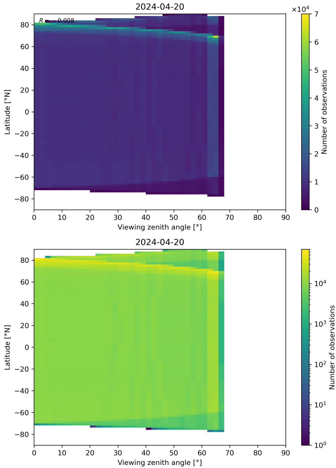
Figure 123: Scatter density plot of “Viewing zenith angle” against “Latitude” for 2024-04-19 to 2024-04-21.
