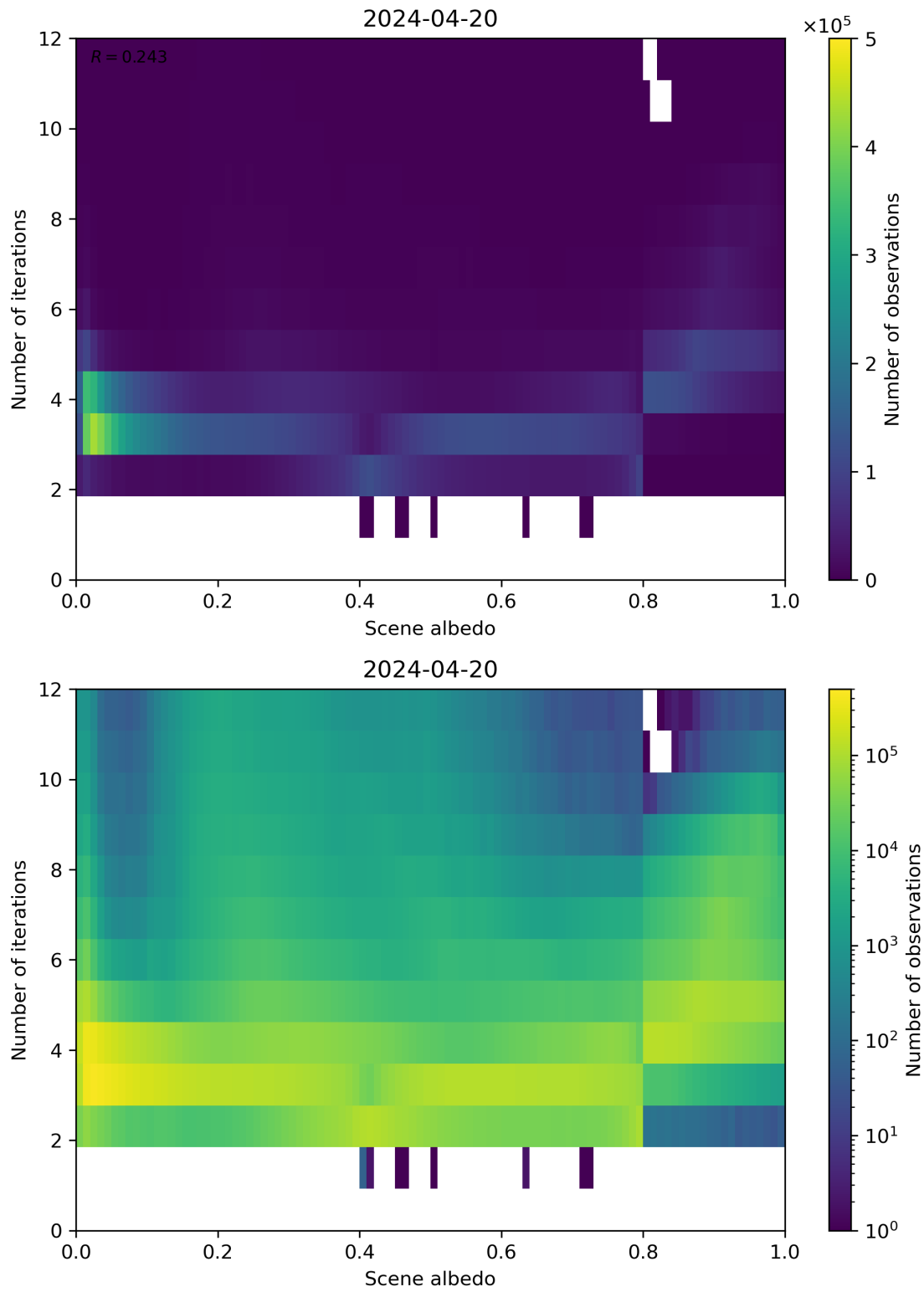
Figure 105: Scatter density plot of “Scene albedo” against “Number of iterations” for 2024-04-19 to 2024-04-21.
