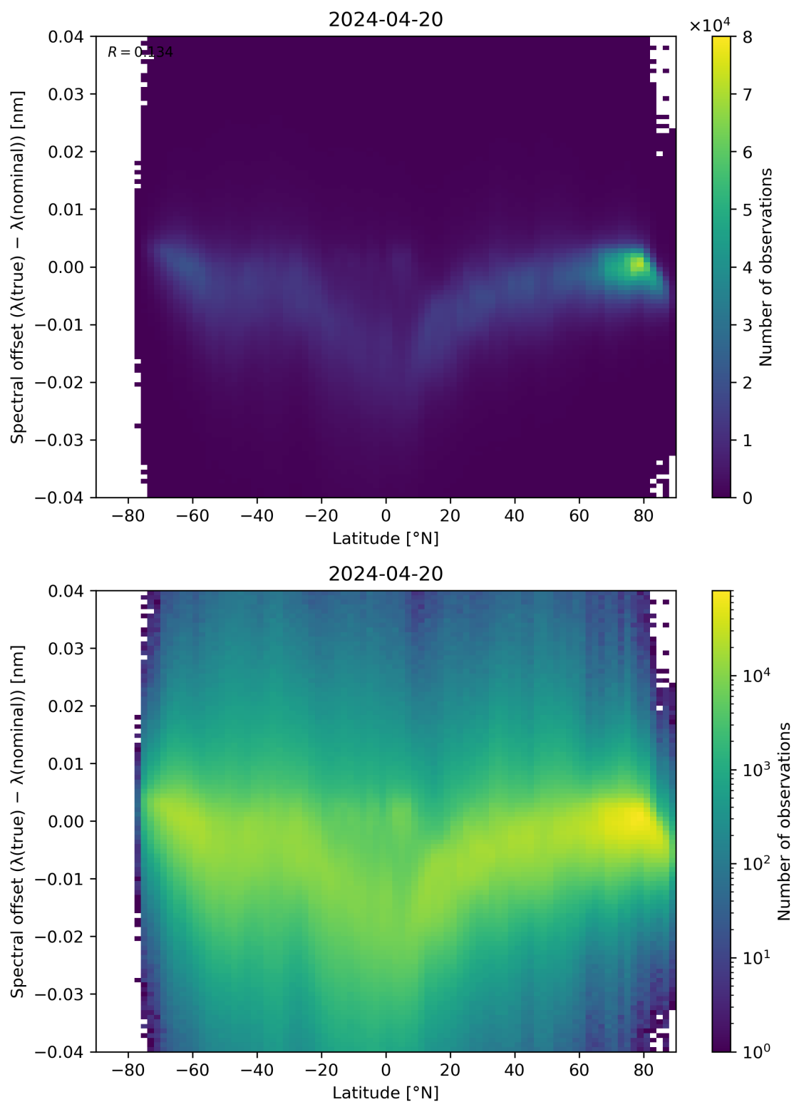
Figure 96: Scatter density plot of “Latitude” against “Spectral offset ( \lambda(\text{true}) - \lambda(\text{nominal}) )” for 2024-04-19 to 2024-04-21.
