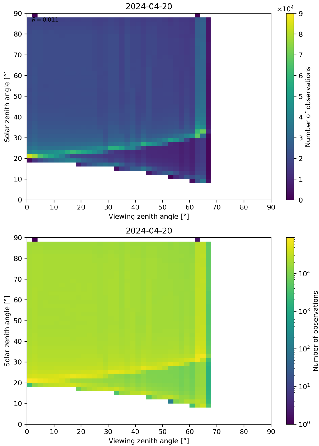
Figure 127: Scatter density plot of “Viewing zenith angle” against “Solar zenith angle” for 2024-04-19 to 2024-04-21.
