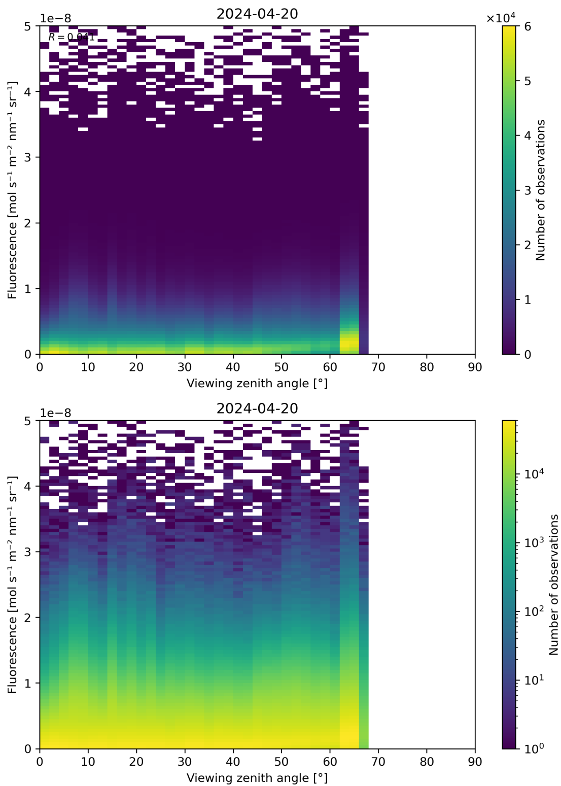
Figure 122: Scatter density plot of “Viewing zenith angle” against “Fluorescence” for 2024-04-19 to 2024-04-21.
