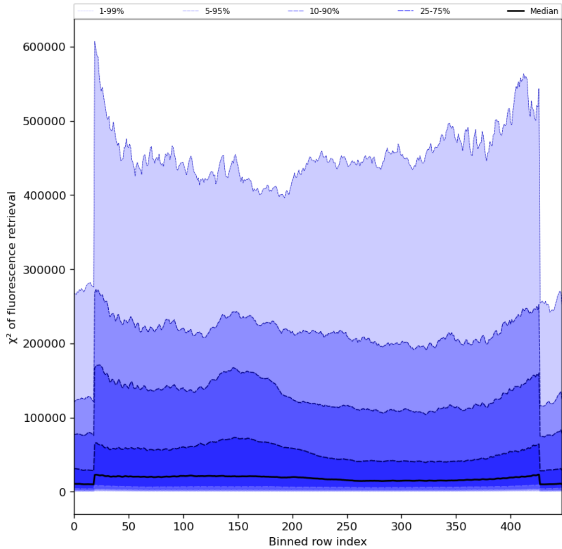
Figure 59: Along track statistics of “ \chi^2 of fluorescence retrieval” for 2024-04-19 to 2024-04-21
