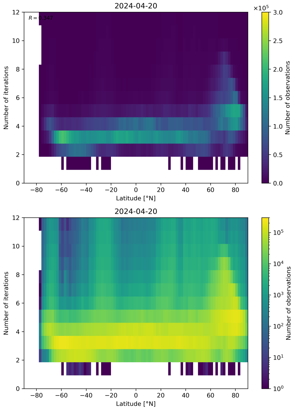
Figure 93: Scatter density plot of “Latitude” against “Number of iterations” for 2024-04-19 to 2024-04-21.
