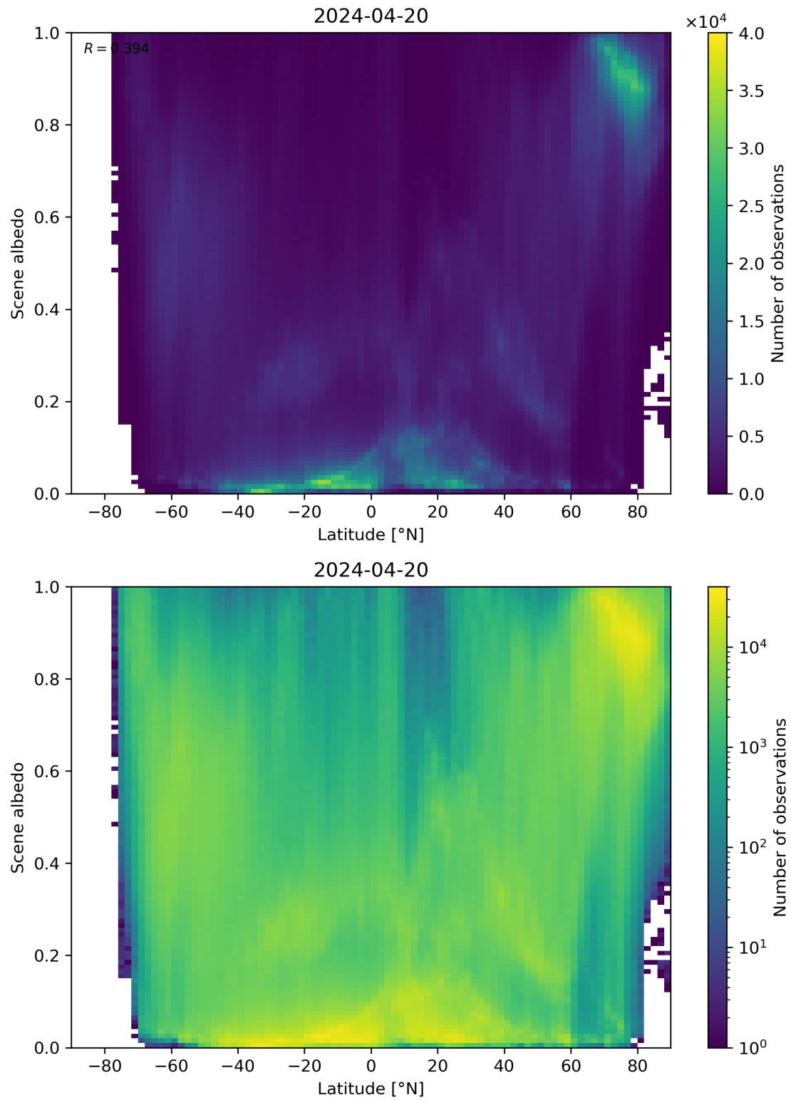
Figure 95: Scatter density plot of “Latitude” against “Scene albedo” for 2024-04-19 to 2024-04-21.
