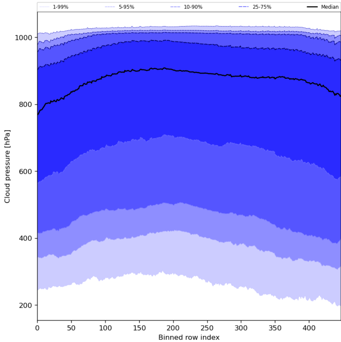
Figure 47: Along track statistics of “Cloud pressure” for 2024-04-19 to 2024-04-21
