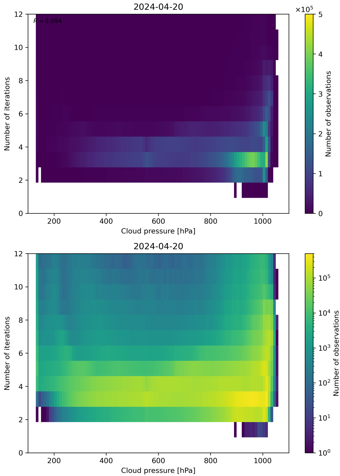
Figure 81: Scatter density plot of “Cloud pressure” against “Number of iterations” for 2024-04-19 to 2024-04-21.
