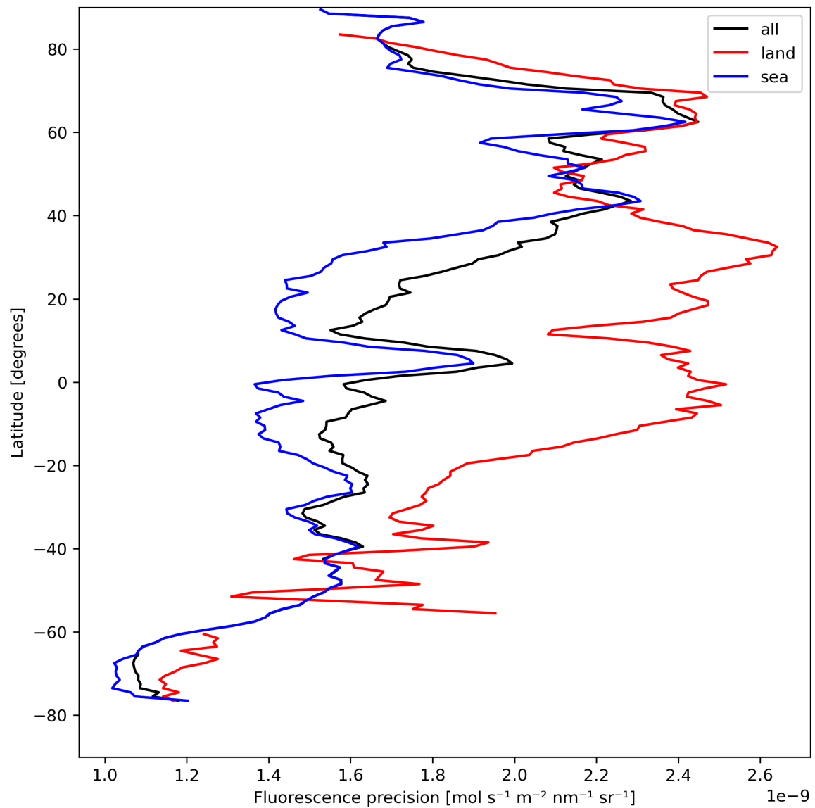
Figure 24: Zonal average of “Fluorescence precision” for 2024-04-19 to 2024-04-21.
