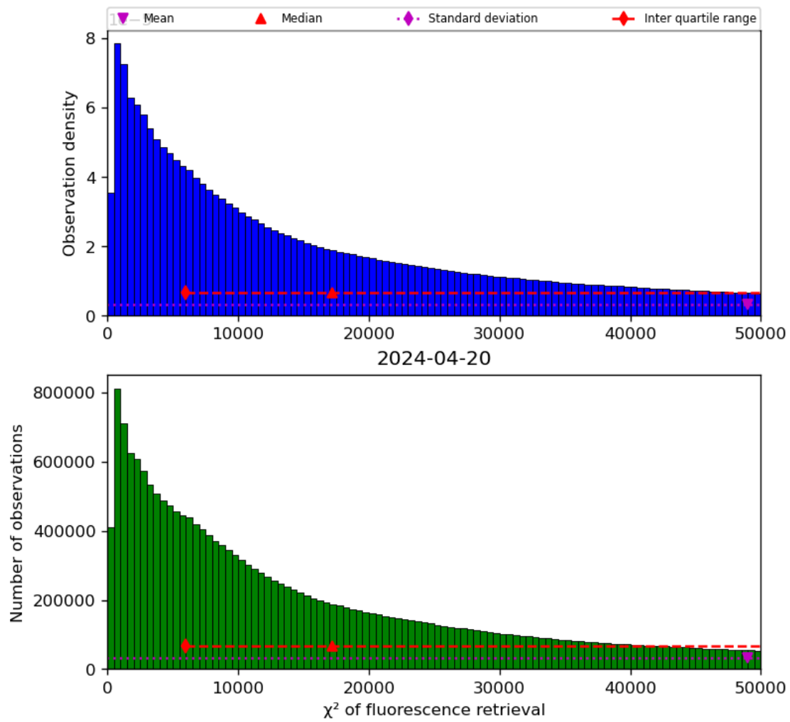
Figure 42: Histogram of “ \chi^2 of fluorescence retrieval” for 2024-04-19 to 2024-04-21
