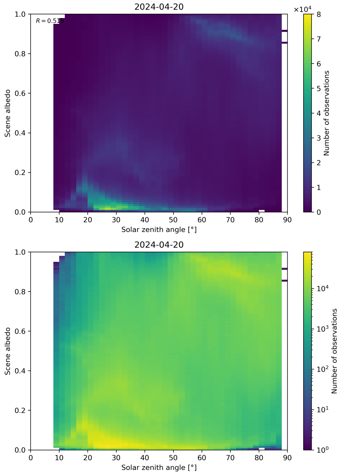
Figure 116: Scatter density plot of “Solar zenith angle” against “Scene albedo” for 2024-04-19 to 2024-04-21.
