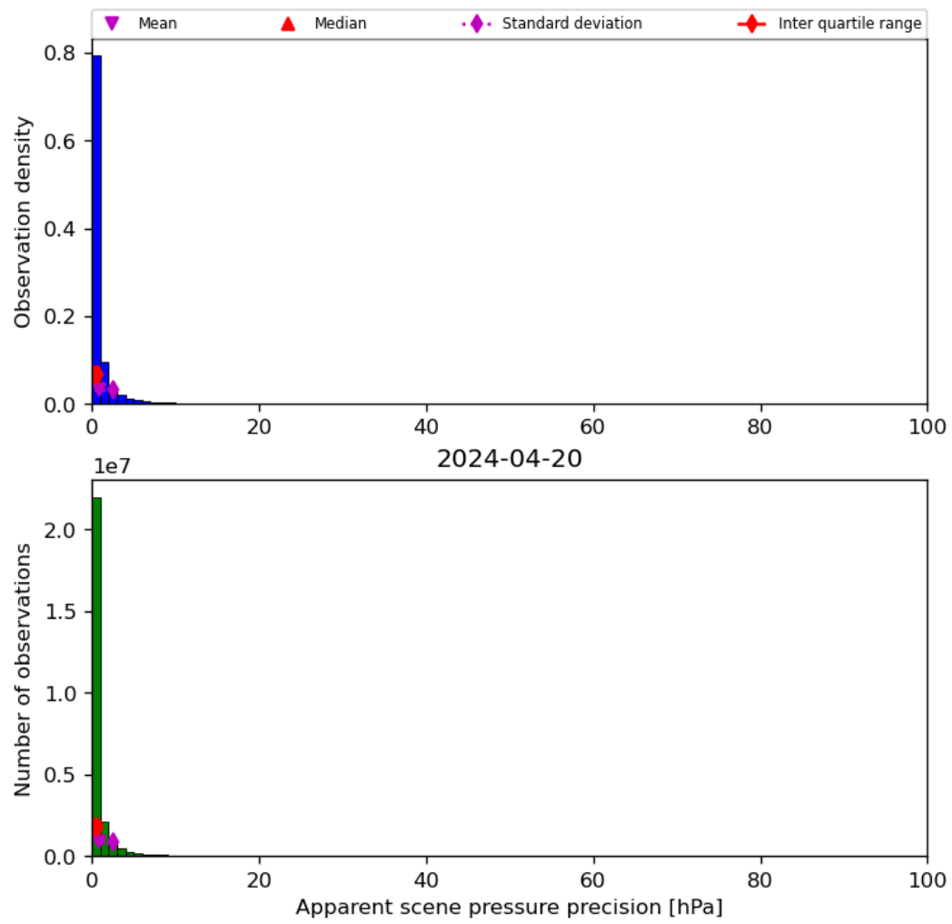
Figure 37: Histogram of “Apparent scene pressure precision” for 2024-04-19 to 2024-04-21
