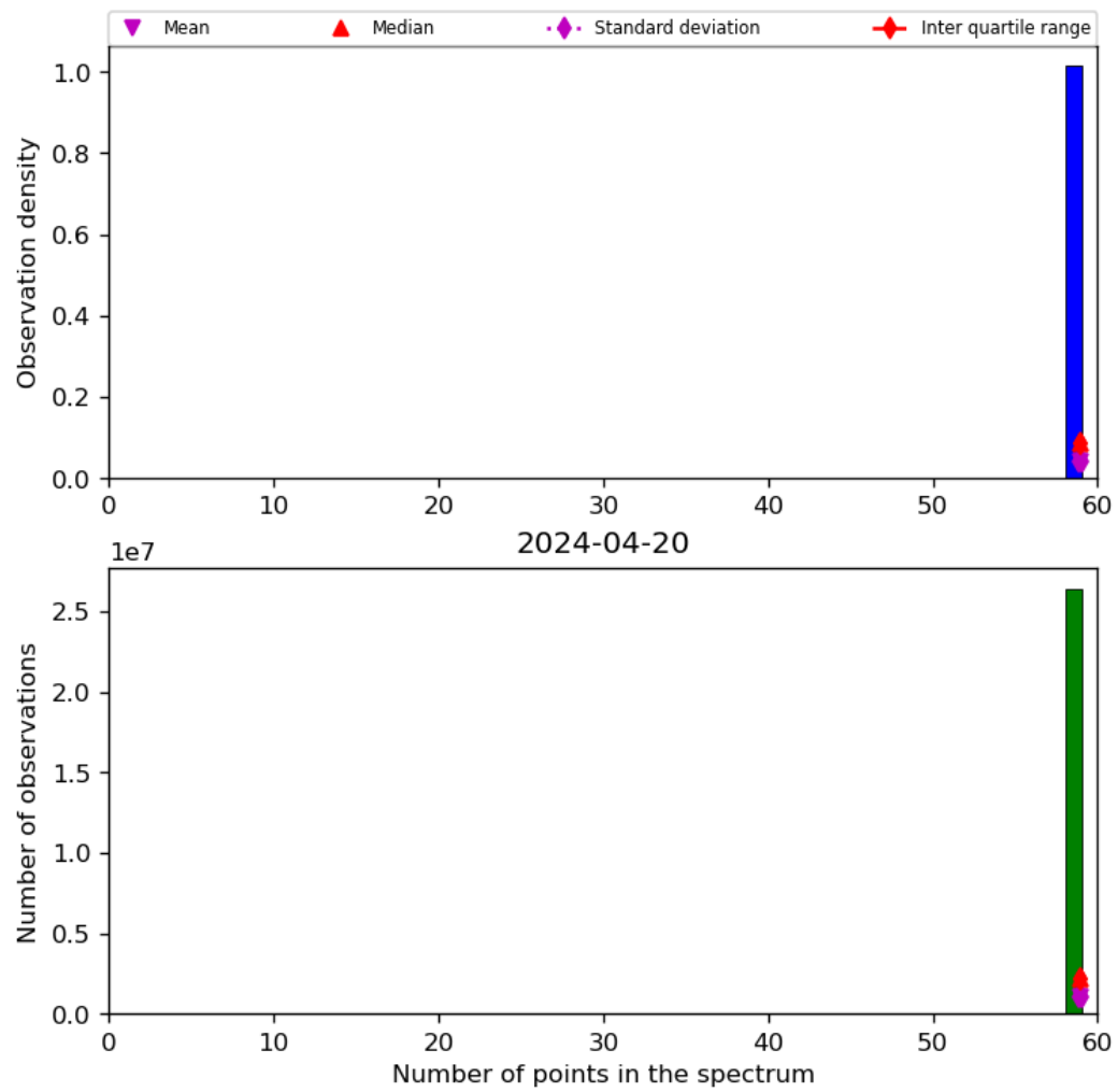
Figure 44: Histogram of “Number of points in the spectrum” for 2024-04-19 to 2024-04-21
