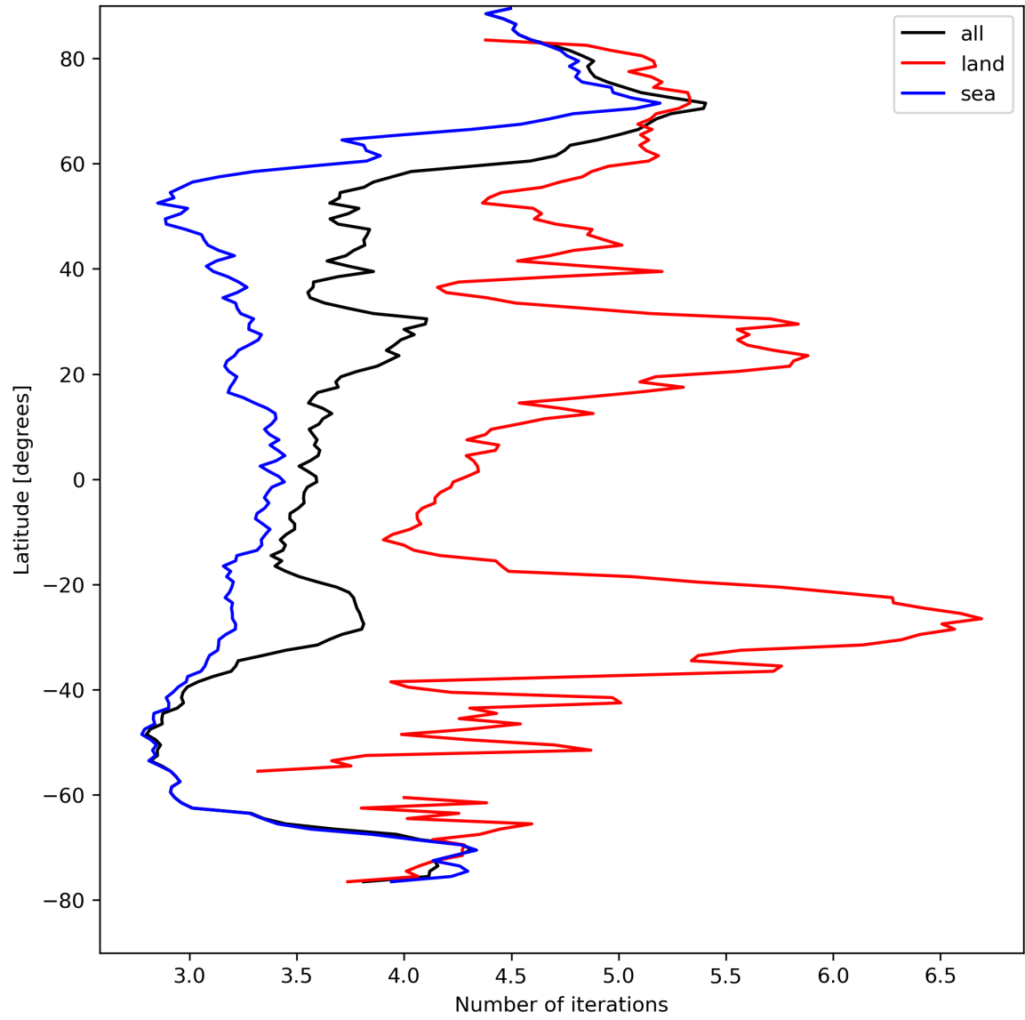
Figure 22: Zonal average of “Number of iterations” for 2024-04-19 to 2024-04-21.
