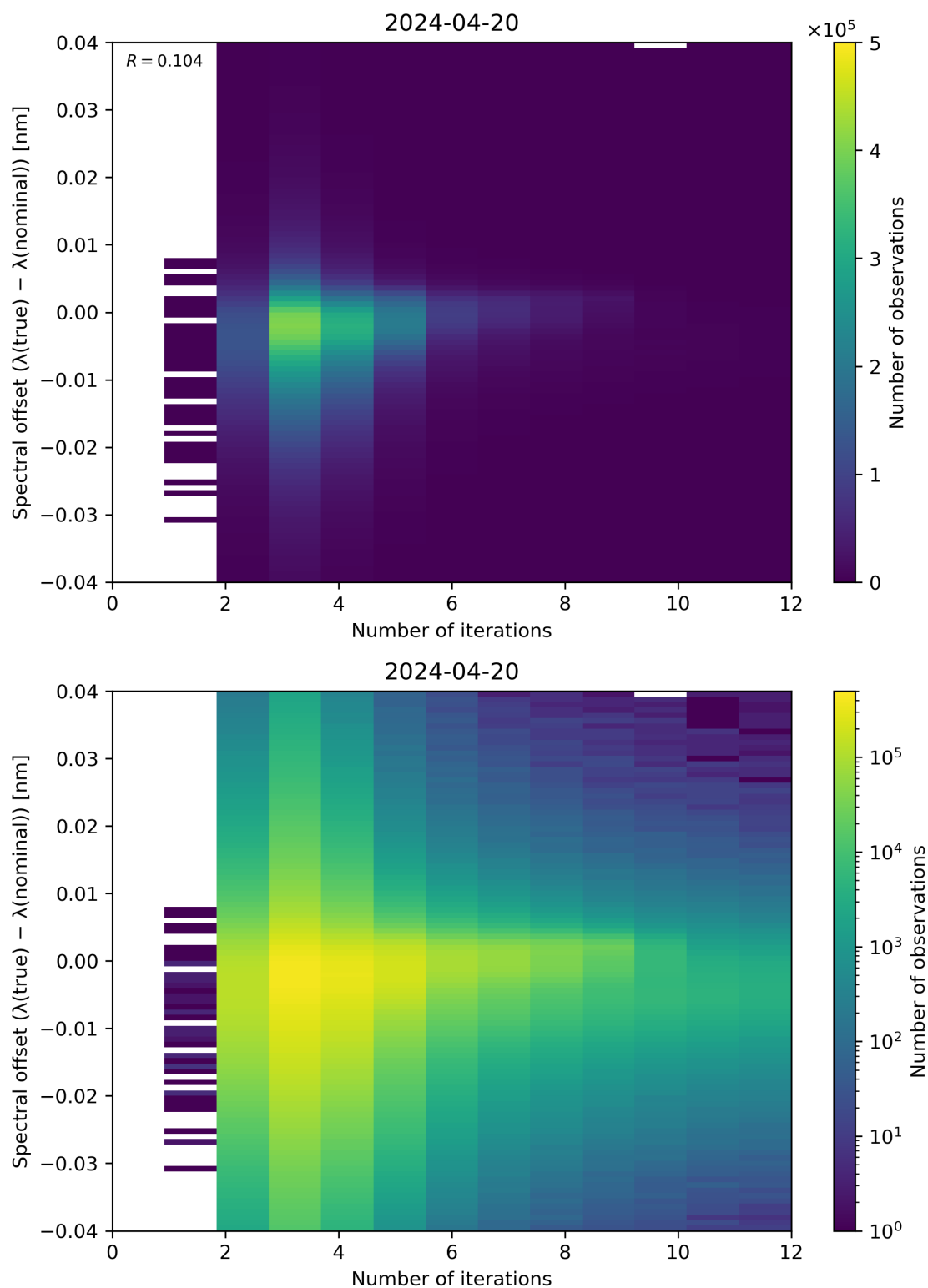
Figure 100: Scatter density plot of “Number of iterations” against “Spectral offset ( \lambda(\text{true}) - \lambda(\text{nominal}) )” for 2024-04-19 to 2024-04-21.
