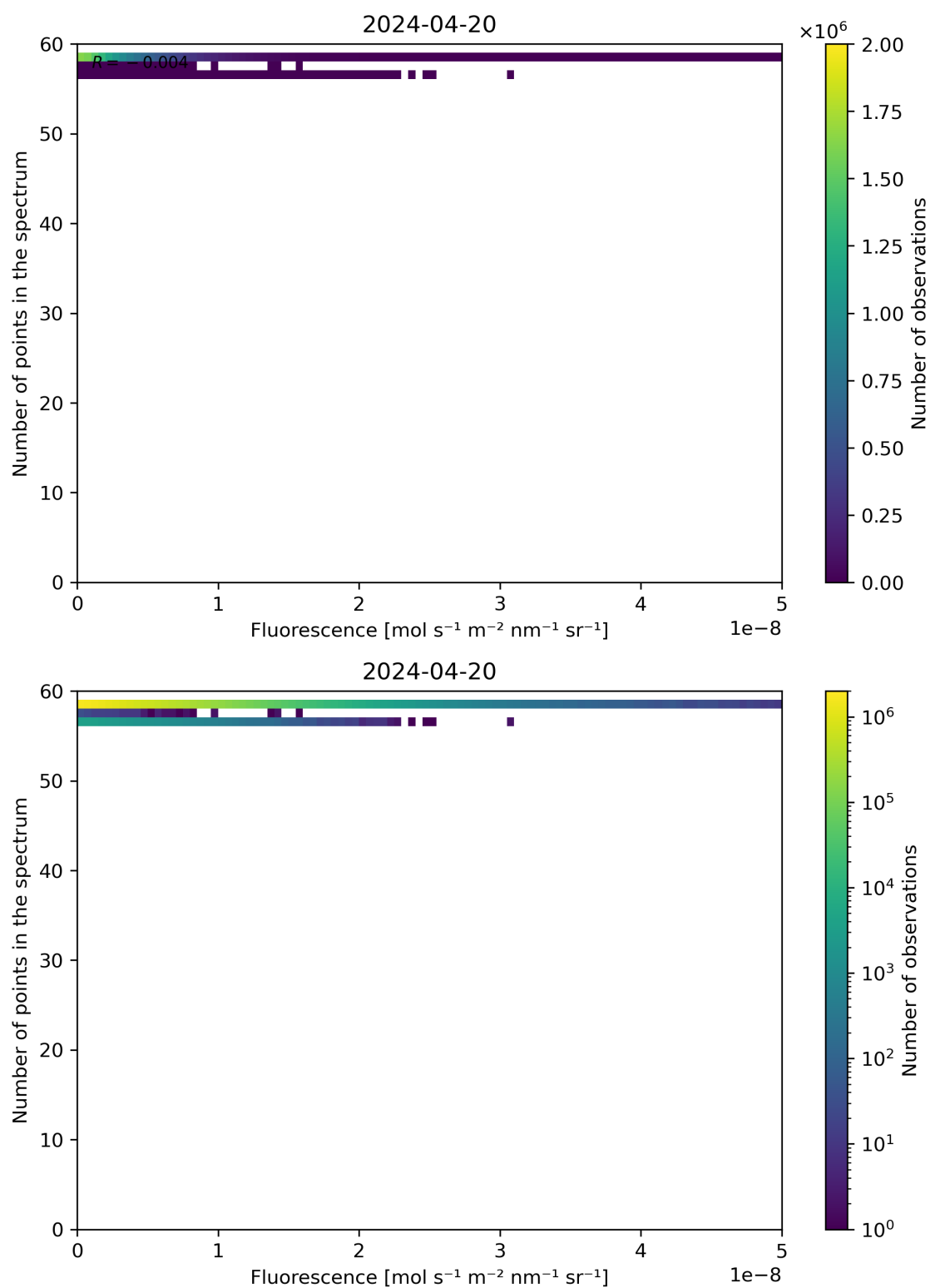
Figure 86: Scatter density plot of “Fluorescence” against “Number of points in the spectrum” for 2024-04-19 to 2024-04-21.
