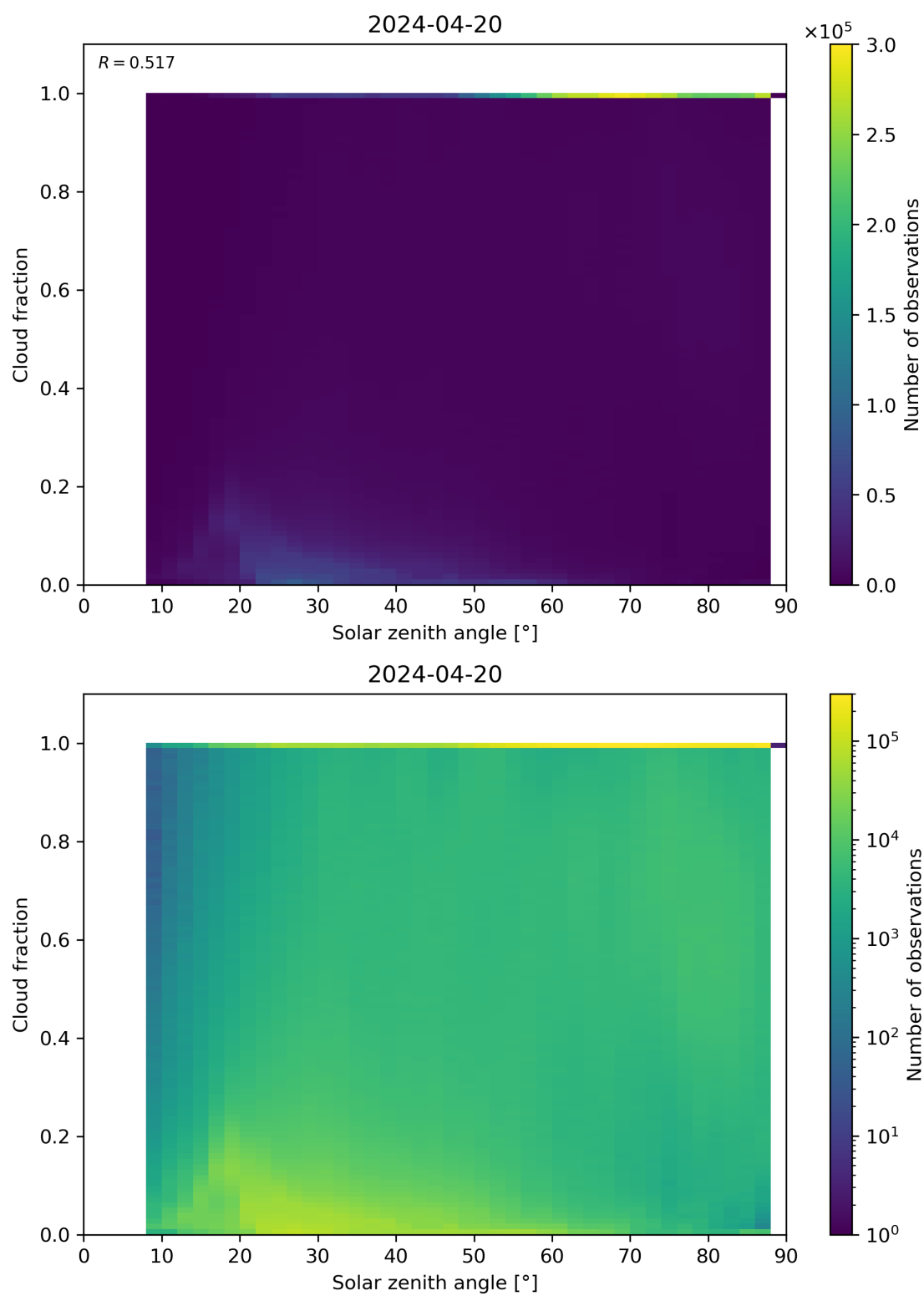
Figure 110: Scatter density plot of “Solar zenith angle” against “Cloud fraction” for 2024-04-19 to 2024-04-21.
