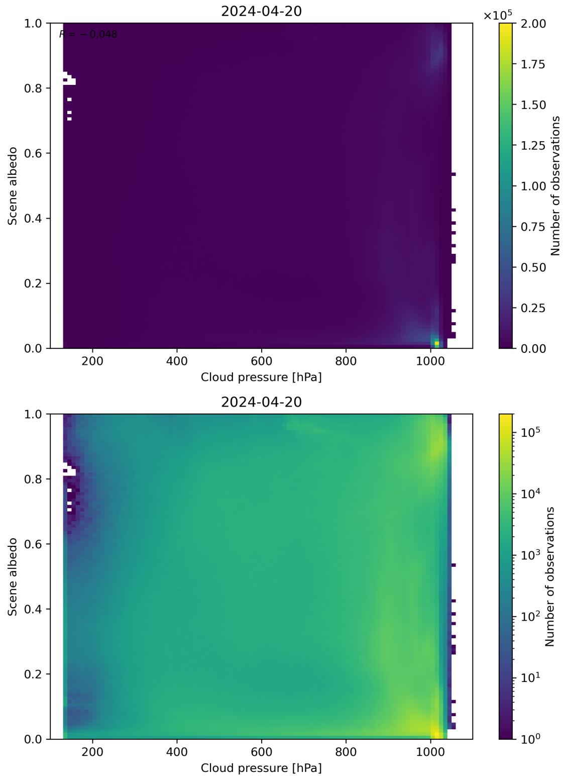
Figure 83: Scatter density plot of “Cloud pressure” against “Scene albedo” for 2024-04-19 to 2024-04-21.
