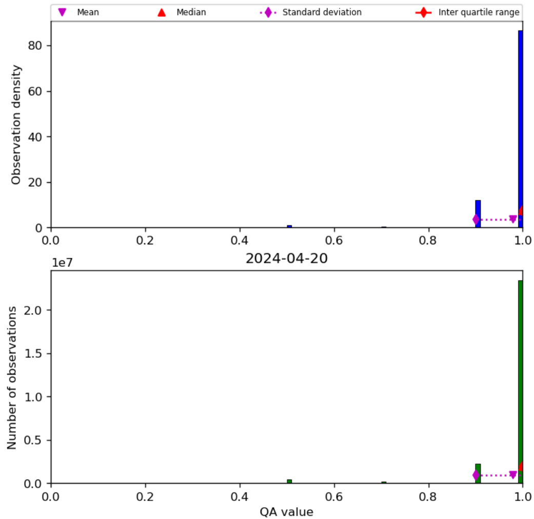
Figure 29: Histogram of “QA value” for 2024-04-19 to 2024-04-21
