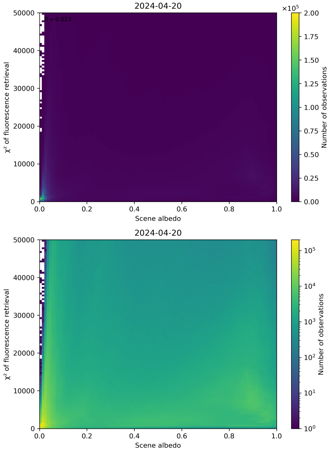
Figure 103: Scatter density plot of “Scene albedo” against “ \chi^2 of fluorescence retrieval” for 2024-04-19 to 2024-04-21.
