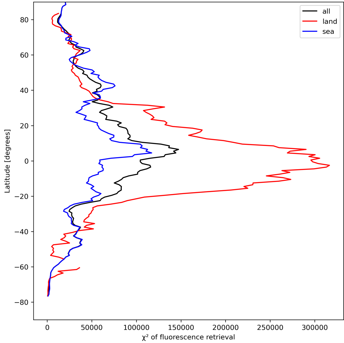
Figure 25: Zonal average of “ \chi^2 of fluorescence retrieval” for 2024-04-19 to 2024-04-21.
