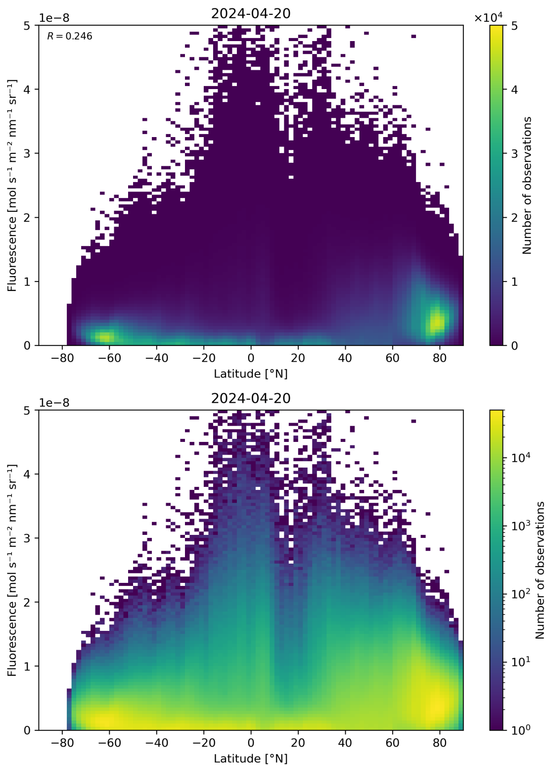
Figure 92: Scatter density plot of “Latitude” against “Fluorescence” for 2024-04-19 to 2024-04-21.
