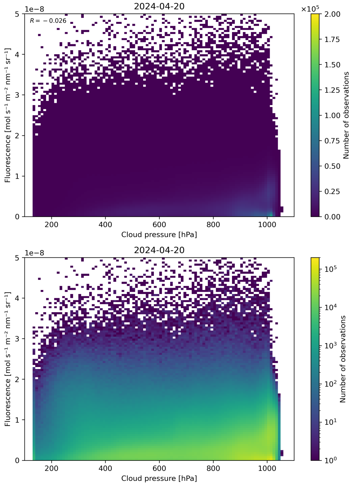
Figure 80: Scatter density plot of “Cloud pressure” against “Fluorescence” for 2024-04-19 to 2024-04-21.
