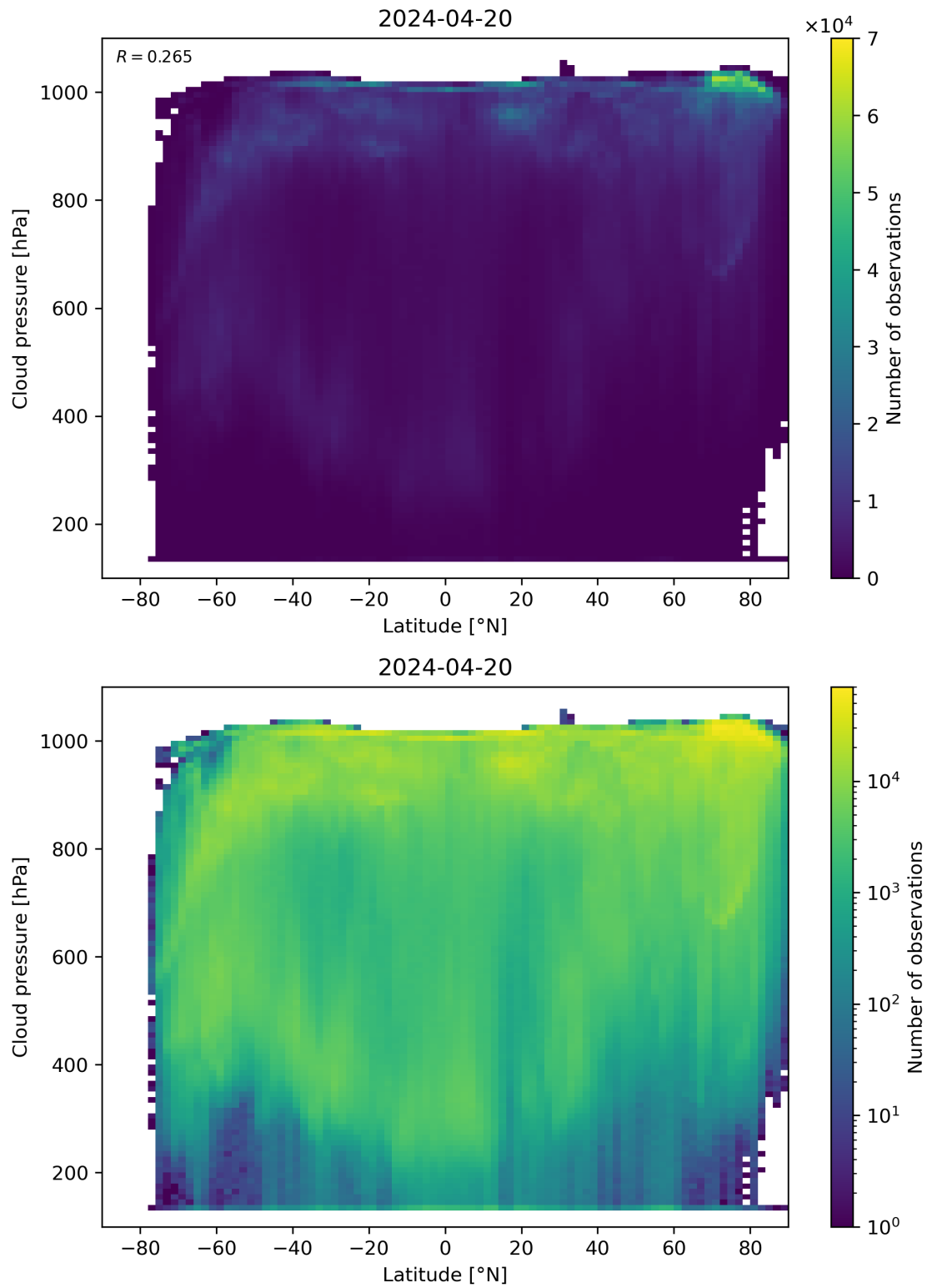
Figure 91: Scatter density plot of “Latitude” against “Cloud pressure” for 2024-04-19 to 2024-04-21.
