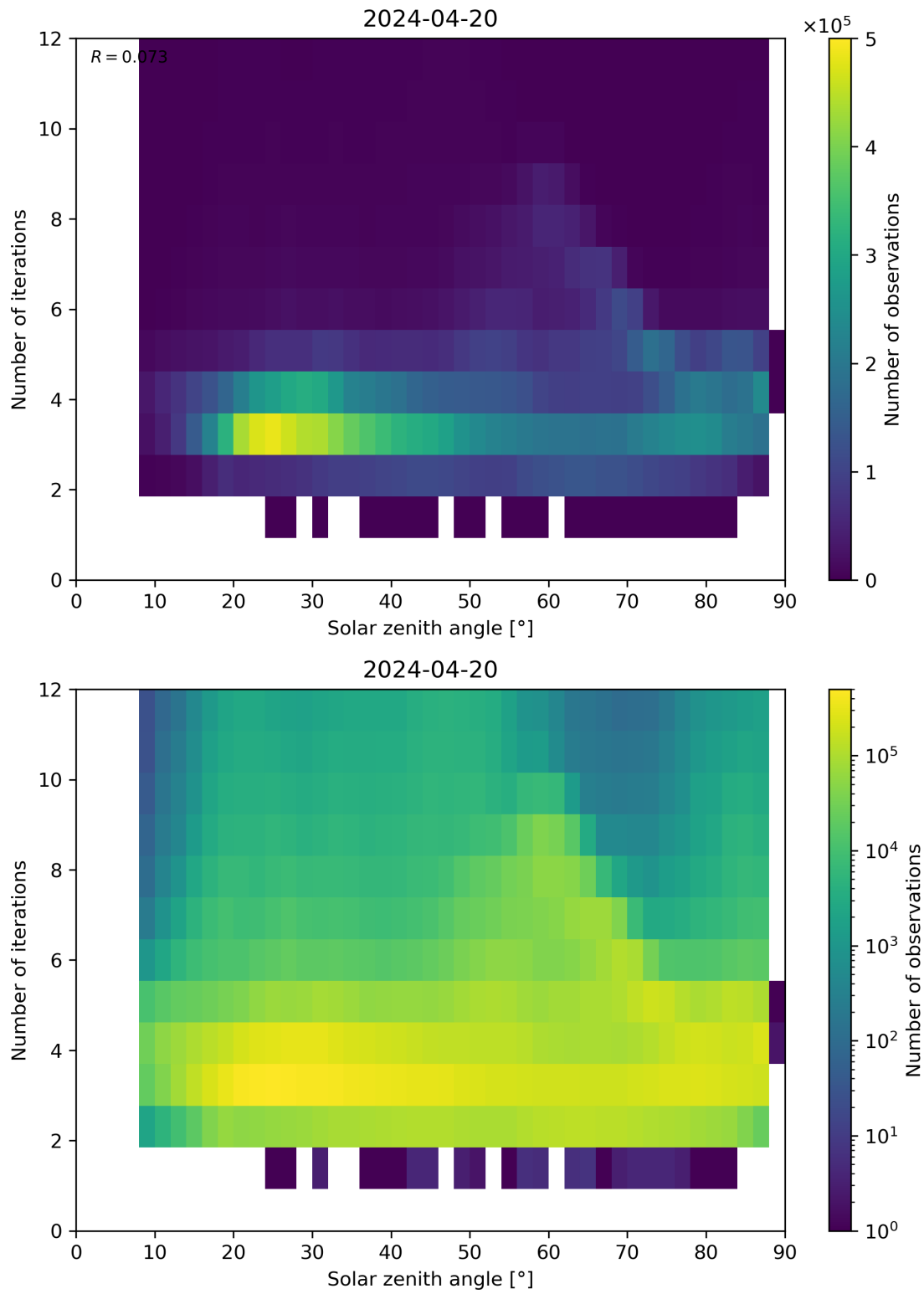
Figure 114: Scatter density plot of “Solar zenith angle” against “Number of iterations” for 2024-04-19 to 2024-04-21.
