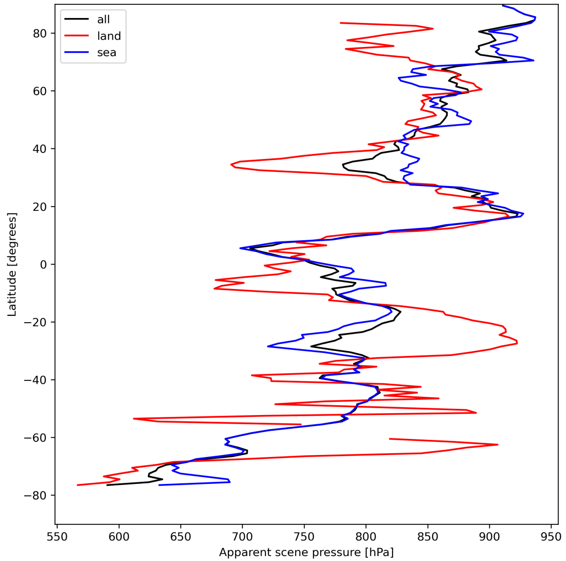
Figure 19: Zonal average of “Apparent scene pressure” for 2024-04-19 to 2024-04-21.
