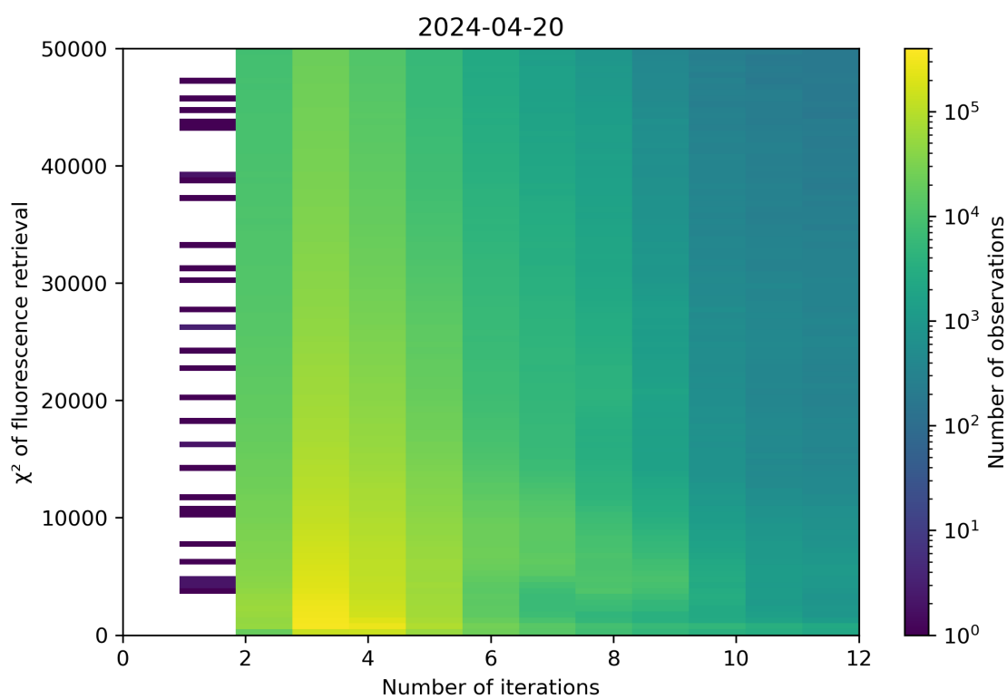
Figure 97: Scatter density plot of “Number of iterations” against “ \chi^2 of fluorescence retrieval” for 2024-04-19 to 2024-04-21.
