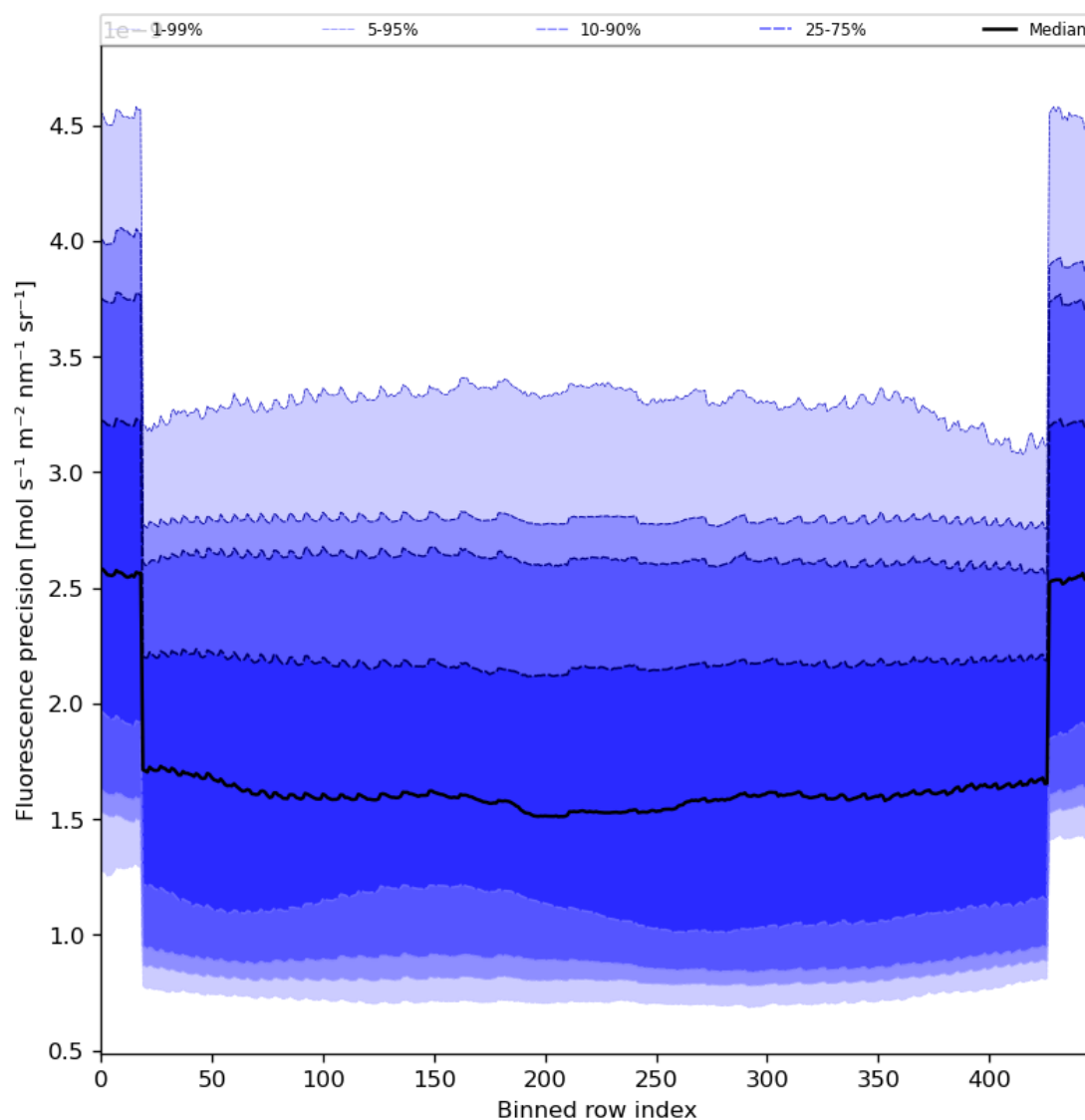
Figure 58: Along track statistics of “Fluorescence precision” for 2024-04-19 to 2024-04-21
