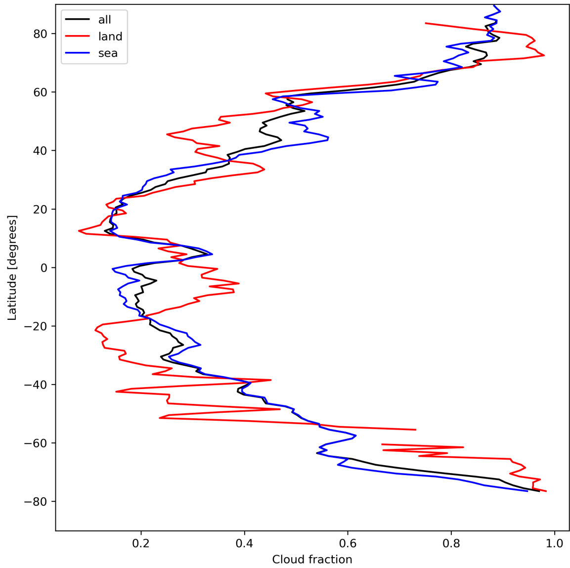
Figure 15: Zonal average of “Cloud fraction” for 2024-04-19 to 2024-04-21.
