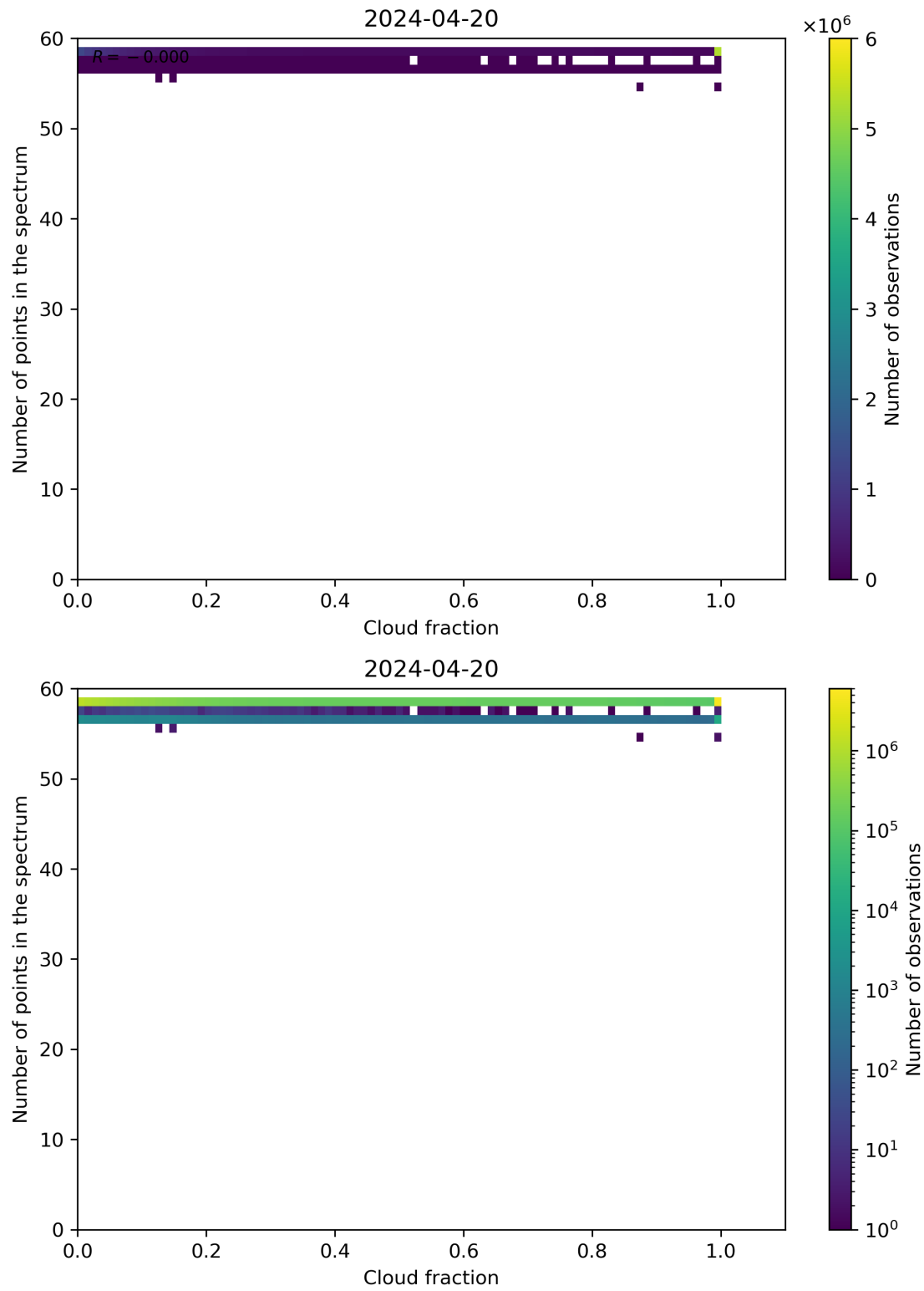
Figure 74: Scatter density plot of “Cloud fraction” against “Number of points in the spectrum” for 2024-04-19 to 2024-04-21.
