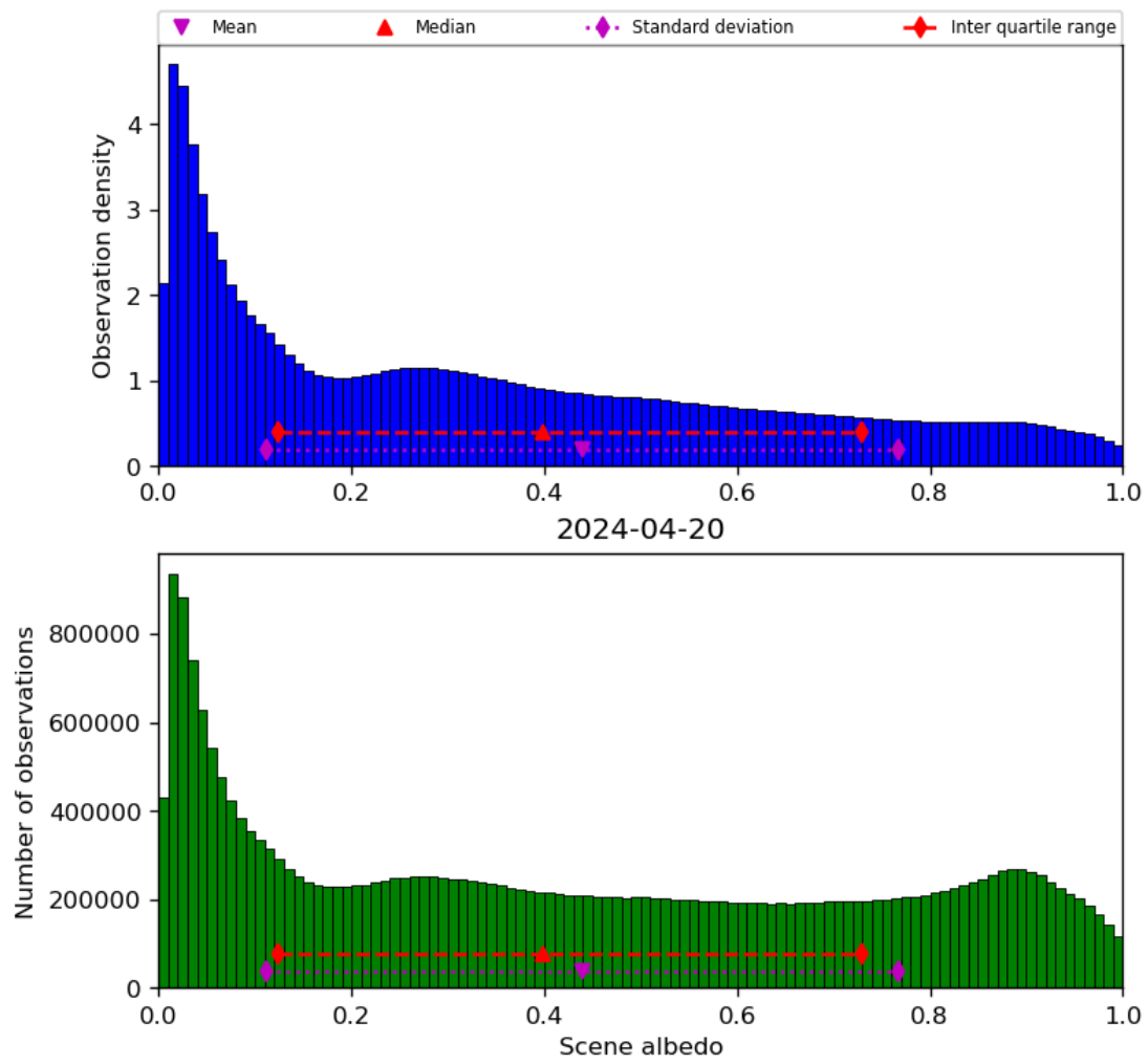
Figure 34: Histogram of “Scene albedo” for 2024-04-19 to 2024-04-21
