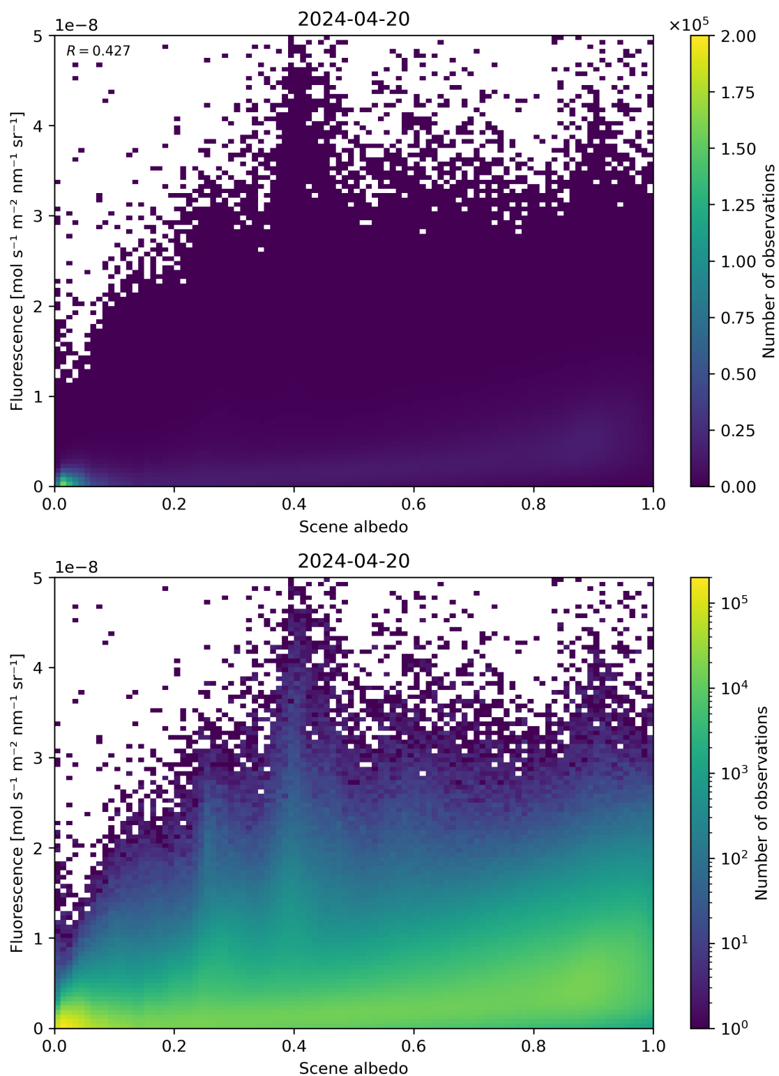
Figure 104: Scatter density plot of “Scene albedo” against “Fluorescence” for 2024-04-19 to 2024-04-21.
