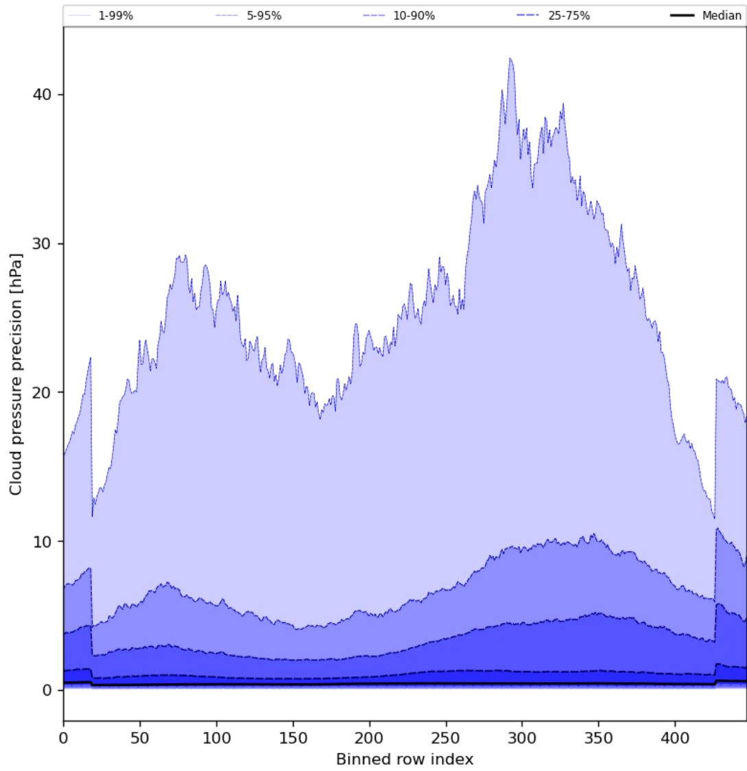
Figure 48: Along track statistics of “Cloud pressure precision” for 2024-04-19 to 2024-04-21
