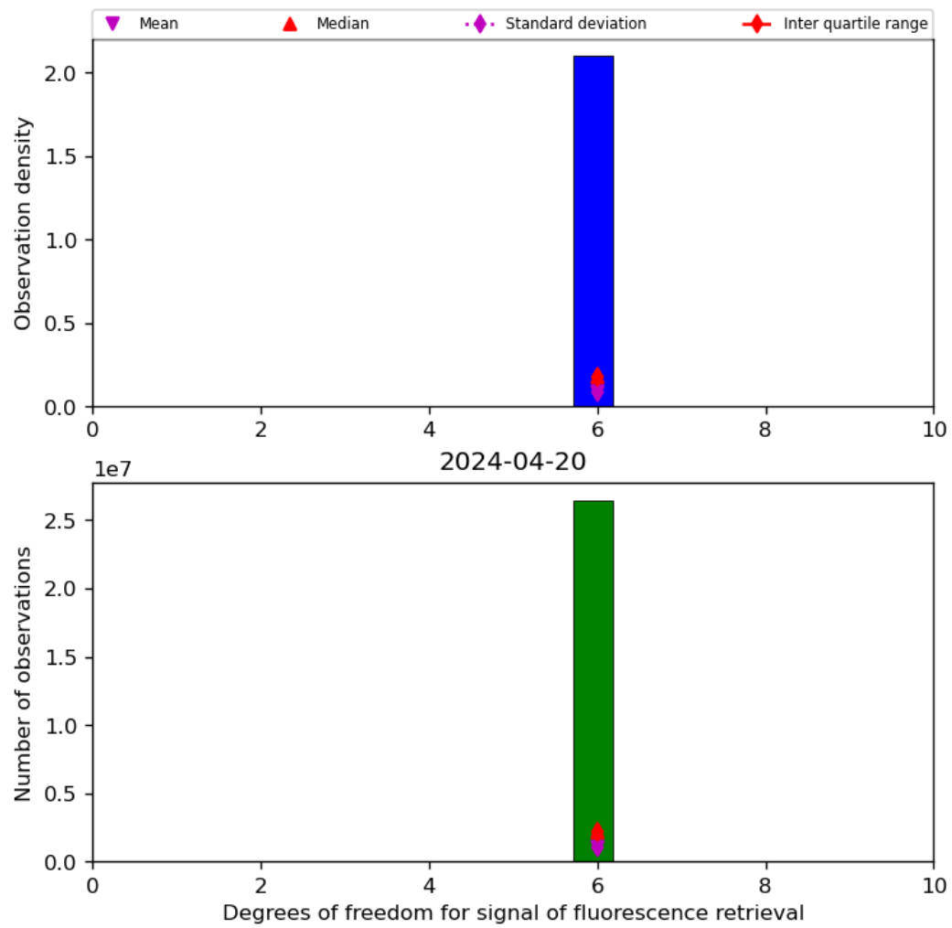
Figure 43: Histogram of “Degrees of freedom for signal of fluorescence retrieval” for 2024-04-19 to 2024-04-21
