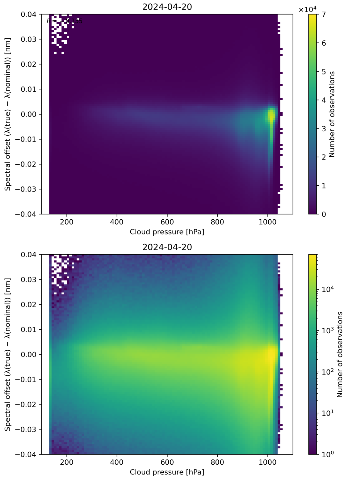
Figure 84: Scatter density plot of “Cloud pressure” against “Spectral offset ( \lambda(\text{true}) - \lambda(\text{nominal}) )” for 2024-04-19 to 2024-04-21.
