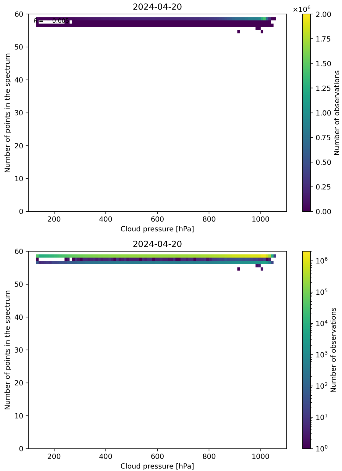
Figure 82: Scatter density plot of “Cloud pressure” against “Number of points in the spectrum” for 2024-04-19 to 2024-04-21.
