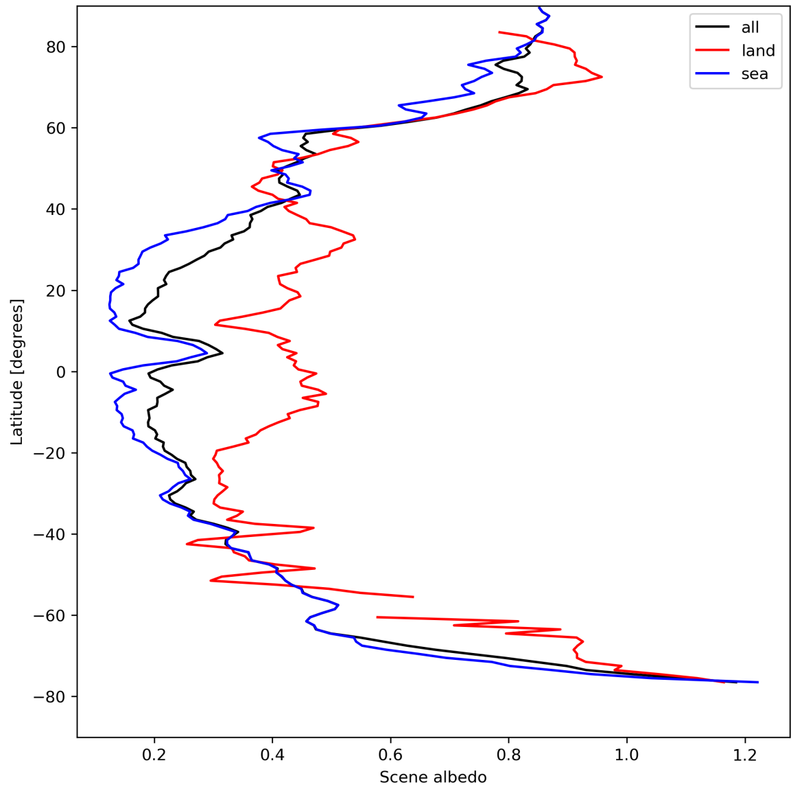
Figure 17: Zonal average of “Scene albedo” for 2024-04-19 to 2024-04-21.
