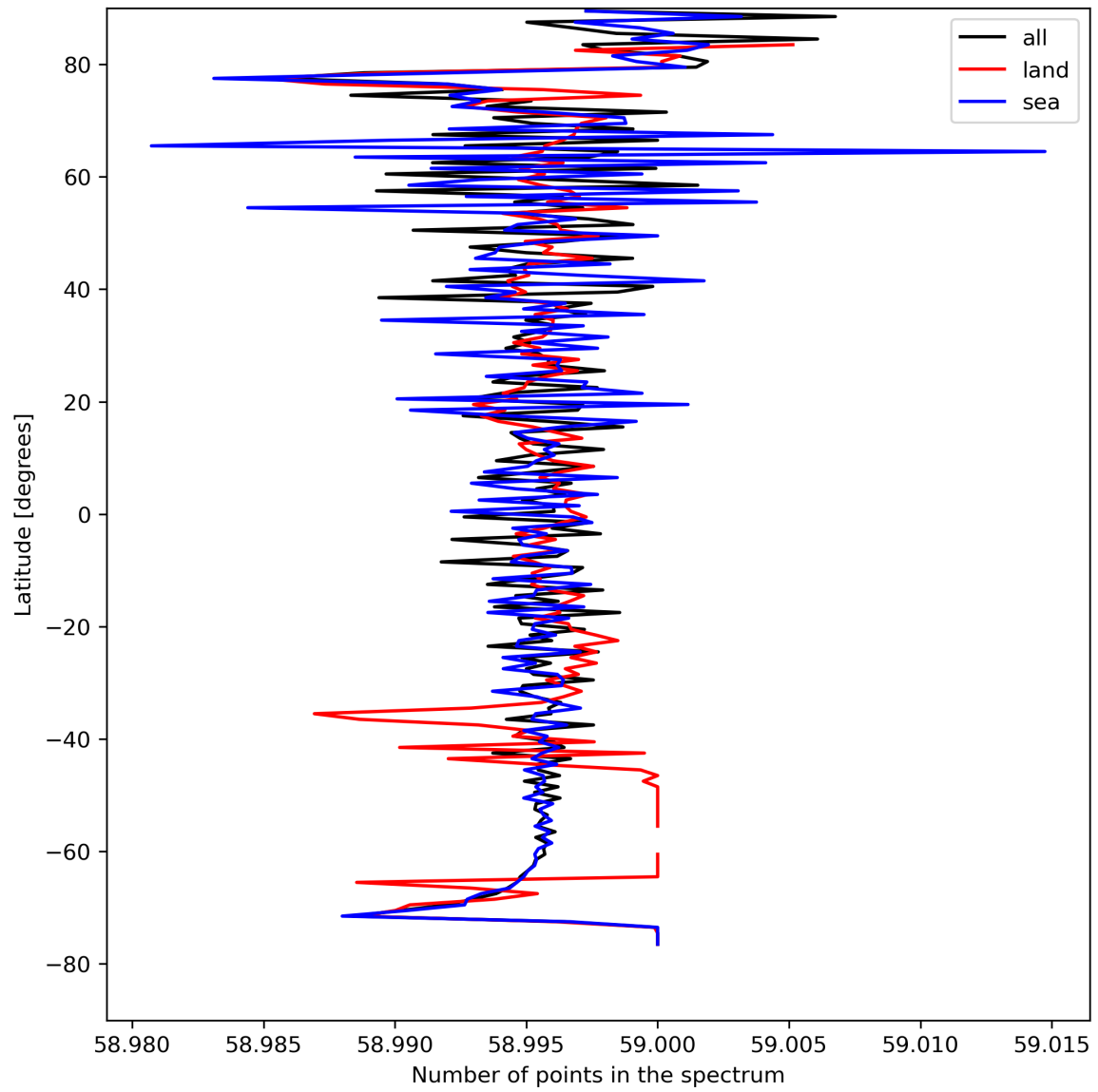
Figure 27: Zonal average of “Number of points in the spectrum” for 2024-04-19 to 2024-04-21.
