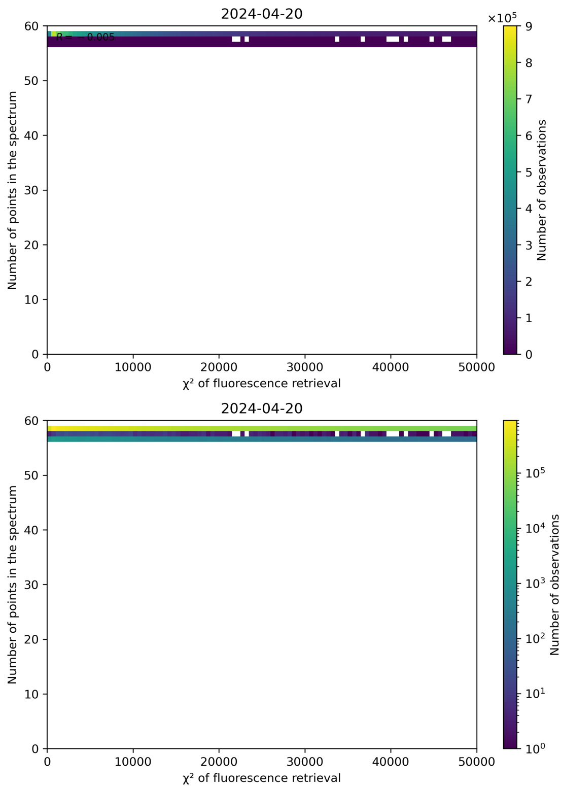
Figure 68: Scatter density plot of " \chi^2 of fluorescence retrieval" against "Number of points in the spectrum" for 2024-04-19 to 2024-04-21.
