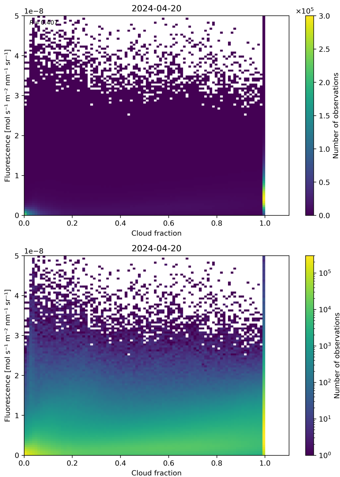
Figure 72: Scatter density plot of “Cloud fraction” against “Fluorescence” for 2024-04-19 to 2024-04-21.
