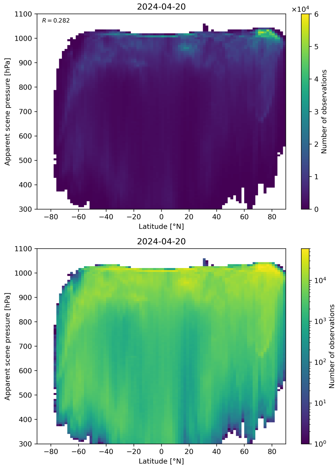
Figure 88: Scatter density plot of “Latitude” against “Apparent scene pressure” for 2024-04-19 to 2024-04-21.
