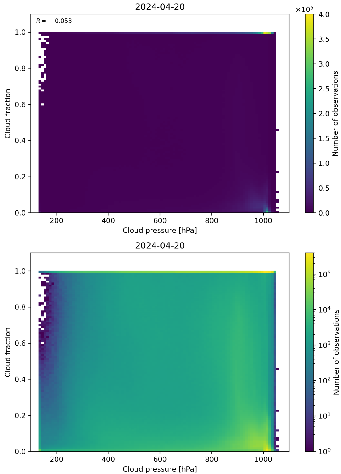
Figure 79: Scatter density plot of “Cloud pressure” against “Cloud fraction” for 2024-04-19 to 2024-04-21.
