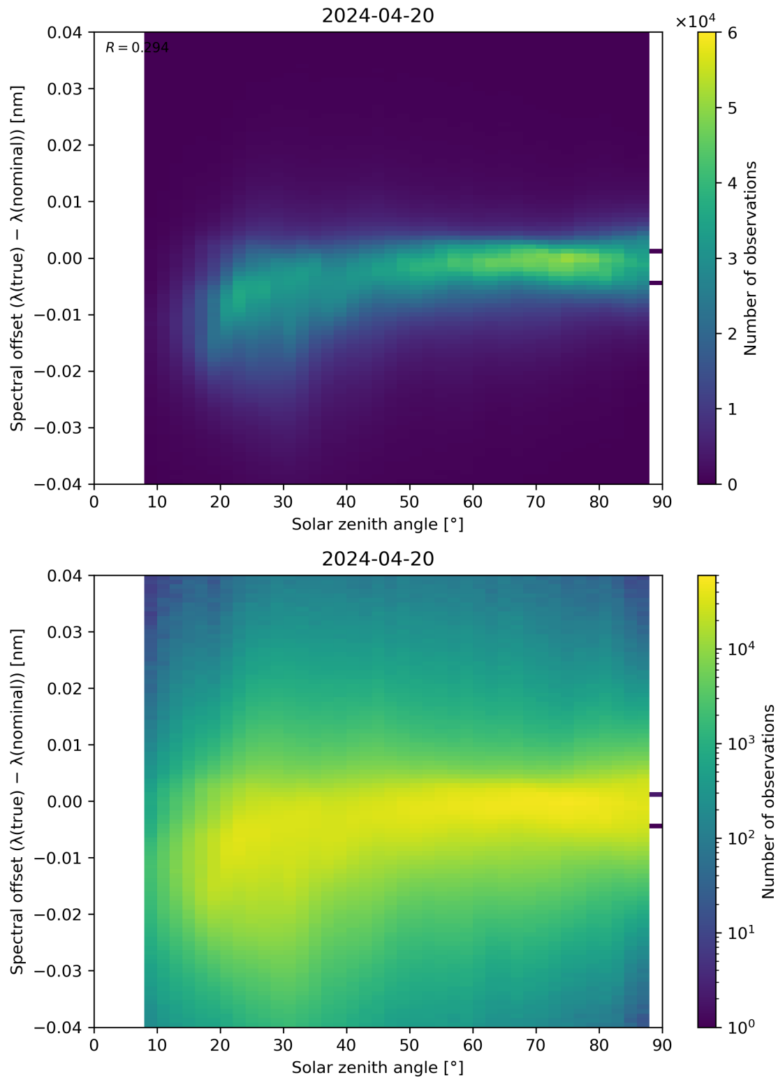
Figure 117: Scatter density plot of “Solar zenith angle” against “Spectral offset ( \lambda(\text{true}) - \lambda(\text{nominal}) )” for 2024-04-19 to 2024-04-21.
