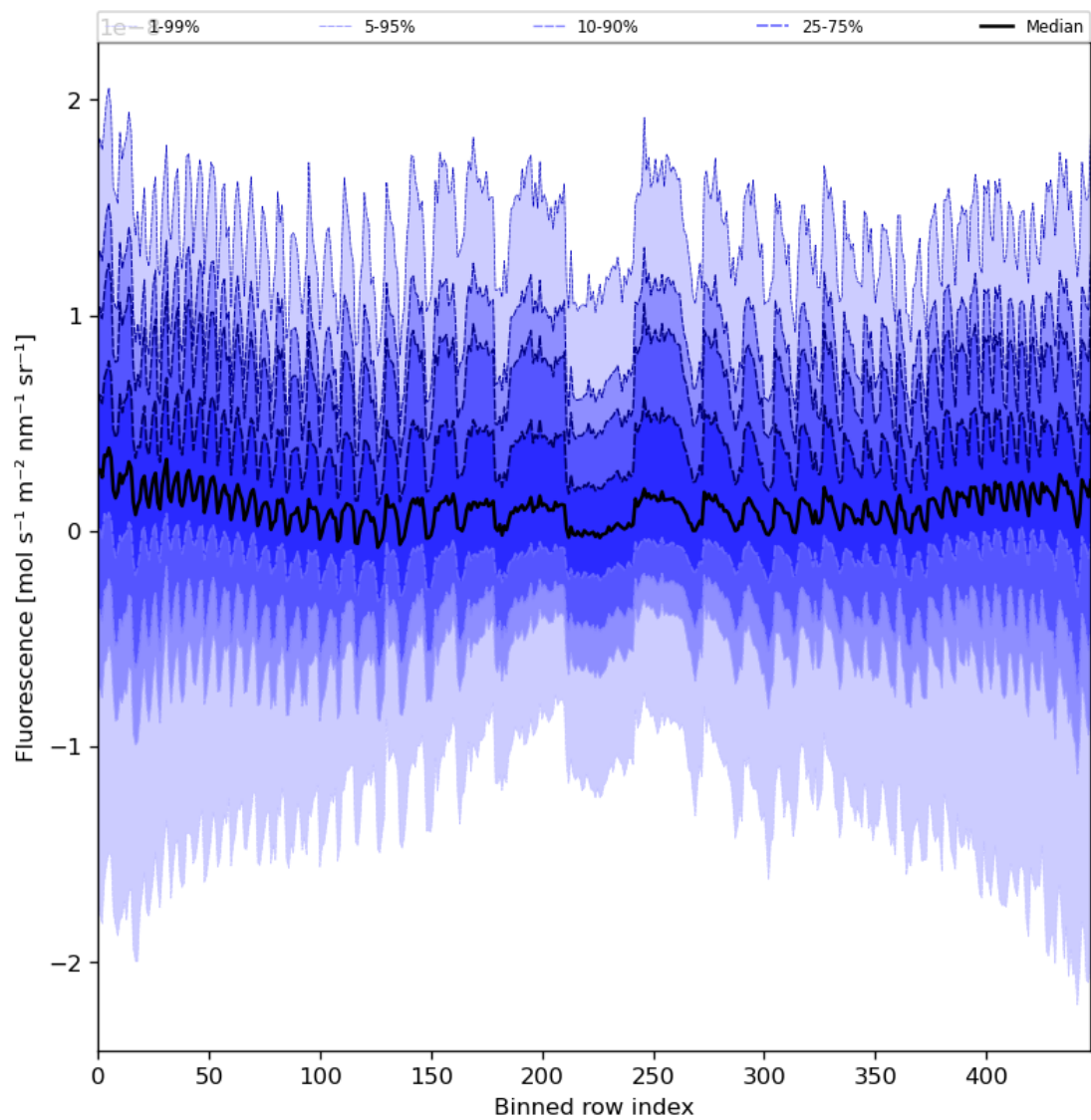
Figure 57: Along track statistics of “Fluorescence” for 2024-04-19 to 2024-04-21
