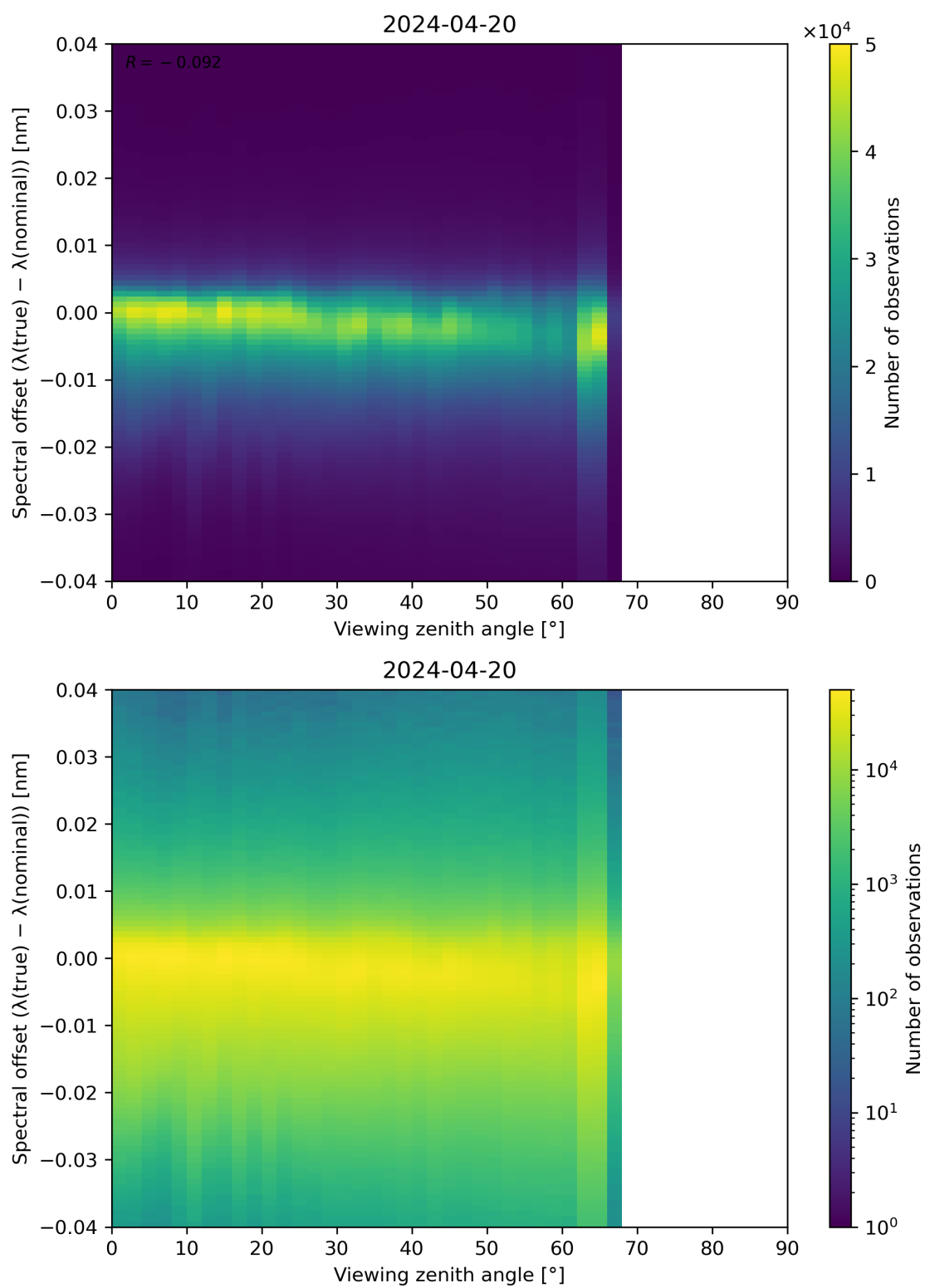
Figure 128: Scatter density plot of “Viewing zenith angle” against “Spectral offset ( \lambda(\text{true}) - \lambda(\text{nominal}) )” for 2024-04-19 to 2024-04-21.
