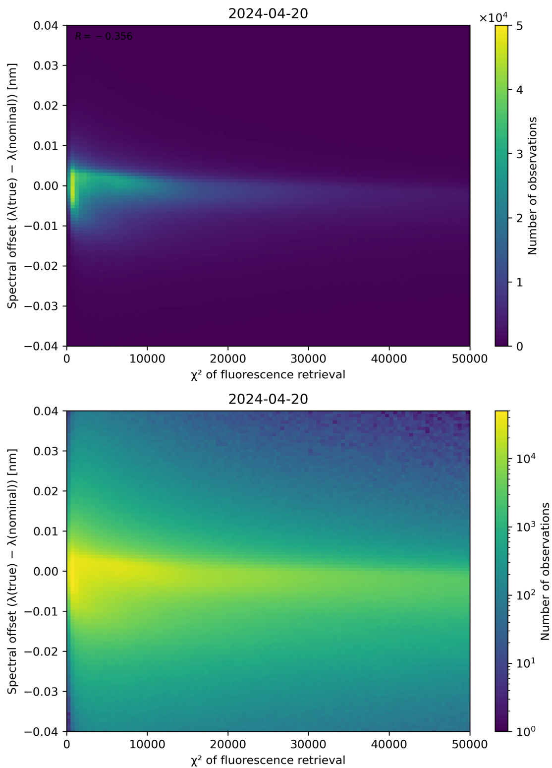
Figure 69: Scatter density plot of " \chi^2 of fluorescence retrieval" against "Spectral offset ( \lambda(\text{true}) - \lambda(\text{nominal}) )" for 2024-04-19 to 2024-04-21.
