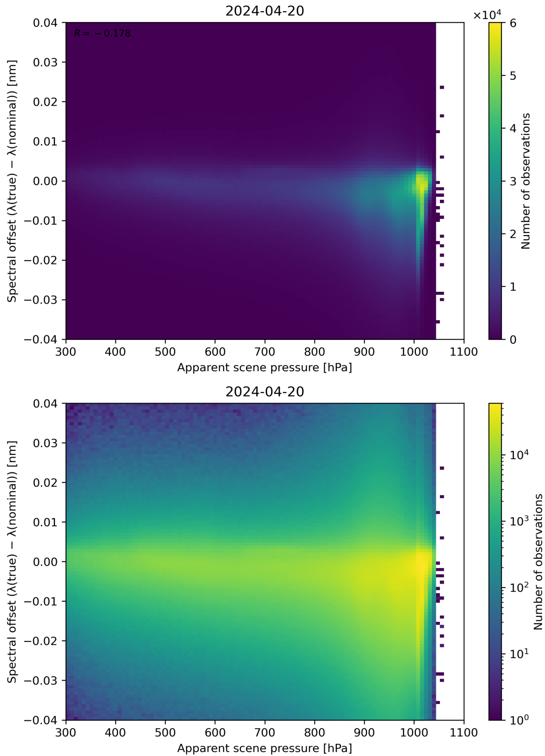
Figure 67: Scatter density plot of “Apparent scene pressure” against “Spectral offset ( \lambda(\text{true}) - \lambda(\text{nominal}) )” for 2024-04-19 to 2024-04-21.
