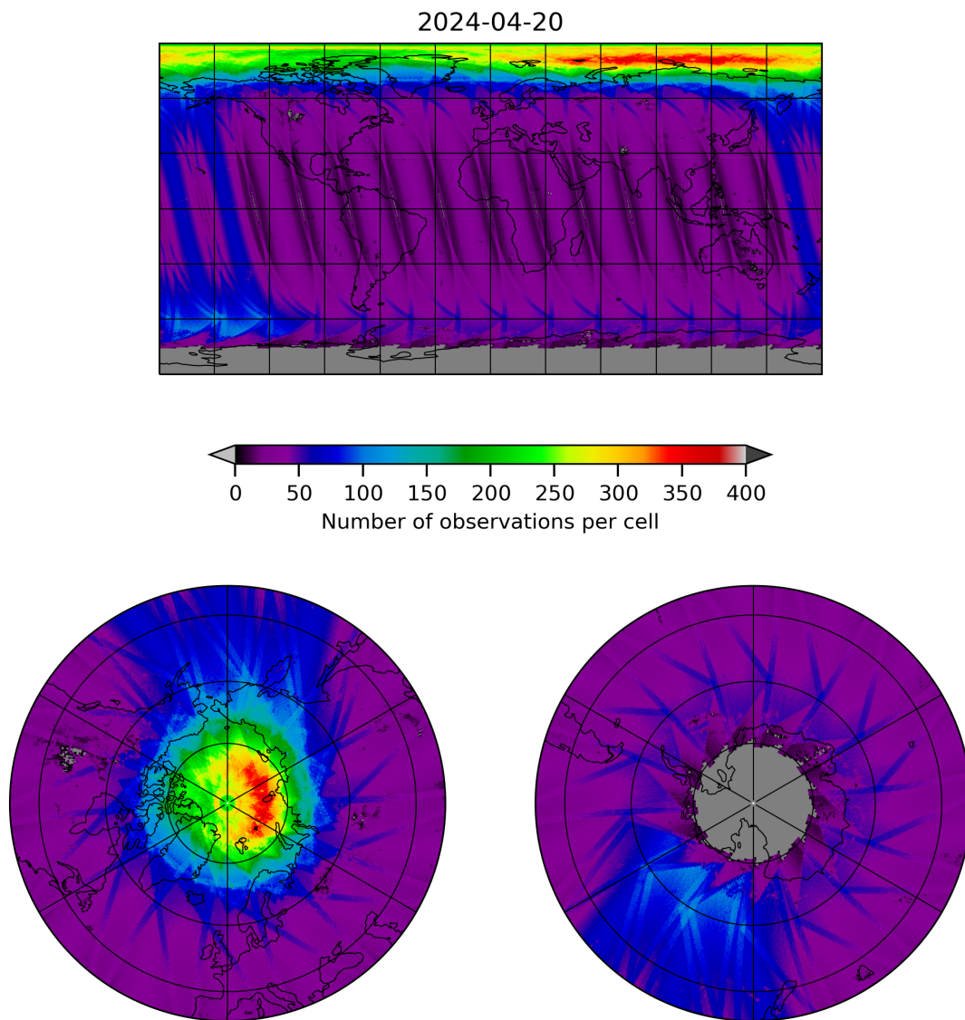
Figure 11: Map of the number of observations for 2024-04-19 to 2024-04-21
