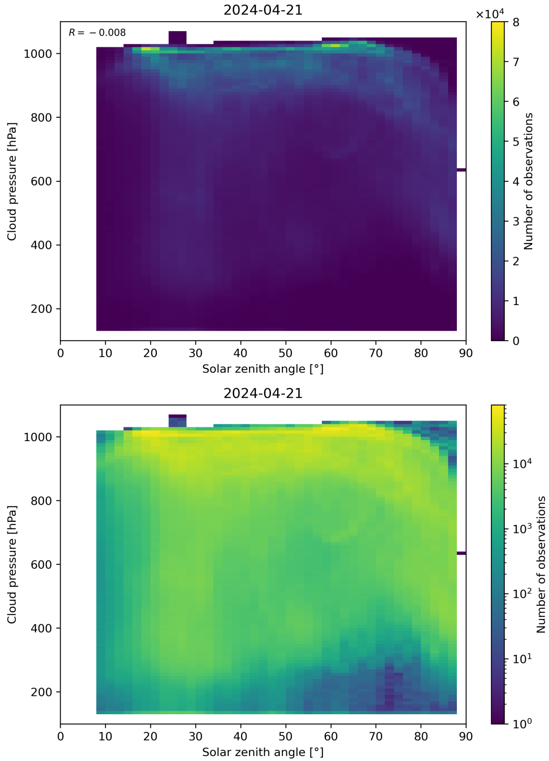
Figure 111: Scatter density plot of “Solar zenith angle” against “Cloud pressure” for 2024-04-21 to 2024-04-22.
