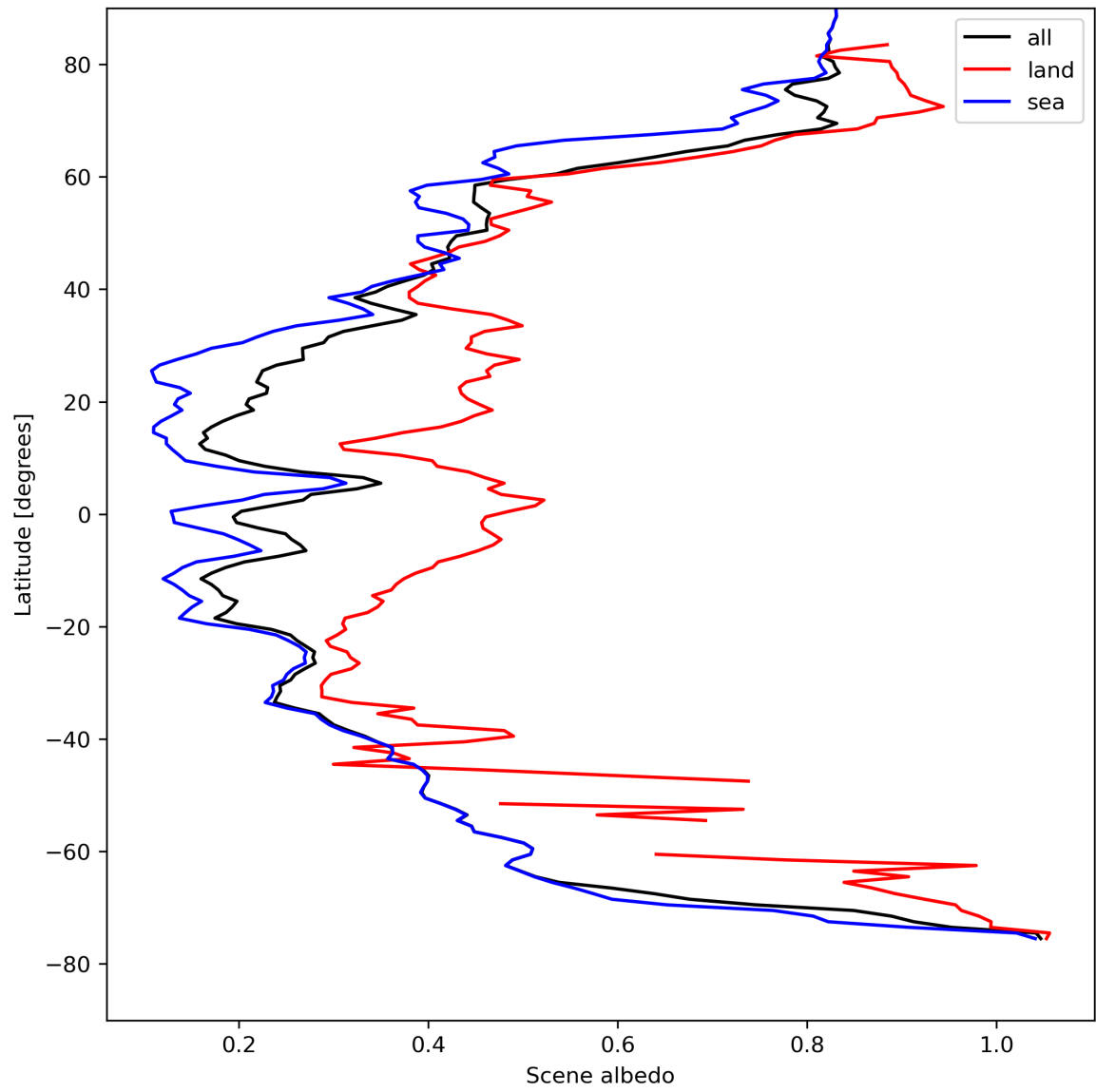
Figure 17: Zonal average of “Scene albedo” for 2024-04-21 to 2024-04-22.
