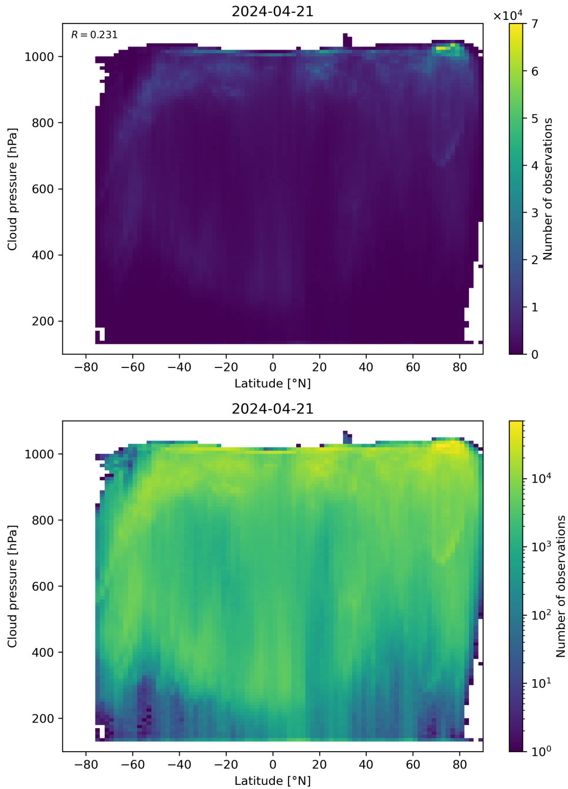
Figure 91: Scatter density plot of “Latitude” against “Cloud pressure” for 2024-04-21 to 2024-04-22.
