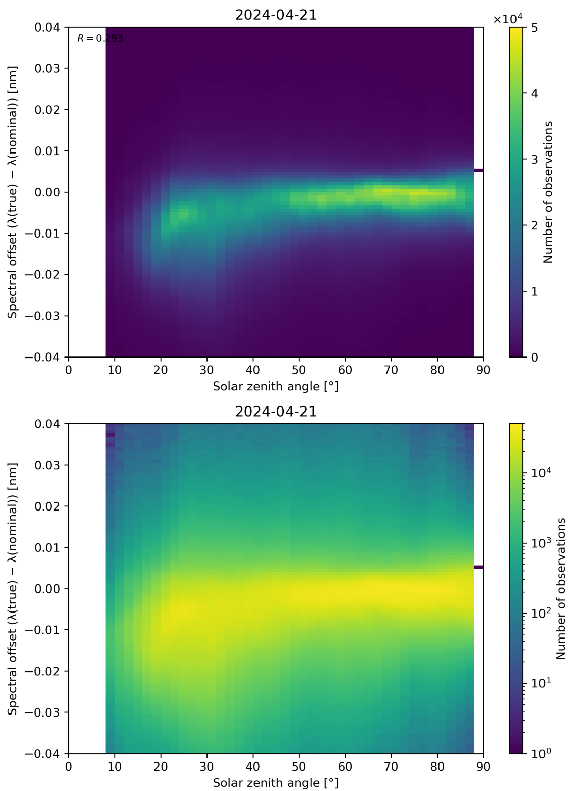
Figure 117: Scatter density plot of “Solar zenith angle” against “Spectral offset ( \lambda(\text{true}) - \lambda(\text{nominal}) )” for 2024-04-21 to 2024-04-22.
