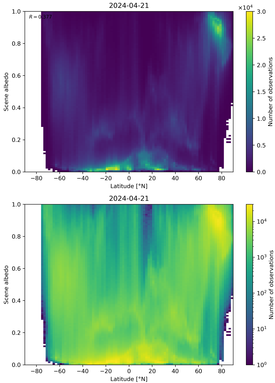
Figure 95: Scatter density plot of “Latitude” against “Scene albedo” for 2024-04-21 to 2024-04-22.
