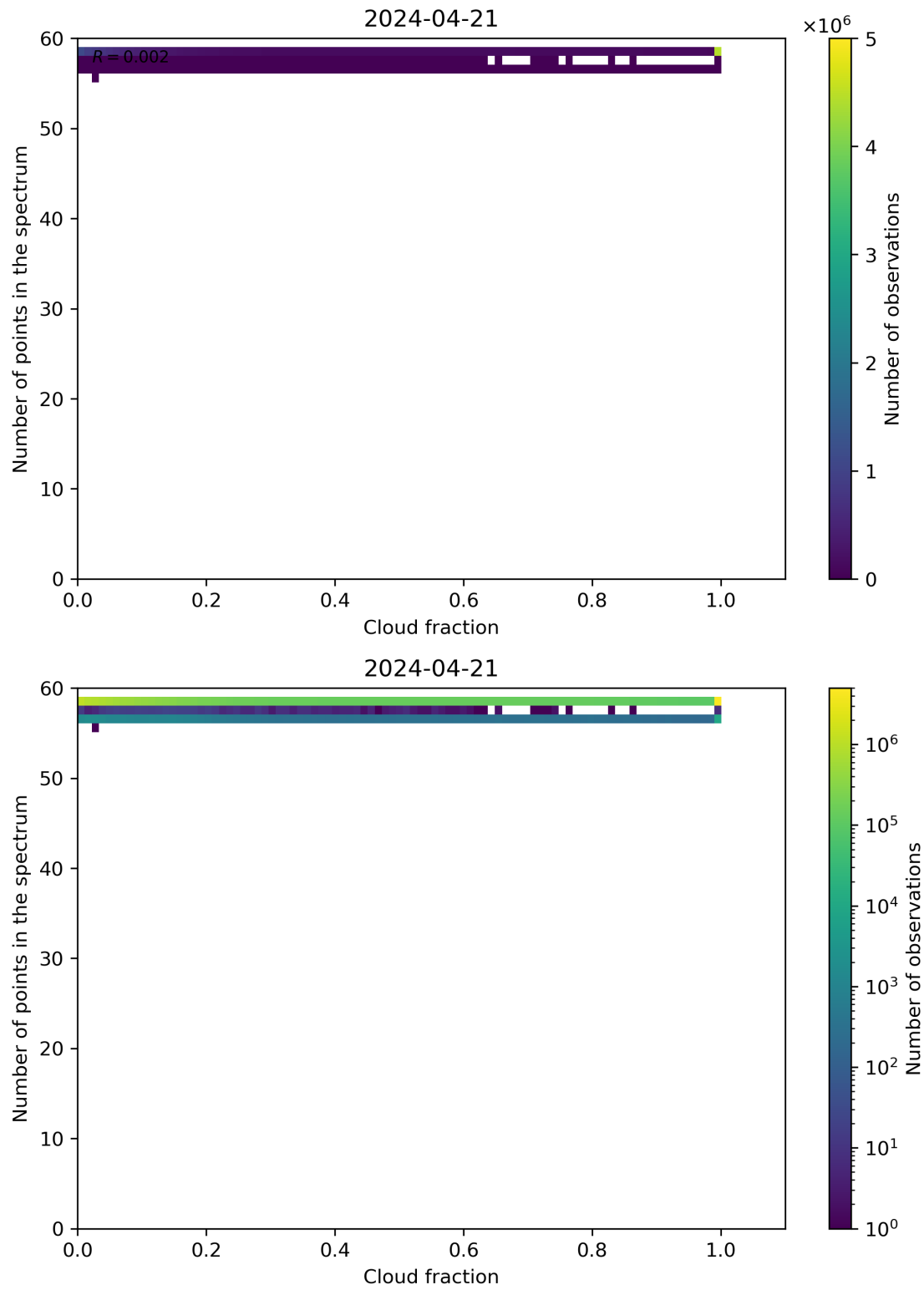
Figure 74: Scatter density plot of “Cloud fraction” against “Number of points in the spectrum” for 2024-04-21 to 2024-04-22.
