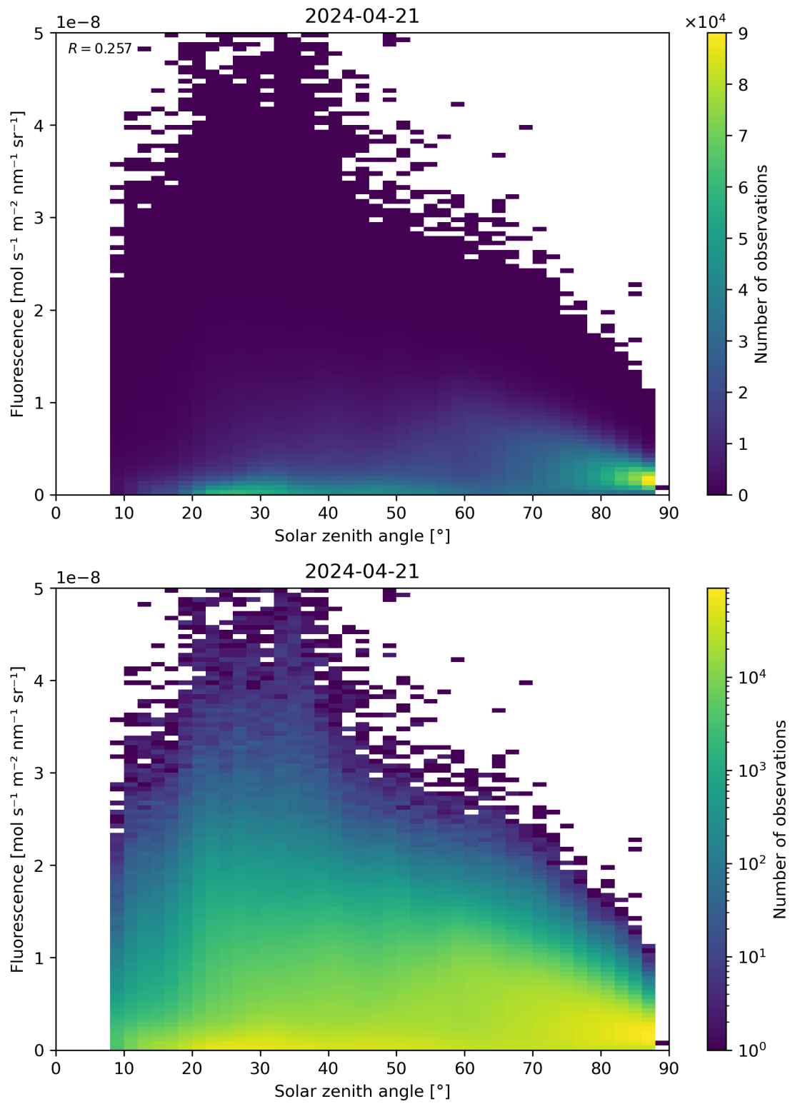
Figure 112: Scatter density plot of “Solar zenith angle” against “Fluorescence” for 2024-04-21 to 2024-04-22.
