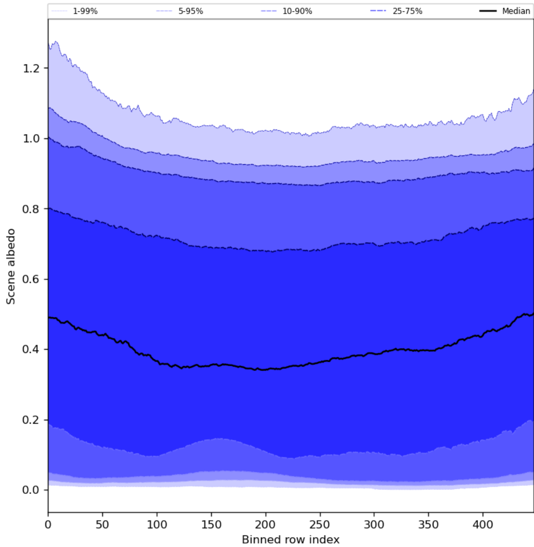
Figure 51: Along track statistics of “Scene albedo” for 2024-04-21 to 2024-04-22
