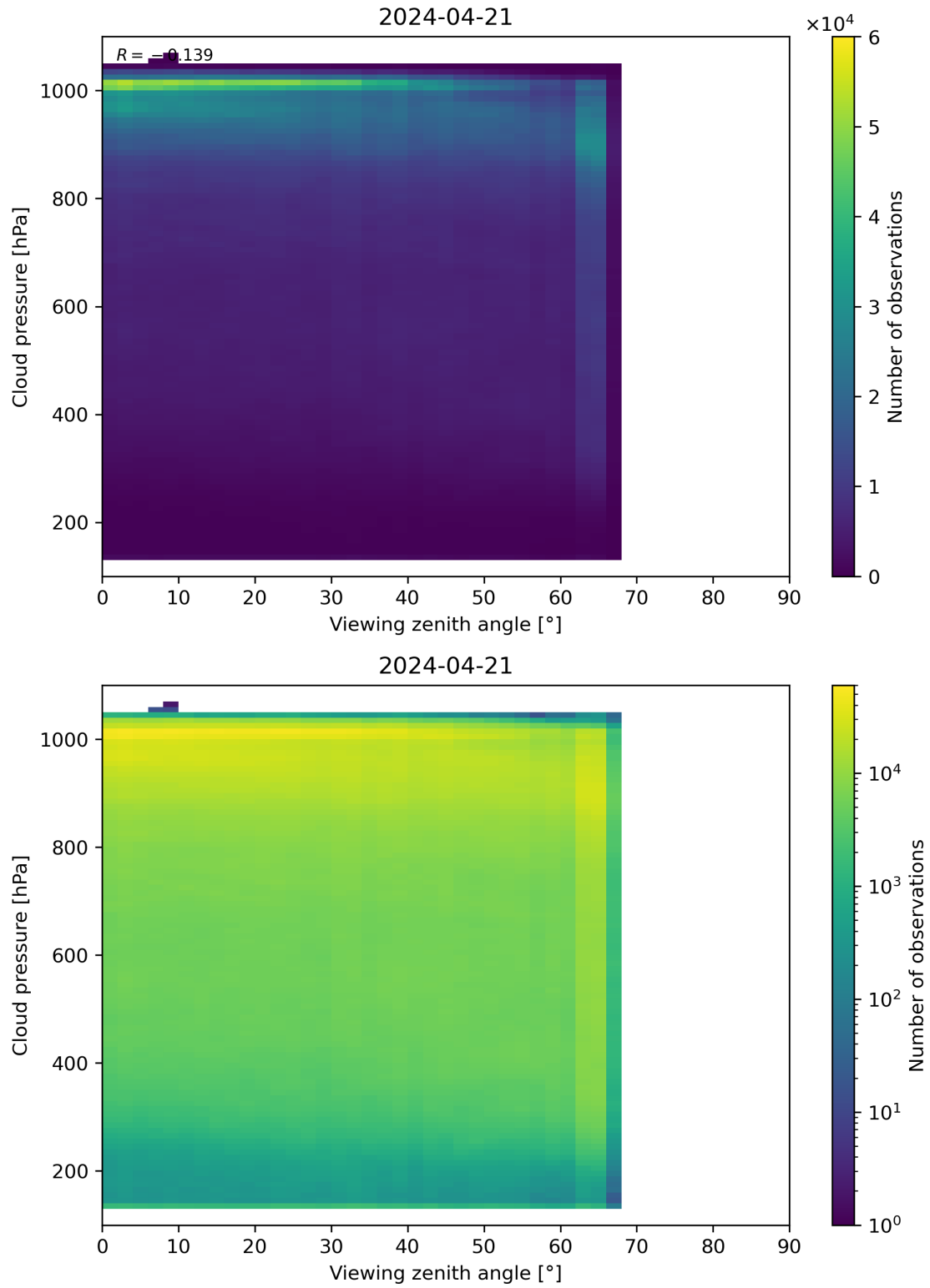
Figure 121: Scatter density plot of “Viewing zenith angle” against “Cloud pressure” for 2024-04-21 to 2024-04-22.
