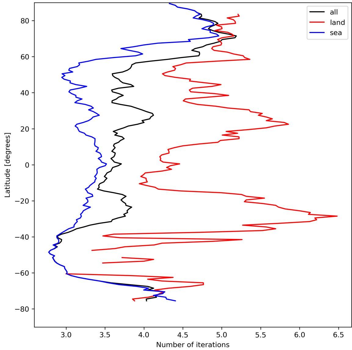
Figure 22: Zonal average of “Number of iterations” for 2024-04-21 to 2024-04-22.
