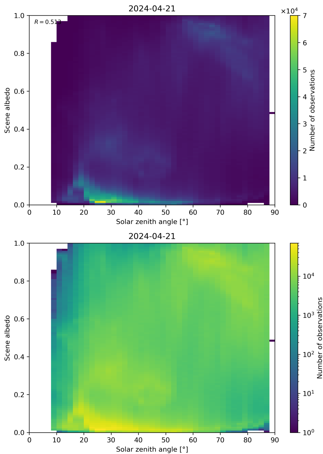
Figure 116: Scatter density plot of “Solar zenith angle” against “Scene albedo” for 2024-04-21 to 2024-04-22.
