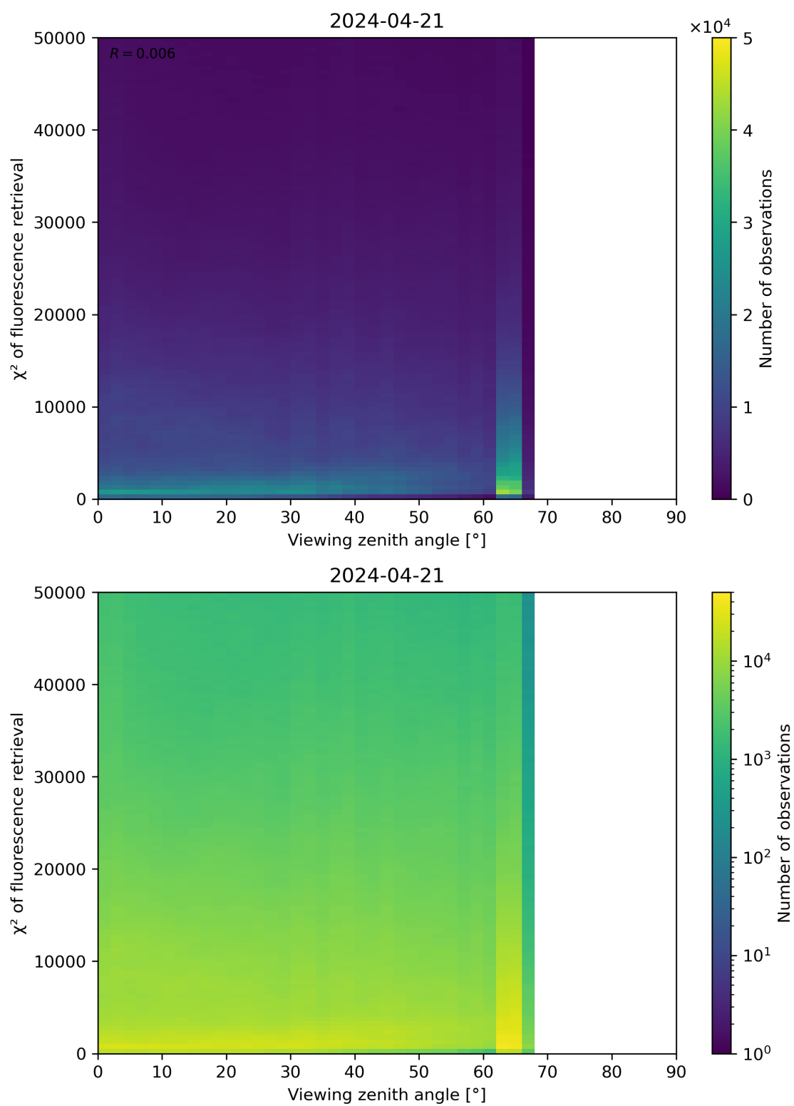
Figure 119: Scatter density plot of “Viewing zenith angle” against “ \chi^2 of fluorescence retrieval” for 2024-04-21 to 2024-04-22.
