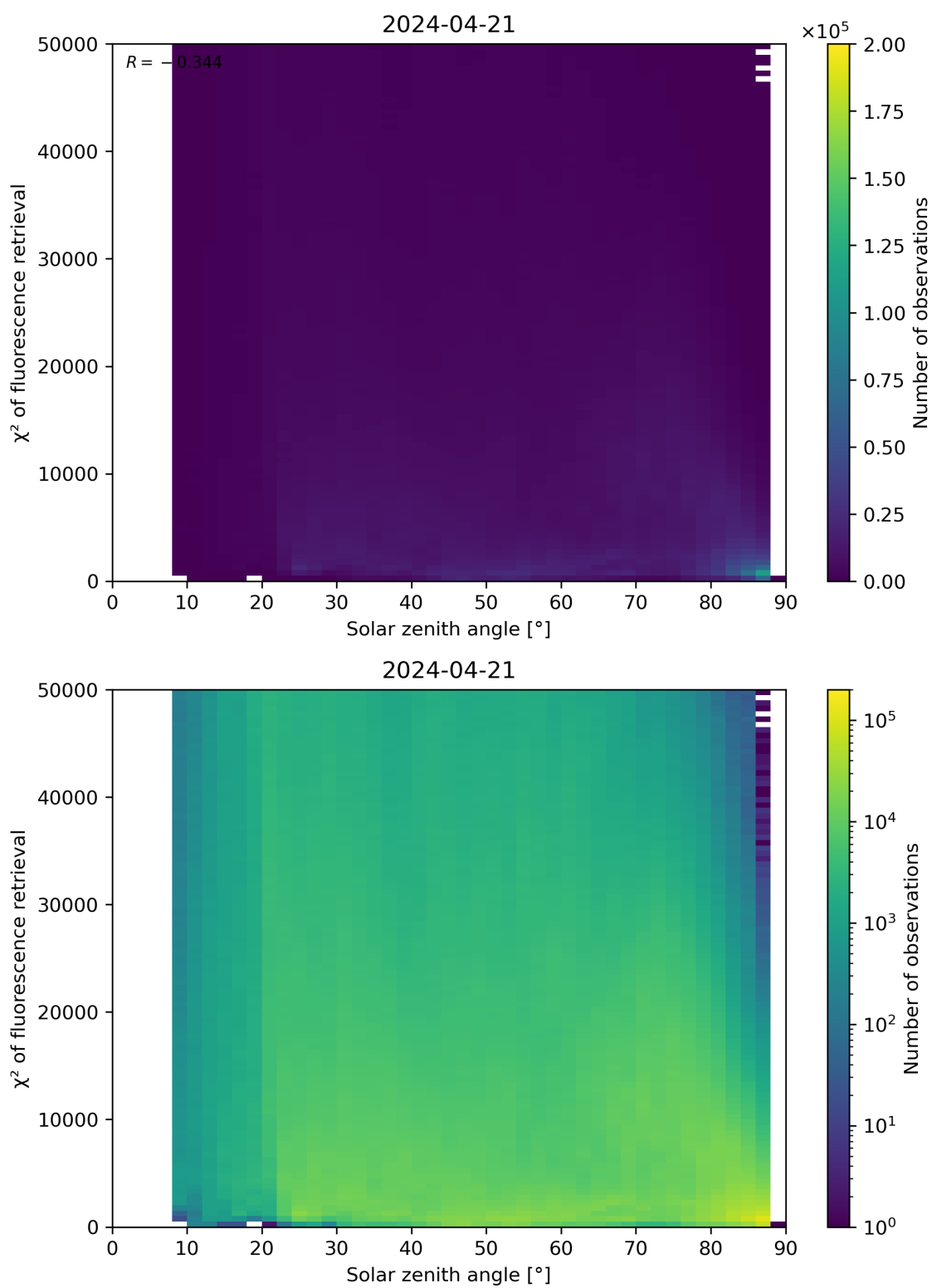
Figure 109: Scatter density plot of “Solar zenith angle” against “ \chi^2 of fluorescence retrieval” for 2024-04-21 to 2024-04-22.
