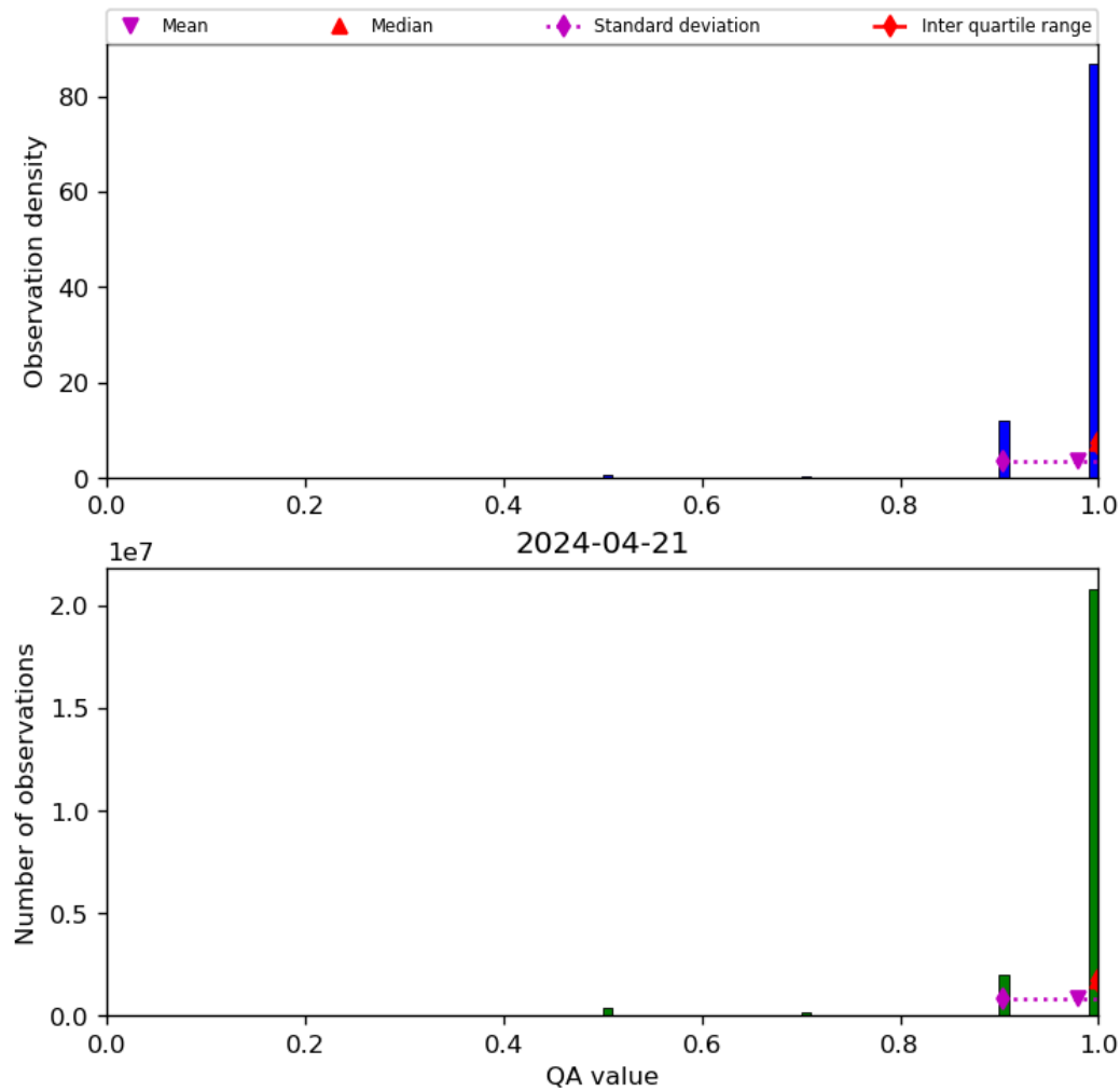
Figure 29: Histogram of “QA value” for 2024-04-21 to 2024-04-22
