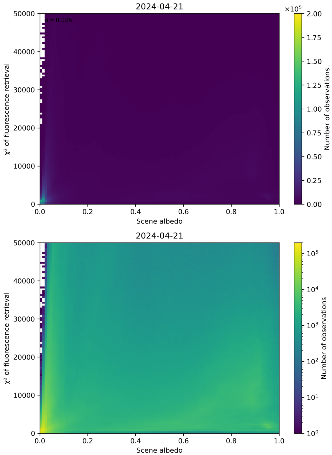
Figure 103: Scatter density plot of “Scene albedo” against “ \chi^2 of fluorescence retrieval” for 2024-04-21 to 2024-04-22.
