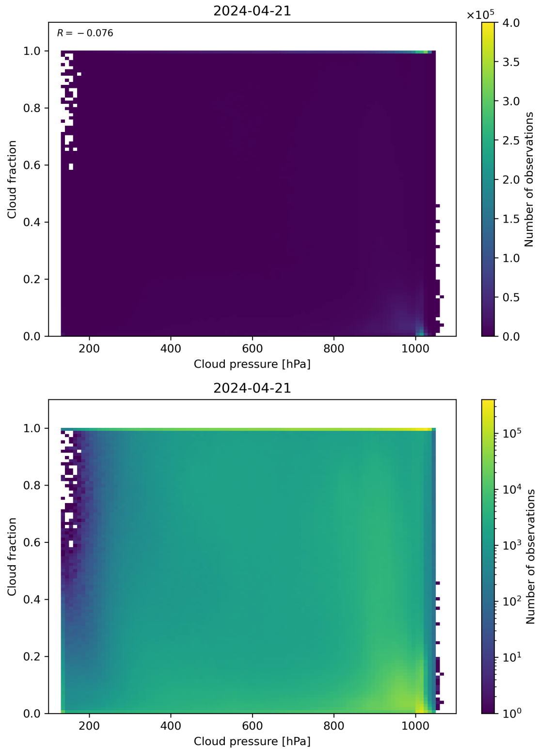
Figure 79: Scatter density plot of “Cloud pressure” against “Cloud fraction” for 2024-04-21 to 2024-04-22.
