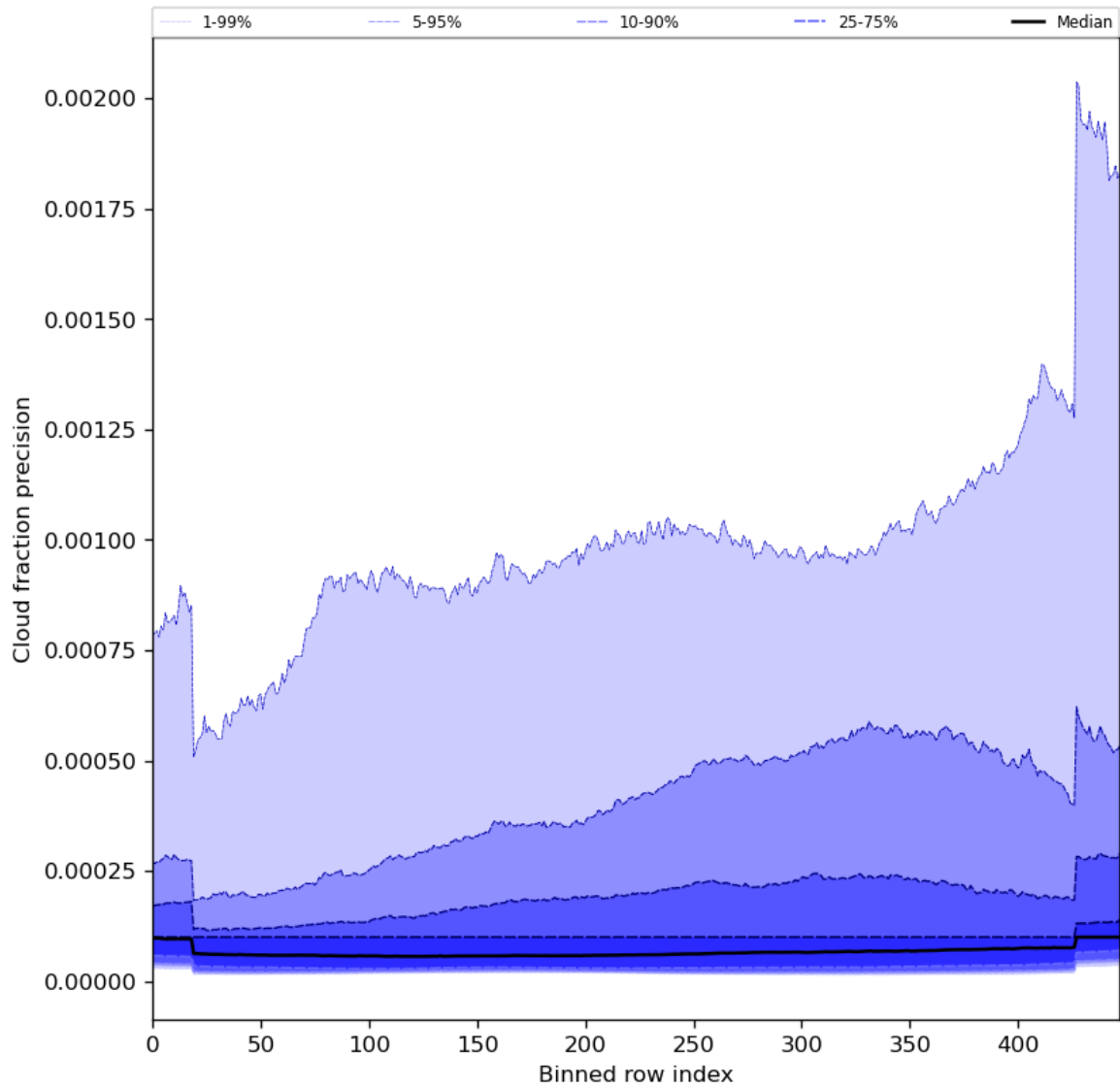
Figure 50: Along track statistics of “Cloud fraction precision” for 2024-04-21 to 2024-04-22
