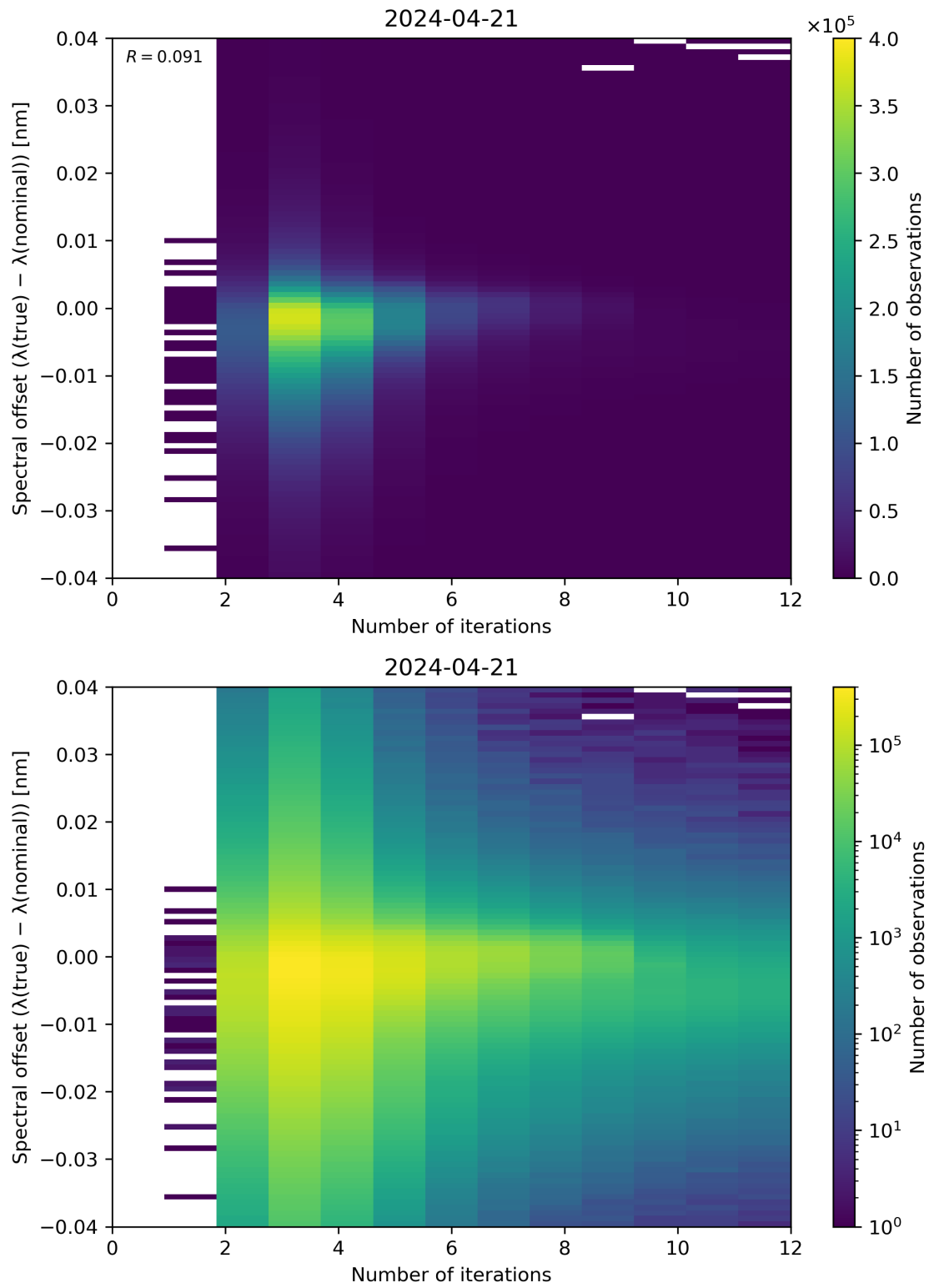
Figure 100: Scatter density plot of “Number of iterations” against “Spectral offset ( \lambda(\text{true}) - \lambda(\text{nominal}) )” for 2024-04-21 to 2024-04-22.
