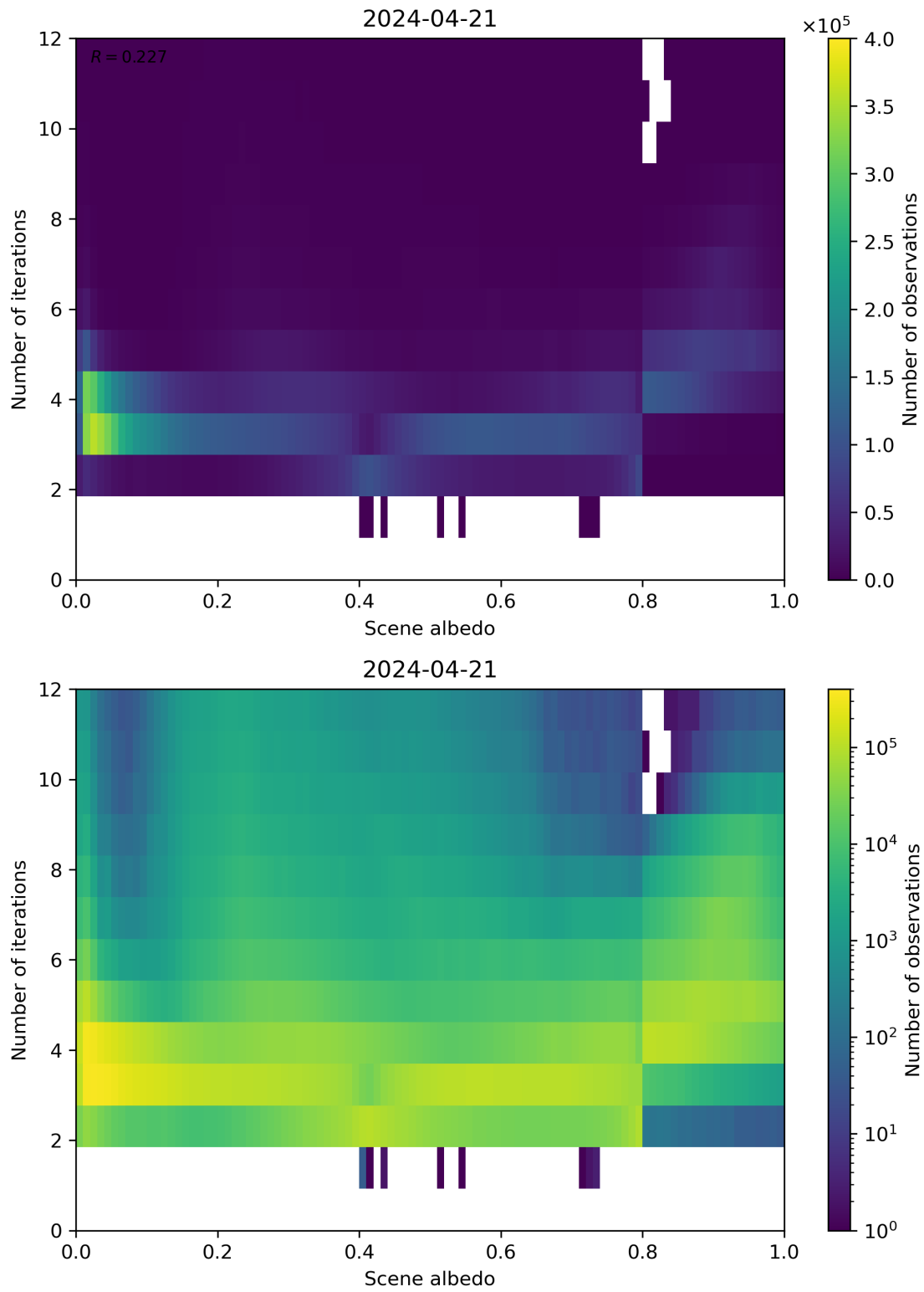
Figure 105: Scatter density plot of “Scene albedo” against “Number of iterations” for 2024-04-21 to 2024-04-22.
