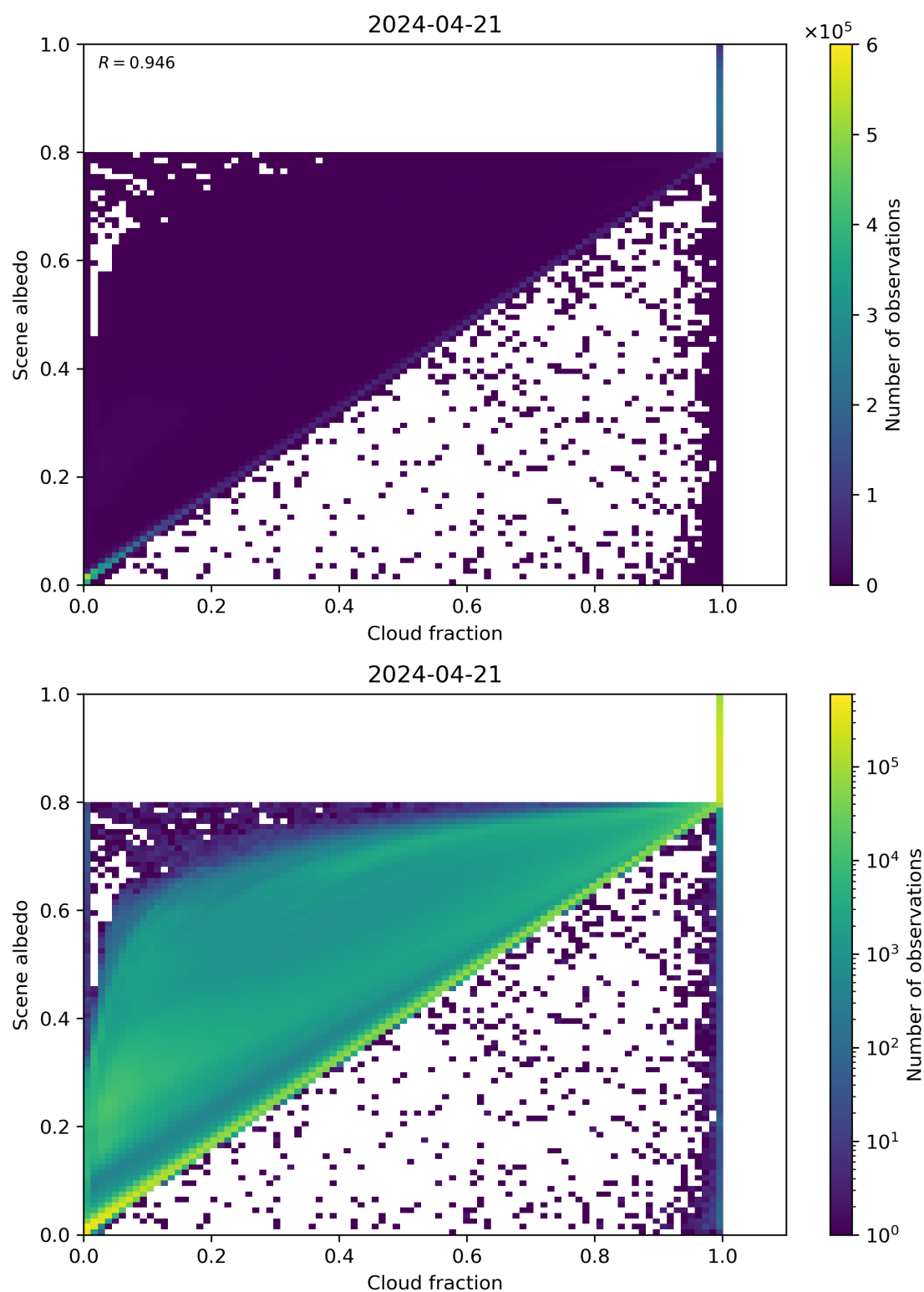
Figure 75: Scatter density plot of “Cloud fraction” against “Scene albedo” for 2024-04-21 to 2024-04-22.
