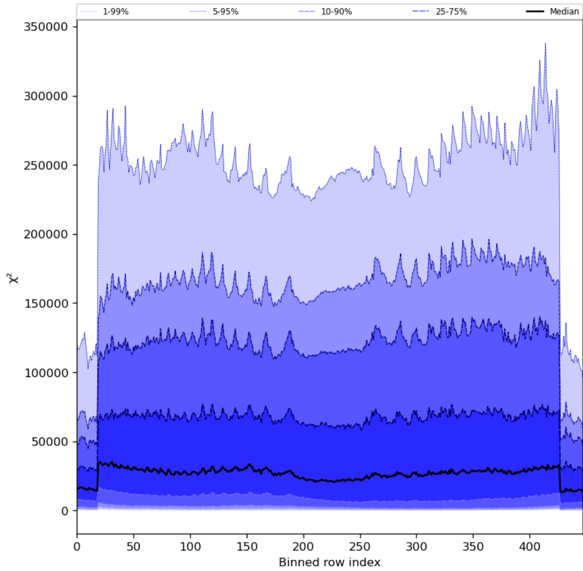
Figure 55: Along track statistics of “ \chi^2 ” for 2024-04-21 to 2024-04-22
