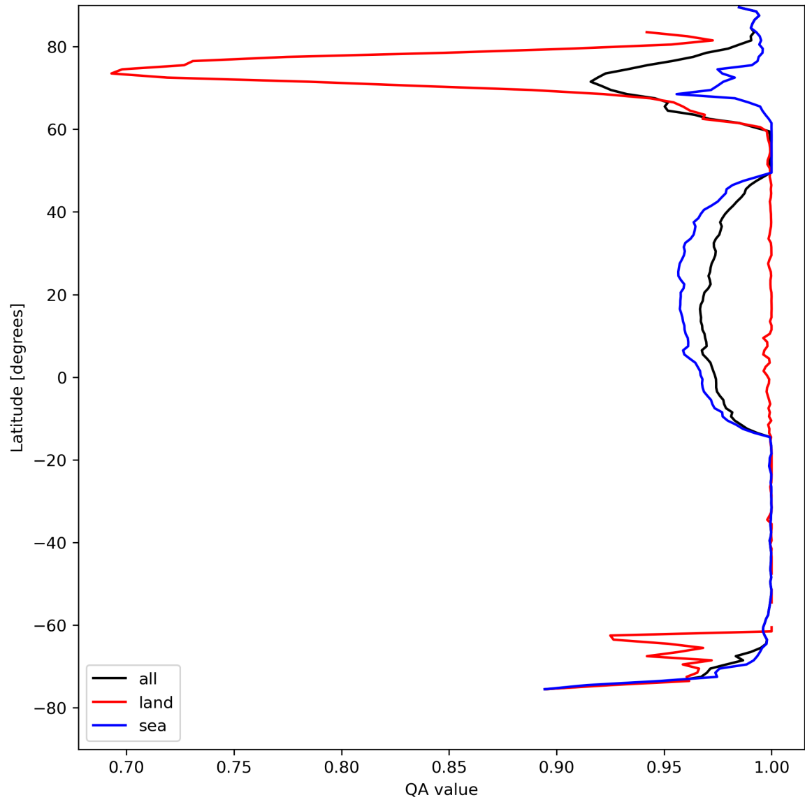
Figure 12: Zonal average of “QA value” for 2024-04-21 to 2024-04-22.
