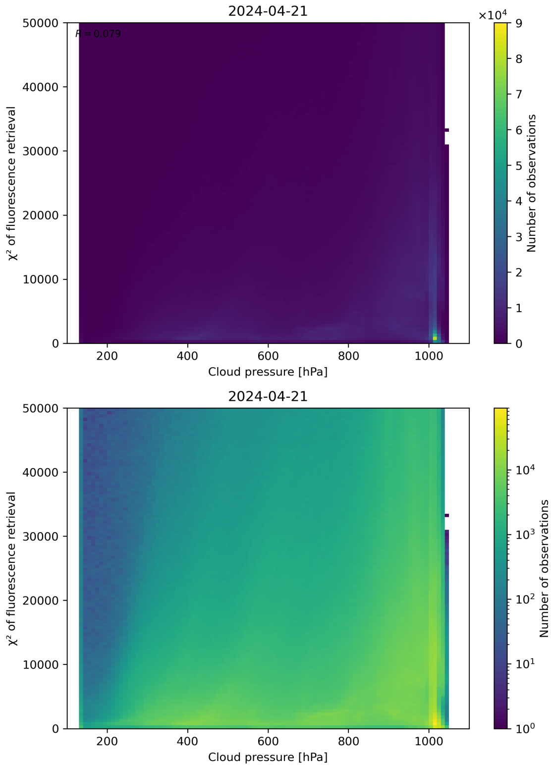
Figure 78: Scatter density plot of “Cloud pressure” against “ \chi^2 of fluorescence retrieval” for 2024-04-21 to 2024-04-22.
