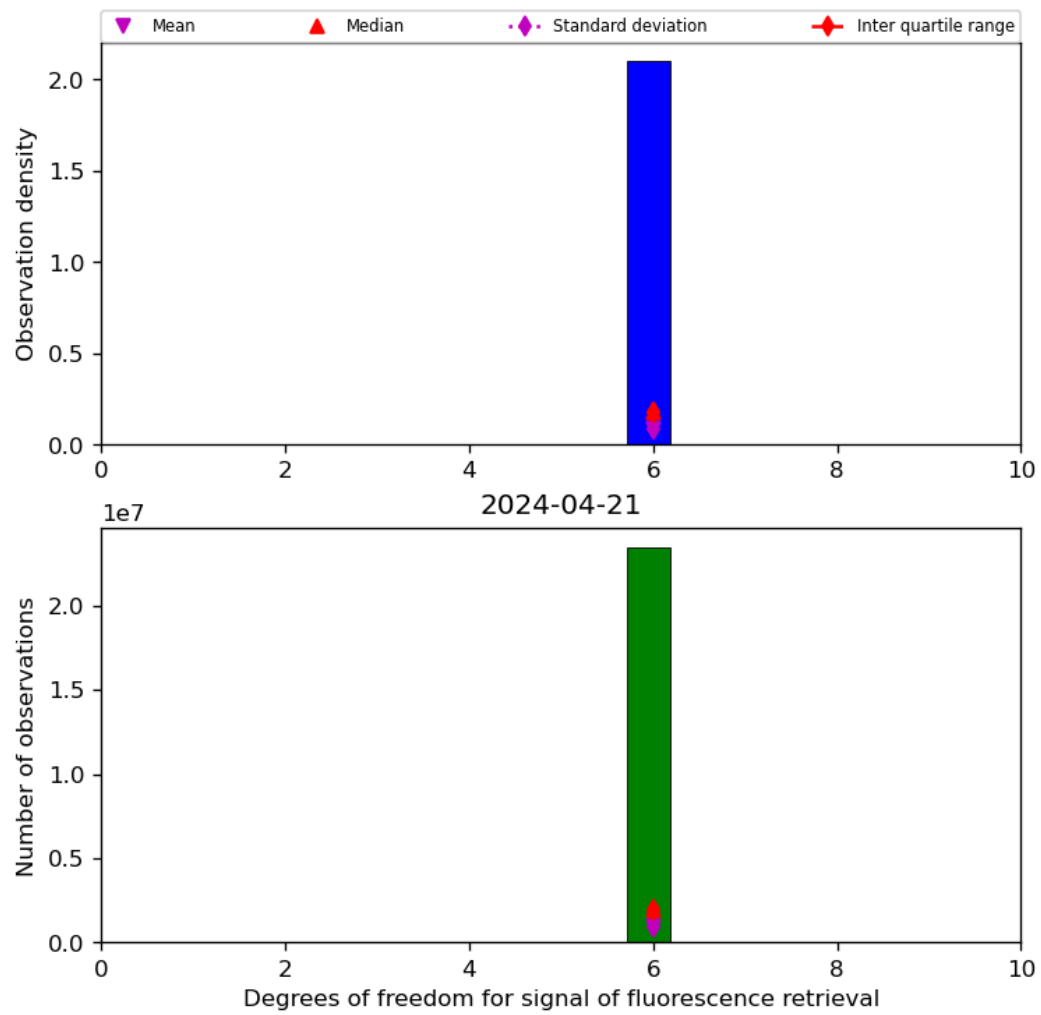
Figure 43: Histogram of “Degrees of freedom for signal of fluorescence retrieval” for 2024-04-21 to 2024-04-22
