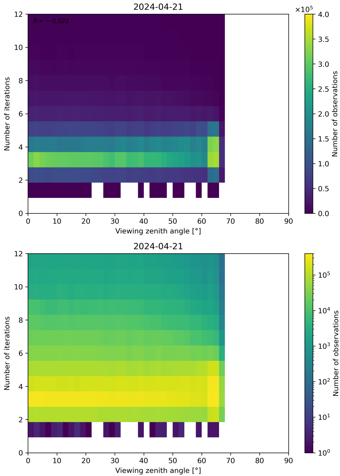
Figure 124: Scatter density plot of “Viewing zenith angle” against “Number of iterations” for 2024-04-21 to 2024-04-22.
