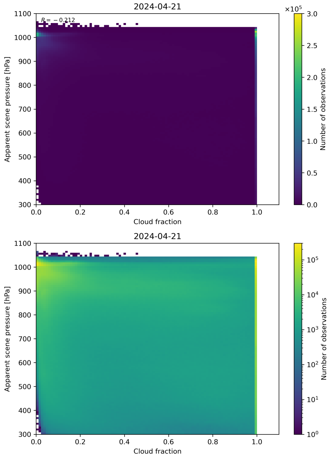
Figure 70: Scatter density plot of “Cloud fraction” against “Apparent scene pressure” for 2024-04-21 to 2024-04-22.
