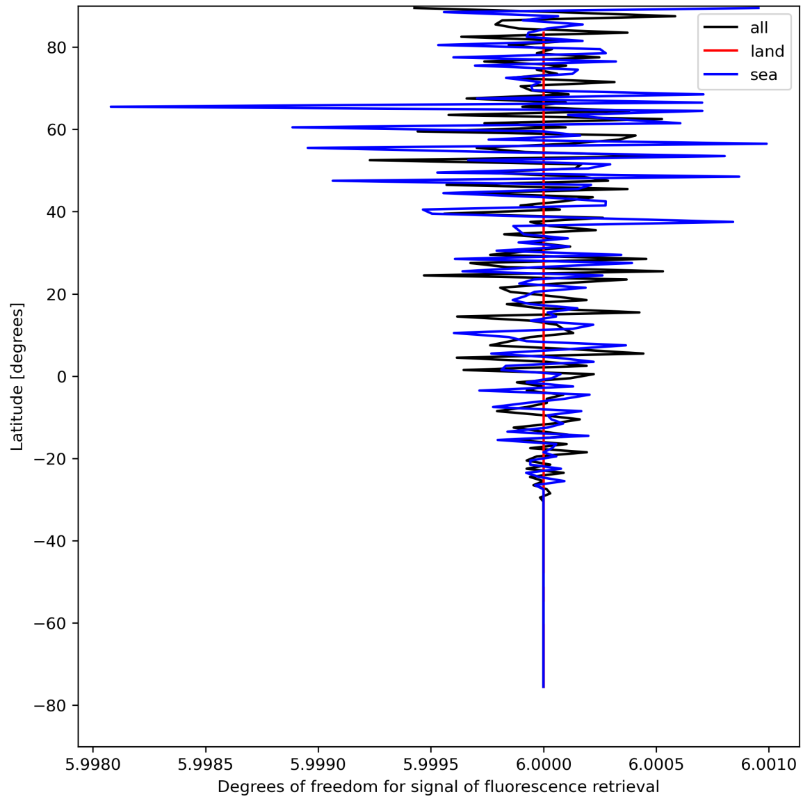
Figure 26: Zonal average of “Degrees of freedom for signal of fluorescence retrieval” for 2024-04-21 to 2024-04-22.
