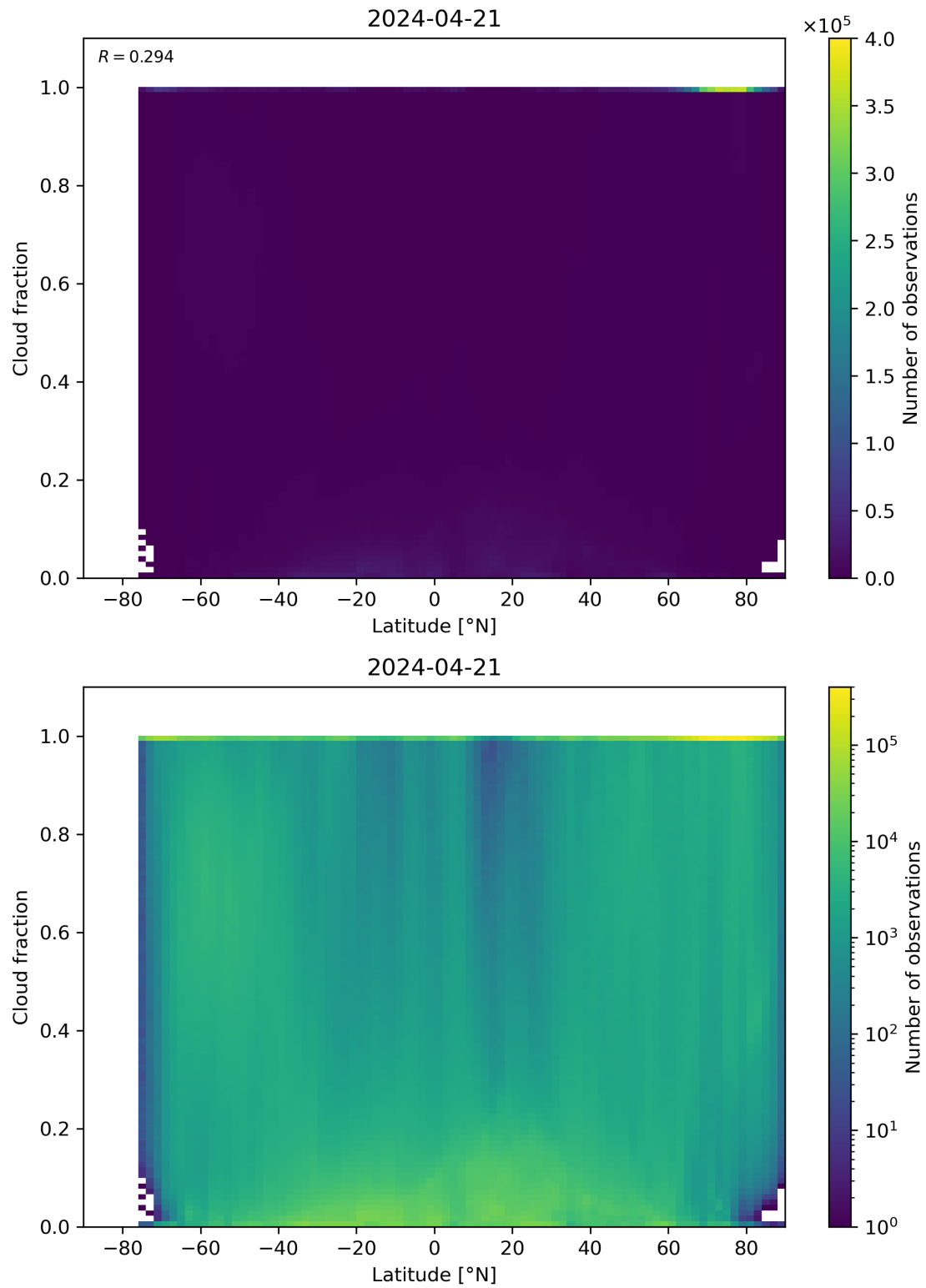
Figure 90: Scatter density plot of “Latitude” against “Cloud fraction” for 2024-04-21 to 2024-04-22.
