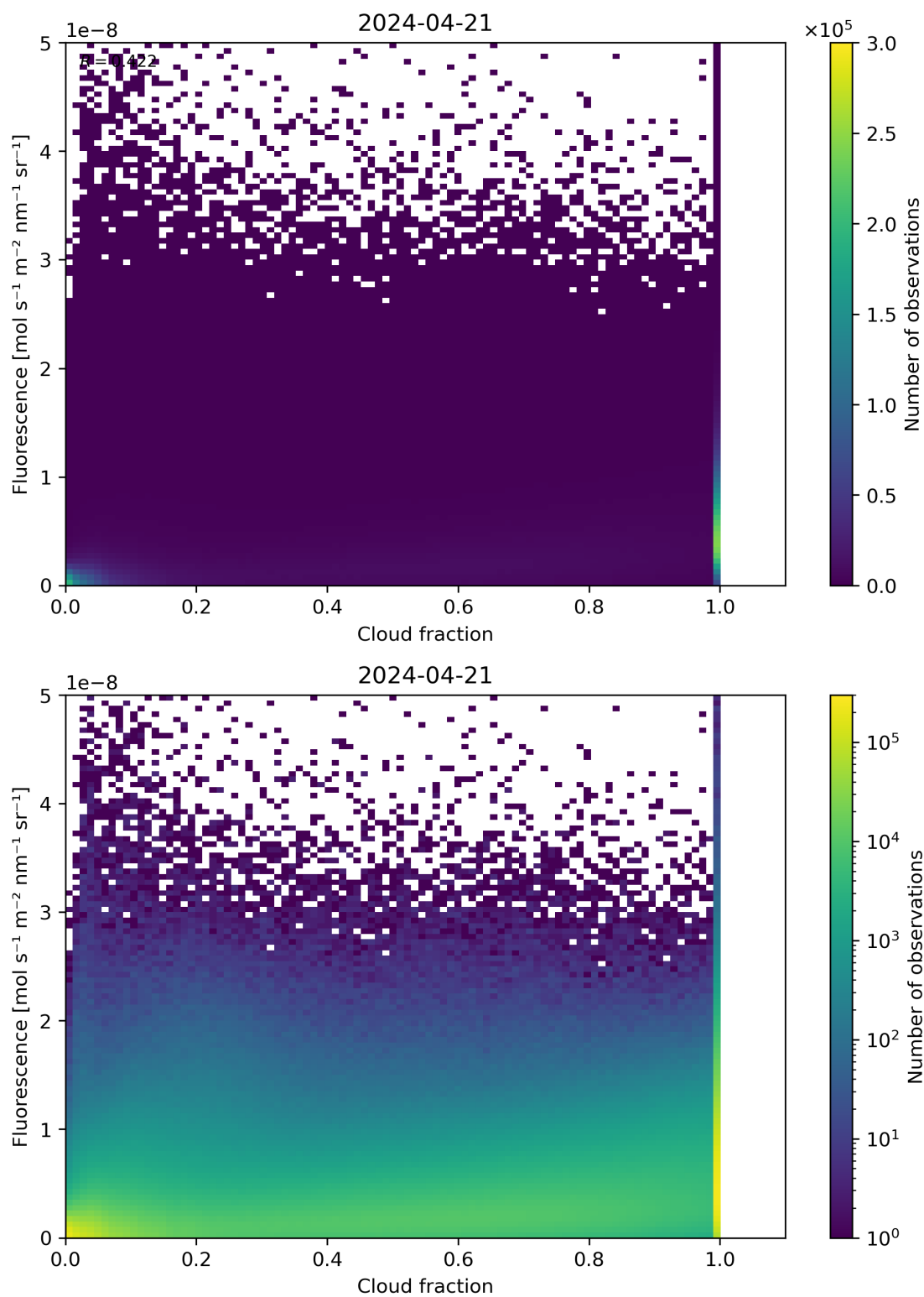
Figure 72: Scatter density plot of “Cloud fraction” against “Fluorescence” for 2024-04-21 to 2024-04-22.
