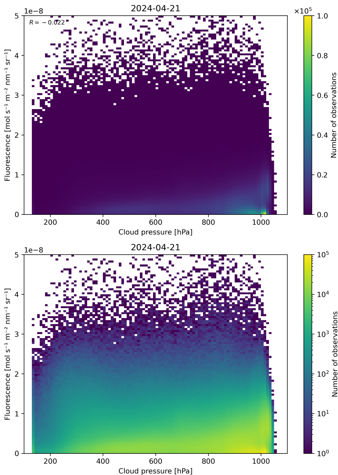
Figure 80: Scatter density plot of “Cloud pressure” against “Fluorescence” for 2024-04-21 to 2024-04-22.
