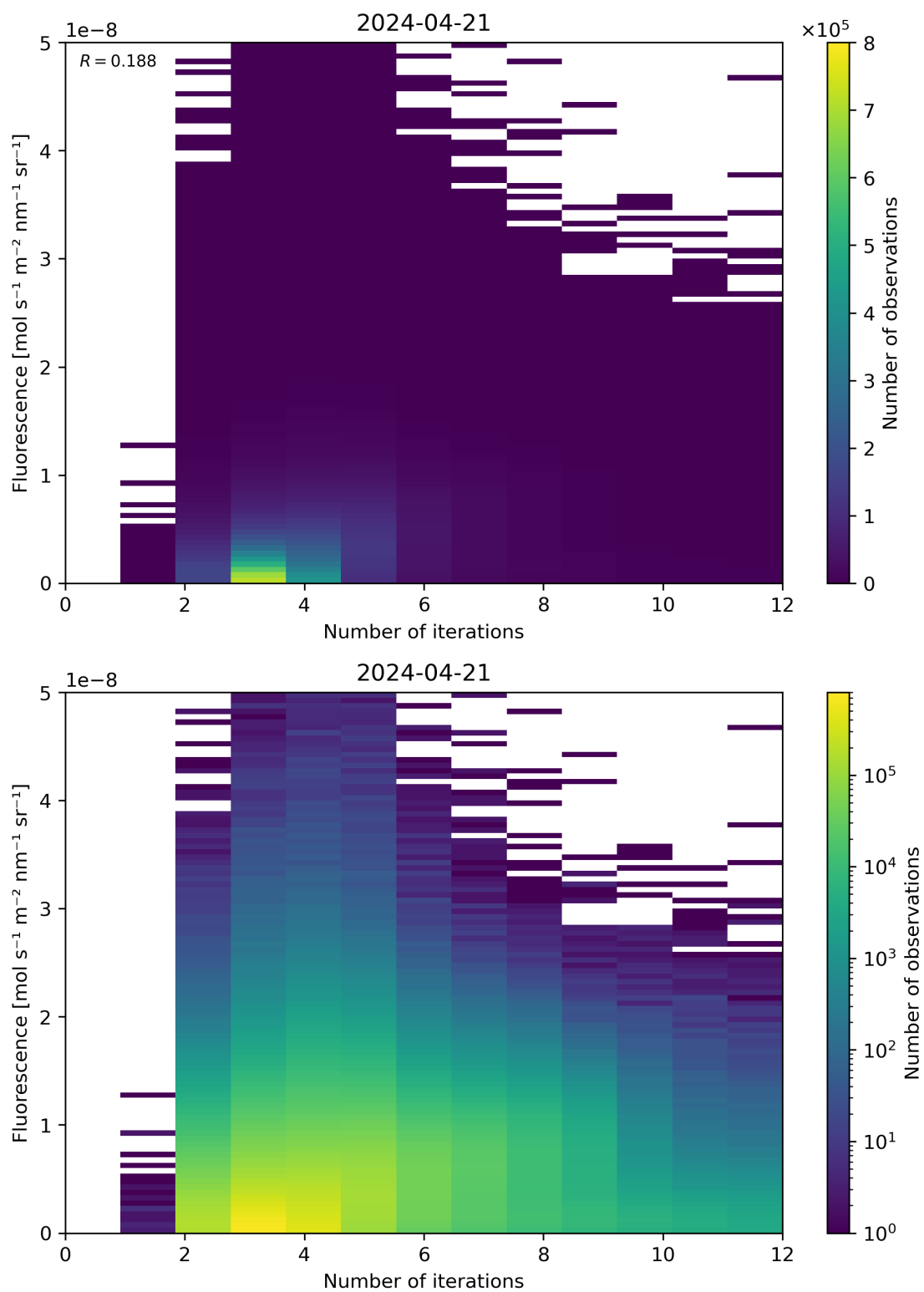
Figure 98: Scatter density plot of “Number of iterations” against “Fluorescence” for 2024-04-21 to 2024-04-22.
