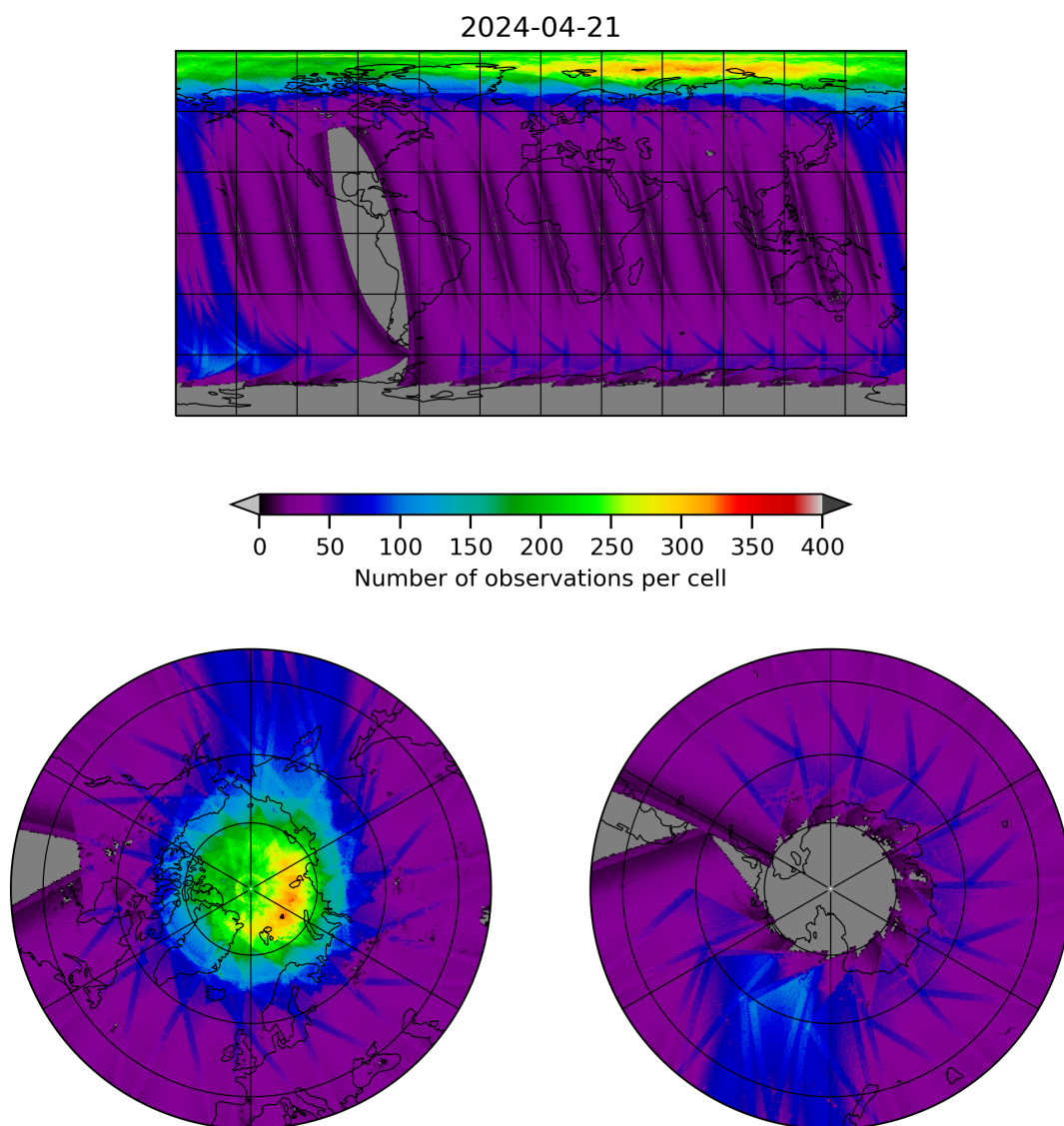
Figure 11: Map of the number of observations for 2024-04-21 to 2024-04-22
