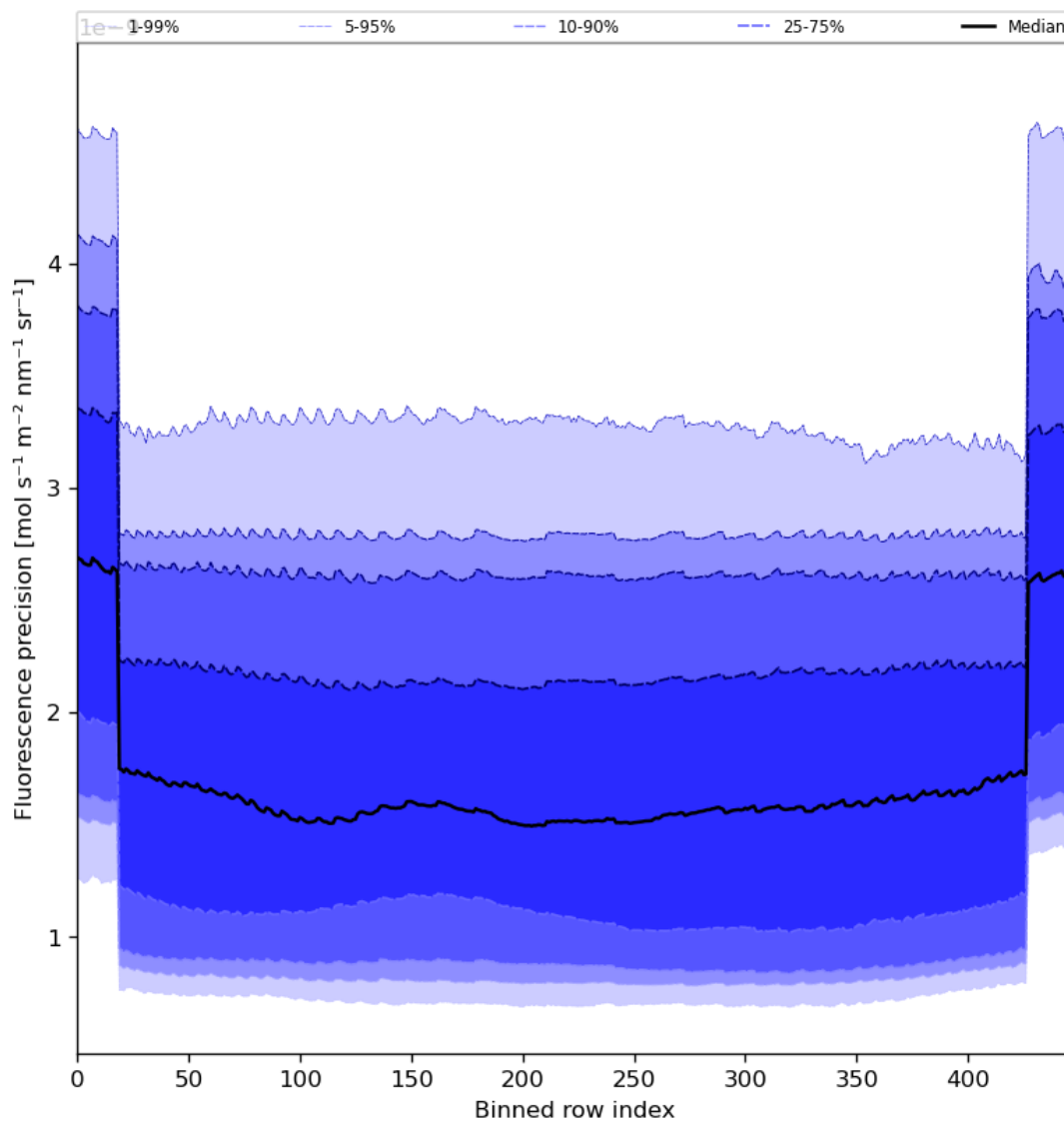
Figure 58: Along track statistics of “Fluorescence precision” for 2024-04-21 to 2024-04-22
