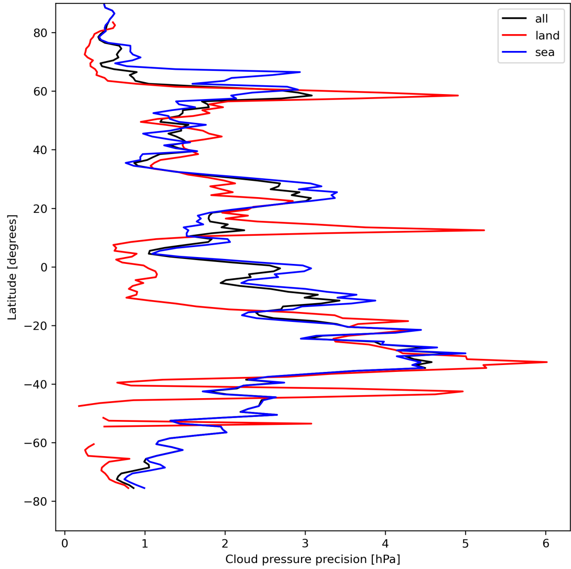
Figure 14: Zonal average of “Cloud pressure precision” for 2024-04-21 to 2024-04-22.
