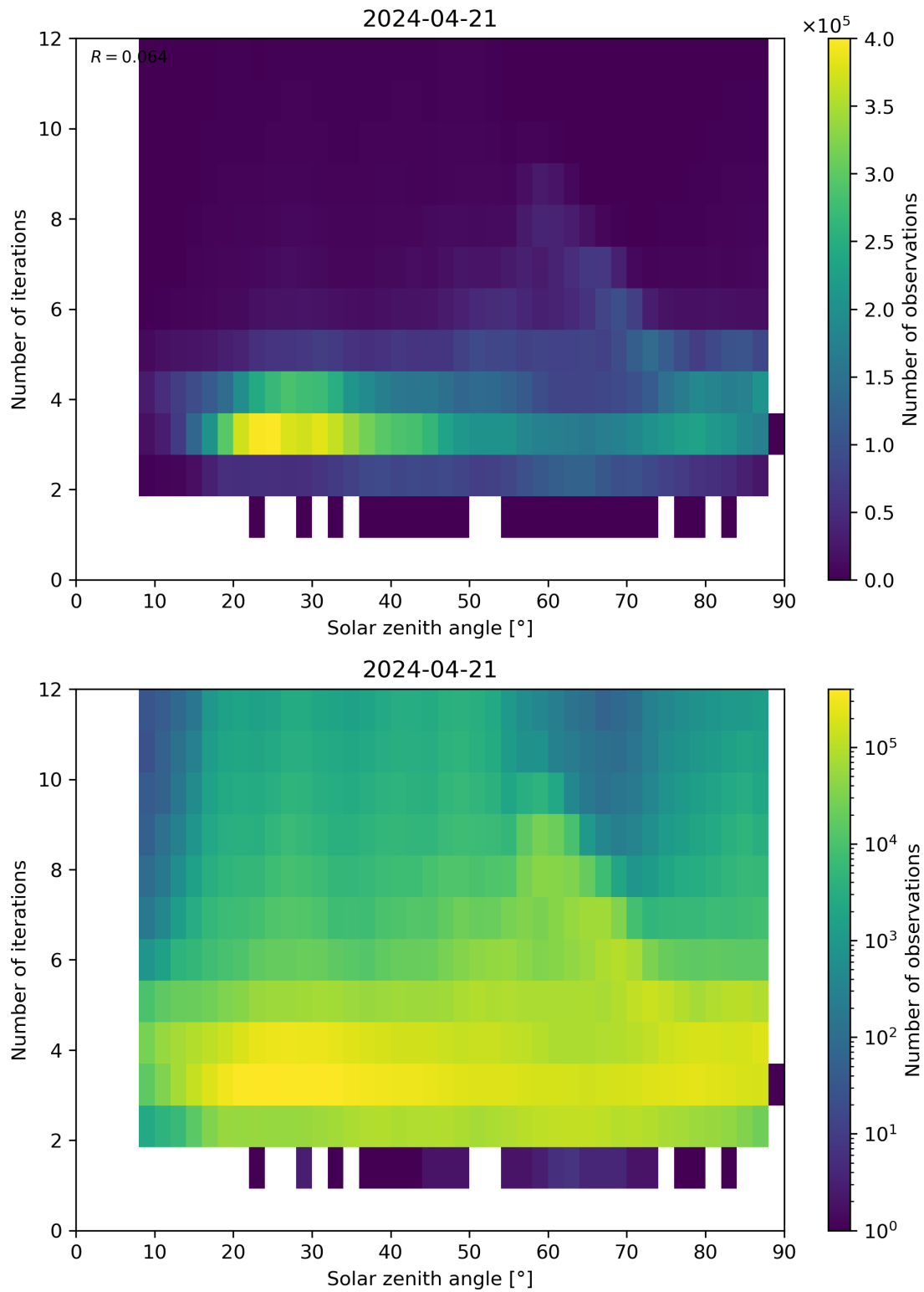
Figure 114: Scatter density plot of “Solar zenith angle” against “Number of iterations” for 2024-04-21 to 2024-04-22.
