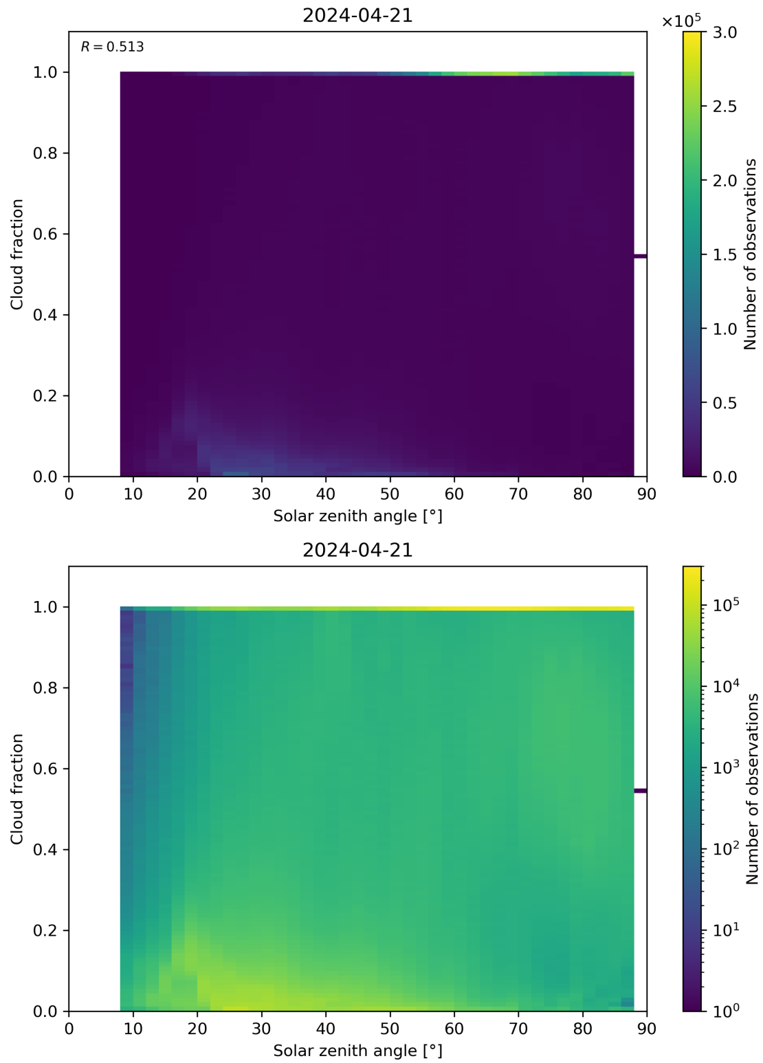
Figure 110: Scatter density plot of “Solar zenith angle” against “Cloud fraction” for 2024-04-21 to 2024-04-22.
