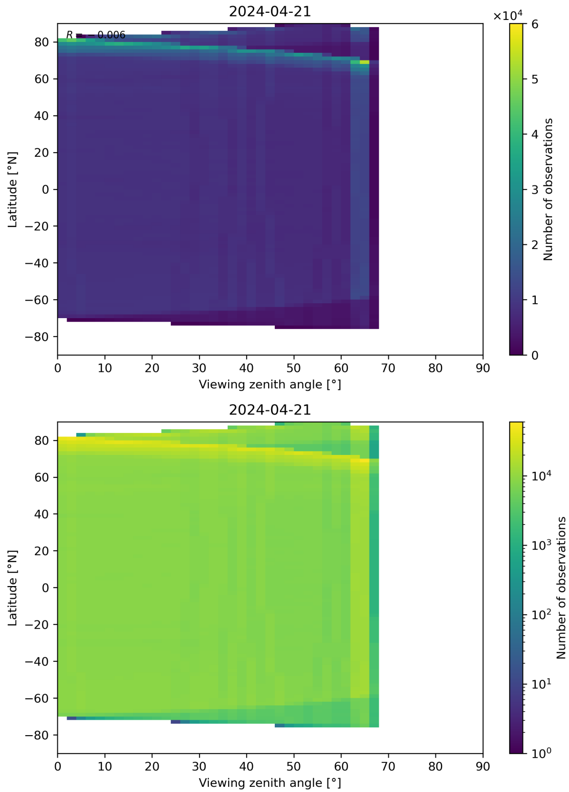
Figure 123: Scatter density plot of “Viewing zenith angle” against “Latitude” for 2024-04-21 to 2024-04-22.
