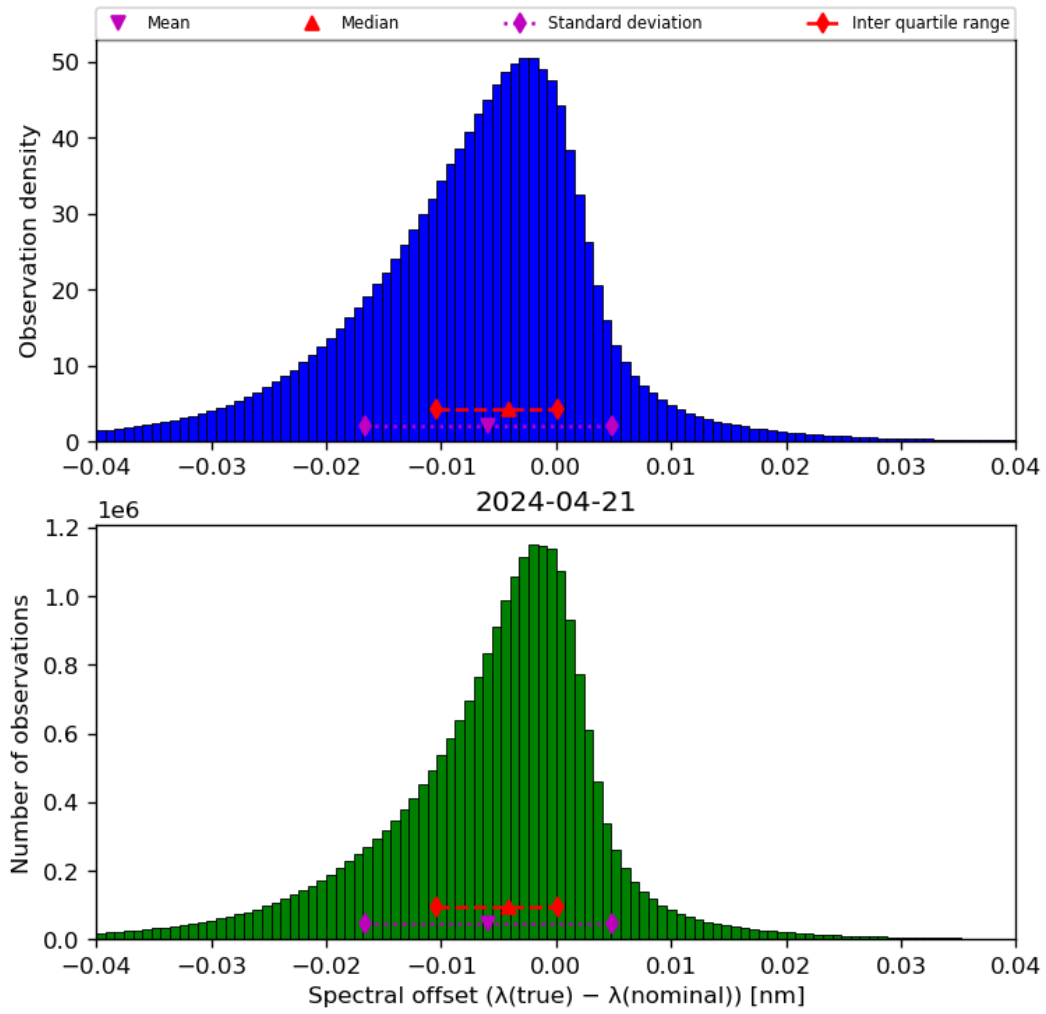
Figure 45: Histogram of “Spectral offset ( \lambda(\text{true}) - \lambda(\text{nominal}) )” for 2024-04-21 to 2024-04-22
