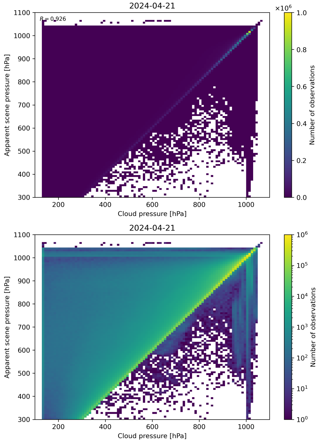
Figure 77: Scatter density plot of “Cloud pressure” against “Apparent scene pressure” for 2024-04-21 to 2024-04-22.
