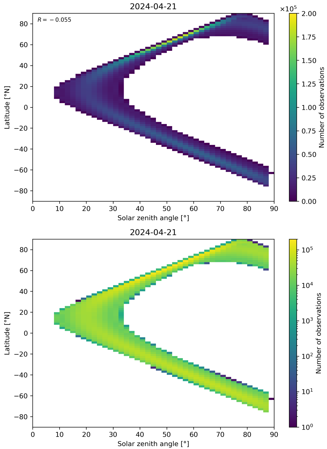
Figure 113: Scatter density plot of “Solar zenith angle” against “Latitude” for 2024-04-21 to 2024-04-22.
