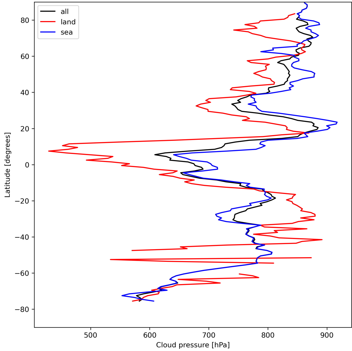
Figure 13: Zonal average of “Cloud pressure” for 2024-04-21 to 2024-04-22.
