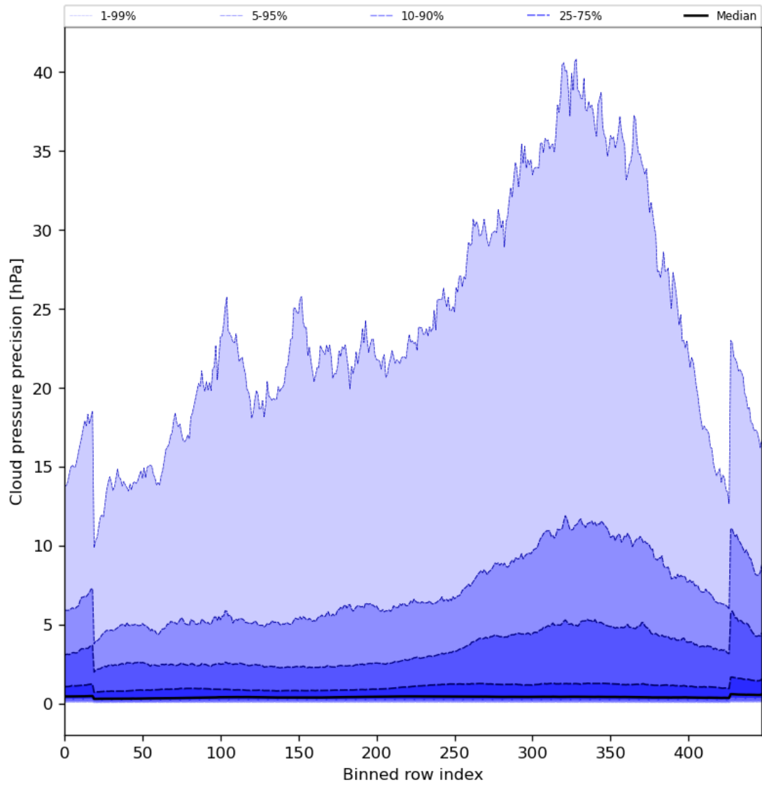
Figure 48: Along track statistics of “Cloud pressure precision” for 2024-04-21 to 2024-04-22
