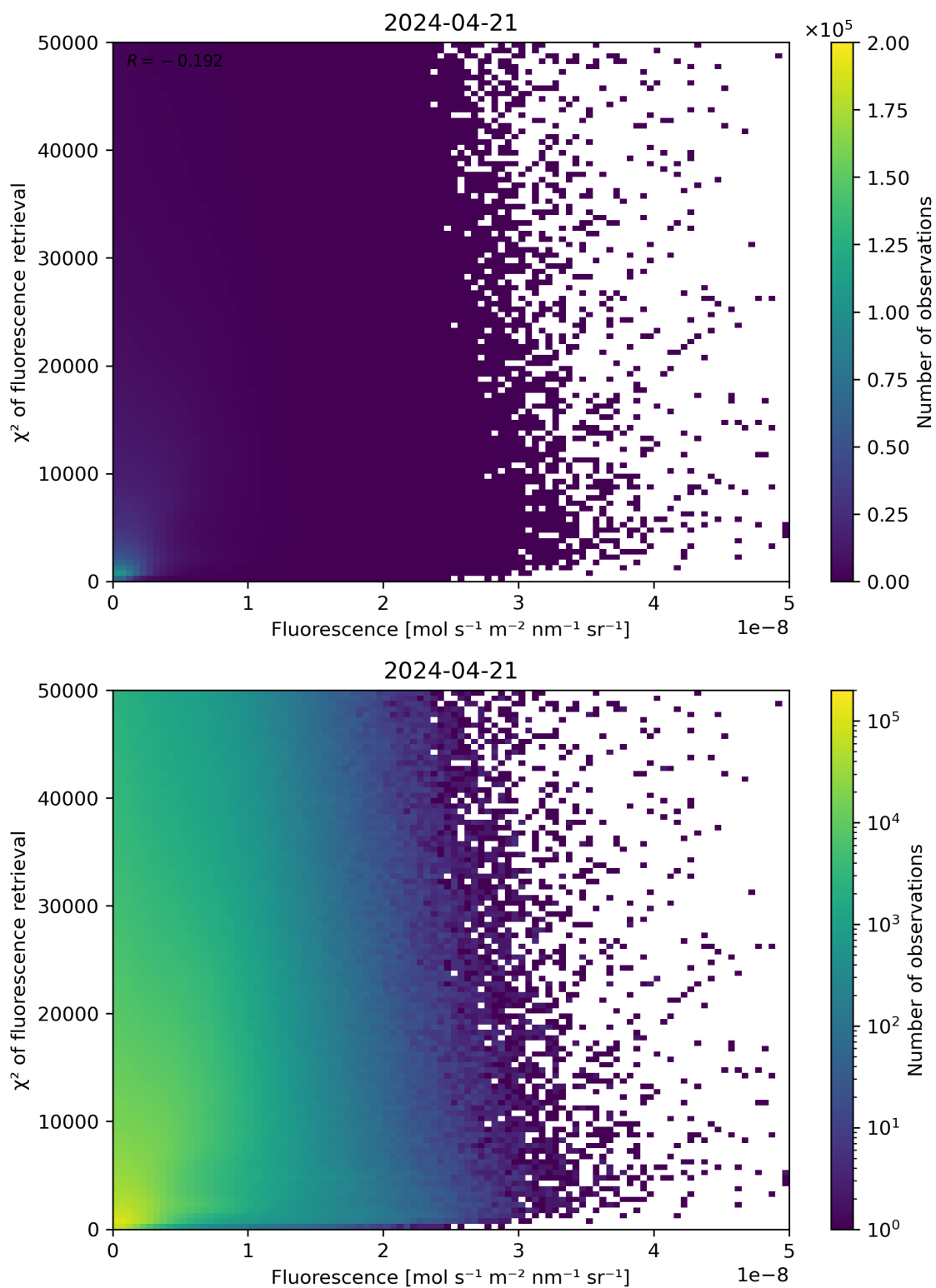
Figure 85: Scatter density plot of “Fluorescence” against “ \chi^2 of fluorescence retrieval” for 2024-04-21 to 2024-04-22.
