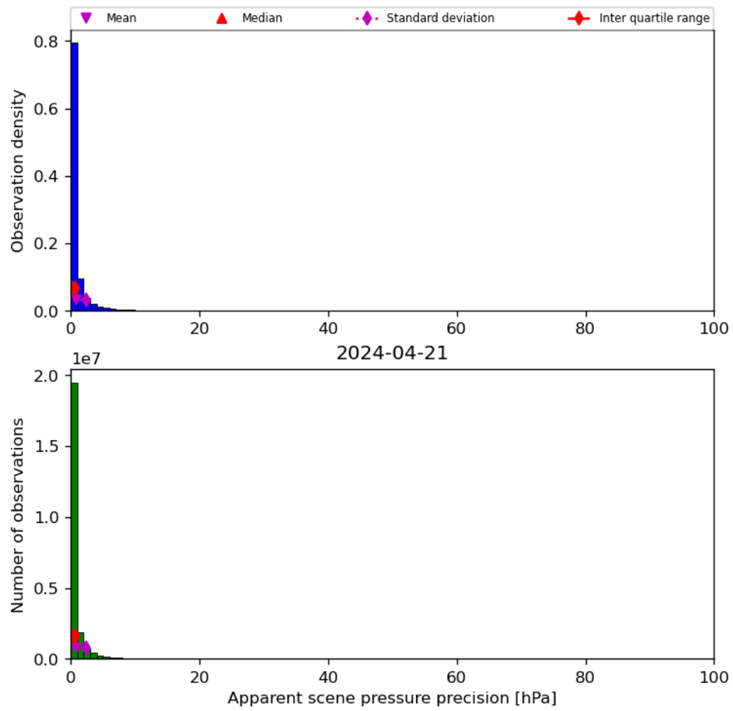
Figure 37: Histogram of “Apparent scene pressure precision” for 2024-04-21 to 2024-04-22
