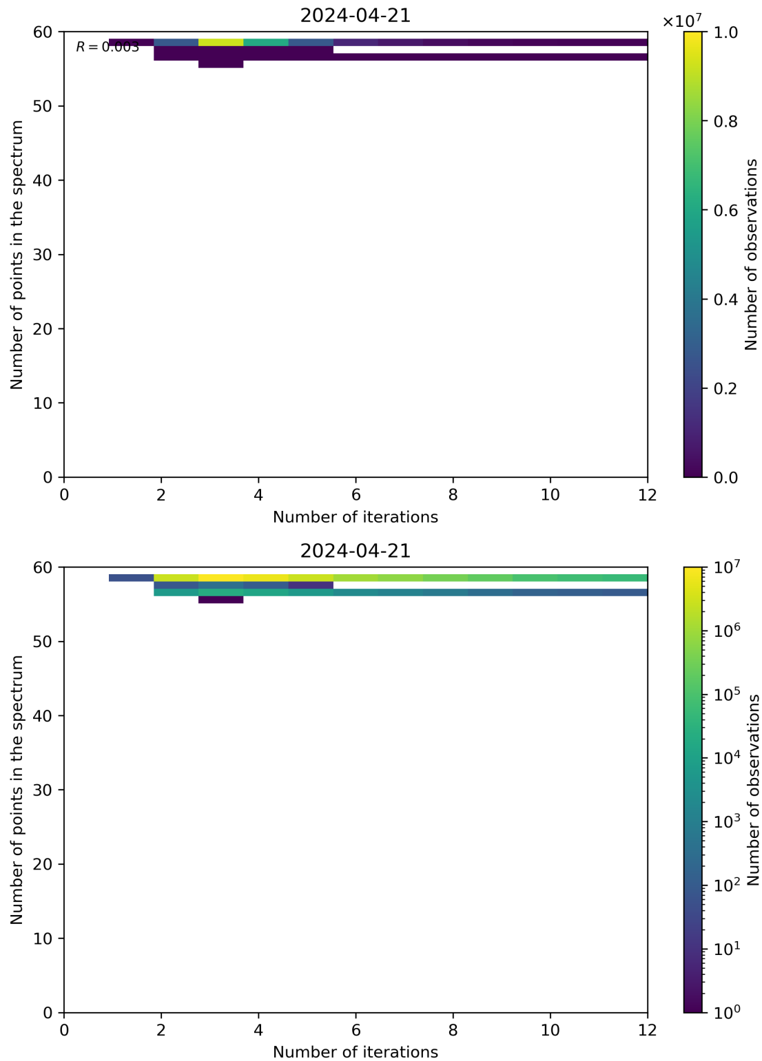
Figure 99: Scatter density plot of “Number of iterations” against “Number of points in the spectrum” for 2024-04-21 to 2024-04-22.
