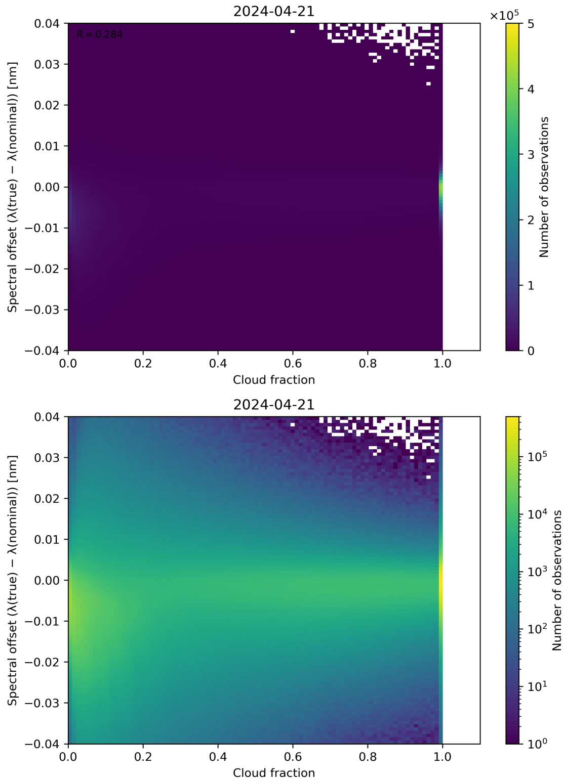
Figure 76: Scatter density plot of “Cloud fraction” against “Spectral offset ( \lambda(\text{true}) - \lambda(\text{nominal}) )” for 2024-04-21 to 2024-04-22.
