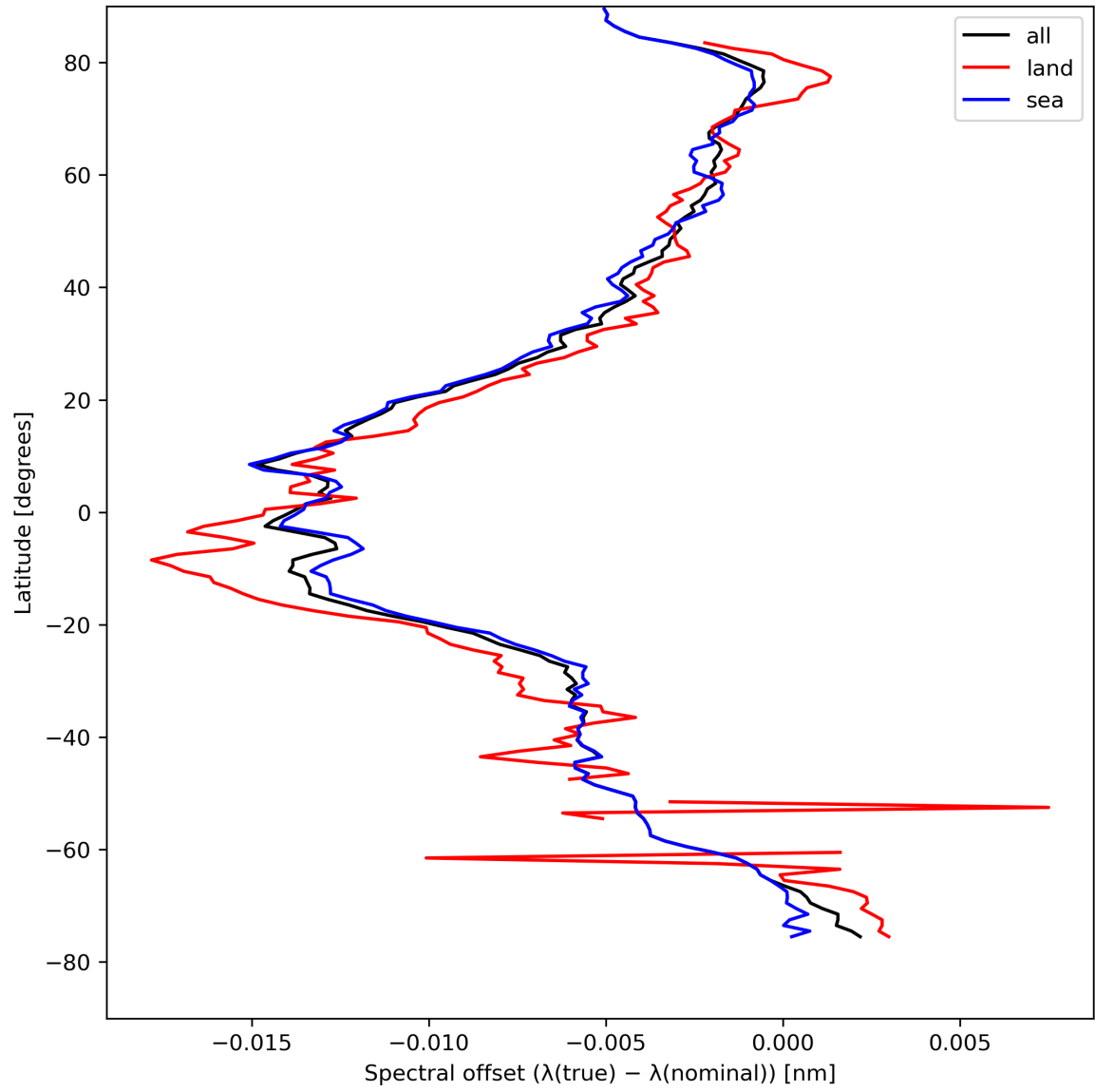
Figure 28: Zonal average of “Spectral offset ( \lambda(\text{true}) - \lambda(\text{nominal}) )” for 2024-04-21 to 2024-04-22.
