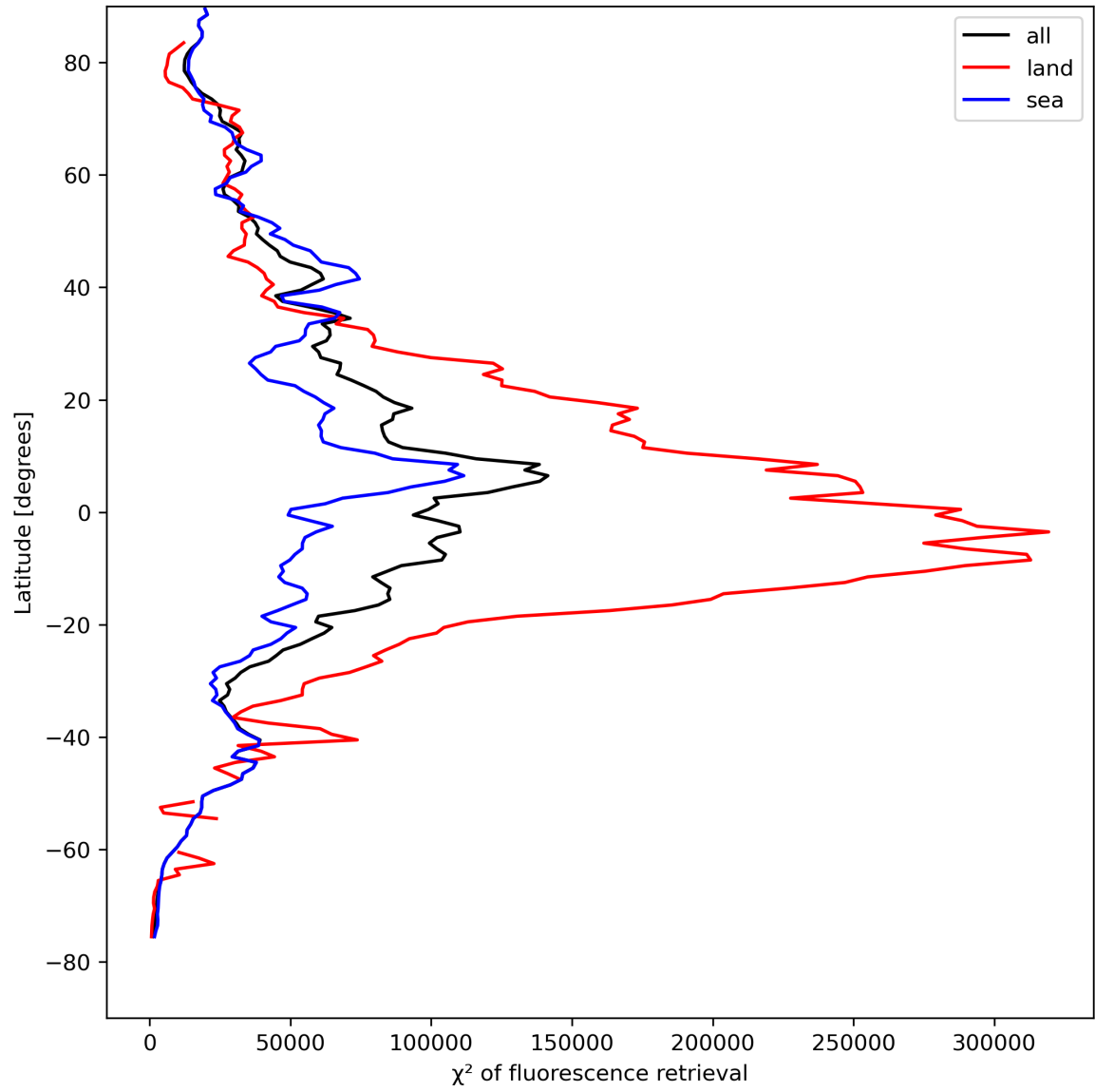
Figure 25: Zonal average of “ \chi^2 of fluorescence retrieval” for 2024-04-21 to 2024-04-22.
