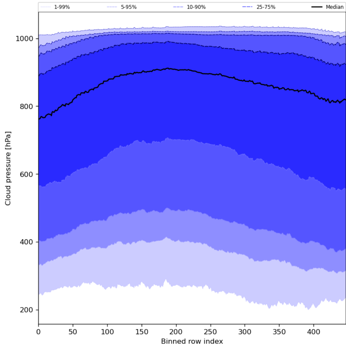
Figure 47: Along track statistics of “Cloud pressure” for 2024-04-21 to 2024-04-22
