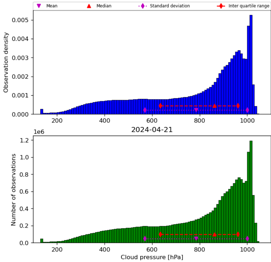
Figure 30: Histogram of “Cloud pressure” for 2024-04-21 to 2024-04-22
