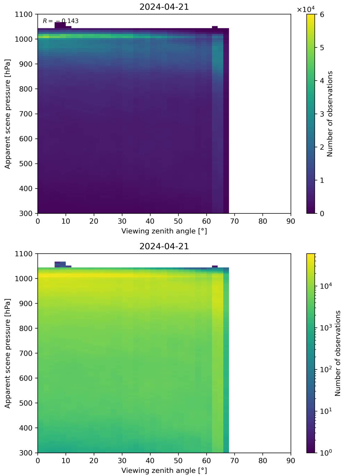
Figure 118: Scatter density plot of “Viewing zenith angle” against “Apparent scene pressure” for 2024-04-21 to 2024-04-22.
