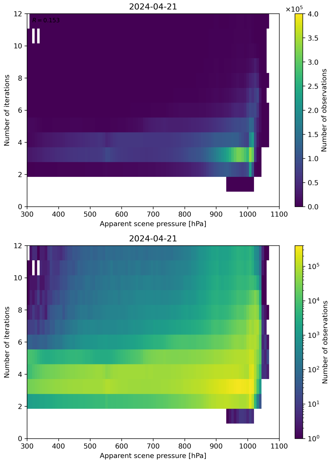
Figure 65: Scatter density plot of “Apparent scene pressure” against “Number of iterations” for 2024-04-21 to 2024-04-22.
