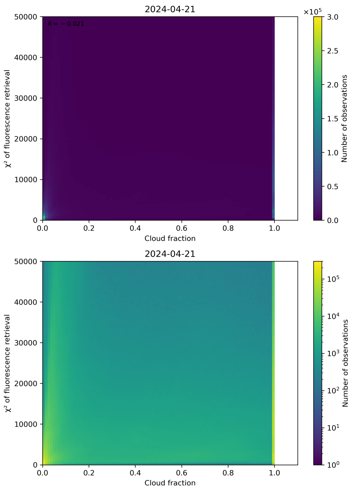
Figure 71: Scatter density plot of “Cloud fraction” against “ \chi^2 of fluorescence retrieval” for 2024-04-21 to 2024-04-22.
