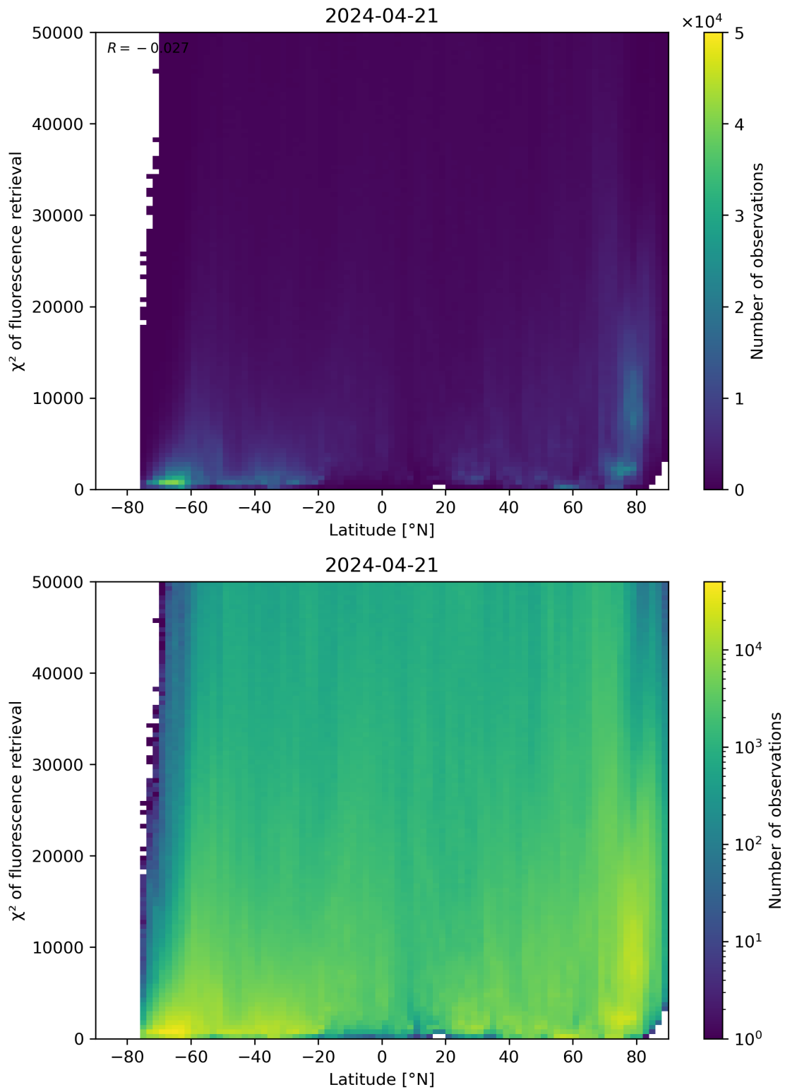
Figure 89: Scatter density plot of “Latitude” against “ \chi^2 of fluorescence retrieval” for 2024-04-21 to 2024-04-22.
