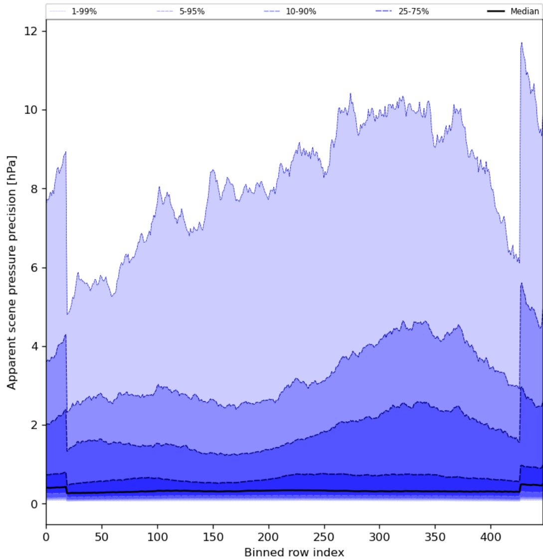
Figure 54: Along track statistics of “Apparent scene pressure precision” for 2024-04-21 to 2024-04-22
