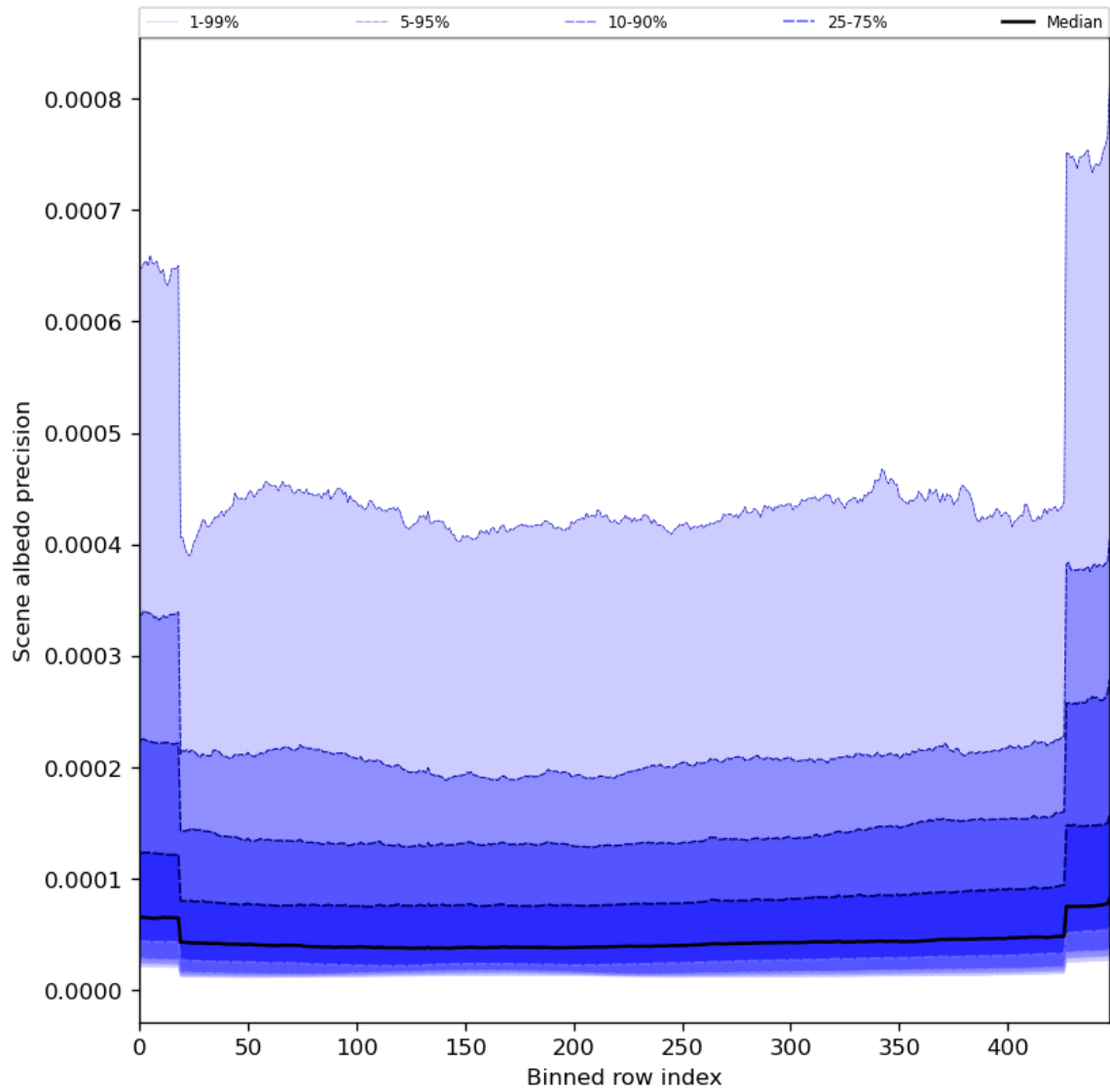
Figure 52: Along track statistics of “Scene albedo precision” for 2024-04-21 to 2024-04-22
