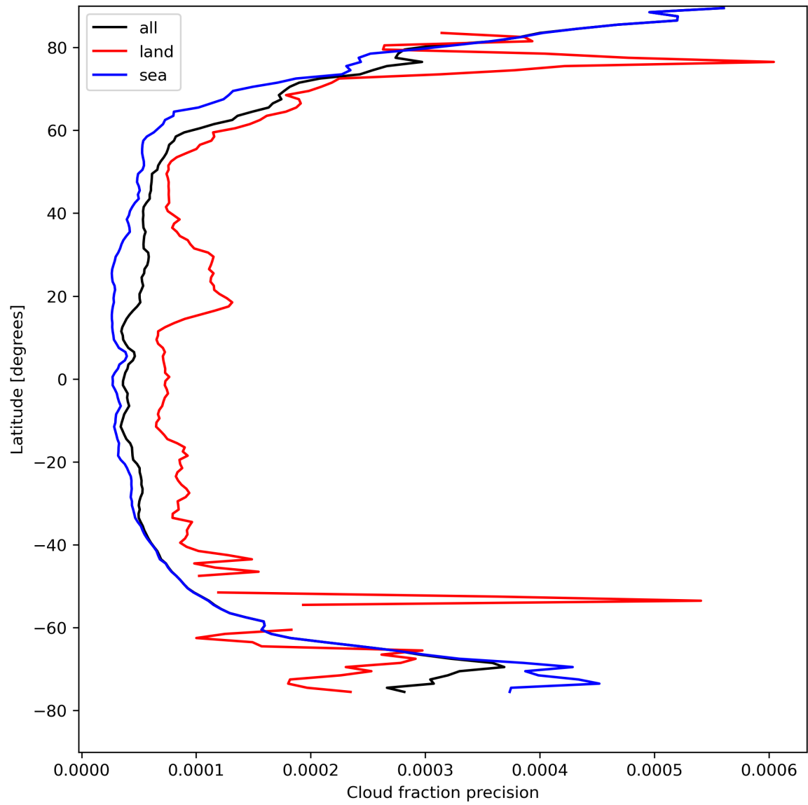
Figure 16: Zonal average of “Cloud fraction precision” for 2024-04-21 to 2024-04-22.
