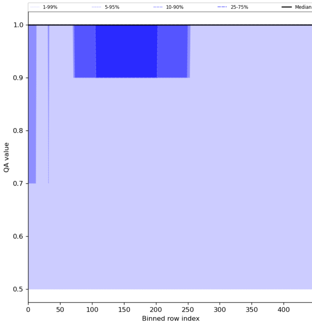
Figure 46: Along track statistics of “QA value” for 2024-04-21 to 2024-04-22
