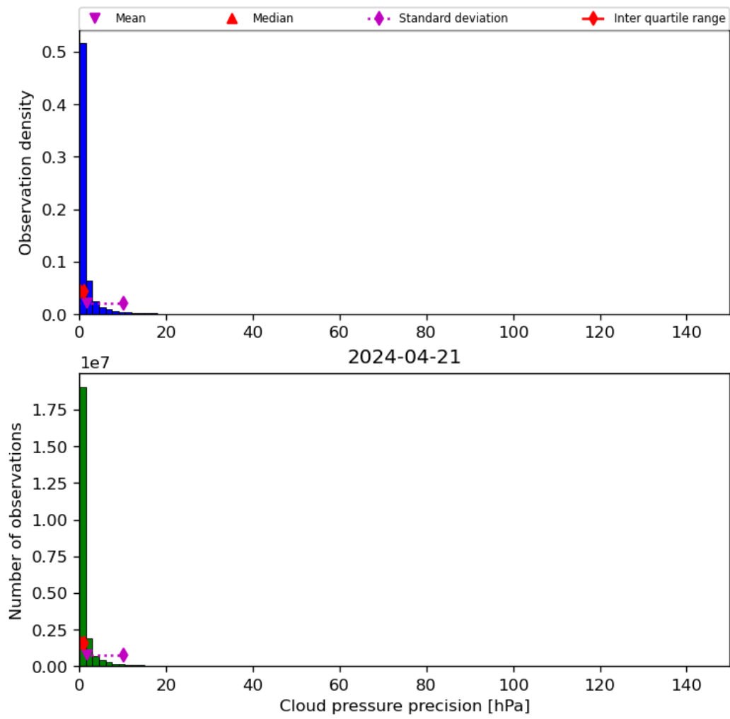
Figure 31: Histogram of “Cloud pressure precision” for 2024-04-21 to 2024-04-22
