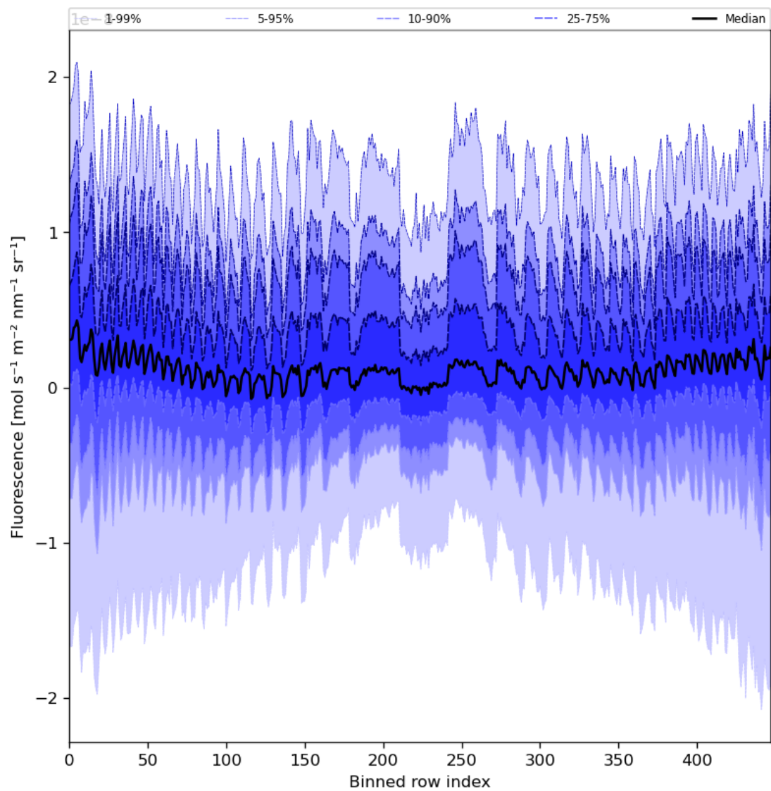
Figure 57: Along track statistics of “Fluorescence” for 2024-04-21 to 2024-04-22
