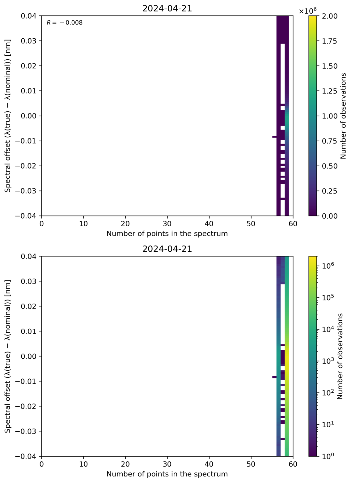
Figure 101: Scatter density plot of “Number of points in the spectrum” against “Spectral offset ( \lambda(\text{true}) - \lambda(\text{nominal}) )” for 2024-04-21 to 2024-04-22.
