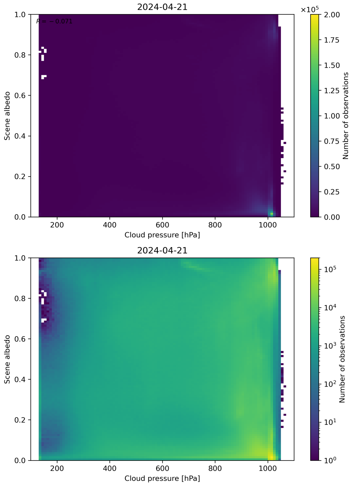
Figure 83: Scatter density plot of “Cloud pressure” against “Scene albedo” for 2024-04-21 to 2024-04-22.
