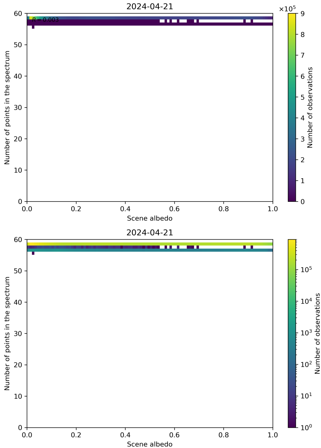
Figure 106: Scatter density plot of “Scene albedo” against “Number of points in the spectrum” for 2024-04-21 to 2024-04-22.
