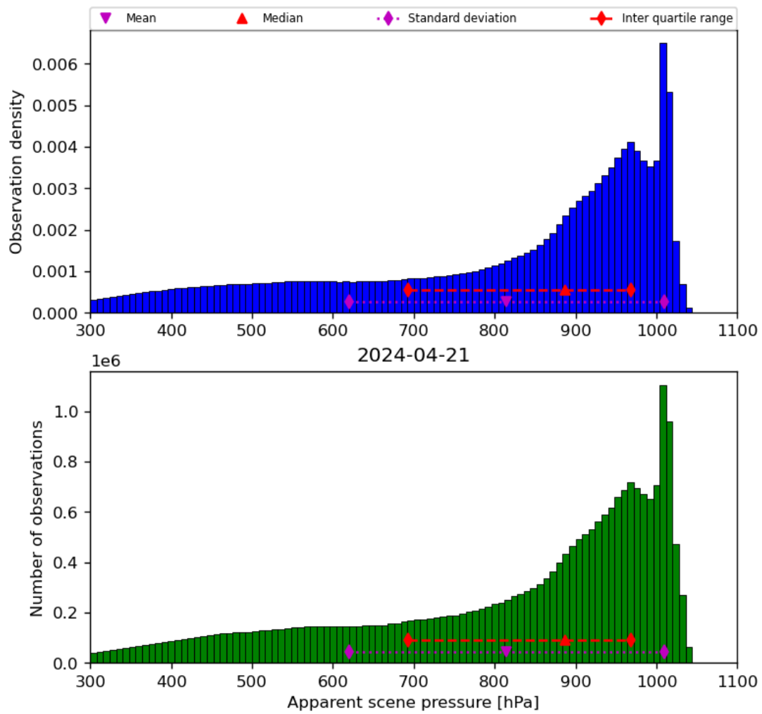
Figure 36: Histogram of “Apparent scene pressure” for 2024-04-21 to 2024-04-22
