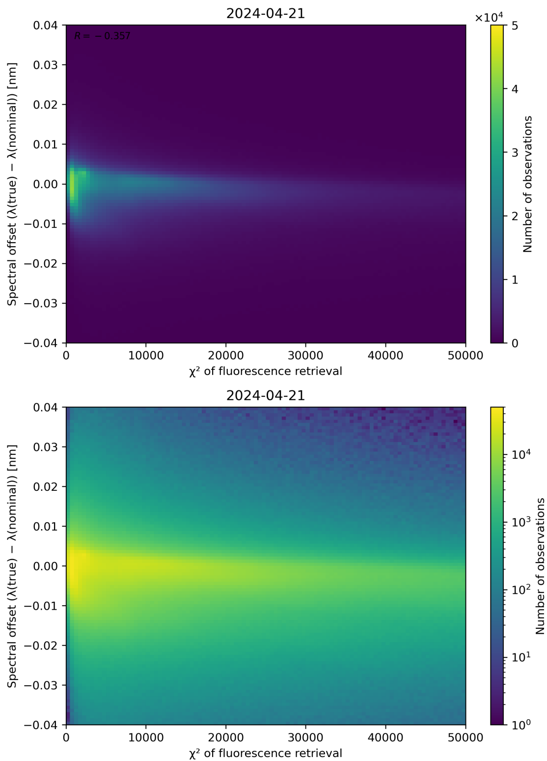
Figure 69: Scatter density plot of " \chi^2 of fluorescence retrieval" against "Spectral offset ( \lambda(\text{true}) - \lambda(\text{nominal}) )" for 2024-04-21 to 2024-04-22.
