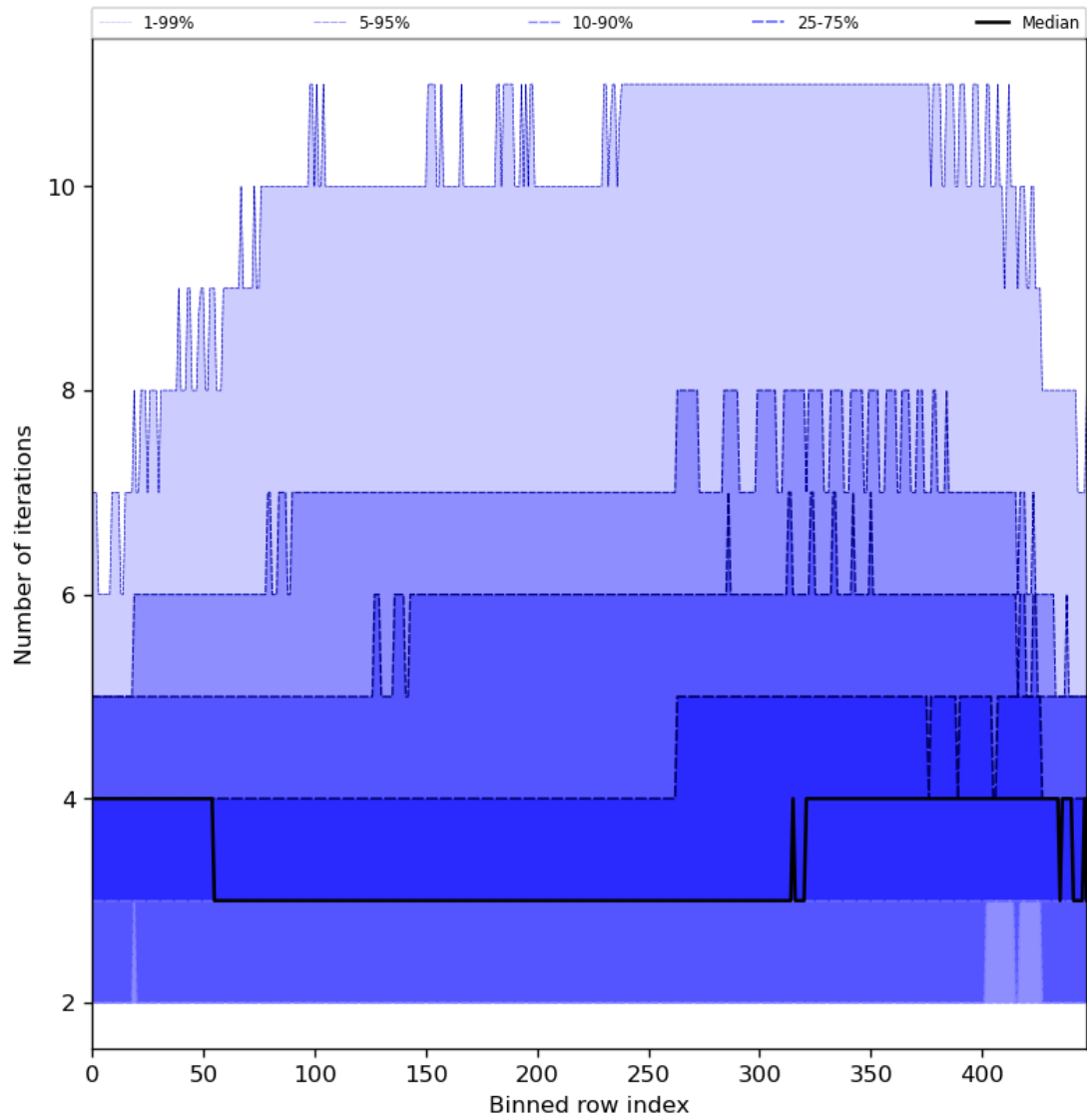
Figure 56: Along track statistics of “Number of iterations” for 2024-04-21 to 2024-04-22
