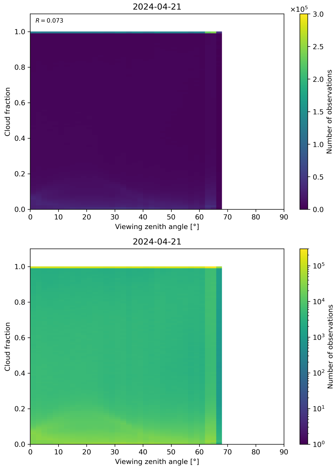
Figure 120: Scatter density plot of “Viewing zenith angle” against “Cloud fraction” for 2024-04-21 to 2024-04-22.
