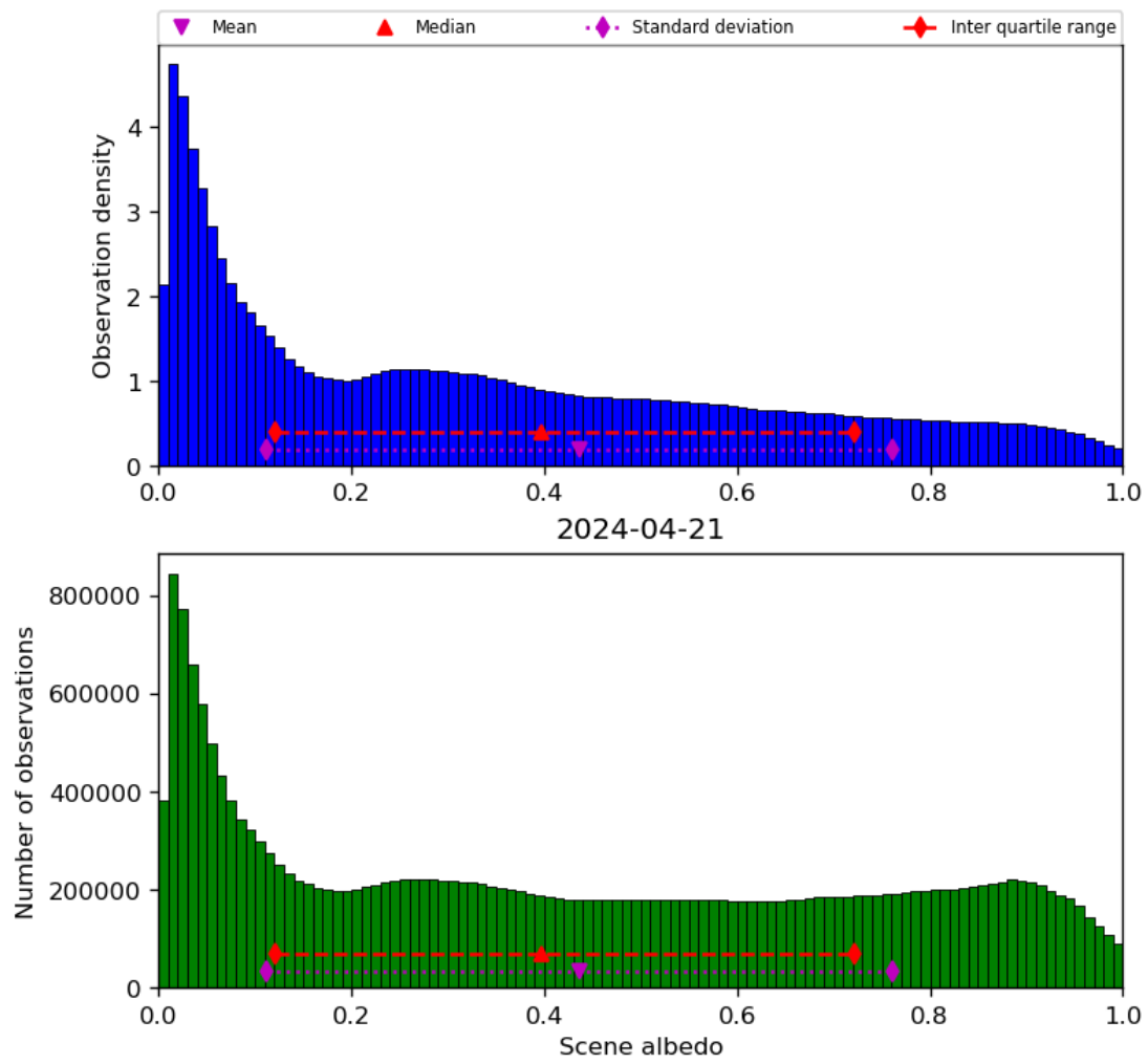
Figure 34: Histogram of “Scene albedo” for 2024-04-21 to 2024-04-22
