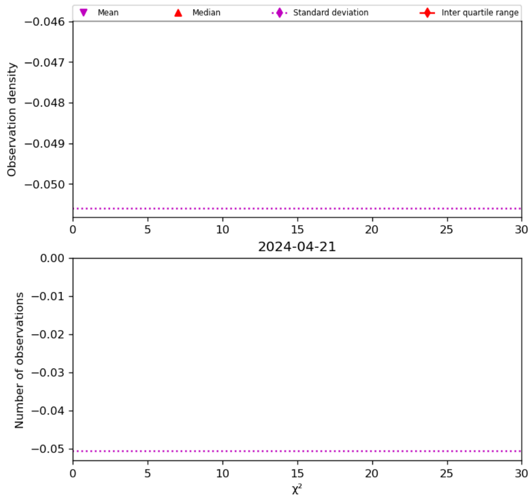
Figure 38: Histogram of “ \chi^2 ” for 2024-04-21 to 2024-04-22
