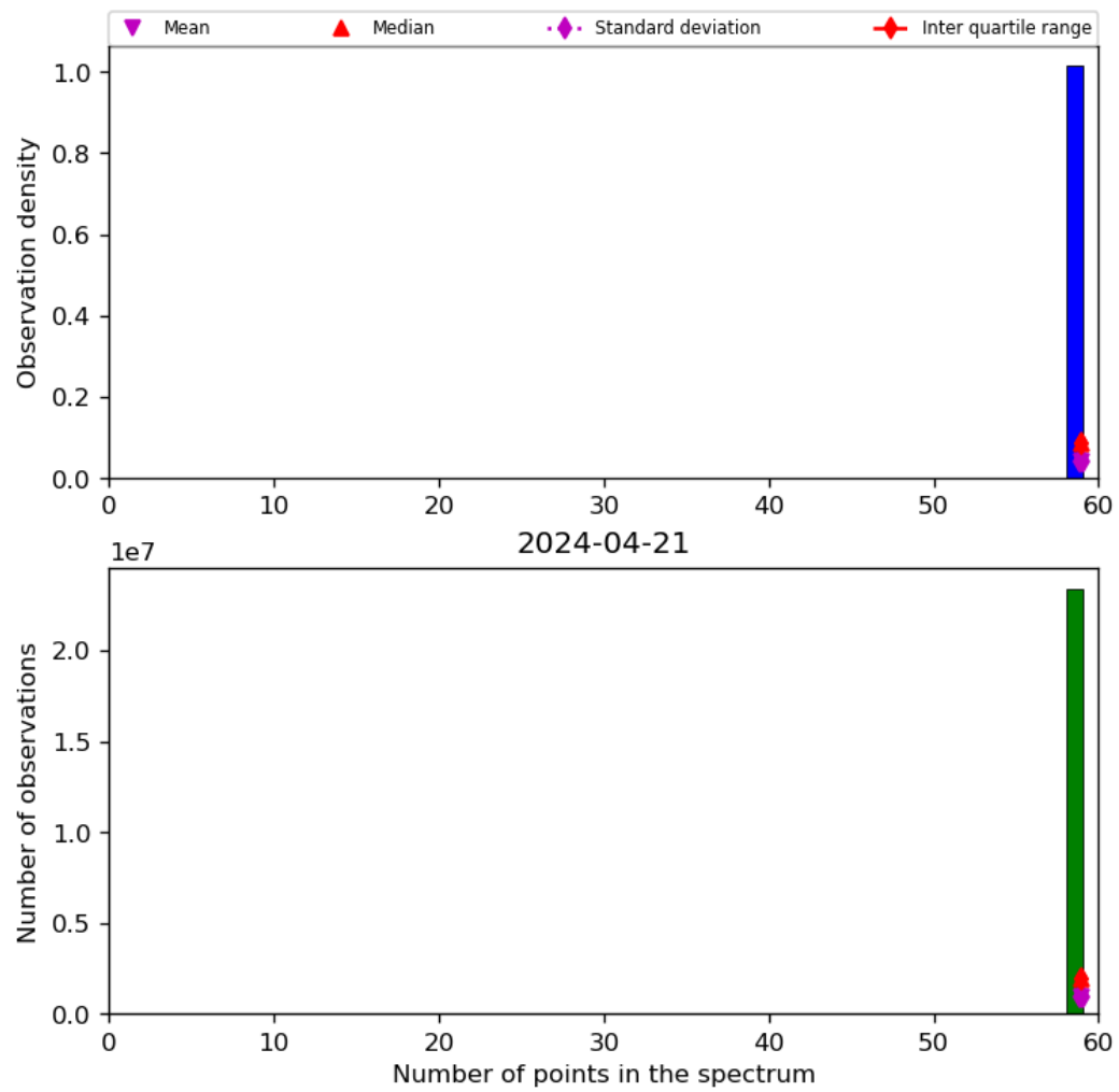
Figure 44: Histogram of “Number of points in the spectrum” for 2024-04-21 to 2024-04-22
