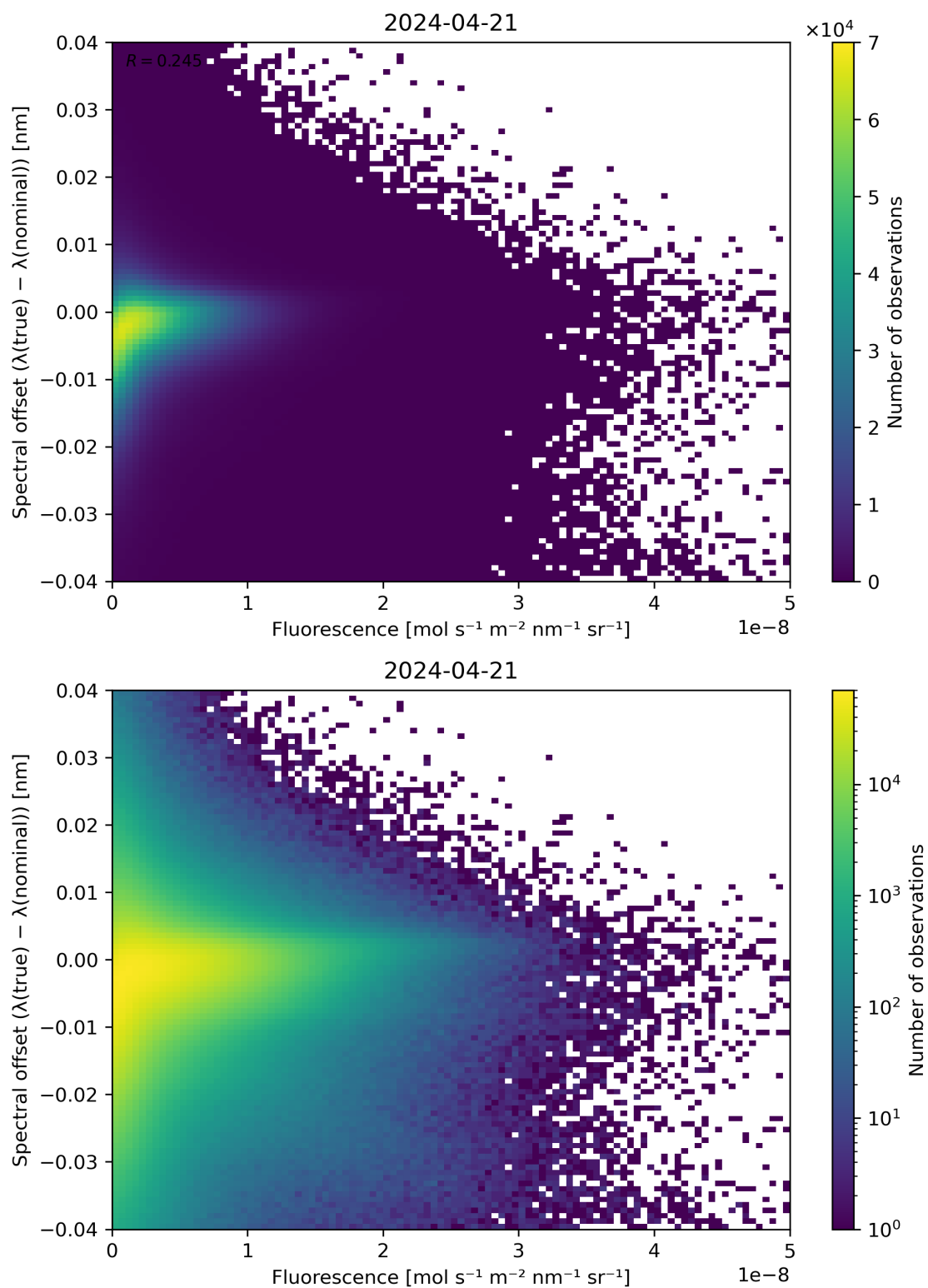
Figure 87: Scatter density plot of “Fluorescence” against “Spectral offset ( \lambda(\text{true}) - \lambda(\text{nominal}) )” for 2024-04-21 to 2024-04-22.
