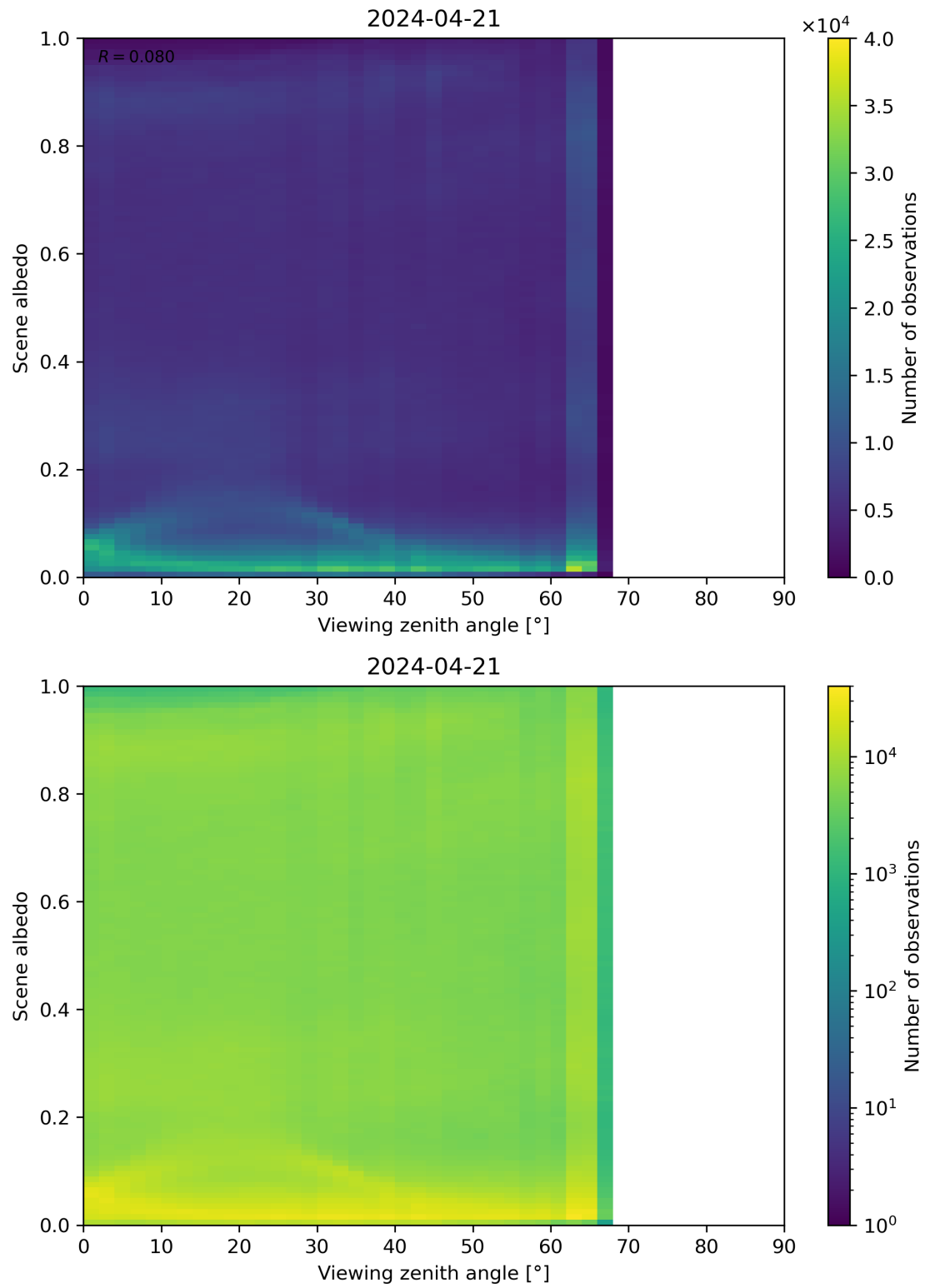
Figure 126: Scatter density plot of “Viewing zenith angle” against “Scene albedo” for 2024-04-21 to 2024-04-22.
