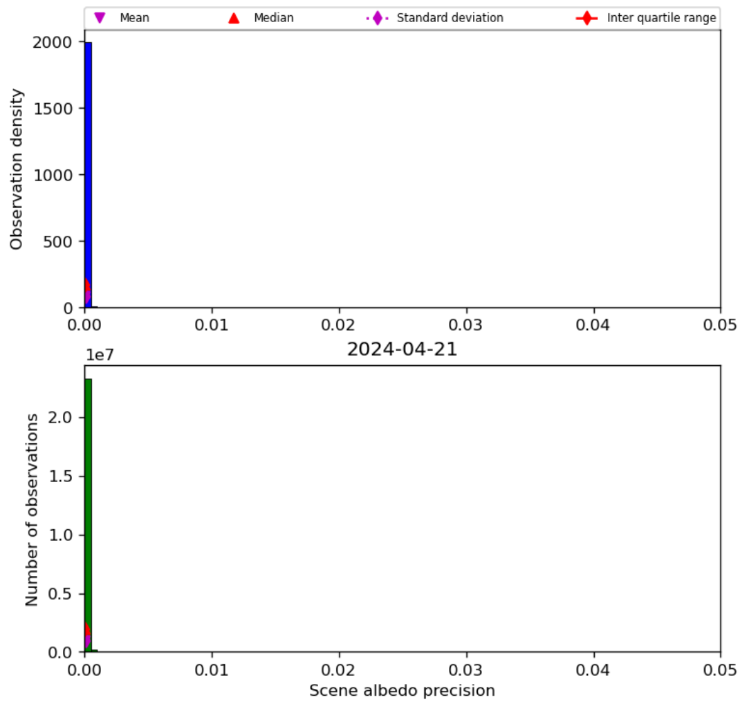
Figure 35: Histogram of “Scene albedo precision” for 2024-04-21 to 2024-04-22
