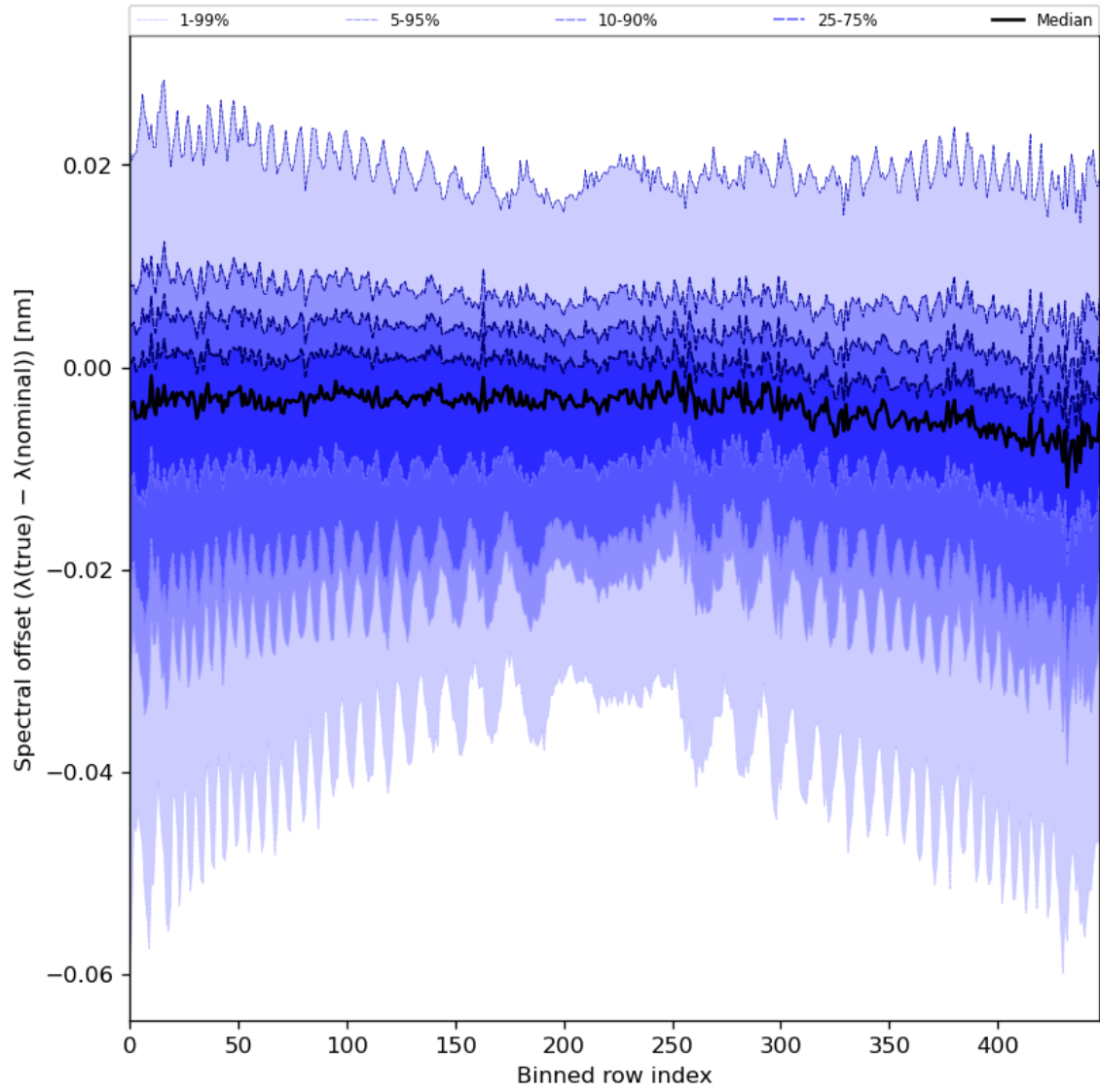
Figure 62: Along track statistics of “Spectral offset ( \lambda(\text{true}) - \lambda(\text{nominal}) )” for 2024-04-21 to 2024-04-22
