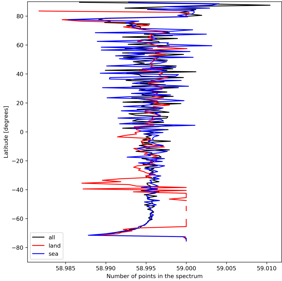
Figure 27: Zonal average of “Number of points in the spectrum” for 2024-04-21 to 2024-04-22.
