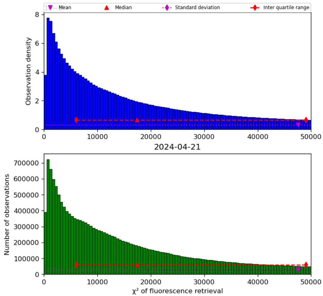
Figure 42: Histogram of “ \chi^2 of fluorescence retrieval” for 2024-04-21 to 2024-04-22
