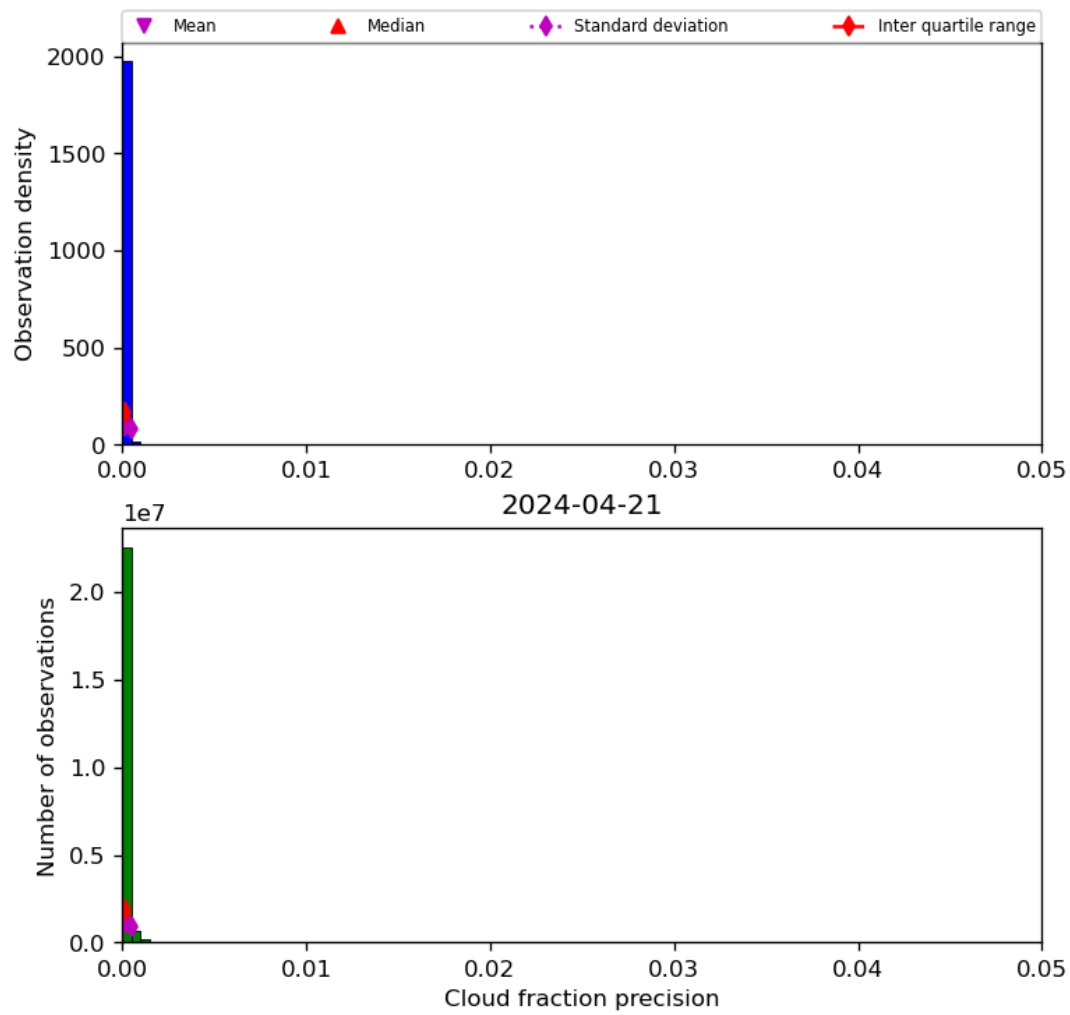
Figure 33: Histogram of “Cloud fraction precision” for 2024-04-21 to 2024-04-22
