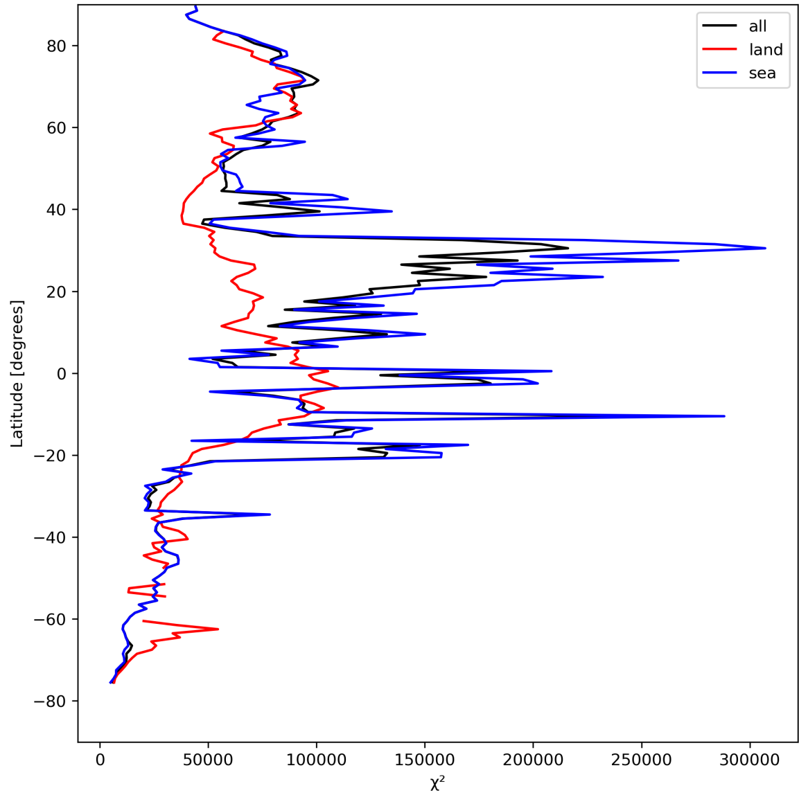
Figure 21: Zonal average of “ \chi^2 ” for 2024-04-21 to 2024-04-22.
