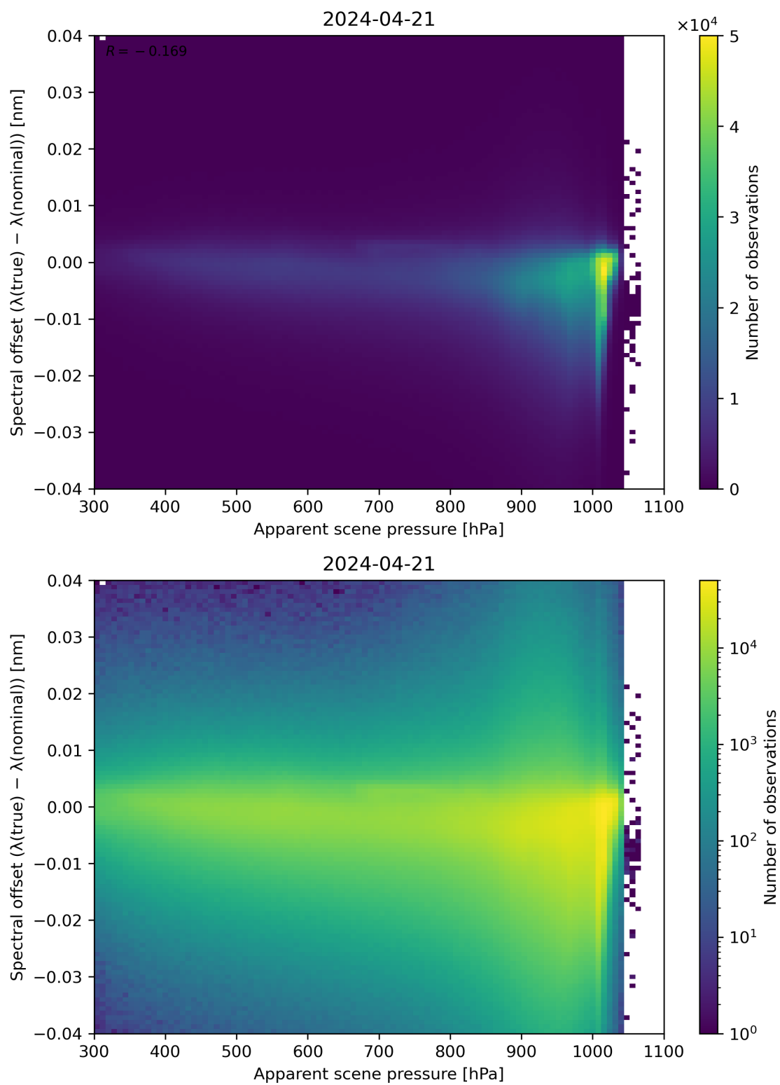
Figure 67: Scatter density plot of “Apparent scene pressure” against “Spectral offset ( \lambda(\text{true}) - \lambda(\text{nominal}) )” for 2024-04-21 to 2024-04-22.
