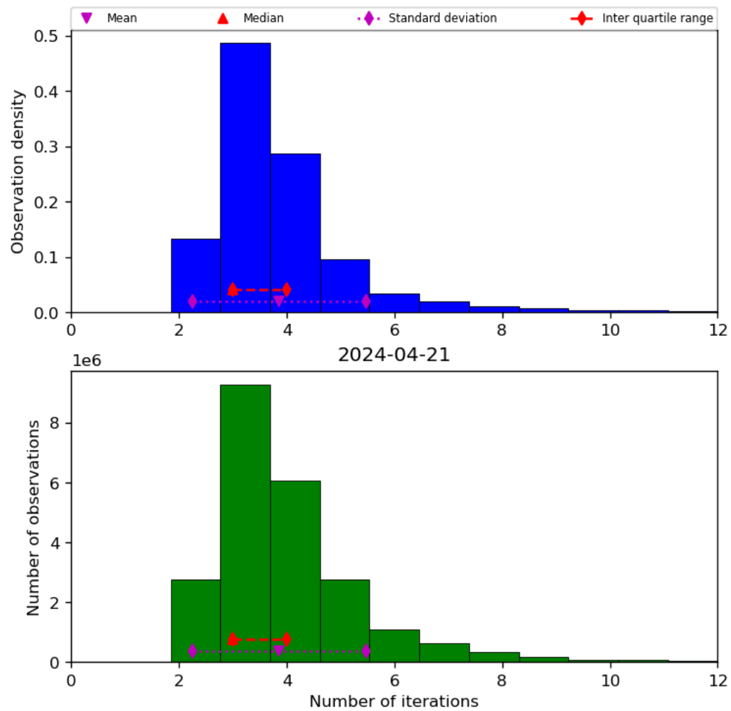
Figure 39: Histogram of “Number of iterations” for 2024-04-21 to 2024-04-22
