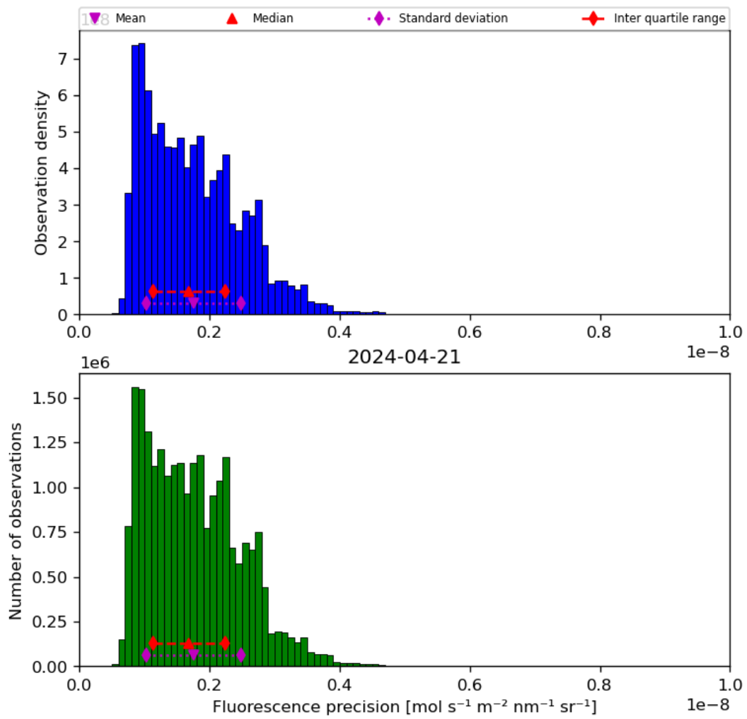
Figure 41: Histogram of “Fluorescence precision” for 2024-04-21 to 2024-04-22
