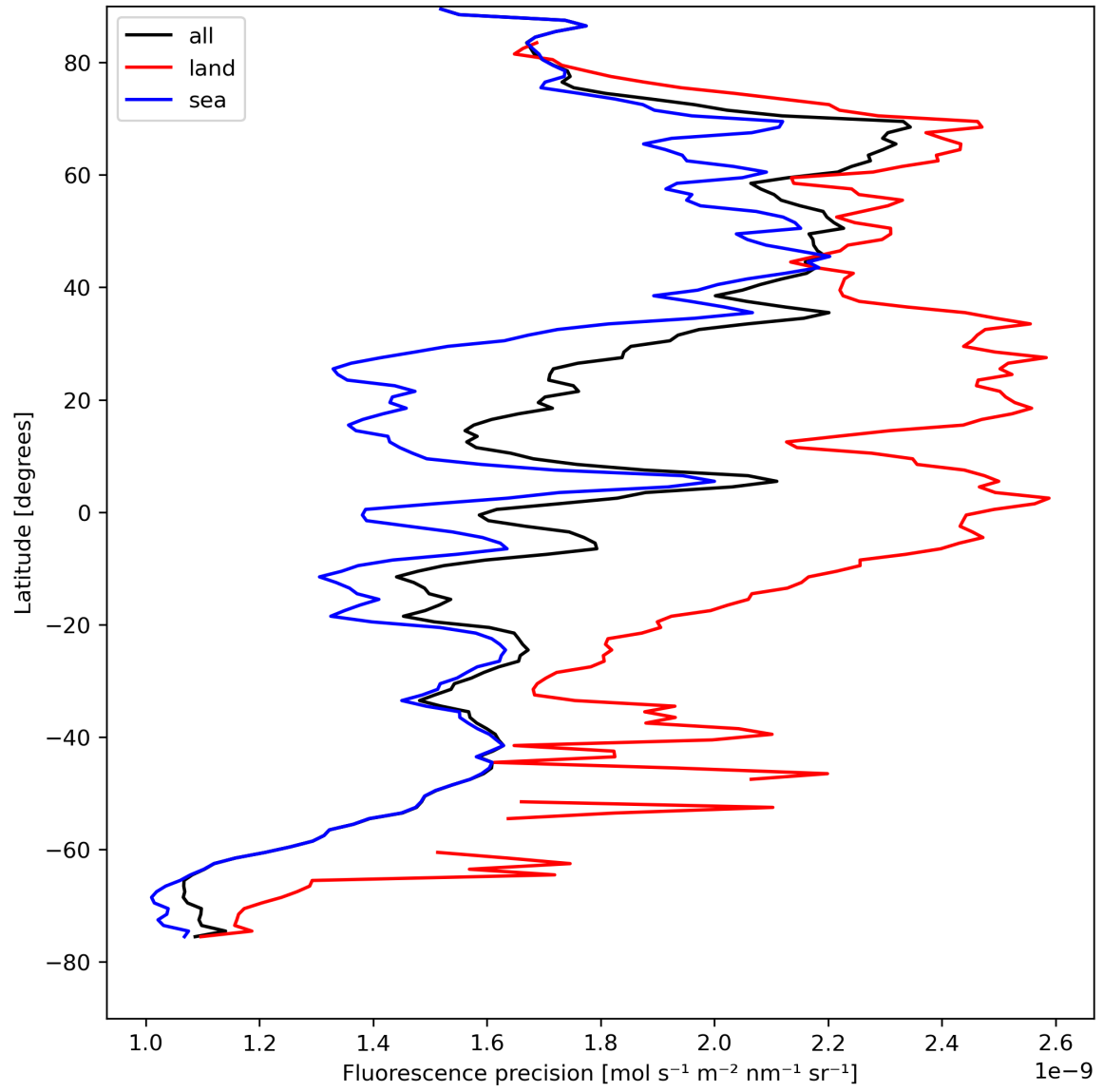
Figure 24: Zonal average of “Fluorescence precision” for 2024-04-21 to 2024-04-22.
