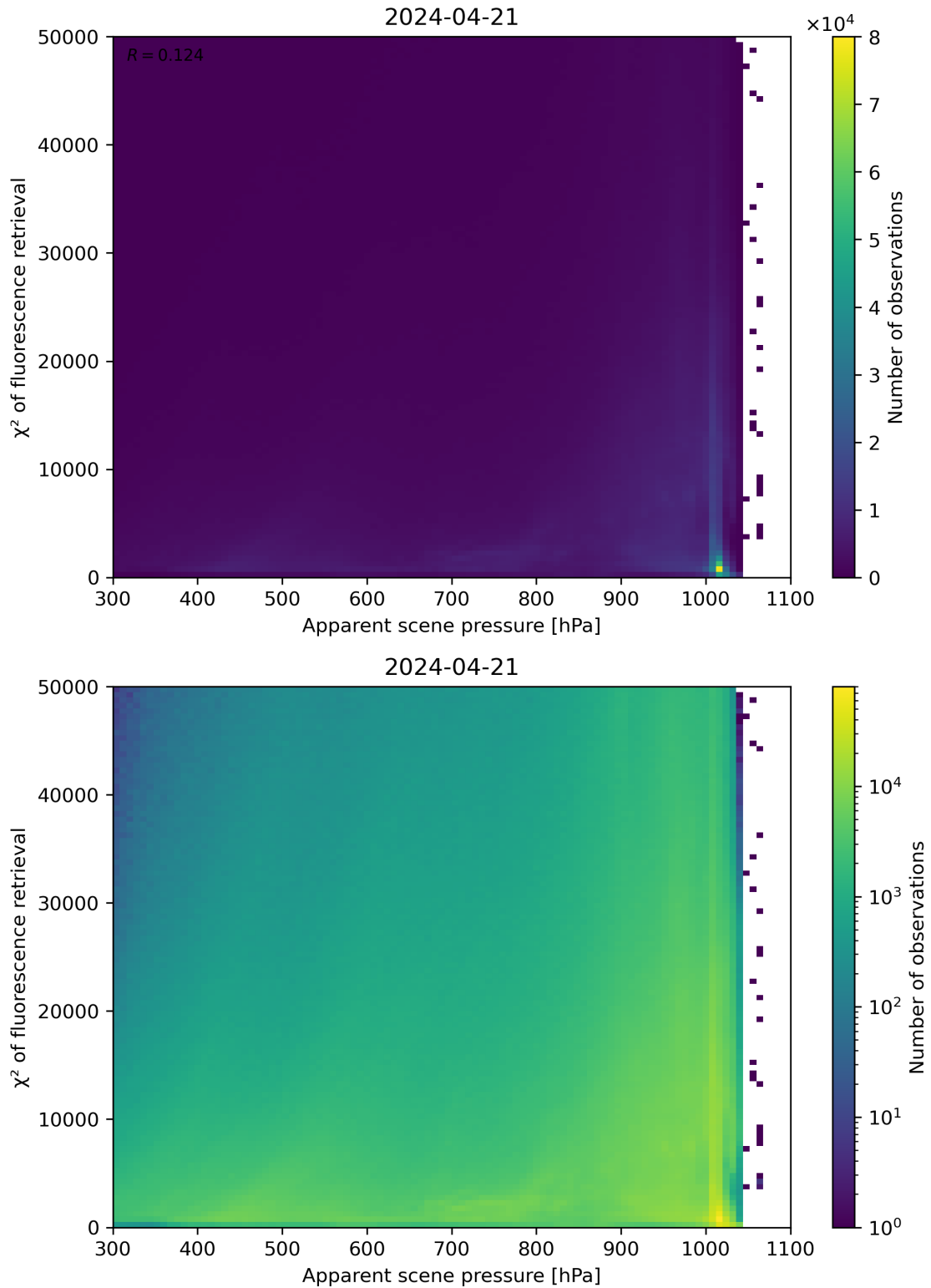
Figure 63: Scatter density plot of “Apparent scene pressure” against “ \chi^2 of fluorescence retrieval” for 2024-04-21 to 2024-04-22.
