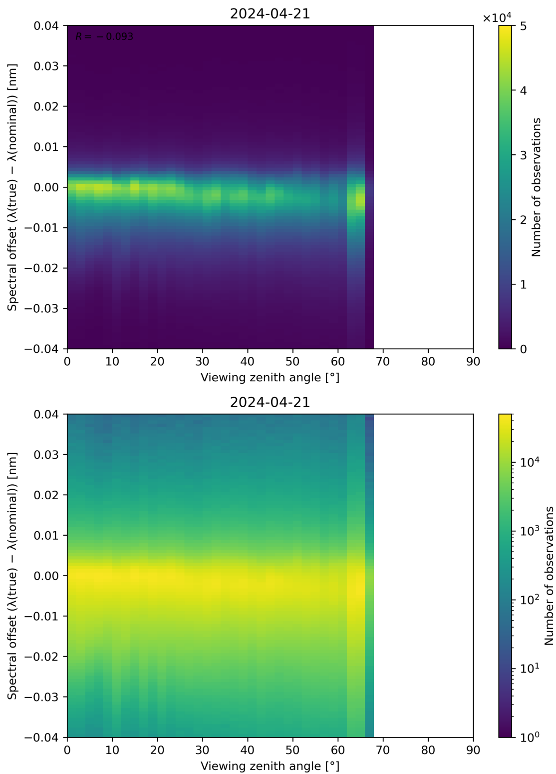
Figure 128: Scatter density plot of “Viewing zenith angle” against “Spectral offset ( \lambda(\text{true}) - \lambda(\text{nominal}) )” for 2024-04-21 to 2024-04-22.
