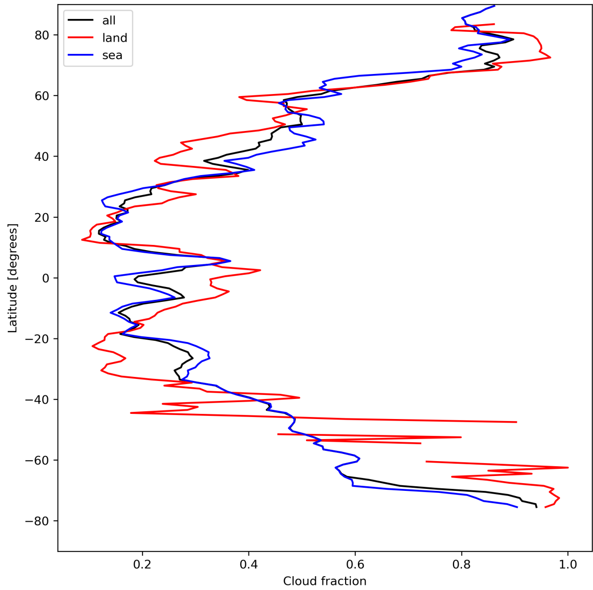
Figure 15: Zonal average of “Cloud fraction” for 2024-04-21 to 2024-04-22.
