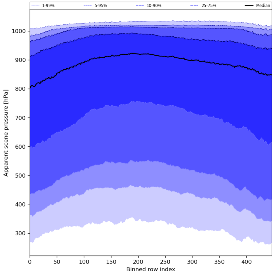
Figure 53: Along track statistics of “Apparent scene pressure” for 2024-04-21 to 2024-04-22
