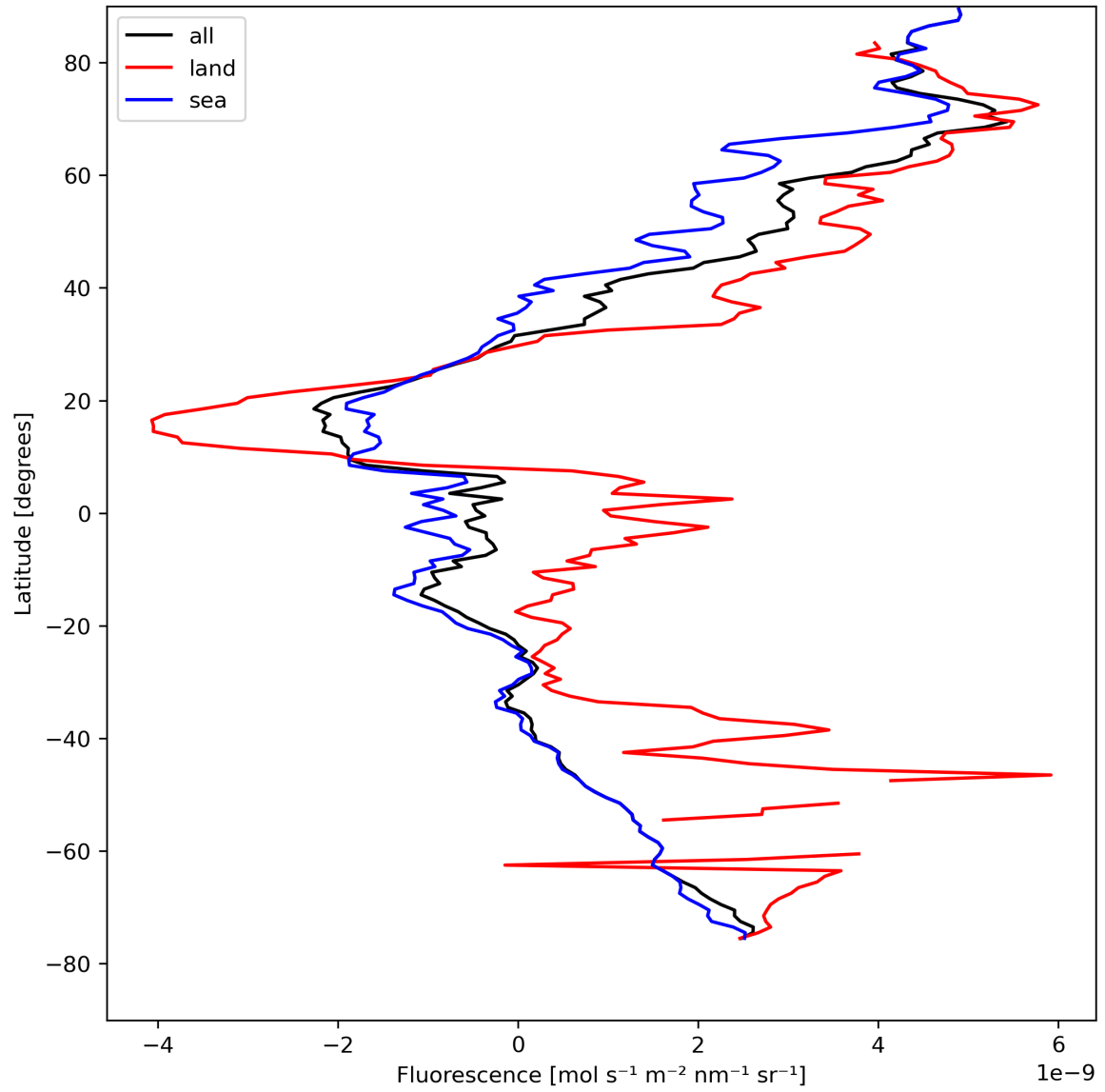
Figure 23: Zonal average of “Fluorescence” for 2024-04-21 to 2024-04-22.
