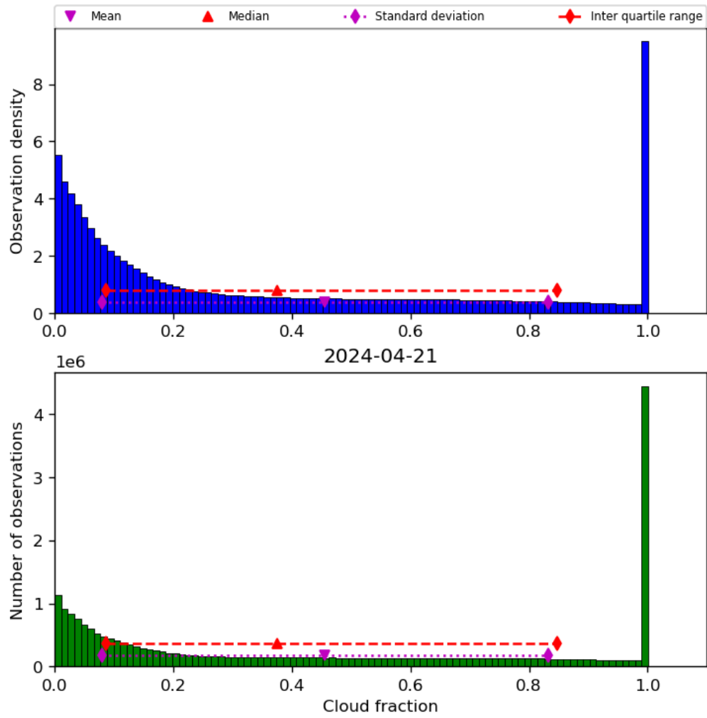
Figure 32: Histogram of “Cloud fraction” for 2024-04-21 to 2024-04-22
