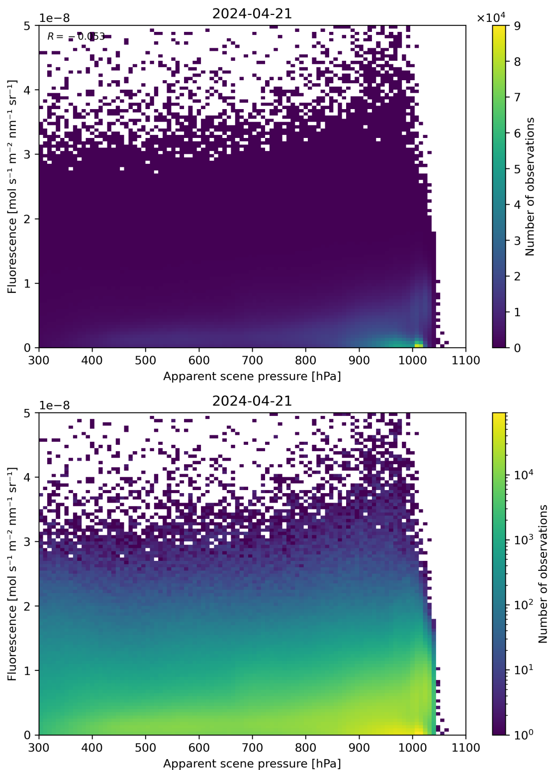
Figure 64: Scatter density plot of “Apparent scene pressure” against “Fluorescence” for 2024-04-21 to 2024-04-22.
