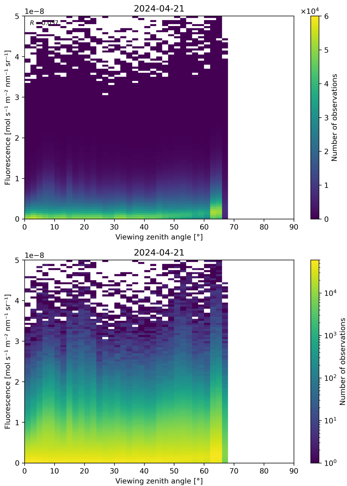
Figure 122: Scatter density plot of “Viewing zenith angle” against “Fluorescence” for 2024-04-21 to 2024-04-22.
