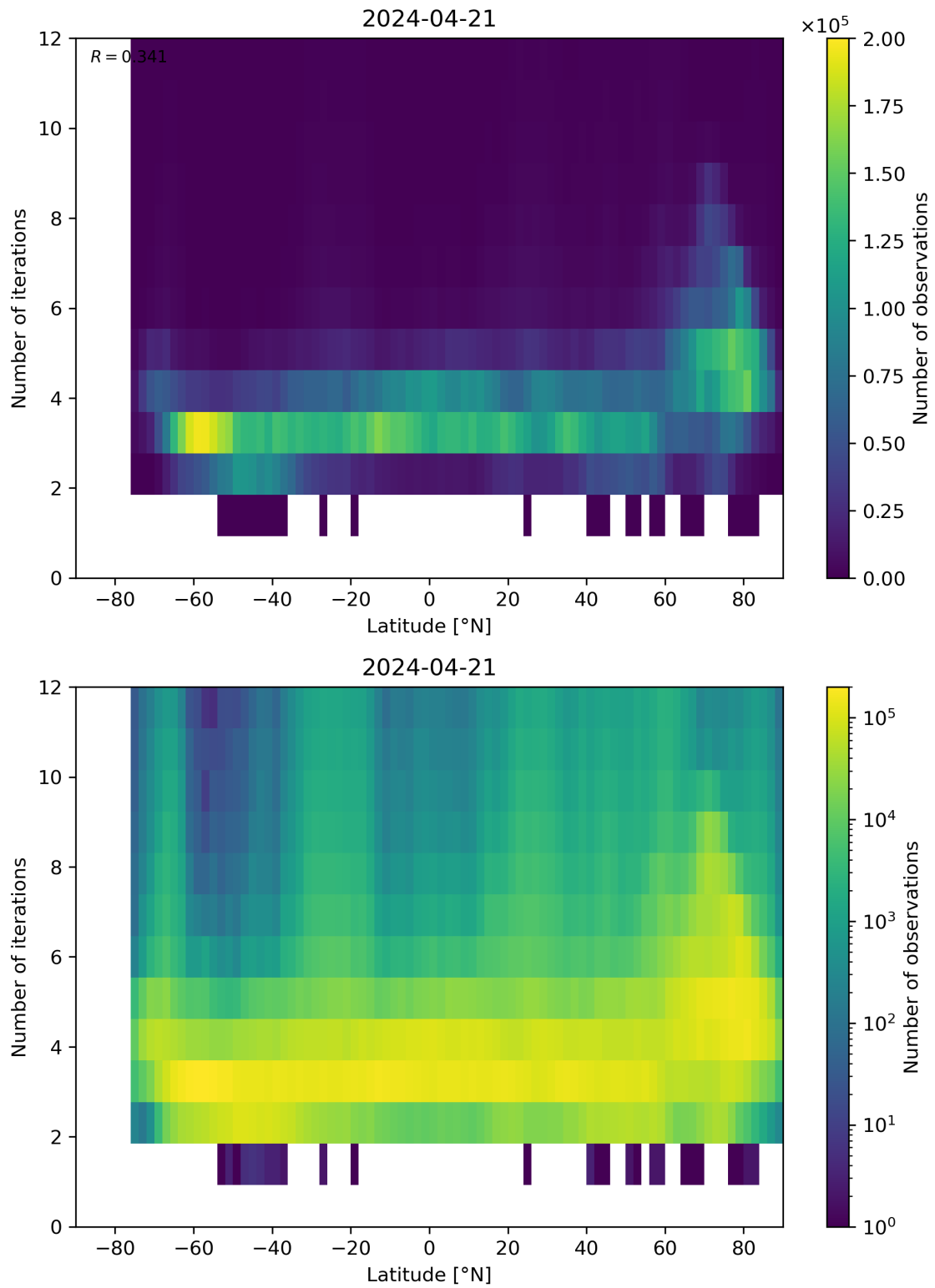
Figure 93: Scatter density plot of “Latitude” against “Number of iterations” for 2024-04-21 to 2024-04-22.
