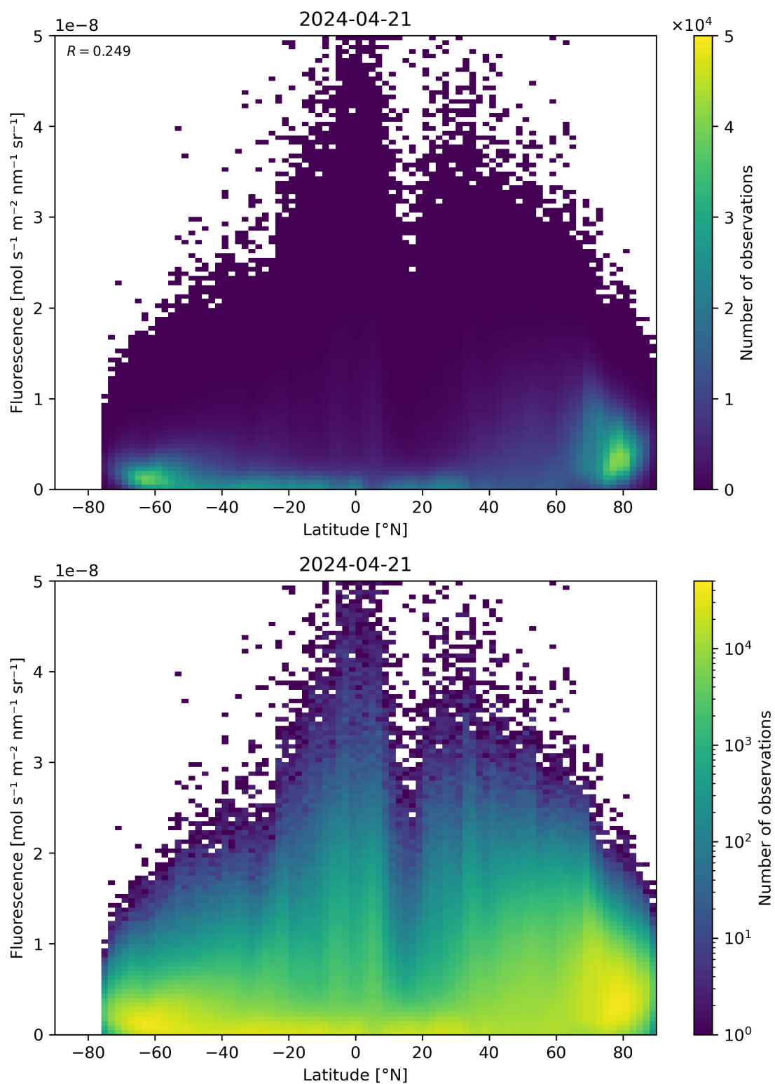
Figure 92: Scatter density plot of “Latitude” against “Fluorescence” for 2024-04-21 to 2024-04-22.
