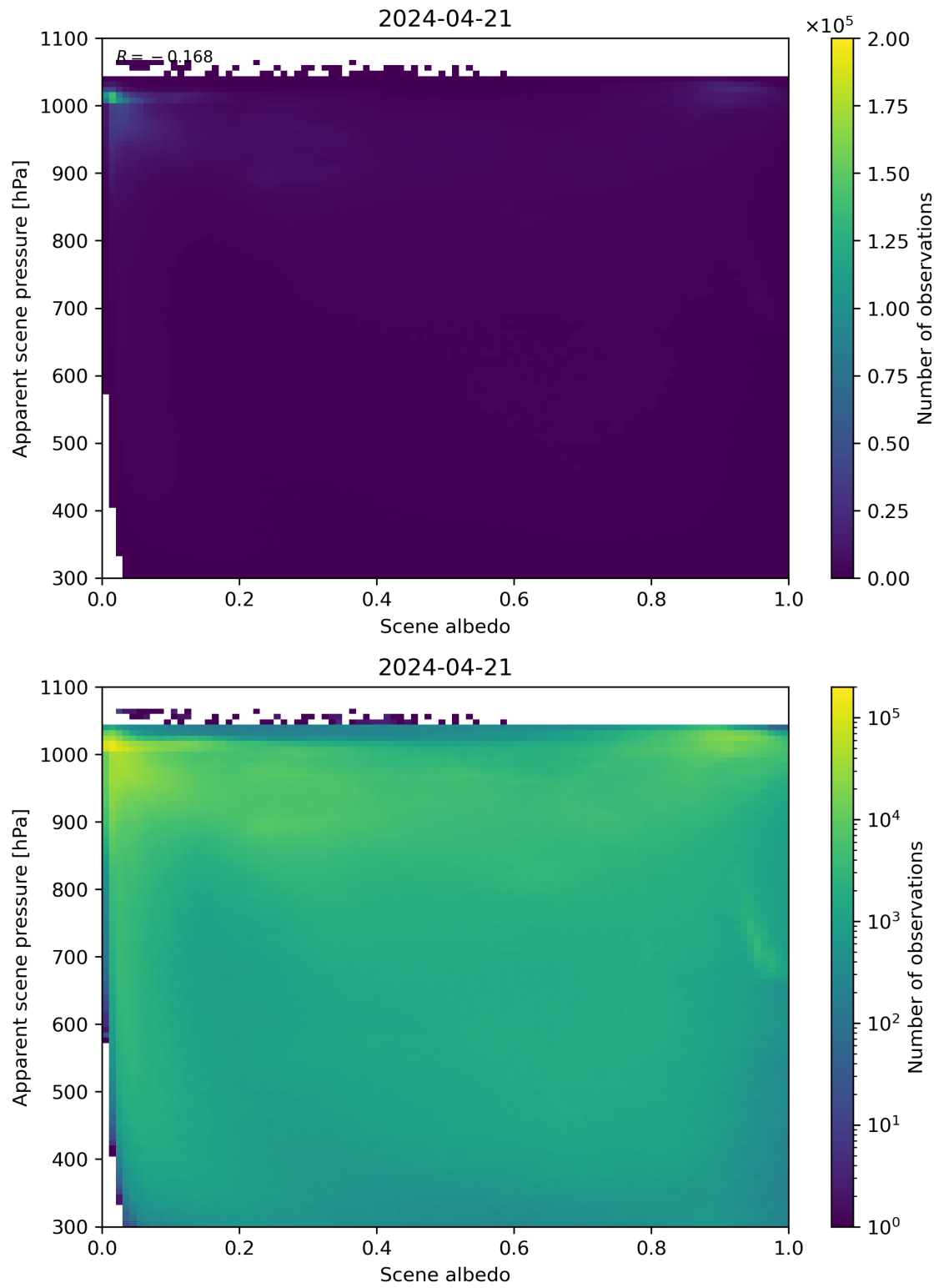
Figure 102: Scatter density plot of “Scene albedo” against “Apparent scene pressure” for 2024-04-21 to 2024-04-22.
