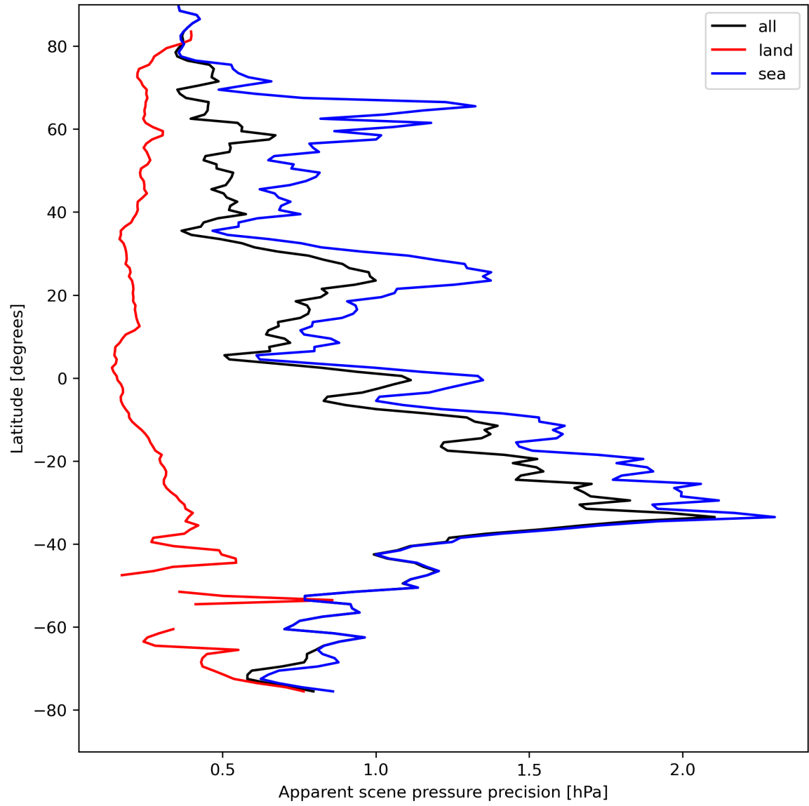
Figure 20: Zonal average of “Apparent scene pressure precision” for 2024-04-21 to 2024-04-22.
