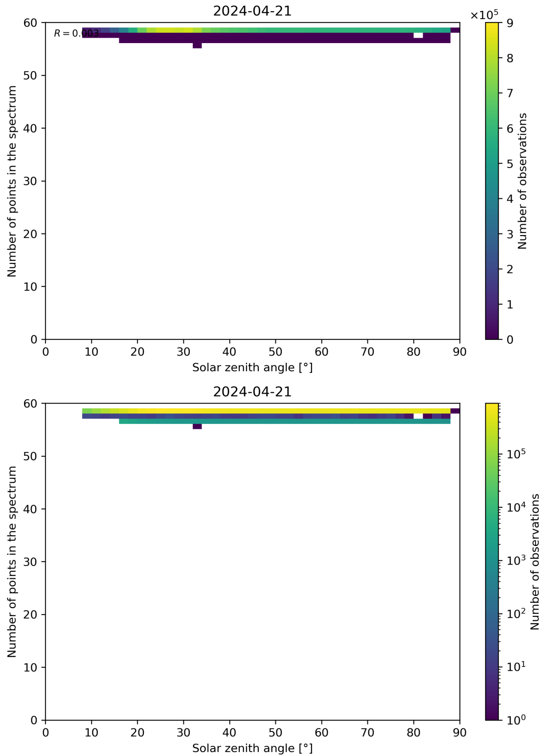
Figure 115: Scatter density plot of “Solar zenith angle” against “Number of points in the spectrum” for 2024-04-21 to 2024-04-22.
