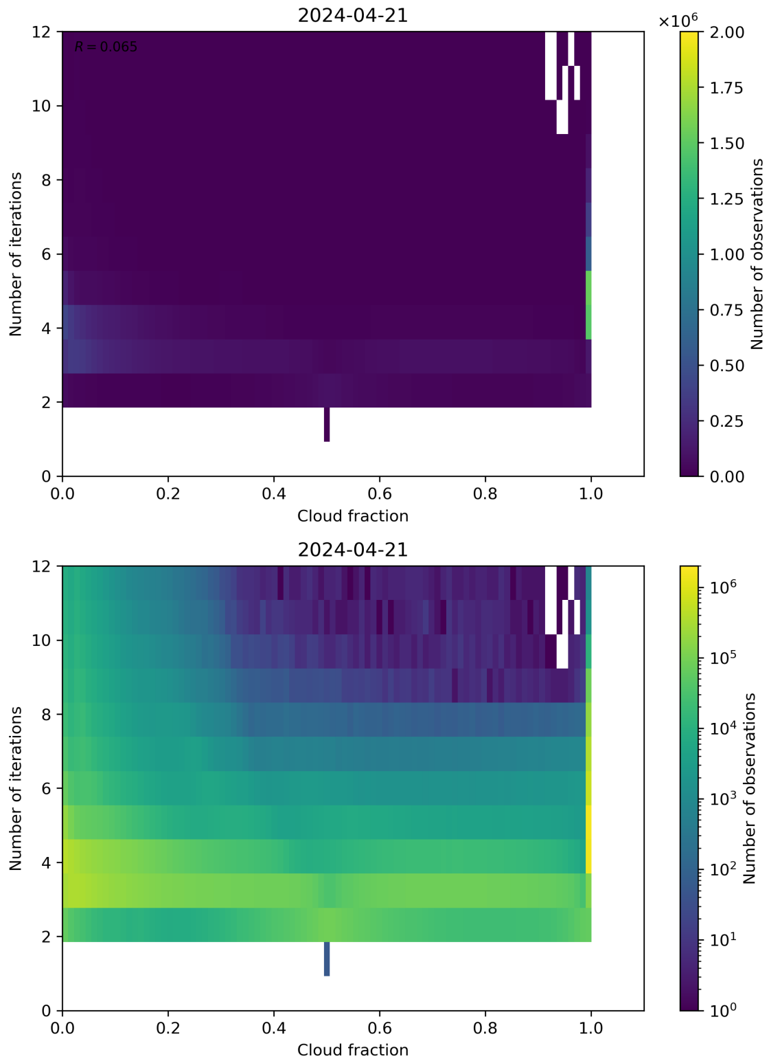
Figure 73: Scatter density plot of “Cloud fraction” against “Number of iterations” for 2024-04-21 to 2024-04-22.
