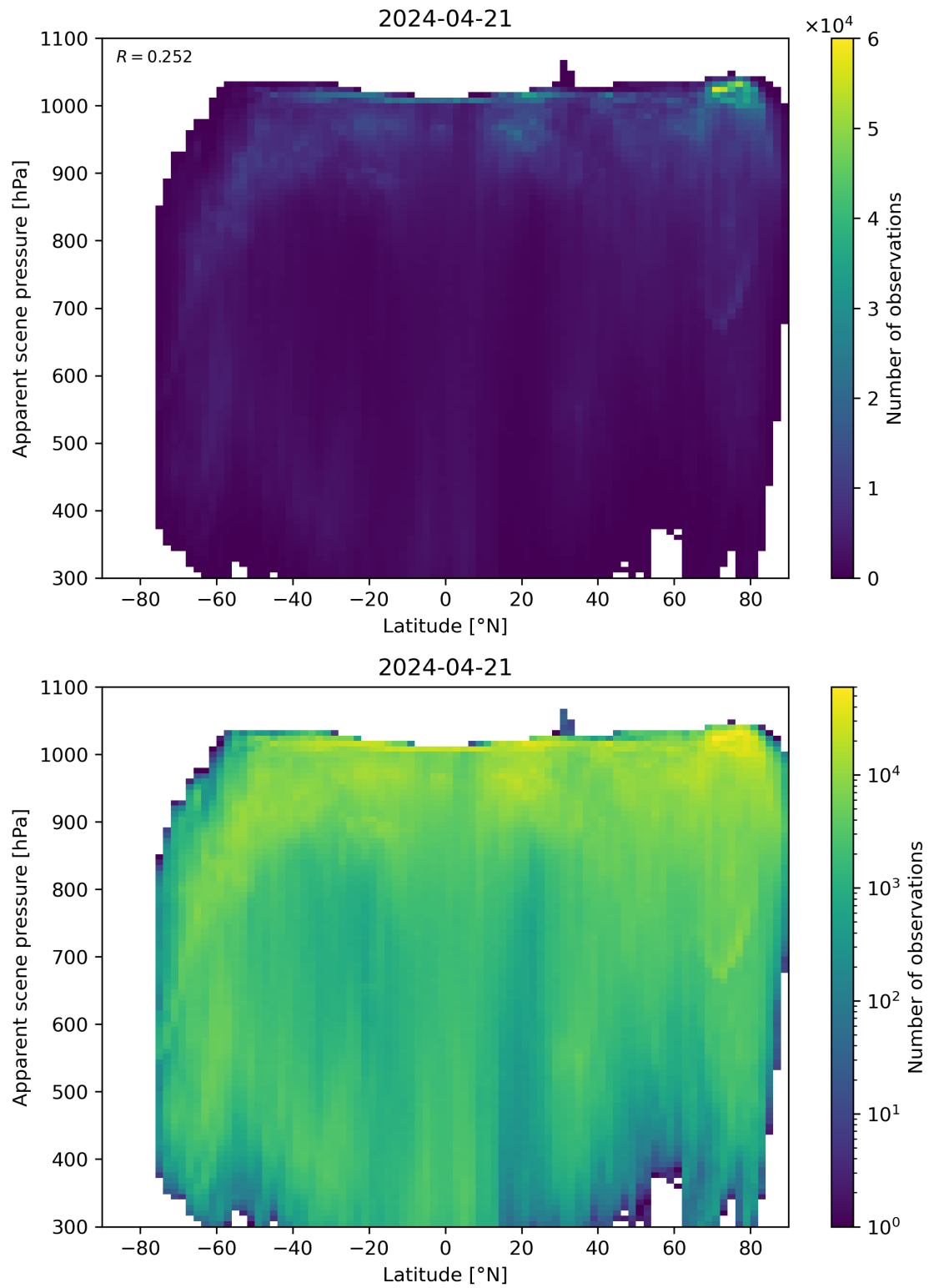
Figure 88: Scatter density plot of “Latitude” against “Apparent scene pressure” for 2024-04-21 to 2024-04-22.
