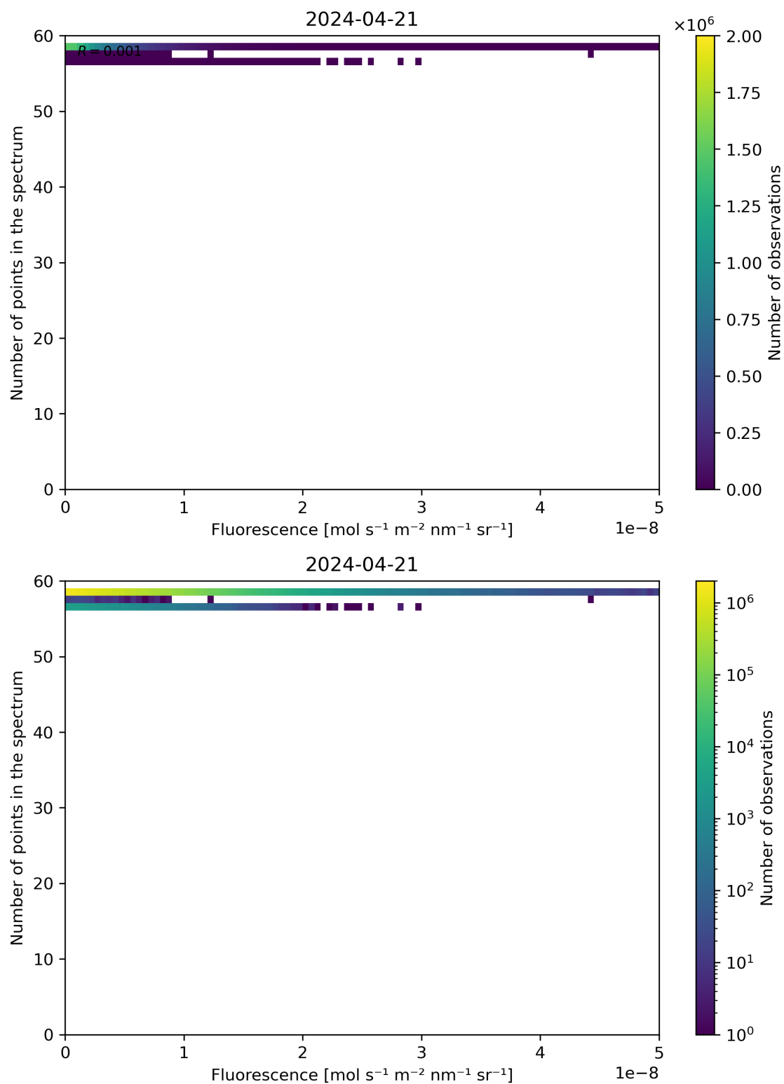
Figure 86: Scatter density plot of “Fluorescence” against “Number of points in the spectrum” for 2024-04-21 to 2024-04-22.
