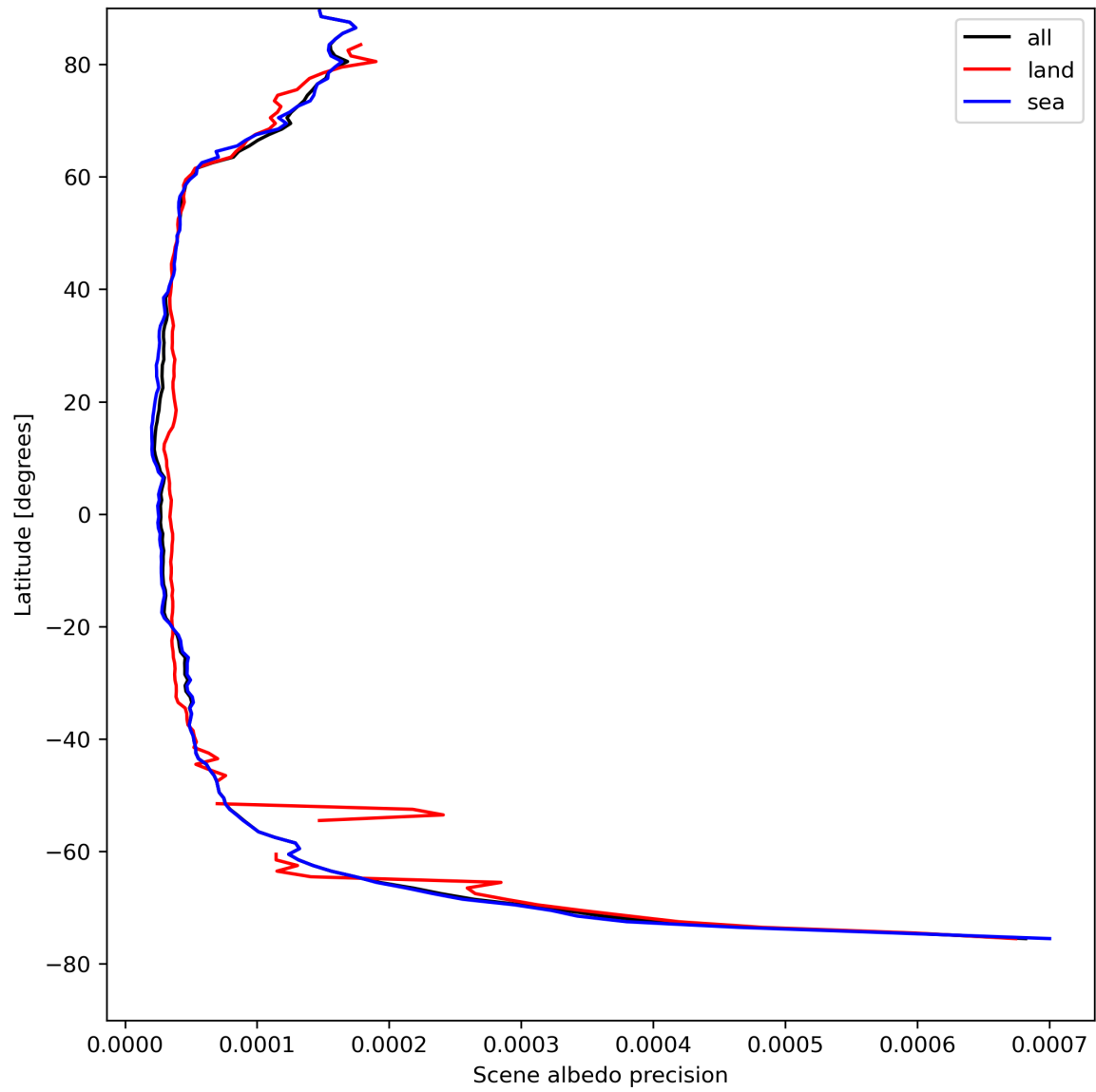
Figure 18: Zonal average of “Scene albedo precision” for 2024-04-21 to 2024-04-22.
