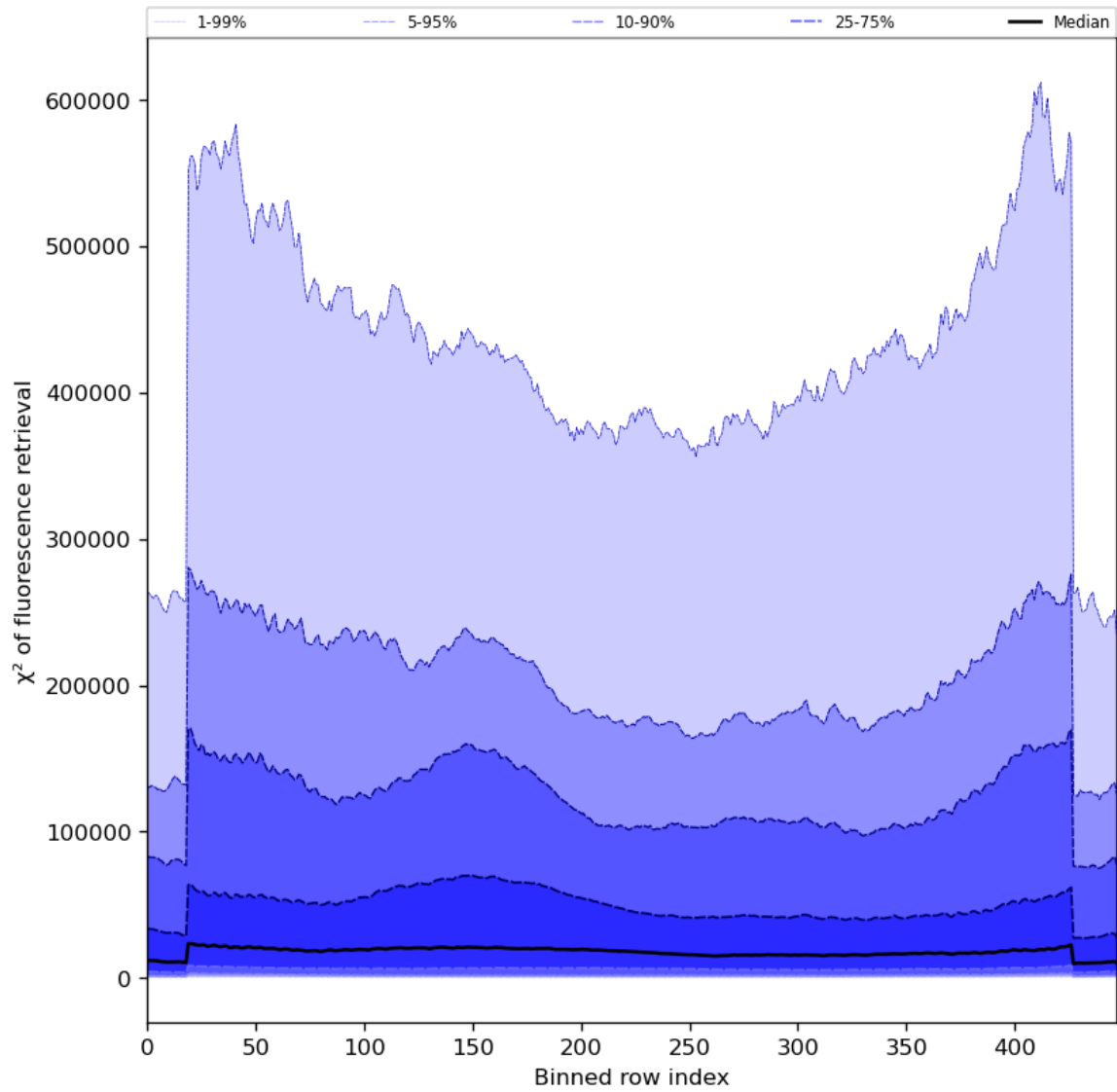
Figure 59: Along track statistics of “ \chi^2 of fluorescence retrieval” for 2024-04-21 to 2024-04-22
