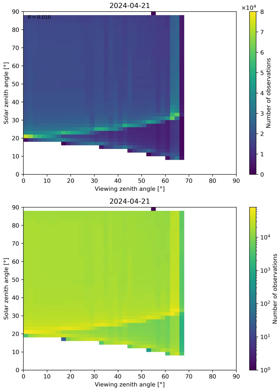
Figure 127: Scatter density plot of “Viewing zenith angle” against “Solar zenith angle” for 2024-04-21 to 2024-04-22.
