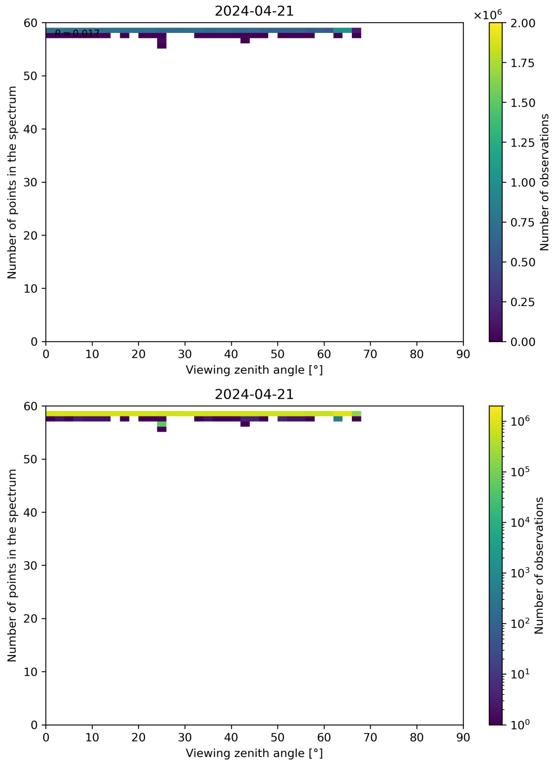
Figure 125: Scatter density plot of “Viewing zenith angle” against “Number of points in the spectrum” for 2024-04-21 to 2024-04-22.
