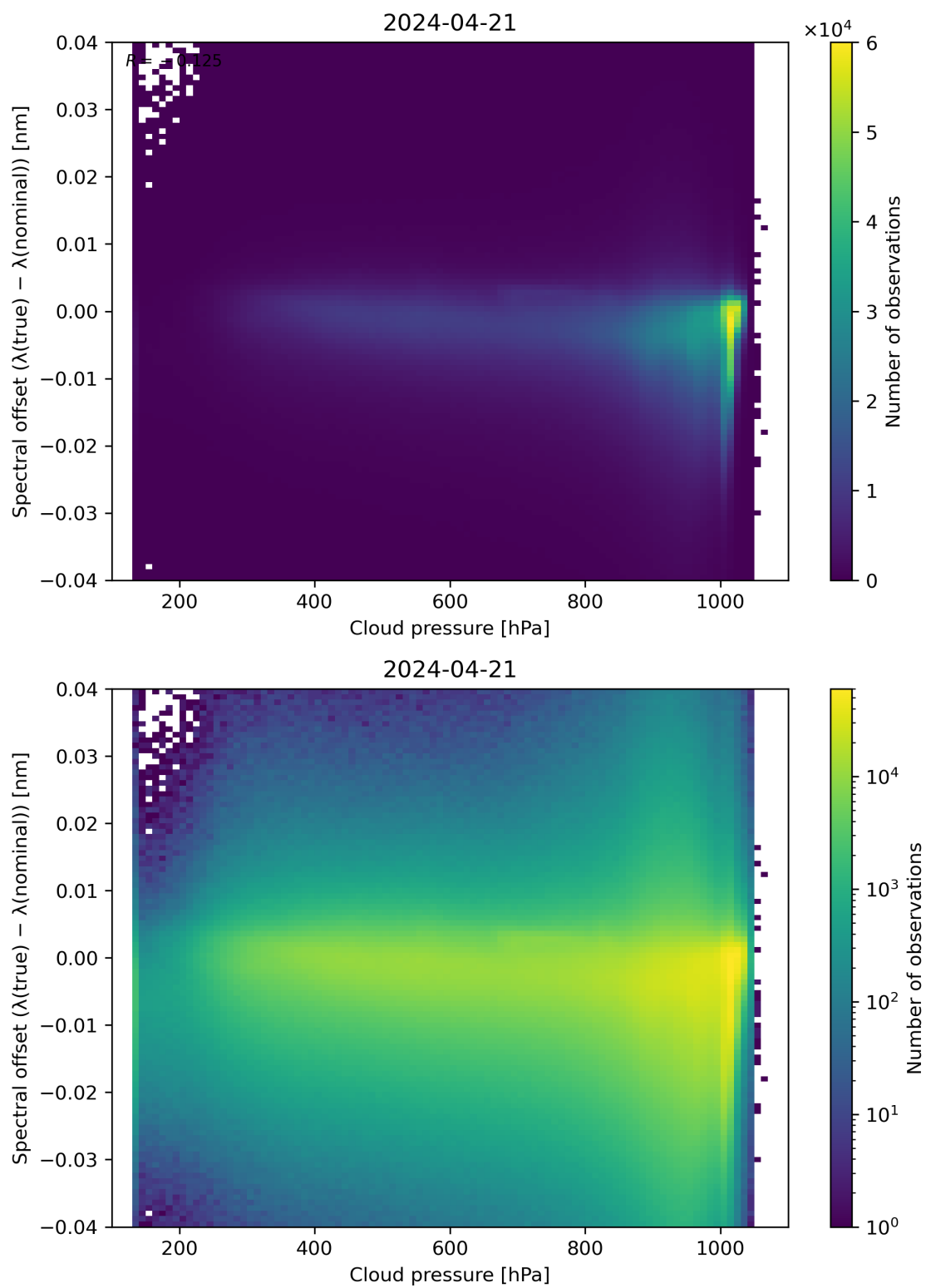
Figure 84: Scatter density plot of “Cloud pressure” against “Spectral offset ( \lambda(\text{true}) - \lambda(\text{nominal}) )” for 2024-04-21 to 2024-04-22.
