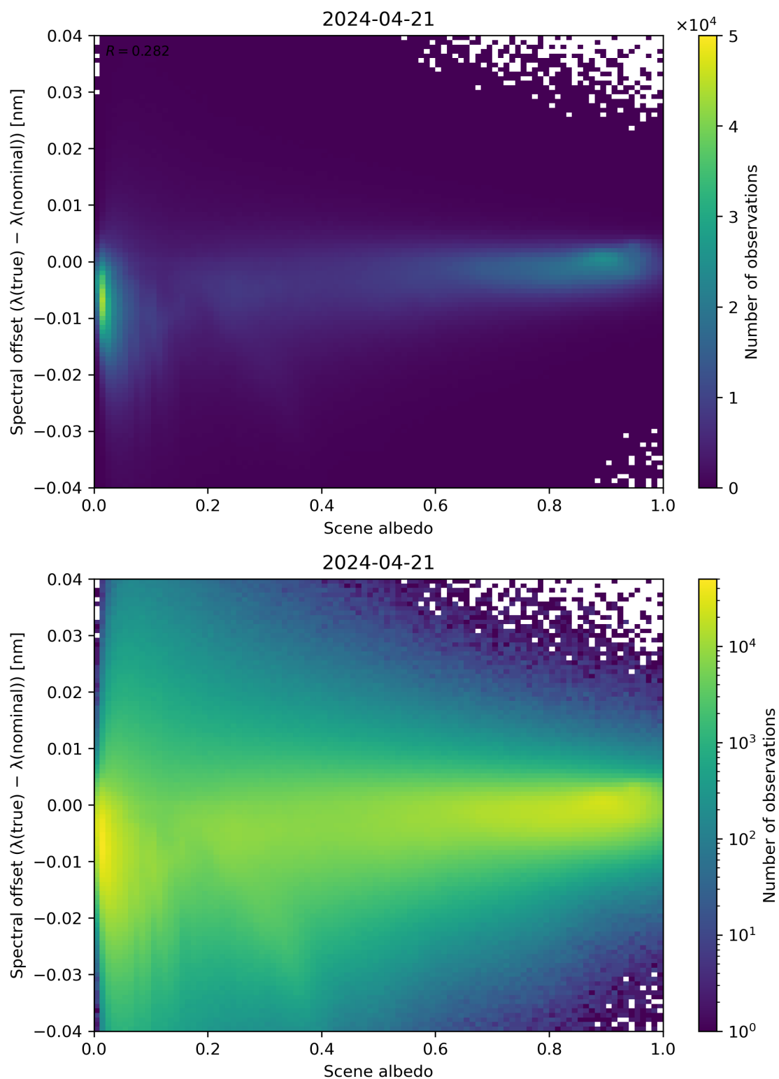
Figure 107: Scatter density plot of “Scene albedo” against “Spectral offset ( \lambda(\text{true}) - \lambda(\text{nominal}) )” for 2024-04-21 to 2024-04-22.
