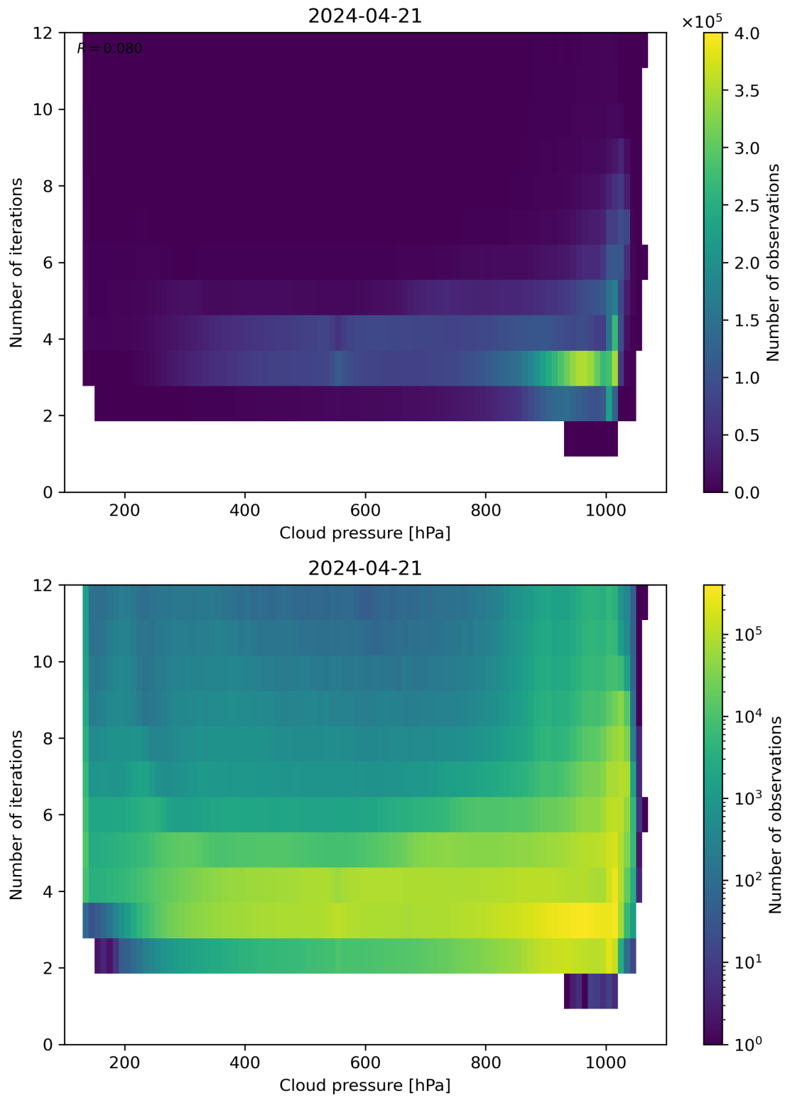
Figure 81: Scatter density plot of “Cloud pressure” against “Number of iterations” for 2024-04-21 to 2024-04-22.
