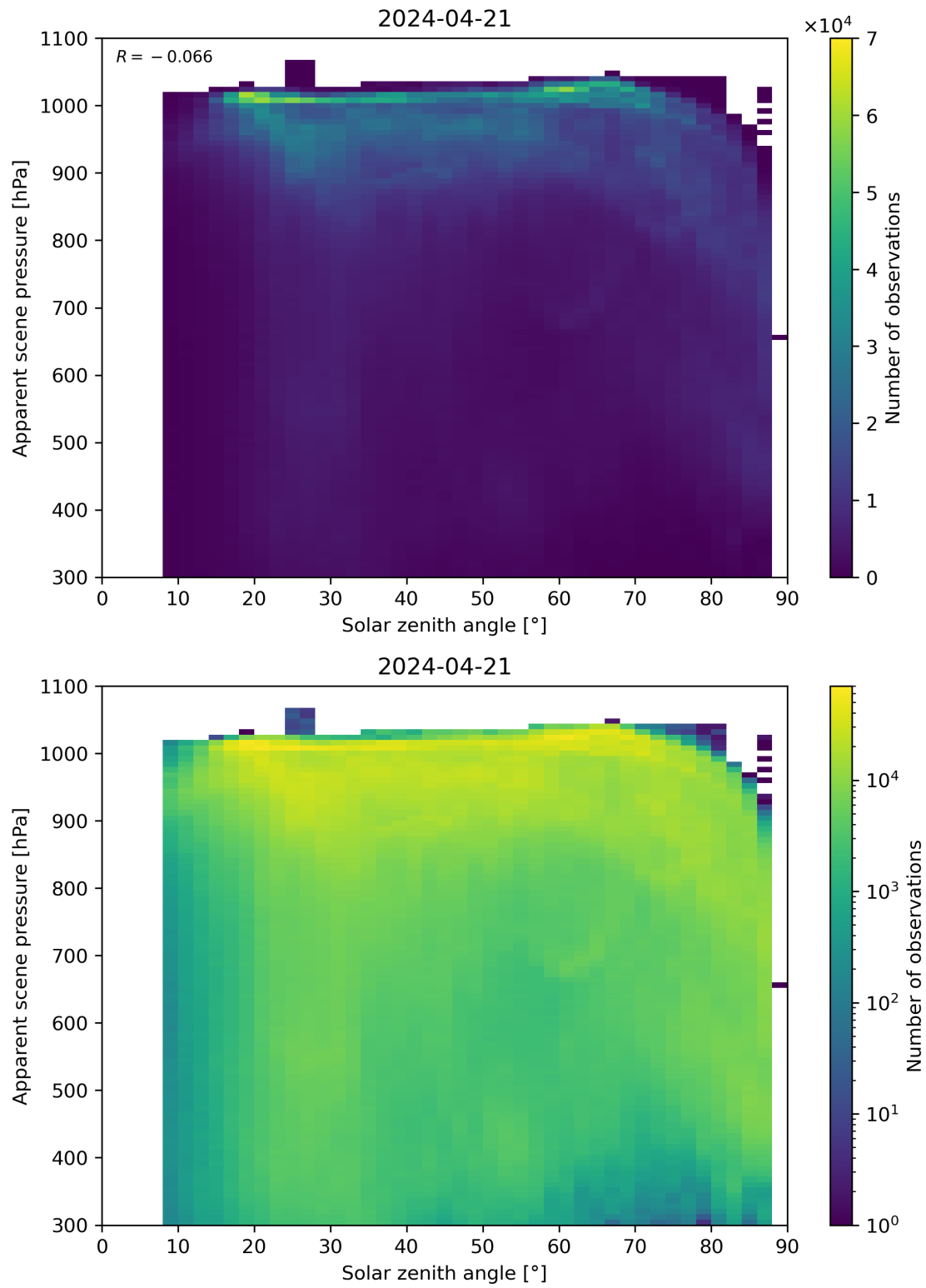
Figure 108: Scatter density plot of “Solar zenith angle” against “Apparent scene pressure” for 2024-04-21 to 2024-04-22.
