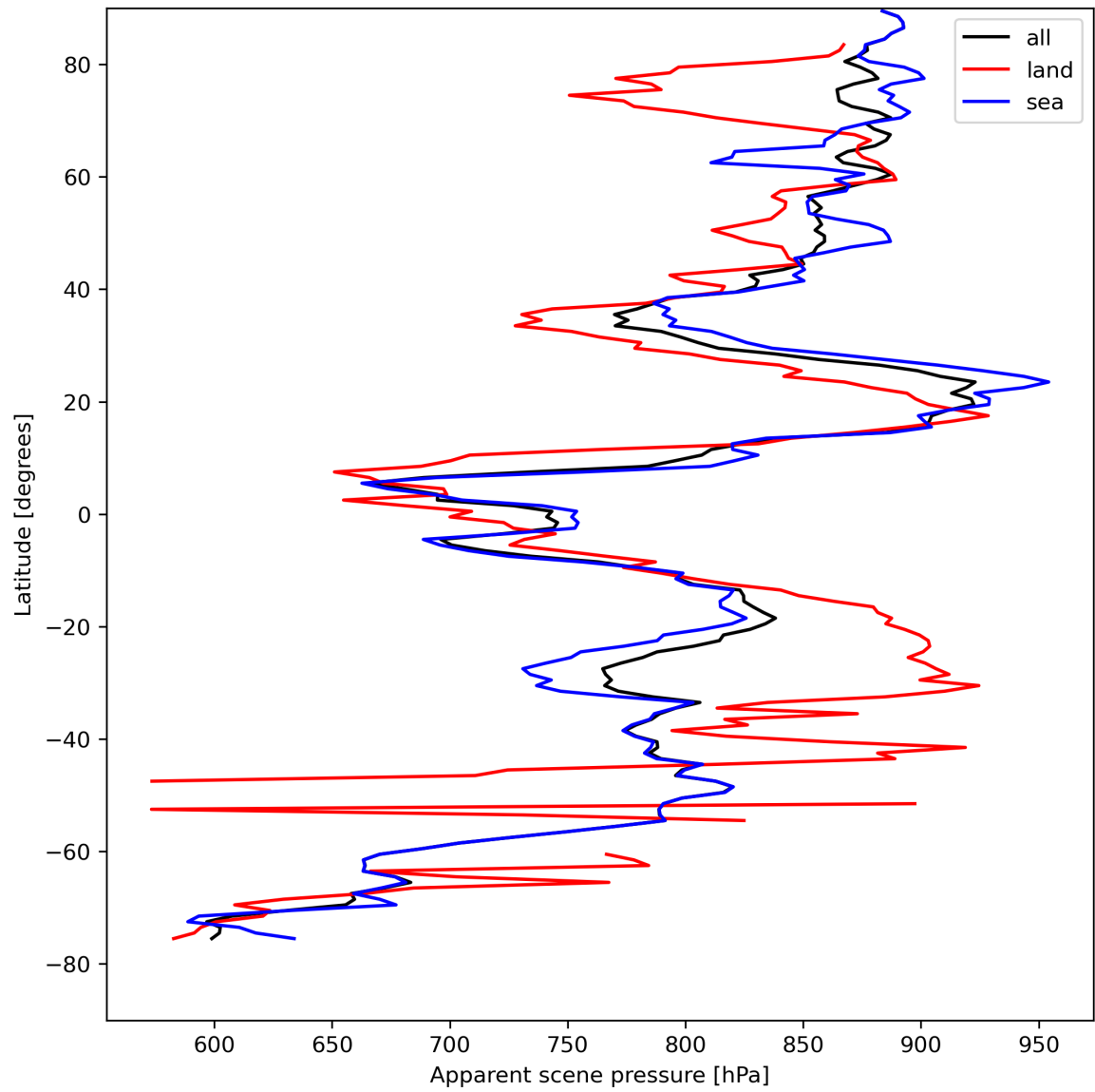
Figure 19: Zonal average of “Apparent scene pressure” for 2024-04-21 to 2024-04-22.
