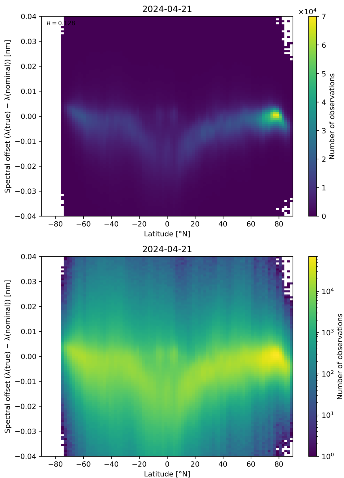
Figure 96: Scatter density plot of “Latitude” against “Spectral offset ( \lambda(\text{true}) - \lambda(\text{nominal}) )” for 2024-04-21 to 2024-04-22.
