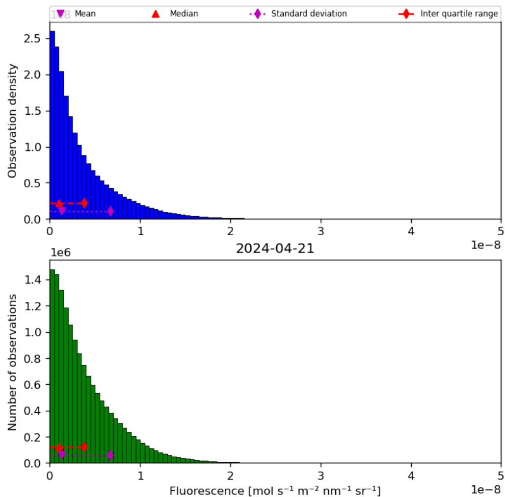
Figure 40: Histogram of “Fluorescence” for 2024-04-21 to 2024-04-22
