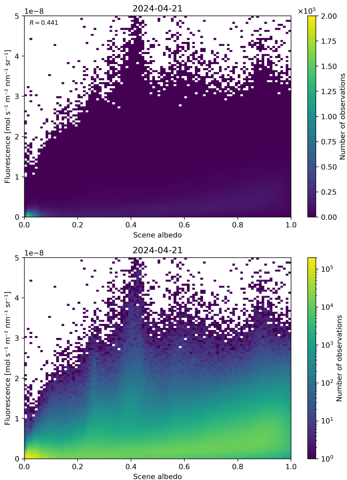
Figure 104: Scatter density plot of “Scene albedo” against “Fluorescence” for 2024-04-21 to 2024-04-22.
