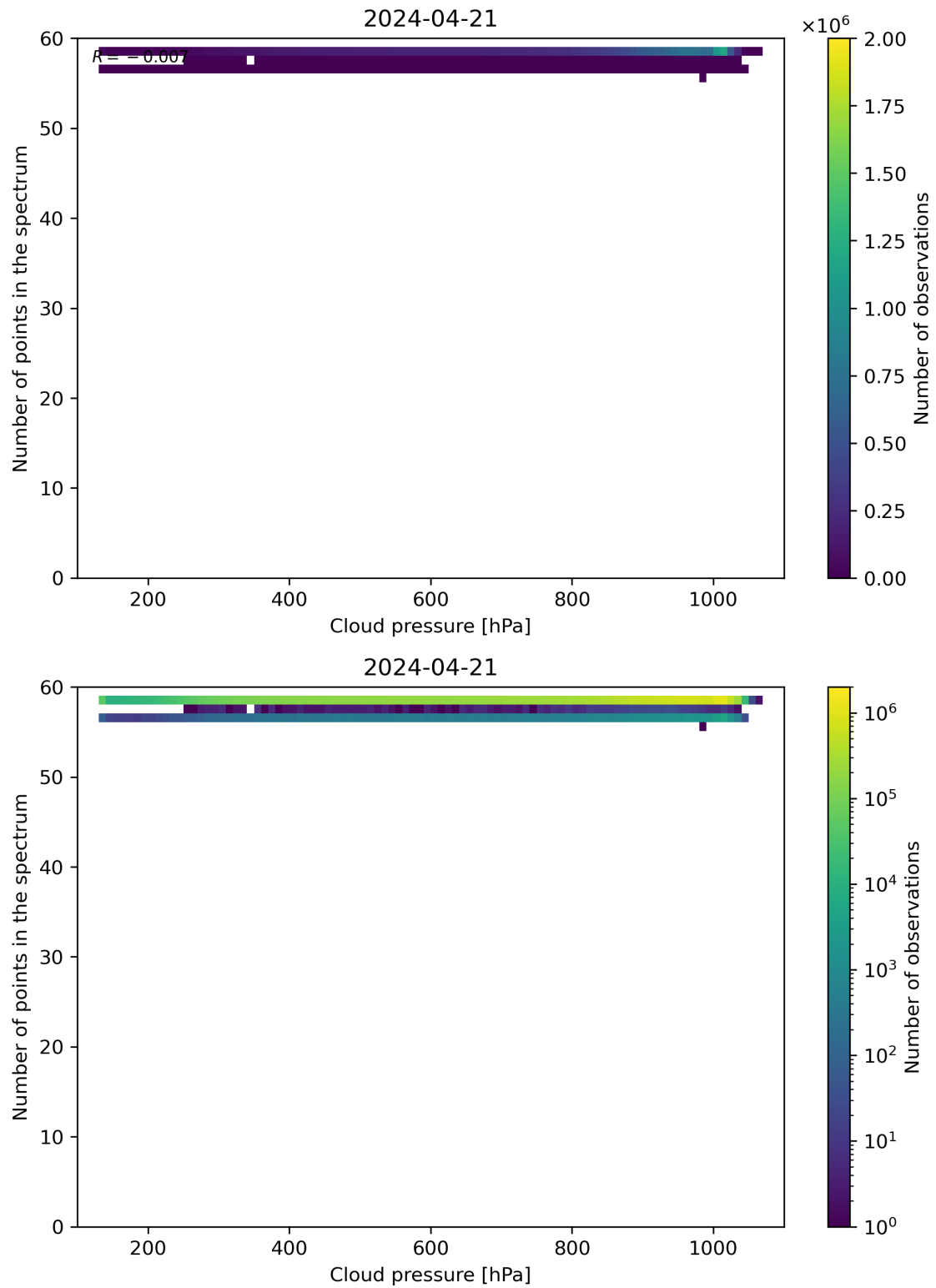
Figure 82: Scatter density plot of “Cloud pressure” against “Number of points in the spectrum” for 2024-04-21 to 2024-04-22.
