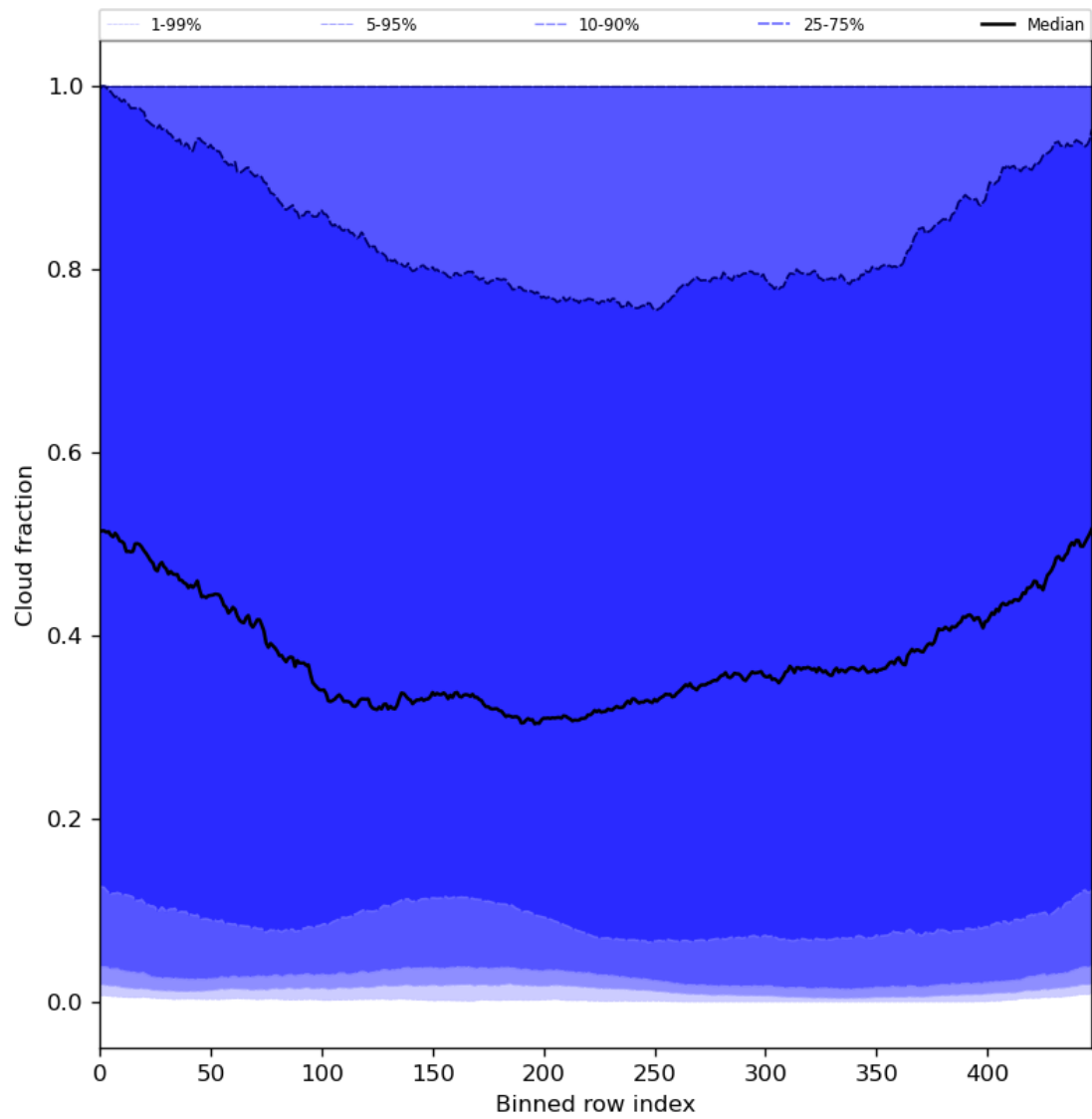
Figure 49: Along track statistics of “Cloud fraction” for 2024-04-21 to 2024-04-22
