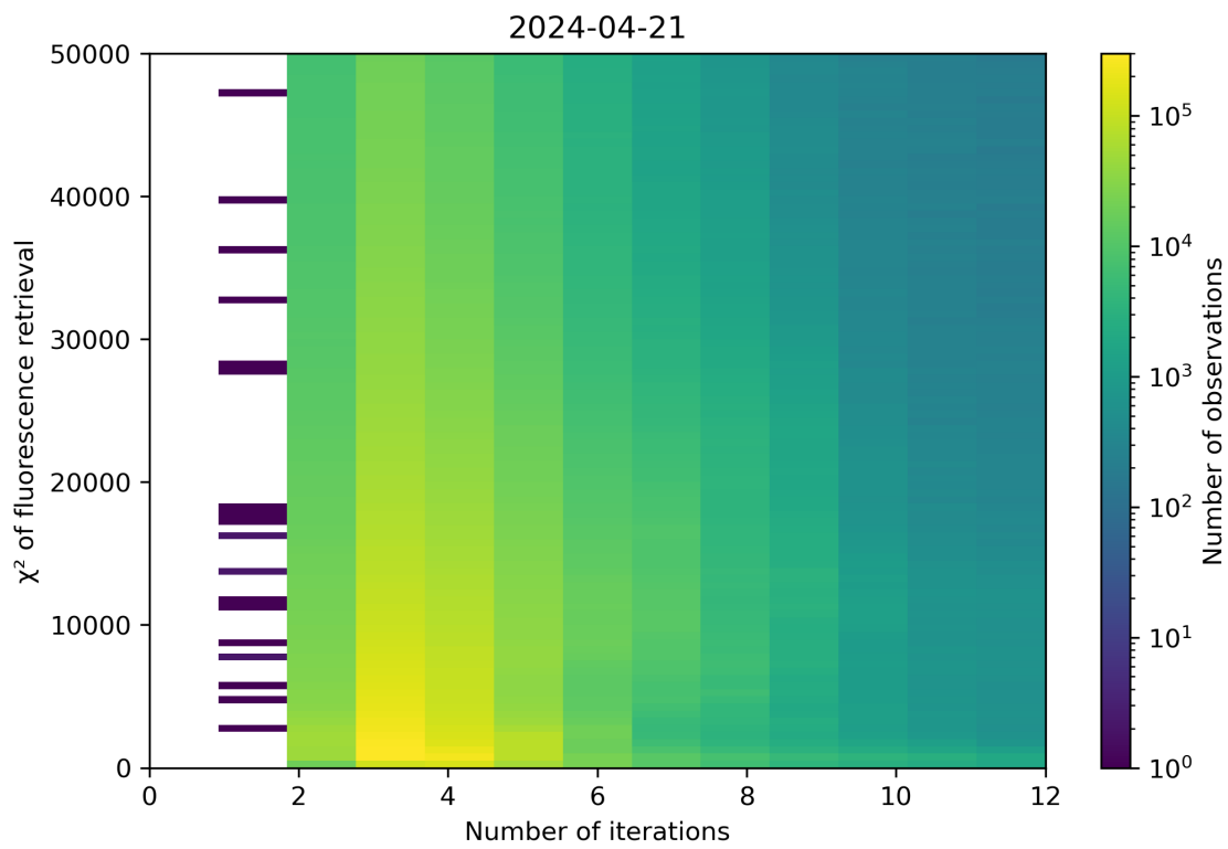
Figure 97: Scatter density plot of “Number of iterations” against “ \chi^2 of fluorescence retrieval” for 2024-04-21 to 2024-04-22.
