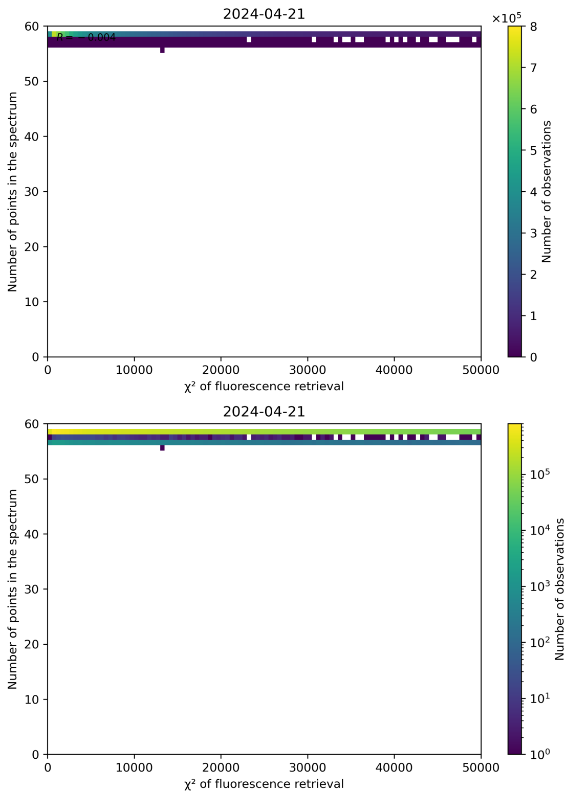
Figure 68: Scatter density plot of “ \chi^2 of fluorescence retrieval” against “Number of points in the spectrum” for 2024-04-21 to 2024-04-22.
