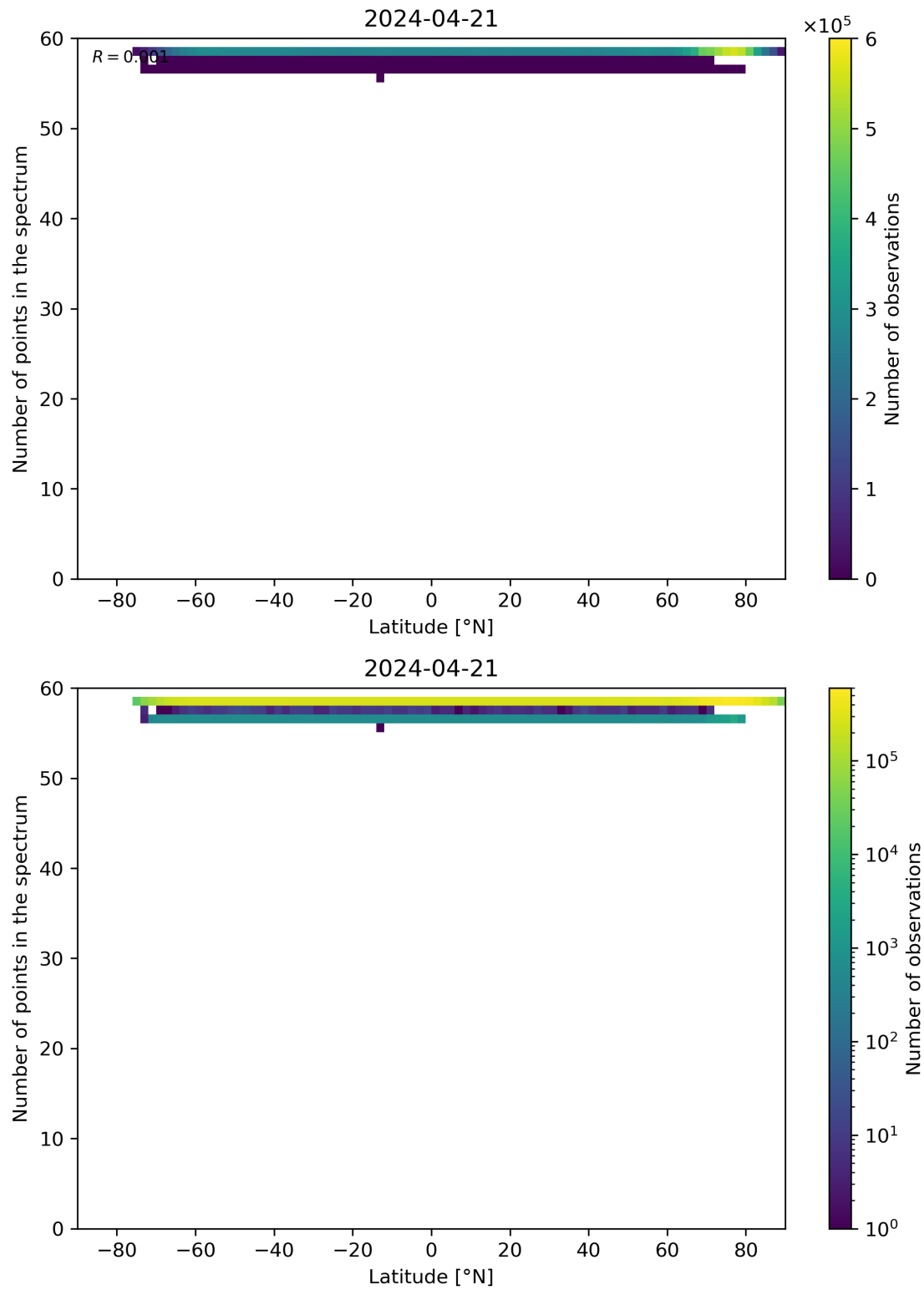
Figure 94: Scatter density plot of “Latitude” against “Number of points in the spectrum” for 2024-04-21 to 2024-04-22.
