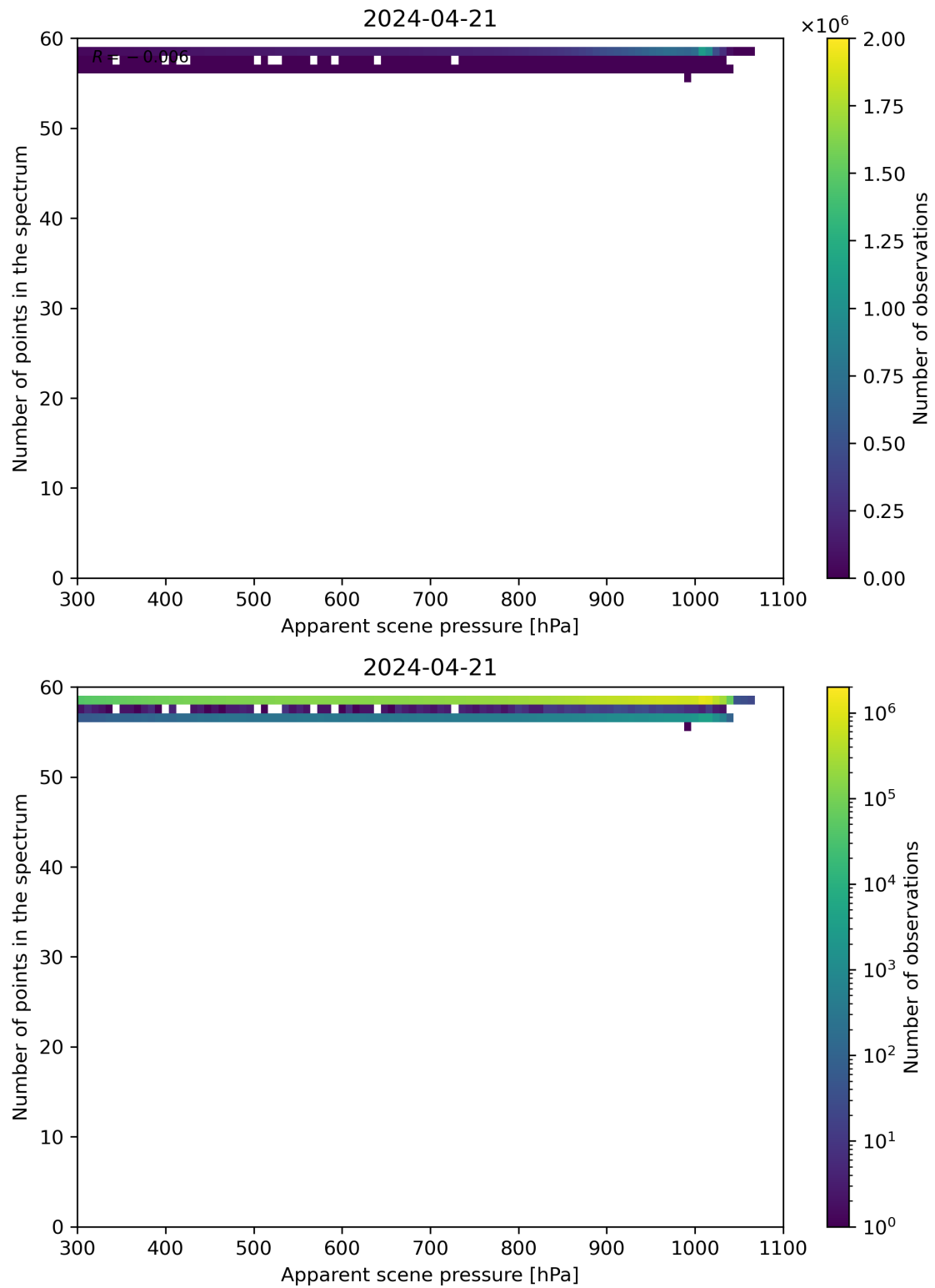
Figure 66: Scatter density plot of “Apparent scene pressure” against “Number of points in the spectrum” for 2024-04-21 to 2024-04-22.
