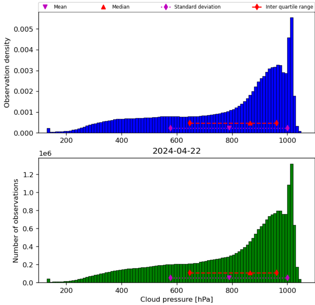
Figure 30: Histogram of “Cloud pressure” for 2024-04-21 to 2024-04-23
