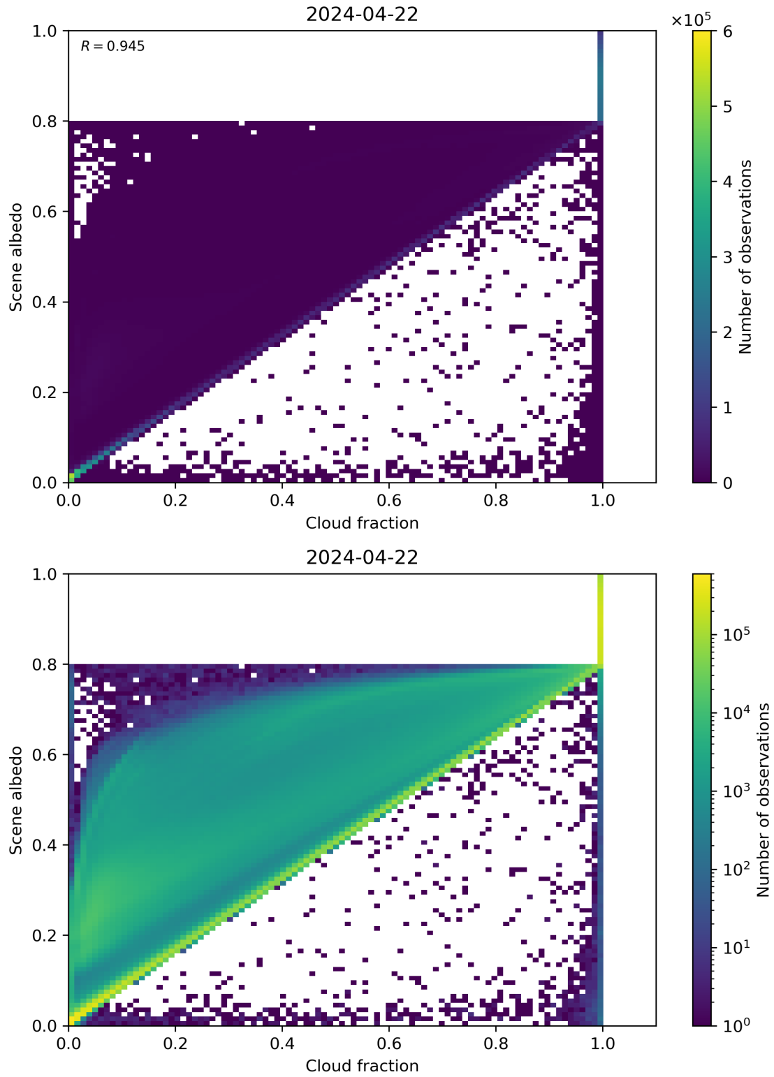
Figure 75: Scatter density plot of “Cloud fraction” against “Scene albedo” for 2024-04-21 to 2024-04-23.
