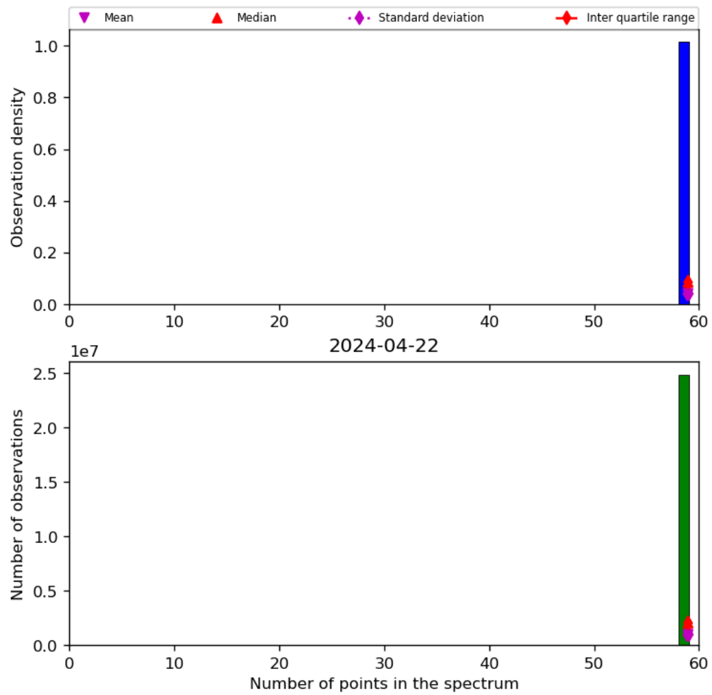
Figure 44: Histogram of “Number of points in the spectrum” for 2024-04-21 to 2024-04-23
