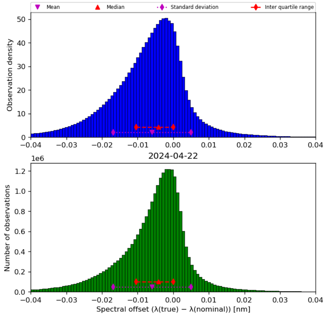
Figure 45: Histogram of “Spectral offset ( \lambda(\text{true}) - \lambda(\text{nominal}) )” for 2024-04-21 to 2024-04-23
