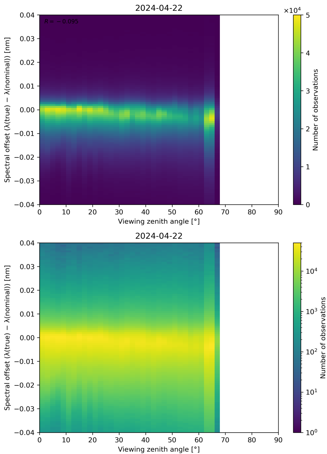
Figure 128: Scatter density plot of “Viewing zenith angle” against “Spectral offset ( \lambda(\text{true}) - \lambda(\text{nominal}) )” for 2024-04-21 to 2024-04-23.
