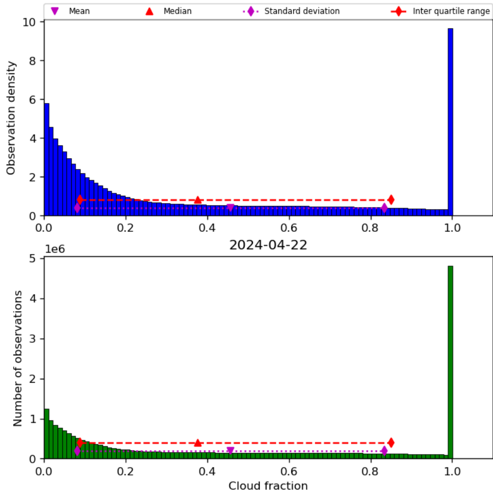
Figure 32: Histogram of “Cloud fraction” for 2024-04-21 to 2024-04-23
