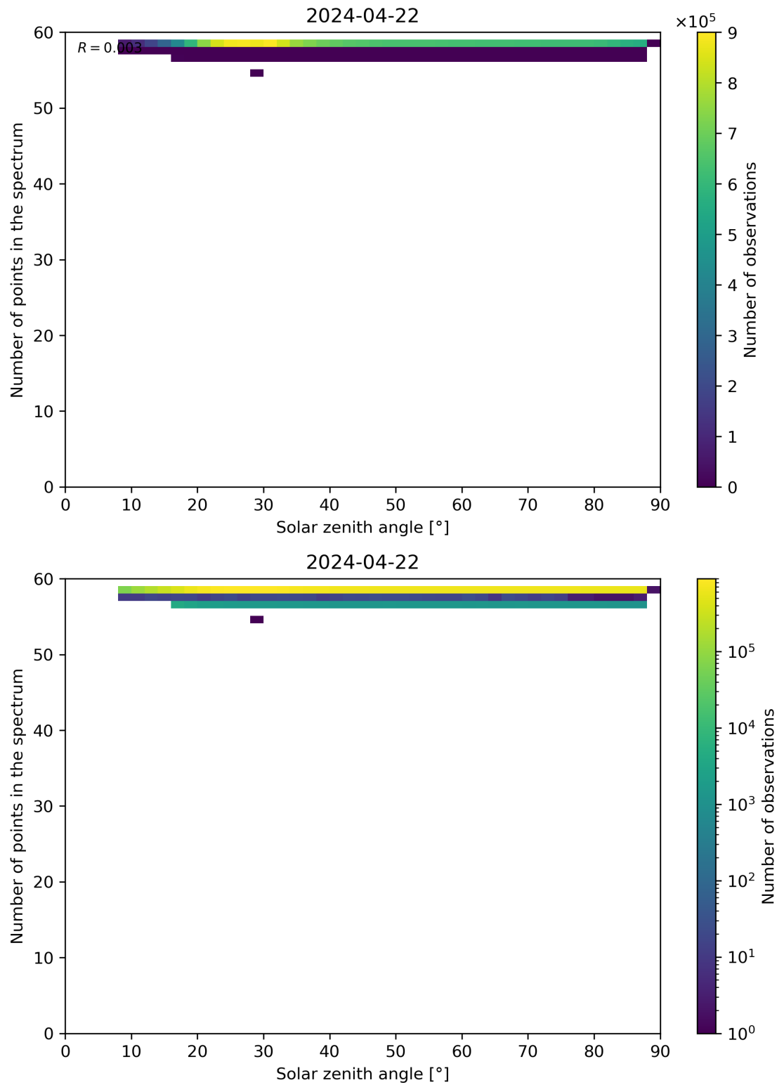
Figure 115: Scatter density plot of “Solar zenith angle” against “Number of points in the spectrum” for 2024-04-21 to 2024-04-23.
