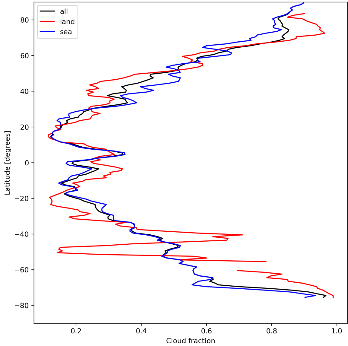
Figure 15: Zonal average of “Cloud fraction” for 2024-04-21 to 2024-04-23.
