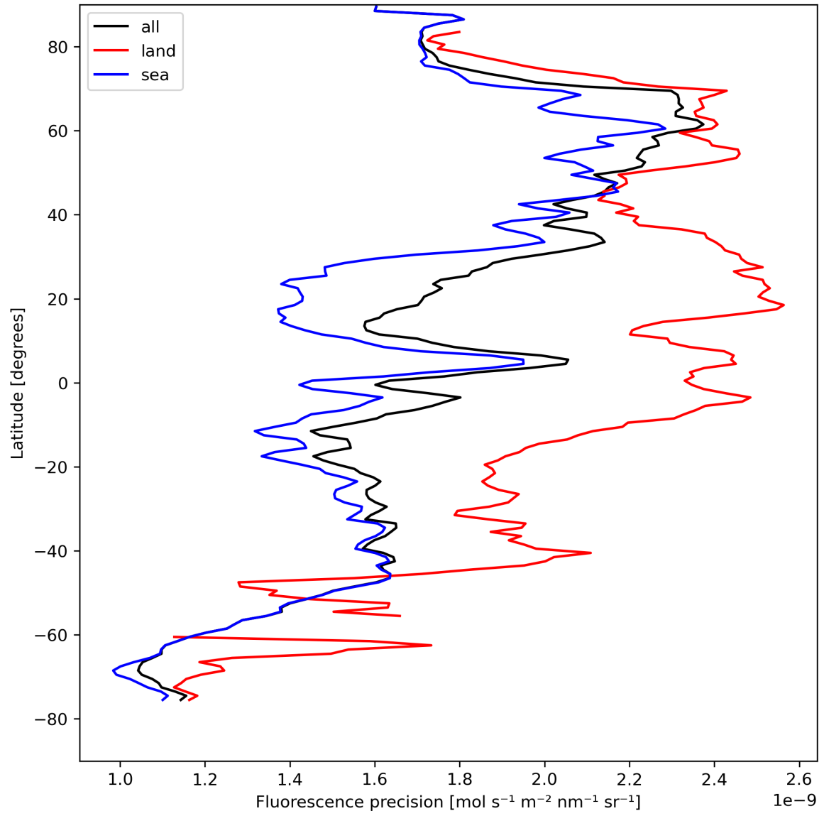
Figure 24: Zonal average of “Fluorescence precision” for 2024-04-21 to 2024-04-23.
