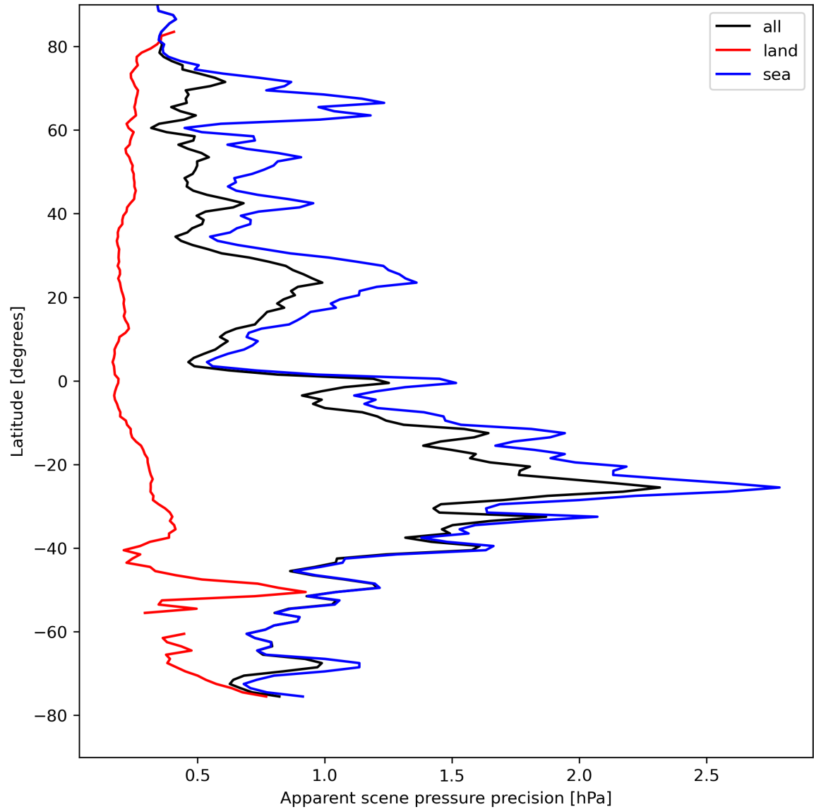
Figure 20: Zonal average of “Apparent scene pressure precision” for 2024-04-21 to 2024-04-23.
