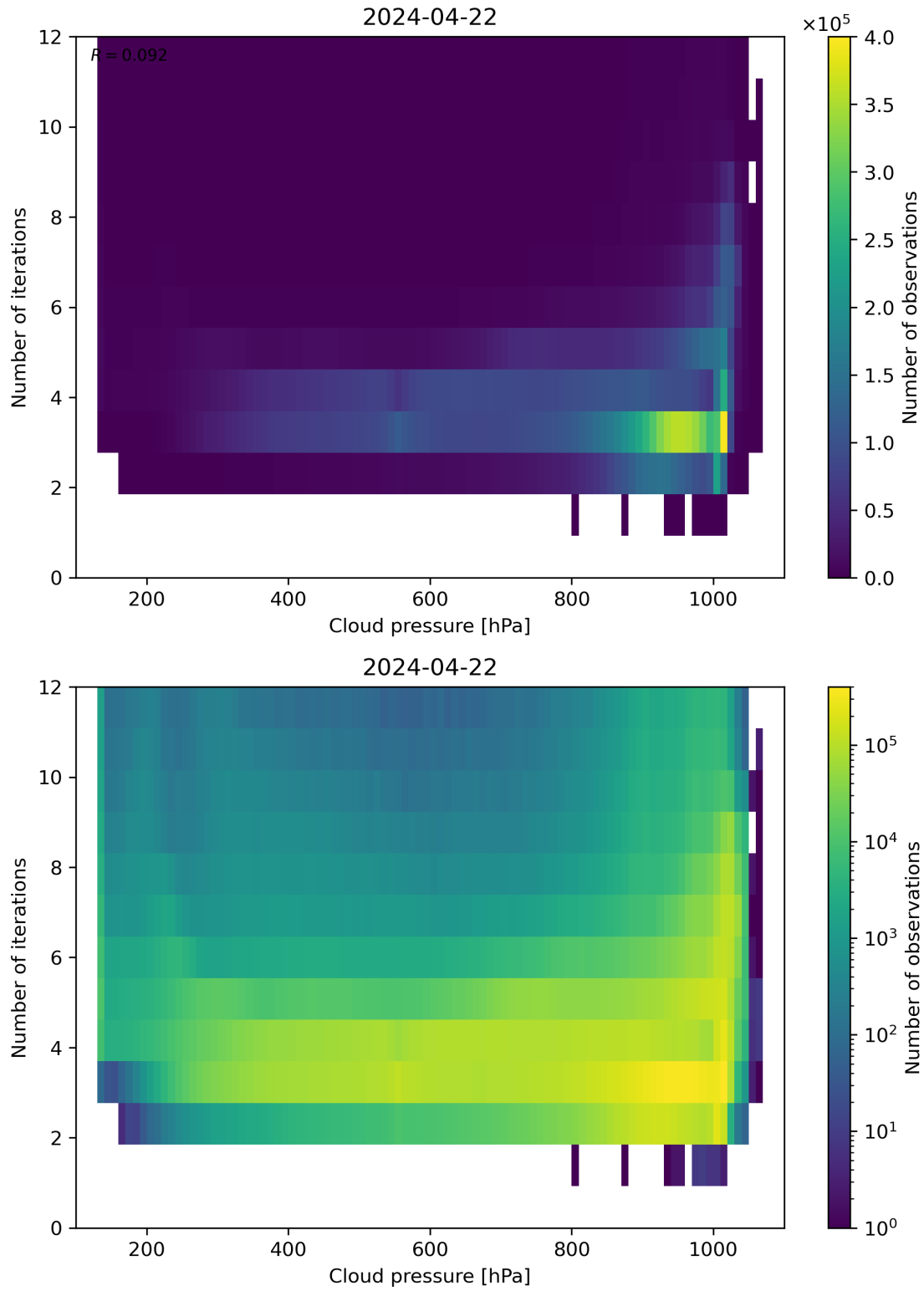
Figure 81: Scatter density plot of “Cloud pressure” against “Number of iterations” for 2024-04-21 to 2024-04-23.
