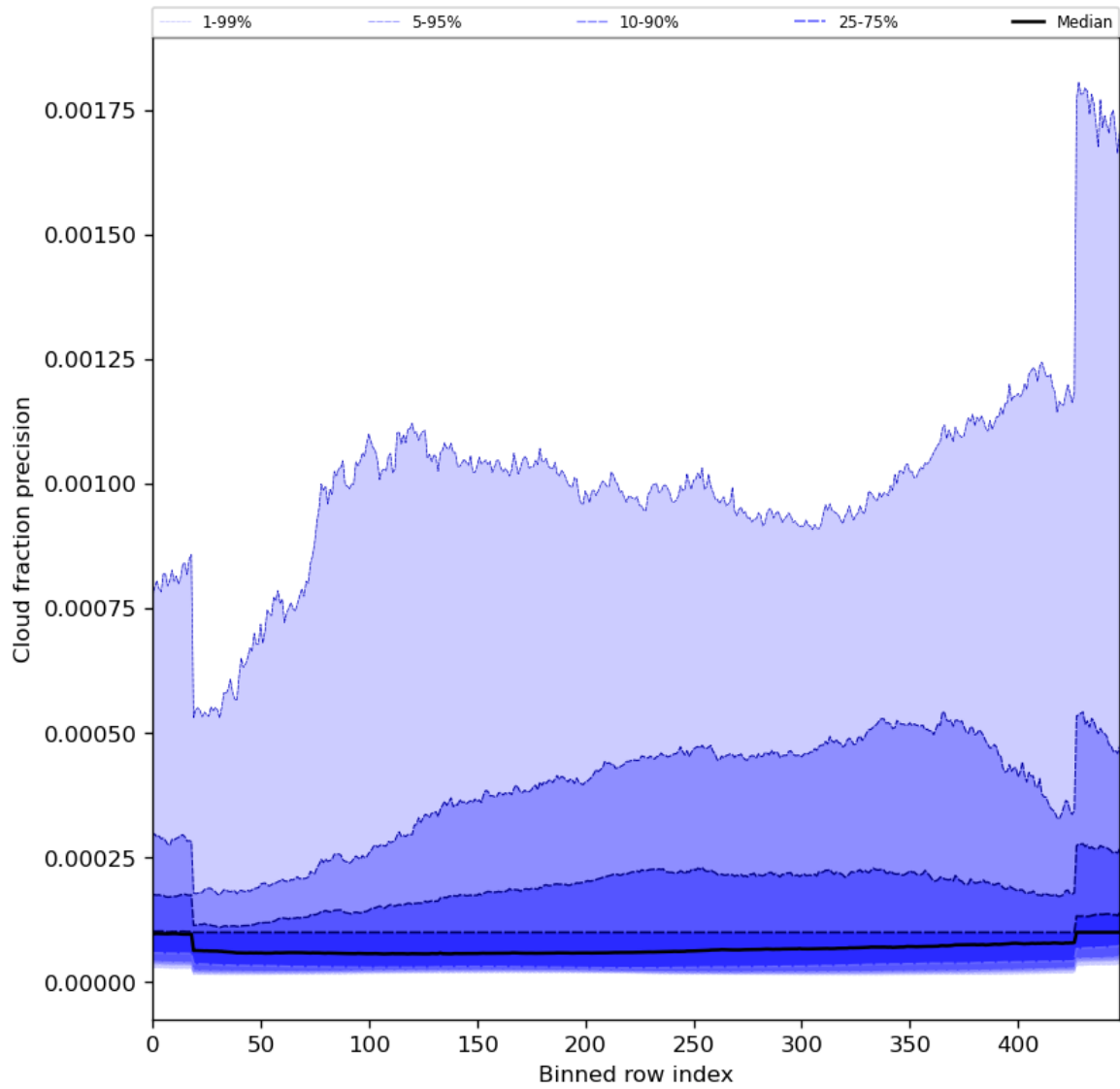
Figure 50: Along track statistics of “Cloud fraction precision” for 2024-04-21 to 2024-04-23
