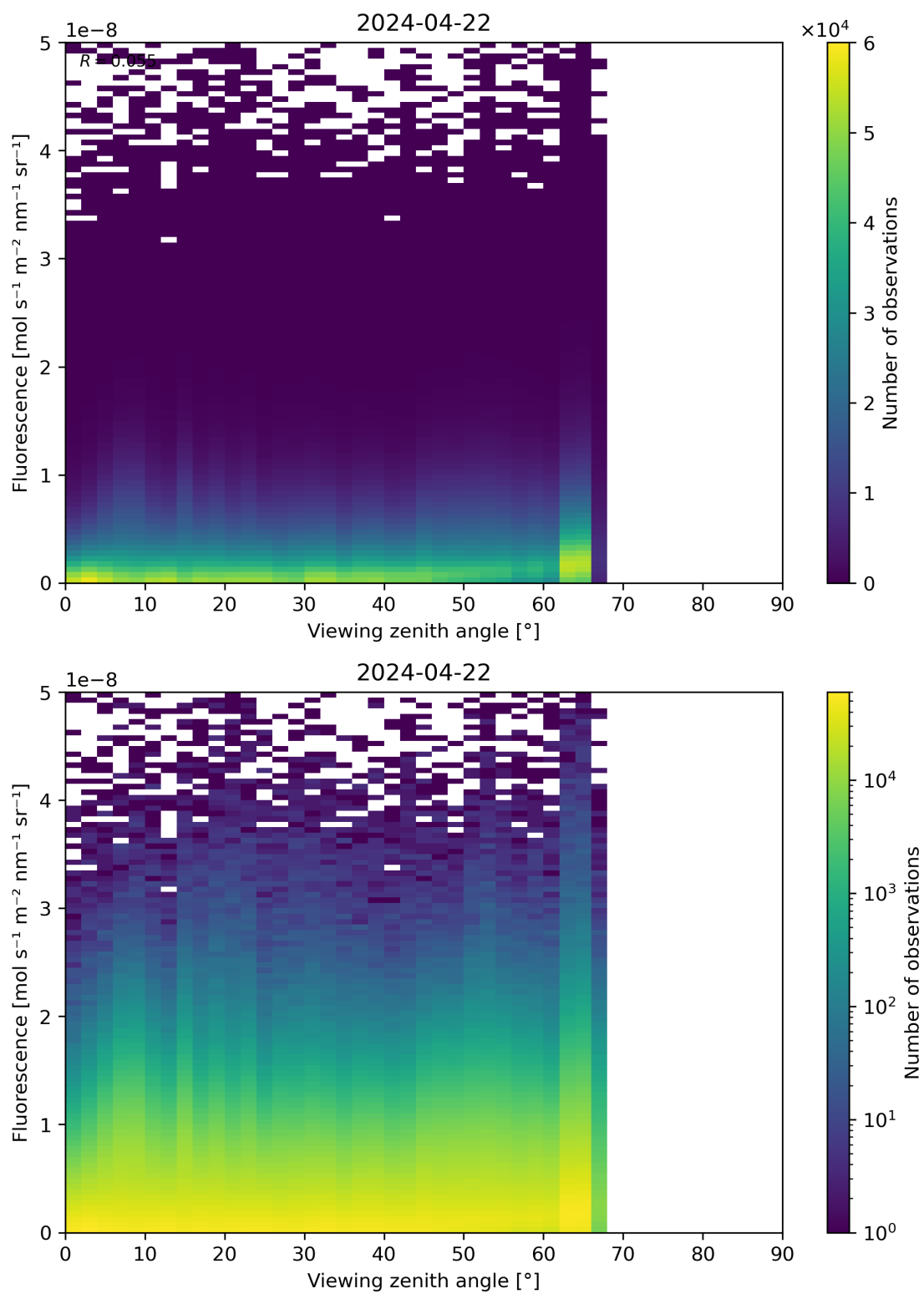
Figure 122: Scatter density plot of “Viewing zenith angle” against “Fluorescence” for 2024-04-21 to 2024-04-23.
