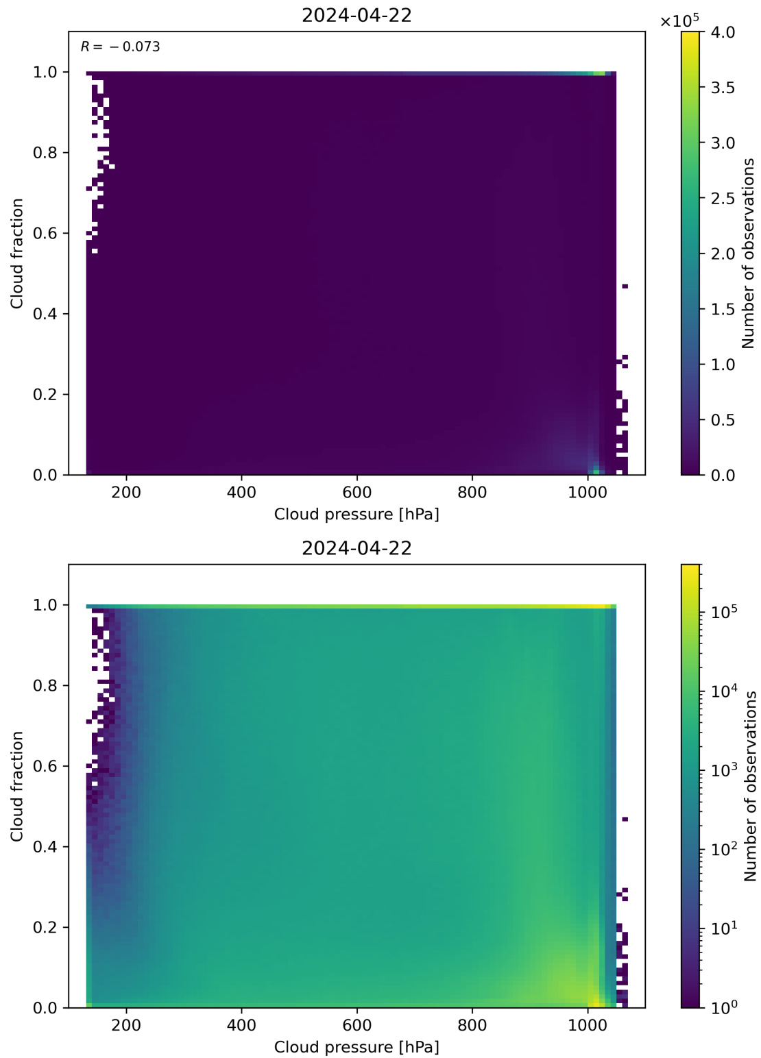
Figure 79: Scatter density plot of “Cloud pressure” against “Cloud fraction” for 2024-04-21 to 2024-04-23.
