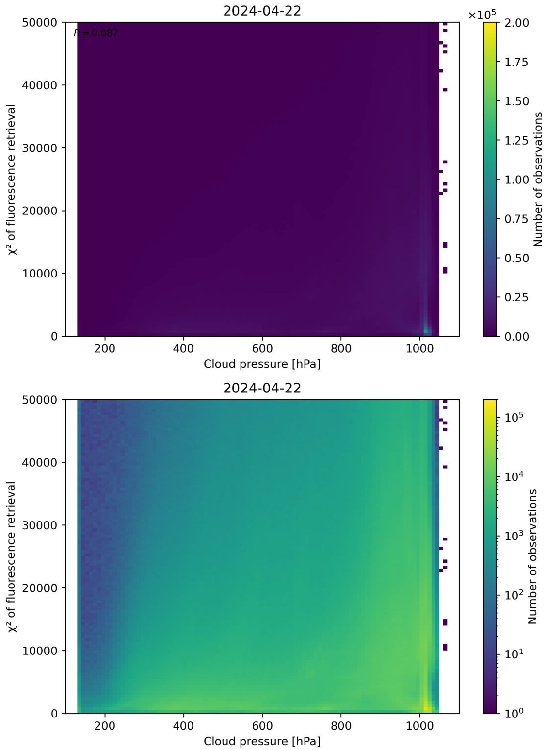
Figure 78: Scatter density plot of “Cloud pressure” against “ \chi^2 of fluorescence retrieval” for 2024-04-21 to 2024-04-23.
