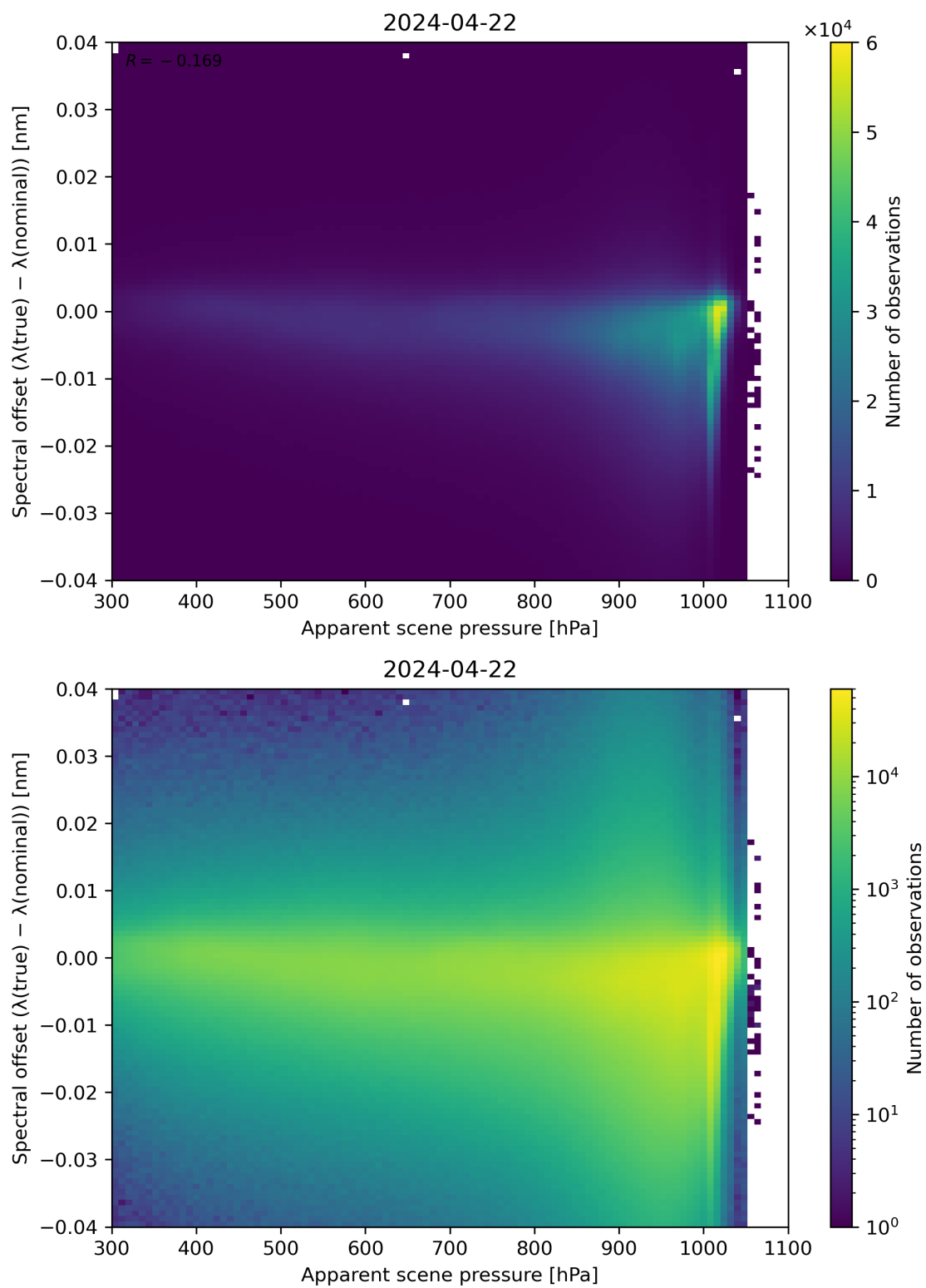
Figure 67: Scatter density plot of “Apparent scene pressure” against “Spectral offset ( \lambda(\text{true}) - \lambda(\text{nominal}) )” for 2024-04-21 to 2024-04-23.
