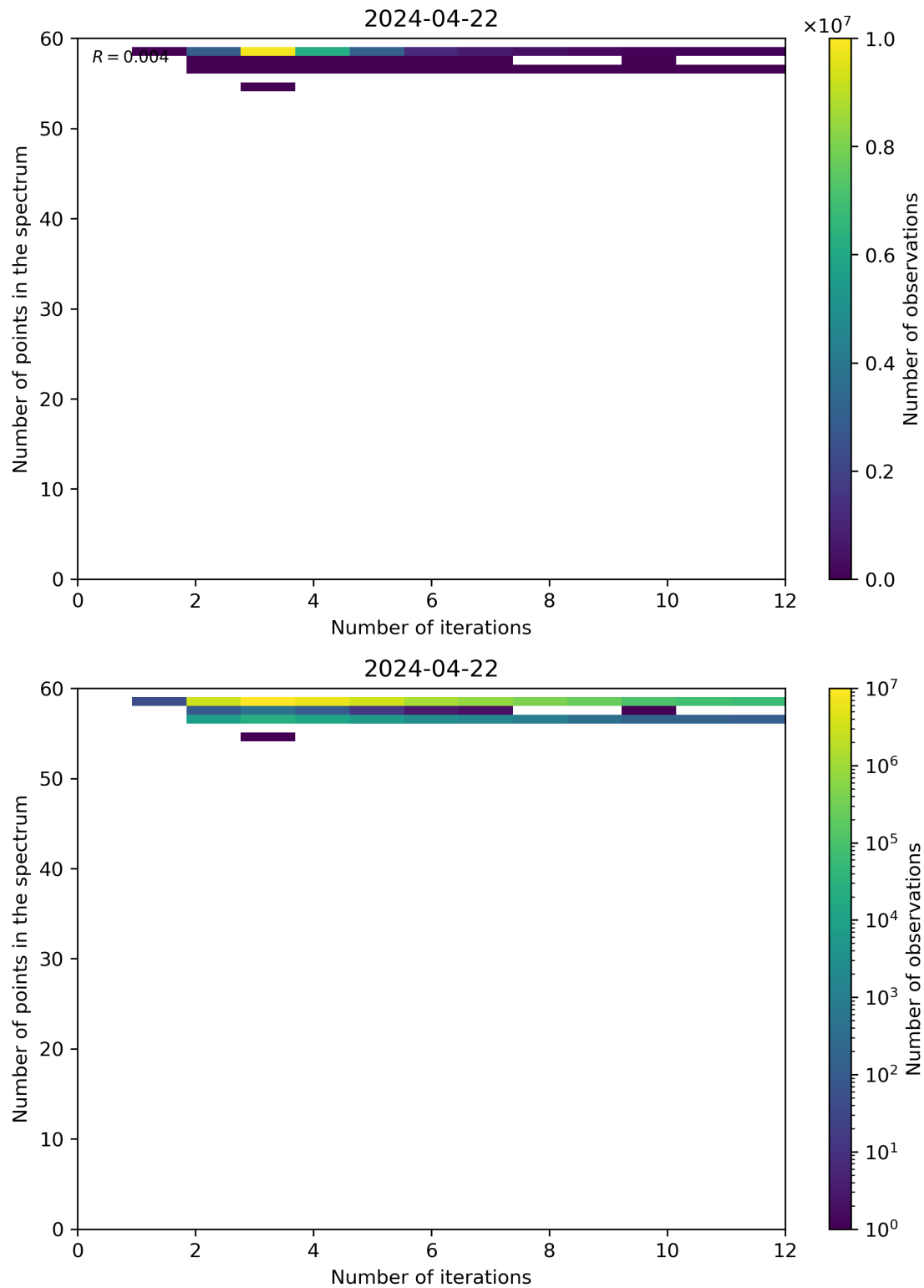
Figure 99: Scatter density plot of “Number of iterations” against “Number of points in the spectrum” for 2024-04-21 to 2024-04-23.
