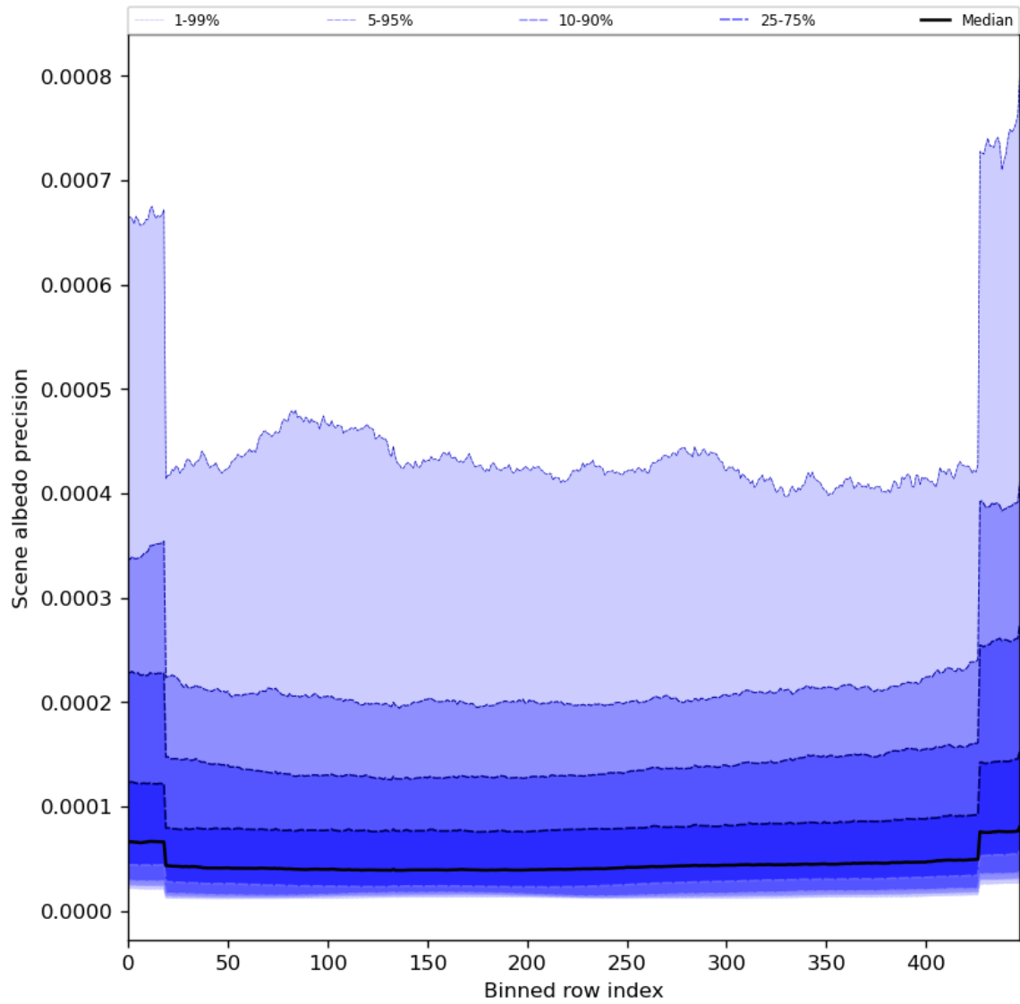
Figure 52: Along track statistics of “Scene albedo precision” for 2024-04-21 to 2024-04-23
