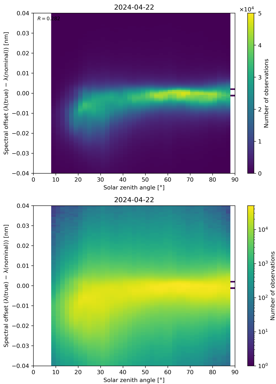
Figure 117: Scatter density plot of “Solar zenith angle” against “Spectral offset ( \lambda(\text{true}) - \lambda(\text{nominal}) )” for 2024-04-21 to 2024-04-23.
