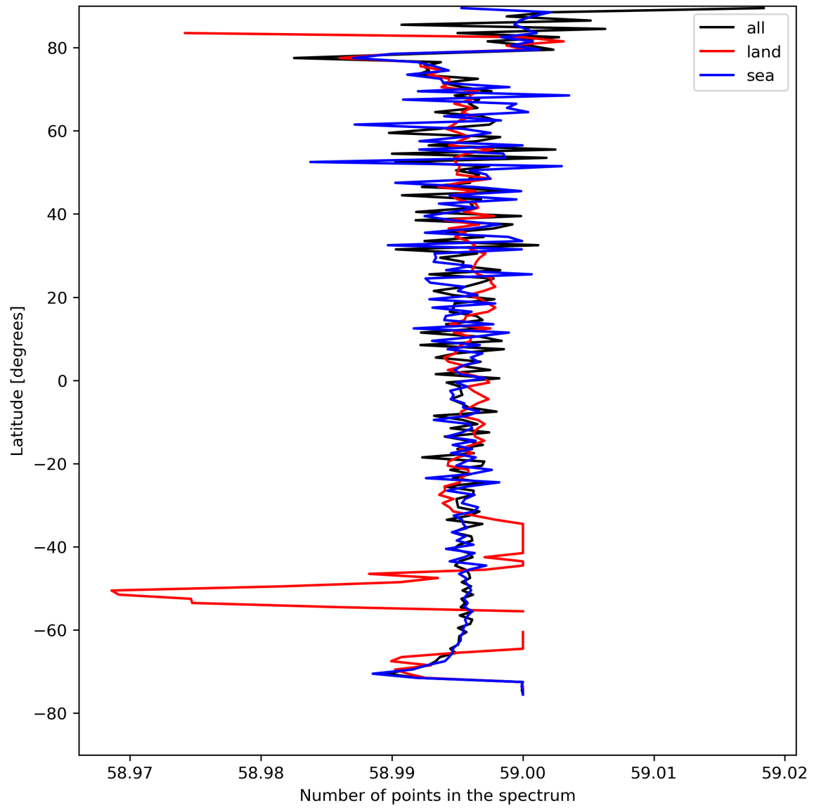
Figure 27: Zonal average of “Number of points in the spectrum” for 2024-04-21 to 2024-04-23.
