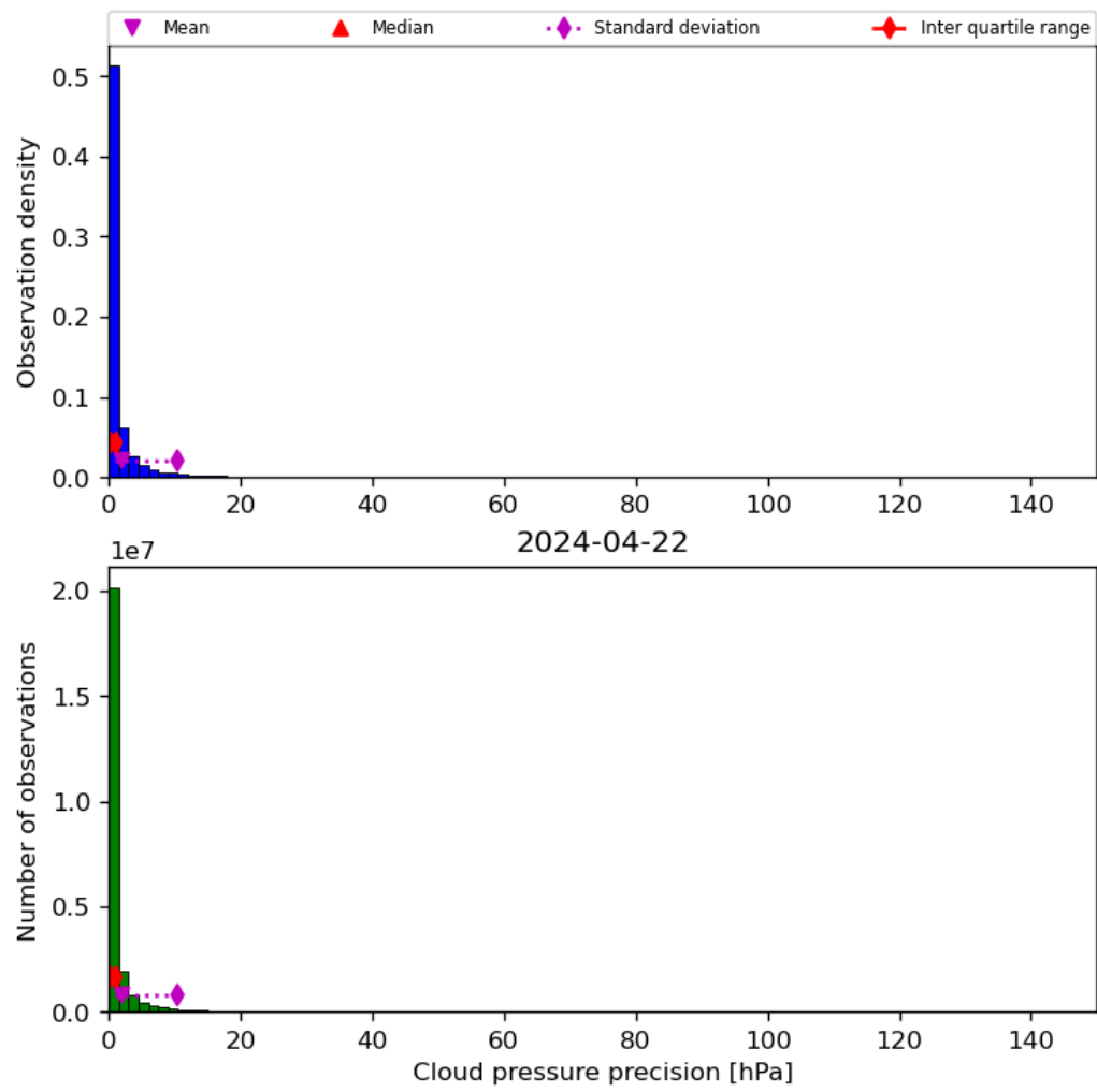
Figure 31: Histogram of “Cloud pressure precision” for 2024-04-21 to 2024-04-23
