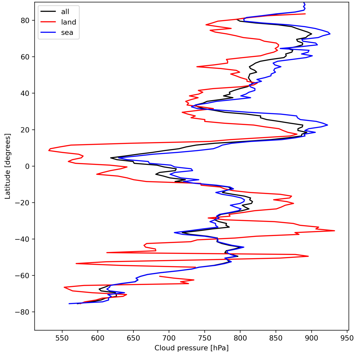
Figure 13: Zonal average of “Cloud pressure” for 2024-04-21 to 2024-04-23.
