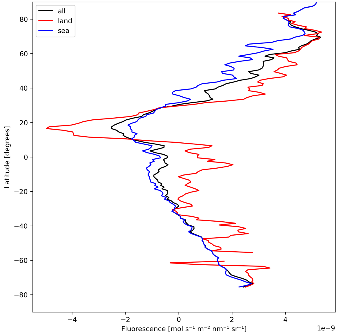
Figure 23: Zonal average of “Fluorescence” for 2024-04-21 to 2024-04-23.
