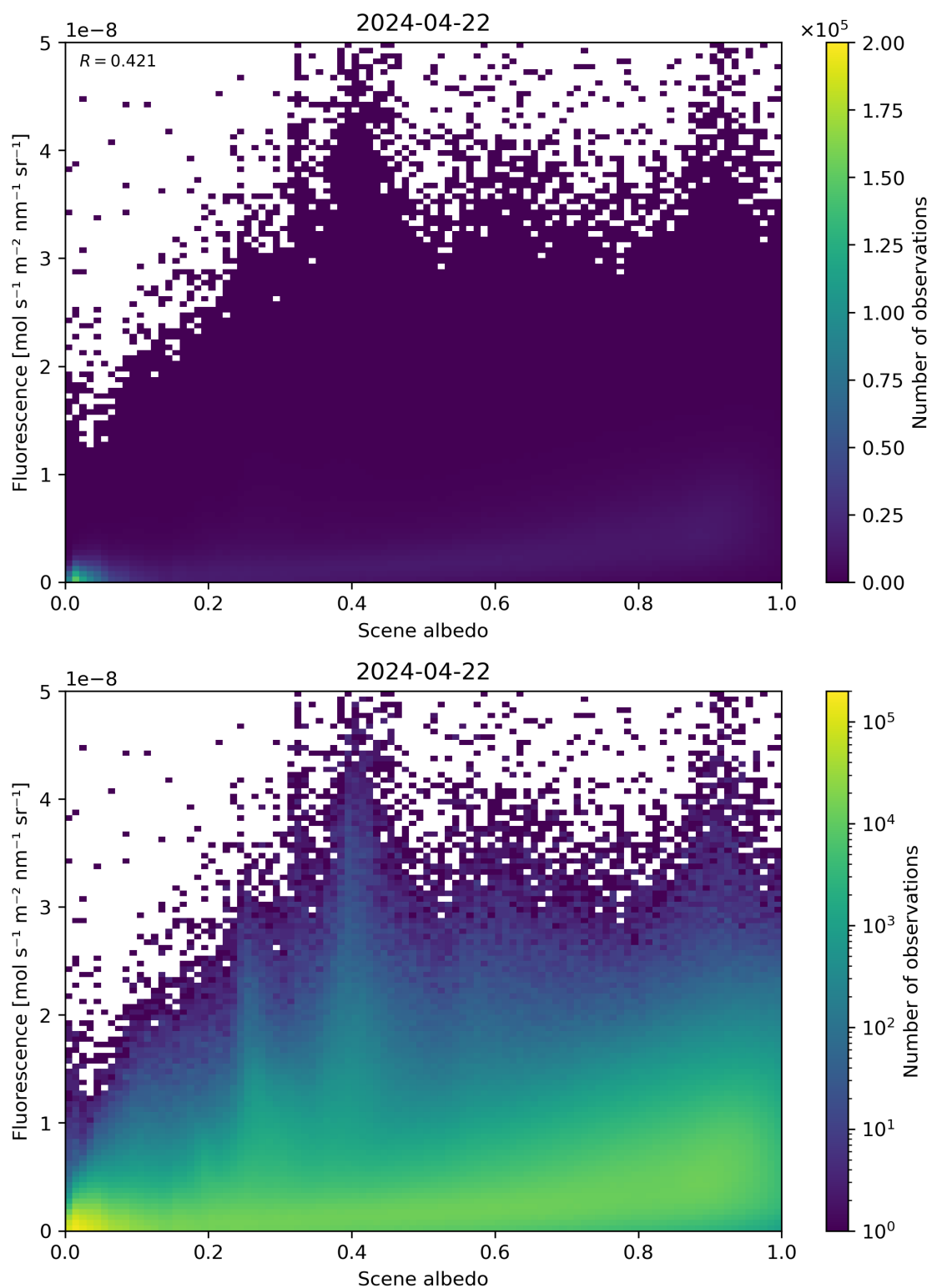
Figure 104: Scatter density plot of “Scene albedo” against “Fluorescence” for 2024-04-21 to 2024-04-23.
