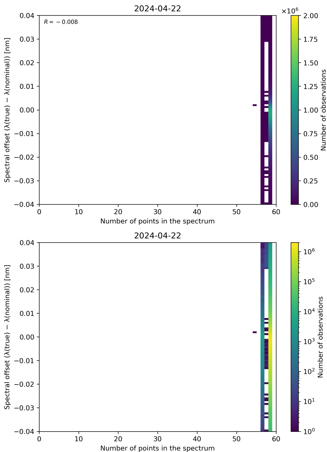
Figure 101: Scatter density plot of “Number of points in the spectrum” against “Spectral offset ( \lambda(\text{true}) - \lambda(\text{nominal}) )” for 2024-04-21 to 2024-04-23.
