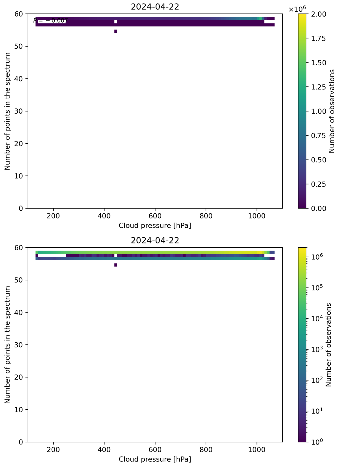
Figure 82: Scatter density plot of “Cloud pressure” against “Number of points in the spectrum” for 2024-04-21 to 2024-04-23.
