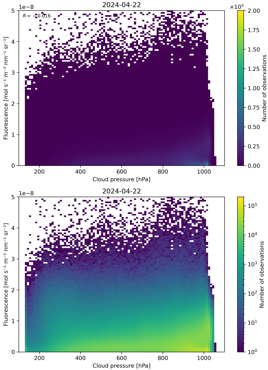
Figure 80: Scatter density plot of “Cloud pressure” against “Fluorescence” for 2024-04-21 to 2024-04-23.
