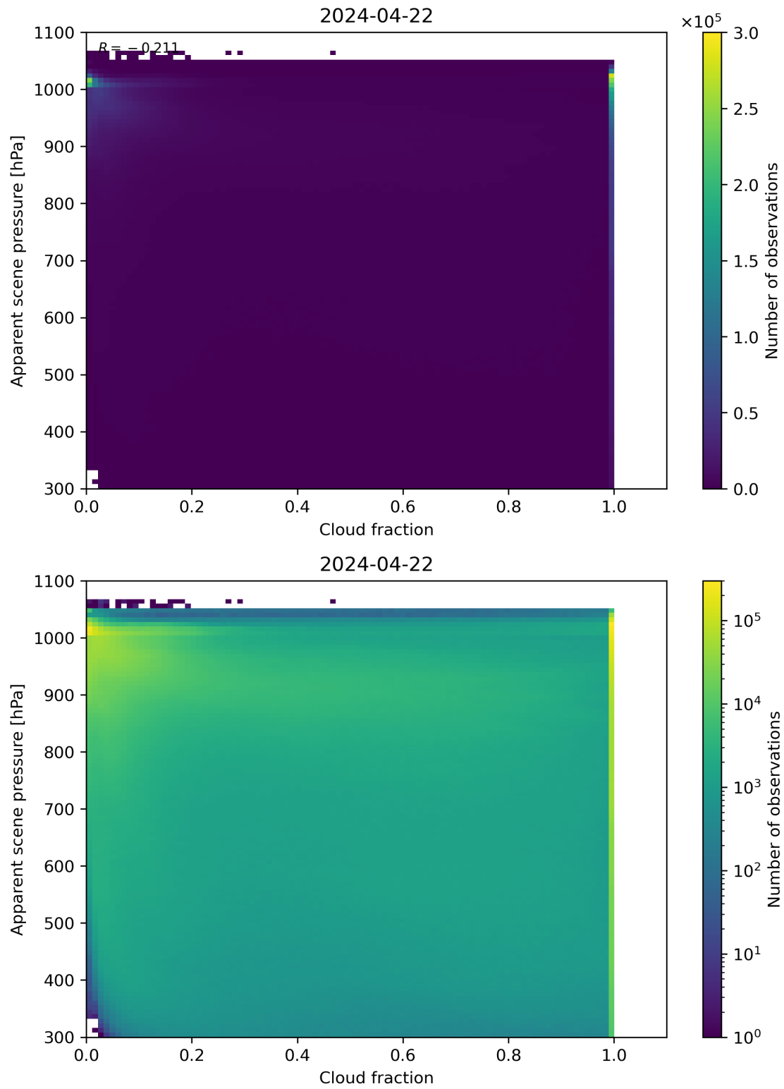
Figure 70: Scatter density plot of “Cloud fraction” against “Apparent scene pressure” for 2024-04-21 to 2024-04-23.
