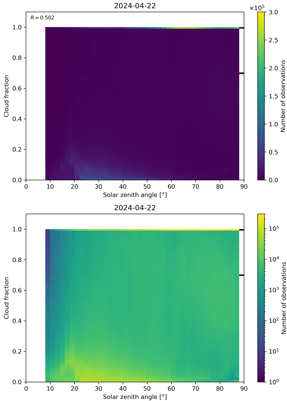
Figure 110: Scatter density plot of “Solar zenith angle” against “Cloud fraction” for 2024-04-21 to 2024-04-23.
