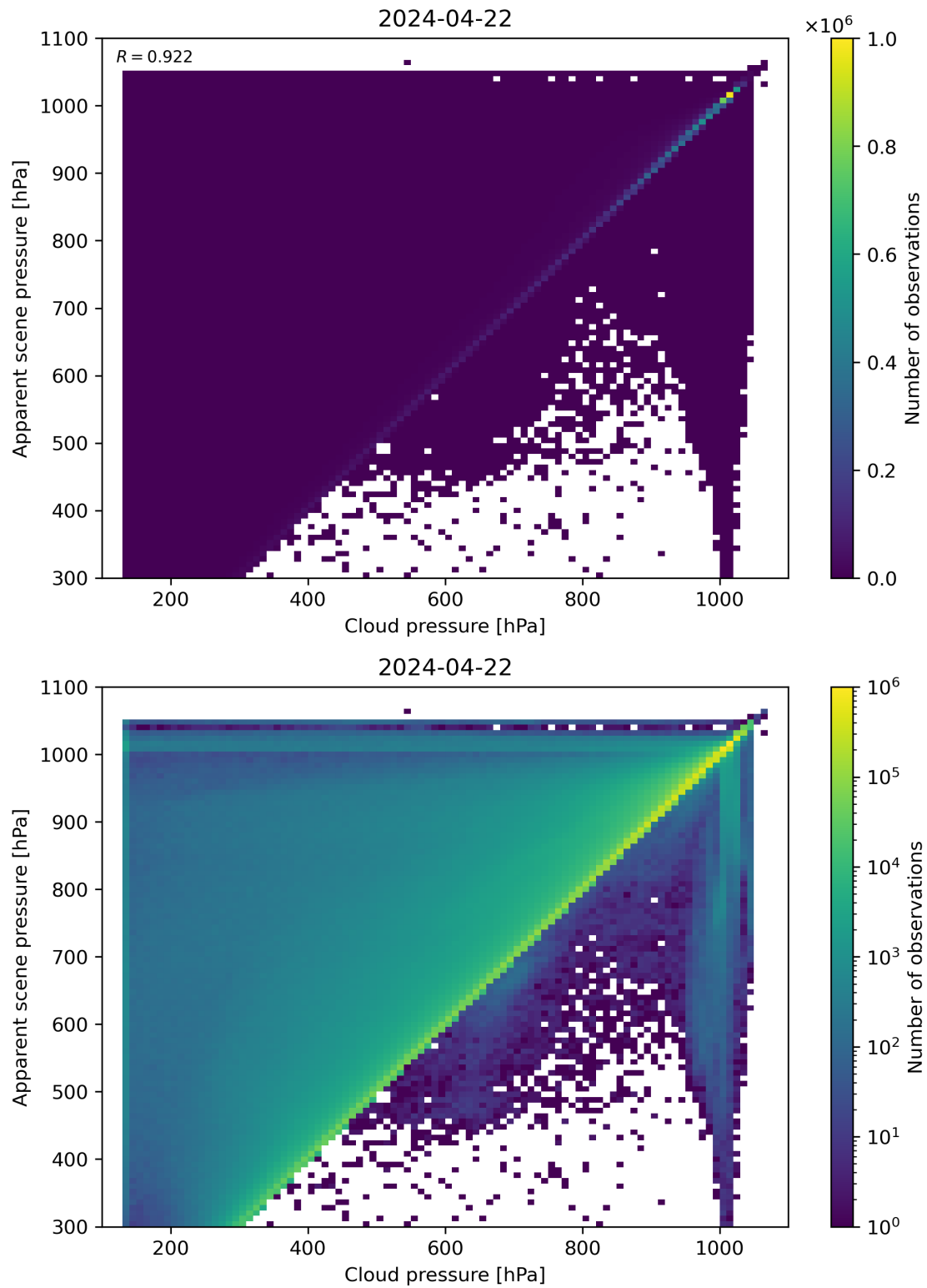
Figure 77: Scatter density plot of “Cloud pressure” against “Apparent scene pressure” for 2024-04-21 to 2024-04-23.
