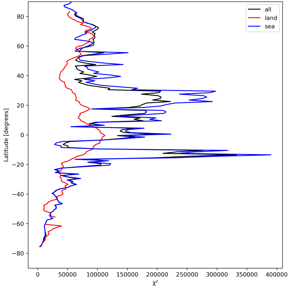
Figure 21: Zonal average of “ \chi^2 ” for 2024-04-21 to 2024-04-23.
