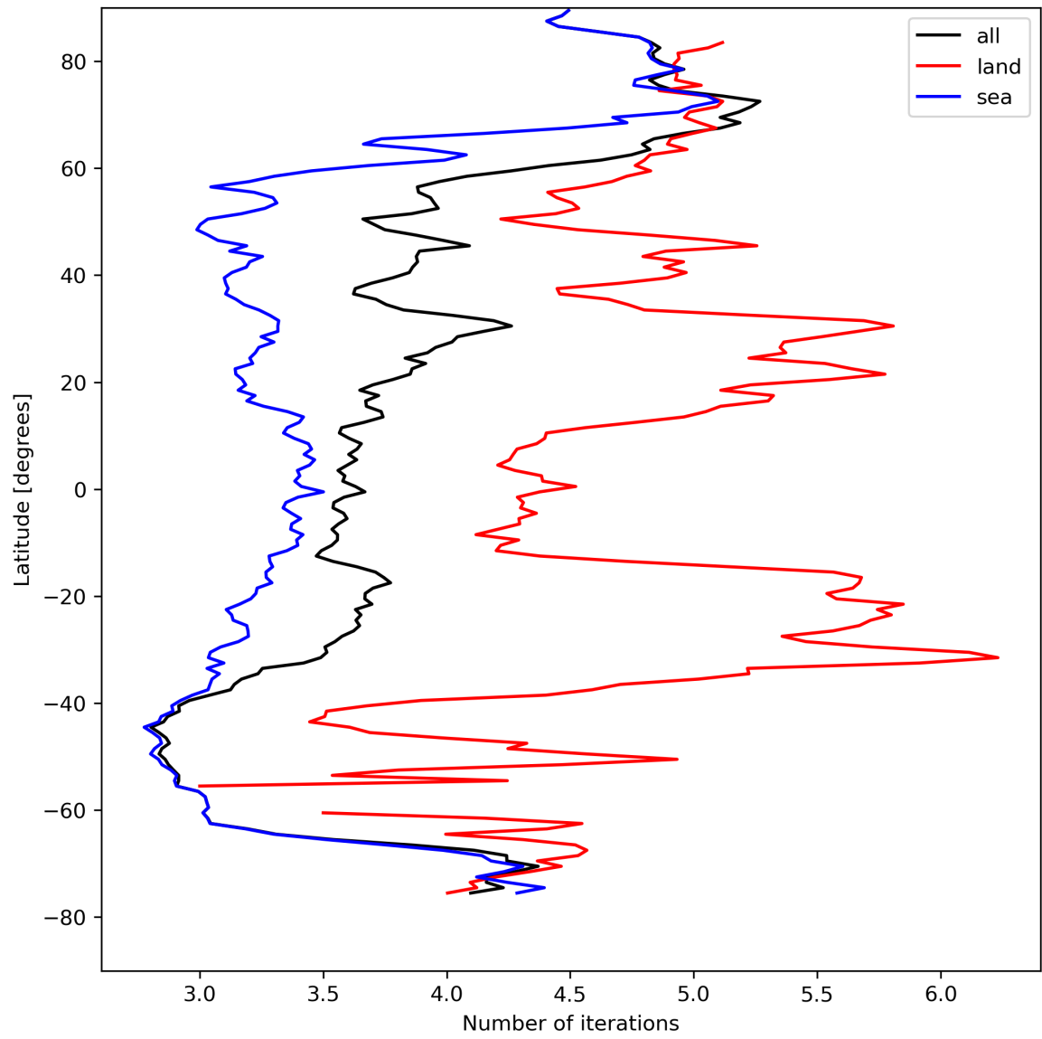
Figure 22: Zonal average of “Number of iterations” for 2024-04-21 to 2024-04-23.
