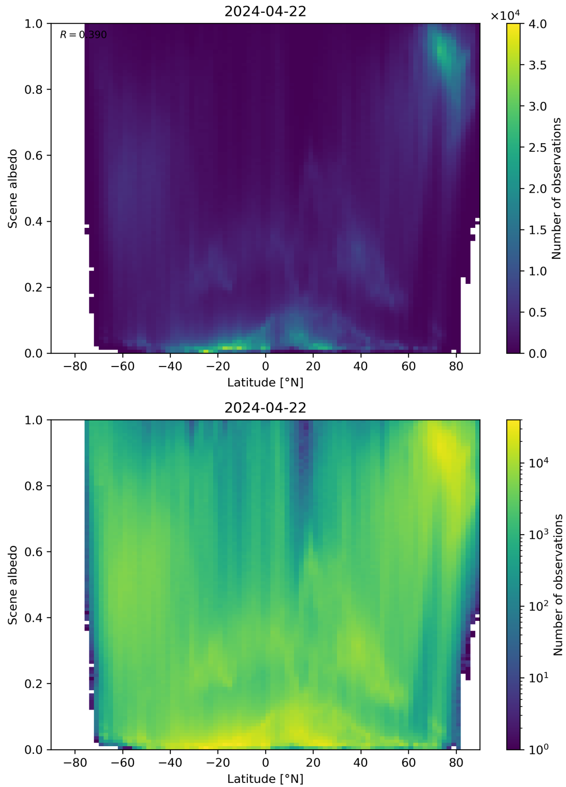
Figure 95: Scatter density plot of “Latitude” against “Scene albedo” for 2024-04-21 to 2024-04-23.
