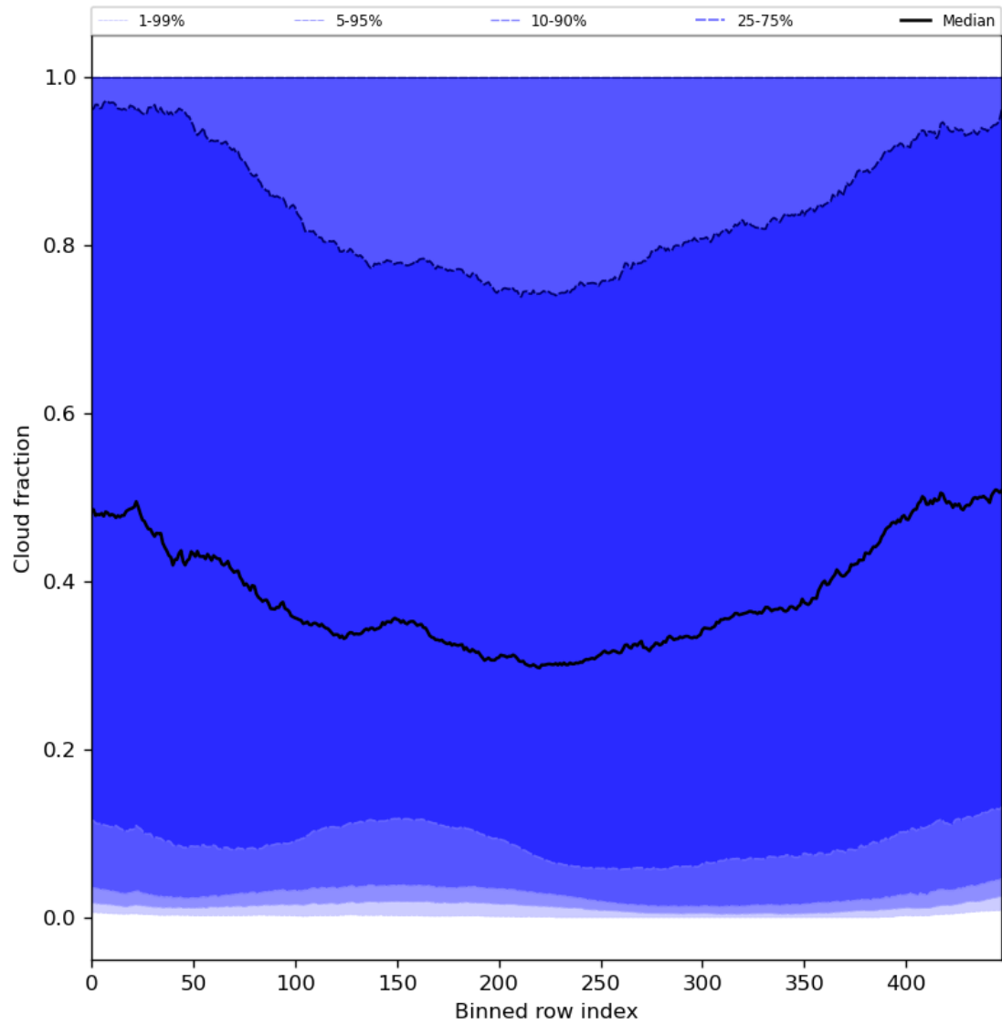
Figure 49: Along track statistics of “Cloud fraction” for 2024-04-21 to 2024-04-23
