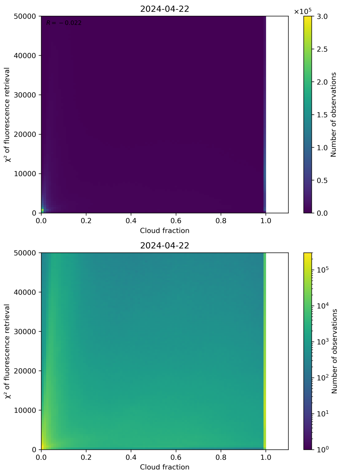
Figure 71: Scatter density plot of “Cloud fraction” against “ \chi^2 of fluorescence retrieval” for 2024-04-21 to 2024-04-23.
