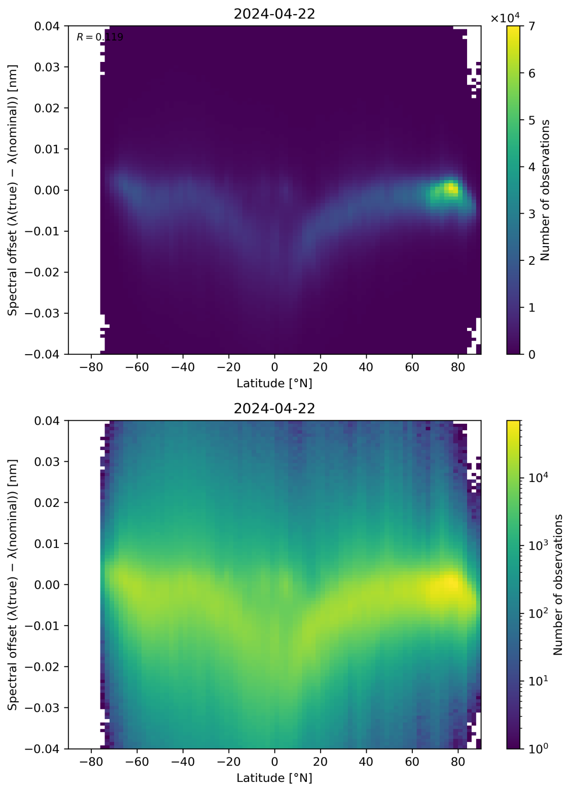
Figure 96: Scatter density plot of “Latitude” against “Spectral offset ( \lambda(\text{true}) - \lambda(\text{nominal}) )” for 2024-04-21 to 2024-04-23.
