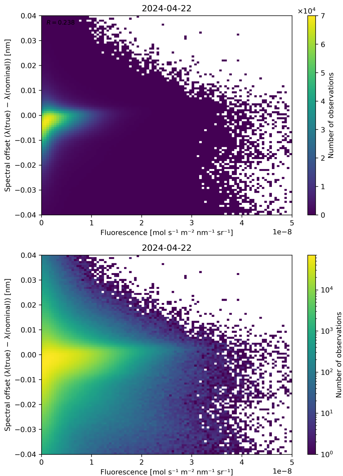
Figure 87: Scatter density plot of “Fluorescence” against “Spectral offset ( \lambda(\text{true}) - \lambda(\text{nominal}) )” for 2024-04-21 to 2024-04-23.
