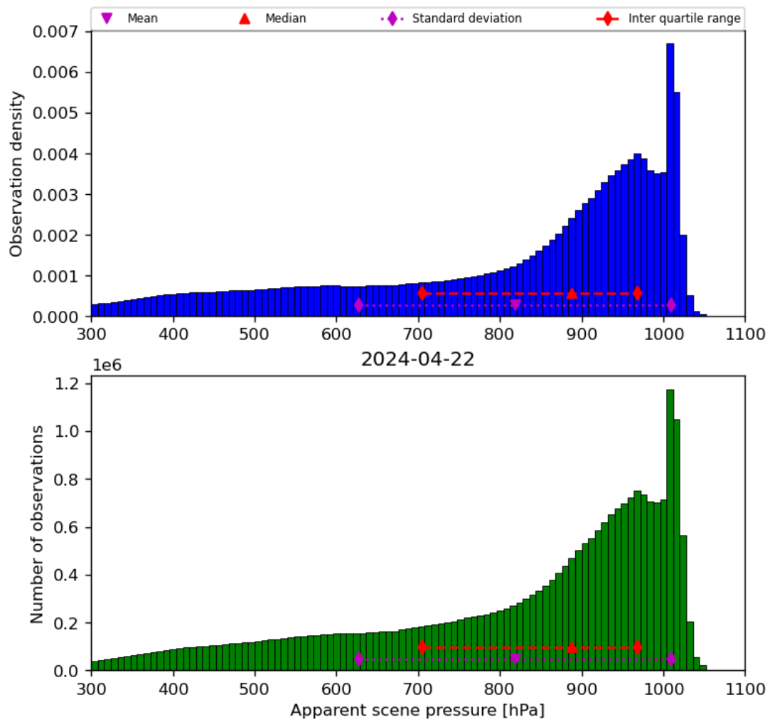
Figure 36: Histogram of “Apparent scene pressure” for 2024-04-21 to 2024-04-23
