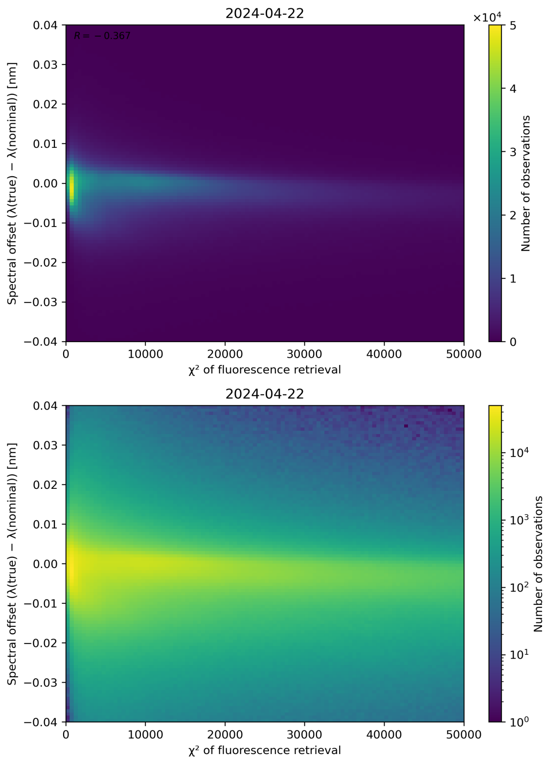
Figure 69: Scatter density plot of " \chi^2 of fluorescence retrieval" against "Spectral offset ( \lambda(\text{true}) - \lambda(\text{nominal})) " for 2024-04-21 to 2024-04-23.
