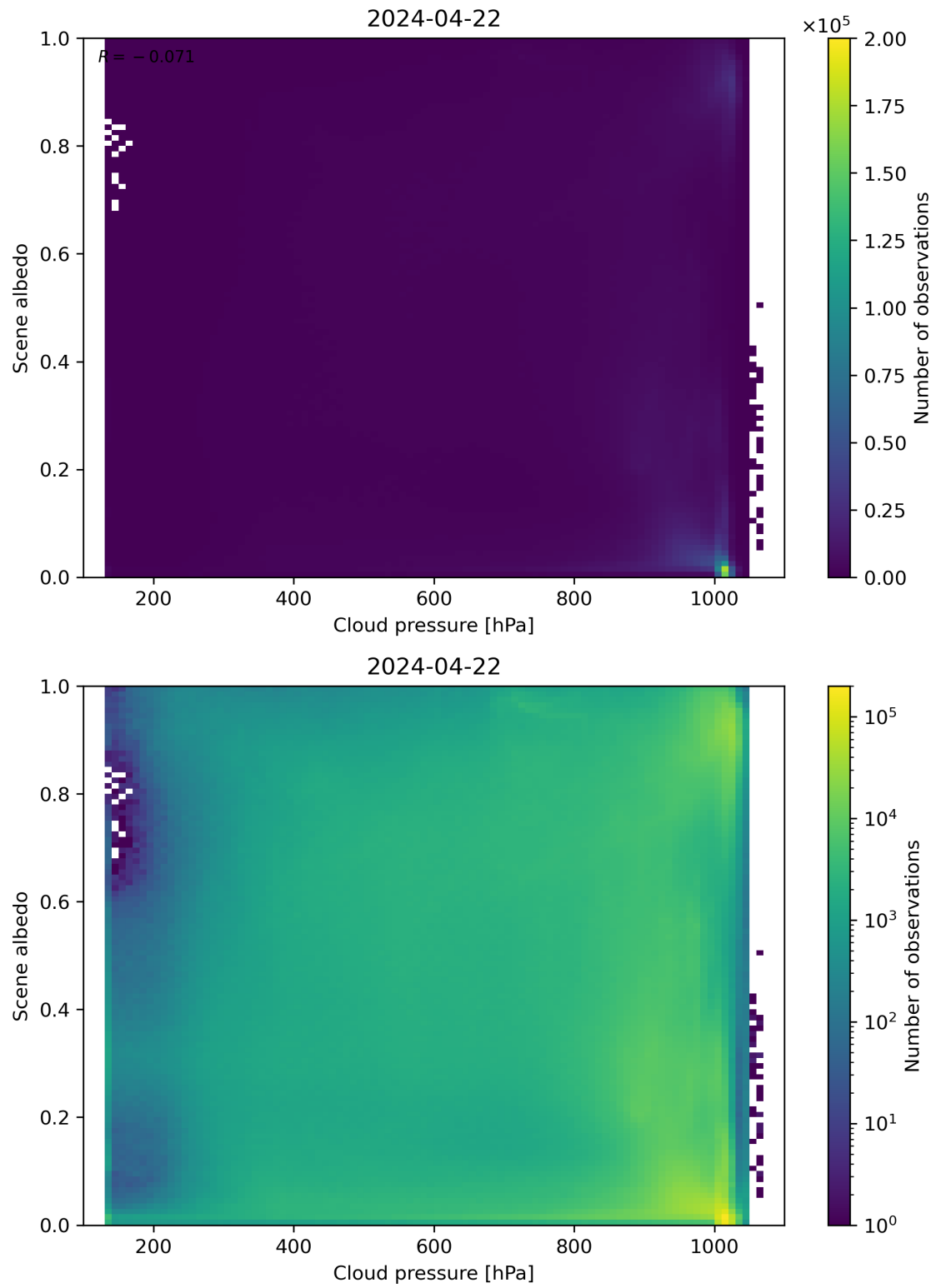
Figure 83: Scatter density plot of “Cloud pressure” against “Scene albedo” for 2024-04-21 to 2024-04-23.
