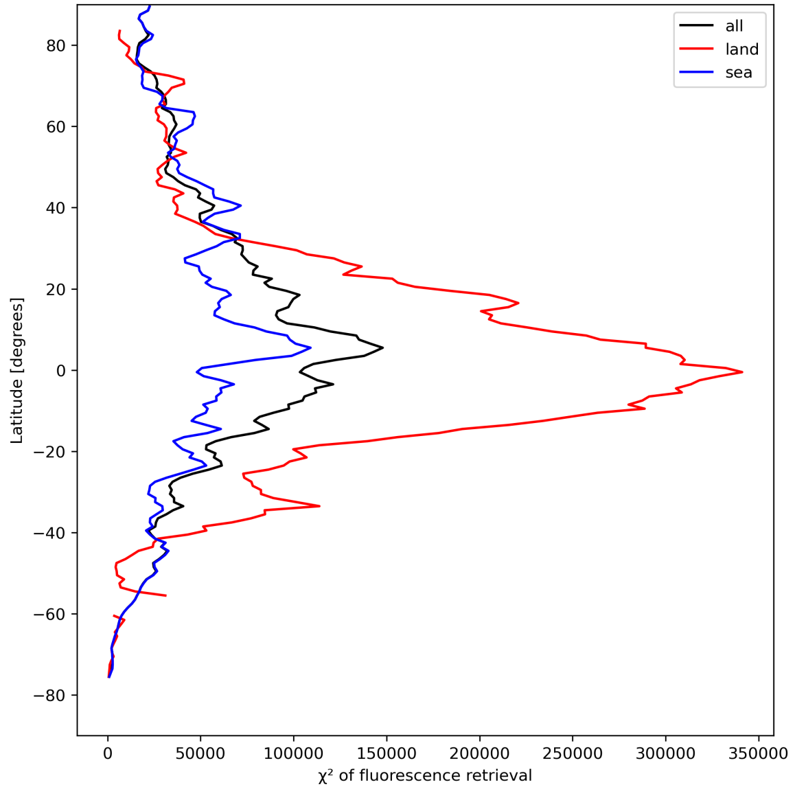
Figure 25: Zonal average of “ \chi^2 of fluorescence retrieval” for 2024-04-21 to 2024-04-23.
