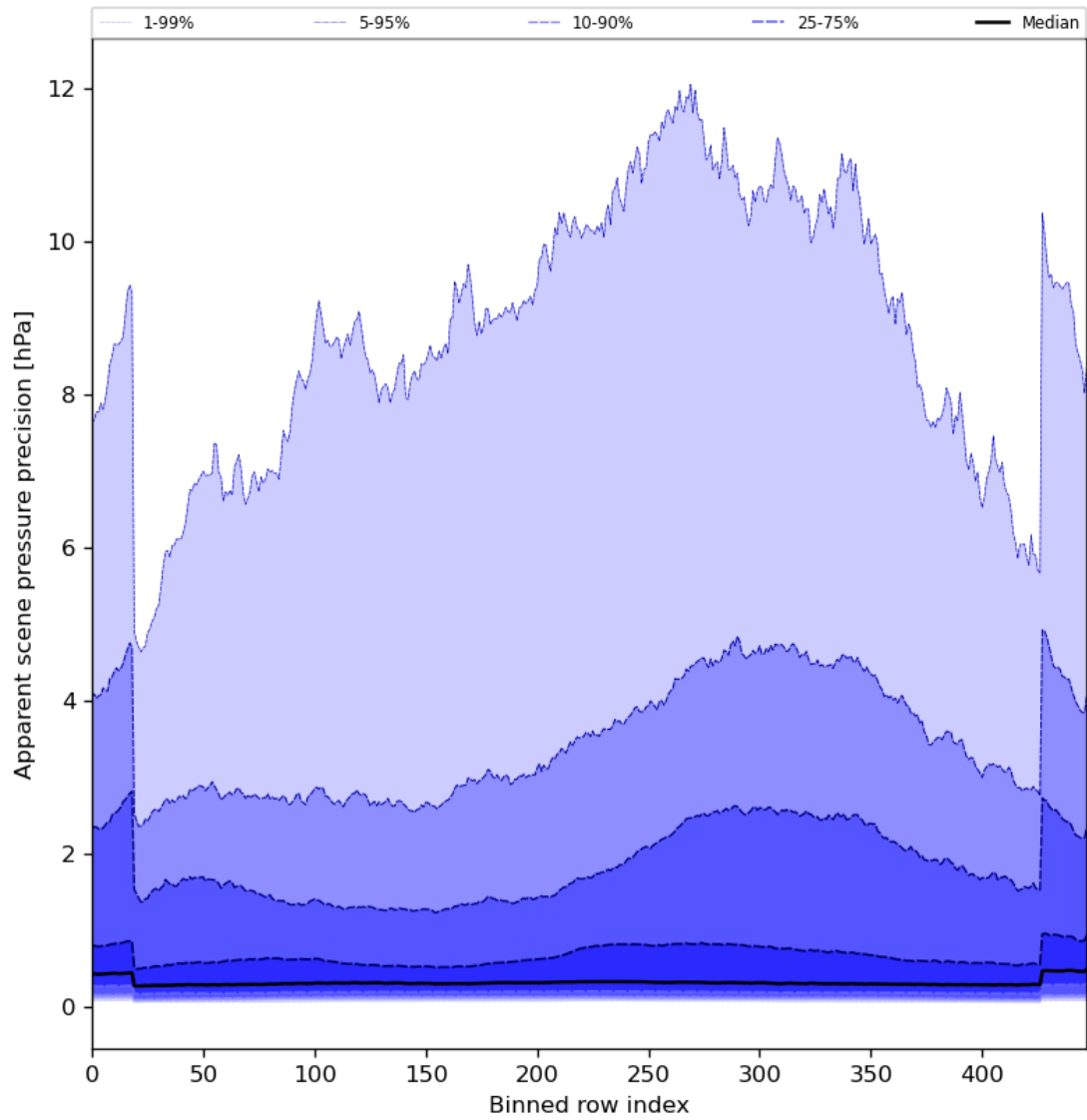
Figure 54: Along track statistics of “Apparent scene pressure precision” for 2024-04-21 to 2024-04-23
