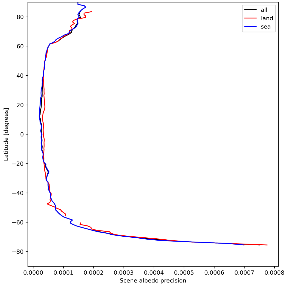
Figure 18: Zonal average of “Scene albedo precision” for 2024-04-21 to 2024-04-23.
