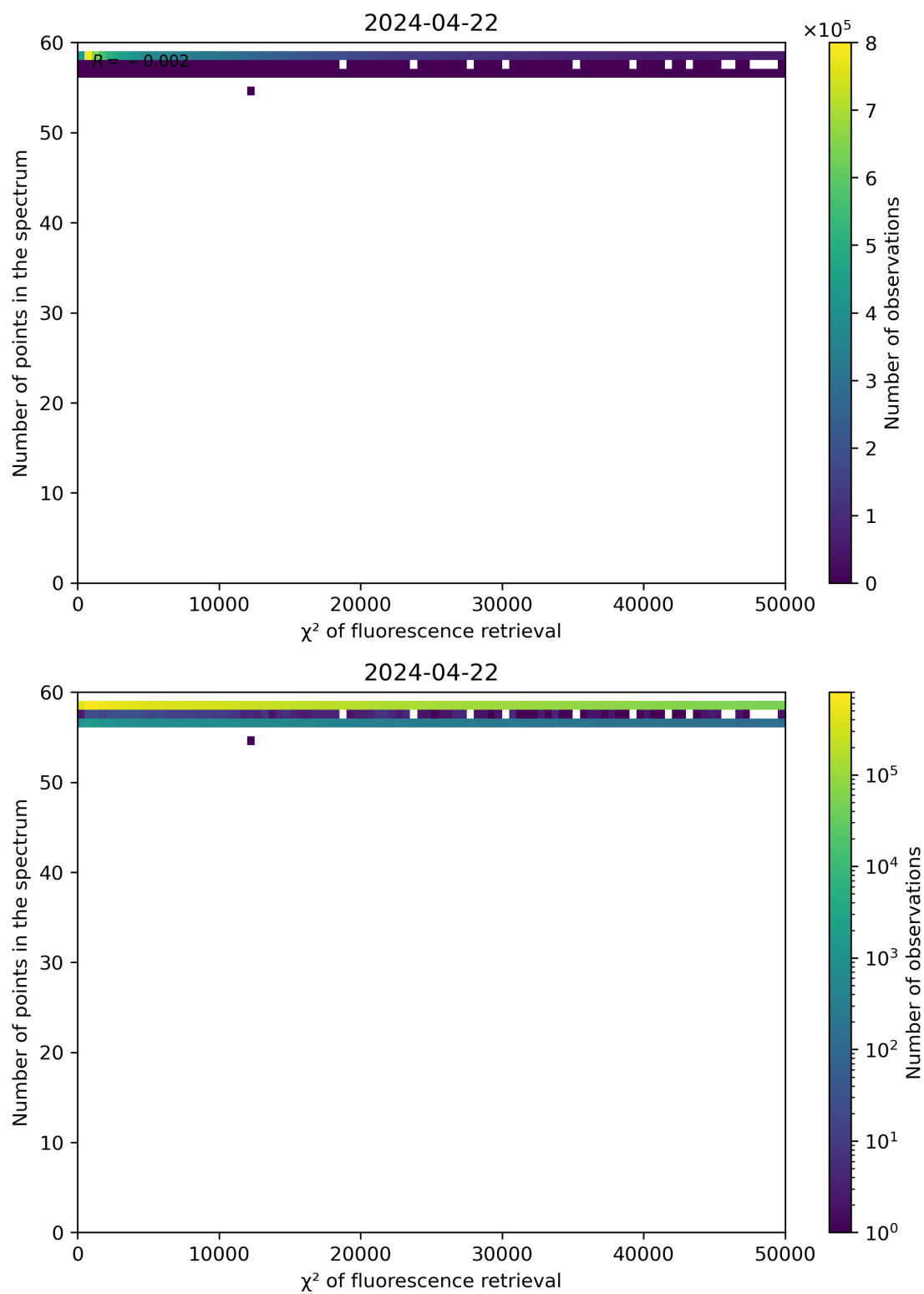
Figure 68: Scatter density plot of “ \chi^2 of fluorescence retrieval” against “Number of points in the spectrum” for 2024-04-21 to 2024-04-23.
