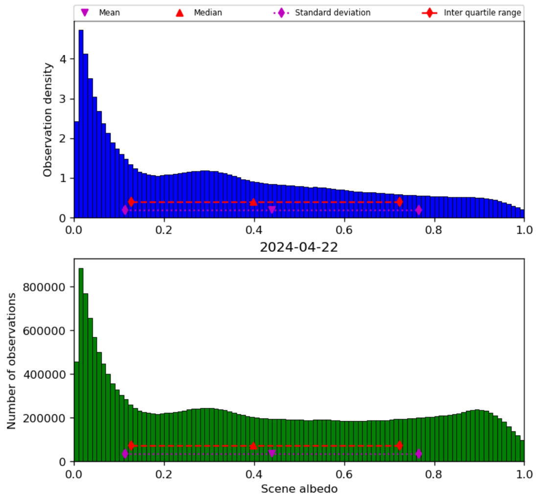
Figure 34: Histogram of “Scene albedo” for 2024-04-21 to 2024-04-23
