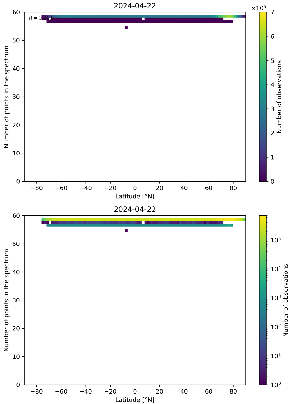
Figure 94: Scatter density plot of “Latitude” against “Number of points in the spectrum” for 2024-04-21 to 2024-04-23.
