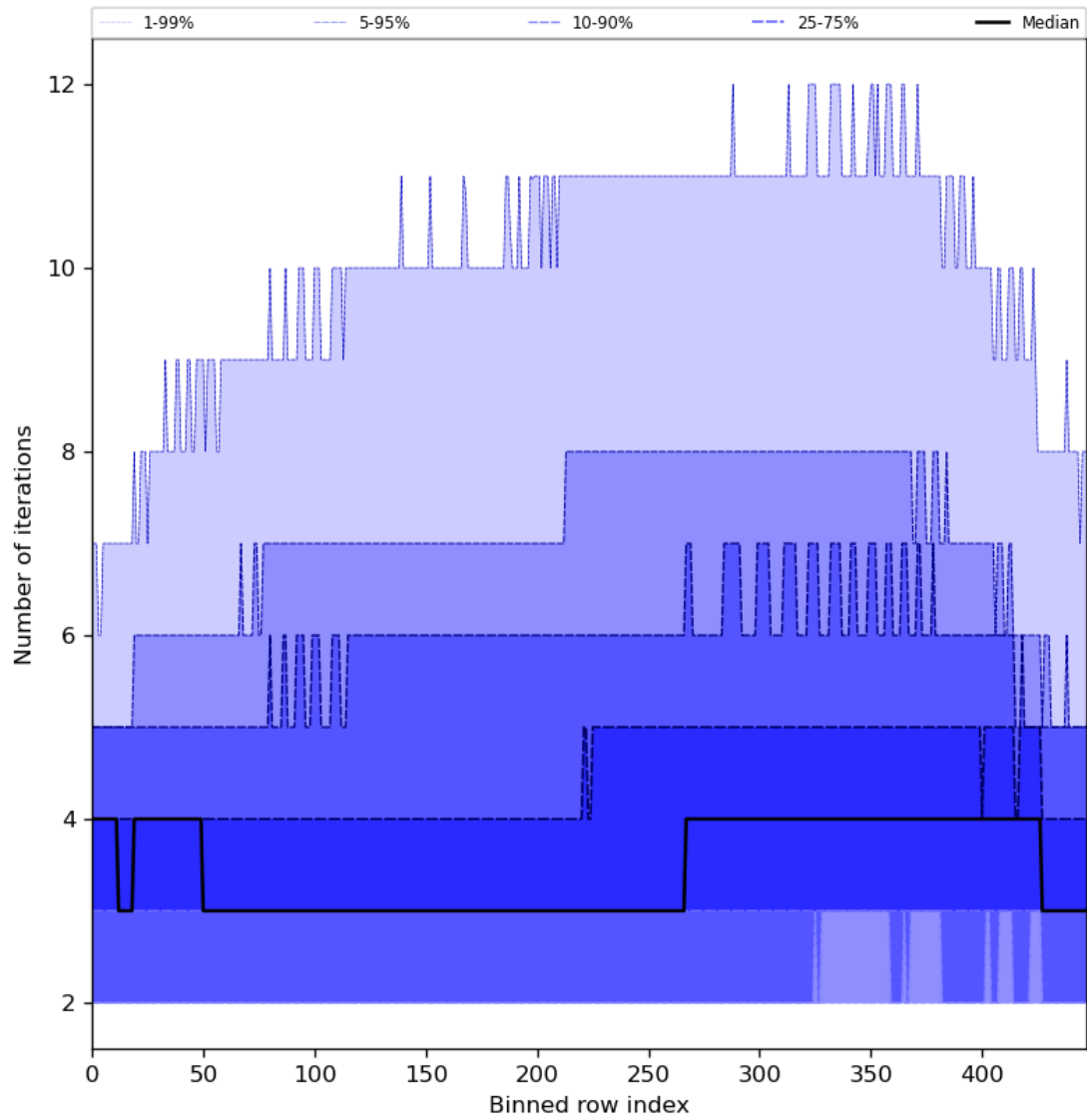
Figure 56: Along track statistics of “Number of iterations” for 2024-04-21 to 2024-04-23
