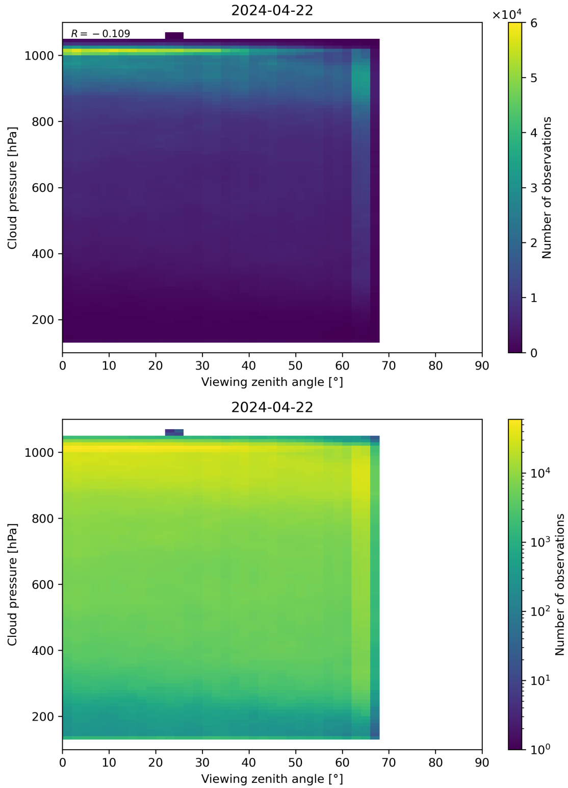
Figure 121: Scatter density plot of “Viewing zenith angle” against “Cloud pressure” for 2024-04-21 to 2024-04-23.
