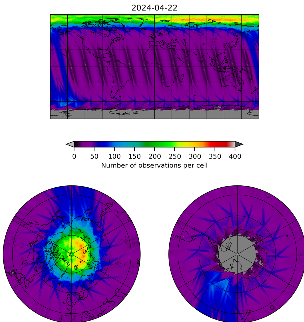
Figure 11: Map of the number of observations for 2024-04-21 to 2024-04-23
