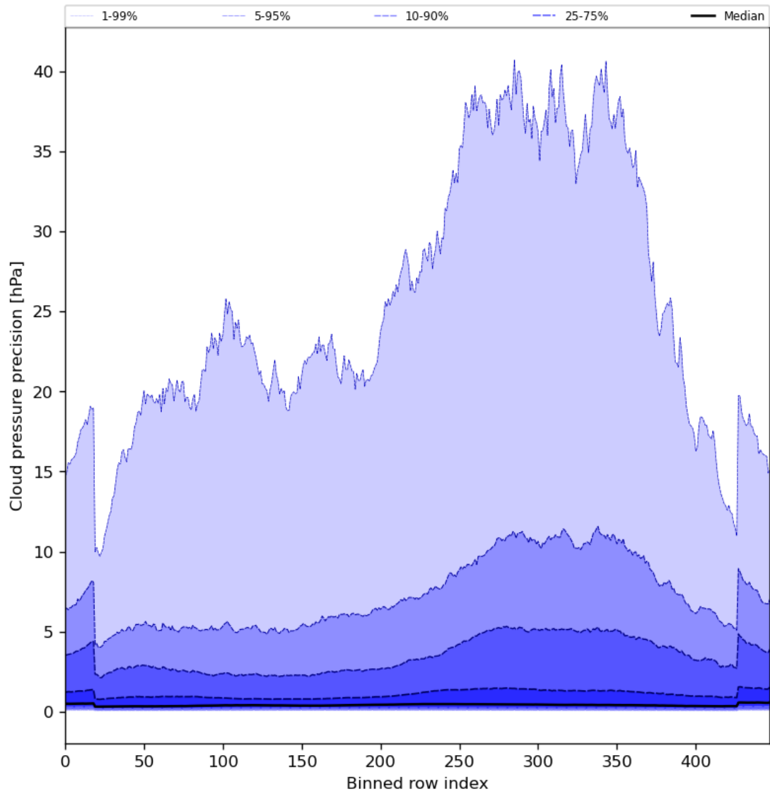
Figure 48: Along track statistics of “Cloud pressure precision” for 2024-04-21 to 2024-04-23
