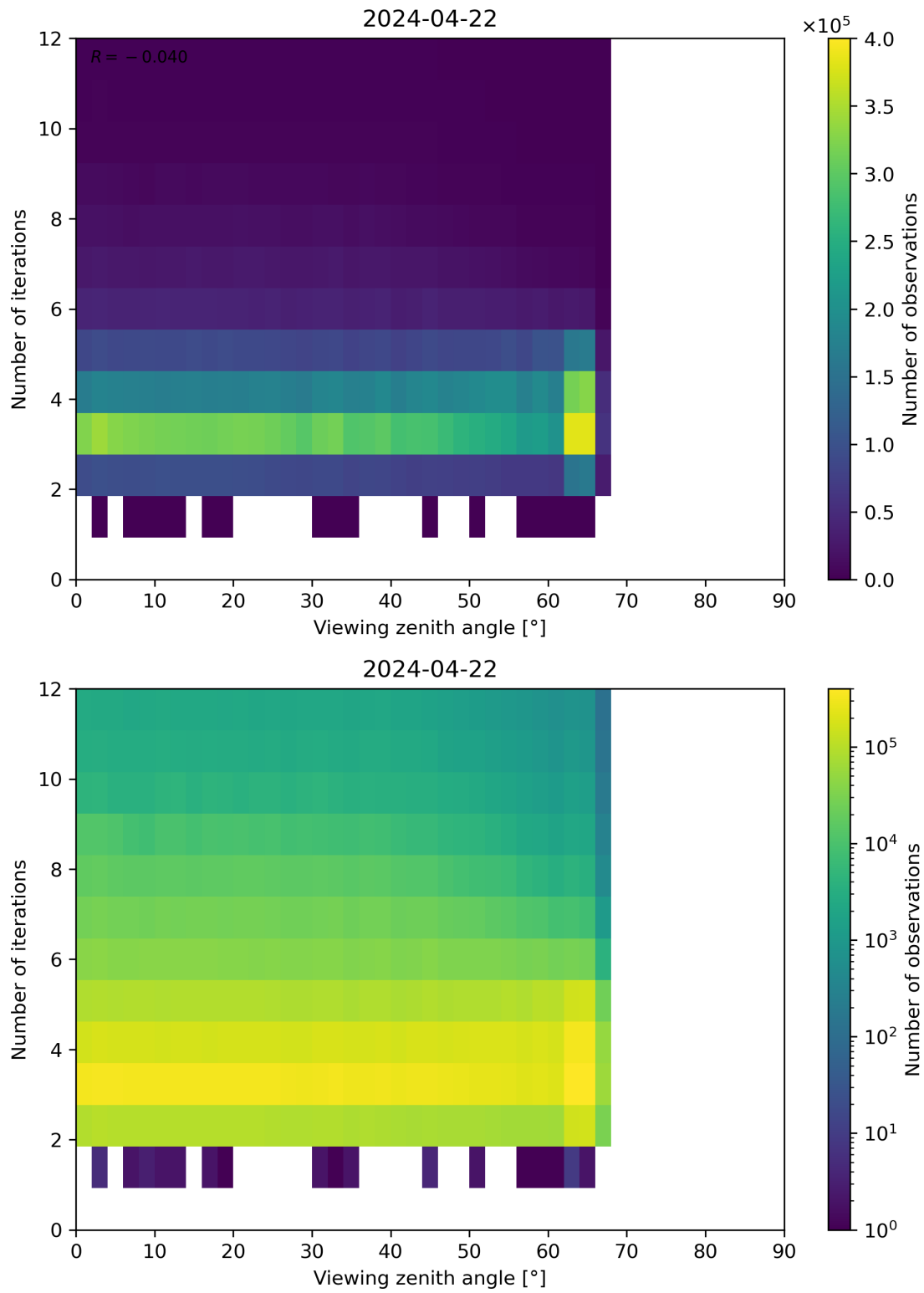
Figure 124: Scatter density plot of “Viewing zenith angle” against “Number of iterations” for 2024-04-21 to 2024-04-23.
