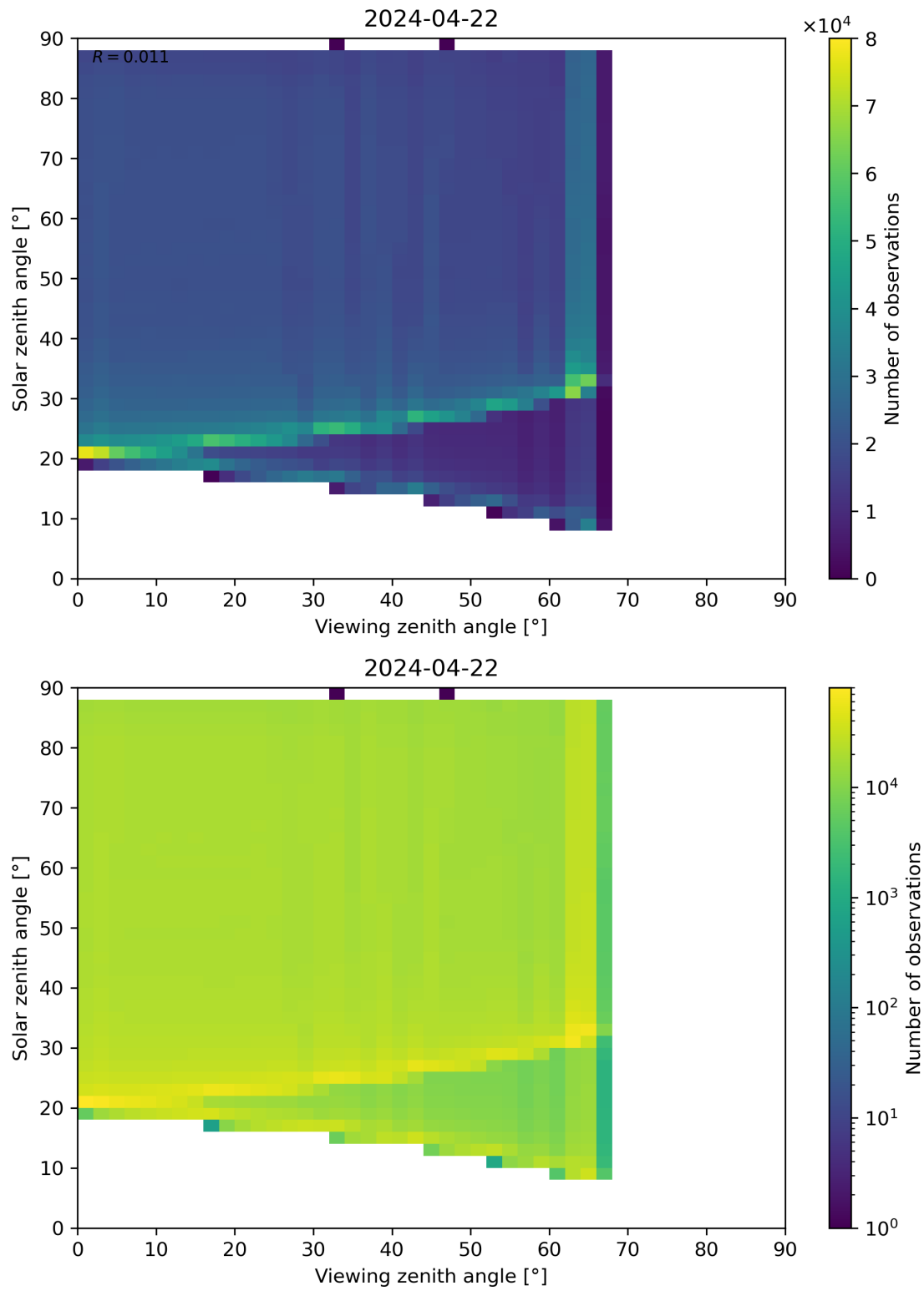
Figure 127: Scatter density plot of “Viewing zenith angle” against “Solar zenith angle” for 2024-04-21 to 2024-04-23.
