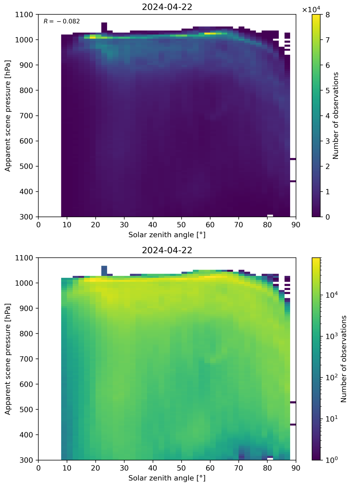
Figure 108: Scatter density plot of “Solar zenith angle” against “Apparent scene pressure” for 2024-04-21 to 2024-04-23.
