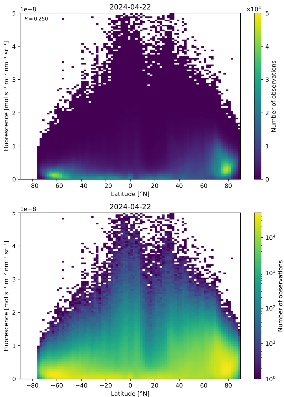
Figure 92: Scatter density plot of “Latitude” against “Fluorescence” for 2024-04-21 to 2024-04-23.
