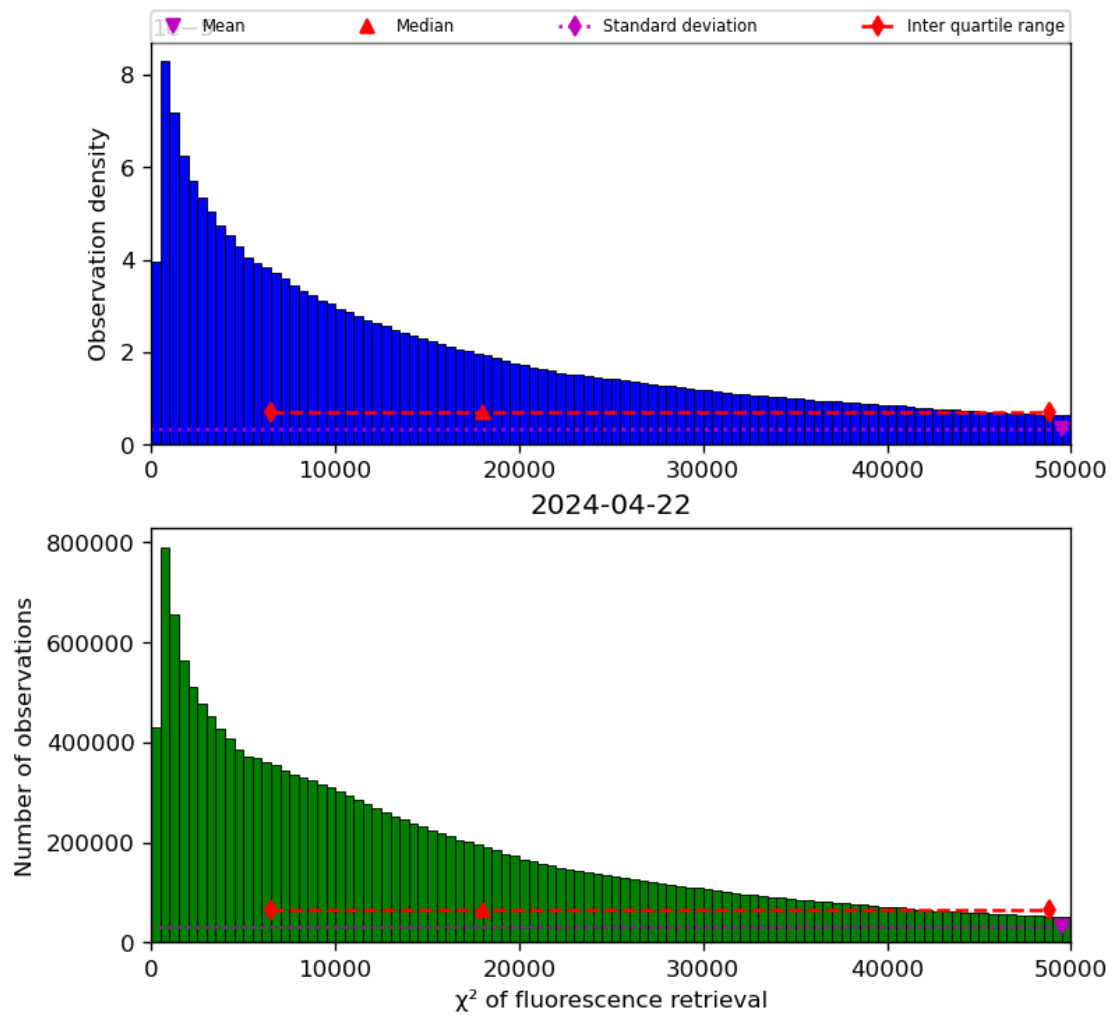
Figure 42: Histogram of “ \chi^2 of fluorescence retrieval” for 2024-04-21 to 2024-04-23
