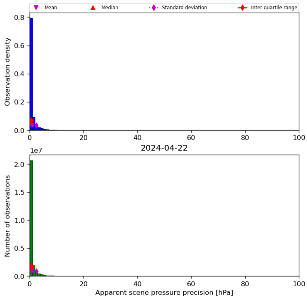
Figure 37: Histogram of “Apparent scene pressure precision” for 2024-04-21 to 2024-04-23
