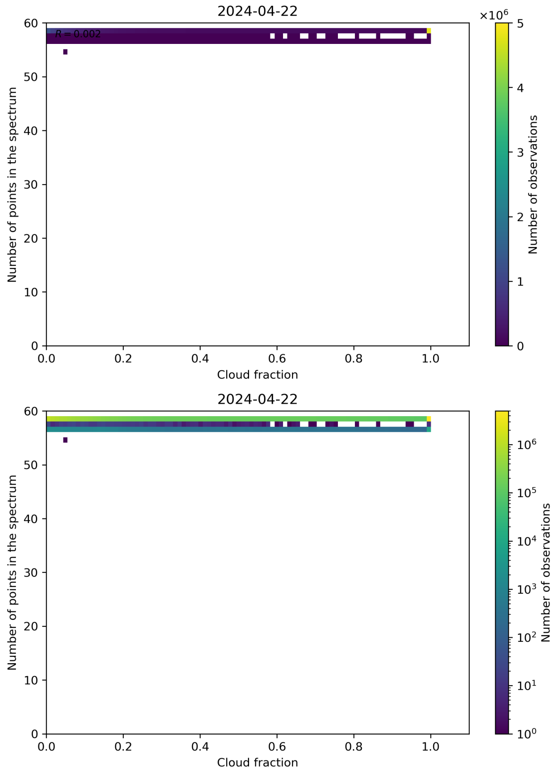
Figure 74: Scatter density plot of “Cloud fraction” against “Number of points in the spectrum” for 2024-04-21 to 2024-04-23.
