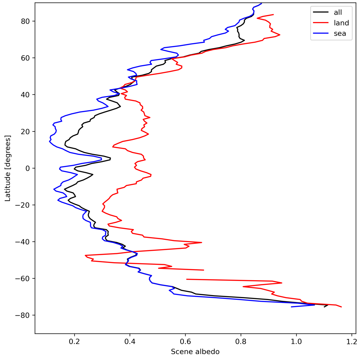
Figure 17: Zonal average of “Scene albedo” for 2024-04-21 to 2024-04-23.
