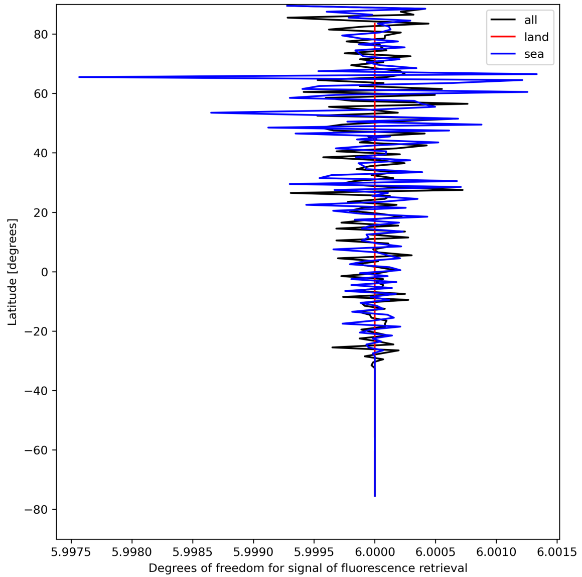
Figure 26: Zonal average of “Degrees of freedom for signal of fluorescence retrieval” for 2024-04-21 to 2024-04-23.
