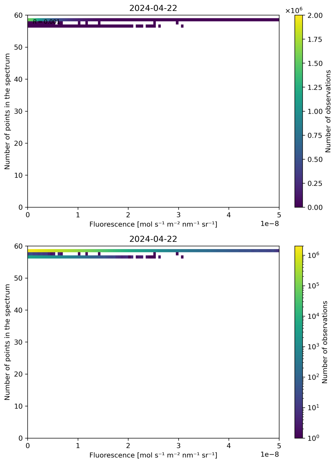
Figure 86: Scatter density plot of “Fluorescence” against “Number of points in the spectrum” for 2024-04-21 to 2024-04-23.
