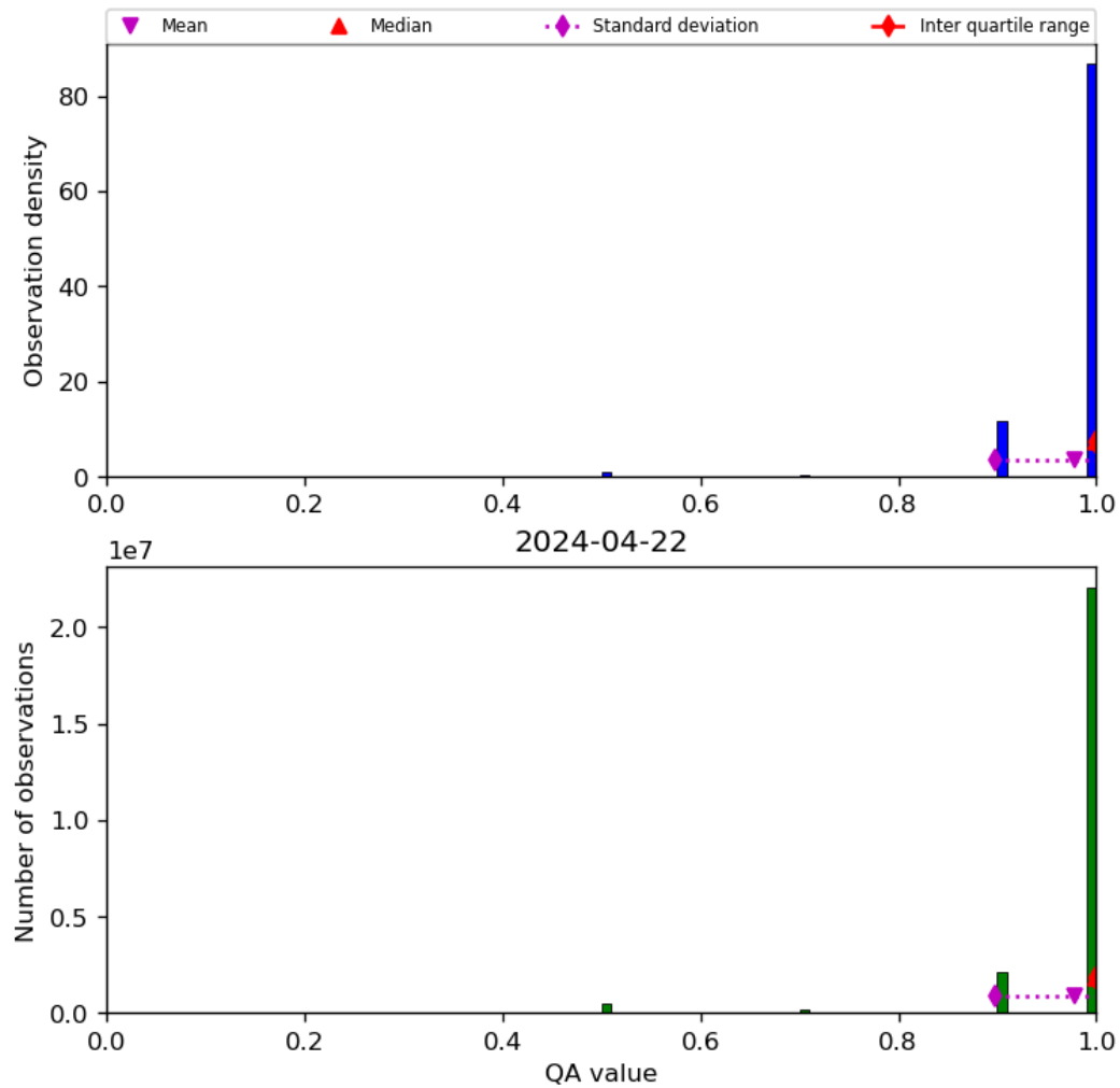
Figure 29: Histogram of “QA value” for 2024-04-21 to 2024-04-23
