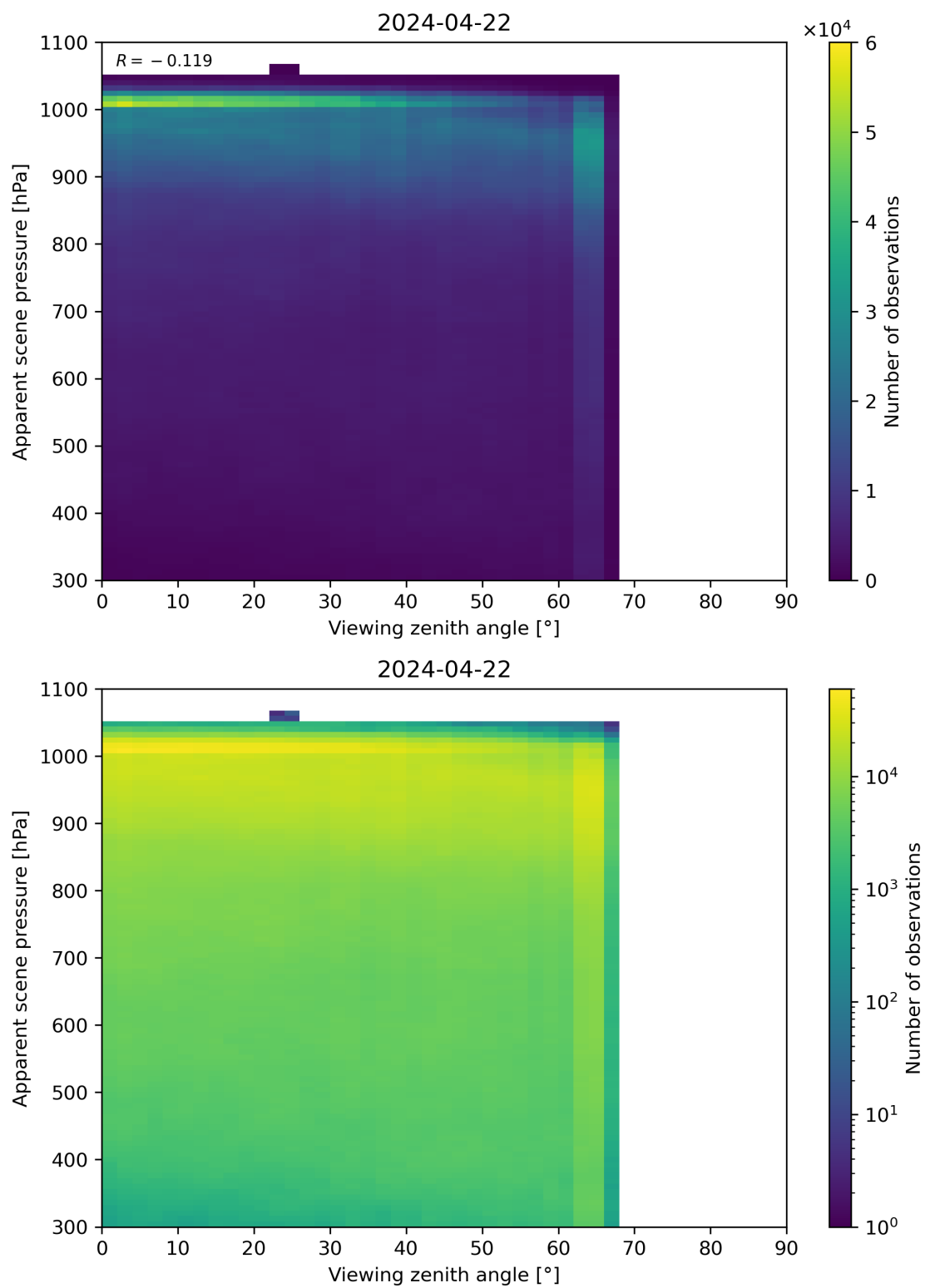
Figure 118: Scatter density plot of “Viewing zenith angle” against “Apparent scene pressure” for 2024-04-21 to 2024-04-23.
