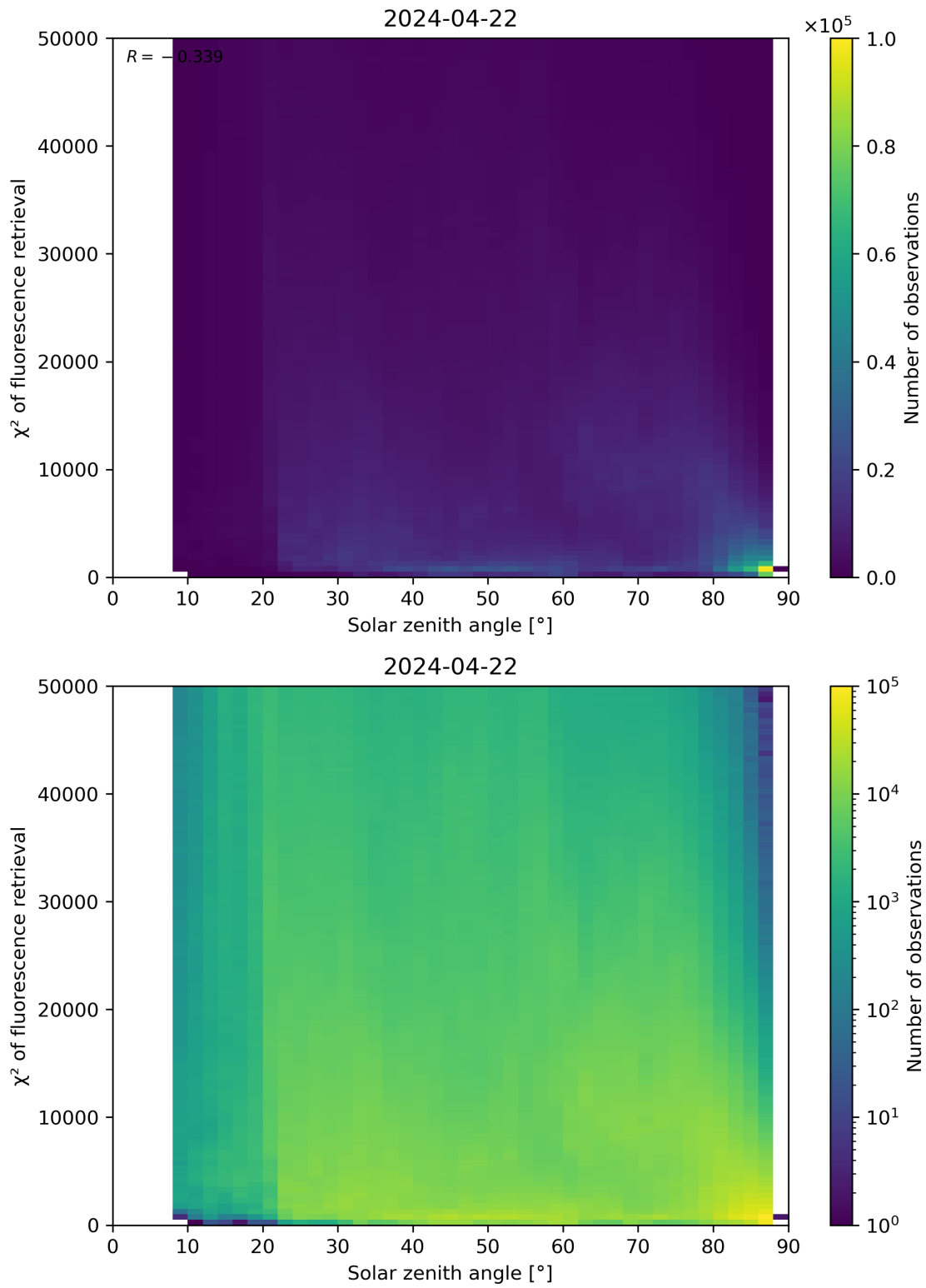
Figure 109: Scatter density plot of “Solar zenith angle” against “ \chi^2 of fluorescence retrieval” for 2024-04-21 to 2024-04-23.
