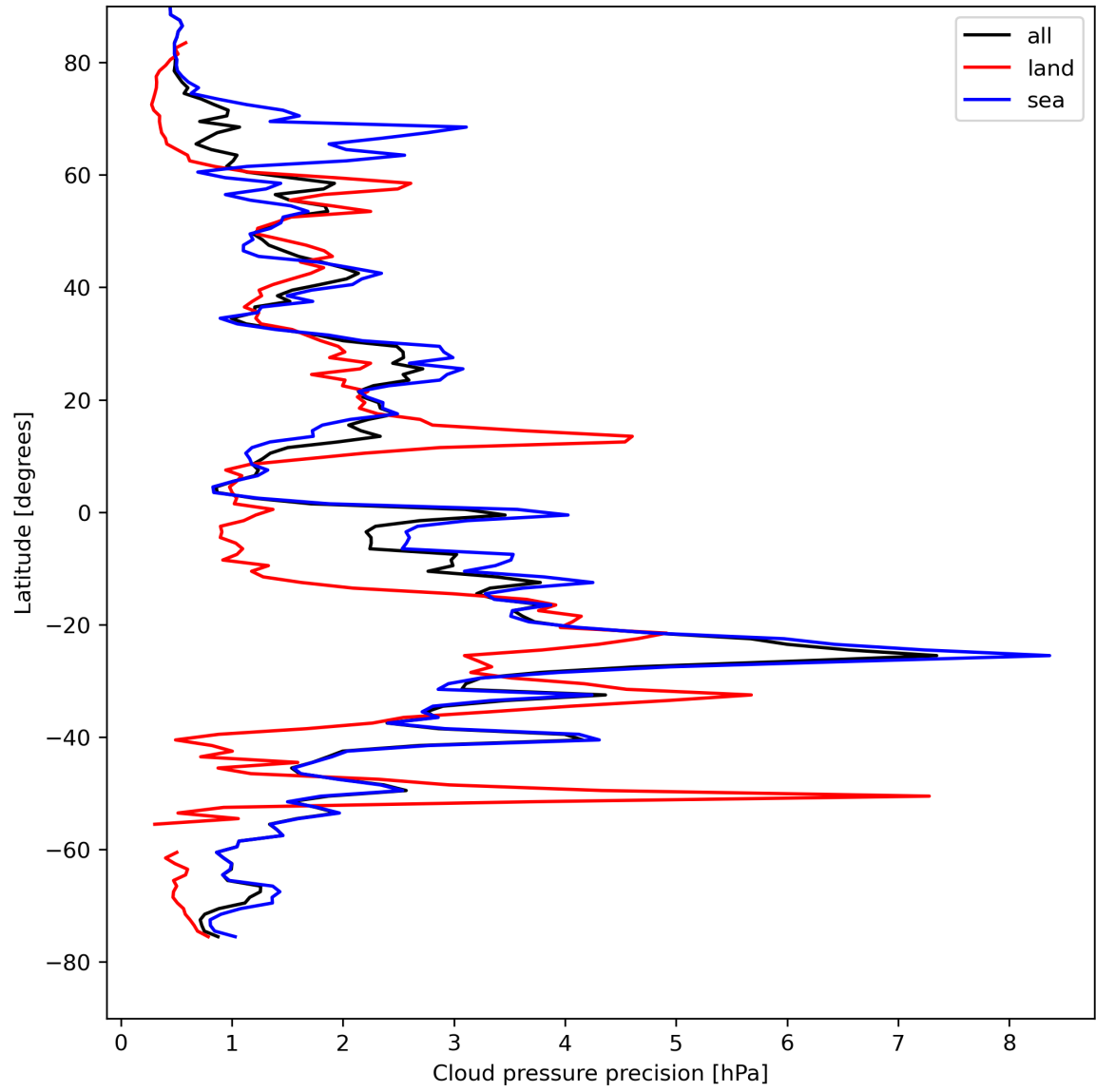
Figure 14: Zonal average of “Cloud pressure precision” for 2024-04-21 to 2024-04-23.
