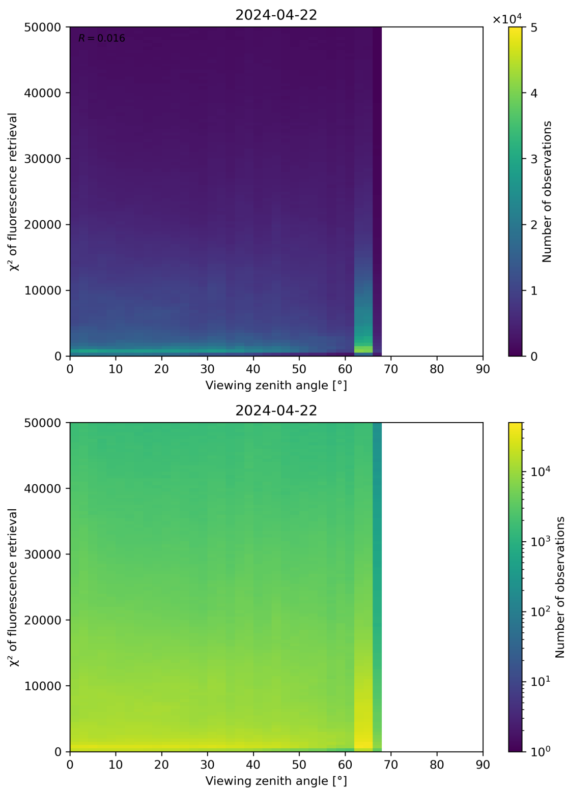
Figure 119: Scatter density plot of “Viewing zenith angle” against “ \chi^2 of fluorescence retrieval” for 2024-04-21 to 2024-04-23.
