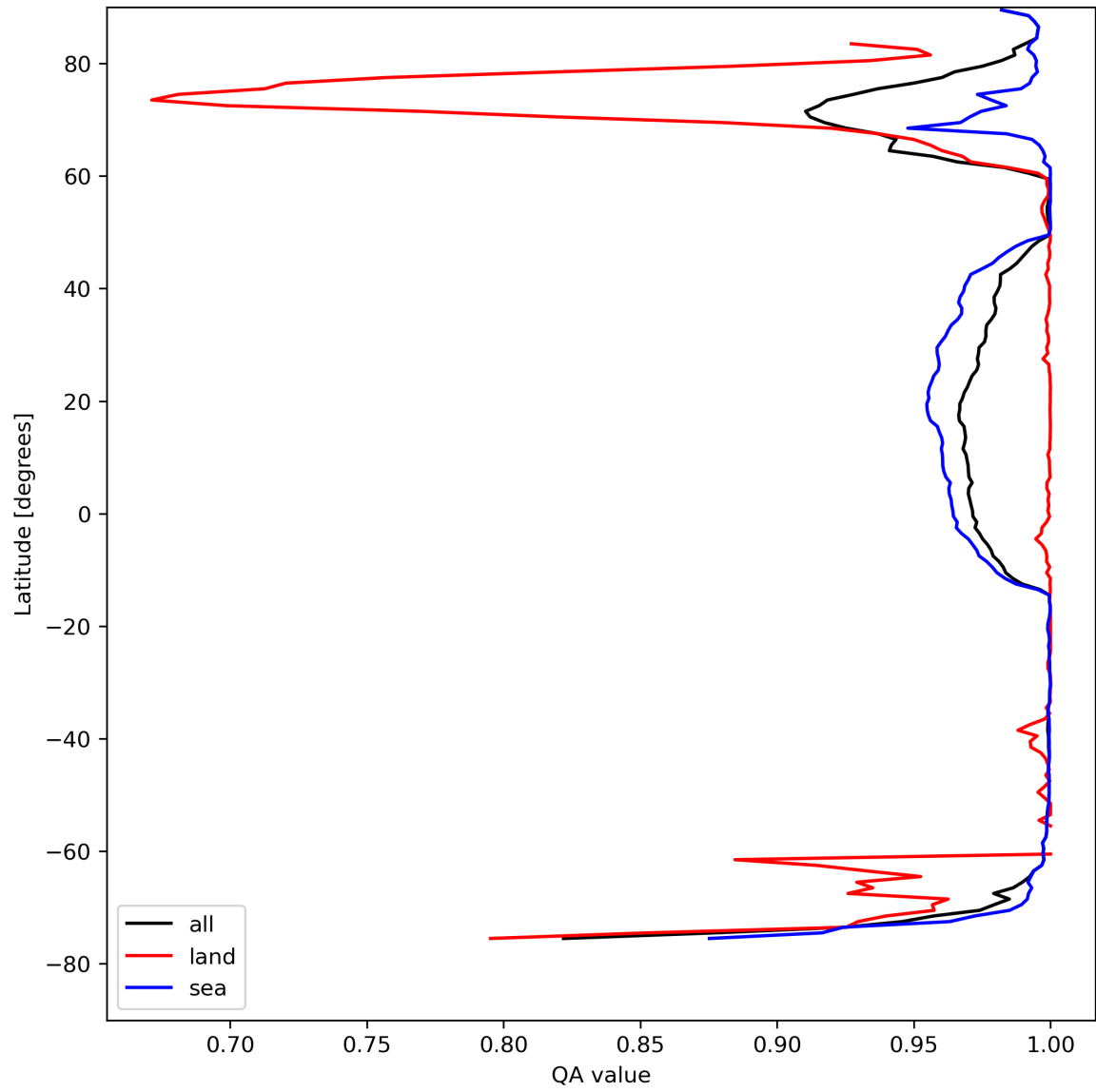
Figure 12: Zonal average of “QA value” for 2024-04-21 to 2024-04-23.
