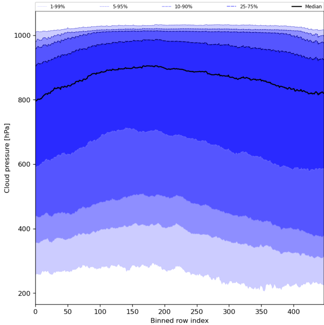
Figure 47: Along track statistics of “Cloud pressure” for 2024-04-21 to 2024-04-23
