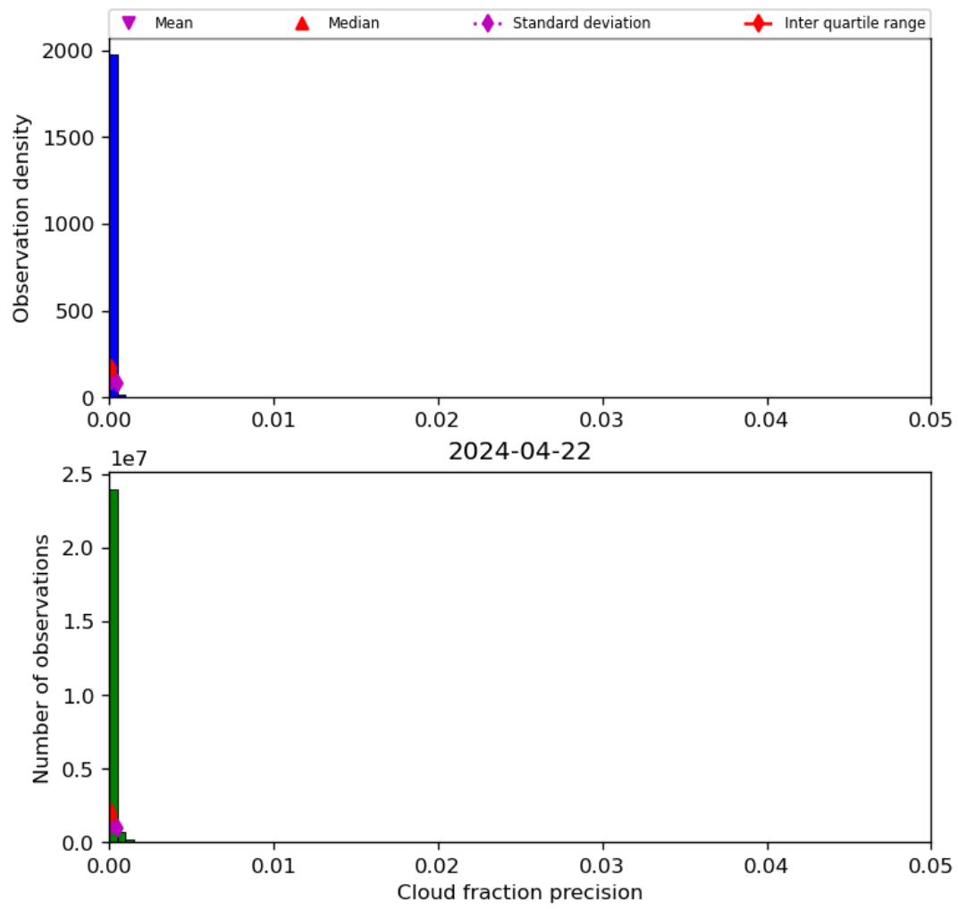
Figure 33: Histogram of “Cloud fraction precision” for 2024-04-21 to 2024-04-23
