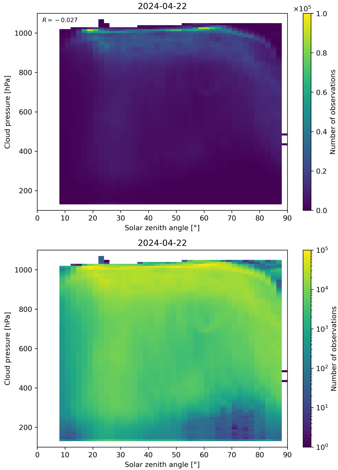
Figure 111: Scatter density plot of “Solar zenith angle” against “Cloud pressure” for 2024-04-21 to 2024-04-23.
