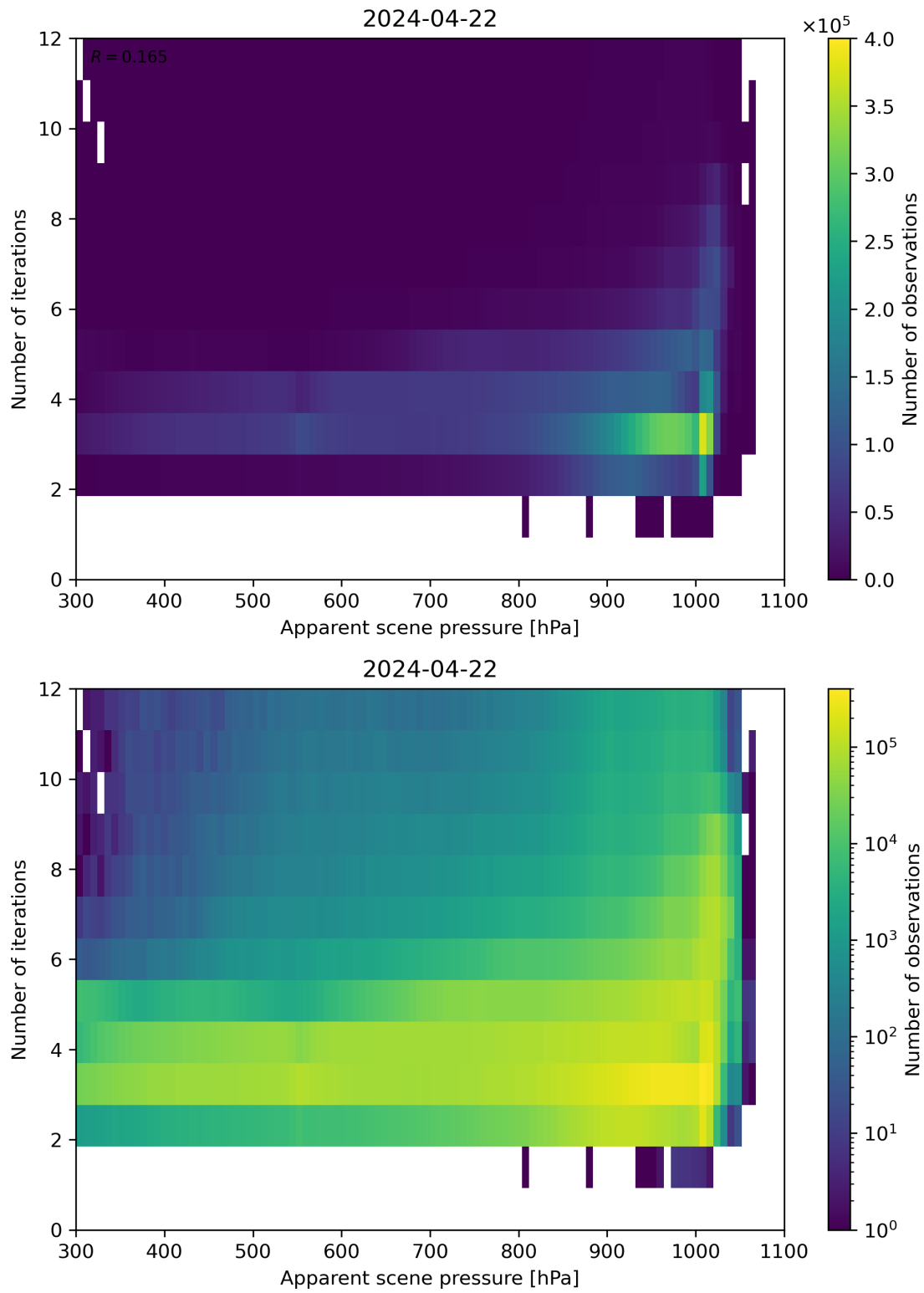
Figure 65: Scatter density plot of “Apparent scene pressure” against “Number of iterations” for 2024-04-21 to 2024-04-23.
