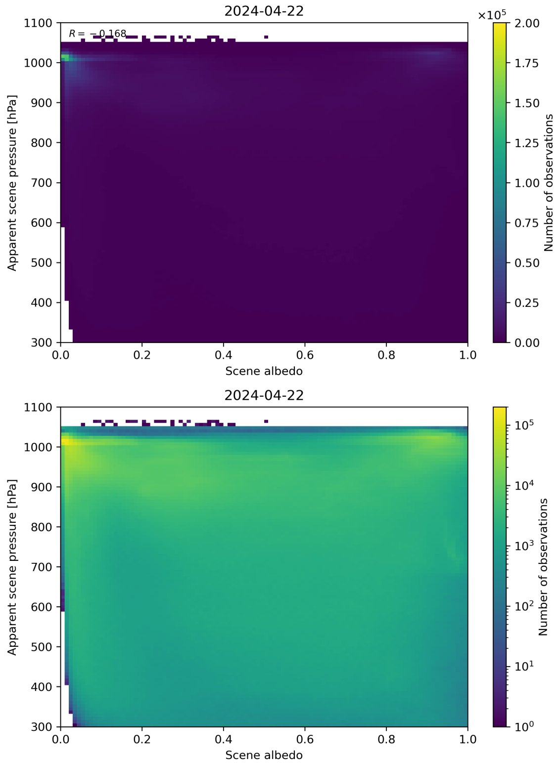
Figure 102: Scatter density plot of “Scene albedo” against “Apparent scene pressure” for 2024-04-21 to 2024-04-23.
