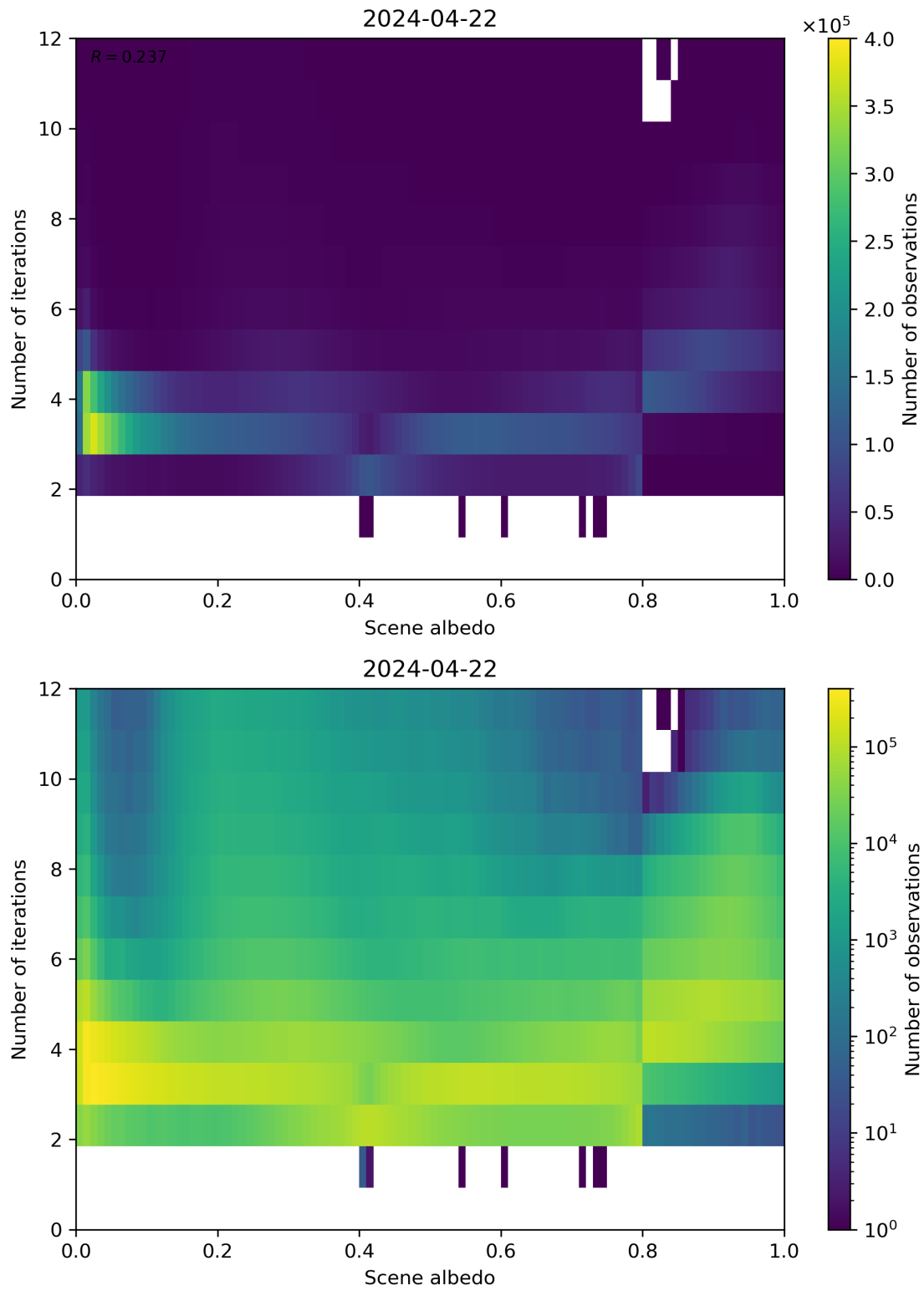
Figure 105: Scatter density plot of “Scene albedo” against “Number of iterations” for 2024-04-21 to 2024-04-23.
