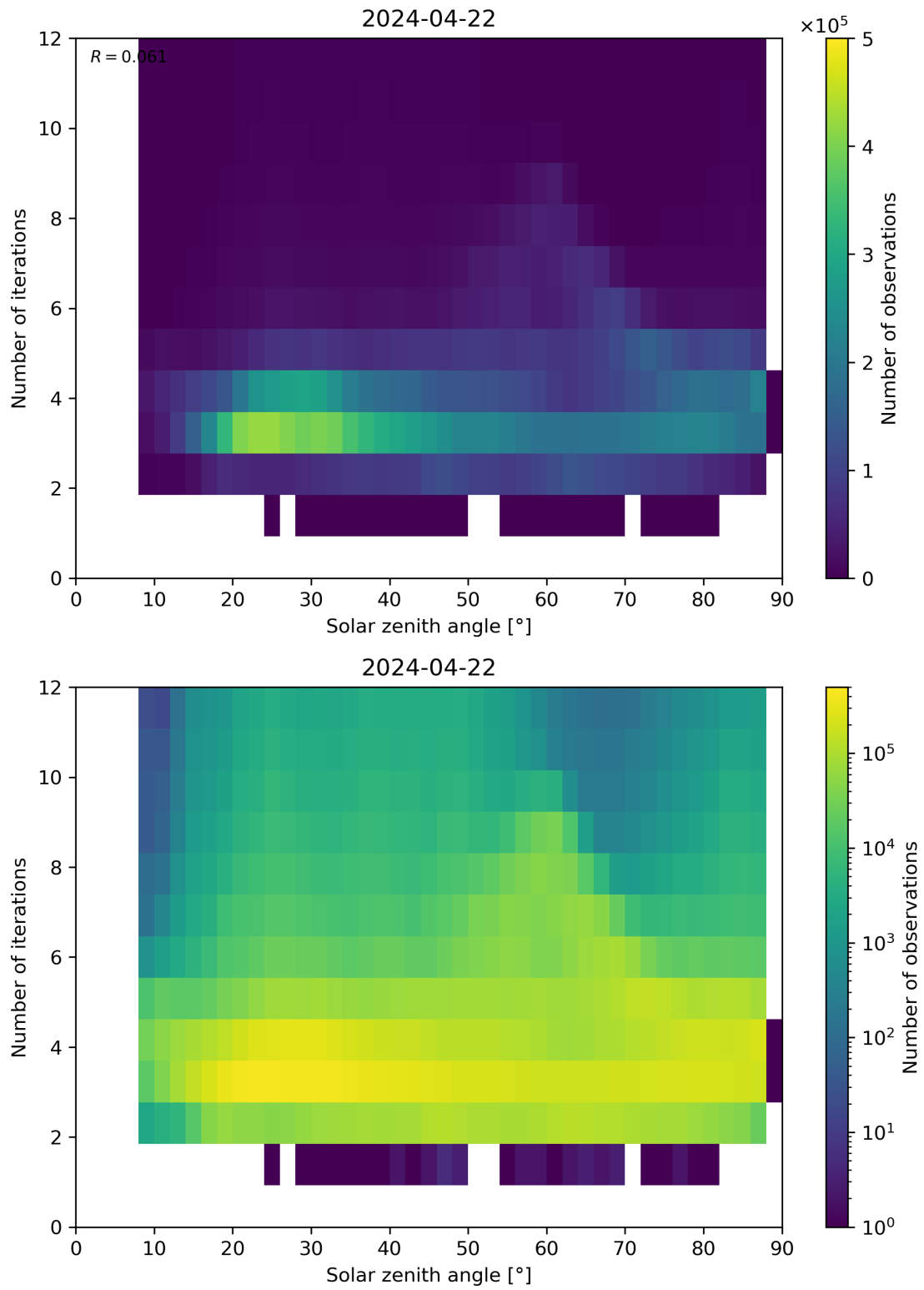
Figure 114: Scatter density plot of “Solar zenith angle” against “Number of iterations” for 2024-04-21 to 2024-04-23.
