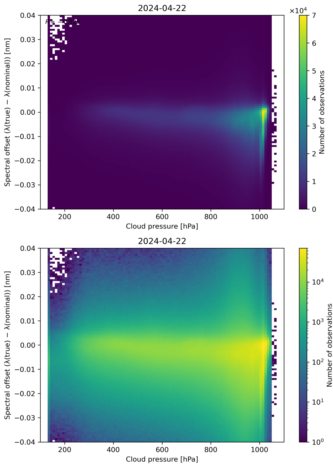
Figure 84: Scatter density plot of “Cloud pressure” against “Spectral offset ( \lambda(\text{true}) - \lambda(\text{nominal}) )” for 2024-04-21 to 2024-04-23.
