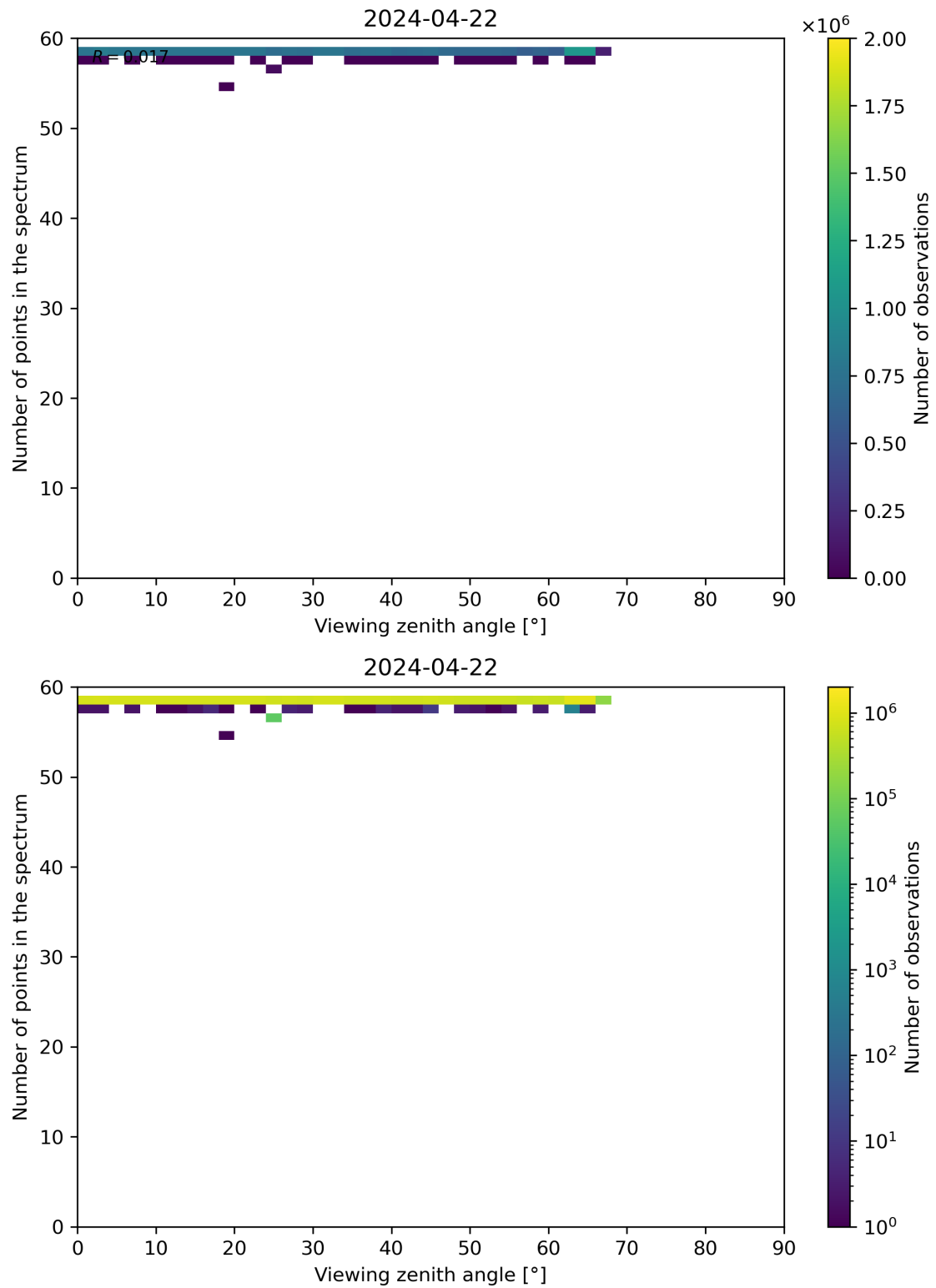
Figure 125: Scatter density plot of “Viewing zenith angle” against “Number of points in the spectrum” for 2024-04-21 to 2024-04-23.
