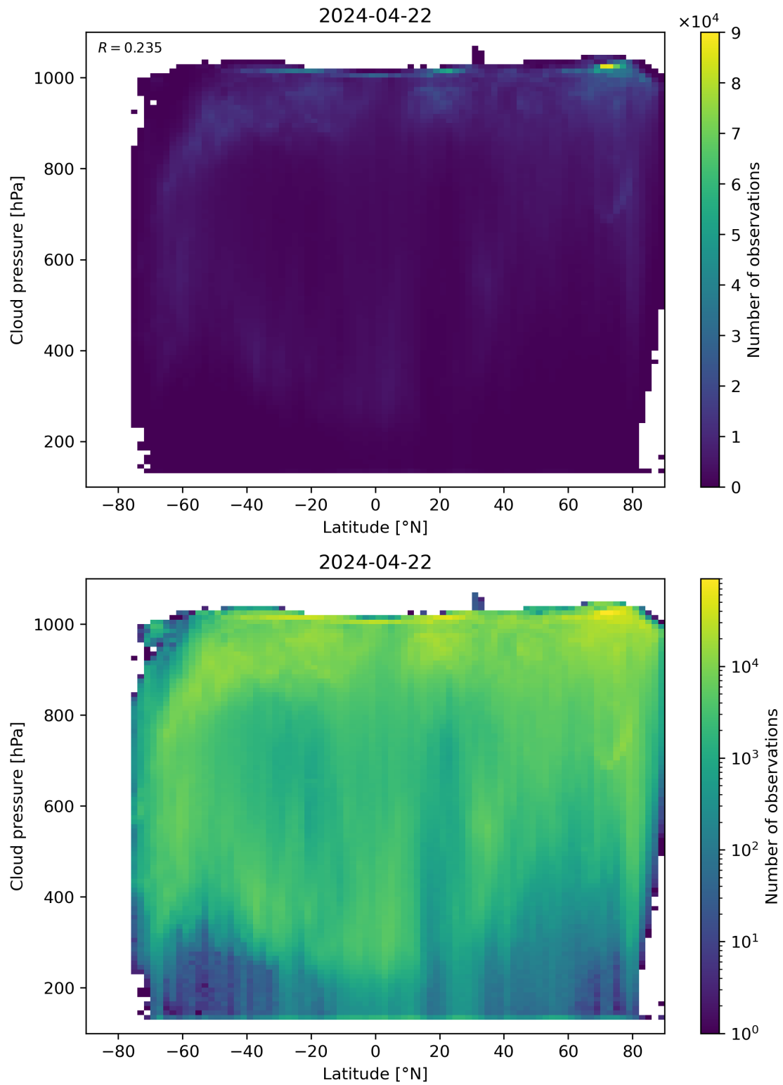
Figure 91: Scatter density plot of “Latitude” against “Cloud pressure” for 2024-04-21 to 2024-04-23.
