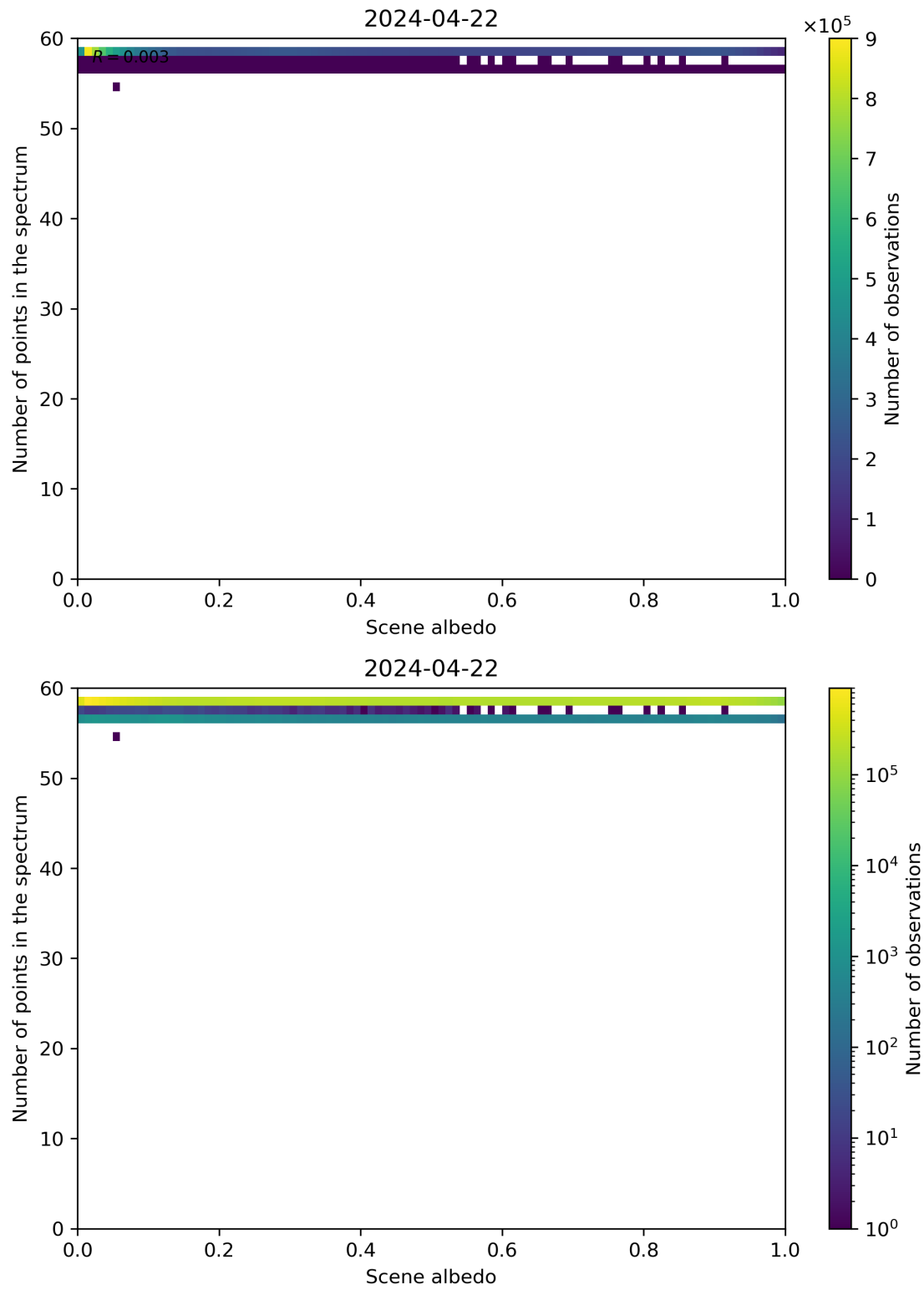
Figure 106: Scatter density plot of “Scene albedo” against “Number of points in the spectrum” for 2024-04-21 to 2024-04-23.
