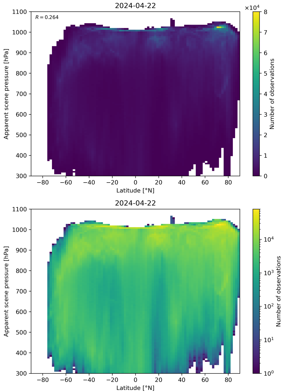
Figure 88: Scatter density plot of “Latitude” against “Apparent scene pressure” for 2024-04-21 to 2024-04-23.
