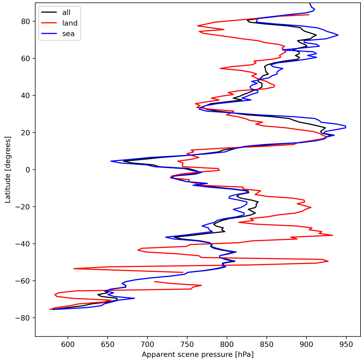
Figure 19: Zonal average of “Apparent scene pressure” for 2024-04-21 to 2024-04-23.
