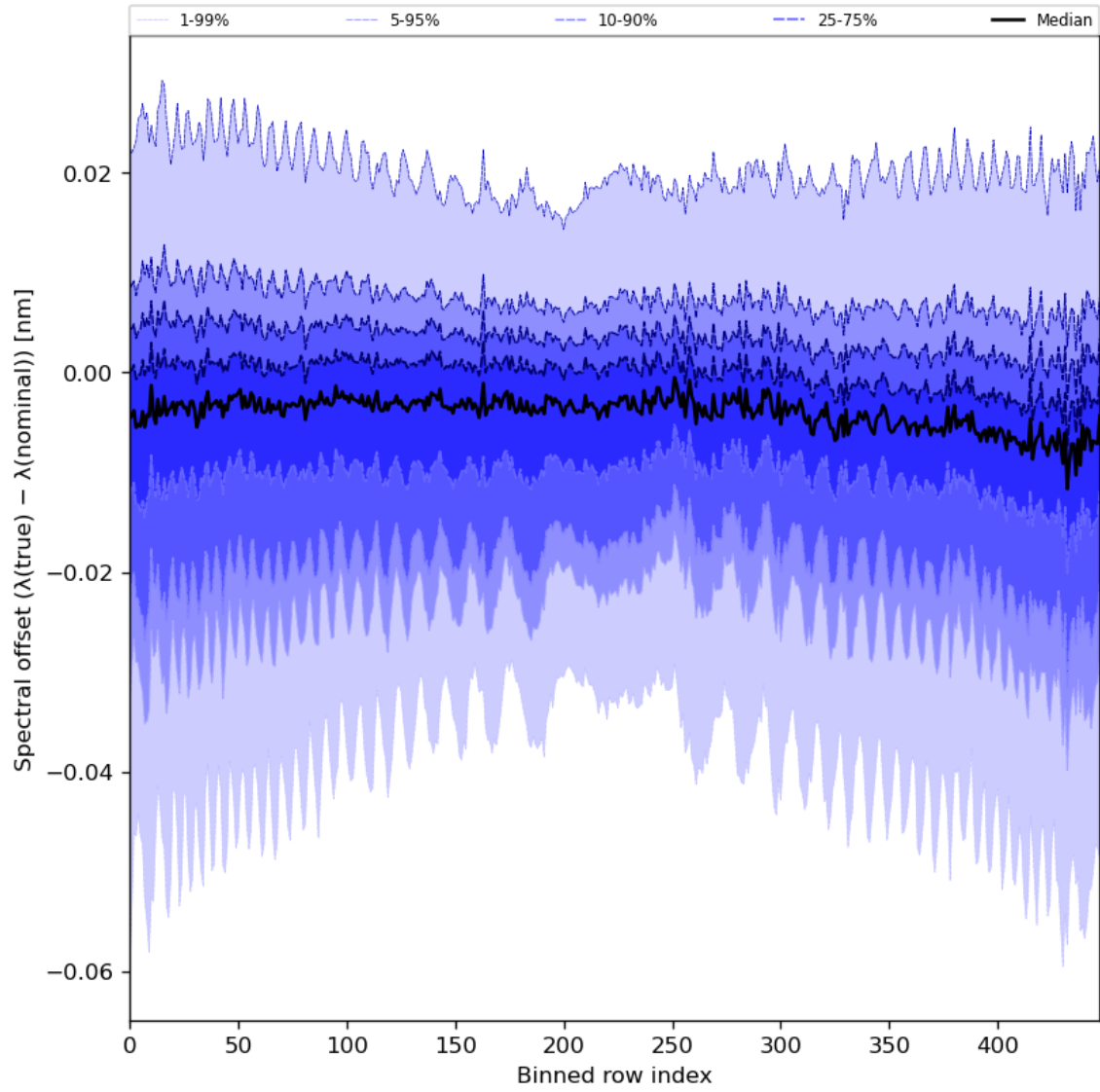
Figure 62: Along track statistics of “Spectral offset ( \lambda(\text{true}) - \lambda(\text{nominal}) )” for 2024-04-21 to 2024-04-23
