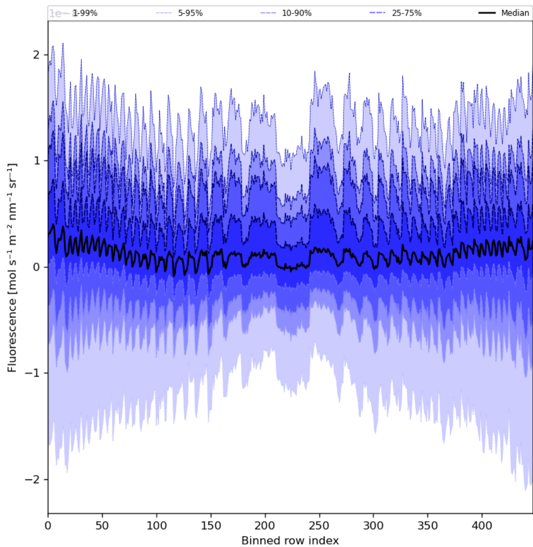
Figure 57: Along track statistics of “Fluorescence” for 2024-04-21 to 2024-04-23
