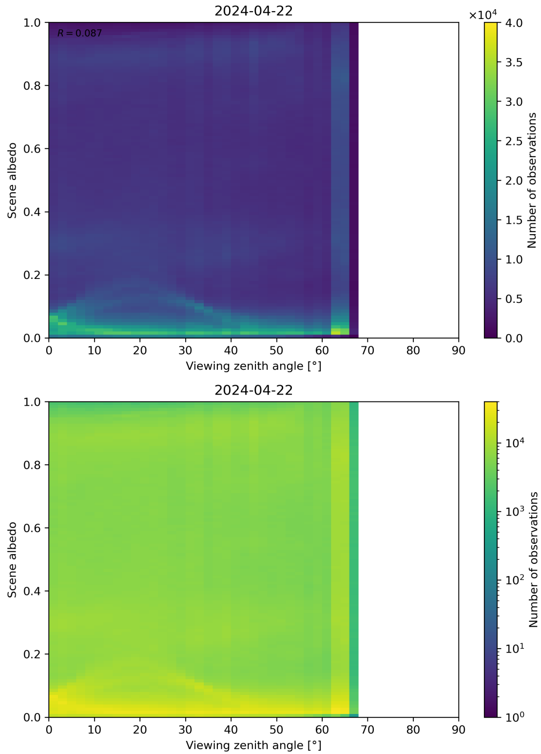
Figure 126: Scatter density plot of “Viewing zenith angle” against “Scene albedo” for 2024-04-21 to 2024-04-23.
