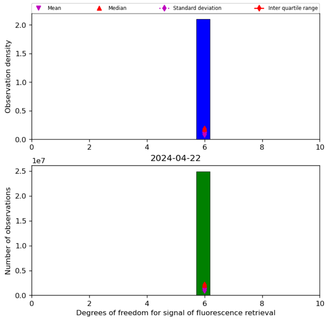
Figure 43: Histogram of “Degrees of freedom for signal of fluorescence retrieval” for 2024-04-21 to 2024-04-23
