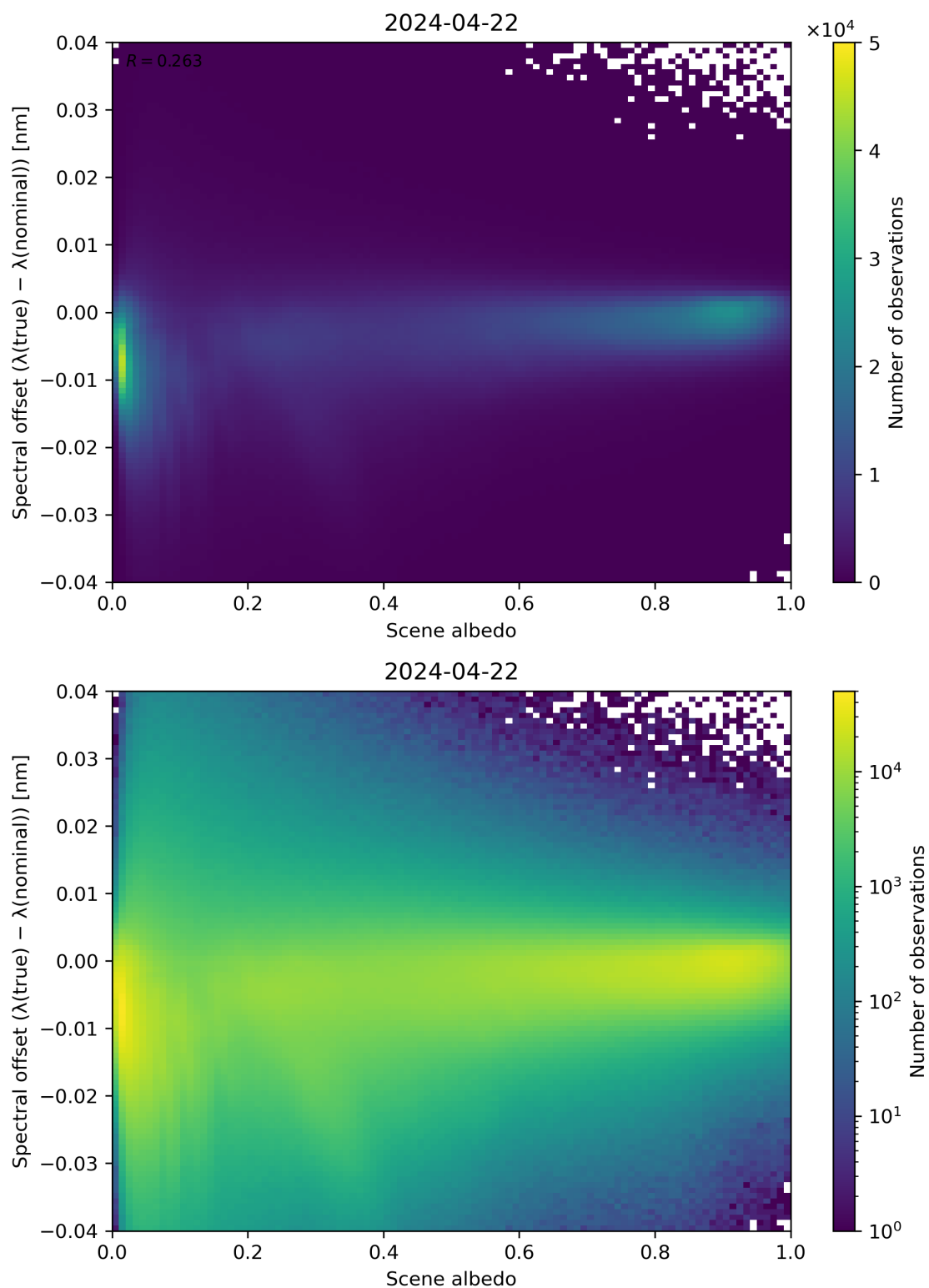
Figure 107: Scatter density plot of “Scene albedo” against “Spectral offset ( \lambda(\text{true}) - \lambda(\text{nominal}) )” for 2024-04-21 to 2024-04-23.
