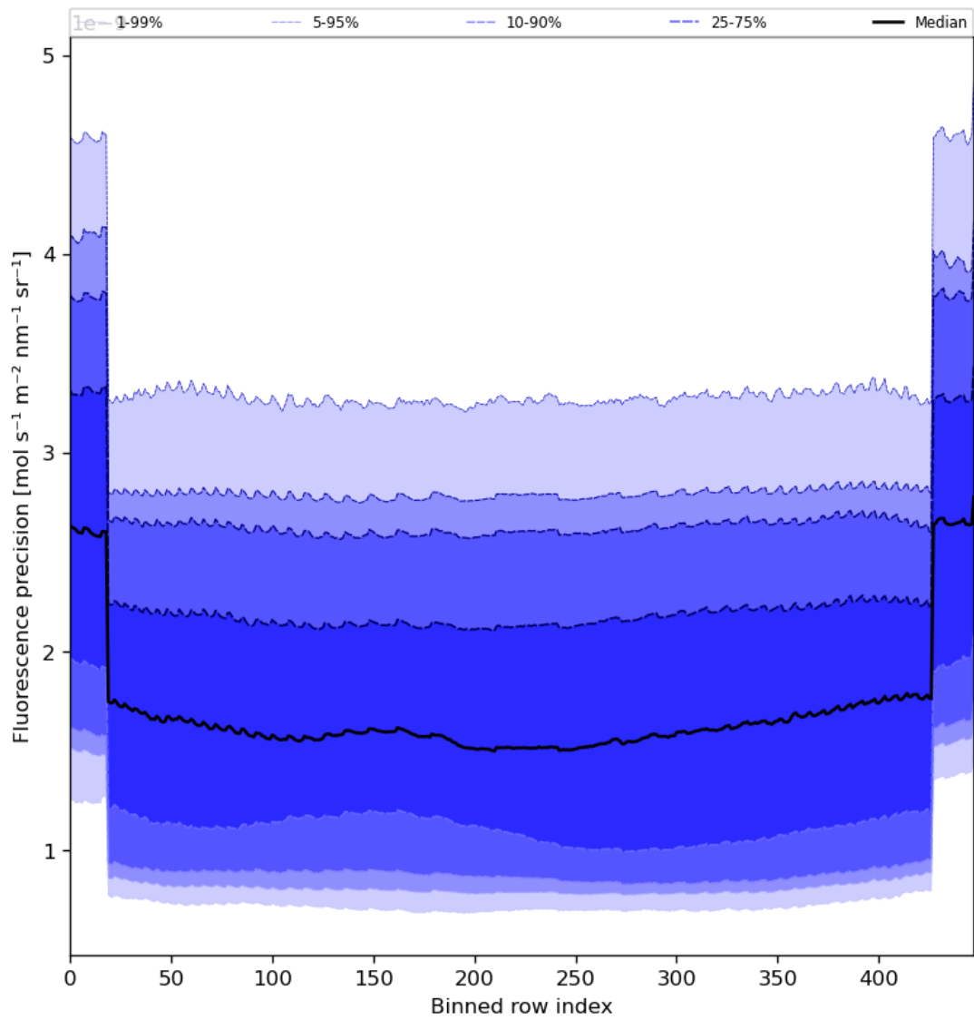
Figure 58: Along track statistics of “Fluorescence precision” for 2024-04-21 to 2024-04-23
