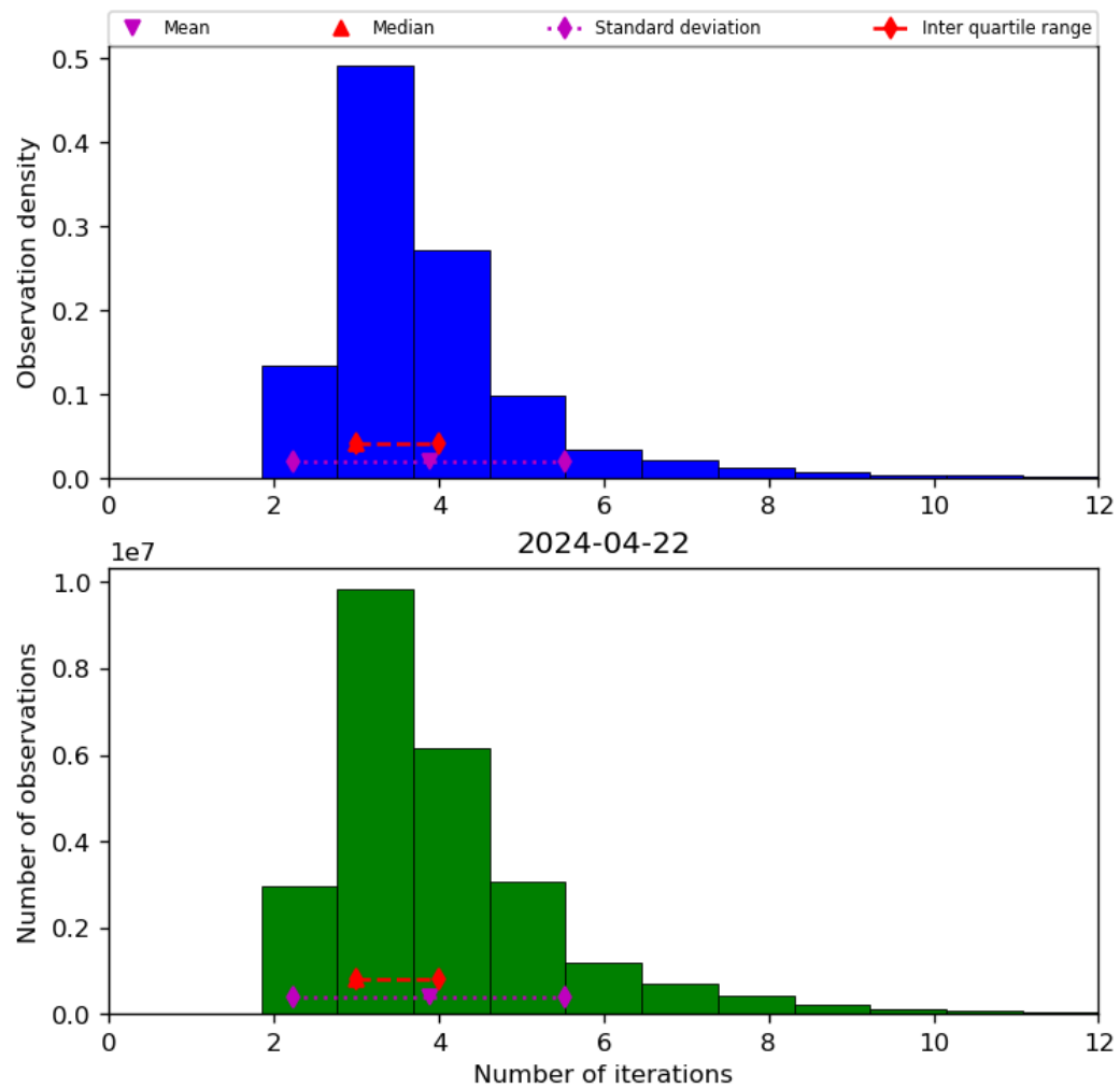
Figure 39: Histogram of “Number of iterations” for 2024-04-21 to 2024-04-23
