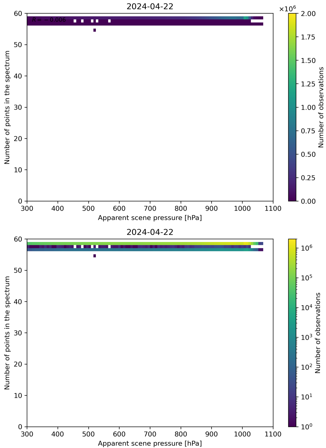
Figure 66: Scatter density plot of “Apparent scene pressure” against “Number of points in the spectrum” for 2024-04-21 to 2024-04-23.
