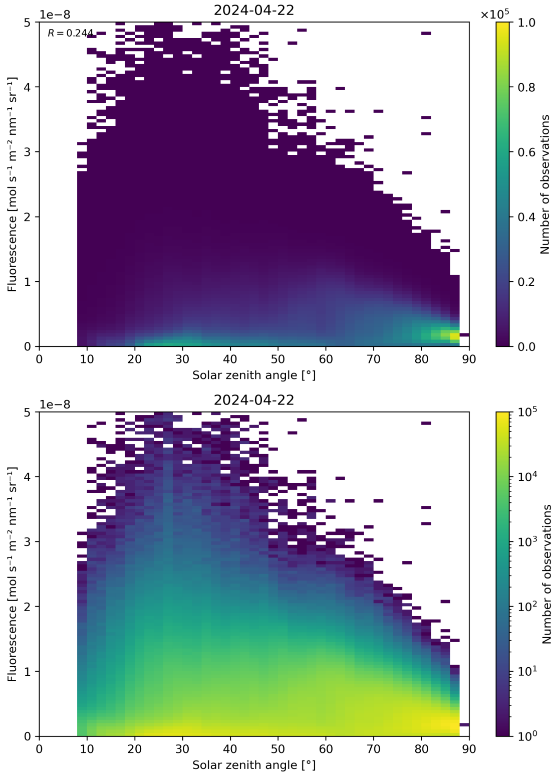
Figure 112: Scatter density plot of “Solar zenith angle” against “Fluorescence” for 2024-04-21 to 2024-04-23.
