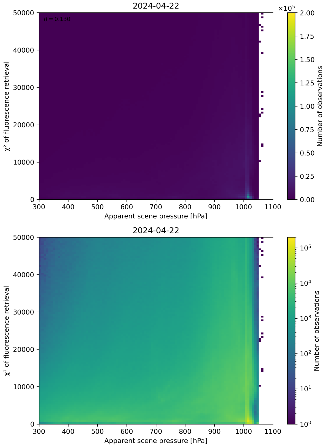
Figure 63: Scatter density plot of “Apparent scene pressure” against “ \chi^2 of fluorescence retrieval” for 2024-04-21 to 2024-04-23.
