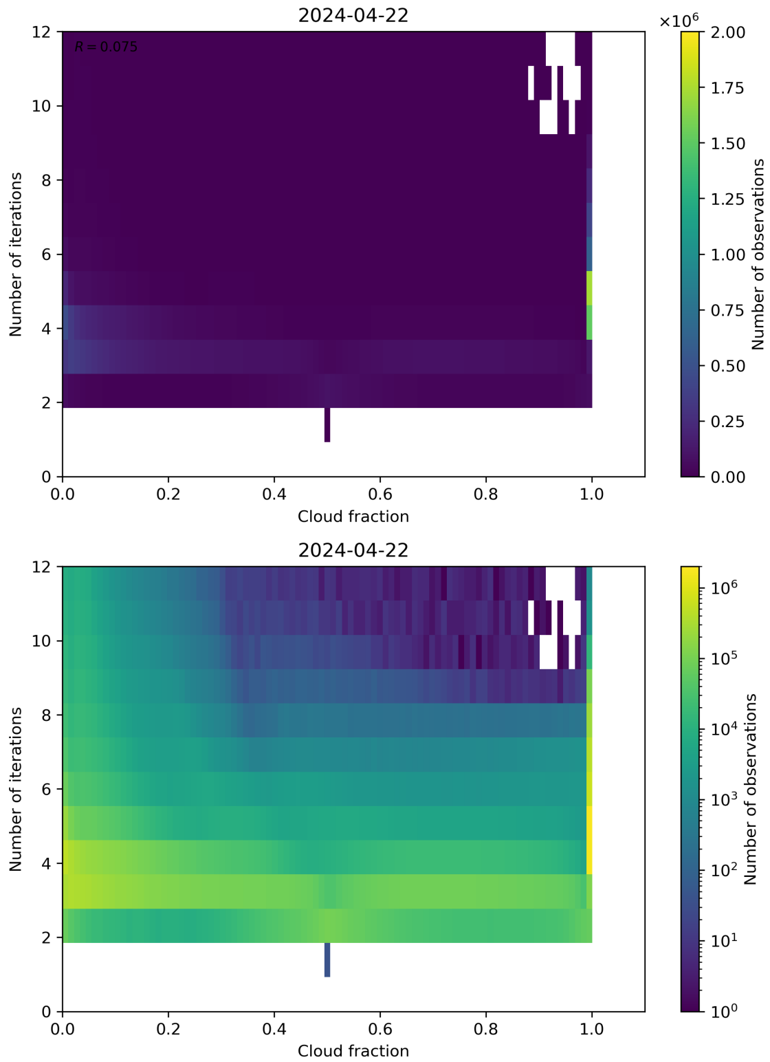
Figure 73: Scatter density plot of “Cloud fraction” against “Number of iterations” for 2024-04-21 to 2024-04-23.
