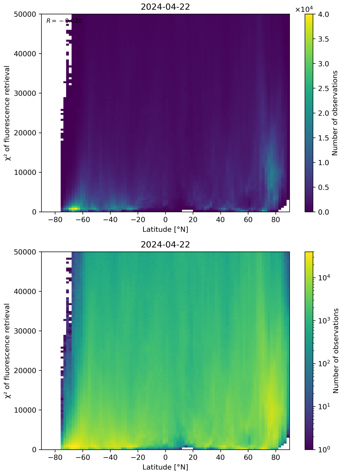
Figure 89: Scatter density plot of “Latitude” against “ \chi^2 of fluorescence retrieval” for 2024-04-21 to 2024-04-23.
