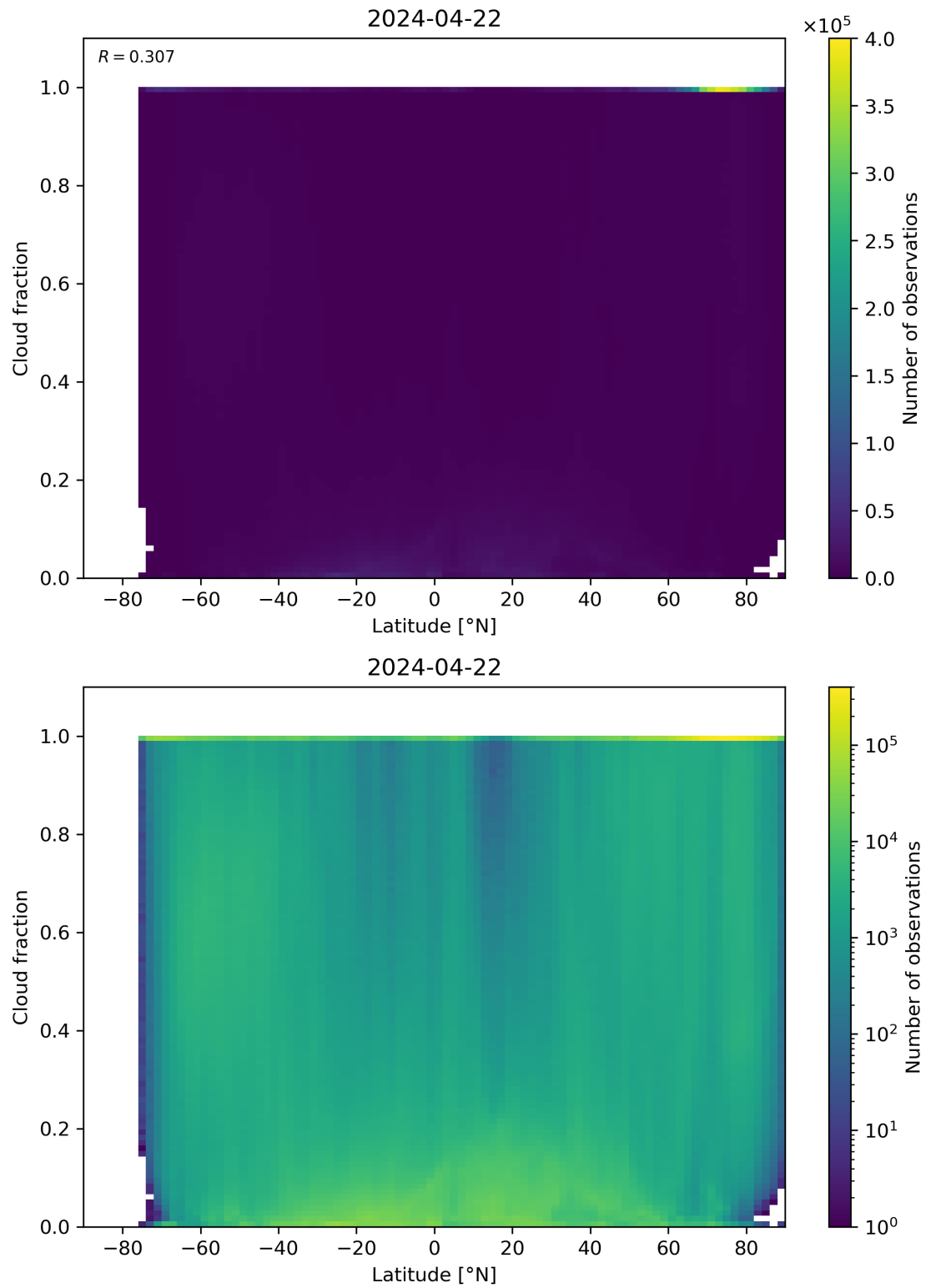
Figure 90: Scatter density plot of “Latitude” against “Cloud fraction” for 2024-04-21 to 2024-04-23.
