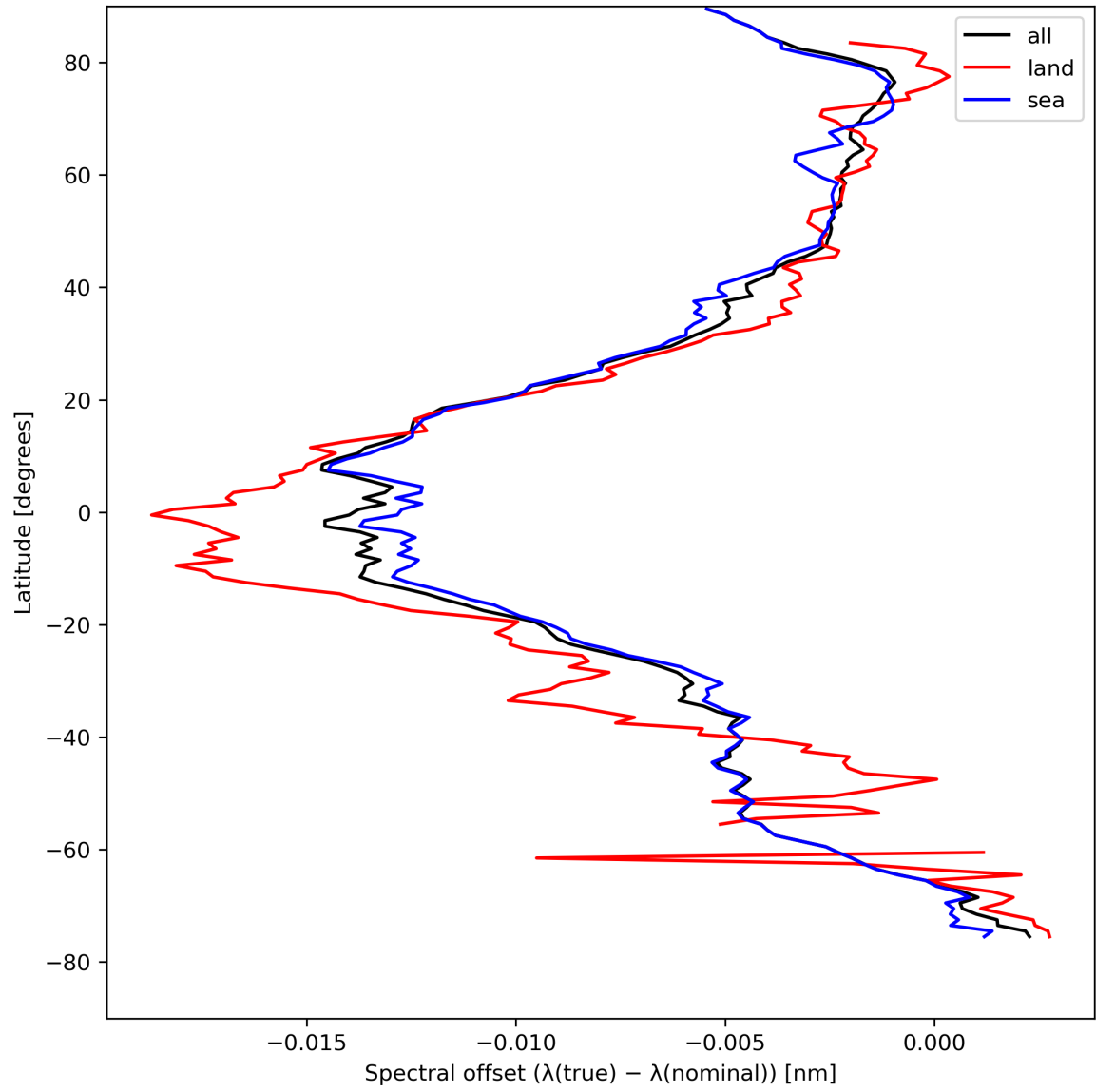
Figure 28: Zonal average of “Spectral offset ( \lambda(\text{true}) - \lambda(\text{nominal}) )” for 2024-04-21 to 2024-04-23.
