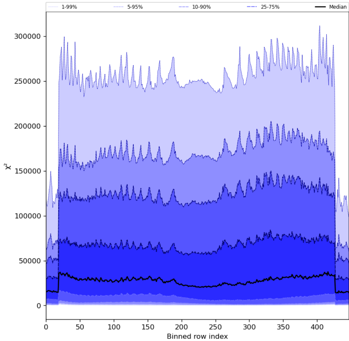
Figure 55: Along track statistics of “ \chi^2 ” for 2024-04-21 to 2024-04-23
