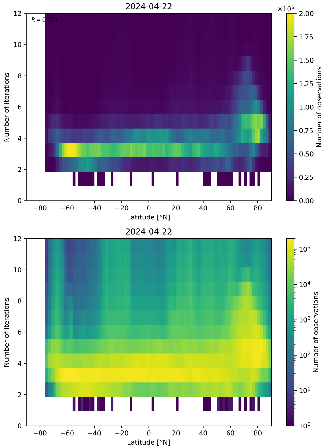
Figure 93: Scatter density plot of “Latitude” against “Number of iterations” for 2024-04-21 to 2024-04-23.
