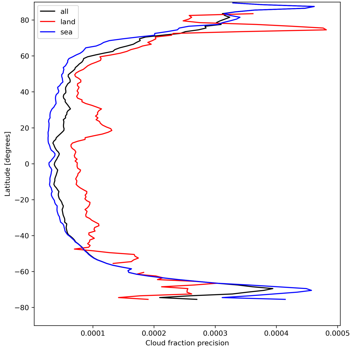
Figure 16: Zonal average of “Cloud fraction precision” for 2024-04-21 to 2024-04-23.
