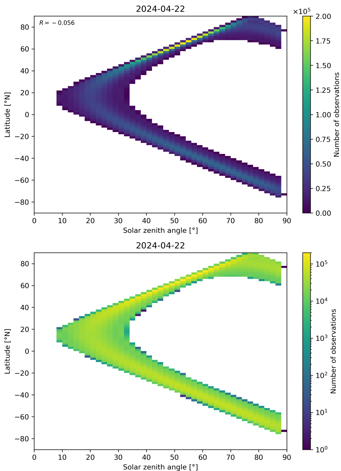
Figure 113: Scatter density plot of “Solar zenith angle” against “Latitude” for 2024-04-21 to 2024-04-23.
