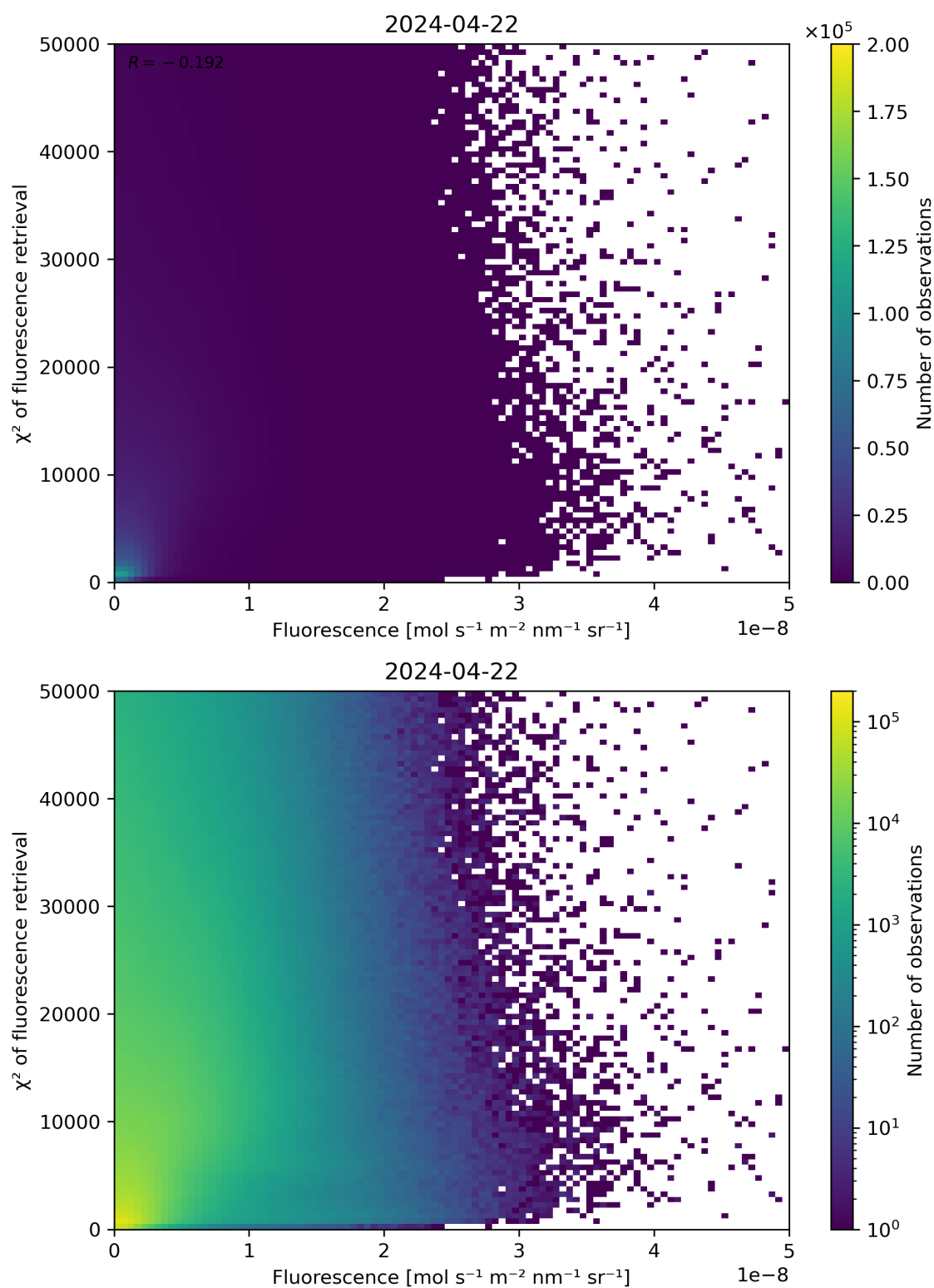
Figure 85: Scatter density plot of “Fluorescence” against “ \chi^2 of fluorescence retrieval” for 2024-04-21 to 2024-04-23.
