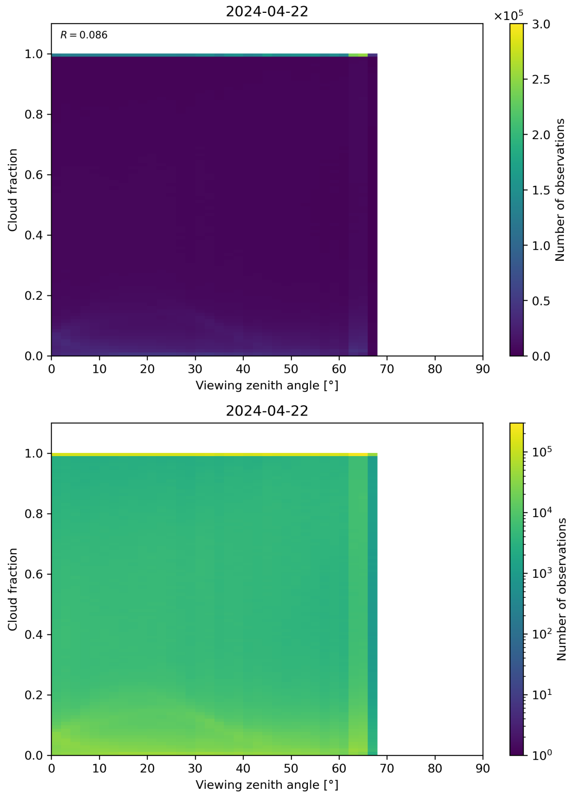
Figure 120: Scatter density plot of “Viewing zenith angle” against “Cloud fraction” for 2024-04-21 to 2024-04-23.
