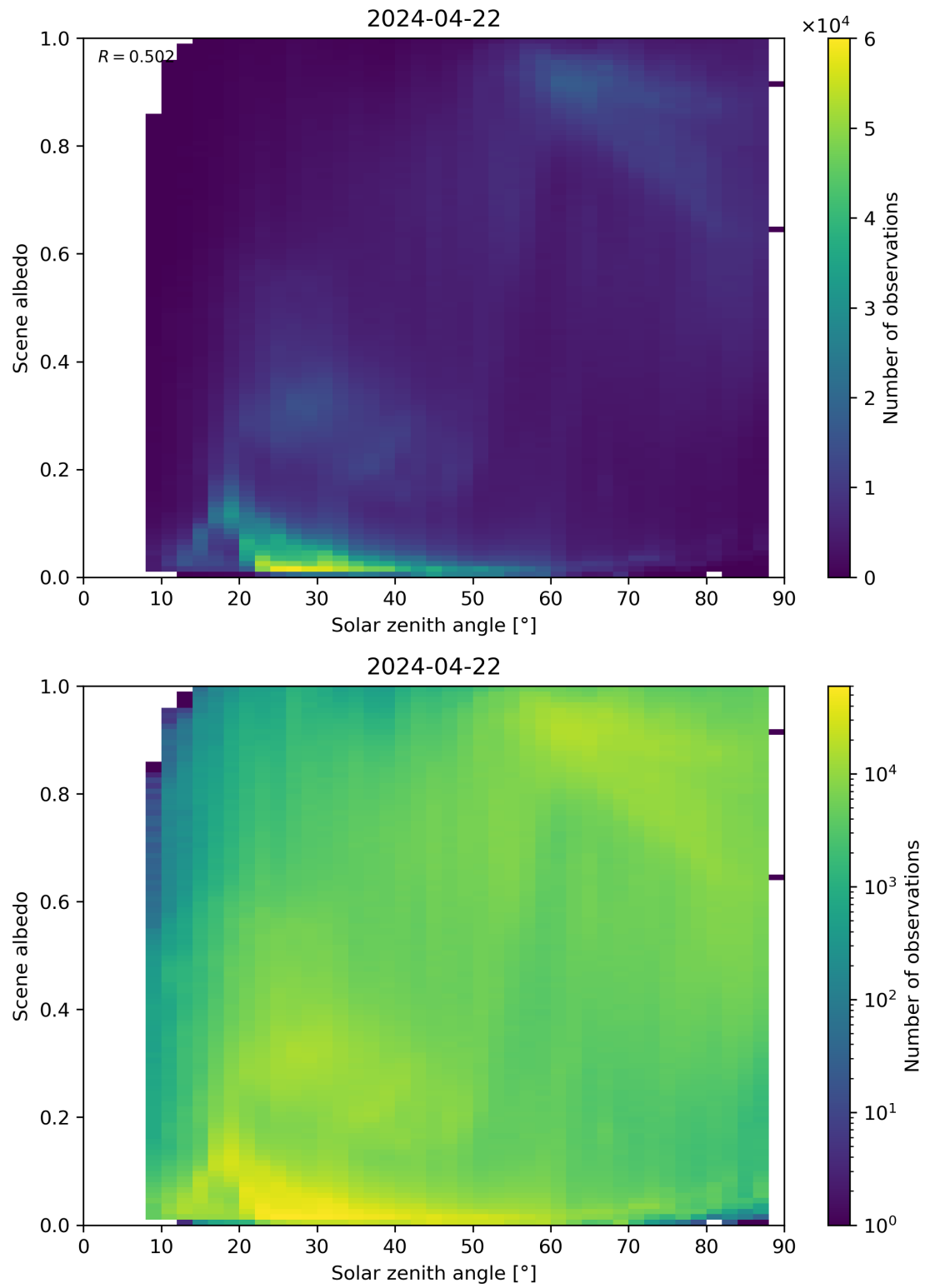
Figure 116: Scatter density plot of “Solar zenith angle” against “Scene albedo” for 2024-04-21 to 2024-04-23.
