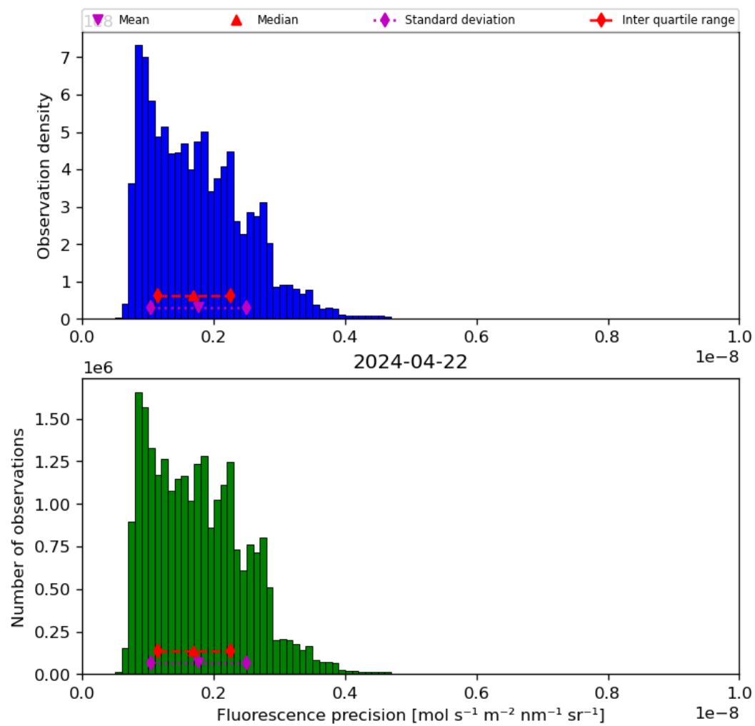
Figure 41: Histogram of “Fluorescence precision” for 2024-04-21 to 2024-04-23
