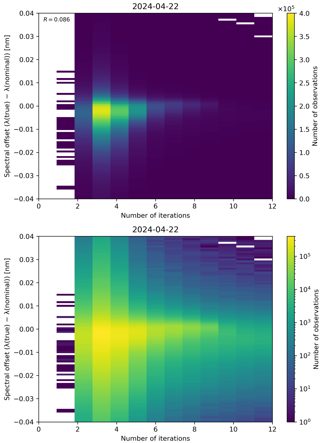
Figure 100: Scatter density plot of “Number of iterations” against “Spectral offset ( \lambda(\text{true}) - \lambda(\text{nominal}) )” for 2024-04-21 to 2024-04-23.
