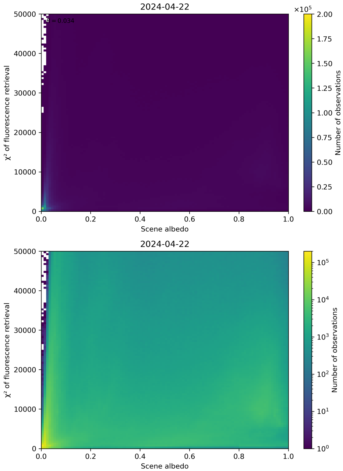
Figure 103: Scatter density plot of “Scene albedo” against “ \chi^2 of fluorescence retrieval” for 2024-04-21 to 2024-04-23.
