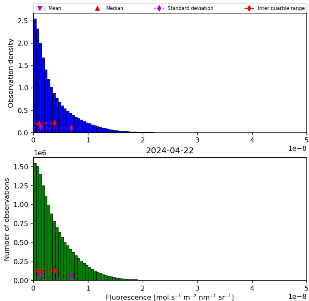
Figure 40: Histogram of “Fluorescence” for 2024-04-21 to 2024-04-23
