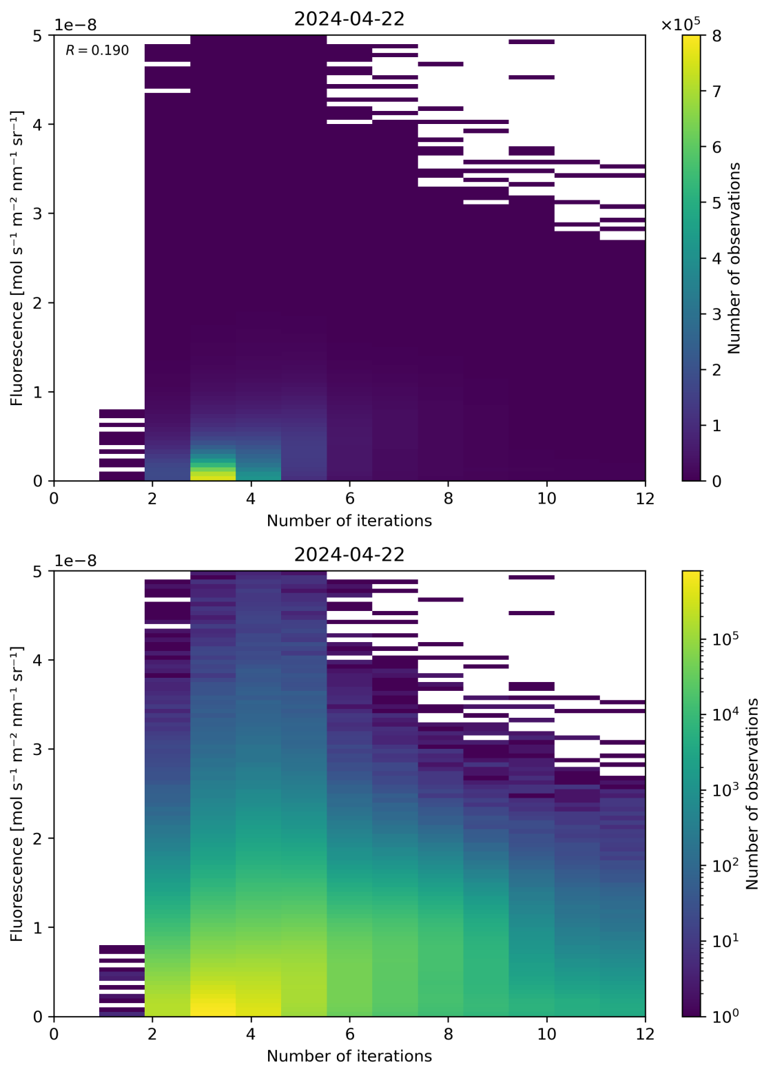
Figure 98: Scatter density plot of “Number of iterations” against “Fluorescence” for 2024-04-21 to 2024-04-23.
