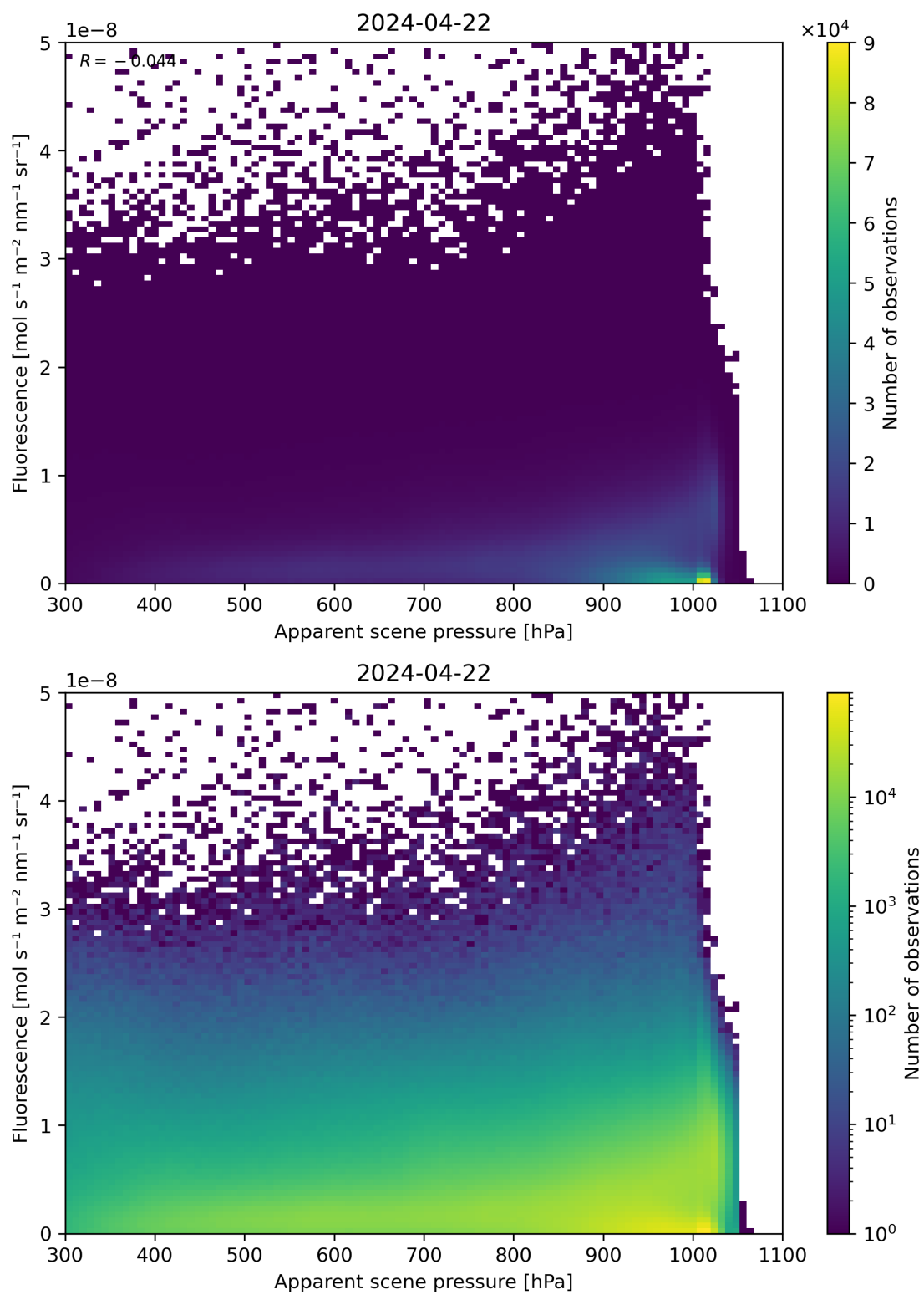
Figure 64: Scatter density plot of “Apparent scene pressure” against “Fluorescence” for 2024-04-21 to 2024-04-23.
