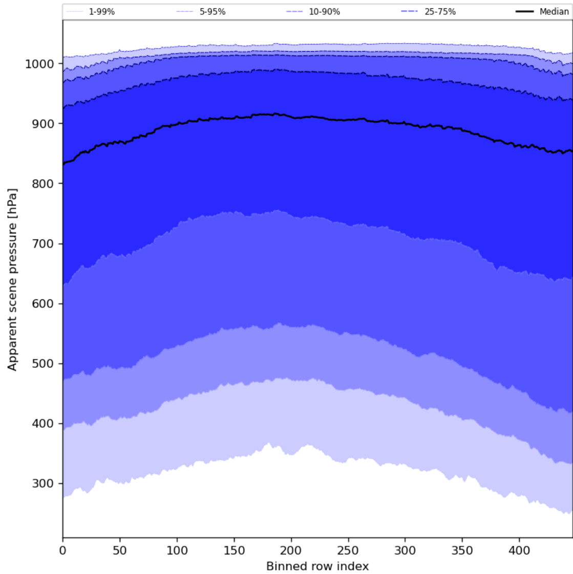
Figure 53: Along track statistics of “Apparent scene pressure” for 2024-04-21 to 2024-04-23
