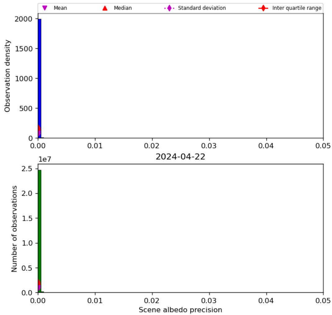
Figure 35: Histogram of “Scene albedo precision” for 2024-04-21 to 2024-04-23
