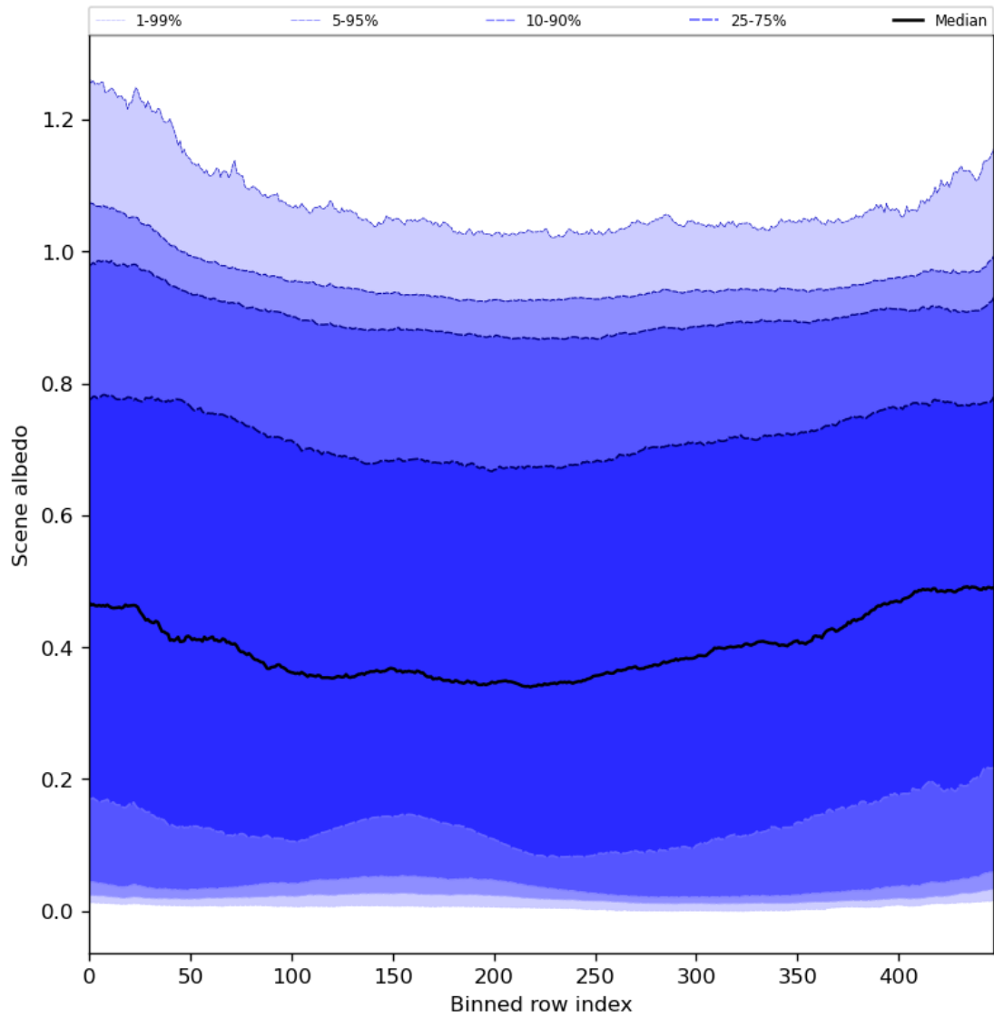
Figure 51: Along track statistics of “Scene albedo” for 2024-04-21 to 2024-04-23
