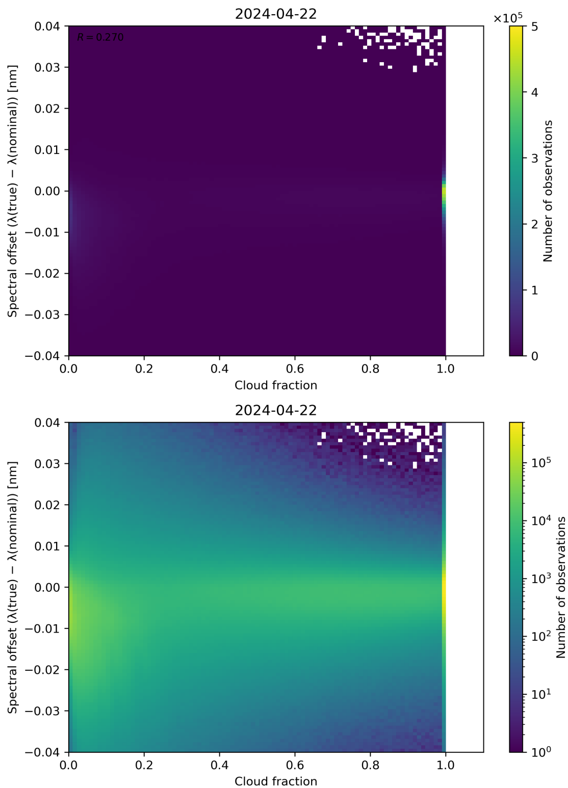
Figure 76: Scatter density plot of “Cloud fraction” against “Spectral offset ( \lambda(\text{true}) - \lambda(\text{nominal}) )” for 2024-04-21 to 2024-04-23.
