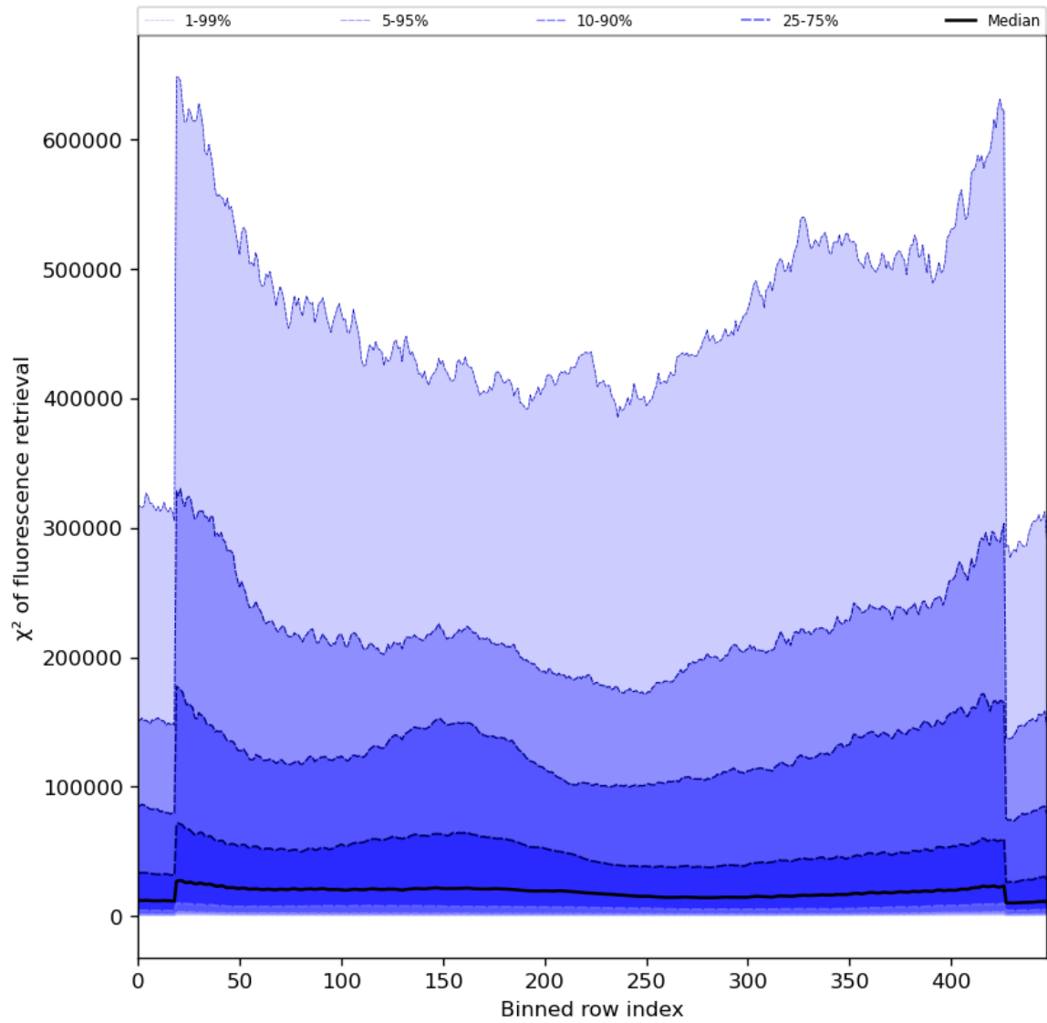
Figure 59: Along track statistics of “ \chi^2 of fluorescence retrieval” for 2024-04-21 to 2024-04-23
