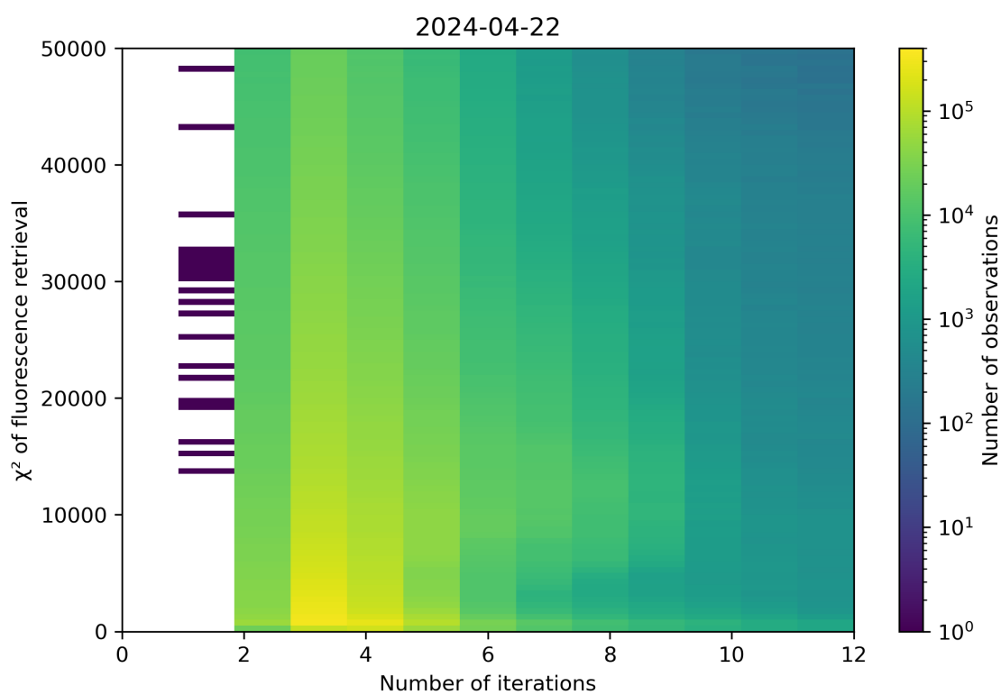
Figure 97: Scatter density plot of “Number of iterations” against “ \chi^2 of fluorescence retrieval” for 2024-04-21 to 2024-04-23.
