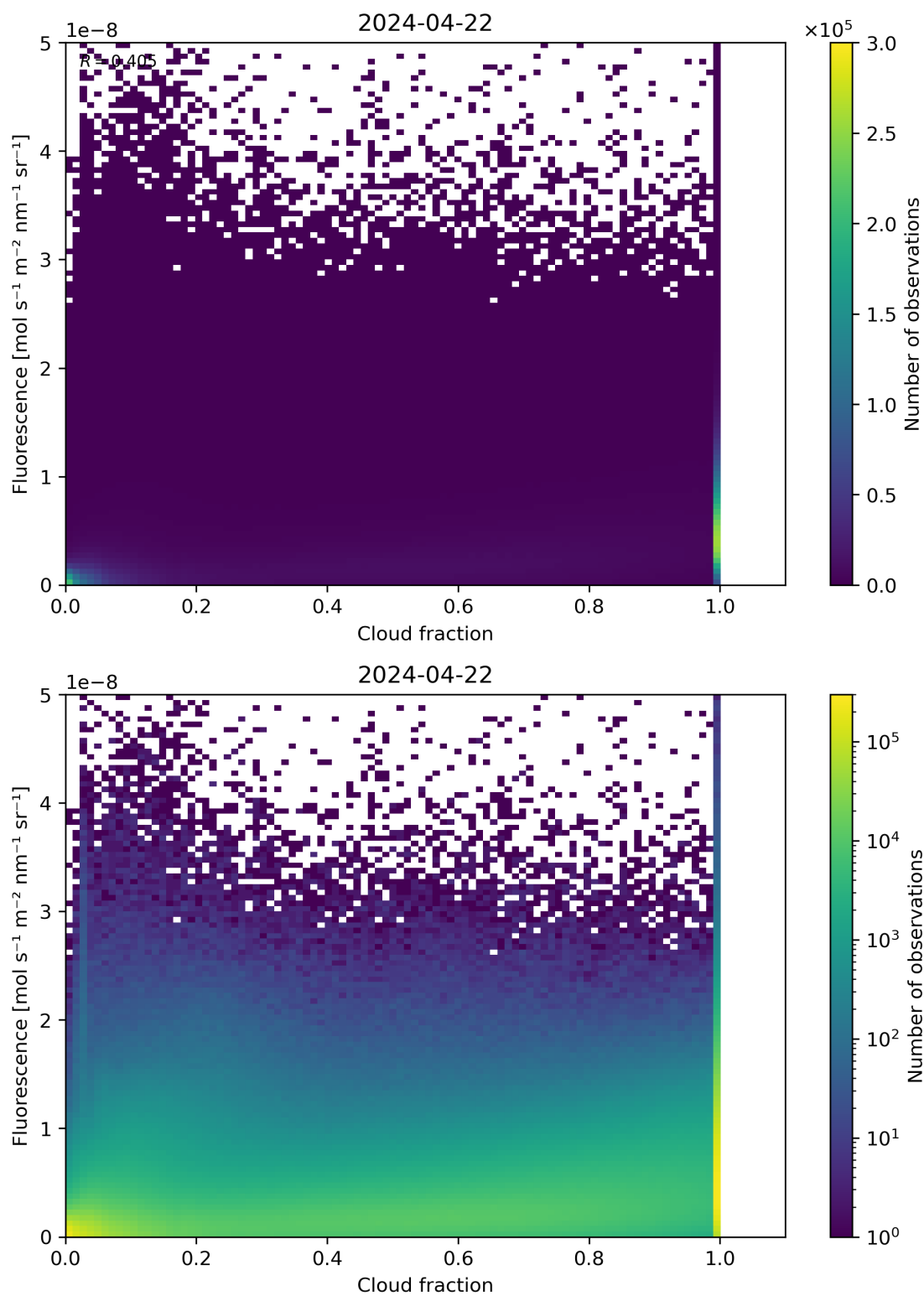
Figure 72: Scatter density plot of “Cloud fraction” against “Fluorescence” for 2024-04-21 to 2024-04-23.
