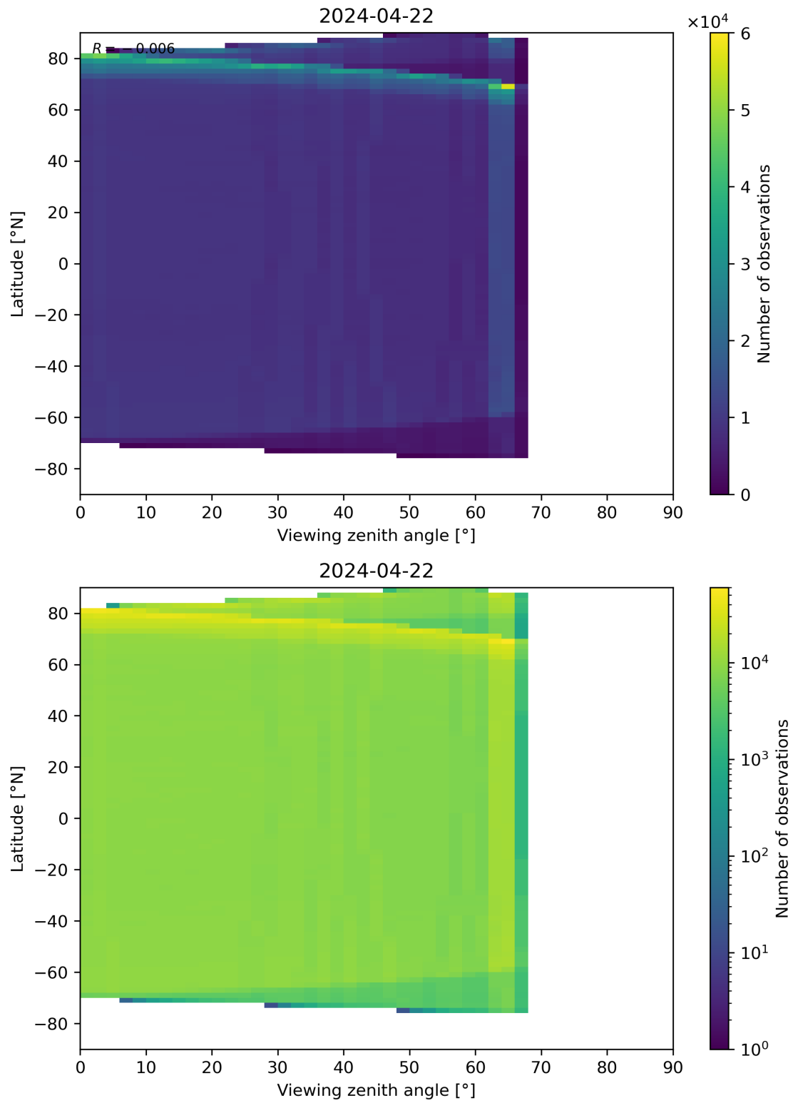
Figure 123: Scatter density plot of “Viewing zenith angle” against “Latitude” for 2024-04-21 to 2024-04-23.
