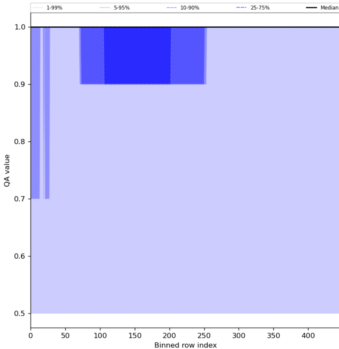
Figure 46: Along track statistics of “QA value” for 2024-04-21 to 2024-04-23
