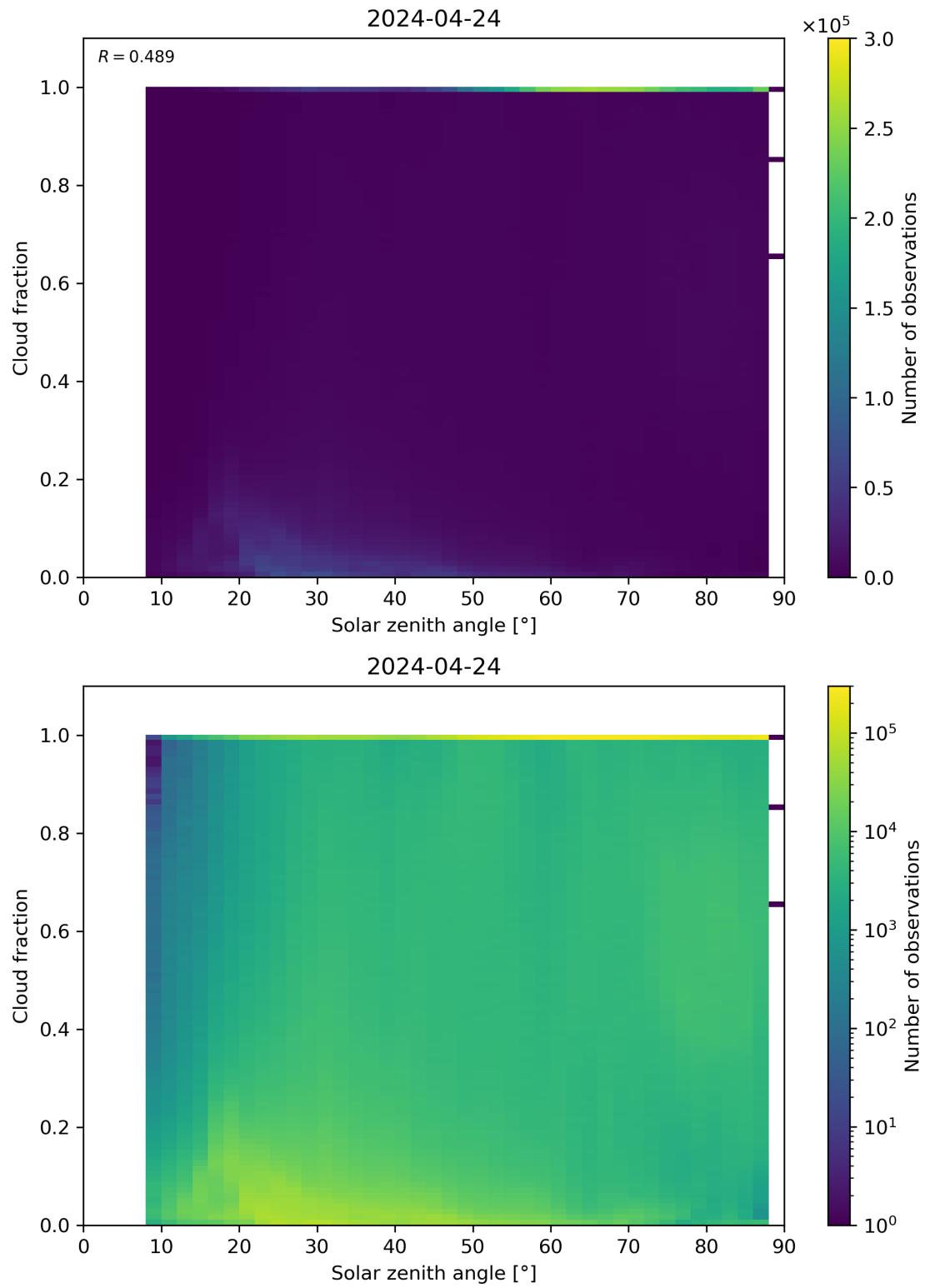
Figure 110: Scatter density plot of “Solar zenith angle” against “Cloud fraction” for 2024-04-23 to 2024-04-25.
