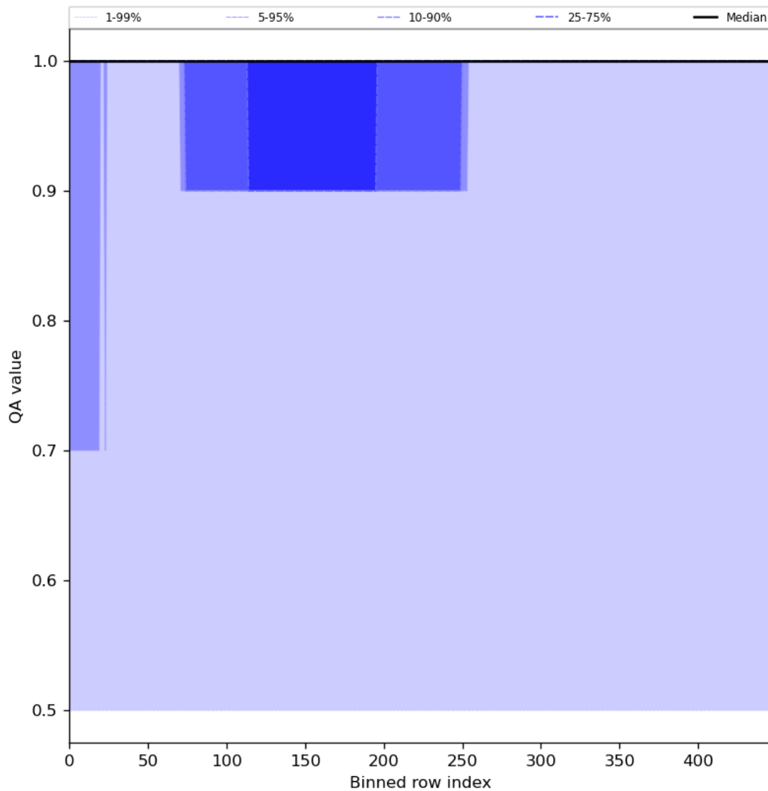
Figure 46: Along track statistics of "QA value" for 2024-04-23 to 2024-04-25
