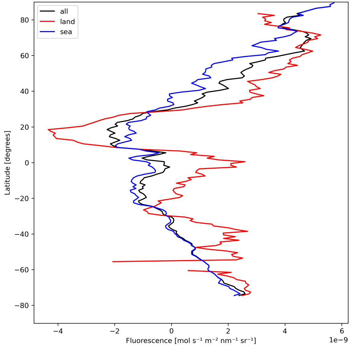
Figure 23: Zonal average of “Fluorescence” for 2024-04-23 to 2024-04-25.
