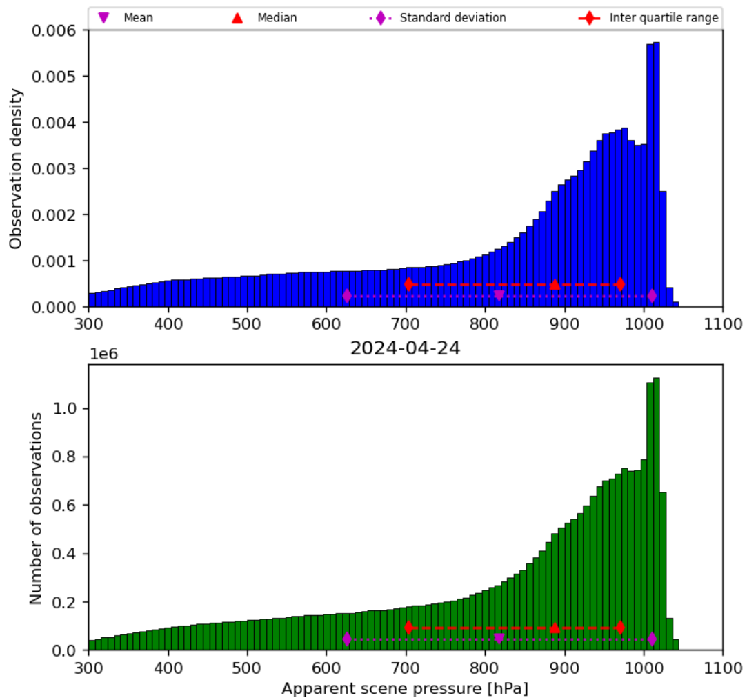
Figure 36: Histogram of “Apparent scene pressure” for 2024-04-23 to 2024-04-25
