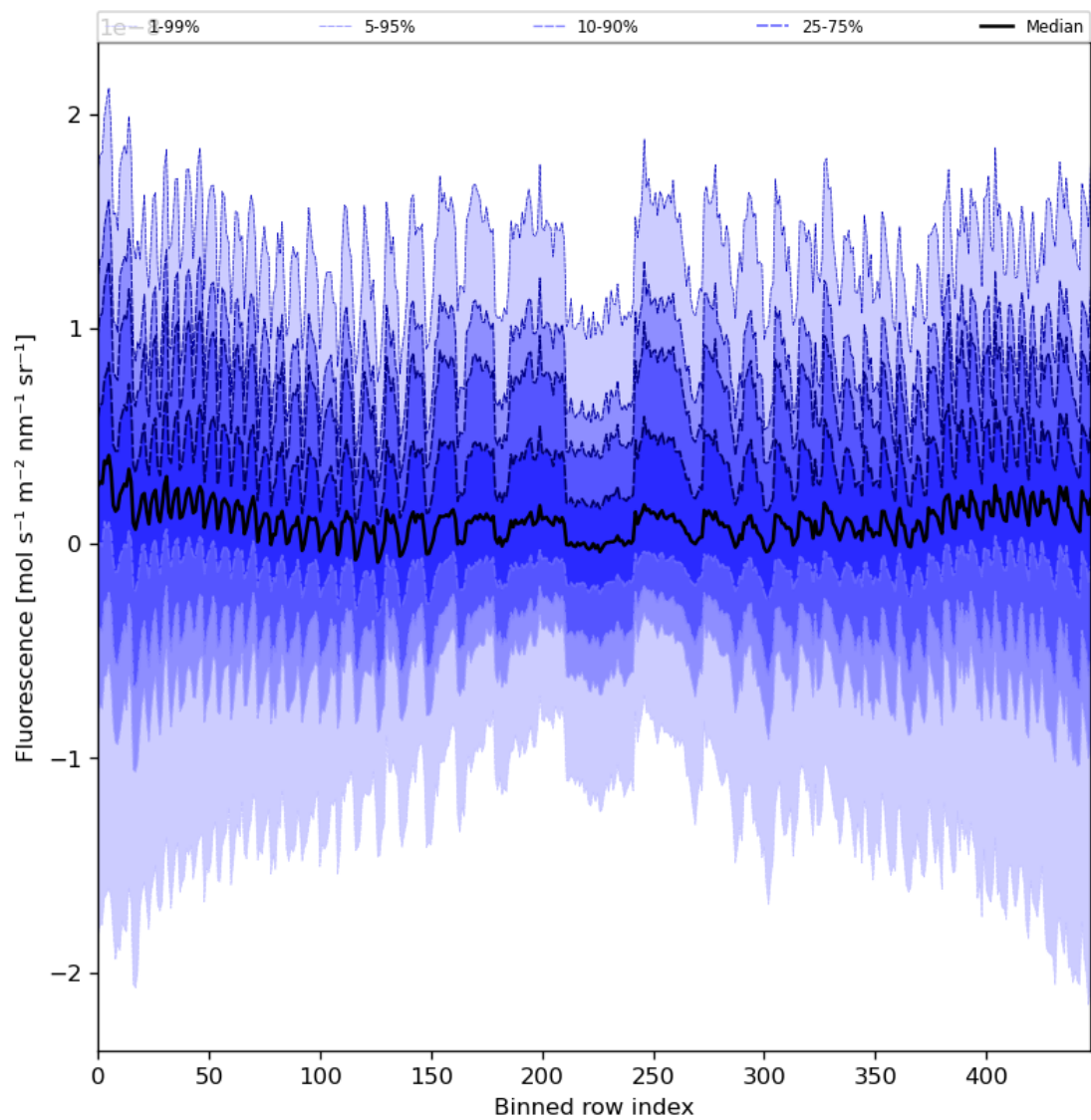
Figure 57: Along track statistics of “Fluorescence” for 2024-04-23 to 2024-04-25
