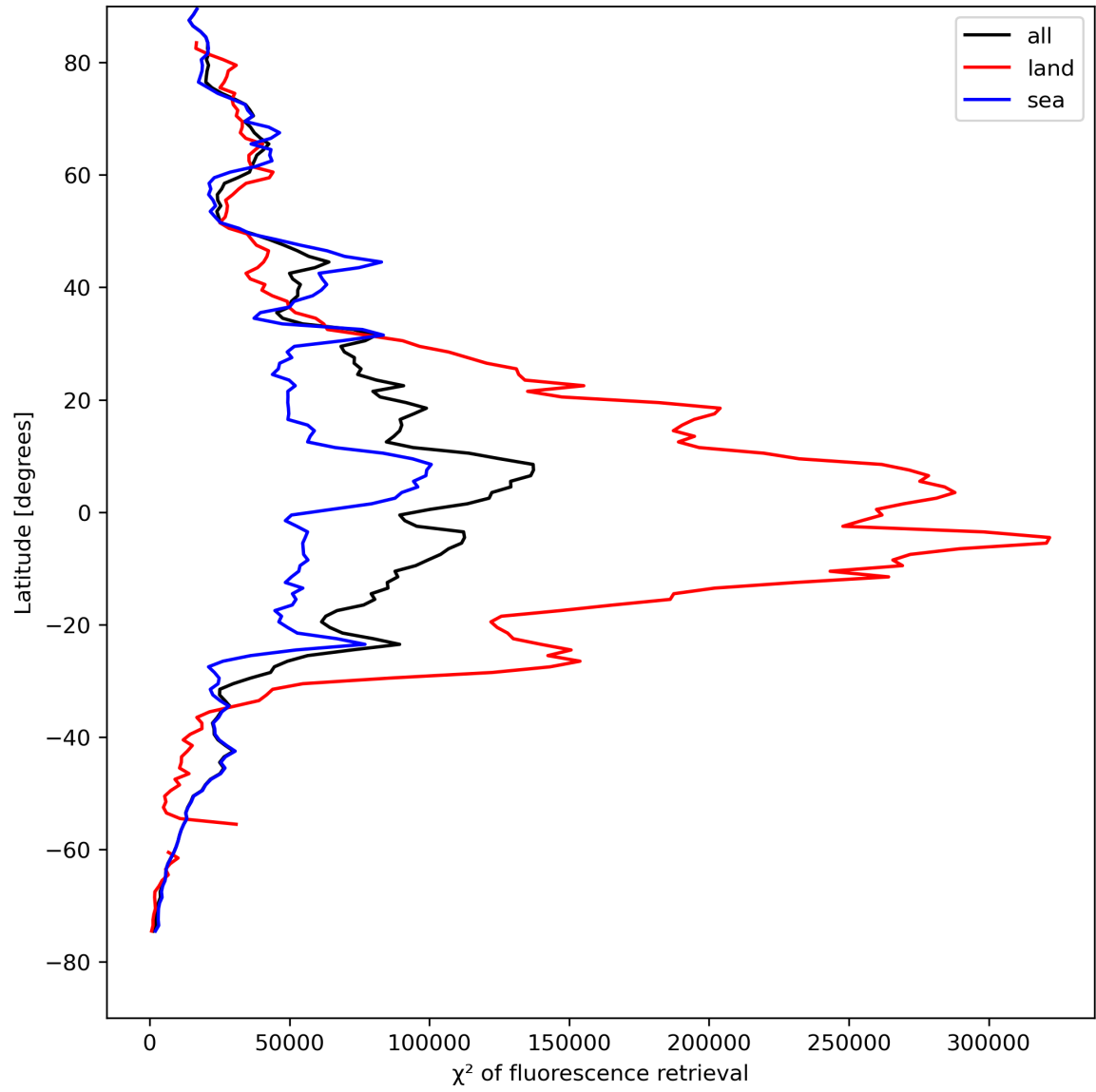
Figure 25: Zonal average of “ \chi^2 of fluorescence retrieval” for 2024-04-23 to 2024-04-25.
