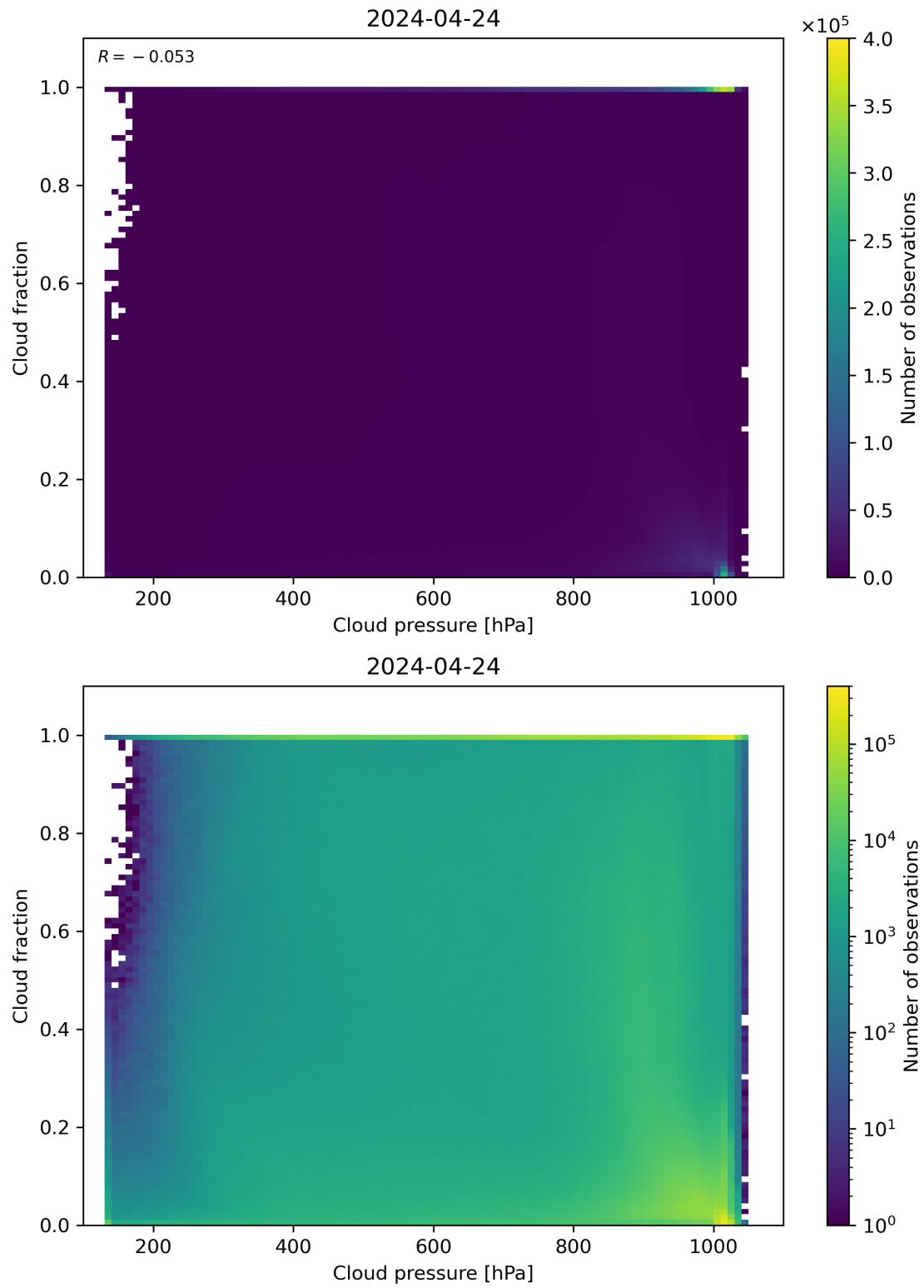
Figure 79: Scatter density plot of “Cloud pressure” against “Cloud fraction” for 2024-04-23 to 2024-04-25.
