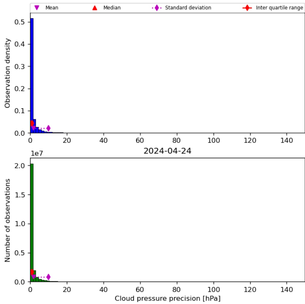
Figure 31: Histogram of “Cloud pressure precision” for 2024-04-23 to 2024-04-25
