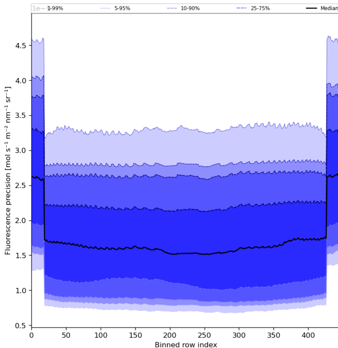
Figure 58: Along track statistics of “Fluorescence precision” for 2024-04-23 to 2024-04-25
