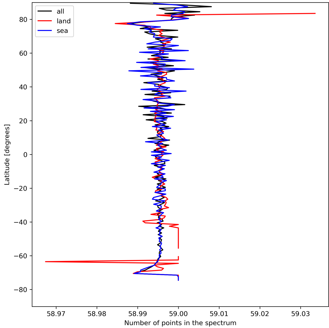
Figure 27: Zonal average of “Number of points in the spectrum” for 2024-04-23 to 2024-04-25.
