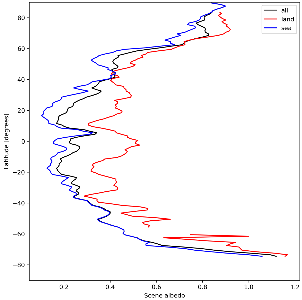
Figure 17: Zonal average of “Scene albedo” for 2024-04-23 to 2024-04-25.
