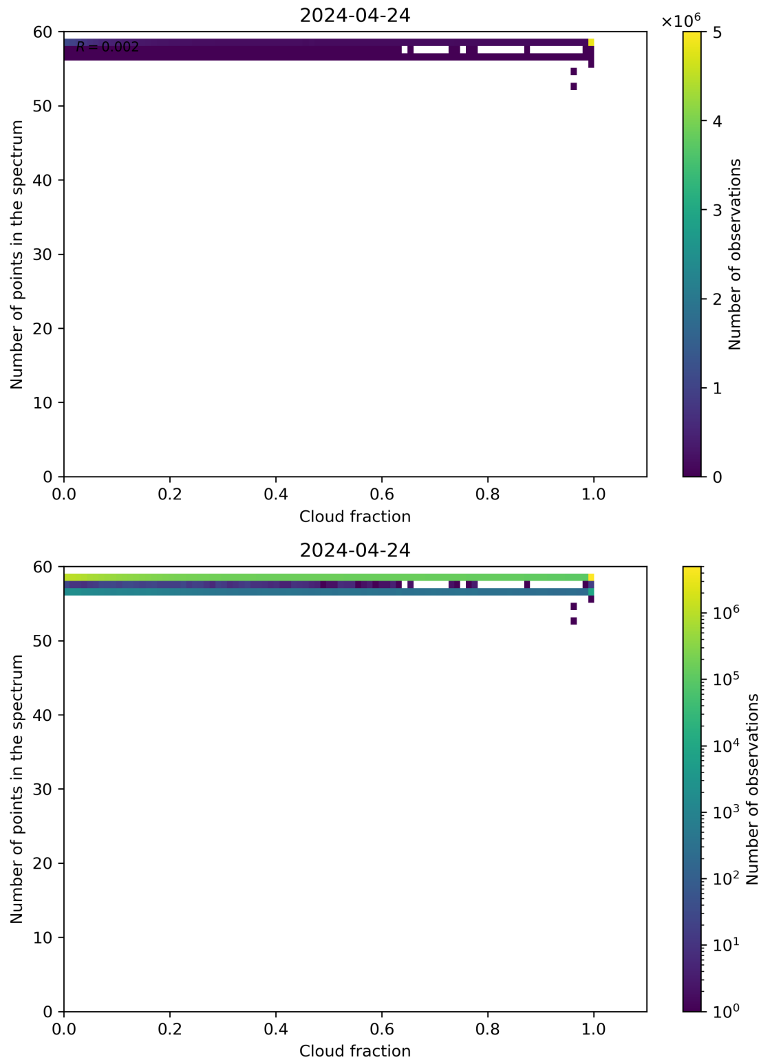
Figure 74: Scatter density plot of “Cloud fraction” against “Number of points in the spectrum” for 2024-04-23 to 2024-04-25.
