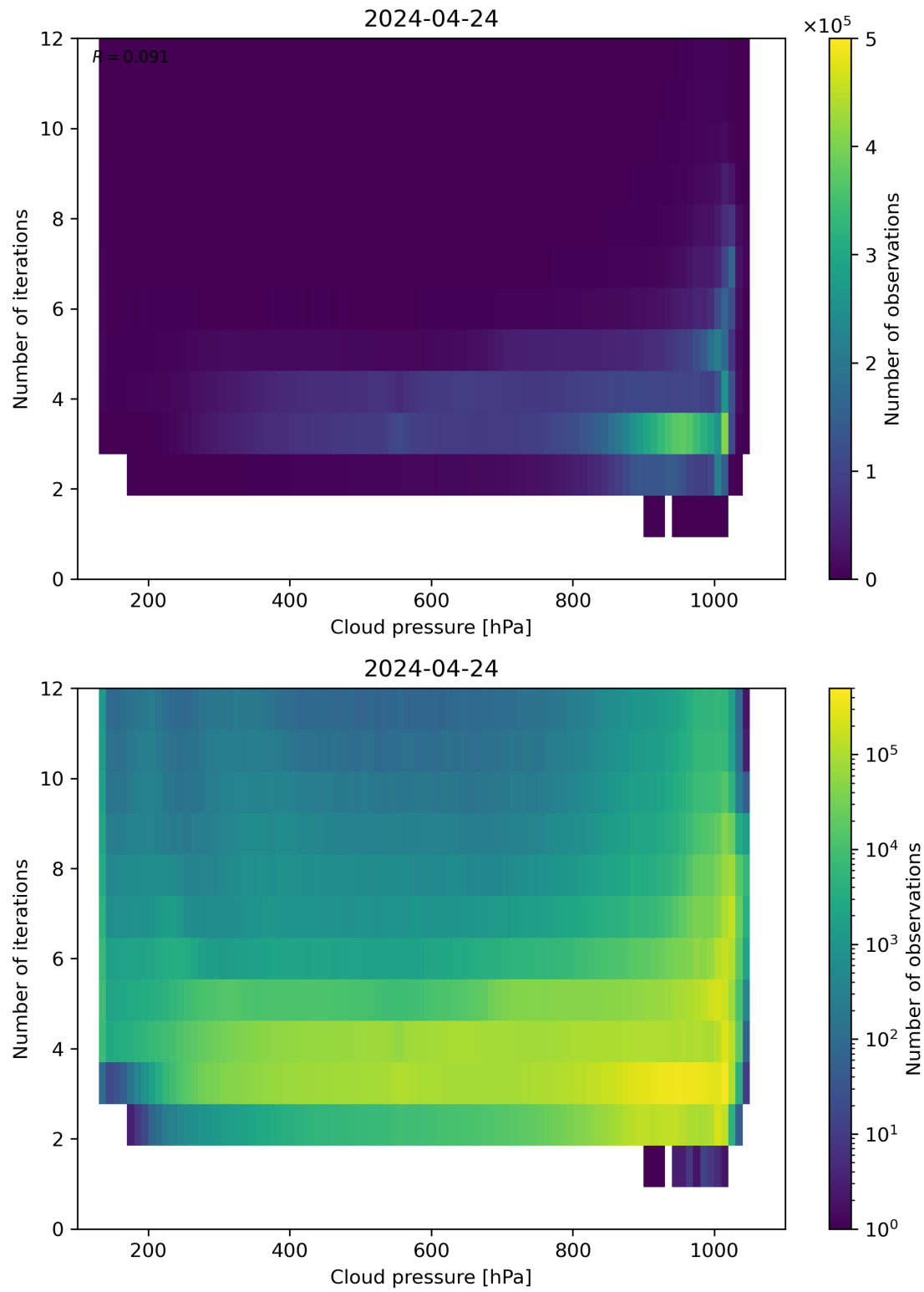
Figure 81: Scatter density plot of “Cloud pressure” against “Number of iterations” for 2024-04-23 to 2024-04-25.
