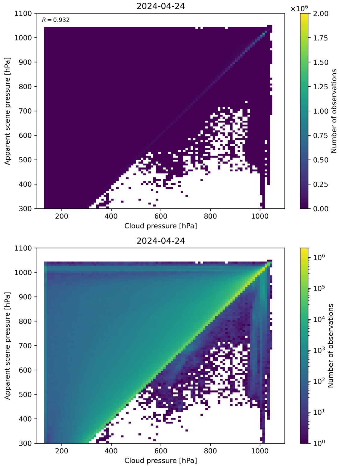
Figure 77: Scatter density plot of “Cloud pressure” against “Apparent scene pressure” for 2024-04-23 to 2024-04-25.
