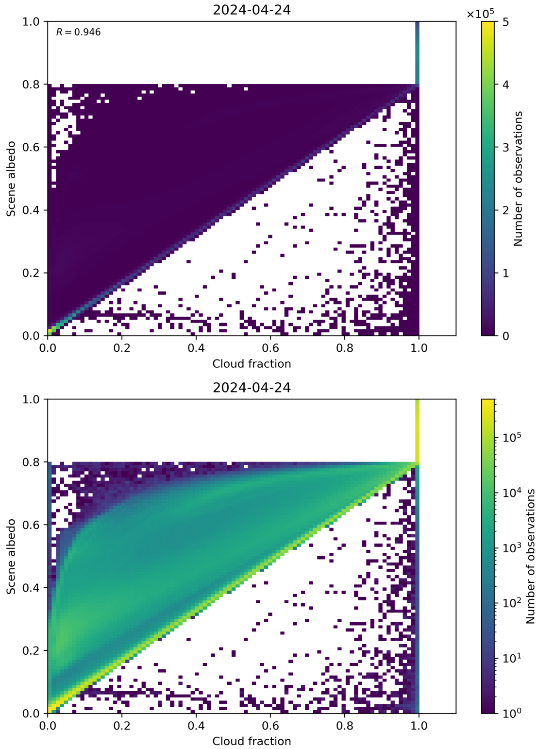
Figure 75: Scatter density plot of “Cloud fraction” against “Scene albedo” for 2024-04-23 to 2024-04-25.
