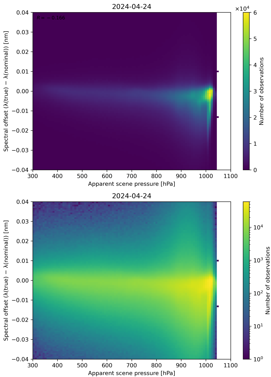
Figure 67: Scatter density plot of “Apparent scene pressure” against “Spectral offset ( \lambda(\text{true}) - \lambda(\text{nominal}) )” for 2024-04-23 to 2024-04-25.
