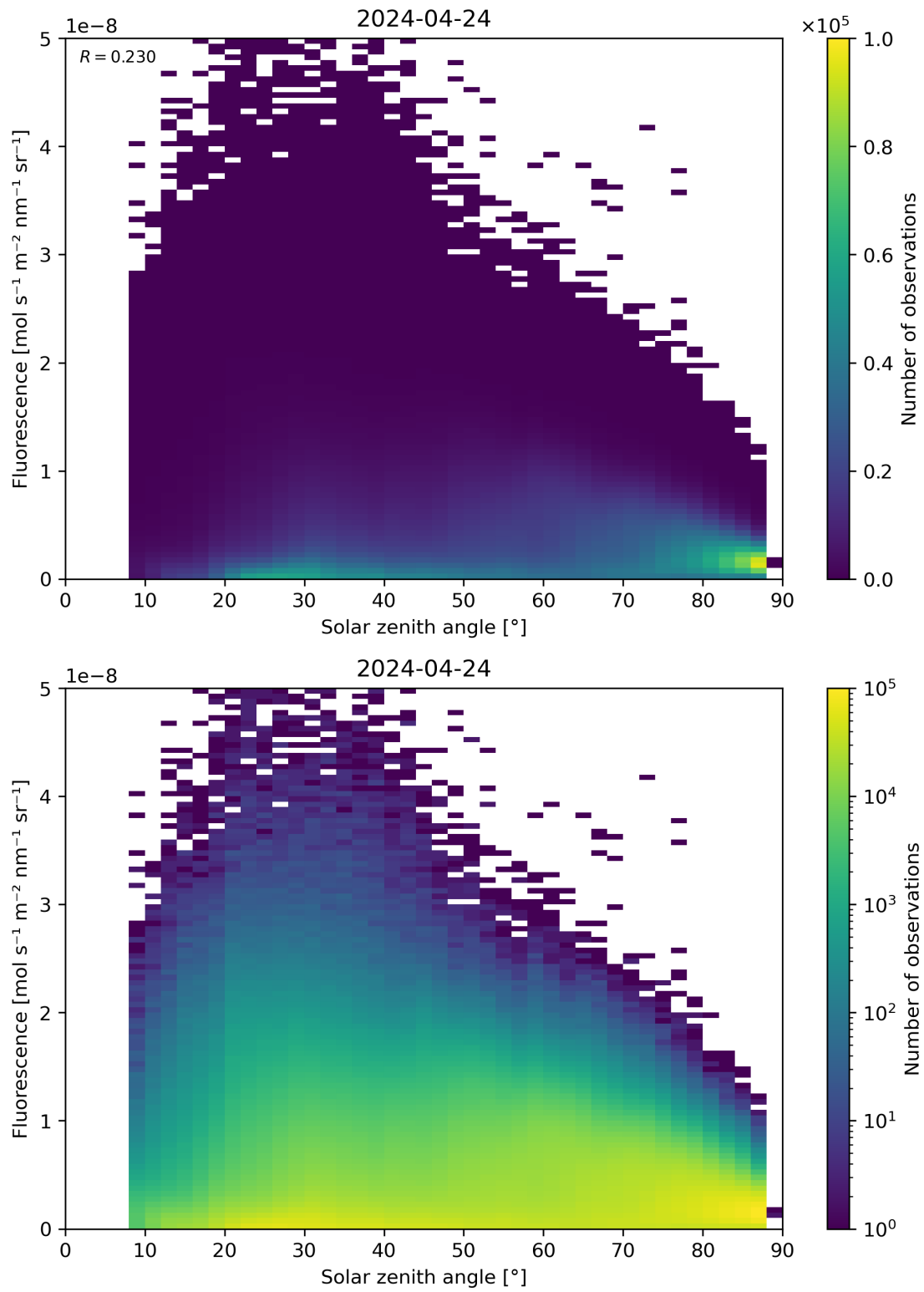
Figure 112: Scatter density plot of “Solar zenith angle” against “Fluorescence” for 2024-04-23 to 2024-04-25.
