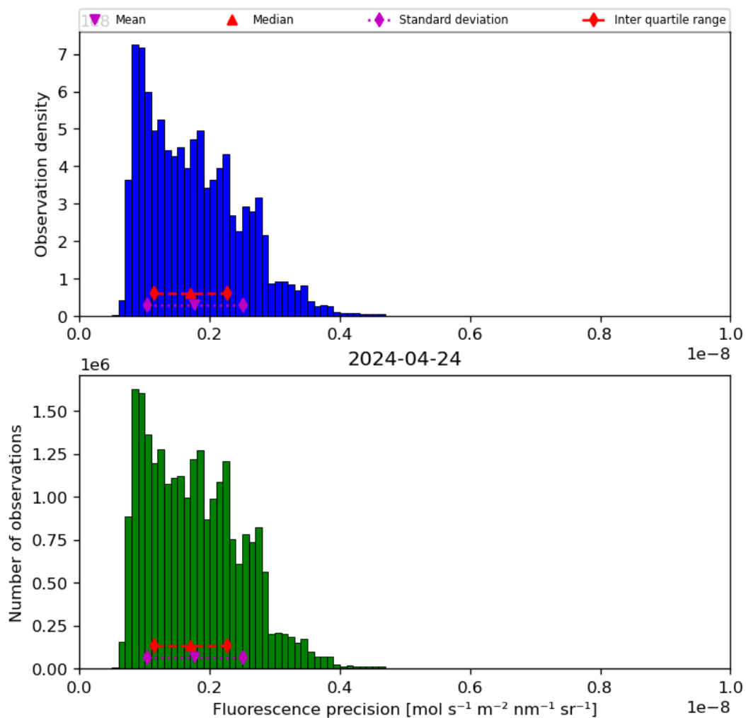
Figure 41: Histogram of “Fluorescence precision” for 2024-04-23 to 2024-04-25
