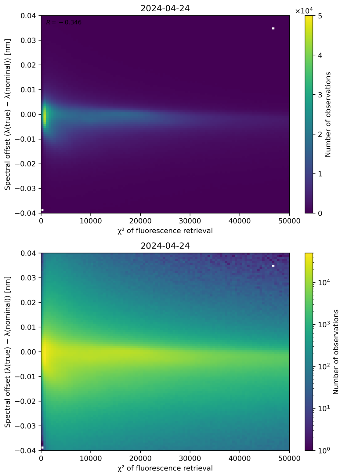
Figure 69: Scatter density plot of “ \chi^2 of fluorescence retrieval” against “Spectral offset ( \lambda(\text{true}) - \lambda(\text{nominal}) )” for 2024-04-23 to 2024-04-25.
