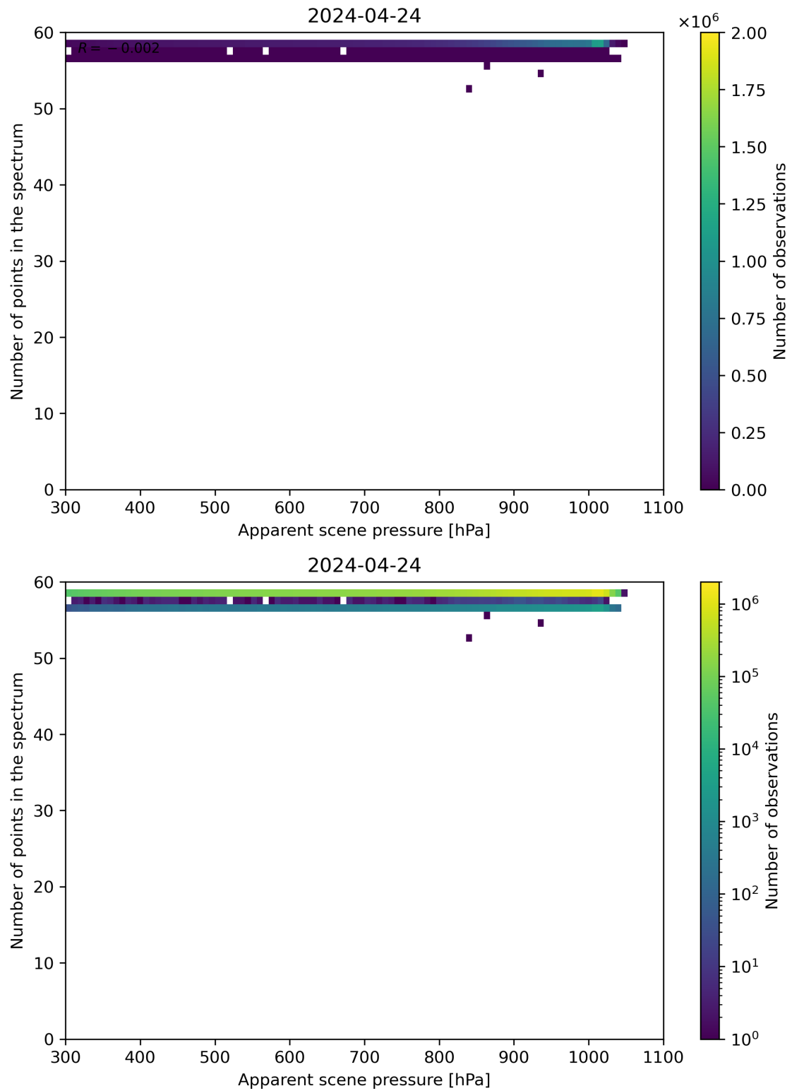
Figure 66: Scatter density plot of “Apparent scene pressure” against “Number of points in the spectrum” for 2024-04-23 to 2024-04-25.
