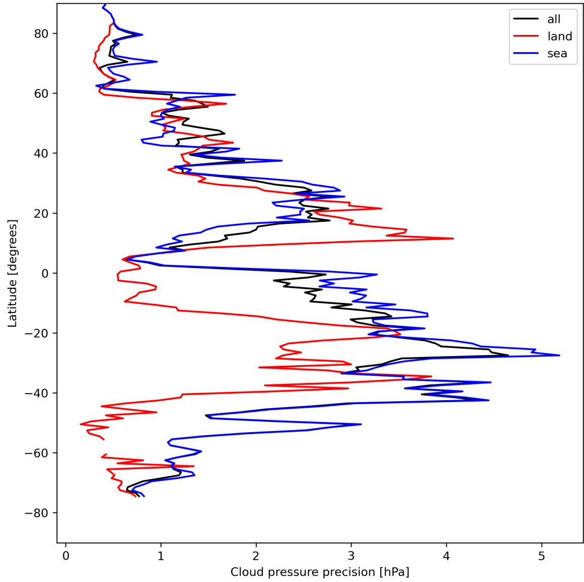
Figure 14: Zonal average of “Cloud pressure precision” for 2024-04-23 to 2024-04-25.
