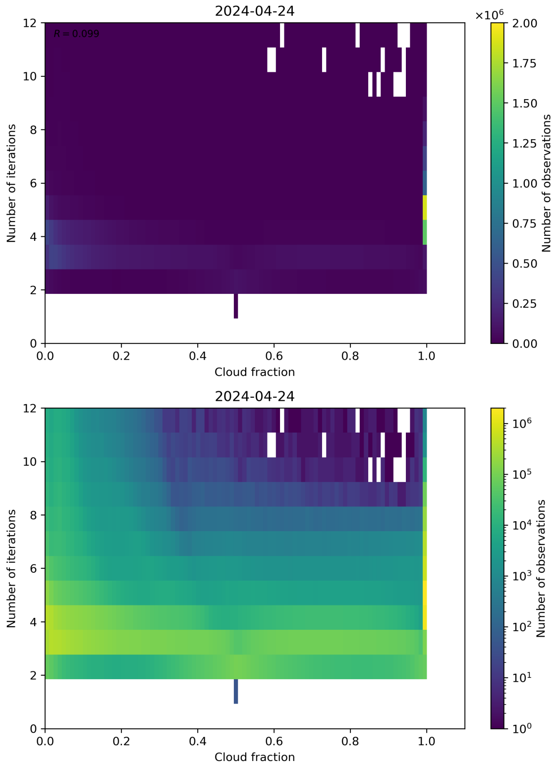
Figure 73: Scatter density plot of “Cloud fraction” against “Number of iterations” for 2024-04-23 to 2024-04-25.
