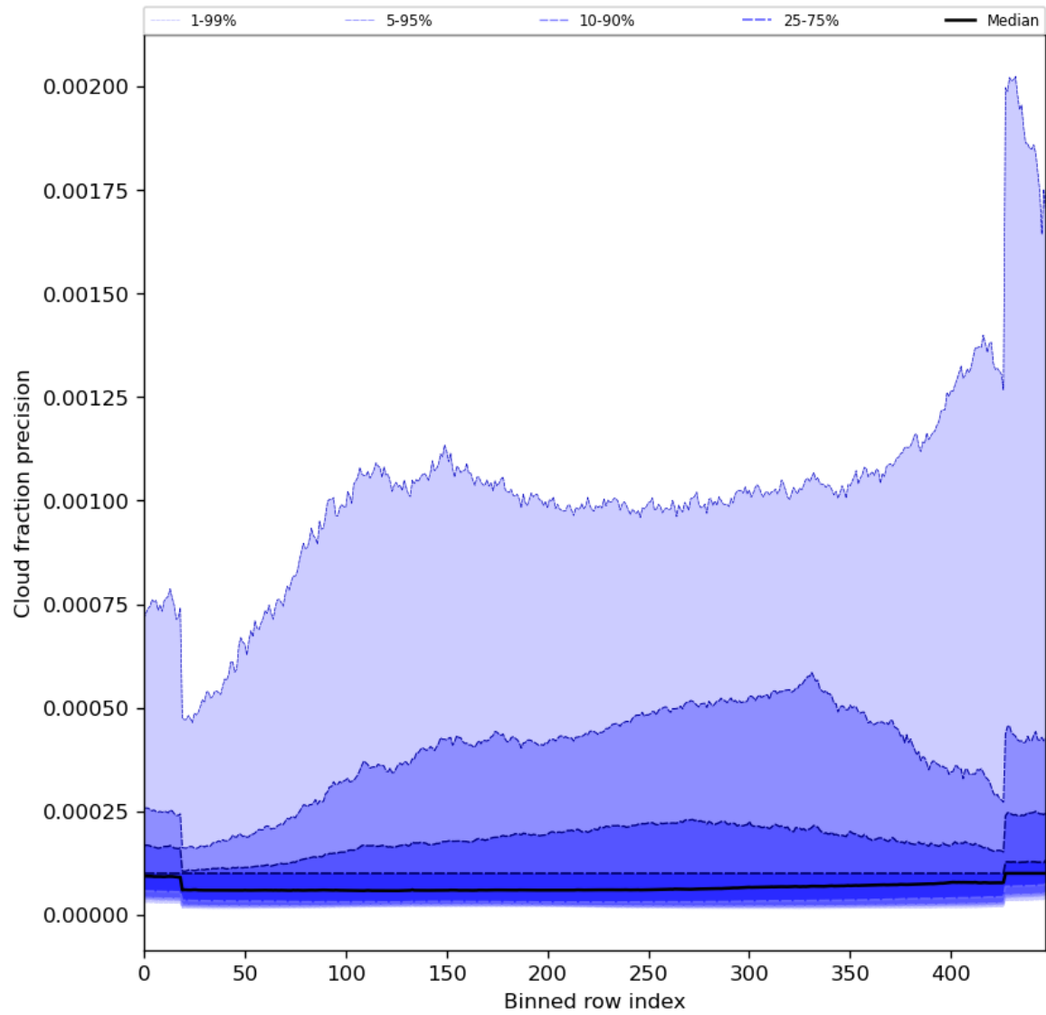
Figure 50: Along track statistics of “Cloud fraction precision” for 2024-04-23 to 2024-04-25
