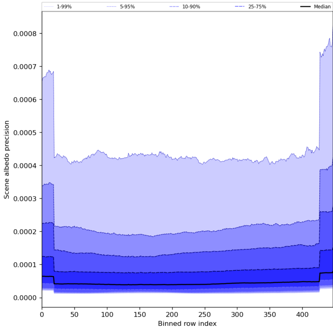
Figure 52: Along track statistics of “Scene albedo precision” for 2024-04-23 to 2024-04-25
