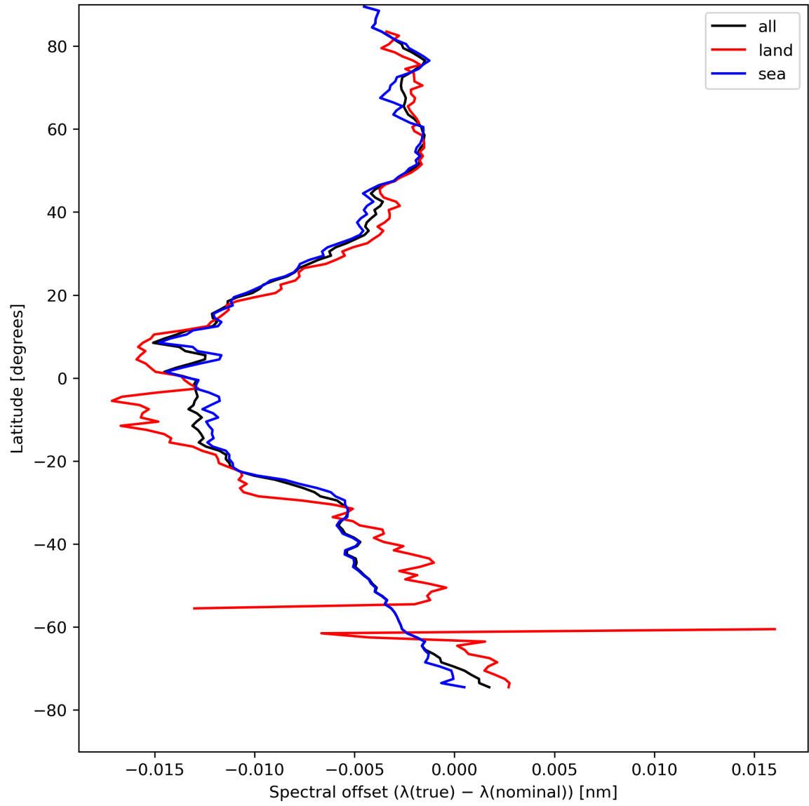
Figure 28: Zonal average of “Spectral offset ( \lambda(\text{true}) - \lambda(\text{nominal}) )” for 2024-04-23 to 2024-04-25.
