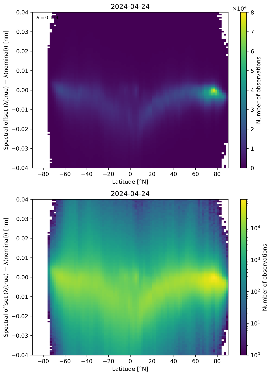
Figure 96: Scatter density plot of “Latitude” against “Spectral offset ( \lambda(\text{true}) - \lambda(\text{nominal}) )” for 2024-04-23 to 2024-04-25.
