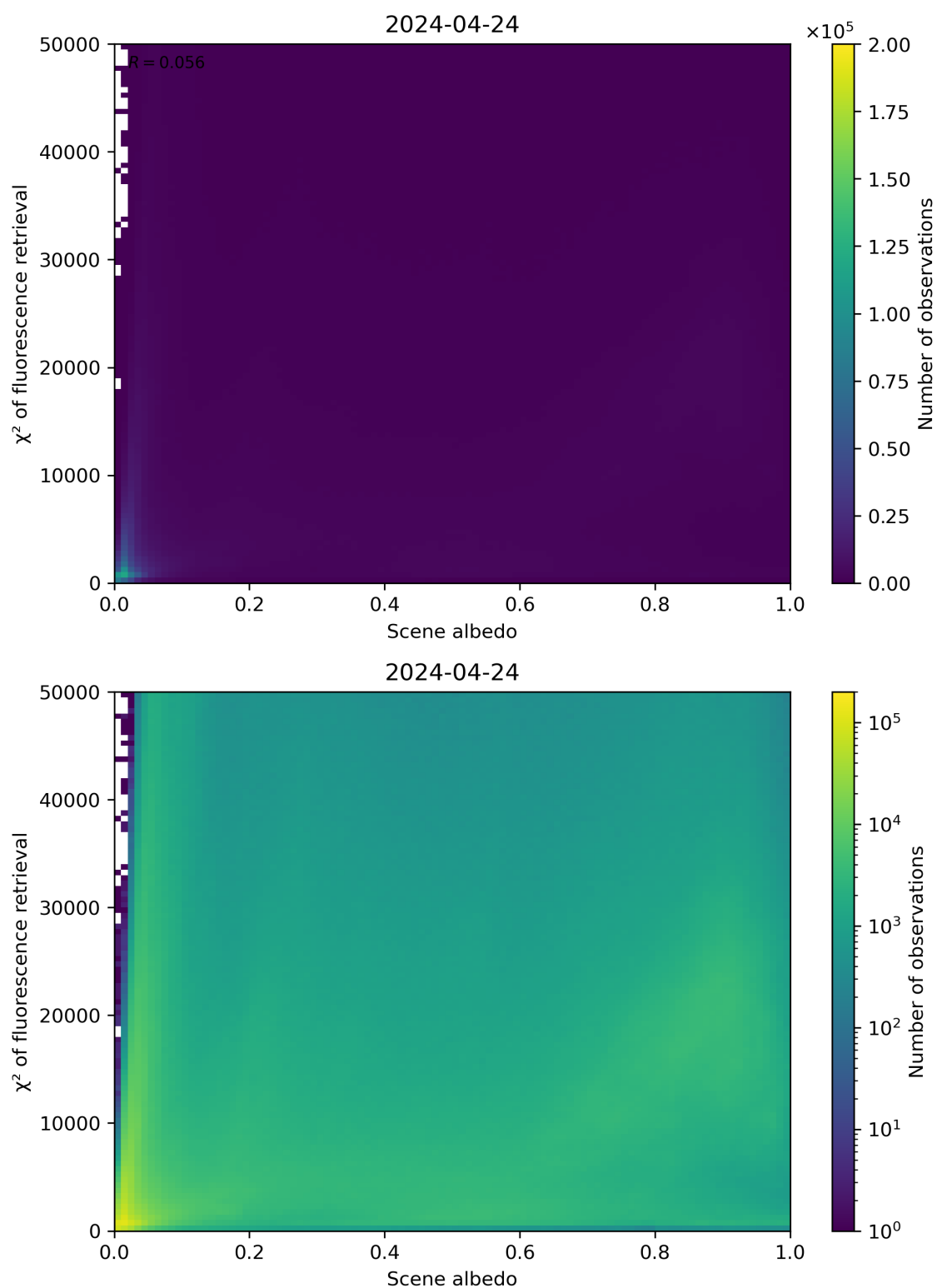
Figure 103: Scatter density plot of “Scene albedo” against “ \chi^2 of fluorescence retrieval” for 2024-04-23 to 2024-04-25.
