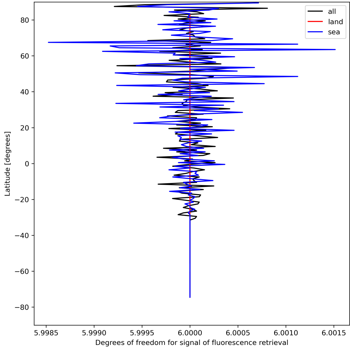
Figure 26: Zonal average of “Degrees of freedom for signal of fluorescence retrieval” for 2024-04-23 to 2024-04-25.
