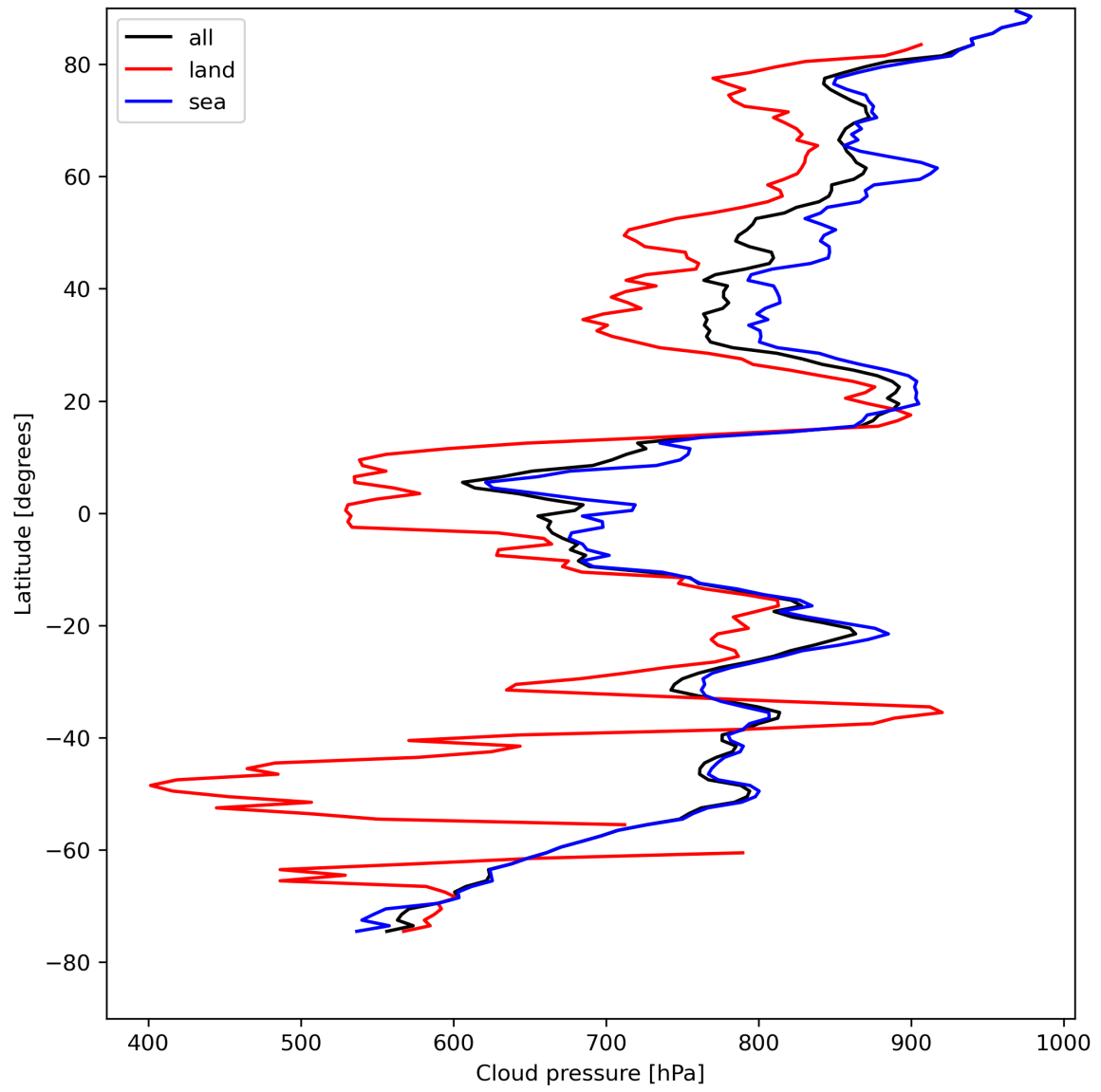
Figure 13: Zonal average of “Cloud pressure” for 2024-04-23 to 2024-04-25.
