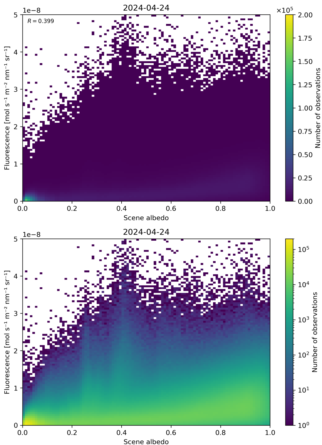
Figure 104: Scatter density plot of “Scene albedo” against “Fluorescence” for 2024-04-23 to 2024-04-25.
