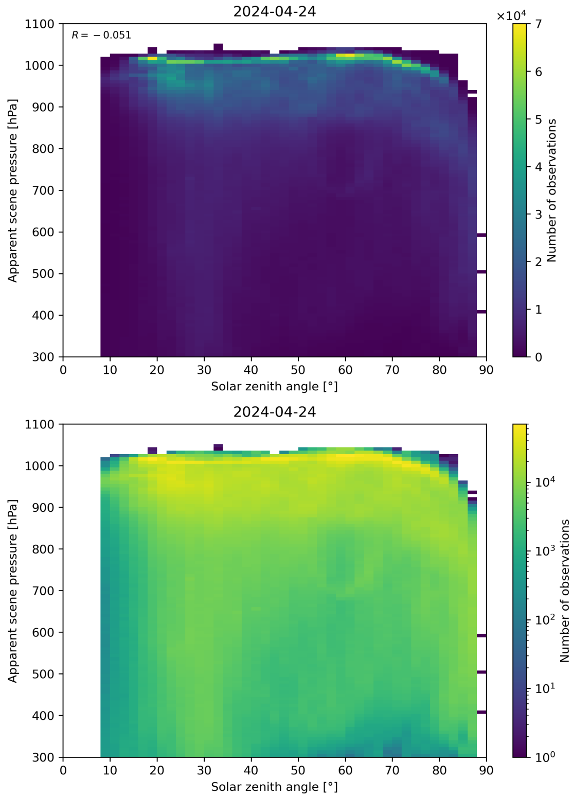
Figure 108: Scatter density plot of “Solar zenith angle” against “Apparent scene pressure” for 2024-04-23 to 2024-04-25.
