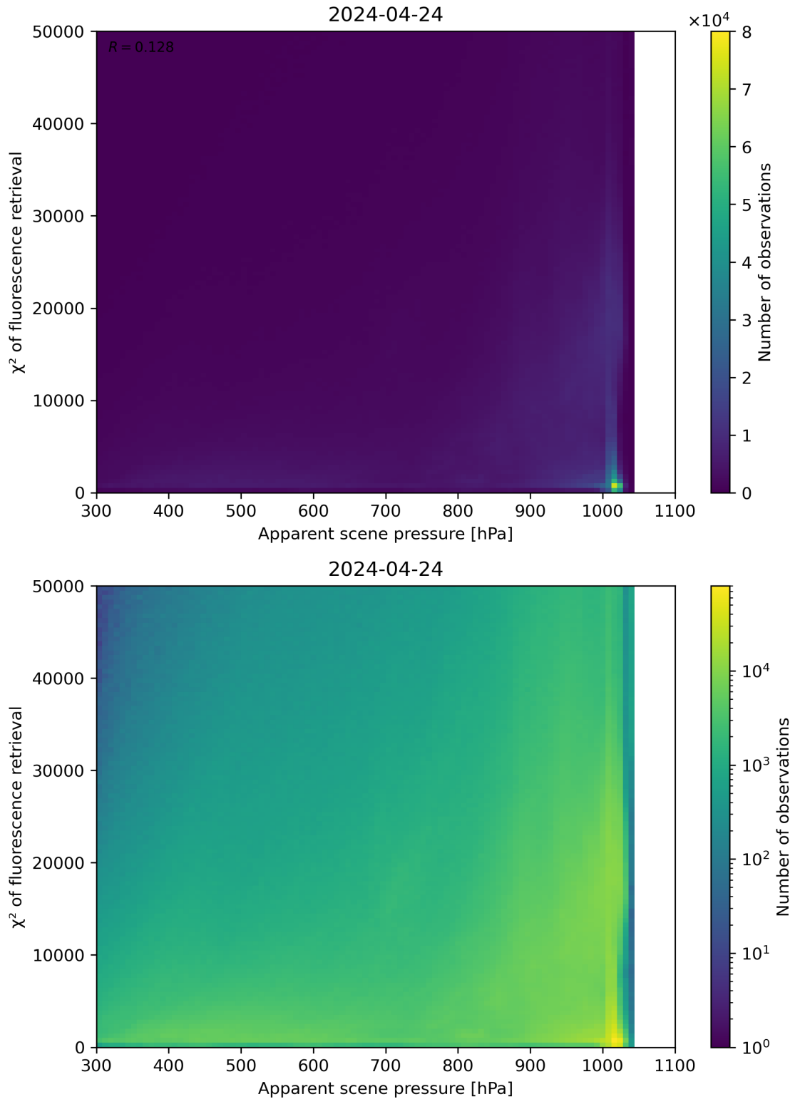
Figure 63: Scatter density plot of “Apparent scene pressure” against “ \chi^2 of fluorescence retrieval” for 2024-04-23 to 2024-04-25.
