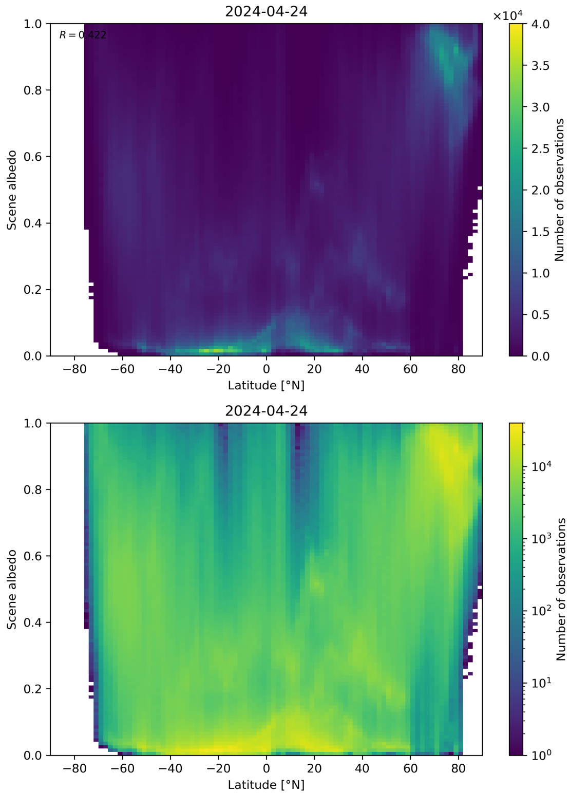
Figure 95: Scatter density plot of “Latitude” against “Scene albedo” for 2024-04-23 to 2024-04-25.
