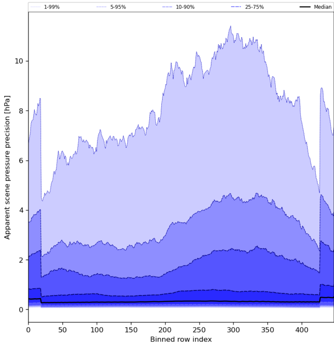
Figure 54: Along track statistics of “Apparent scene pressure precision” for 2024-04-23 to 2024-04-25
