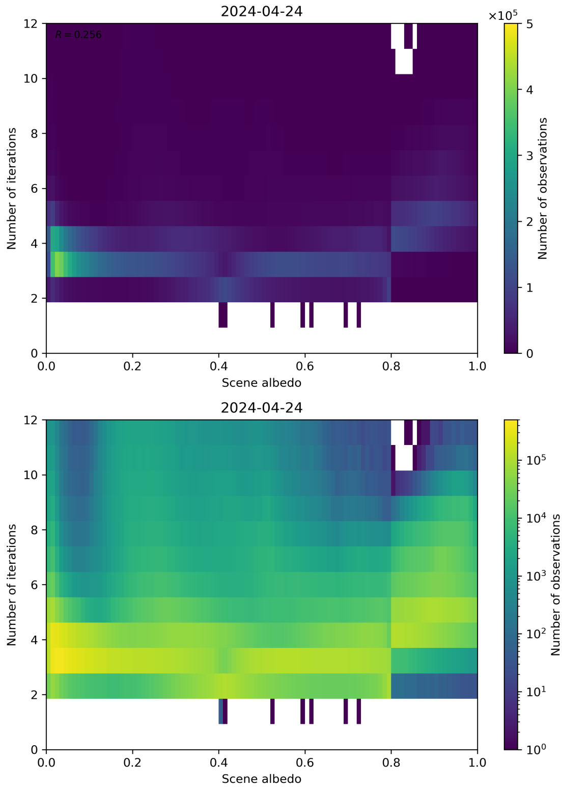
Figure 105: Scatter density plot of “Scene albedo” against “Number of iterations” for 2024-04-23 to 2024-04-25.
