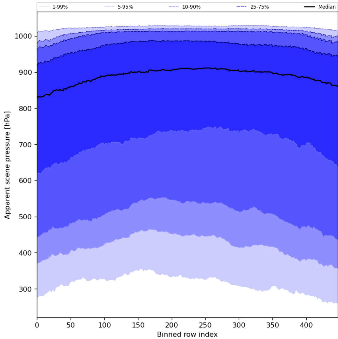
Figure 53: Along track statistics of “Apparent scene pressure” for 2024-04-23 to 2024-04-25
