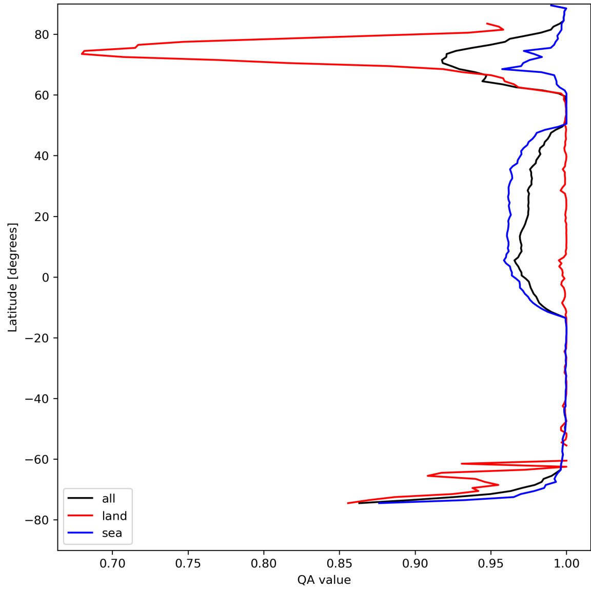
Figure 12: Zonal average of “QA value” for 2024-04-23 to 2024-04-25.
