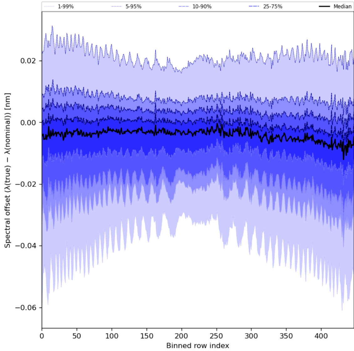
Figure 62: Along track statistics of “Spectral offset ( \lambda(\text{true}) - \lambda(\text{nominal}) )” for 2024-04-23 to 2024-04-25
