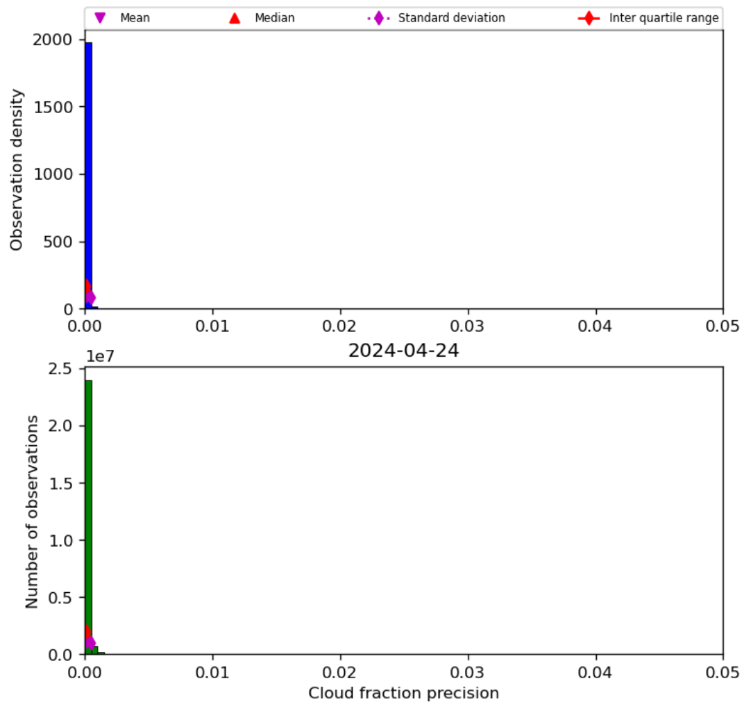
Figure 33: Histogram of “Cloud fraction precision” for 2024-04-23 to 2024-04-25
