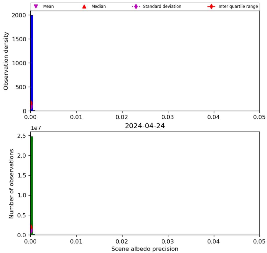
Figure 35: Histogram of “Scene albedo precision” for 2024-04-23 to 2024-04-25
