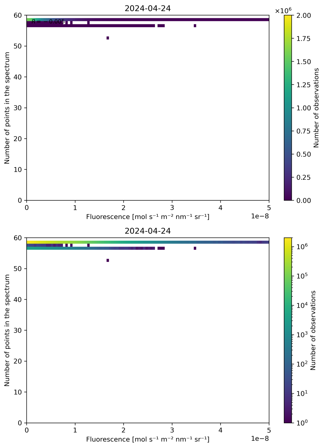
Figure 86: Scatter density plot of “Fluorescence” against “Number of points in the spectrum” for 2024-04-23 to 2024-04-25.
