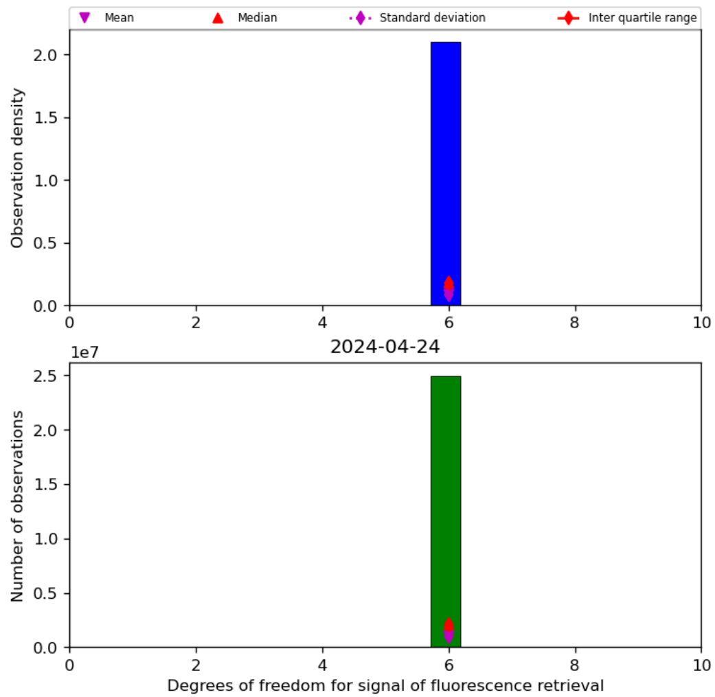
Figure 43: Histogram of "Degrees of freedom for signal of fluorescence retrieval" for 2024-04-23 to 2024-04-25
