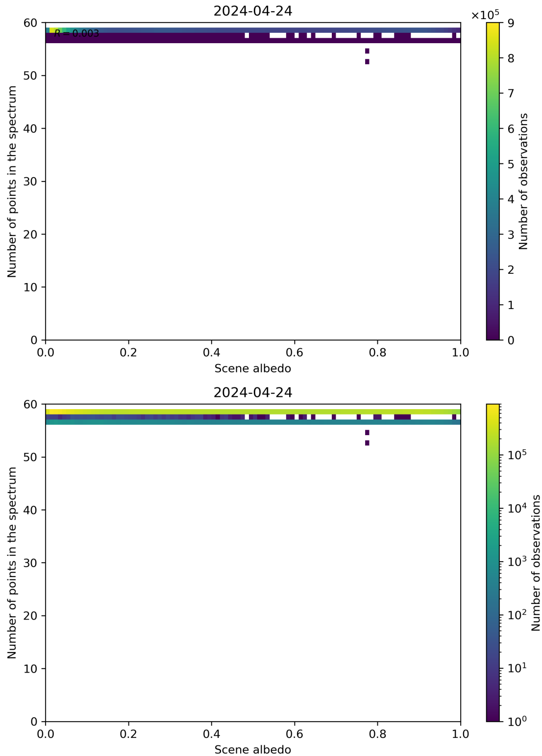
Figure 106: Scatter density plot of “Scene albedo” against “Number of points in the spectrum” for 2024-04-23 to 2024-04-25.
