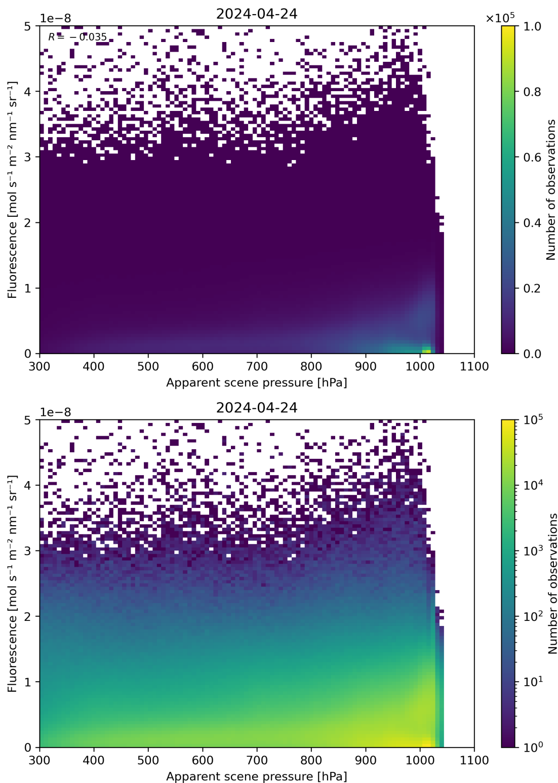
Figure 64: Scatter density plot of “Apparent scene pressure” against “Fluorescence” for 2024-04-23 to 2024-04-25.
