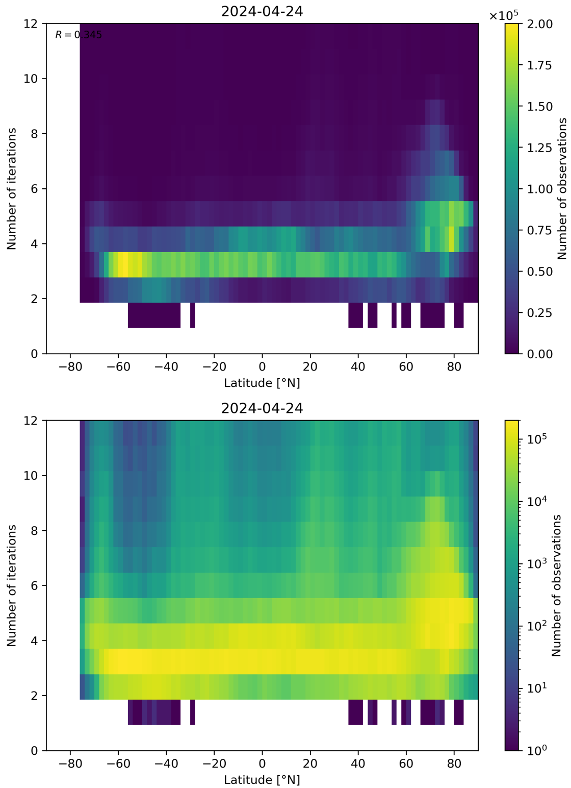
Figure 93: Scatter density plot of “Latitude” against “Number of iterations” for 2024-04-23 to 2024-04-25.
