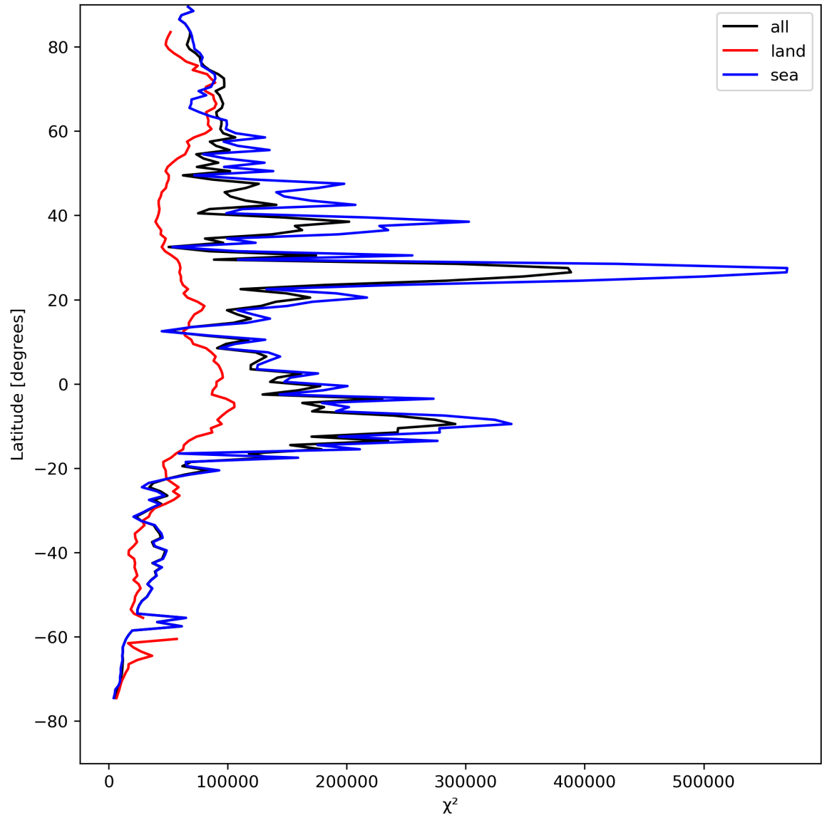
Figure 21: Zonal average of “ \chi^2 ” for 2024-04-23 to 2024-04-25.
