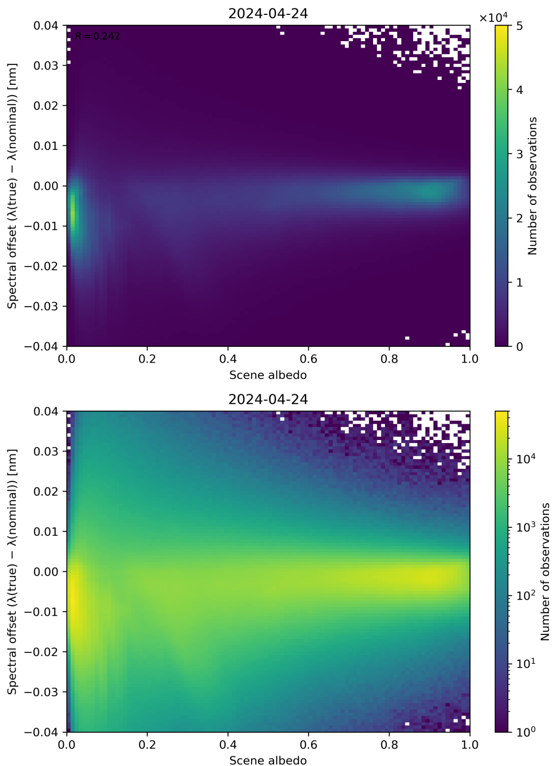
Figure 107: Scatter density plot of “Scene albedo” against “Spectral offset ( \lambda(\text{true}) - \lambda(\text{nominal}) )” for 2024-04-23 to 2024-04-25.
