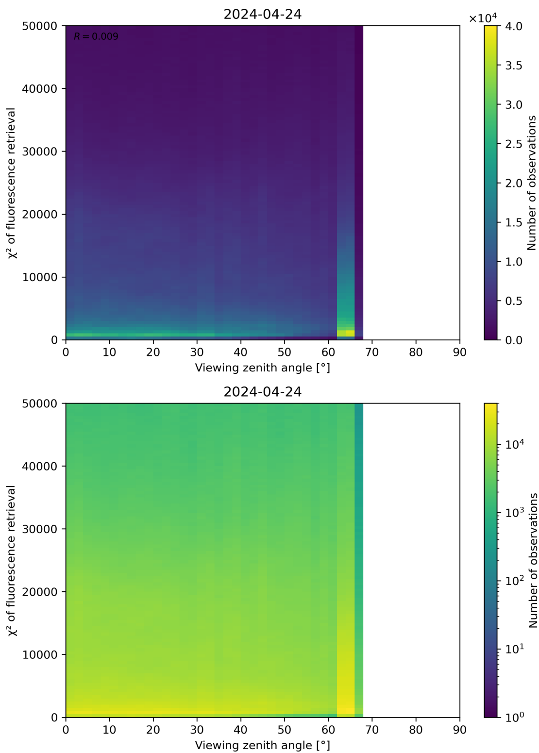
Figure 119: Scatter density plot of “Viewing zenith angle” against “ \chi^2 of fluorescence retrieval” for 2024-04-23 to 2024-04-25.
