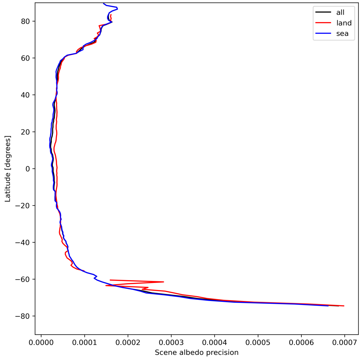
Figure 18: Zonal average of “Scene albedo precision” for 2024-04-23 to 2024-04-25.
