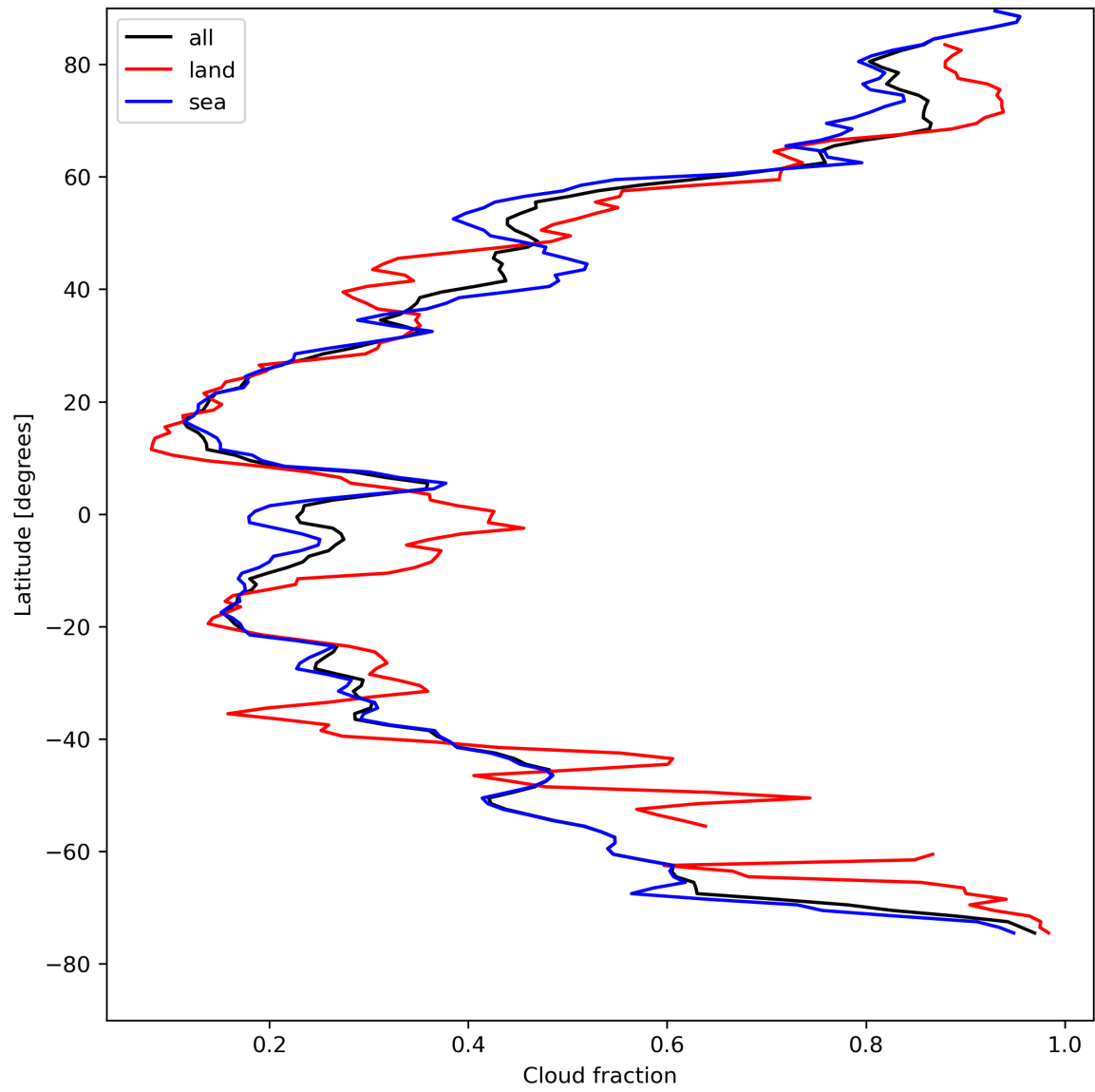
Figure 15: Zonal average of “Cloud fraction” for 2024-04-23 to 2024-04-25.
