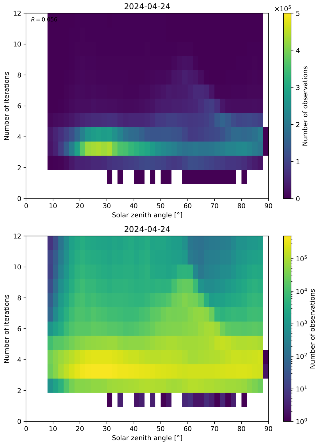
Figure 114: Scatter density plot of “Solar zenith angle” against “Number of iterations” for 2024-04-23 to 2024-04-25.
