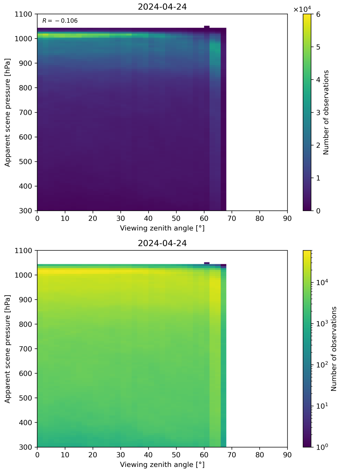
Figure 118: Scatter density plot of “Viewing zenith angle” against “Apparent scene pressure” for 2024-04-23 to 2024-04-25.
