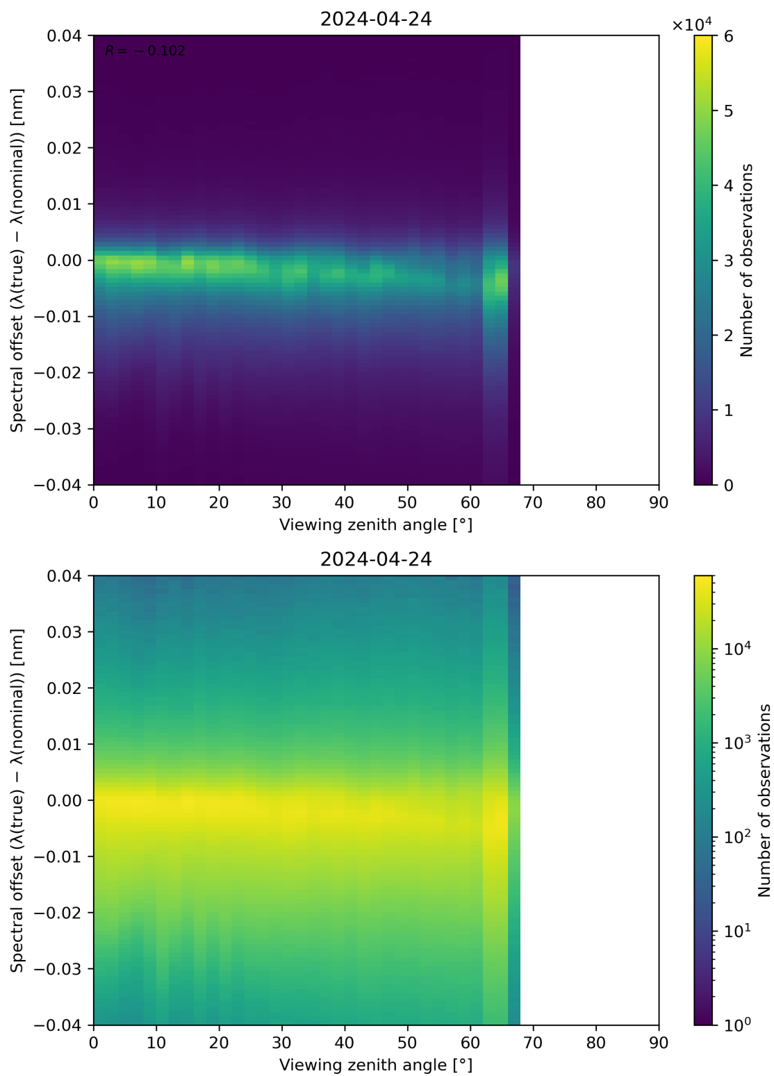
Figure 128: Scatter density plot of “Viewing zenith angle” against “Spectral offset ( \lambda(\text{true}) - \lambda(\text{nominal}) )” for 2024-04-23 to 2024-04-25.
