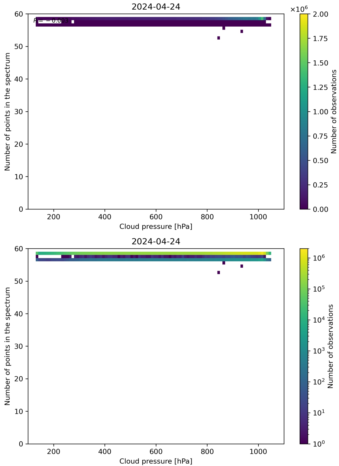
Figure 82: Scatter density plot of “Cloud pressure” against “Number of points in the spectrum” for 2024-04-23 to 2024-04-25.
