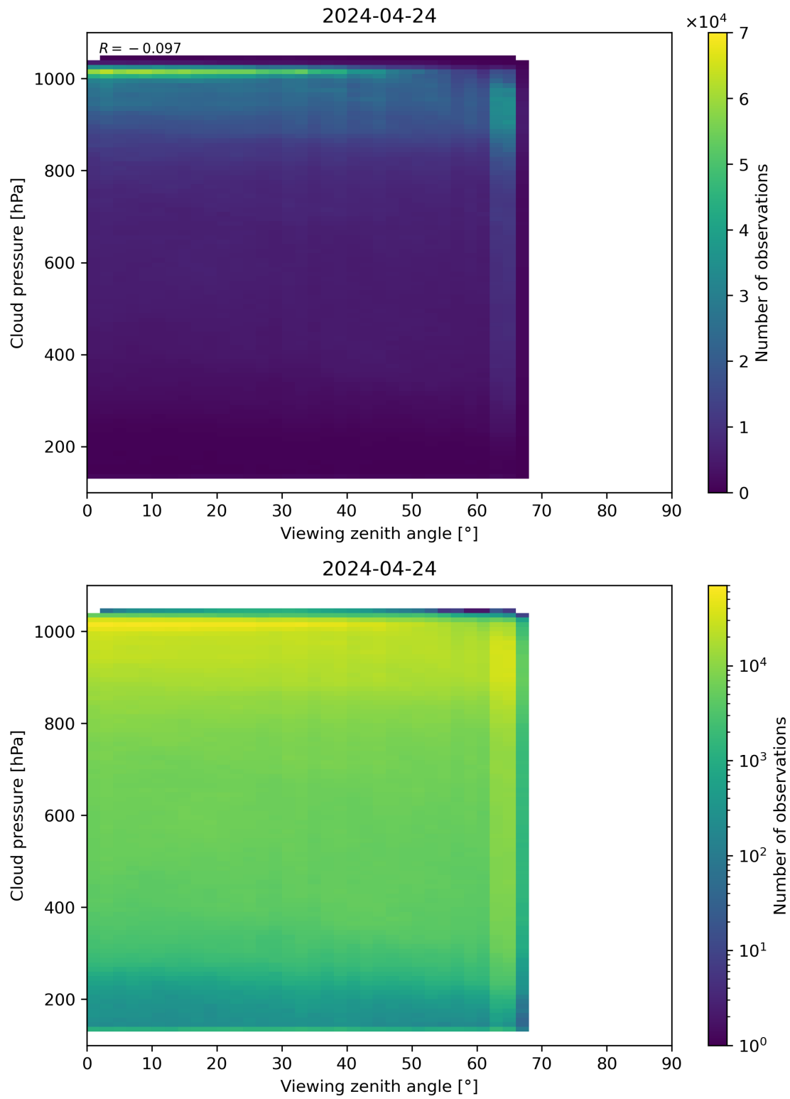
Figure 121: Scatter density plot of “Viewing zenith angle” against “Cloud pressure” for 2024-04-23 to 2024-04-25.
