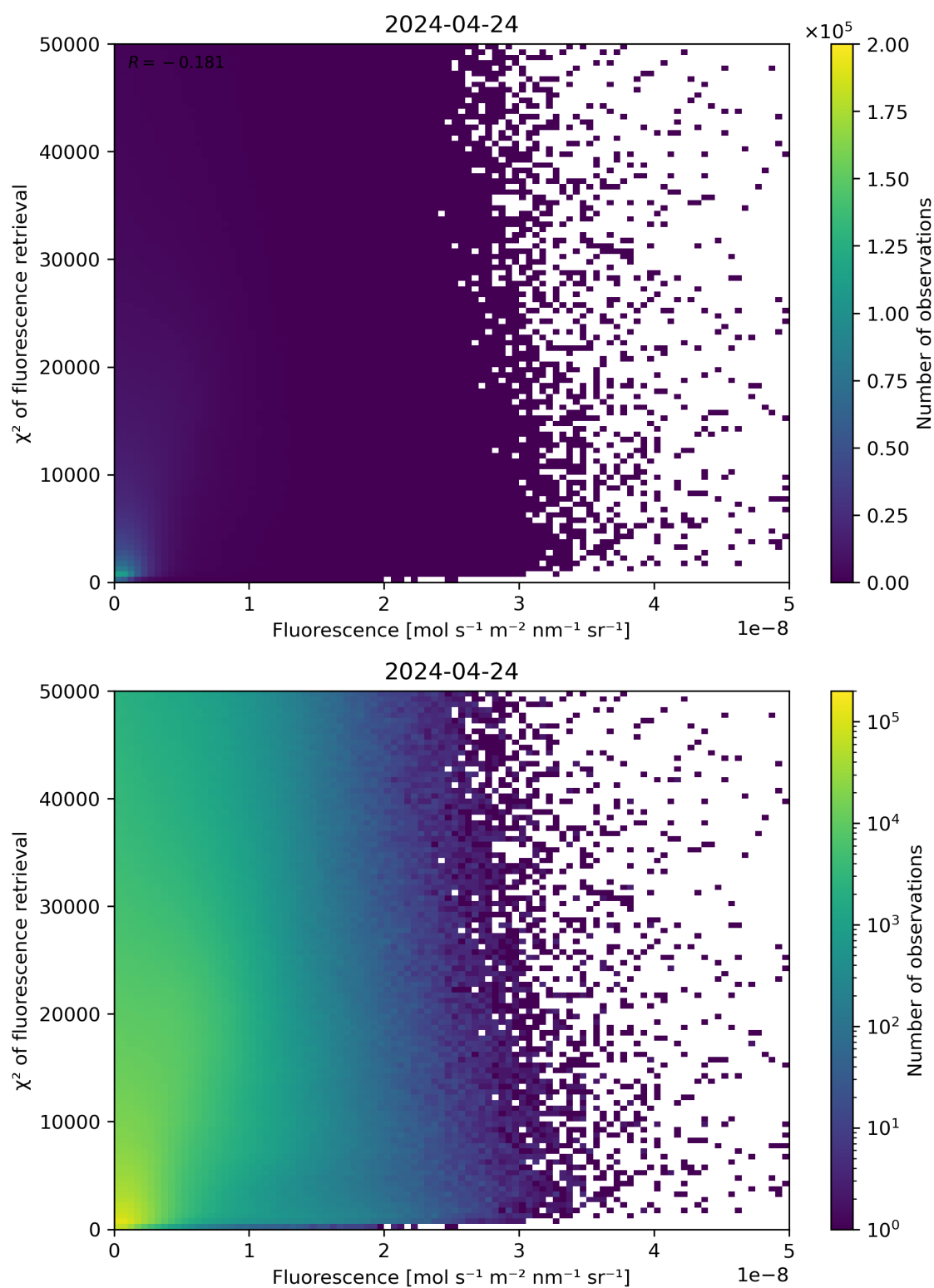
Figure 85: Scatter density plot of “Fluorescence” against “ \chi^2 of fluorescence retrieval” for 2024-04-23 to 2024-04-25.
