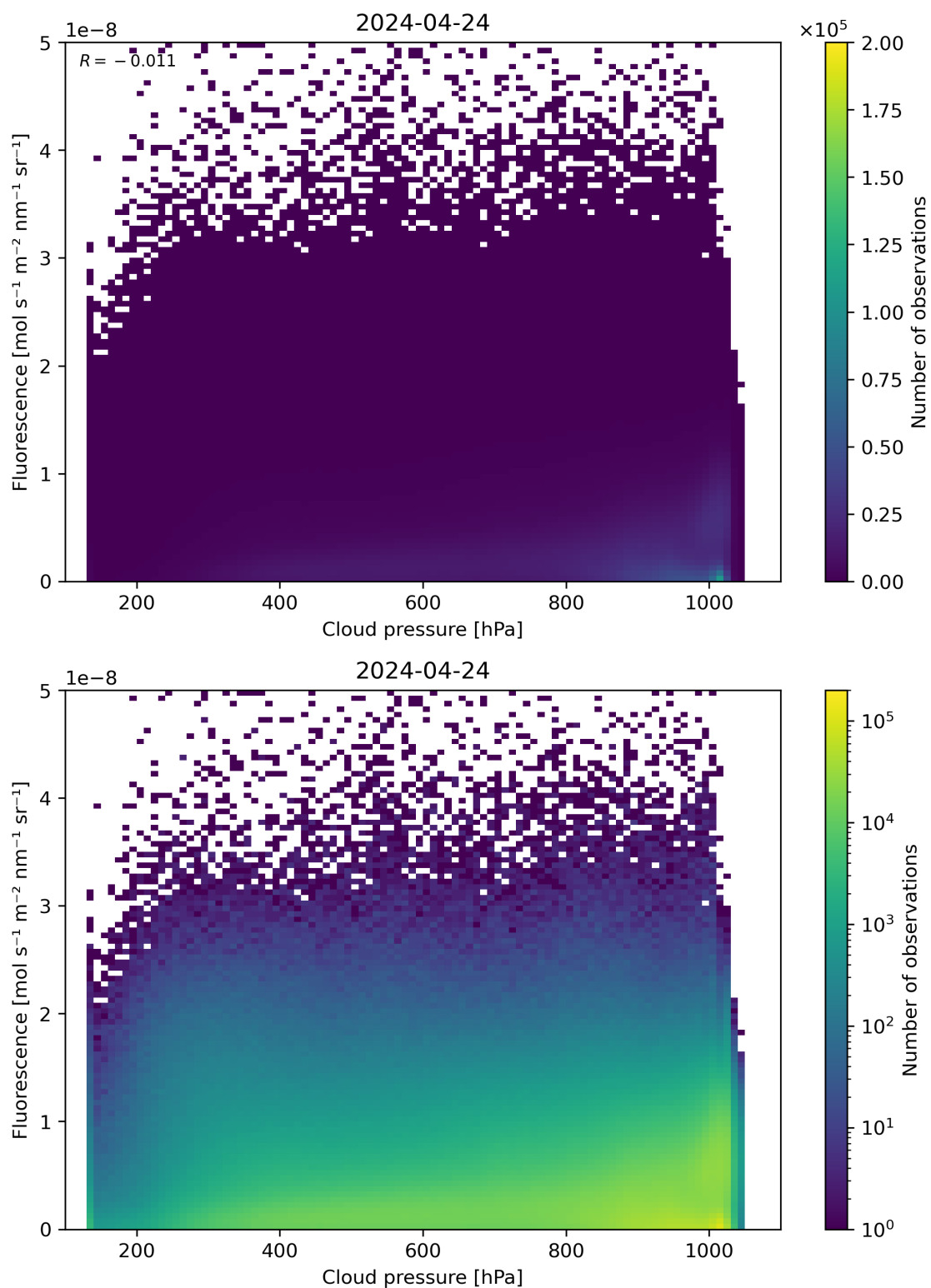
Figure 80: Scatter density plot of “Cloud pressure” against “Fluorescence” for 2024-04-23 to 2024-04-25.
