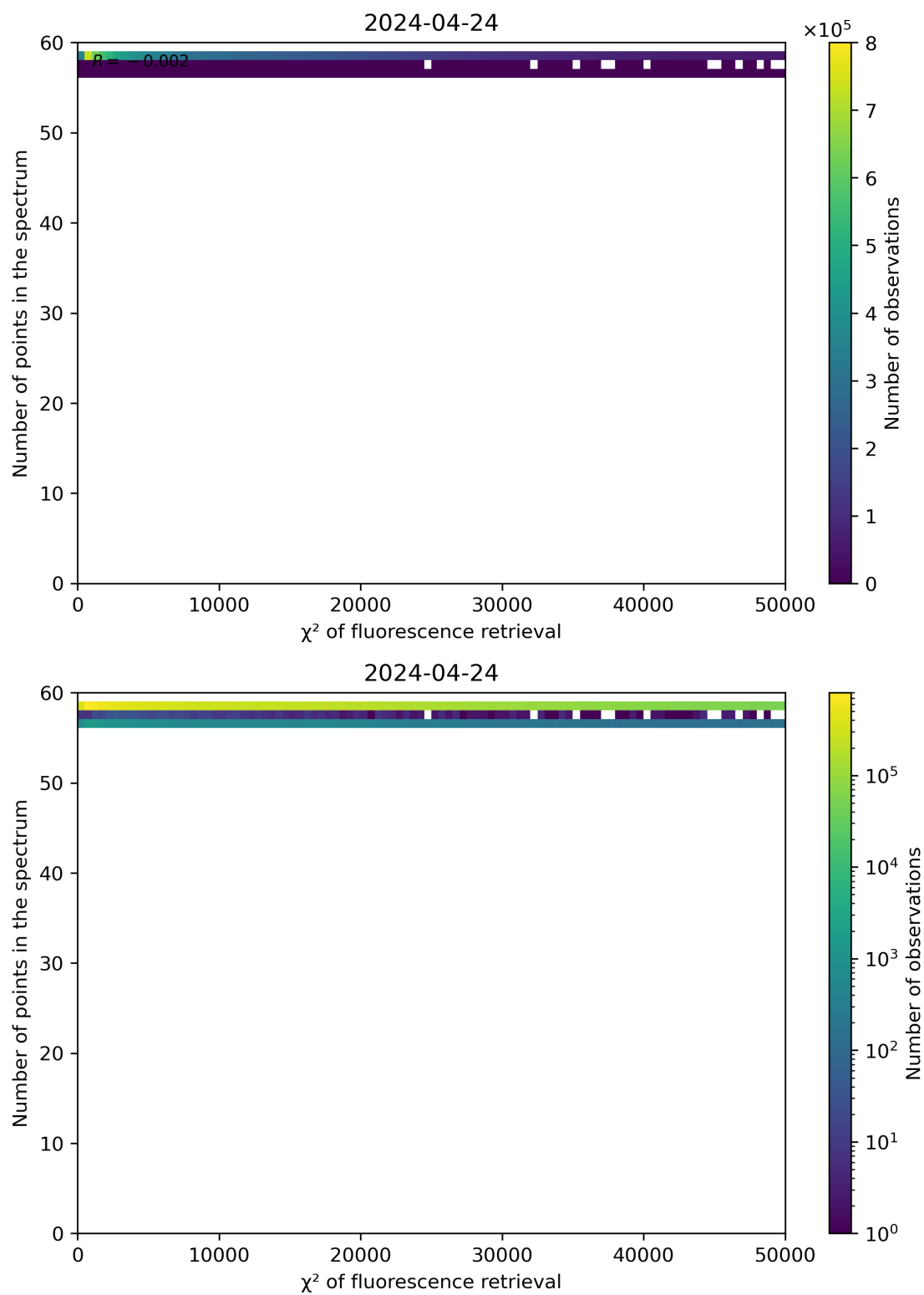
Figure 68: Scatter density plot of " \chi^2 of fluorescence retrieval" against "Number of points in the spectrum" for 2024-04-23 to 2024-04-25.
