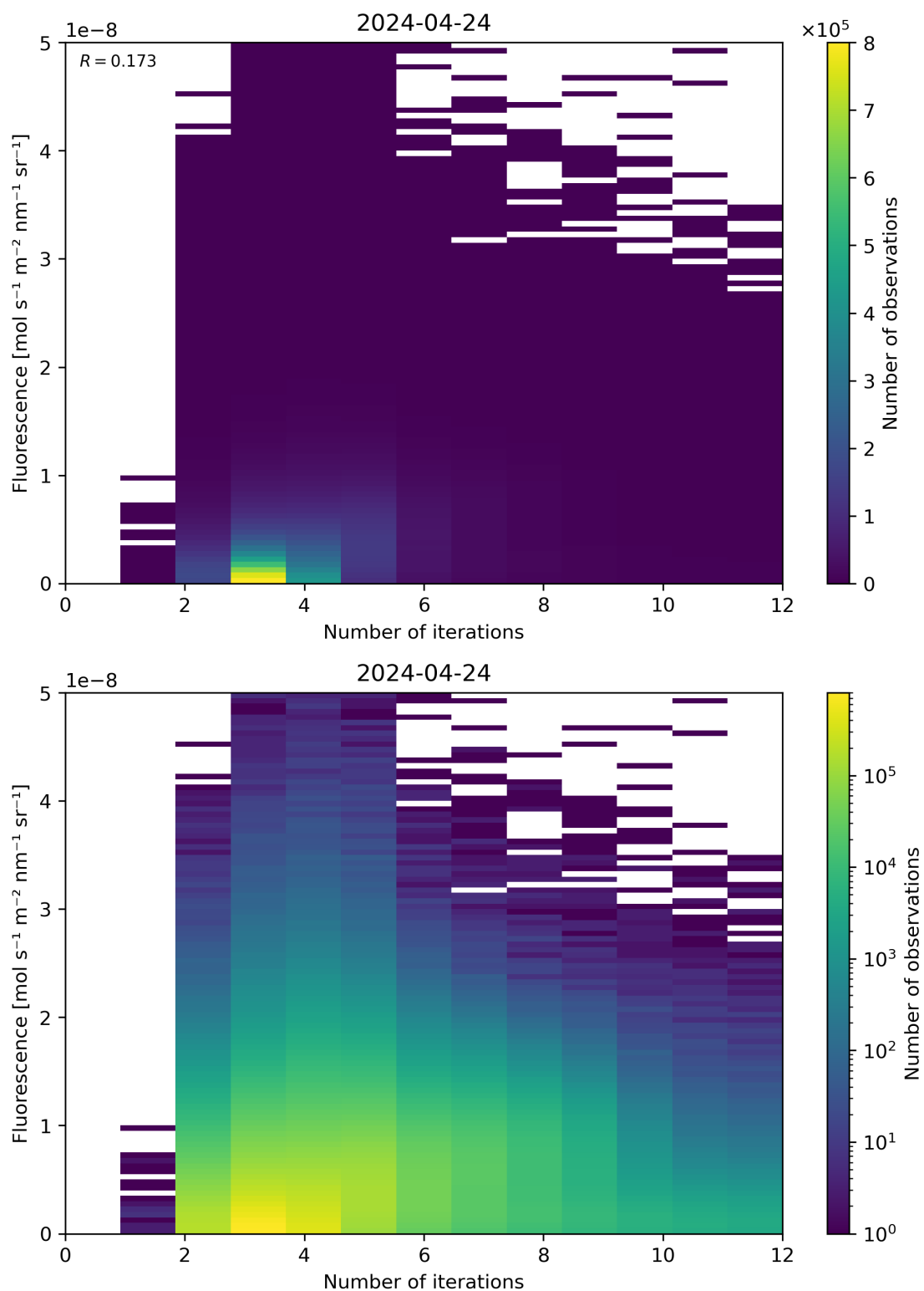
Figure 98: Scatter density plot of “Number of iterations” against “Fluorescence” for 2024-04-23 to 2024-04-25.
