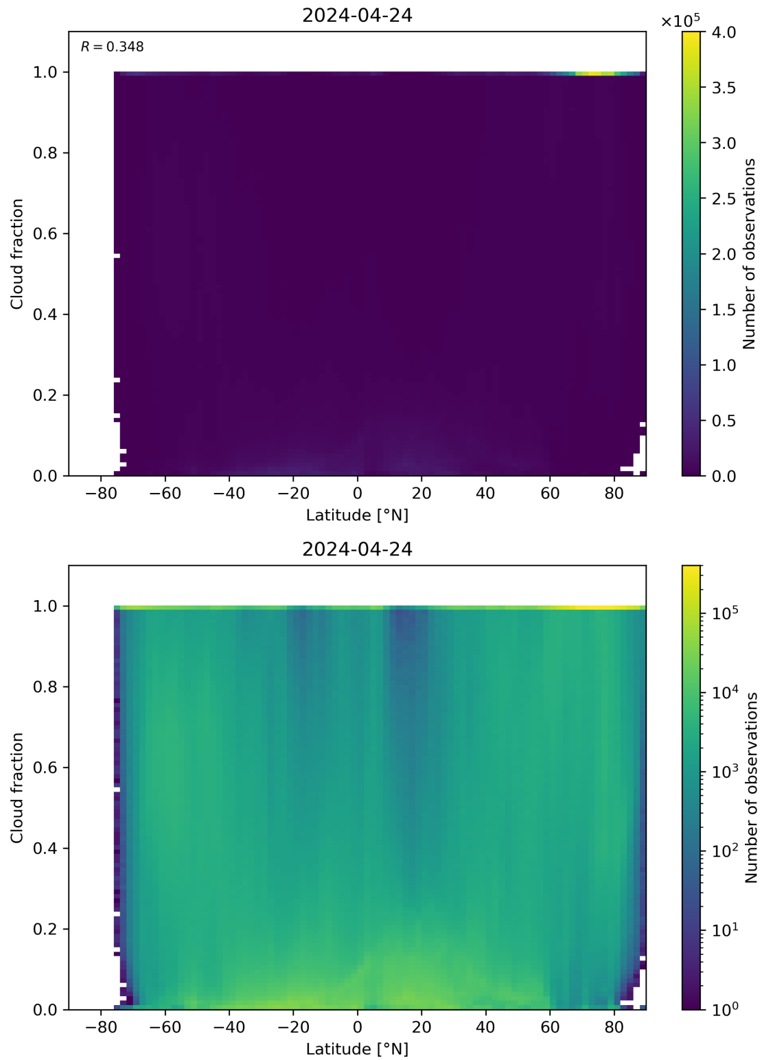
Figure 90: Scatter density plot of “Latitude” against “Cloud fraction” for 2024-04-23 to 2024-04-25.
