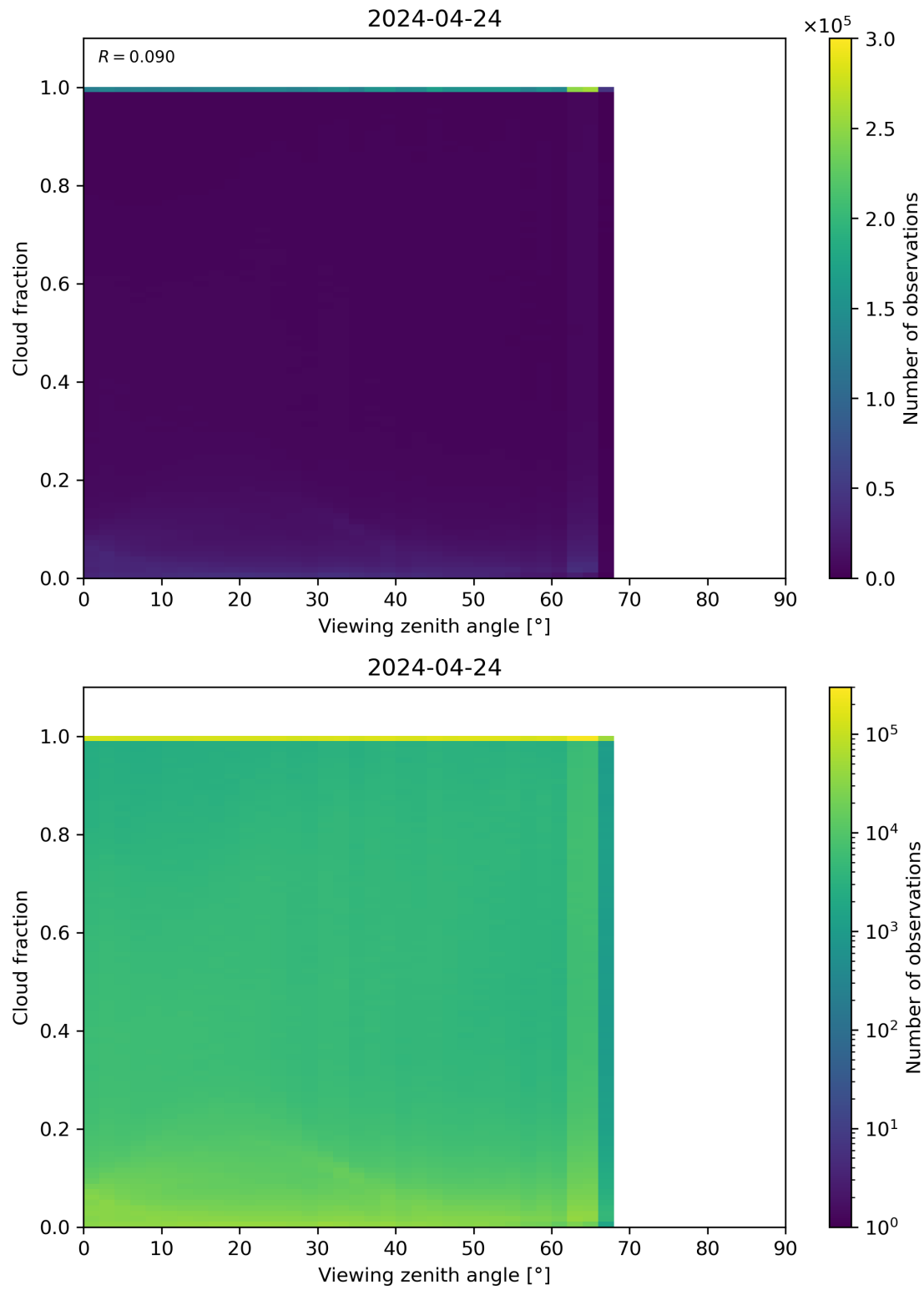
Figure 120: Scatter density plot of “Viewing zenith angle” against “Cloud fraction” for 2024-04-23 to 2024-04-25.
