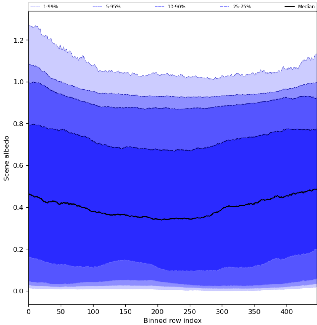
Figure 51: Along track statistics of “Scene albedo” for 2024-04-23 to 2024-04-25
