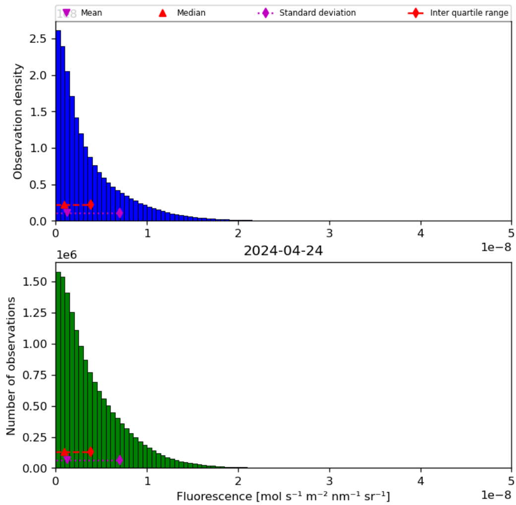
Figure 40: Histogram of “Fluorescence” for 2024-04-23 to 2024-04-25
