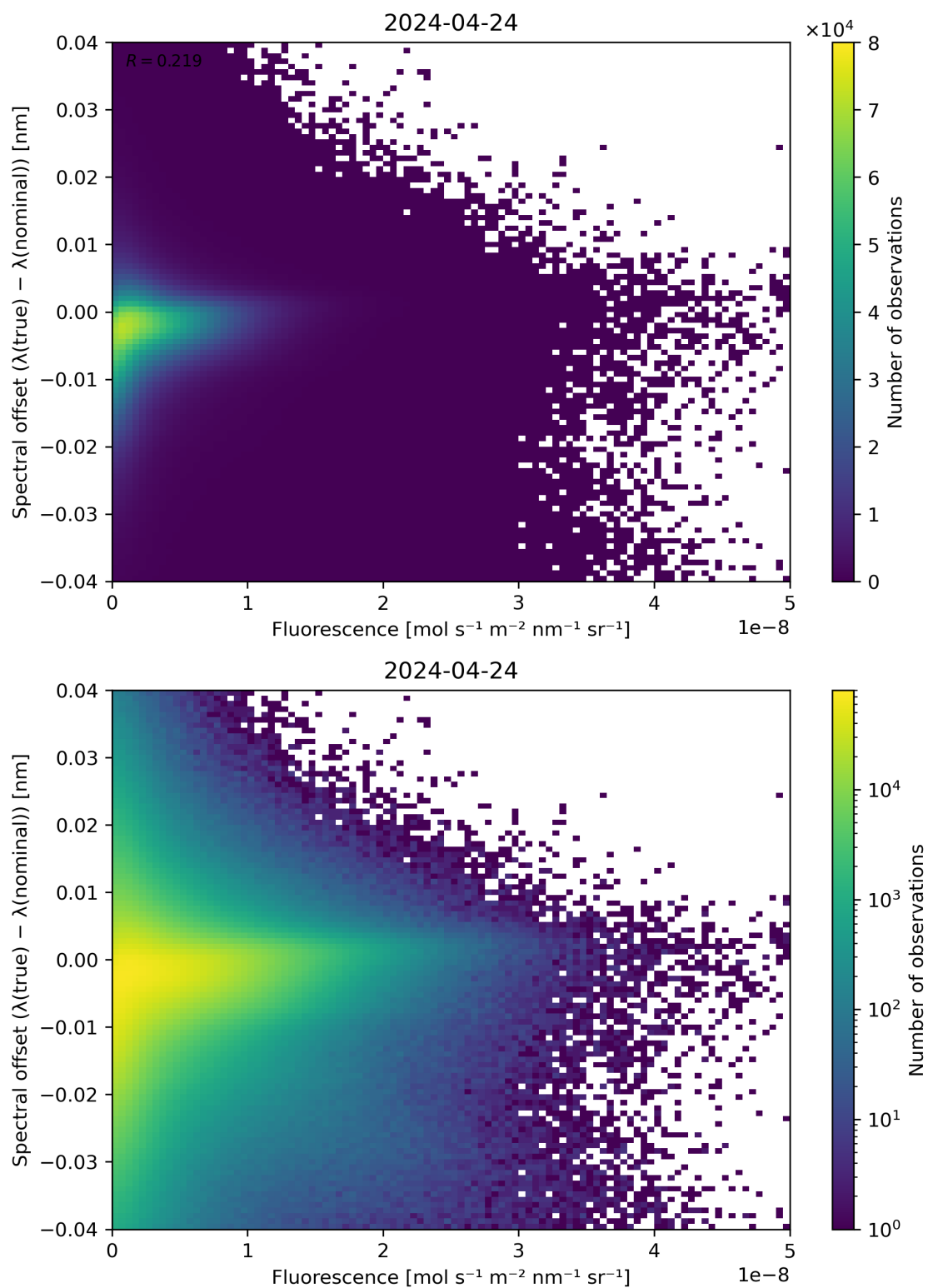
Figure 87: Scatter density plot of “Fluorescence” against “Spectral offset ( \lambda(\text{true}) - \lambda(\text{nominal}) )” for 2024-04-23 to 2024-04-25.
