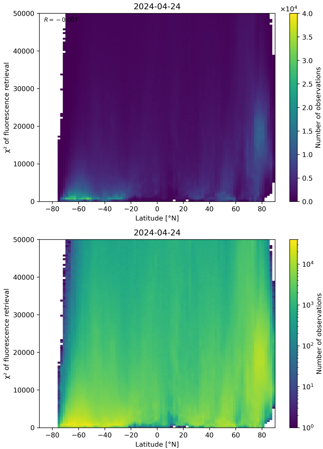
Figure 89: Scatter density plot of “Latitude” against “ \chi^2 of fluorescence retrieval” for 2024-04-23 to 2024-04-25.
