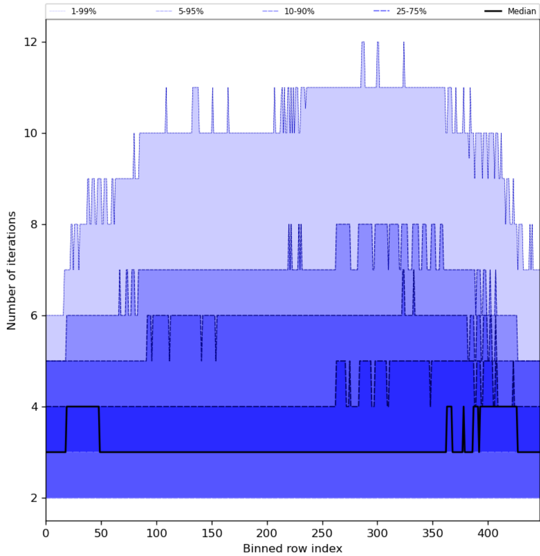
Figure 56: Along track statistics of “Number of iterations” for 2024-04-23 to 2024-04-25
