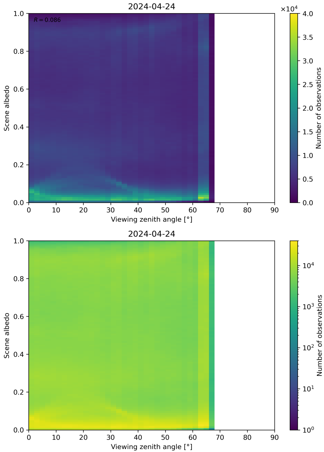
Figure 126: Scatter density plot of “Viewing zenith angle” against “Scene albedo” for 2024-04-23 to 2024-04-25.
