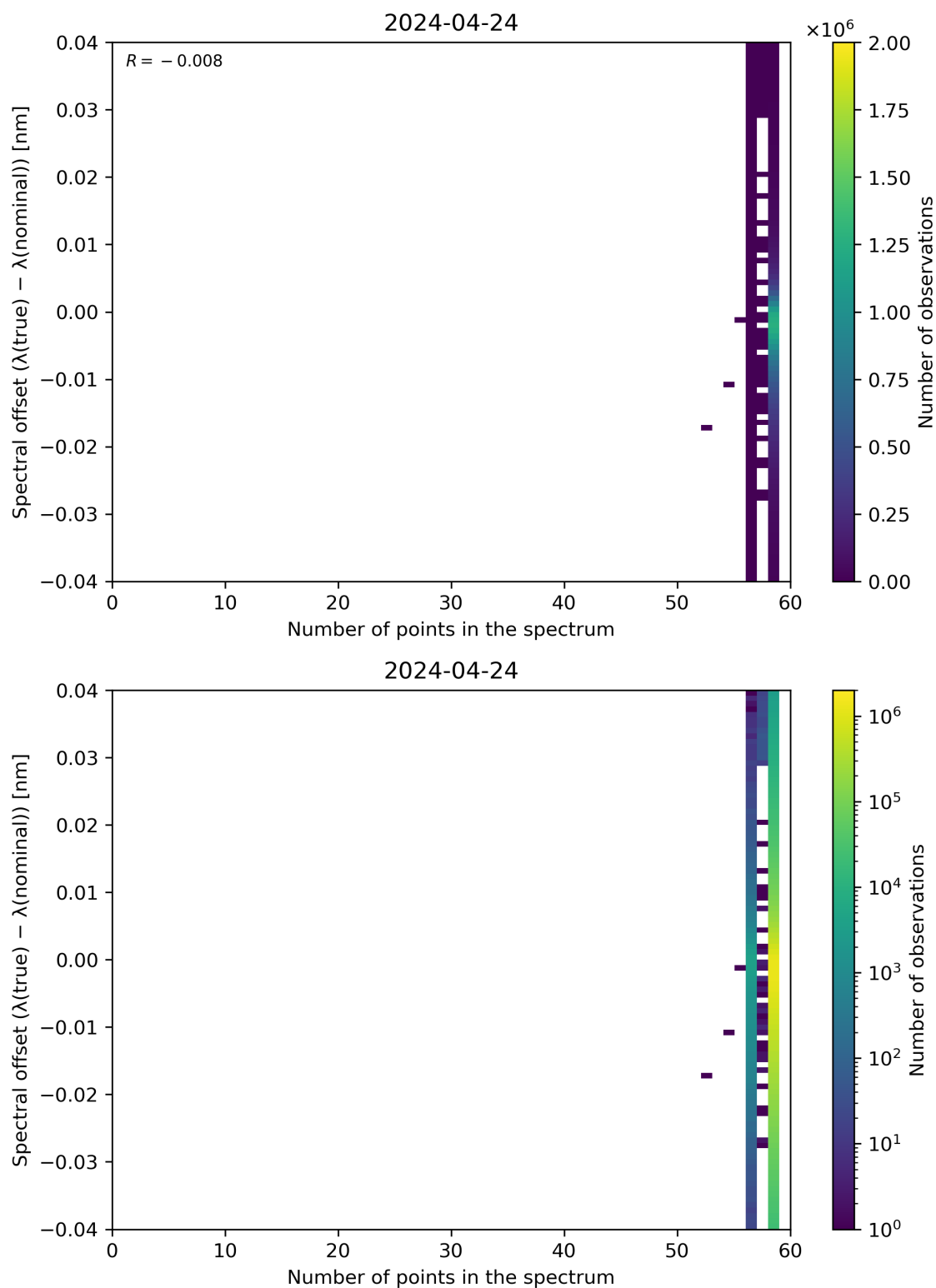
Figure 101: Scatter density plot of “Number of points in the spectrum” against “Spectral offset ( \lambda(\text{true}) - \lambda(\text{nominal}) )” for 2024-04-23 to 2024-04-25.
