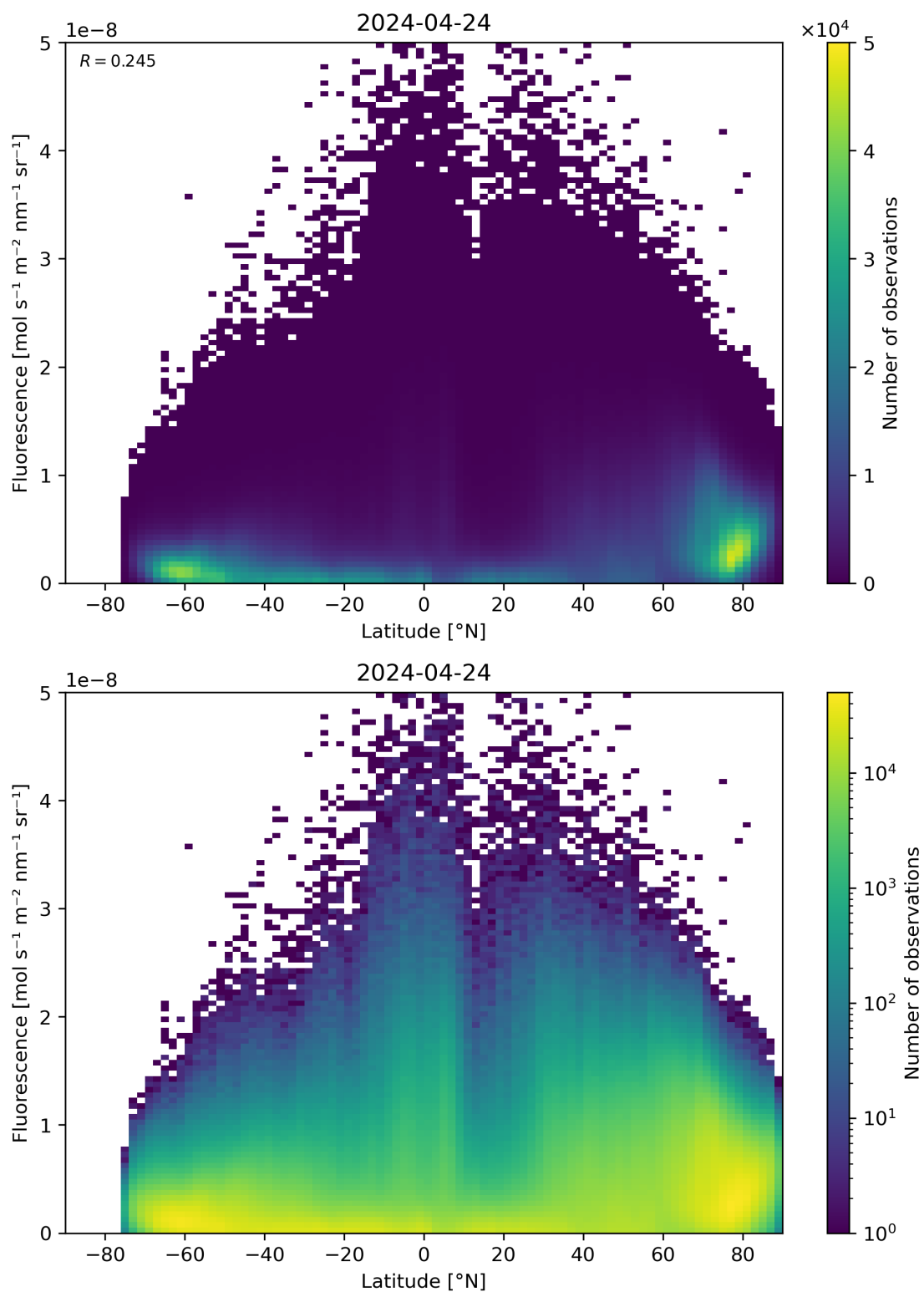
Figure 92: Scatter density plot of “Latitude” against “Fluorescence” for 2024-04-23 to 2024-04-25.
