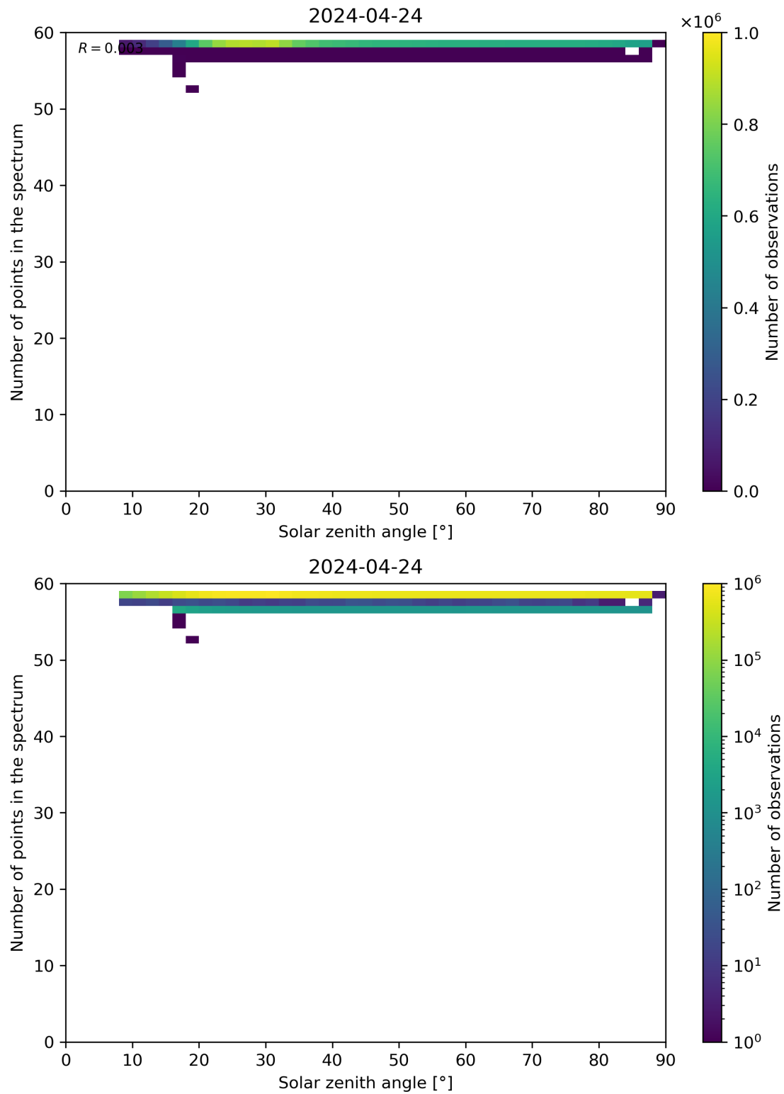
Figure 115: Scatter density plot of “Solar zenith angle” against “Number of points in the spectrum” for 2024-04-23 to 2024-04-25.
