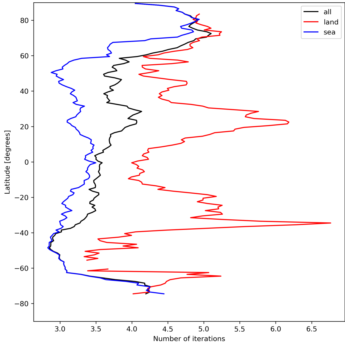
Figure 22: Zonal average of “Number of iterations” for 2024-04-23 to 2024-04-25.
