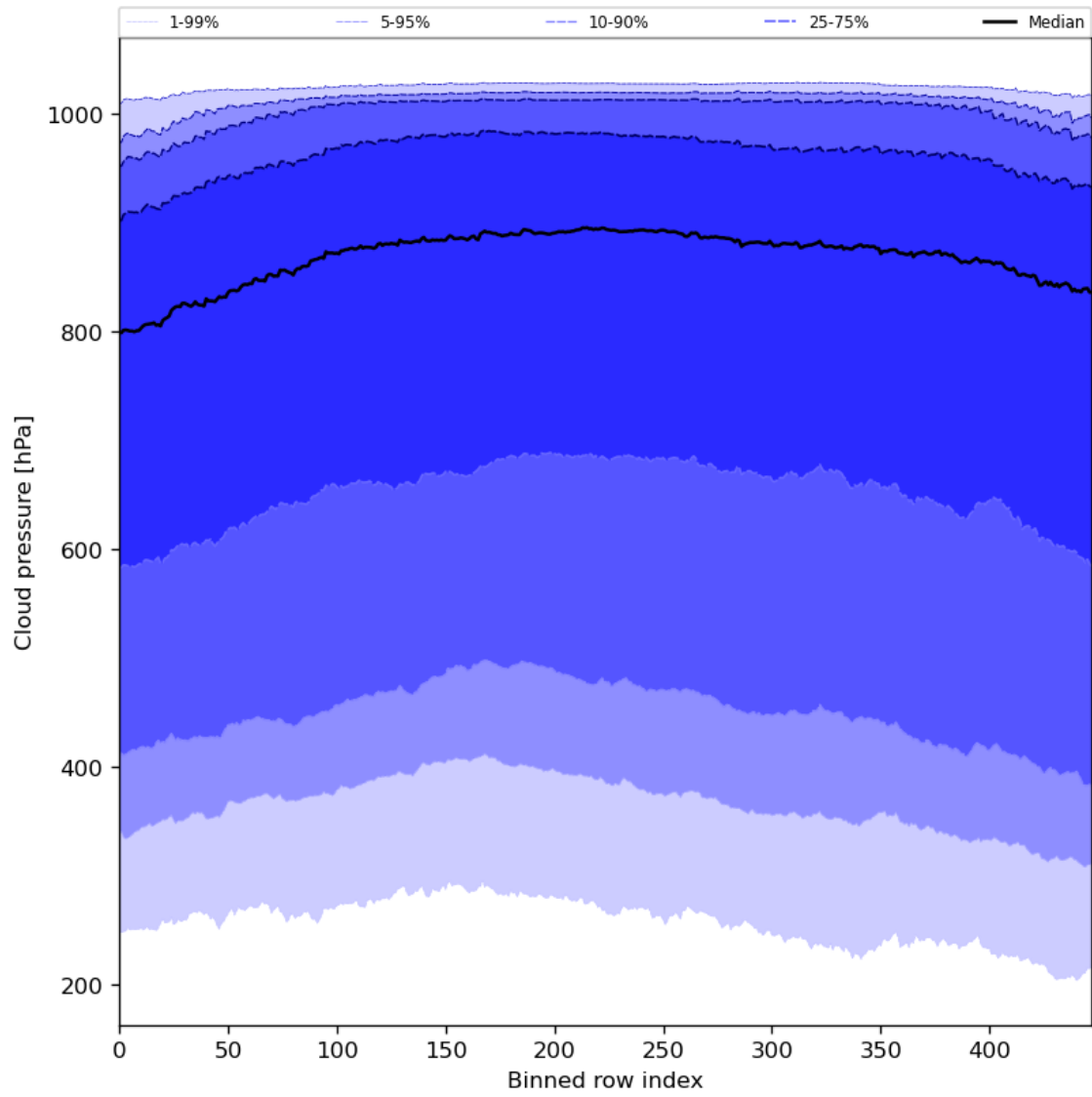
Figure 47: Along track statistics of “Cloud pressure” for 2024-04-23 to 2024-04-25
