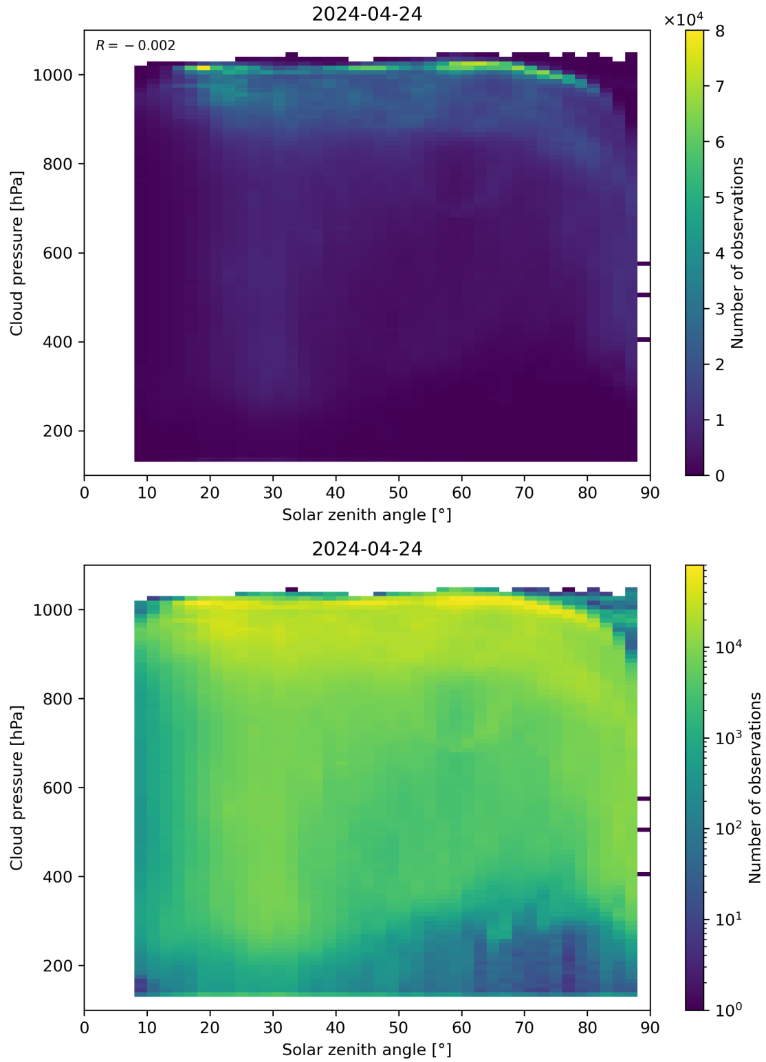
Figure 111: Scatter density plot of “Solar zenith angle” against “Cloud pressure” for 2024-04-23 to 2024-04-25.
