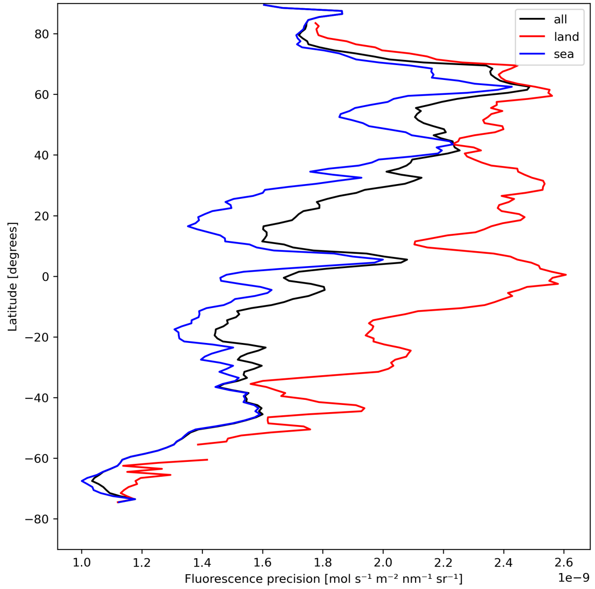
Figure 24: Zonal average of “Fluorescence precision” for 2024-04-23 to 2024-04-25.
