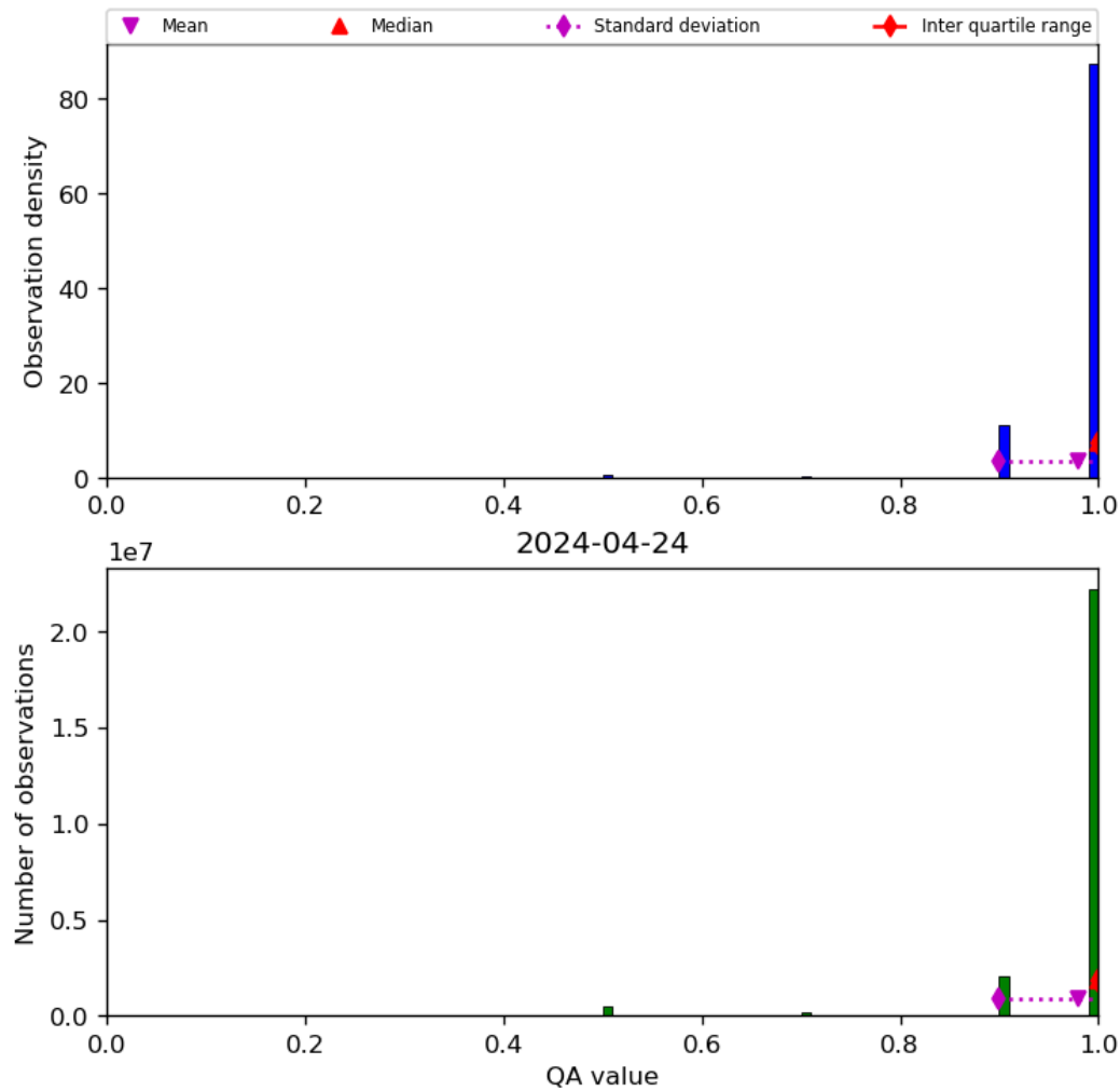
Figure 29: Histogram of “QA value” for 2024-04-23 to 2024-04-25
