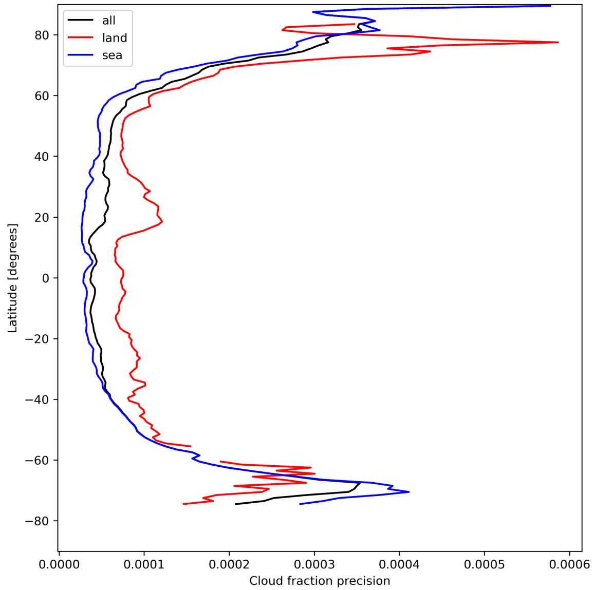
Figure 16: Zonal average of “Cloud fraction precision” for 2024-04-23 to 2024-04-25.
