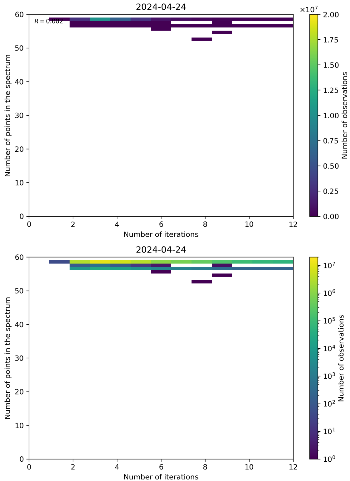
Figure 99: Scatter density plot of “Number of iterations” against “Number of points in the spectrum” for 2024-04-23 to 2024-04-25.
