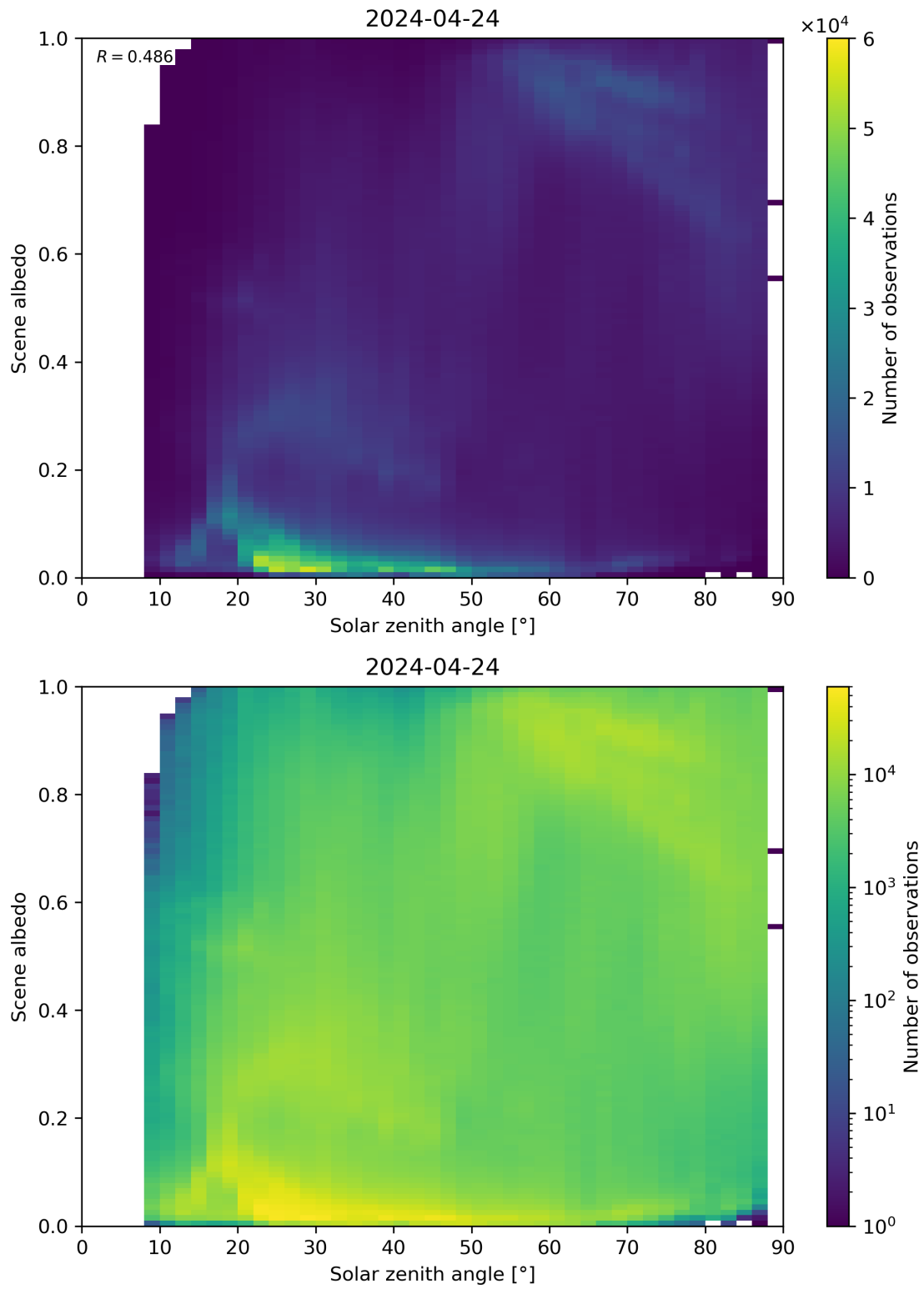
Figure 116: Scatter density plot of “Solar zenith angle” against “Scene albedo” for 2024-04-23 to 2024-04-25.
