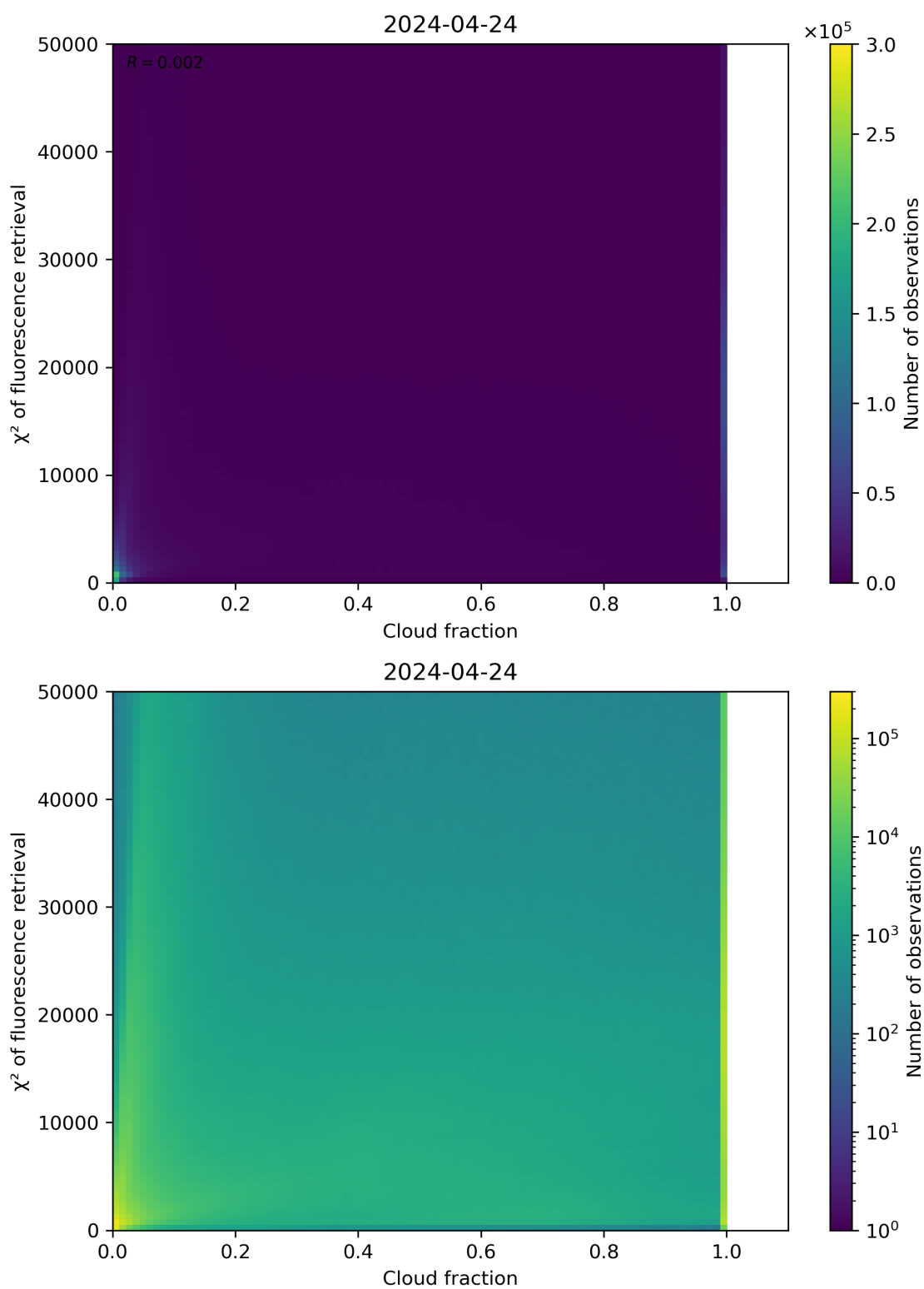
Figure 71: Scatter density plot of “Cloud fraction” against “ \chi^2 of fluorescence retrieval” for 2024-04-23 to 2024-04-25.
