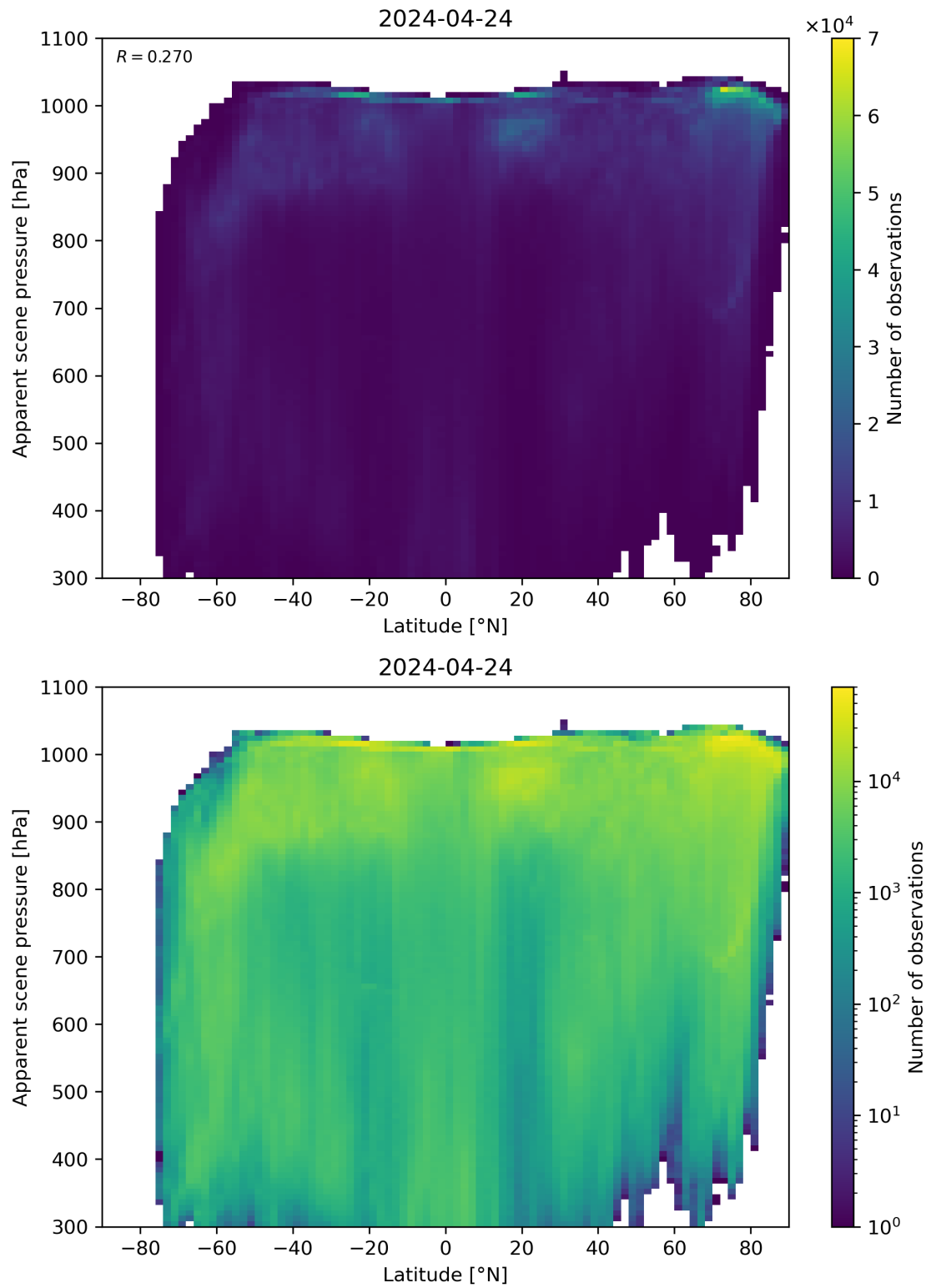
Figure 88: Scatter density plot of “Latitude” against “Apparent scene pressure” for 2024-04-23 to 2024-04-25.
