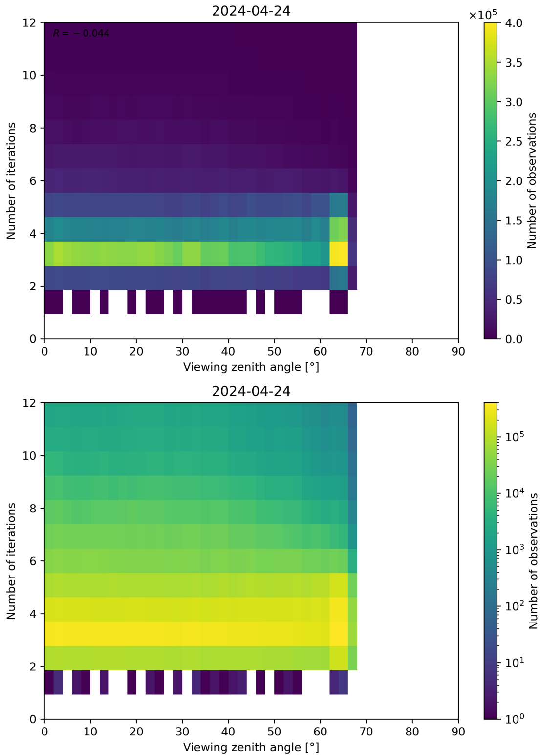
Figure 124: Scatter density plot of “Viewing zenith angle” against “Number of iterations” for 2024-04-23 to 2024-04-25.
