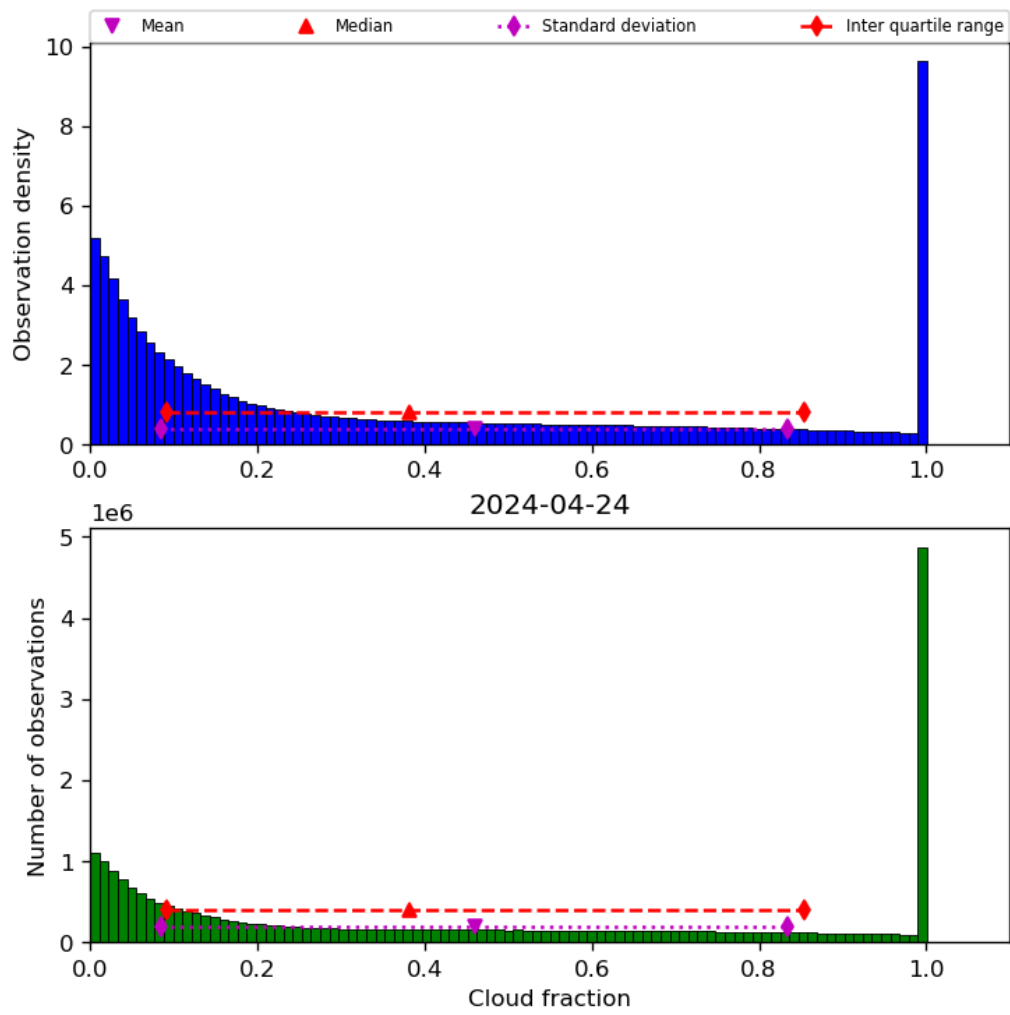
Figure 32: Histogram of “Cloud fraction” for 2024-04-23 to 2024-04-25
