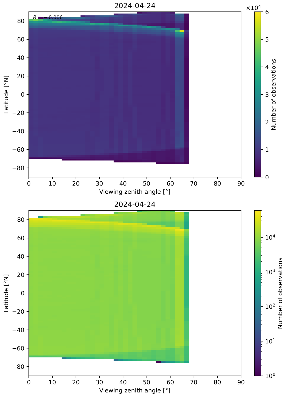
Figure 123: Scatter density plot of “Viewing zenith angle” against “Latitude” for 2024-04-23 to 2024-04-25.
