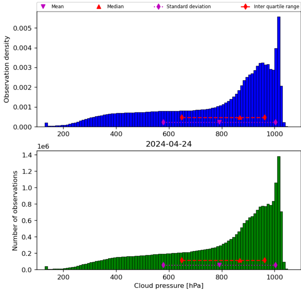
Figure 30: Histogram of “Cloud pressure” for 2024-04-23 to 2024-04-25
