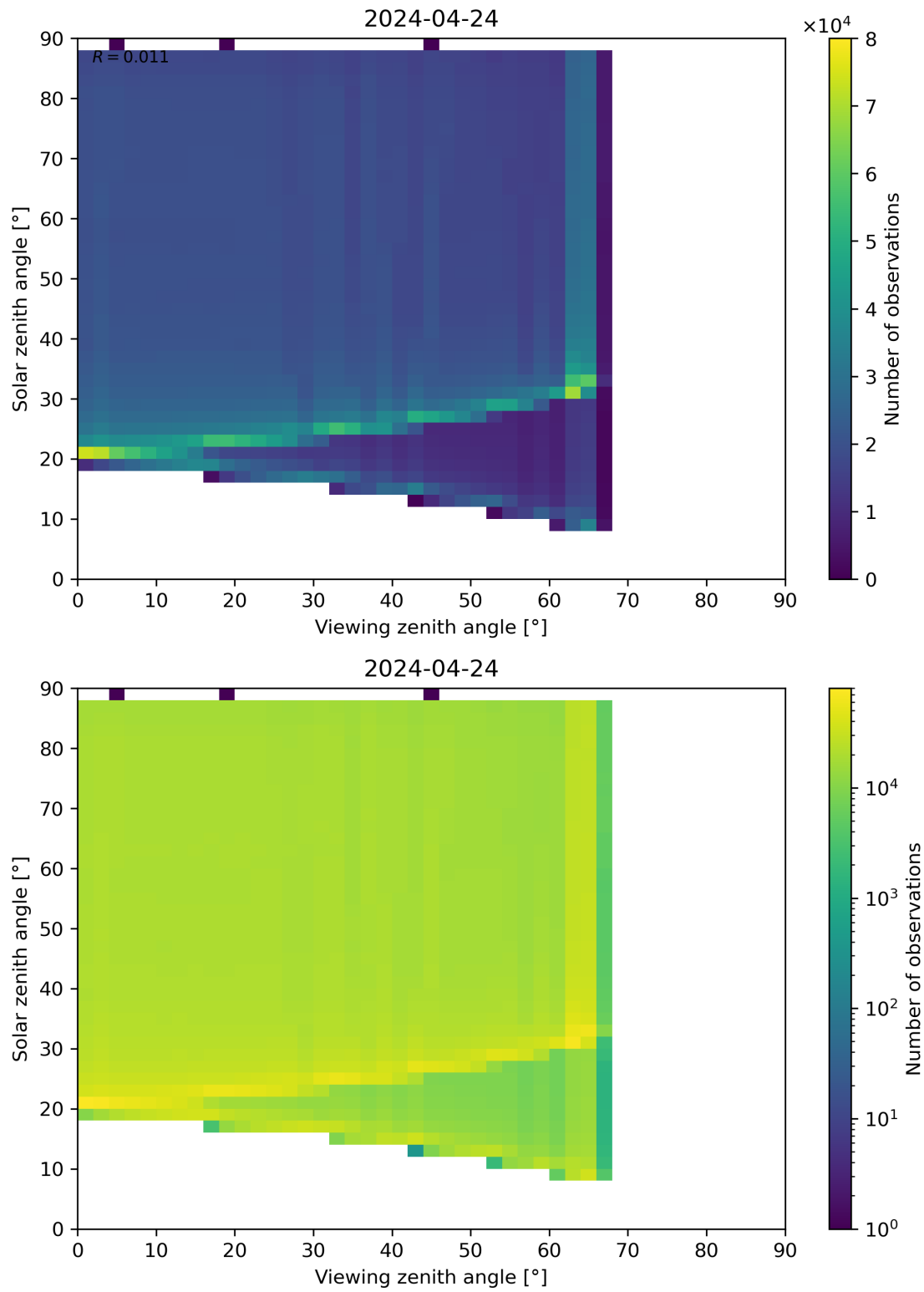
Figure 127: Scatter density plot of “Viewing zenith angle” against “Solar zenith angle” for 2024-04-23 to 2024-04-25.
