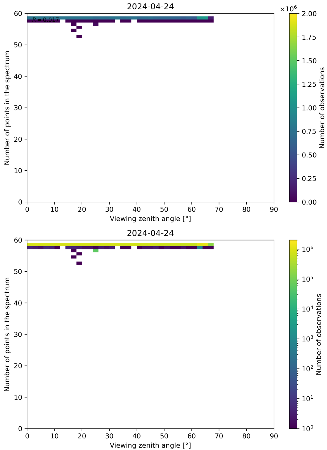
Figure 125: Scatter density plot of “Viewing zenith angle” against “Number of points in the spectrum” for 2024-04-23 to 2024-04-25.
