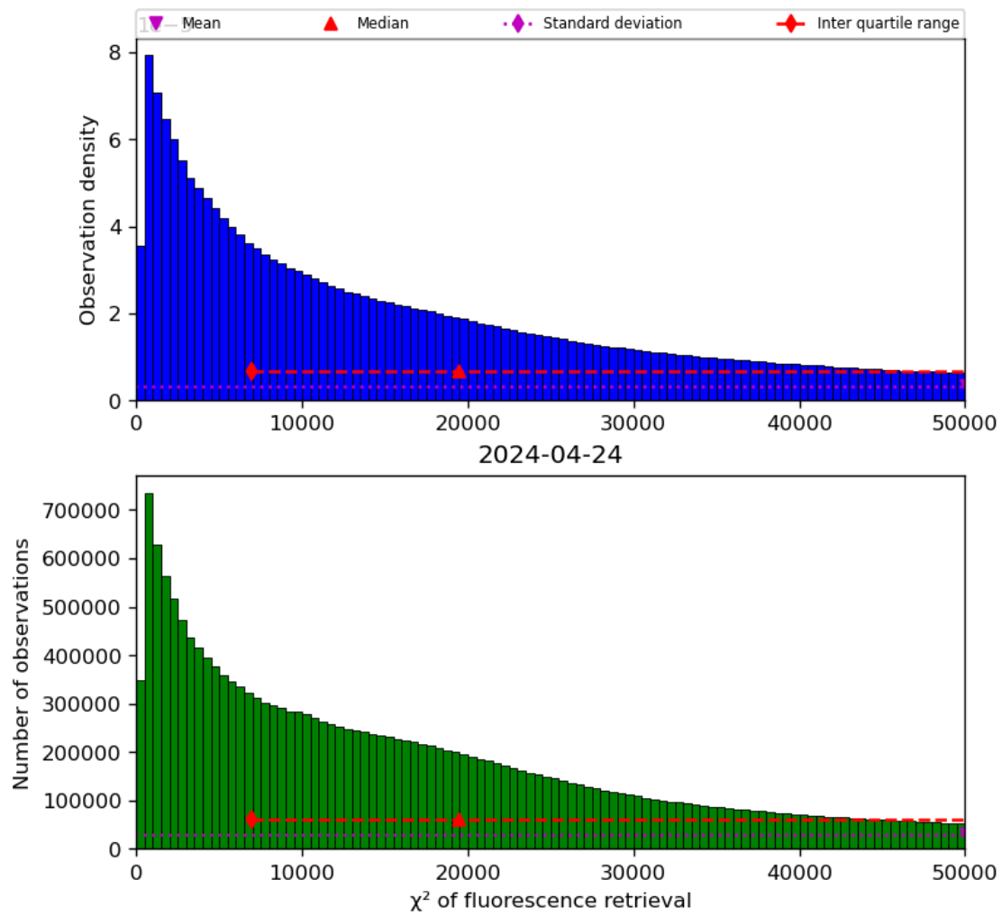
Figure 42: Histogram of “ \chi^2 of fluorescence retrieval” for 2024-04-23 to 2024-04-25
