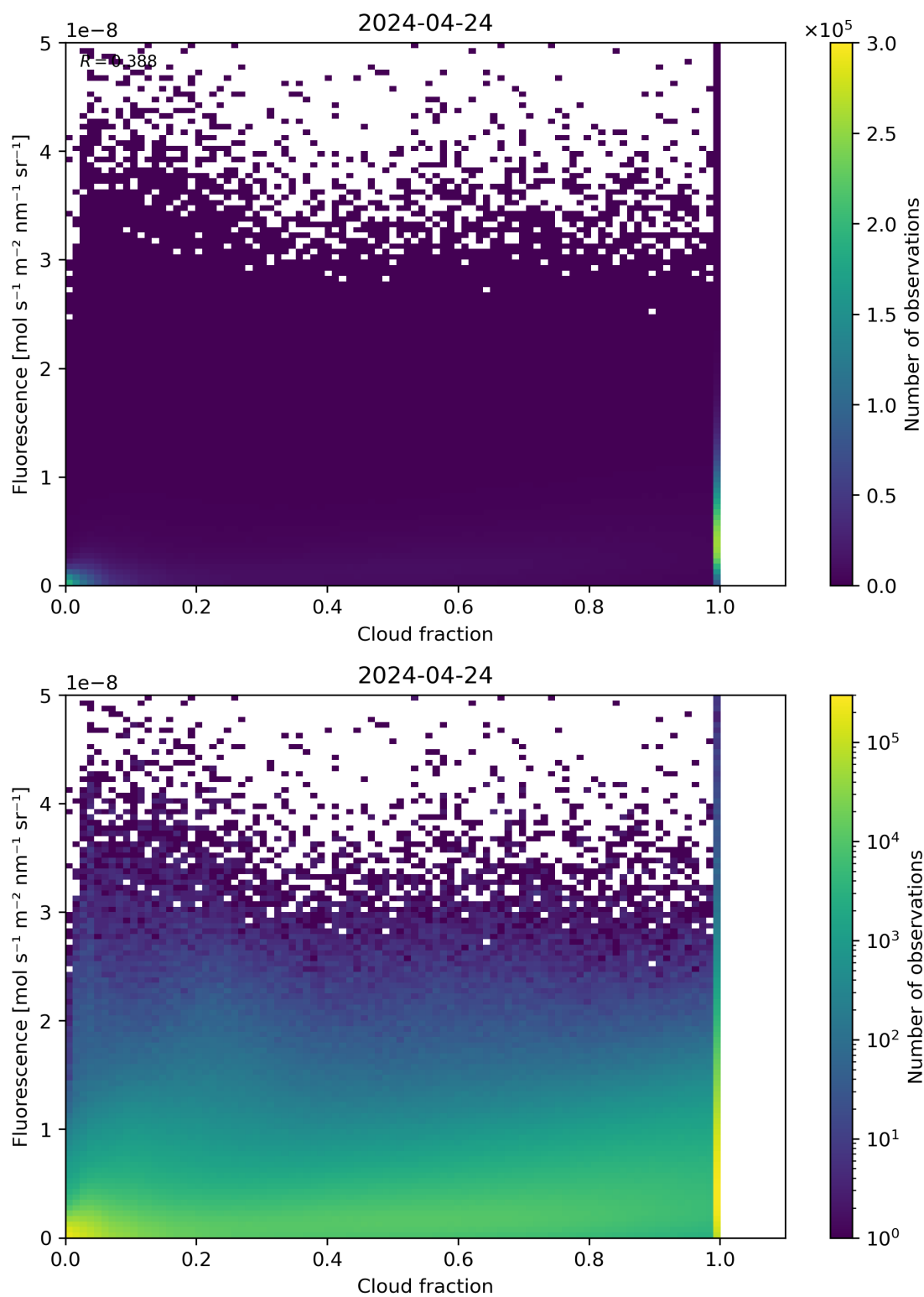
Figure 72: Scatter density plot of “Cloud fraction” against “Fluorescence” for 2024-04-23 to 2024-04-25.
