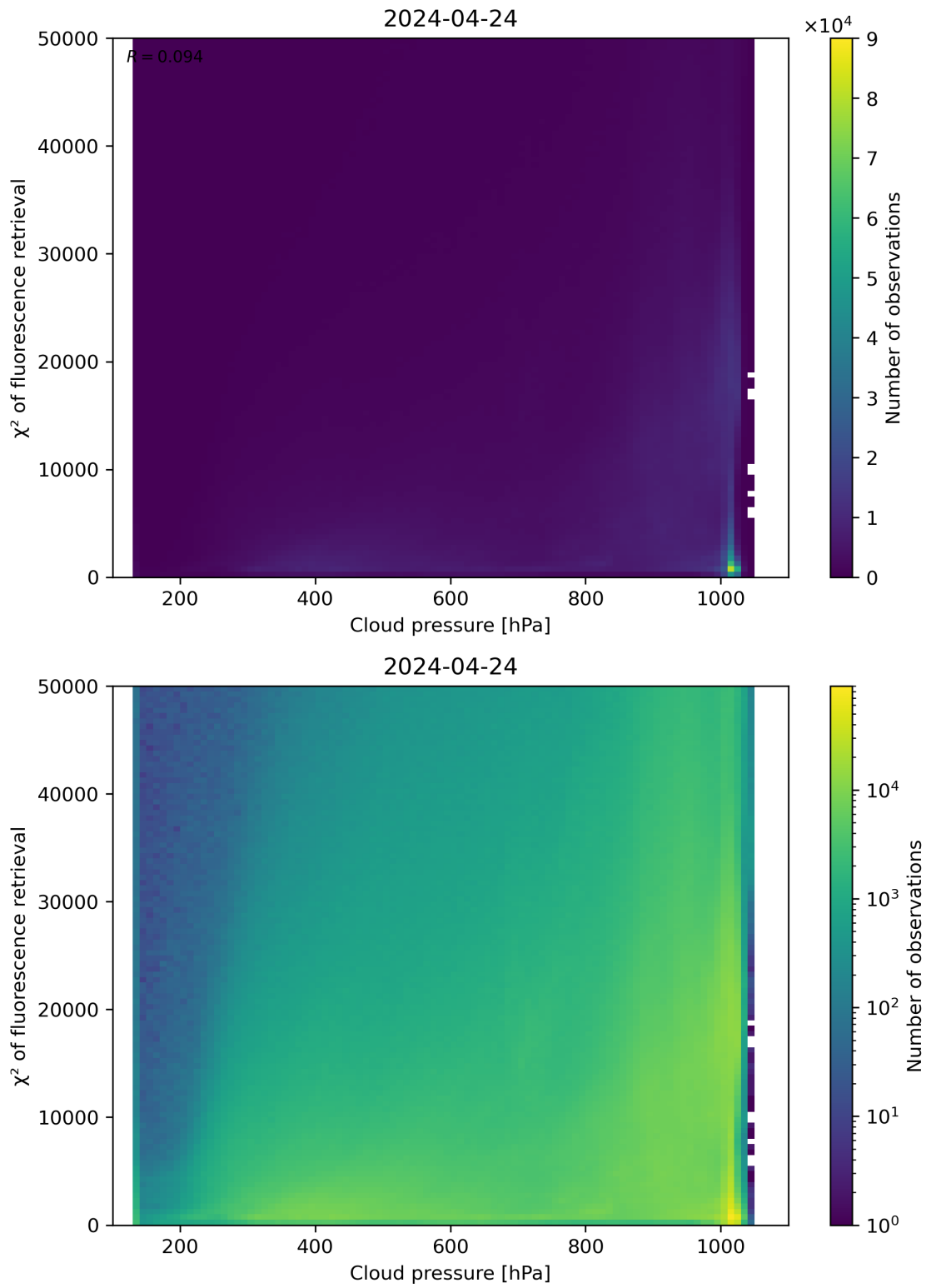
Figure 78: Scatter density plot of “Cloud pressure” against “ \chi^2 of fluorescence retrieval” for 2024-04-23 to 2024-04-25.
