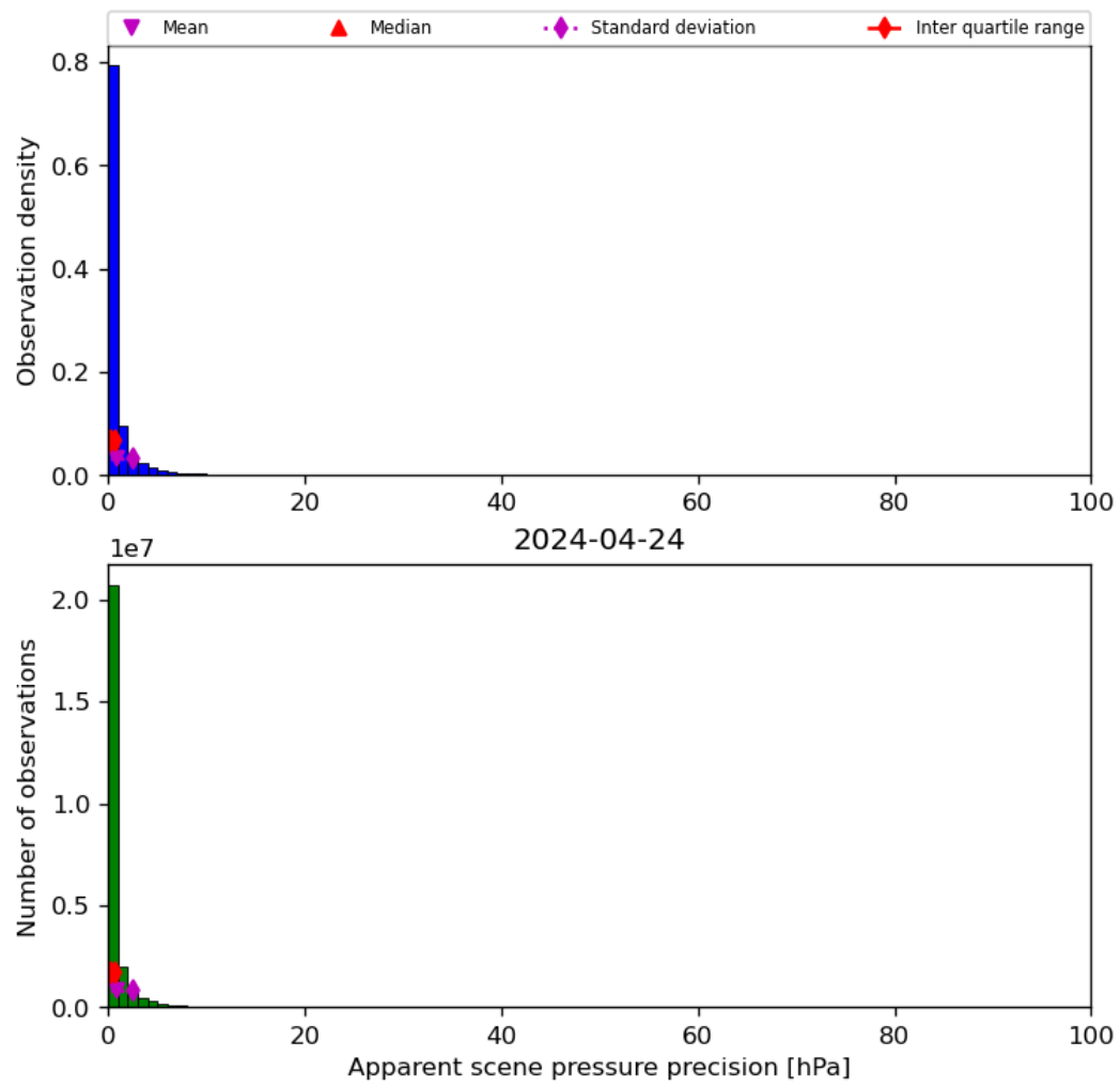
Figure 37: Histogram of “Apparent scene pressure precision” for 2024-04-23 to 2024-04-25
