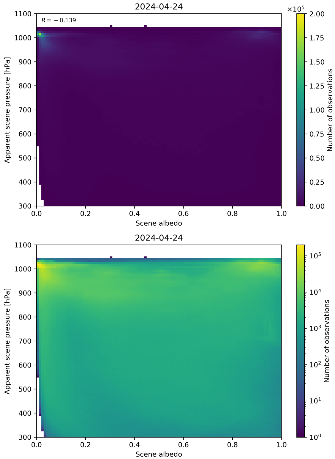
Figure 102: Scatter density plot of “Scene albedo” against “Apparent scene pressure” for 2024-04-23 to 2024-04-25.
