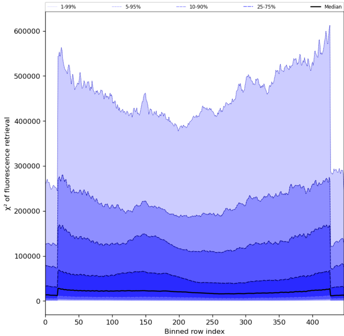
Figure 59: Along track statistics of “ \chi^2 of fluorescence retrieval” for 2024-04-23 to 2024-04-25
