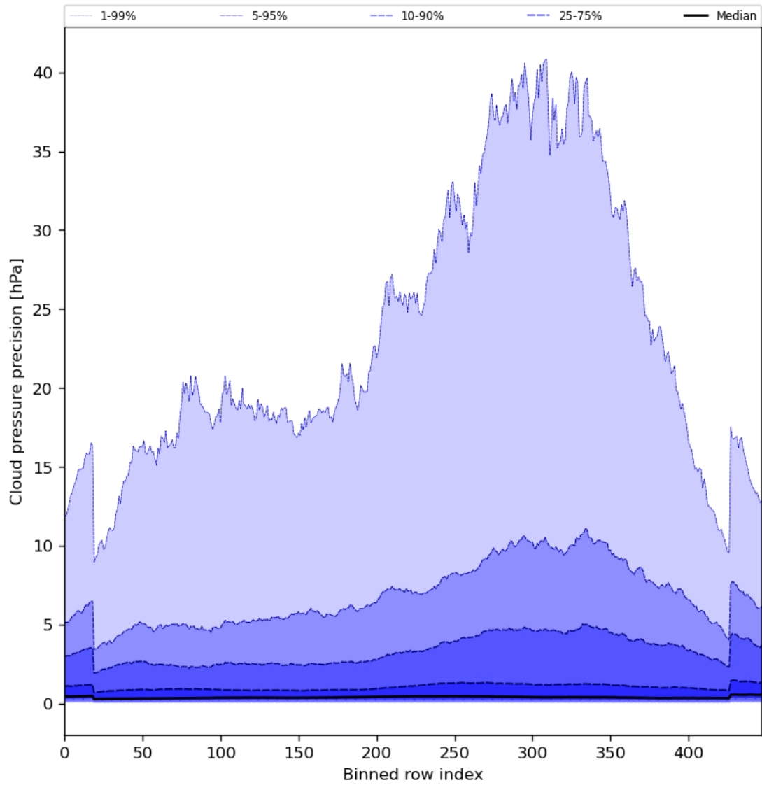
Figure 48: Along track statistics of “Cloud pressure precision” for 2024-04-23 to 2024-04-25
