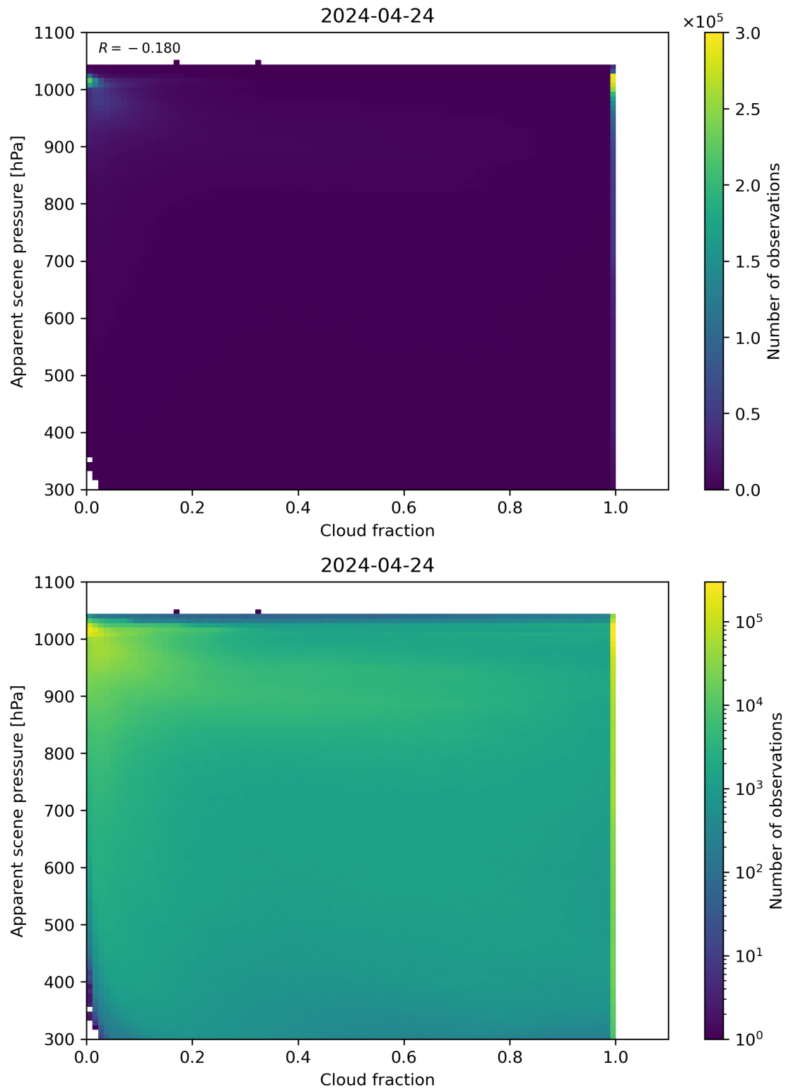
Figure 70: Scatter density plot of “Cloud fraction” against “Apparent scene pressure” for 2024-04-23 to 2024-04-25.
