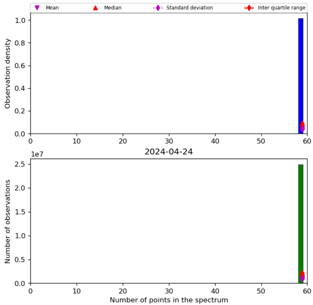
Figure 44: Histogram of “Number of points in the spectrum” for 2024-04-23 to 2024-04-25
