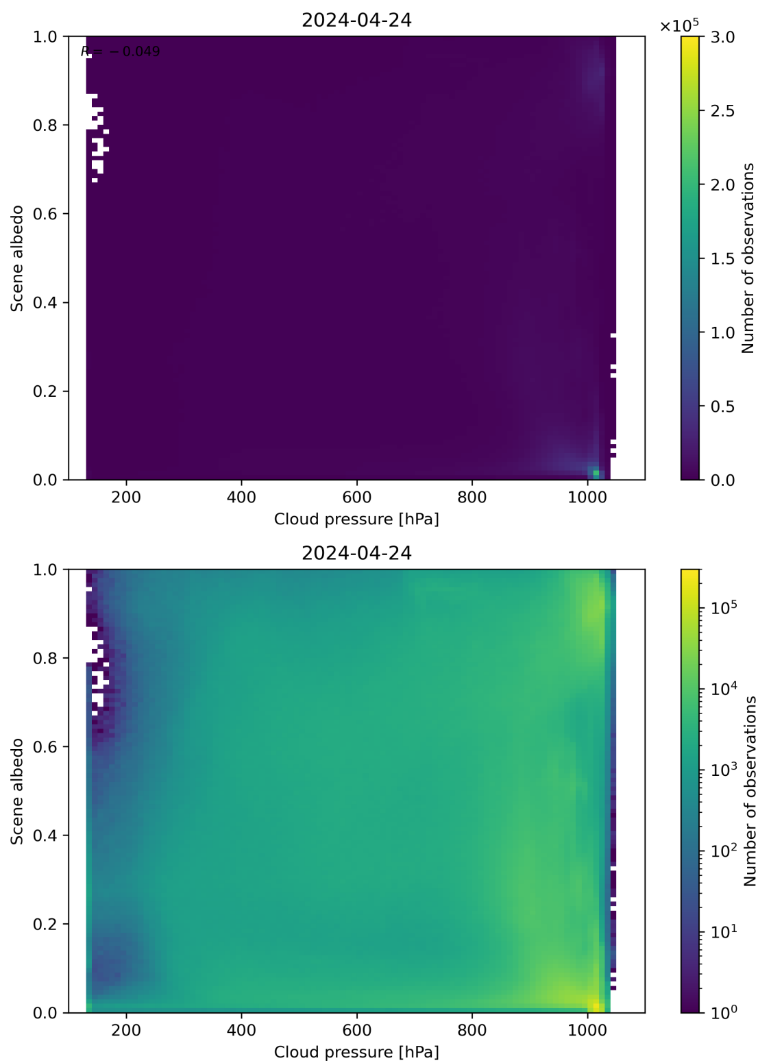
Figure 83: Scatter density plot of “Cloud pressure” against “Scene albedo” for 2024-04-23 to 2024-04-25.
