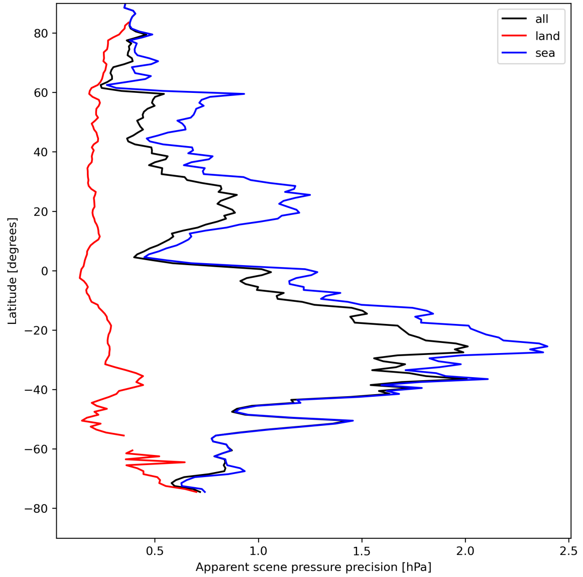
Figure 20: Zonal average of “Apparent scene pressure precision” for 2024-04-23 to 2024-04-25.
