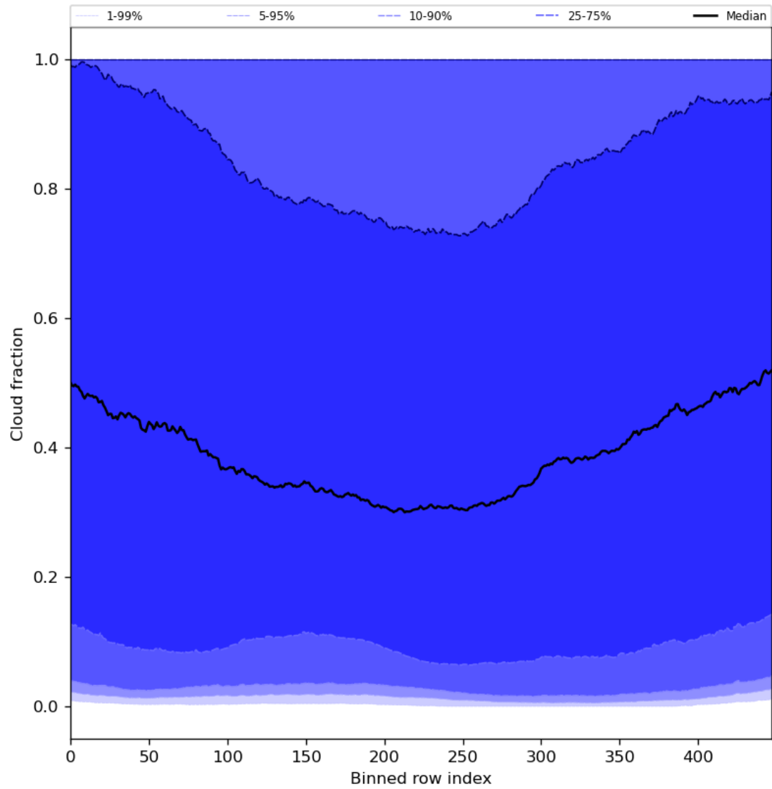
Figure 49: Along track statistics of “Cloud fraction” for 2024-04-23 to 2024-04-25
