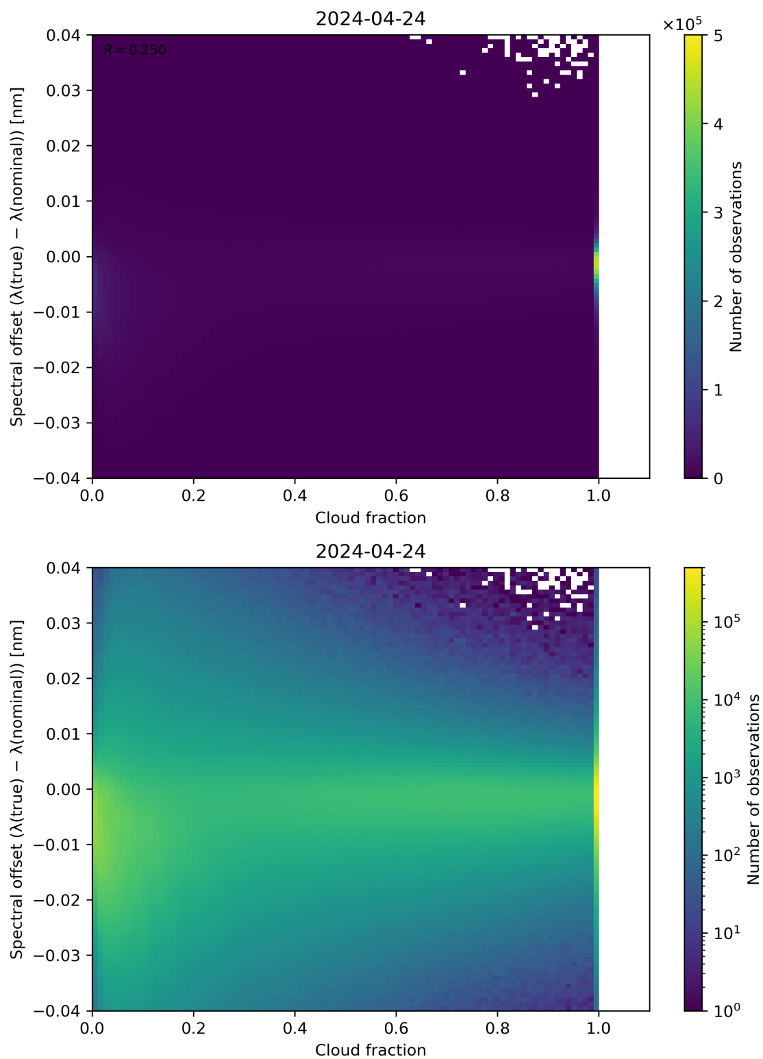
Figure 76: Scatter density plot of “Cloud fraction” against “Spectral offset ( \lambda(\text{true}) - \lambda(\text{nominal}) )” for 2024-04-23 to 2024-04-25.
