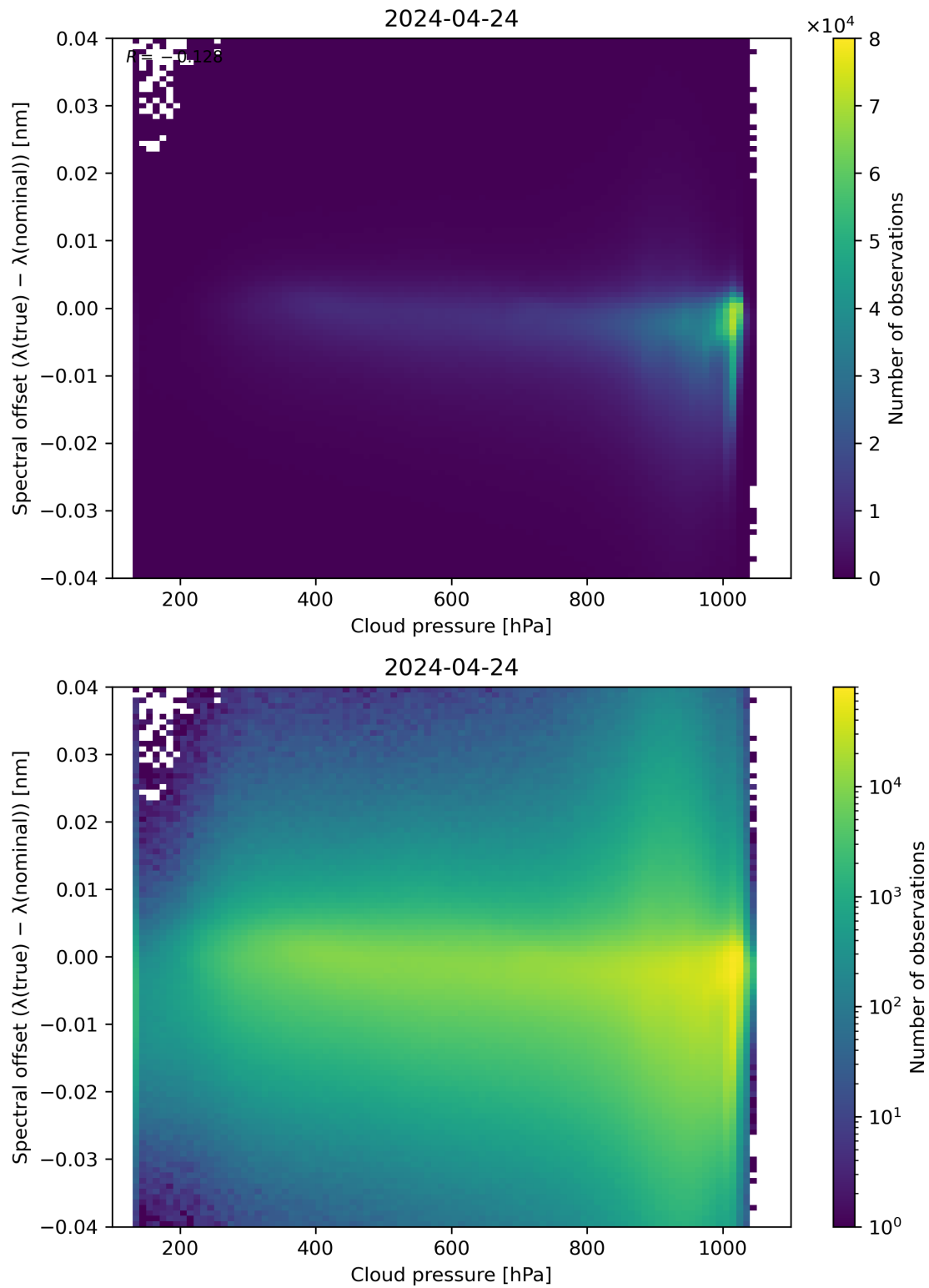
Figure 84: Scatter density plot of “Cloud pressure” against “Spectral offset ( \lambda(\text{true}) - \lambda(\text{nominal}) )” for 2024-04-23 to 2024-04-25.
