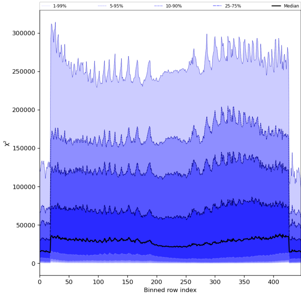
Figure 55: Along track statistics of “ \chi^2 ” for 2024-04-23 to 2024-04-25
