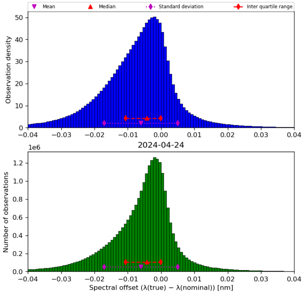
Figure 45: Histogram of “Spectral offset ( \lambda(\text{true}) - \lambda(\text{nominal}) )” for 2024-04-23 to 2024-04-25
