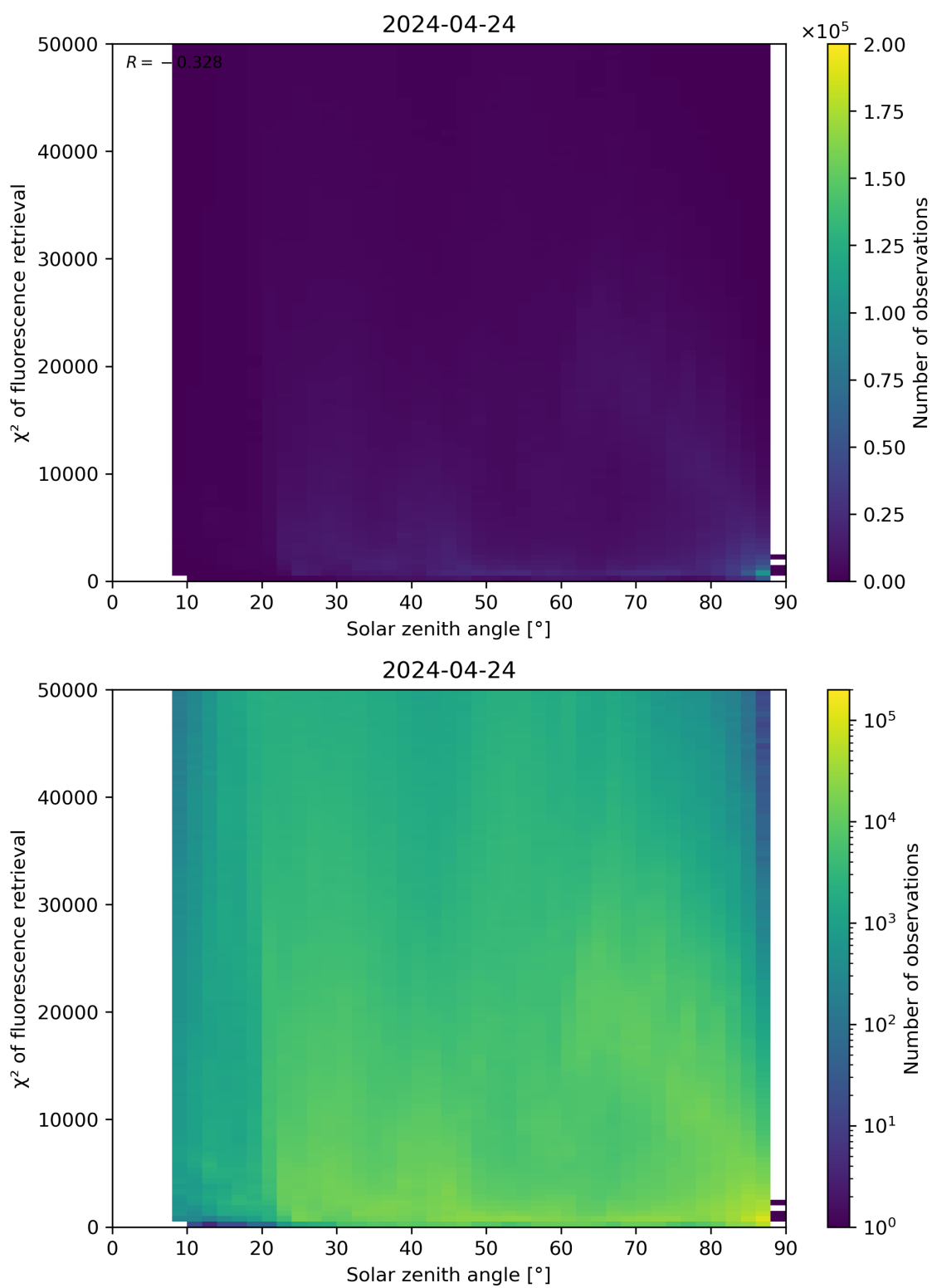
Figure 109: Scatter density plot of “Solar zenith angle” against “ \chi^2 of fluorescence retrieval” for 2024-04-23 to 2024-04-25.
