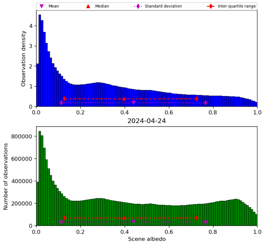
Figure 34: Histogram of “Scene albedo” for 2024-04-23 to 2024-04-25
