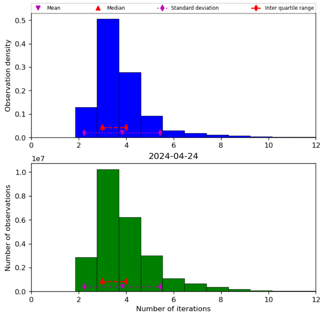
Figure 39: Histogram of “Number of iterations” for 2024-04-23 to 2024-04-25
