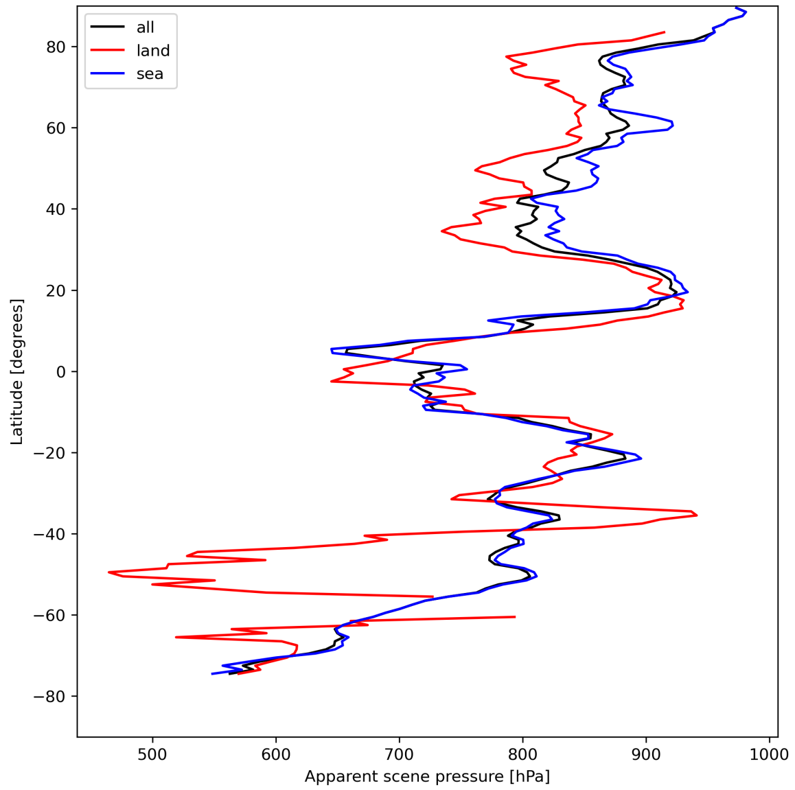
Figure 19: Zonal average of “Apparent scene pressure” for 2024-04-23 to 2024-04-25.
