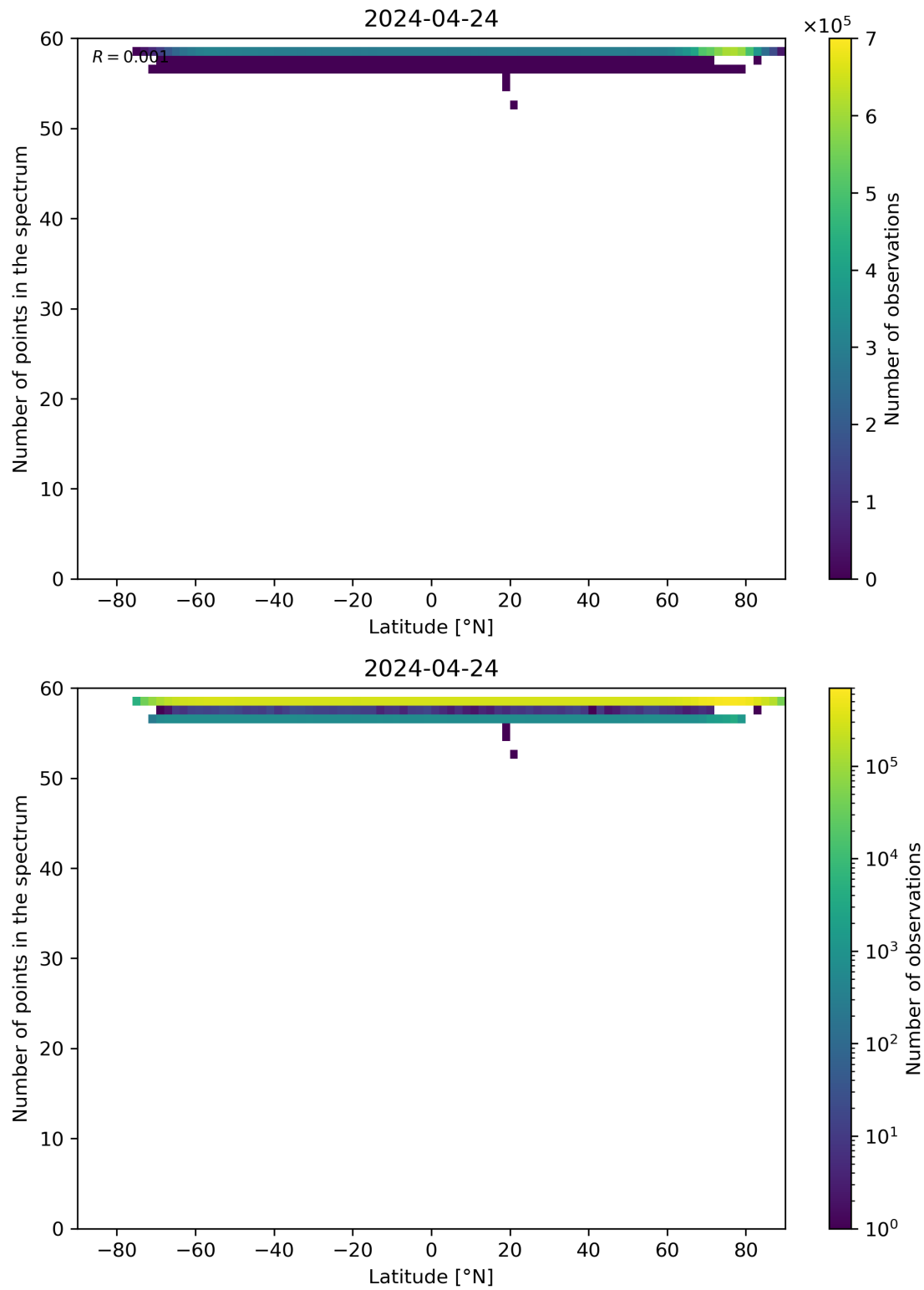
Figure 94: Scatter density plot of “Latitude” against “Number of points in the spectrum” for 2024-04-23 to 2024-04-25.
