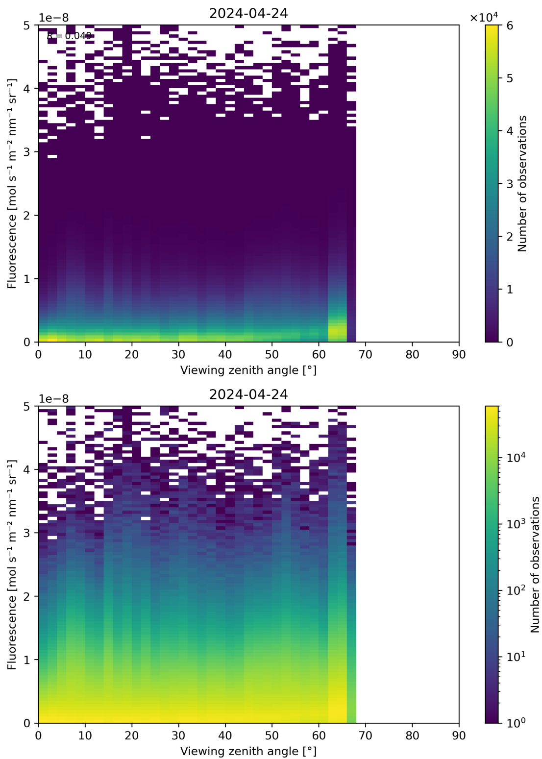
Figure 122: Scatter density plot of “Viewing zenith angle” against “Fluorescence” for 2024-04-23 to 2024-04-25.
