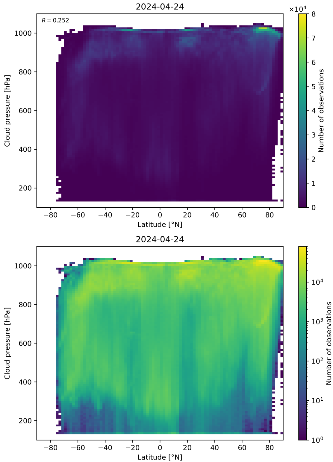
Figure 91: Scatter density plot of “Latitude” against “Cloud pressure” for 2024-04-23 to 2024-04-25.
