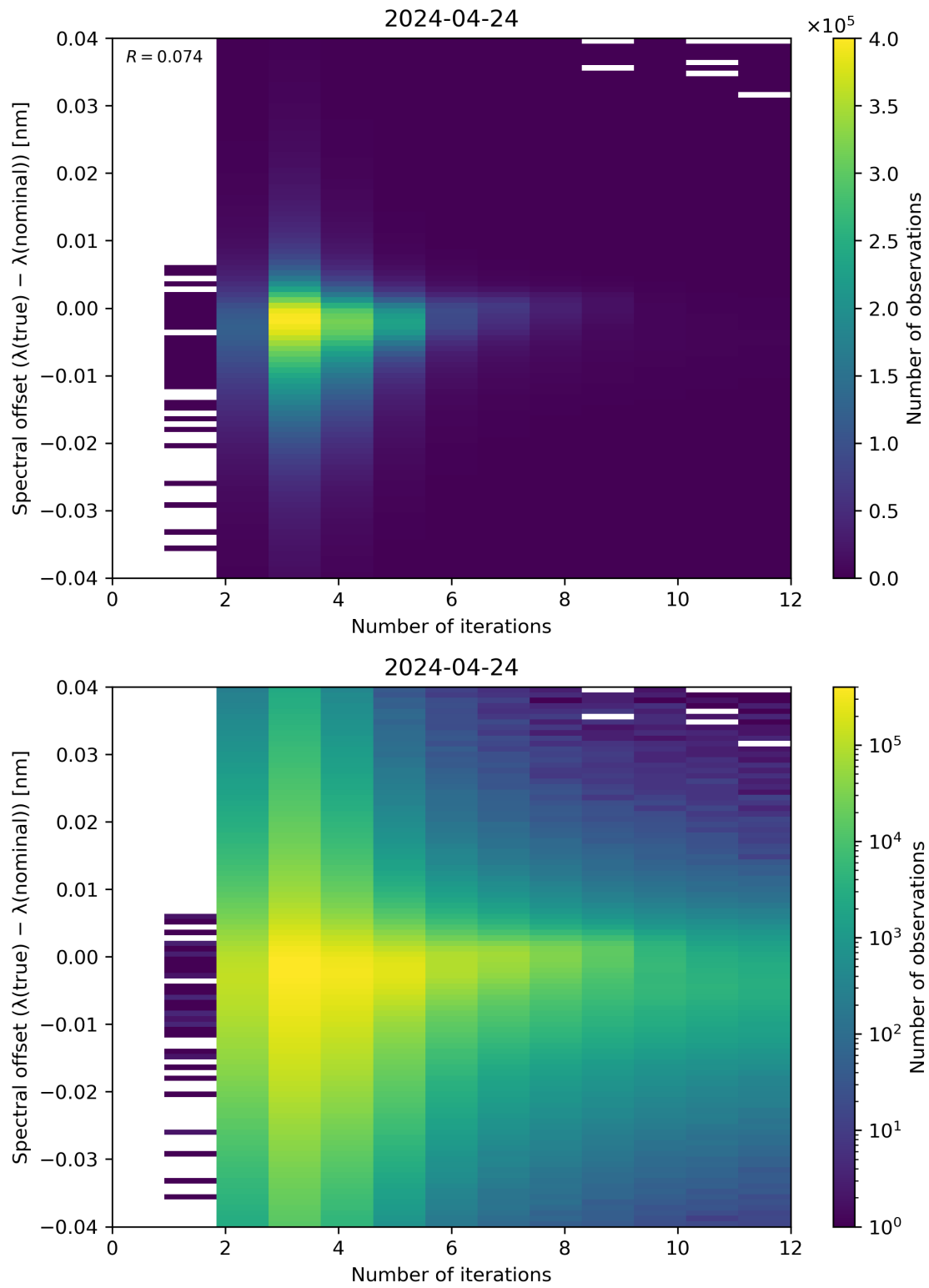
Figure 100: Scatter density plot of “Number of iterations” against “Spectral offset ( \lambda(\text{true}) - \lambda(\text{nominal}) )” for 2024-04-23 to 2024-04-25.
