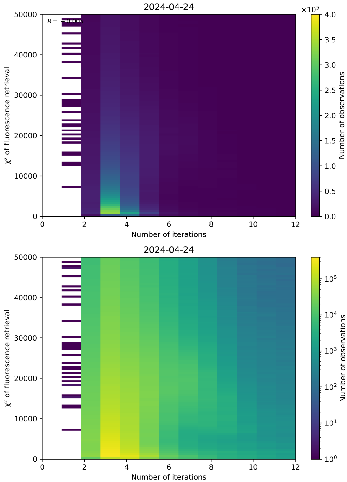
Figure 97: Scatter density plot of “Number of iterations” against “ \chi^2 of fluorescence retrieval” for 2024-04-23 to 2024-04-25.
