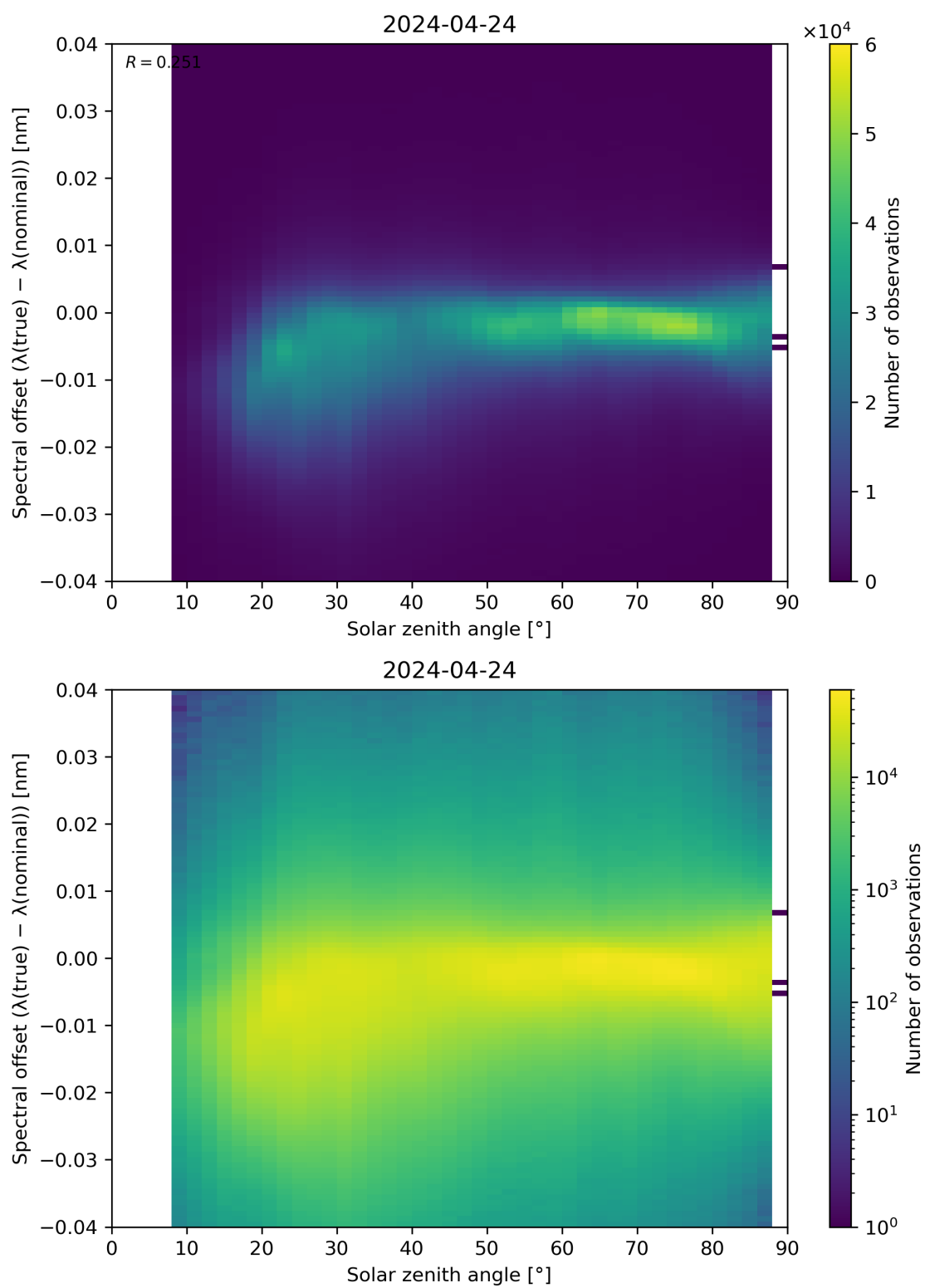
Figure 117: Scatter density plot of “Solar zenith angle” against “Spectral offset ( \lambda(\text{true}) - \lambda(\text{nominal}) )” for 2024-04-23 to 2024-04-25.
