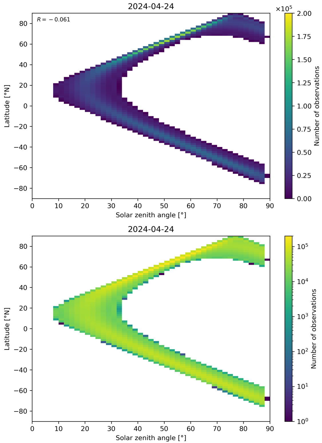
Figure 113: Scatter density plot of “Solar zenith angle” against “Latitude” for 2024-04-23 to 2024-04-25.
