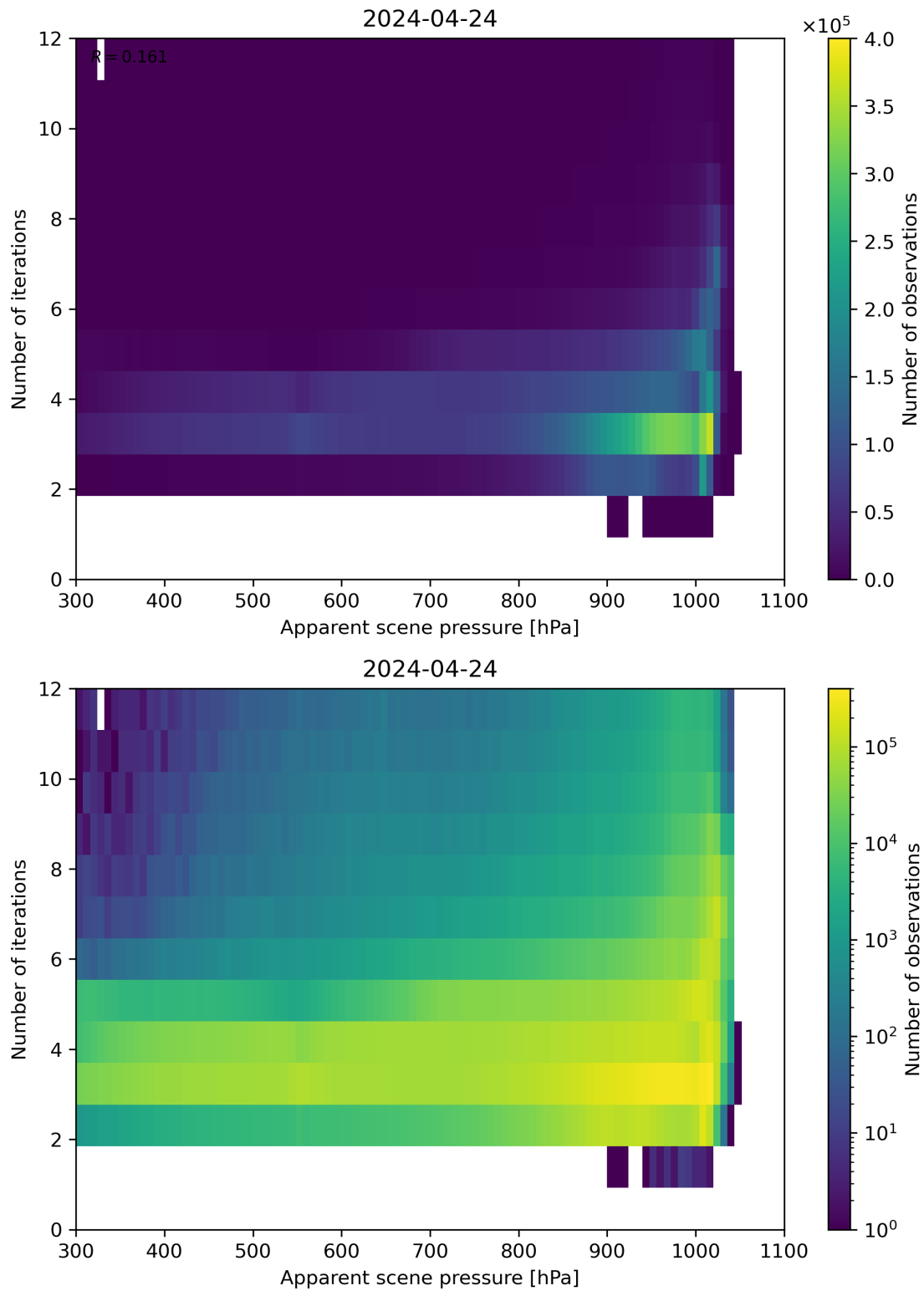
Figure 65: Scatter density plot of “Apparent scene pressure” against “Number of iterations” for 2024-04-23 to 2024-04-25.
