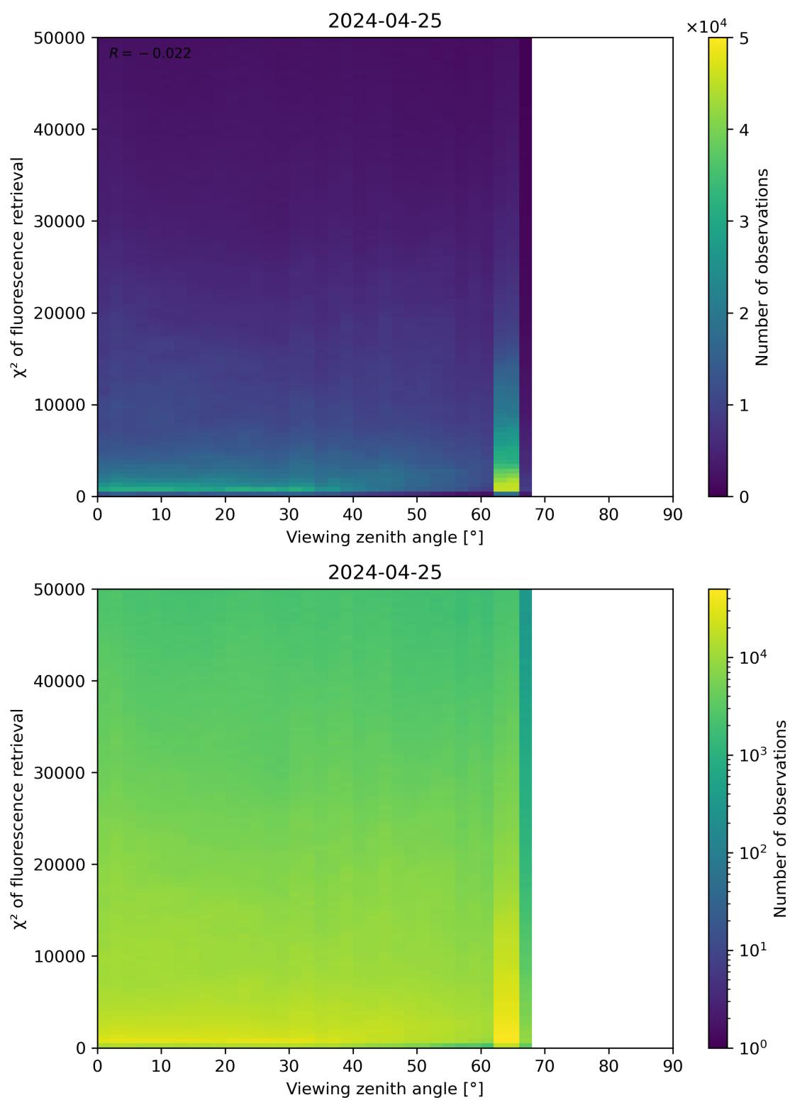
Figure 119: Scatter density plot of “Viewing zenith angle” against “ \chi^2 of fluorescence retrieval” for 2024-04-24 to 2024-04-26.
