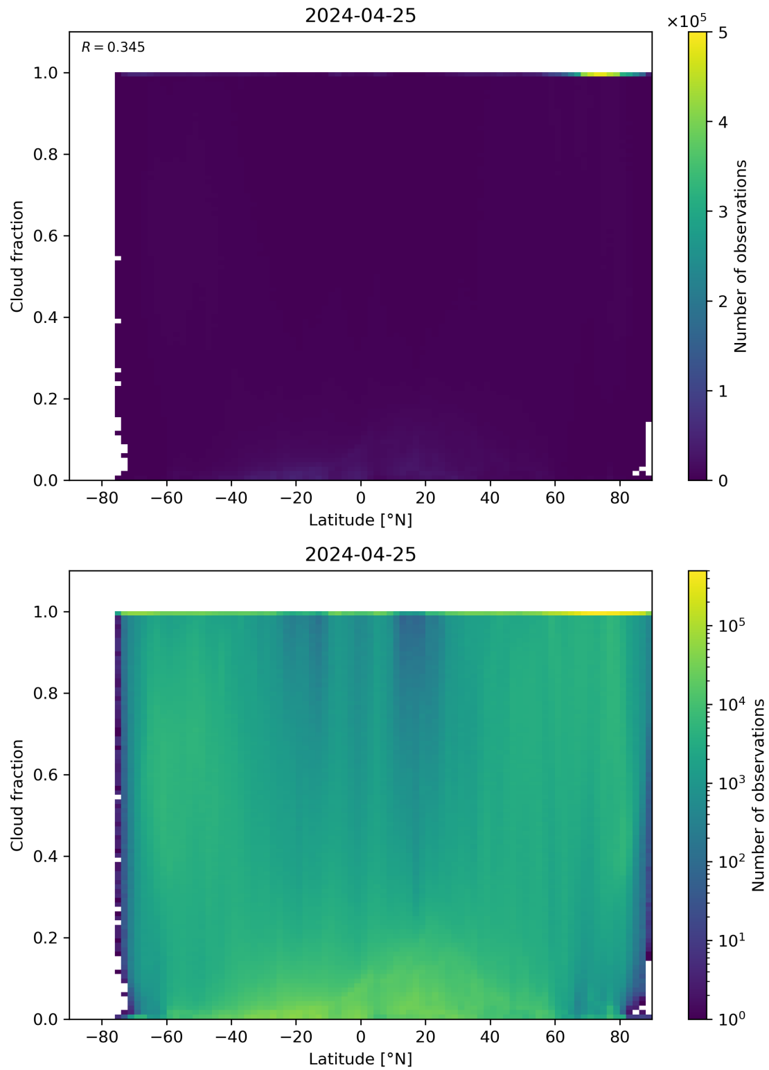
Figure 90: Scatter density plot of “Latitude” against “Cloud fraction” for 2024-04-24 to 2024-04-26.
