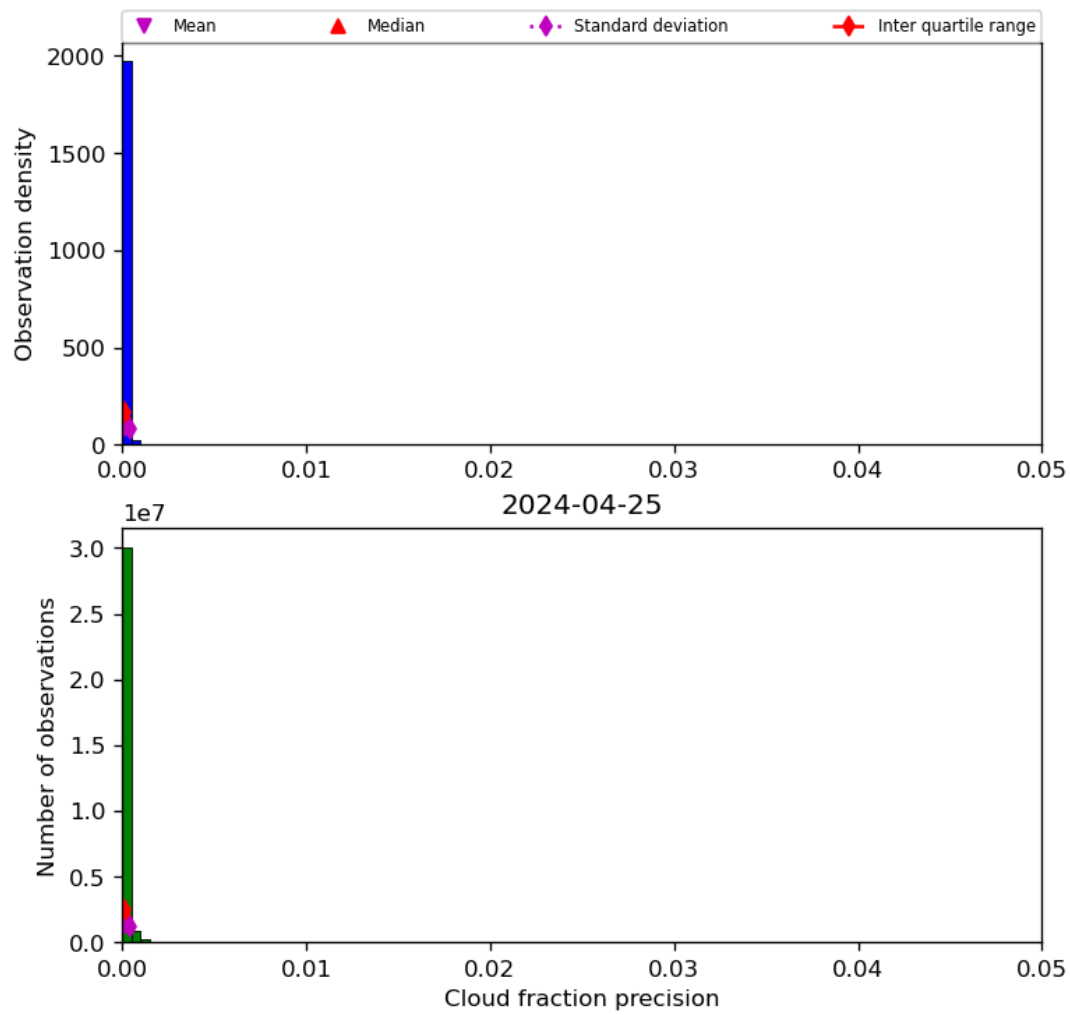
Figure 33: Histogram of “Cloud fraction precision” for 2024-04-24 to 2024-04-26
