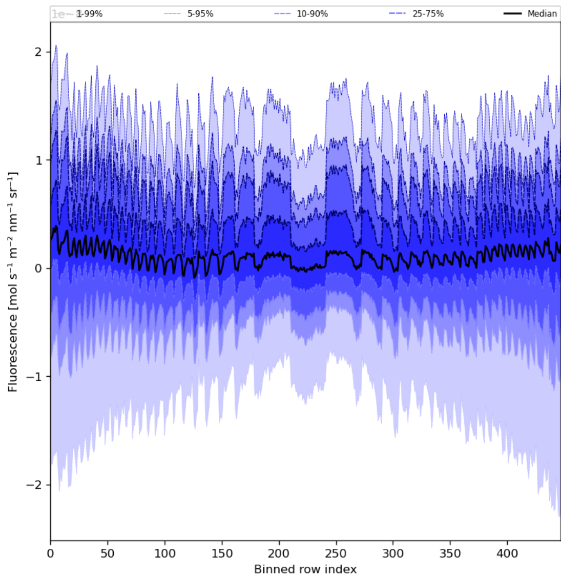
Figure 57: Along track statistics of “Fluorescence” for 2024-04-24 to 2024-04-26
