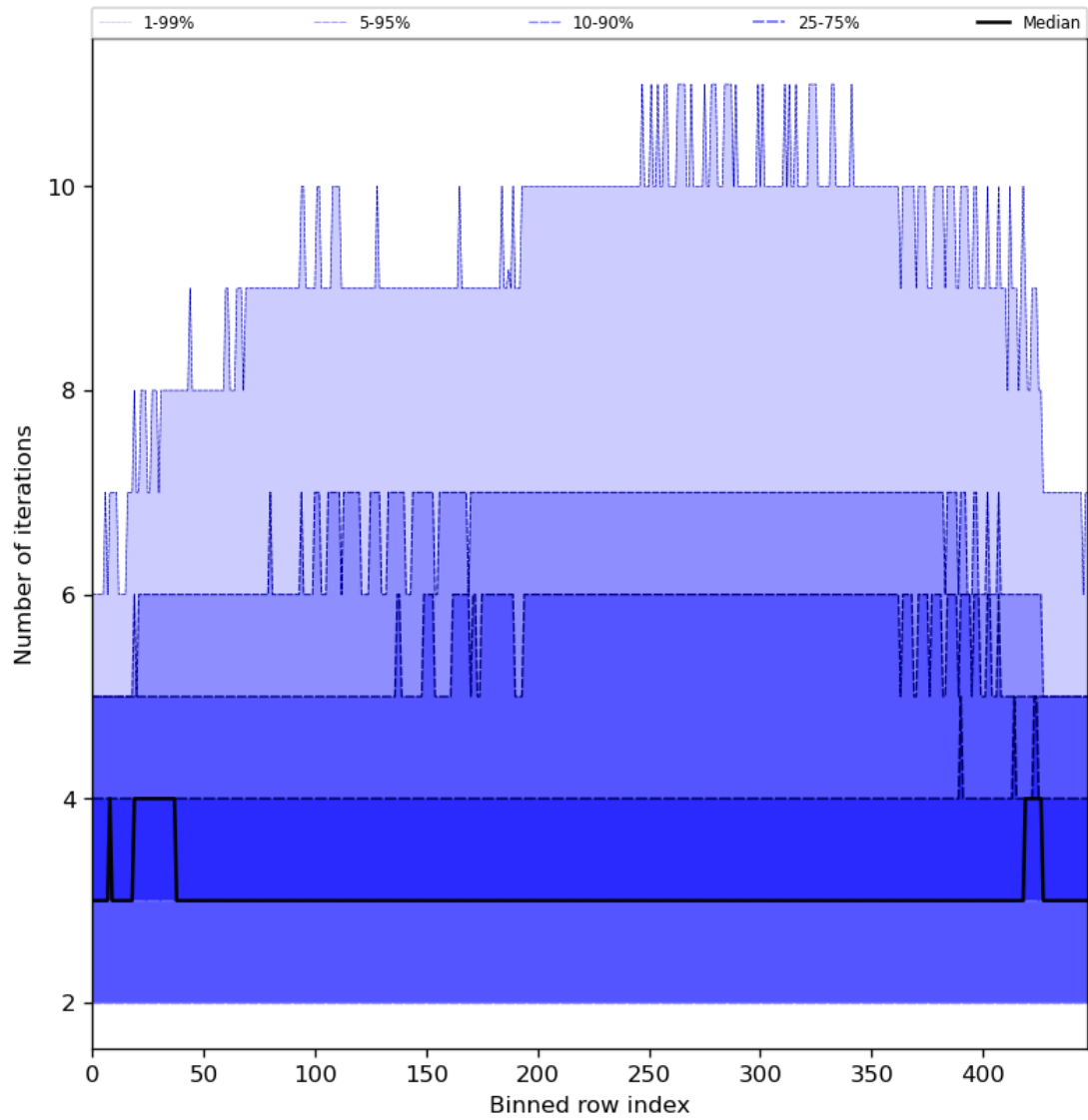
Figure 56: Along track statistics of “Number of iterations” for 2024-04-24 to 2024-04-26
