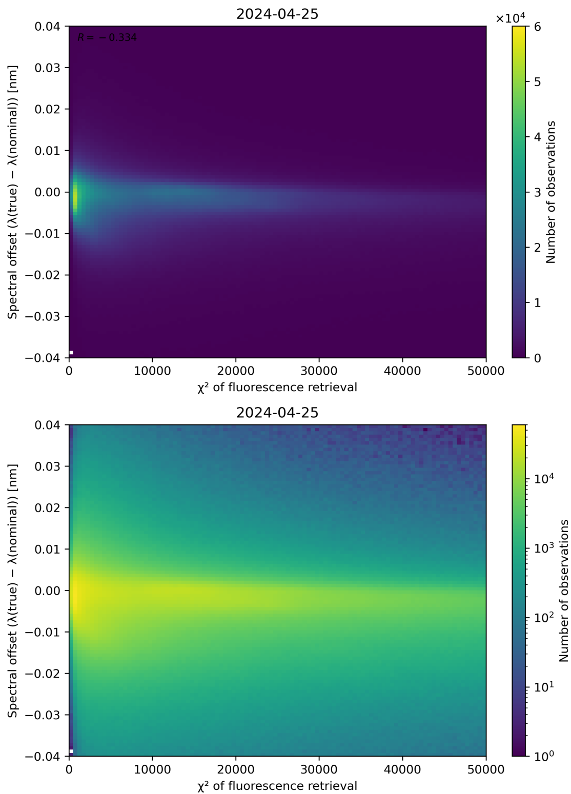
Figure 69: Scatter density plot of " \chi^2 of fluorescence retrieval" against "Spectral offset ( \lambda(\text{true}) - \lambda(\text{nominal}) )" for 2024-04-24 to 2024-04-26.
