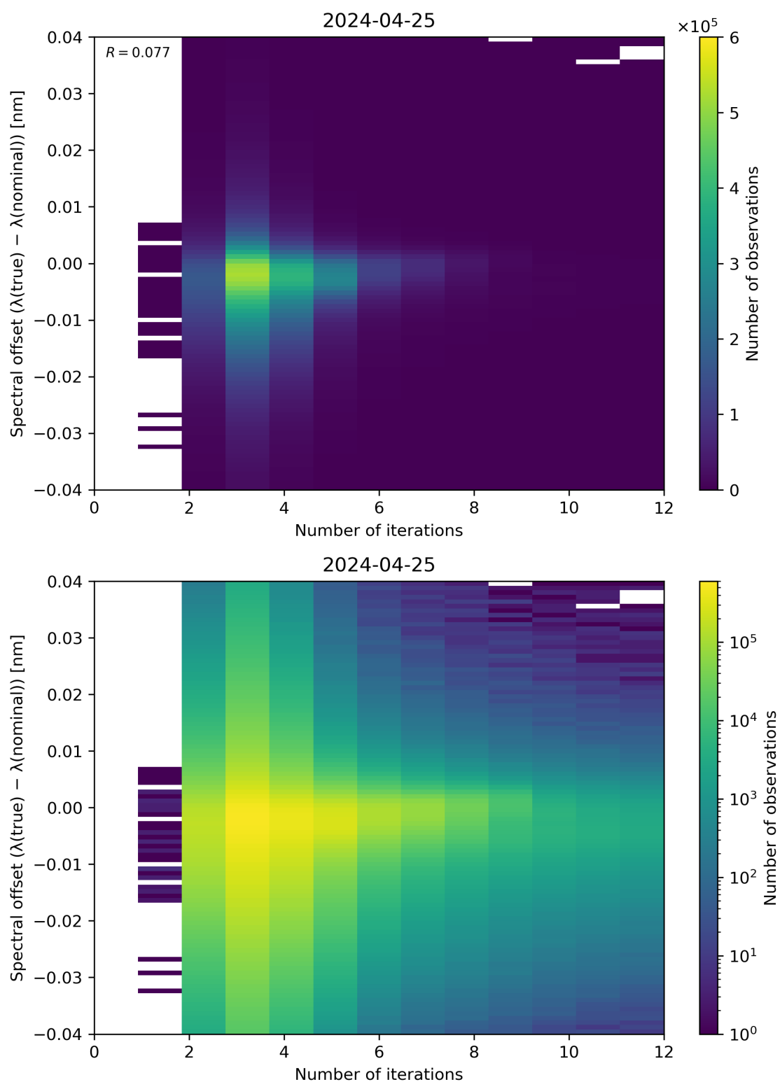
Figure 100: Scatter density plot of “Number of iterations” against “Spectral offset ( \lambda(\text{true}) - \lambda(\text{nominal}) )” for 2024-04-24 to 2024-04-26.
