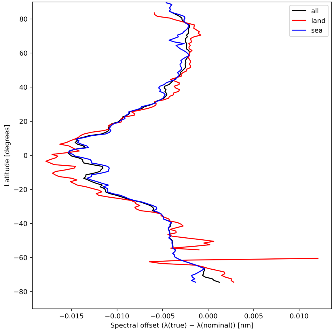
Figure 28: Zonal average of “Spectral offset ( \lambda(\text{true}) - \lambda(\text{nominal}) )” for 2024-04-24 to 2024-04-26.
