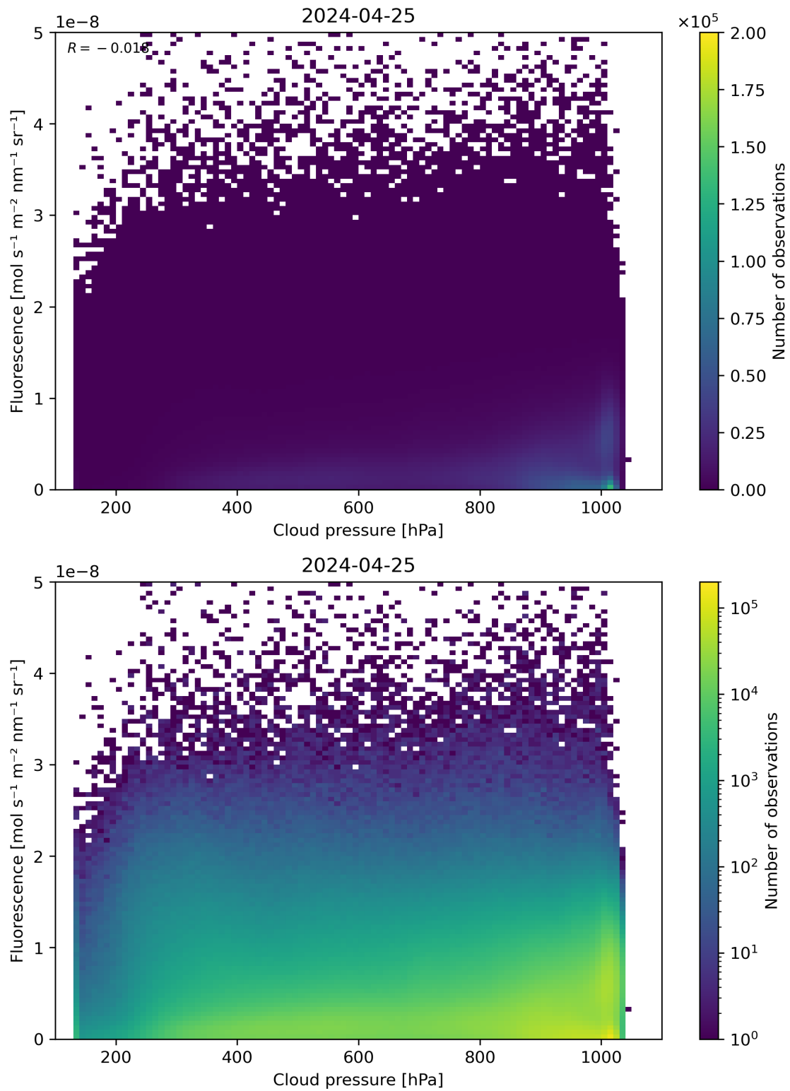
Figure 80: Scatter density plot of “Cloud pressure” against “Fluorescence” for 2024-04-24 to 2024-04-26.
