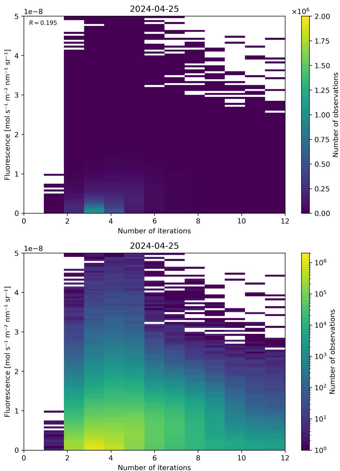
Figure 98: Scatter density plot of “Number of iterations” against “Fluorescence” for 2024-04-24 to 2024-04-26.
