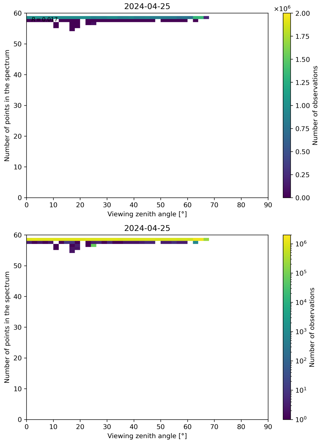
Figure 125: Scatter density plot of “Viewing zenith angle” against “Number of points in the spectrum” for 2024-04-24 to 2024-04-26.
