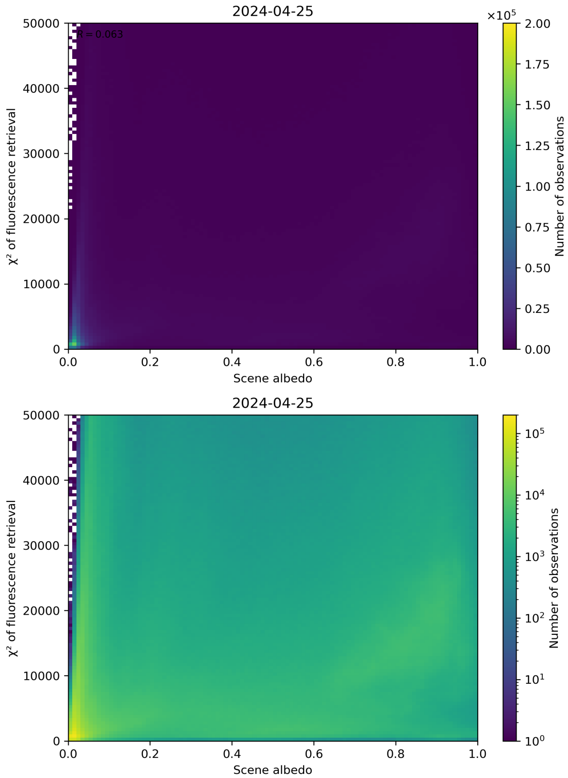
Figure 103: Scatter density plot of “Scene albedo” against “ \chi^2 of fluorescence retrieval” for 2024-04-24 to 2024-04-26.
