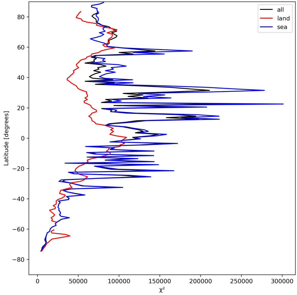
Figure 21: Zonal average of “ \chi^2 ” for 2024-04-24 to 2024-04-26.
