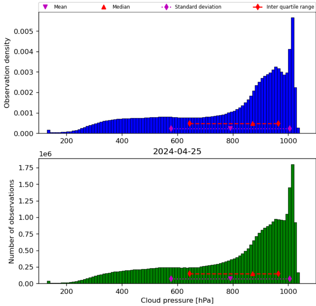
Figure 30: Histogram of “Cloud pressure” for 2024-04-24 to 2024-04-26
