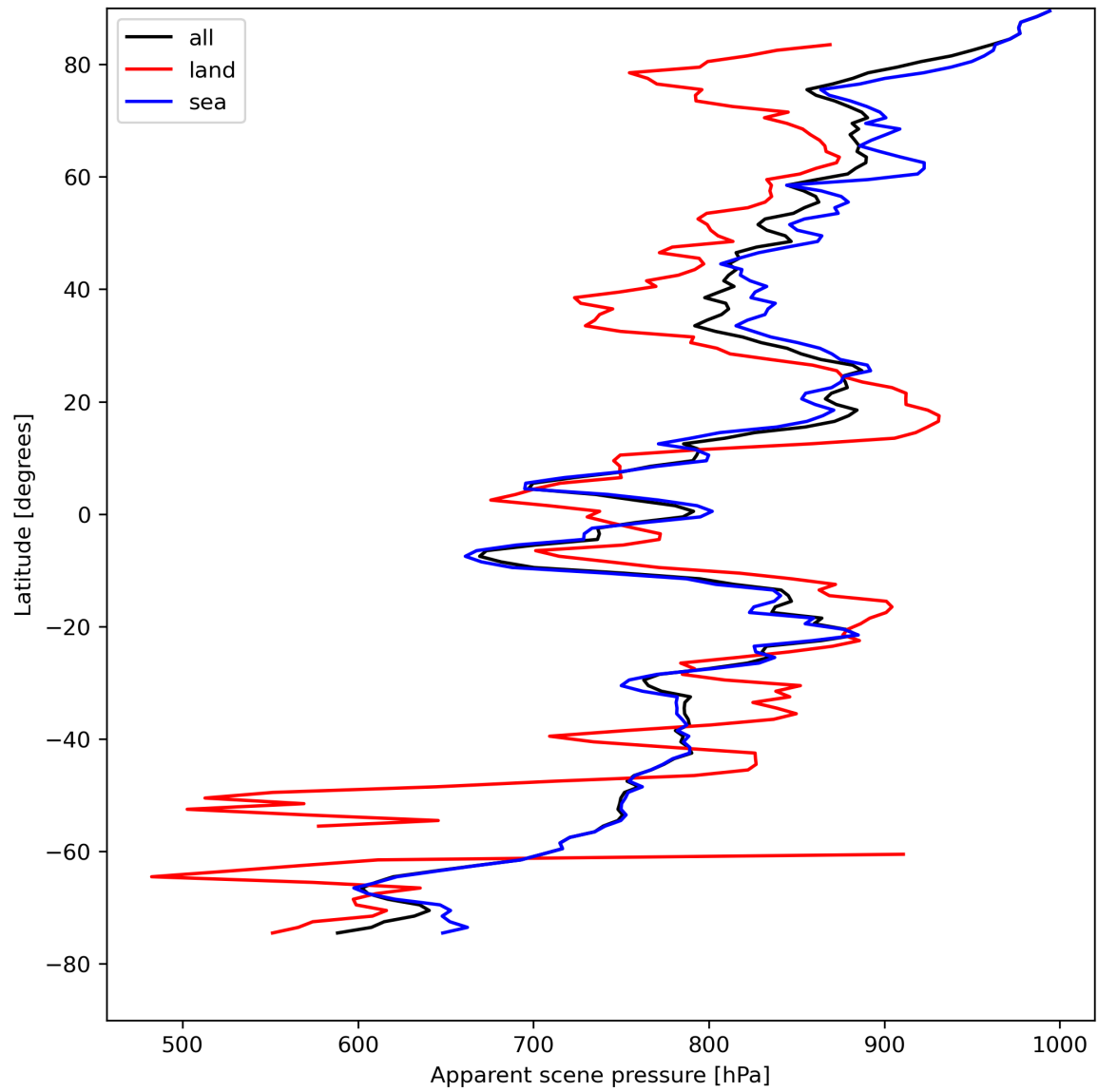
Figure 19: Zonal average of “Apparent scene pressure” for 2024-04-24 to 2024-04-26.
