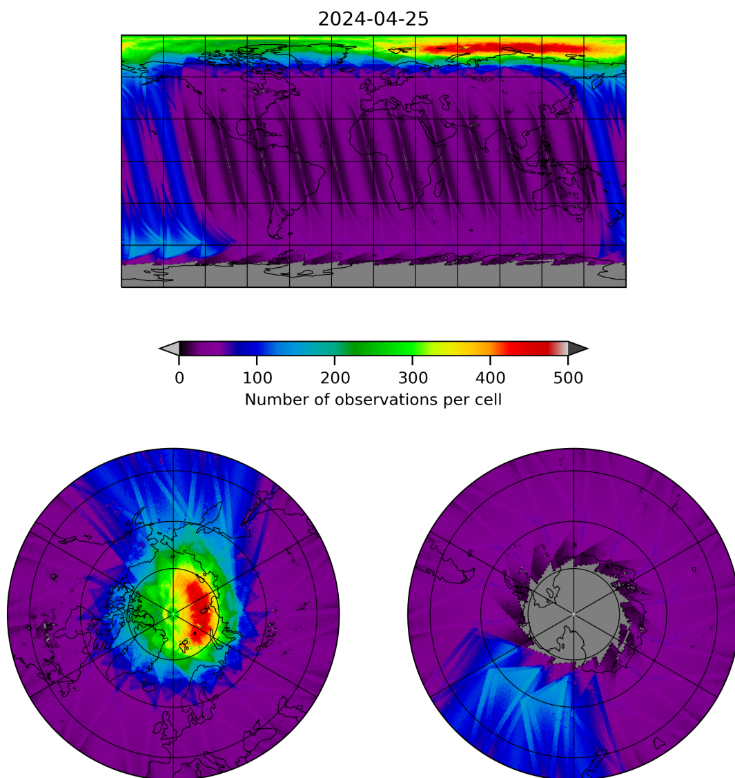
Figure 11: Map of the number of observations for 2024-04-24 to 2024-04-26
