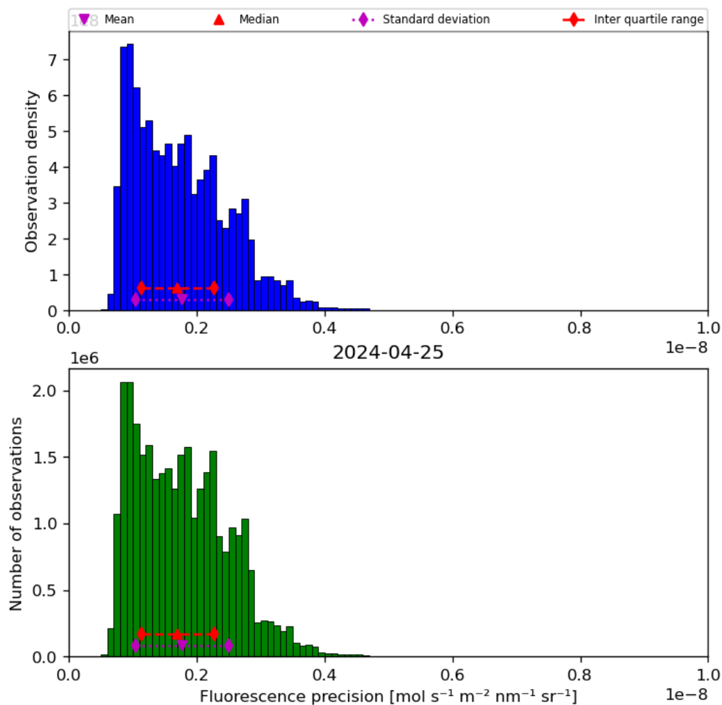
Figure 41: Histogram of “Fluorescence precision” for 2024-04-24 to 2024-04-26
