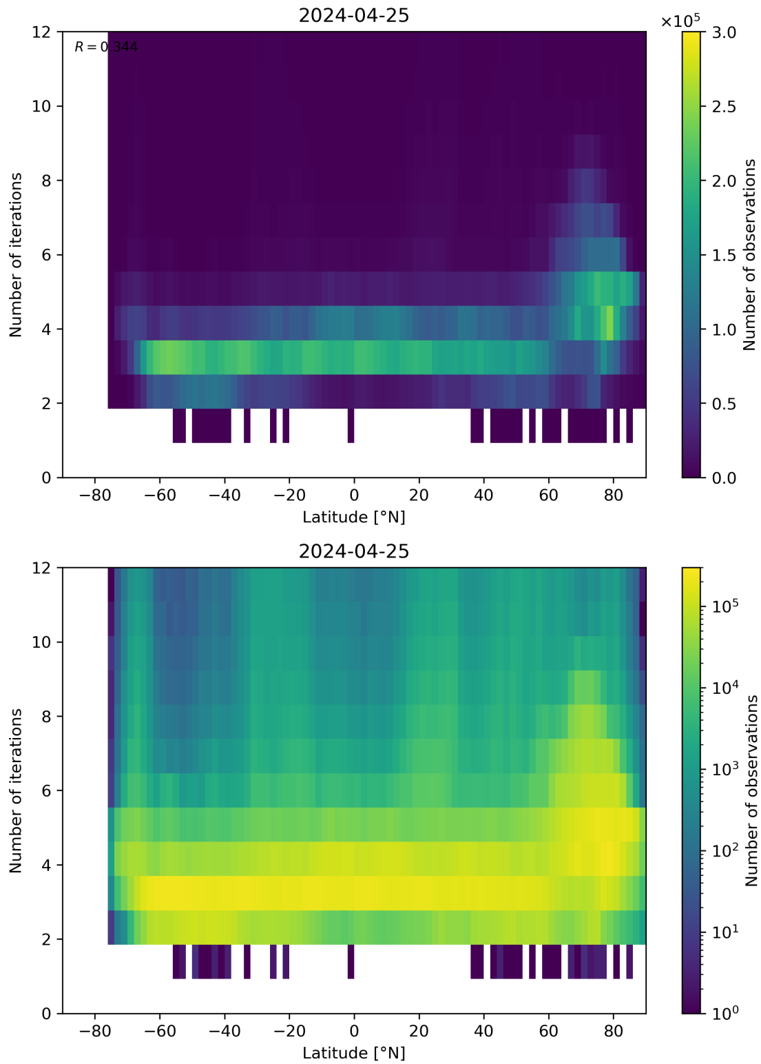
Figure 93: Scatter density plot of “Latitude” against “Number of iterations” for 2024-04-24 to 2024-04-26.
