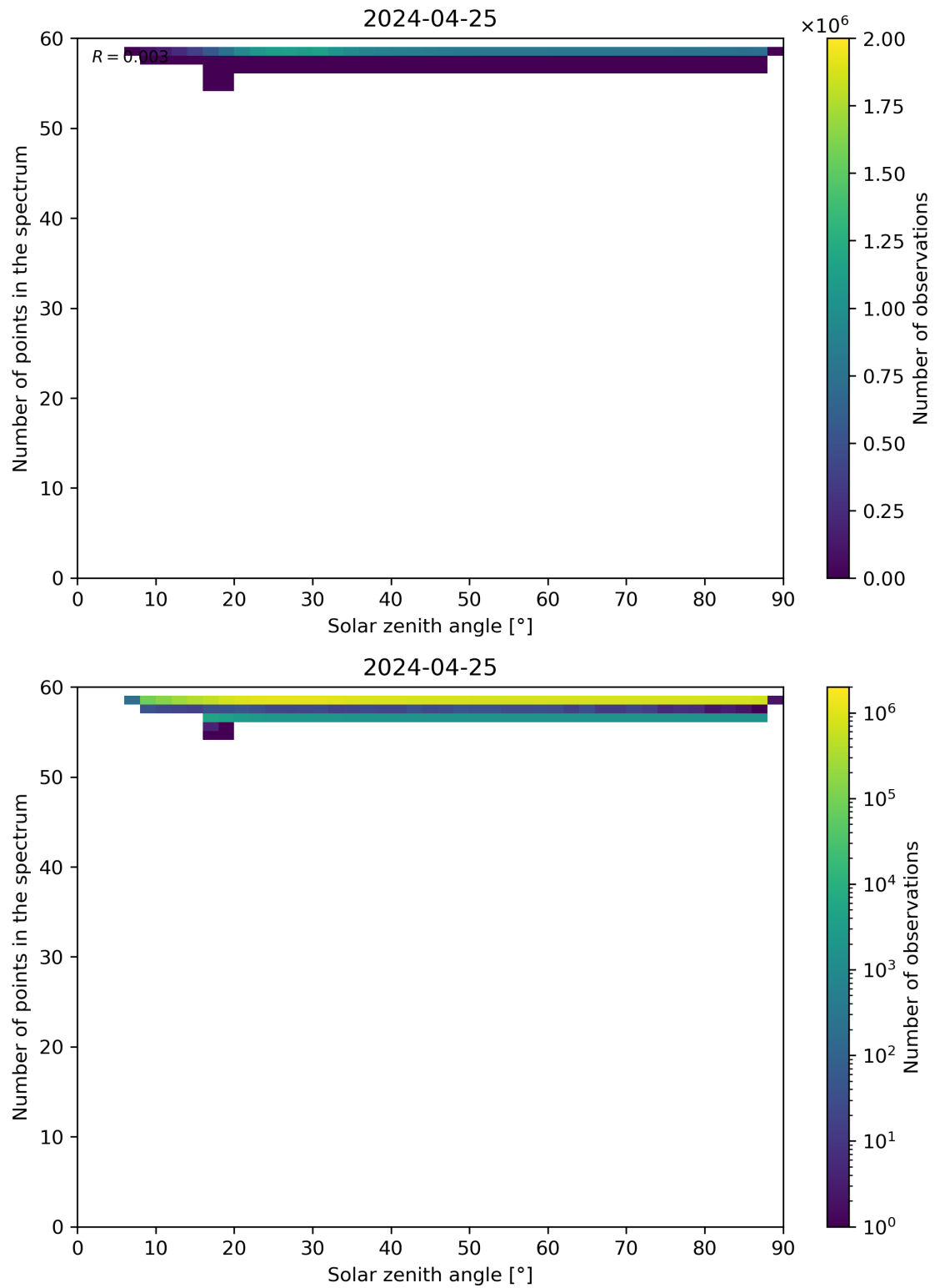
Figure 115: Scatter density plot of “Solar zenith angle” against “Number of points in the spectrum” for 2024-04-24 to 2024-04-26.
