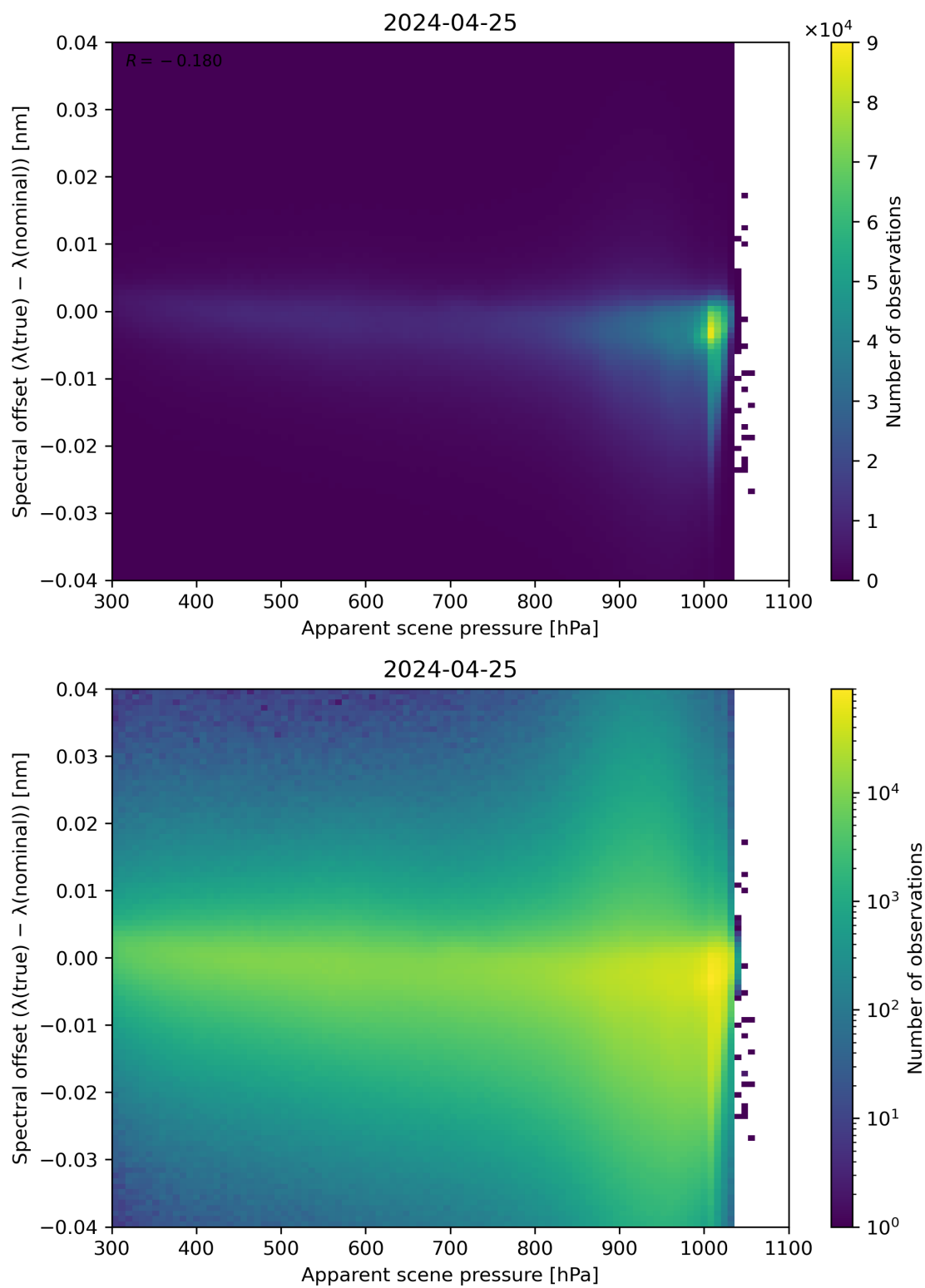
Figure 67: Scatter density plot of “Apparent scene pressure” against “Spectral offset ( \lambda(\text{true}) - \lambda(\text{nominal}) )” for 2024-04-24 to 2024-04-26.
