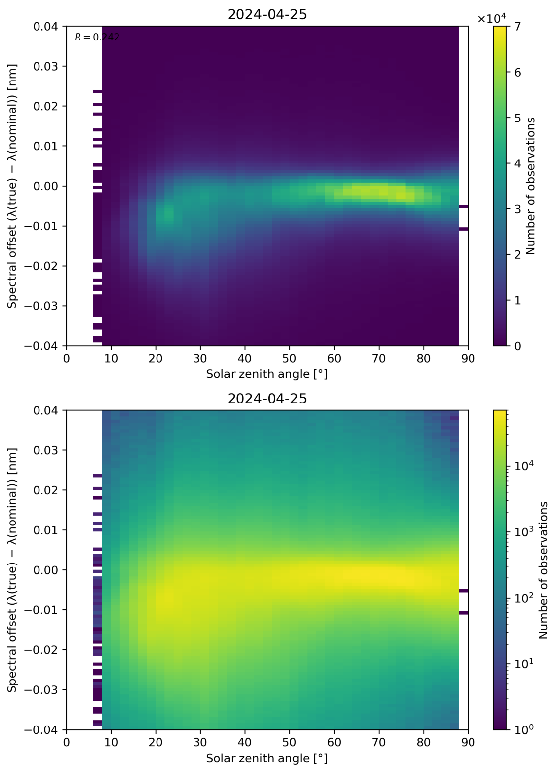
Figure 117: Scatter density plot of “Solar zenith angle” against “Spectral offset ( \lambda(\text{true}) - \lambda(\text{nominal}) )” for 2024-04-24 to 2024-04-26.
