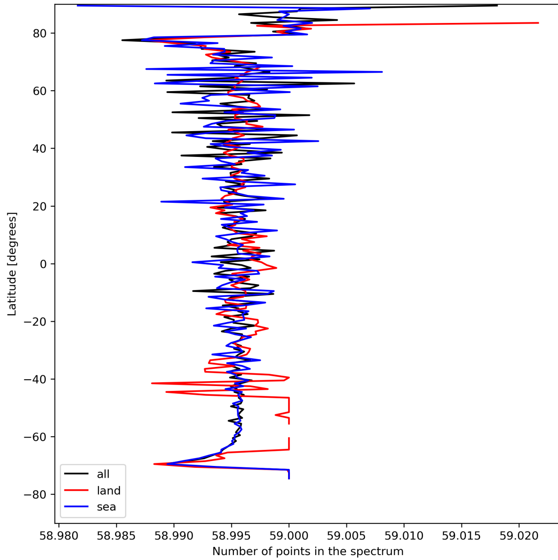
Figure 27: Zonal average of “Number of points in the spectrum” for 2024-04-24 to 2024-04-26.
