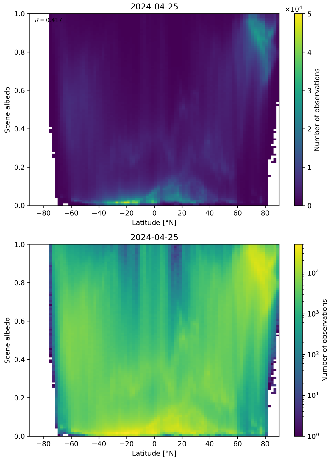
Figure 95: Scatter density plot of “Latitude” against “Scene albedo” for 2024-04-24 to 2024-04-26.
