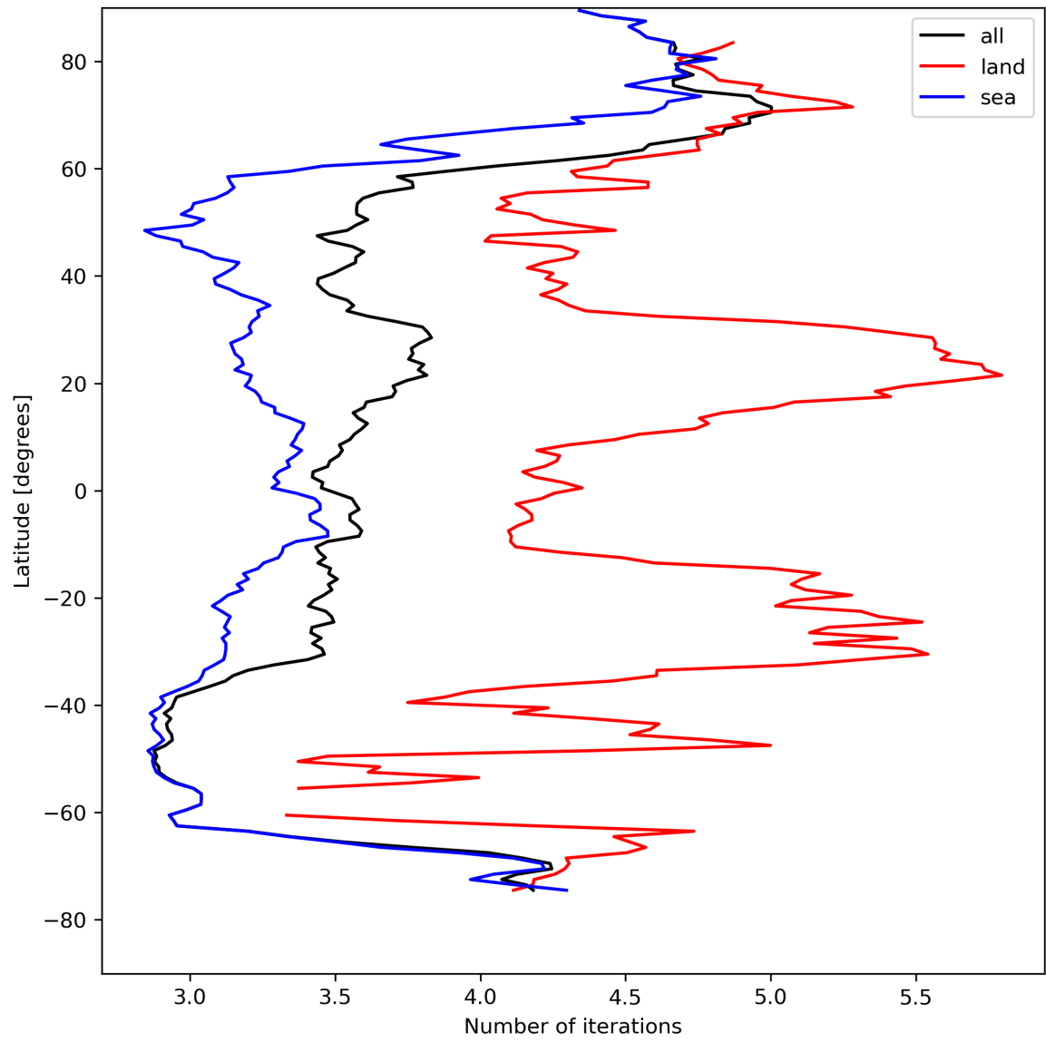
Figure 22: Zonal average of “Number of iterations” for 2024-04-24 to 2024-04-26.
