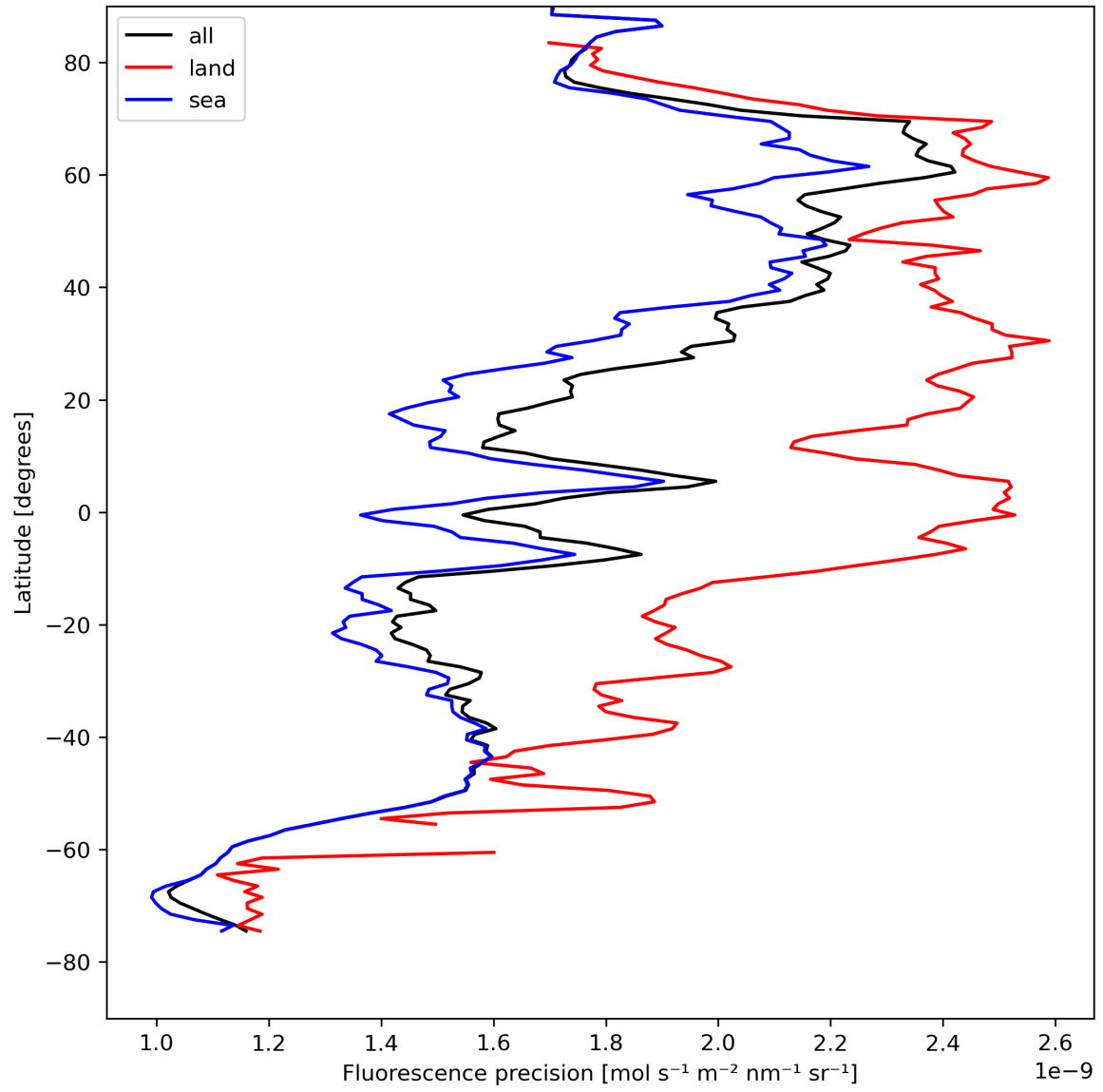
Figure 24: Zonal average of “Fluorescence precision” for 2024-04-24 to 2024-04-26.
