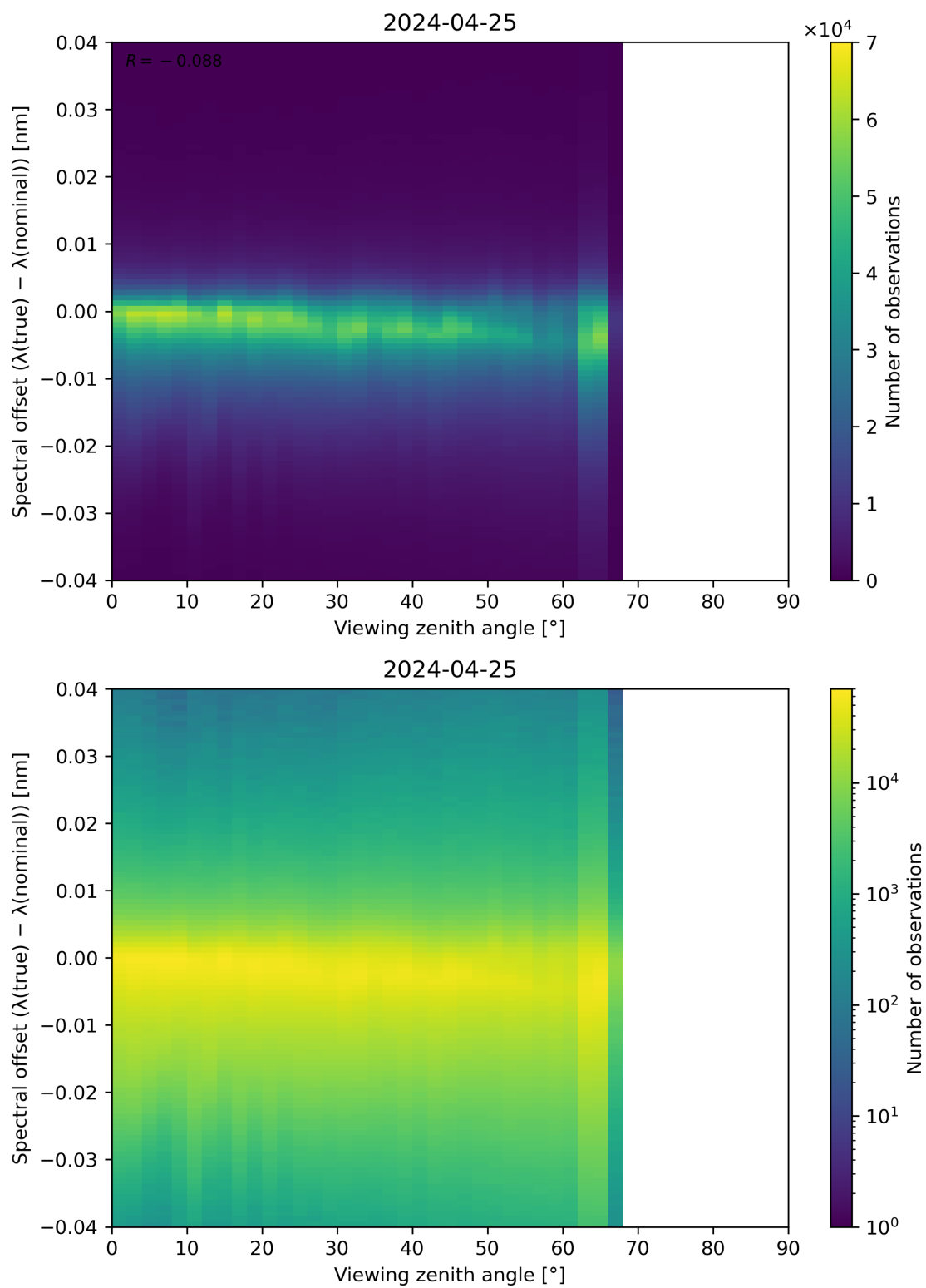
Figure 128: Scatter density plot of “Viewing zenith angle” against “Spectral offset ( \lambda(\text{true}) - \lambda(\text{nominal}) )” for 2024-04-24 to 2024-04-26.
