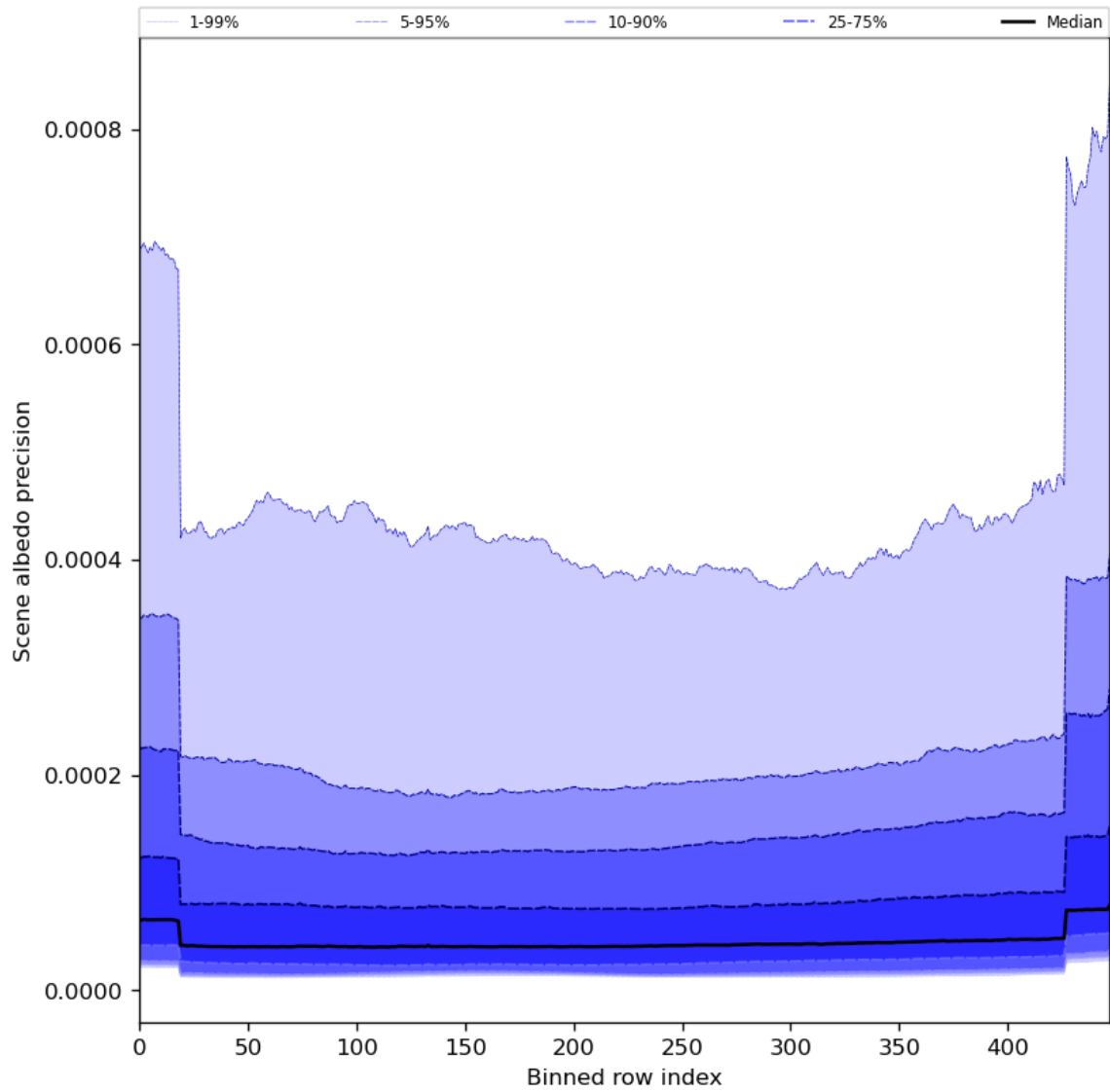
Figure 52: Along track statistics of “Scene albedo precision” for 2024-04-24 to 2024-04-26
