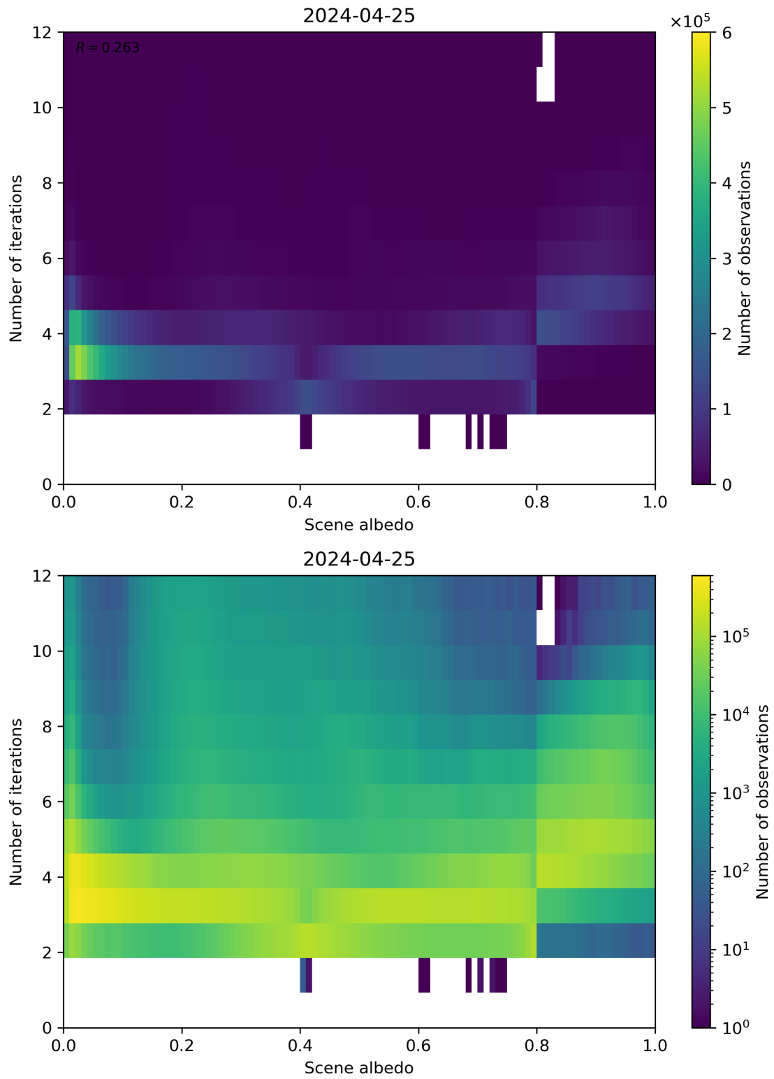
Figure 105: Scatter density plot of “Scene albedo” against “Number of iterations” for 2024-04-24 to 2024-04-26.
