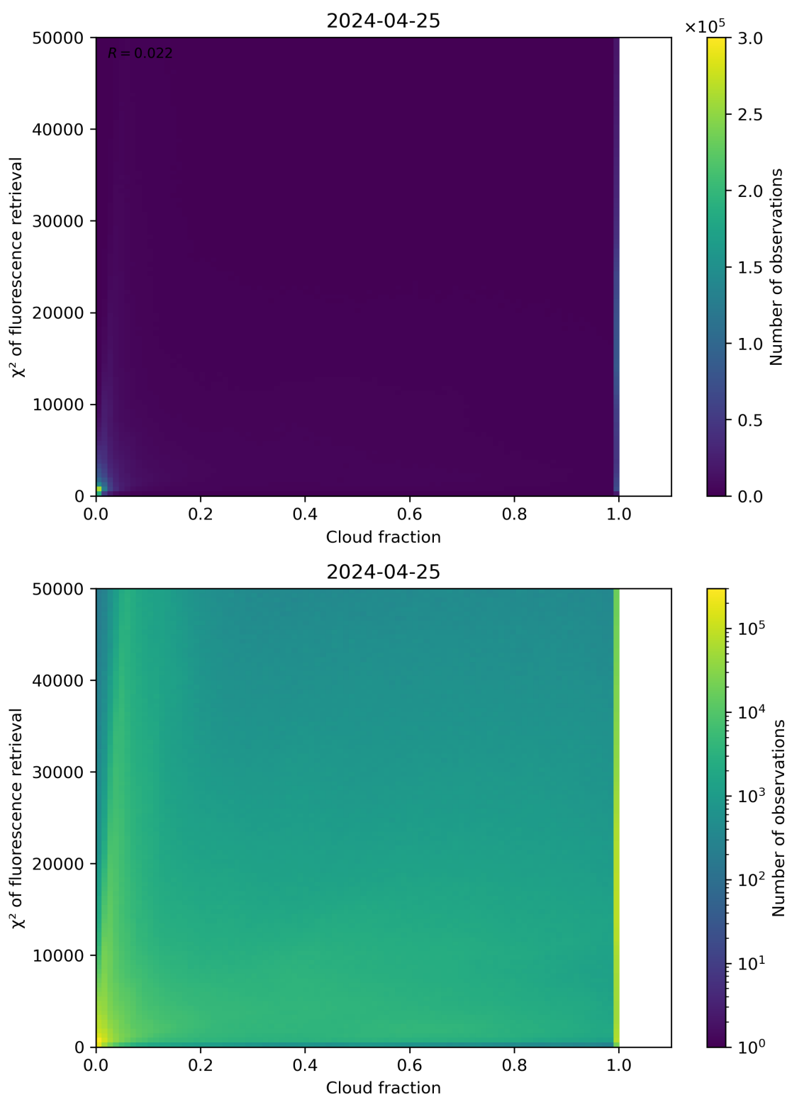
Figure 71: Scatter density plot of “Cloud fraction” against “ \chi^2 of fluorescence retrieval” for 2024-04-24 to 2024-04-26.
