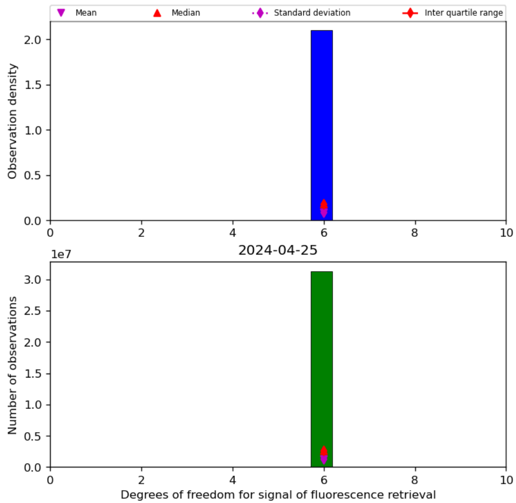
Figure 43: Histogram of "Degrees of freedom for signal of fluorescence retrieval" for 2024-04-24 to 2024-04-26
