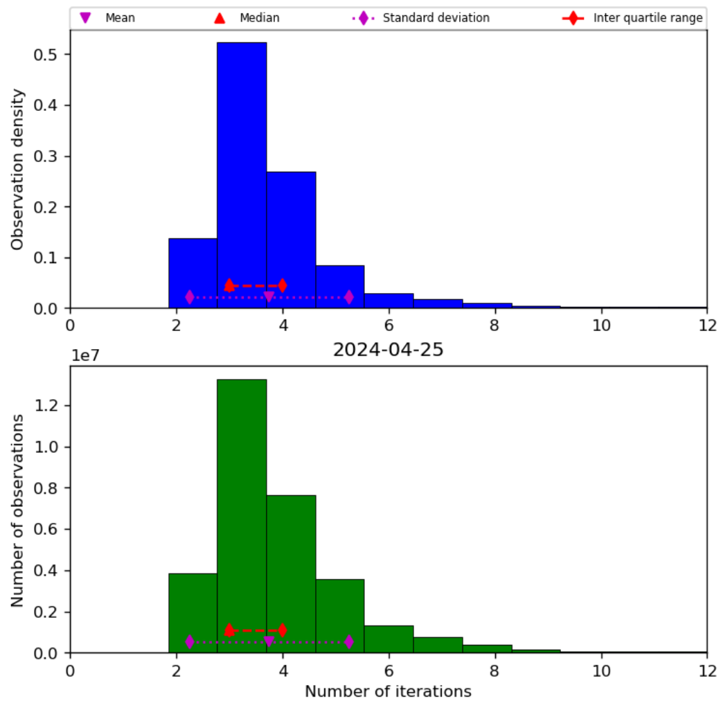
Figure 39: Histogram of “Number of iterations” for 2024-04-24 to 2024-04-26
