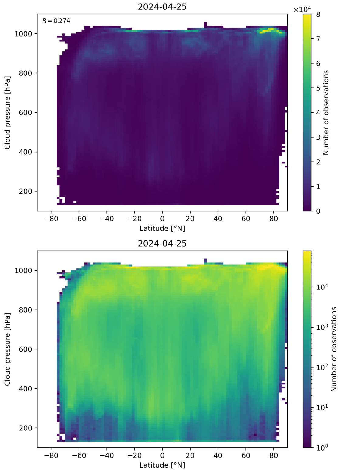
Figure 91: Scatter density plot of “Latitude” against “Cloud pressure” for 2024-04-24 to 2024-04-26.
