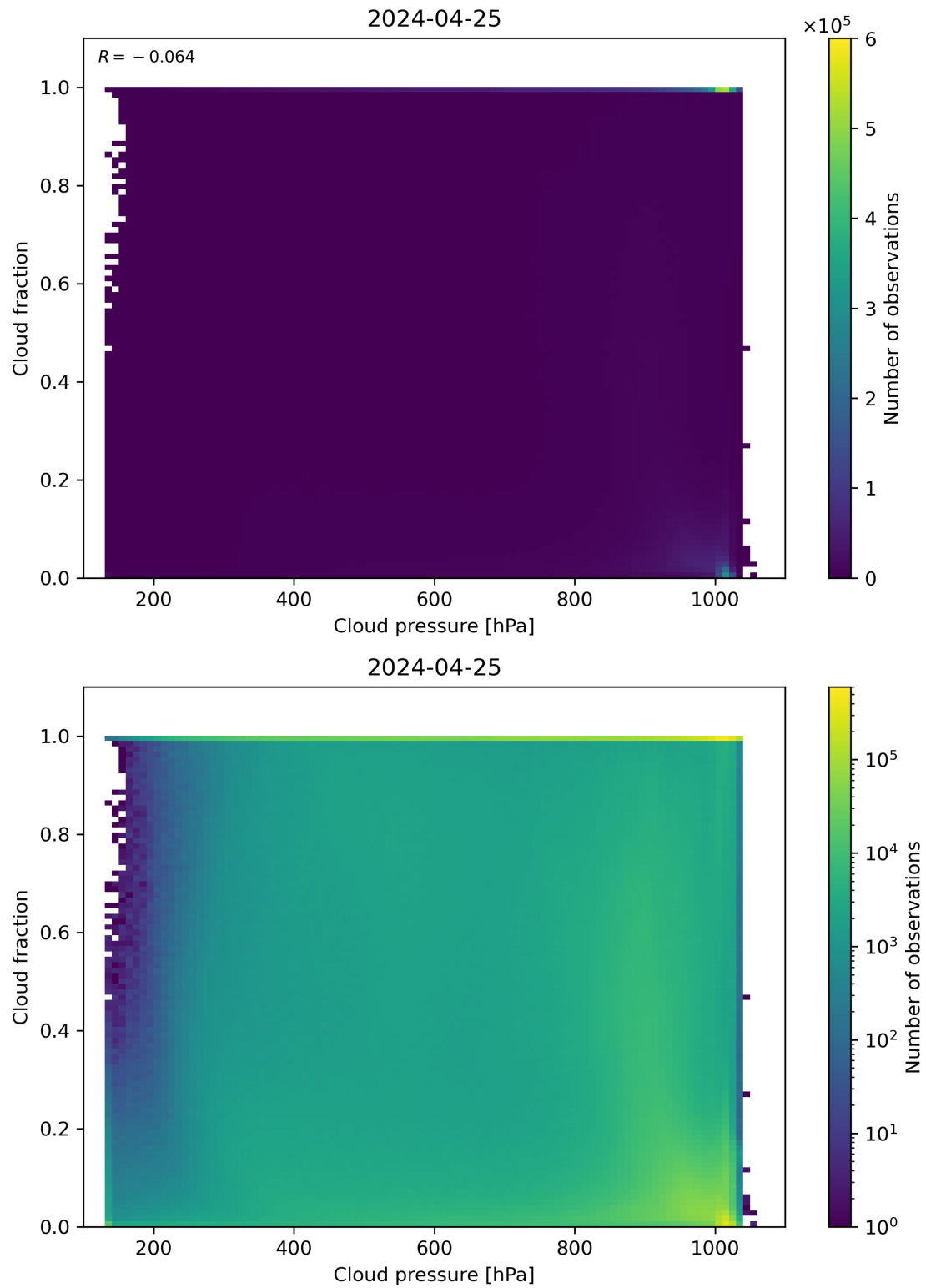
Figure 79: Scatter density plot of “Cloud pressure” against “Cloud fraction” for 2024-04-24 to 2024-04-26.
