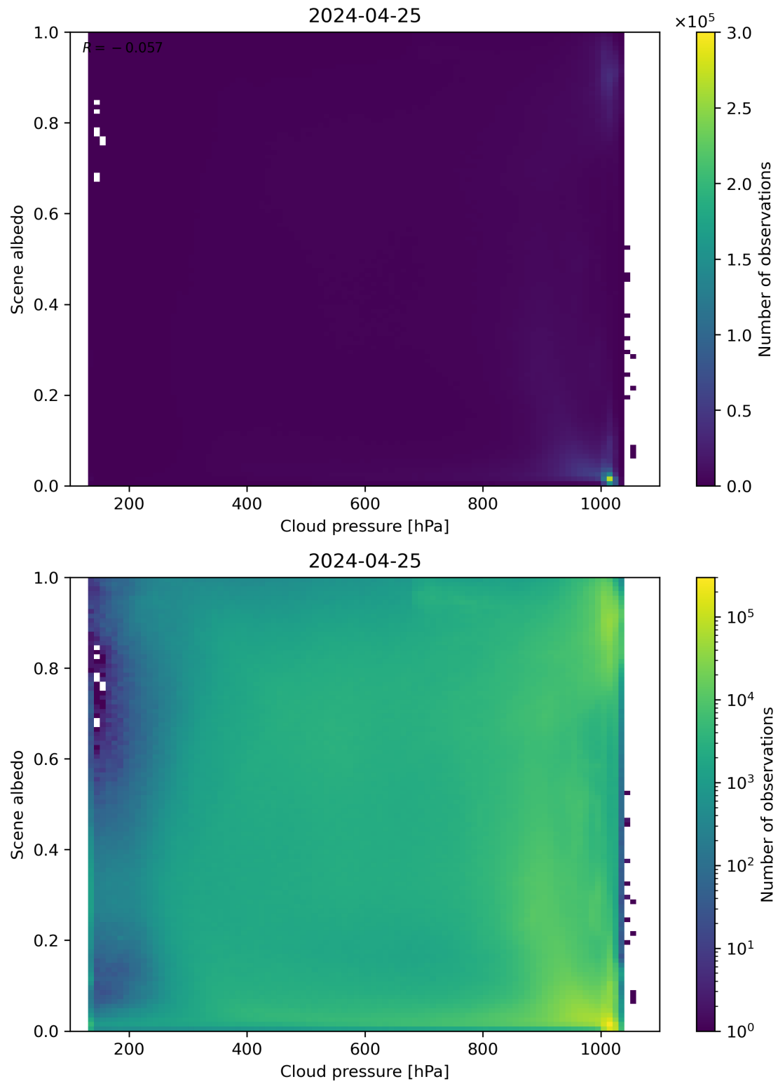
Figure 83: Scatter density plot of “Cloud pressure” against “Scene albedo” for 2024-04-24 to 2024-04-26.
