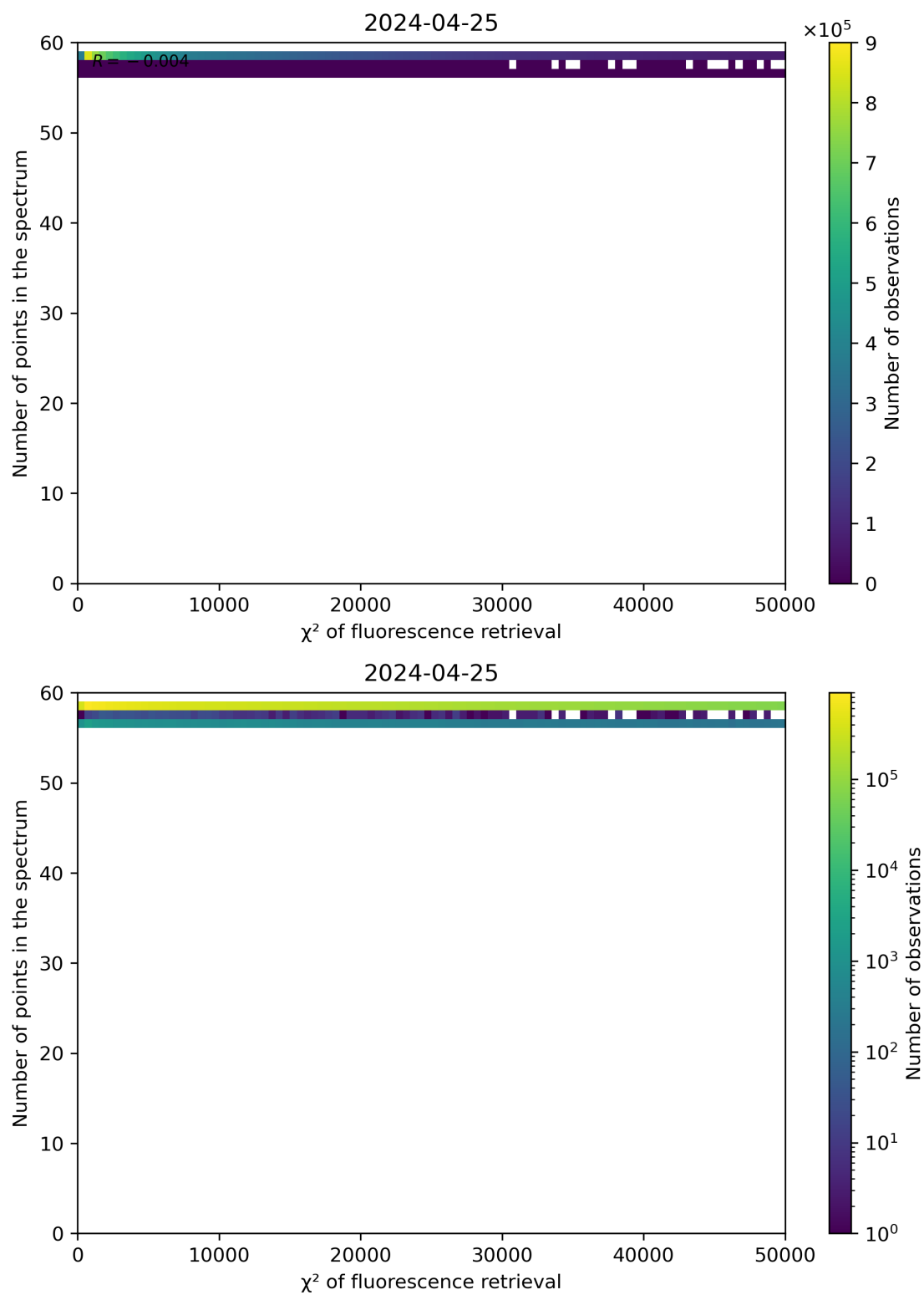
Figure 68: Scatter density plot of " \chi^2 of fluorescence retrieval" against "Number of points in the spectrum" for 2024-04-24 to 2024-04-26.
