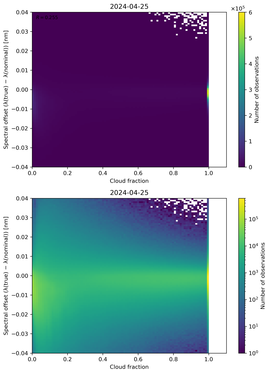
Figure 76: Scatter density plot of “Cloud fraction” against “Spectral offset ( \lambda(\text{true}) - \lambda(\text{nominal}) )” for 2024-04-24 to 2024-04-26.
