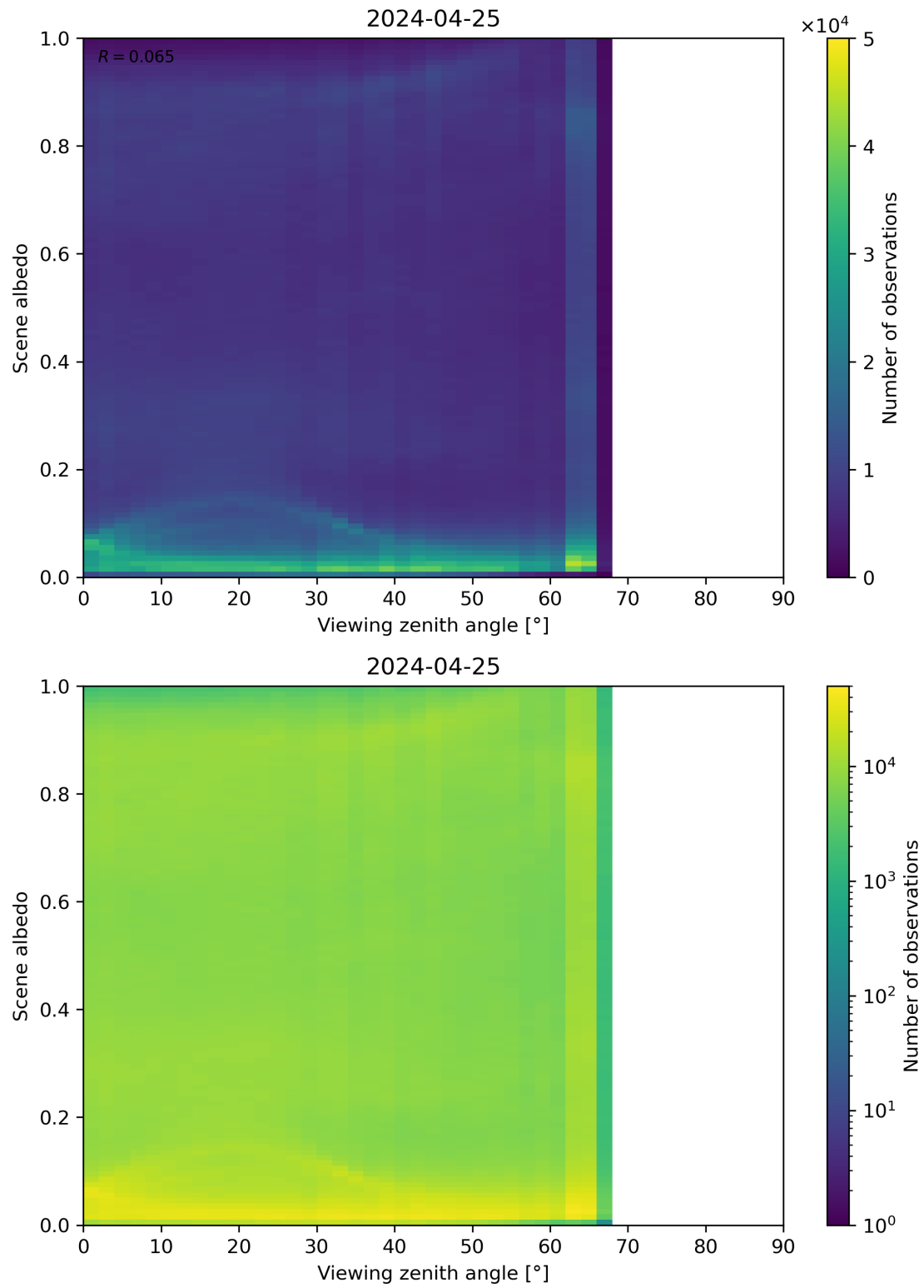
Figure 126: Scatter density plot of “Viewing zenith angle” against “Scene albedo” for 2024-04-24 to 2024-04-26.
