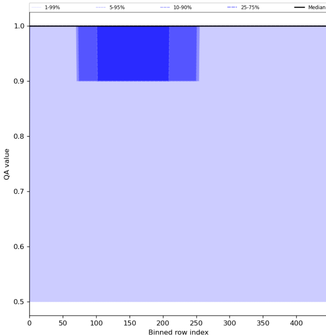
Figure 46: Along track statistics of “QA value” for 2024-04-24 to 2024-04-26
