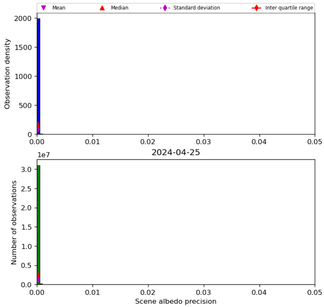
Figure 35: Histogram of “Scene albedo precision” for 2024-04-24 to 2024-04-26
