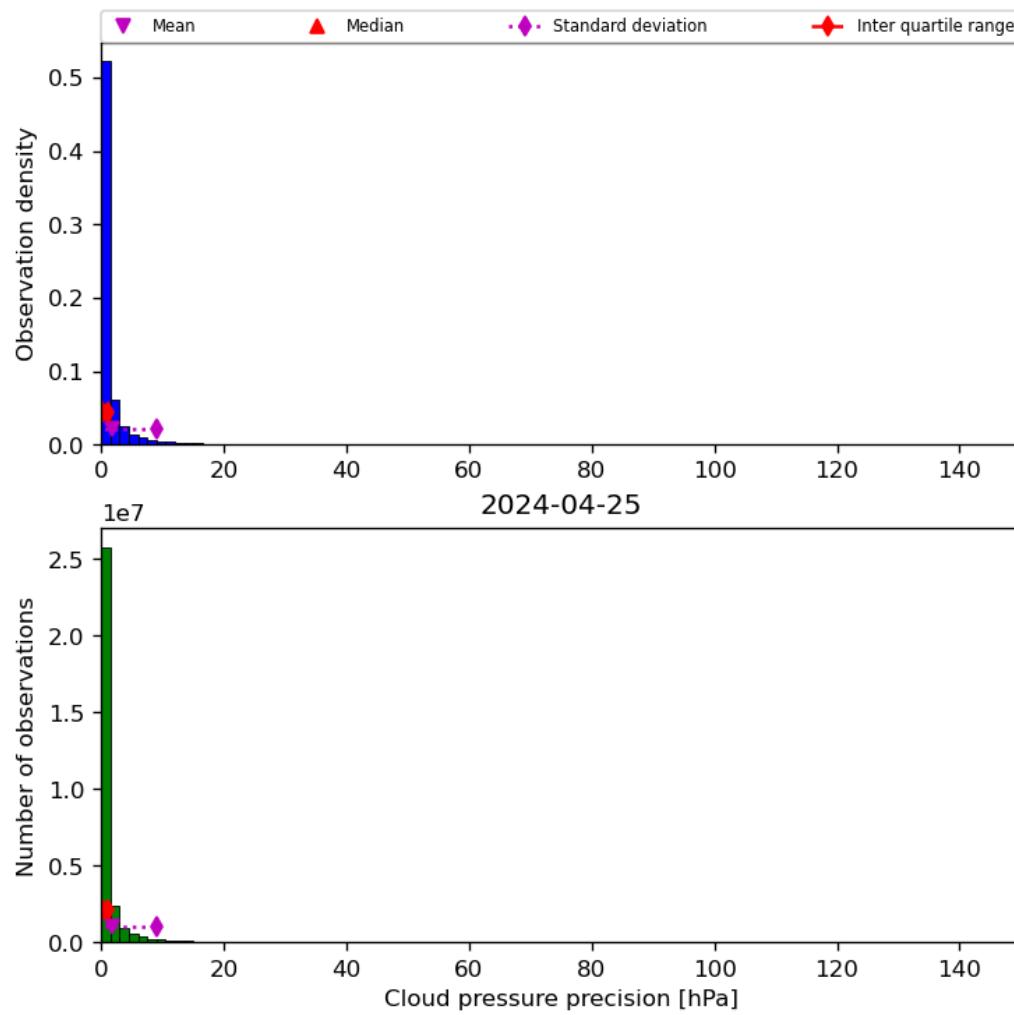
Figure 31: Histogram of “Cloud pressure precision” for 2024-04-24 to 2024-04-26
