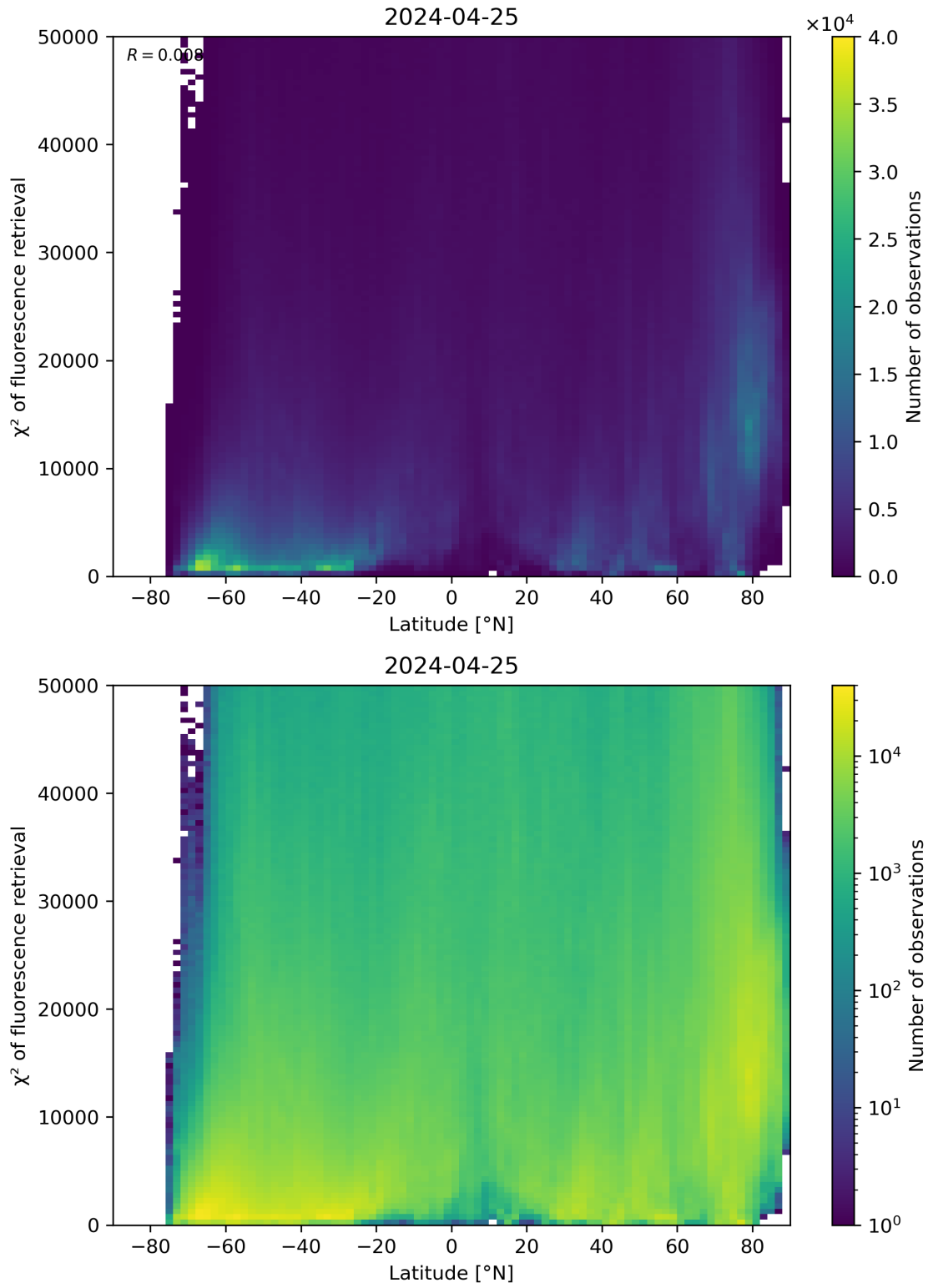
Figure 89: Scatter density plot of “Latitude” against “ \chi^2 of fluorescence retrieval” for 2024-04-24 to 2024-04-26.
