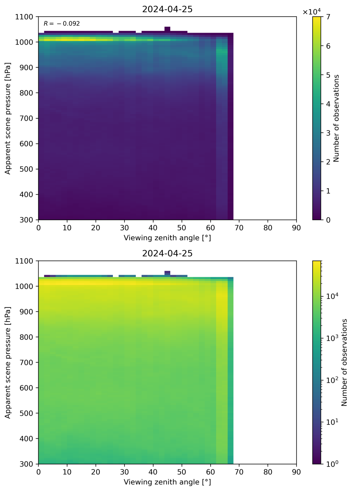
Figure 118: Scatter density plot of “Viewing zenith angle” against “Apparent scene pressure” for 2024-04-24 to 2024-04-26.
