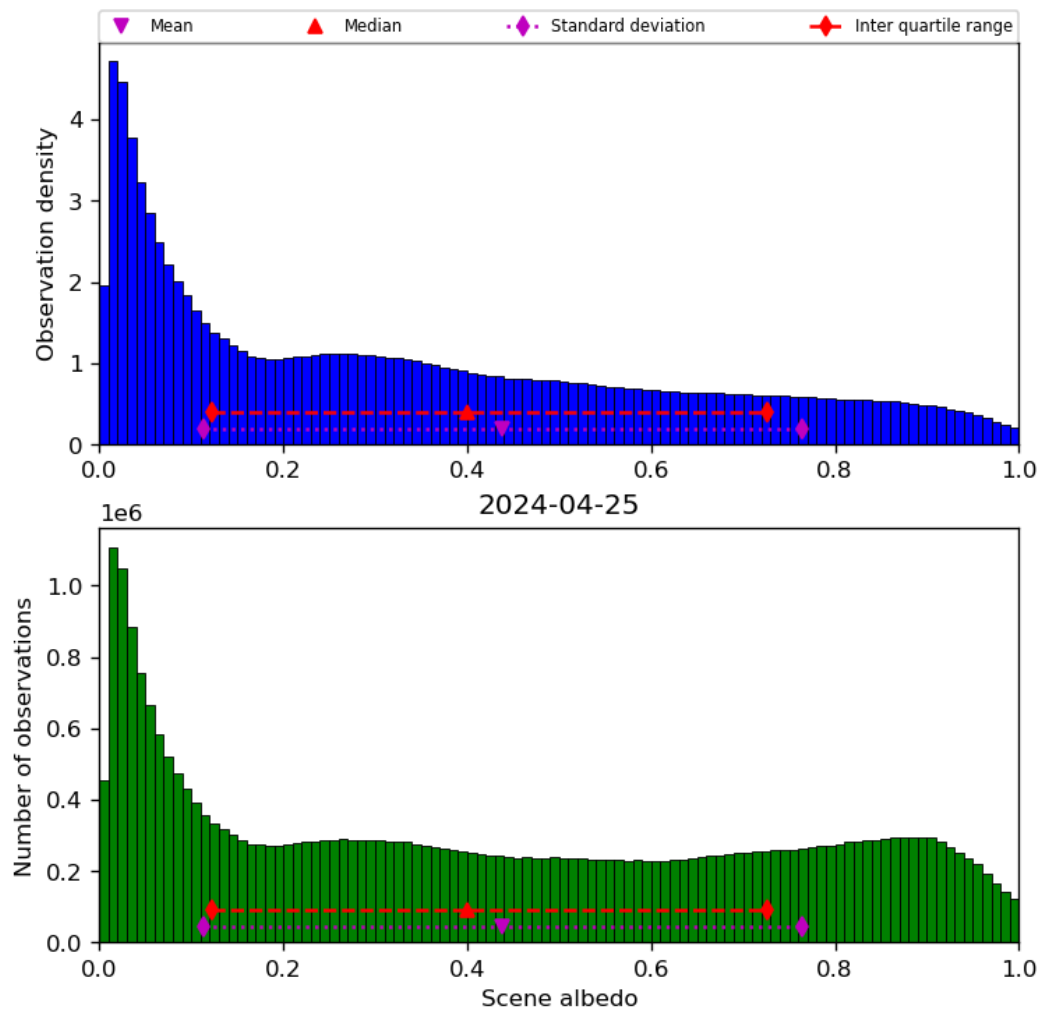
Figure 34: Histogram of “Scene albedo” for 2024-04-24 to 2024-04-26
