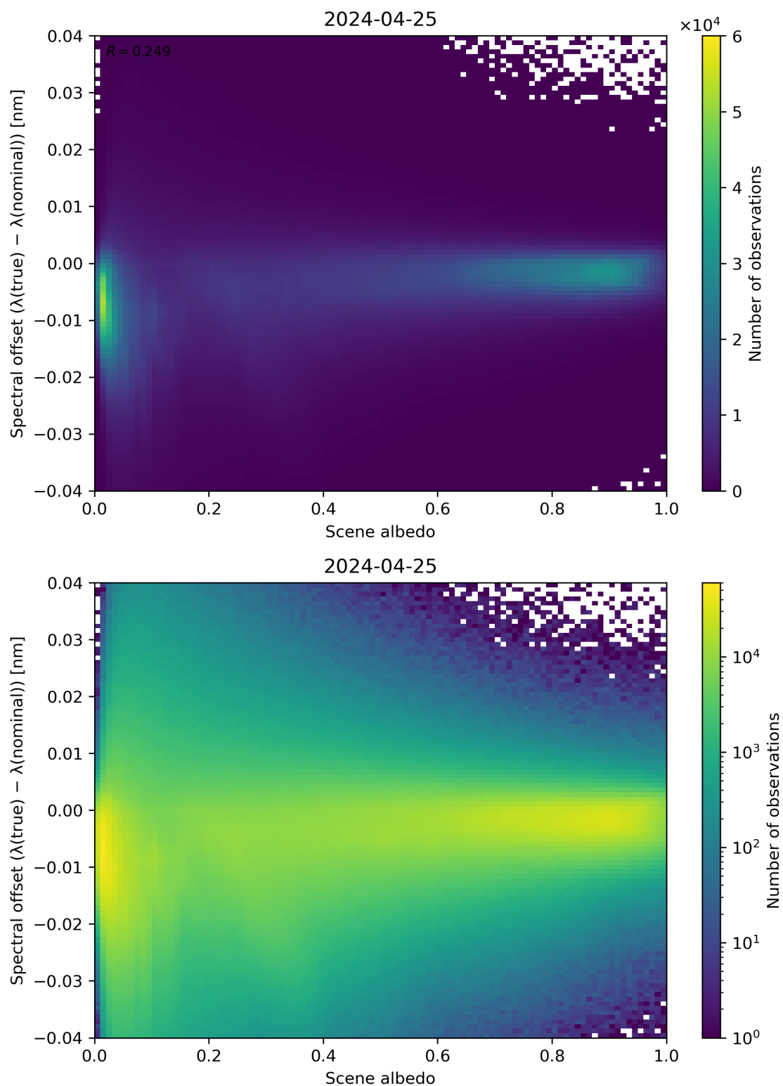
Figure 107: Scatter density plot of “Scene albedo” against “Spectral offset ( \lambda(\text{true}) - \lambda(\text{nominal}) )” for 2024-04-24 to 2024-04-26.
