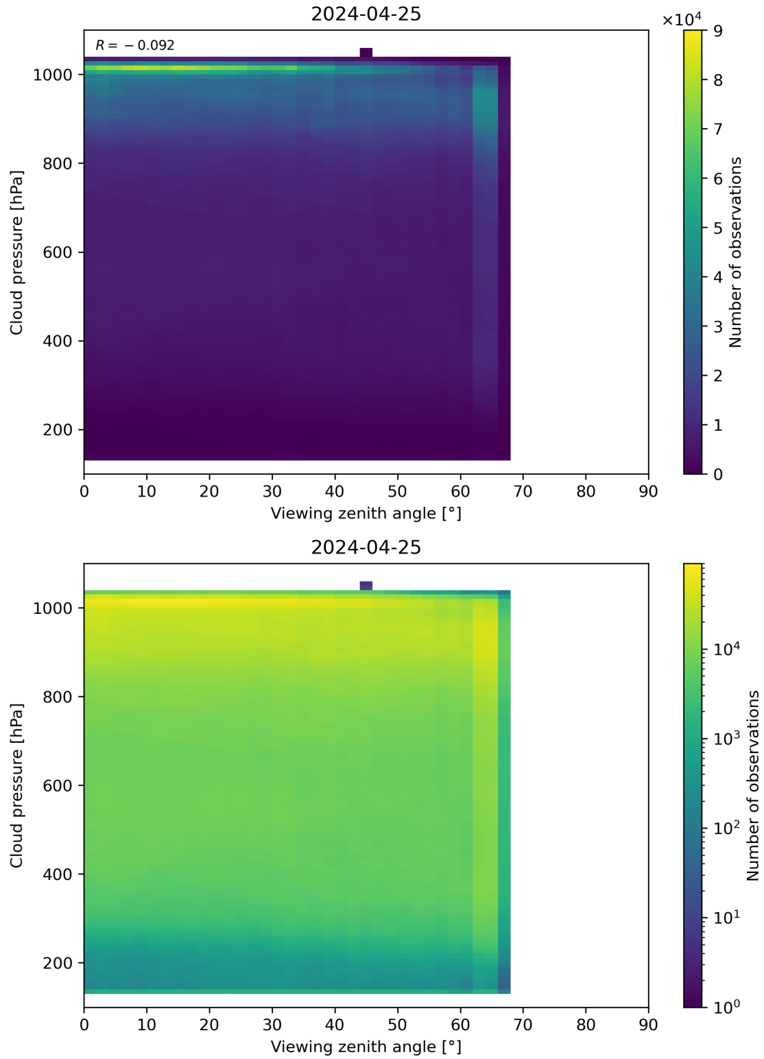
Figure 121: Scatter density plot of “Viewing zenith angle” against “Cloud pressure” for 2024-04-24 to 2024-04-26.
