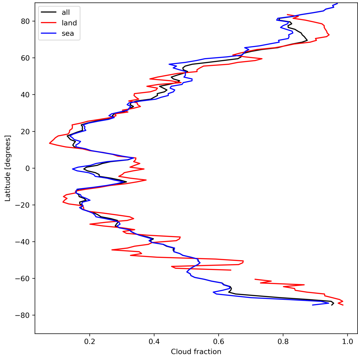
Figure 15: Zonal average of “Cloud fraction” for 2024-04-24 to 2024-04-26.
