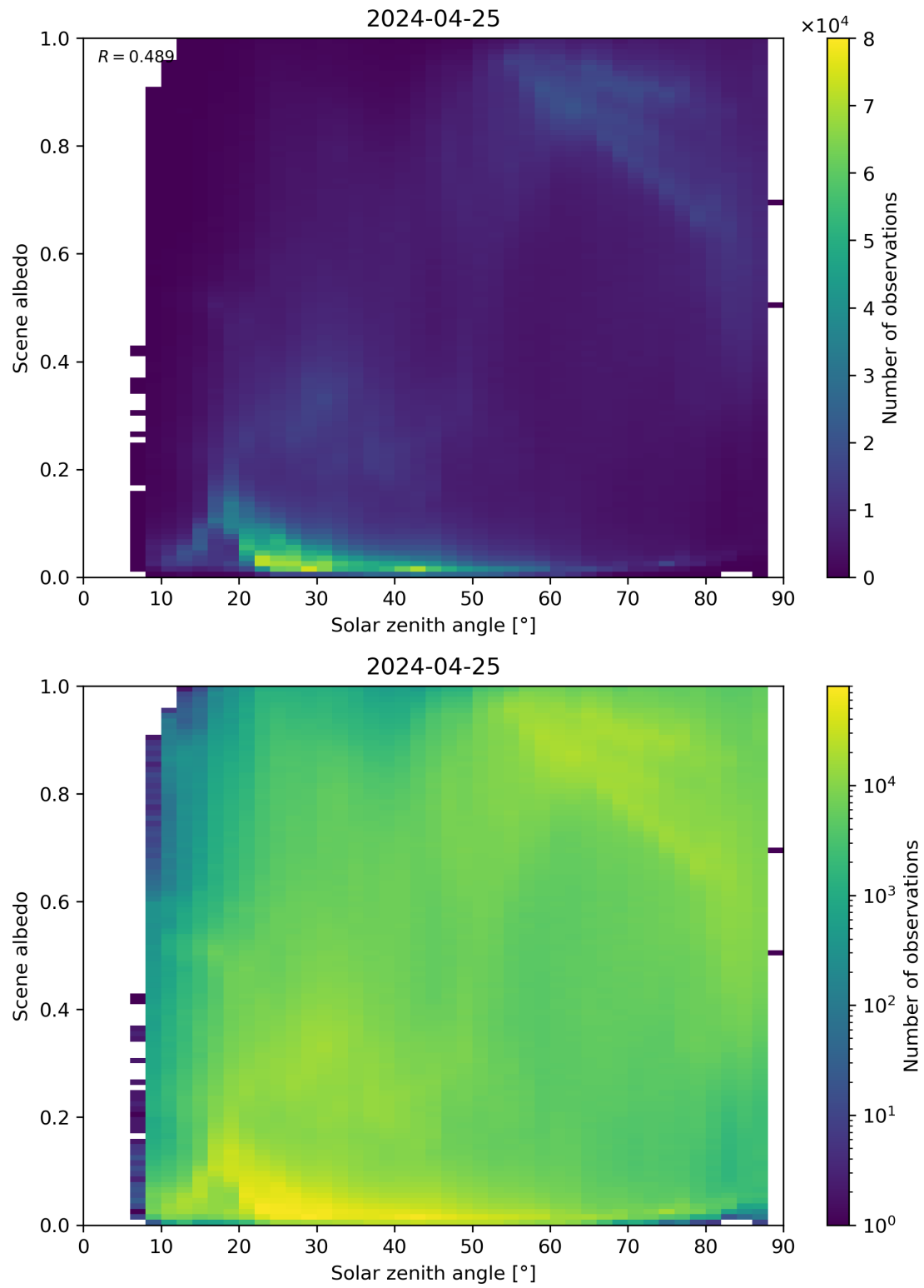
Figure 116: Scatter density plot of “Solar zenith angle” against “Scene albedo” for 2024-04-24 to 2024-04-26.
