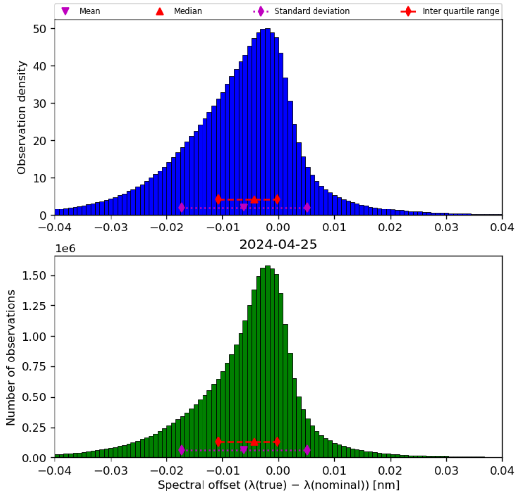
Figure 45: Histogram of “Spectral offset ( \lambda(\text{true}) - \lambda(\text{nominal}) )” for 2024-04-24 to 2024-04-26
