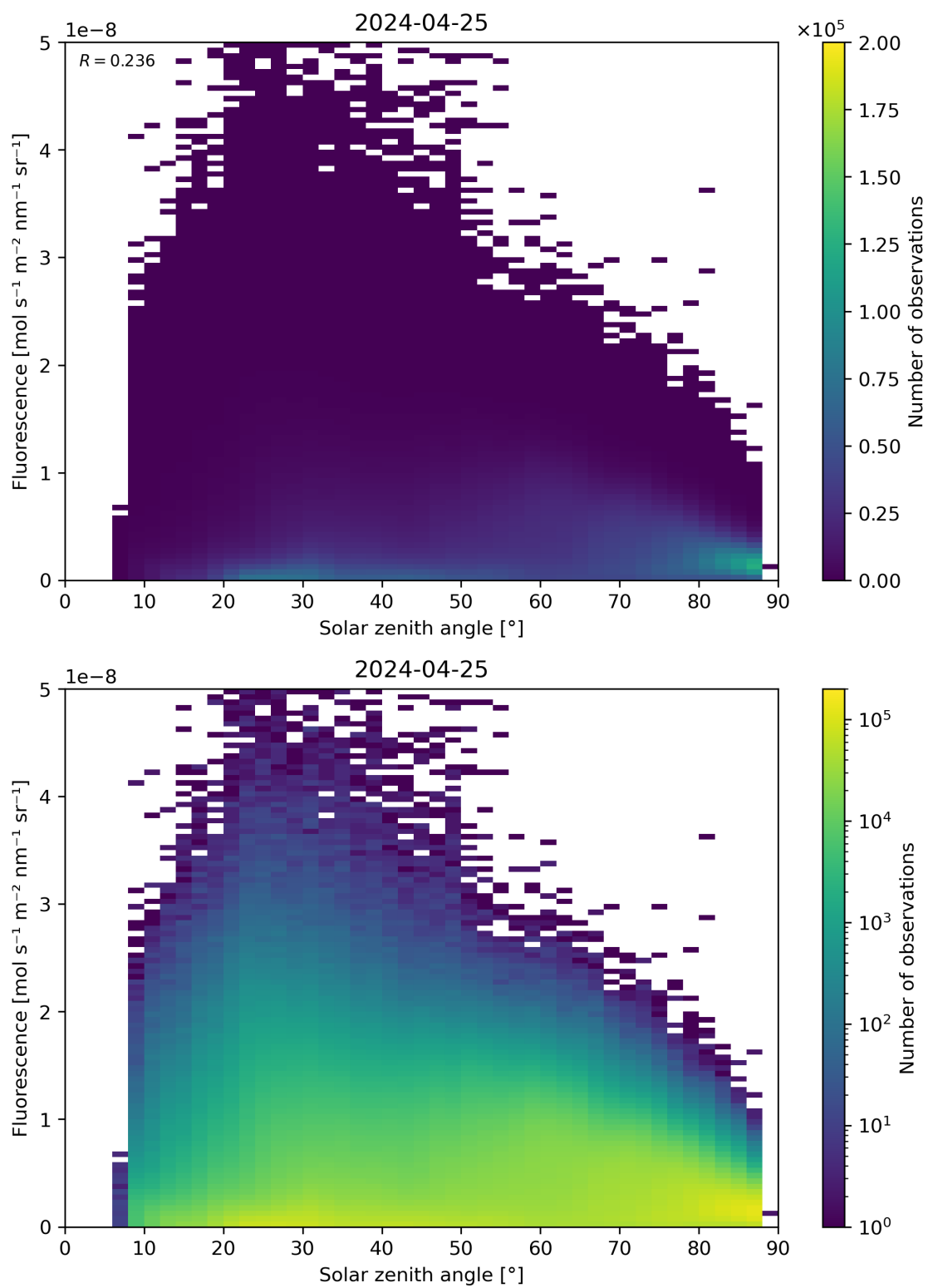
Figure 112: Scatter density plot of “Solar zenith angle” against “Fluorescence” for 2024-04-24 to 2024-04-26.
