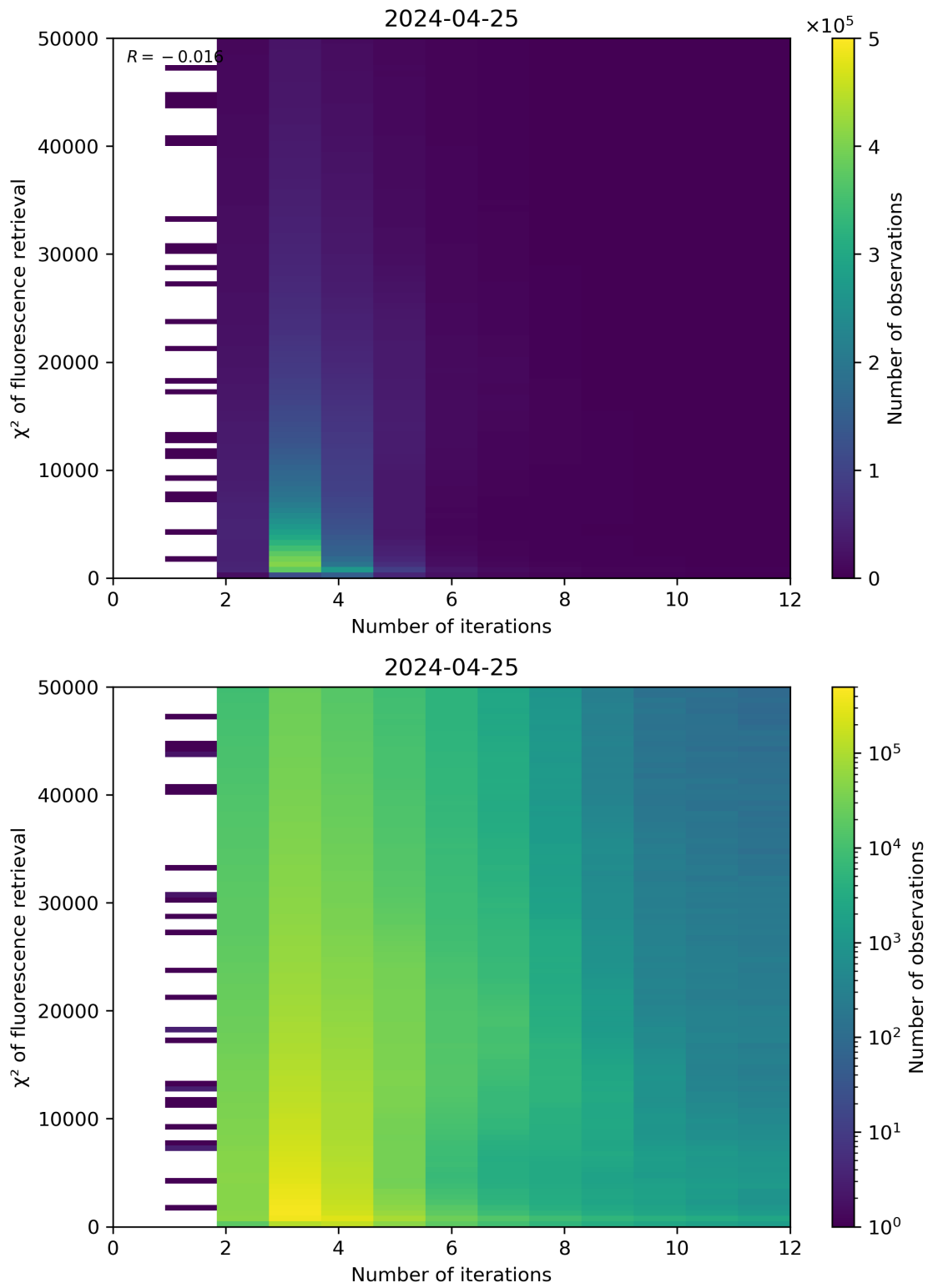
Figure 97: Scatter density plot of “Number of iterations” against “ \chi^2 of fluorescence retrieval” for 2024-04-24 to 2024-04-26.
