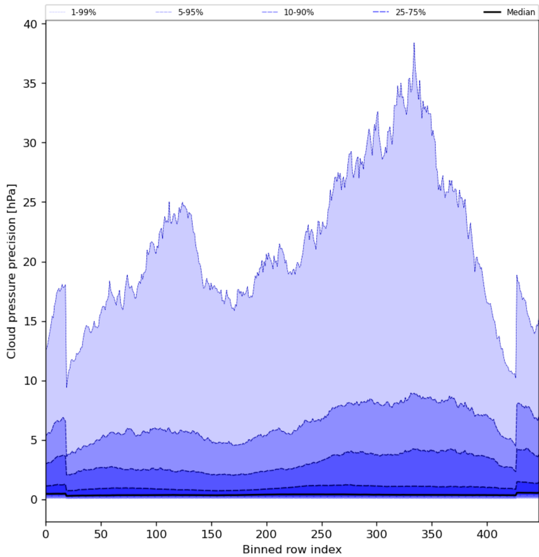
Figure 48: Along track statistics of “Cloud pressure precision” for 2024-04-24 to 2024-04-26
