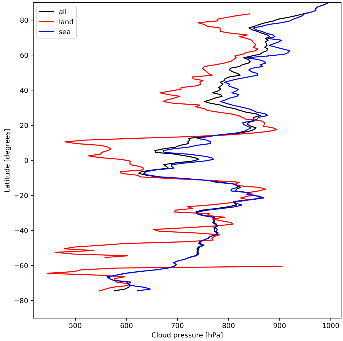
Figure 13: Zonal average of “Cloud pressure” for 2024-04-24 to 2024-04-26.
