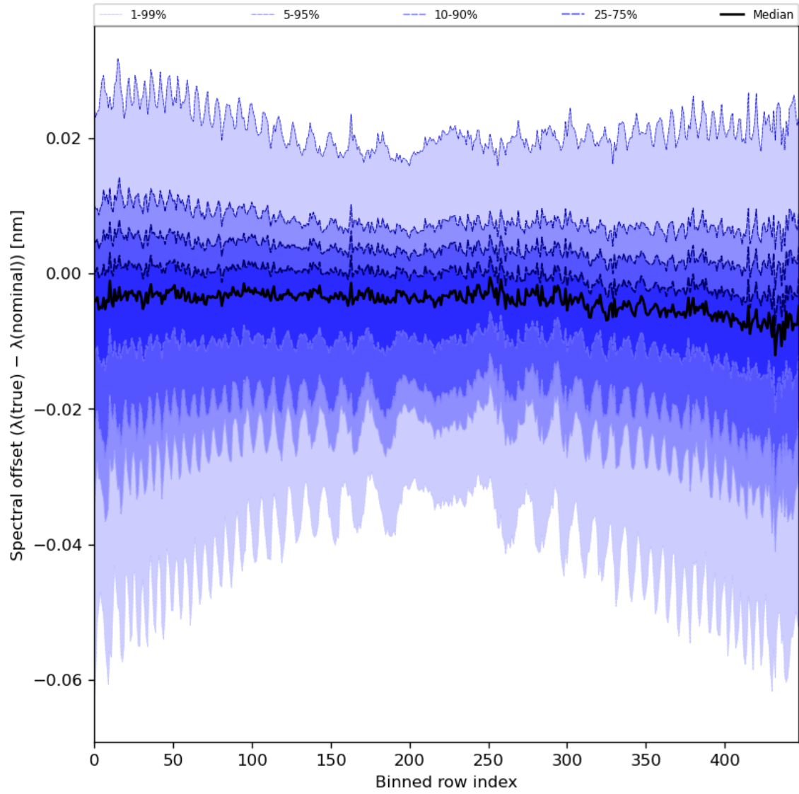
Figure 62: Along track statistics of “Spectral offset ( \lambda(\text{true}) - \lambda(\text{nominal}) )” for 2024-04-24 to 2024-04-26
