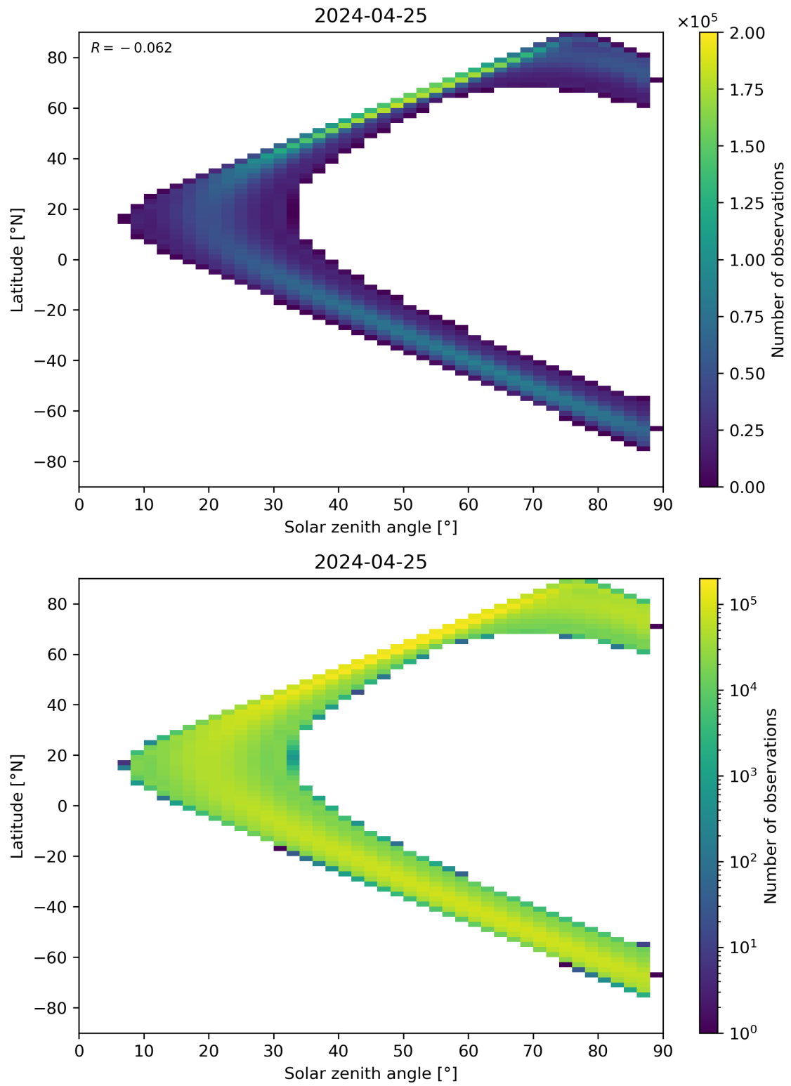
Figure 113: Scatter density plot of “Solar zenith angle” against “Latitude” for 2024-04-24 to 2024-04-26.
