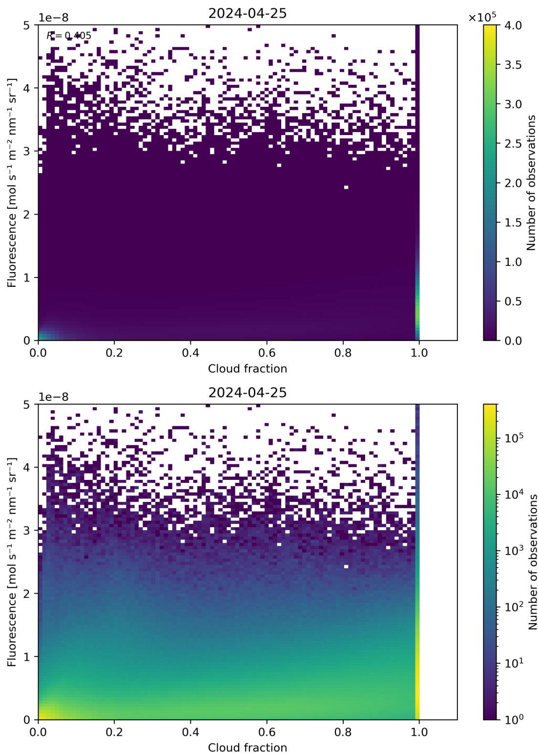
Figure 72: Scatter density plot of “Cloud fraction” against “Fluorescence” for 2024-04-24 to 2024-04-26.
