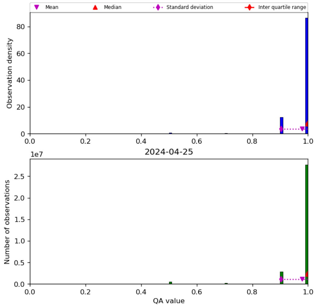
Figure 29: Histogram of “QA value” for 2024-04-24 to 2024-04-26
