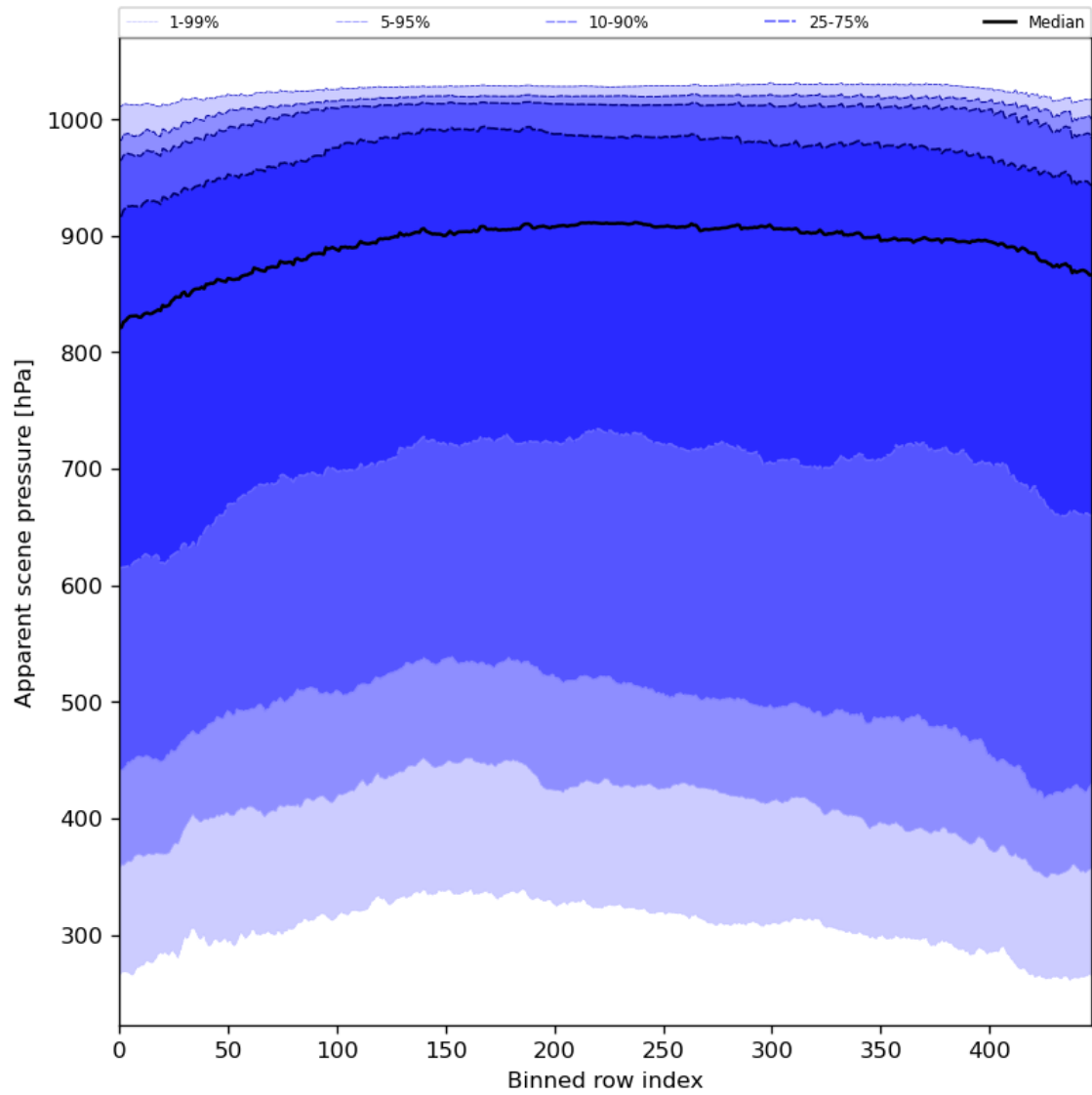
Figure 53: Along track statistics of “Apparent scene pressure” for 2024-04-24 to 2024-04-26
