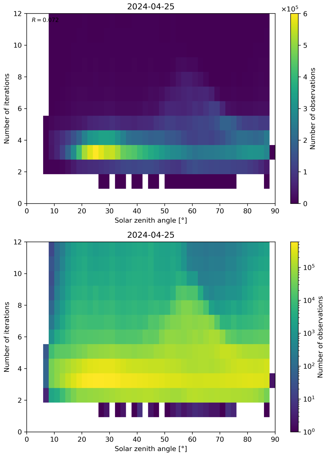
Figure 114: Scatter density plot of “Solar zenith angle” against “Number of iterations” for 2024-04-24 to 2024-04-26.
