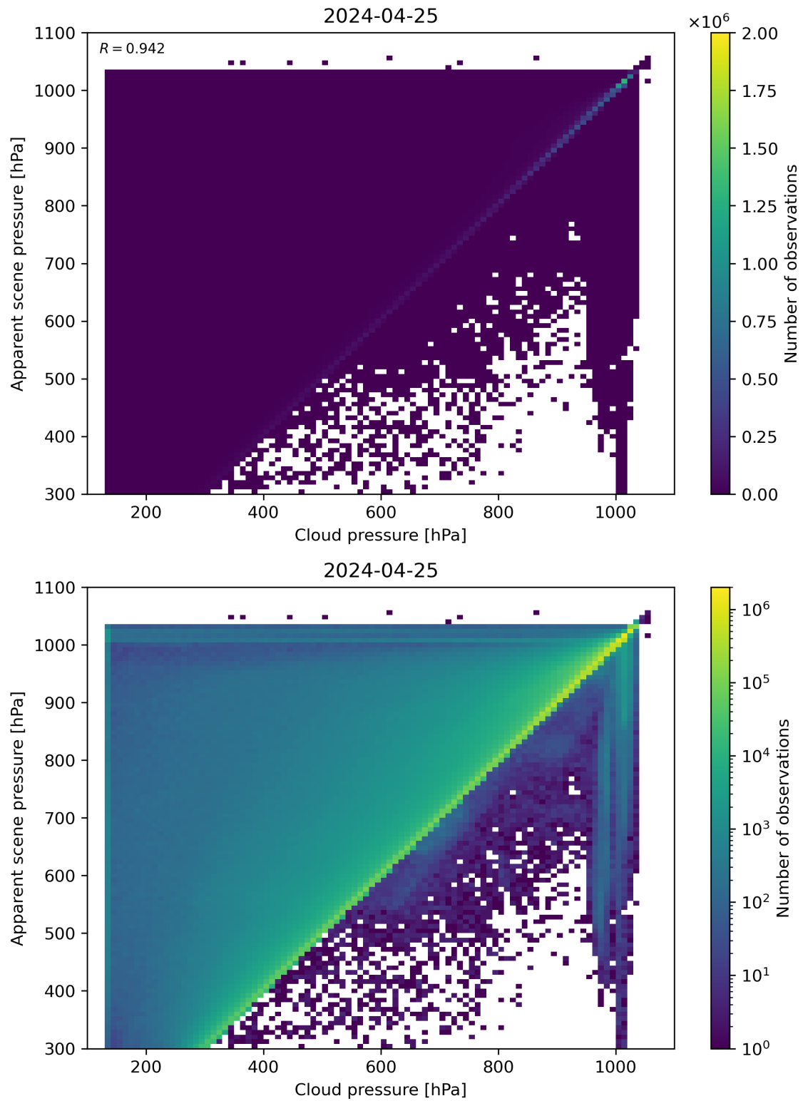
Figure 77: Scatter density plot of “Cloud pressure” against “Apparent scene pressure” for 2024-04-24 to 2024-04-26.
