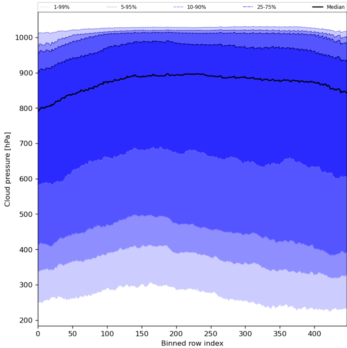
Figure 47: Along track statistics of “Cloud pressure” for 2024-04-24 to 2024-04-26
