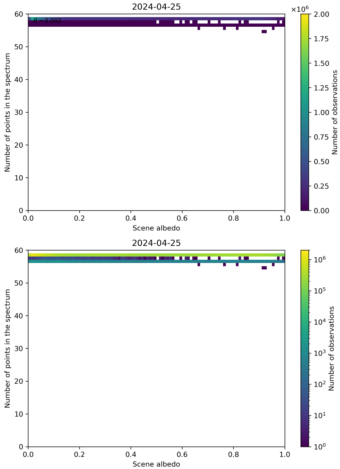
Figure 106: Scatter density plot of “Scene albedo” against “Number of points in the spectrum” for 2024-04-24 to 2024-04-26.
