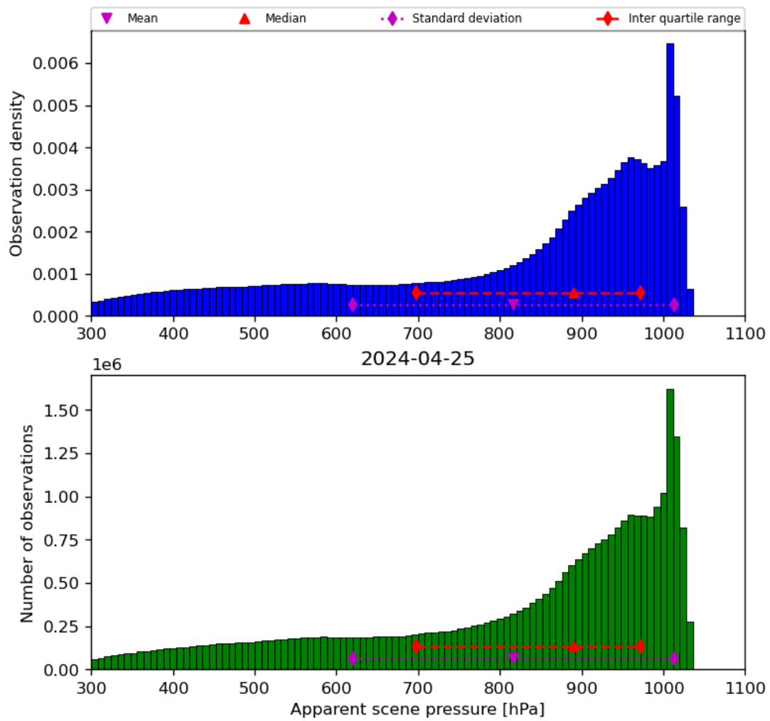
Figure 36: Histogram of “Apparent scene pressure” for 2024-04-24 to 2024-04-26
