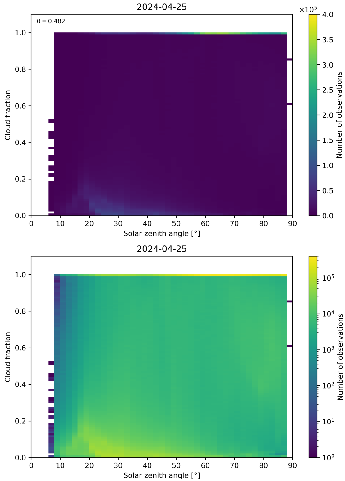
Figure 110: Scatter density plot of “Solar zenith angle” against “Cloud fraction” for 2024-04-24 to 2024-04-26.
