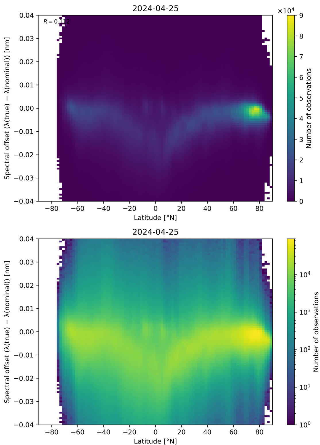
Figure 96: Scatter density plot of “Latitude” against “Spectral offset ( \lambda(\text{true}) - \lambda(\text{nominal}) )” for 2024-04-24 to 2024-04-26.
