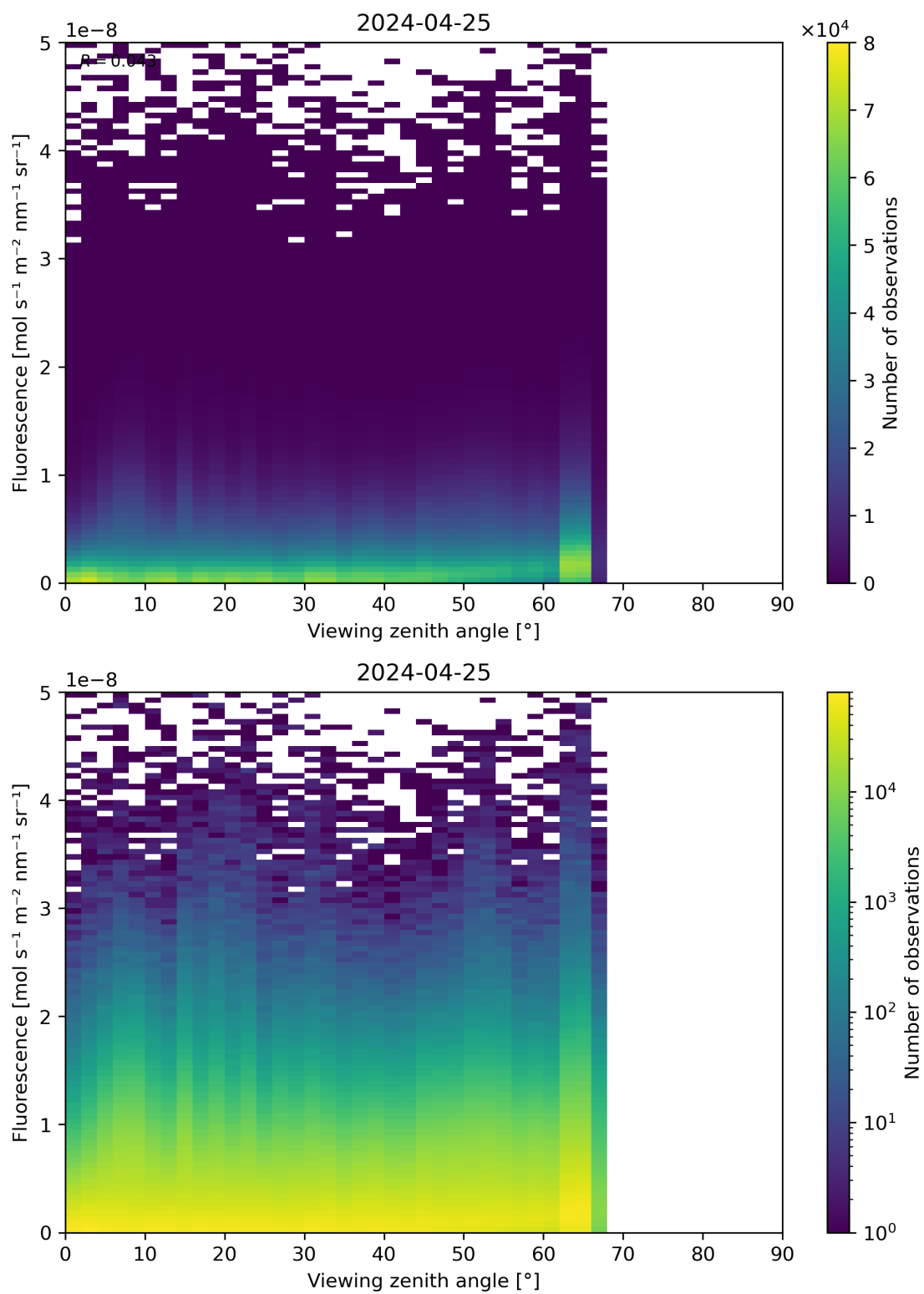
Figure 122: Scatter density plot of “Viewing zenith angle” against “Fluorescence” for 2024-04-24 to 2024-04-26.
