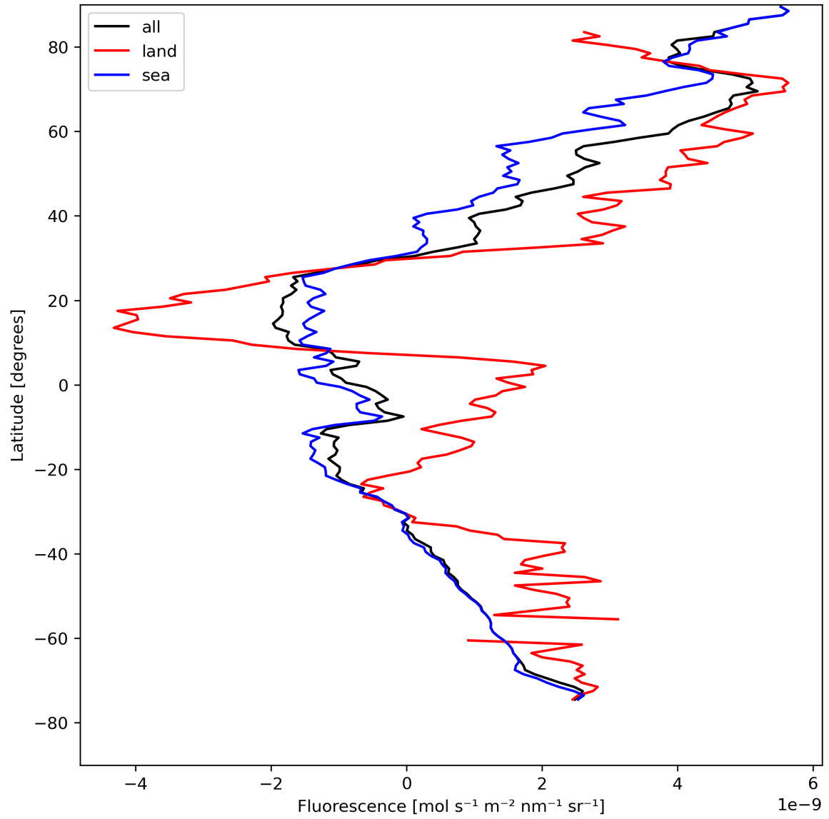
Figure 23: Zonal average of “Fluorescence” for 2024-04-24 to 2024-04-26.
