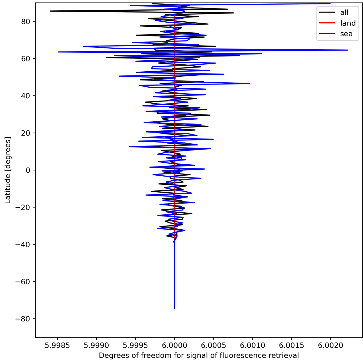
Figure 26: Zonal average of “Degrees of freedom for signal of fluorescence retrieval” for 2024-04-24 to 2024-04-26.
