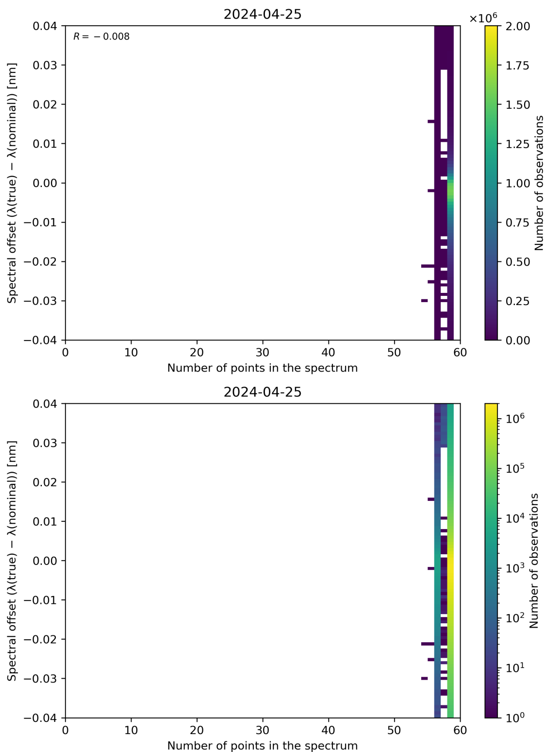
Figure 101: Scatter density plot of “Number of points in the spectrum” against “Spectral offset ( \lambda(\text{true}) - \lambda(\text{nominal}) )” for 2024-04-24 to 2024-04-26.
