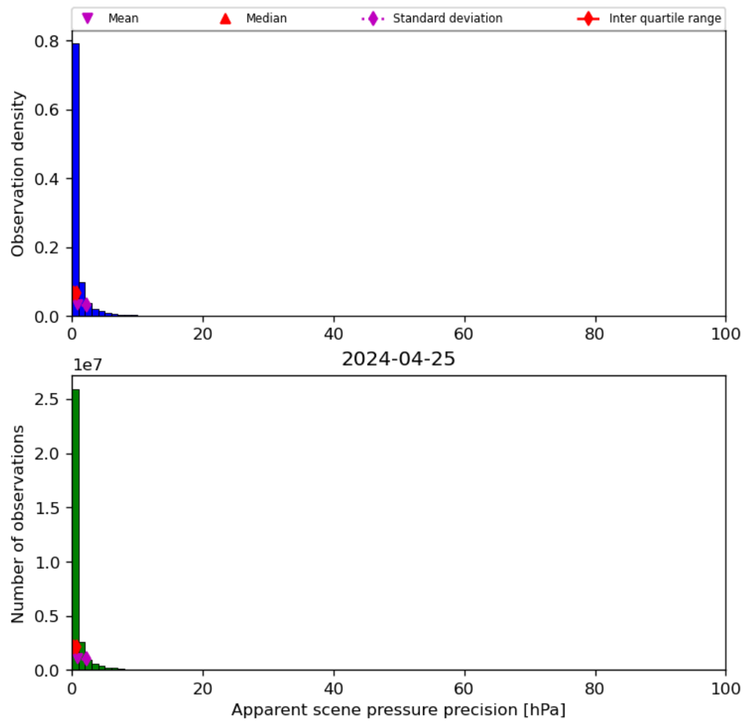
Figure 37: Histogram of “Apparent scene pressure precision” for 2024-04-24 to 2024-04-26
