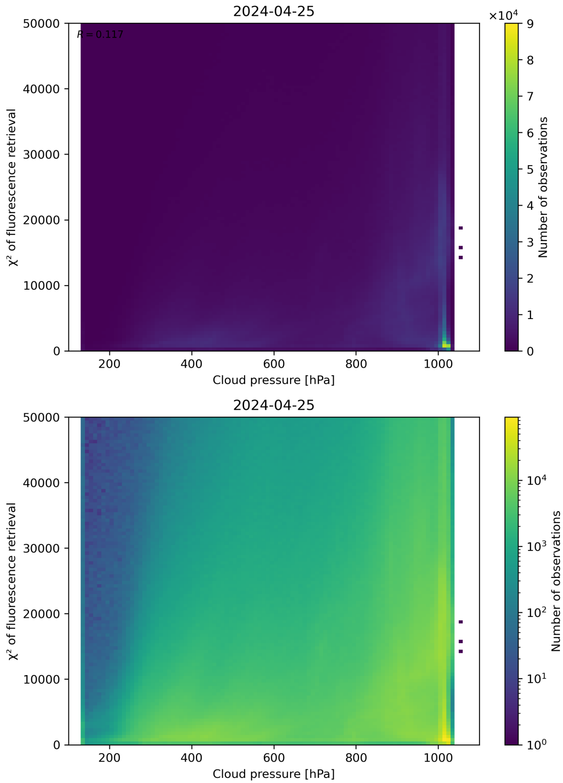
Figure 78: Scatter density plot of “Cloud pressure” against “ \chi^2 of fluorescence retrieval” for 2024-04-24 to 2024-04-26.
