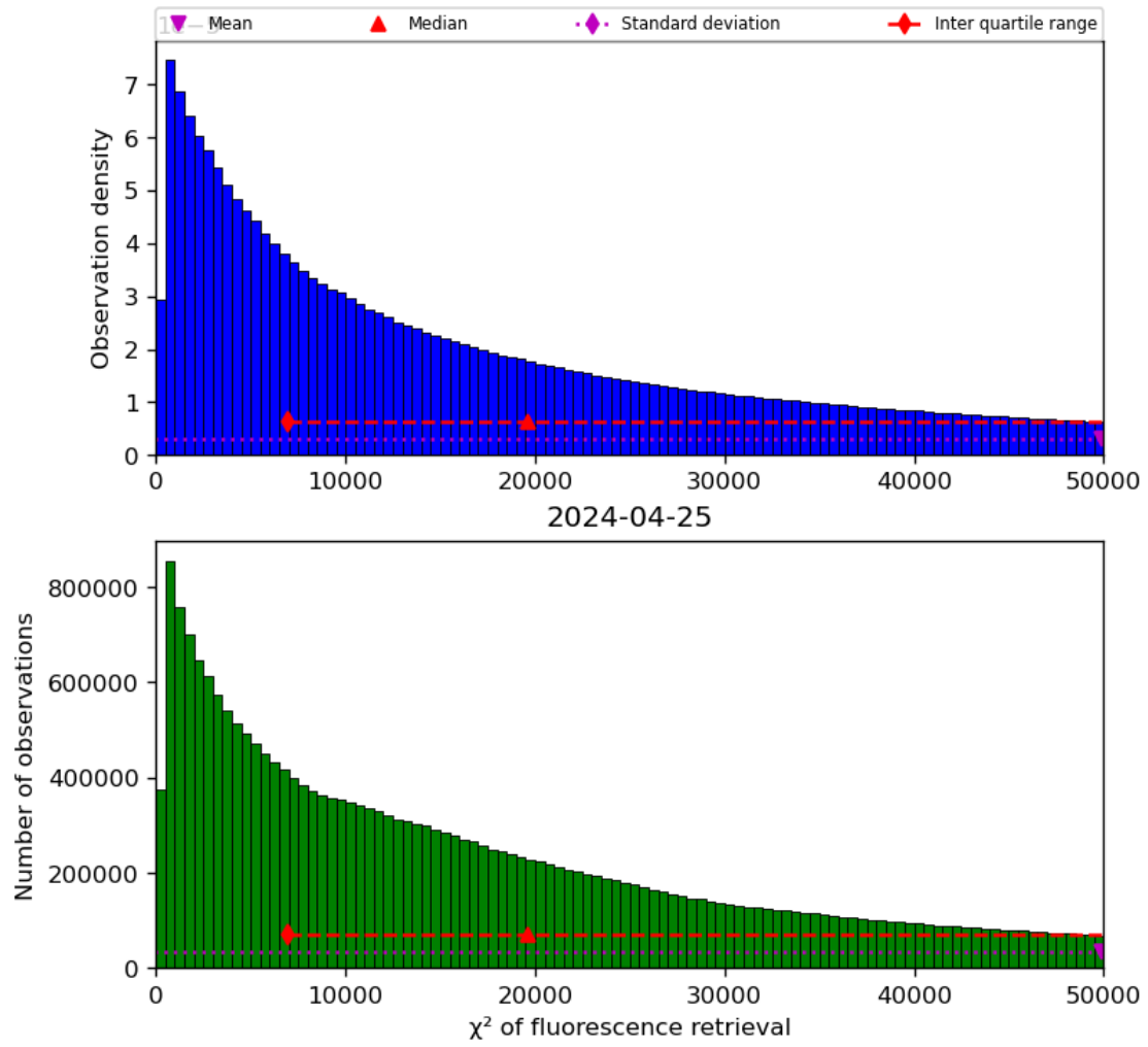
Figure 42: Histogram of “ \chi^2 of fluorescence retrieval” for 2024-04-24 to 2024-04-26
