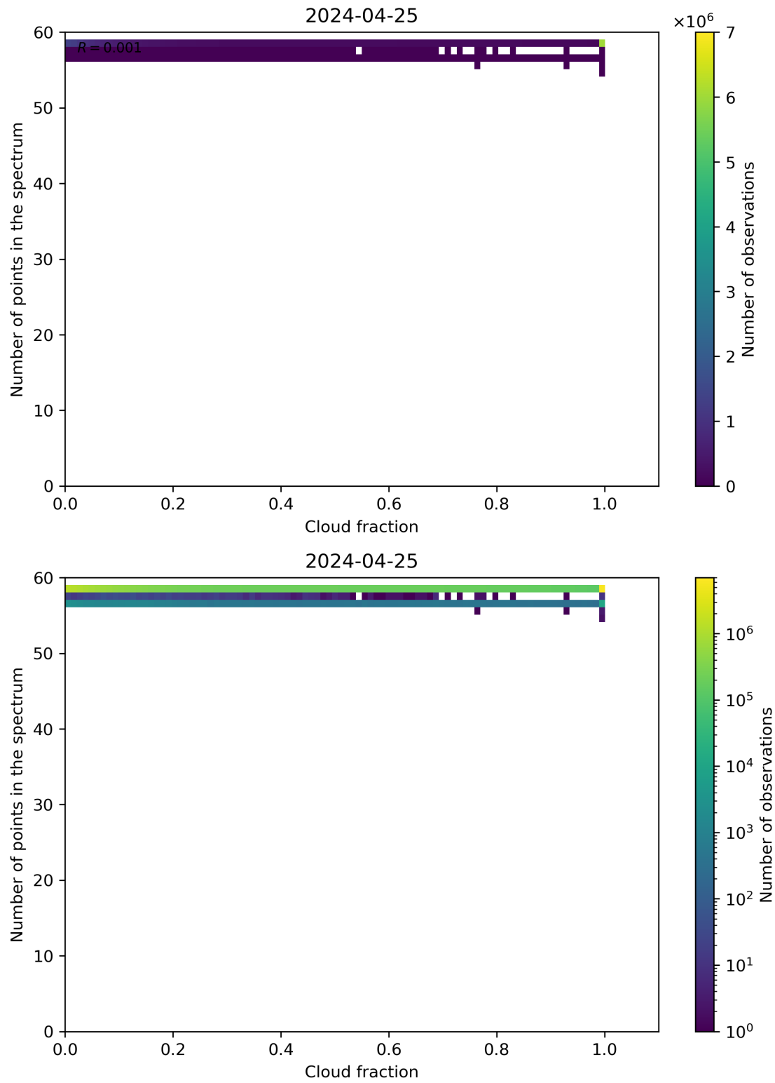
Figure 74: Scatter density plot of “Cloud fraction” against “Number of points in the spectrum” for 2024-04-24 to 2024-04-26.
