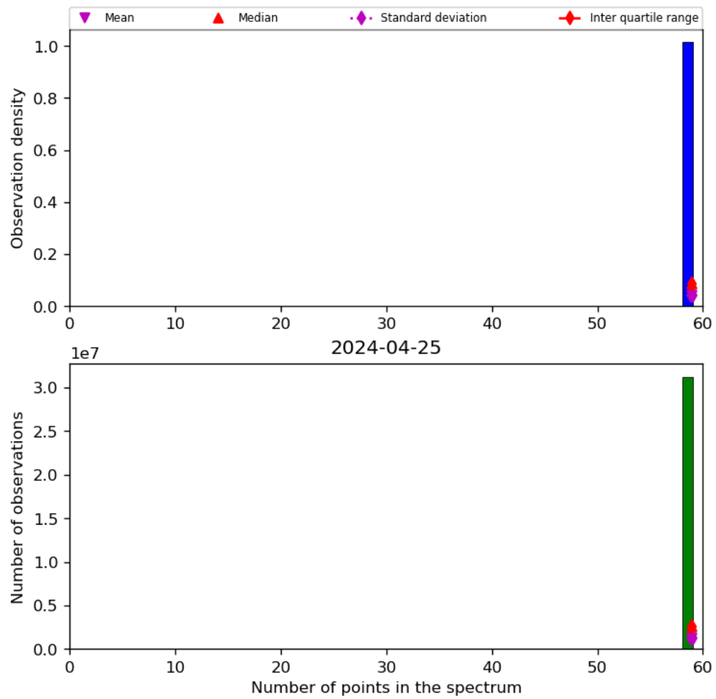
Figure 44: Histogram of “Number of points in the spectrum” for 2024-04-24 to 2024-04-26
