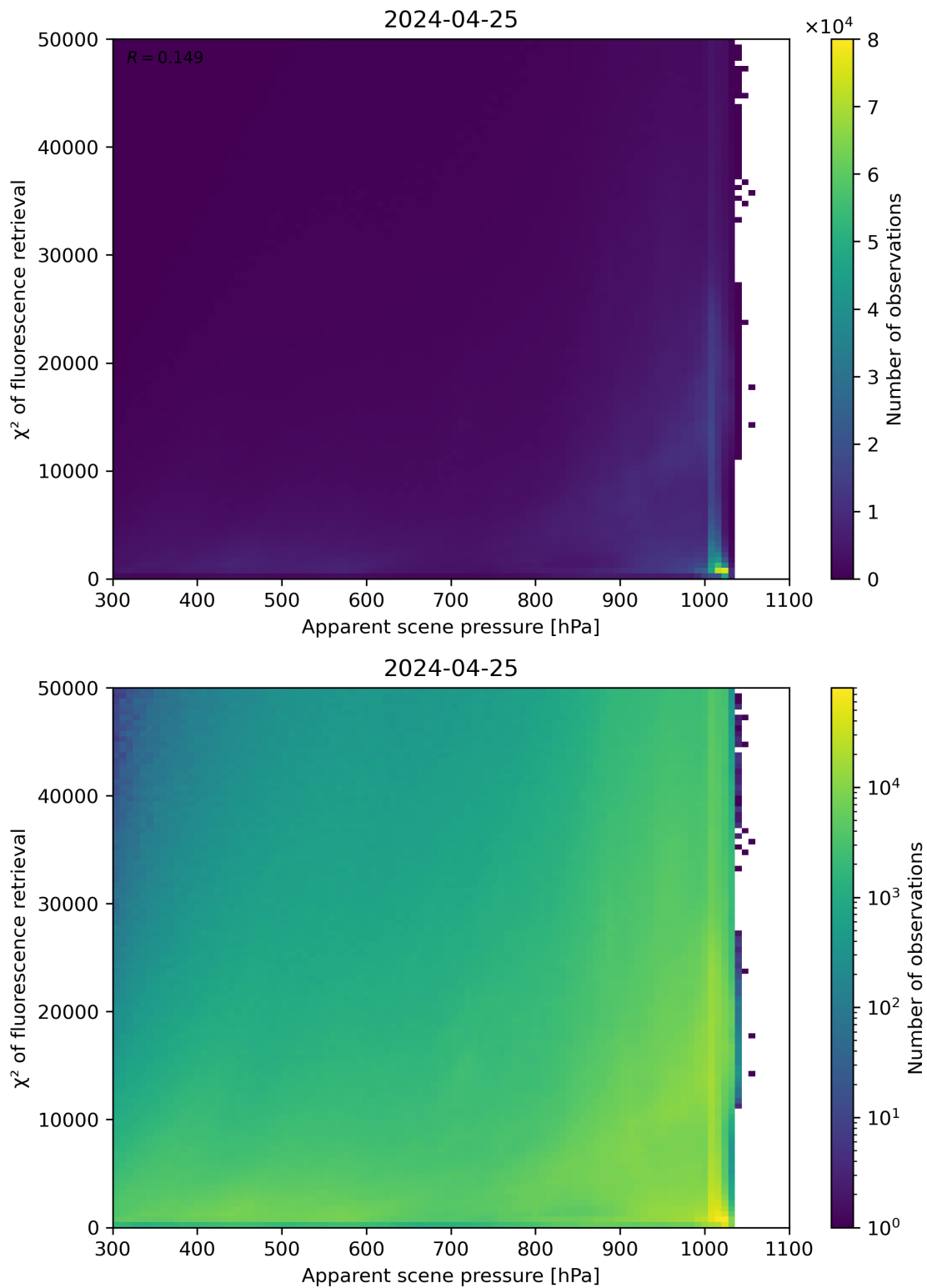
Figure 63: Scatter density plot of “Apparent scene pressure” against “ \chi^2 of fluorescence retrieval” for 2024-04-24 to 2024-04-26.
