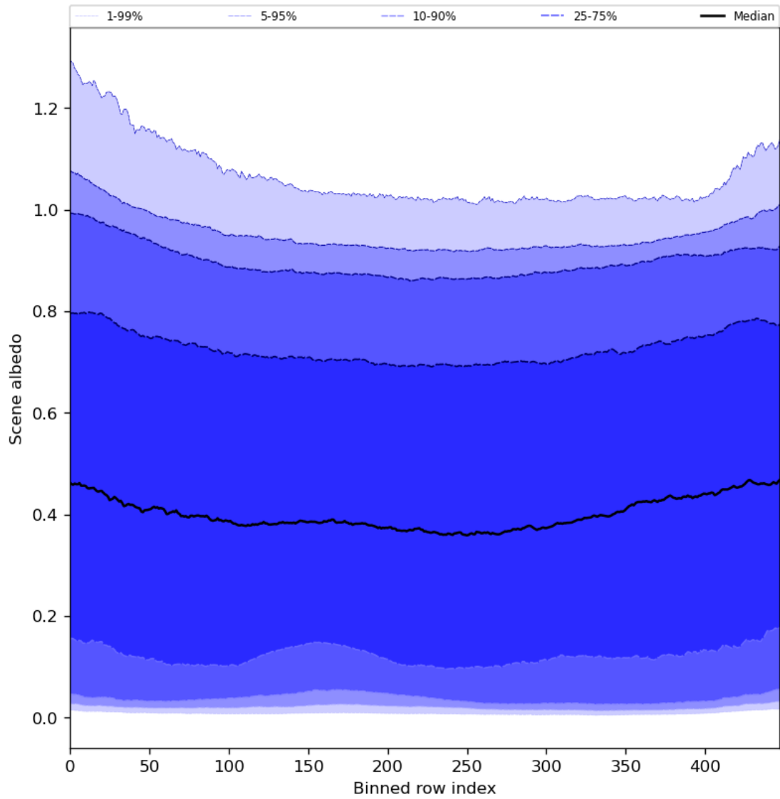
Figure 51: Along track statistics of “Scene albedo” for 2024-04-24 to 2024-04-26
