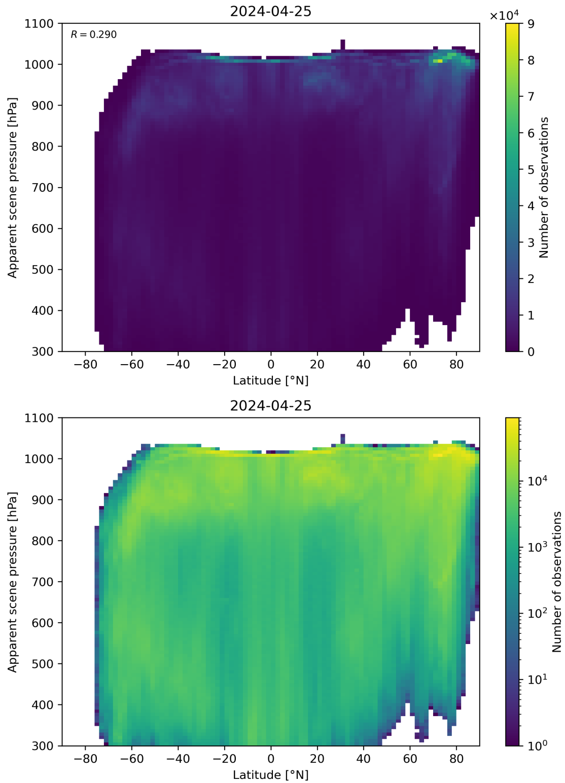
Figure 88: Scatter density plot of “Latitude” against “Apparent scene pressure” for 2024-04-24 to 2024-04-26.
