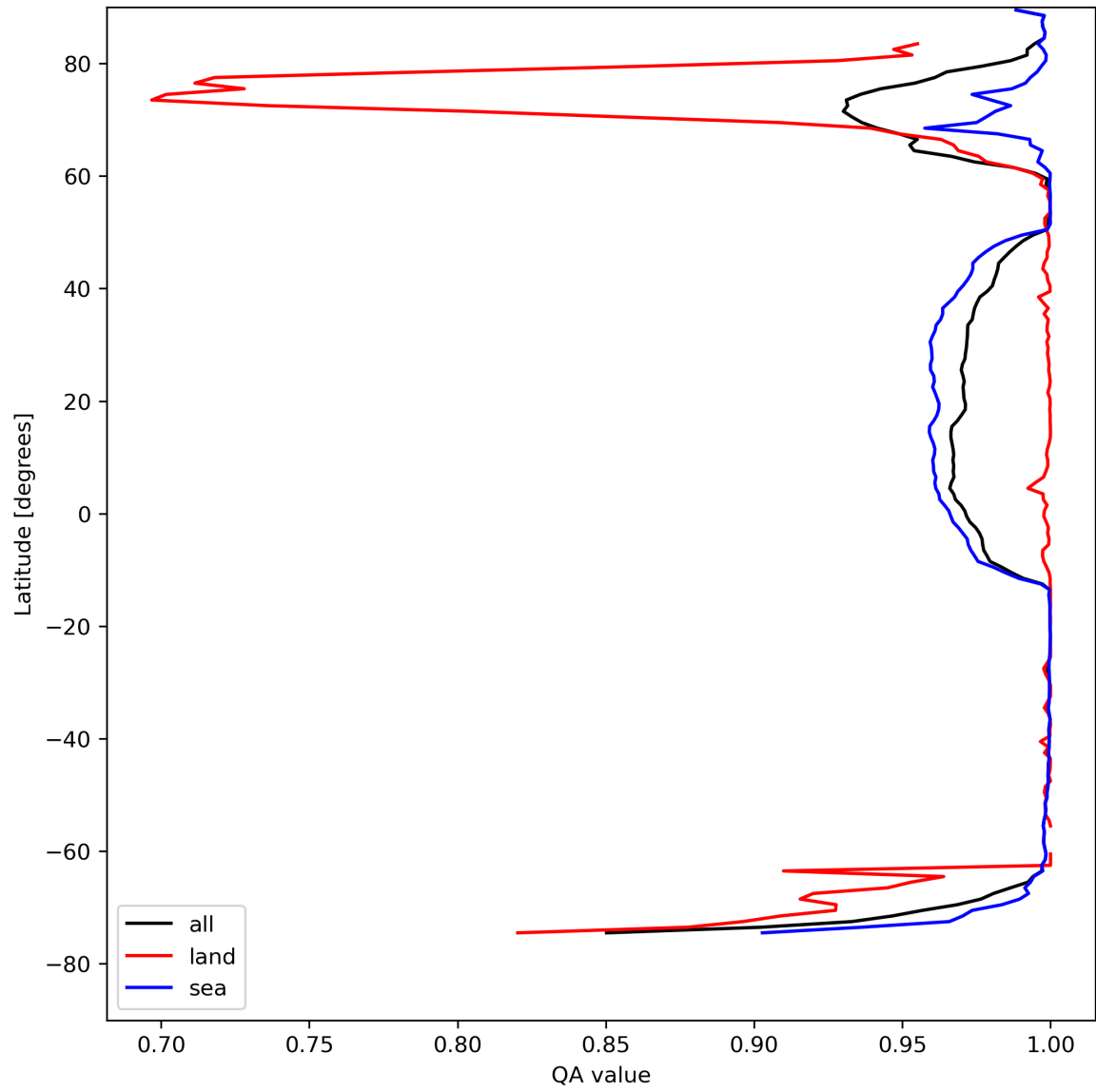
Figure 12: Zonal average of “QA value” for 2024-04-24 to 2024-04-26.
