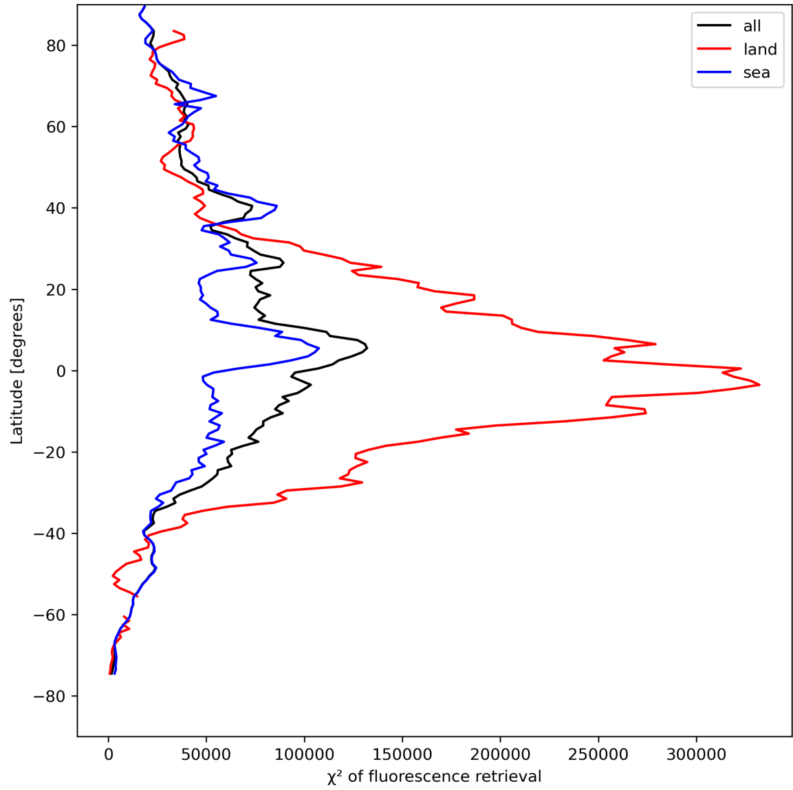
Figure 25: Zonal average of “ \chi^2 of fluorescence retrieval” for 2024-04-24 to 2024-04-26.
