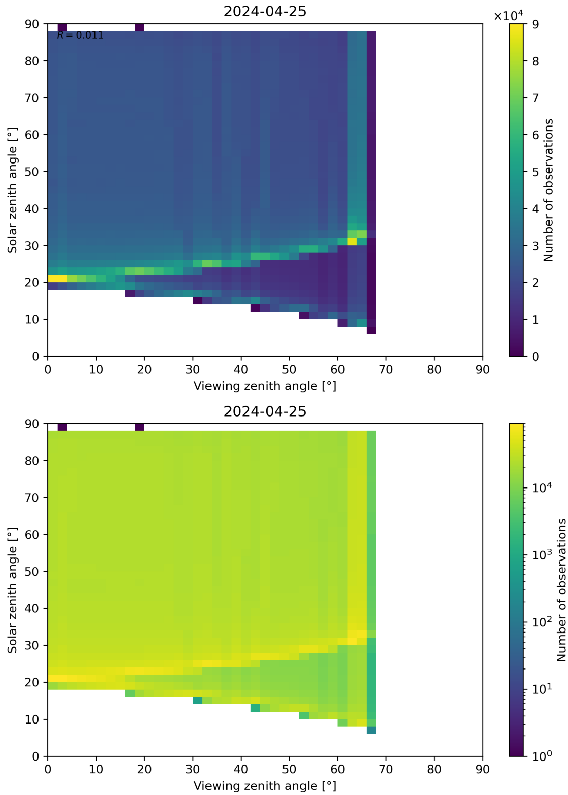
Figure 127: Scatter density plot of “Viewing zenith angle” against “Solar zenith angle” for 2024-04-24 to 2024-04-26.
