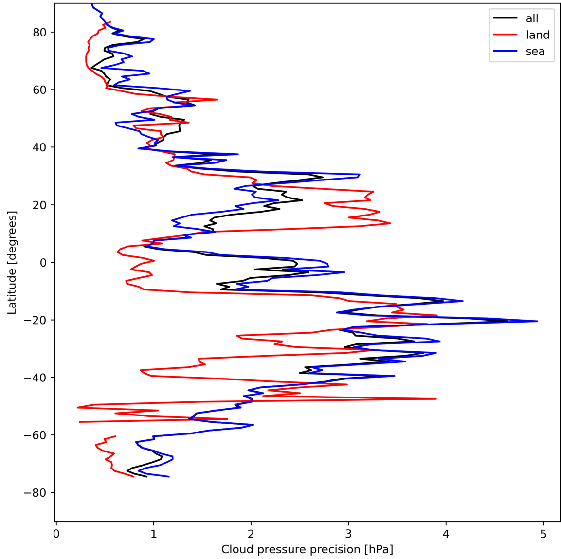
Figure 14: Zonal average of “Cloud pressure precision” for 2024-04-24 to 2024-04-26.
