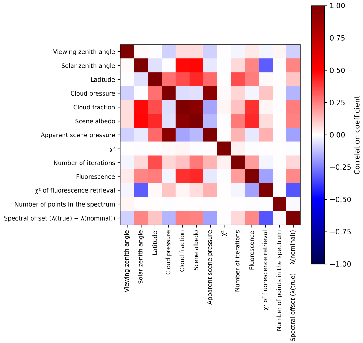
Figure 2: Map of correlation matrix for 2024-04-24 to 2024-04-26.
