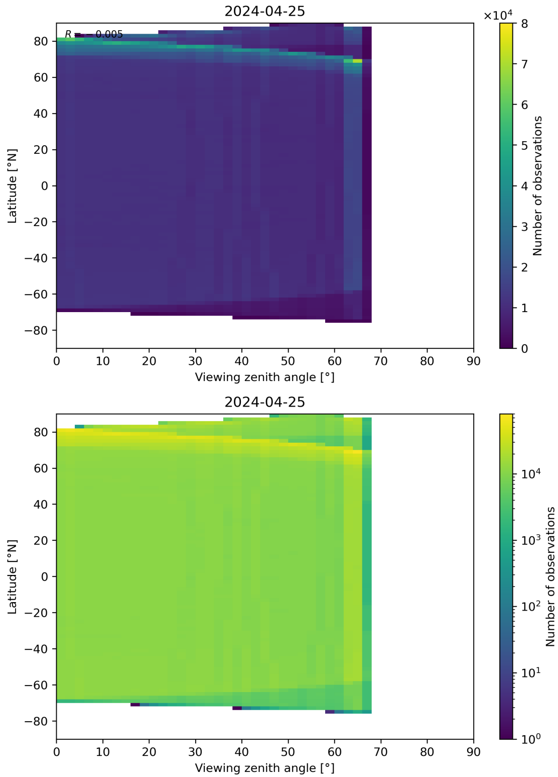
Figure 123: Scatter density plot of “Viewing zenith angle” against “Latitude” for 2024-04-24 to 2024-04-26.
