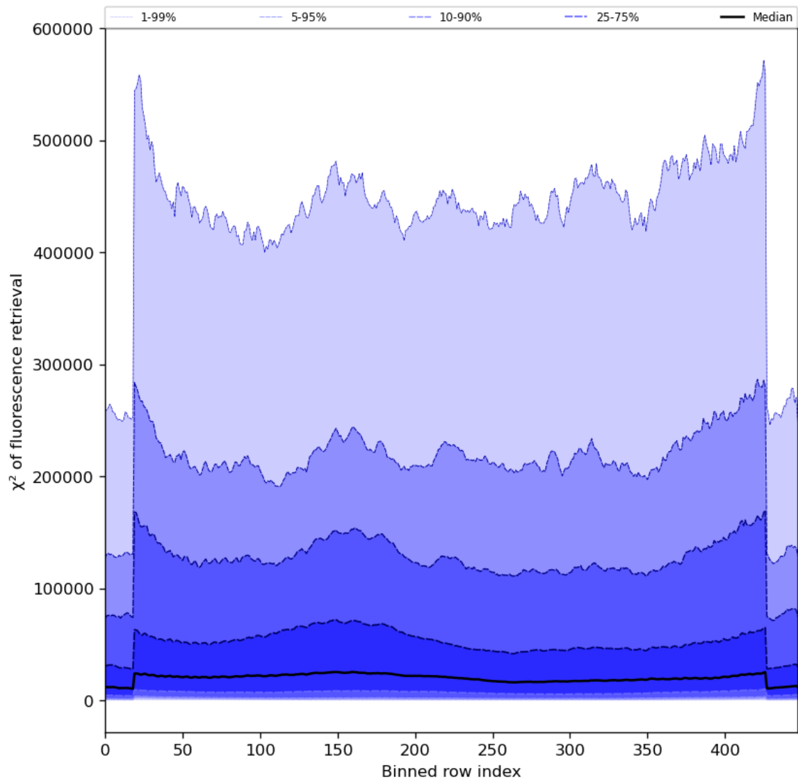
Figure 59: Along track statistics of “ \chi^2 of fluorescence retrieval” for 2024-04-24 to 2024-04-26
