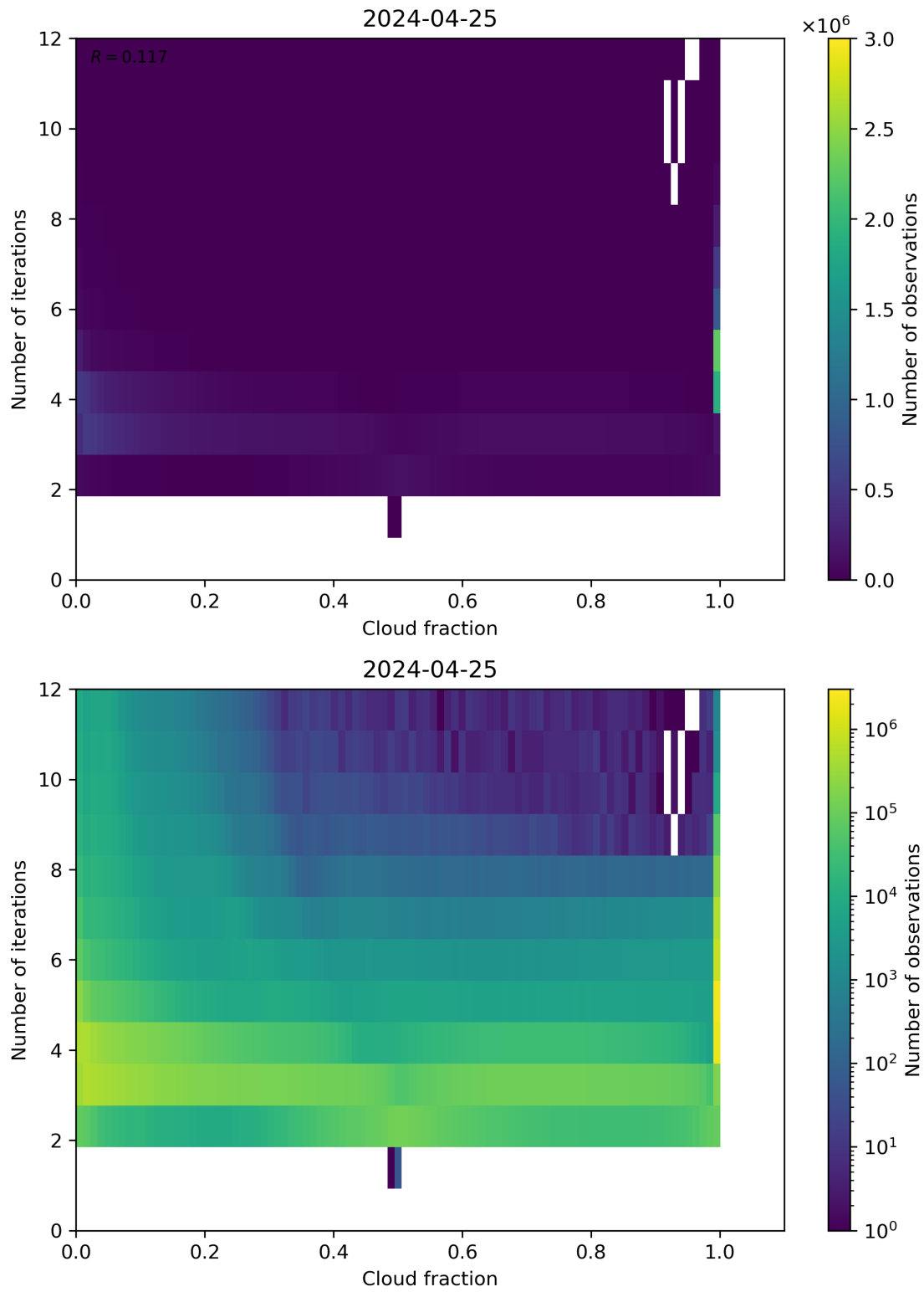
Figure 73: Scatter density plot of “Cloud fraction” against “Number of iterations” for 2024-04-24 to 2024-04-26.
