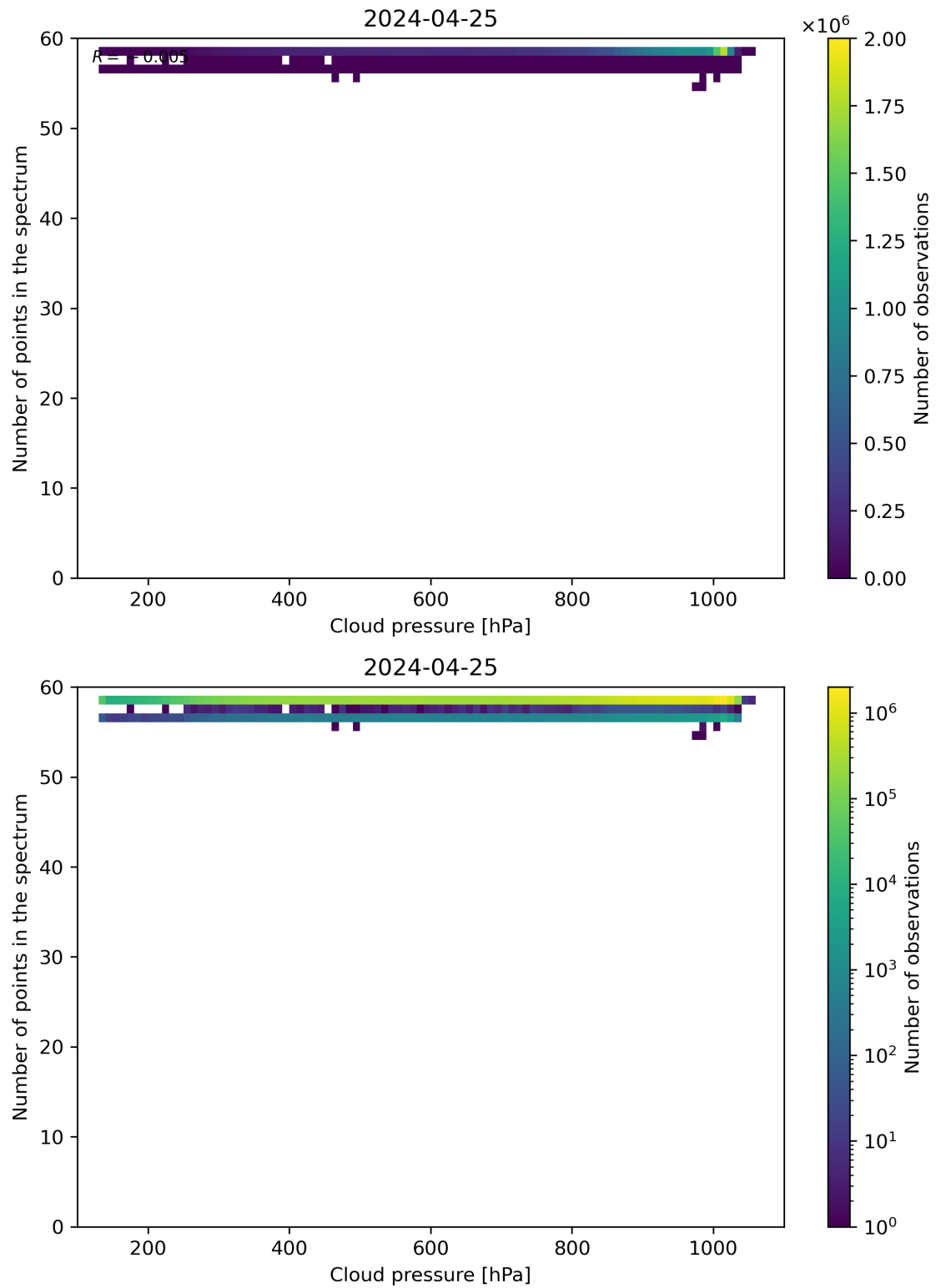
Figure 82: Scatter density plot of “Cloud pressure” against “Number of points in the spectrum” for 2024-04-24 to 2024-04-26.
