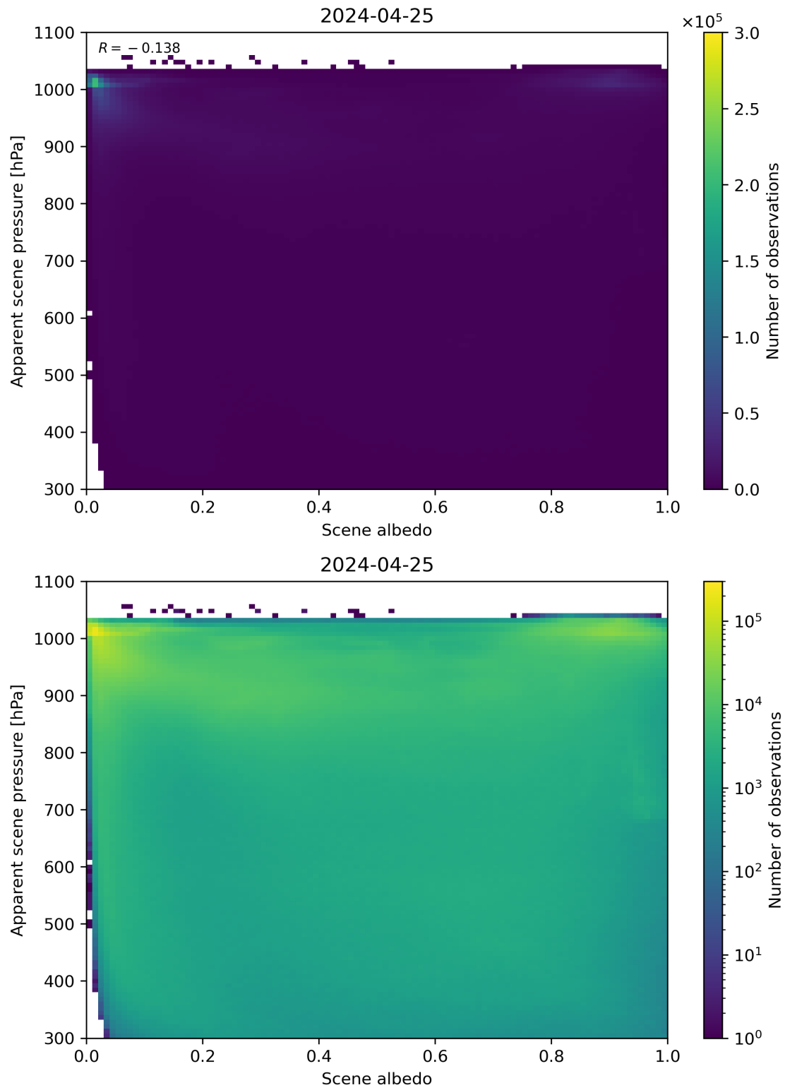
Figure 102: Scatter density plot of “Scene albedo” against “Apparent scene pressure” for 2024-04-24 to 2024-04-26.
