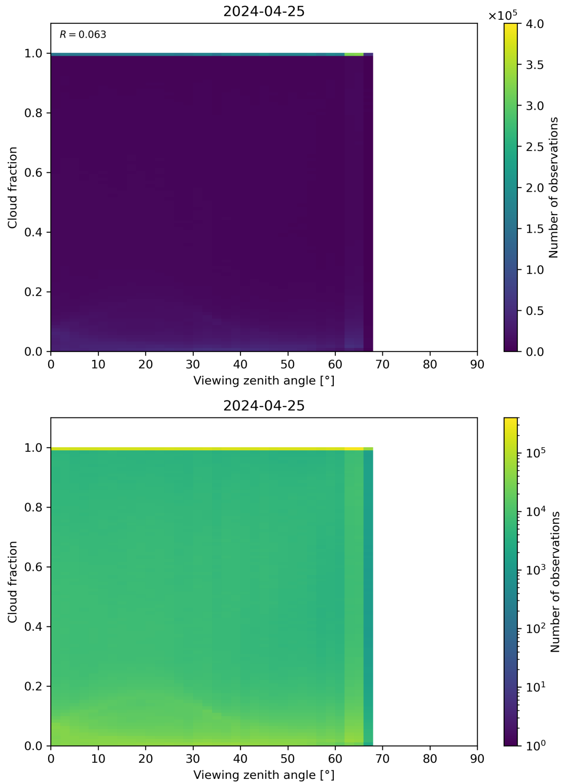
Figure 120: Scatter density plot of “Viewing zenith angle” against “Cloud fraction” for 2024-04-24 to 2024-04-26.
