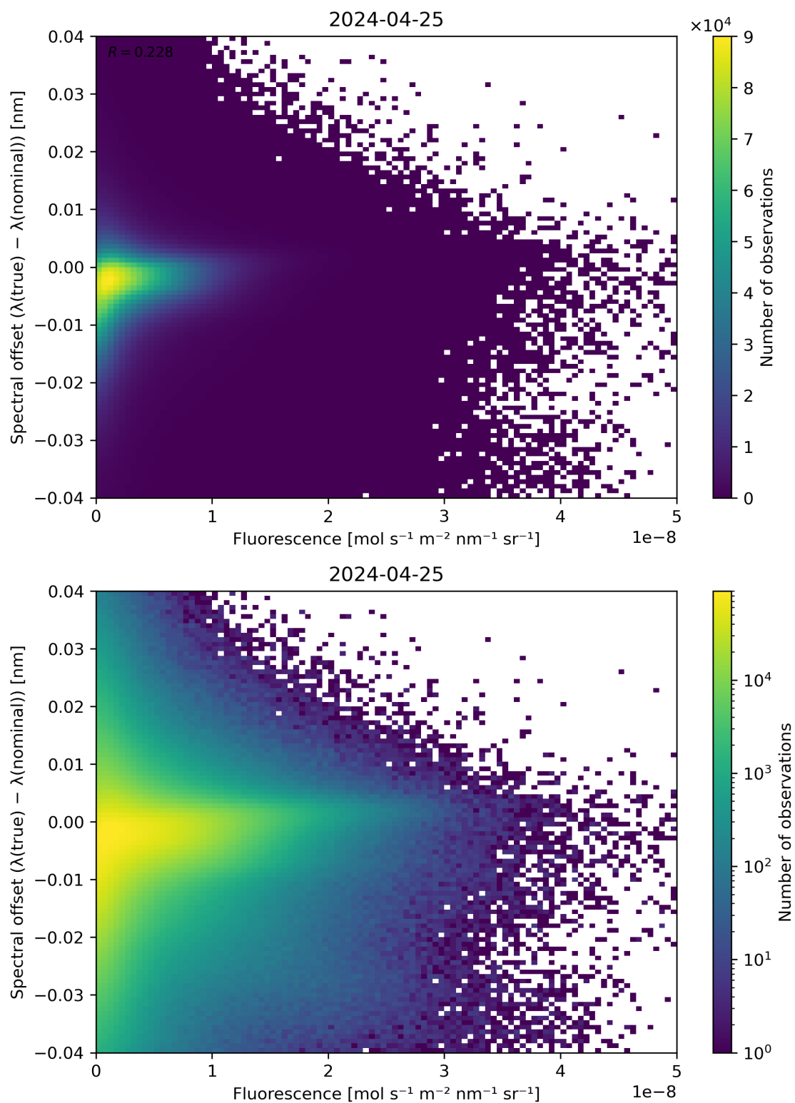
Figure 87: Scatter density plot of “Fluorescence” against “Spectral offset ( \lambda(\text{true}) - \lambda(\text{nominal}) )” for 2024-04-24 to 2024-04-26.
