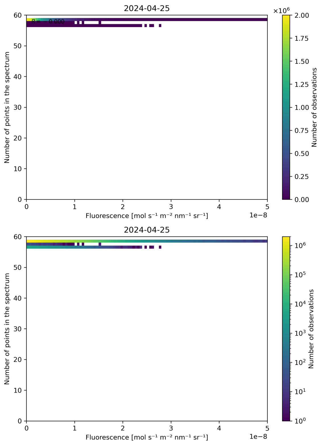
Figure 86: Scatter density plot of “Fluorescence” against “Number of points in the spectrum” for 2024-04-24 to 2024-04-26.
