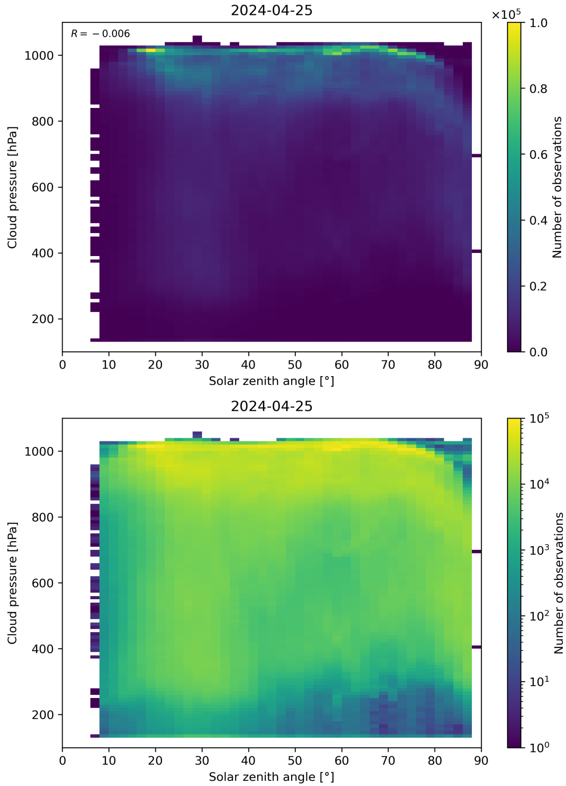
Figure 111: Scatter density plot of “Solar zenith angle” against “Cloud pressure” for 2024-04-24 to 2024-04-26.
