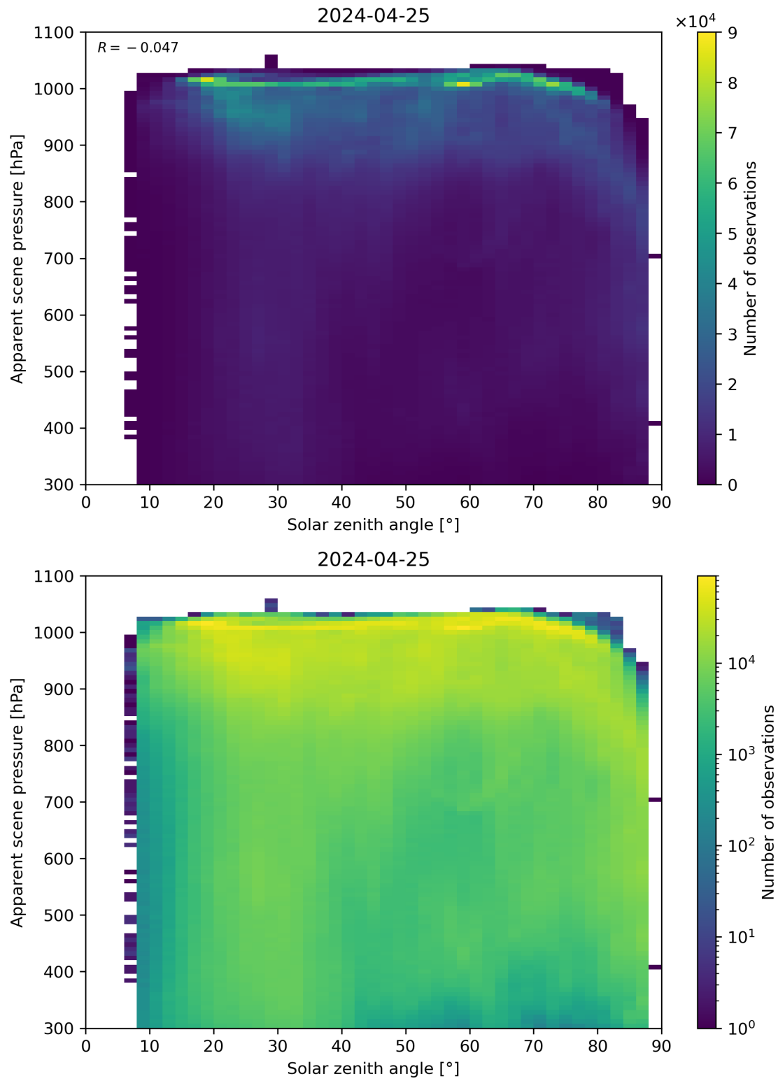
Figure 108: Scatter density plot of “Solar zenith angle” against “Apparent scene pressure” for 2024-04-24 to 2024-04-26.
