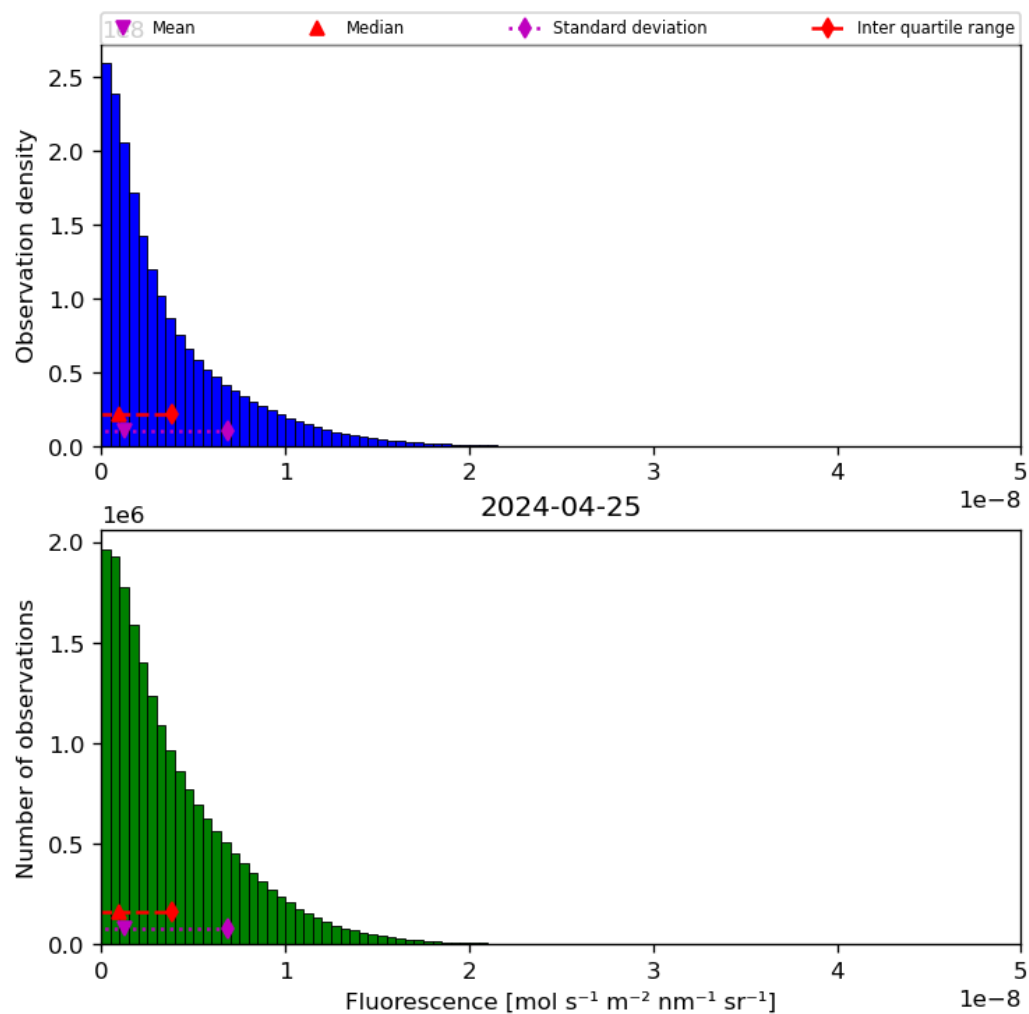
Figure 40: Histogram of “Fluorescence” for 2024-04-24 to 2024-04-26
