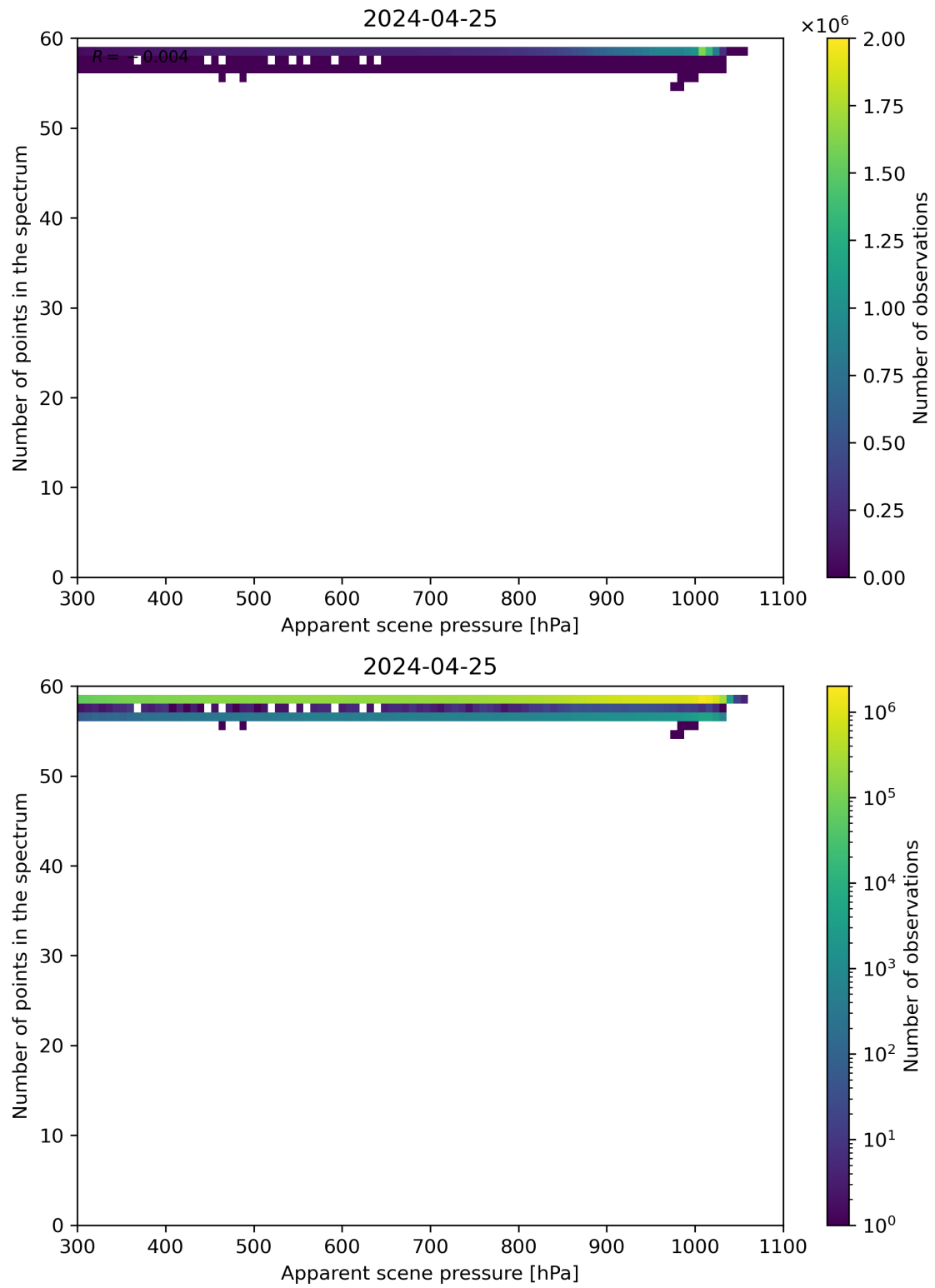
Figure 66: Scatter density plot of “Apparent scene pressure” against “Number of points in the spectrum” for 2024-04-24 to 2024-04-26.
