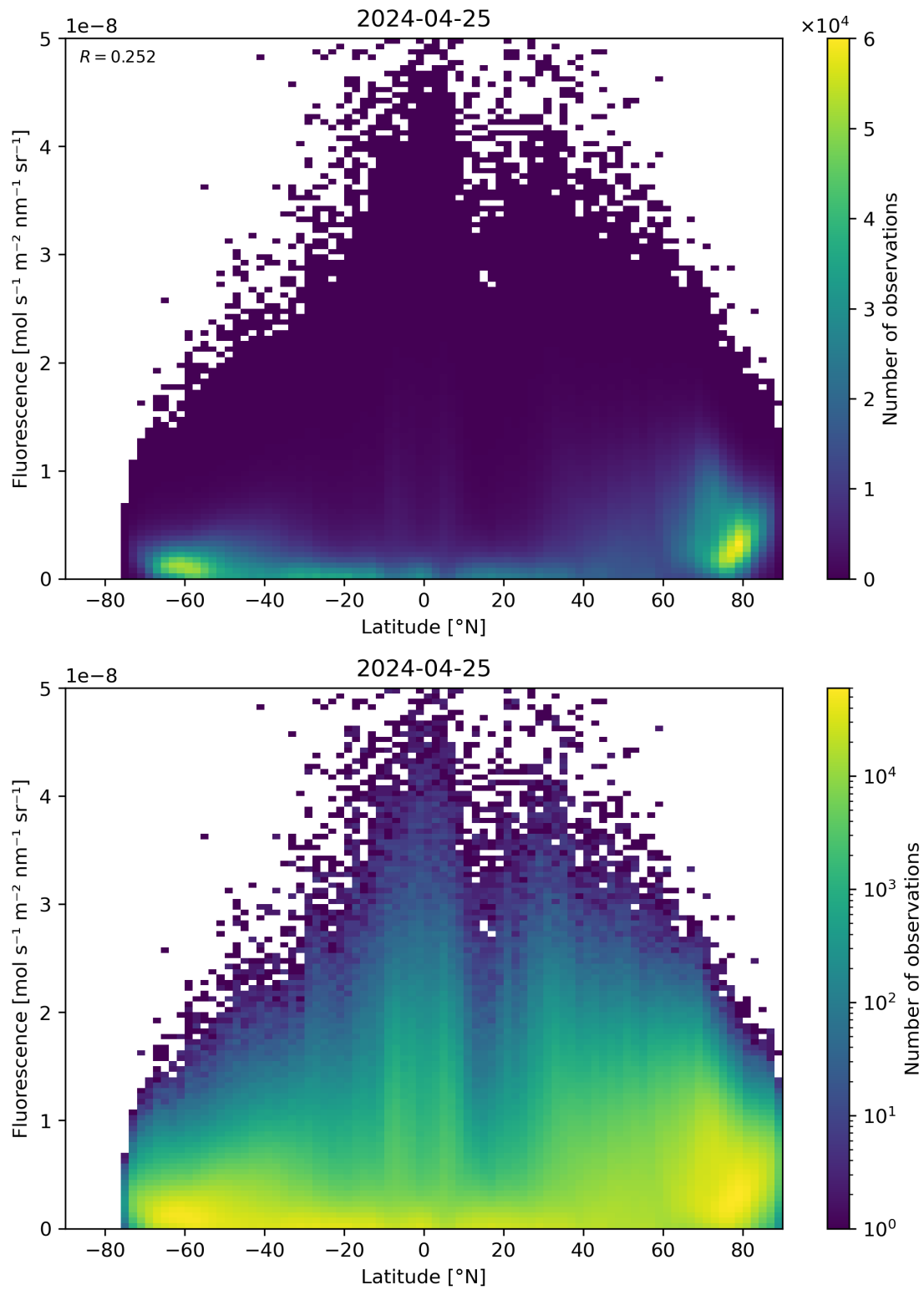
Figure 92: Scatter density plot of “Latitude” against “Fluorescence” for 2024-04-24 to 2024-04-26.
