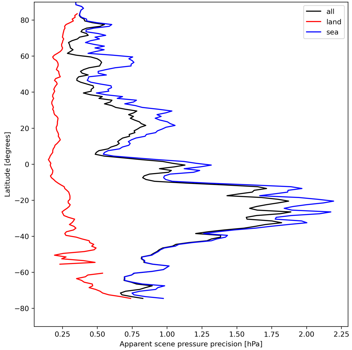
Figure 20: Zonal average of “Apparent scene pressure precision” for 2024-04-24 to 2024-04-26.
