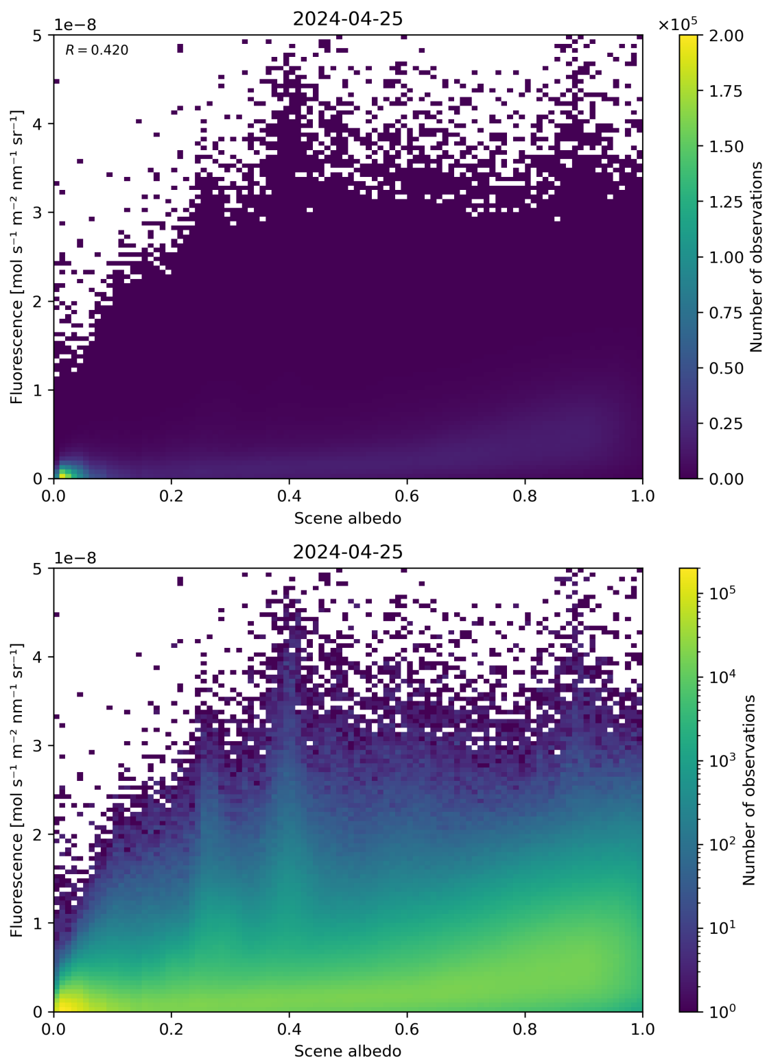
Figure 104: Scatter density plot of “Scene albedo” against “Fluorescence” for 2024-04-24 to 2024-04-26.
