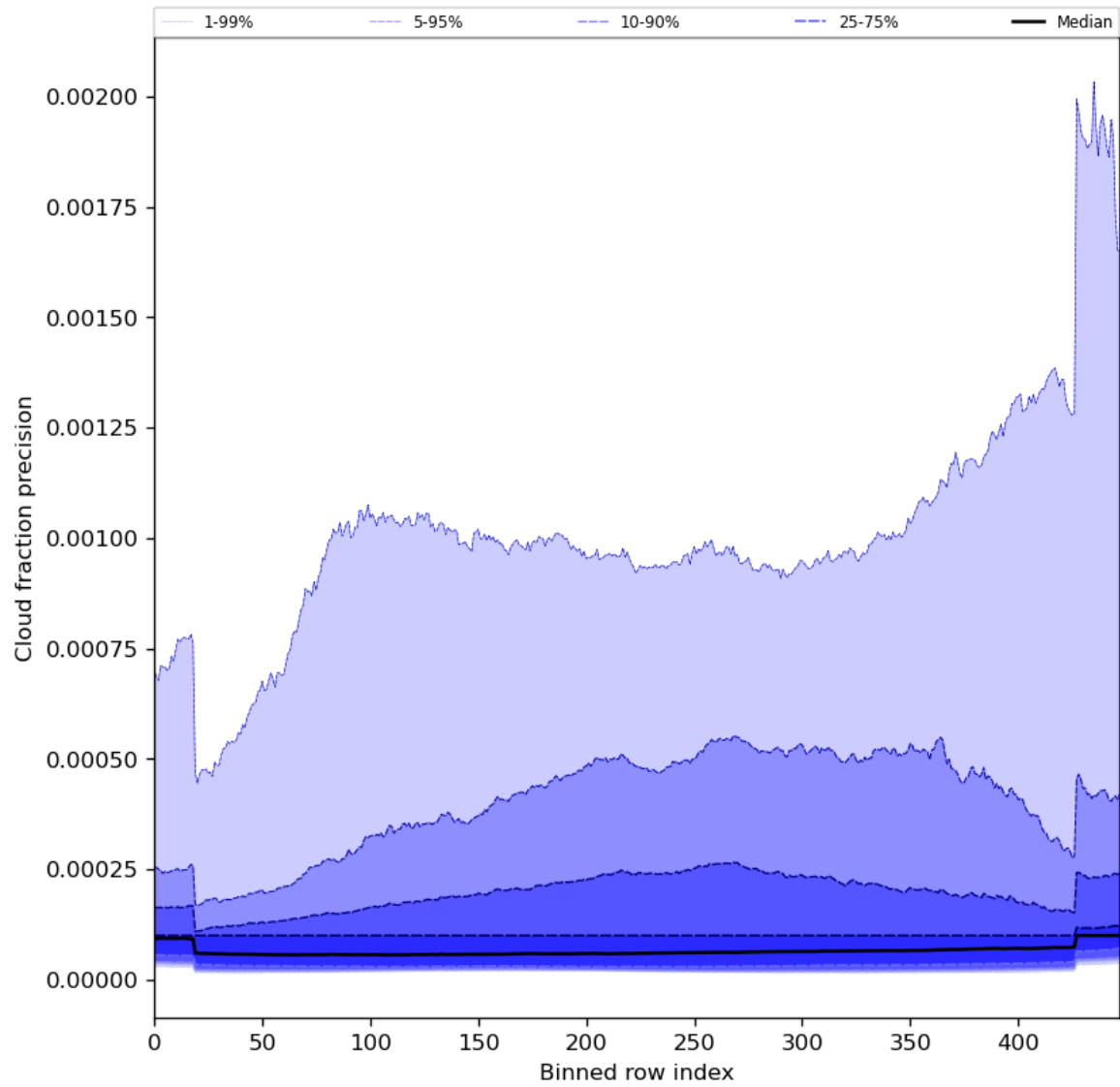
Figure 50: Along track statistics of “Cloud fraction precision” for 2024-04-24 to 2024-04-26
