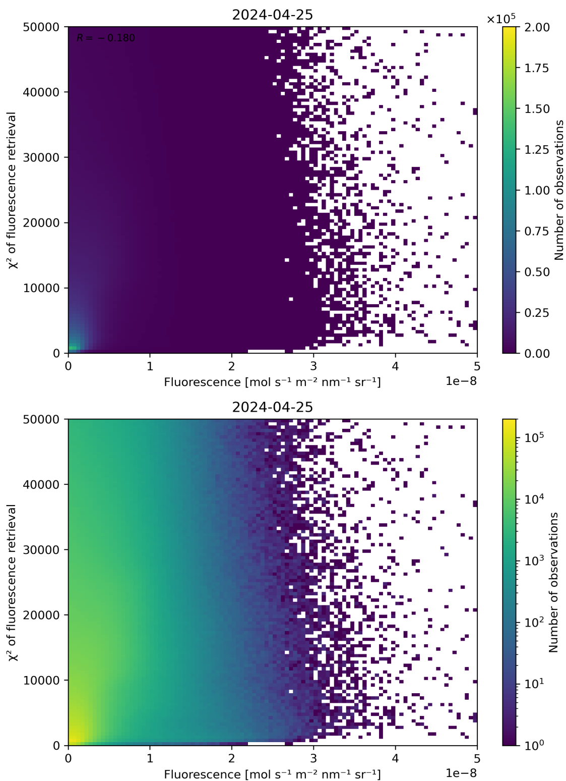
Figure 85: Scatter density plot of “Fluorescence” against “ \chi^2 of fluorescence retrieval” for 2024-04-24 to 2024-04-26.
