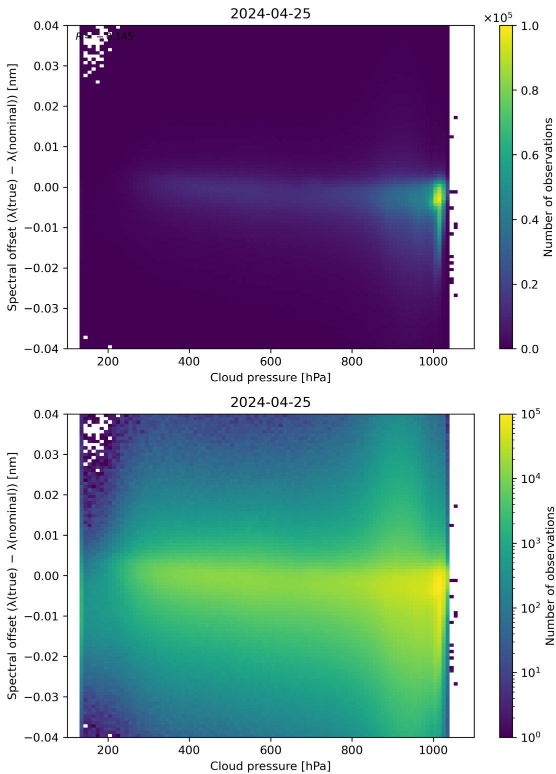
Figure 84: Scatter density plot of “Cloud pressure” against “Spectral offset ( \lambda(\text{true}) - \lambda(\text{nominal}) )” for 2024-04-24 to 2024-04-26.
