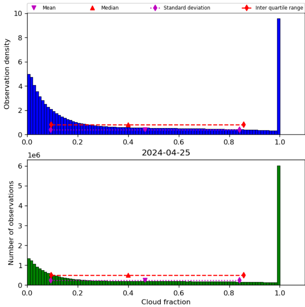
Figure 32: Histogram of “Cloud fraction” for 2024-04-24 to 2024-04-26
