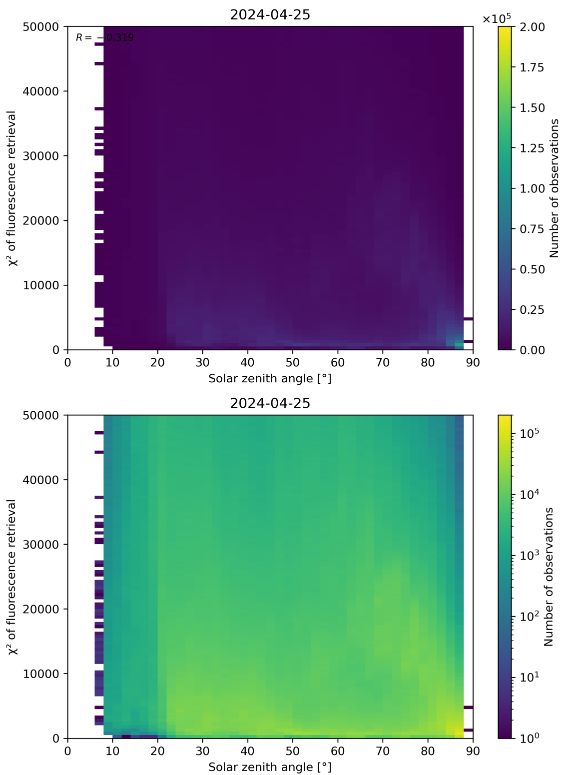
Figure 109: Scatter density plot of “Solar zenith angle” against “ \chi^2 of fluorescence retrieval” for 2024-04-24 to 2024-04-26.
