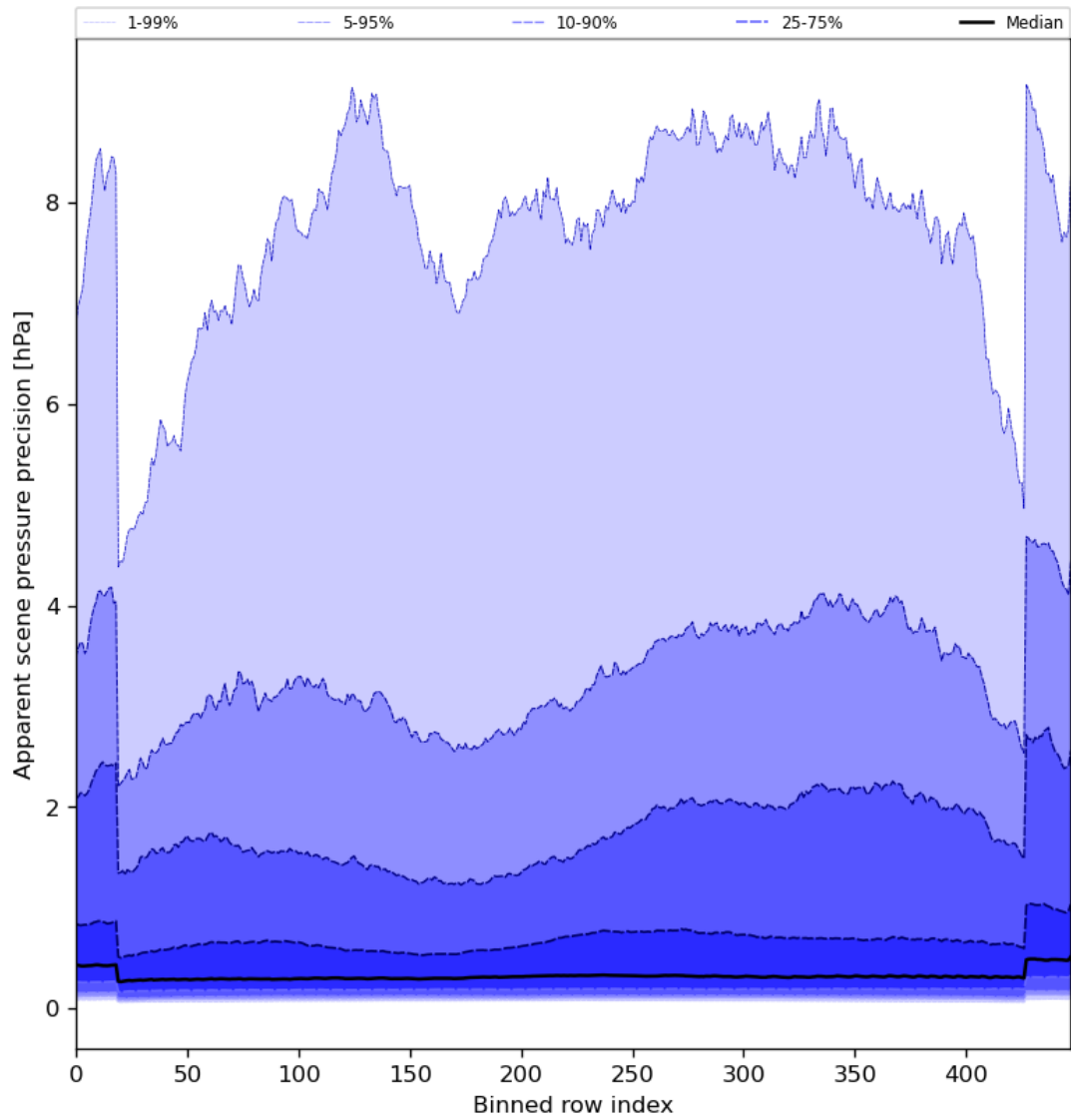
Figure 54: Along track statistics of “Apparent scene pressure precision” for 2024-04-24 to 2024-04-26
