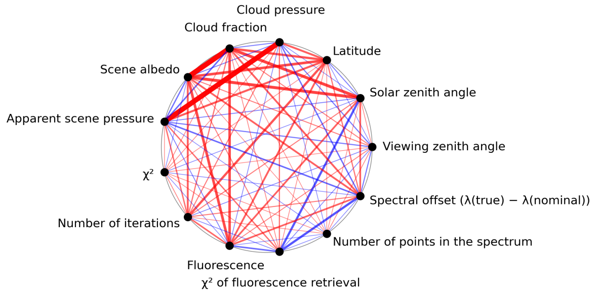
Figure 1: Map of correlation graph for 2024-04-24 to 2024-04-26.
