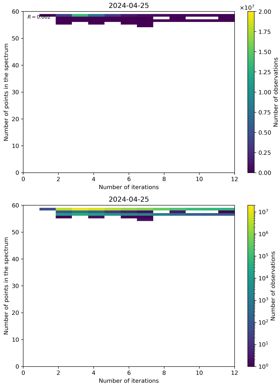
Figure 99: Scatter density plot of “Number of iterations” against “Number of points in the spectrum” for 2024-04-24 to 2024-04-26.
