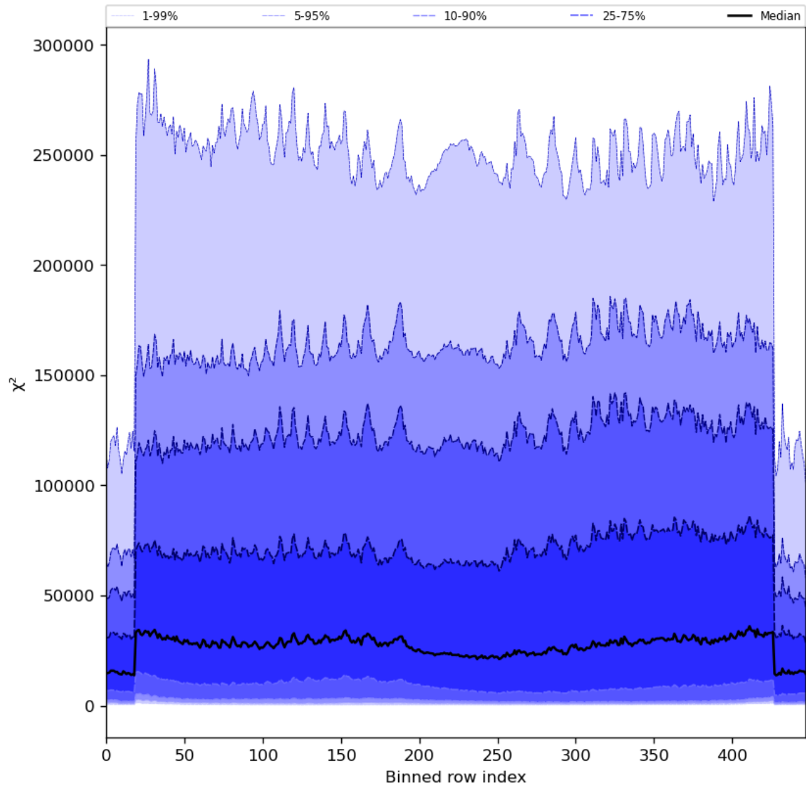
Figure 55: Along track statistics of “ \chi^2 ” for 2024-04-24 to 2024-04-26
