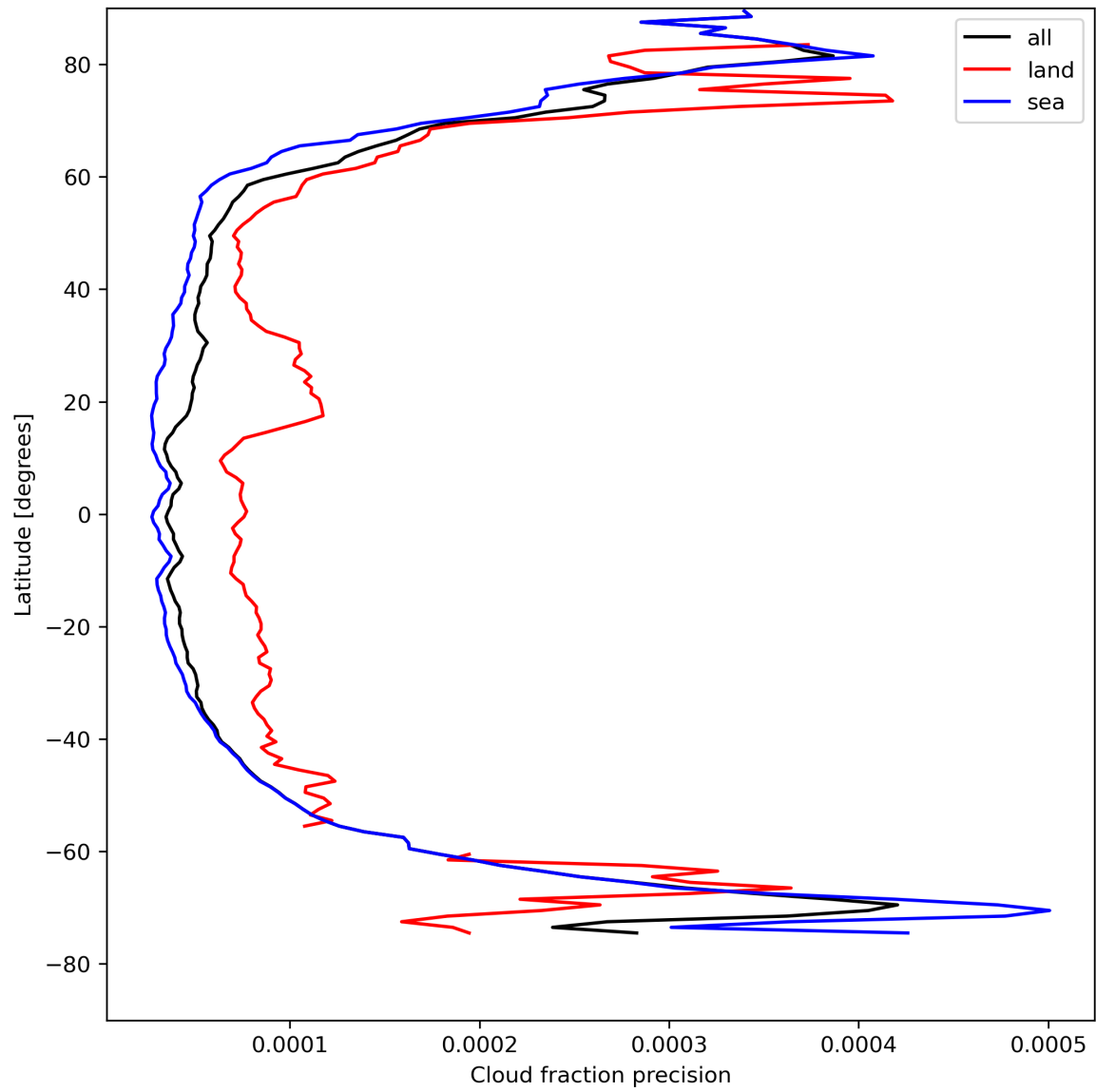
Figure 16: Zonal average of “Cloud fraction precision” for 2024-04-24 to 2024-04-26.
