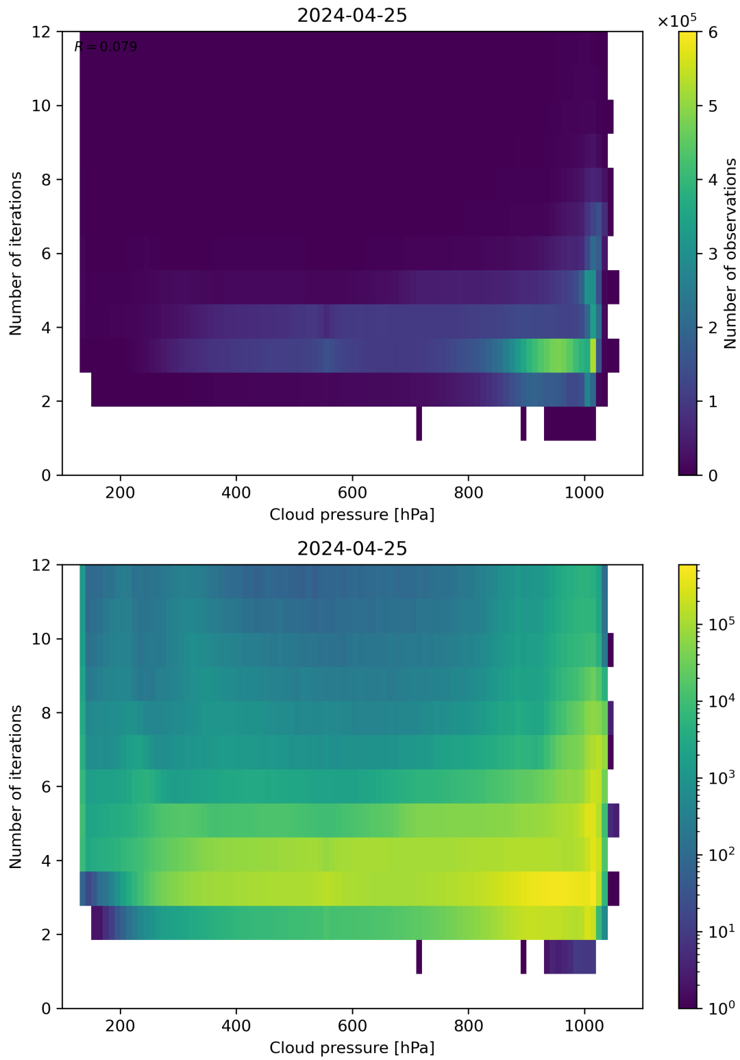
Figure 81: Scatter density plot of “Cloud pressure” against “Number of iterations” for 2024-04-24 to 2024-04-26.
