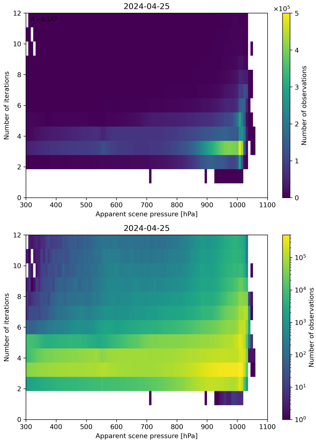
Figure 65: Scatter density plot of “Apparent scene pressure” against “Number of iterations” for 2024-04-24 to 2024-04-26.
