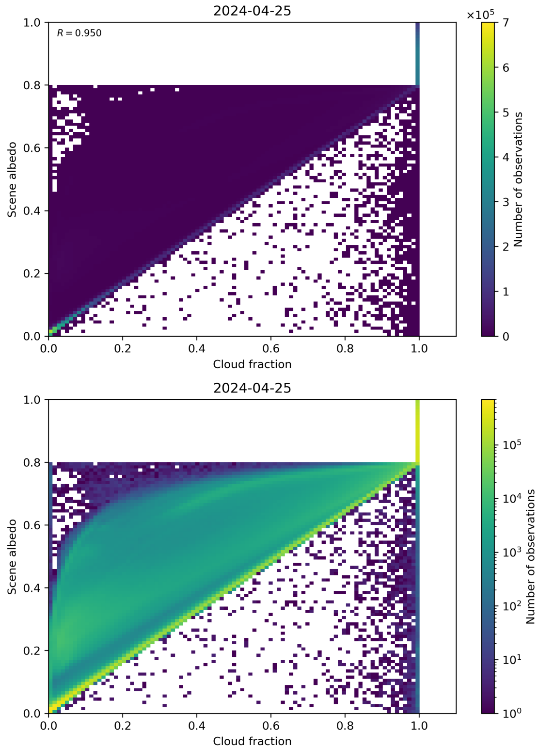
Figure 75: Scatter density plot of “Cloud fraction” against “Scene albedo” for 2024-04-24 to 2024-04-26.
