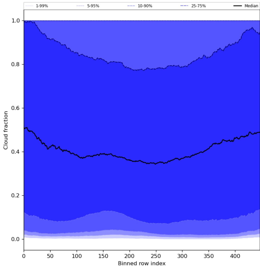
Figure 49: Along track statistics of “Cloud fraction” for 2024-04-24 to 2024-04-26
