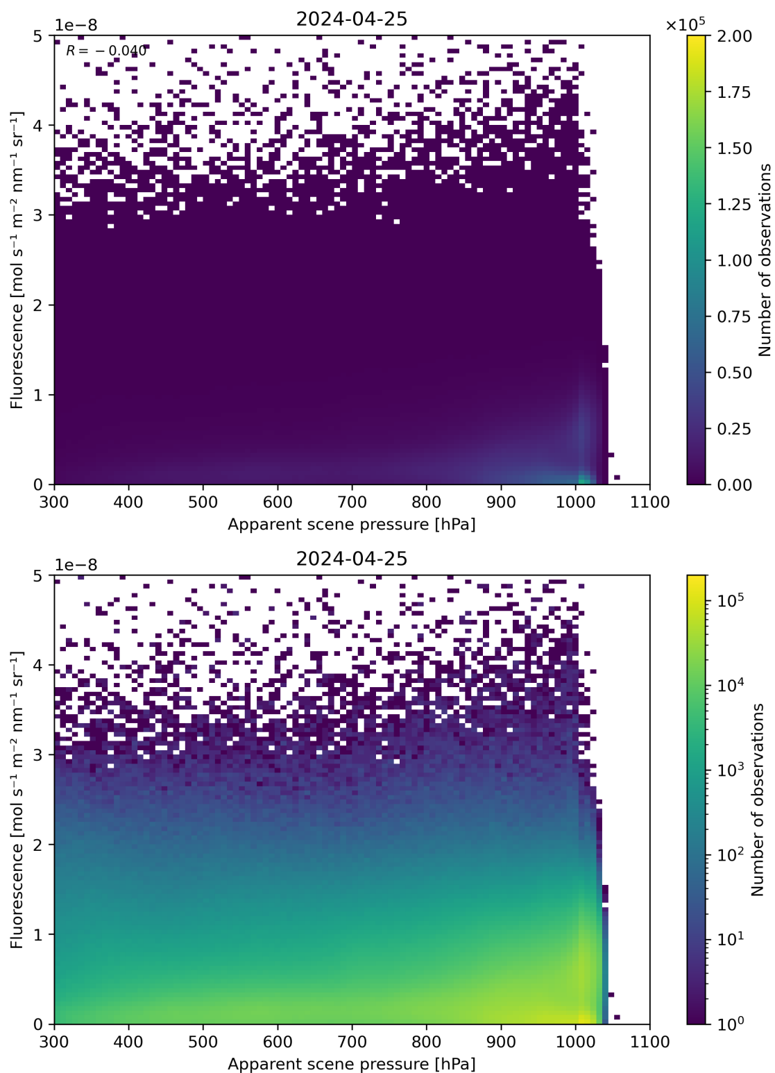
Figure 64: Scatter density plot of “Apparent scene pressure” against “Fluorescence” for 2024-04-24 to 2024-04-26.
