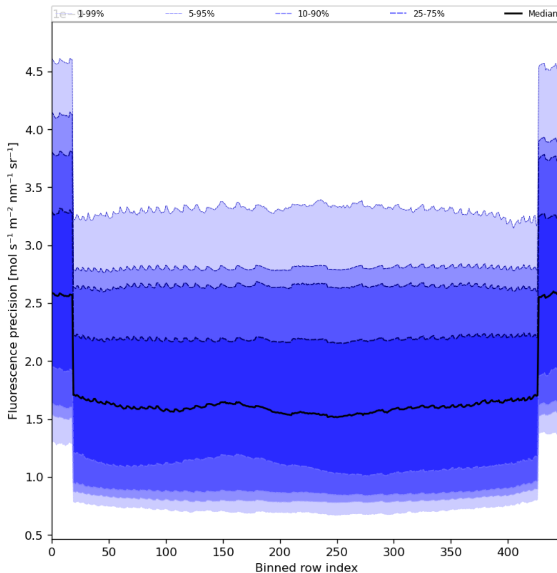
Figure 58: Along track statistics of “Fluorescence precision” for 2024-04-24 to 2024-04-26
