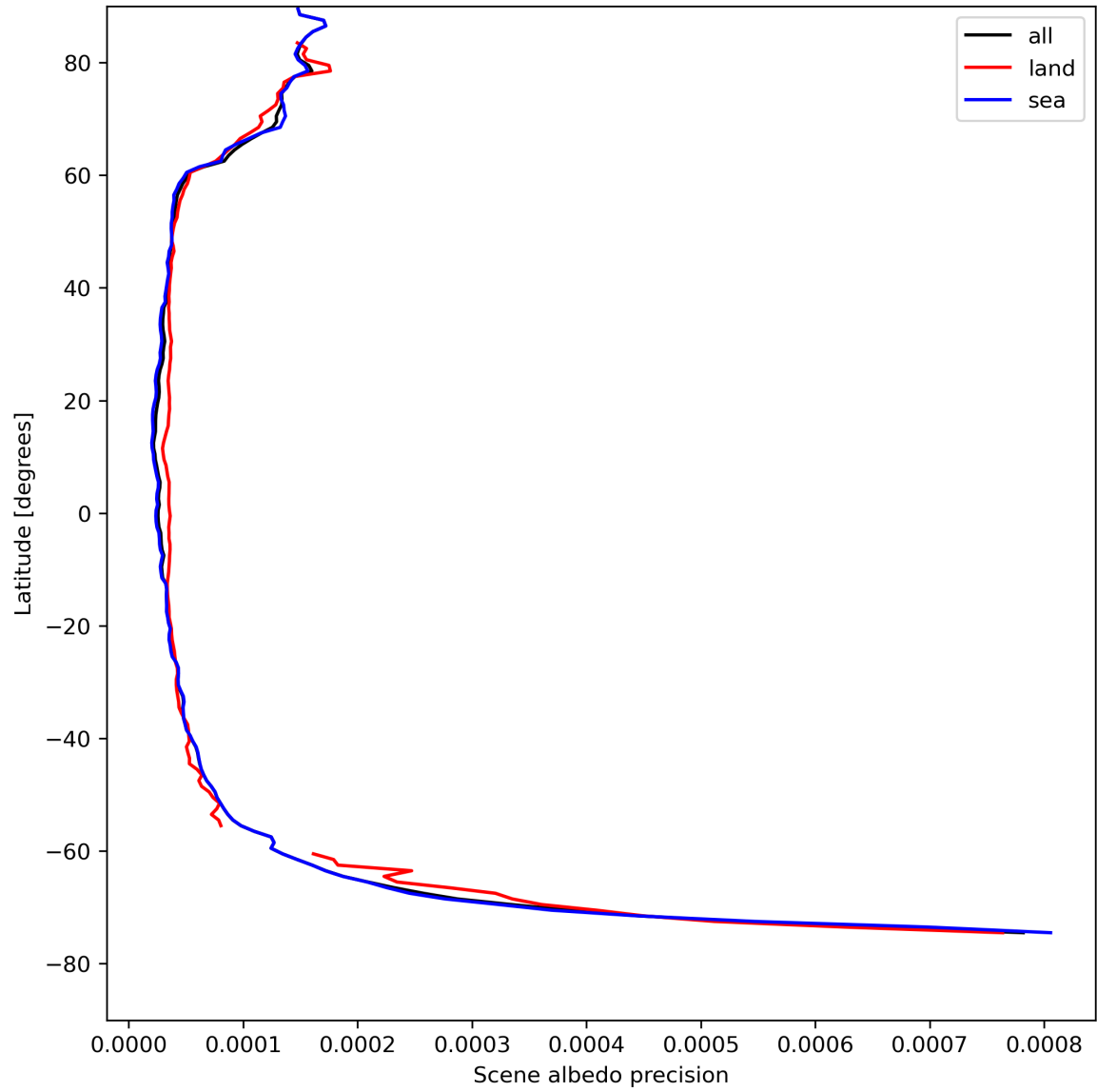
Figure 18: Zonal average of “Scene albedo precision” for 2024-04-24 to 2024-04-26.
