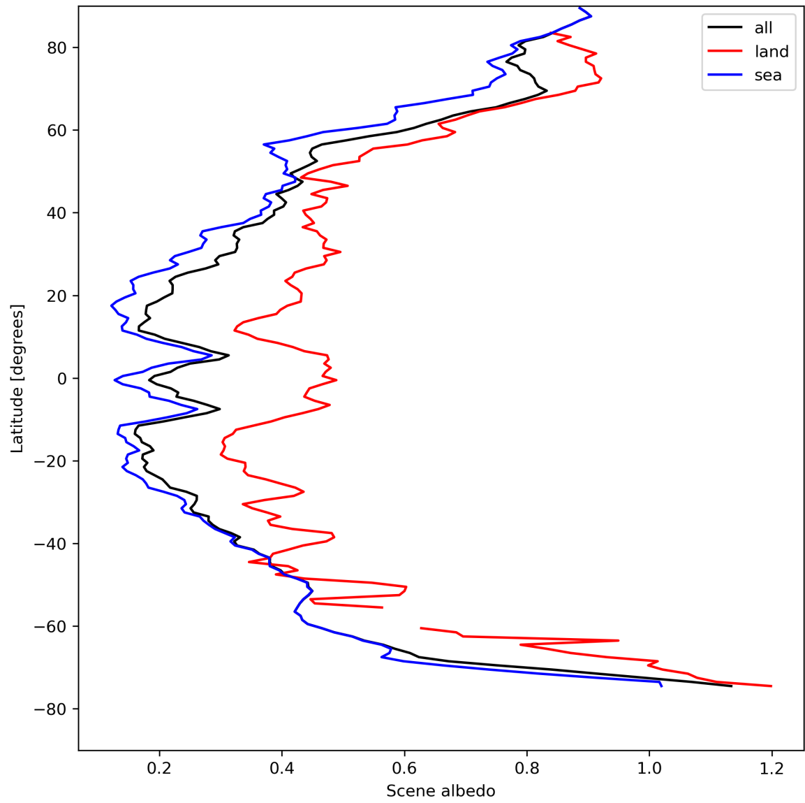
Figure 17: Zonal average of “Scene albedo” for 2024-04-24 to 2024-04-26.
