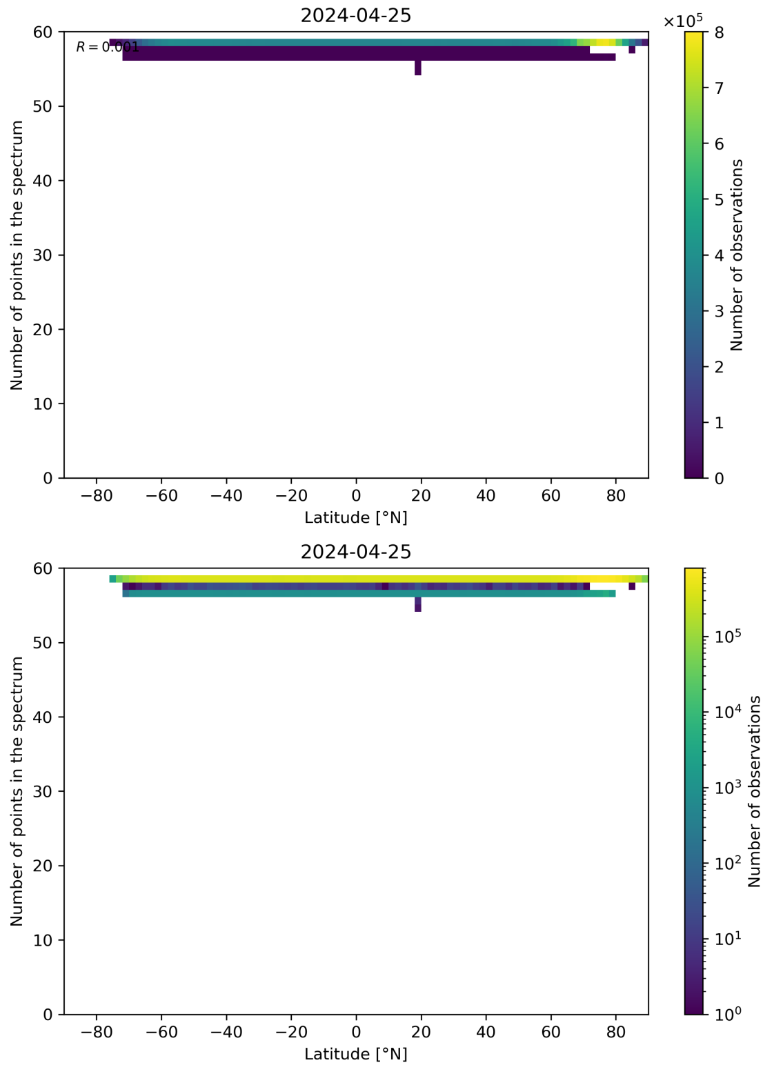
Figure 94: Scatter density plot of “Latitude” against “Number of points in the spectrum” for 2024-04-24 to 2024-04-26.
