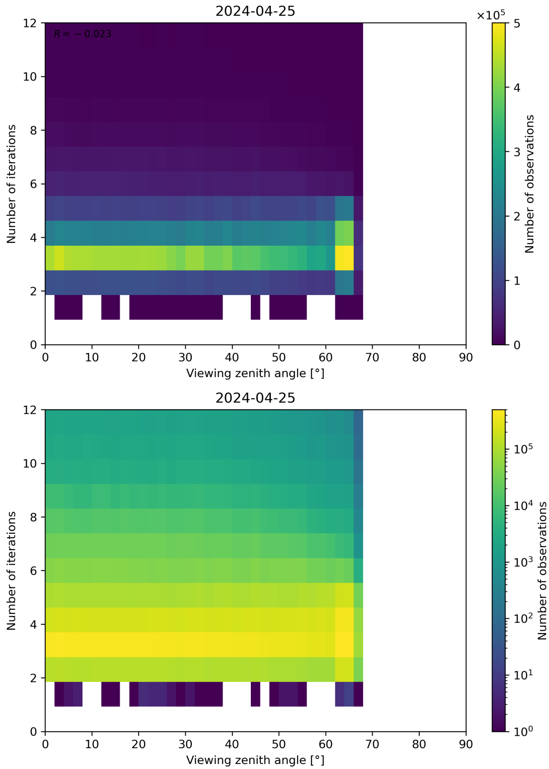
Figure 124: Scatter density plot of “Viewing zenith angle” against “Number of iterations” for 2024-04-24 to 2024-04-26.
