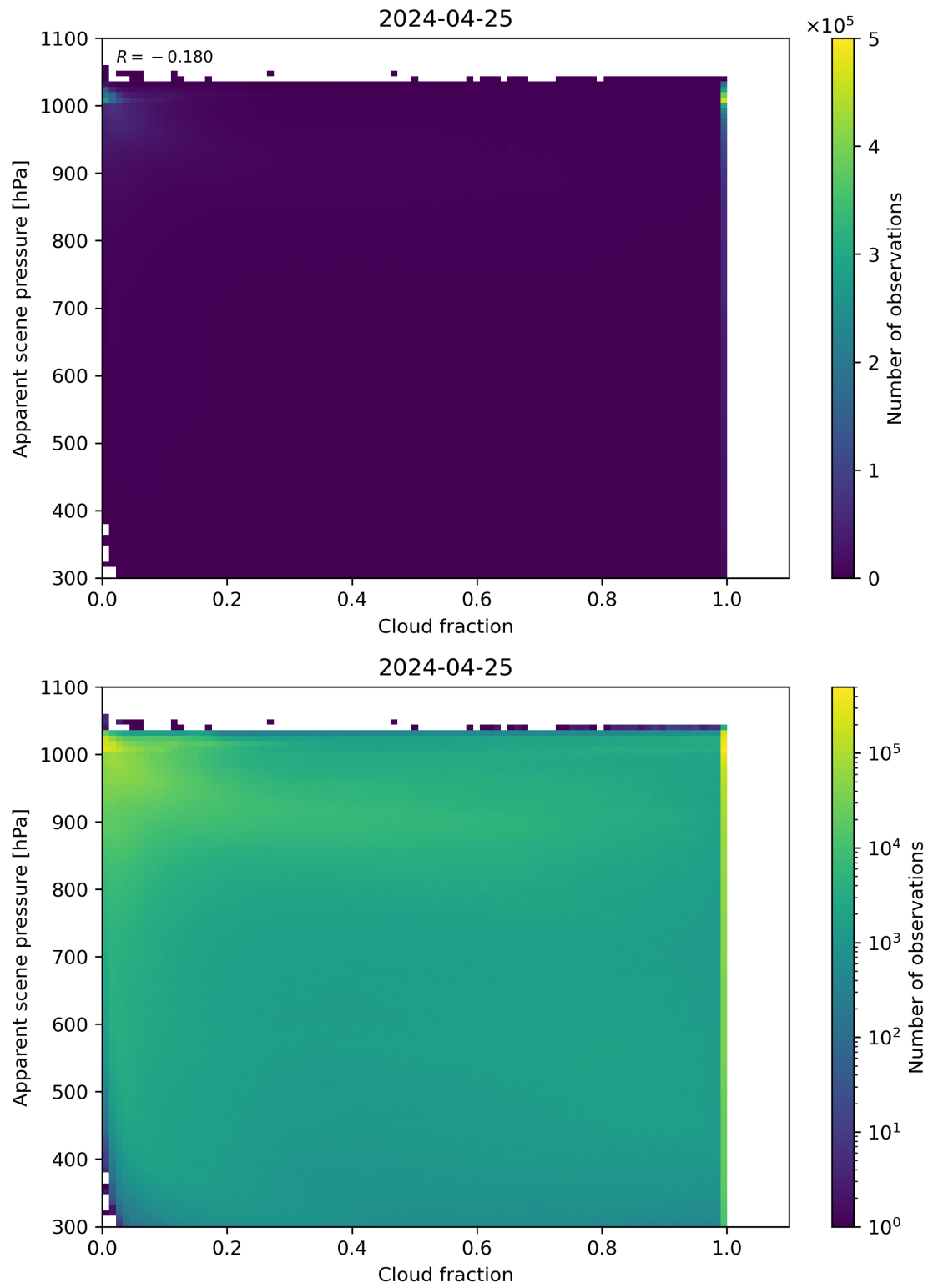
Figure 70: Scatter density plot of “Cloud fraction” against “Apparent scene pressure” for 2024-04-24 to 2024-04-26.
