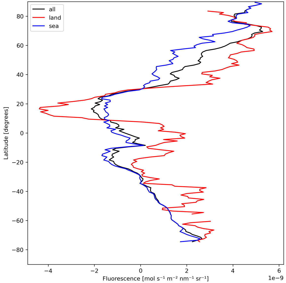
Figure 23: Zonal average of “Fluorescence” for 2024-04-26 to 2024-04-27.
