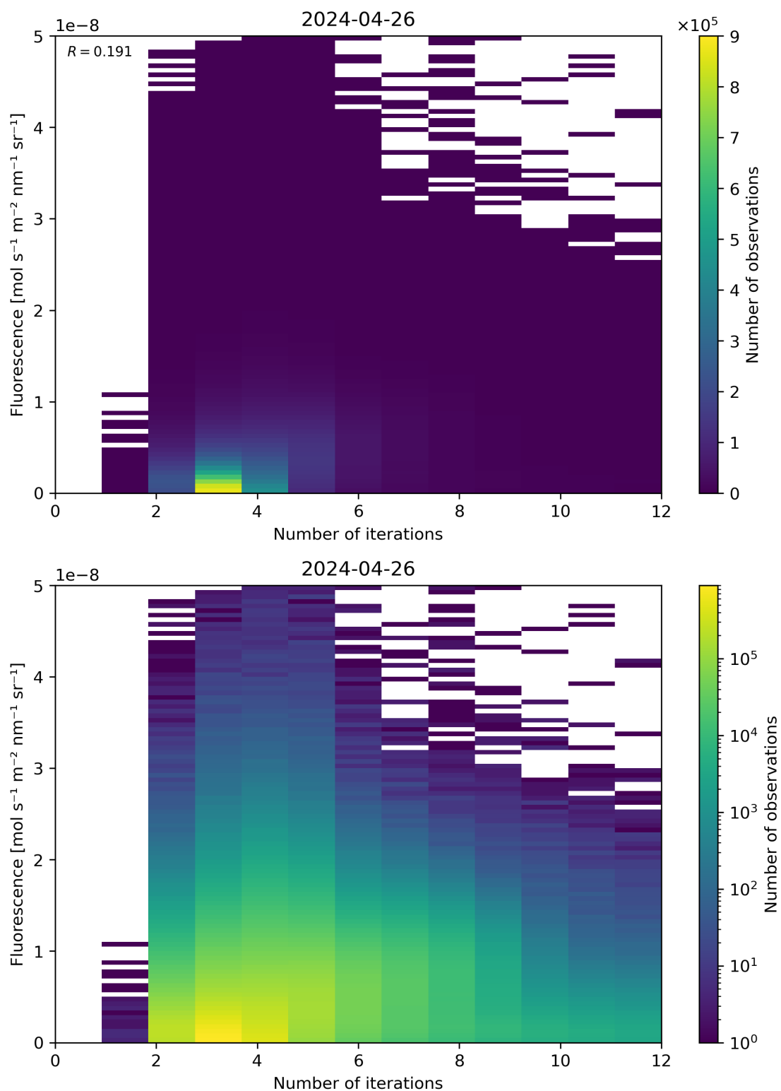
Figure 98: Scatter density plot of “Number of iterations” against “Fluorescence” for 2024-04-26 to 2024-04-27.
