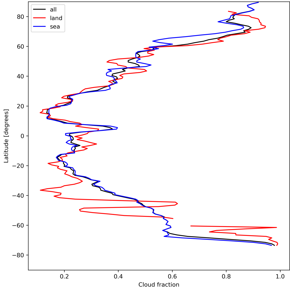
Figure 15: Zonal average of “Cloud fraction” for 2024-04-26 to 2024-04-28.
