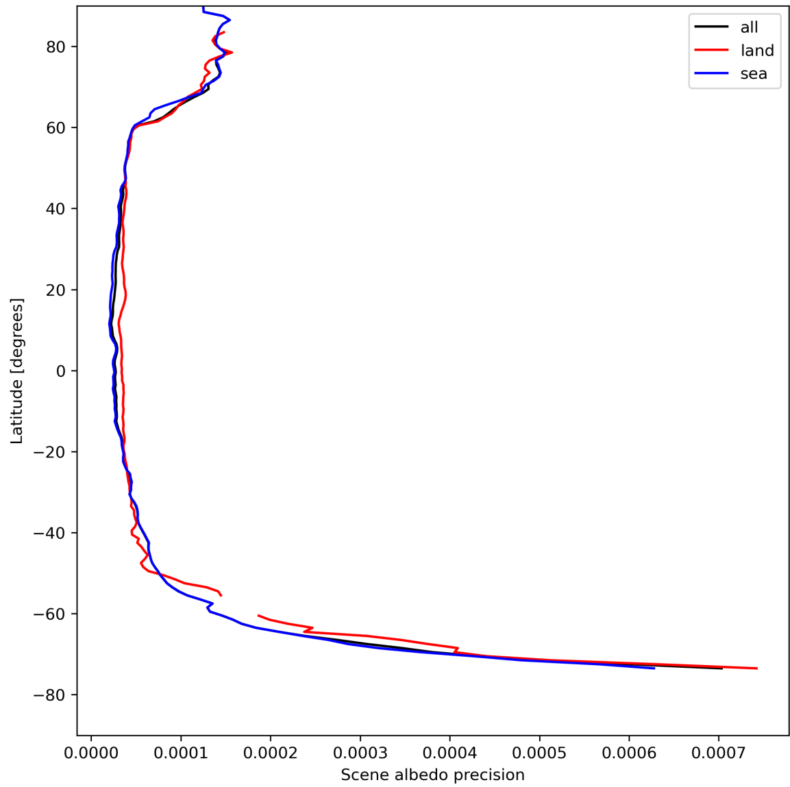
Figure 18: Zonal average of “Scene albedo precision” for 2024-04-26 to 2024-04-28.
