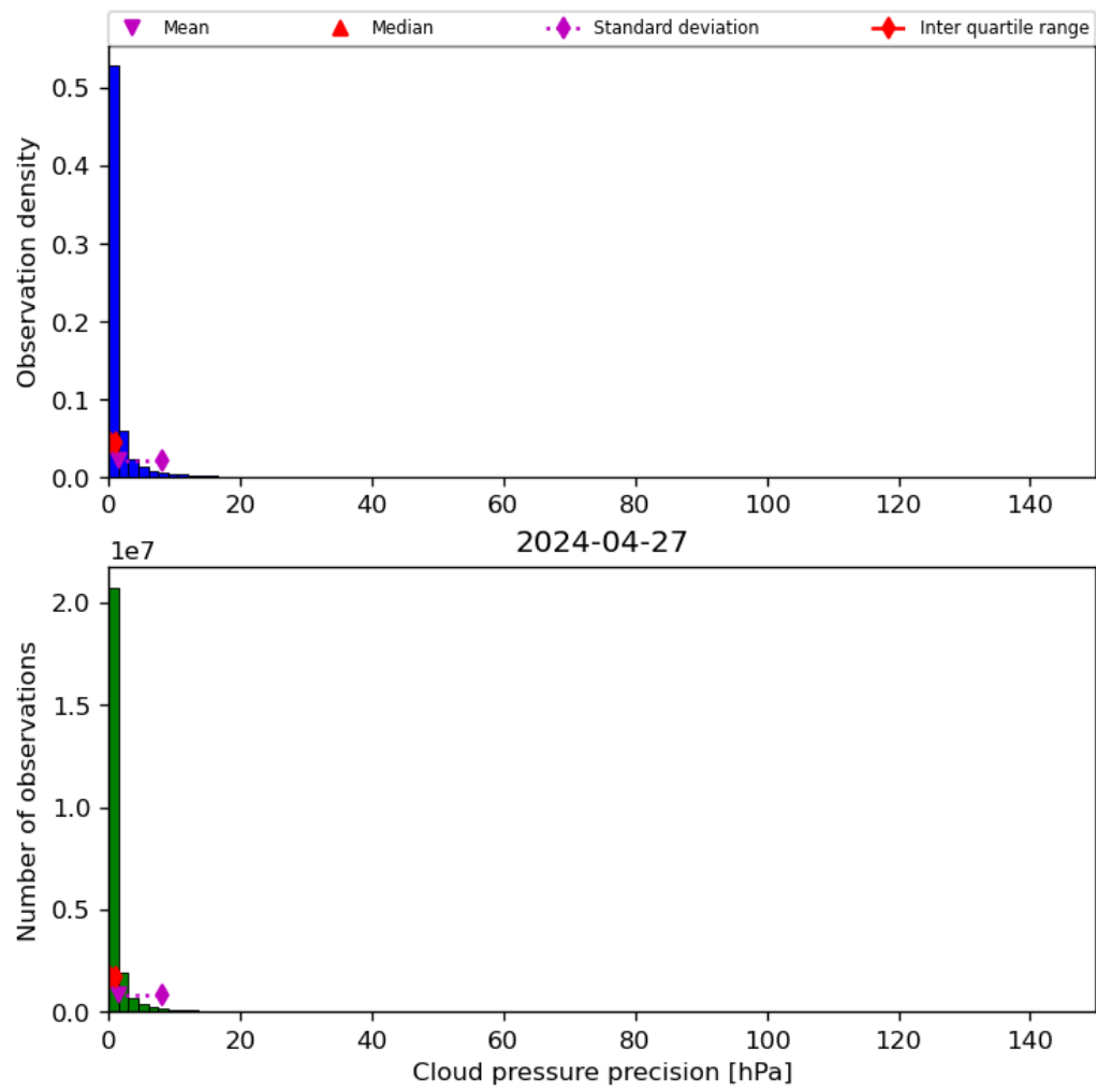
Figure 31: Histogram of "Cloud pressure precision" for 2024-04-26 to 2024-04-28
