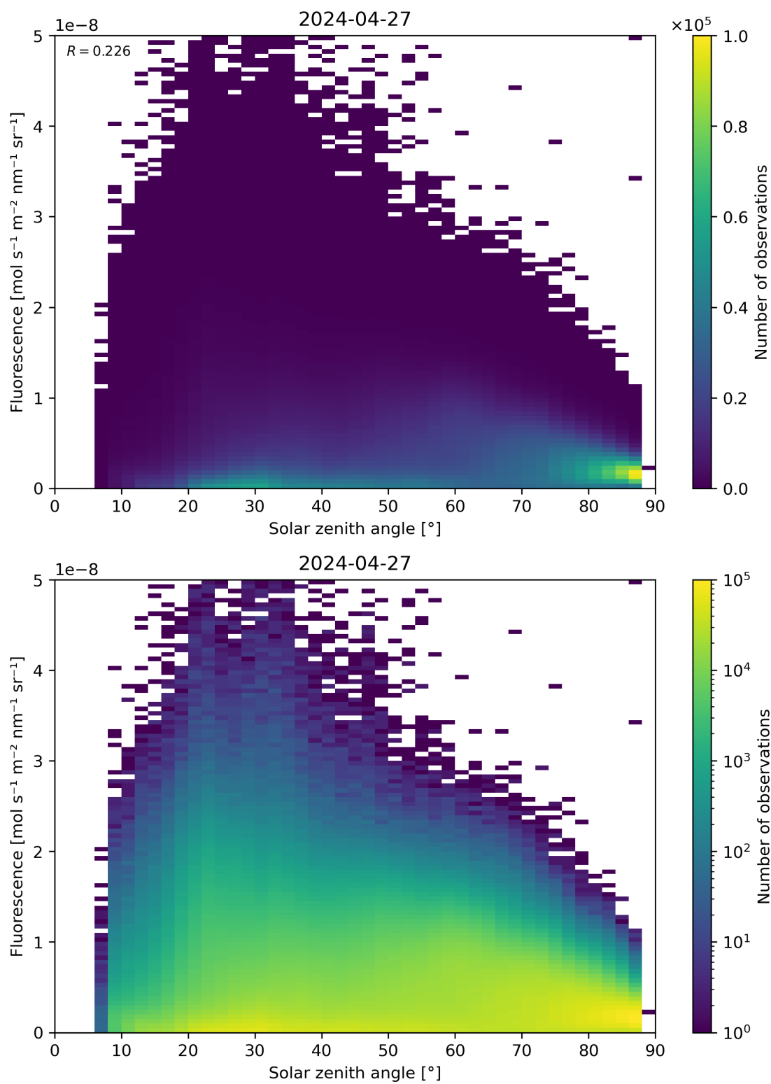
Figure 112: Scatter density plot of “Solar zenith angle” against “Fluorescence” for 2024-04-26 to 2024-04-28.
