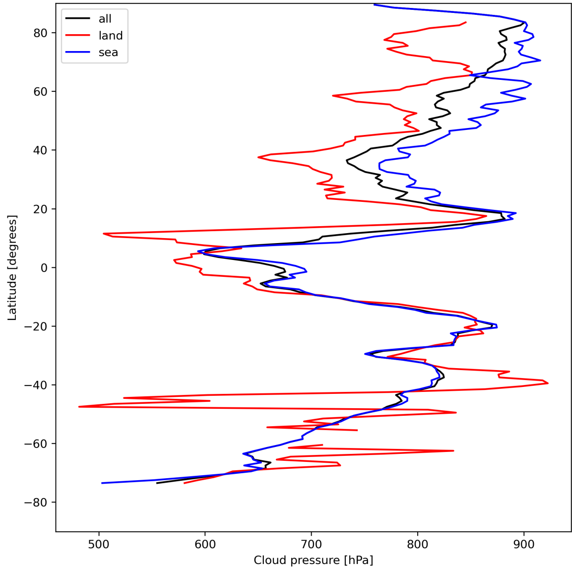
Figure 13: Zonal average of “Cloud pressure” for 2024-04-26 to 2024-04-28.
