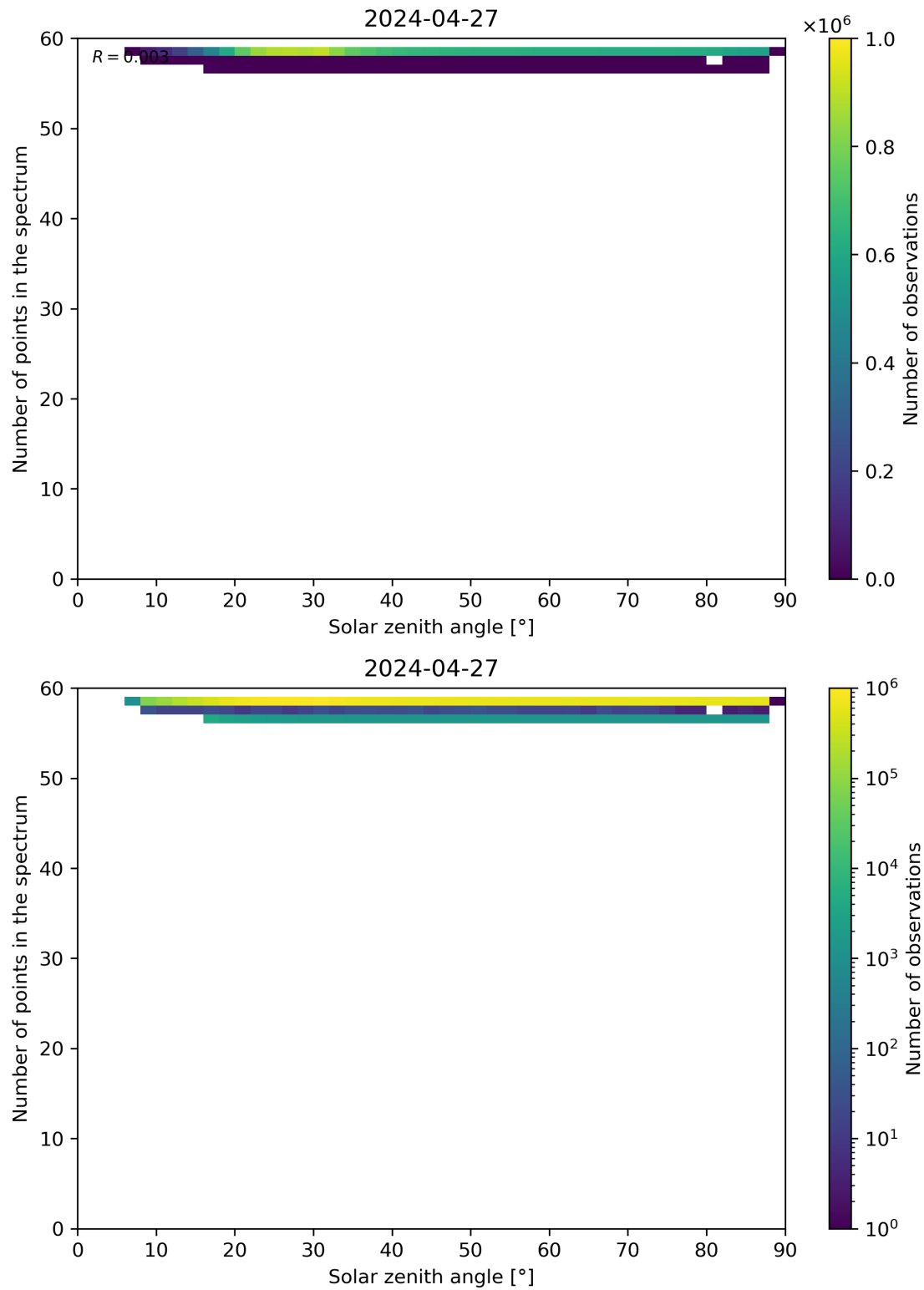
Figure 115: Scatter density plot of “Solar zenith angle” against “Number of points in the spectrum” for 2024-04-26 to 2024-04-28.
