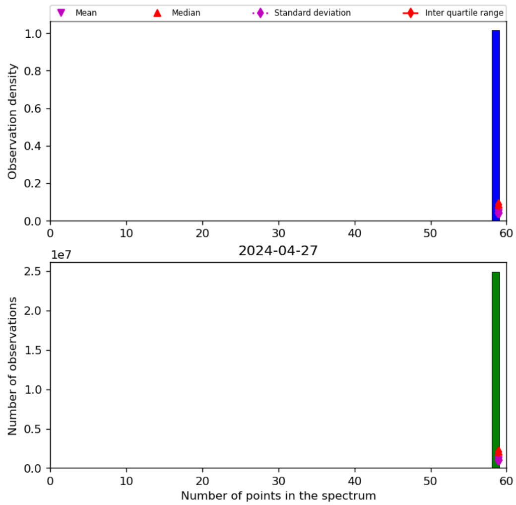
Figure 44: Histogram of “Number of points in the spectrum” for 2024-04-26 to 2024-04-28
