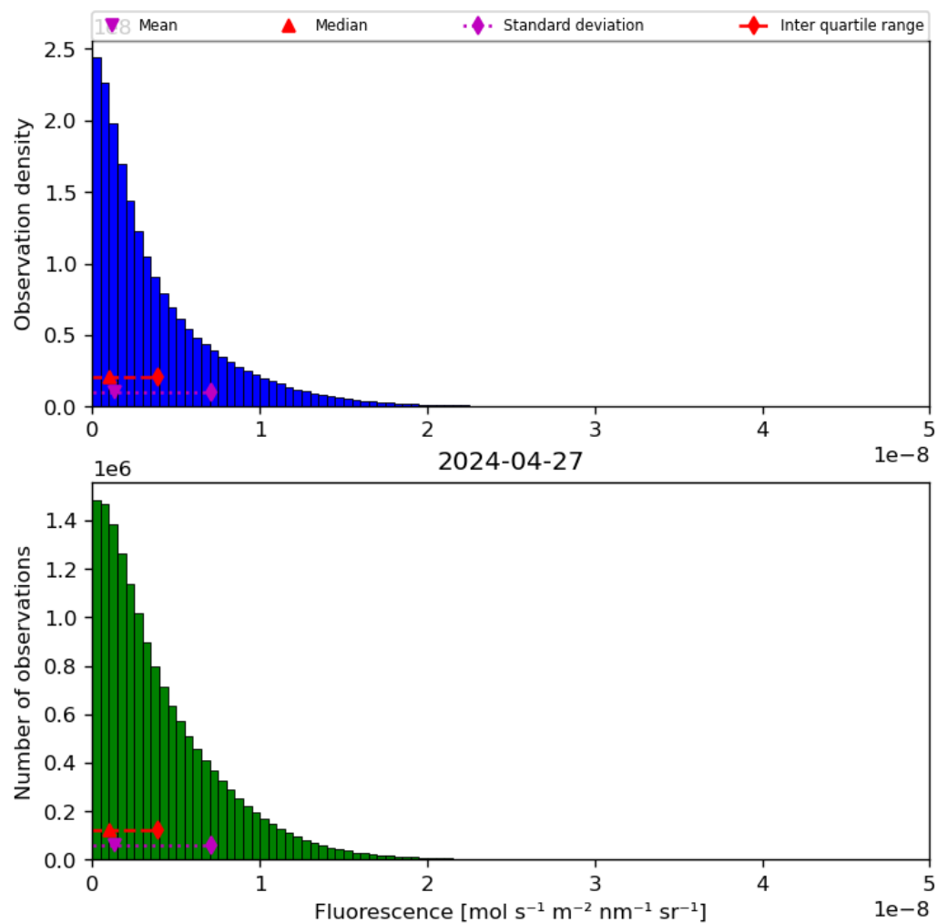
Figure 40: Histogram of “Fluorescence” for 2024-04-26 to 2024-04-28
