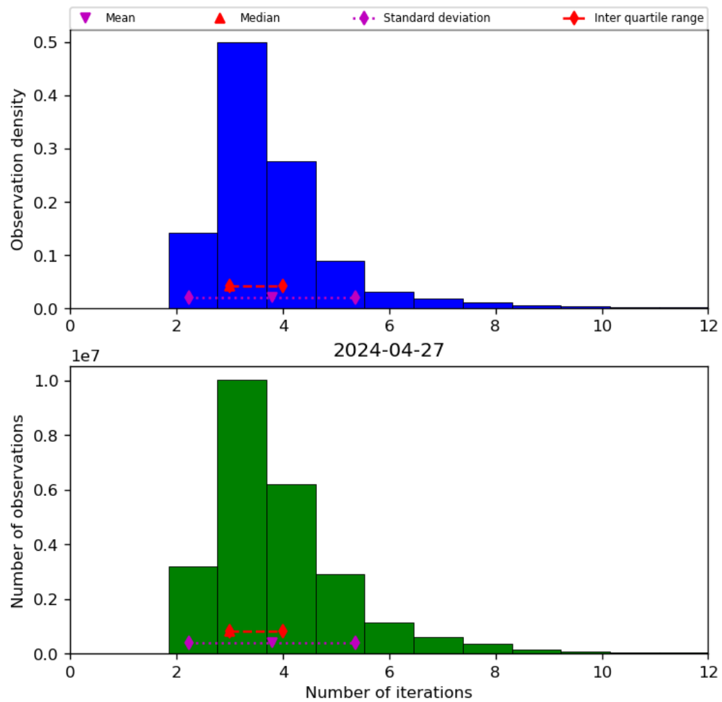
Figure 39: Histogram of “Number of iterations” for 2024-04-26 to 2024-04-28
