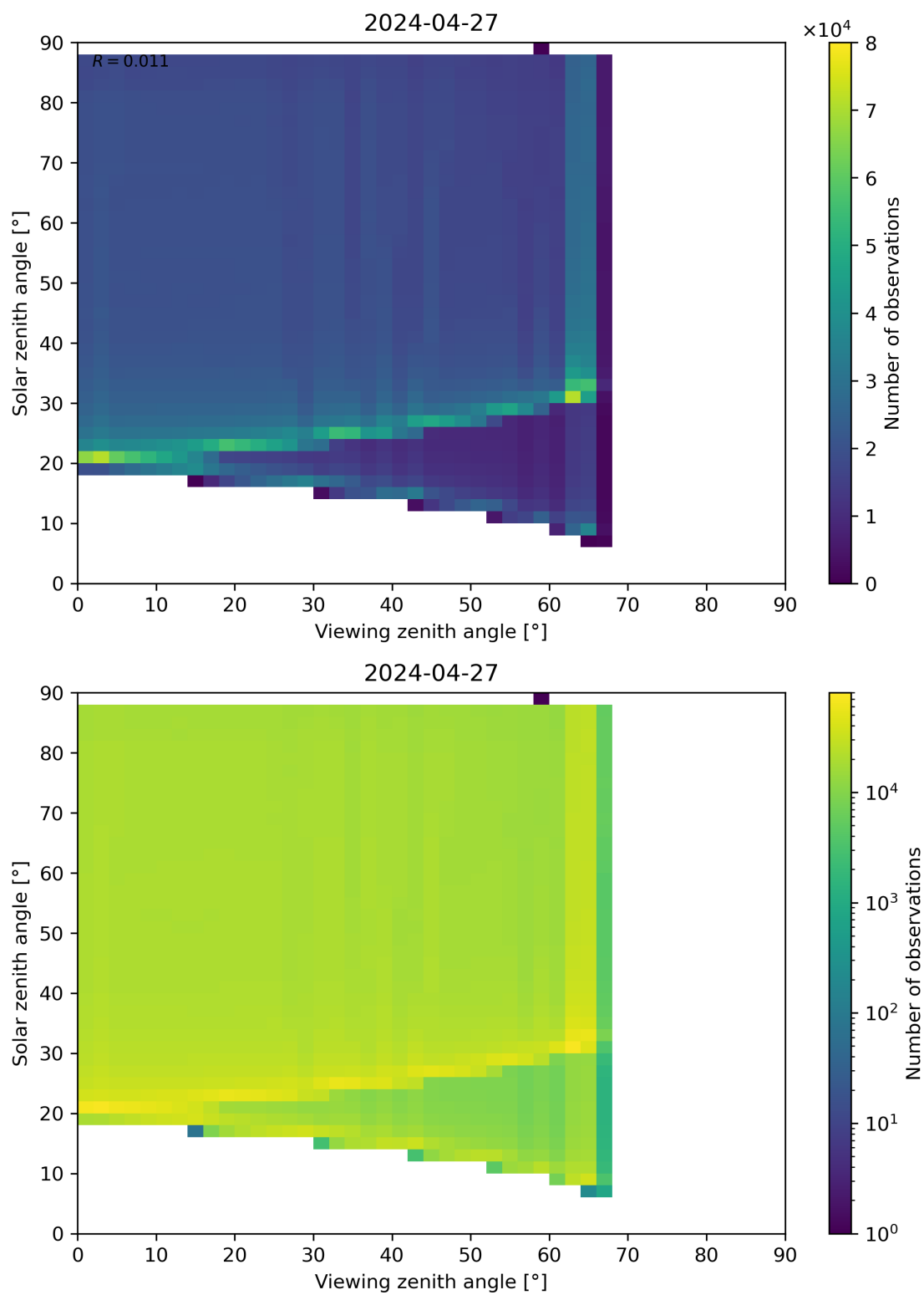
Figure 127: Scatter density plot of “Viewing zenith angle” against “Solar zenith angle” for 2024-04-26 to 2024-04-28.
