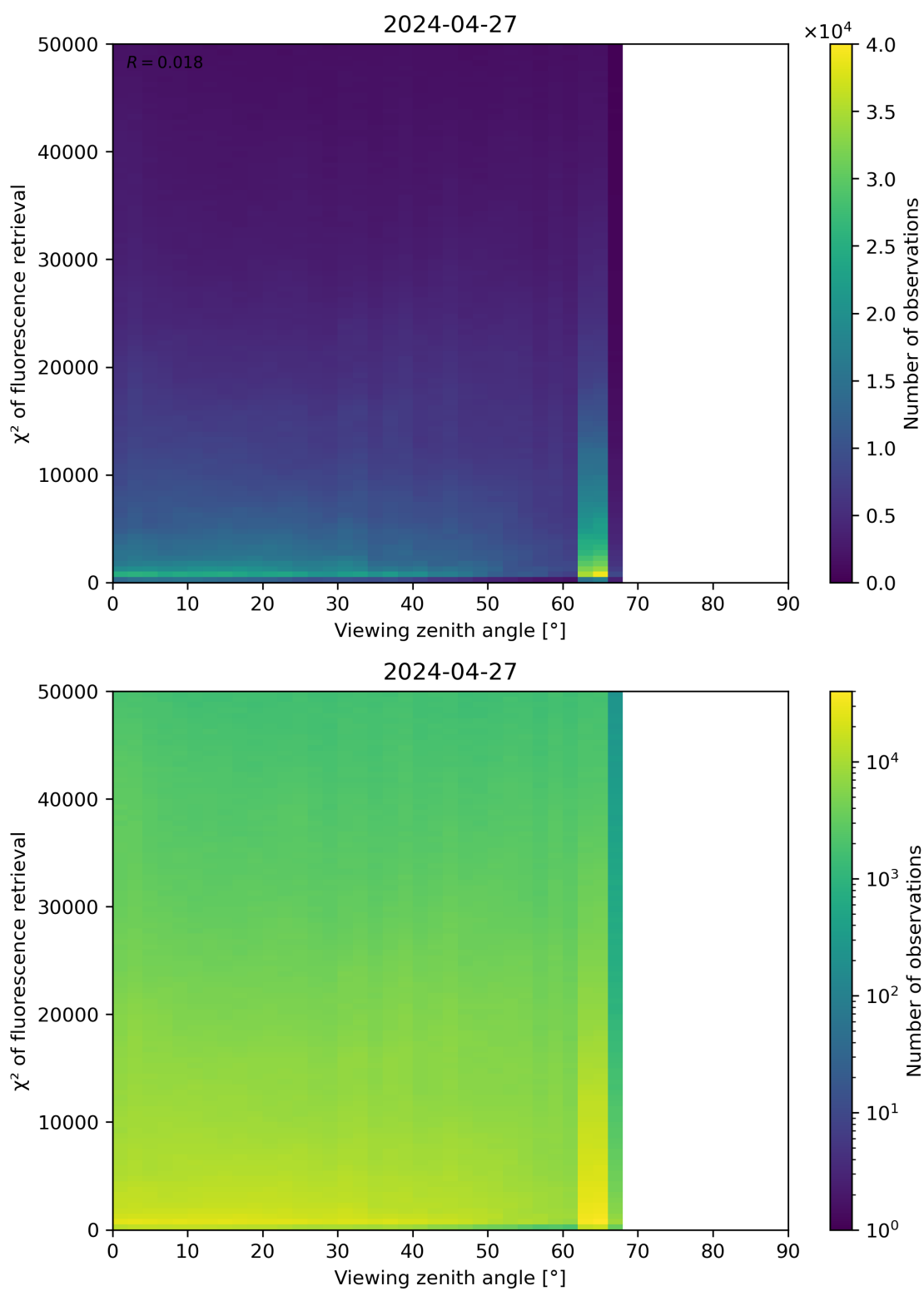
Figure 119: Scatter density plot of “Viewing zenith angle” against “ \chi^2 of fluorescence retrieval” for 2024-04-26 to 2024-04-28.
