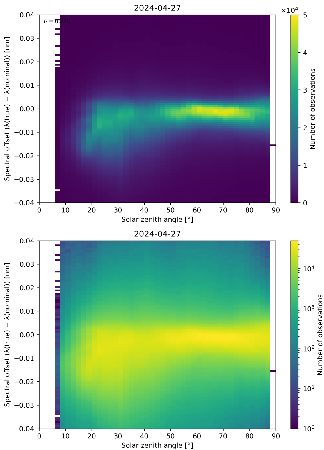
Figure 117: Scatter density plot of “Solar zenith angle” against “Spectral offset ( \lambda(\text{true}) - \lambda(\text{nominal}) )” for 2024-04-26 to 2024-04-28.
