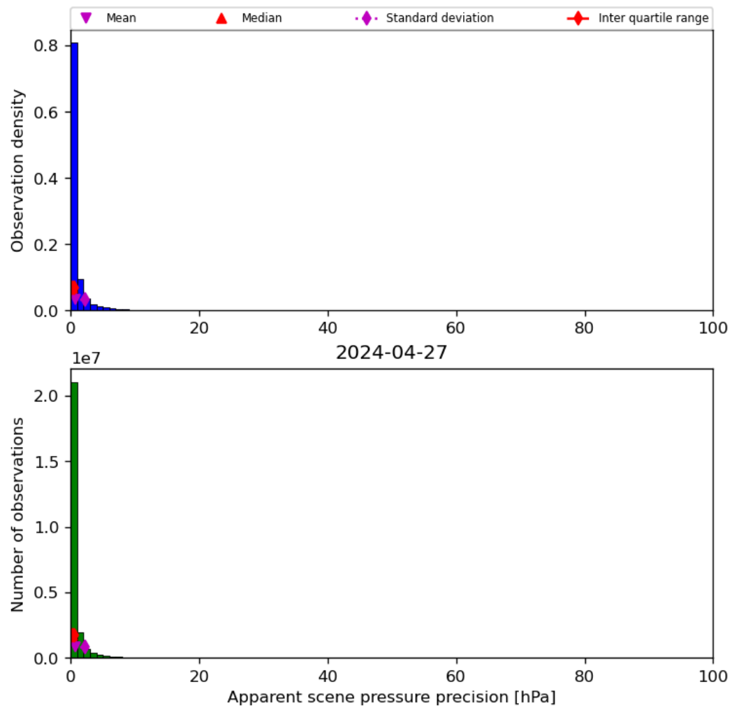
Figure 37: Histogram of “Apparent scene pressure precision” for 2024-04-26 to 2024-04-28
