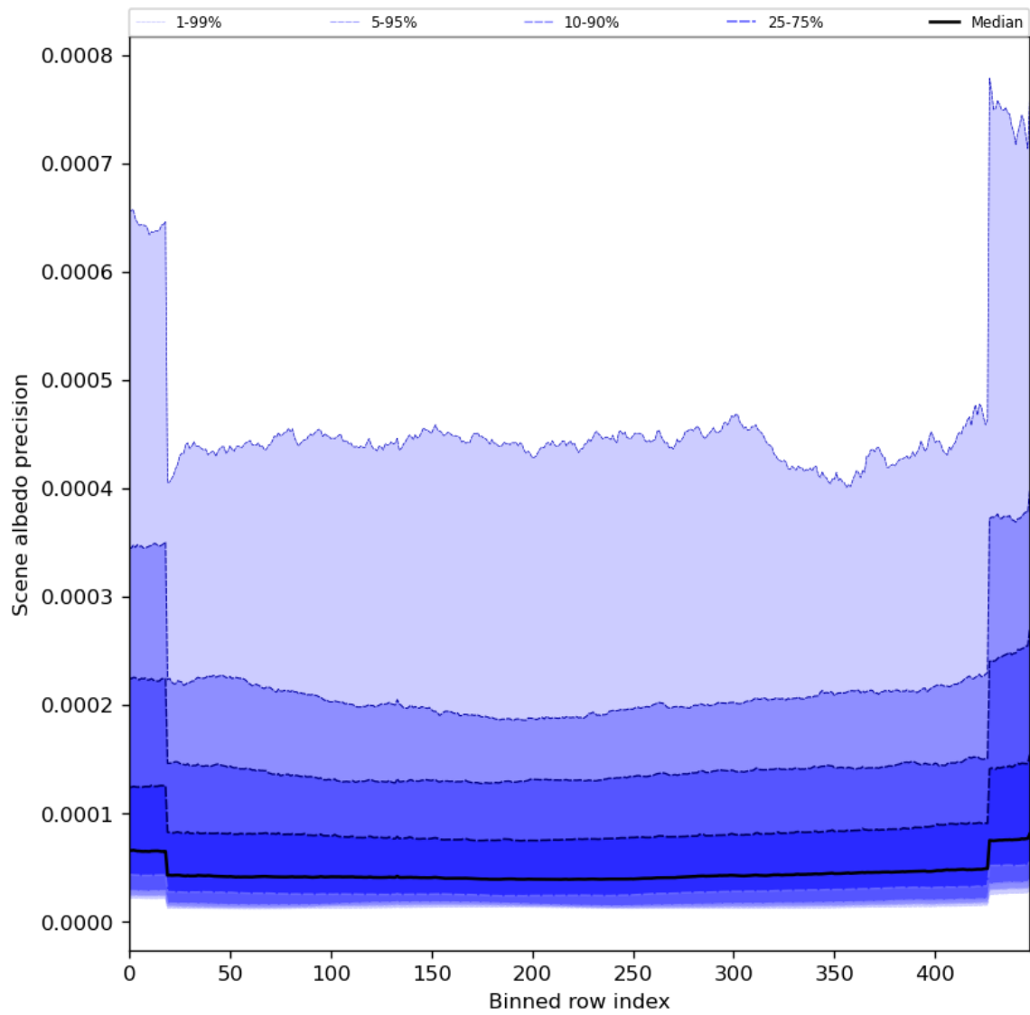
Figure 52: Along track statistics of “Scene albedo precision” for 2024-04-26 to 2024-04-28
