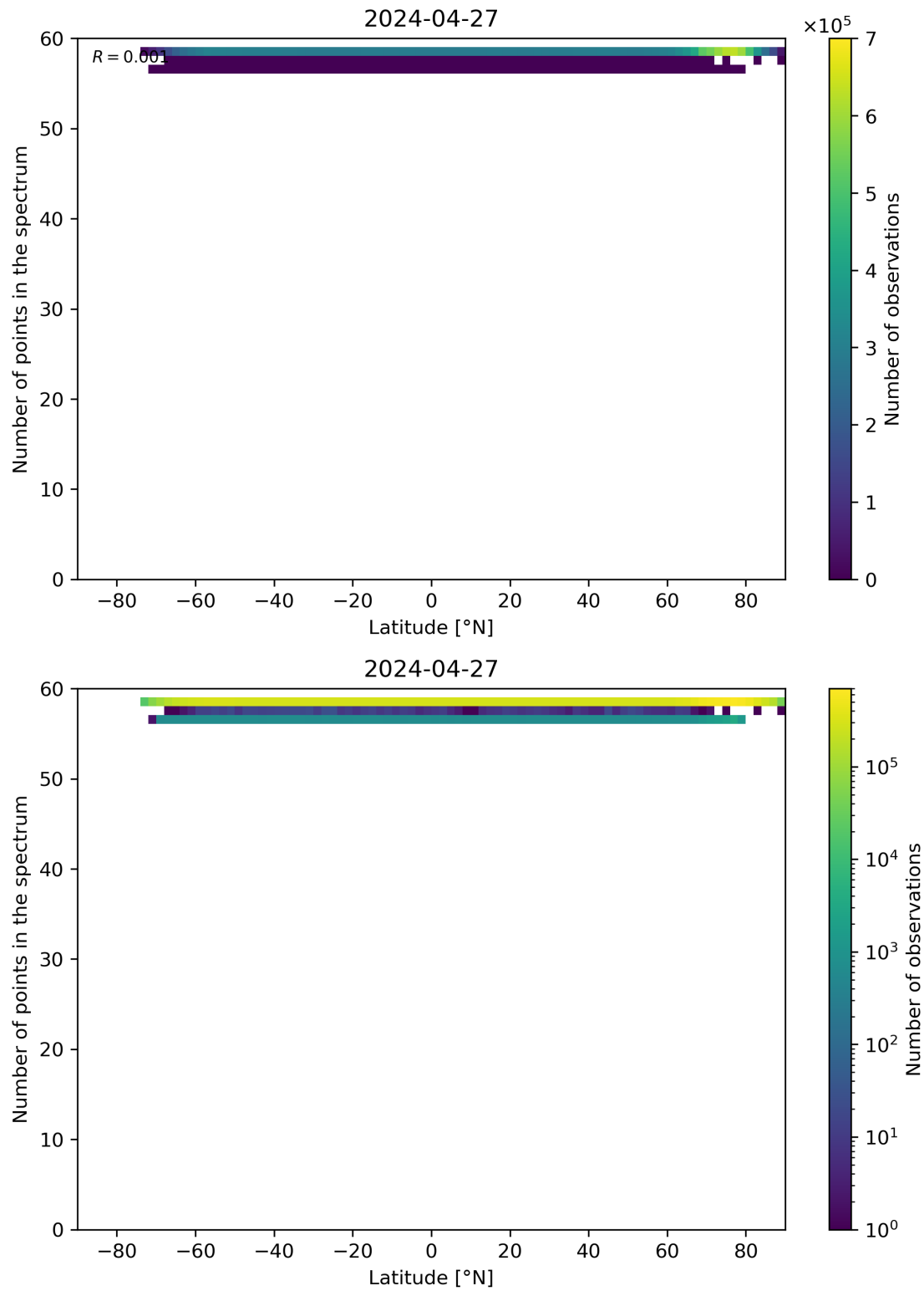
Figure 94: Scatter density plot of “Latitude” against “Number of points in the spectrum” for 2024-04-26 to 2024-04-28.
