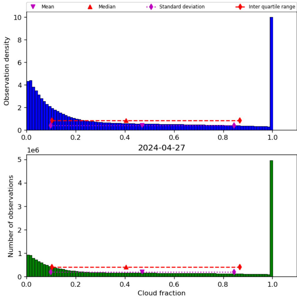
Figure 32: Histogram of “Cloud fraction” for 2024-04-26 to 2024-04-28
