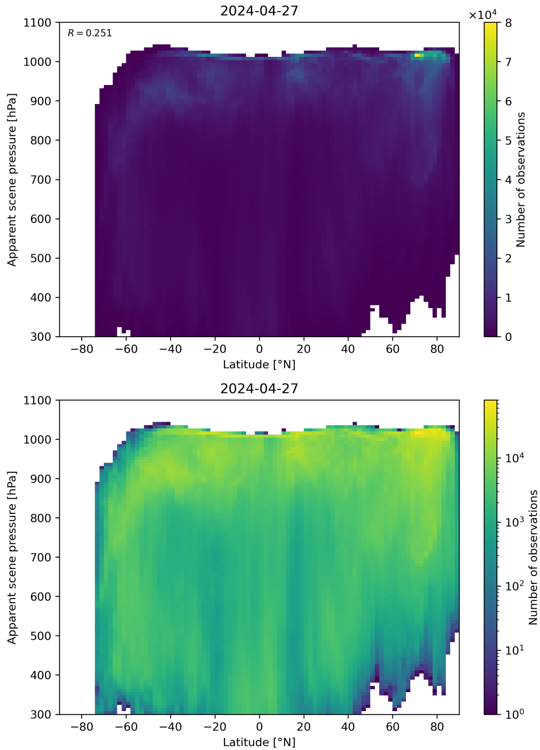
Figure 88: Scatter density plot of “Latitude” against “Apparent scene pressure” for 2024-04-26 to 2024-04-28.
