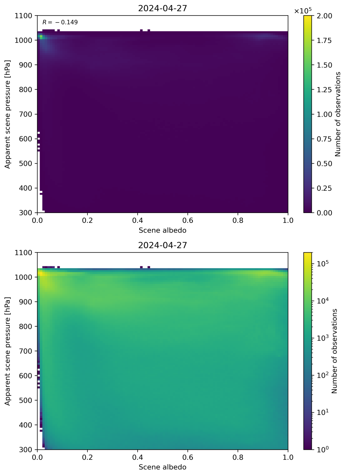
Figure 102: Scatter density plot of “Scene albedo” against “Apparent scene pressure” for 2024-04-26 to 2024-04-28.
