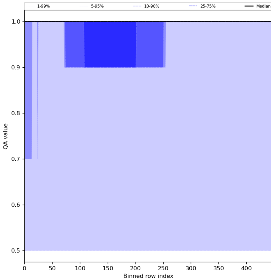
Figure 46: Along track statistics of "QA value" for 2024-04-26 to 2024-04-28
