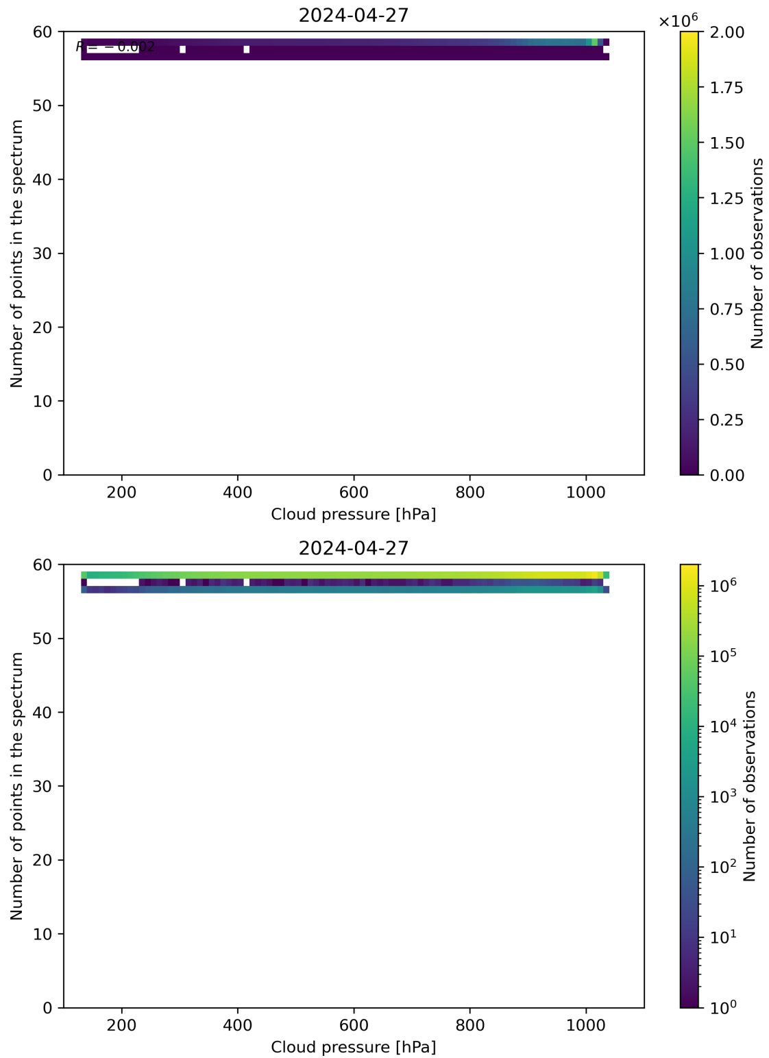
Figure 82: Scatter density plot of “Cloud pressure” against “Number of points in the spectrum” for 2024-04-26 to 2024-04-28.
