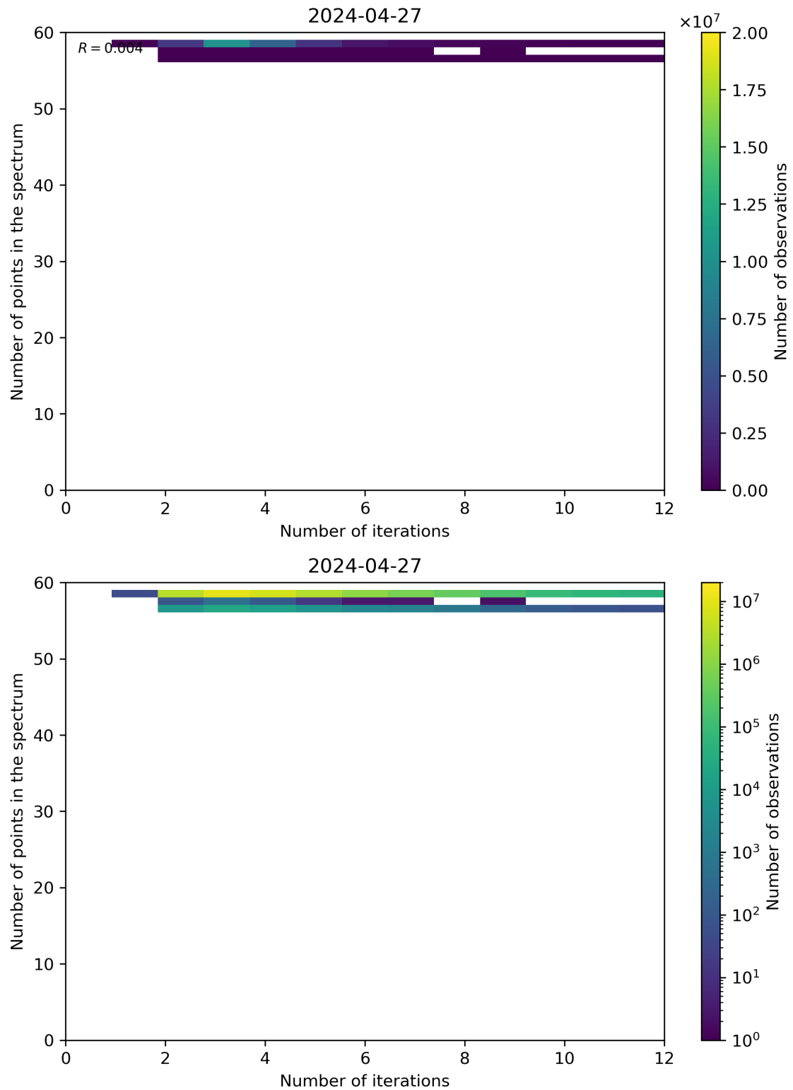
Figure 99: Scatter density plot of “Number of iterations” against “Number of points in the spectrum” for 2024-04-26 to 2024-04-28.
