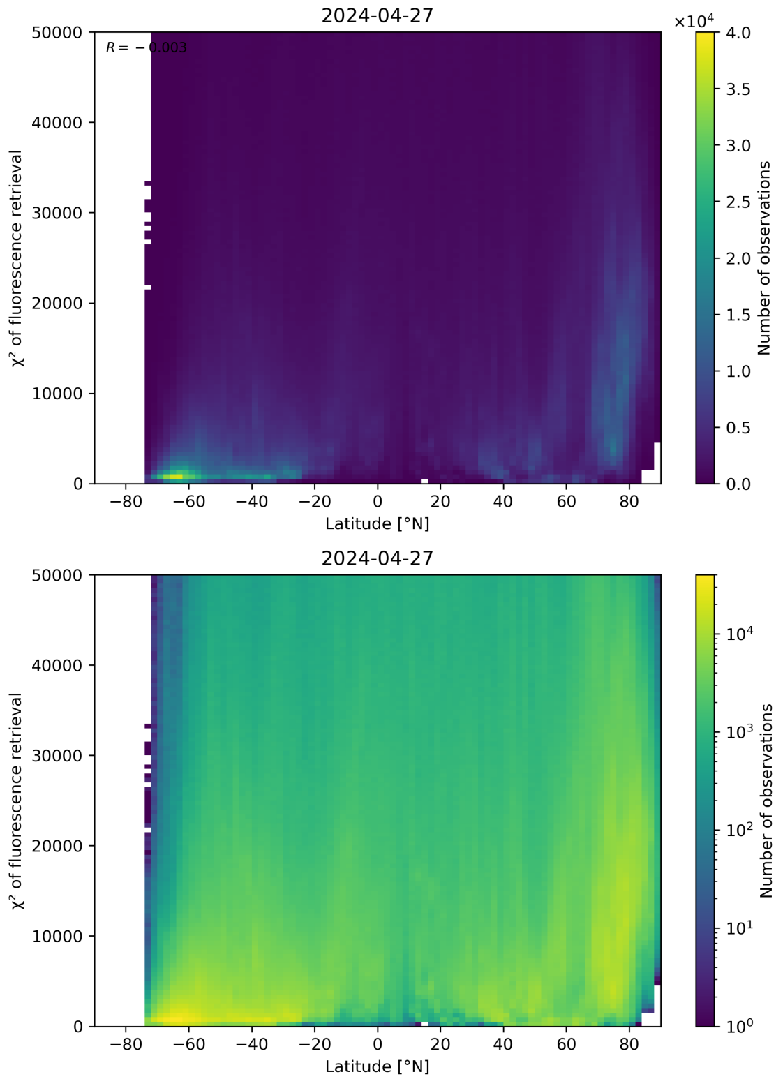
Figure 89: Scatter density plot of “Latitude” against “ \chi^2 of fluorescence retrieval” for 2024-04-26 to 2024-04-28.
