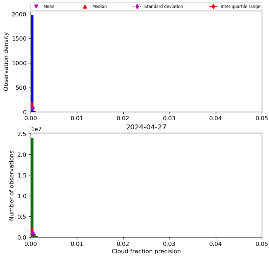
Figure 33: Histogram of “Cloud fraction precision” for 2024-04-26 to 2024-04-28
