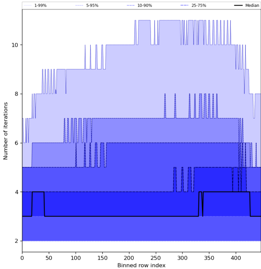
Figure 56: Along track statistics of “Number of iterations” for 2024-04-26 to 2024-04-28
