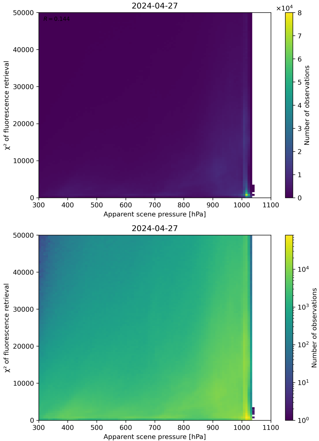
Figure 63: Scatter density plot of “Apparent scene pressure” against “ \chi^2 of fluorescence retrieval” for 2024-04-26 to 2024-04-28.
