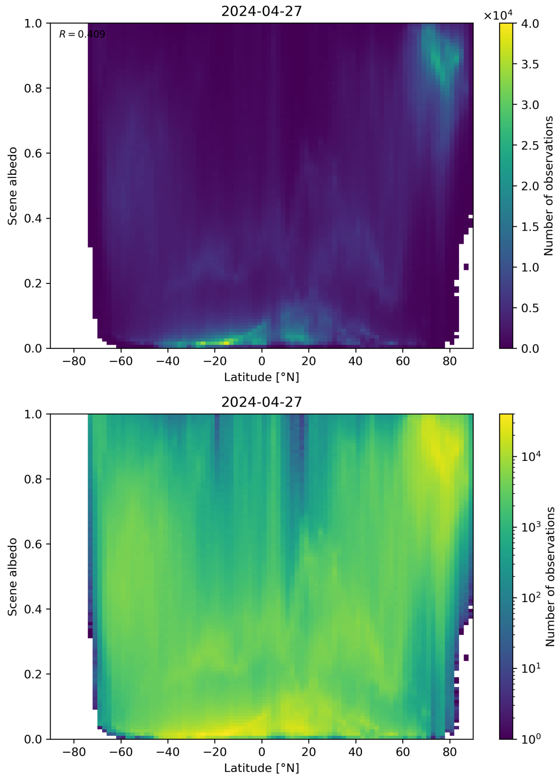
Figure 95: Scatter density plot of “Latitude” against “Scene albedo” for 2024-04-26 to 2024-04-28.
