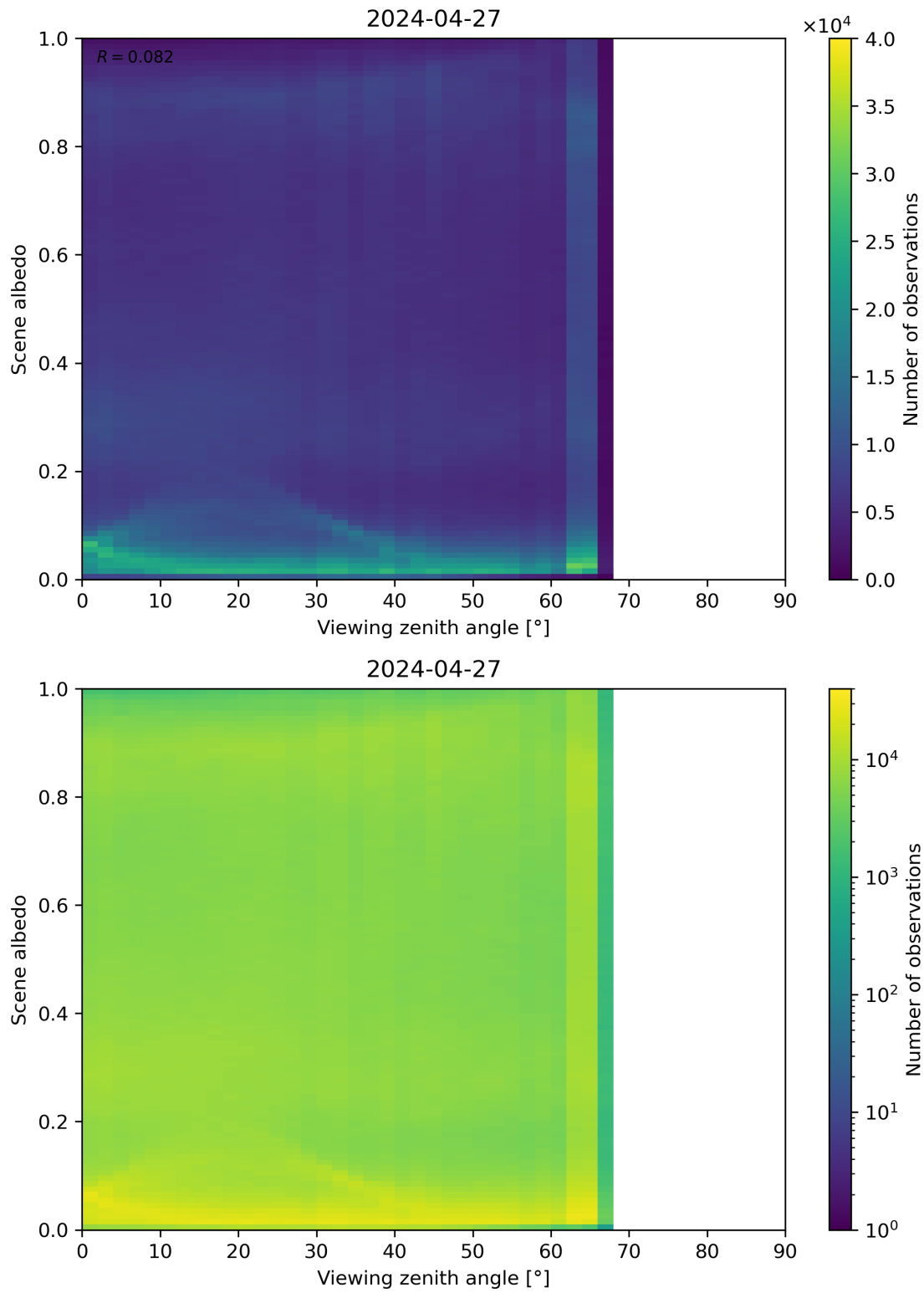
Figure 126: Scatter density plot of “Viewing zenith angle” against “Scene albedo” for 2024-04-26 to 2024-04-28.
