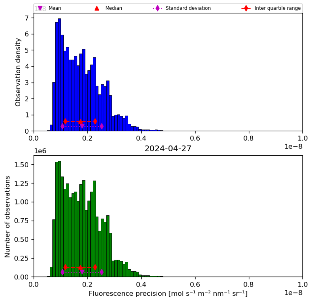
Figure 41: Histogram of “Fluorescence precision” for 2024-04-26 to 2024-04-28
