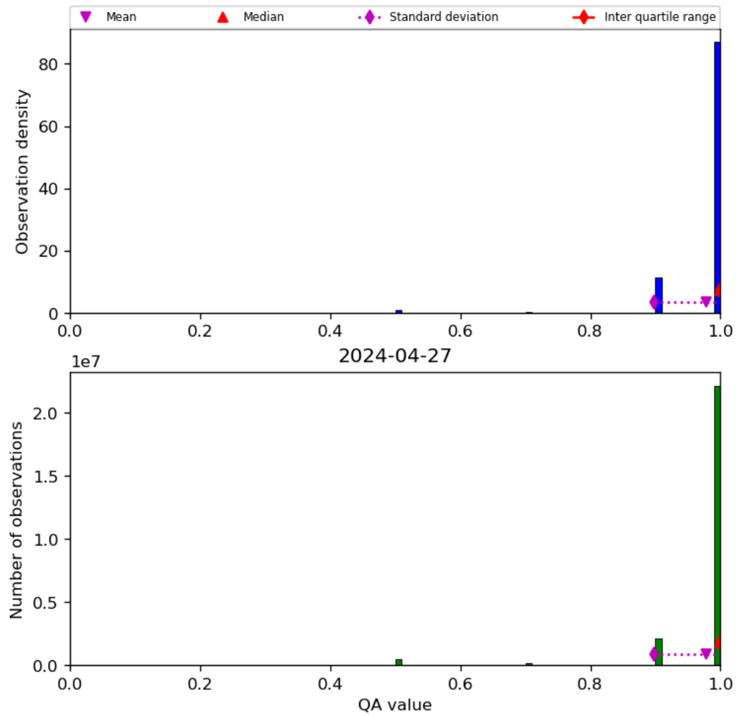
Figure 29: Histogram of “QA value” for 2024-04-26 to 2024-04-28
