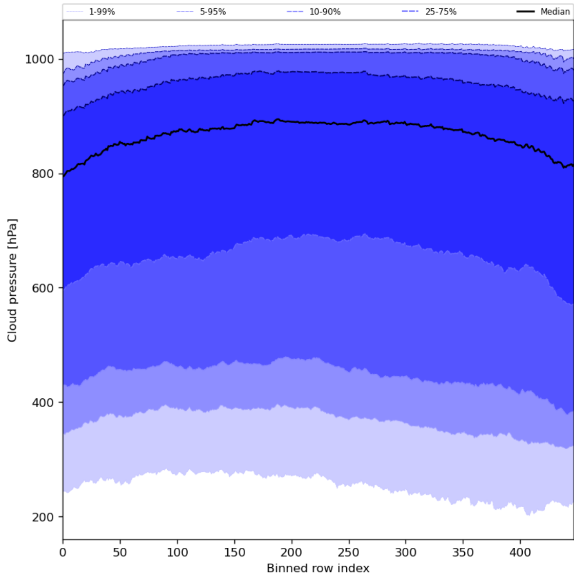
Figure 47: Along track statistics of “Cloud pressure” for 2024-04-26 to 2024-04-28
