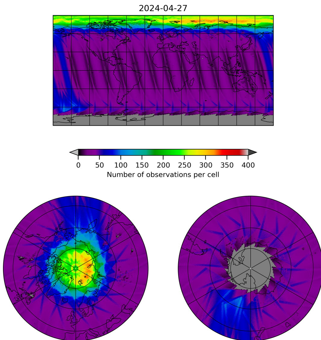
Figure 11: Map of the number of observations for 2024-04-26 to 2024-04-28
