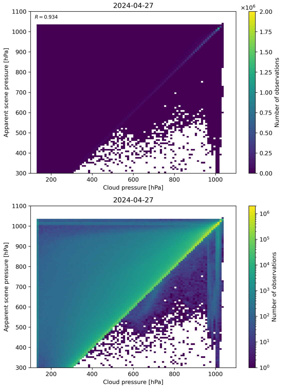
Figure 77: Scatter density plot of “Cloud pressure” against “Apparent scene pressure” for 2024-04-26 to 2024-04-28.
