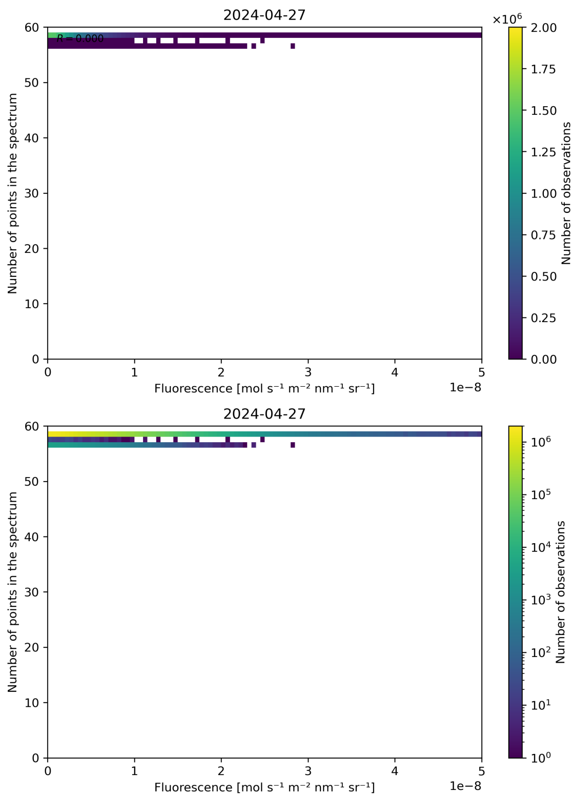
Figure 86: Scatter density plot of “Fluorescence” against “Number of points in the spectrum” for 2024-04-26 to 2024-04-28.
