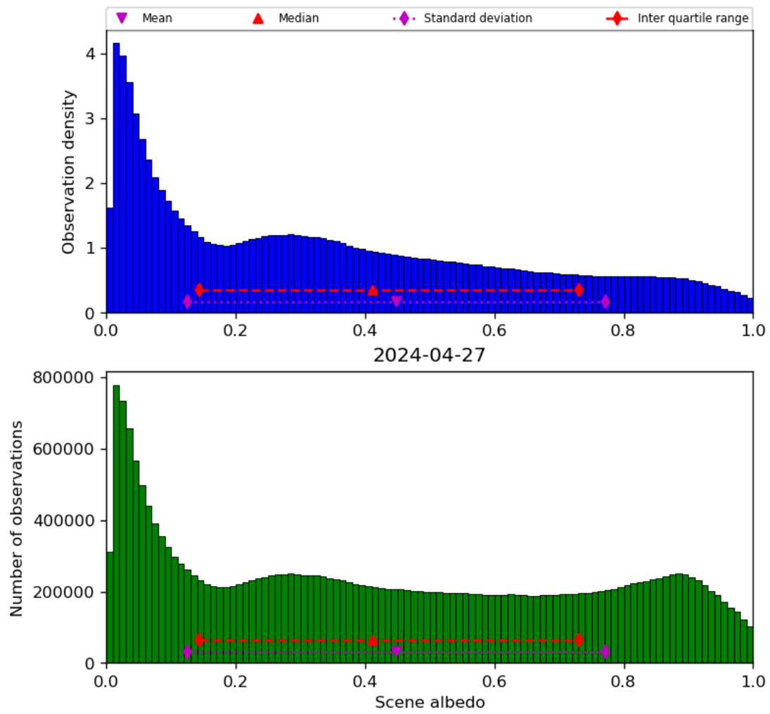
Figure 34: Histogram of “Scene albedo” for 2024-04-26 to 2024-04-28
