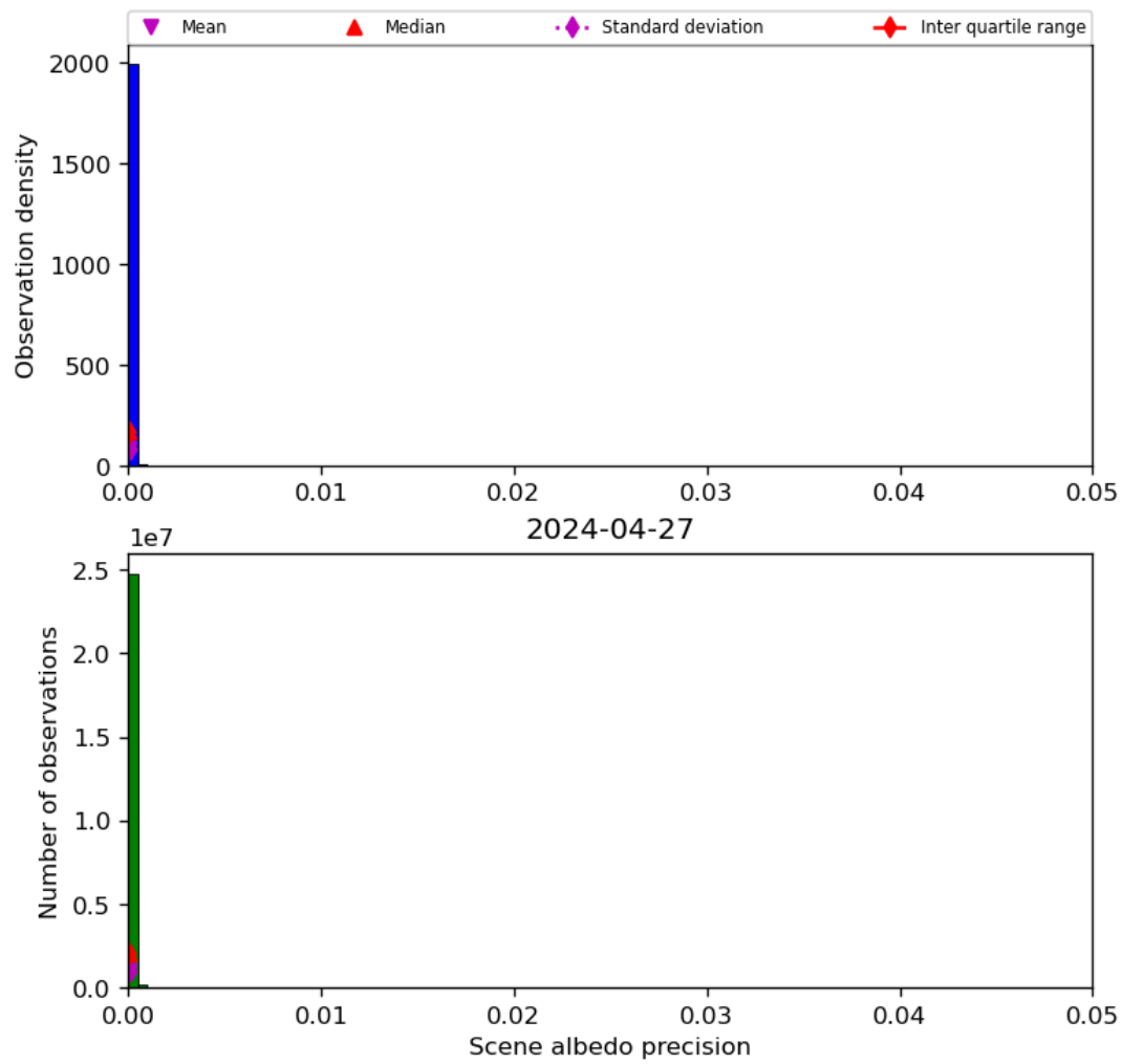
Figure 35: Histogram of “Scene albedo precision” for 2024-04-26 to 2024-04-28
