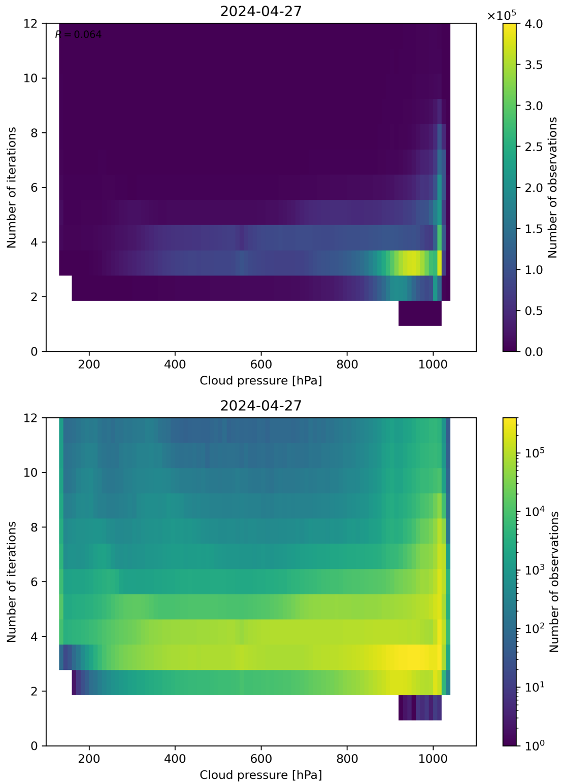
Figure 81: Scatter density plot of “Cloud pressure” against “Number of iterations” for 2024-04-26 to 2024-04-28.
