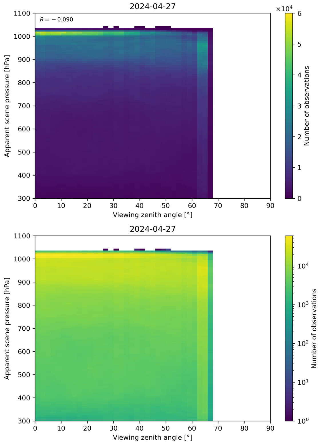
Figure 118: Scatter density plot of “Viewing zenith angle” against “Apparent scene pressure” for 2024-04-26 to 2024-04-28.
