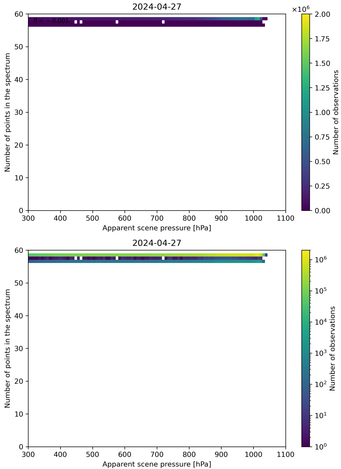
Figure 66: Scatter density plot of “Apparent scene pressure” against “Number of points in the spectrum” for 2024-04-26 to 2024-04-28.
