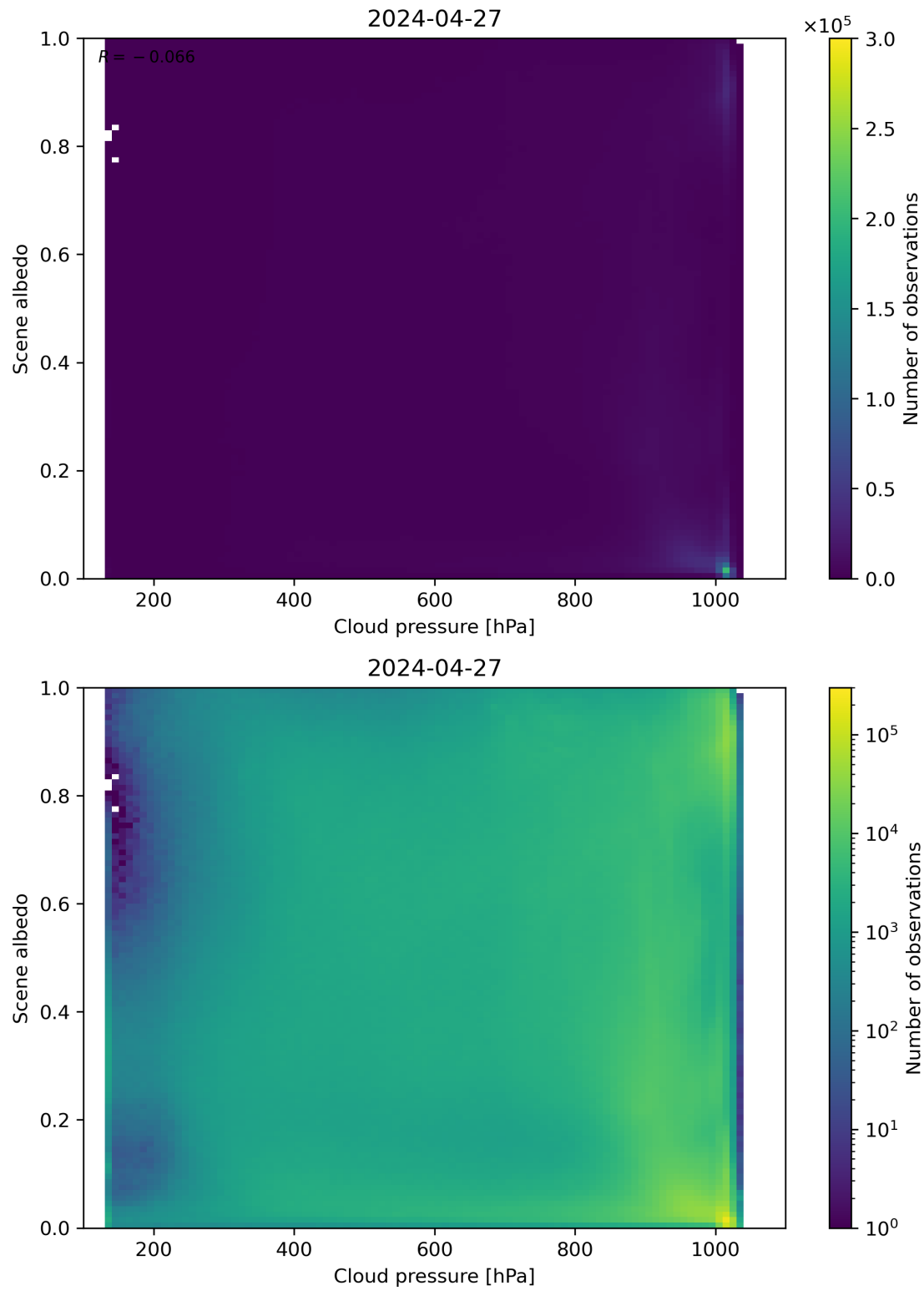
Figure 83: Scatter density plot of “Cloud pressure” against “Scene albedo” for 2024-04-26 to 2024-04-28.
