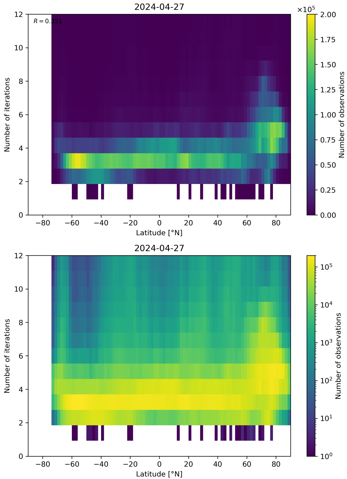
Figure 93: Scatter density plot of “Latitude” against “Number of iterations” for 2024-04-26 to 2024-04-28.
