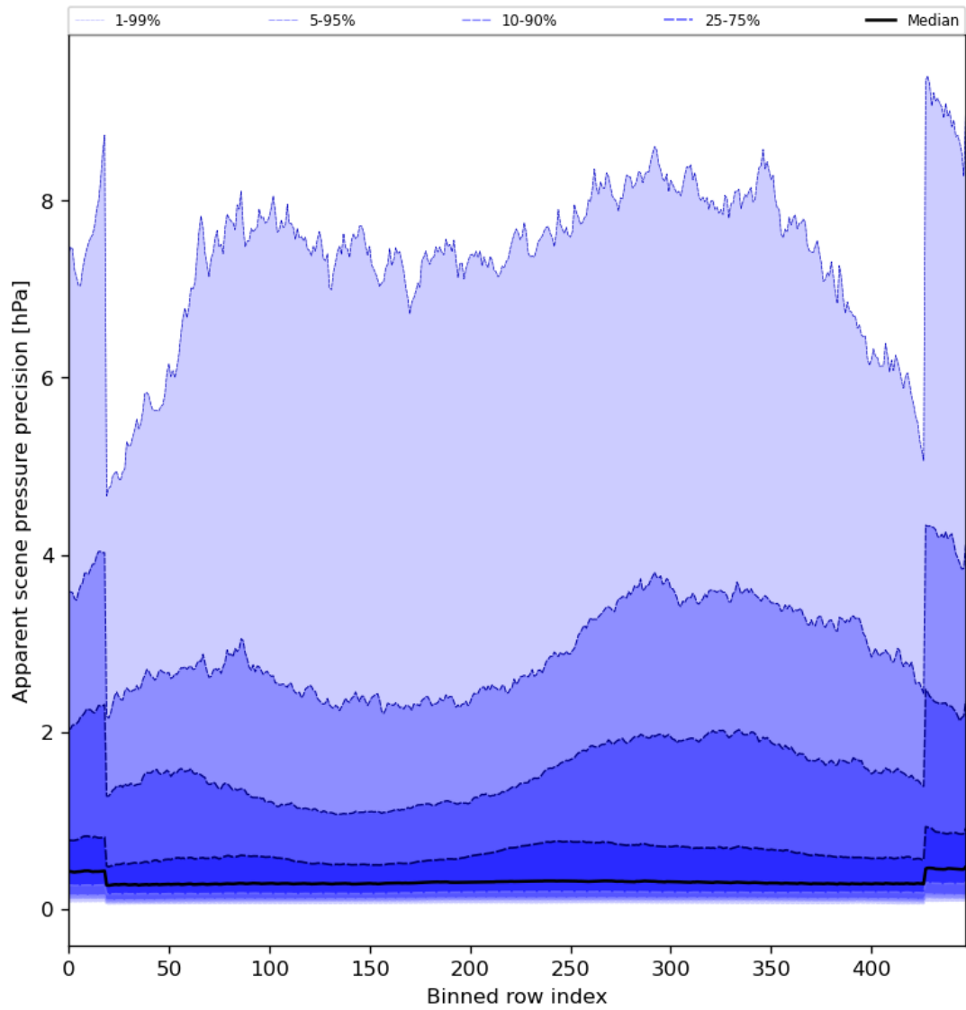
Figure 54: Along track statistics of “Apparent scene pressure precision” for 2024-04-26 to 2024-04-28
