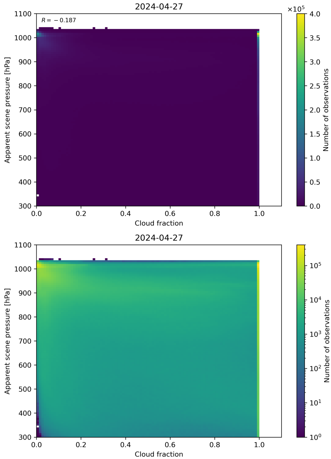
Figure 70: Scatter density plot of “Cloud fraction” against “Apparent scene pressure” for 2024-04-26 to 2024-04-28.
