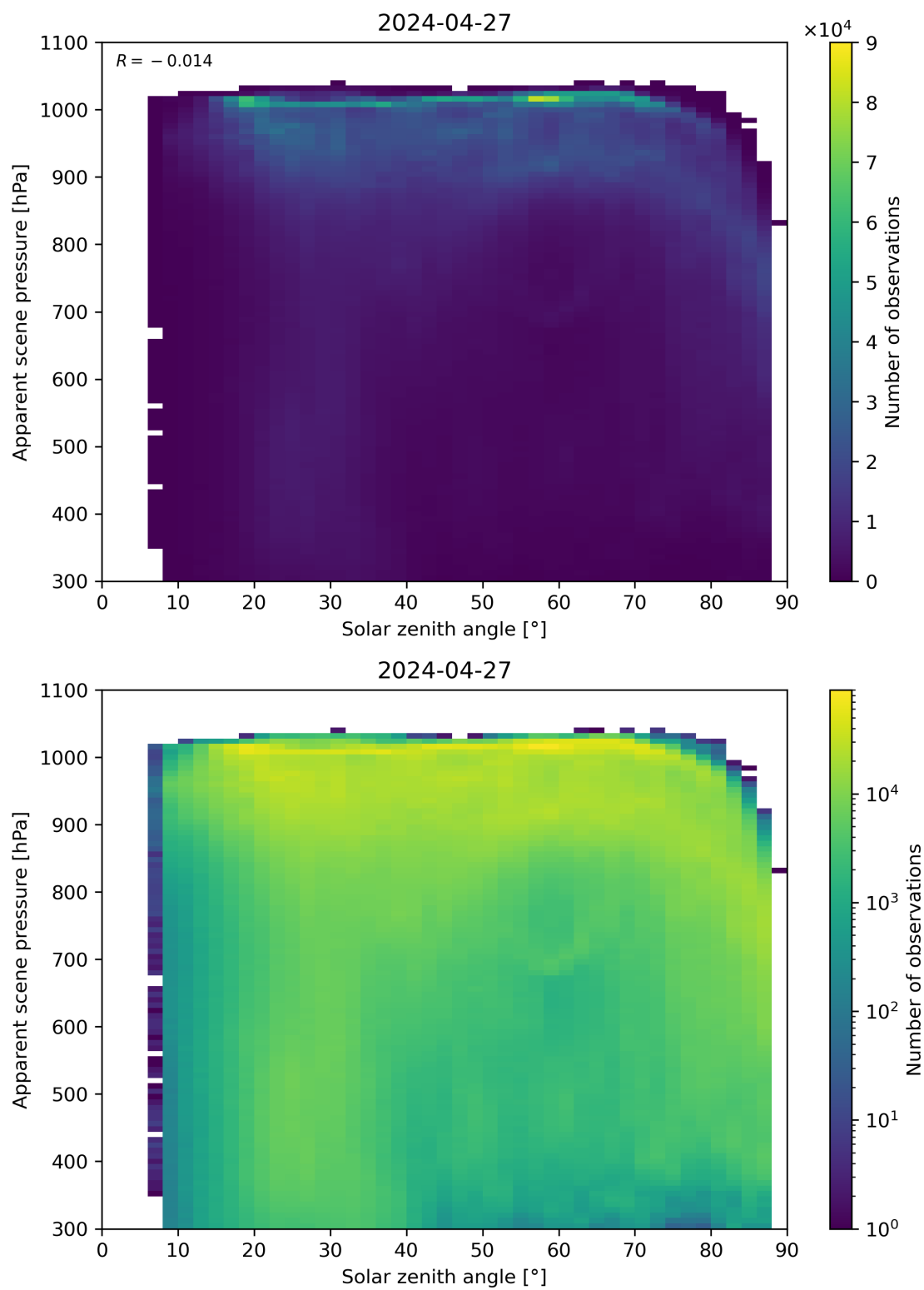
Figure 108: Scatter density plot of “Solar zenith angle” against “Apparent scene pressure” for 2024-04-26 to 2024-04-28.
