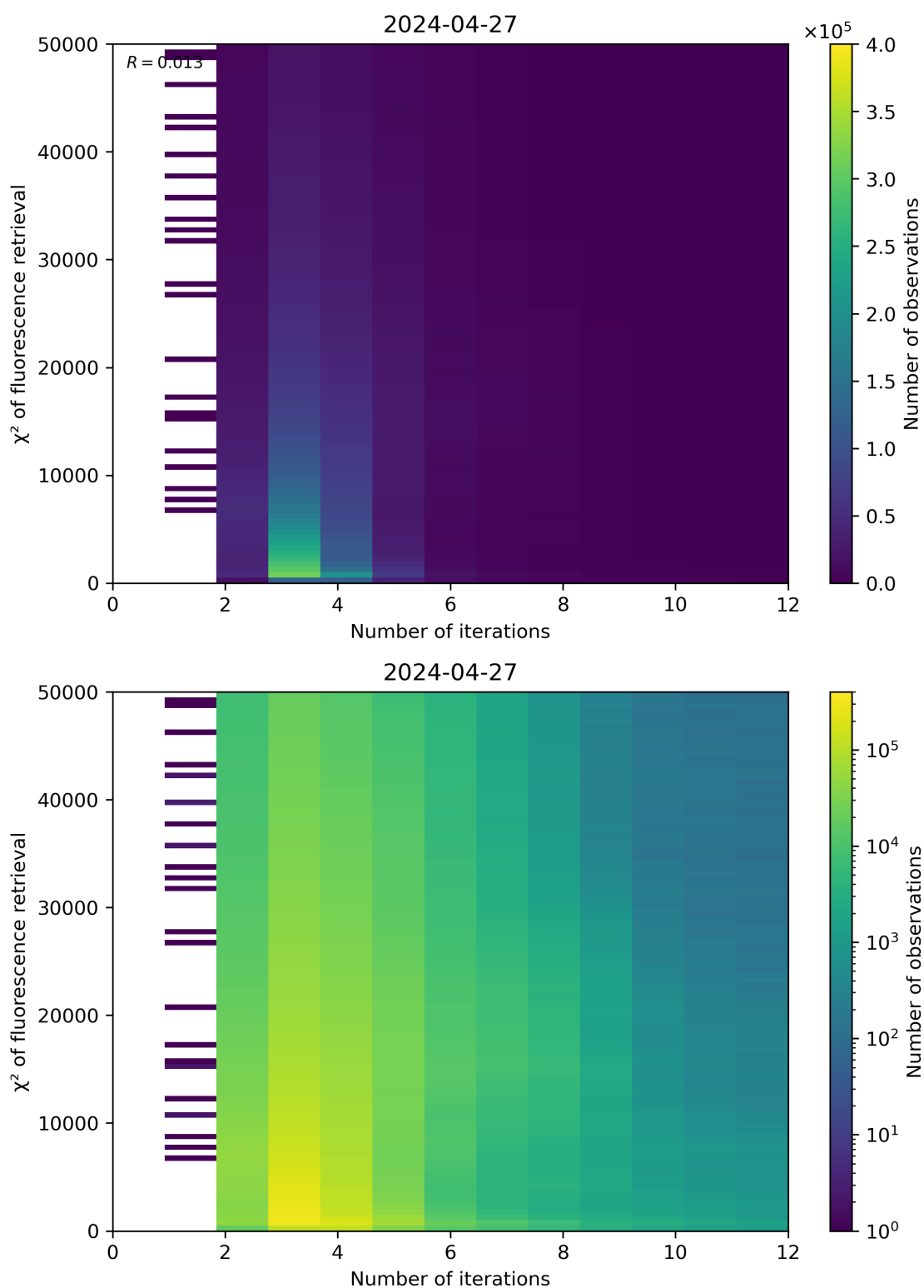
Figure 97: Scatter density plot of “Number of iterations” against “ \chi^2 of fluorescence retrieval” for 2024-04-26 to 2024-04-28.
