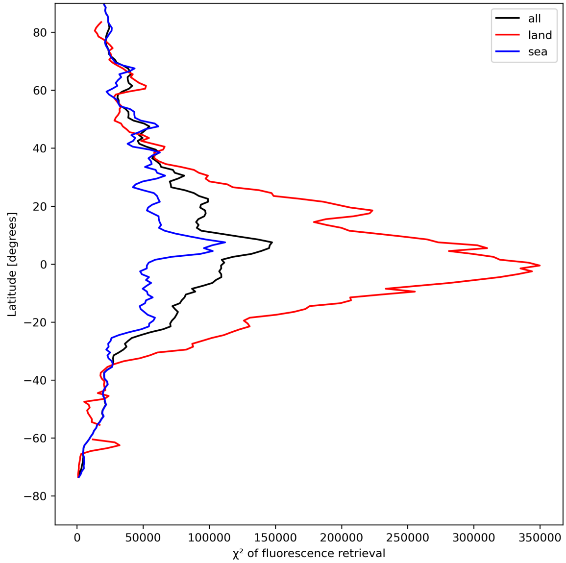
Figure 25: Zonal average of “ \chi^2 of fluorescence retrieval” for 2024-04-26 to 2024-04-28.
