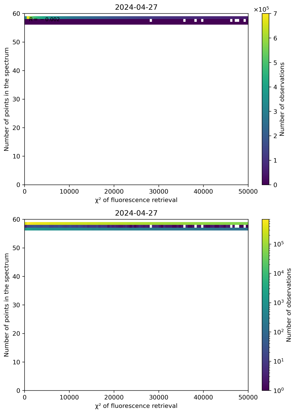
Figure 68: Scatter density plot of " \chi^2 of fluorescence retrieval" against "Number of points in the spectrum" for 2024-04-26 to 2024-04-28.
