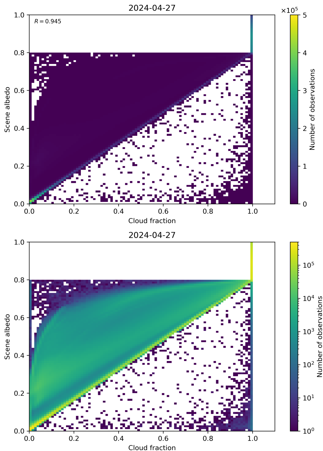
Figure 75: Scatter density plot of “Cloud fraction” against “Scene albedo” for 2024-04-26 to 2024-04-28.
