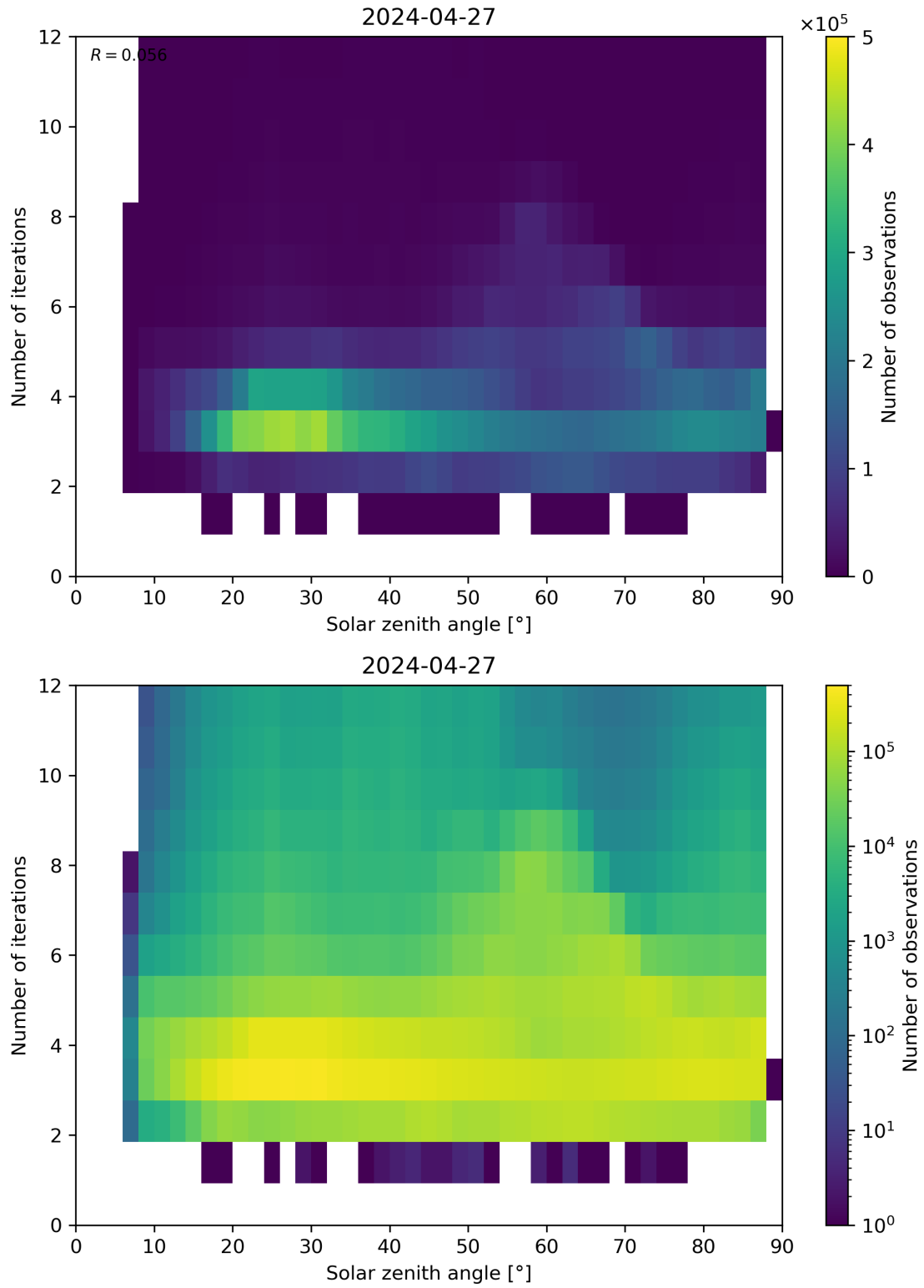
Figure 114: Scatter density plot of “Solar zenith angle” against “Number of iterations” for 2024-04-26 to 2024-04-28.
