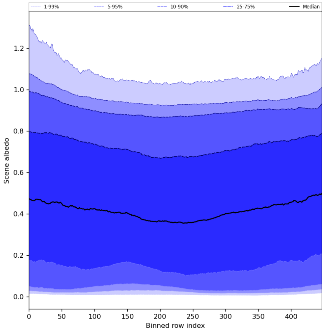
Figure 51: Along track statistics of “Scene albedo” for 2024-04-26 to 2024-04-28
