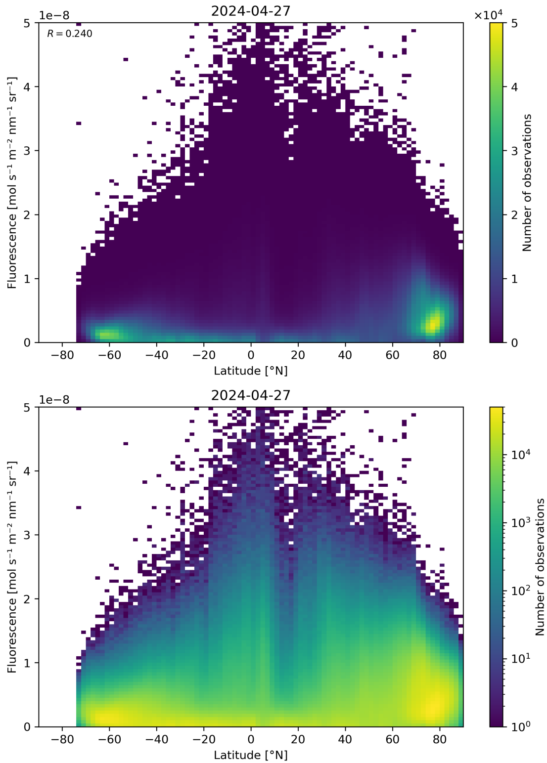
Figure 92: Scatter density plot of “Latitude” against “Fluorescence” for 2024-04-26 to 2024-04-28.
