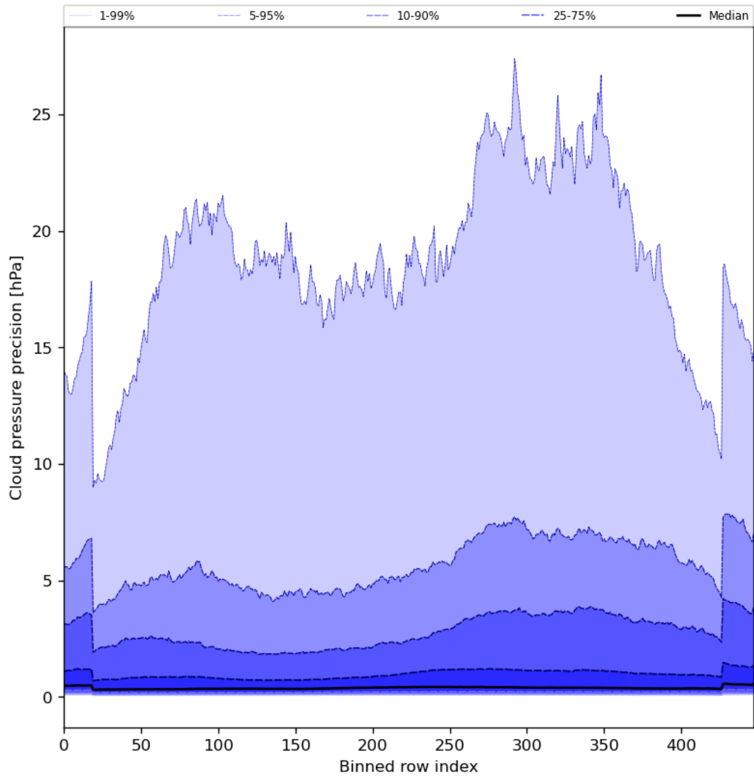
Figure 48: Along track statistics of “Cloud pressure precision” for 2024-04-26 to 2024-04-28
