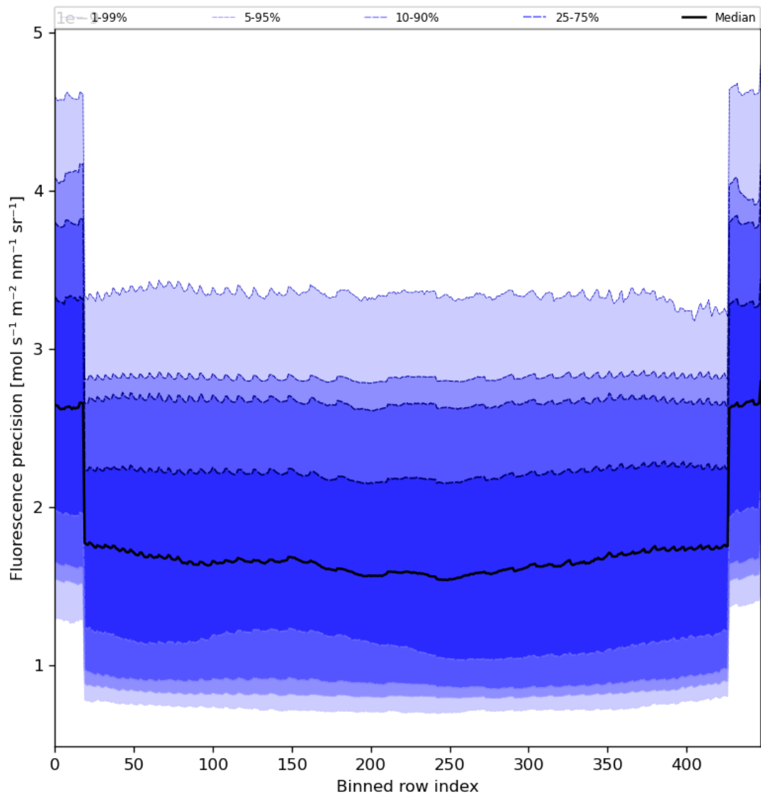
Figure 58: Along track statistics of “Fluorescence precision” for 2024-04-26 to 2024-04-28
