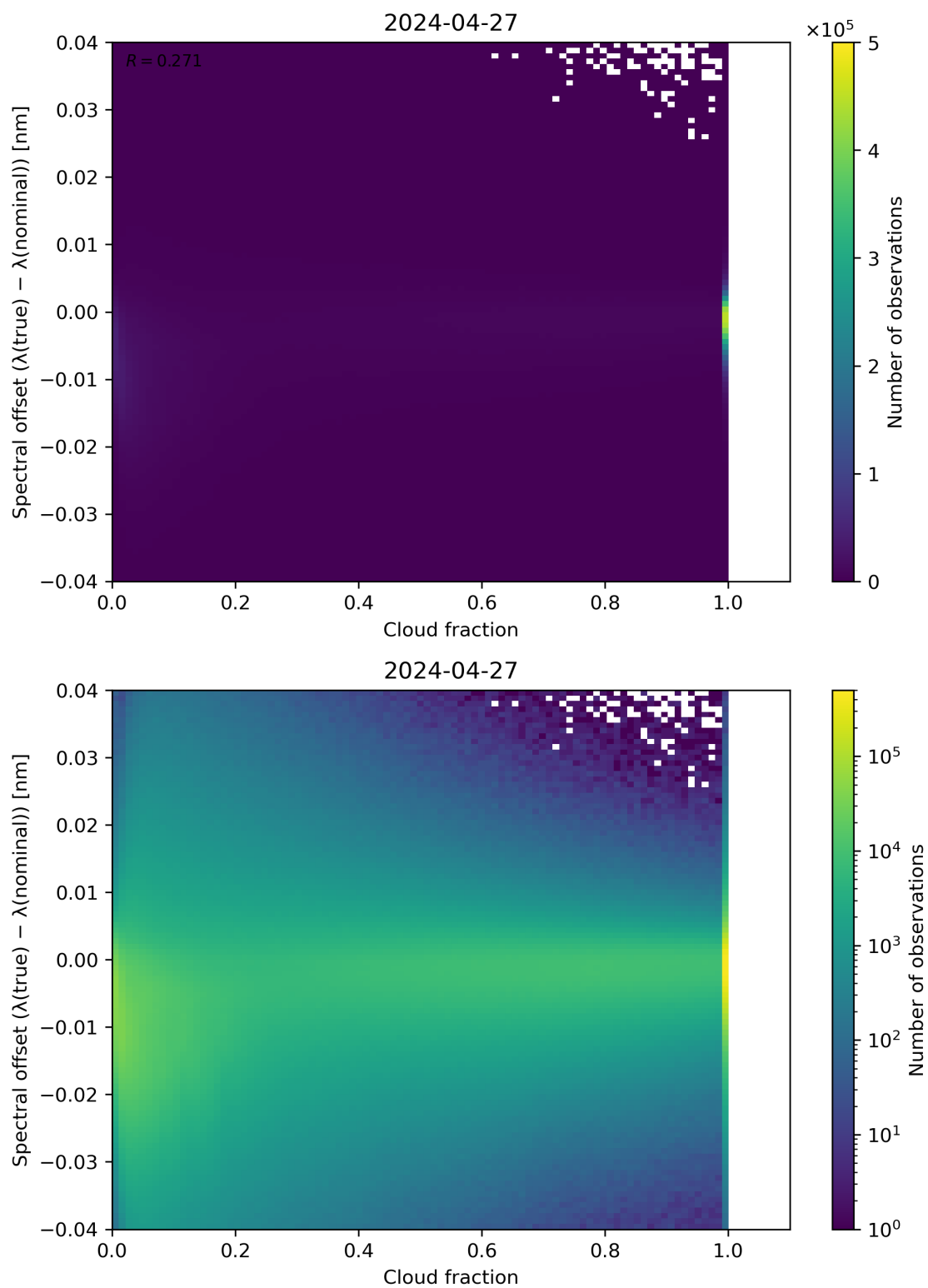
Figure 76: Scatter density plot of “Cloud fraction” against “Spectral offset ( \lambda(\text{true}) - \lambda(\text{nominal}) )” for 2024-04-26 to 2024-04-28.
