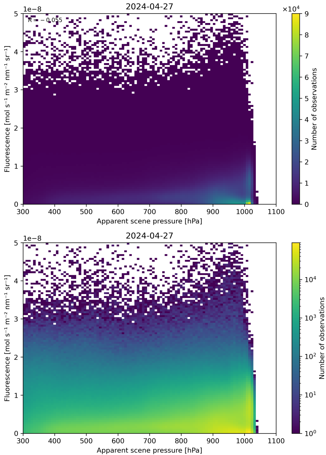
Figure 64: Scatter density plot of “Apparent scene pressure” against “Fluorescence” for 2024-04-26 to 2024-04-28.
