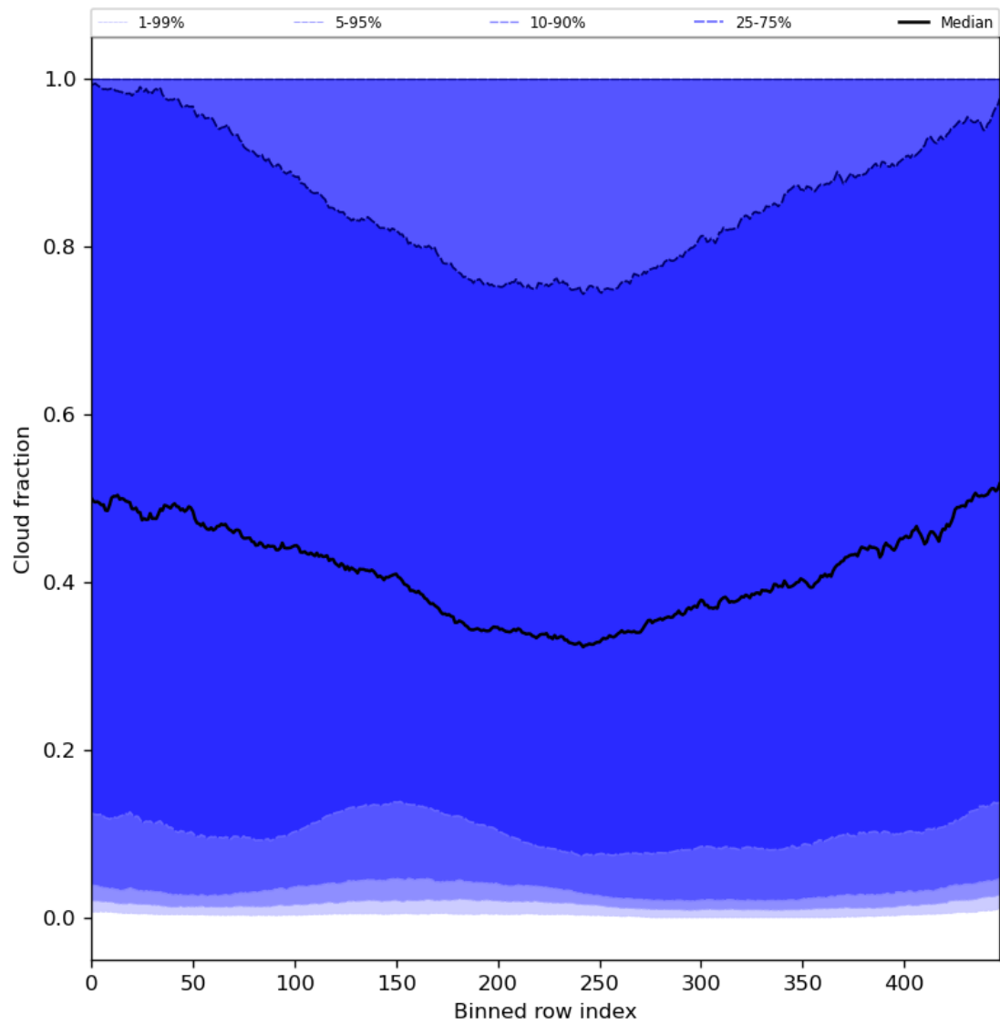
Figure 49: Along track statistics of “Cloud fraction” for 2024-04-26 to 2024-04-28
