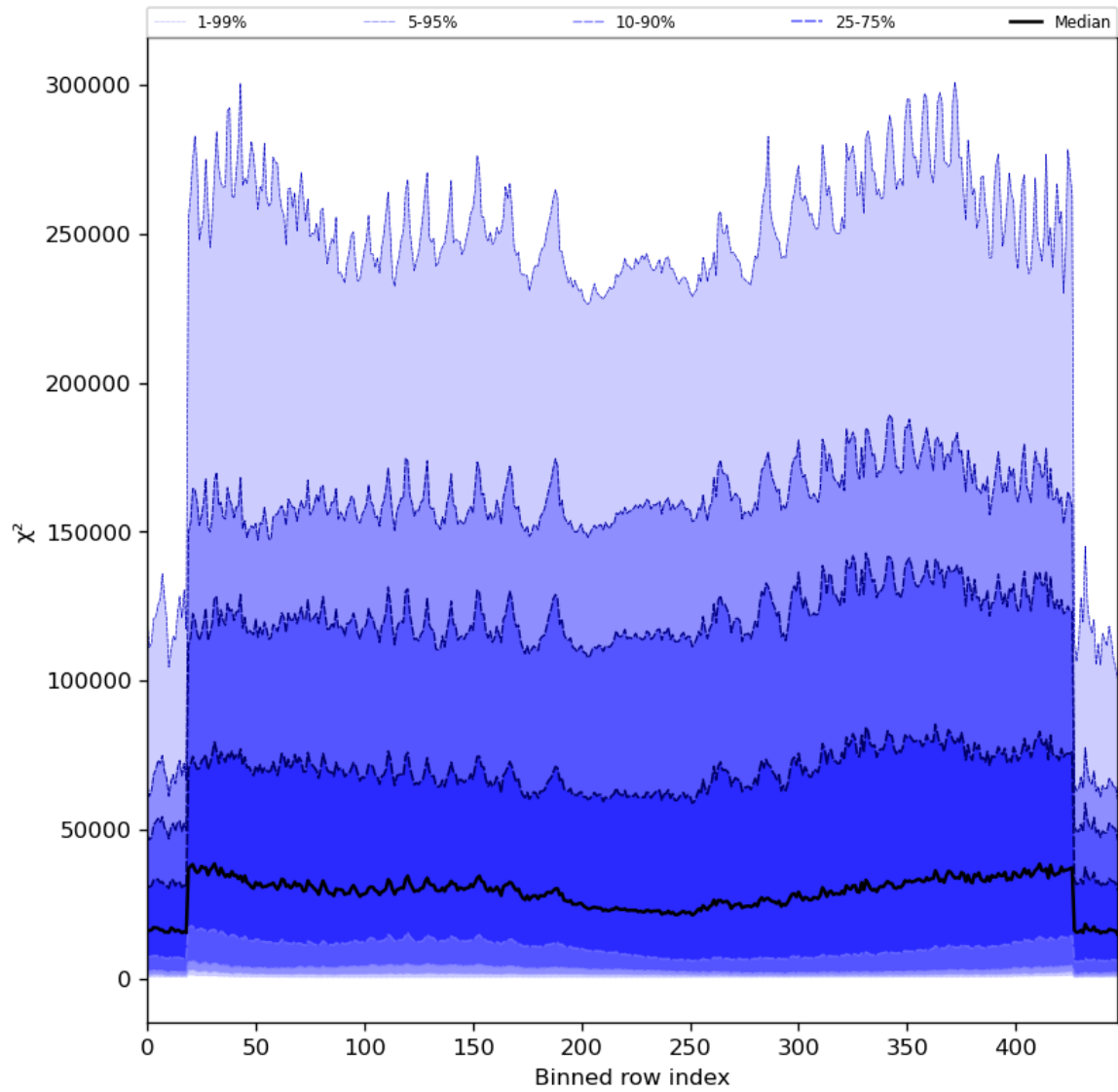
Figure 55: Along track statistics of “ \chi^2 ” for 2024-04-26 to 2024-04-28
