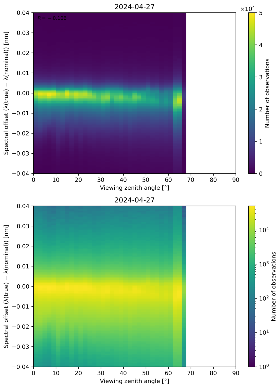
Figure 128: Scatter density plot of “Viewing zenith angle” against “Spectral offset ( \lambda(\text{true}) - \lambda(\text{nominal}) )” for 2024-04-26 to 2024-04-28.
