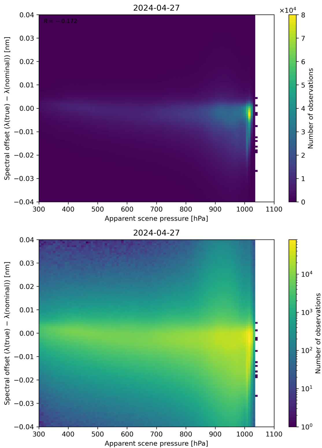
Figure 67: Scatter density plot of “Apparent scene pressure” against “Spectral offset ( \lambda(\text{true}) - \lambda(\text{nominal}) )” for 2024-04-26 to 2024-04-28.
