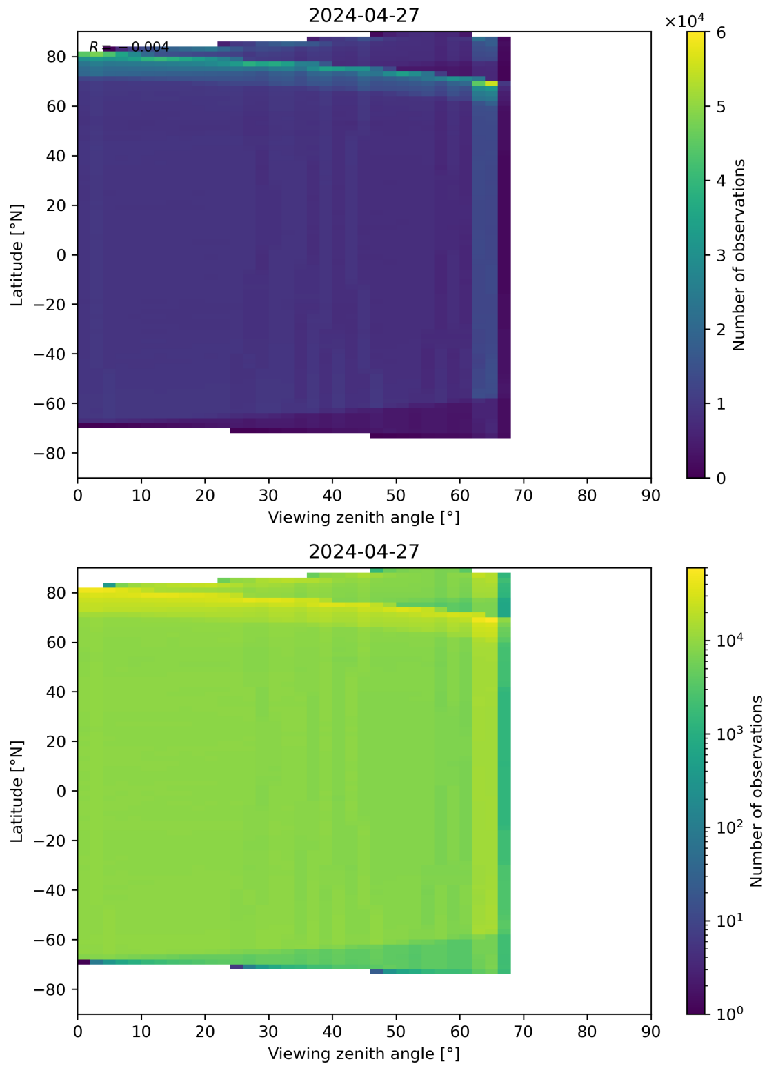
Figure 123: Scatter density plot of “Viewing zenith angle” against “Latitude” for 2024-04-26 to 2024-04-28.
