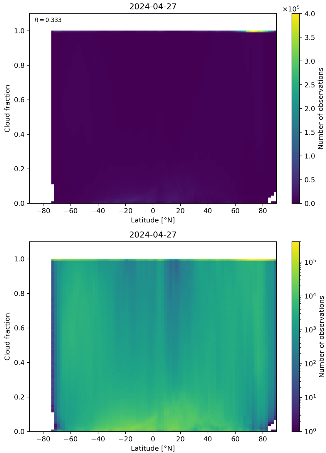
Figure 90: Scatter density plot of “Latitude” against “Cloud fraction” for 2024-04-26 to 2024-04-28.
