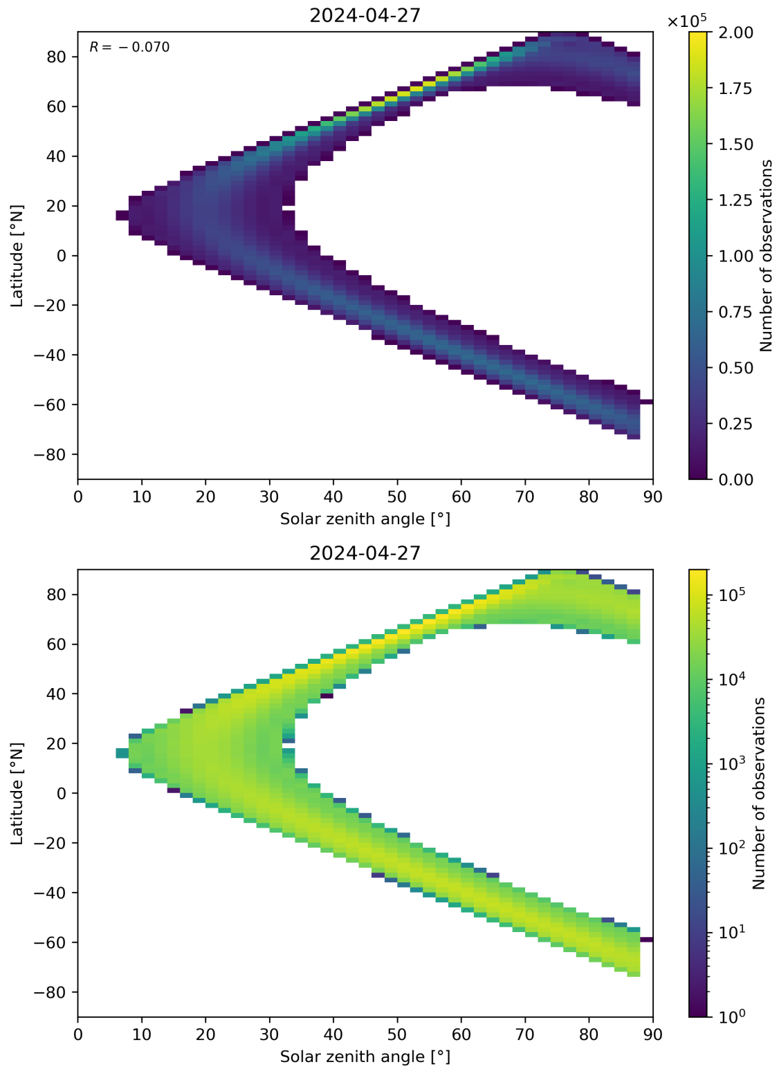
Figure 113: Scatter density plot of “Solar zenith angle” against “Latitude” for 2024-04-26 to 2024-04-28.
