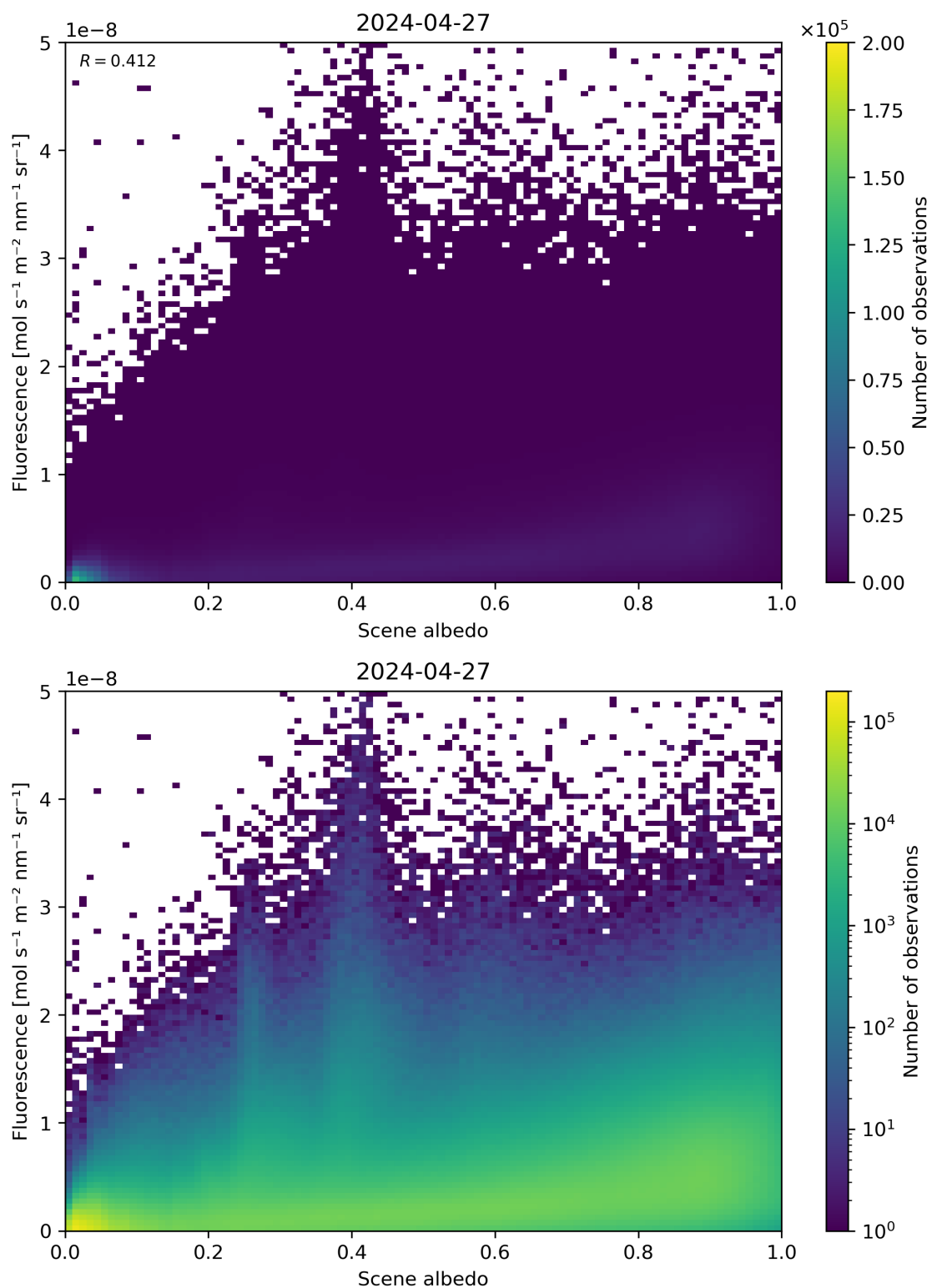
Figure 104: Scatter density plot of “Scene albedo” against “Fluorescence” for 2024-04-26 to 2024-04-28.
