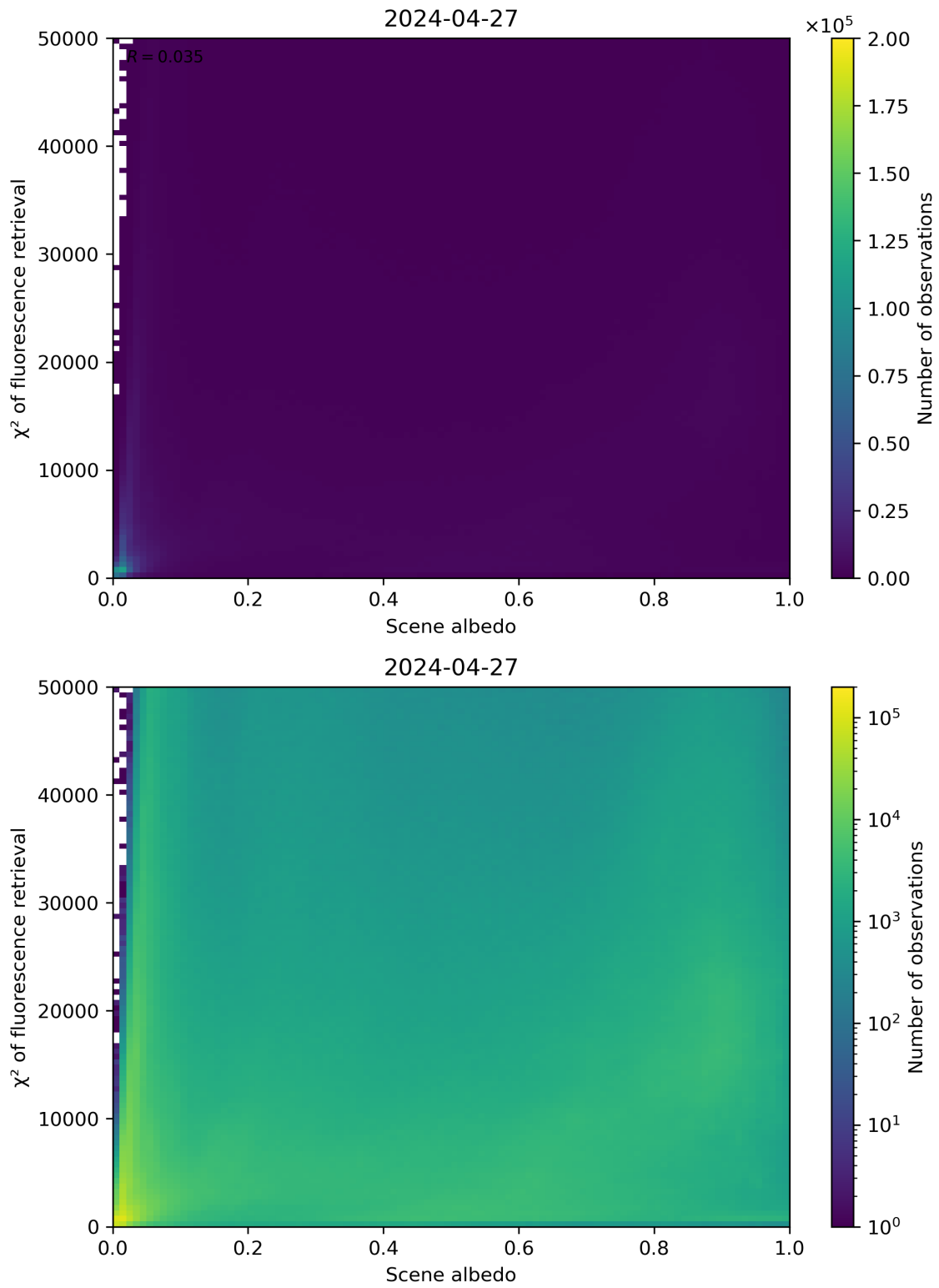
Figure 103: Scatter density plot of “Scene albedo” against “ \chi^2 of fluorescence retrieval” for 2024-04-26 to 2024-04-28.
