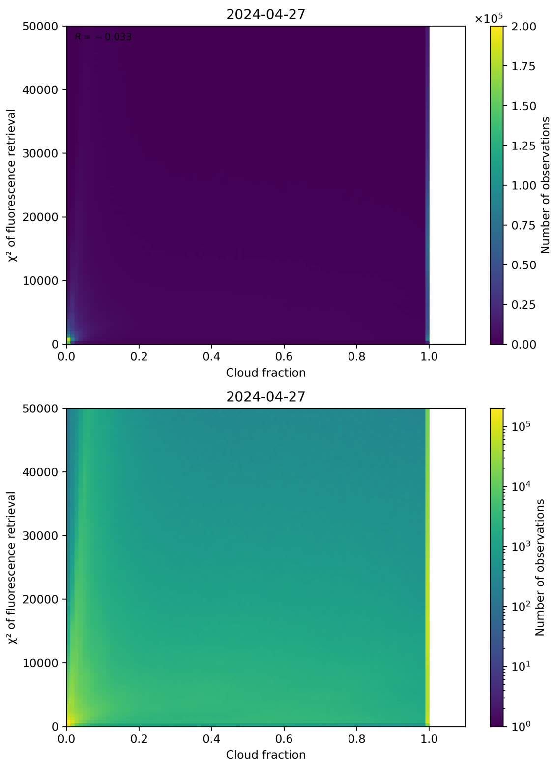
Figure 71: Scatter density plot of “Cloud fraction” against “ \chi^2 of fluorescence retrieval” for 2024-04-26 to 2024-04-28.
