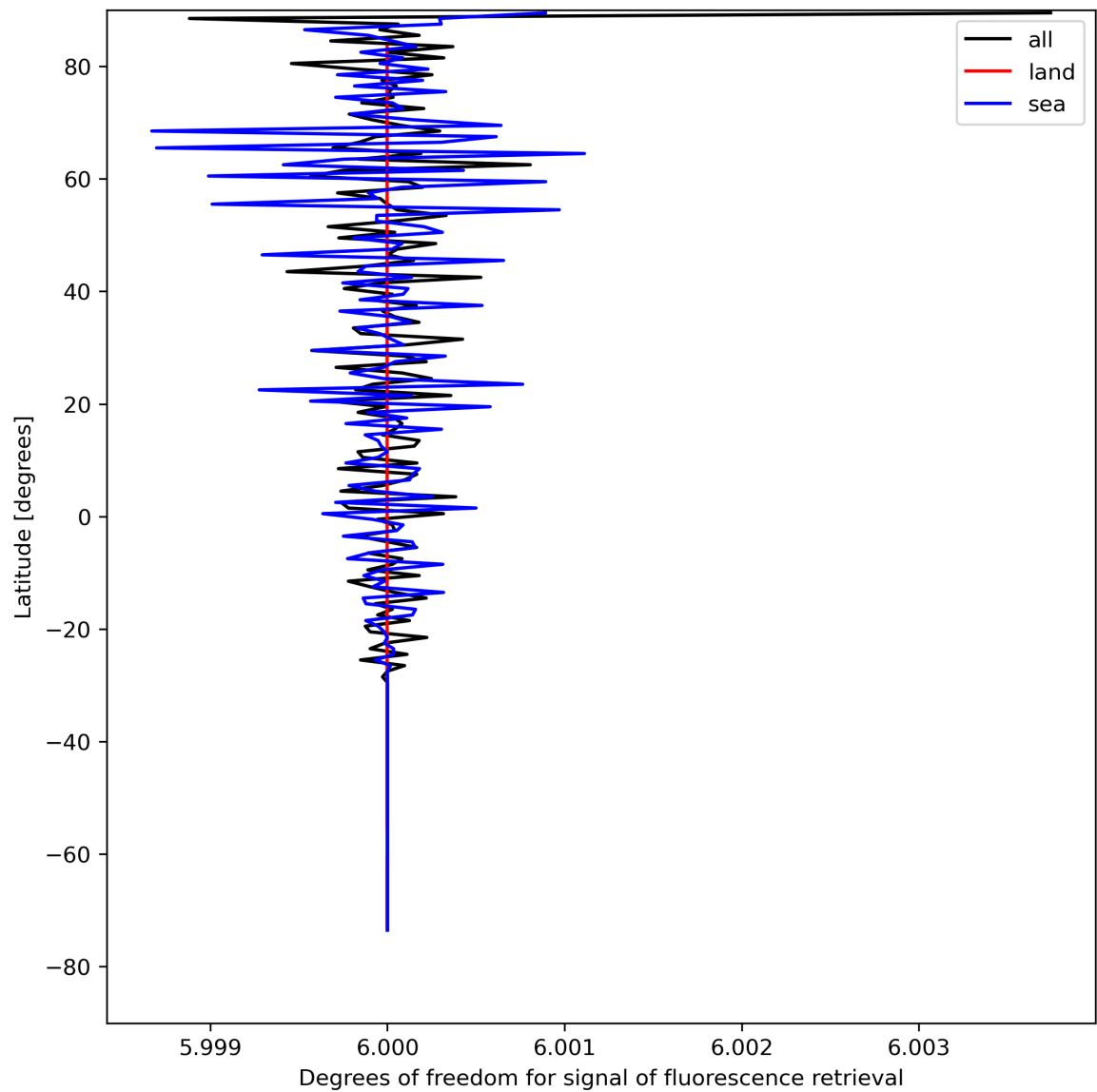
Figure 26: Zonal average of “Degrees of freedom for signal of fluorescence retrieval” for 2024-04-26 to 2024-04-28.
