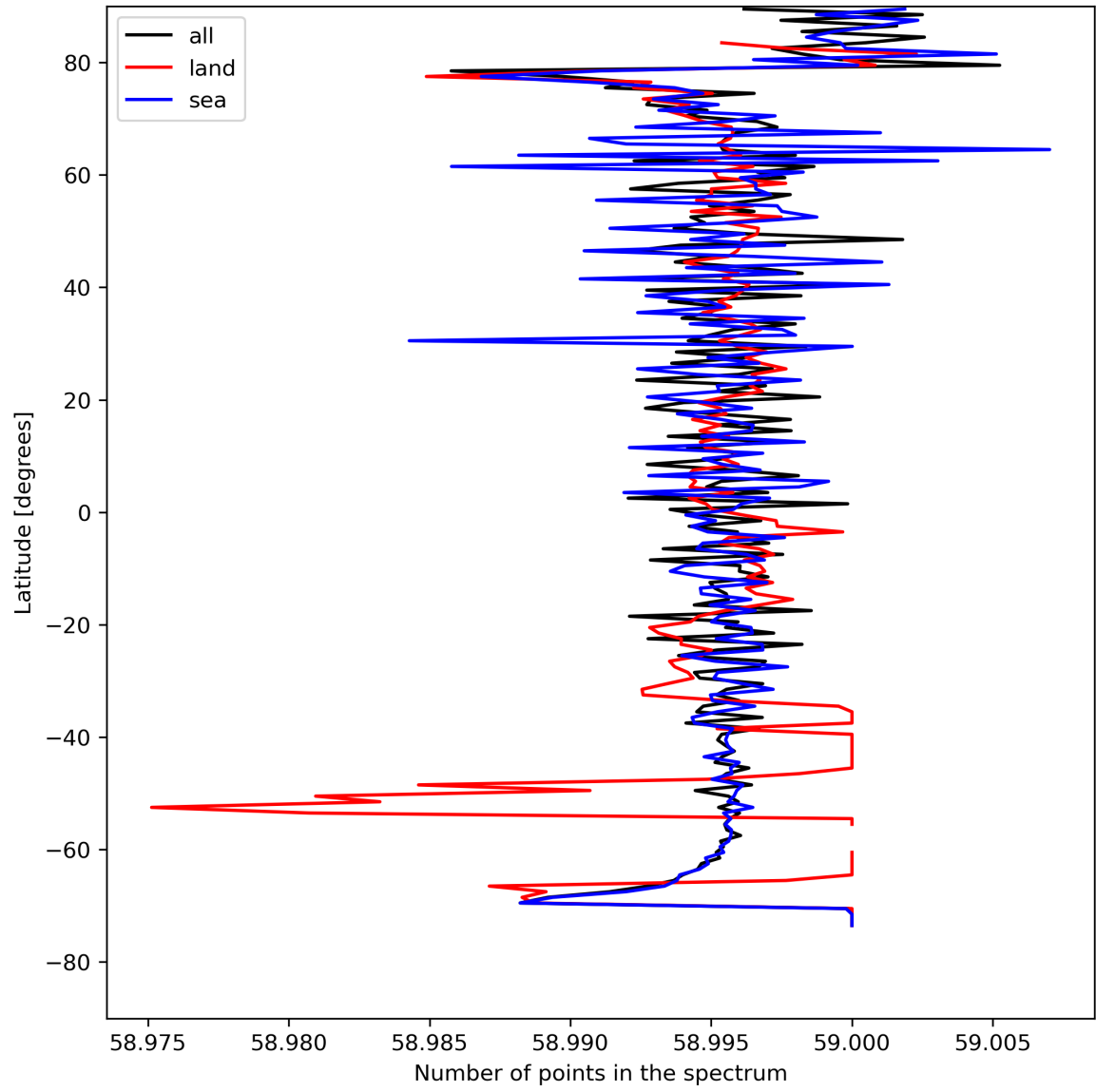
Figure 27: Zonal average of “Number of points in the spectrum” for 2024-04-26 to 2024-04-28.
