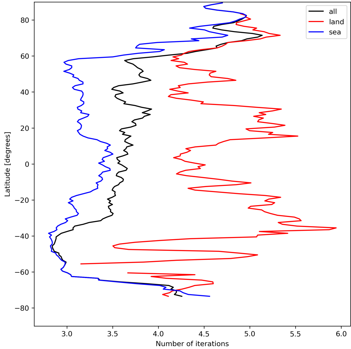
Figure 22: Zonal average of “Number of iterations” for 2024-04-26 to 2024-04-28.
