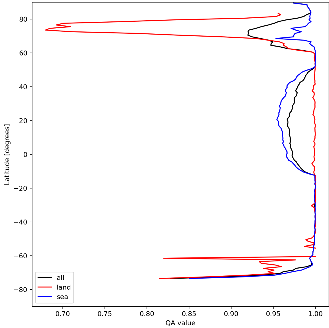
Figure 12: Zonal average of “QA value” for 2024-04-26 to 2024-04-28.
