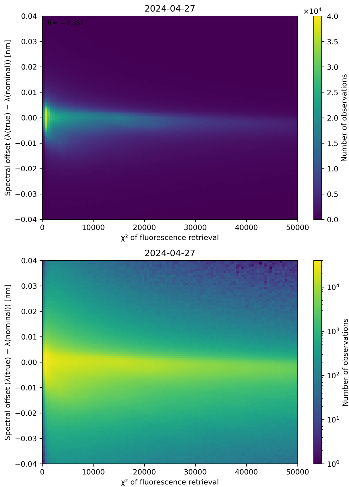
Figure 69: Scatter density plot of " \chi^2 of fluorescence retrieval" against "Spectral offset ( \lambda(\text{true}) - \lambda(\text{nominal}) )" for 2024-04-26 to 2024-04-28.
