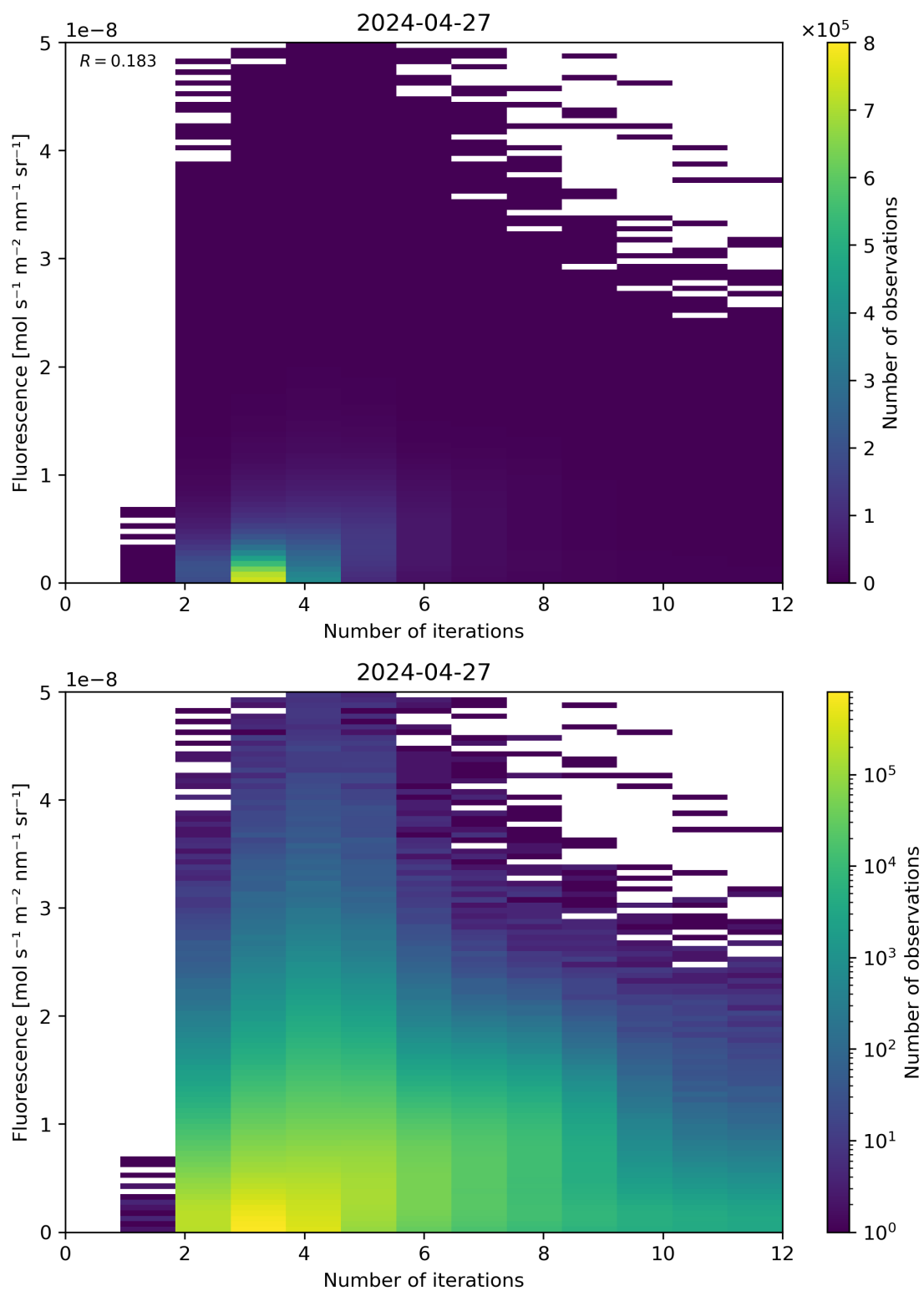
Figure 98: Scatter density plot of “Number of iterations” against “Fluorescence” for 2024-04-26 to 2024-04-28.
