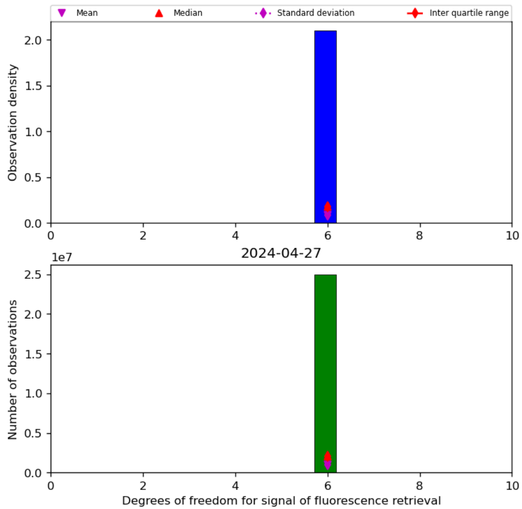
Figure 43: Histogram of “Degrees of freedom for signal of fluorescence retrieval” for 2024-04-26 to 2024-04-28
