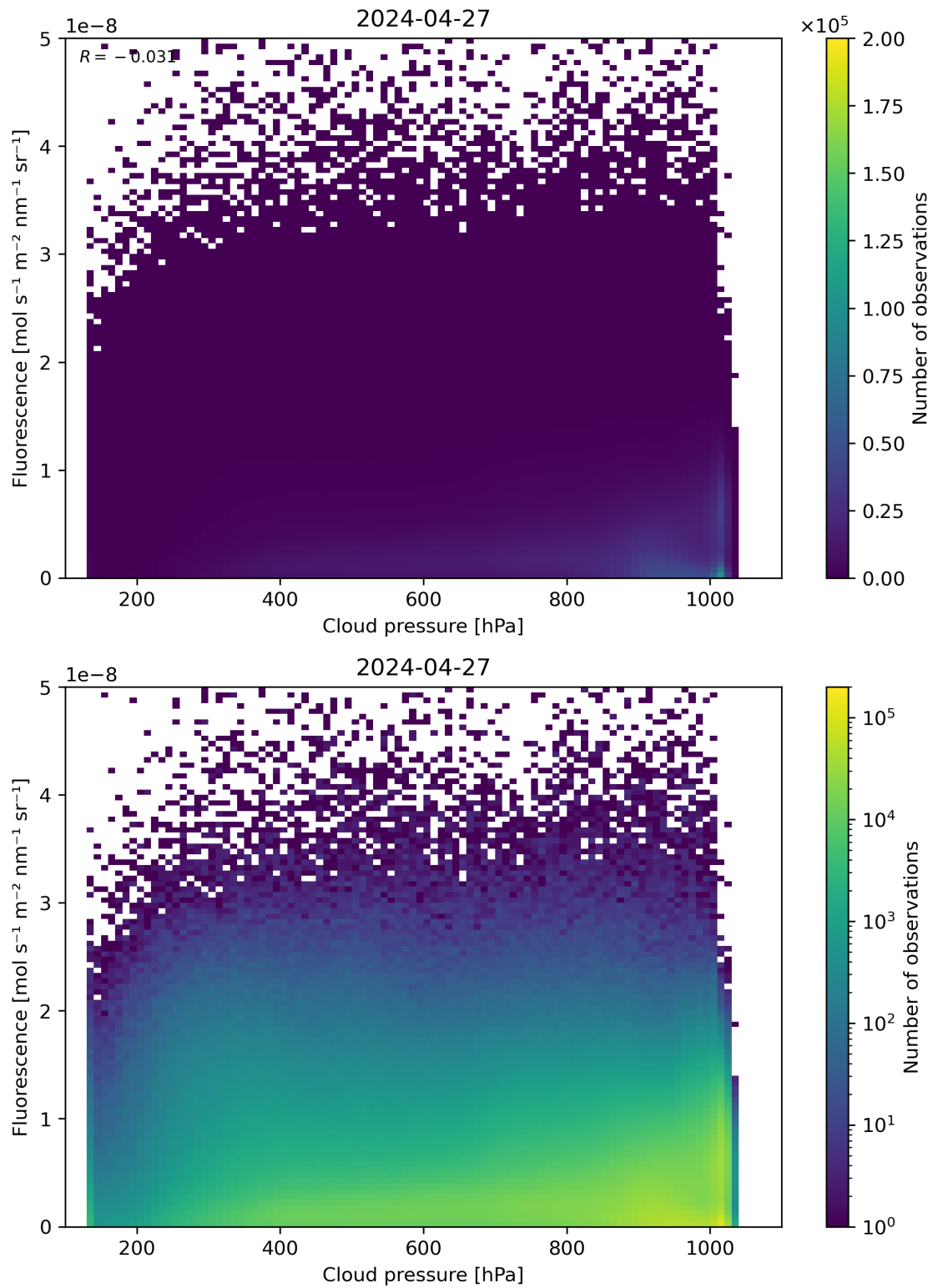
Figure 80: Scatter density plot of “Cloud pressure” against “Fluorescence” for 2024-04-26 to 2024-04-28.
