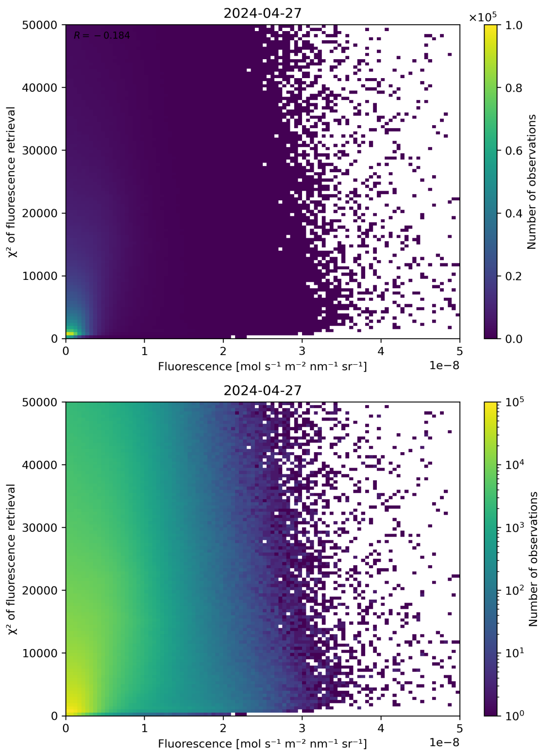
Figure 85: Scatter density plot of “Fluorescence” against “ \chi^2 of fluorescence retrieval” for 2024-04-26 to 2024-04-28.
