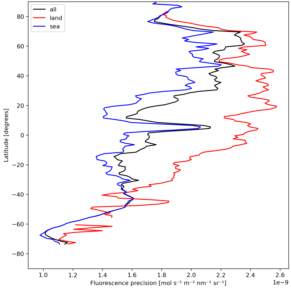
Figure 24: Zonal average of “Fluorescence precision” for 2024-04-26 to 2024-04-28.
