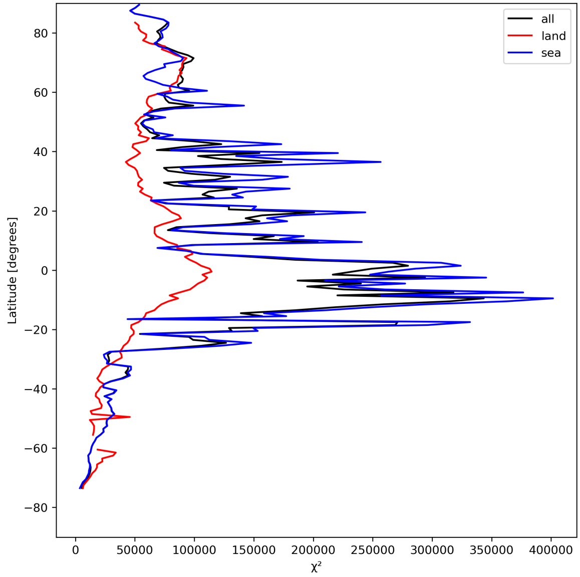
Figure 21: Zonal average of “ \chi^2 ” for 2024-04-26 to 2024-04-28.
