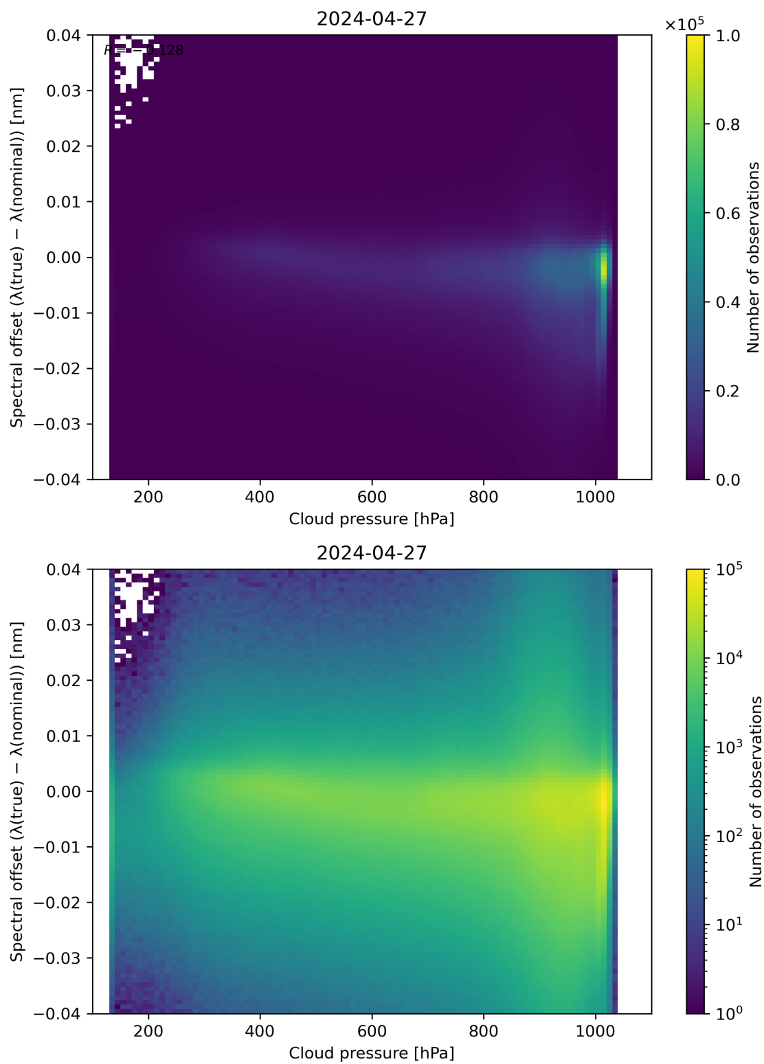
Figure 84: Scatter density plot of “Cloud pressure” against “Spectral offset ( \lambda(\text{true}) - \lambda(\text{nominal}) )” for 2024-04-26 to 2024-04-28.
