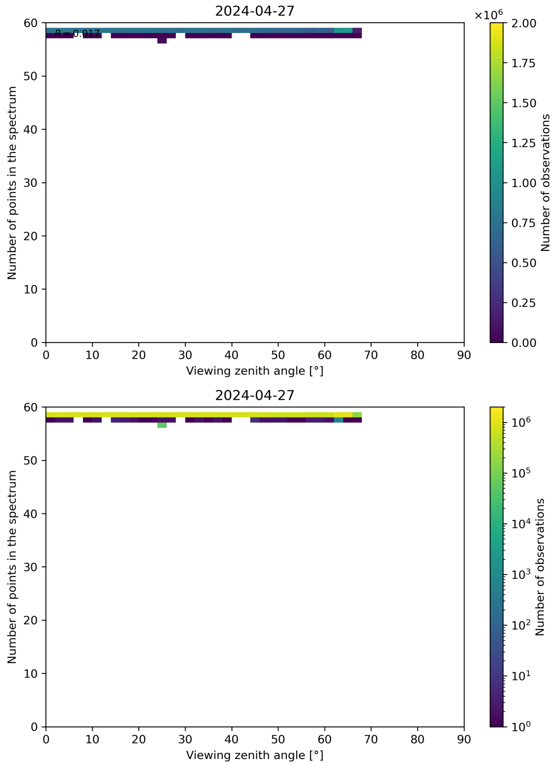
Figure 125: Scatter density plot of “Viewing zenith angle” against “Number of points in the spectrum” for 2024-04-26 to 2024-04-28.
