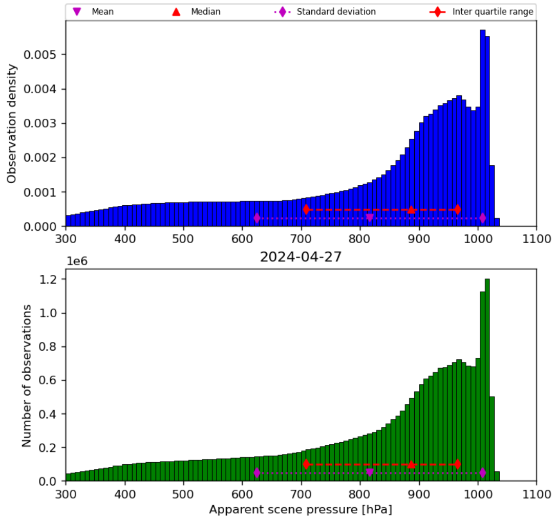
Figure 36: Histogram of “Apparent scene pressure” for 2024-04-26 to 2024-04-28
