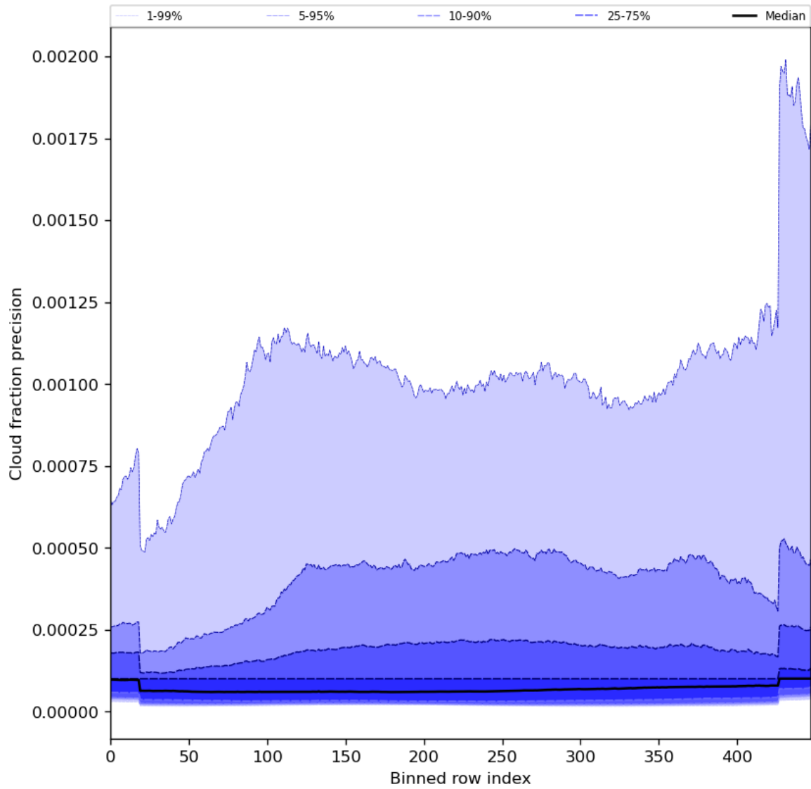
Figure 50: Along track statistics of “Cloud fraction precision” for 2024-04-26 to 2024-04-28
