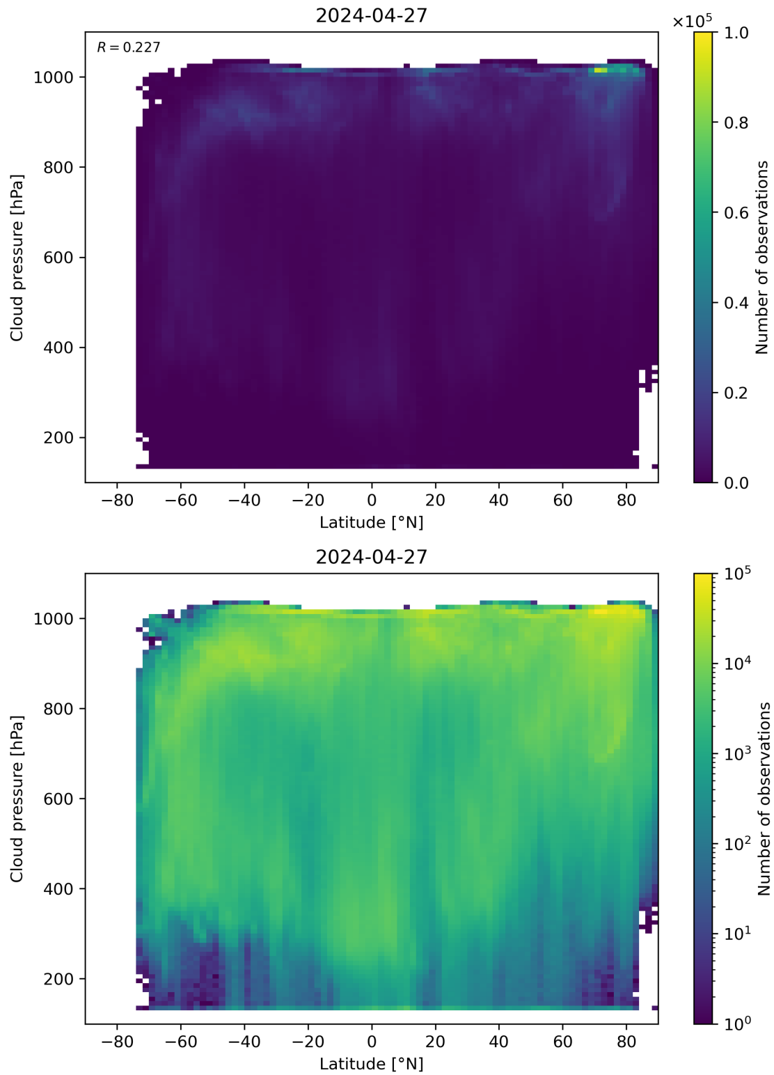
Figure 91: Scatter density plot of “Latitude” against “Cloud pressure” for 2024-04-26 to 2024-04-28.
