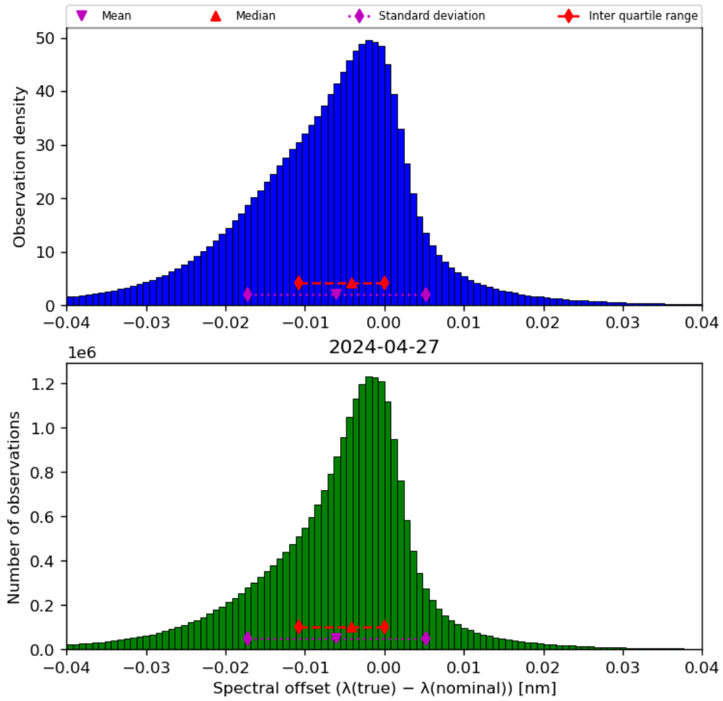
Figure 45: Histogram of “Spectral offset ( \lambda(\text{true}) - \lambda(\text{nominal}) )” for 2024-04-26 to 2024-04-28
