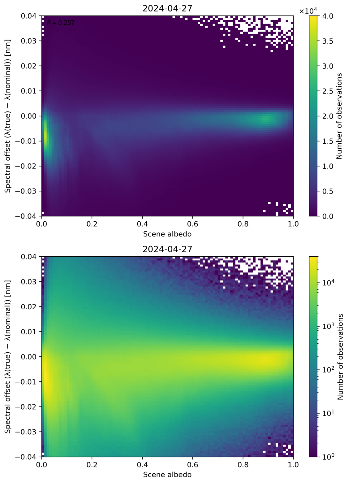
Figure 107: Scatter density plot of “Scene albedo” against “Spectral offset ( \lambda(\text{true}) - \lambda(\text{nominal}) )” for 2024-04-26 to 2024-04-28.
