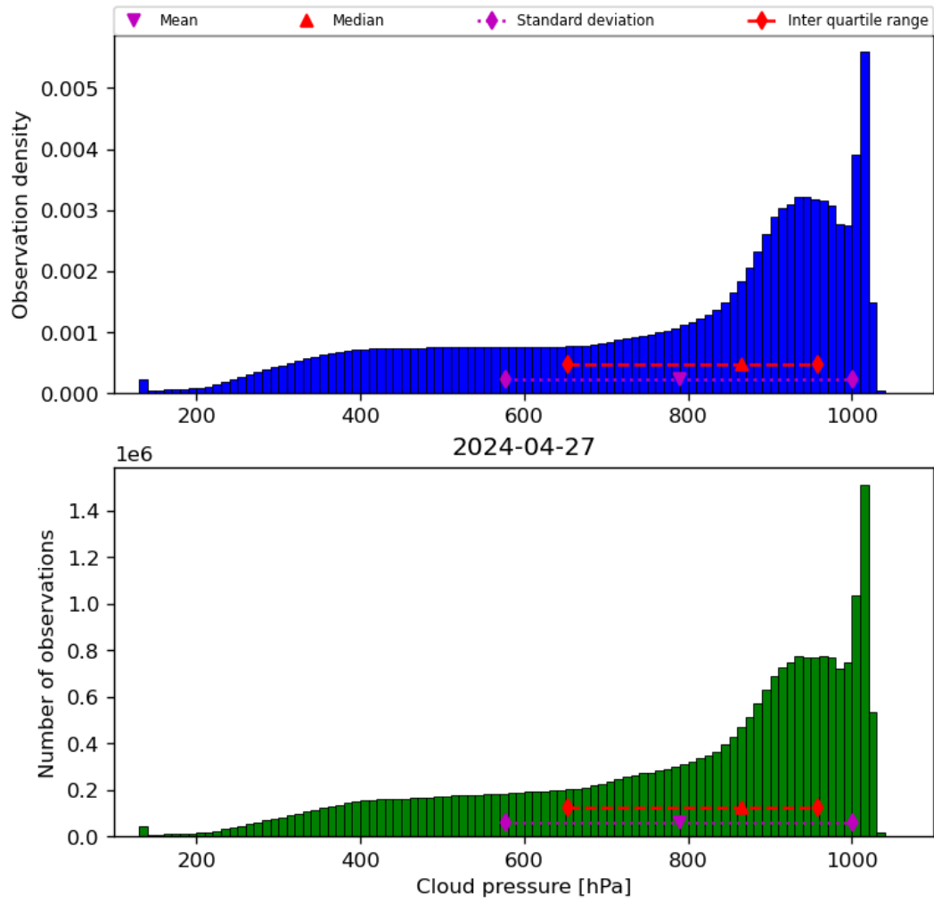
Figure 30: Histogram of “Cloud pressure” for 2024-04-26 to 2024-04-28
