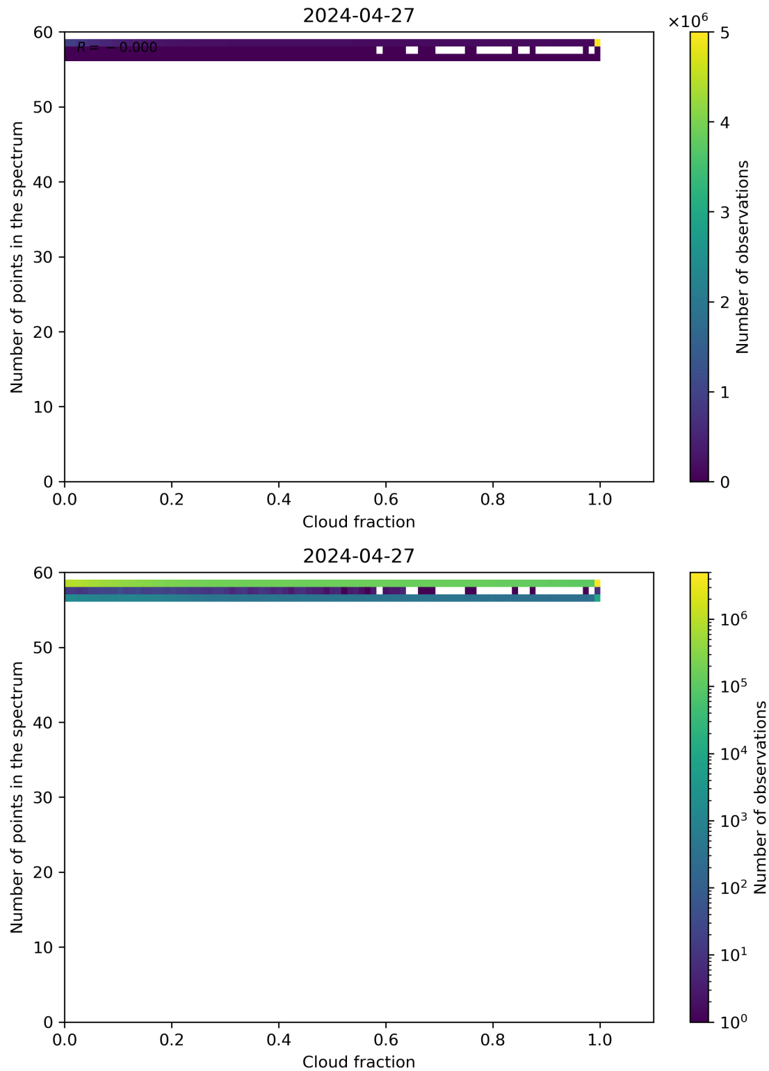
Figure 74: Scatter density plot of “Cloud fraction” against “Number of points in the spectrum” for 2024-04-26 to 2024-04-28.
