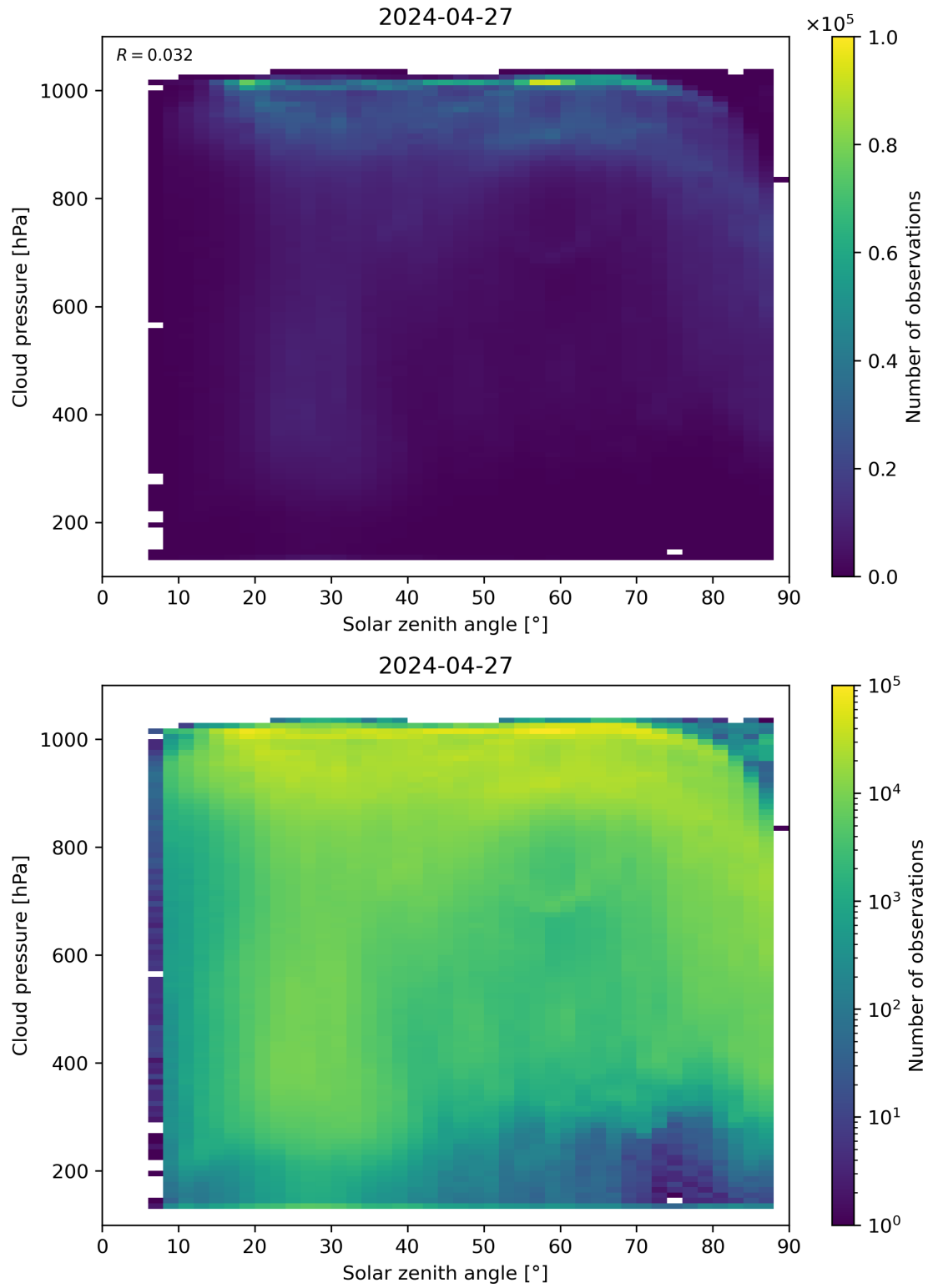
Figure 111: Scatter density plot of “Solar zenith angle” against “Cloud pressure” for 2024-04-26 to 2024-04-28.
