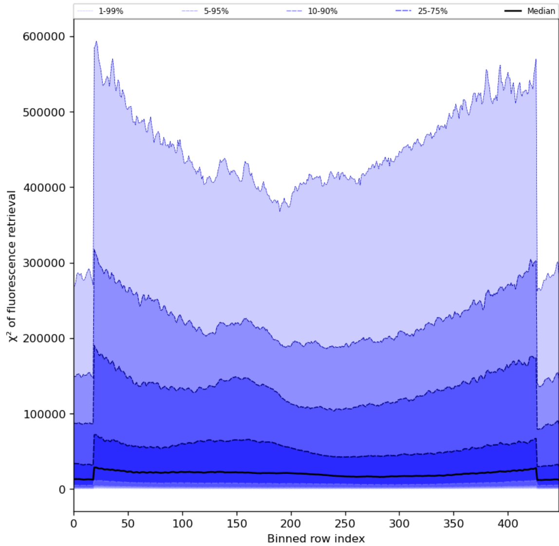
Figure 59: Along track statistics of “ \chi^2 of fluorescence retrieval” for 2024-04-26 to 2024-04-28
