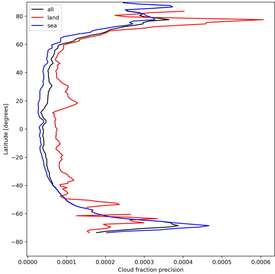
Figure 16: Zonal average of “Cloud fraction precision” for 2024-04-26 to 2024-04-28.
