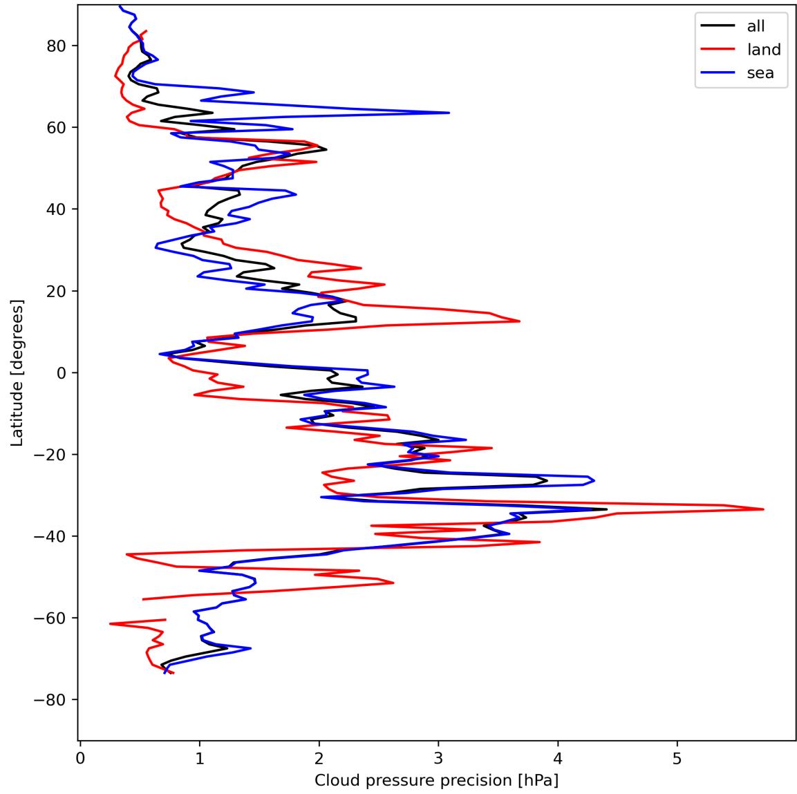
Figure 14: Zonal average of “Cloud pressure precision” for 2024-04-26 to 2024-04-28.
