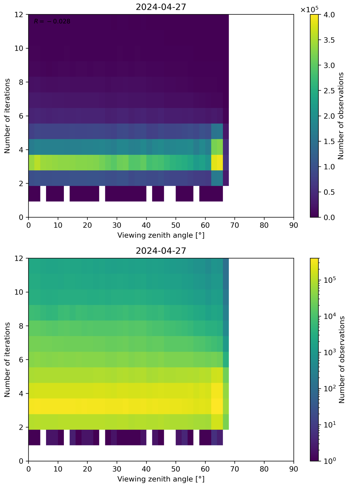
Figure 124: Scatter density plot of “Viewing zenith angle” against “Number of iterations” for 2024-04-26 to 2024-04-28.
