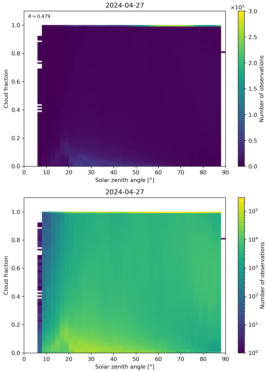
Figure 110: Scatter density plot of “Solar zenith angle” against “Cloud fraction” for 2024-04-26 to 2024-04-28.
