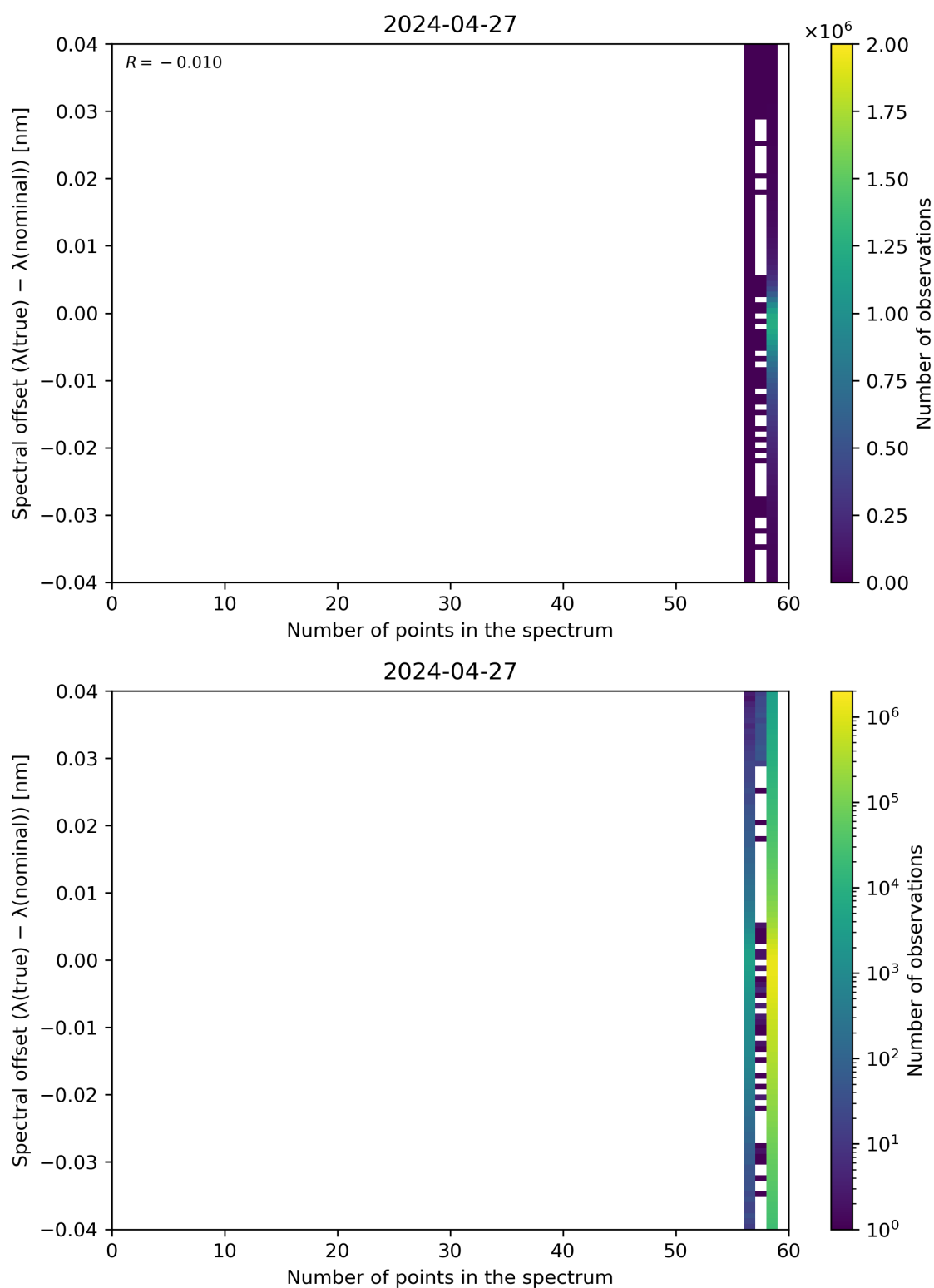
Figure 101: Scatter density plot of “Number of points in the spectrum” against “Spectral offset ( \lambda(\text{true}) - \lambda(\text{nominal}) )” for 2024-04-26 to 2024-04-28.
