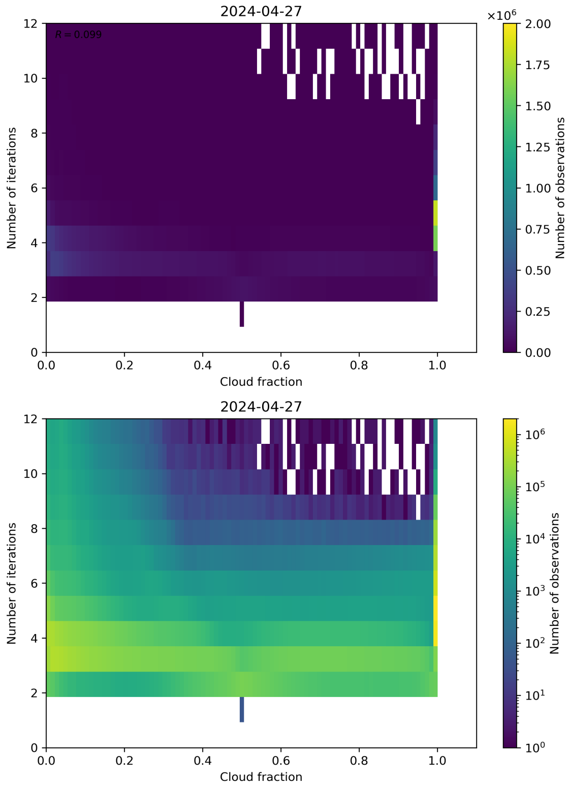
Figure 73: Scatter density plot of “Cloud fraction” against “Number of iterations” for 2024-04-26 to 2024-04-28.
