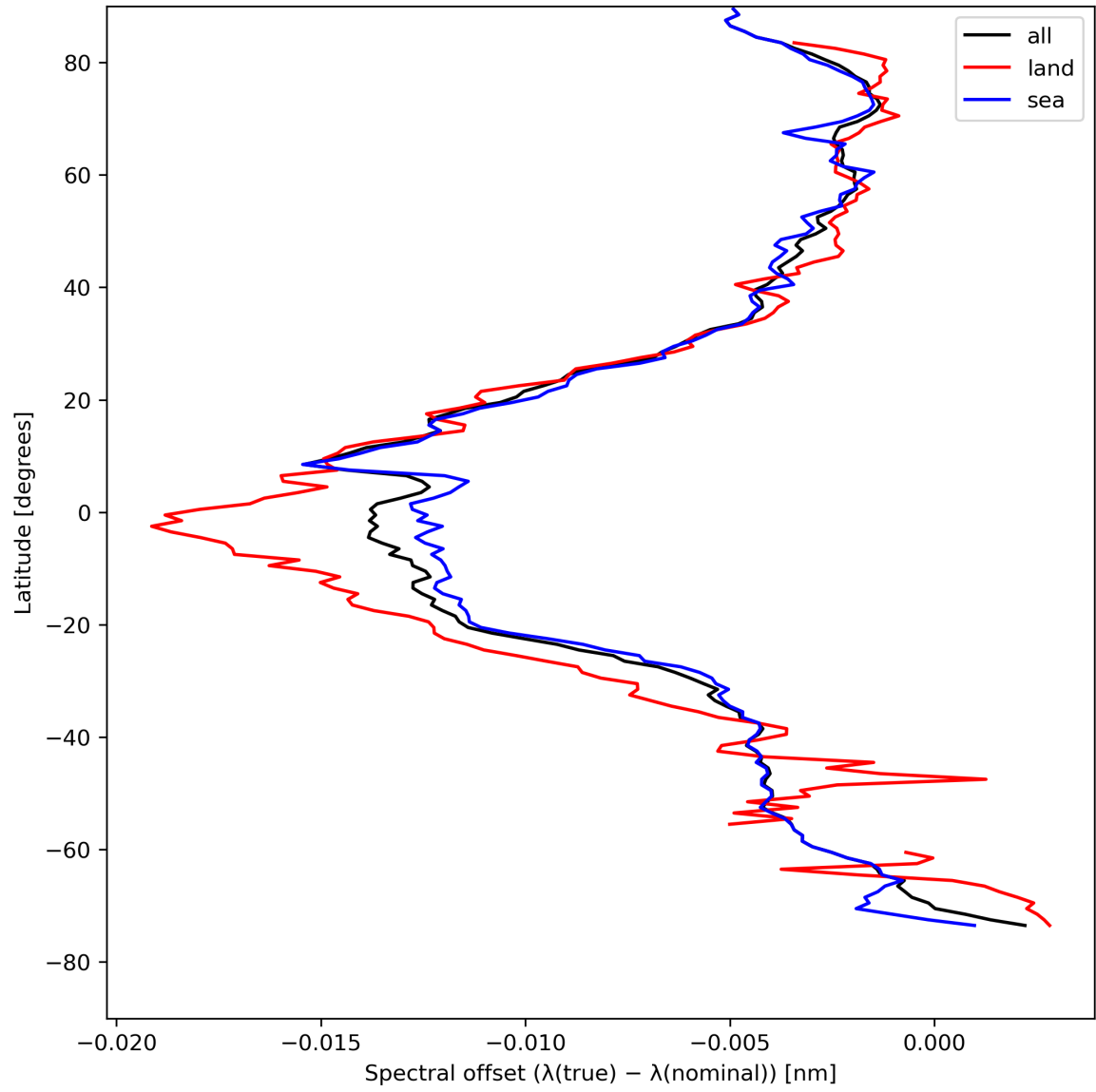
Figure 28: Zonal average of “Spectral offset ( \lambda(\text{true}) - \lambda(\text{nominal}) )” for 2024-04-26 to 2024-04-28.
