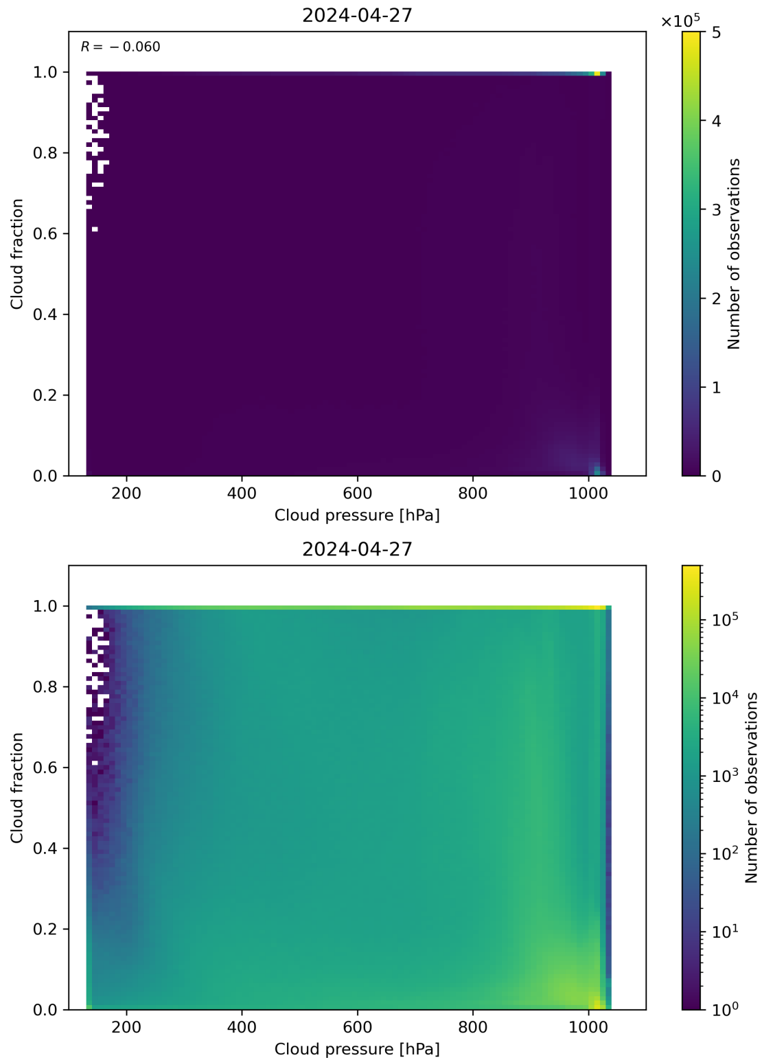
Figure 79: Scatter density plot of “Cloud pressure” against “Cloud fraction” for 2024-04-26 to 2024-04-28.
