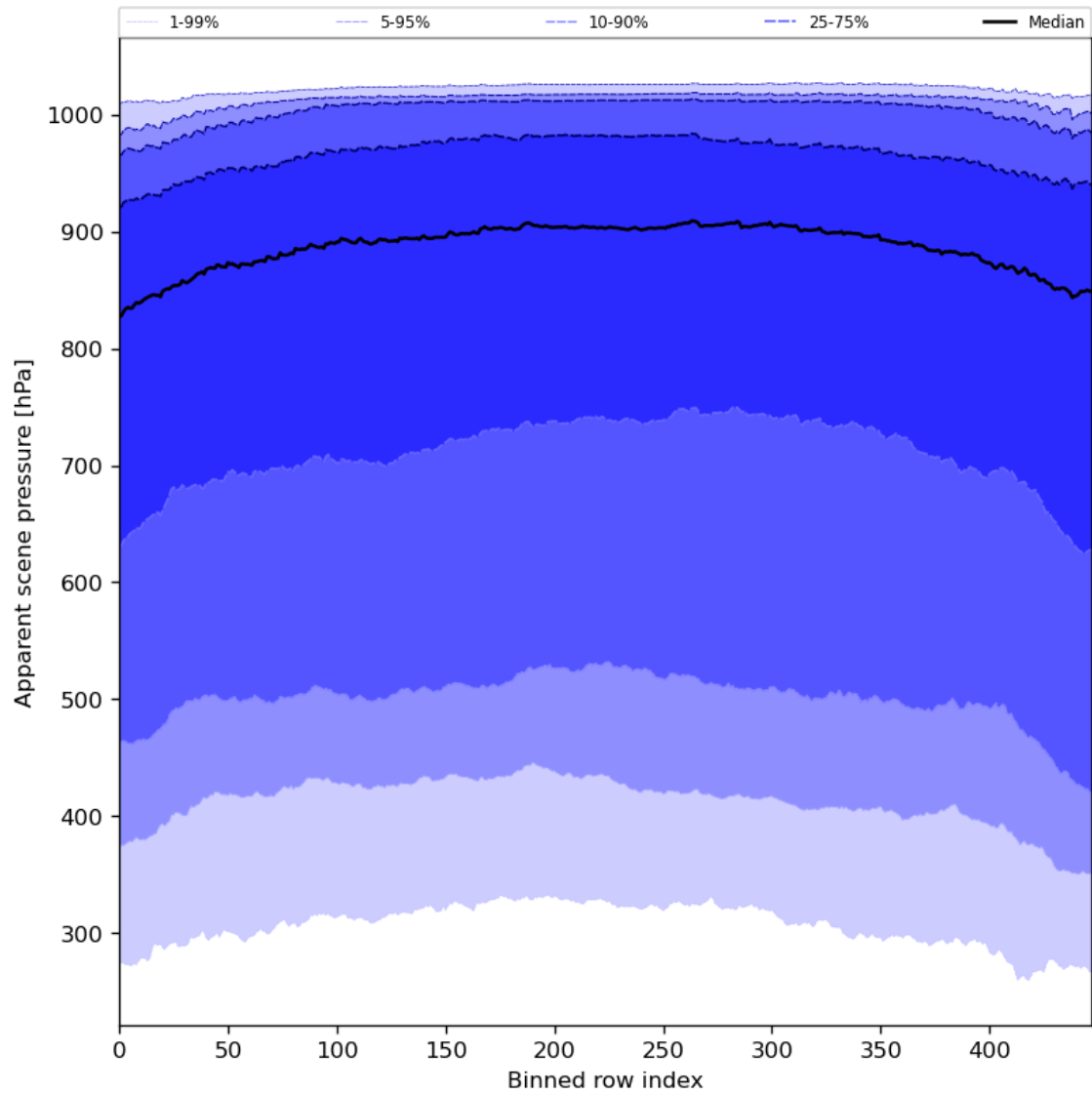
Figure 53: Along track statistics of “Apparent scene pressure” for 2024-04-26 to 2024-04-28
