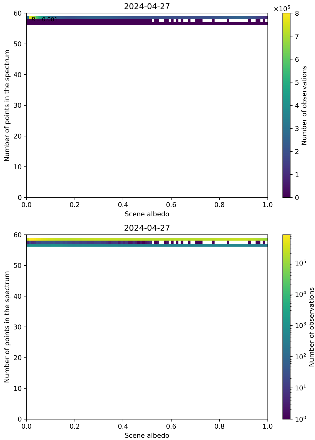
Figure 106: Scatter density plot of “Scene albedo” against “Number of points in the spectrum” for 2024-04-26 to 2024-04-28.
