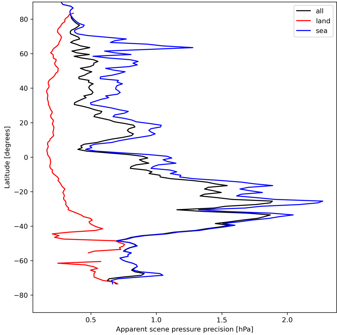
Figure 20: Zonal average of “Apparent scene pressure precision” for 2024-04-26 to 2024-04-28.
