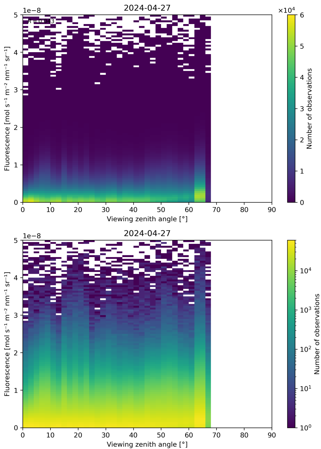
Figure 122: Scatter density plot of “Viewing zenith angle” against “Fluorescence” for 2024-04-26 to 2024-04-28.
