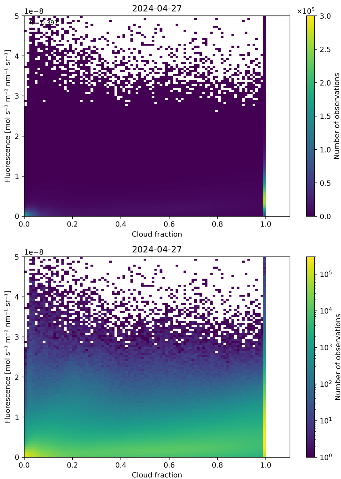
Figure 72: Scatter density plot of "Cloud fraction" against "Fluorescence" for 2024-04-26 to 2024-04-28.
