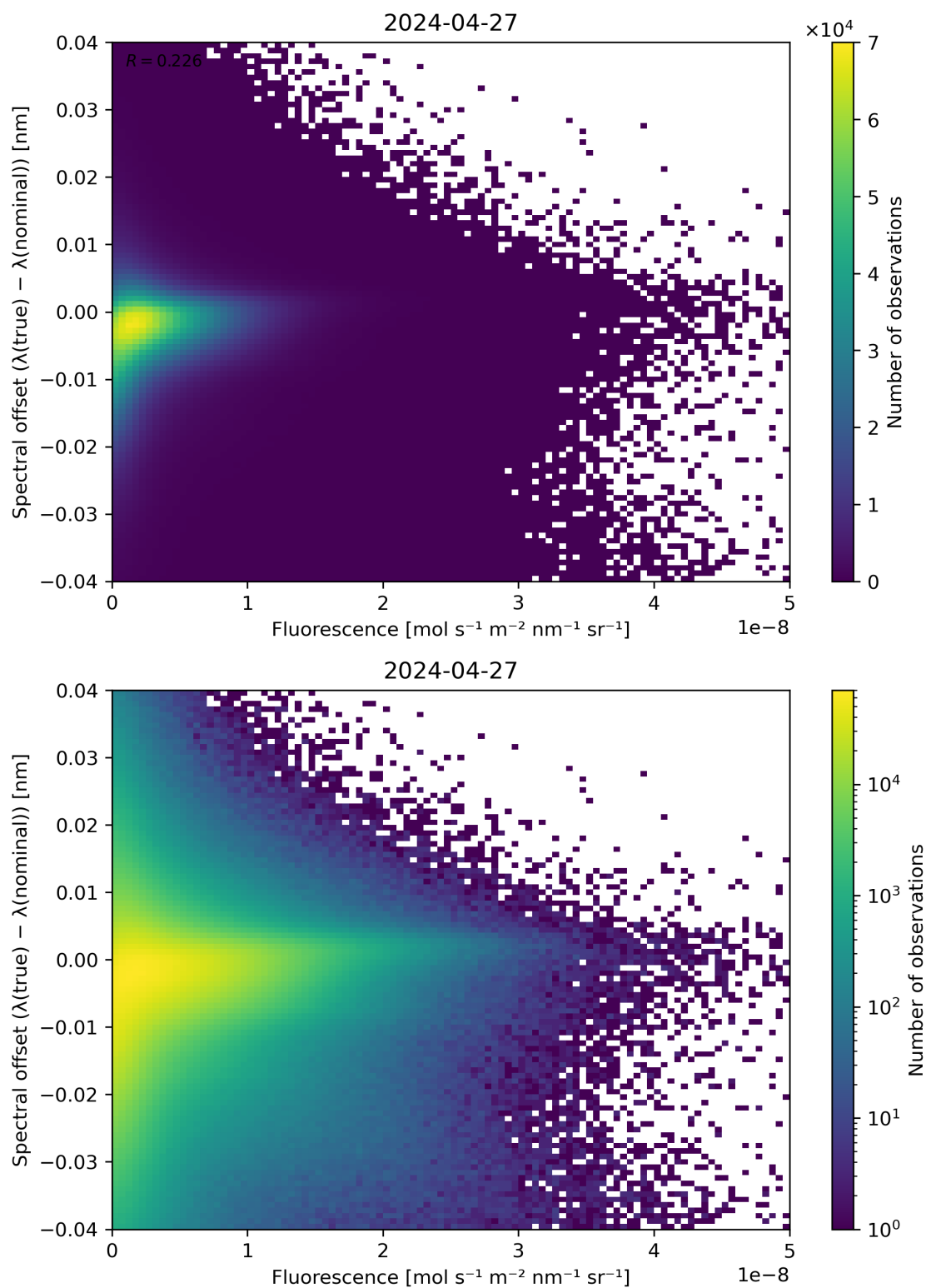
Figure 87: Scatter density plot of “Fluorescence” against “Spectral offset ( \lambda(\text{true}) - \lambda(\text{nominal}) )” for 2024-04-26 to 2024-04-28.
