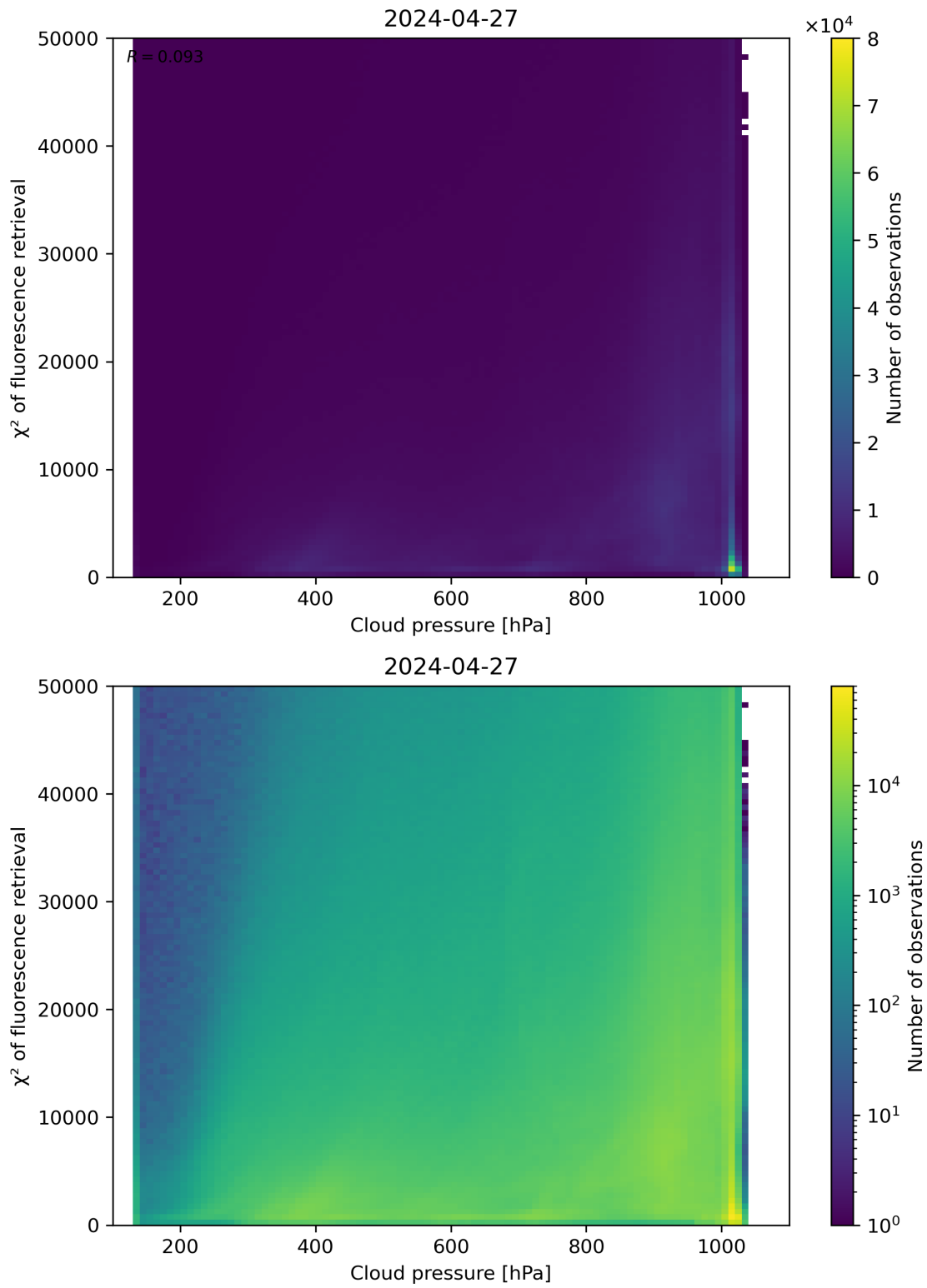
Figure 78: Scatter density plot of “Cloud pressure” against “ \chi^2 of fluorescence retrieval” for 2024-04-26 to 2024-04-28.
