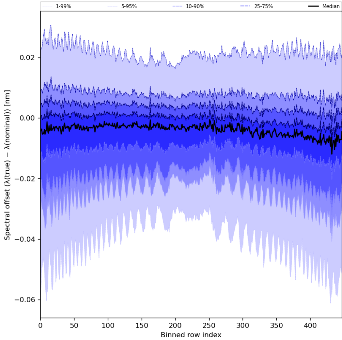
Figure 62: Along track statistics of “Spectral offset ( \lambda(\text{true}) - \lambda(\text{nominal}) )” for 2024-04-26 to 2024-04-28
