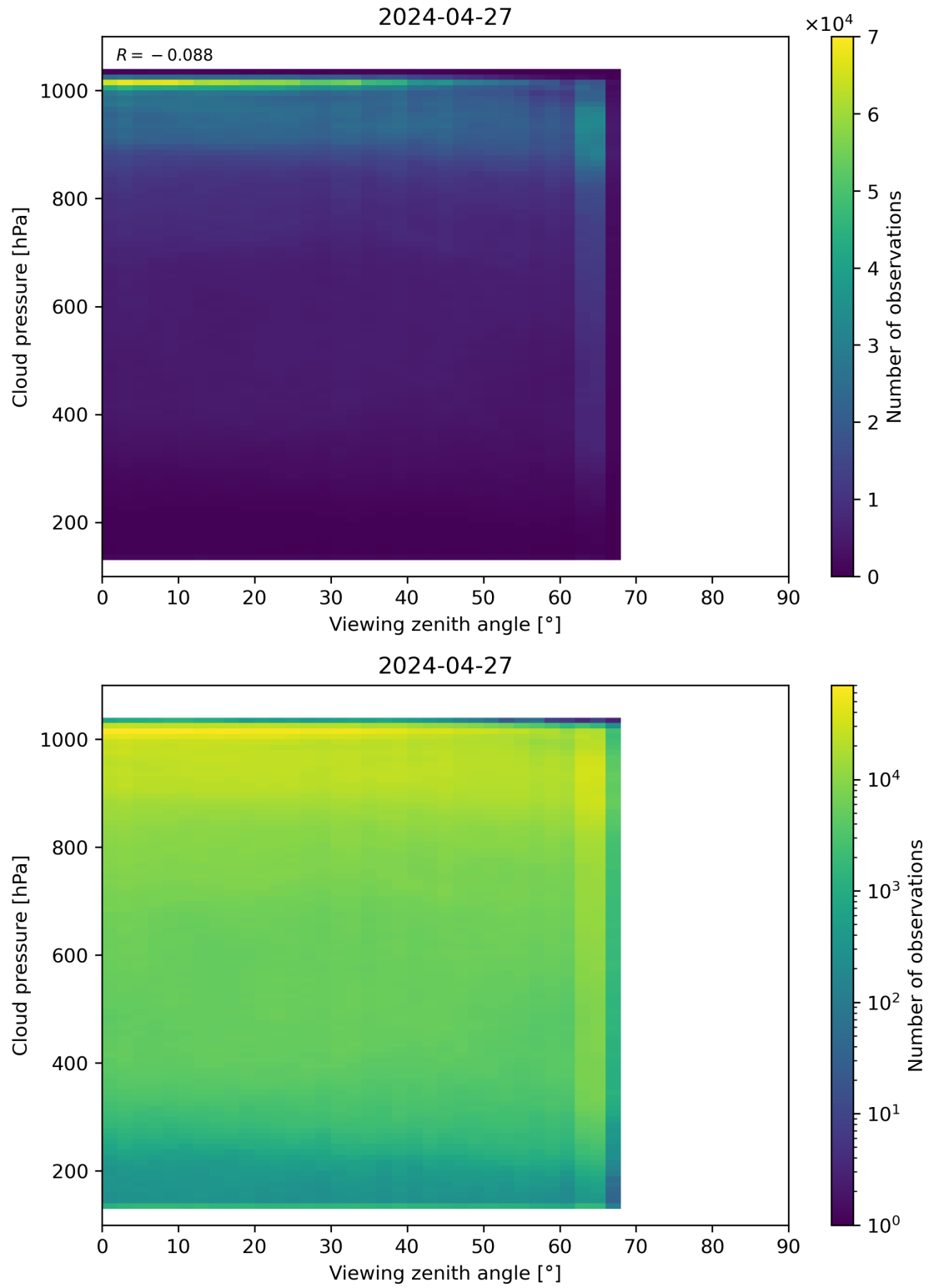
Figure 121: Scatter density plot of “Viewing zenith angle” against “Cloud pressure” for 2024-04-26 to 2024-04-28.
