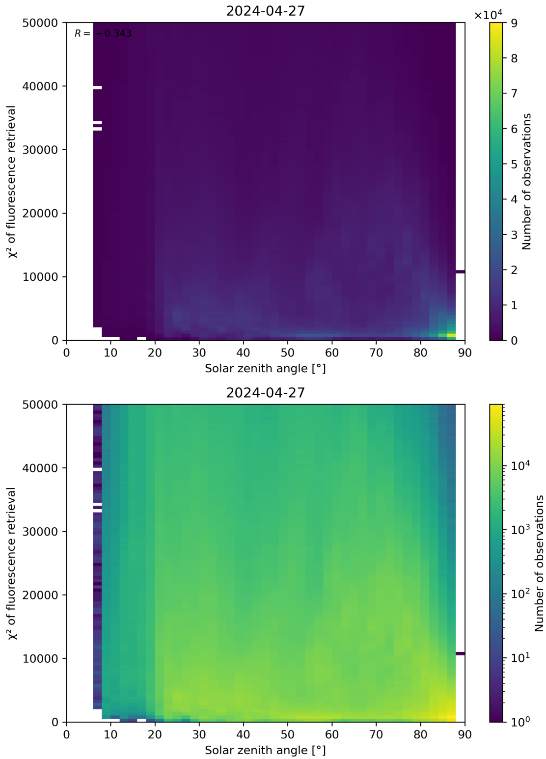
Figure 109: Scatter density plot of “Solar zenith angle” against “ \chi^2 of fluorescence retrieval” for 2024-04-26 to 2024-04-28.
