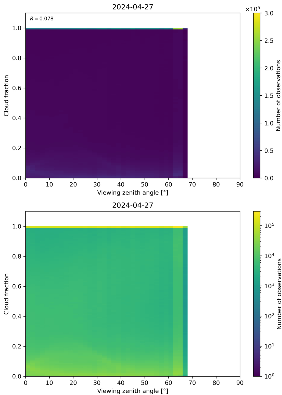
Figure 120: Scatter density plot of “Viewing zenith angle” against “Cloud fraction” for 2024-04-26 to 2024-04-28.
