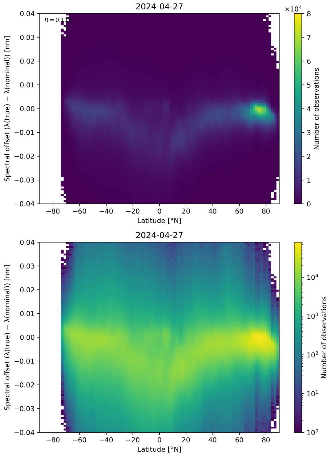
Figure 96: Scatter density plot of “Latitude” against “Spectral offset ( \lambda(\text{true}) - \lambda(\text{nominal}) )” for 2024-04-26 to 2024-04-28.
