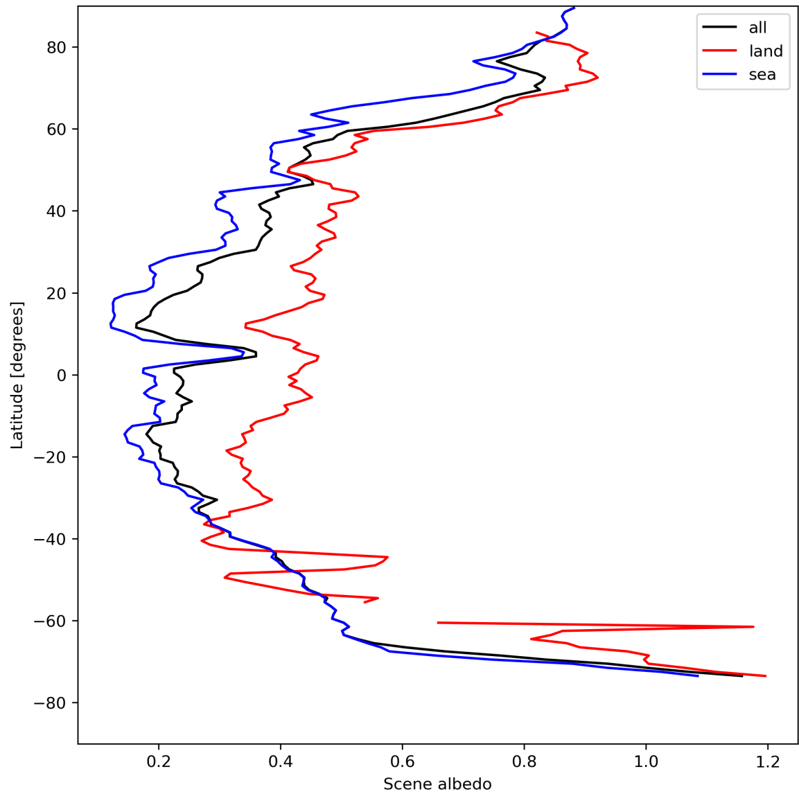
Figure 17: Zonal average of “Scene albedo” for 2024-04-26 to 2024-04-28.
