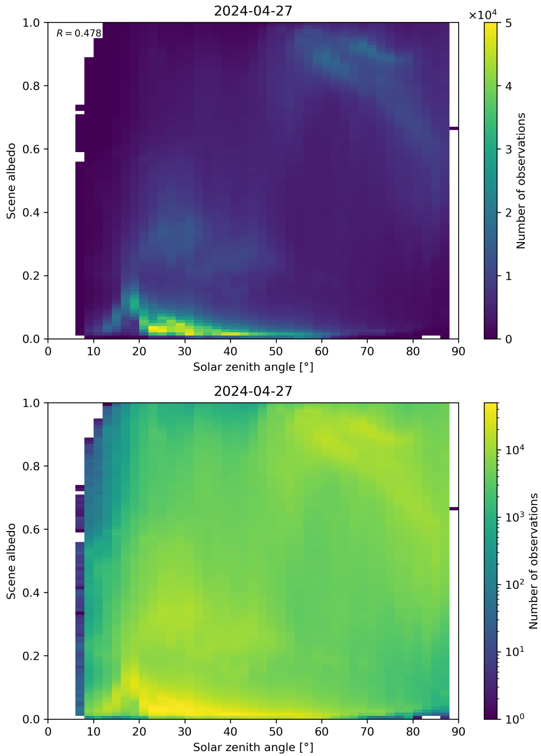
Figure 116: Scatter density plot of “Solar zenith angle” against “Scene albedo” for 2024-04-26 to 2024-04-28.
