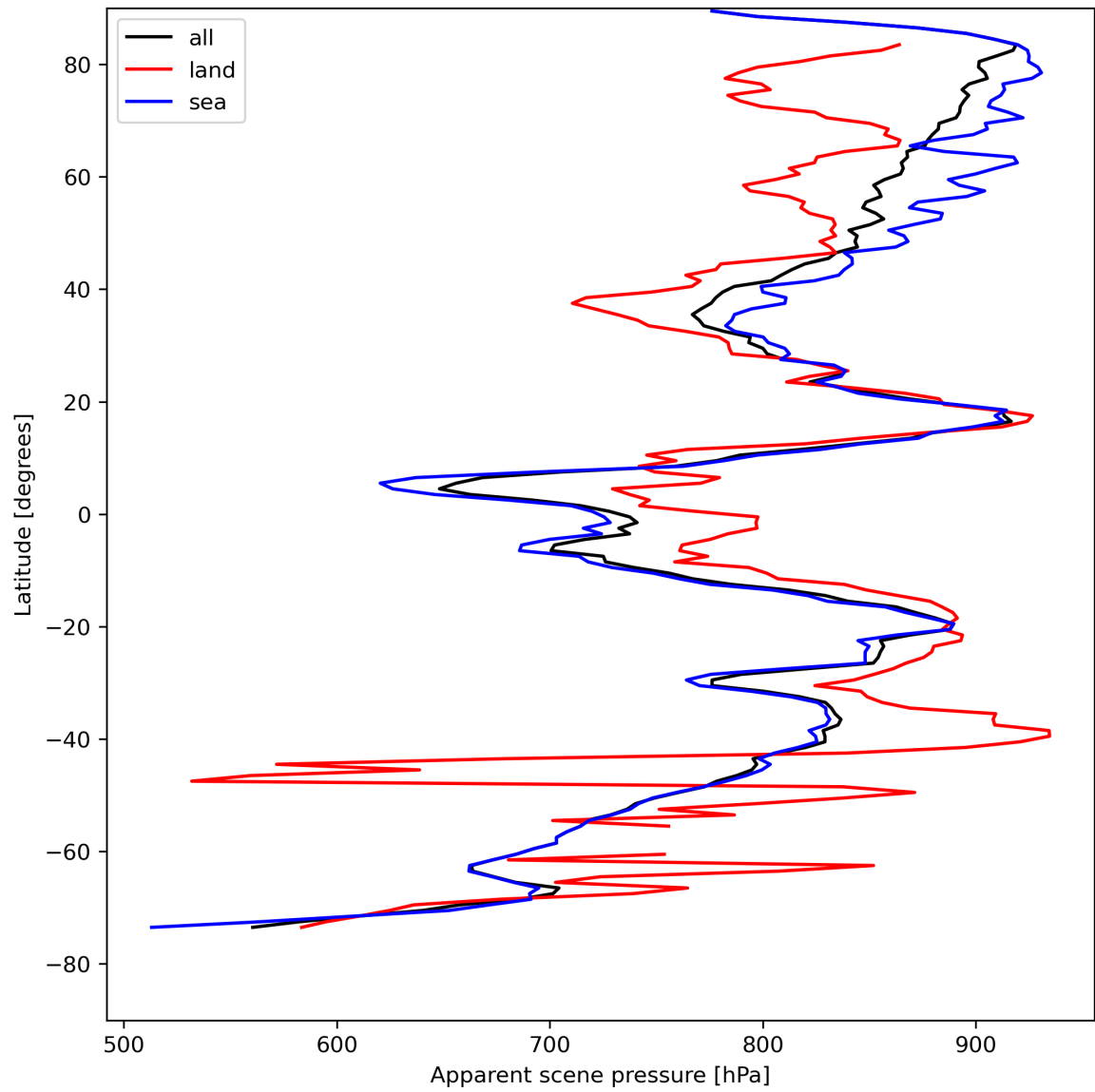
Figure 19: Zonal average of “Apparent scene pressure” for 2024-04-26 to 2024-04-28.
