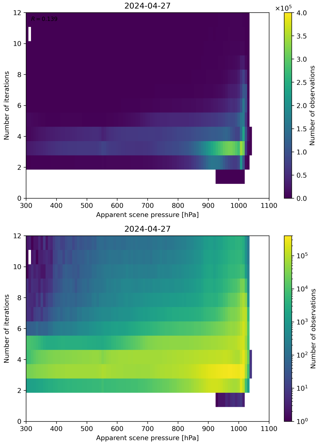
Figure 65: Scatter density plot of “Apparent scene pressure” against “Number of iterations” for 2024-04-26 to 2024-04-28.
