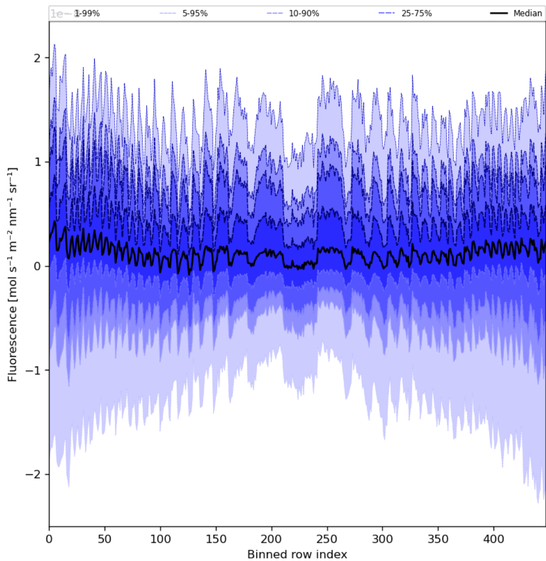
Figure 57: Along track statistics of “Fluorescence” for 2024-04-26 to 2024-04-28
