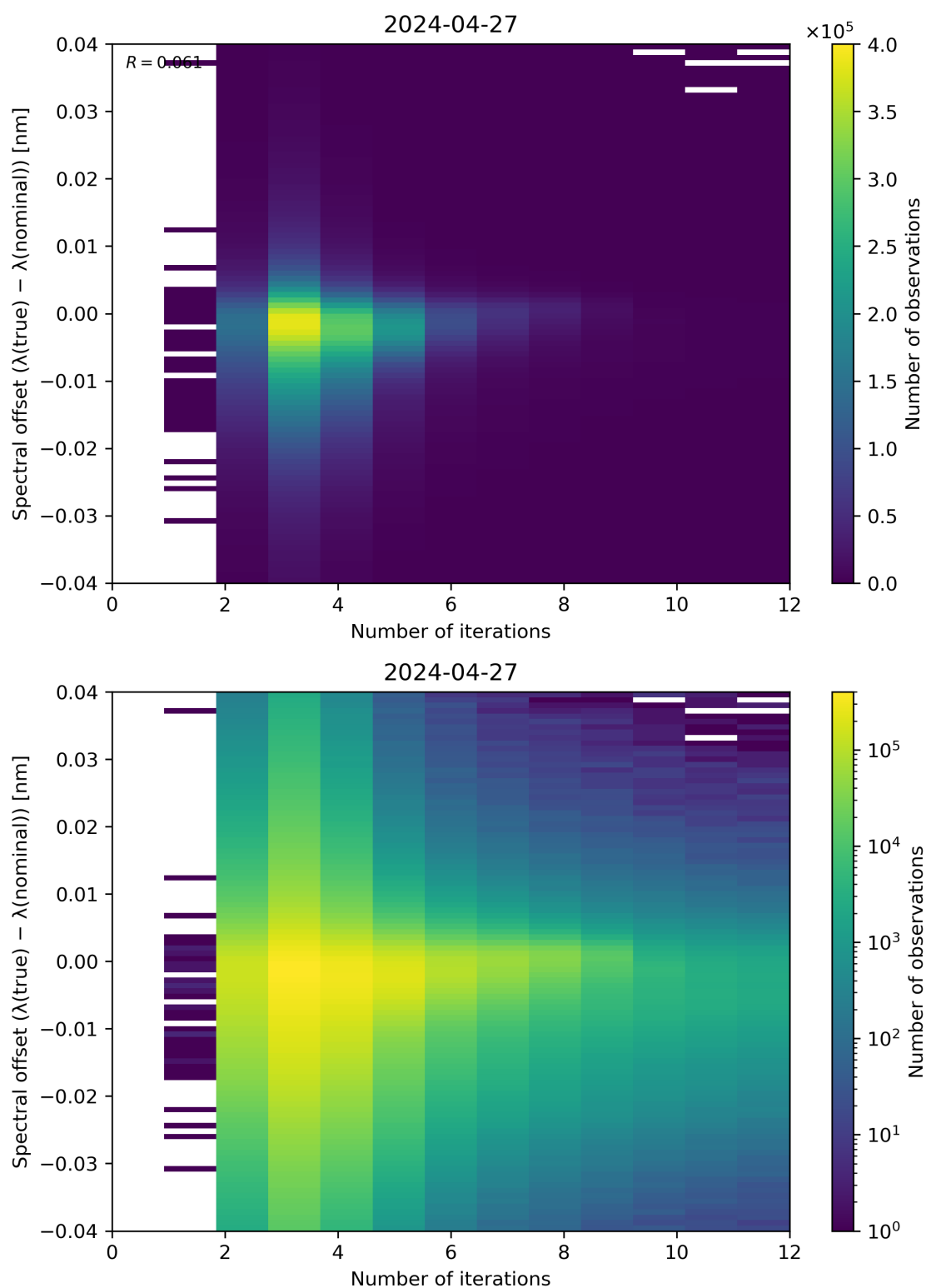
Figure 100: Scatter density plot of “Number of iterations” against “Spectral offset ( \lambda(\text{true}) - \lambda(\text{nominal}) )” for 2024-04-26 to 2024-04-28.
