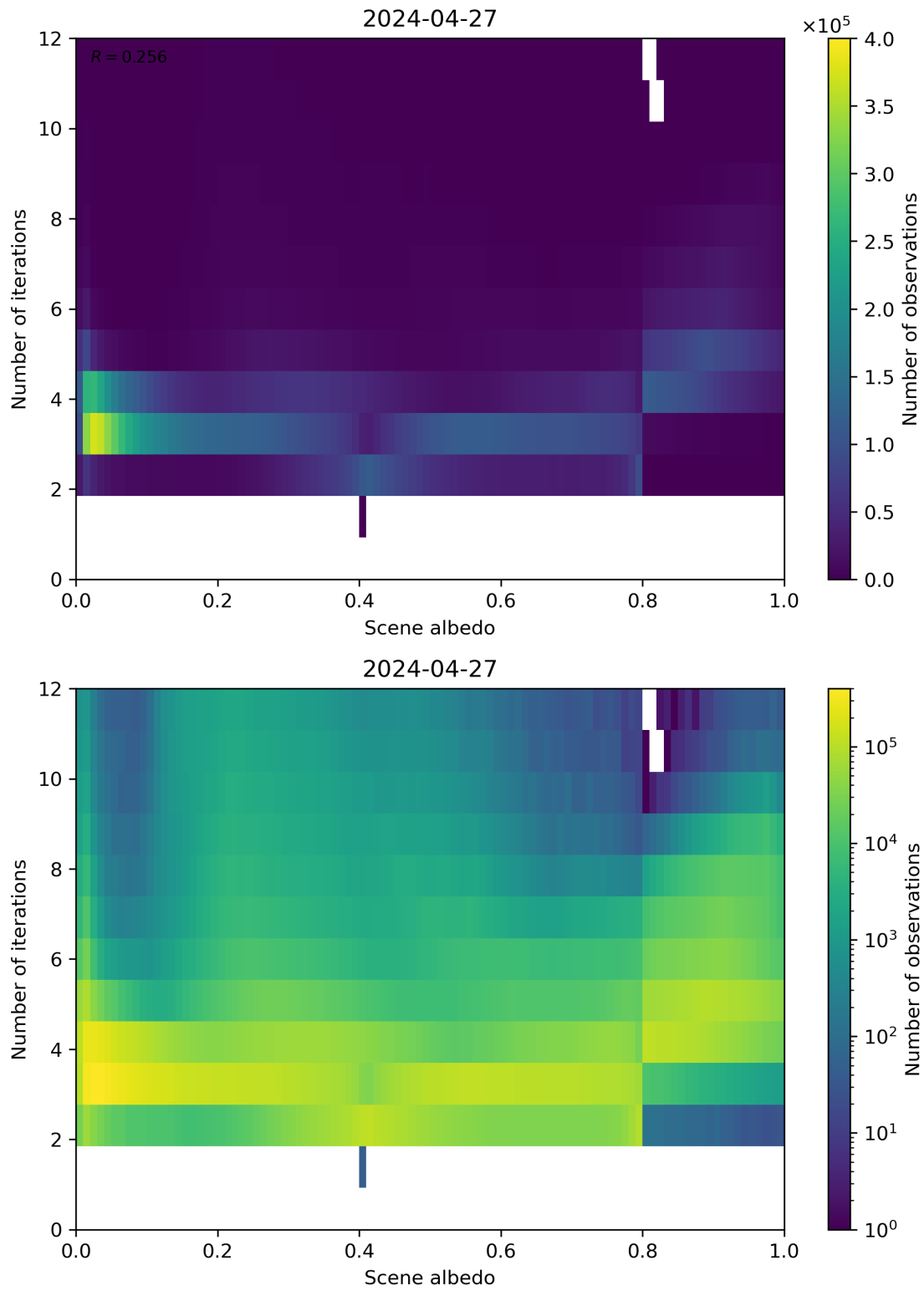
Figure 105: Scatter density plot of “Scene albedo” against “Number of iterations” for 2024-04-26 to 2024-04-28.
