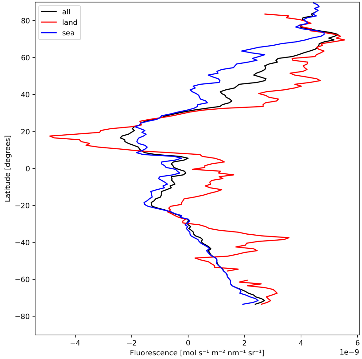
Figure 23: Zonal average of “Fluorescence” for 2024-04-26 to 2024-04-28.
