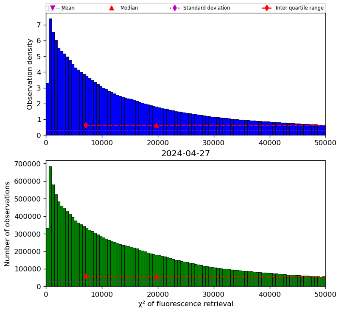
Figure 42: Histogram of “ \chi^2 of fluorescence retrieval” for 2024-04-26 to 2024-04-28
