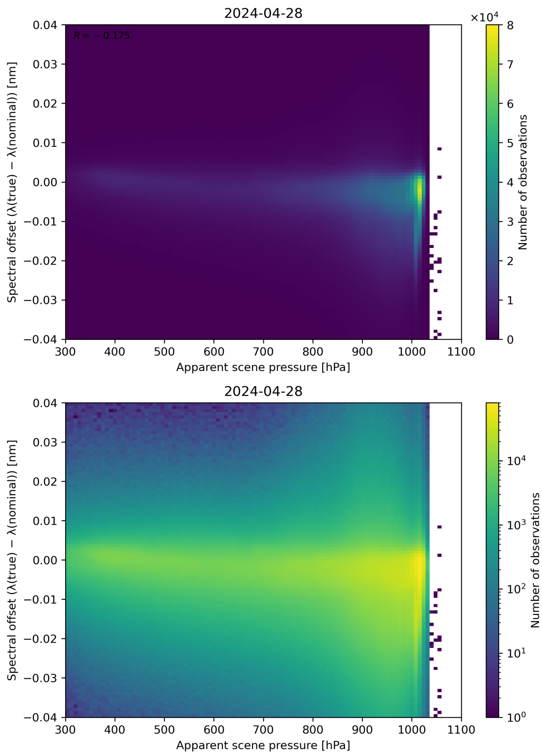
Figure 67: Scatter density plot of “Apparent scene pressure” against “Spectral offset ( \lambda(\text{true}) - \lambda(\text{nominal}) )” for 2024-04-27 to 2024-04-29.
