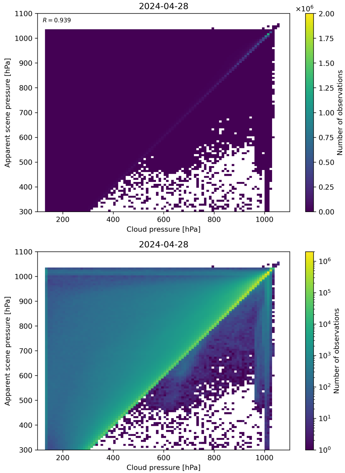
Figure 77: Scatter density plot of “Cloud pressure” against “Apparent scene pressure” for 2024-04-27 to 2024-04-29.
