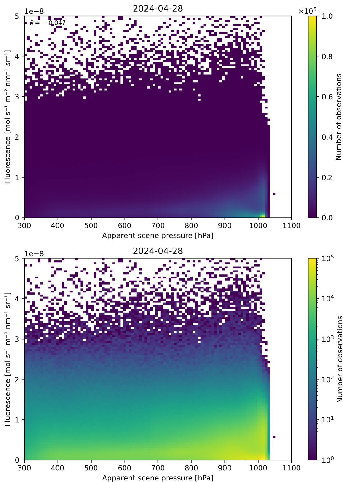
Figure 64: Scatter density plot of “Apparent scene pressure” against “Fluorescence” for 2024-04-27 to 2024-04-29.
