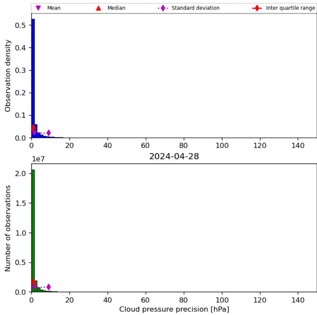
Figure 31: Histogram of “Cloud pressure precision” for 2024-04-27 to 2024-04-29
