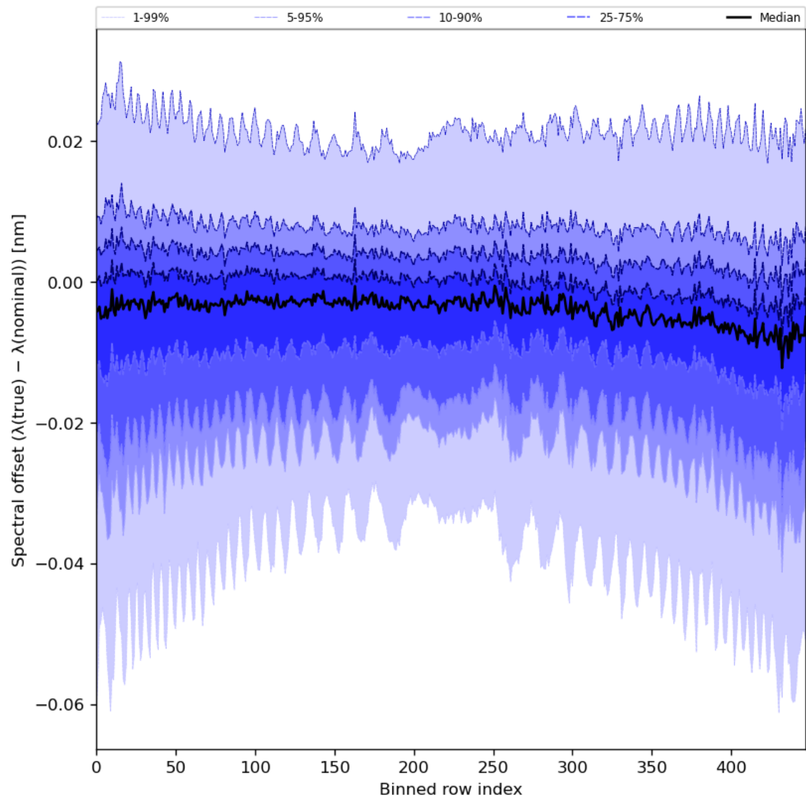
Figure 62: Along track statistics of “Spectral offset ( \lambda(\text{true}) - \lambda(\text{nominal}) )” for 2024-04-27 to 2024-04-29
