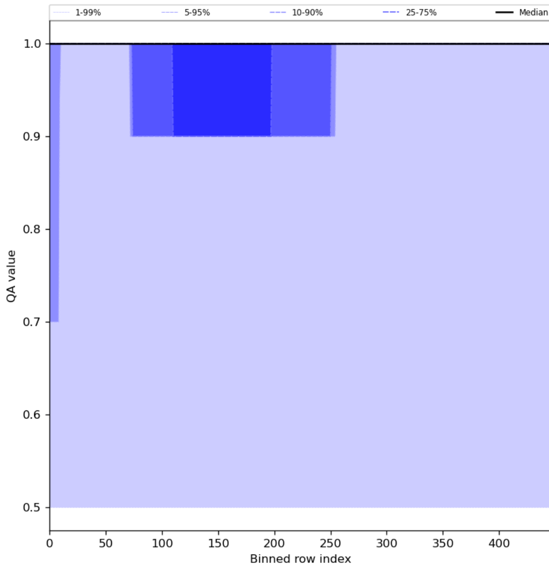
Figure 46: Along track statistics of “QA value” for 2024-04-27 to 2024-04-29
