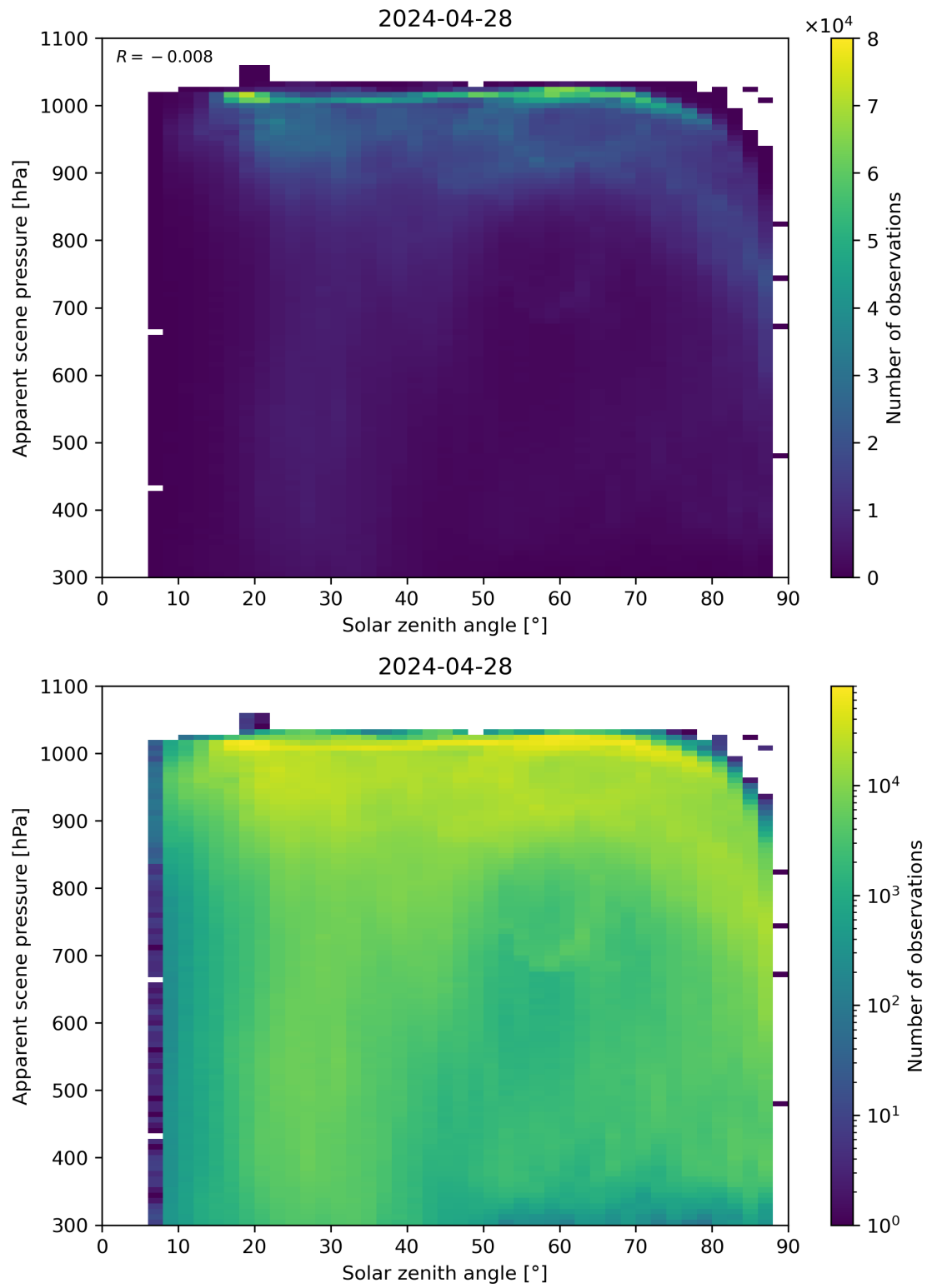
Figure 108: Scatter density plot of “Solar zenith angle” against “Apparent scene pressure” for 2024-04-27 to 2024-04-29.
