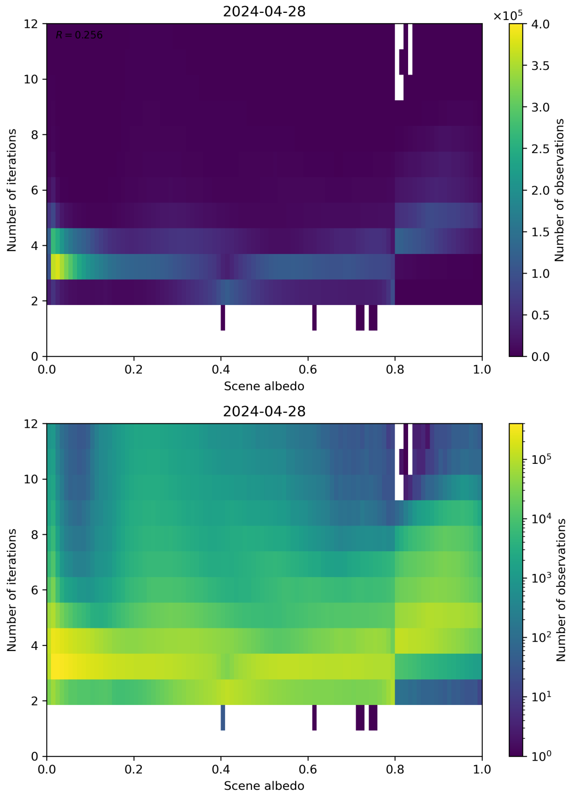
Figure 105: Scatter density plot of “Scene albedo” against “Number of iterations” for 2024-04-27 to 2024-04-29.
