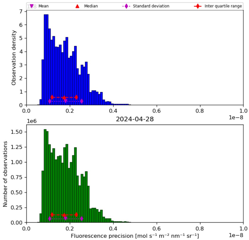
Figure 41: Histogram of “Fluorescence precision” for 2024-04-27 to 2024-04-29
