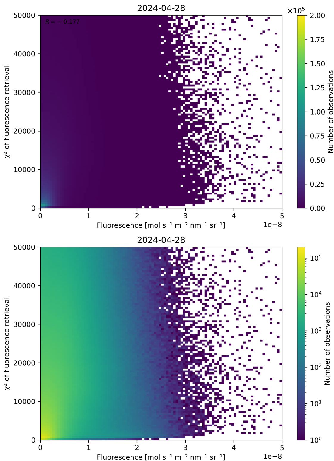
Figure 85: Scatter density plot of “Fluorescence” against “ \chi^2 of fluorescence retrieval” for 2024-04-27 to 2024-04-29.
