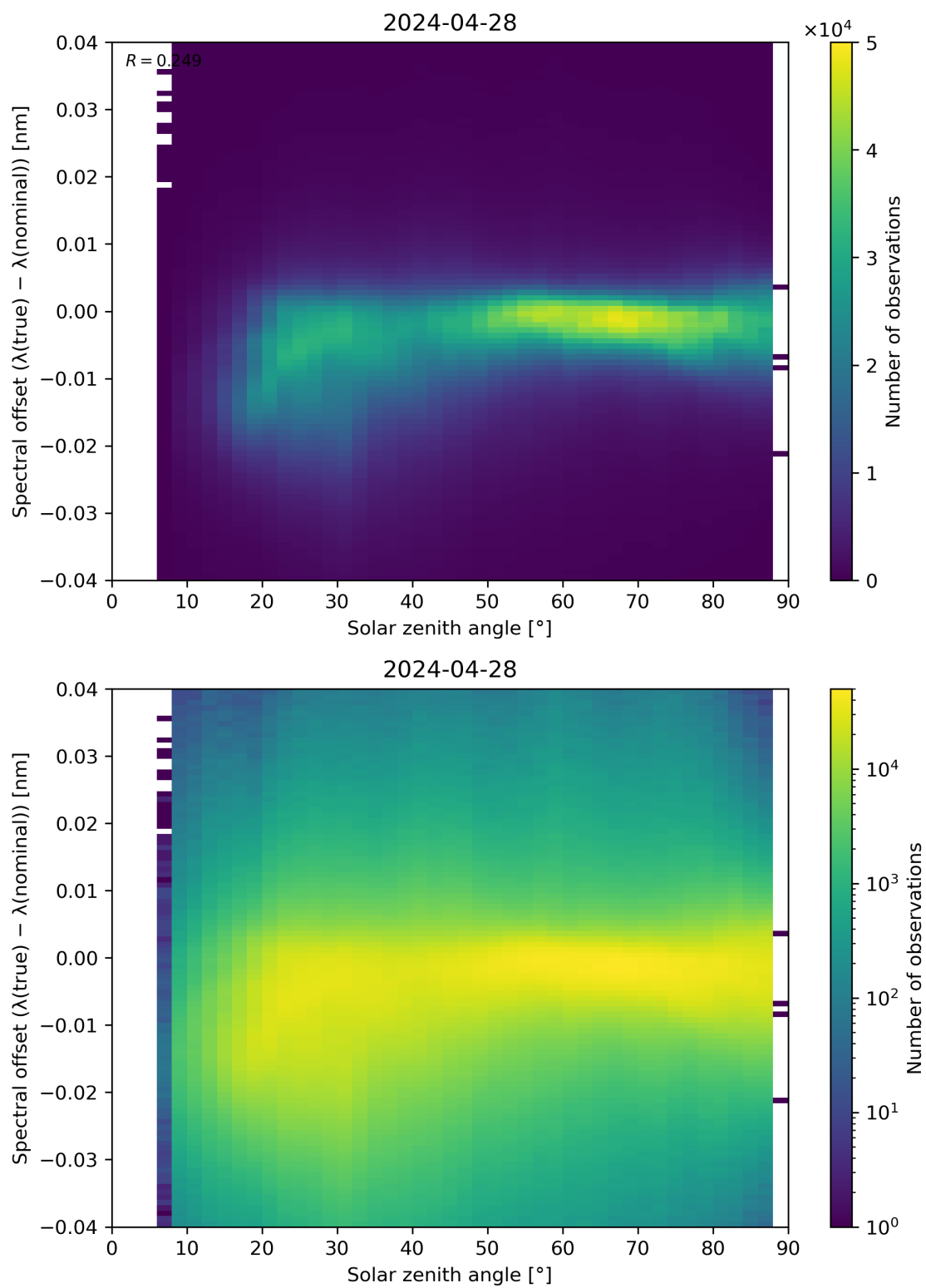
Figure 117: Scatter density plot of “Solar zenith angle” against “Spectral offset ( \lambda(\text{true}) - \lambda(\text{nominal}) )” for 2024-04-27 to 2024-04-29.
