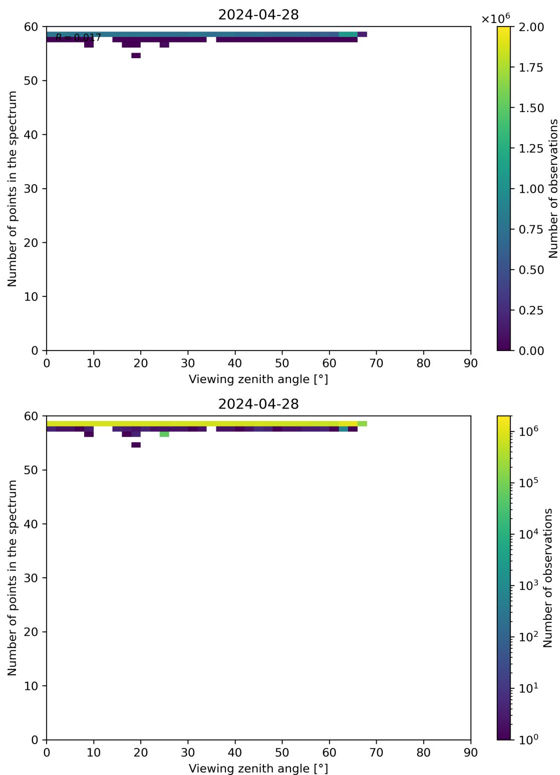
Figure 125: Scatter density plot of “Viewing zenith angle” against “Number of points in the spectrum” for 2024-04-27 to 2024-04-29.
