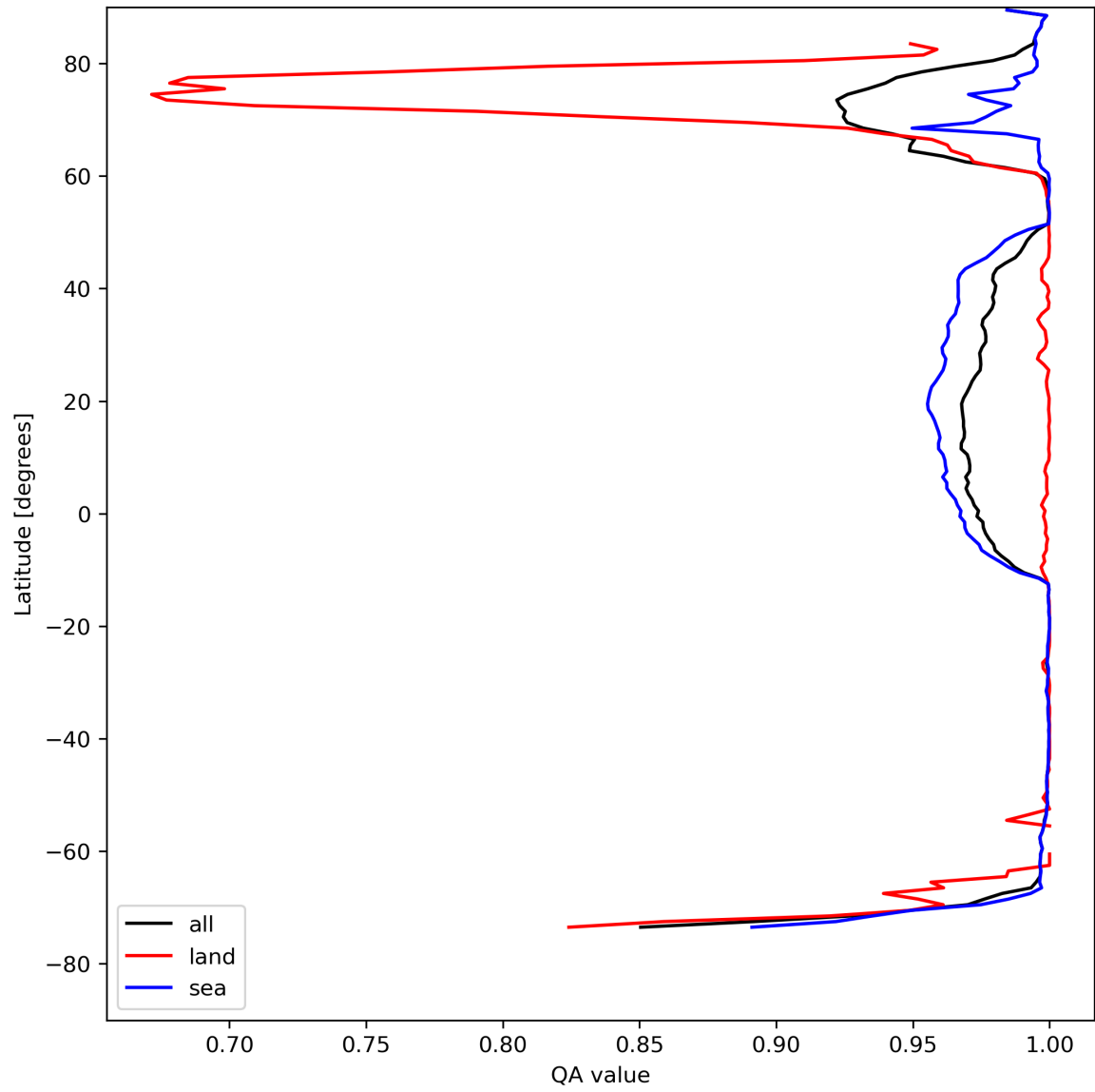
Figure 12: Zonal average of “QA value” for 2024-04-27 to 2024-04-29.
