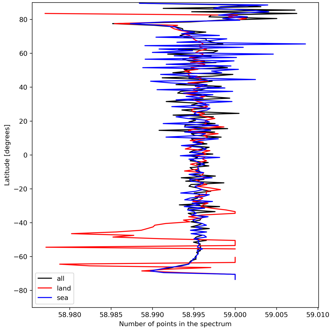
Figure 27: Zonal average of “Number of points in the spectrum” for 2024-04-27 to 2024-04-29.
