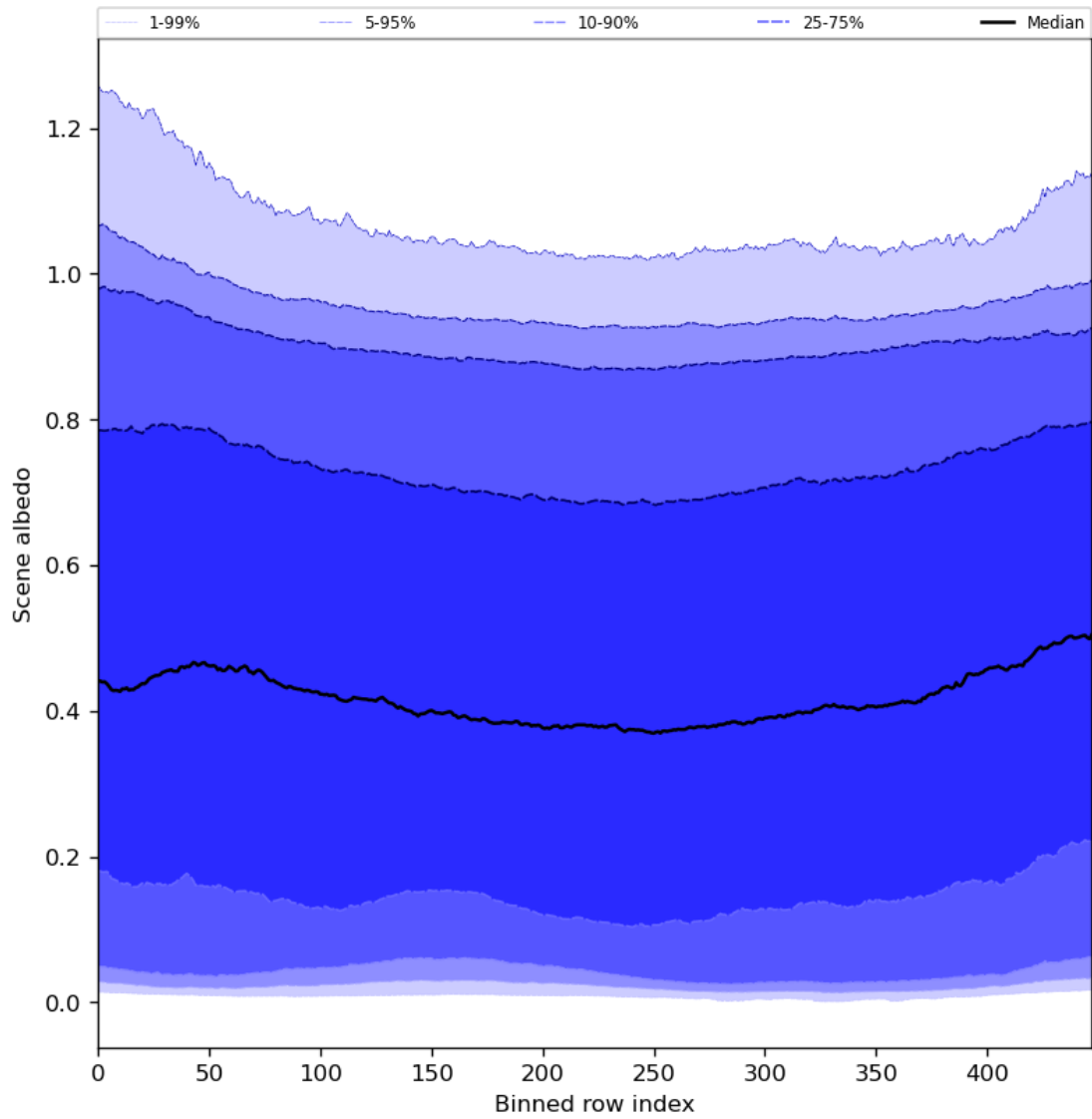
Figure 51: Along track statistics of “Scene albedo” for 2024-04-27 to 2024-04-29
