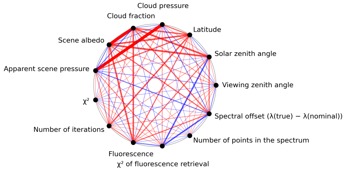
Figure 1: Map of correlation graph for 2024-04-27 to 2024-04-29.
