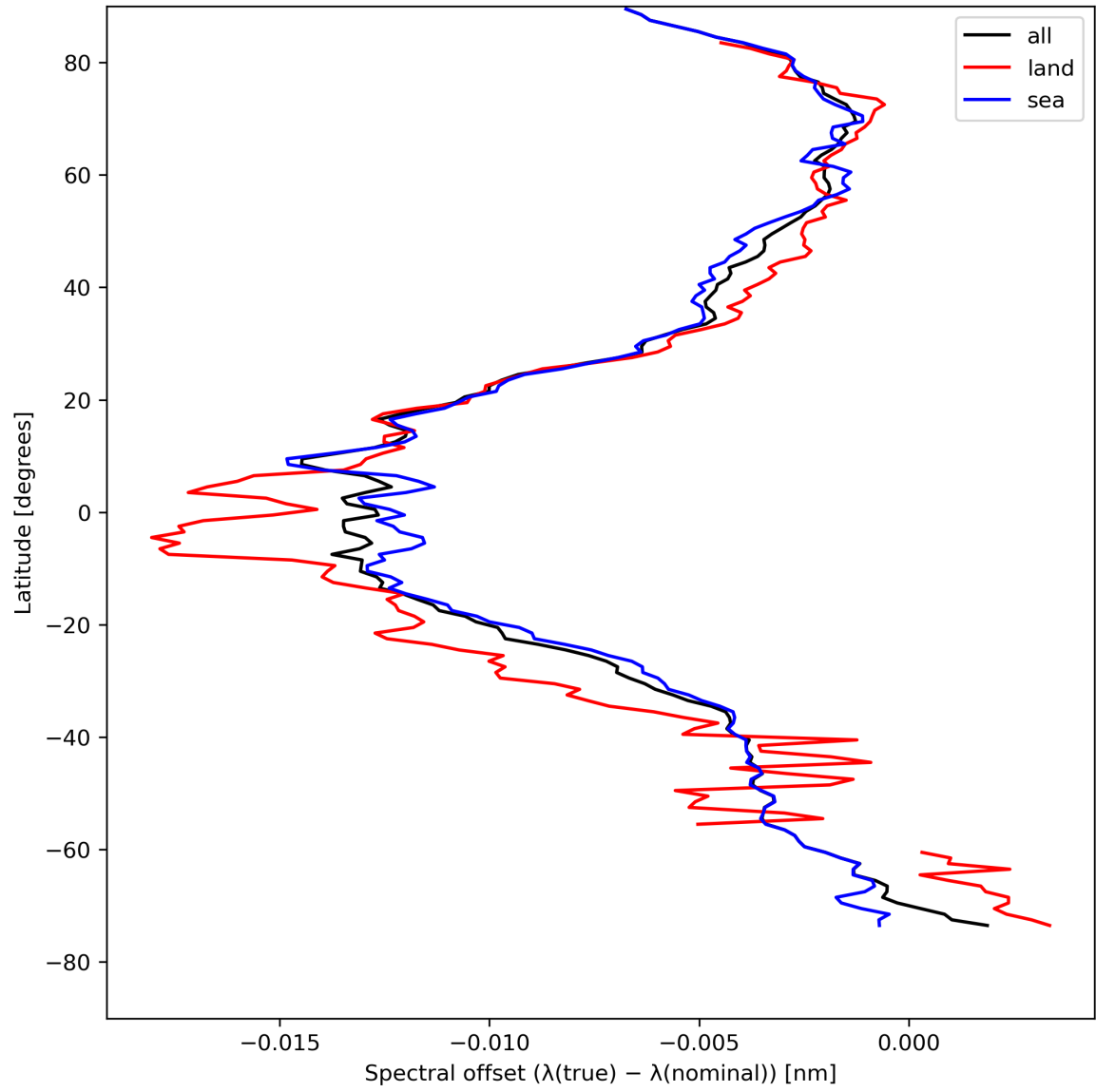
Figure 28: Zonal average of “Spectral offset ( \lambda(\text{true}) - \lambda(\text{nominal}) )” for 2024-04-27 to 2024-04-29.
