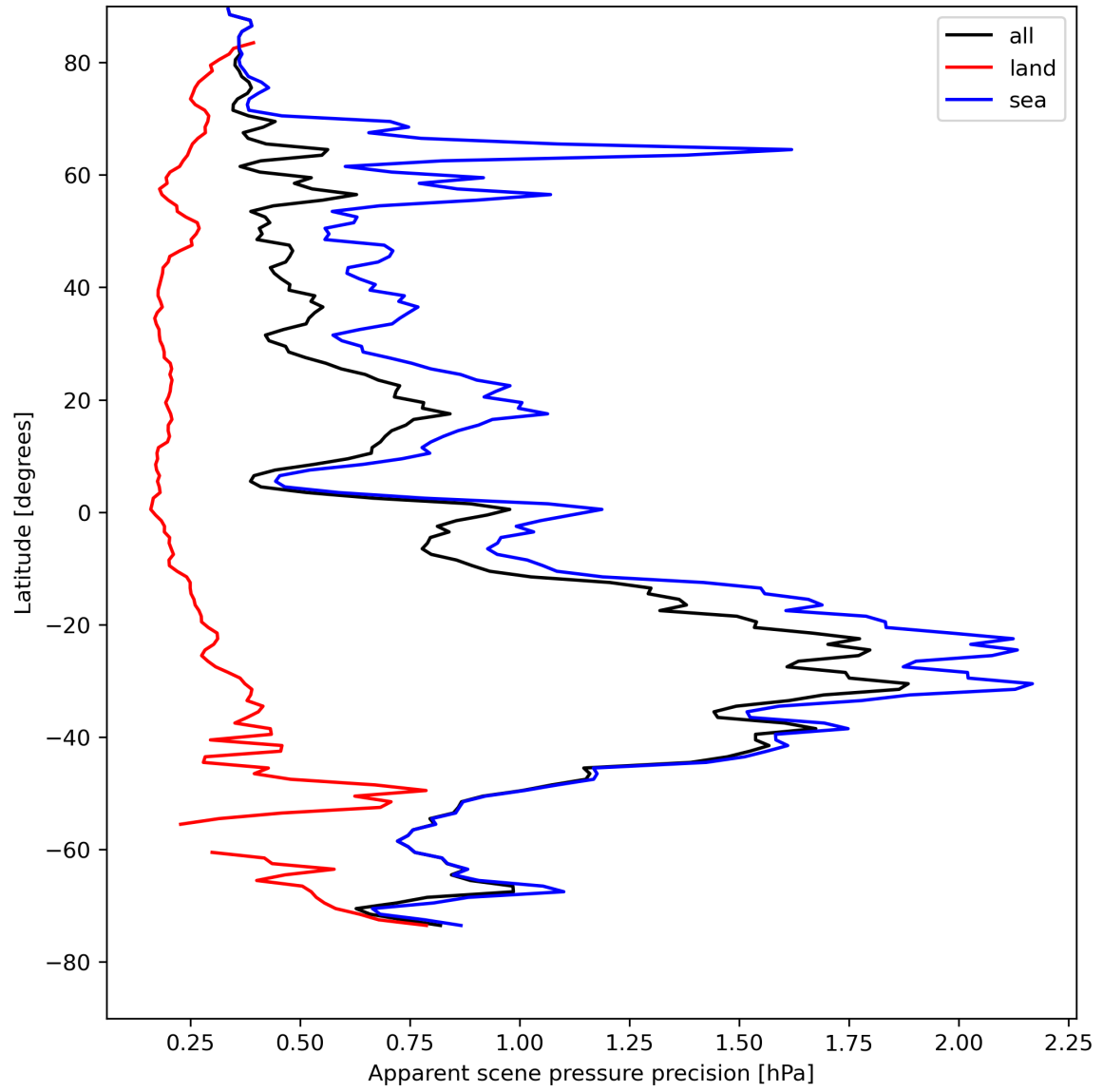
Figure 20: Zonal average of “Apparent scene pressure precision” for 2024-04-27 to 2024-04-29.
