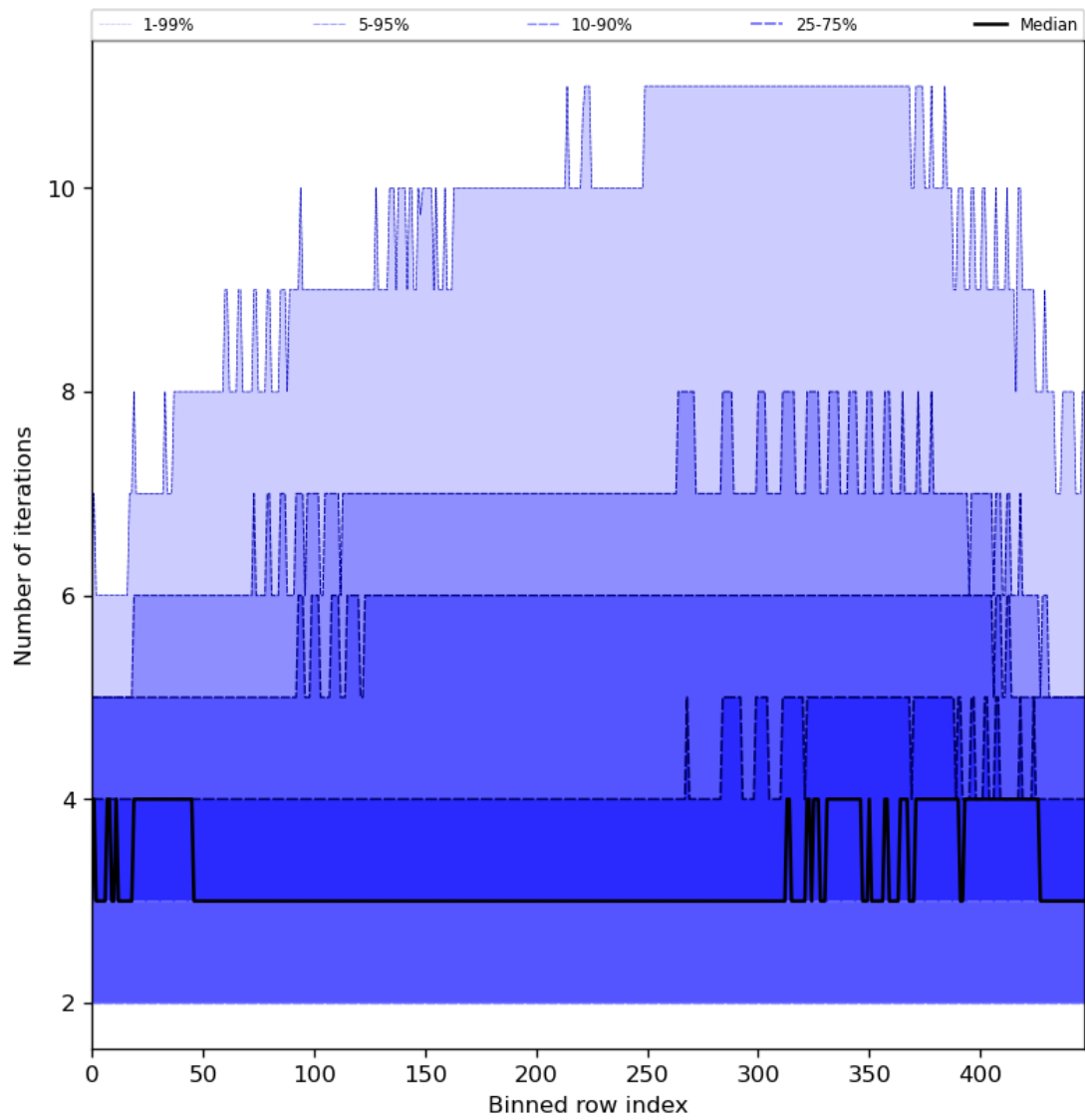
Figure 56: Along track statistics of “Number of iterations” for 2024-04-27 to 2024-04-29
