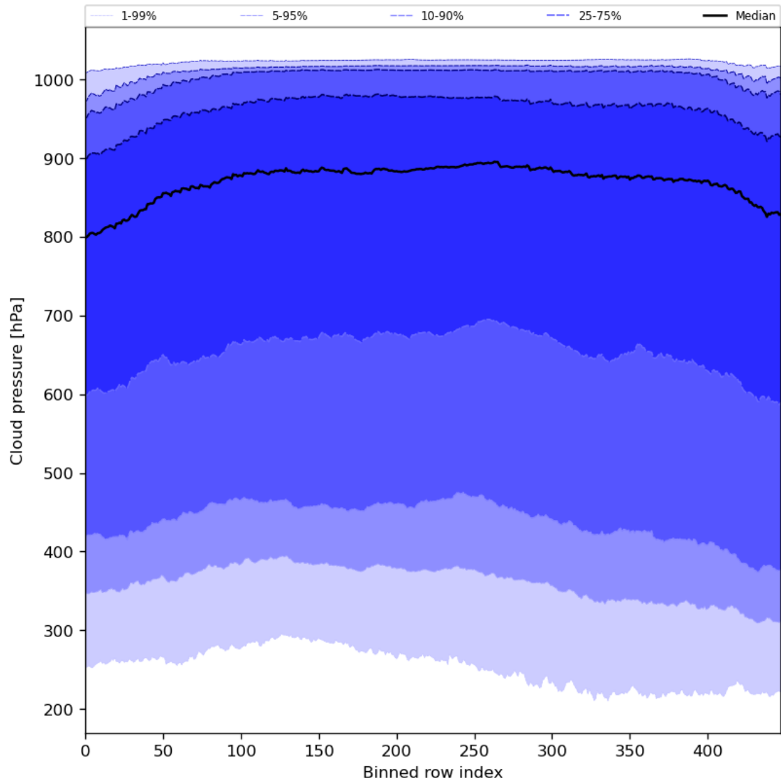
Figure 47: Along track statistics of “Cloud pressure” for 2024-04-27 to 2024-04-29
