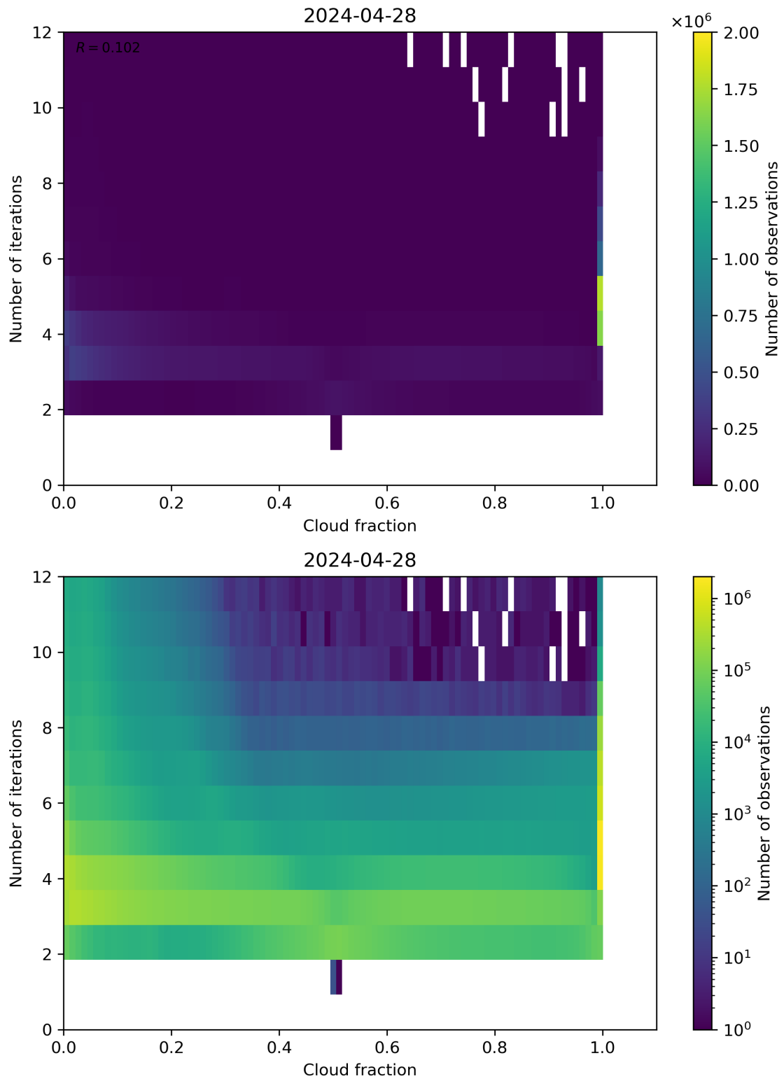
Figure 73: Scatter density plot of “Cloud fraction” against “Number of iterations” for 2024-04-27 to 2024-04-29.
