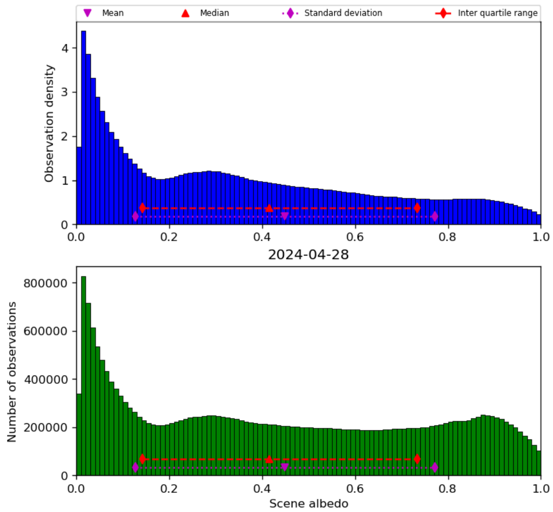
Figure 34: Histogram of “Scene albedo” for 2024-04-27 to 2024-04-29
