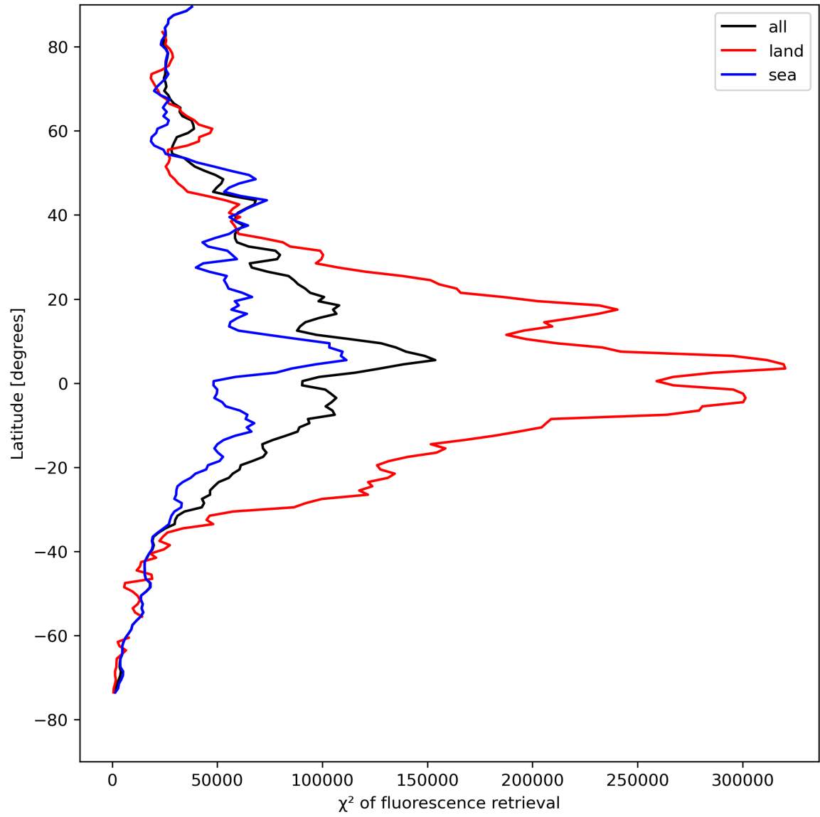
Figure 25: Zonal average of “ \chi^2 of fluorescence retrieval” for 2024-04-27 to 2024-04-29.
