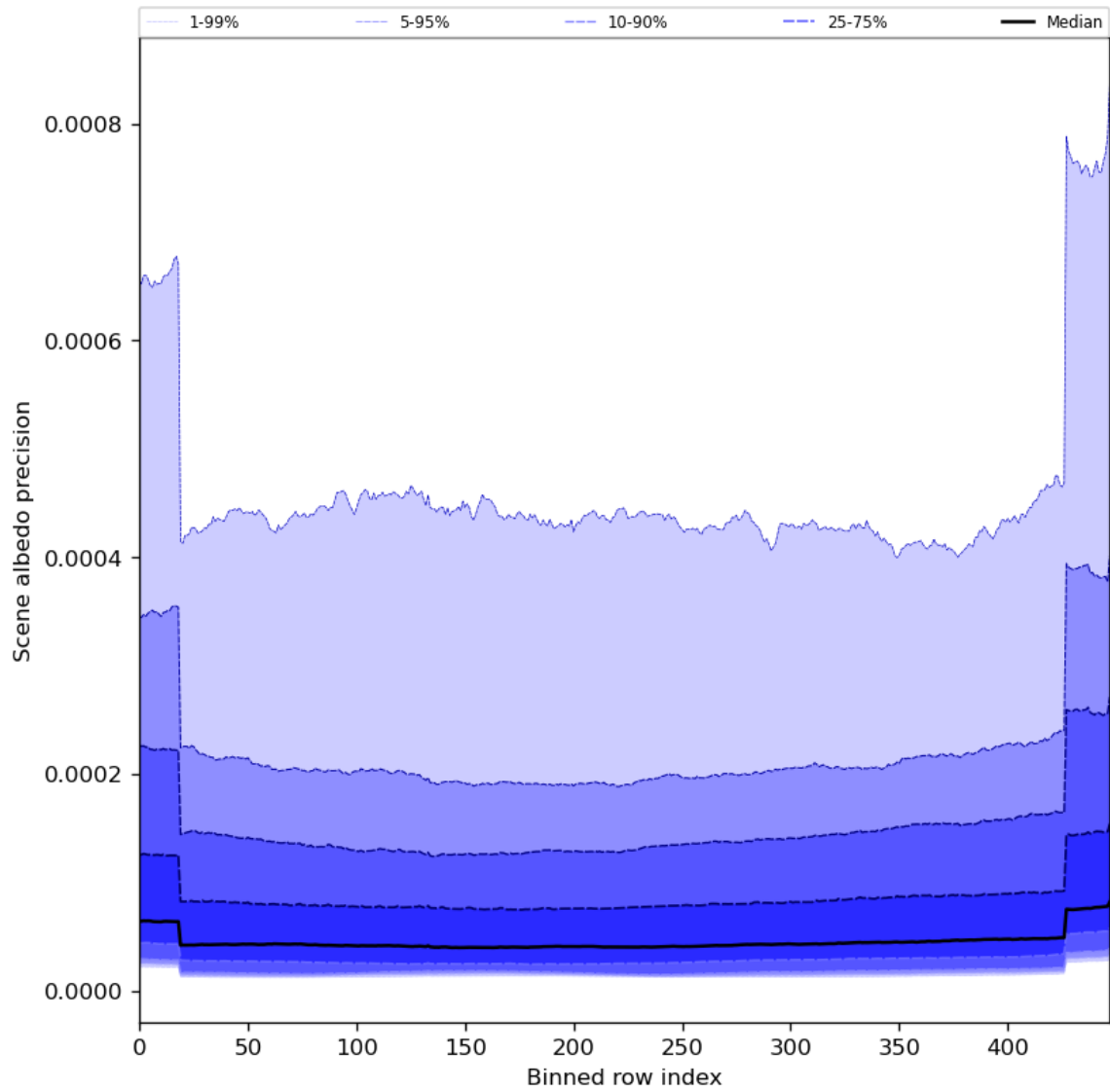
Figure 52: Along track statistics of “Scene albedo precision” for 2024-04-27 to 2024-04-29
