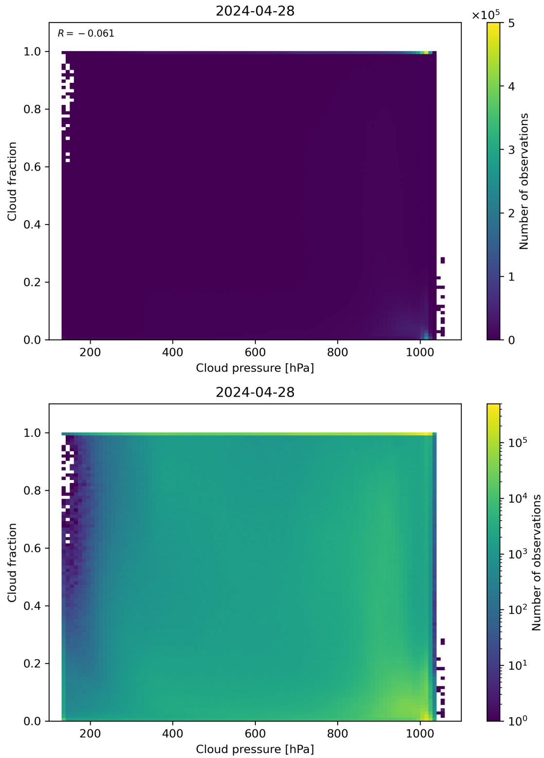
Figure 79: Scatter density plot of “Cloud pressure” against “Cloud fraction” for 2024-04-27 to 2024-04-29.
