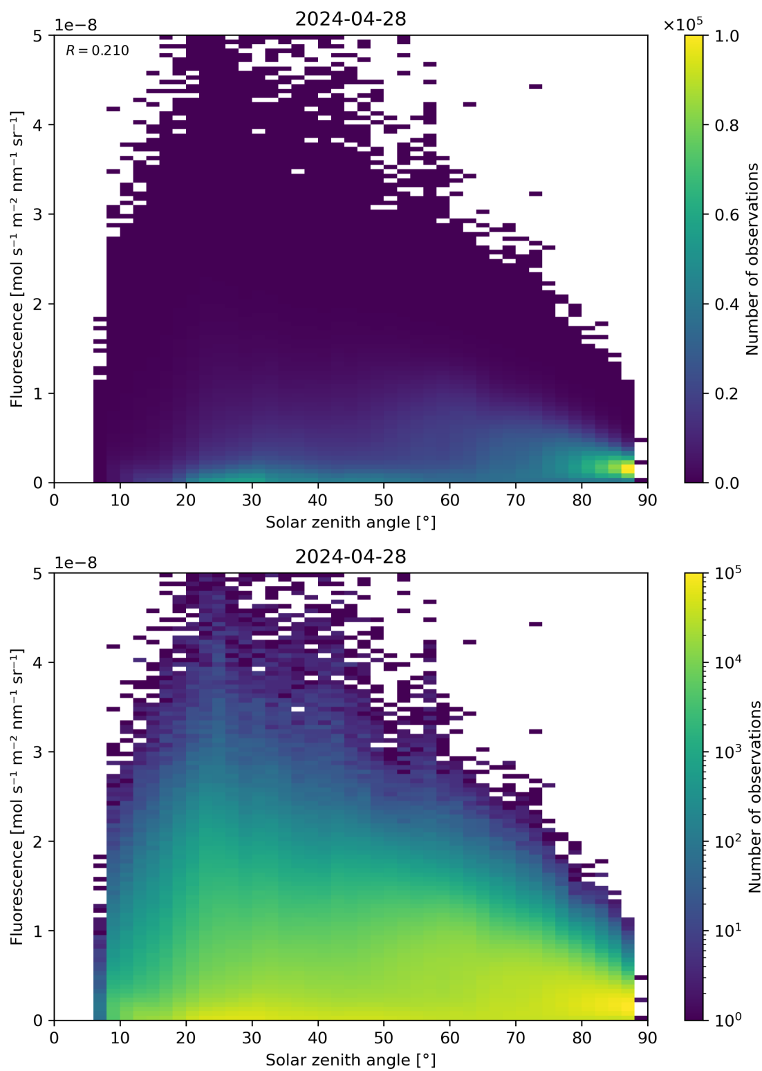
Figure 112: Scatter density plot of “Solar zenith angle” against “Fluorescence” for 2024-04-27 to 2024-04-29.
