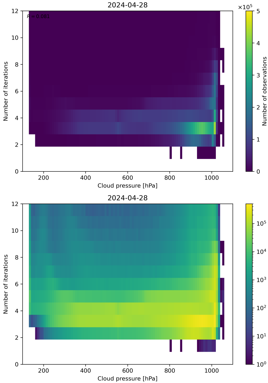
Figure 81: Scatter density plot of “Cloud pressure” against “Number of iterations” for 2024-04-27 to 2024-04-29.
