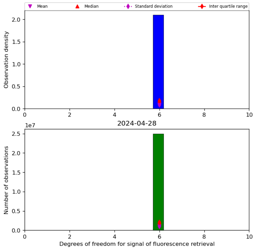
Figure 43: Histogram of “Degrees of freedom for signal of fluorescence retrieval” for 2024-04-27 to 2024-04-29
