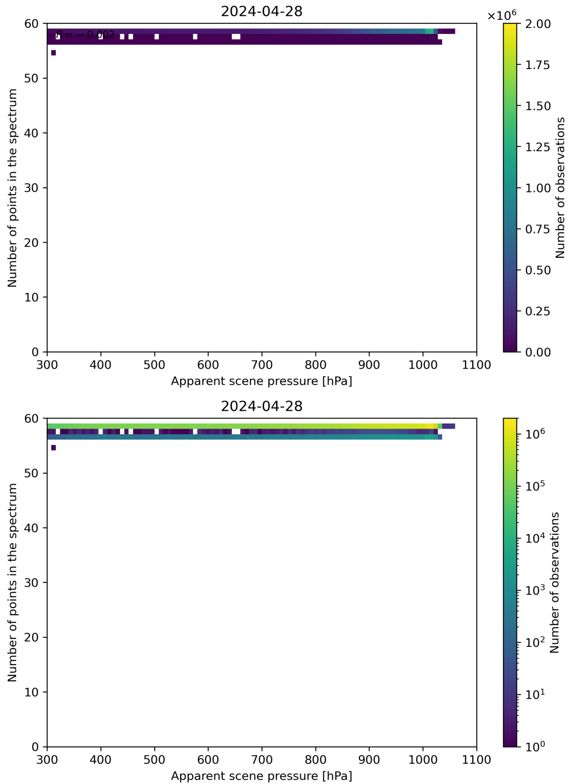
Figure 66: Scatter density plot of “Apparent scene pressure” against “Number of points in the spectrum” for 2024-04-27 to 2024-04-29.
