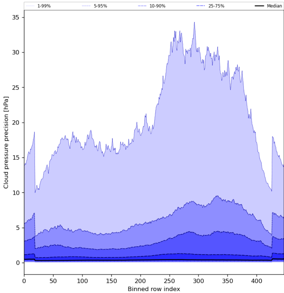
Figure 48: Along track statistics of “Cloud pressure precision” for 2024-04-27 to 2024-04-29
