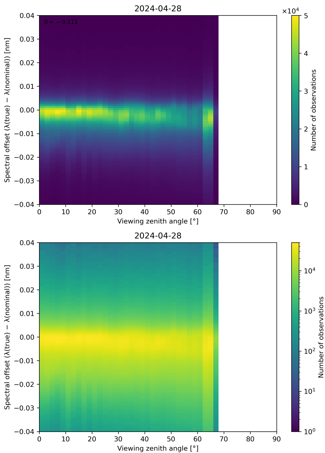
Figure 128: Scatter density plot of “Viewing zenith angle” against “Spectral offset ( \lambda(\text{true}) - \lambda(\text{nominal}) )” for 2024-04-27 to 2024-04-29.
