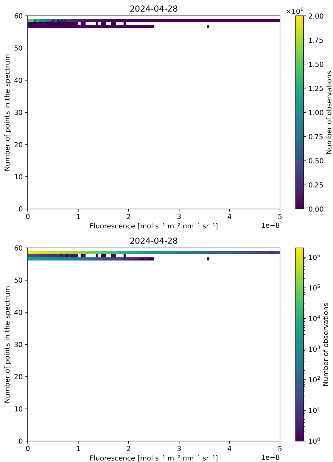
Figure 86: Scatter density plot of “Fluorescence” against “Number of points in the spectrum” for 2024-04-27 to 2024-04-29.
