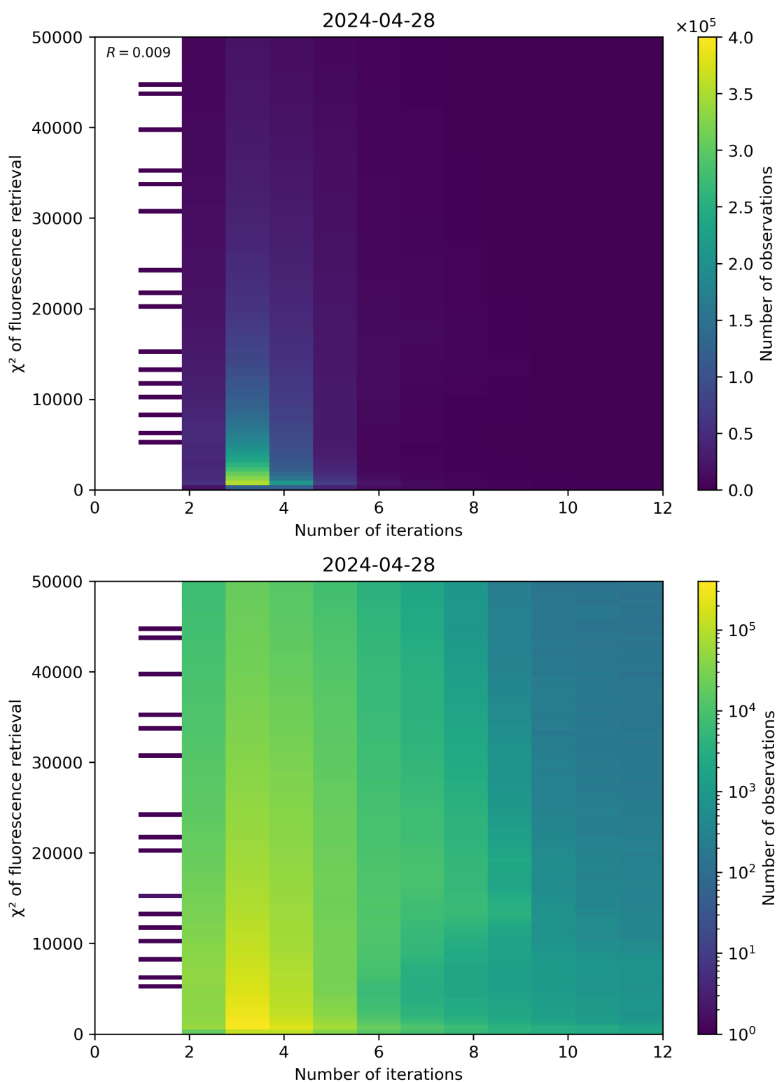
Figure 97: Scatter density plot of “Number of iterations” against “ \chi^2 of fluorescence retrieval” for 2024-04-27 to 2024-04-29.
