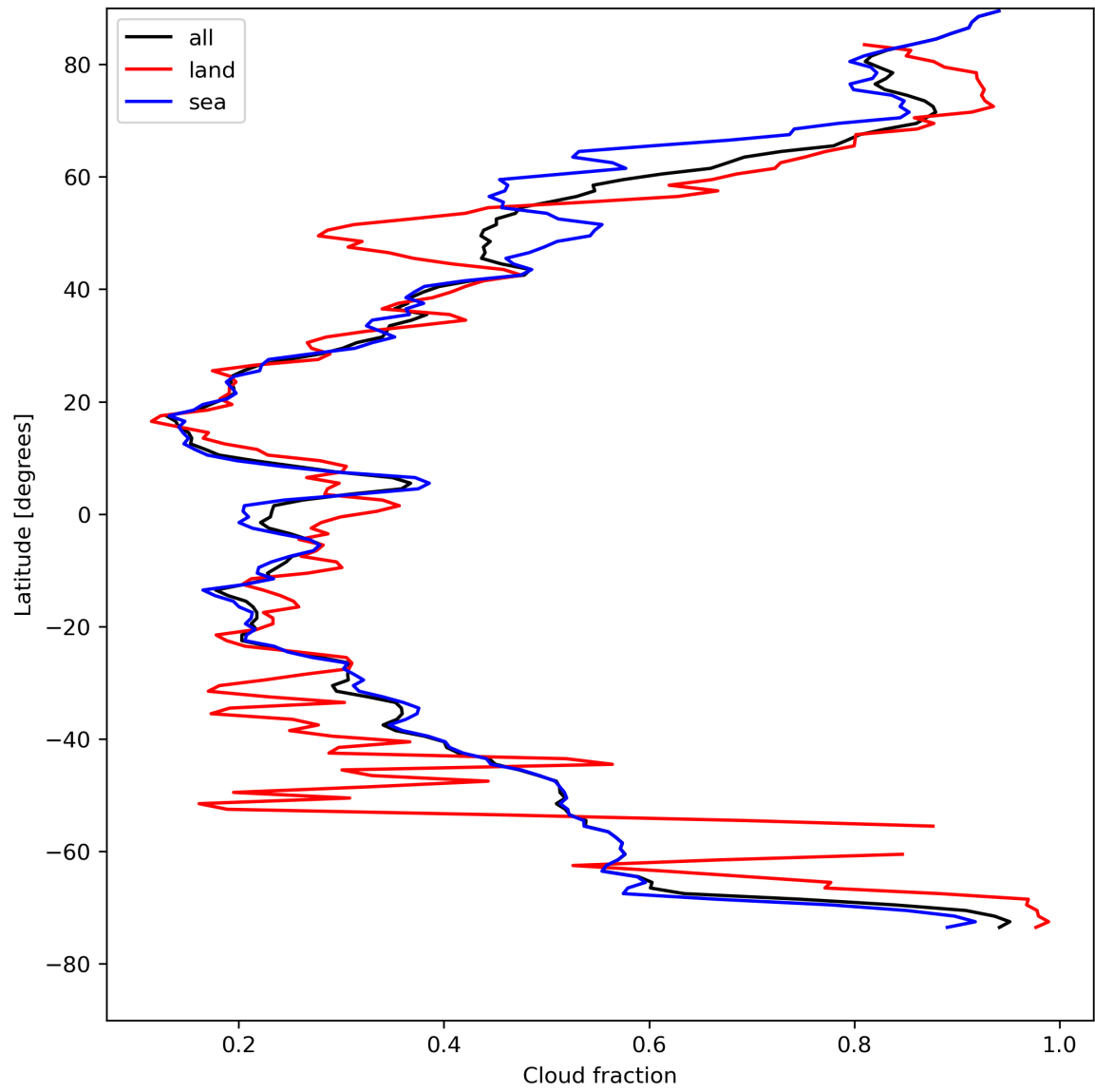
Figure 15: Zonal average of “Cloud fraction” for 2024-04-27 to 2024-04-29.
