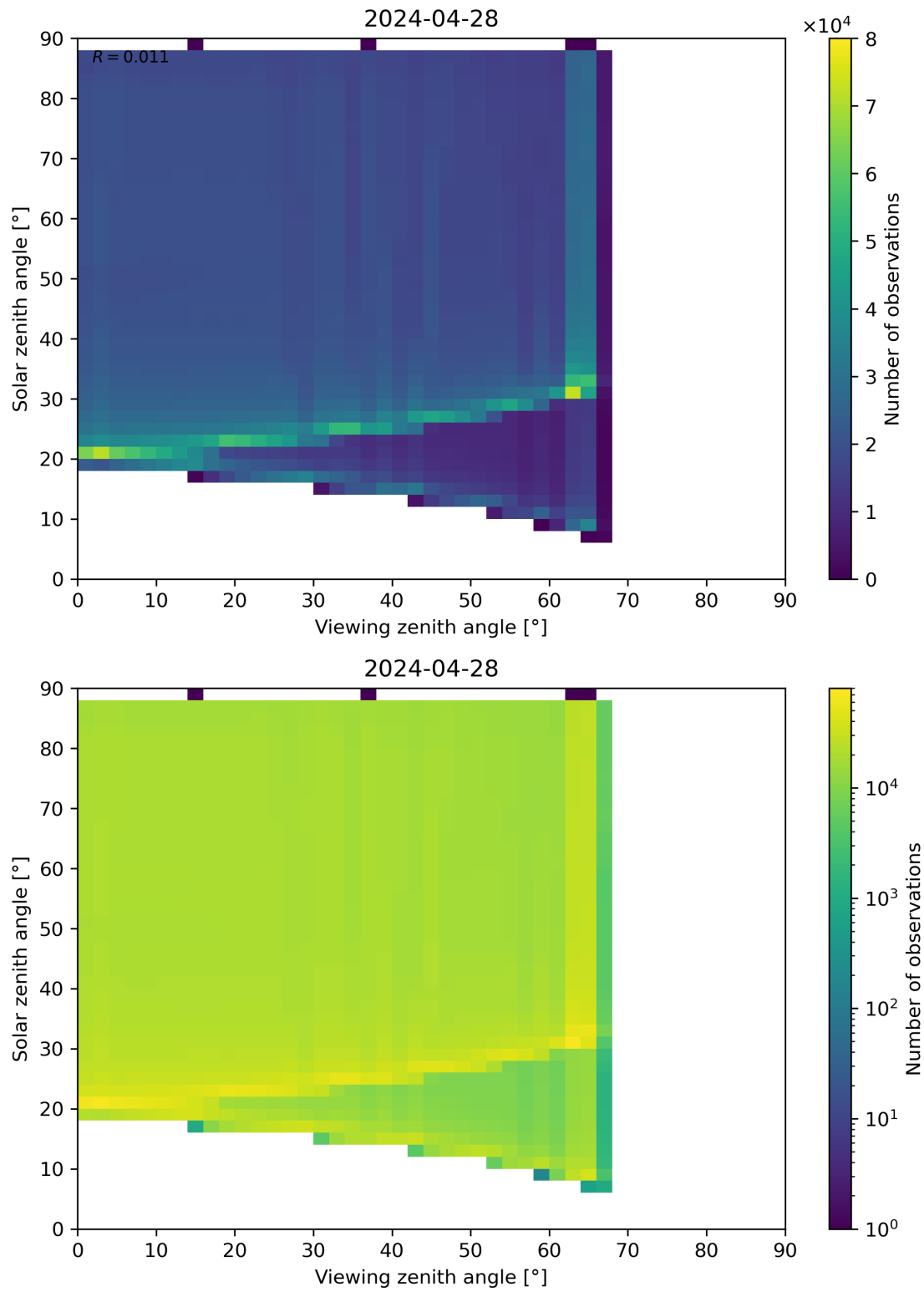
Figure 127: Scatter density plot of “Viewing zenith angle” against “Solar zenith angle” for 2024-04-27 to 2024-04-29.
