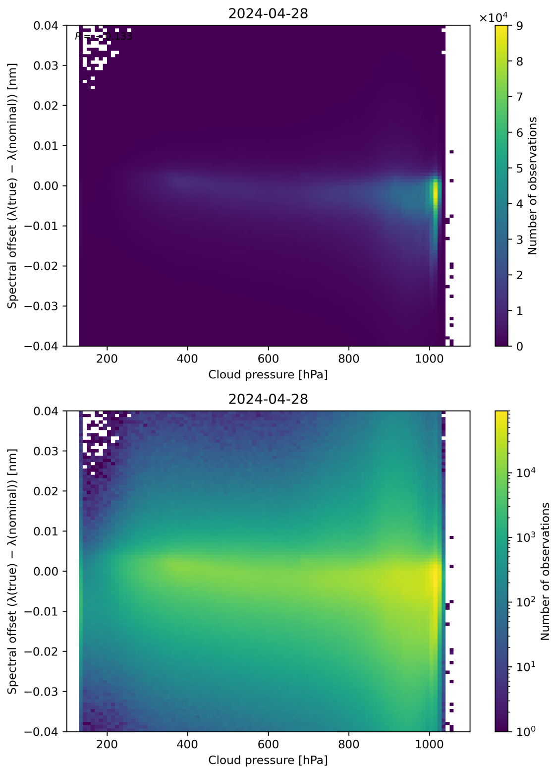
Figure 84: Scatter density plot of “Cloud pressure” against “Spectral offset ( \lambda(\text{true}) - \lambda(\text{nominal}) )” for 2024-04-27 to 2024-04-29.
