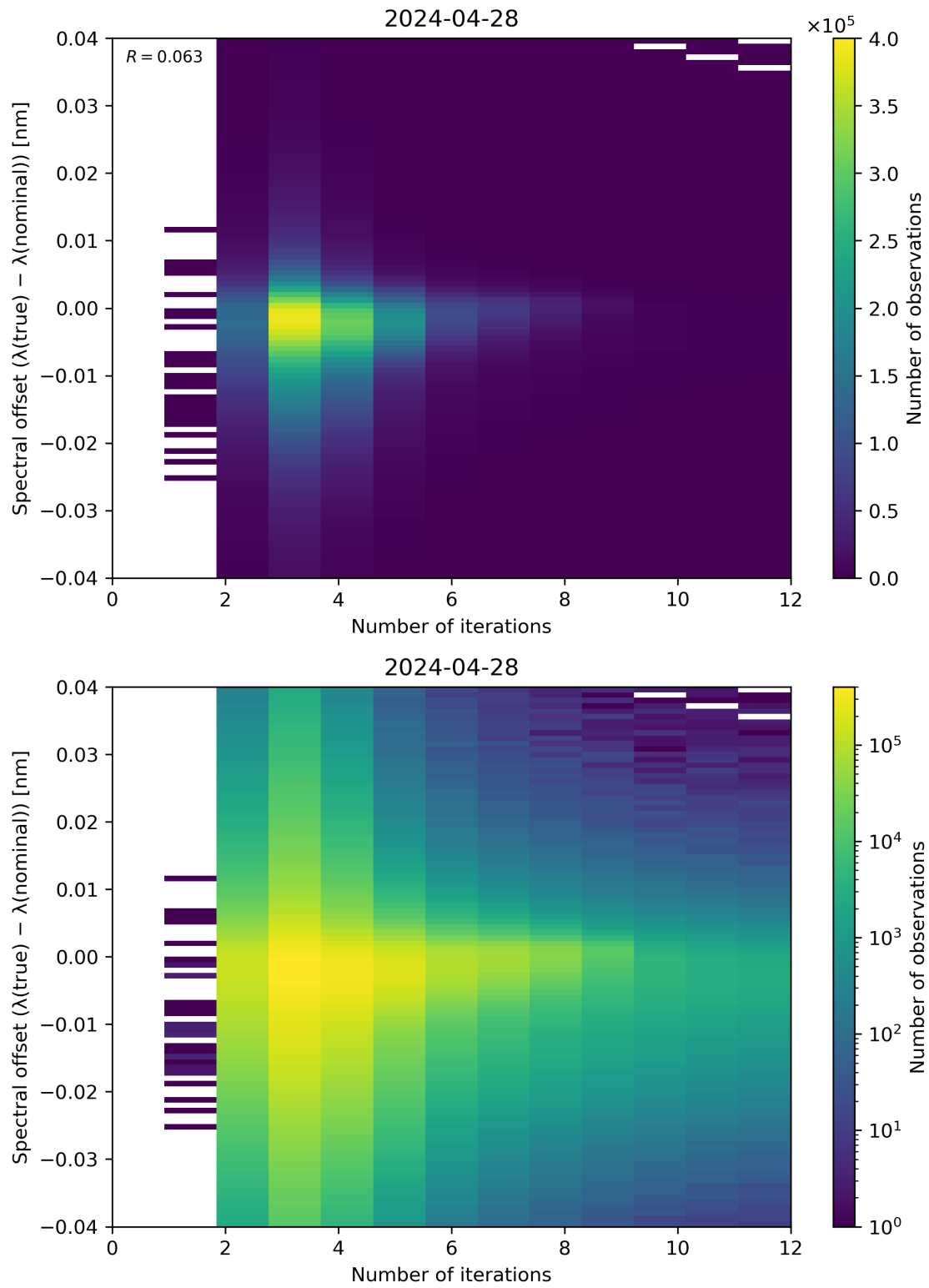
Figure 100: Scatter density plot of “Number of iterations” against “Spectral offset ( \lambda(\text{true}) - \lambda(\text{nominal}) )” for 2024-04-27 to 2024-04-29.
