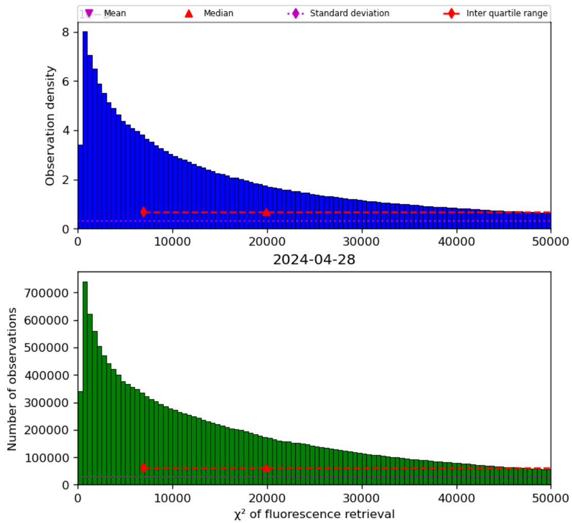
Figure 42: Histogram of “ \chi^2 of fluorescence retrieval” for 2024-04-27 to 2024-04-29
