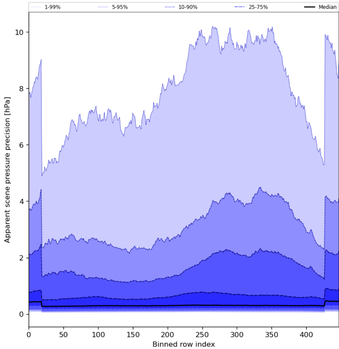
Figure 54: Along track statistics of “Apparent scene pressure precision” for 2024-04-27 to 2024-04-29
