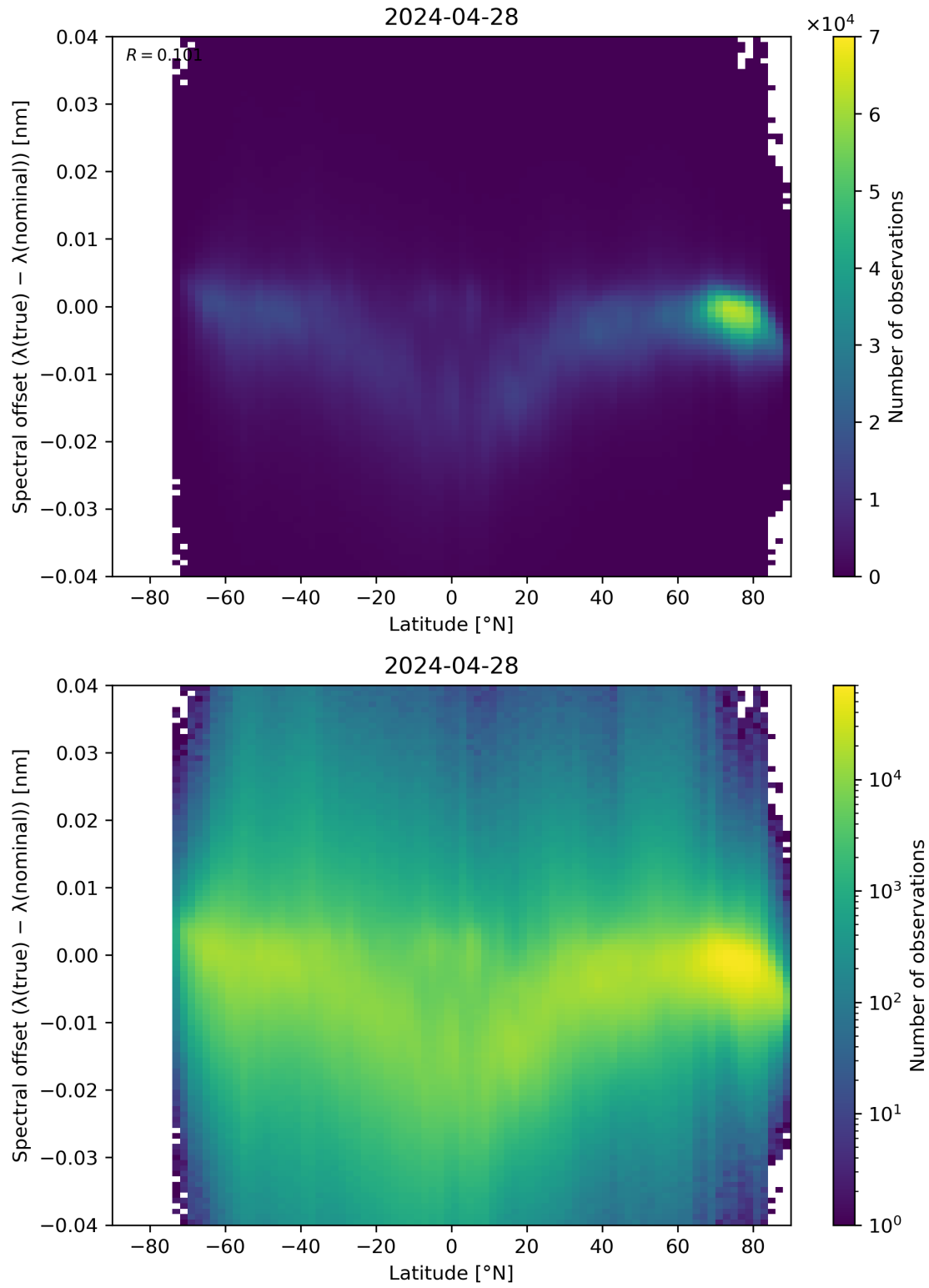
Figure 96: Scatter density plot of “Latitude” against “Spectral offset ( \lambda(\text{true}) - \lambda(\text{nominal}) )” for 2024-04-27 to 2024-04-29.
