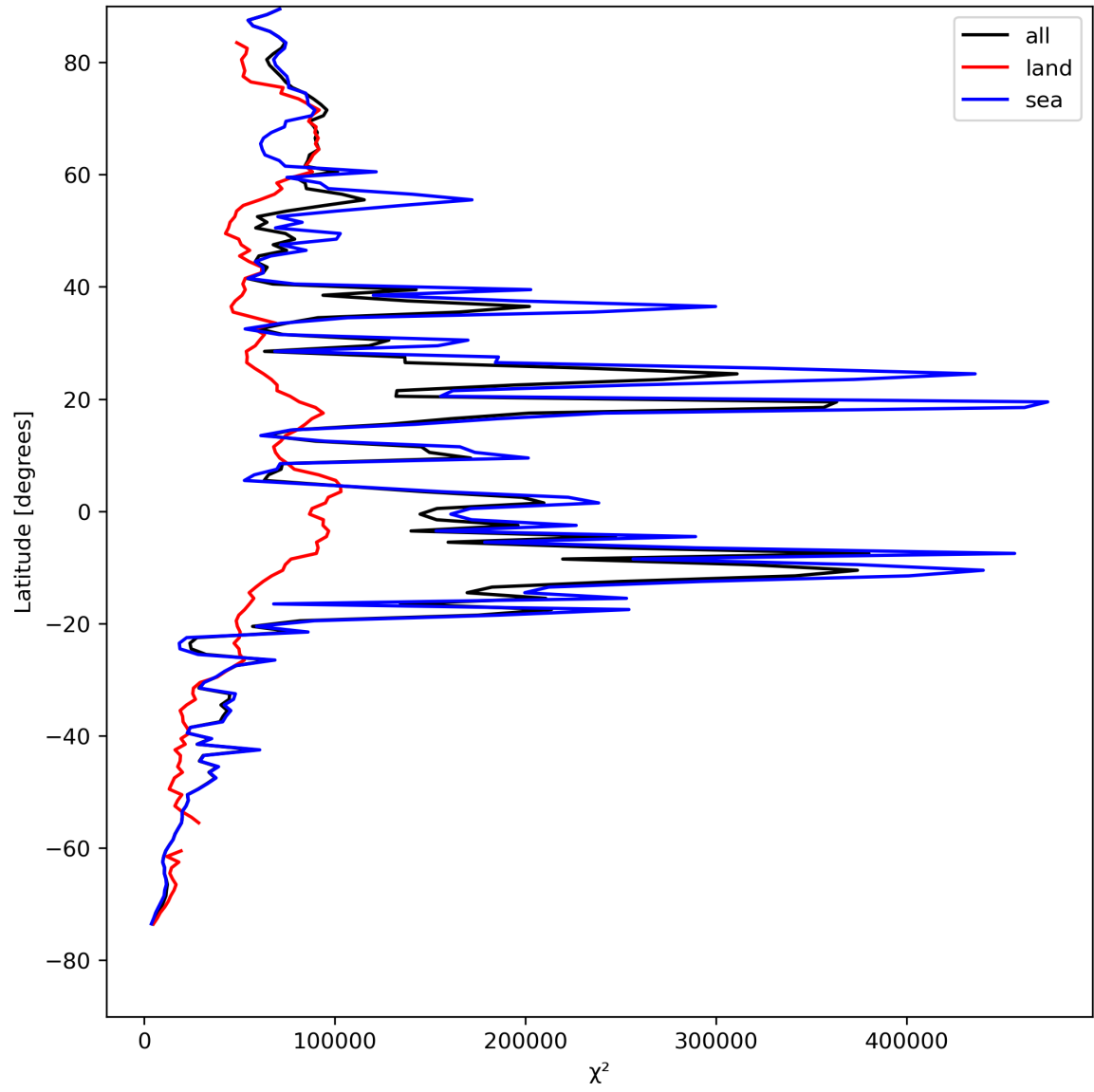
Figure 21: Zonal average of “ \chi^2 ” for 2024-04-27 to 2024-04-29.
