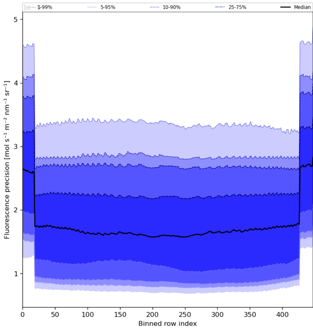
Figure 58: Along track statistics of “Fluorescence precision” for 2024-04-27 to 2024-04-29
