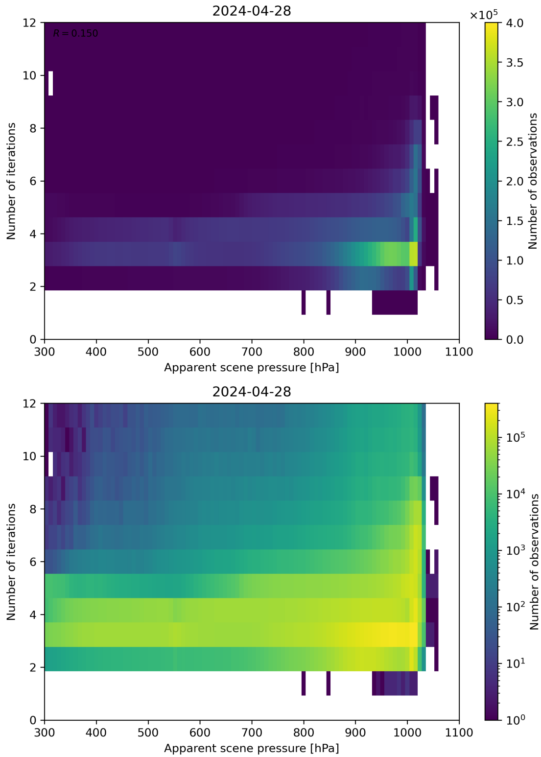
Figure 65: Scatter density plot of “Apparent scene pressure” against “Number of iterations” for 2024-04-27 to 2024-04-29.
