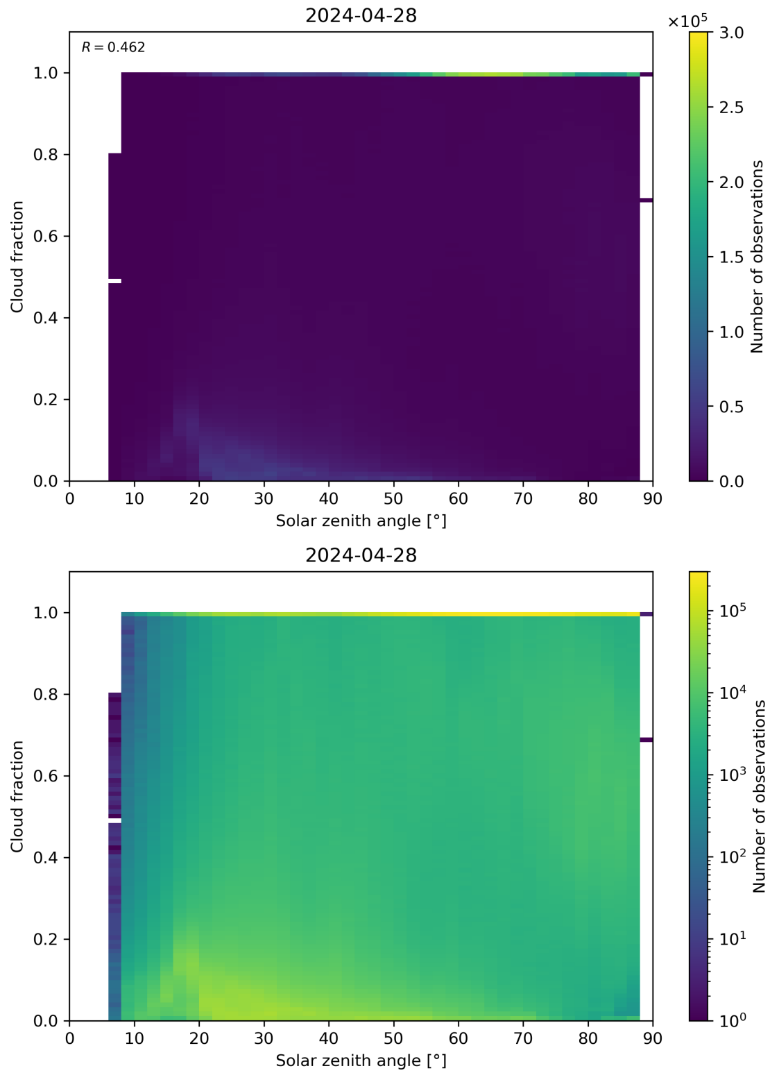
Figure 110: Scatter density plot of “Solar zenith angle” against “Cloud fraction” for 2024-04-27 to 2024-04-29.
