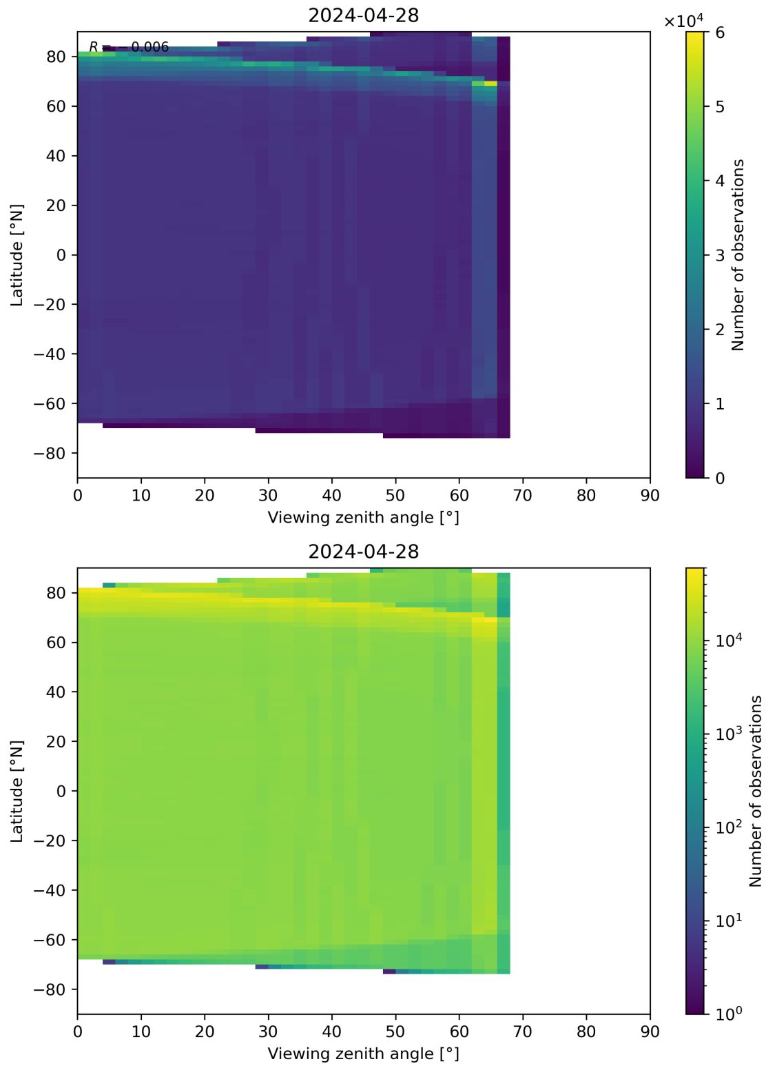
Figure 123: Scatter density plot of “Viewing zenith angle” against “Latitude” for 2024-04-27 to 2024-04-29.
