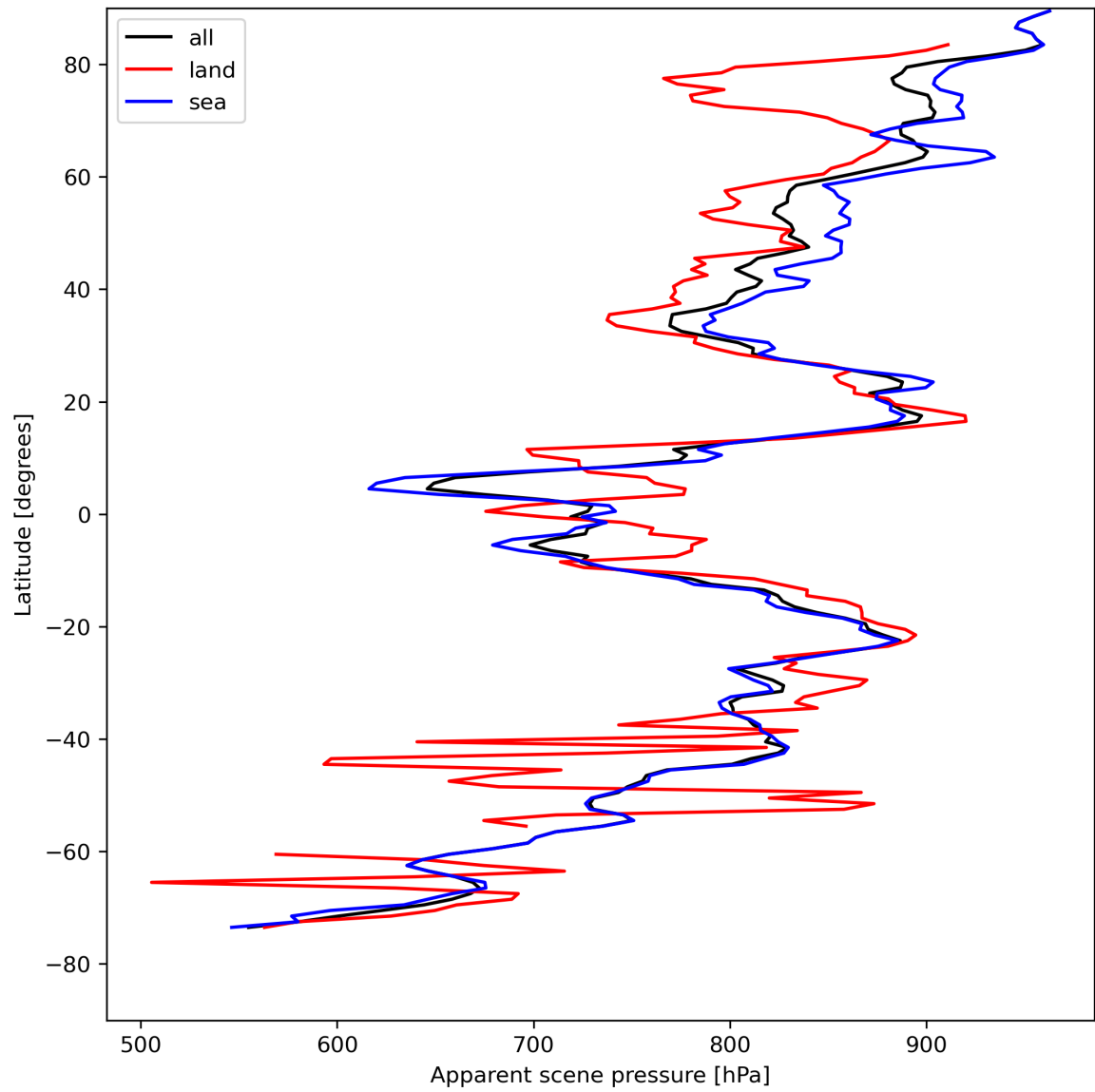
Figure 19: Zonal average of “Apparent scene pressure” for 2024-04-27 to 2024-04-29.
