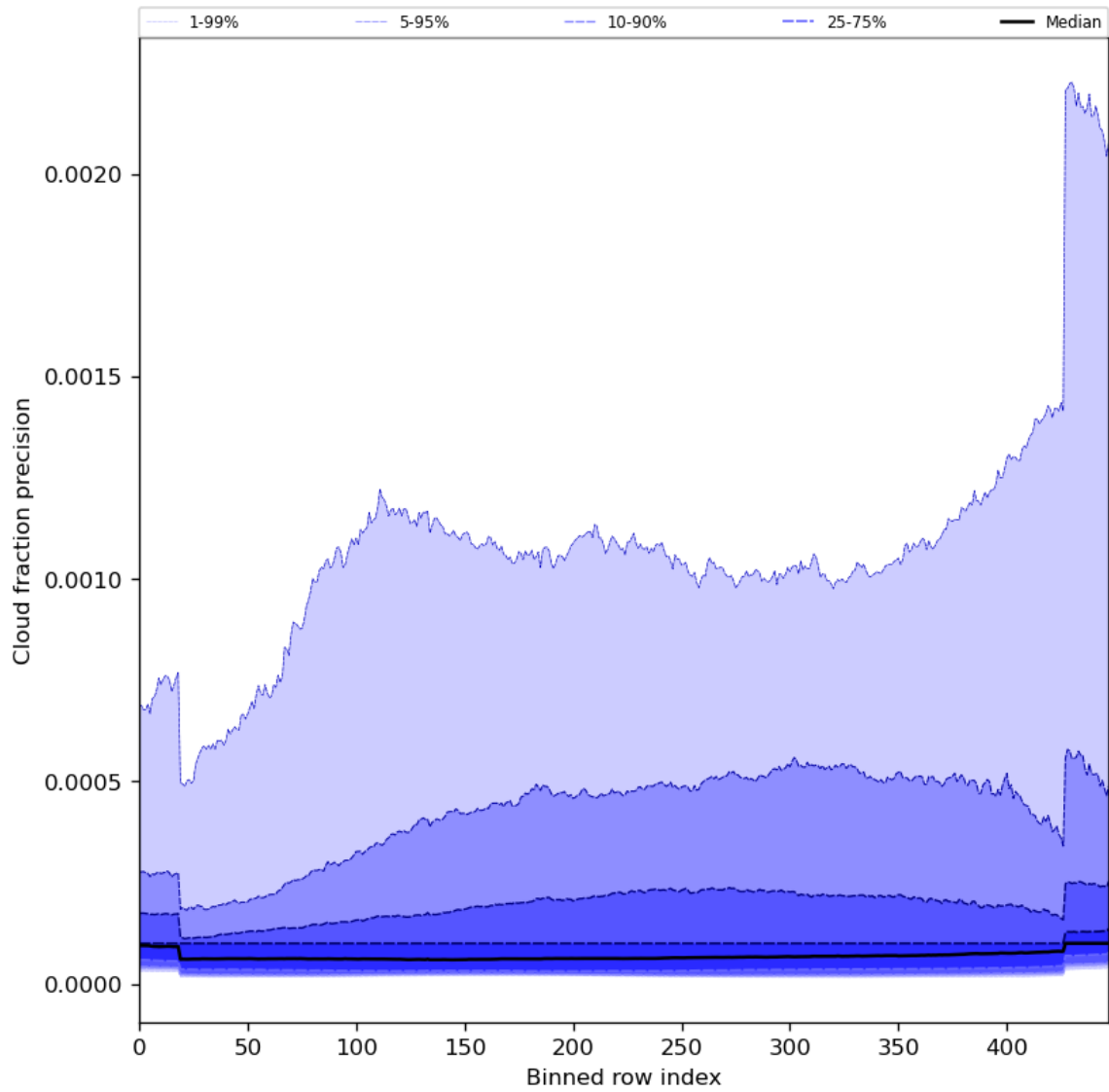
Figure 50: Along track statistics of “Cloud fraction precision” for 2024-04-27 to 2024-04-29
