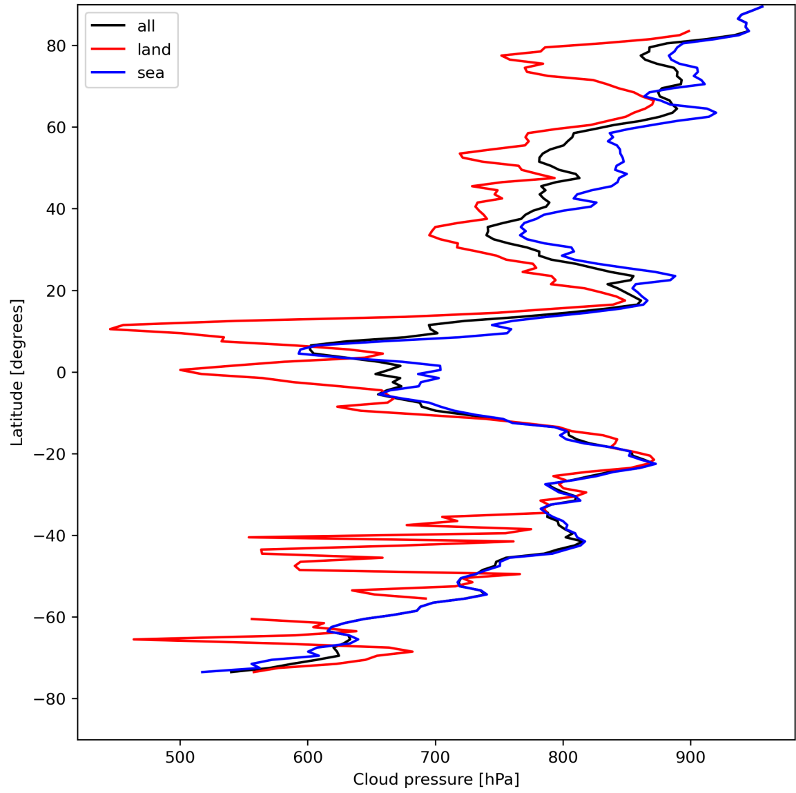
Figure 13: Zonal average of “Cloud pressure” for 2024-04-27 to 2024-04-29.
