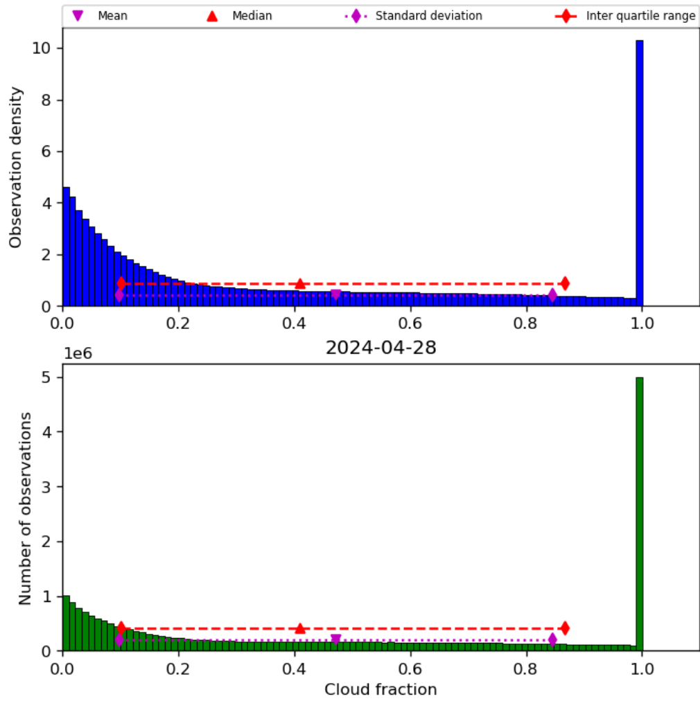
Figure 32: Histogram of “Cloud fraction” for 2024-04-27 to 2024-04-29
