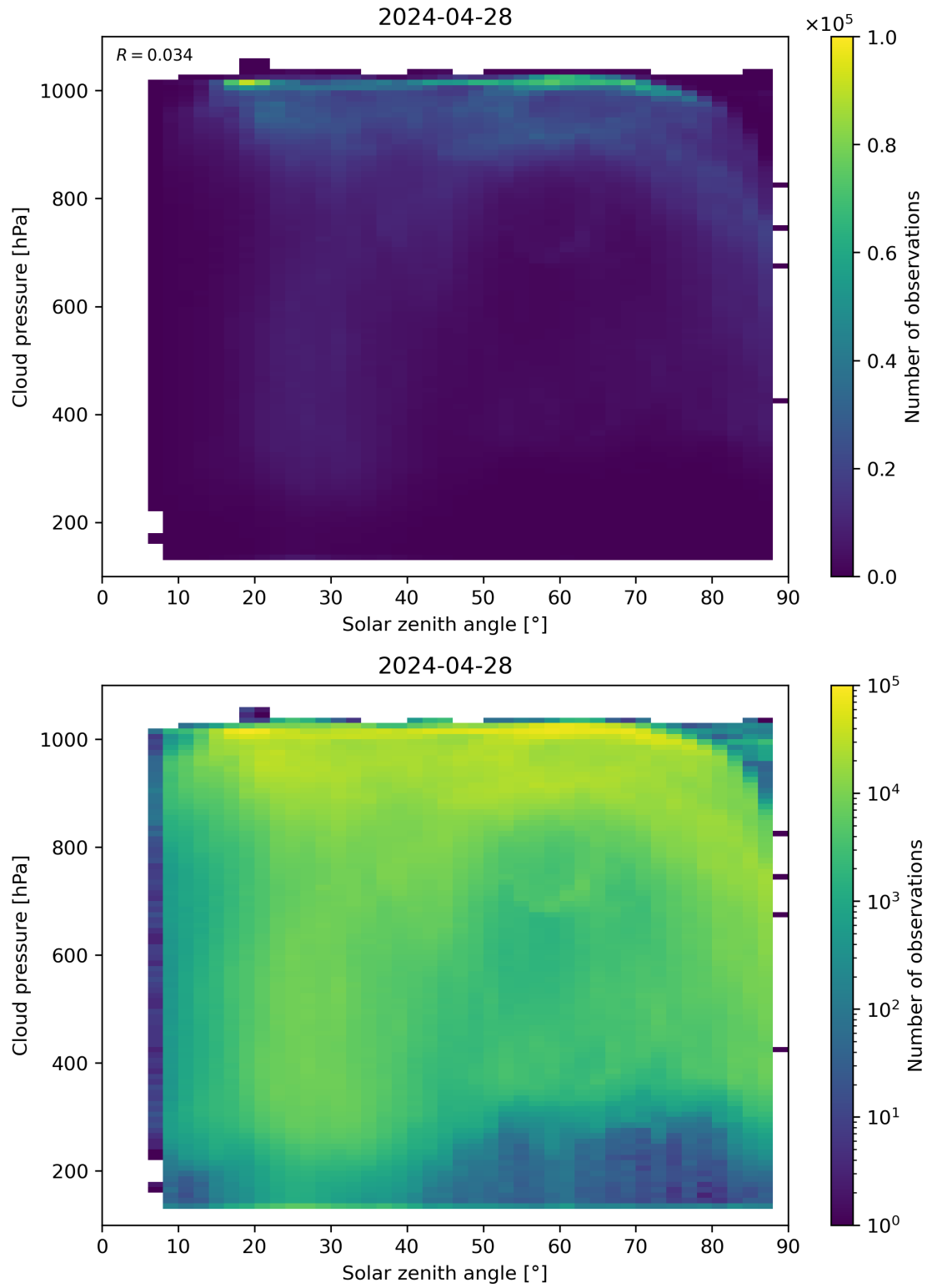
Figure 111: Scatter density plot of “Solar zenith angle” against “Cloud pressure” for 2024-04-27 to 2024-04-29.
