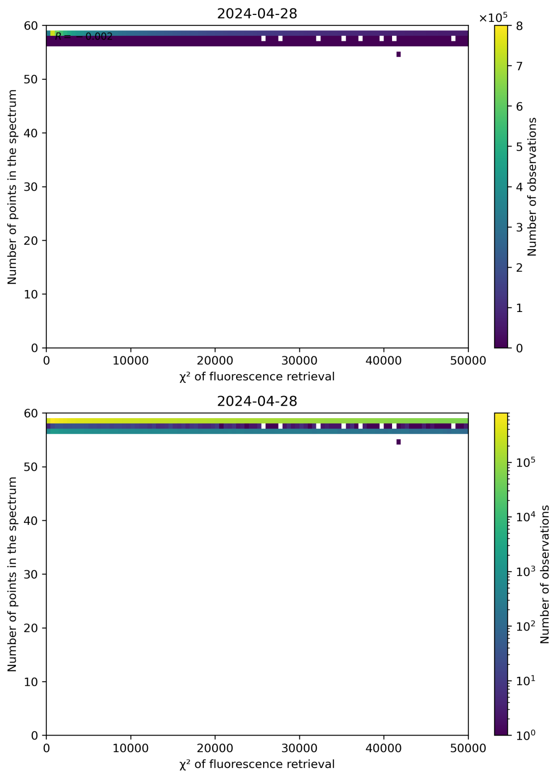
Figure 68: Scatter density plot of " \chi^2 of fluorescence retrieval" against "Number of points in the spectrum" for 2024-04-27 to 2024-04-29.
