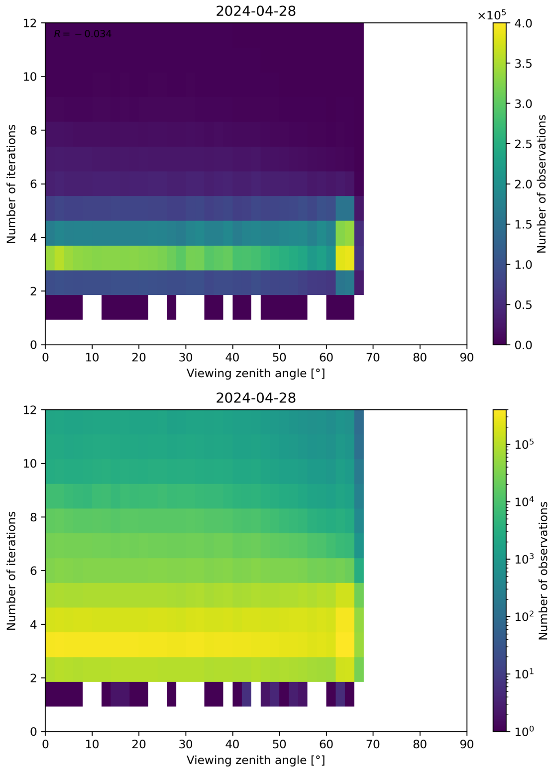
Figure 124: Scatter density plot of “Viewing zenith angle” against “Number of iterations” for 2024-04-27 to 2024-04-29.
