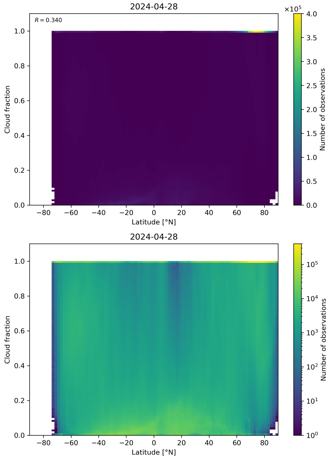
Figure 90: Scatter density plot of “Latitude” against “Cloud fraction” for 2024-04-27 to 2024-04-29.
