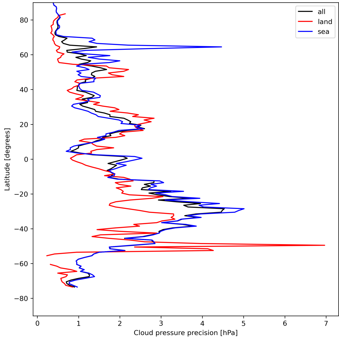
Figure 14: Zonal average of “Cloud pressure precision” for 2024-04-27 to 2024-04-29.
