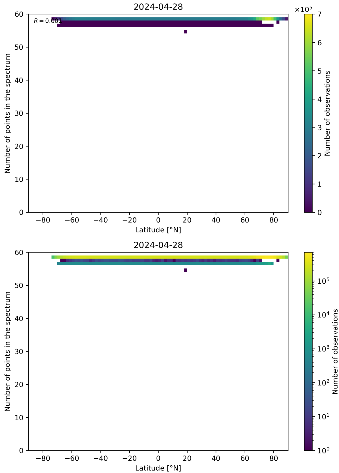
Figure 94: Scatter density plot of “Latitude” against “Number of points in the spectrum” for 2024-04-27 to 2024-04-29.
