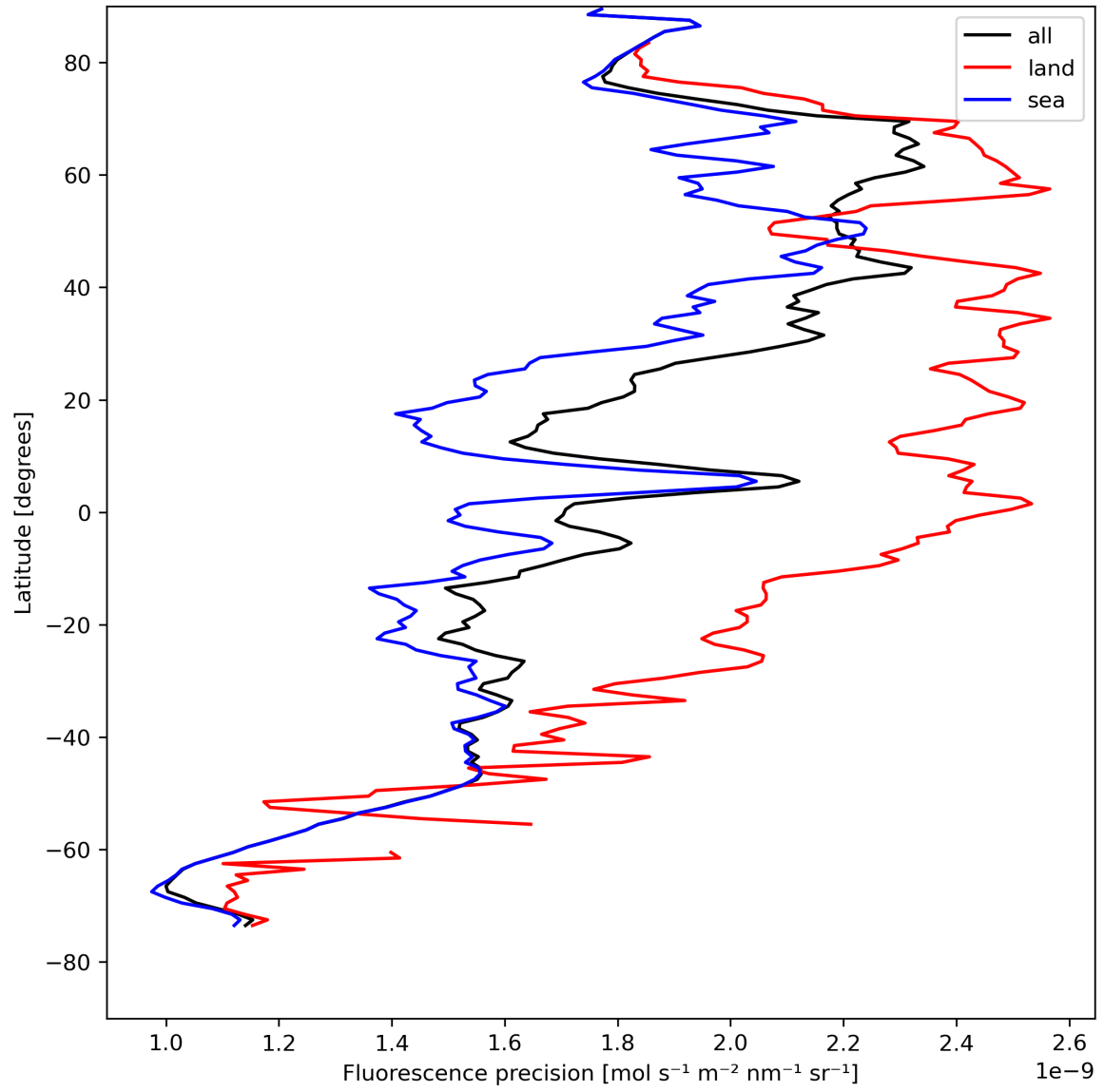
Figure 24: Zonal average of “Fluorescence precision” for 2024-04-27 to 2024-04-29.
