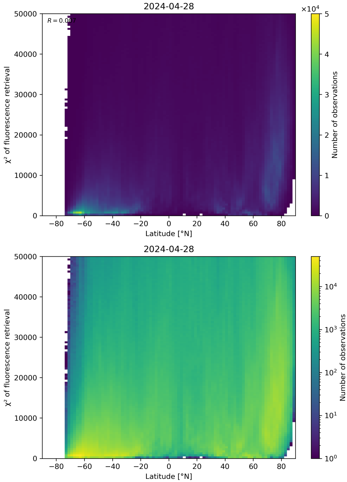
Figure 89: Scatter density plot of “Latitude” against “ \chi^2 of fluorescence retrieval” for 2024-04-27 to 2024-04-29.
