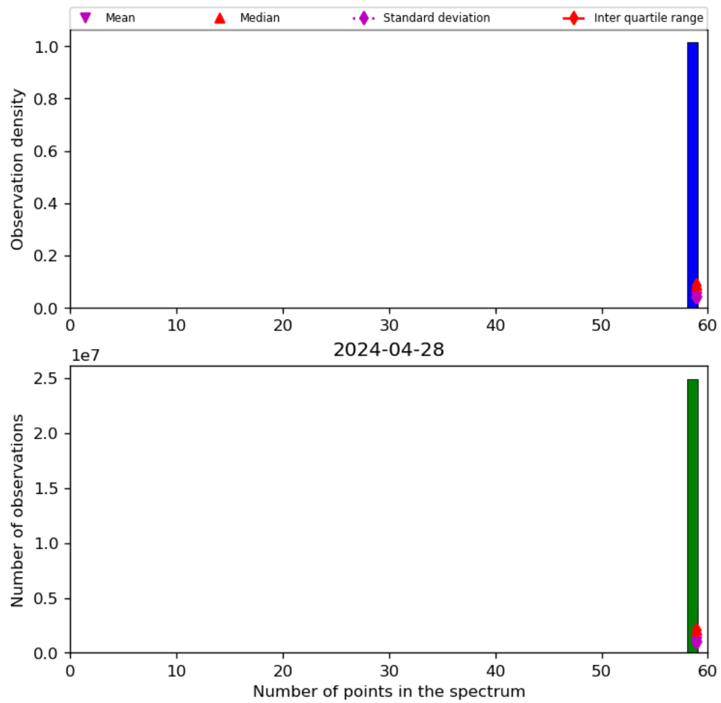
Figure 44: Histogram of “Number of points in the spectrum” for 2024-04-27 to 2024-04-29
