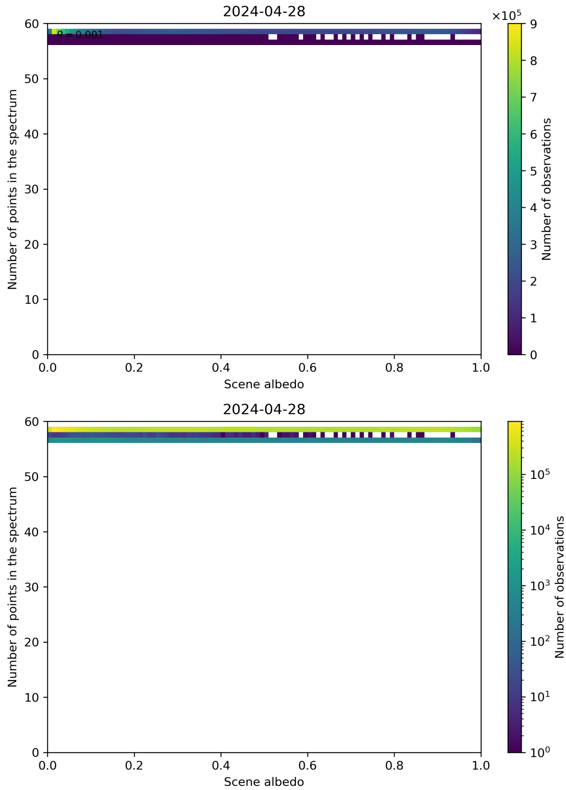
Figure 106: Scatter density plot of “Scene albedo” against “Number of points in the spectrum” for 2024-04-27 to 2024-04-29.
