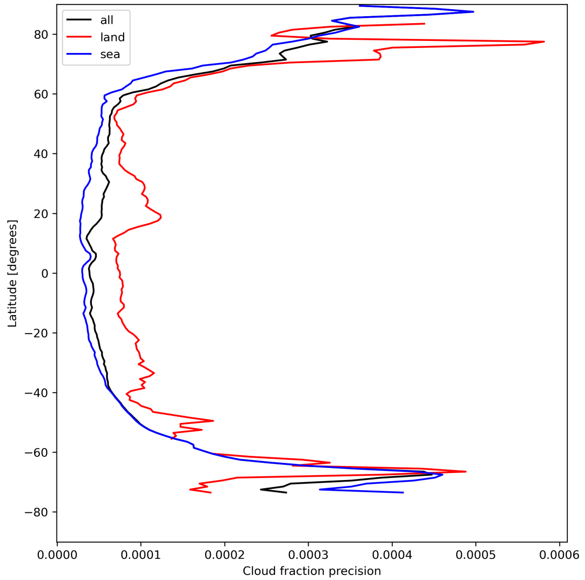
Figure 16: Zonal average of “Cloud fraction precision” for 2024-04-27 to 2024-04-29.
