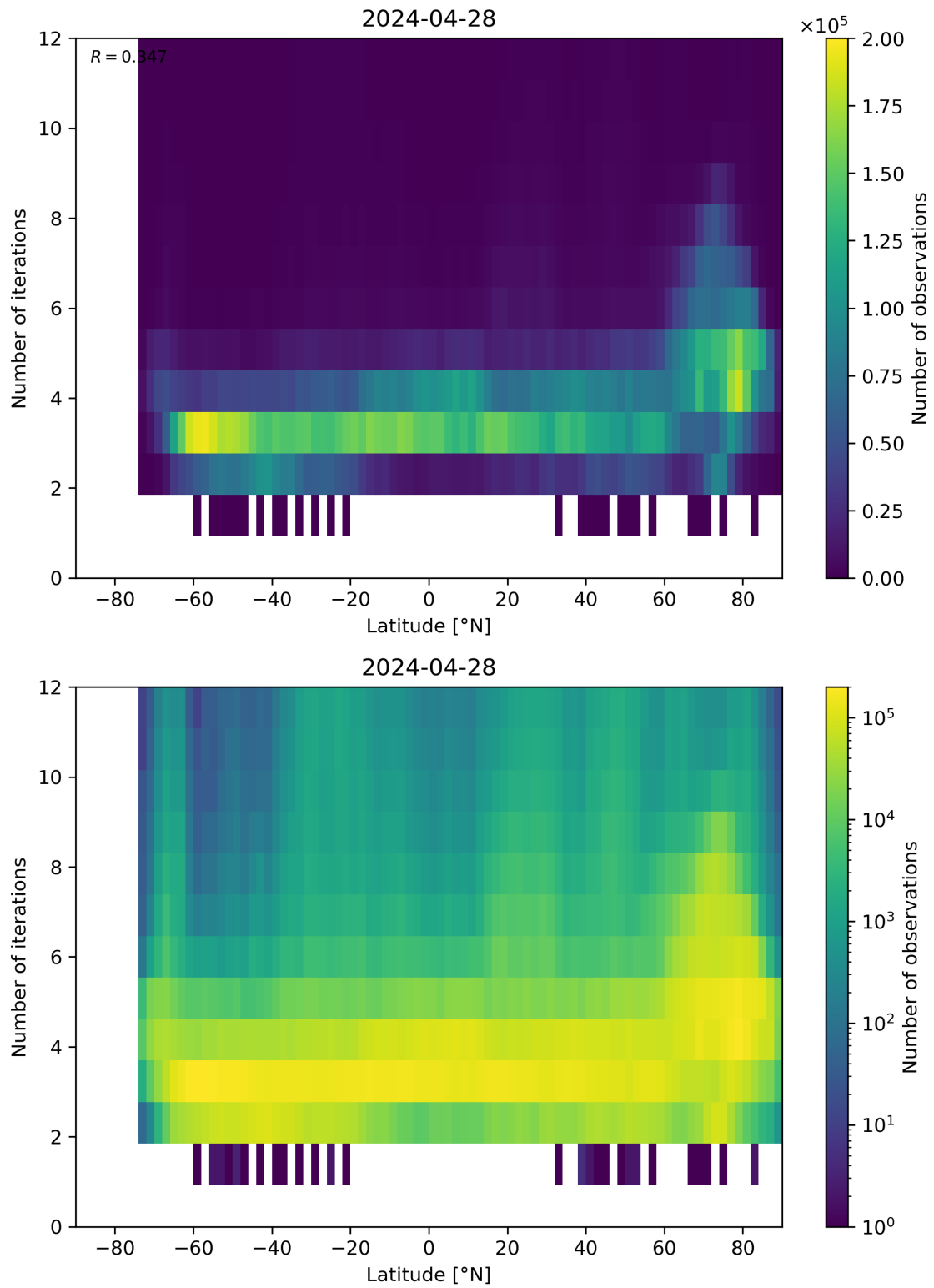
Figure 93: Scatter density plot of “Latitude” against “Number of iterations” for 2024-04-27 to 2024-04-29.
