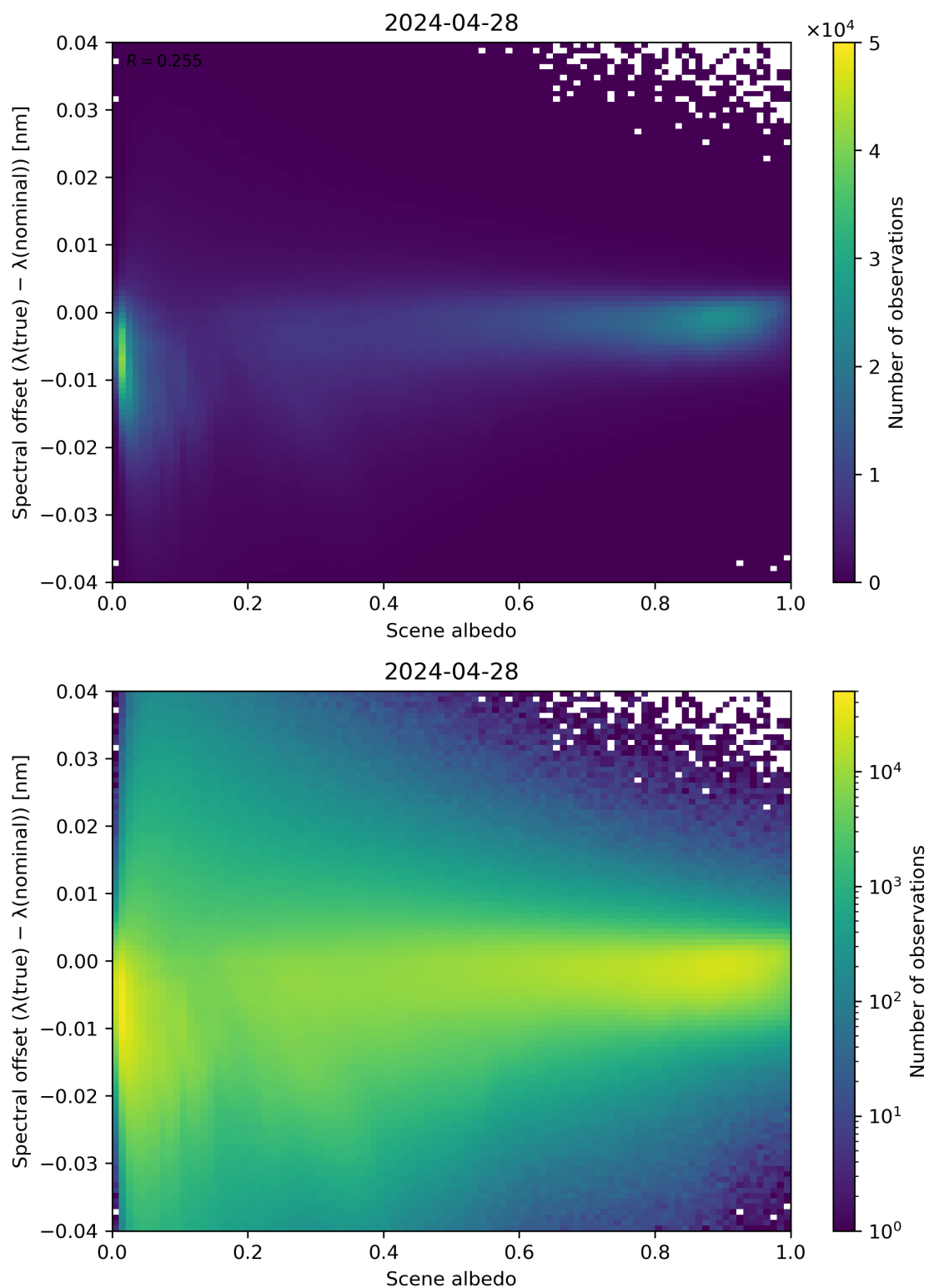
Figure 107: Scatter density plot of “Scene albedo” against “Spectral offset ( \lambda(\text{true}) - \lambda(\text{nominal}) )” for 2024-04-27 to 2024-04-29.
