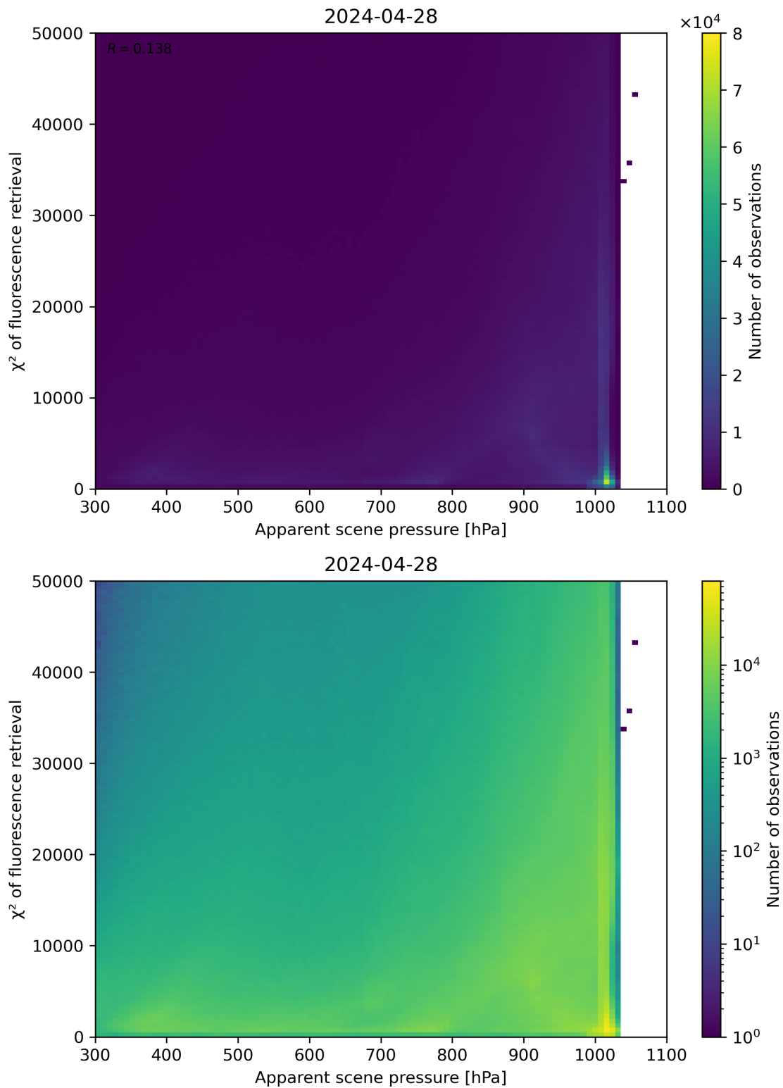
Figure 63: Scatter density plot of “Apparent scene pressure” against “ \chi^2 of fluorescence retrieval” for 2024-04-27 to 2024-04-29.
