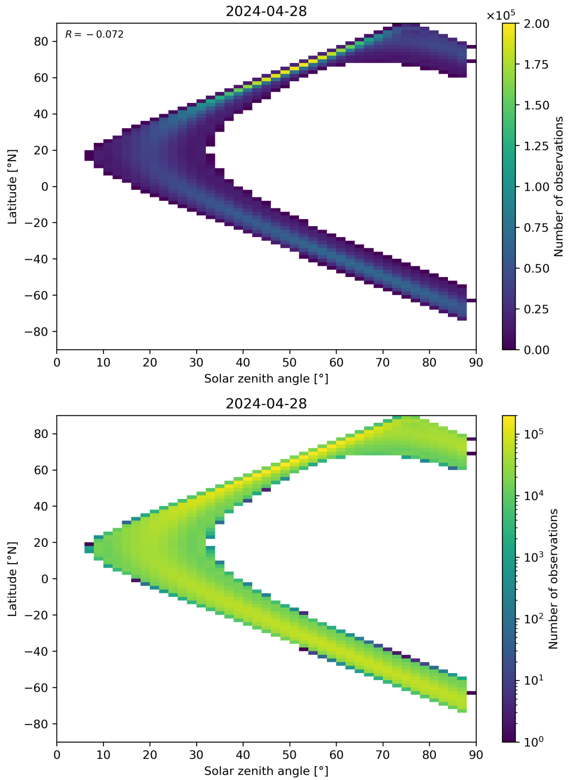
Figure 113: Scatter density plot of “Solar zenith angle” against “Latitude” for 2024-04-27 to 2024-04-29.
