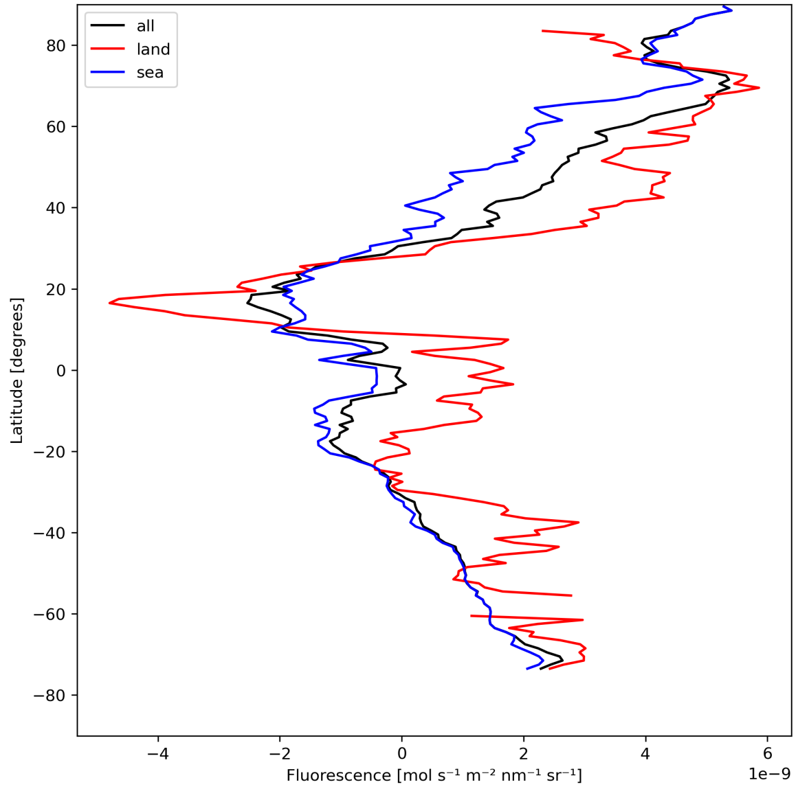
Figure 23: Zonal average of “Fluorescence” for 2024-04-27 to 2024-04-29.
