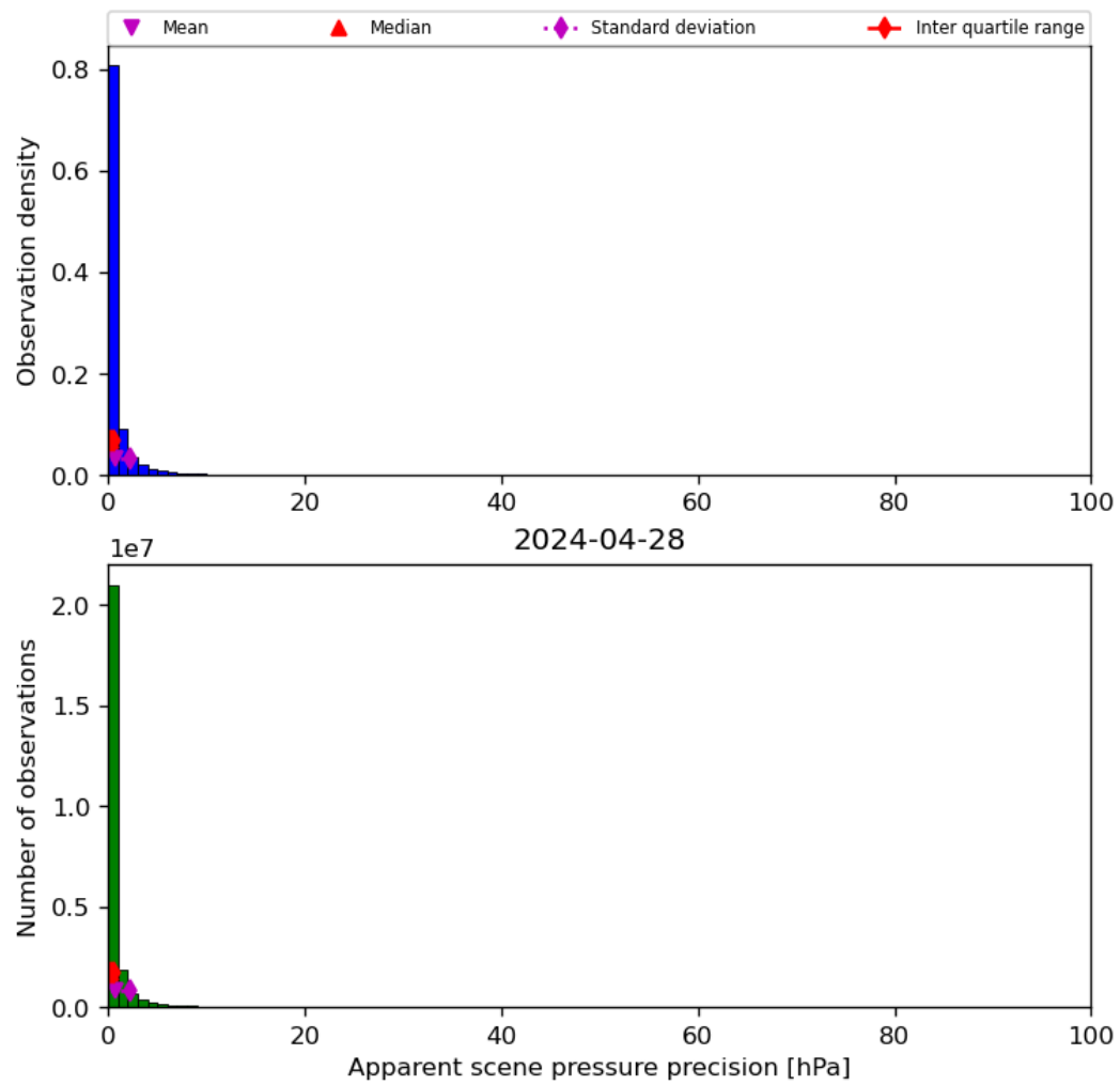
Figure 37: Histogram of “Apparent scene pressure precision” for 2024-04-27 to 2024-04-29
