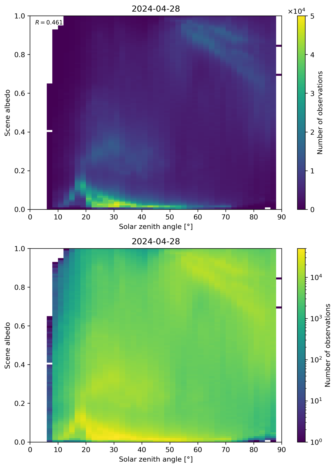
Figure 116: Scatter density plot of “Solar zenith angle” against “Scene albedo” for 2024-04-27 to 2024-04-29.
