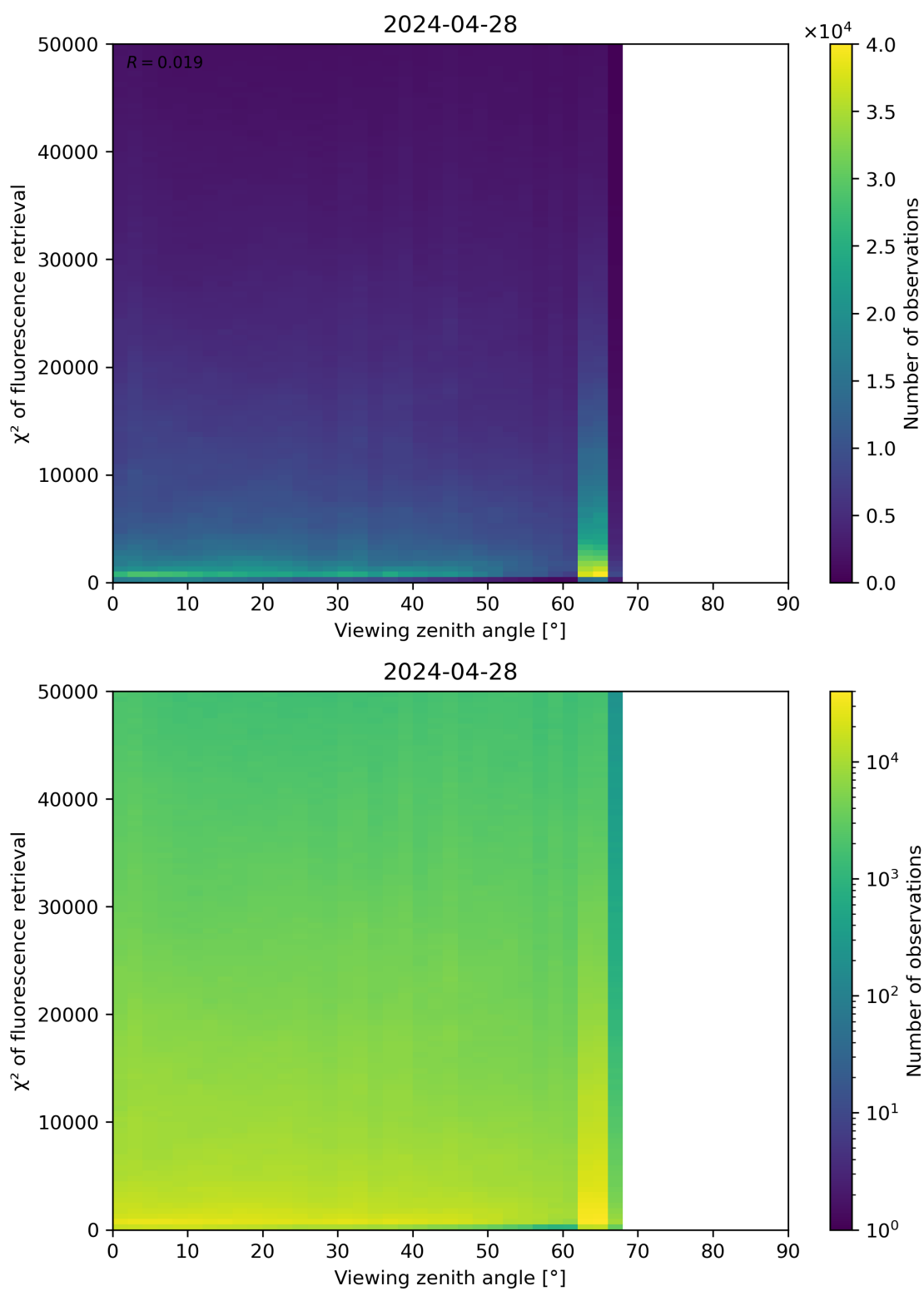
Figure 119: Scatter density plot of “Viewing zenith angle” against “ \chi^2 of fluorescence retrieval” for 2024-04-27 to 2024-04-29.
