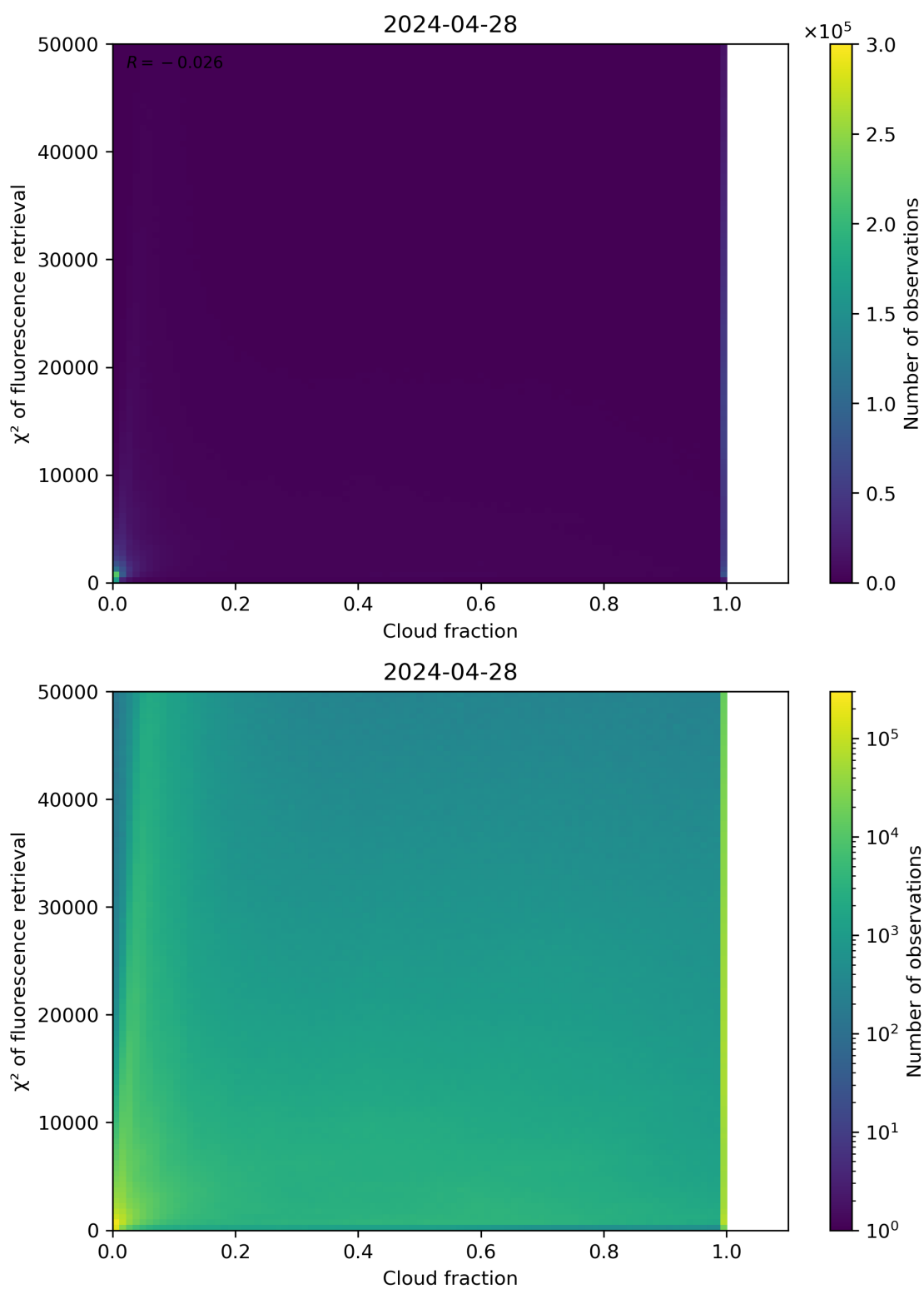
Figure 71: Scatter density plot of “Cloud fraction” against “ \chi^2 of fluorescence retrieval” for 2024-04-27 to 2024-04-29.
