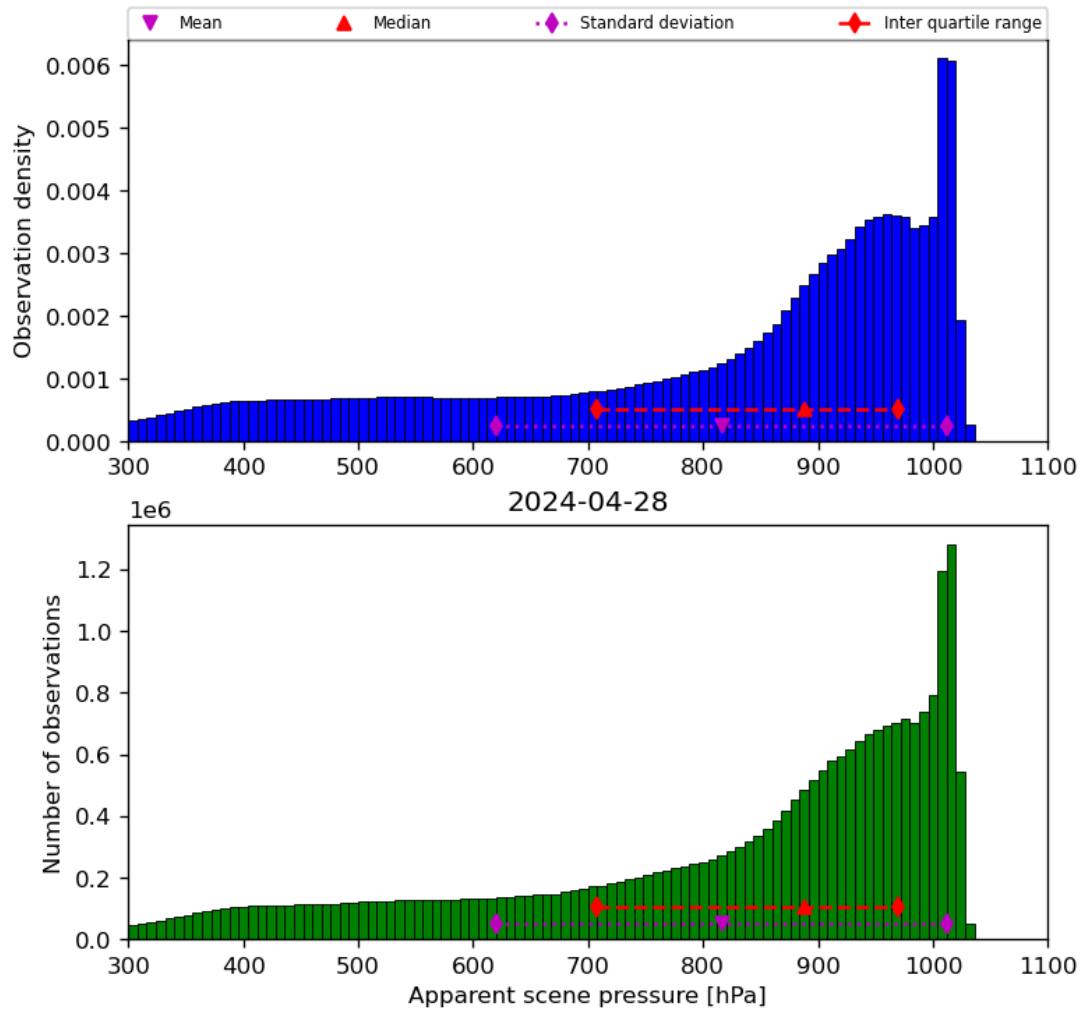
Figure 36: Histogram of “Apparent scene pressure” for 2024-04-27 to 2024-04-29
