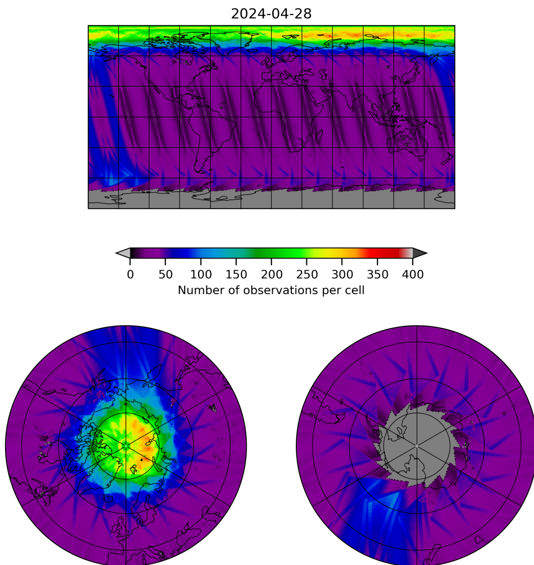
Figure 11: Map of the number of observations for 2024-04-27 to 2024-04-29
