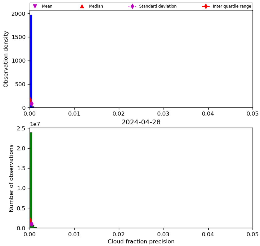
Figure 33: Histogram of “Cloud fraction precision” for 2024-04-27 to 2024-04-29
