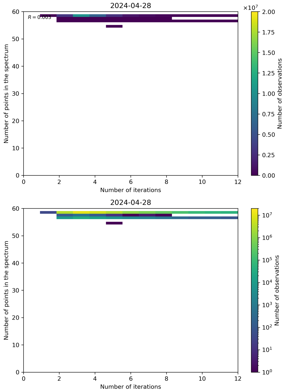
Figure 99: Scatter density plot of “Number of iterations” against “Number of points in the spectrum” for 2024-04-27 to 2024-04-29.
