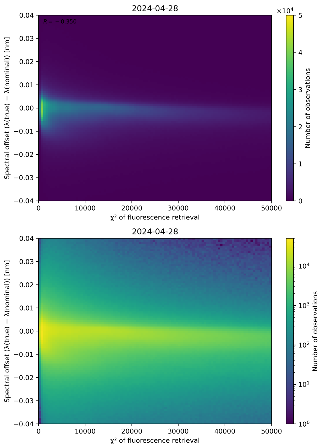
Figure 69: Scatter density plot of " \chi^2 of fluorescence retrieval" against "Spectral offset ( \lambda(\text{true}) - \lambda(\text{nominal}) )" for 2024-04-27 to 2024-04-29.
