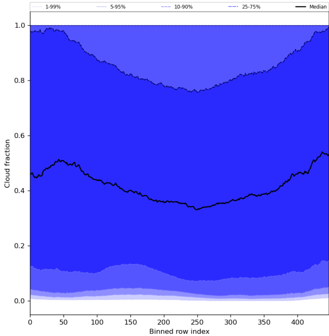
Figure 49: Along track statistics of “Cloud fraction” for 2024-04-27 to 2024-04-29
