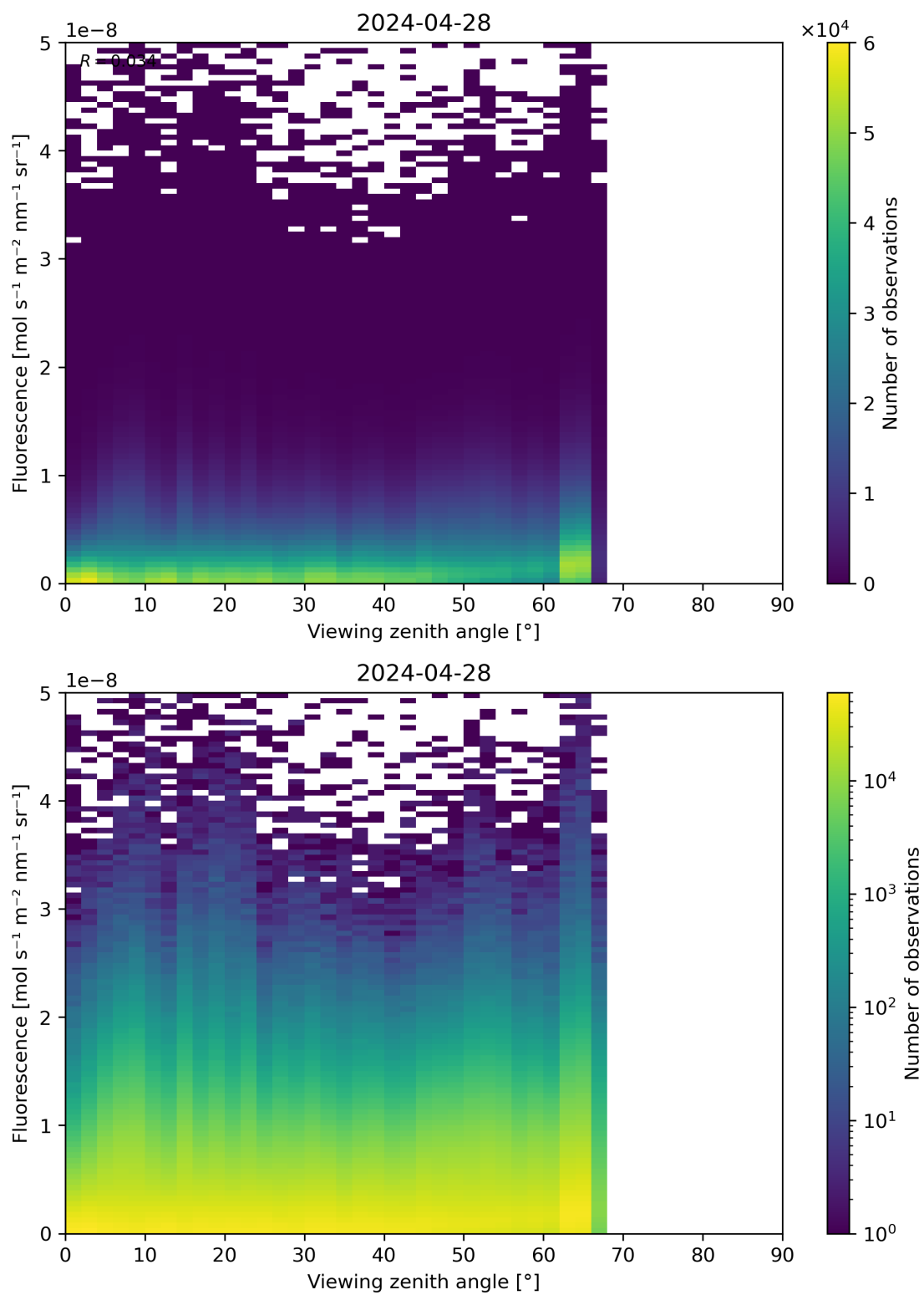
Figure 122: Scatter density plot of “Viewing zenith angle” against “Fluorescence” for 2024-04-27 to 2024-04-29.
