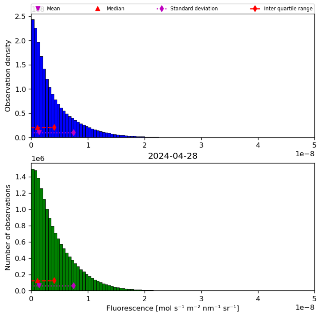
Figure 40: Histogram of “Fluorescence” for 2024-04-27 to 2024-04-29
