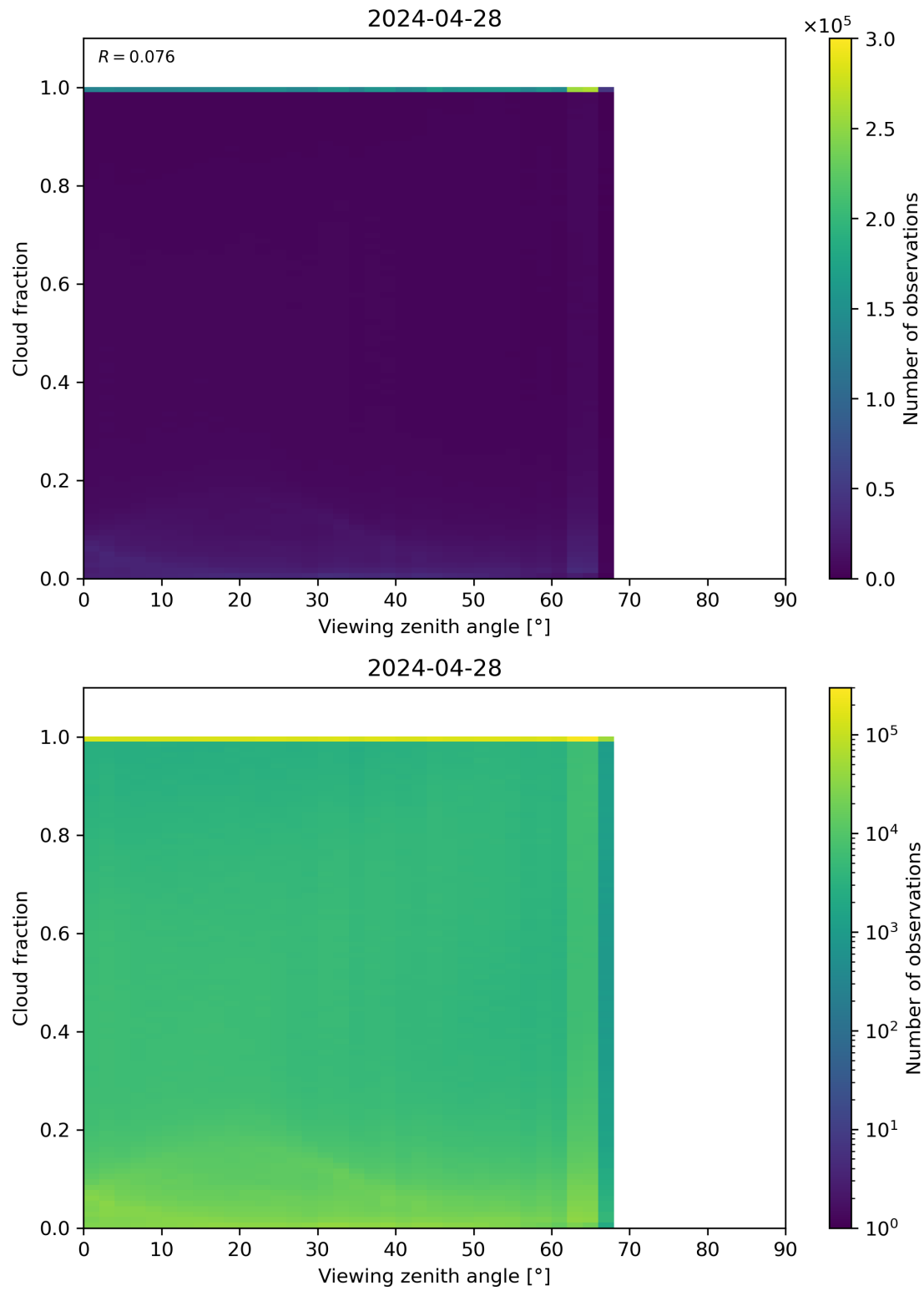
Figure 120: Scatter density plot of “Viewing zenith angle” against “Cloud fraction” for 2024-04-27 to 2024-04-29.
