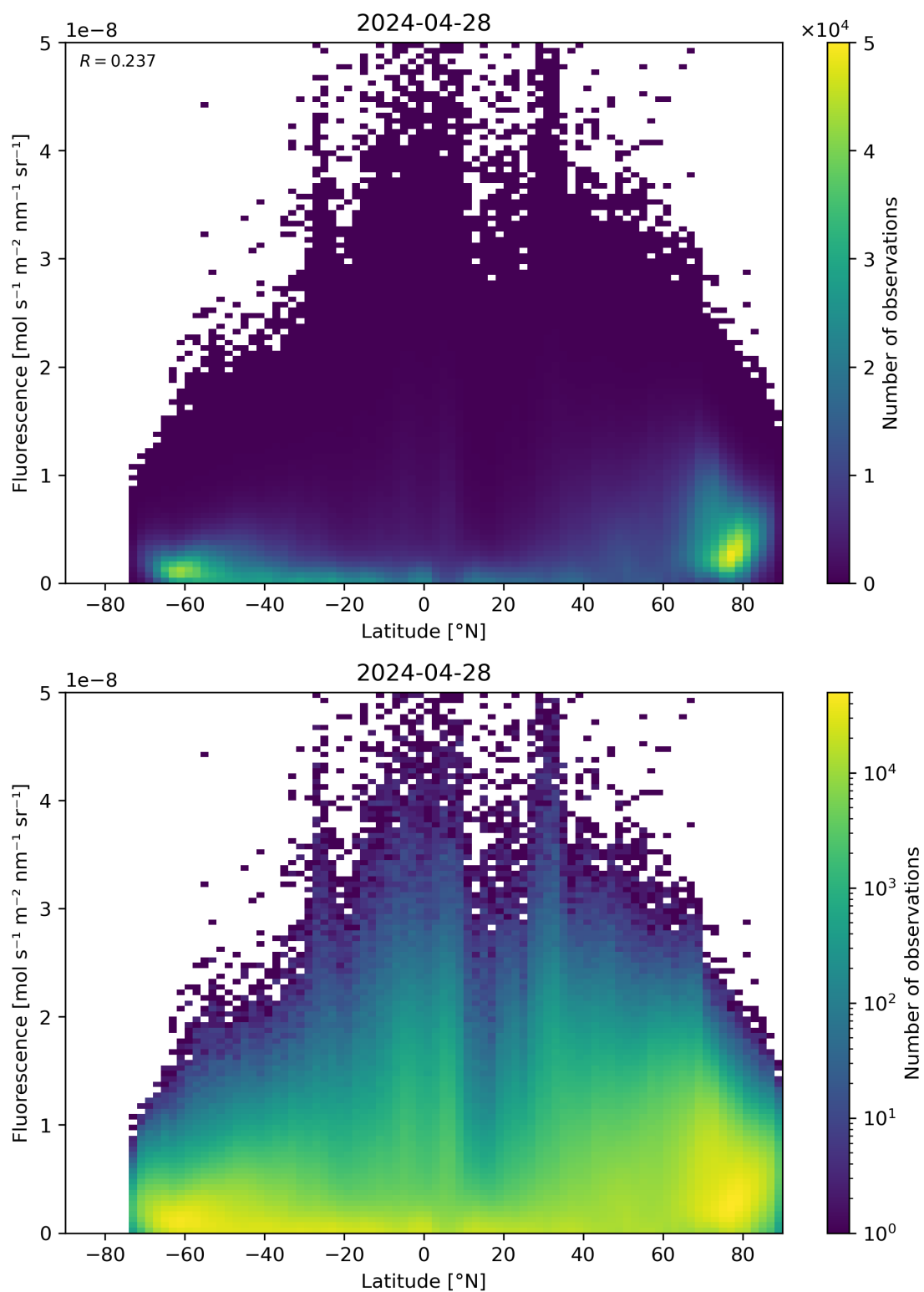
Figure 92: Scatter density plot of “Latitude” against “Fluorescence” for 2024-04-27 to 2024-04-29.
