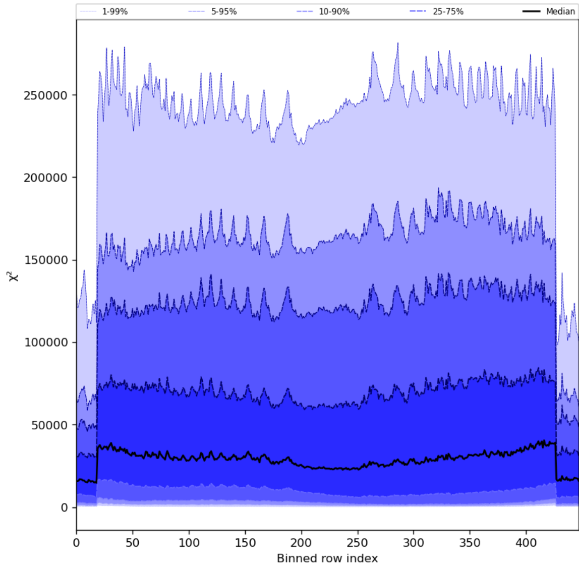
Figure 55: Along track statistics of “ \chi^2 ” for 2024-04-27 to 2024-04-29
