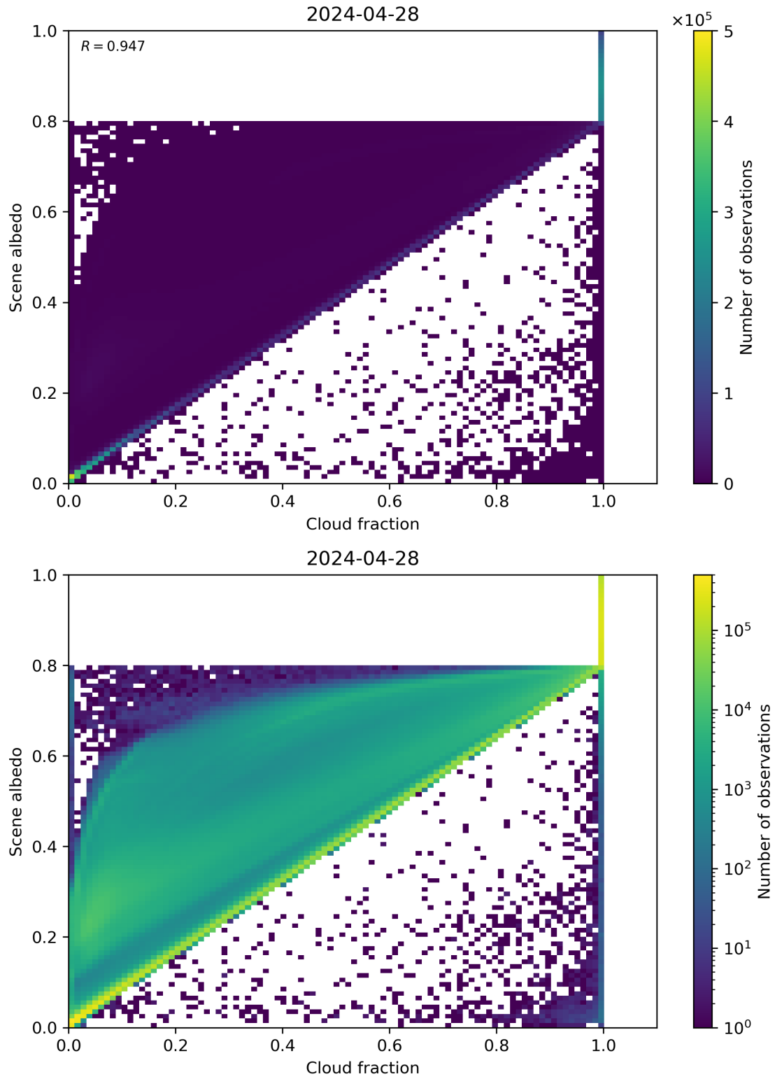
Figure 75: Scatter density plot of “Cloud fraction” against “Scene albedo” for 2024-04-27 to 2024-04-29.
