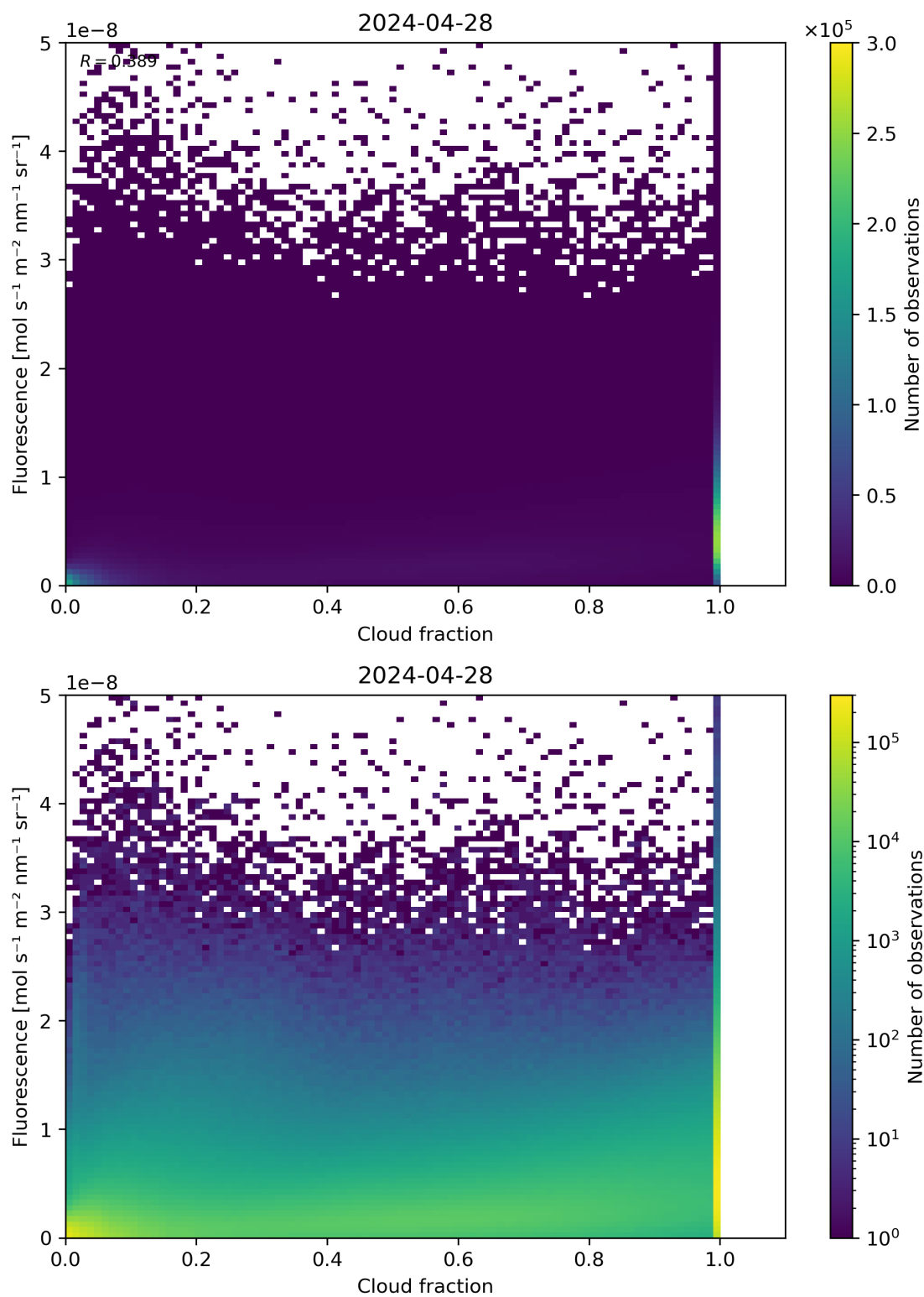
Figure 72: Scatter density plot of “Cloud fraction” against “Fluorescence” for 2024-04-27 to 2024-04-29.
