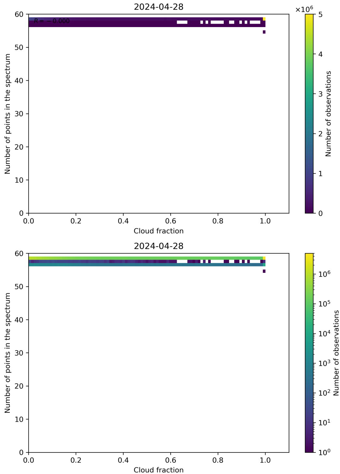
Figure 74: Scatter density plot of “Cloud fraction” against “Number of points in the spectrum” for 2024-04-27 to 2024-04-29.
