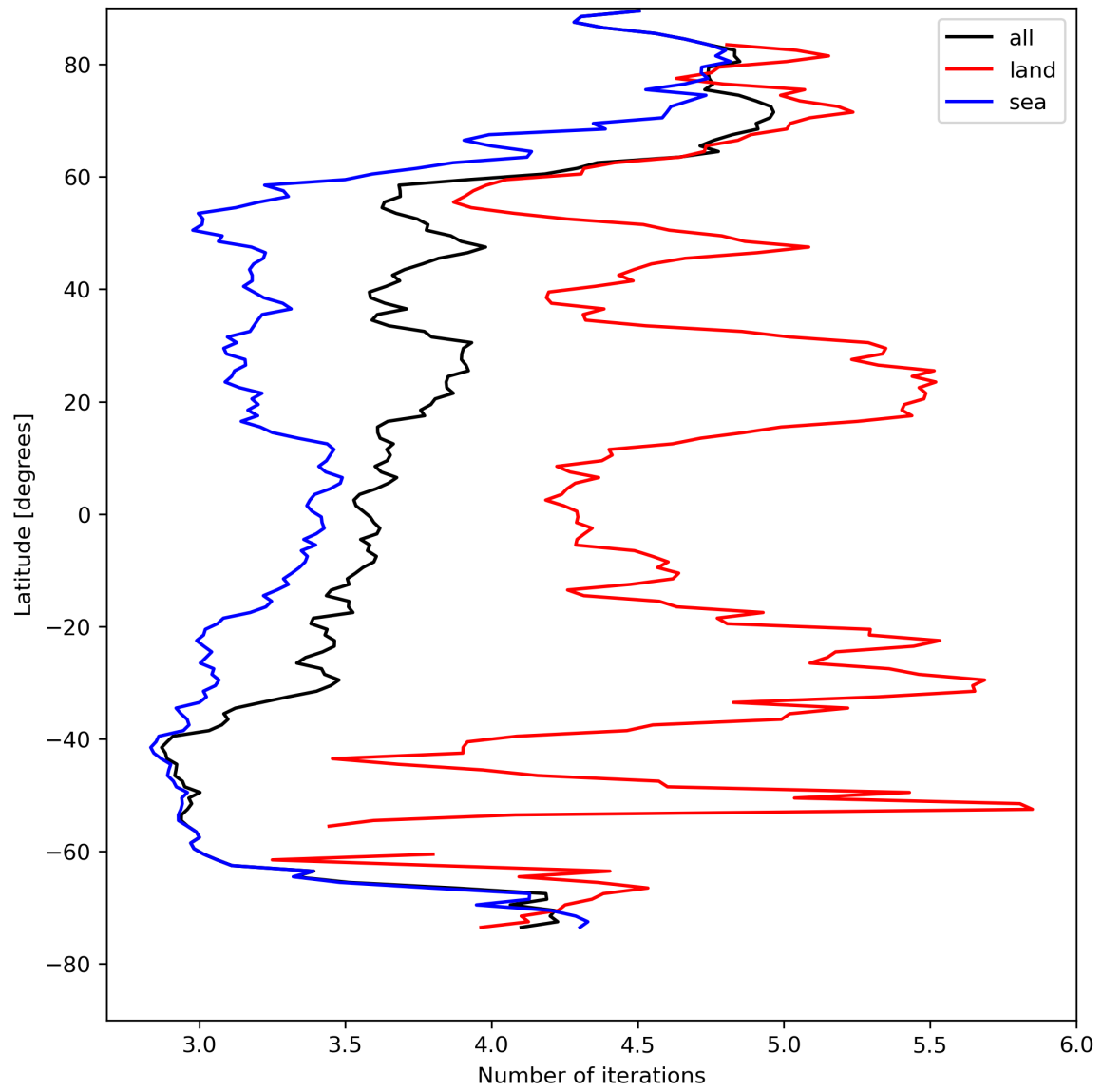
Figure 22: Zonal average of “Number of iterations” for 2024-04-27 to 2024-04-29.
