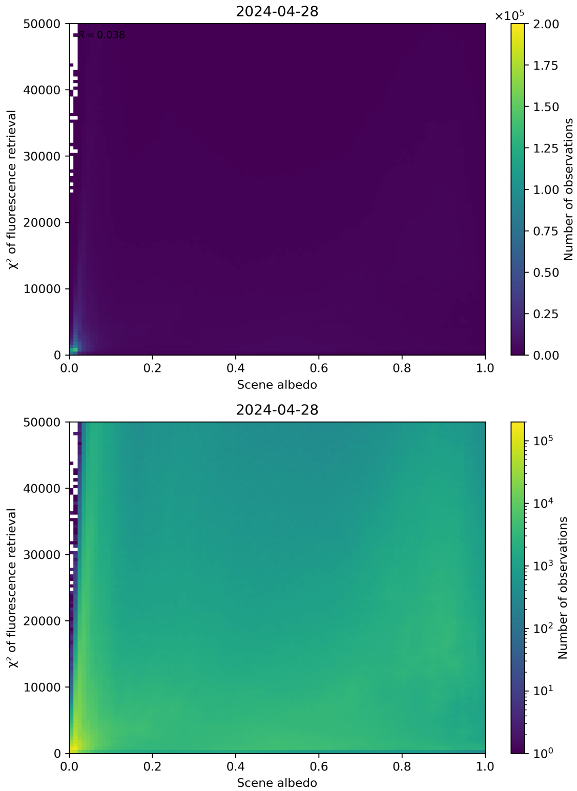
Figure 103: Scatter density plot of “Scene albedo” against “ \chi^2 of fluorescence retrieval” for 2024-04-27 to 2024-04-29.
