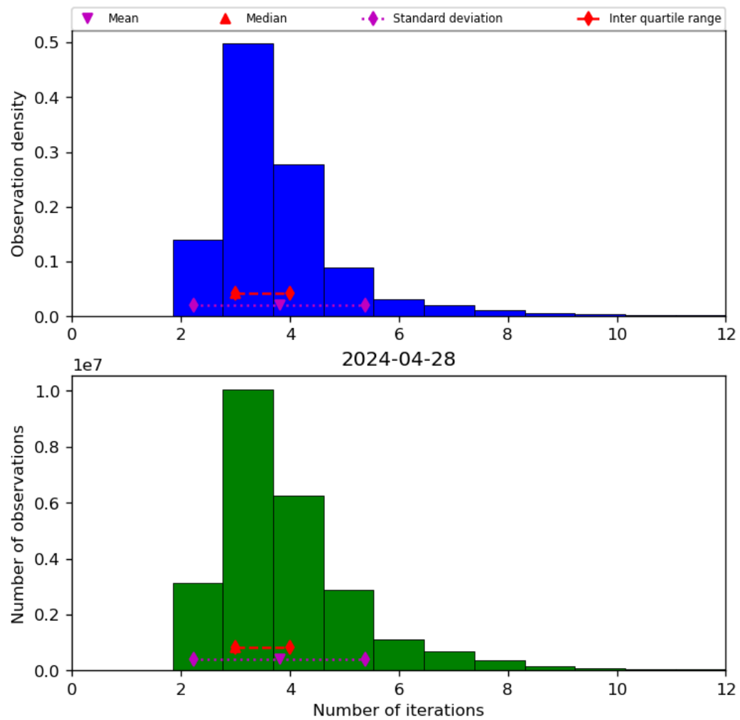
Figure 39: Histogram of “Number of iterations” for 2024-04-27 to 2024-04-29
