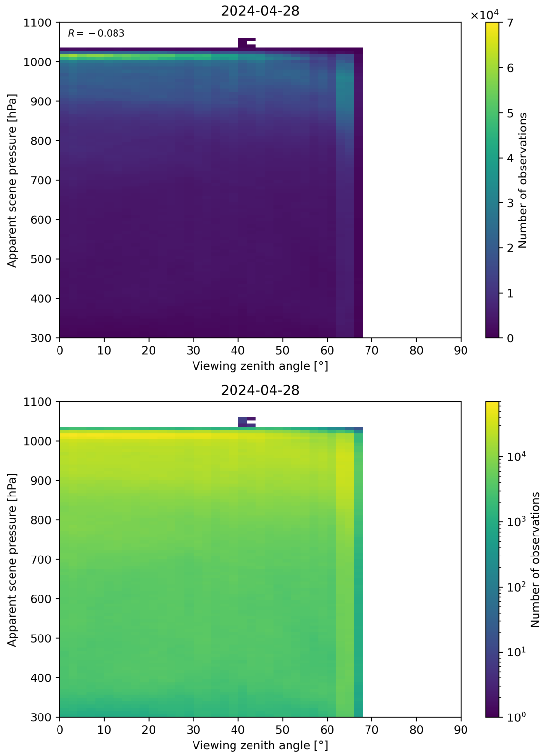
Figure 118: Scatter density plot of “Viewing zenith angle” against “Apparent scene pressure” for 2024-04-27 to 2024-04-29.
