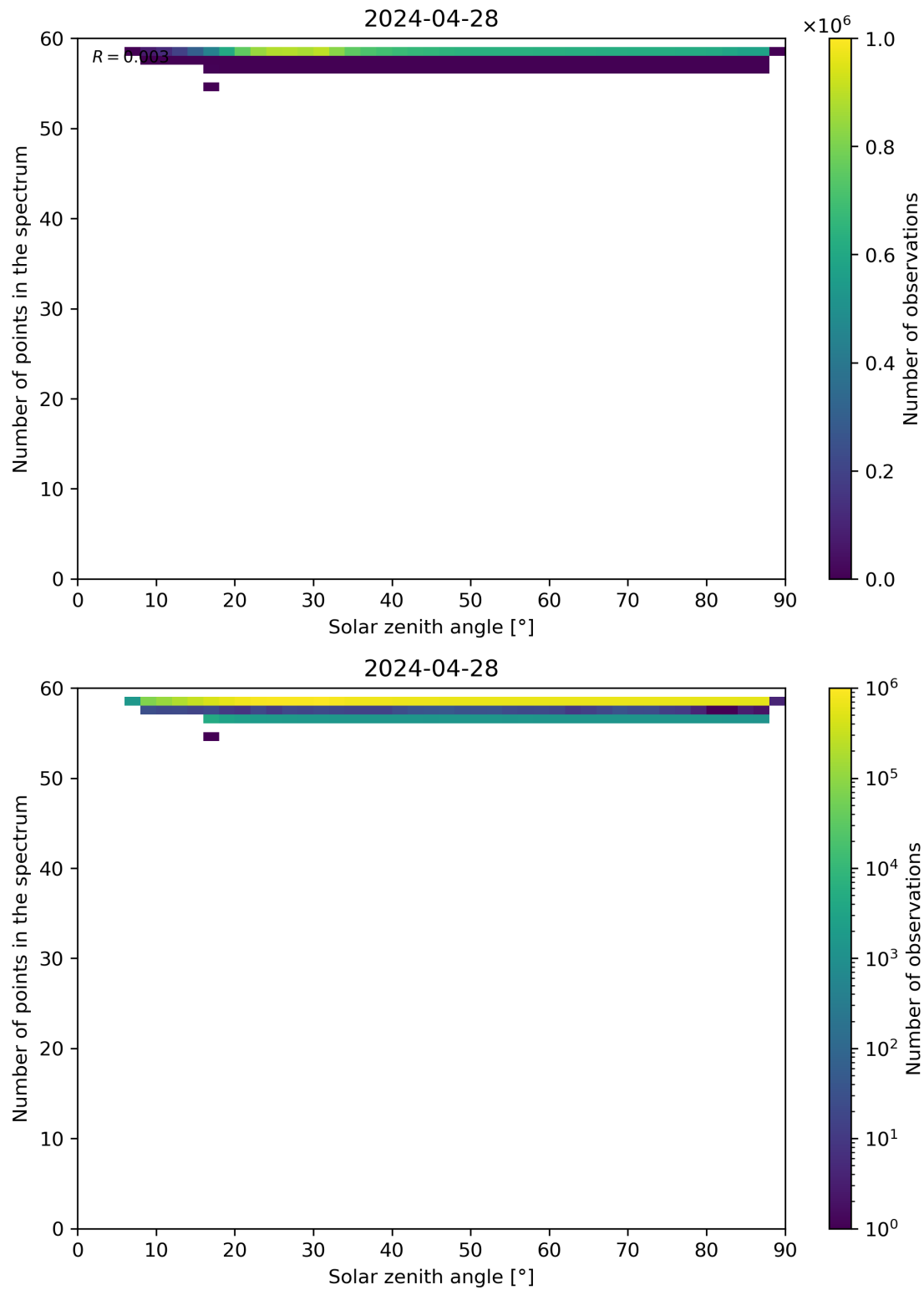
Figure 115: Scatter density plot of “Solar zenith angle” against “Number of points in the spectrum” for 2024-04-27 to 2024-04-29.
