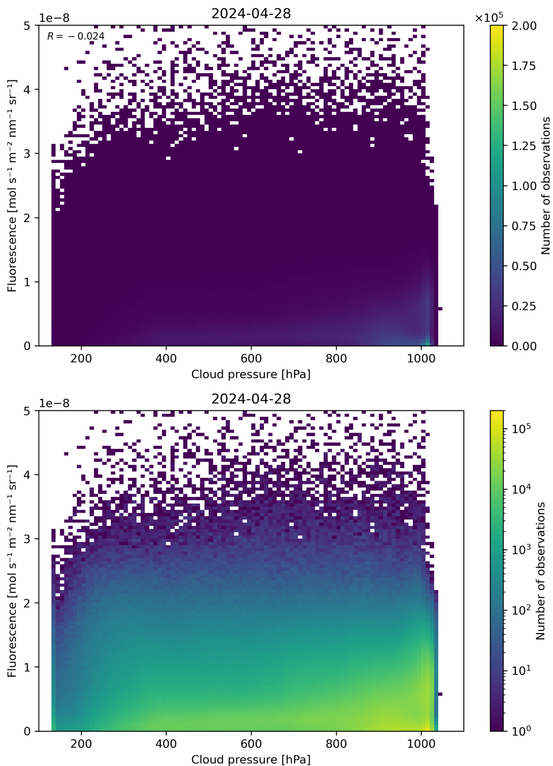
Figure 80: Scatter density plot of “Cloud pressure” against “Fluorescence” for 2024-04-27 to 2024-04-29.
