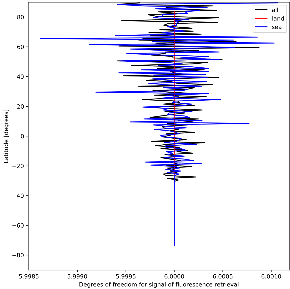
Figure 26: Zonal average of “Degrees of freedom for signal of fluorescence retrieval” for 2024-04-27 to 2024-04-29.
