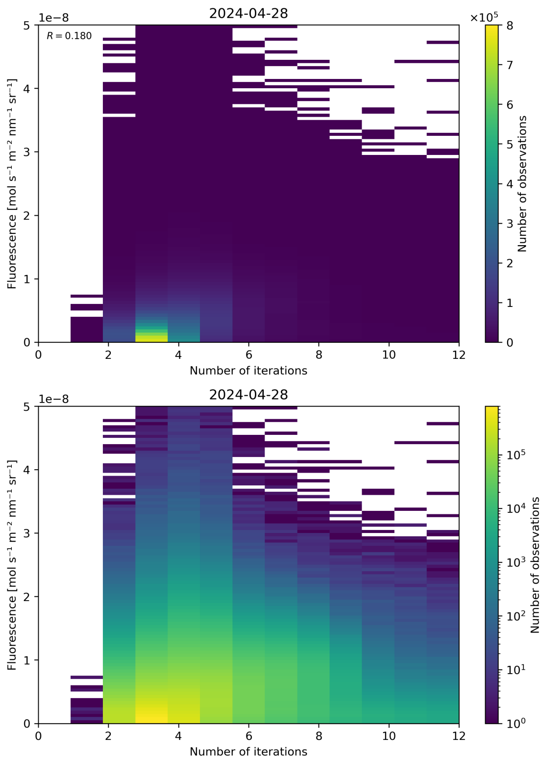
Figure 98: Scatter density plot of “Number of iterations” against “Fluorescence” for 2024-04-27 to 2024-04-29.
