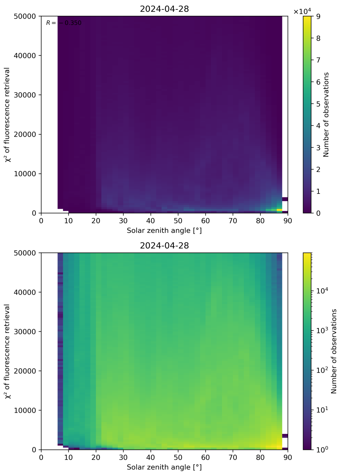
Figure 109: Scatter density plot of “Solar zenith angle” against “ \chi^2 of fluorescence retrieval” for 2024-04-27 to 2024-04-29.
