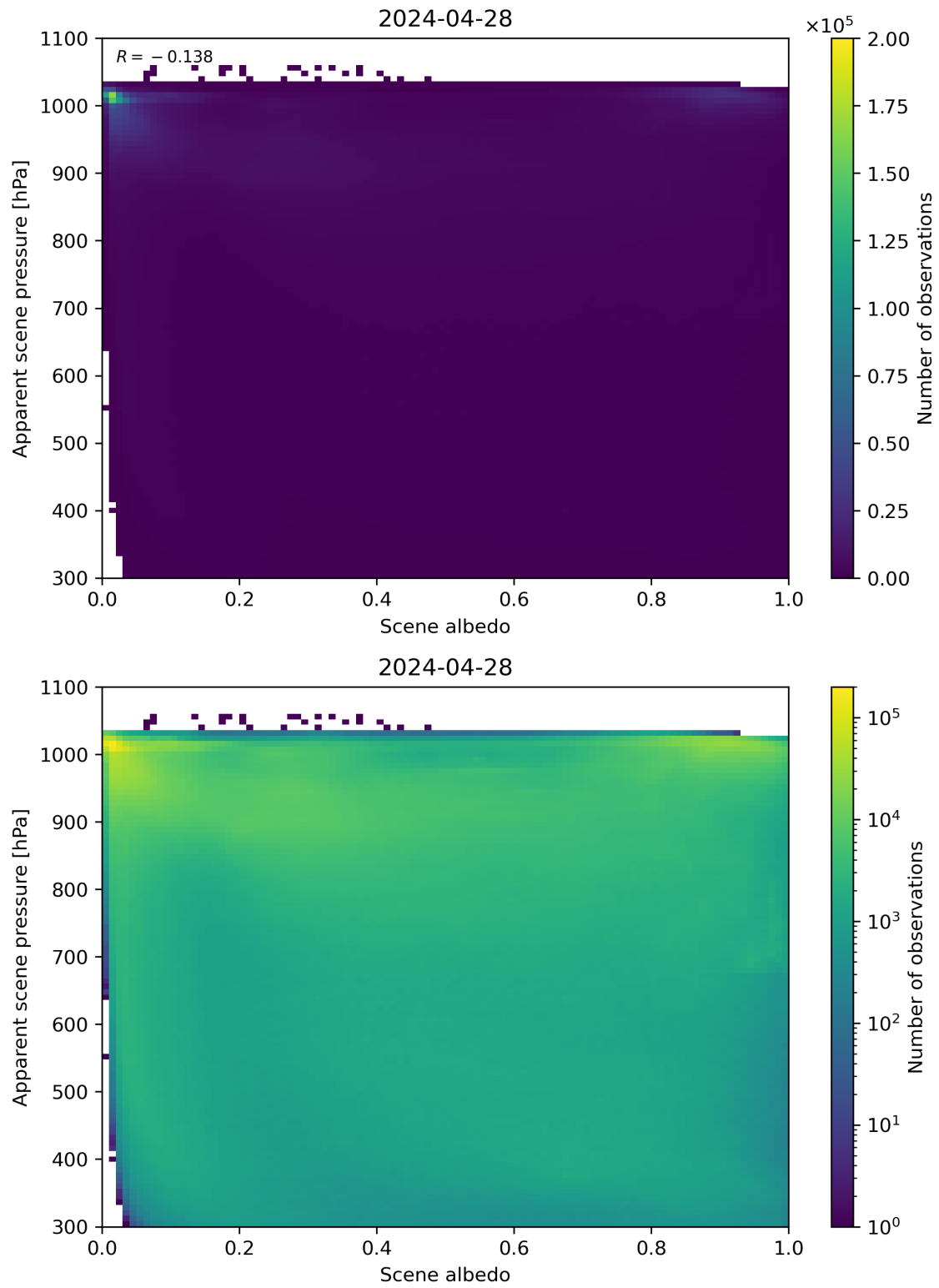
Figure 102: Scatter density plot of “Scene albedo” against “Apparent scene pressure” for 2024-04-27 to 2024-04-29.
