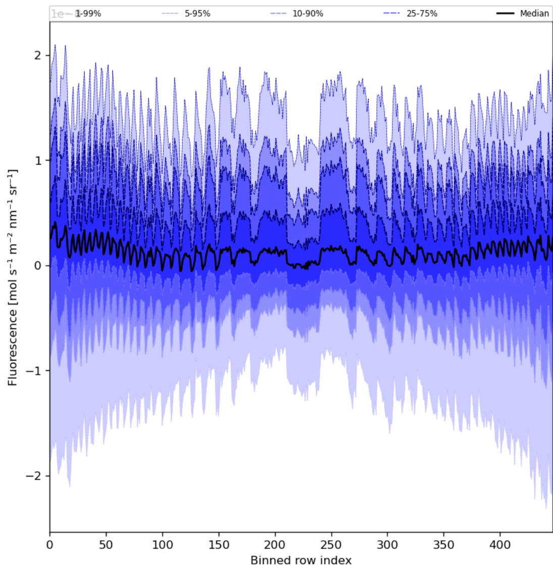
Figure 57: Along track statistics of “Fluorescence” for 2024-04-27 to 2024-04-29
