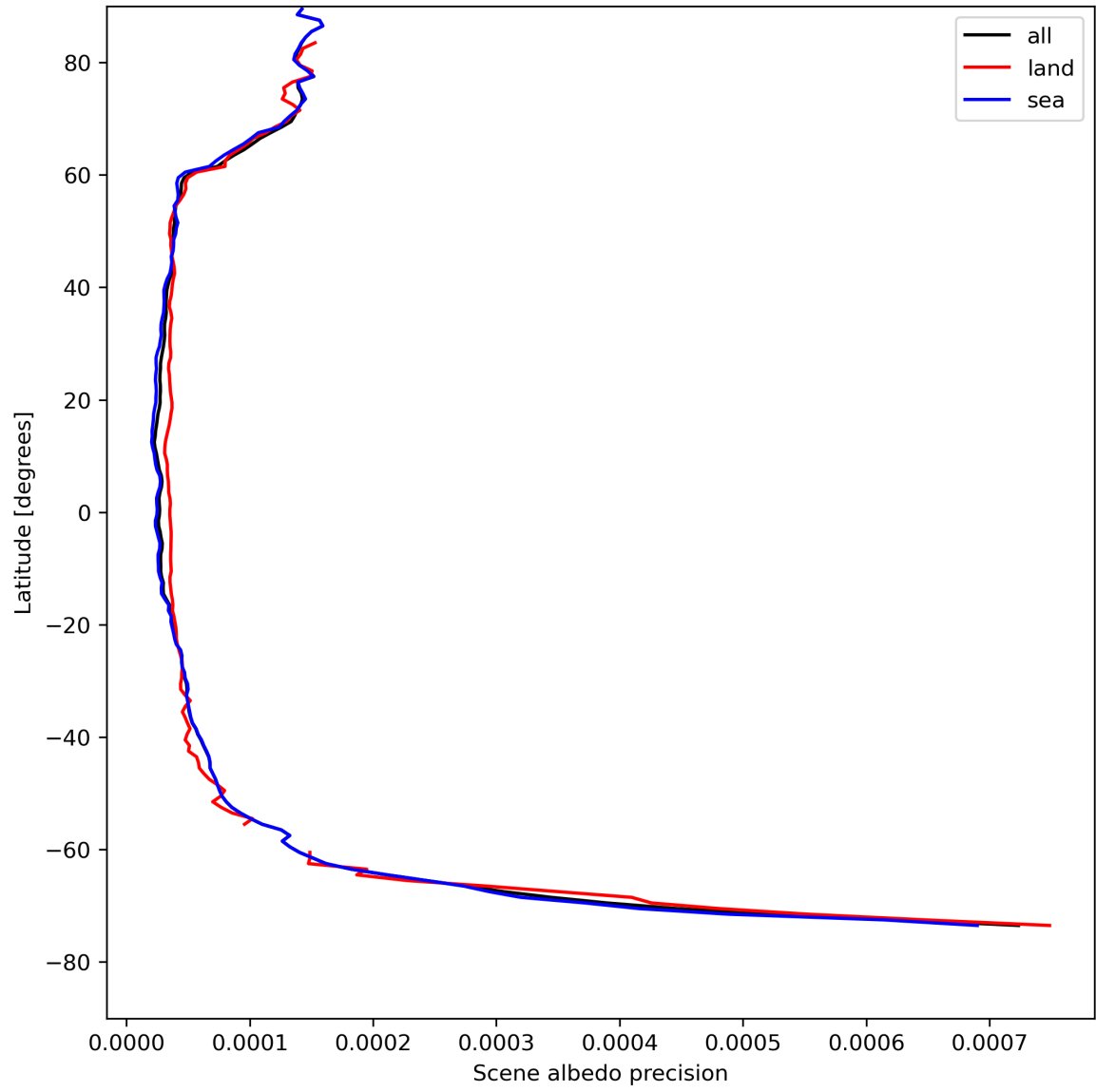
Figure 18: Zonal average of “Scene albedo precision” for 2024-04-27 to 2024-04-29.
