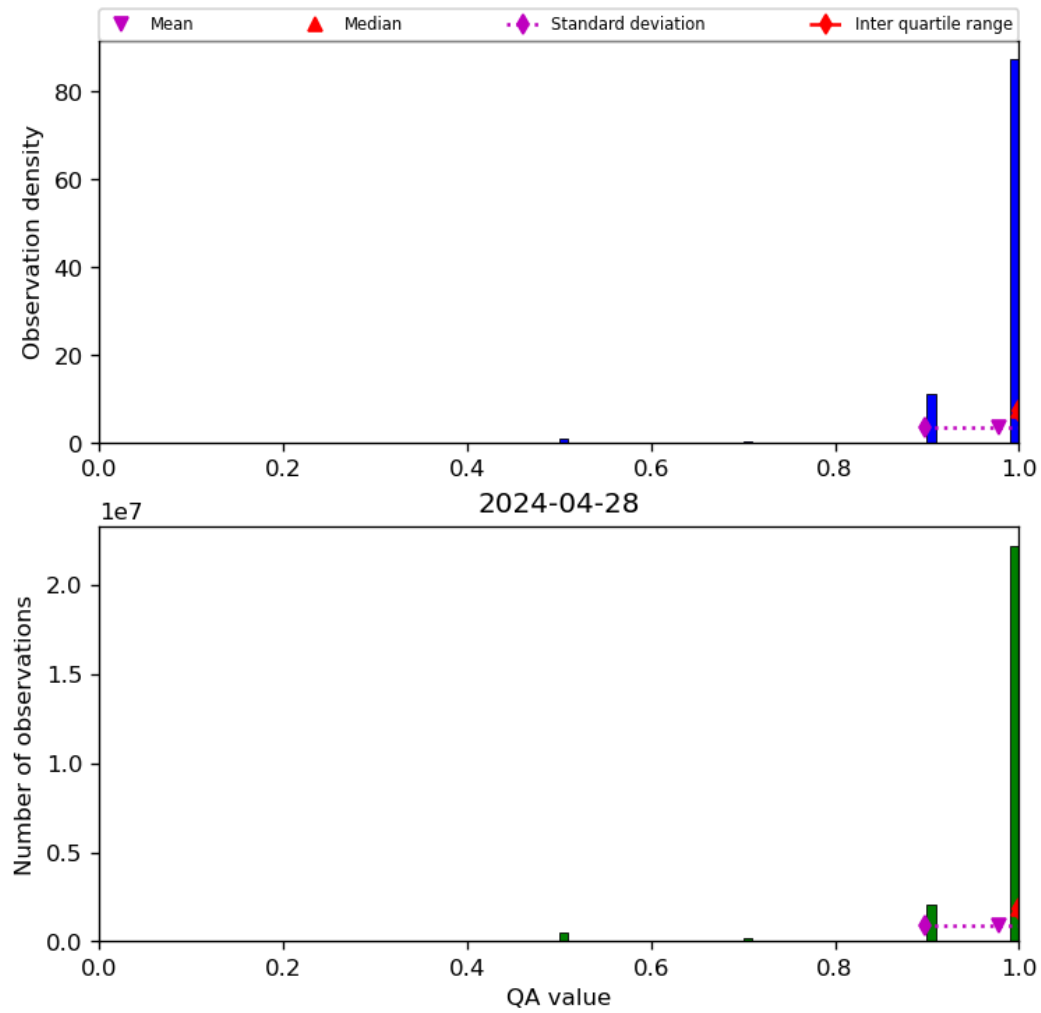
Figure 29: Histogram of “QA value” for 2024-04-27 to 2024-04-29
