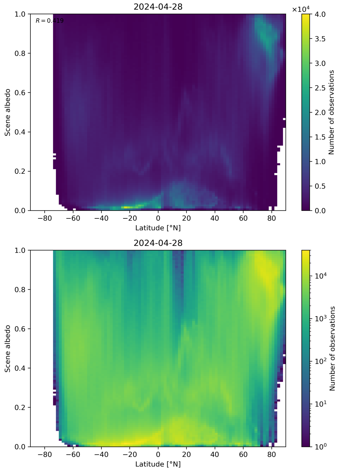
Figure 95: Scatter density plot of “Latitude” against “Scene albedo” for 2024-04-27 to 2024-04-29.
