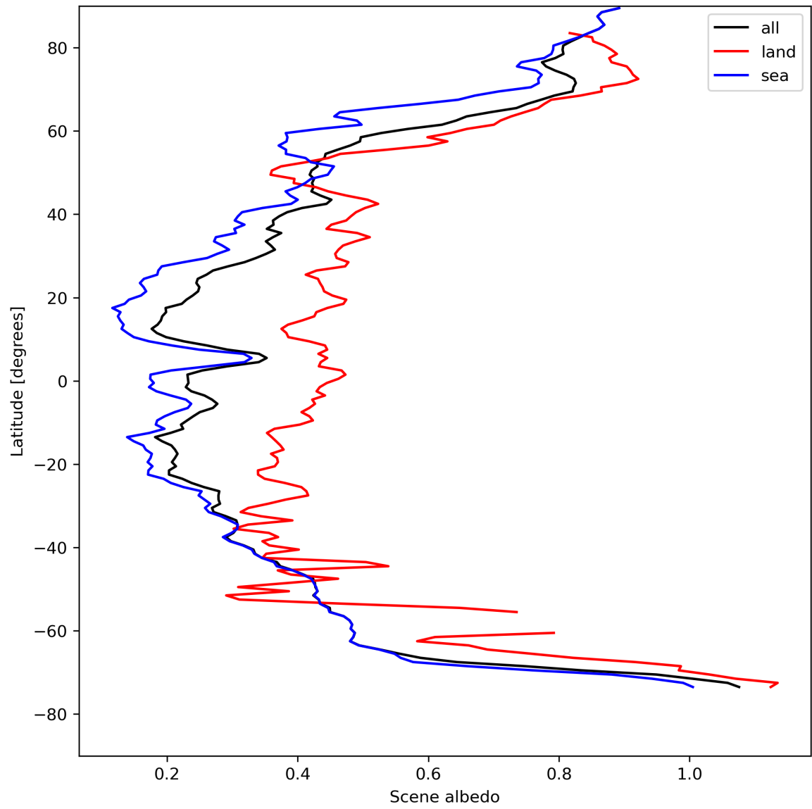
Figure 17: Zonal average of “Scene albedo” for 2024-04-27 to 2024-04-29.
