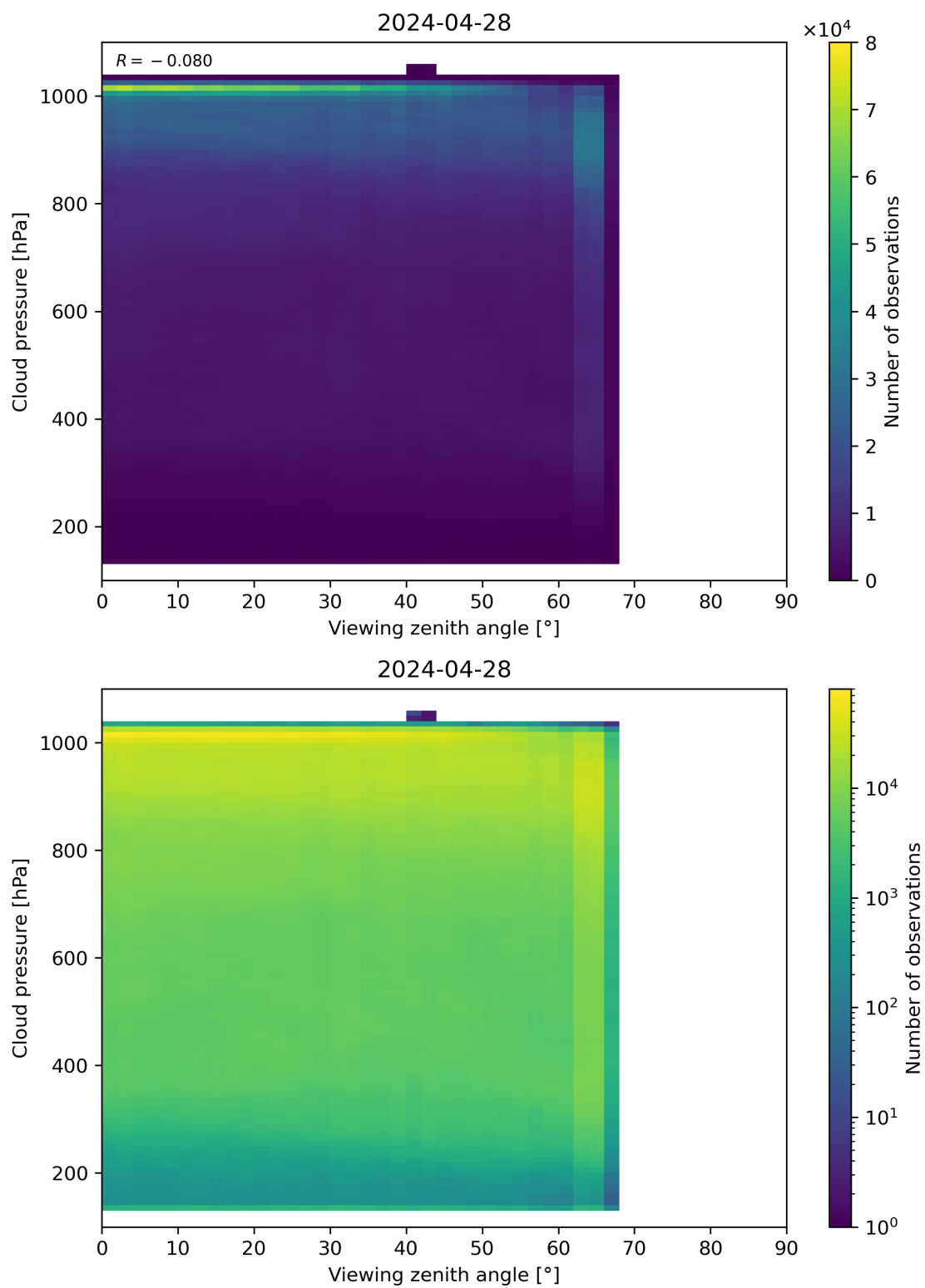
Figure 121: Scatter density plot of “Viewing zenith angle” against “Cloud pressure” for 2024-04-27 to 2024-04-29.
