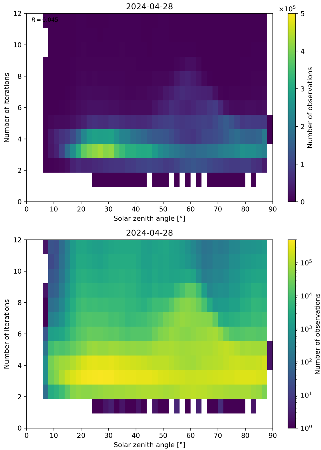
Figure 114: Scatter density plot of “Solar zenith angle” against “Number of iterations” for 2024-04-27 to 2024-04-29.
