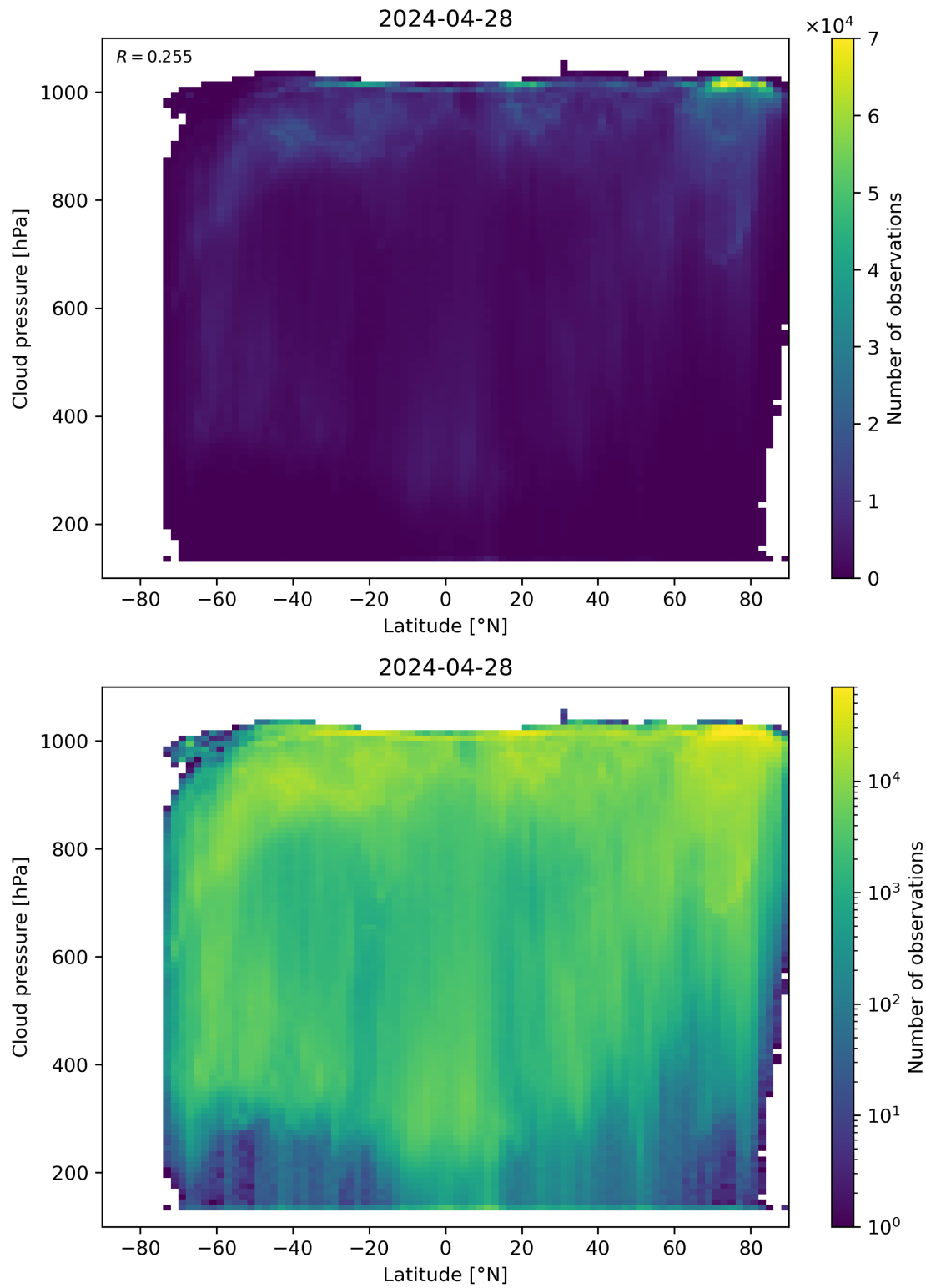
Figure 91: Scatter density plot of “Latitude” against “Cloud pressure” for 2024-04-27 to 2024-04-29.
