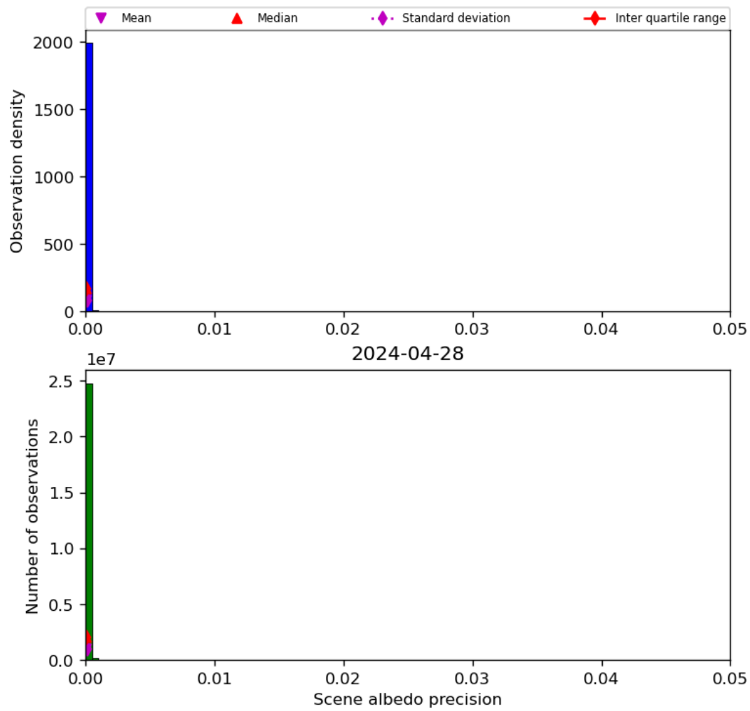
Figure 35: Histogram of “Scene albedo precision” for 2024-04-27 to 2024-04-29
