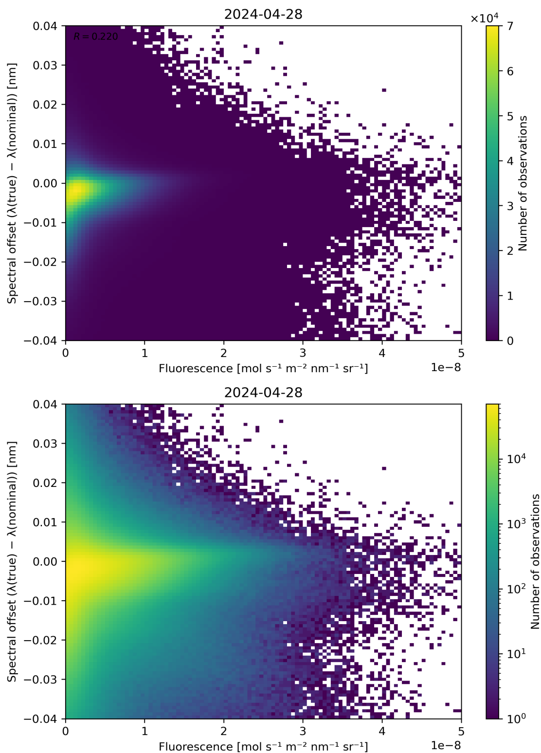
Figure 87: Scatter density plot of “Fluorescence” against “Spectral offset ( \lambda(\text{true}) - \lambda(\text{nominal}) )” for 2024-04-27 to 2024-04-29.
