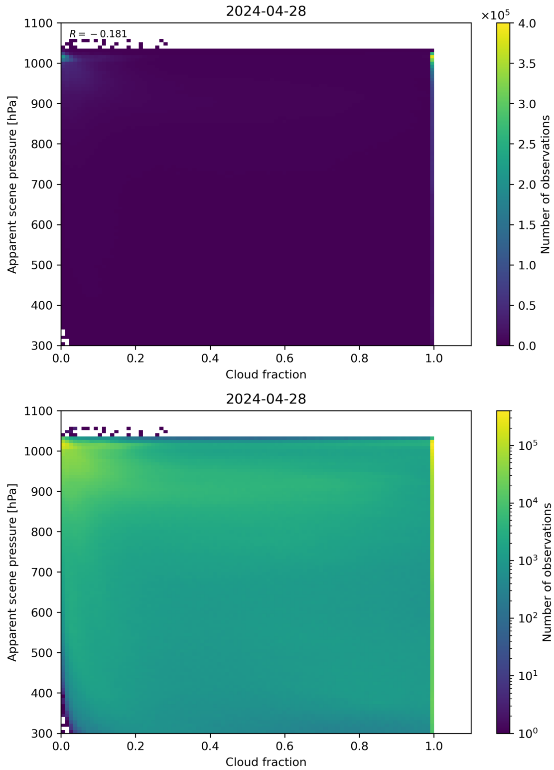
Figure 70: Scatter density plot of “Cloud fraction” against “Apparent scene pressure” for 2024-04-27 to 2024-04-29.
