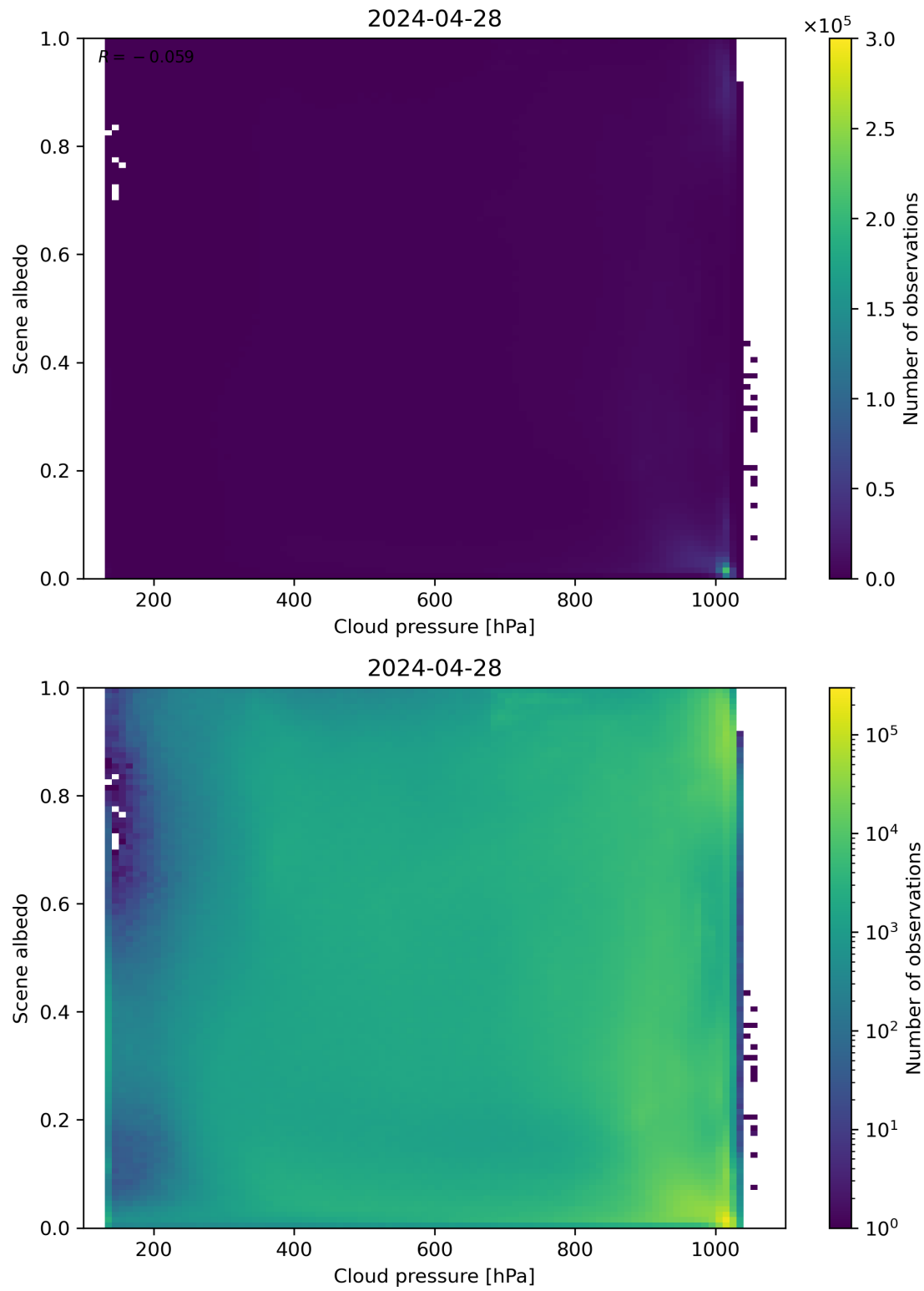
Figure 83: Scatter density plot of “Cloud pressure” against “Scene albedo” for 2024-04-27 to 2024-04-29.
