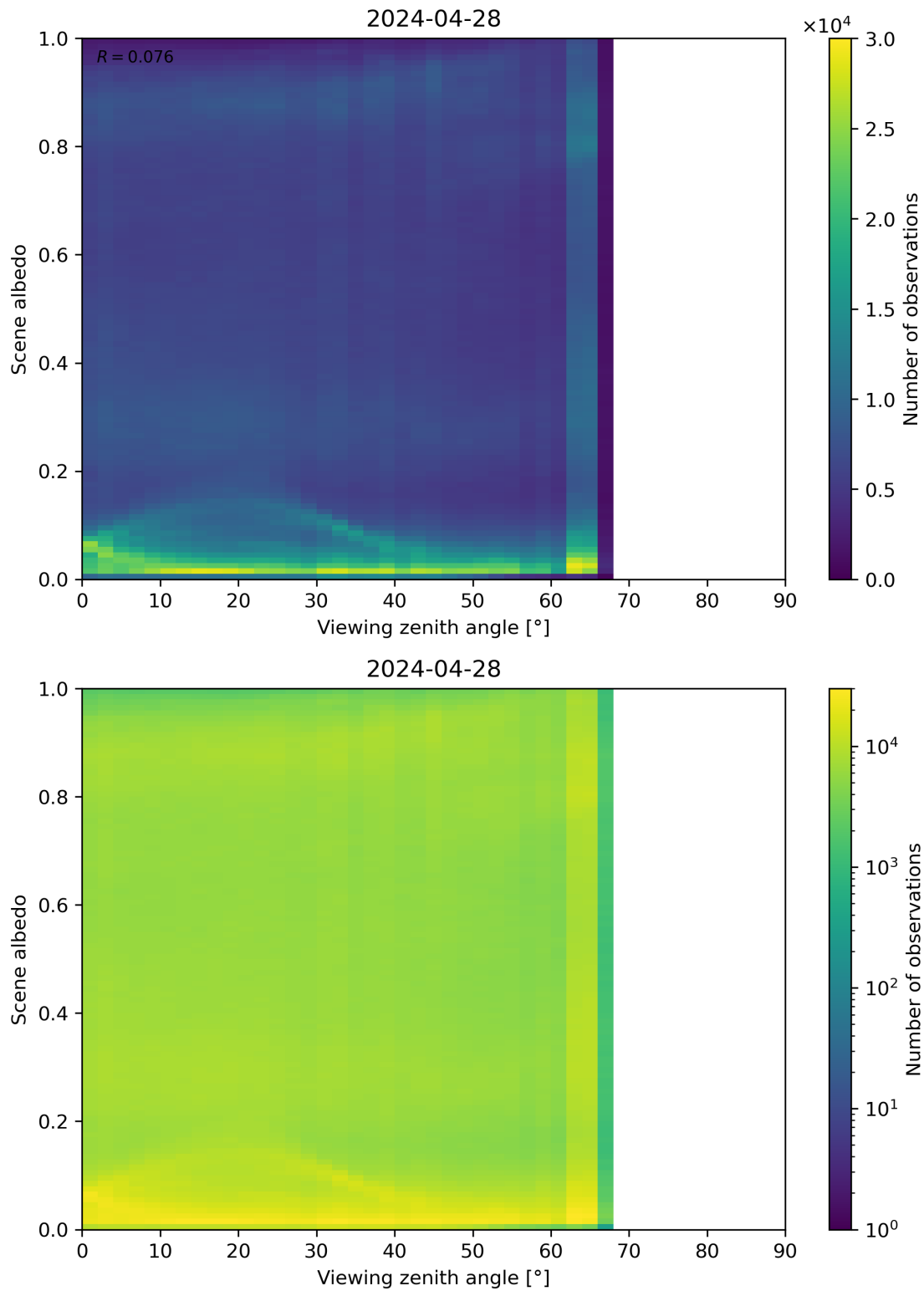
Figure 126: Scatter density plot of “Viewing zenith angle” against “Scene albedo” for 2024-04-27 to 2024-04-29.
