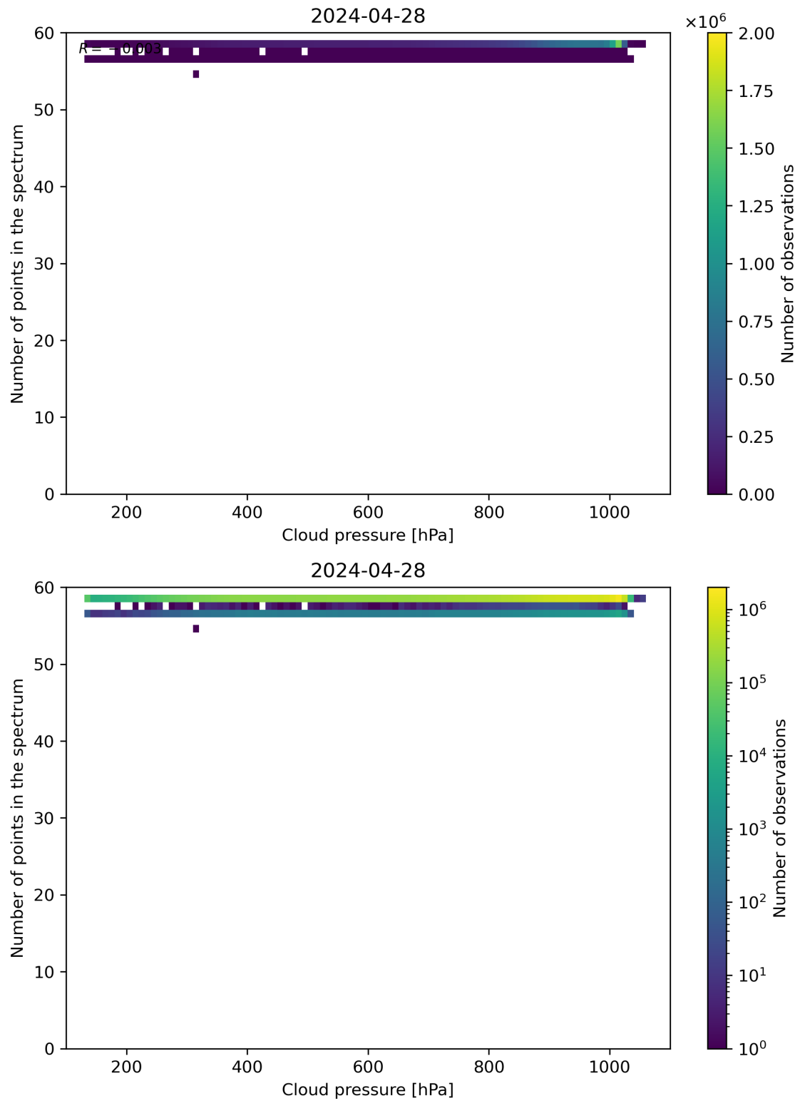
Figure 82: Scatter density plot of “Cloud pressure” against “Number of points in the spectrum” for 2024-04-27 to 2024-04-29.
