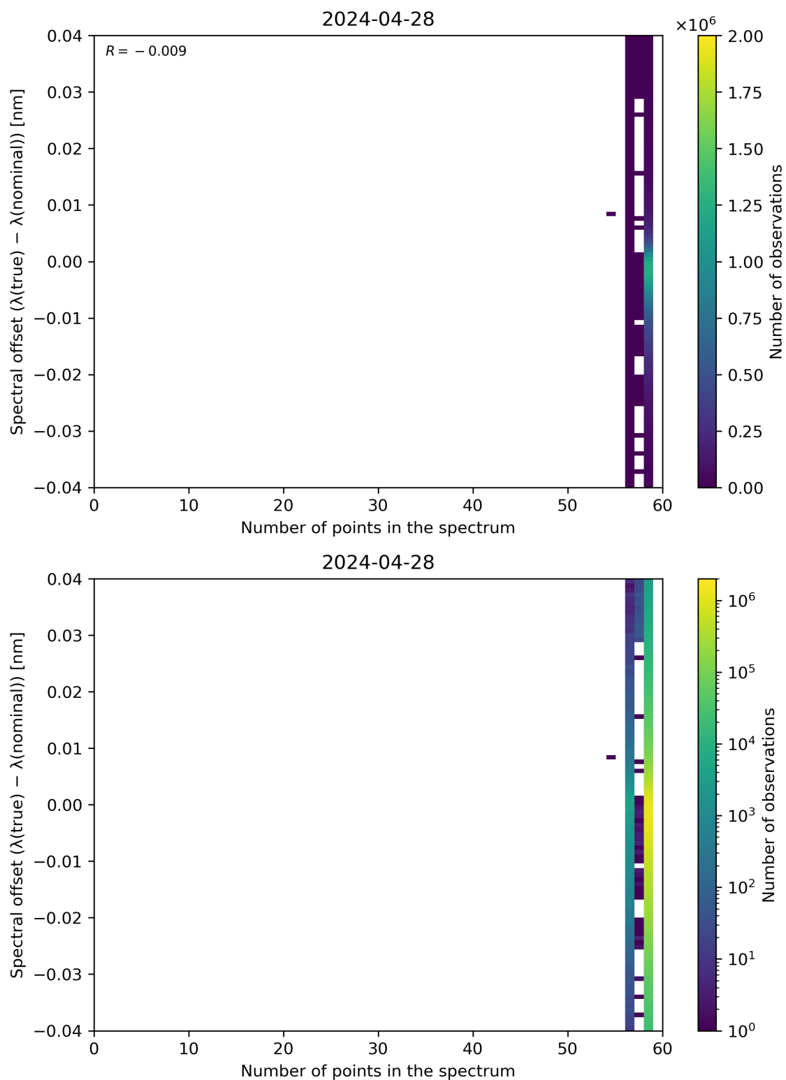
Figure 101: Scatter density plot of “Number of points in the spectrum” against “Spectral offset ( \lambda(\text{true}) - \lambda(\text{nominal}) )” for 2024-04-27 to 2024-04-29.
