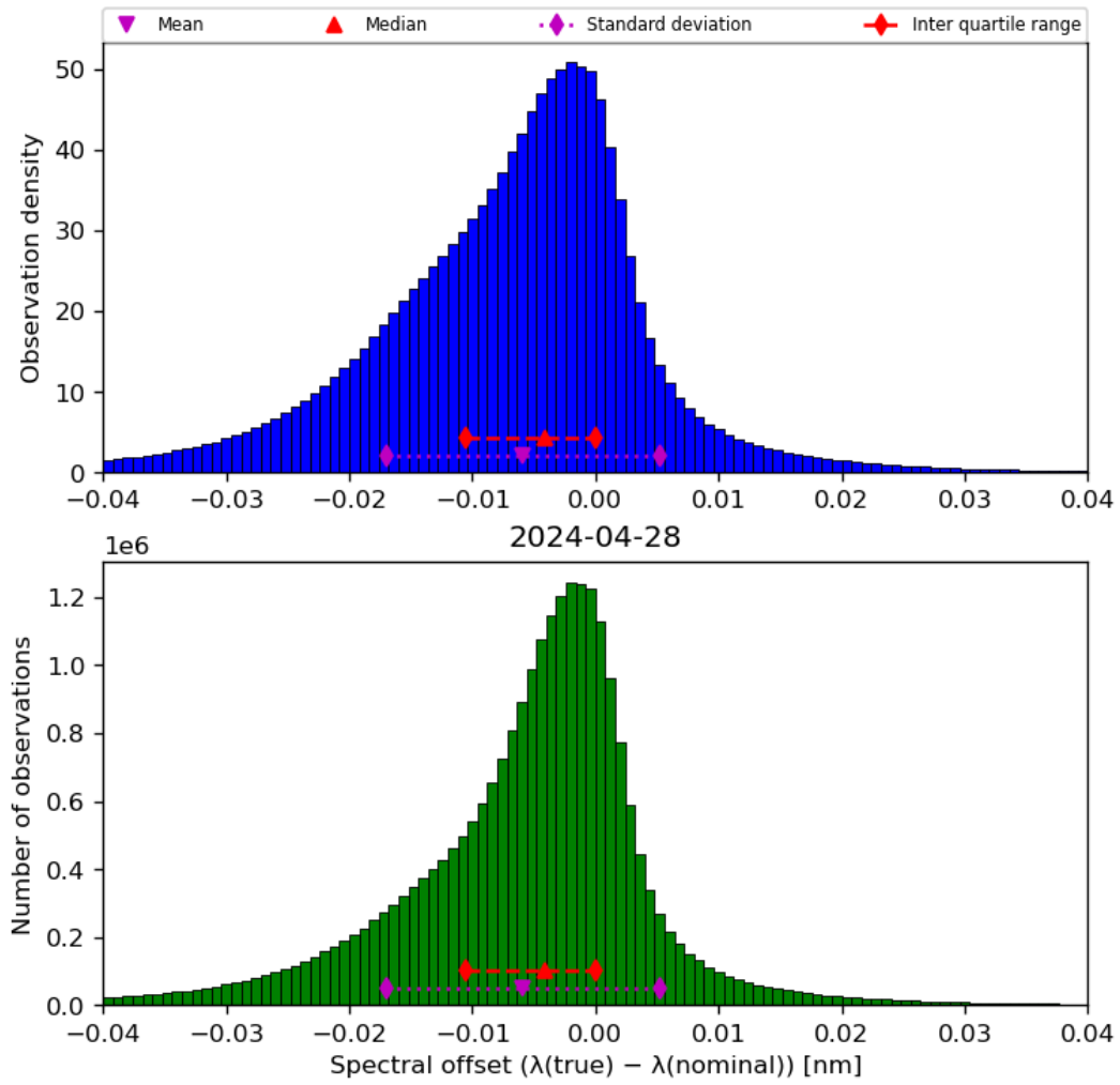
Figure 45: Histogram of “Spectral offset ( \lambda(\text{true}) - \lambda(\text{nominal}) )” for 2024-04-27 to 2024-04-29
