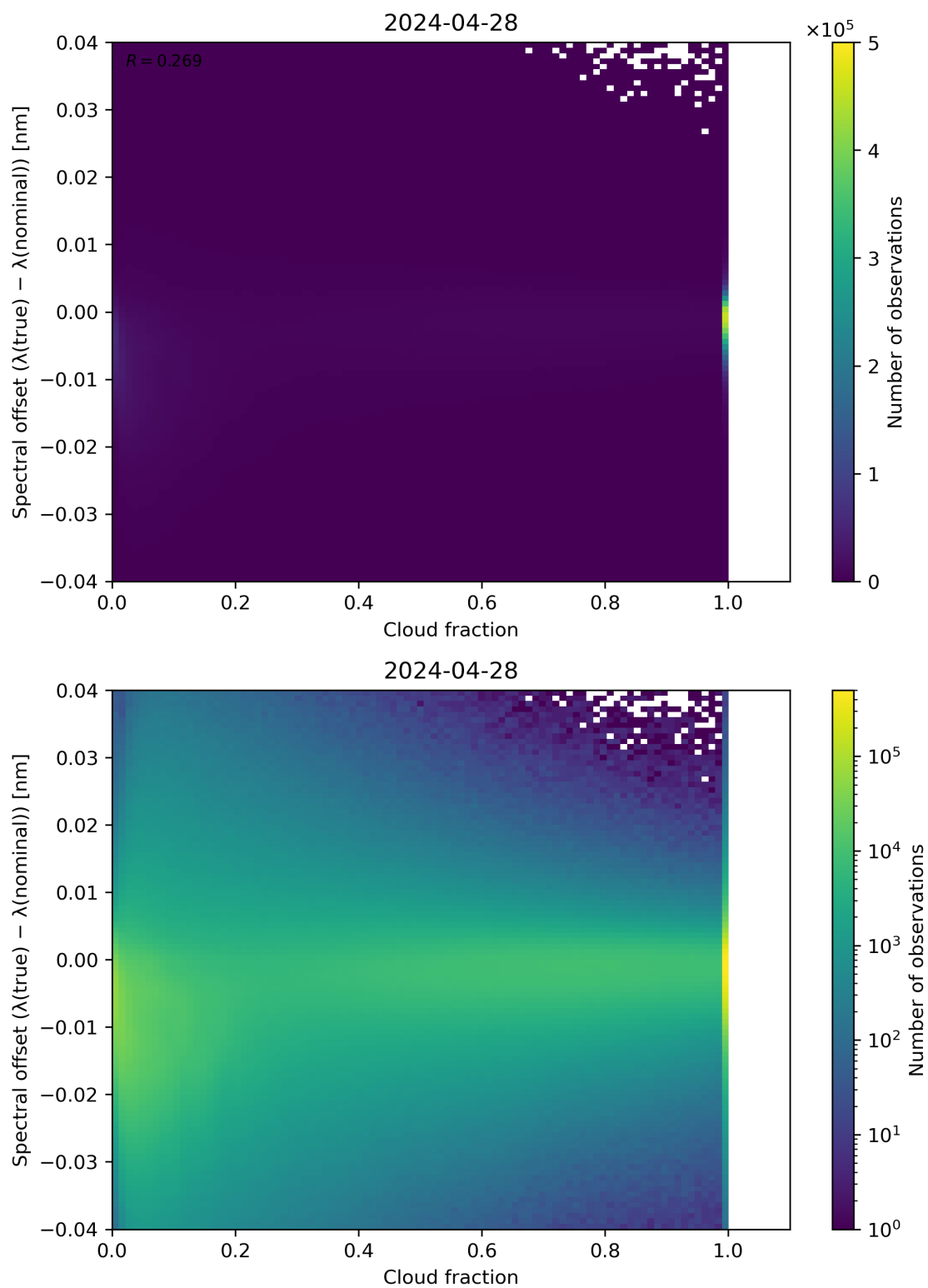
Figure 76: Scatter density plot of “Cloud fraction” against “Spectral offset ( \lambda(\text{true}) - \lambda(\text{nominal}) )” for 2024-04-27 to 2024-04-29.
