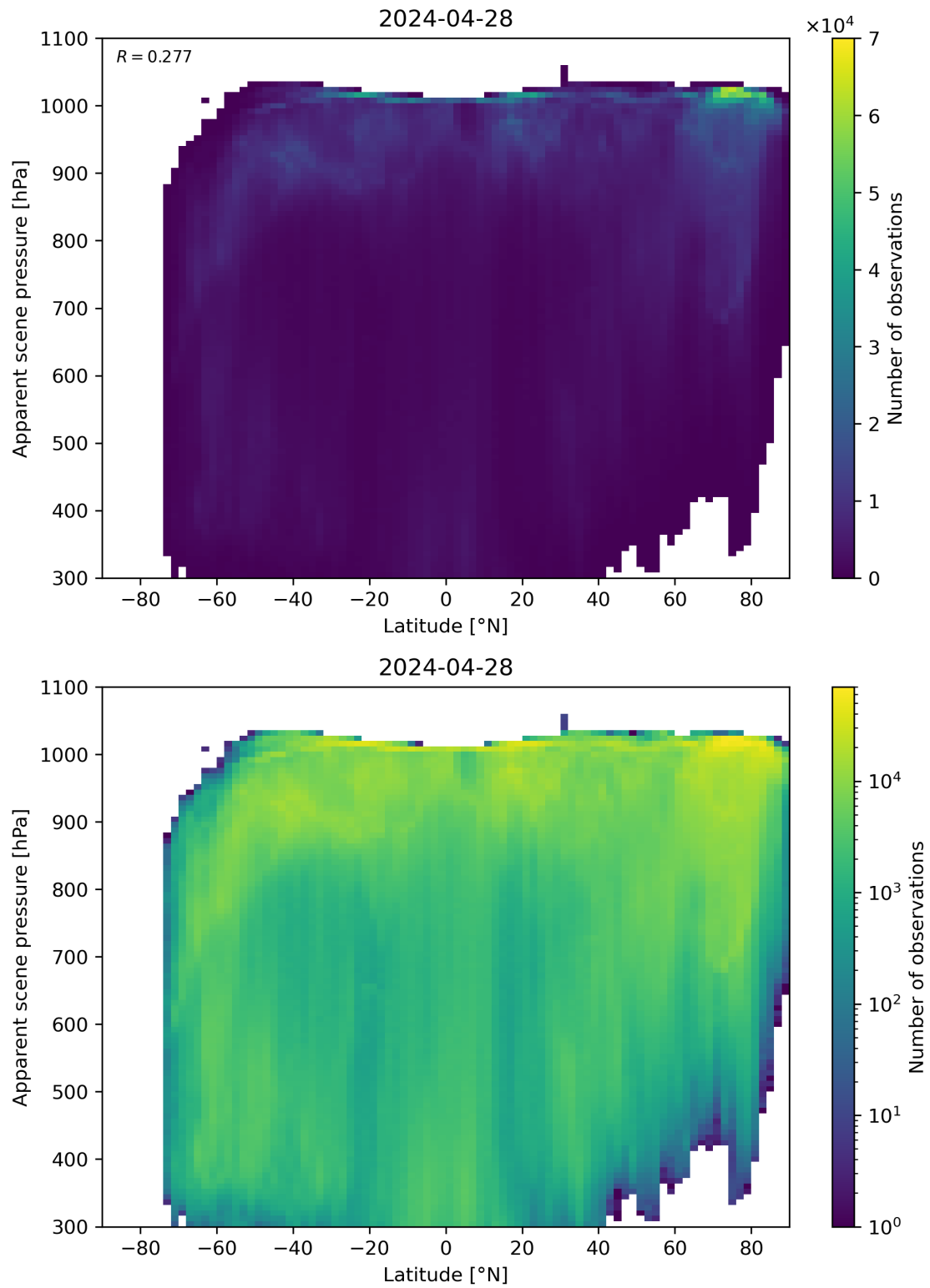
Figure 88: Scatter density plot of “Latitude” against “Apparent scene pressure” for 2024-04-27 to 2024-04-29.
