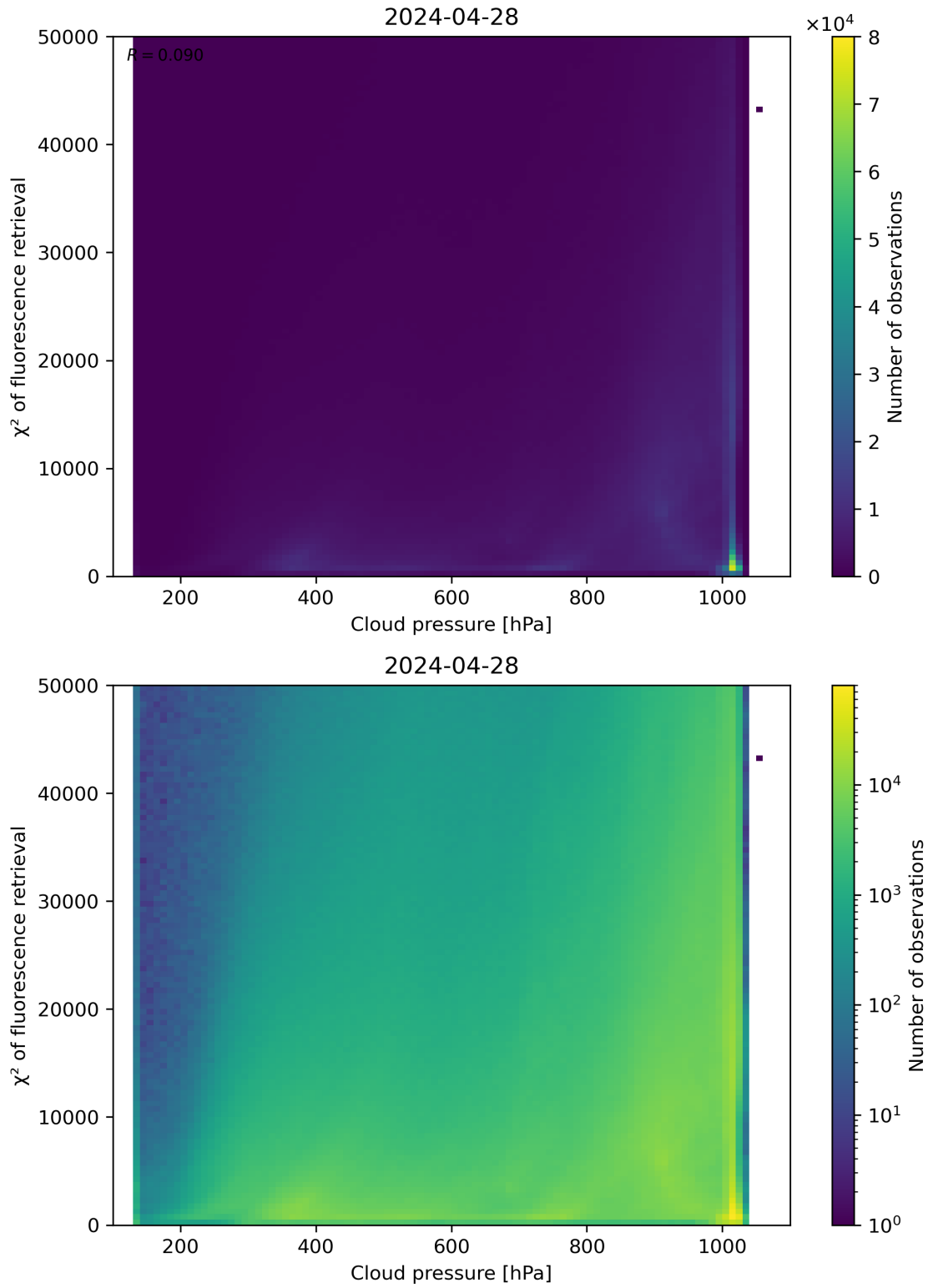
Figure 78: Scatter density plot of “Cloud pressure” against “ \chi^2 of fluorescence retrieval” for 2024-04-27 to 2024-04-29.
