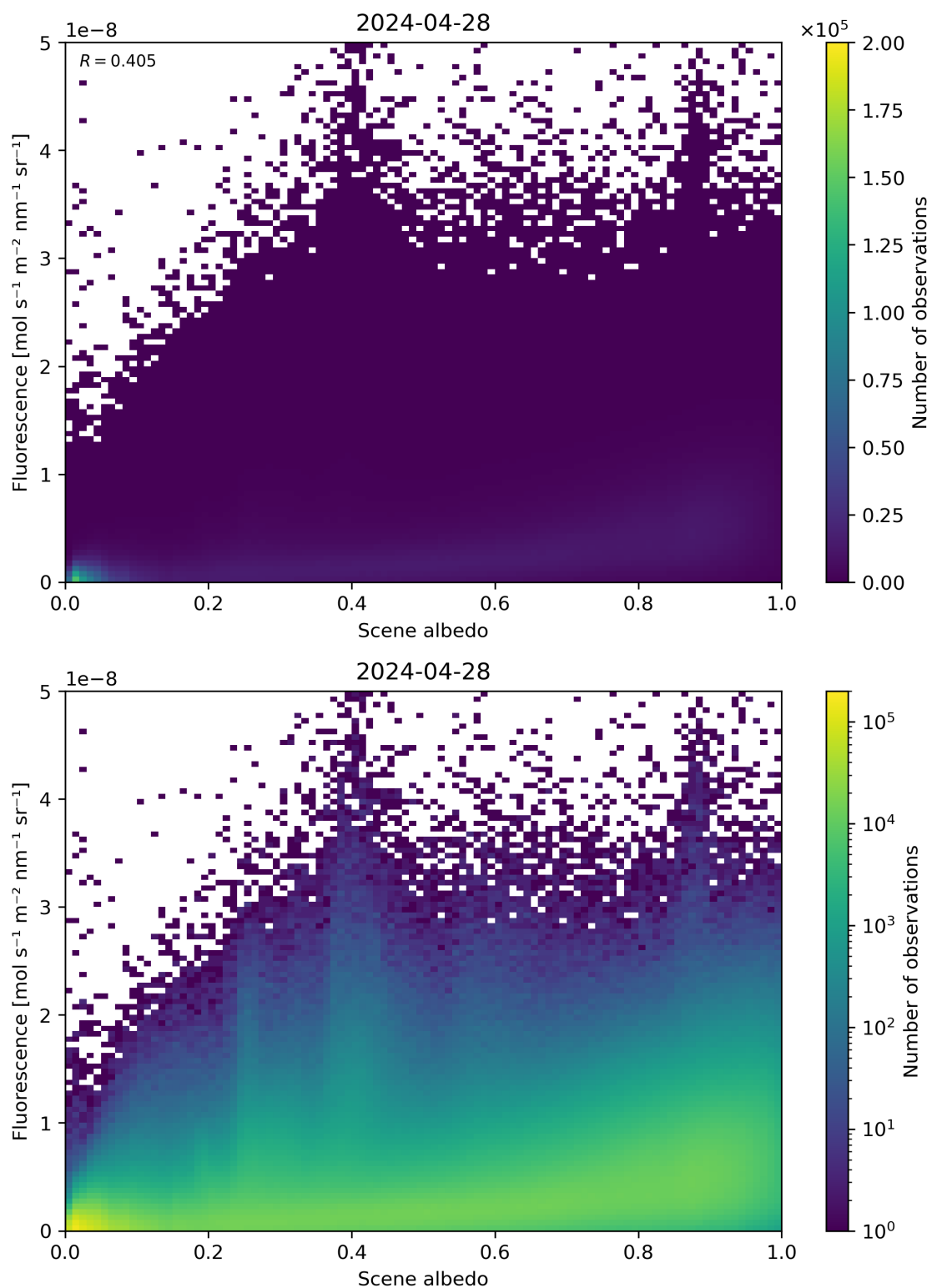
Figure 104: Scatter density plot of “Scene albedo” against “Fluorescence” for 2024-04-27 to 2024-04-29.
