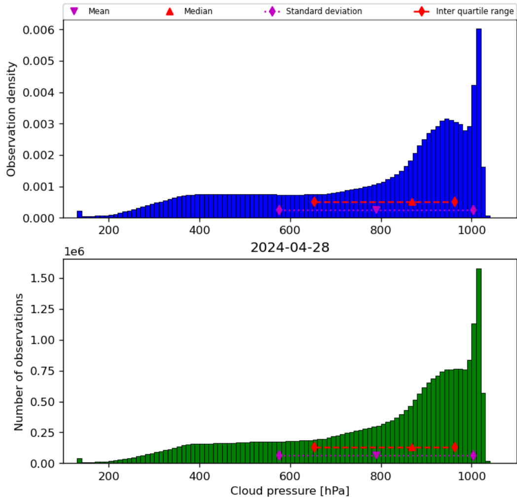
Figure 30: Histogram of “Cloud pressure” for 2024-04-27 to 2024-04-29
