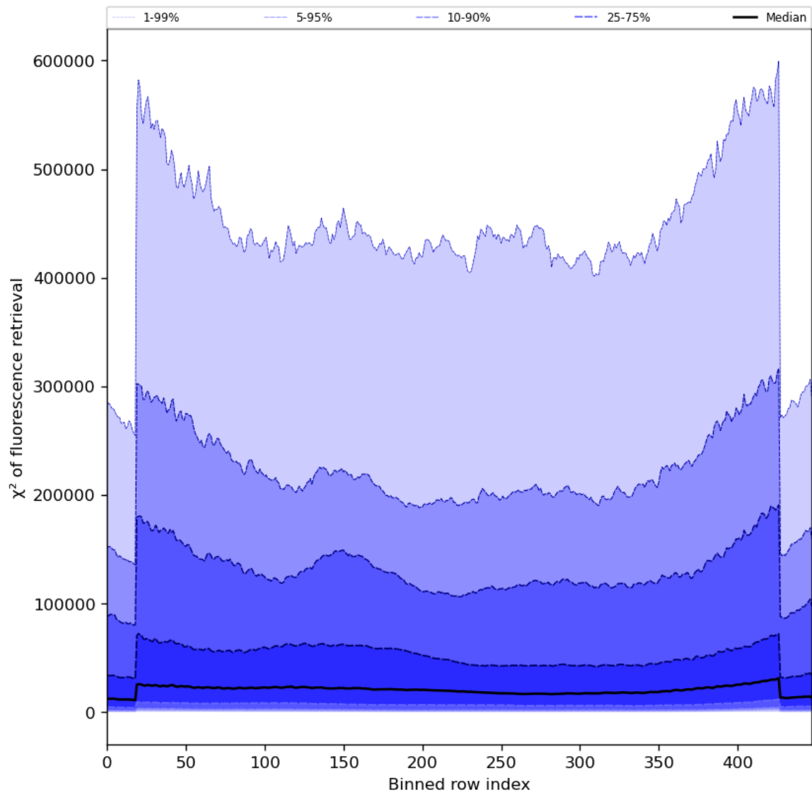
Figure 59: Along track statistics of “ \chi^2 of fluorescence retrieval” for 2024-04-27 to 2024-04-29
