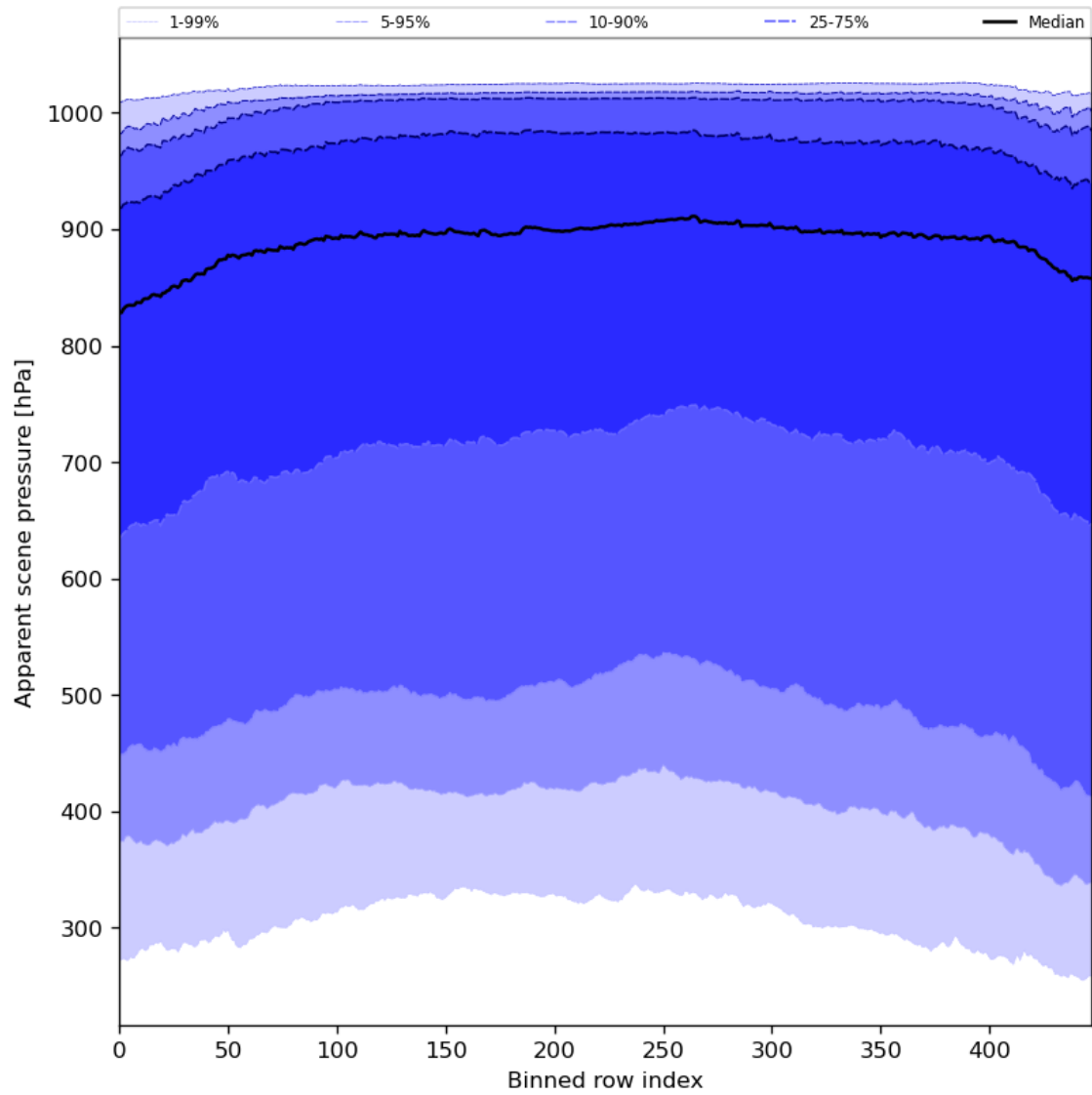
Figure 53: Along track statistics of “Apparent scene pressure” for 2024-04-27 to 2024-04-29
