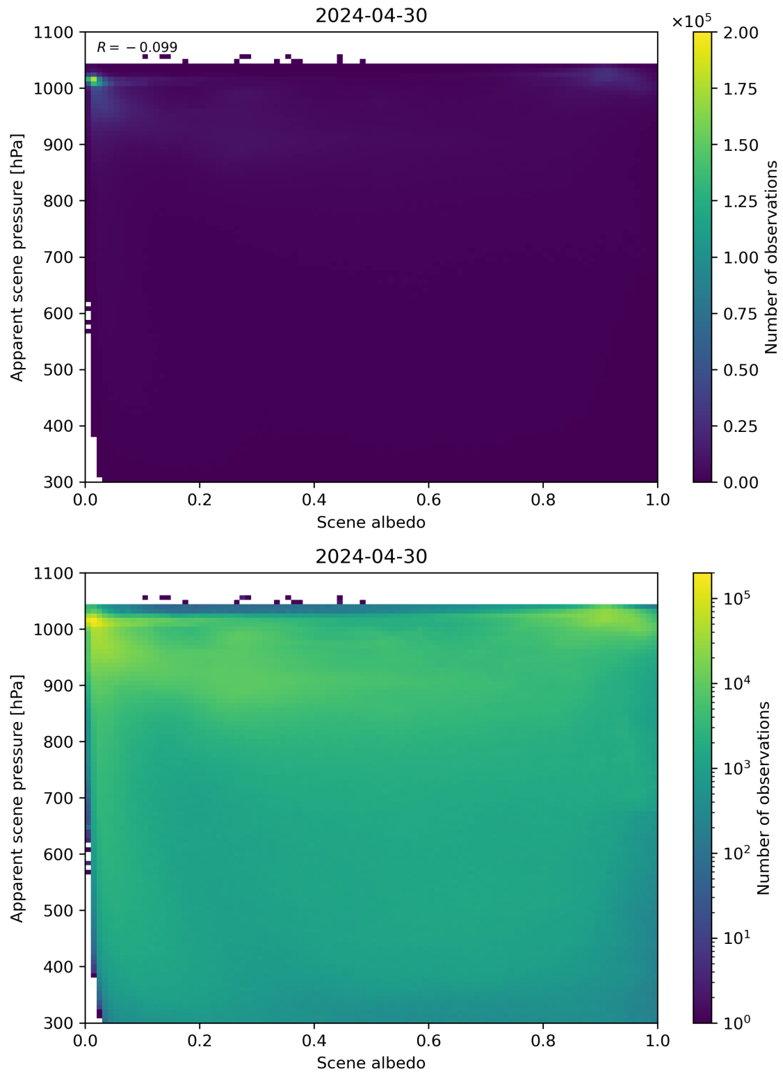
Figure 102: Scatter density plot of “Scene albedo” against “Apparent scene pressure” for 2024-04-29 to 2024-05-01.
