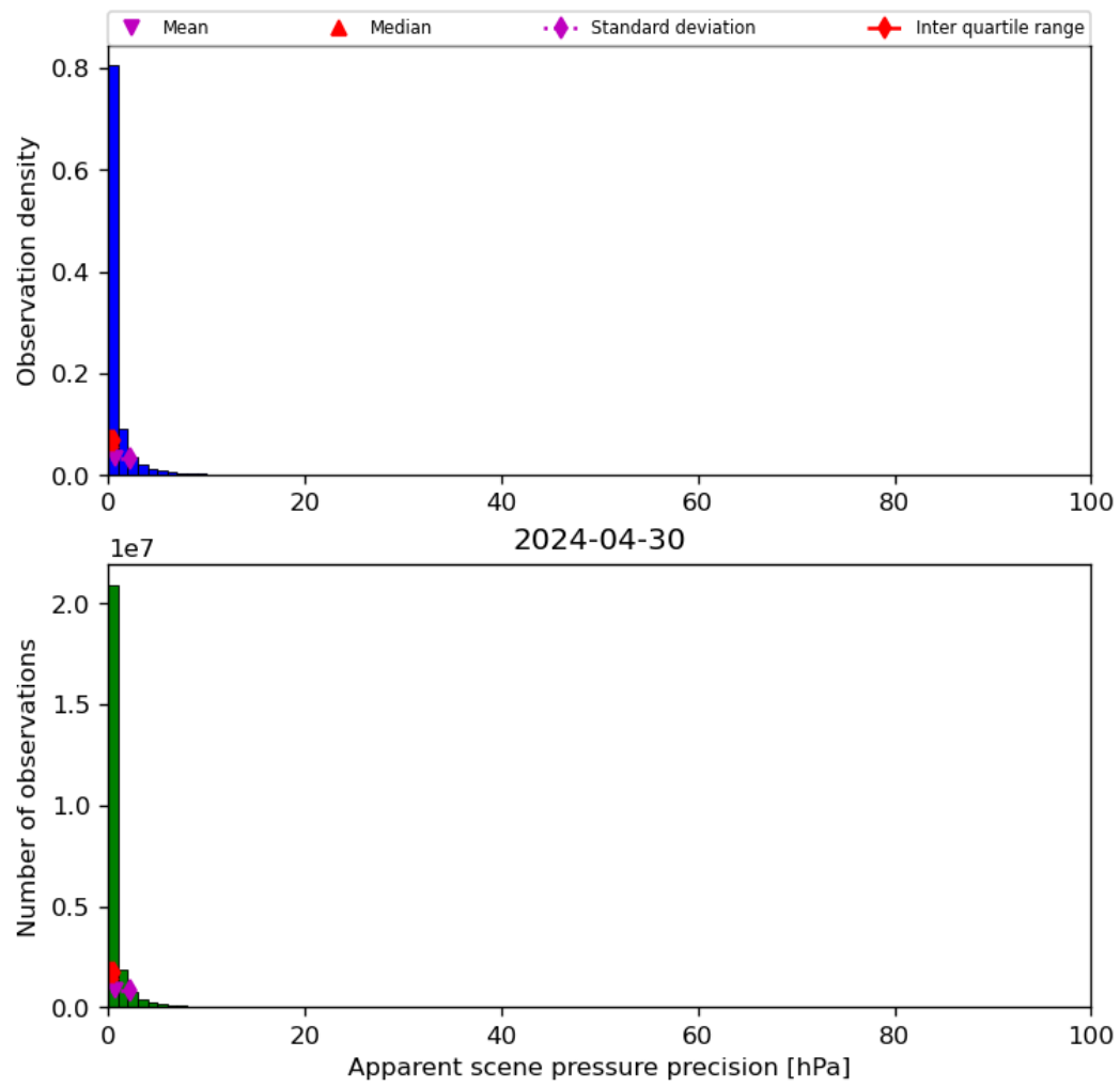
Figure 37: Histogram of “Apparent scene pressure precision” for 2024-04-29 to 2024-05-01
