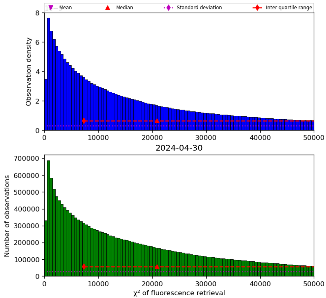
Figure 42: Histogram of “ \chi^2 of fluorescence retrieval” for 2024-04-29 to 2024-05-01
