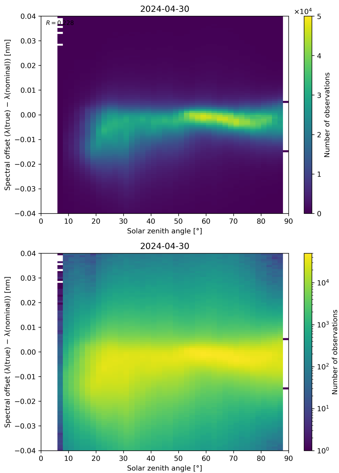
Figure 117: Scatter density plot of “Solar zenith angle” against “Spectral offset ( \lambda(\text{true}) - \lambda(\text{nominal}) )” for 2024-04-29 to 2024-05-01.
