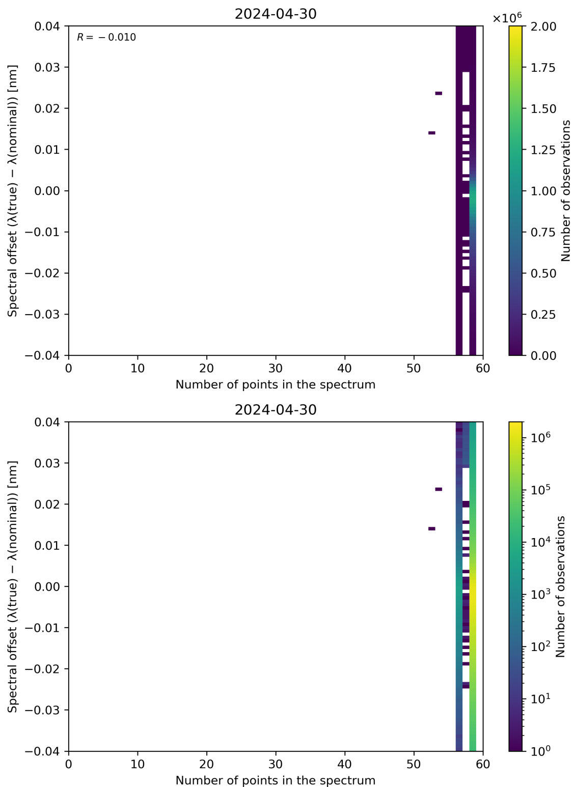
Figure 101: Scatter density plot of “Number of points in the spectrum” against “Spectral offset ( \lambda(\text{true}) - \lambda(\text{nominal}) )” for 2024-04-29 to 2024-05-01.
