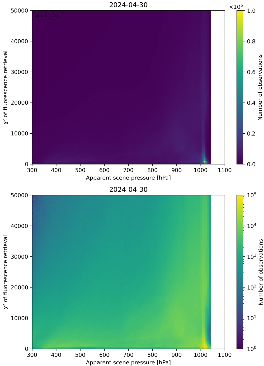
Figure 63: Scatter density plot of “Apparent scene pressure” against “ \chi^2 of fluorescence retrieval” for 2024-04-29 to 2024-05-01.
