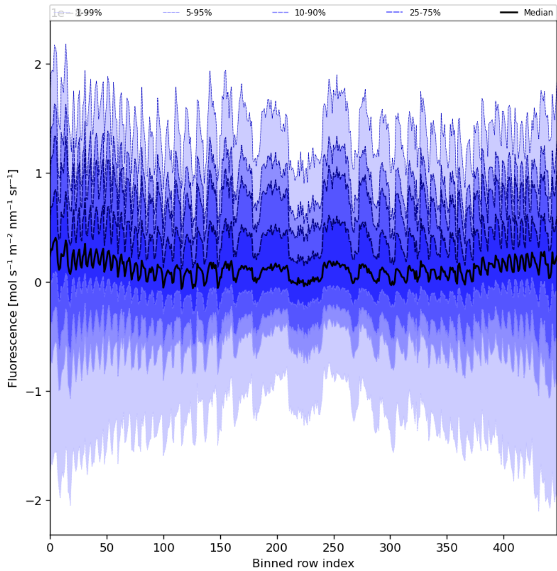
Figure 57: Along track statistics of “Fluorescence” for 2024-04-29 to 2024-05-01
