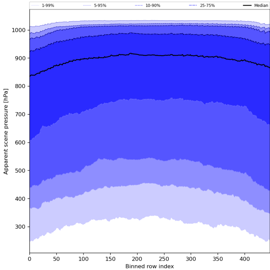
Figure 53: Along track statistics of “Apparent scene pressure” for 2024-04-29 to 2024-05-01
