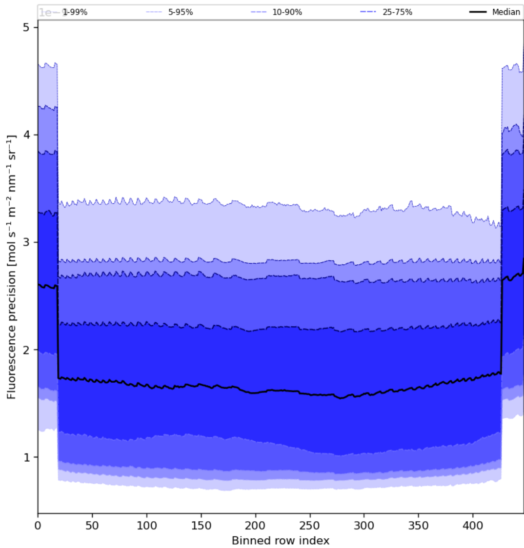
Figure 58: Along track statistics of “Fluorescence precision” for 2024-04-29 to 2024-05-01
