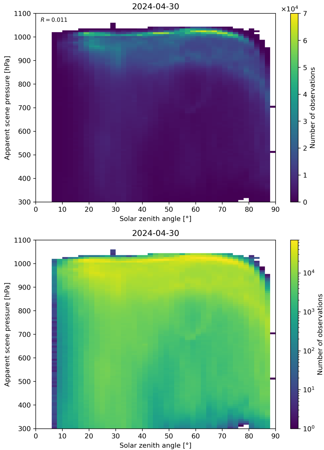
Figure 108: Scatter density plot of “Solar zenith angle” against “Apparent scene pressure” for 2024-04-29 to 2024-05-01.
