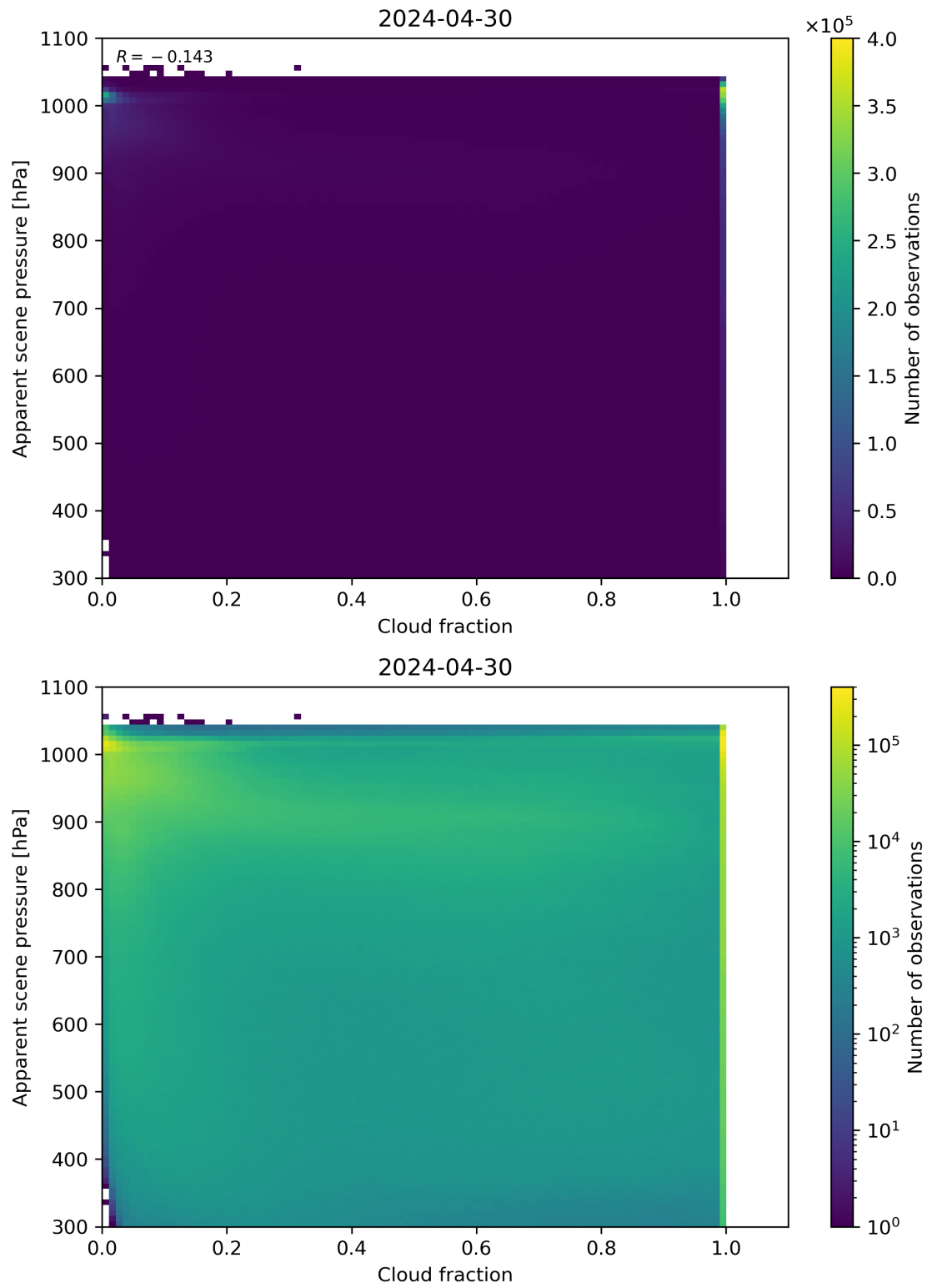
Figure 70: Scatter density plot of “Cloud fraction” against “Apparent scene pressure” for 2024-04-29 to 2024-05-01.
