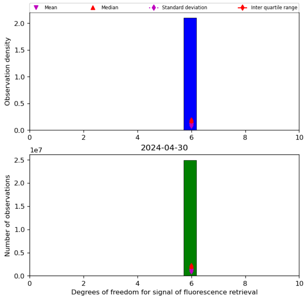
Figure 43: Histogram of “Degrees of freedom for signal of fluorescence retrieval” for 2024-04-29 to 2024-05-01
