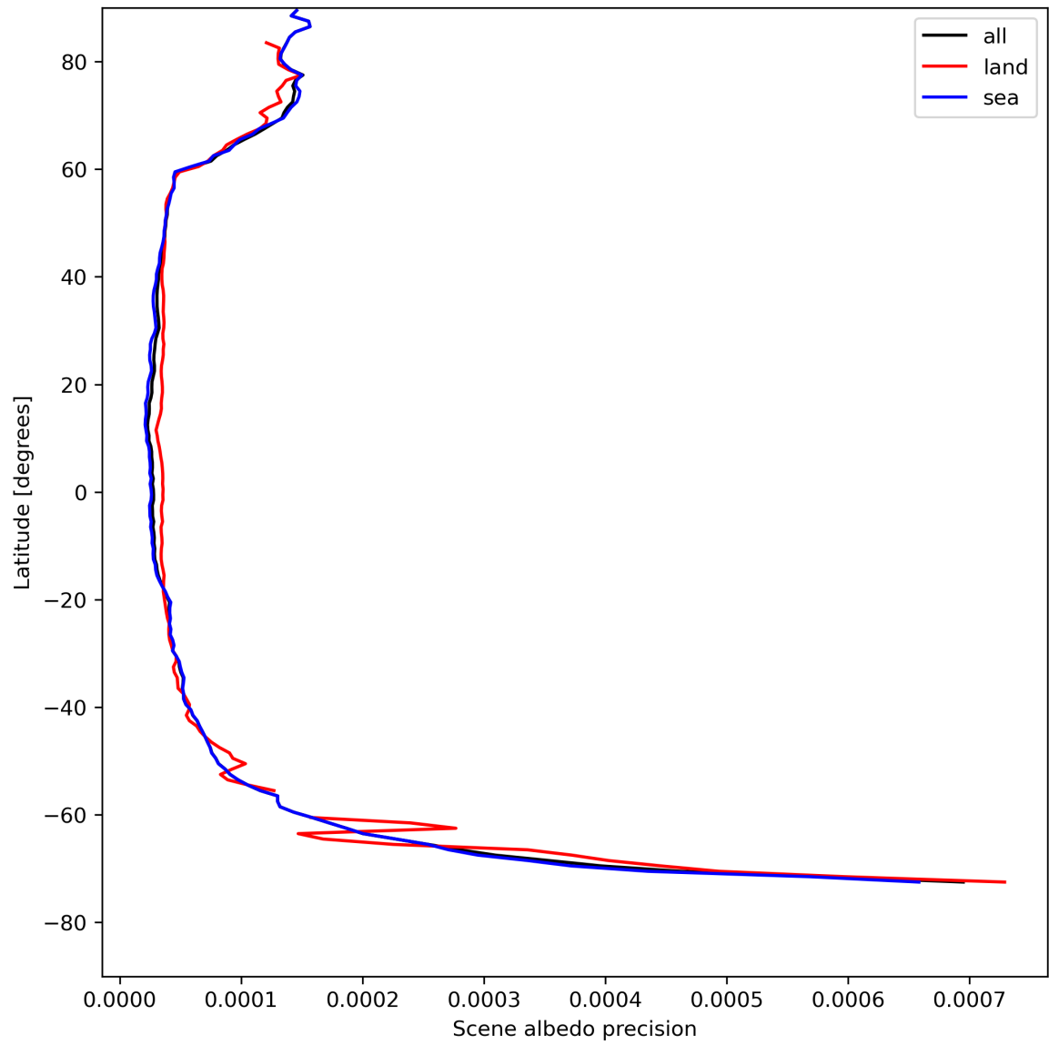
Figure 18: Zonal average of “Scene albedo precision” for 2024-04-29 to 2024-05-01.
