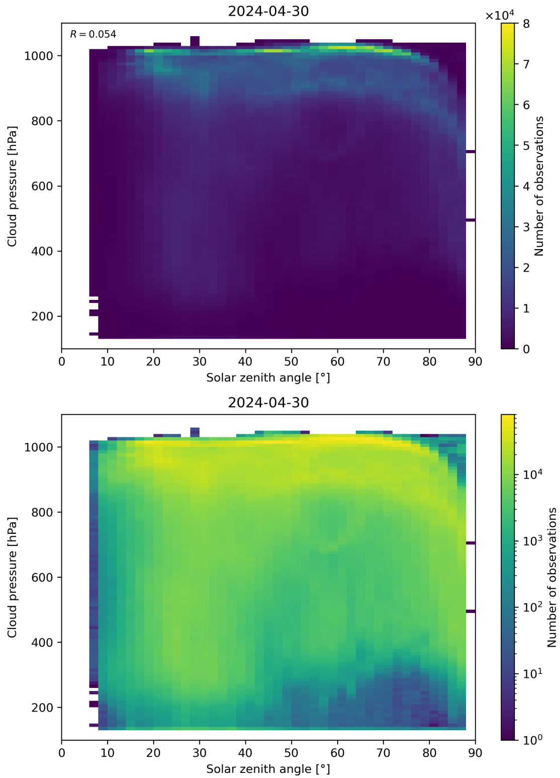
Figure 111: Scatter density plot of “Solar zenith angle” against “Cloud pressure” for 2024-04-29 to 2024-05-01.
