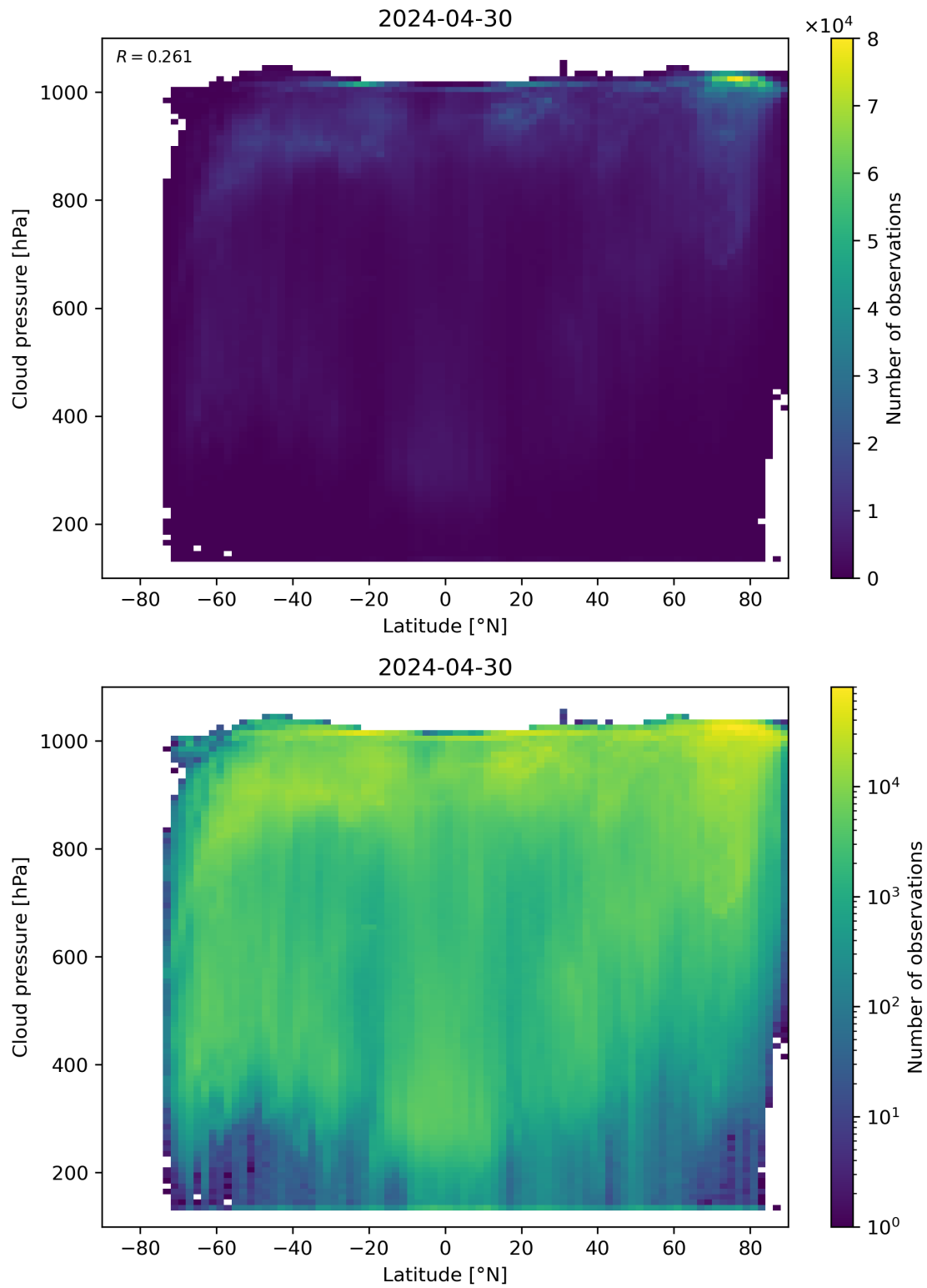
Figure 91: Scatter density plot of “Latitude” against “Cloud pressure” for 2024-04-29 to 2024-05-01.
