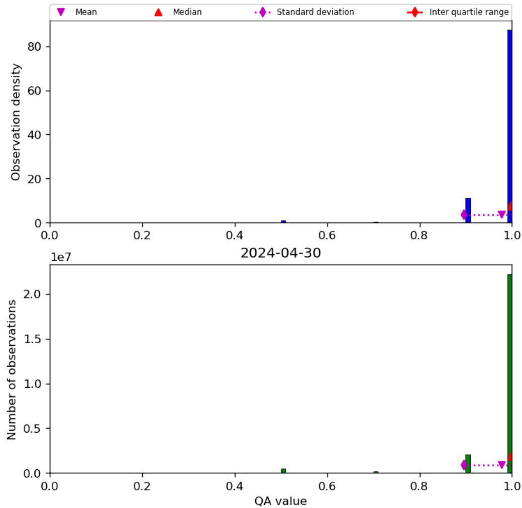
Figure 29: Histogram of “QA value” for 2024-04-29 to 2024-05-01
