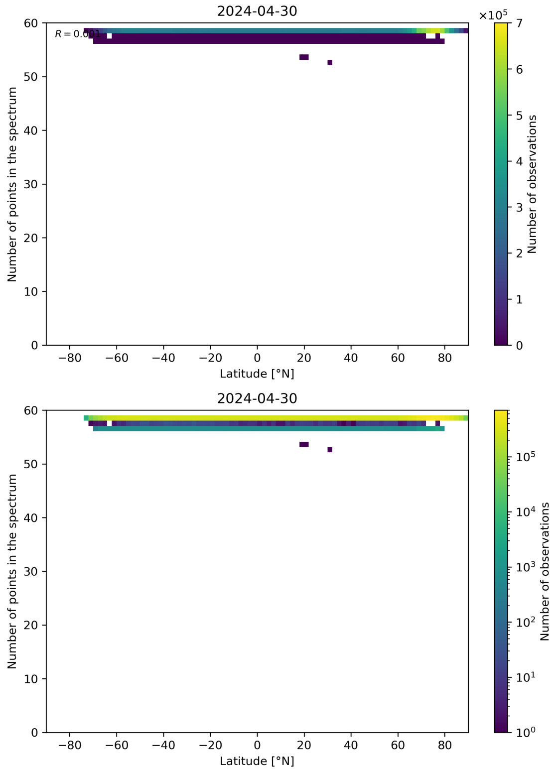
Figure 94: Scatter density plot of “Latitude” against “Number of points in the spectrum” for 2024-04-29 to 2024-05-01.
