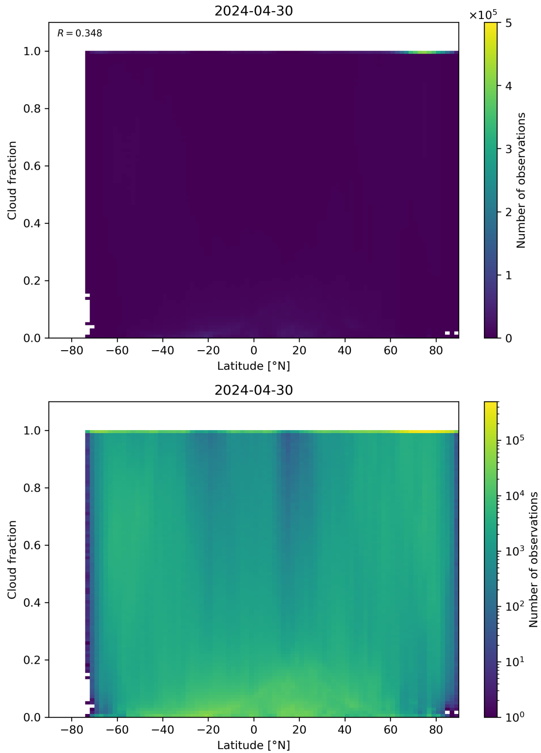
Figure 90: Scatter density plot of “Latitude” against “Cloud fraction” for 2024-04-29 to 2024-05-01.
