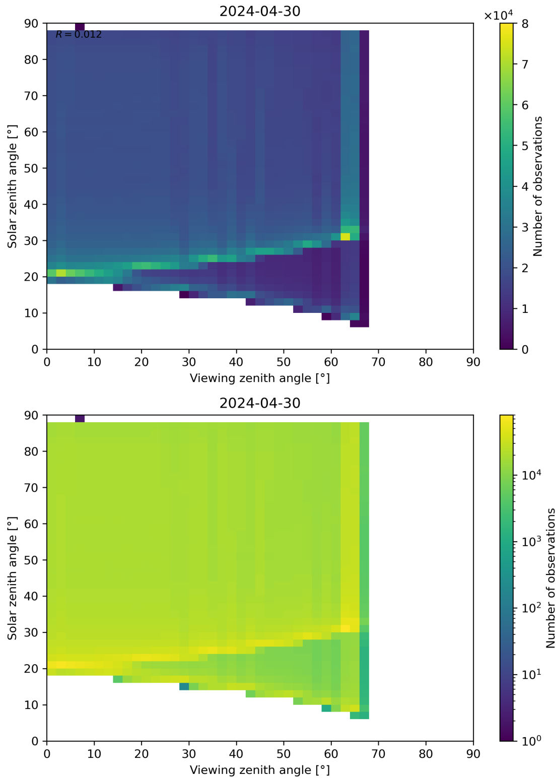
Figure 127: Scatter density plot of “Viewing zenith angle” against “Solar zenith angle” for 2024-04-29 to 2024-05-01.
