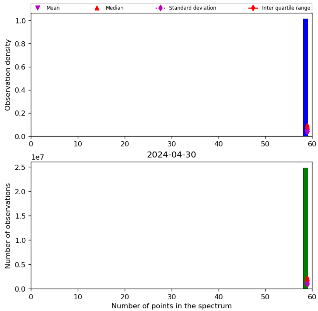
Figure 44: Histogram of “Number of points in the spectrum” for 2024-04-29 to 2024-05-01
