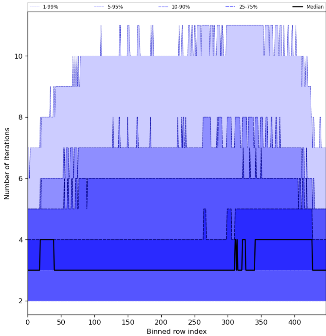
Figure 56: Along track statistics of “Number of iterations” for 2024-04-29 to 2024-05-01
