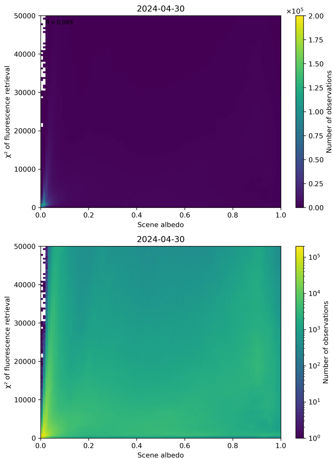
Figure 103: Scatter density plot of “Scene albedo” against “ \chi^2 of fluorescence retrieval” for 2024-04-29 to 2024-05-01.
