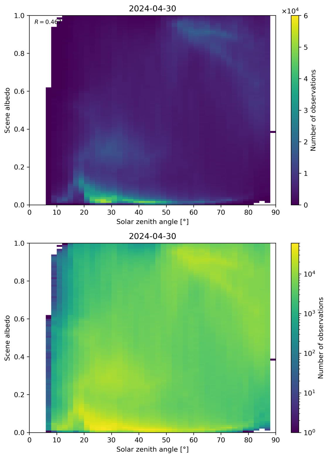
Figure 116: Scatter density plot of “Solar zenith angle” against “Scene albedo” for 2024-04-29 to 2024-05-01.
