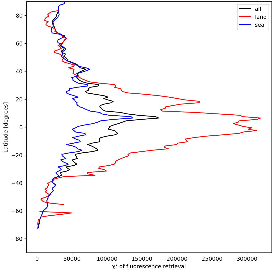
Figure 25: Zonal average of “ \chi^2 of fluorescence retrieval” for 2024-04-29 to 2024-05-01.
