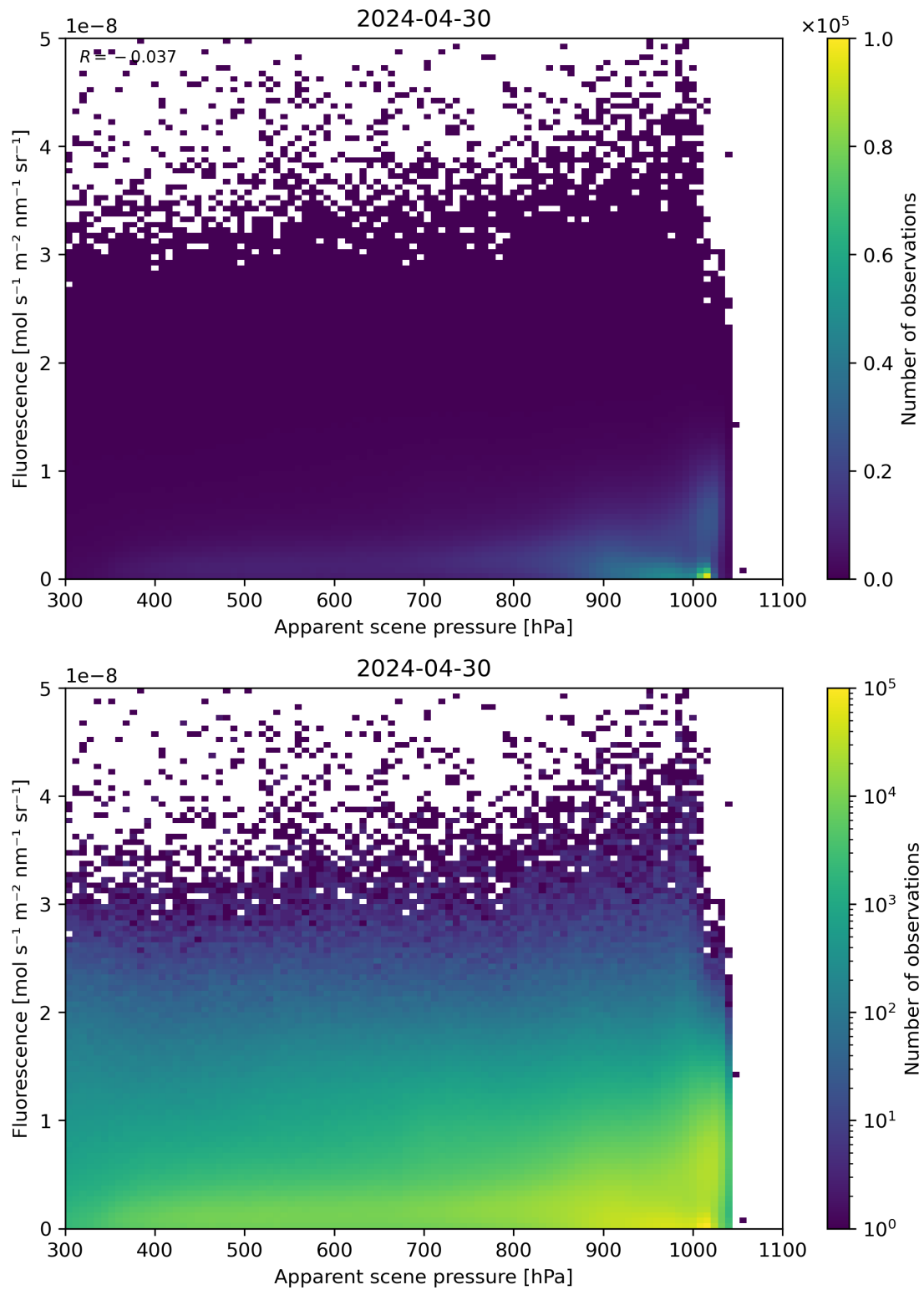
Figure 64: Scatter density plot of “Apparent scene pressure” against “Fluorescence” for 2024-04-29 to 2024-05-01.
