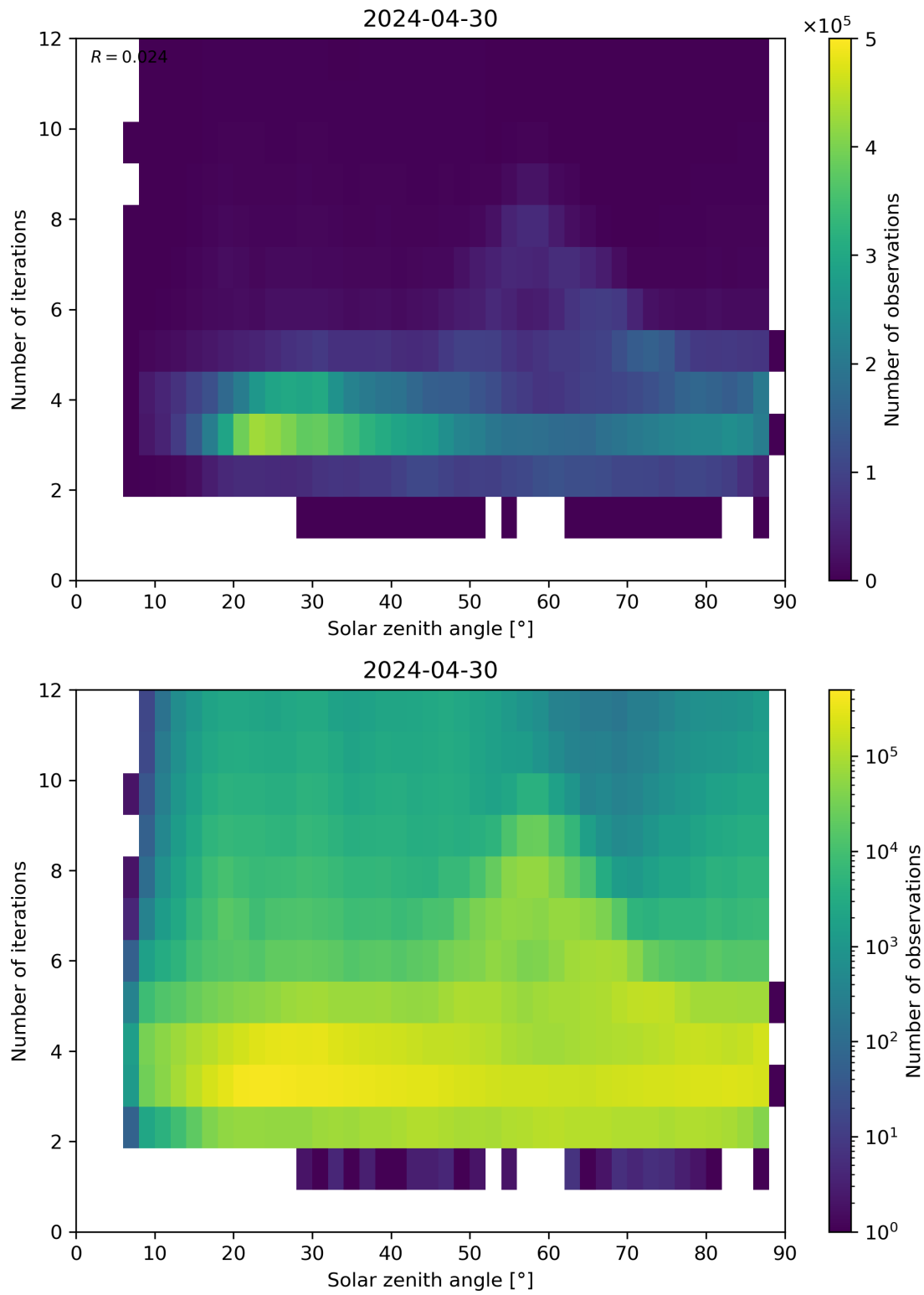
Figure 114: Scatter density plot of “Solar zenith angle” against “Number of iterations” for 2024-04-29 to 2024-05-01.
