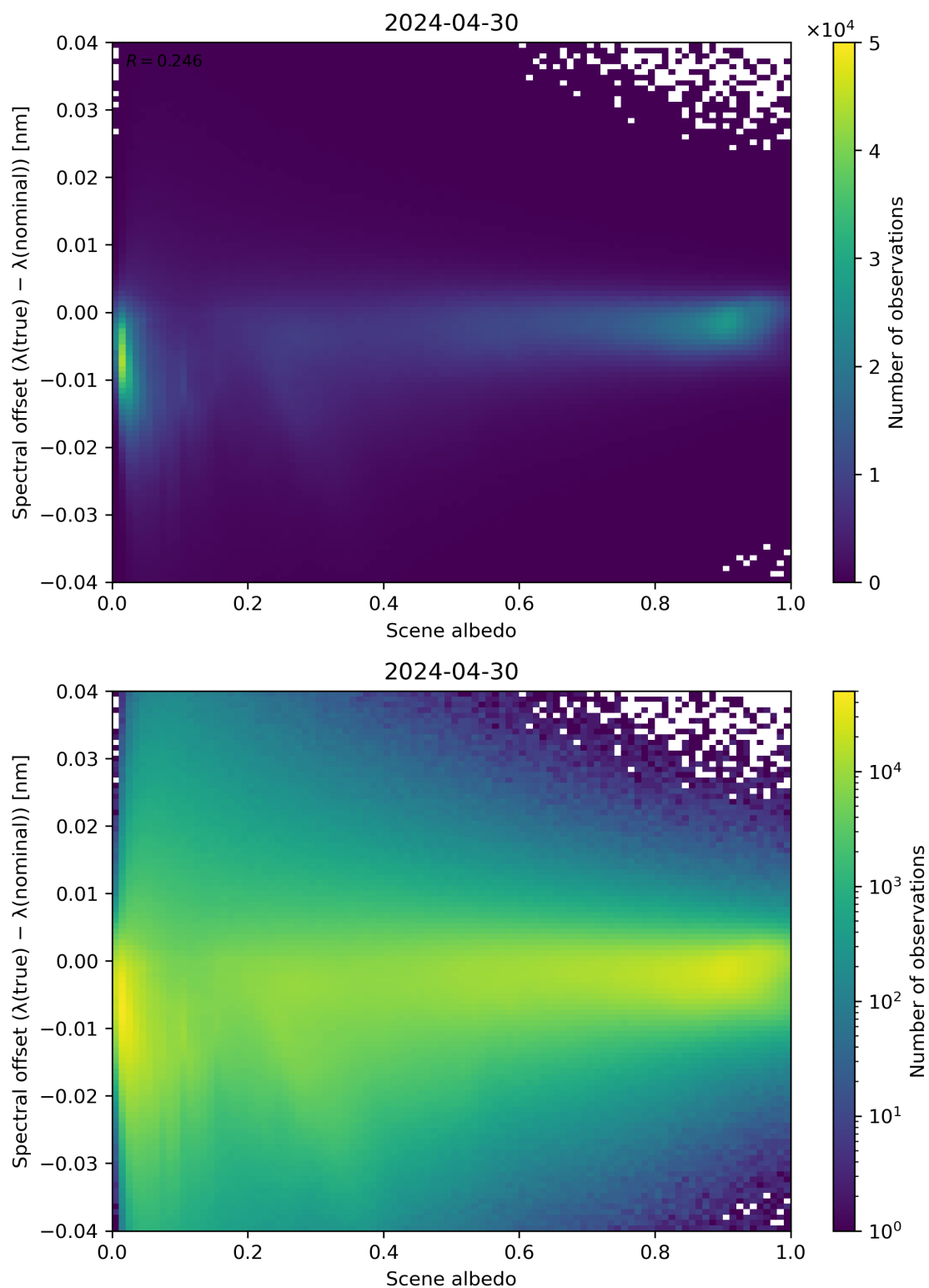
Figure 107: Scatter density plot of “Scene albedo” against “Spectral offset ( \lambda(\text{true}) - \lambda(\text{nominal}) )” for 2024-04-29 to 2024-05-01.
