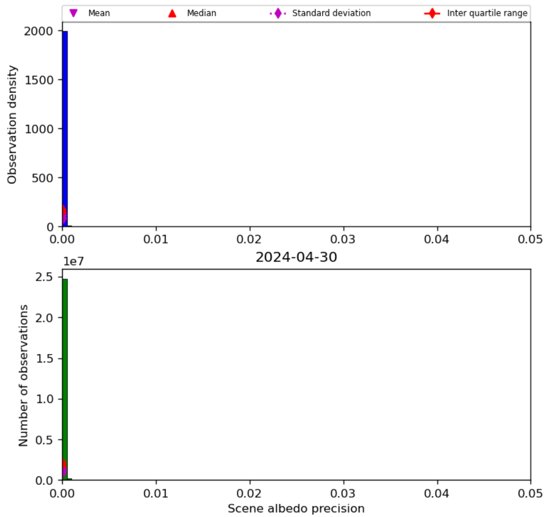
Figure 35: Histogram of “Scene albedo precision” for 2024-04-29 to 2024-05-01
