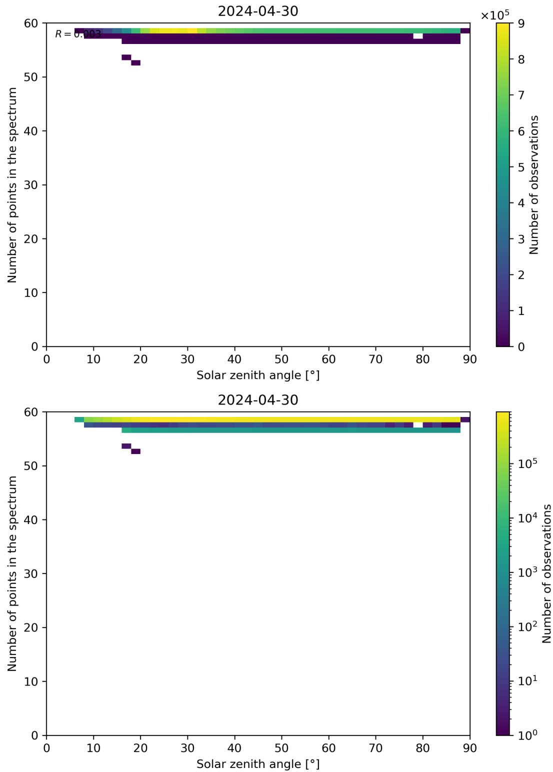
Figure 115: Scatter density plot of “Solar zenith angle” against “Number of points in the spectrum” for 2024-04-29 to 2024-05-01.
