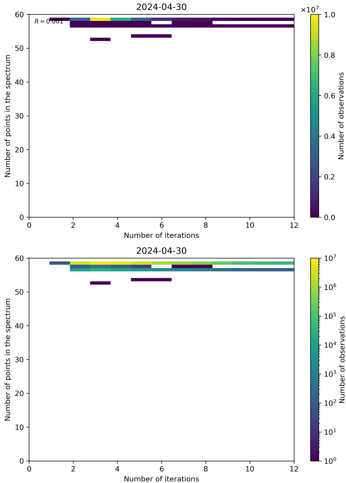
Figure 99: Scatter density plot of “Number of iterations” against “Number of points in the spectrum” for 2024-04-29 to 2024-05-01.
