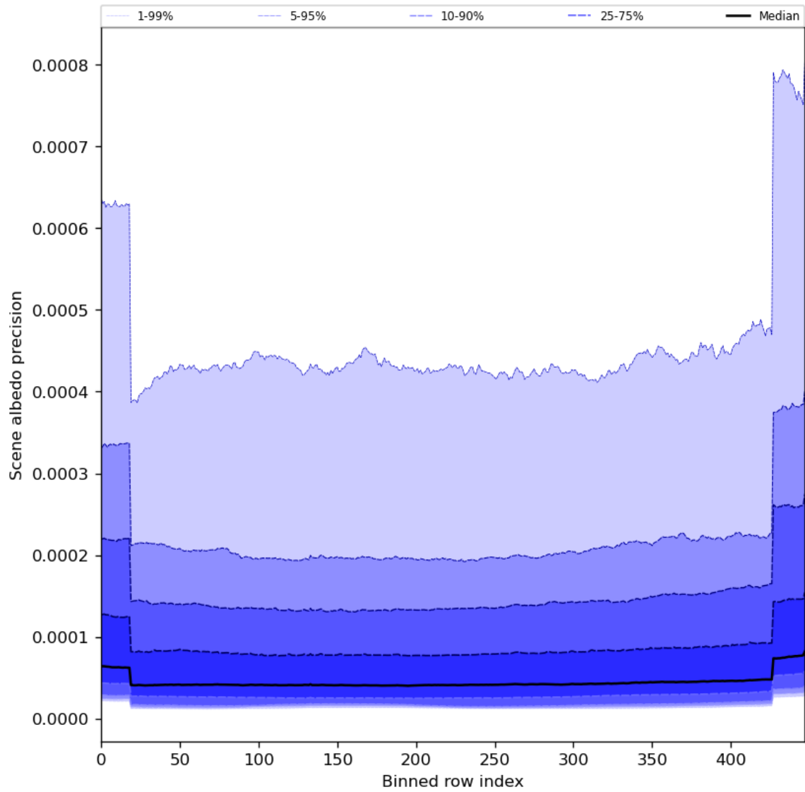
Figure 52: Along track statistics of “Scene albedo precision” for 2024-04-29 to 2024-05-01
