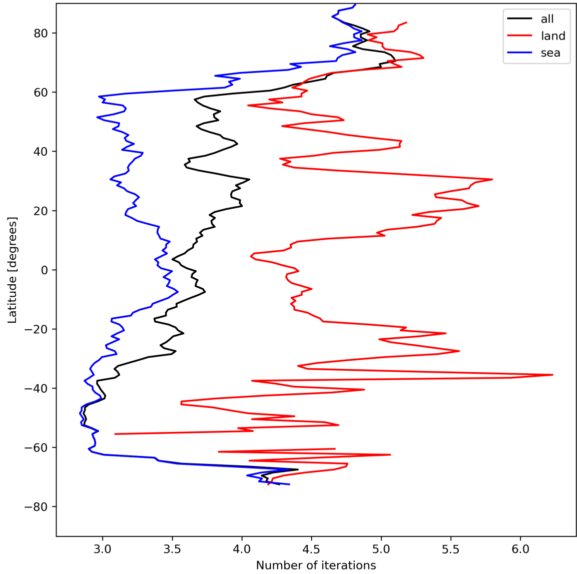
Figure 22: Zonal average of “Number of iterations” for 2024-04-29 to 2024-05-01.
