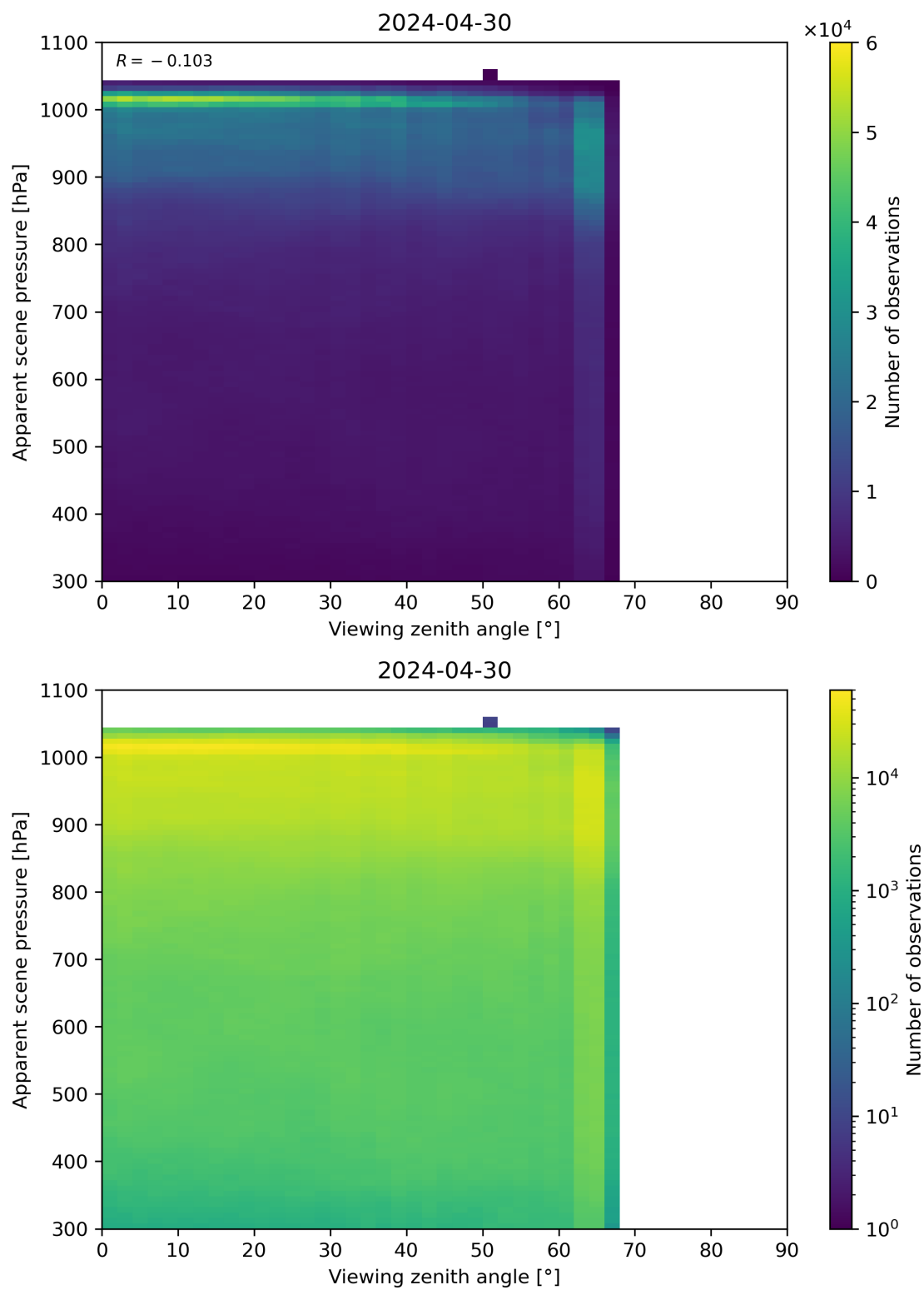
Figure 118: Scatter density plot of “Viewing zenith angle” against “Apparent scene pressure” for 2024-04-29 to 2024-05-01.
