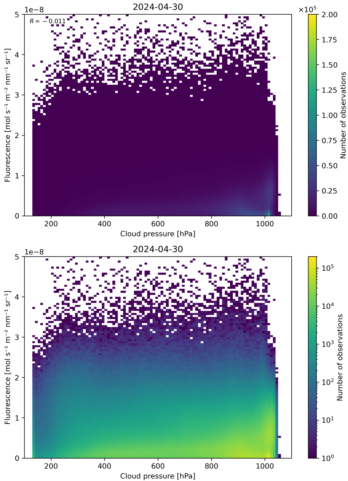
Figure 80: Scatter density plot of “Cloud pressure” against “Fluorescence” for 2024-04-29 to 2024-05-01.
