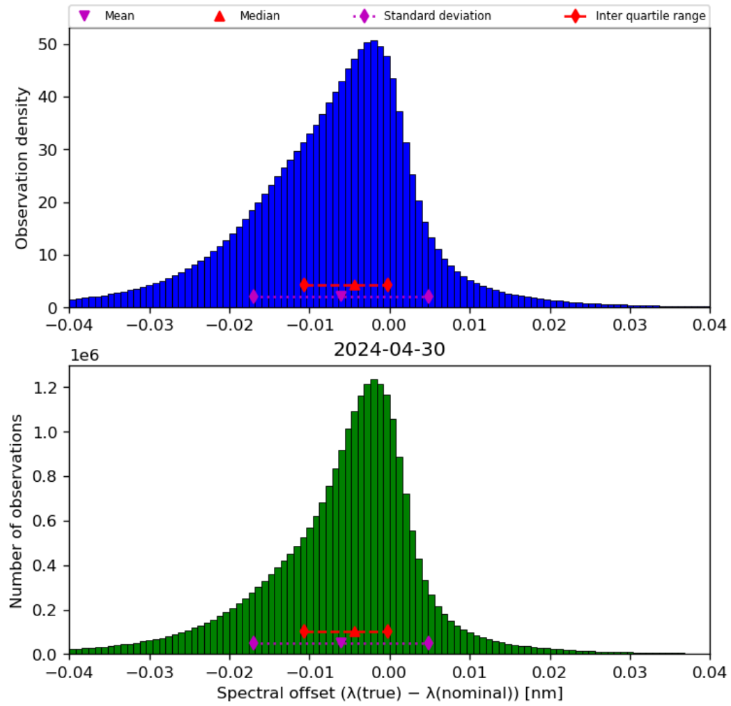
Figure 45: Histogram of “Spectral offset ( \lambda(\text{true}) - \lambda(\text{nominal}) )” for 2024-04-29 to 2024-05-01
