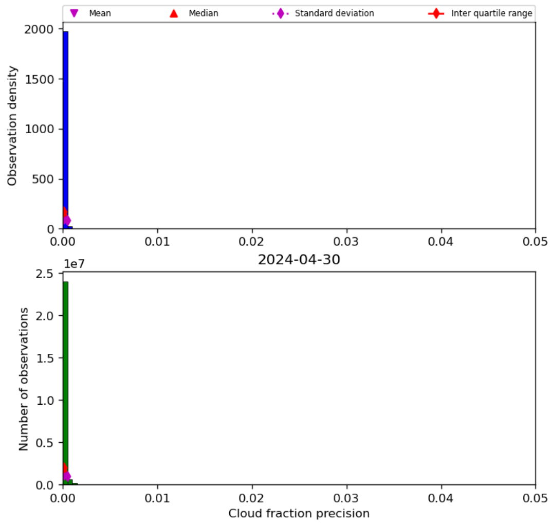
Figure 33: Histogram of “Cloud fraction precision” for 2024-04-29 to 2024-05-01
