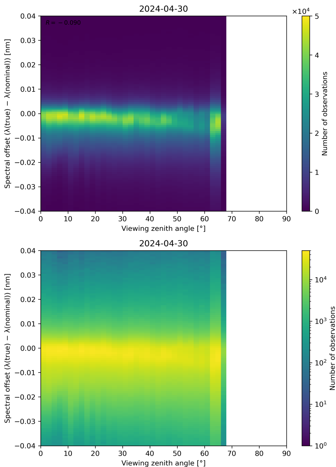
Figure 128: Scatter density plot of “Viewing zenith angle” against “Spectral offset ( \lambda(\text{true}) - \lambda(\text{nominal}) )” for 2024-04-29 to 2024-05-01.
