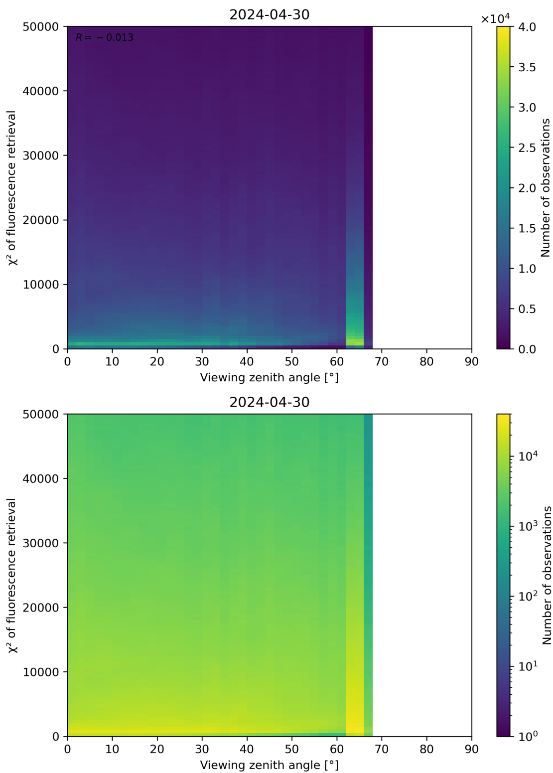
Figure 119: Scatter density plot of “Viewing zenith angle” against “ \chi^2 of fluorescence retrieval” for 2024-04-29 to 2024-05-01.
