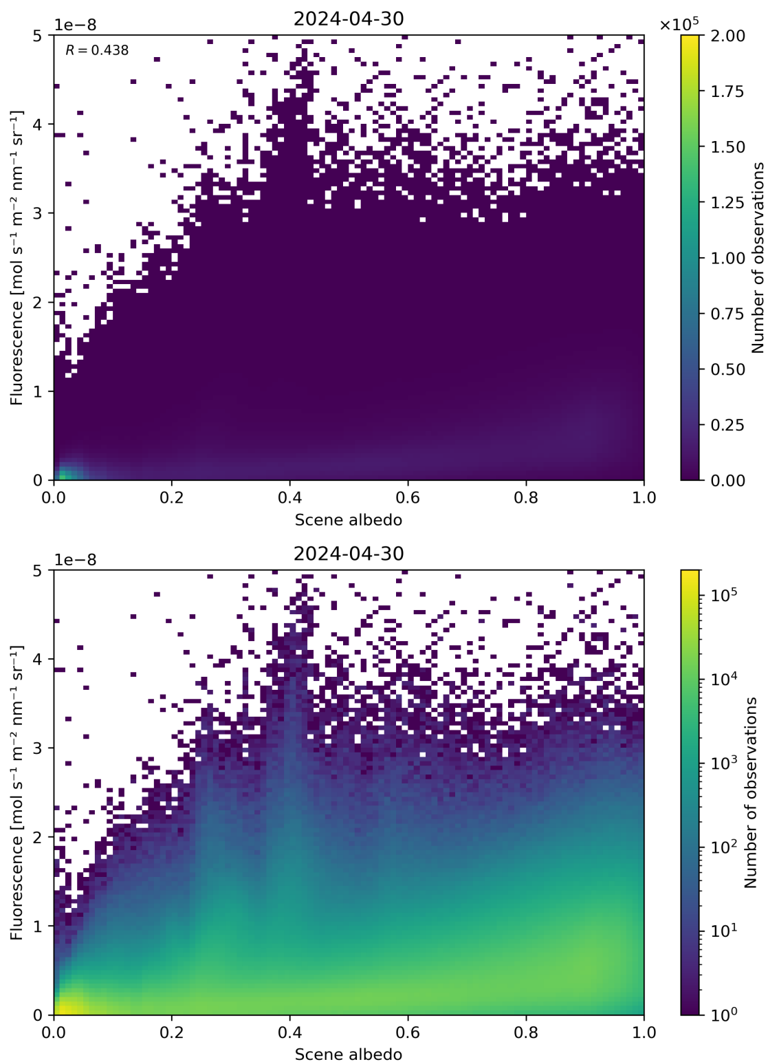
Figure 104: Scatter density plot of “Scene albedo” against “Fluorescence” for 2024-04-29 to 2024-05-01.
