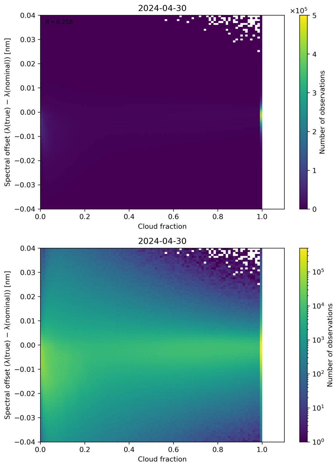
Figure 76: Scatter density plot of “Cloud fraction” against “Spectral offset ( \lambda(\text{true}) - \lambda(\text{nominal}) )” for 2024-04-29 to 2024-05-01.
