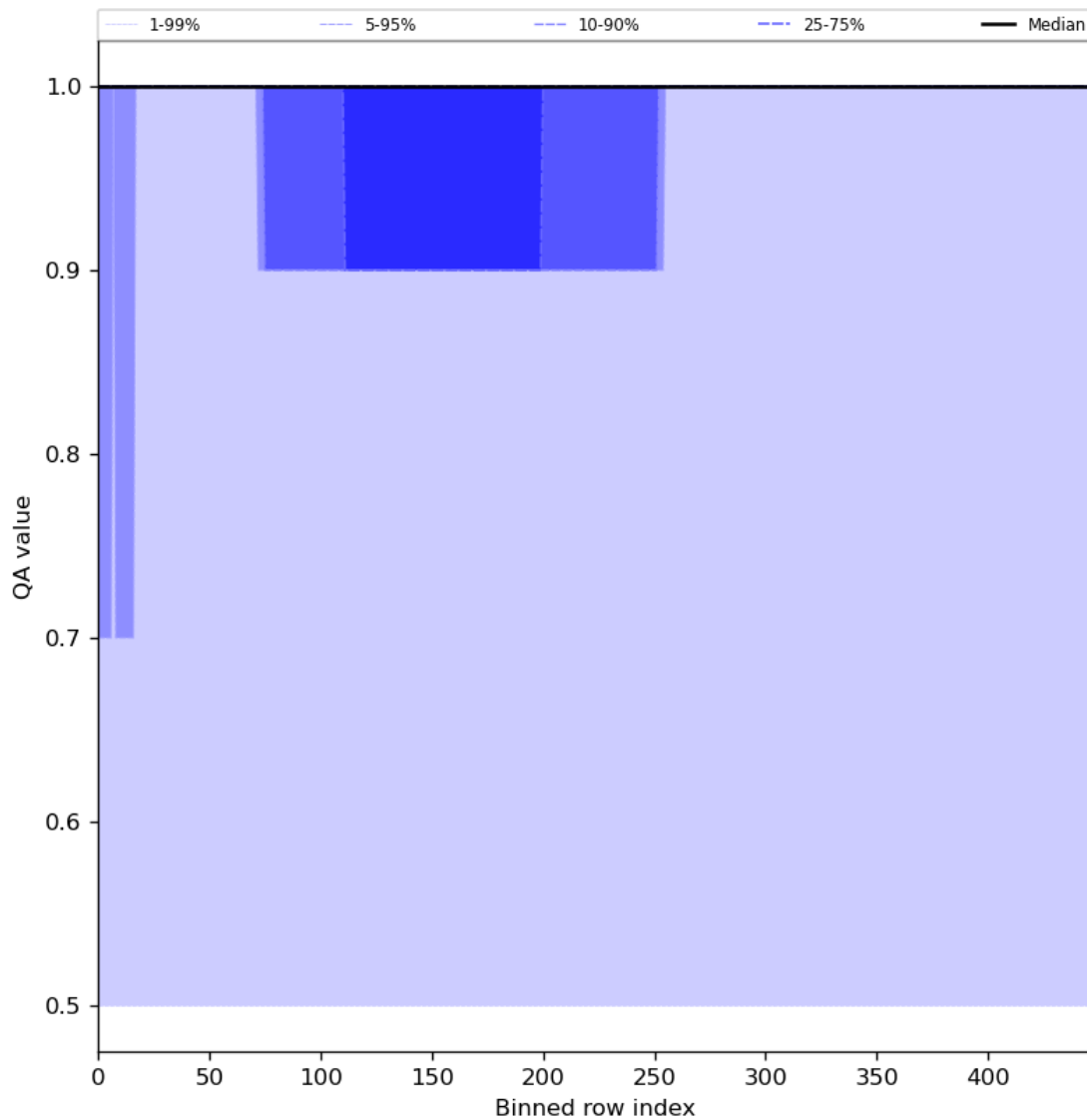
Figure 46: Along track statistics of "QA value" for 2024-04-29 to 2024-05-01
