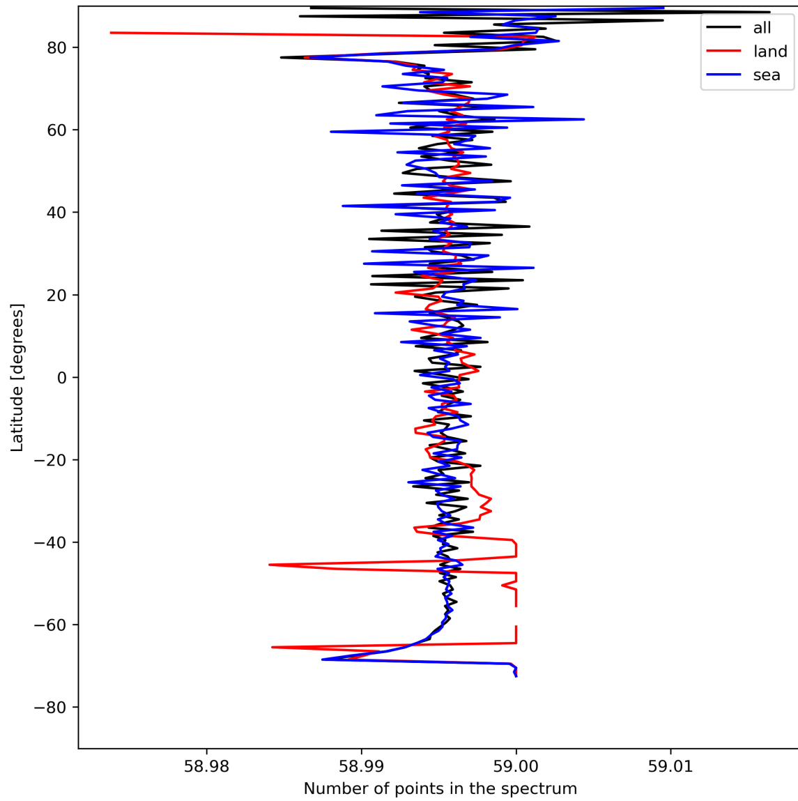
Figure 27: Zonal average of “Number of points in the spectrum” for 2024-04-29 to 2024-05-01.
