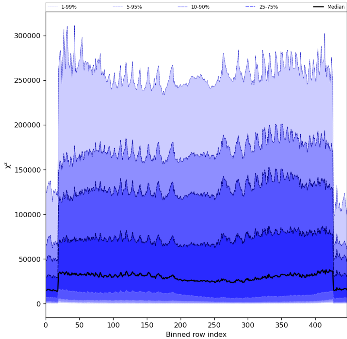
Figure 55: Along track statistics of “ \chi^2 ” for 2024-04-29 to 2024-05-01
