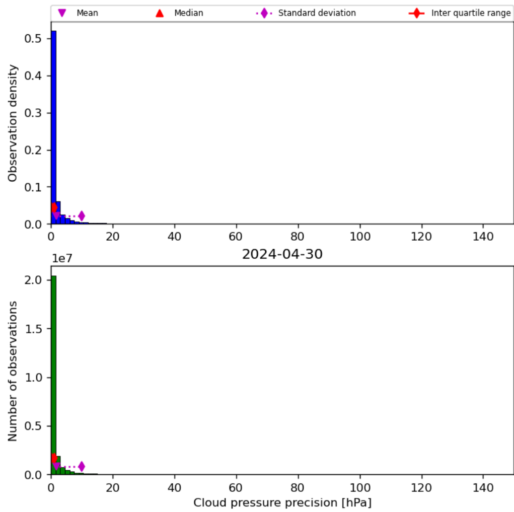
Figure 31: Histogram of “Cloud pressure precision” for 2024-04-29 to 2024-05-01
