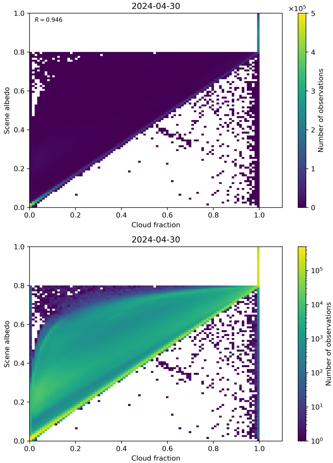
Figure 75: Scatter density plot of “Cloud fraction” against “Scene albedo” for 2024-04-29 to 2024-05-01.
