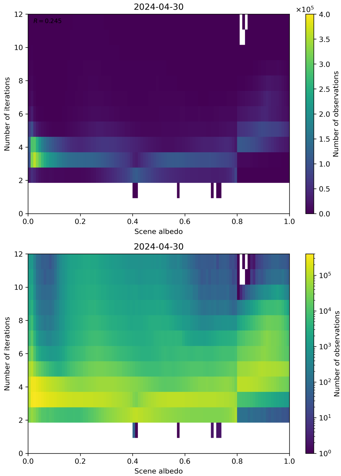
Figure 105: Scatter density plot of “Scene albedo” against “Number of iterations” for 2024-04-29 to 2024-05-01.
