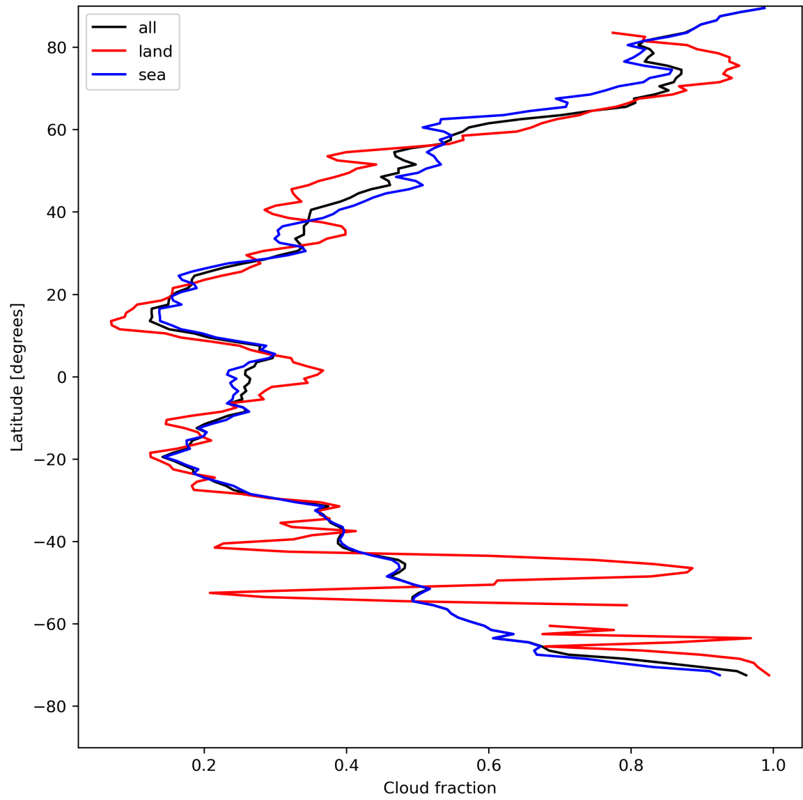
Figure 15: Zonal average of “Cloud fraction” for 2024-04-29 to 2024-05-01.
