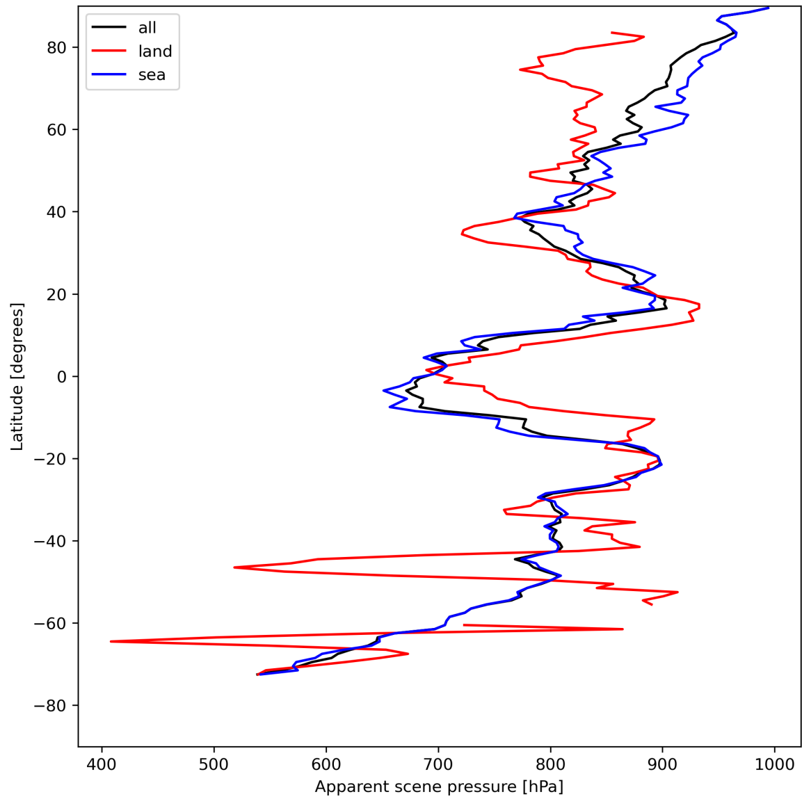
Figure 19: Zonal average of “Apparent scene pressure” for 2024-04-29 to 2024-05-01.
