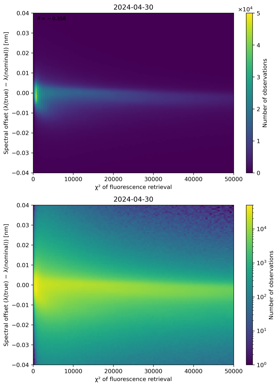
Figure 69: Scatter density plot of " \chi^2 of fluorescence retrieval" against "Spectral offset ( \lambda(\text{true}) - \lambda(\text{nominal}) )" for 2024-04-29 to 2024-05-01.
