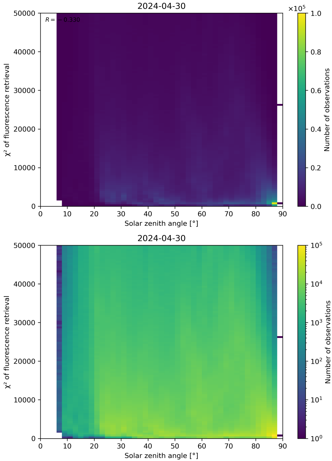
Figure 109: Scatter density plot of “Solar zenith angle” against “ \chi^2 of fluorescence retrieval” for 2024-04-29 to 2024-05-01.
