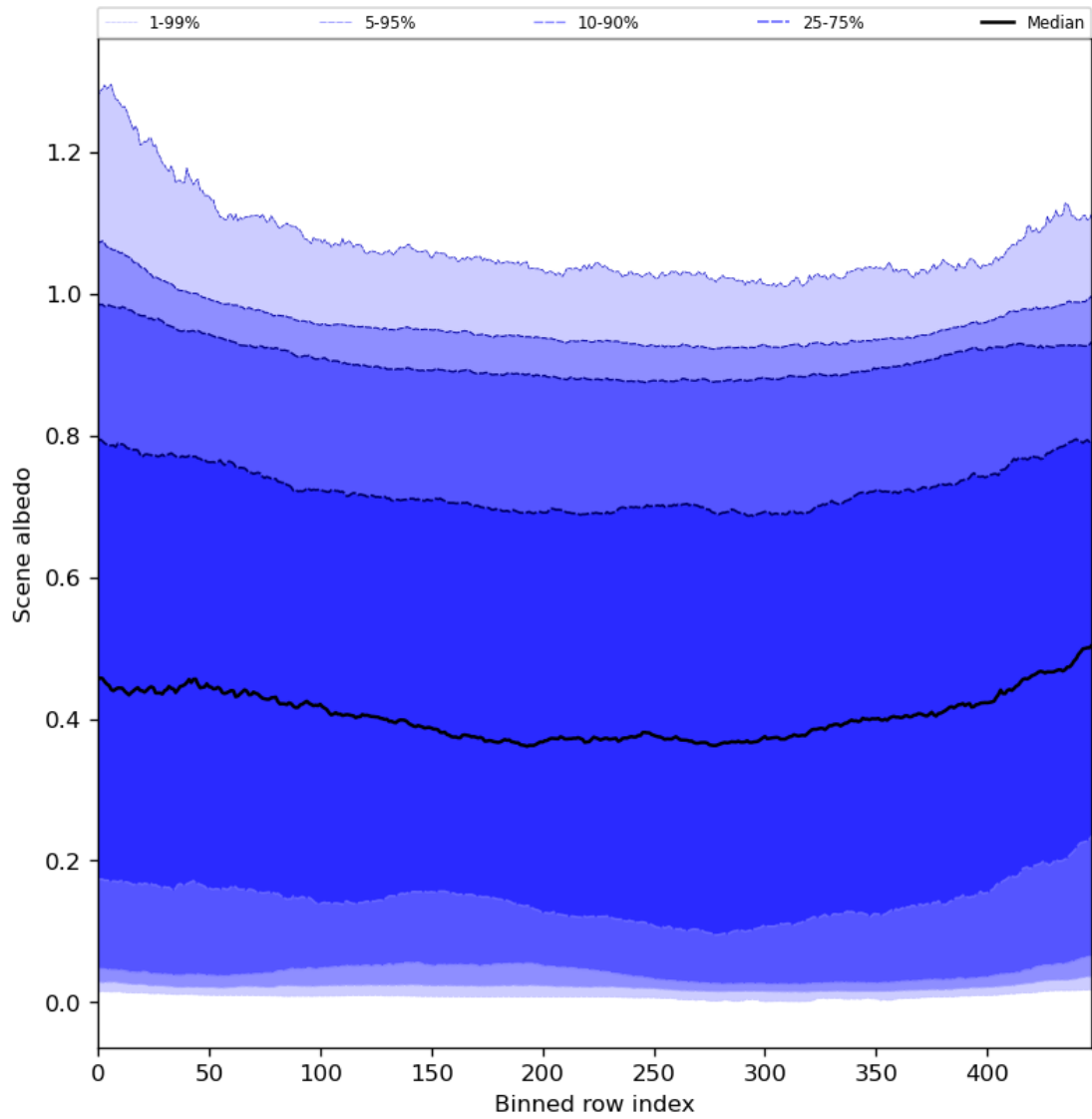
Figure 51: Along track statistics of “Scene albedo” for 2024-04-29 to 2024-05-01
