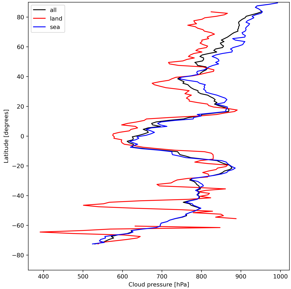
Figure 13: Zonal average of “Cloud pressure” for 2024-04-29 to 2024-05-01.
