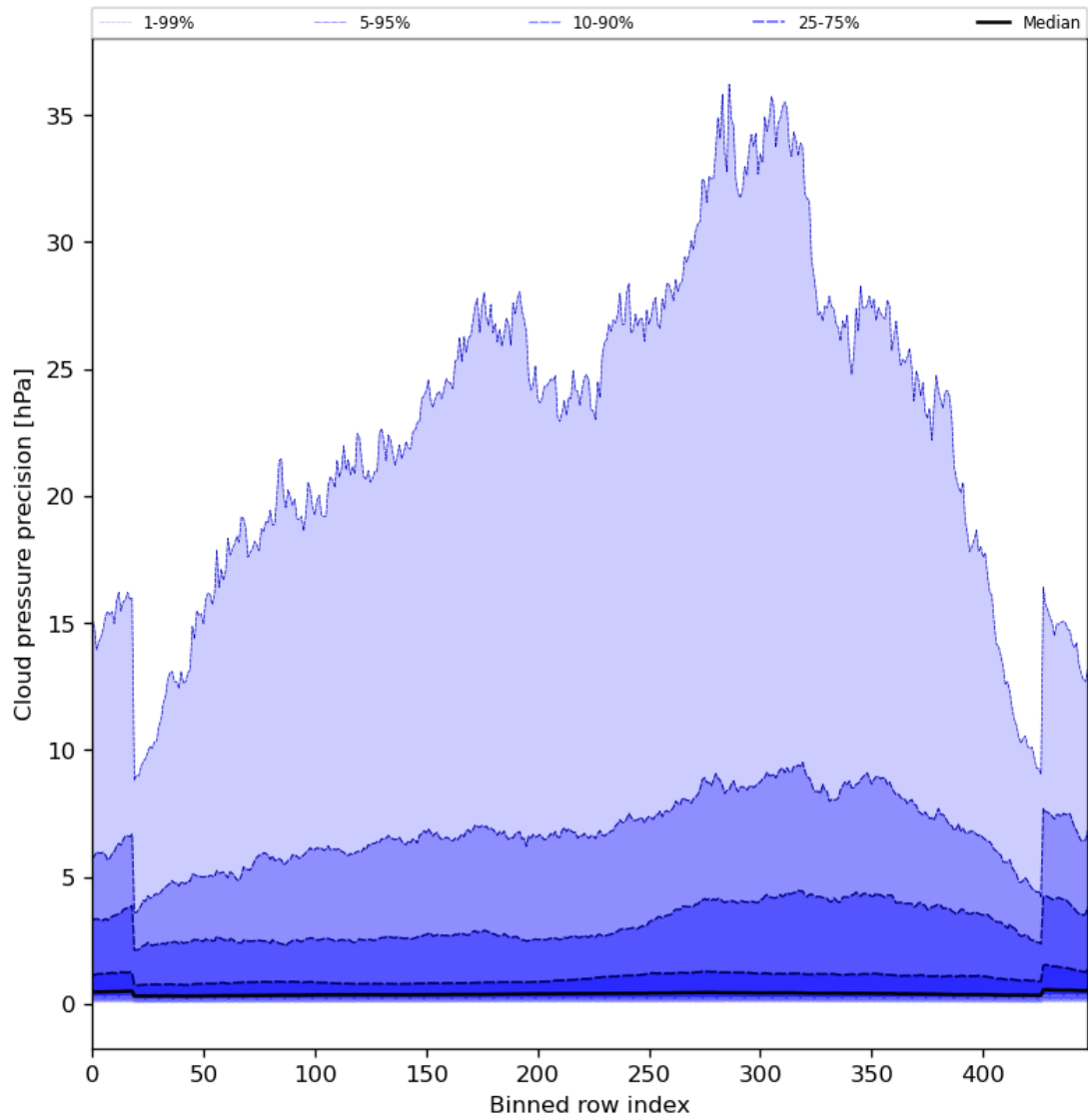
Figure 48: Along track statistics of “Cloud pressure precision” for 2024-04-29 to 2024-05-01
