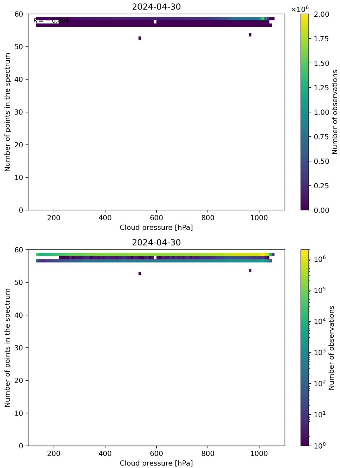
Figure 82: Scatter density plot of “Cloud pressure” against “Number of points in the spectrum” for 2024-04-29 to 2024-05-01.
