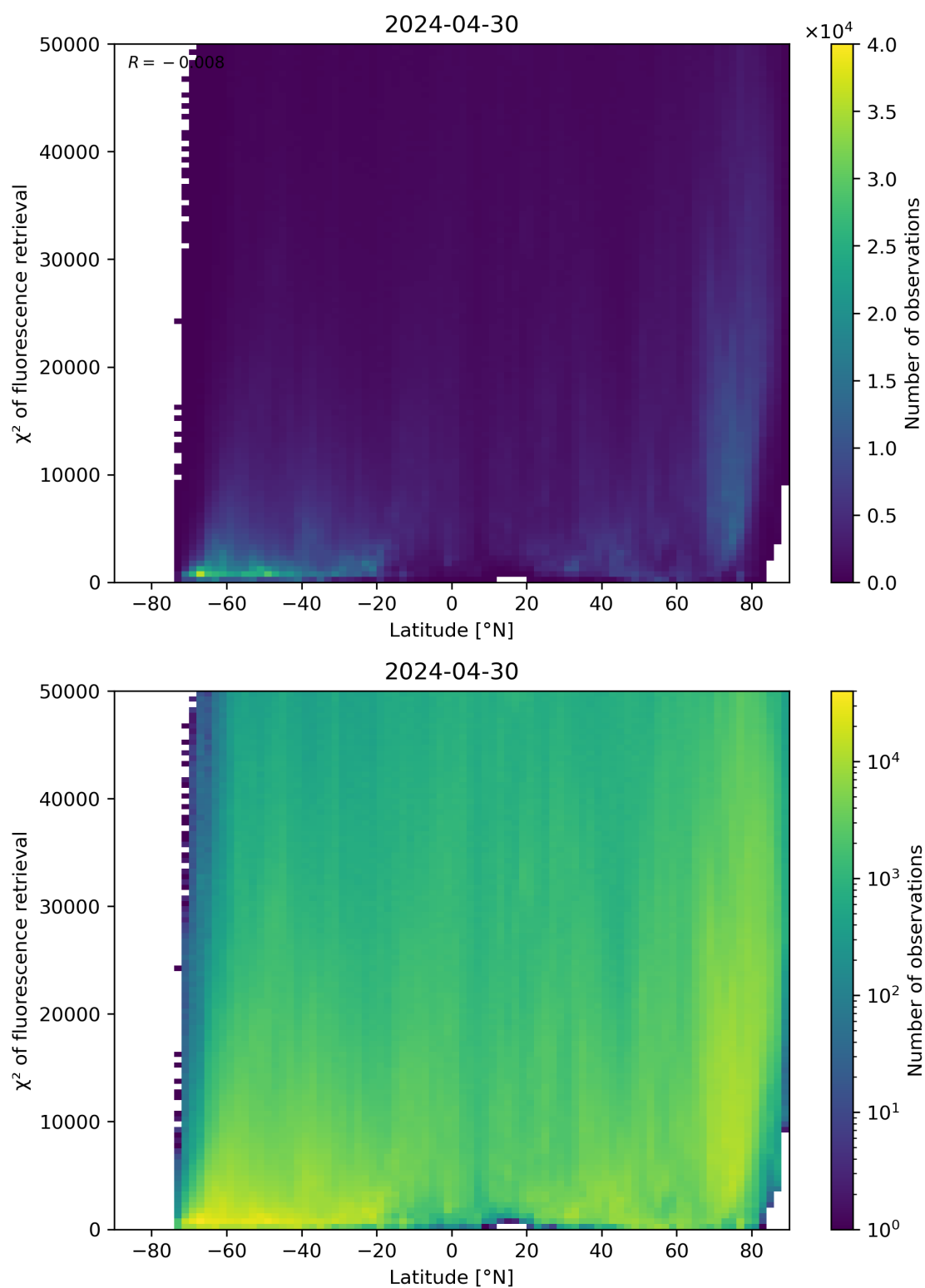
Figure 89: Scatter density plot of “Latitude” against “ \chi^2 of fluorescence retrieval” for 2024-04-29 to 2024-05-01.
