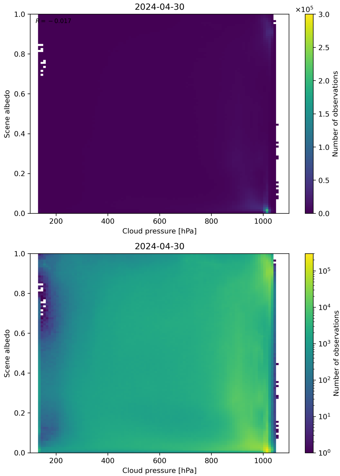
Figure 83: Scatter density plot of “Cloud pressure” against “Scene albedo” for 2024-04-29 to 2024-05-01.
