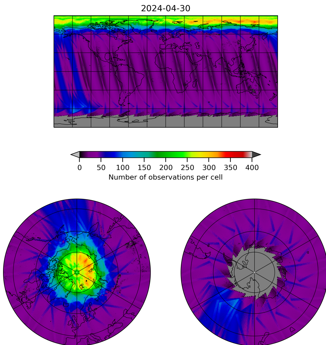
Figure 11: Map of the number of observations for 2024-04-29 to 2024-05-01
