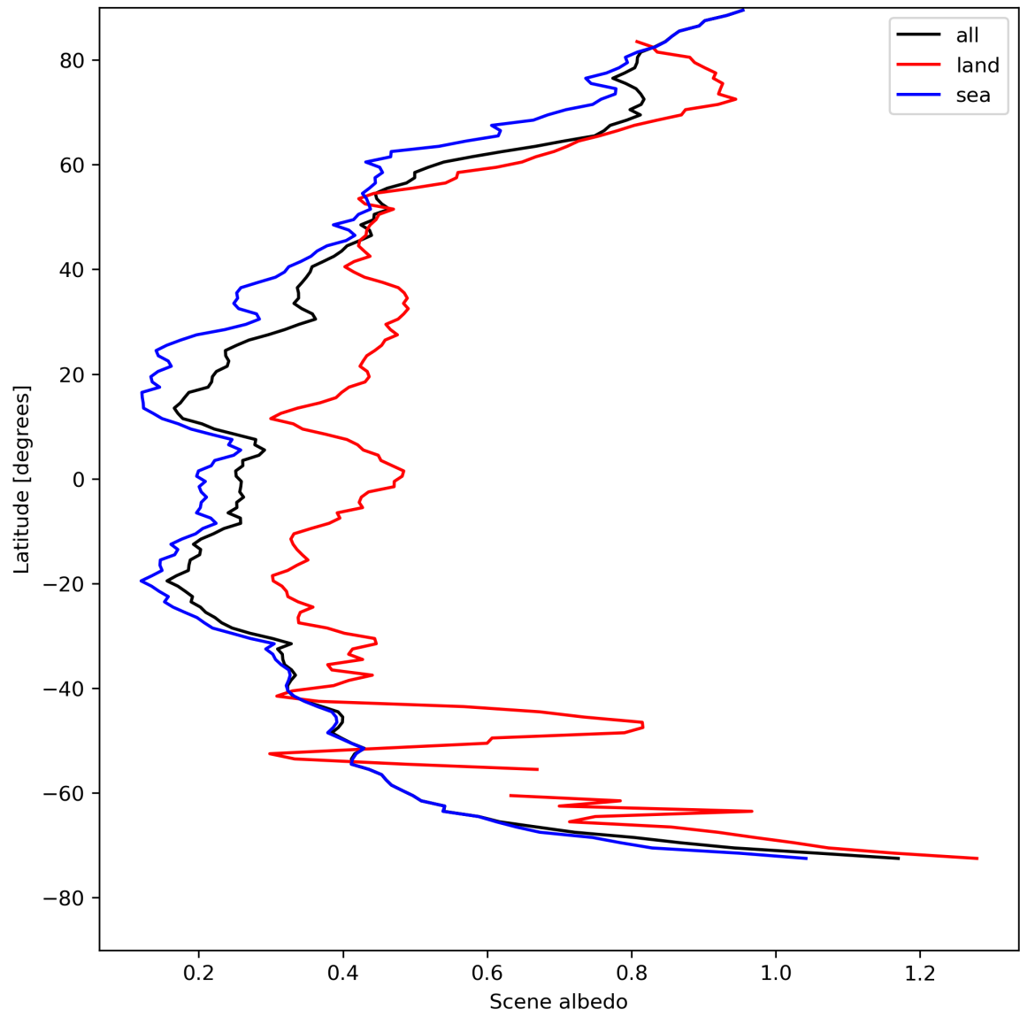
Figure 17: Zonal average of “Scene albedo” for 2024-04-29 to 2024-05-01.
