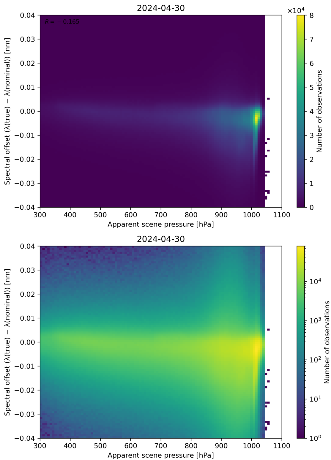
Figure 67: Scatter density plot of “Apparent scene pressure” against “Spectral offset ( \lambda(\text{true}) - \lambda(\text{nominal}) )” for 2024-04-29 to 2024-05-01.
