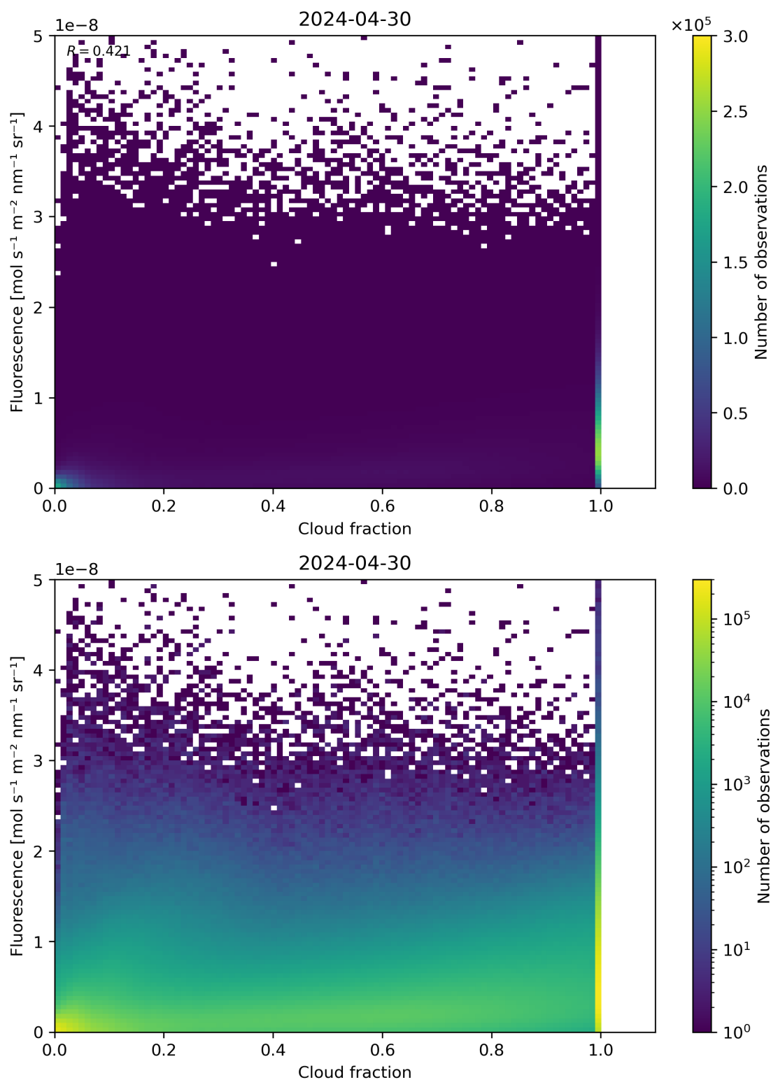
Figure 72: Scatter density plot of “Cloud fraction” against “Fluorescence” for 2024-04-29 to 2024-05-01.
