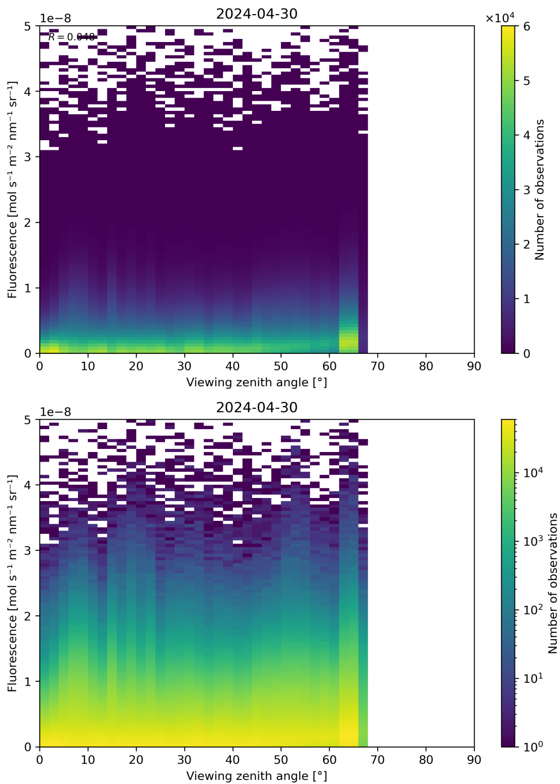
Figure 122: Scatter density plot of “Viewing zenith angle” against “Fluorescence” for 2024-04-29 to 2024-05-01.
