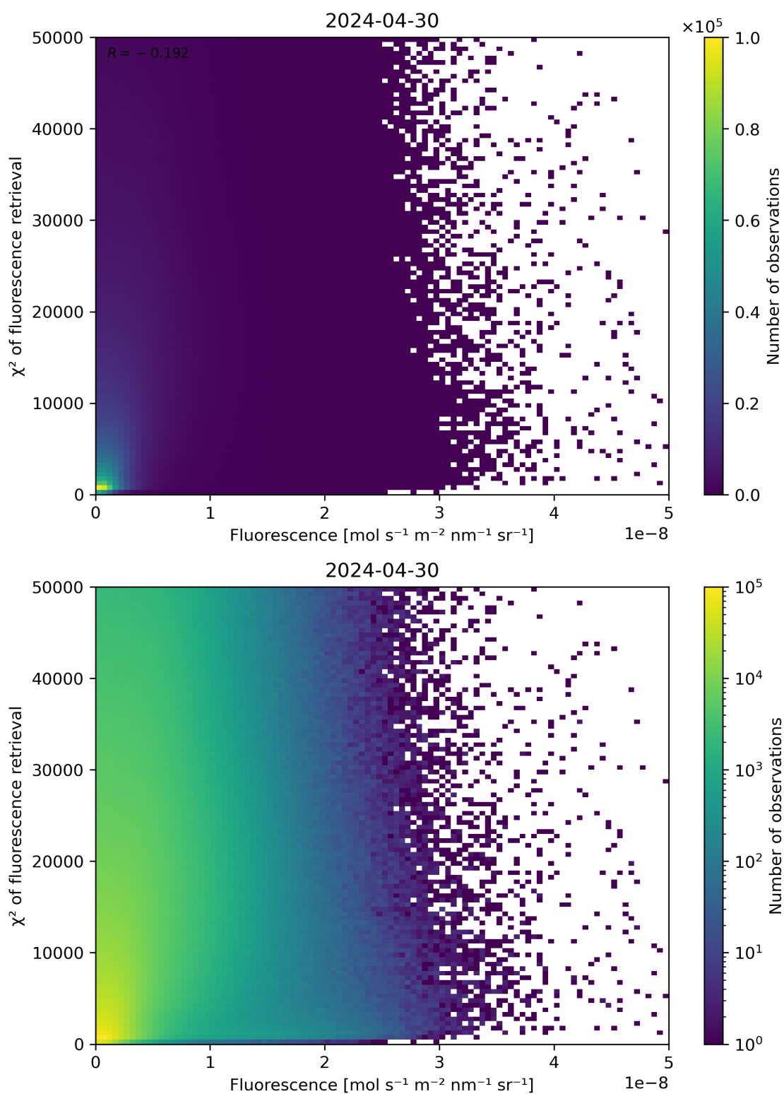
Figure 85: Scatter density plot of “Fluorescence” against “ \chi^2 of fluorescence retrieval” for 2024-04-29 to 2024-05-01.
