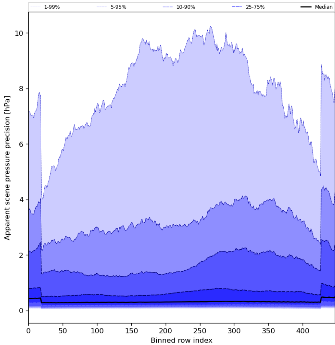
Figure 54: Along track statistics of “Apparent scene pressure precision” for 2024-04-29 to 2024-05-01
