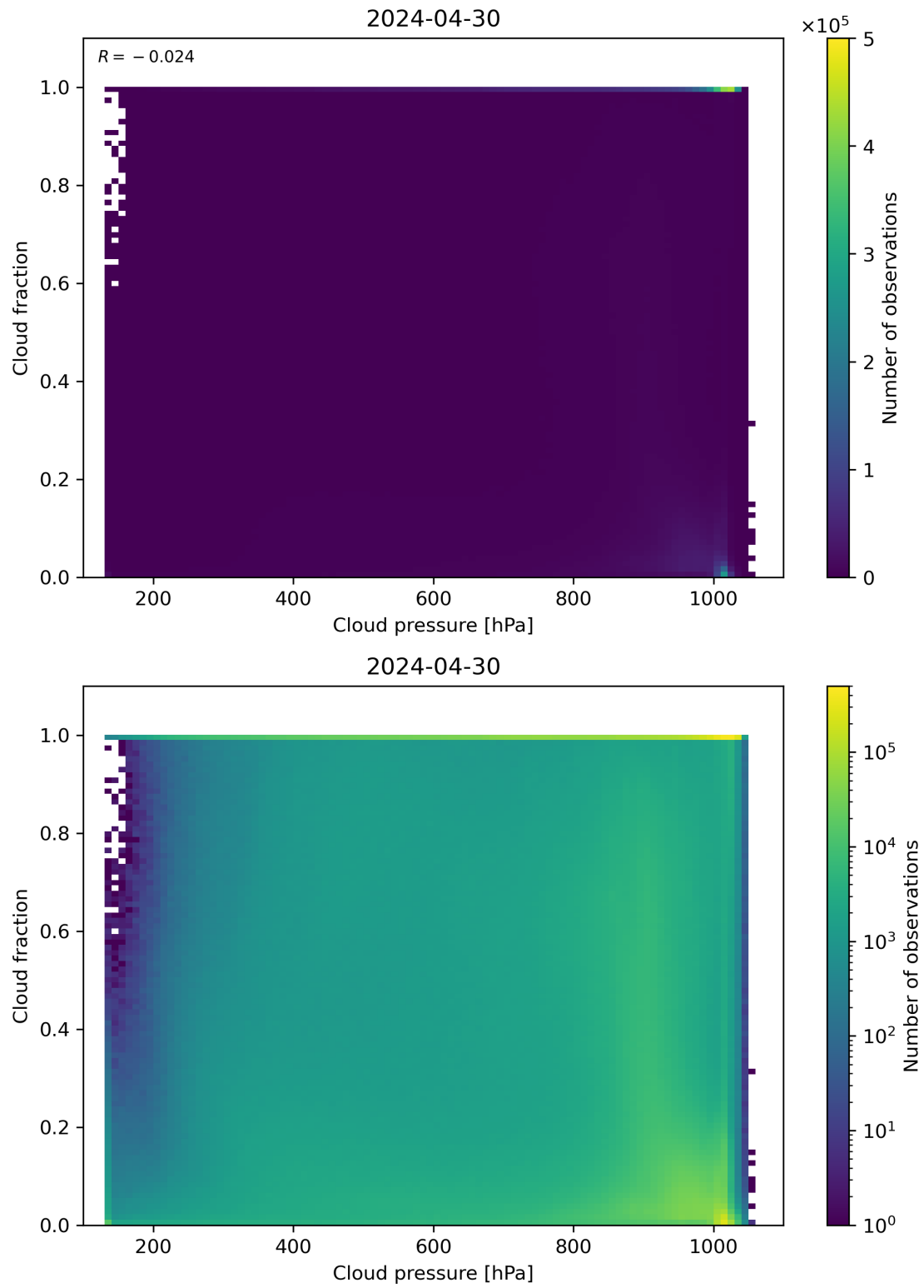
Figure 79: Scatter density plot of “Cloud pressure” against “Cloud fraction” for 2024-04-29 to 2024-05-01.
