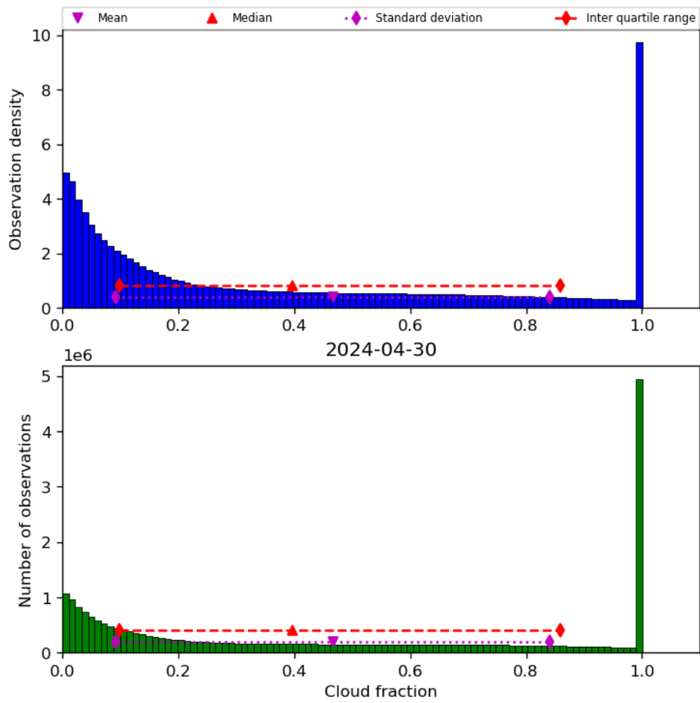
Figure 32: Histogram of “Cloud fraction” for 2024-04-29 to 2024-05-01
