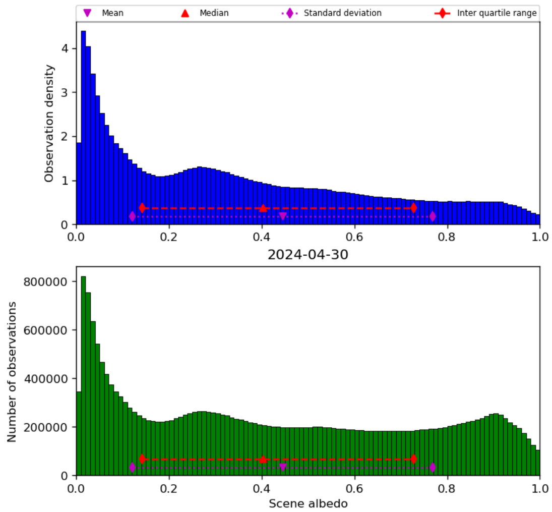
Figure 34: Histogram of “Scene albedo” for 2024-04-29 to 2024-05-01
