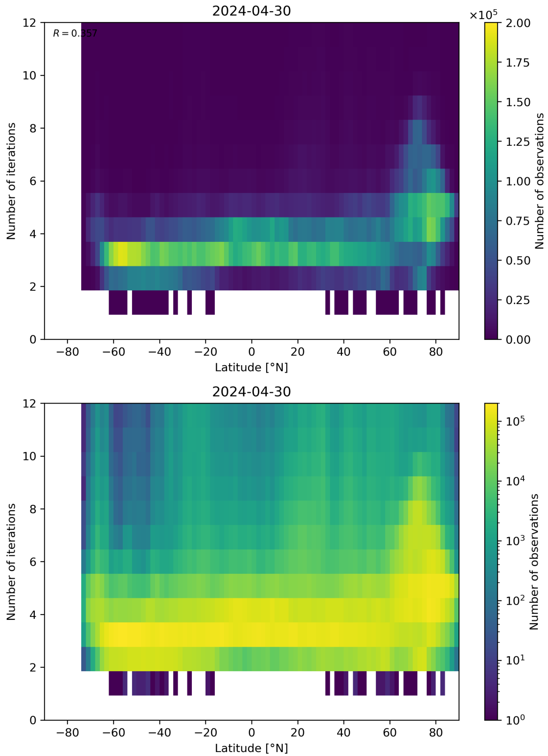
Figure 93: Scatter density plot of “Latitude” against “Number of iterations” for 2024-04-29 to 2024-05-01.
