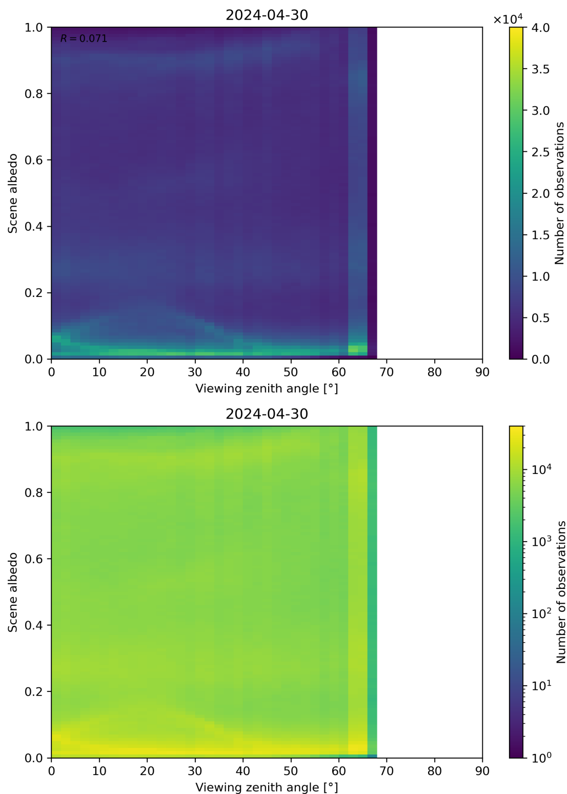
Figure 126: Scatter density plot of “Viewing zenith angle” against “Scene albedo” for 2024-04-29 to 2024-05-01.
