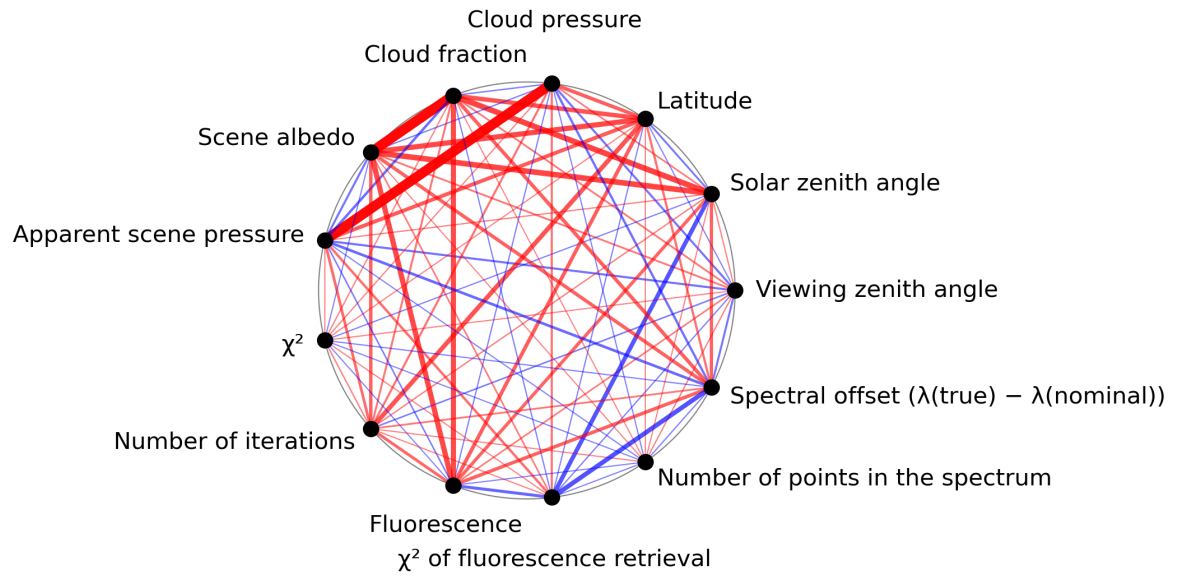
Figure 1: Map of correlation graph for 2024-04-29 to 2024-05-01.
