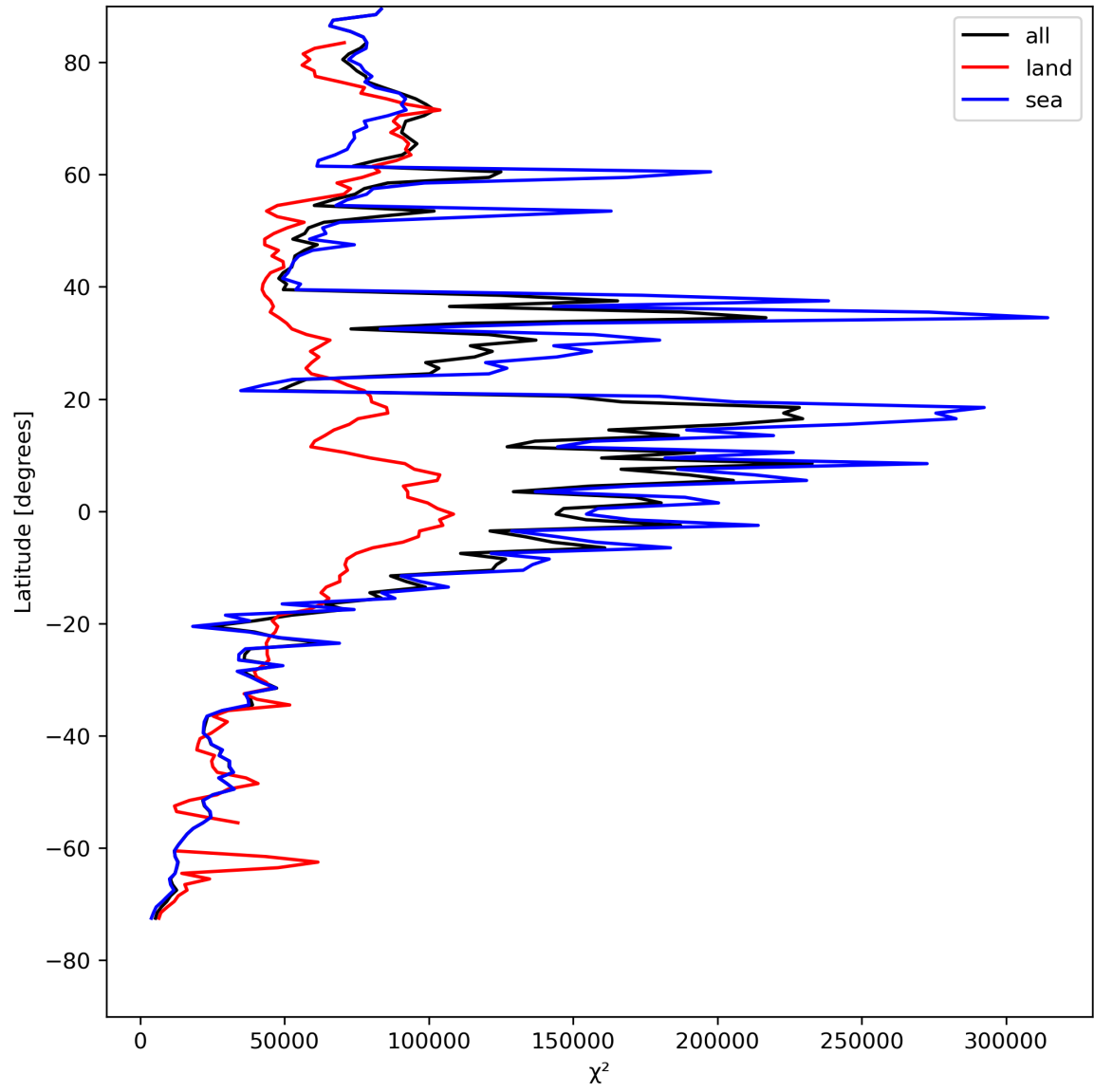
Figure 21: Zonal average of “ \chi^2 ” for 2024-04-29 to 2024-05-01.
