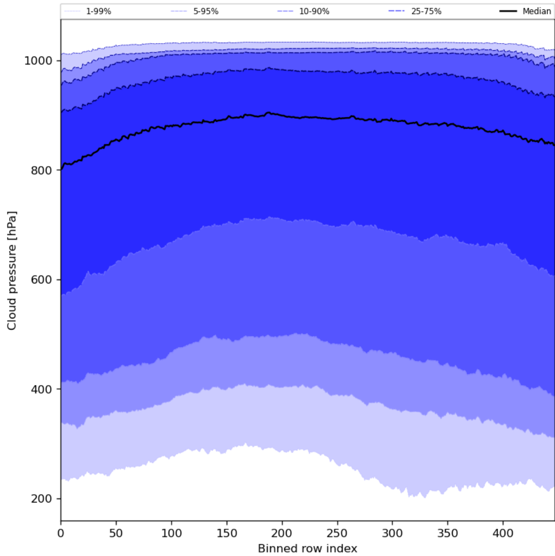
Figure 47: Along track statistics of “Cloud pressure” for 2024-04-29 to 2024-05-01
