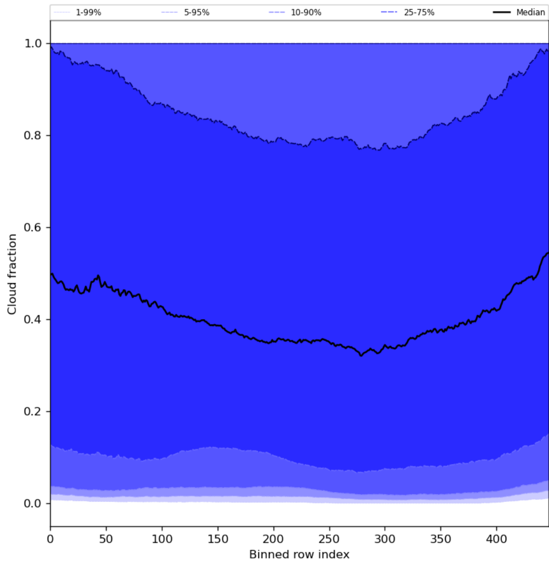
Figure 49: Along track statistics of “Cloud fraction” for 2024-04-29 to 2024-05-01
