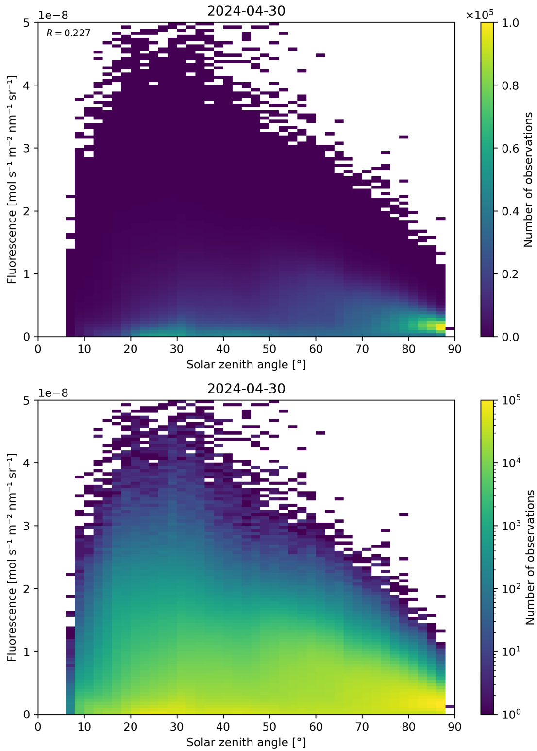
Figure 112: Scatter density plot of “Solar zenith angle” against “Fluorescence” for 2024-04-29 to 2024-05-01.
