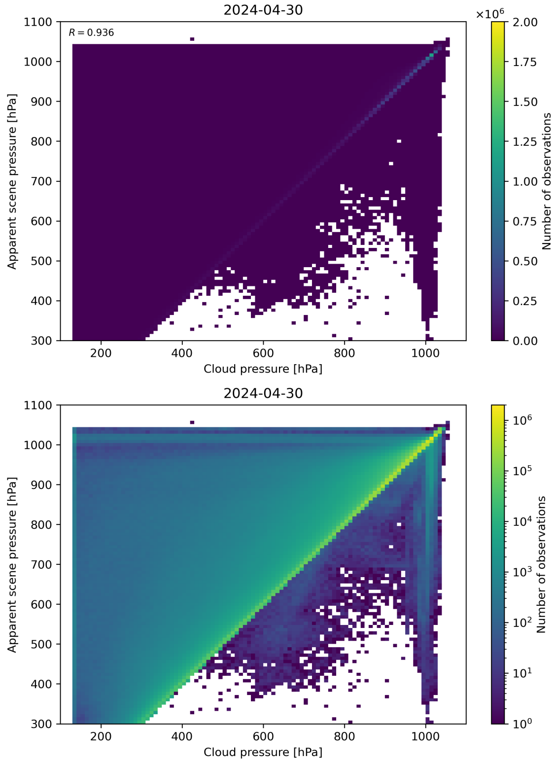
Figure 77: Scatter density plot of “Cloud pressure” against “Apparent scene pressure” for 2024-04-29 to 2024-05-01.
