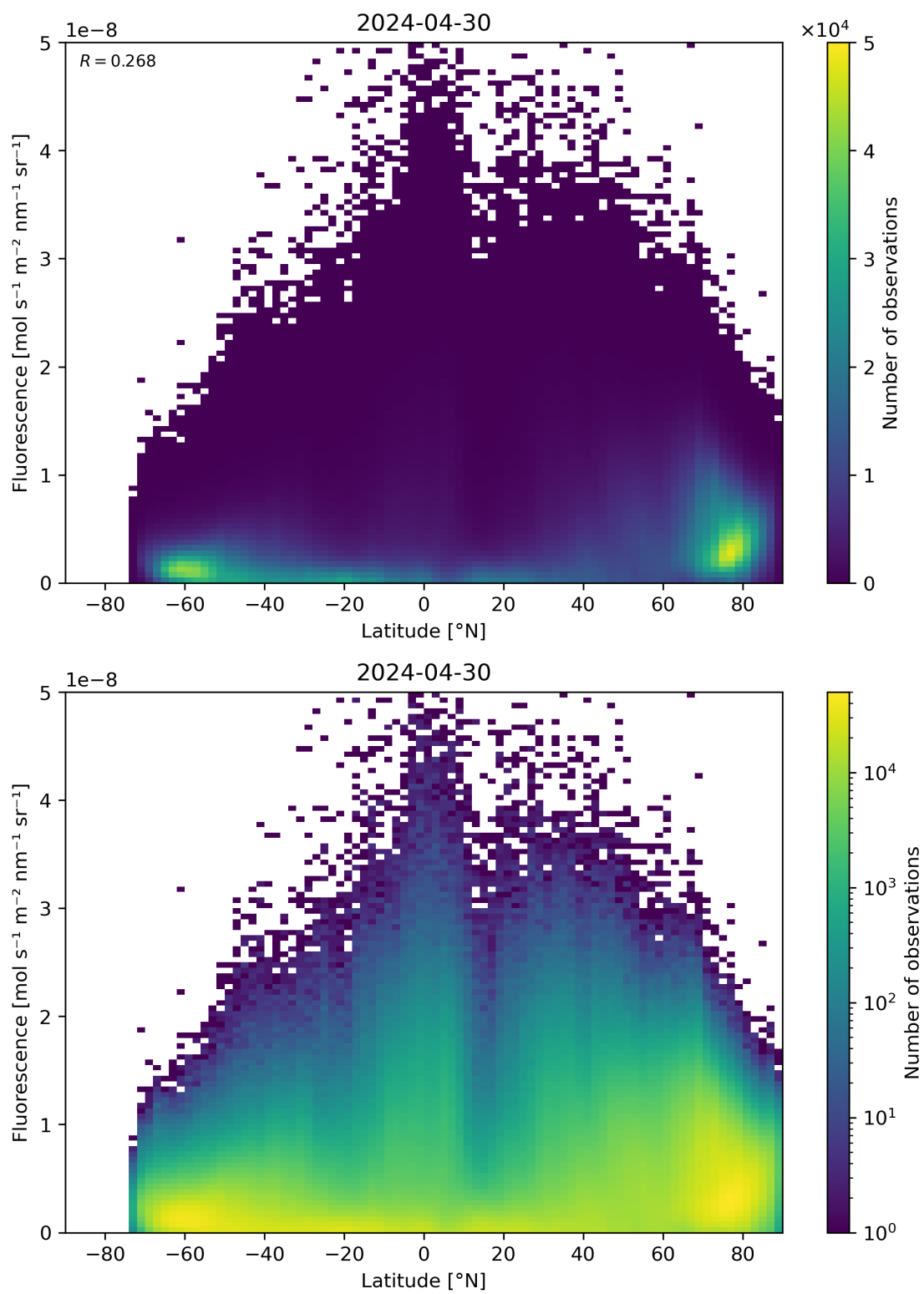
Figure 92: Scatter density plot of “Latitude” against “Fluorescence” for 2024-04-29 to 2024-05-01.
