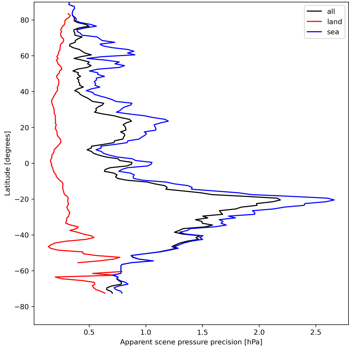
Figure 20: Zonal average of “Apparent scene pressure precision” for 2024-04-29 to 2024-05-01.
