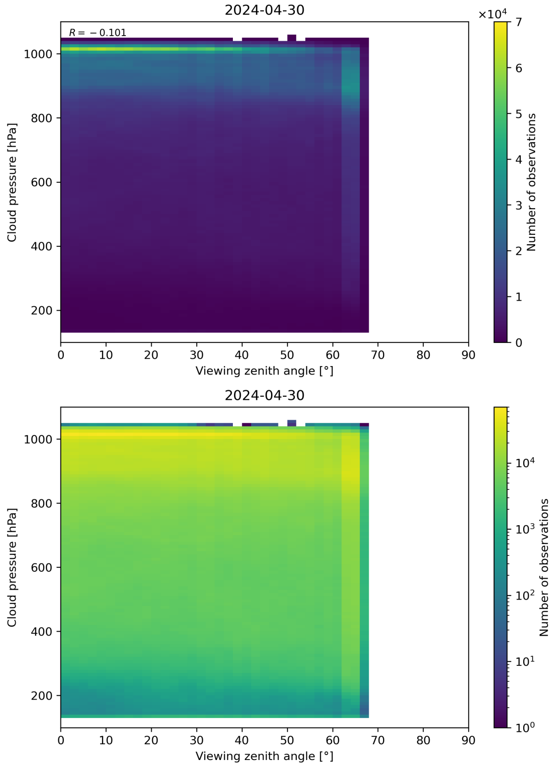
Figure 121: Scatter density plot of “Viewing zenith angle” against “Cloud pressure” for 2024-04-29 to 2024-05-01.
