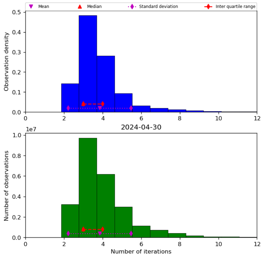
Figure 39: Histogram of “Number of iterations” for 2024-04-29 to 2024-05-01
