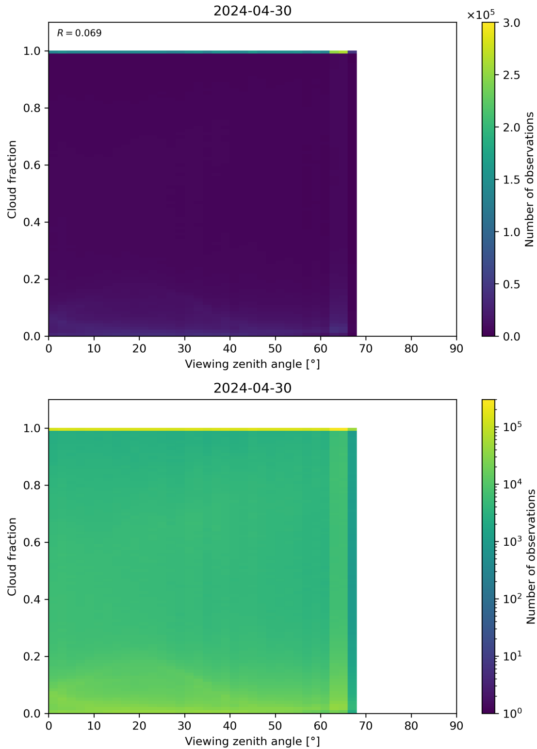
Figure 120: Scatter density plot of “Viewing zenith angle” against “Cloud fraction” for 2024-04-29 to 2024-05-01.
