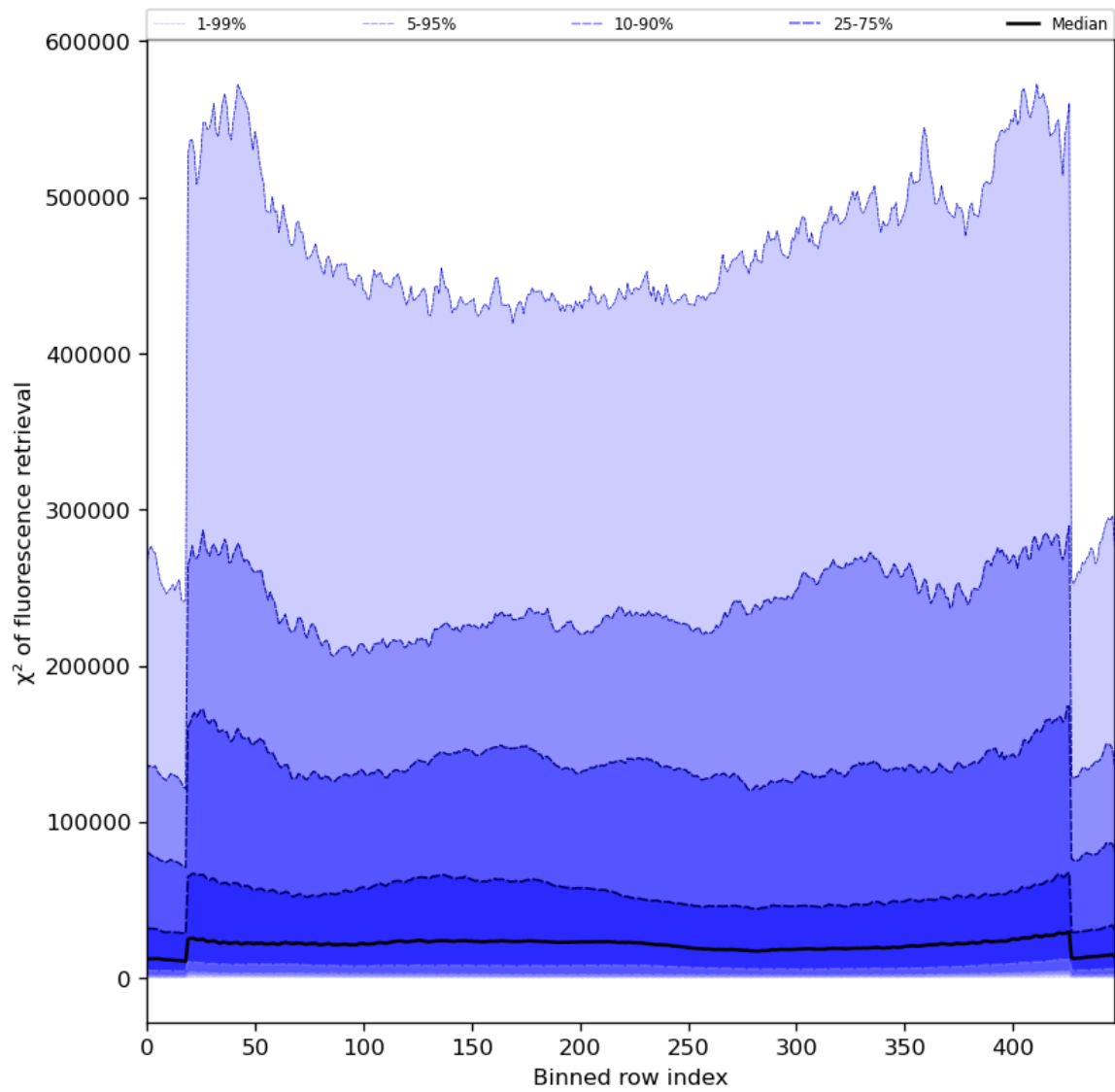
Figure 59: Along track statistics of “ \chi^2 of fluorescence retrieval” for 2024-04-29 to 2024-05-01
