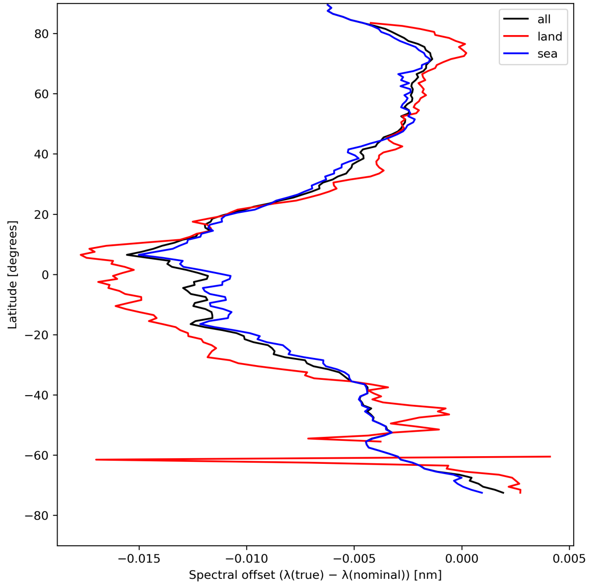
Figure 28: Zonal average of “Spectral offset ( \lambda(\text{true}) - \lambda(\text{nominal}) )” for 2024-04-29 to 2024-05-01.
