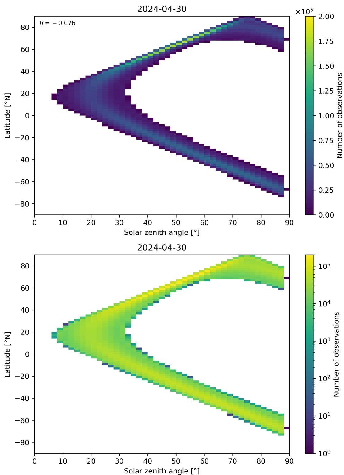
Figure 113: Scatter density plot of “Solar zenith angle” against “Latitude” for 2024-04-29 to 2024-05-01.
