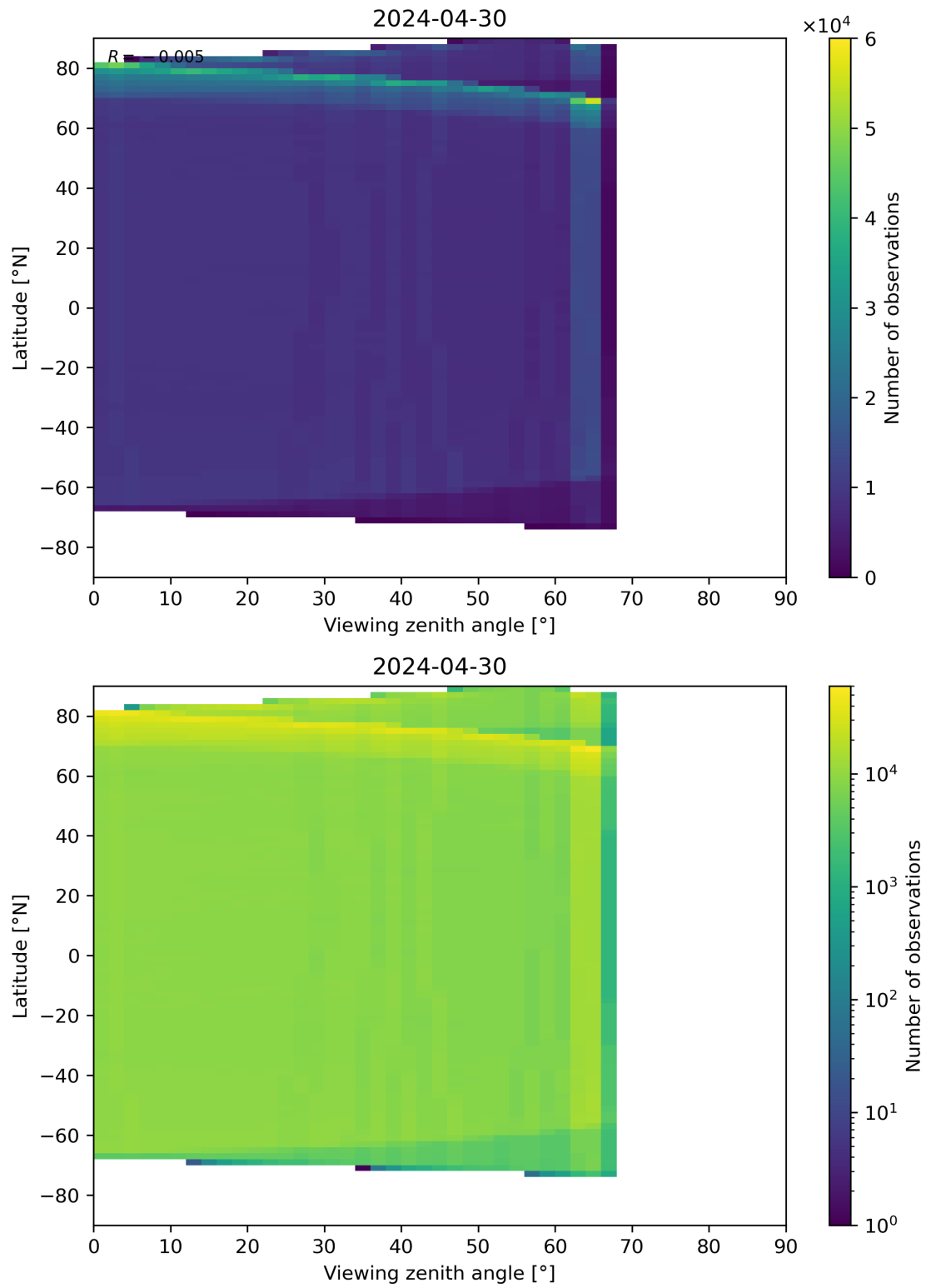
Figure 123: Scatter density plot of “Viewing zenith angle” against “Latitude” for 2024-04-29 to 2024-05-01.
