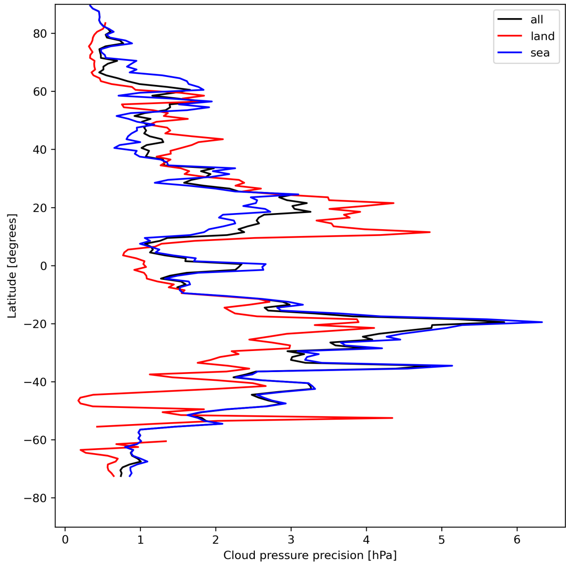
Figure 14: Zonal average of “Cloud pressure precision” for 2024-04-29 to 2024-05-01.
