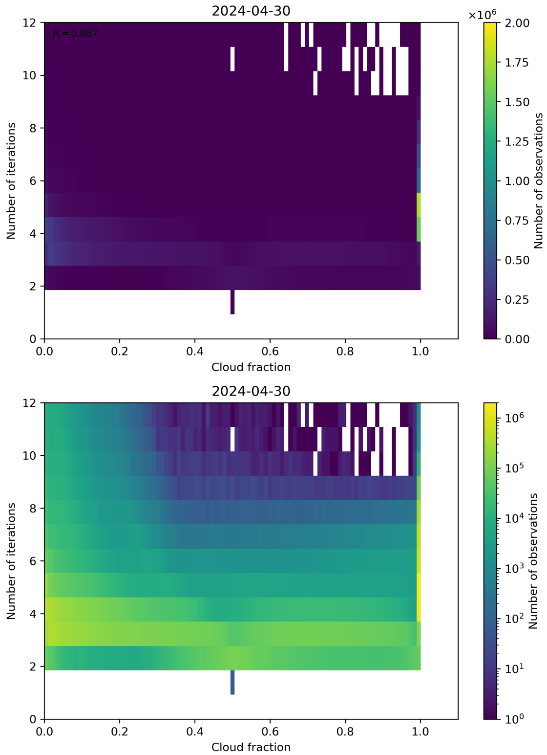
Figure 73: Scatter density plot of “Cloud fraction” against “Number of iterations” for 2024-04-29 to 2024-05-01.
