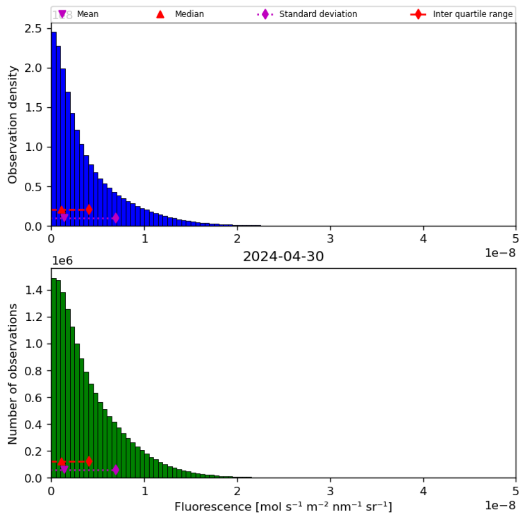
Figure 40: Histogram of “Fluorescence” for 2024-04-29 to 2024-05-01
