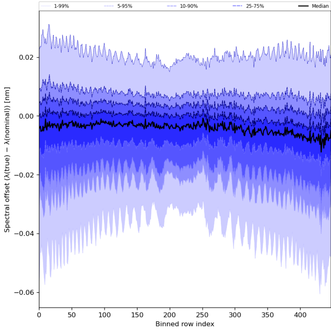
Figure 62: Along track statistics of “Spectral offset ( \lambda(\text{true}) - \lambda(\text{nominal}) )” for 2024-04-29 to 2024-05-01
