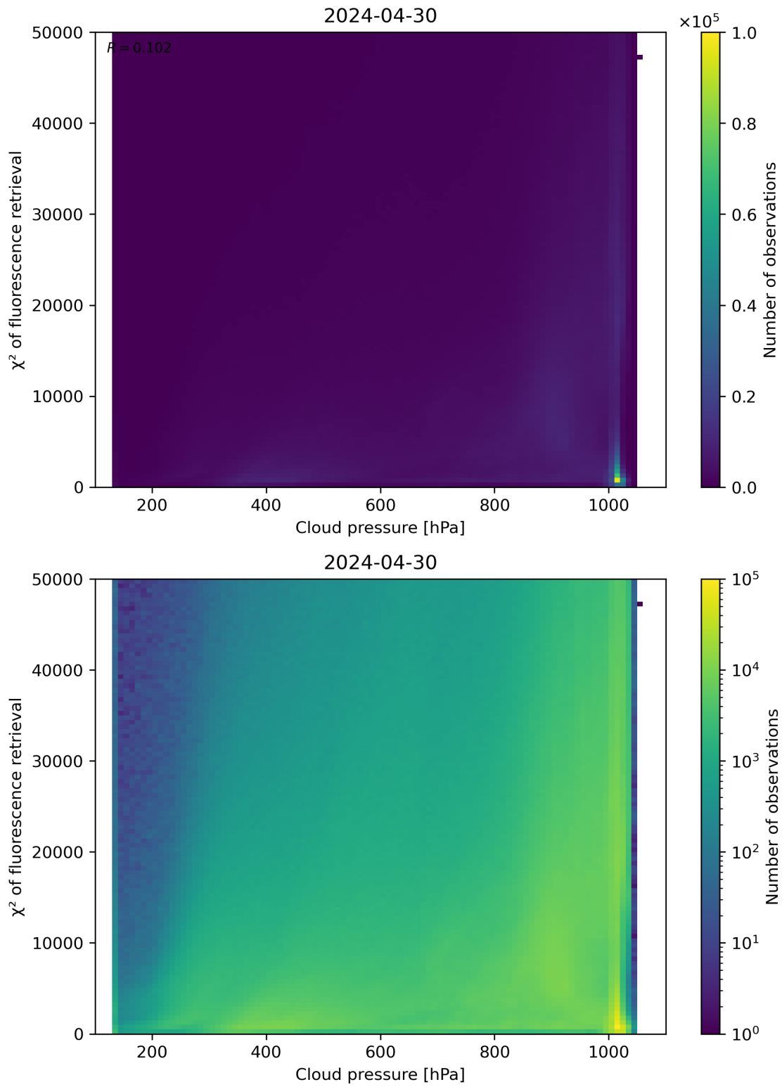
Figure 78: Scatter density plot of “Cloud pressure” against “ \chi^2 of fluorescence retrieval” for 2024-04-29 to 2024-05-01.
