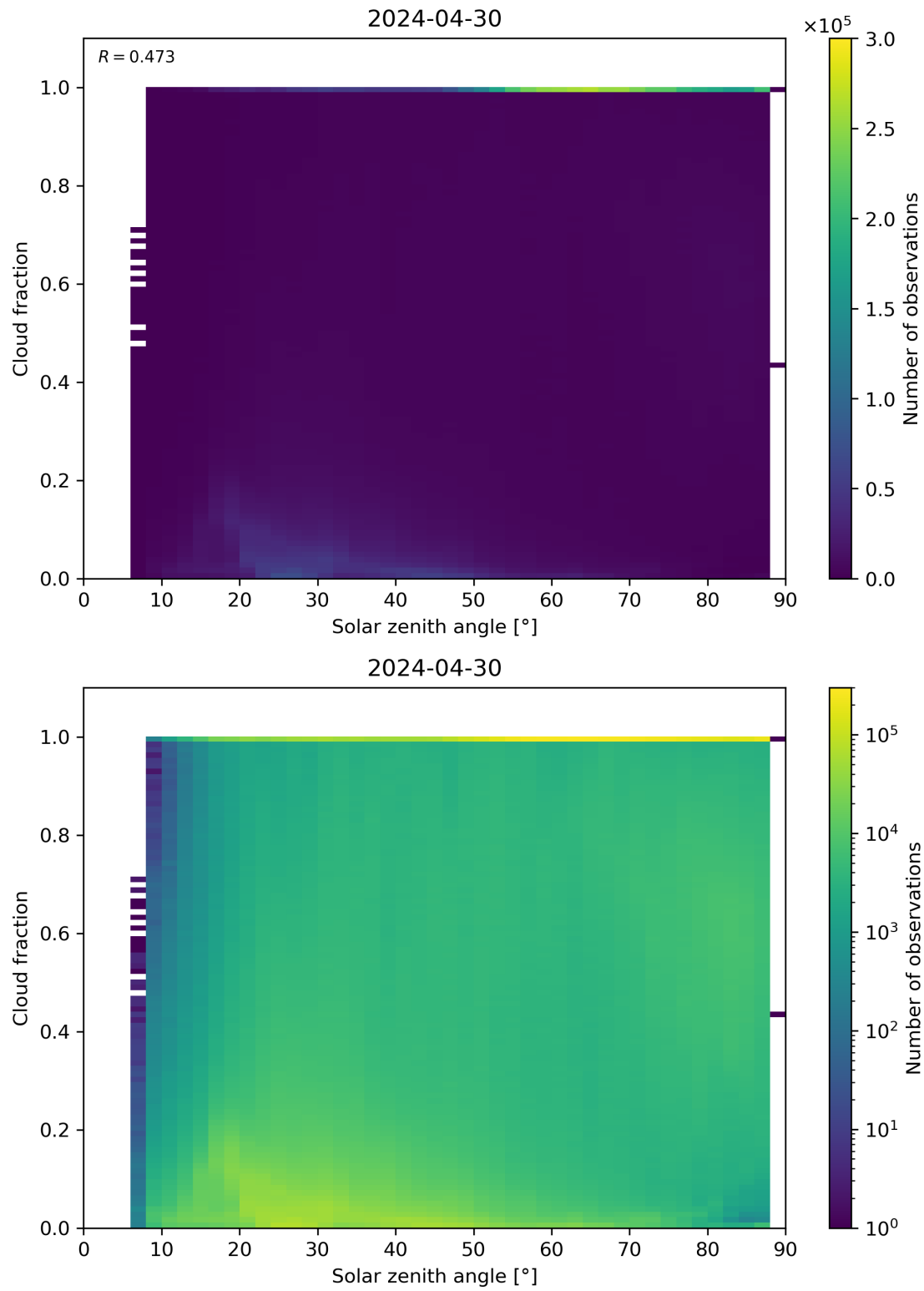
Figure 110: Scatter density plot of “Solar zenith angle” against “Cloud fraction” for 2024-04-29 to 2024-05-01.
