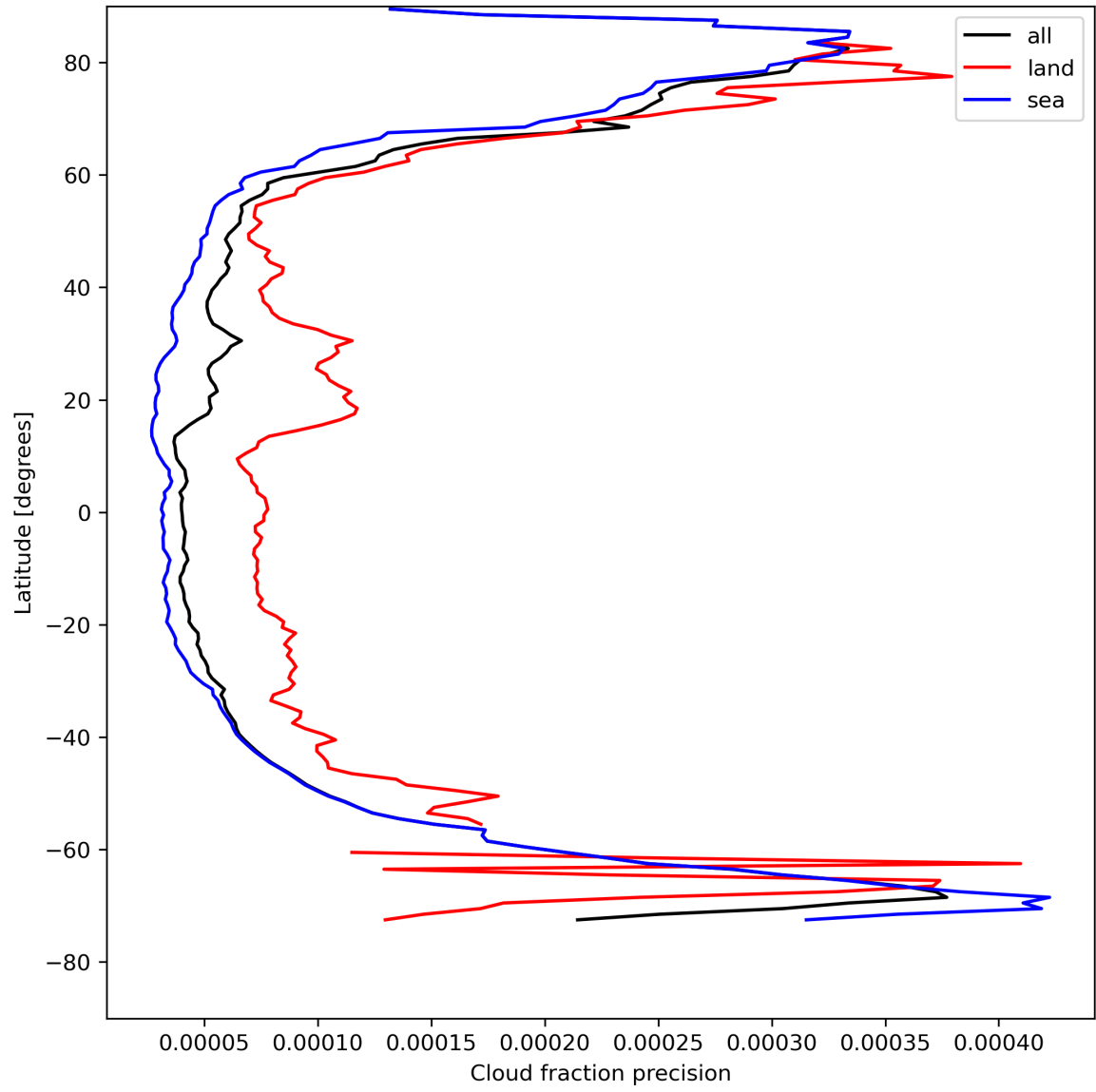
Figure 16: Zonal average of “Cloud fraction precision” for 2024-04-29 to 2024-05-01.
