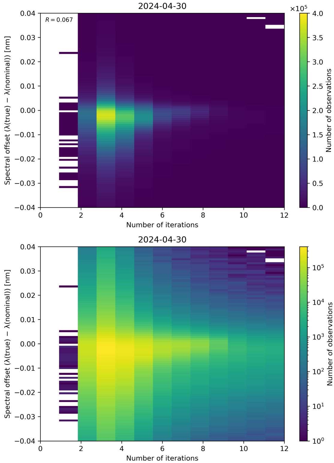
Figure 100: Scatter density plot of “Number of iterations” against “Spectral offset ( \lambda(\text{true}) - \lambda(\text{nominal}) )” for 2024-04-29 to 2024-05-01.
