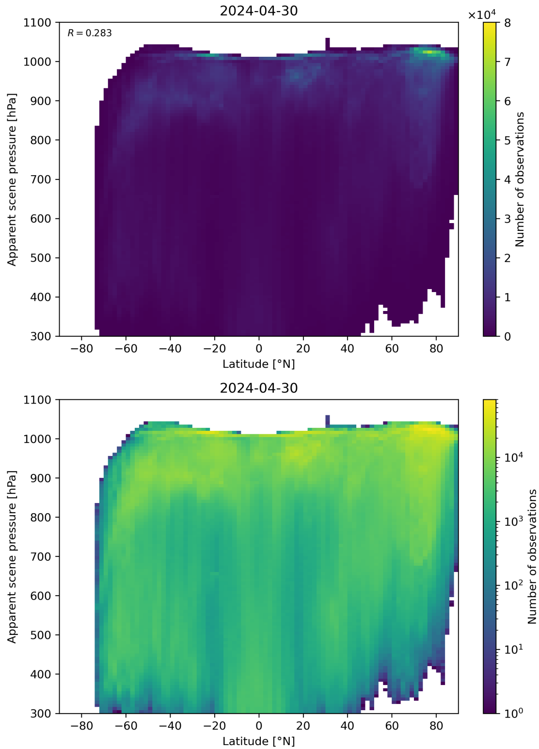
Figure 88: Scatter density plot of “Latitude” against “Apparent scene pressure” for 2024-04-29 to 2024-05-01.
