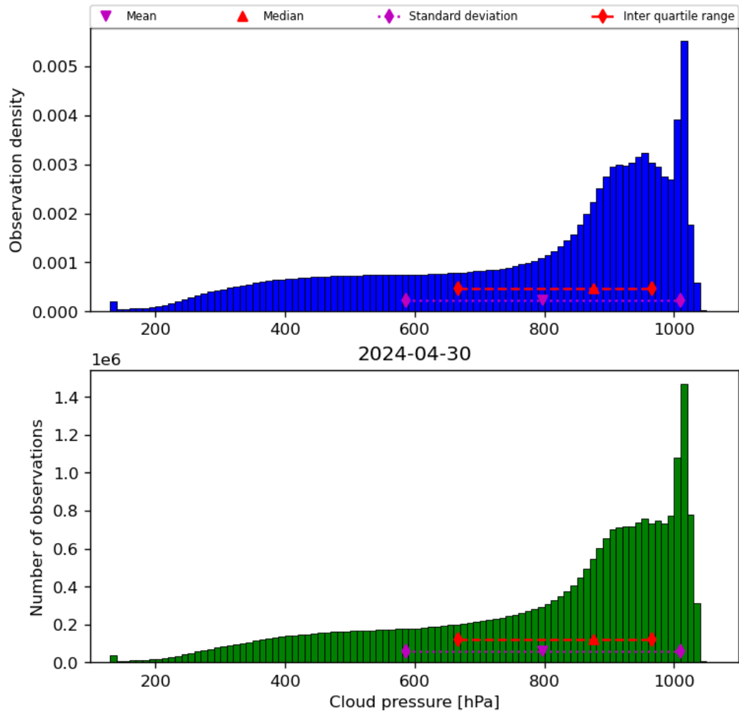
Figure 30: Histogram of “Cloud pressure” for 2024-04-29 to 2024-05-01
