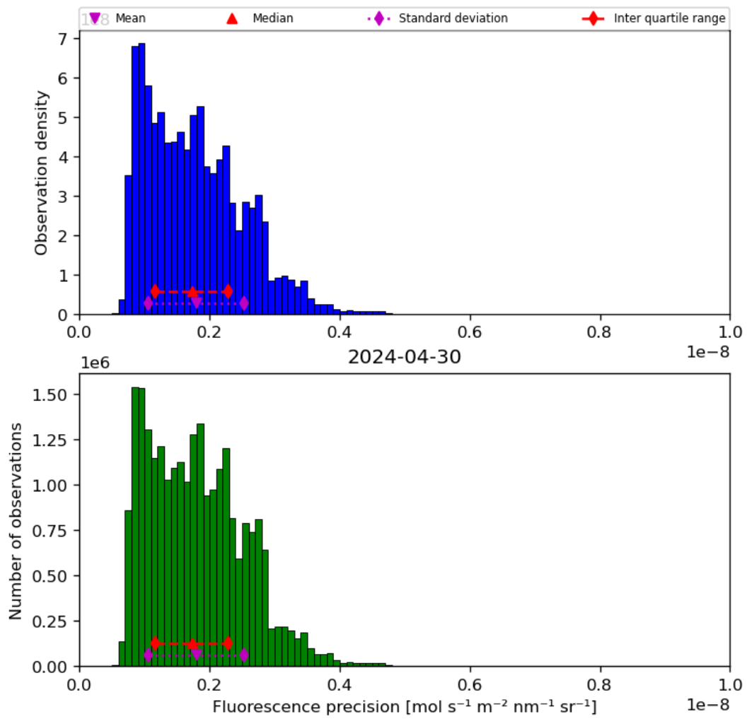
Figure 41: Histogram of “Fluorescence precision” for 2024-04-29 to 2024-05-01
