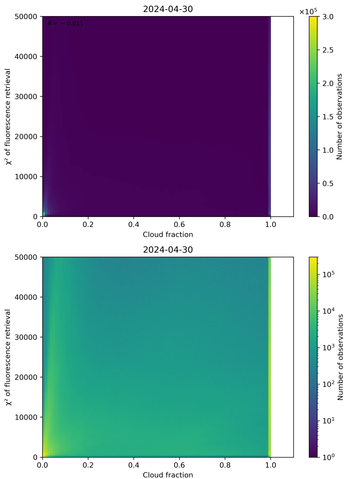
Figure 71: Scatter density plot of “Cloud fraction” against “ \chi^2 of fluorescence retrieval” for 2024-04-29 to 2024-05-01.
