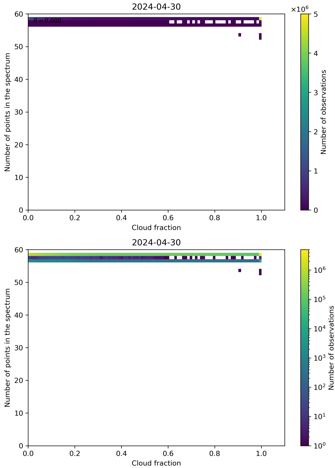
Figure 74: Scatter density plot of “Cloud fraction” against “Number of points in the spectrum” for 2024-04-29 to 2024-05-01.
