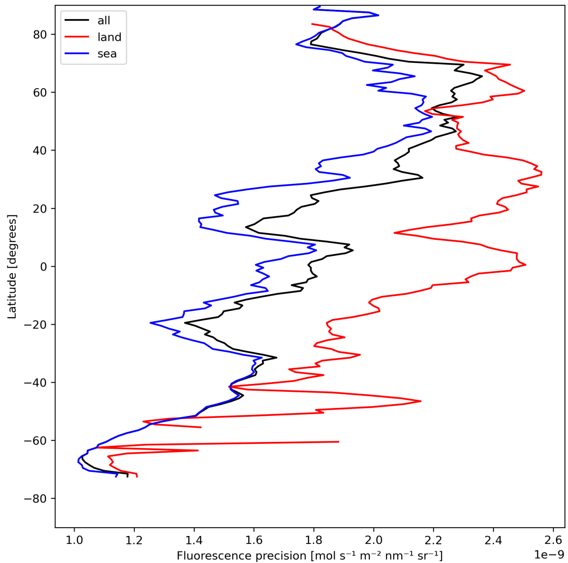
Figure 24: Zonal average of “Fluorescence precision” for 2024-04-29 to 2024-05-01.
