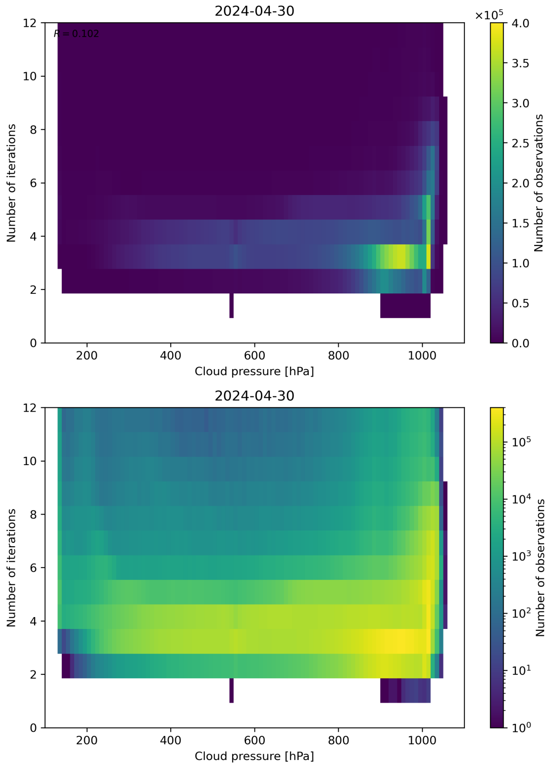
Figure 81: Scatter density plot of “Cloud pressure” against “Number of iterations” for 2024-04-29 to 2024-05-01.
