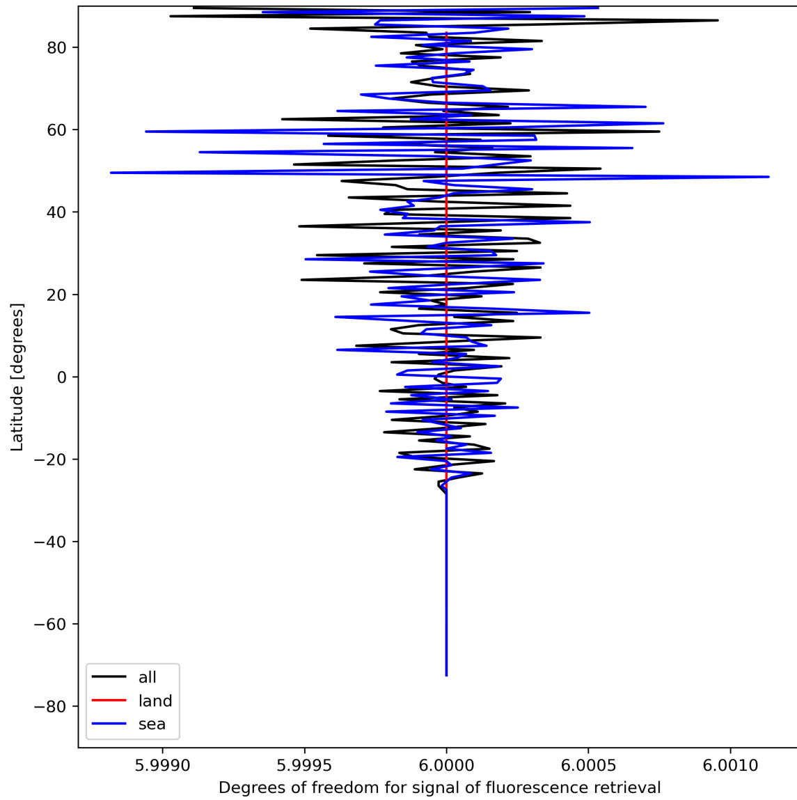
Figure 26: Zonal average of “Degrees of freedom for signal of fluorescence retrieval” for 2024-04-29 to 2024-05-01.
