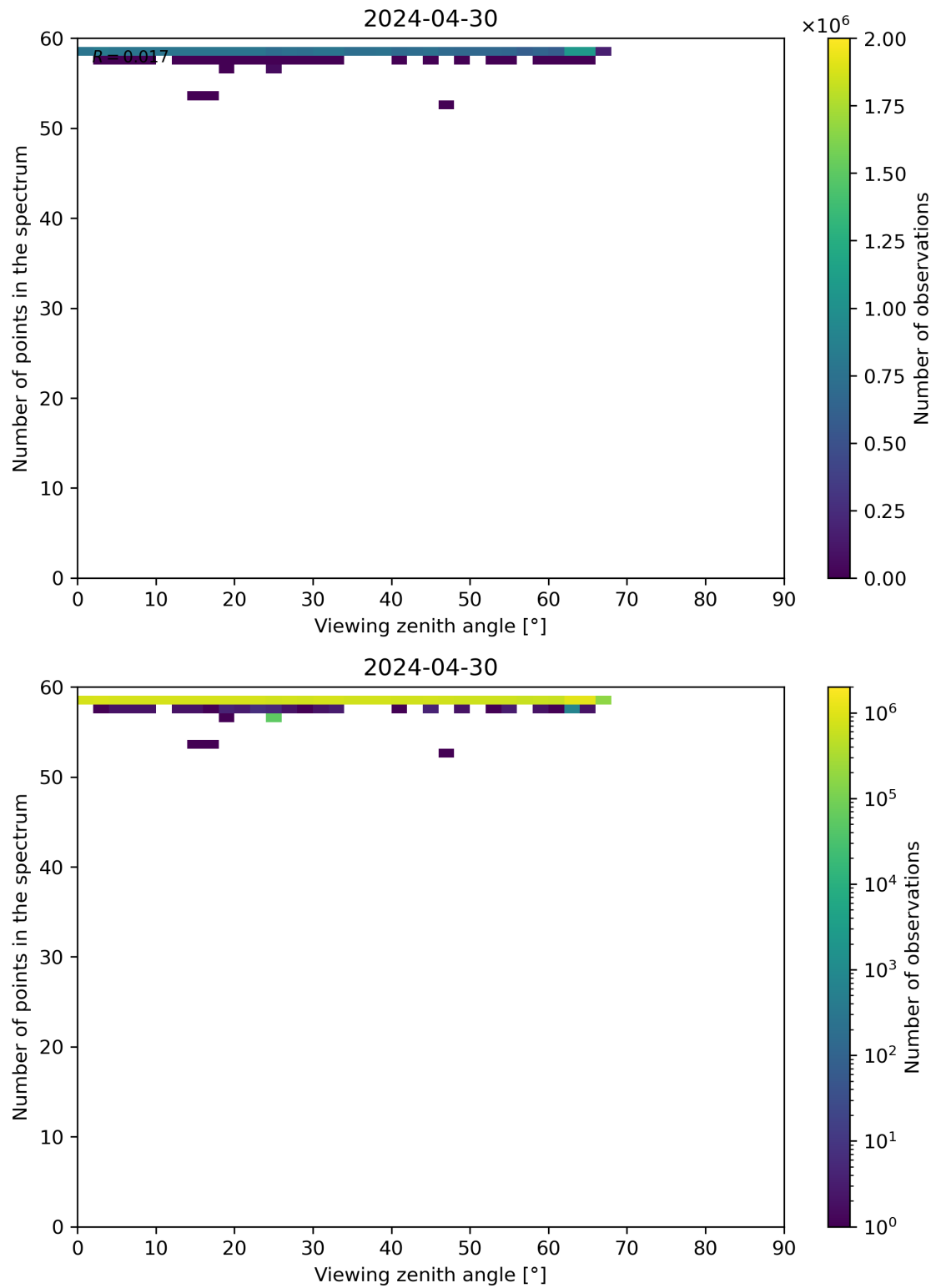
Figure 125: Scatter density plot of “Viewing zenith angle” against “Number of points in the spectrum” for 2024-04-29 to 2024-05-01.
