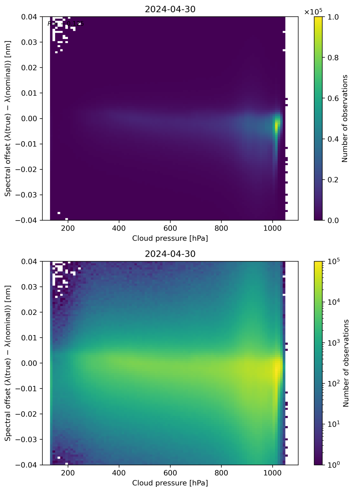
Figure 84: Scatter density plot of “Cloud pressure” against “Spectral offset ( \lambda(\text{true}) - \lambda(\text{nominal}) )” for 2024-04-29 to 2024-05-01.
