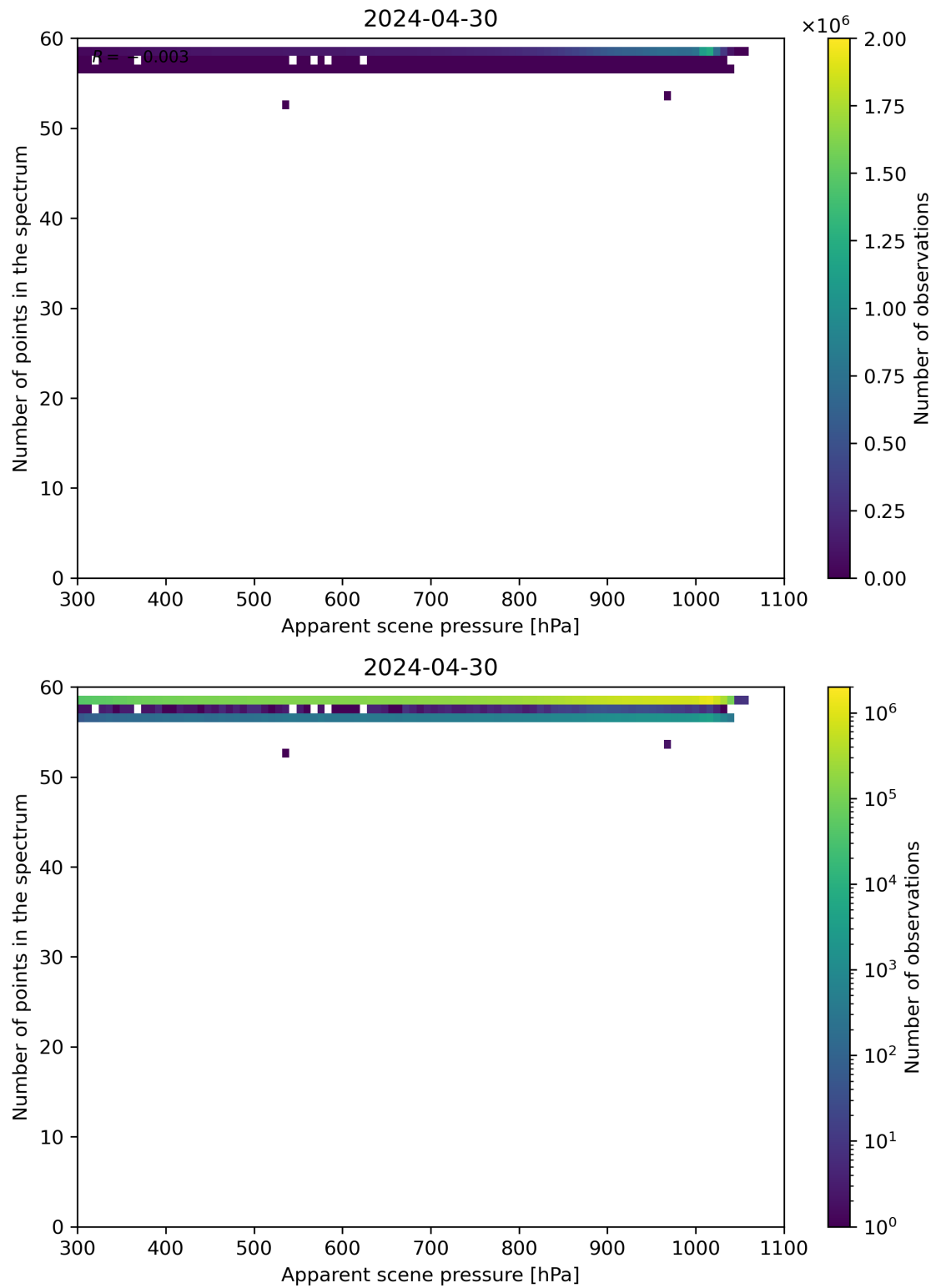
Figure 66: Scatter density plot of “Apparent scene pressure” against “Number of points in the spectrum” for 2024-04-29 to 2024-05-01.
