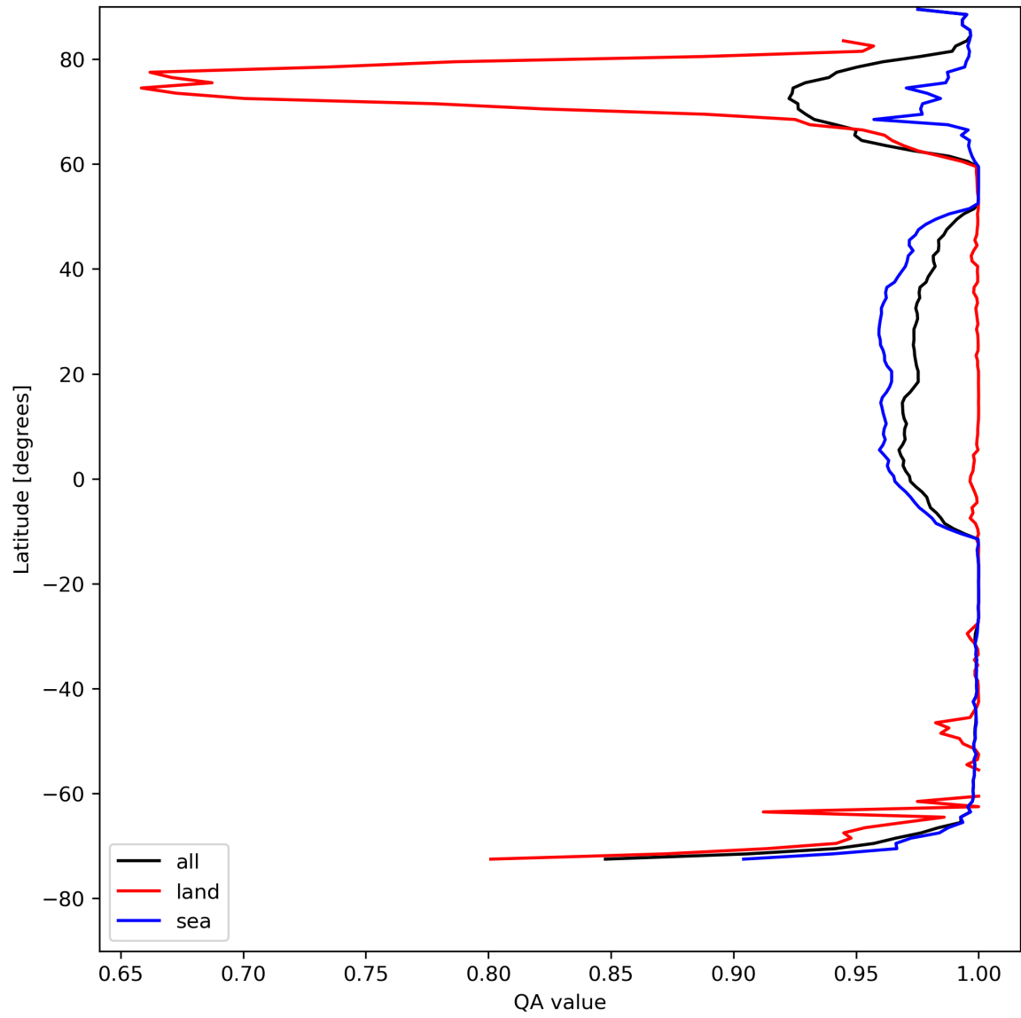
Figure 12: Zonal average of “QA value” for 2024-04-29 to 2024-05-01.
