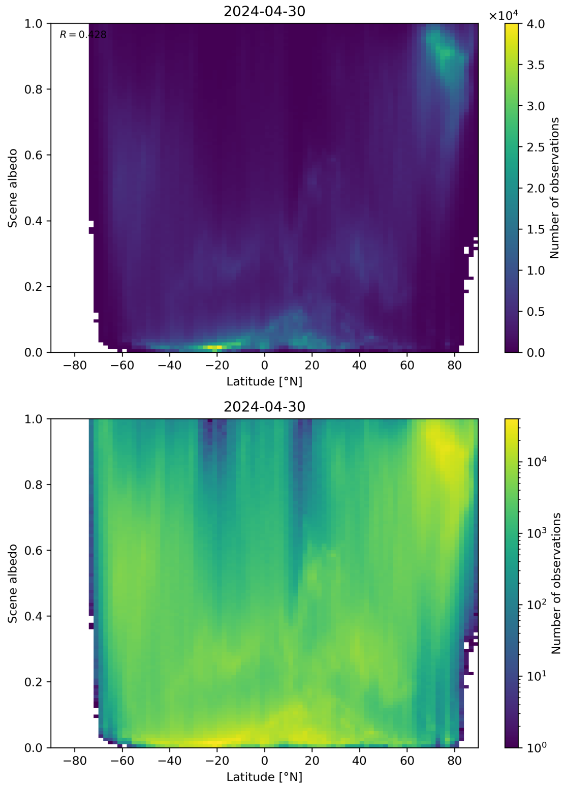
Figure 95: Scatter density plot of “Latitude” against “Scene albedo” for 2024-04-29 to 2024-05-01.
