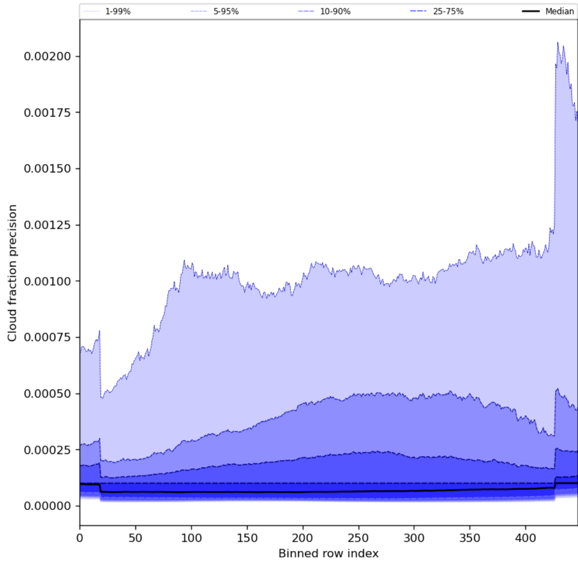
Figure 50: Along track statistics of “Cloud fraction precision” for 2024-04-29 to 2024-05-01
