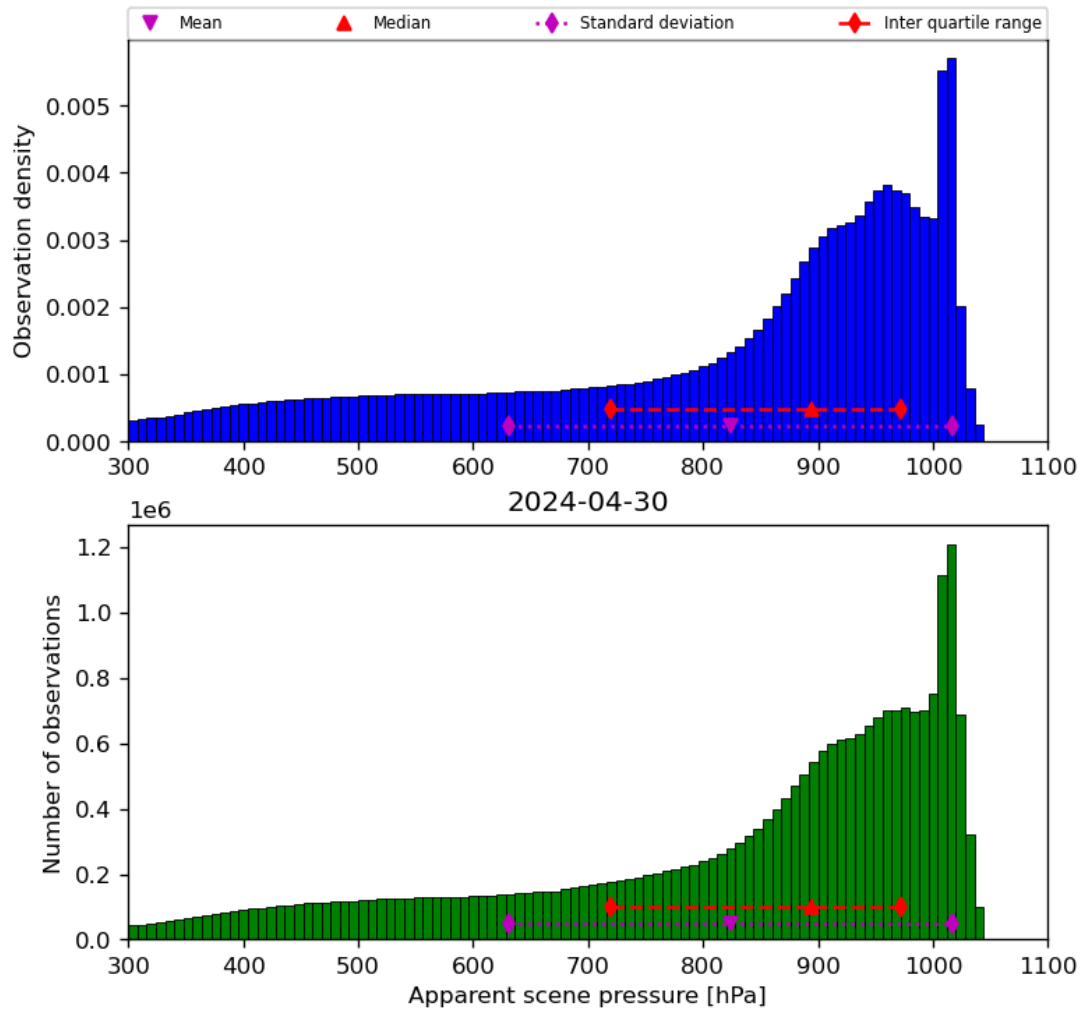
Figure 36: Histogram of “Apparent scene pressure” for 2024-04-29 to 2024-05-01
