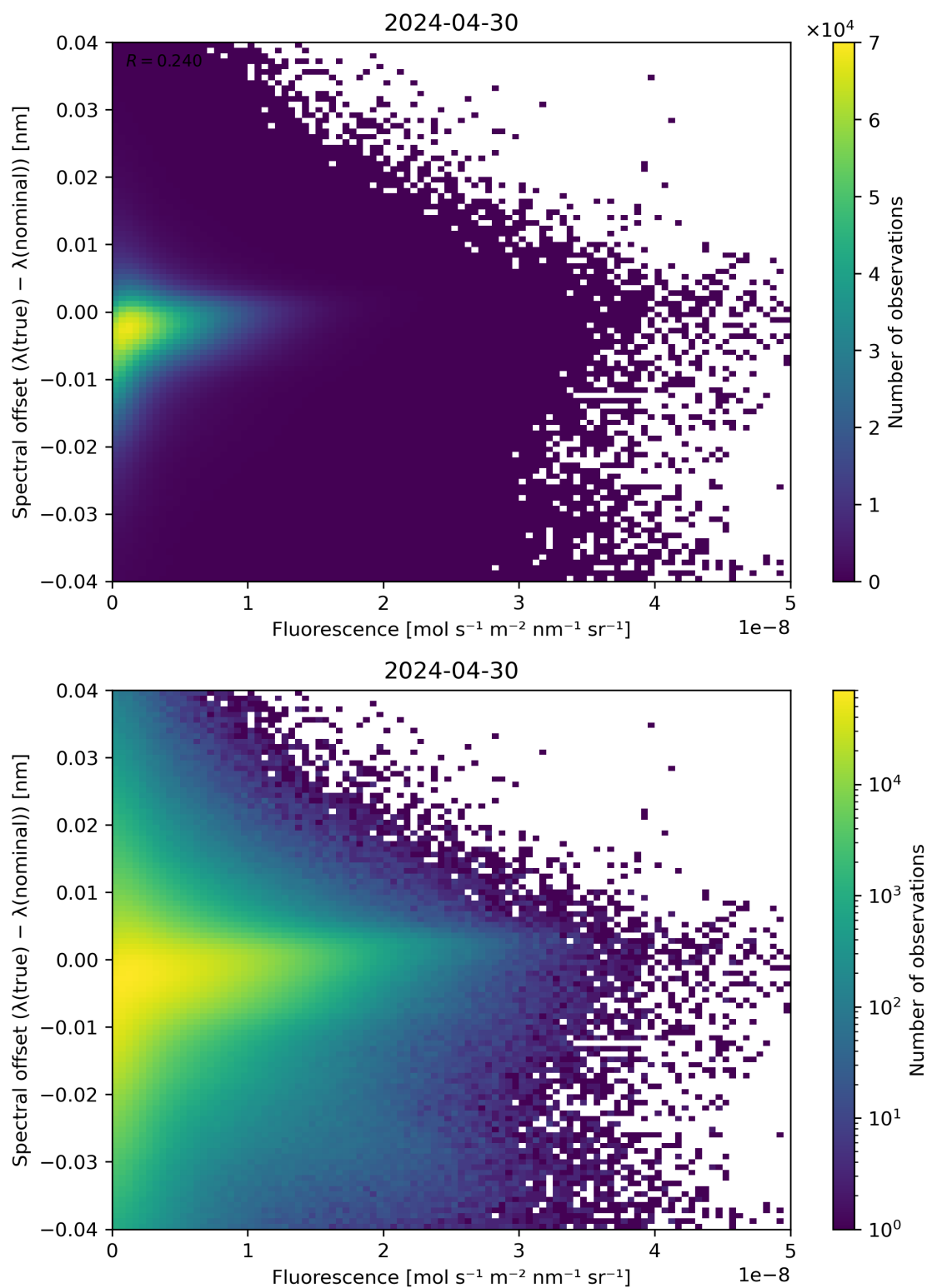
Figure 87: Scatter density plot of “Fluorescence” against “Spectral offset ( \lambda(\text{true}) - \lambda(\text{nominal}) )” for 2024-04-29 to 2024-05-01.
