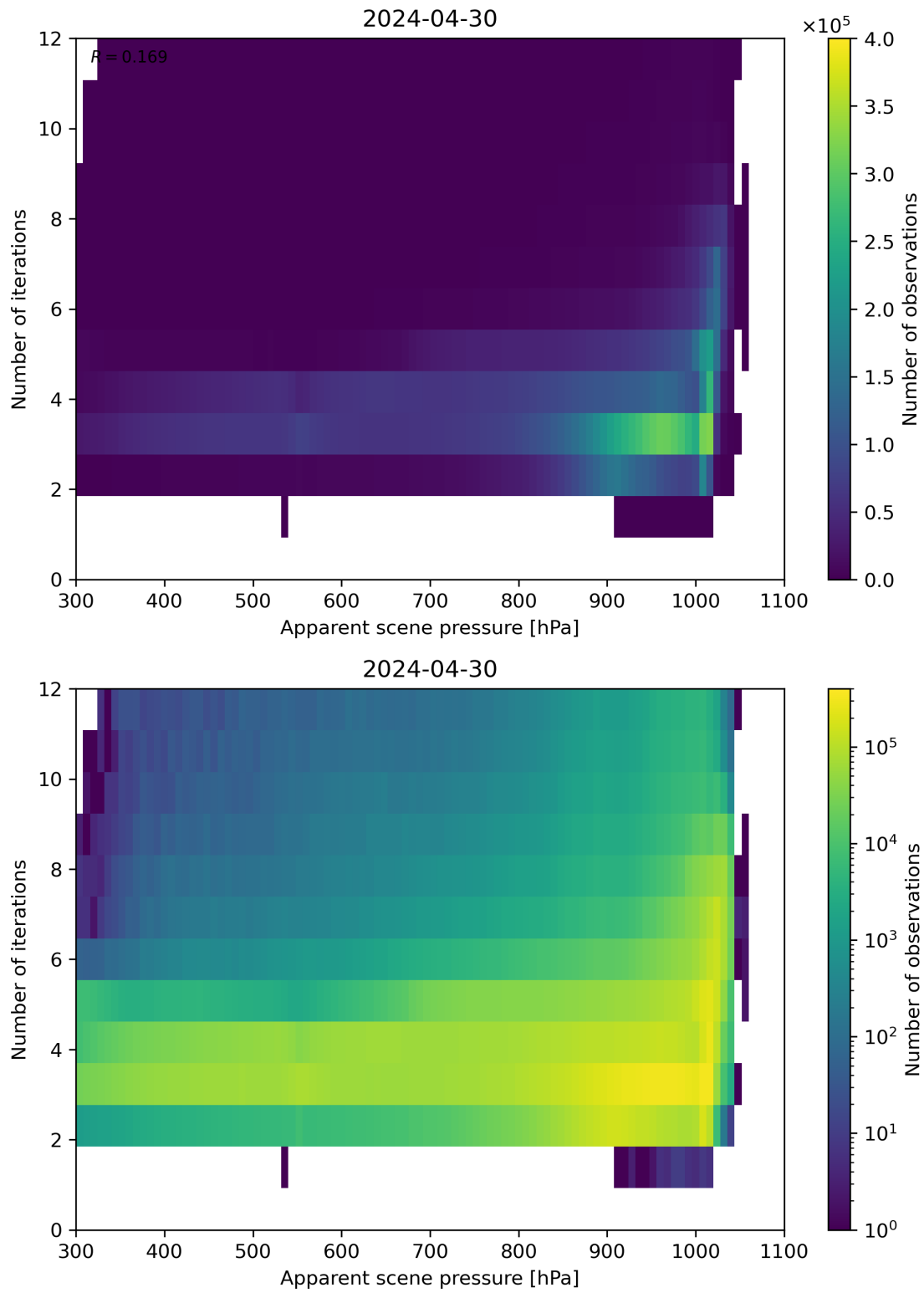
Figure 65: Scatter density plot of “Apparent scene pressure” against “Number of iterations” for 2024-04-29 to 2024-05-01.
