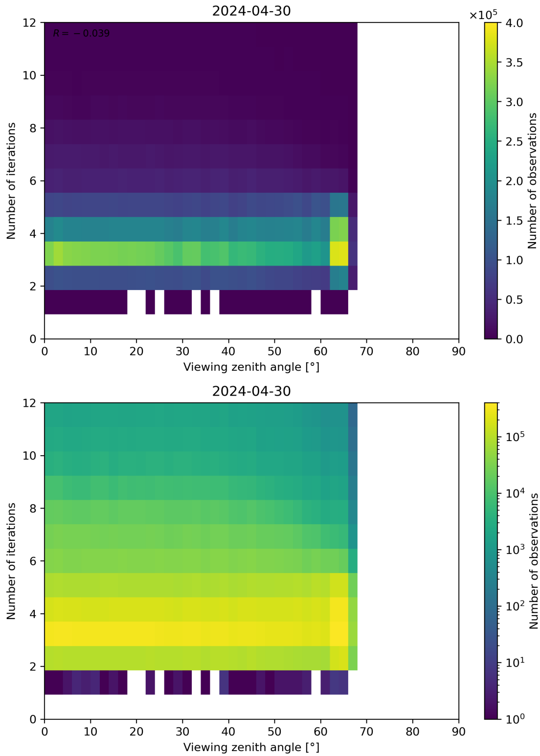
Figure 124: Scatter density plot of “Viewing zenith angle” against “Number of iterations” for 2024-04-29 to 2024-05-01.
