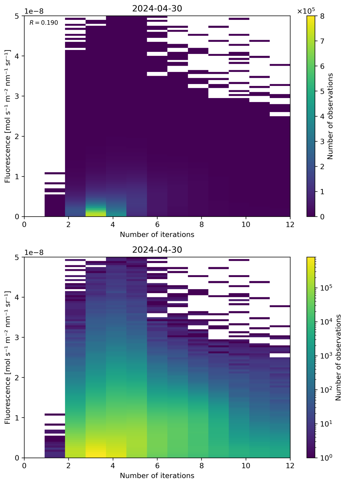
Figure 98: Scatter density plot of “Number of iterations” against “Fluorescence” for 2024-04-29 to 2024-05-01.
