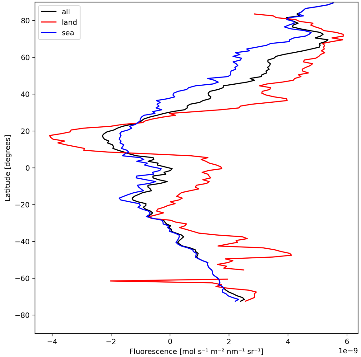
Figure 23: Zonal average of “Fluorescence” for 2024-04-29 to 2024-05-01.
