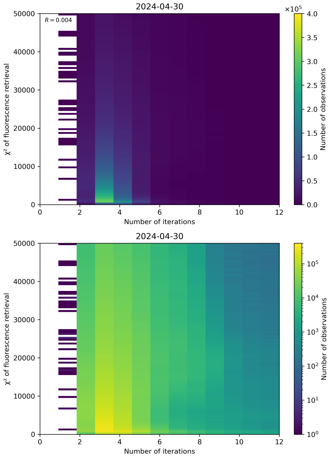
Figure 97: Scatter density plot of “Number of iterations” against “ \chi^2 of fluorescence retrieval” for 2024-04-29 to 2024-05-01.
