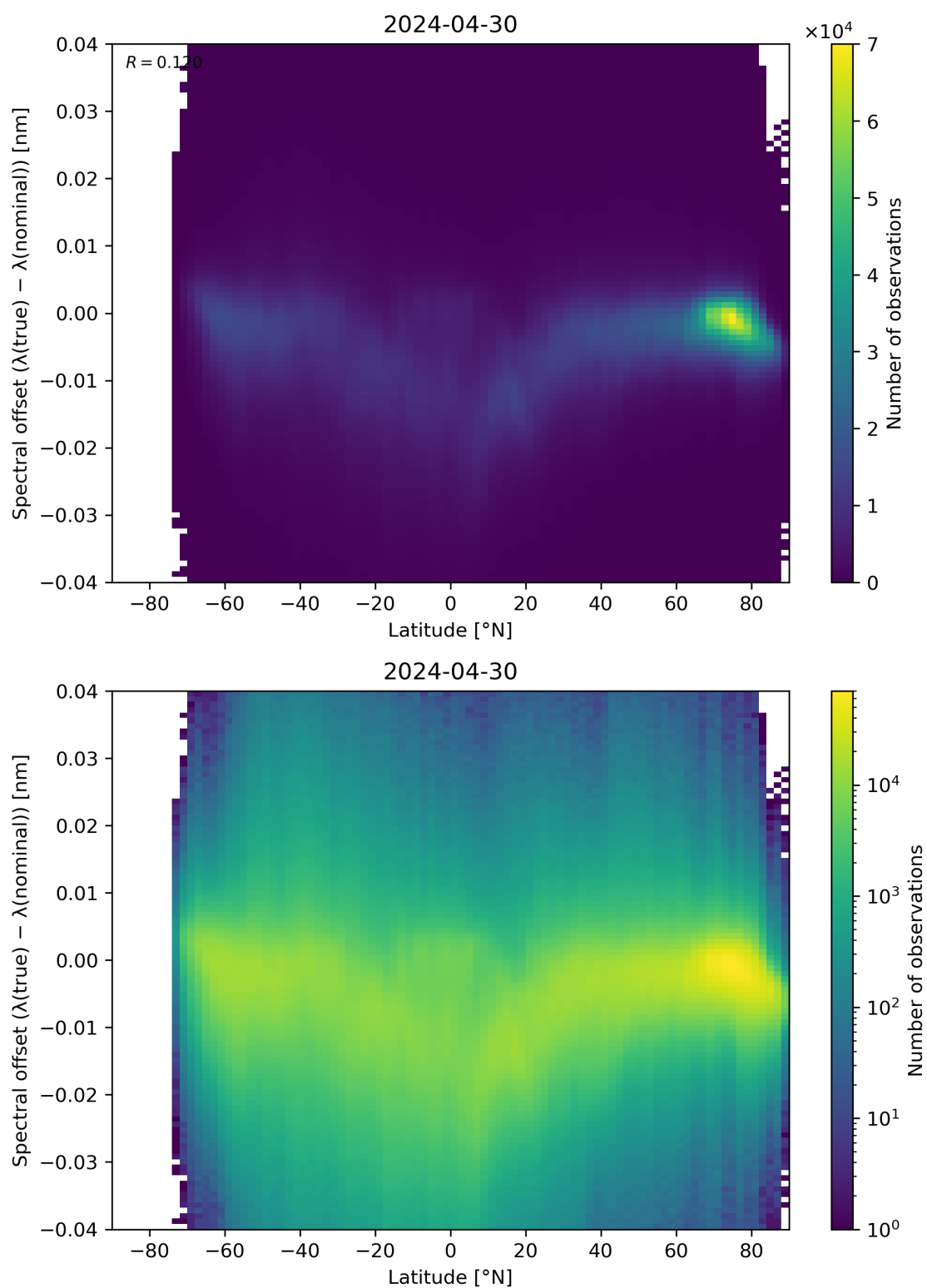
Figure 96: Scatter density plot of “Latitude” against “Spectral offset ( \lambda(\text{true}) - \lambda(\text{nominal}) )” for 2024-04-29 to 2024-05-01.
