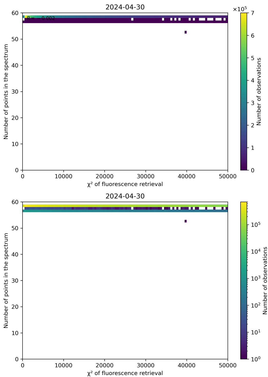
Figure 68: Scatter density plot of " \chi^2 of fluorescence retrieval" against "Number of points in the spectrum" for 2024-04-29 to 2024-05-01.
