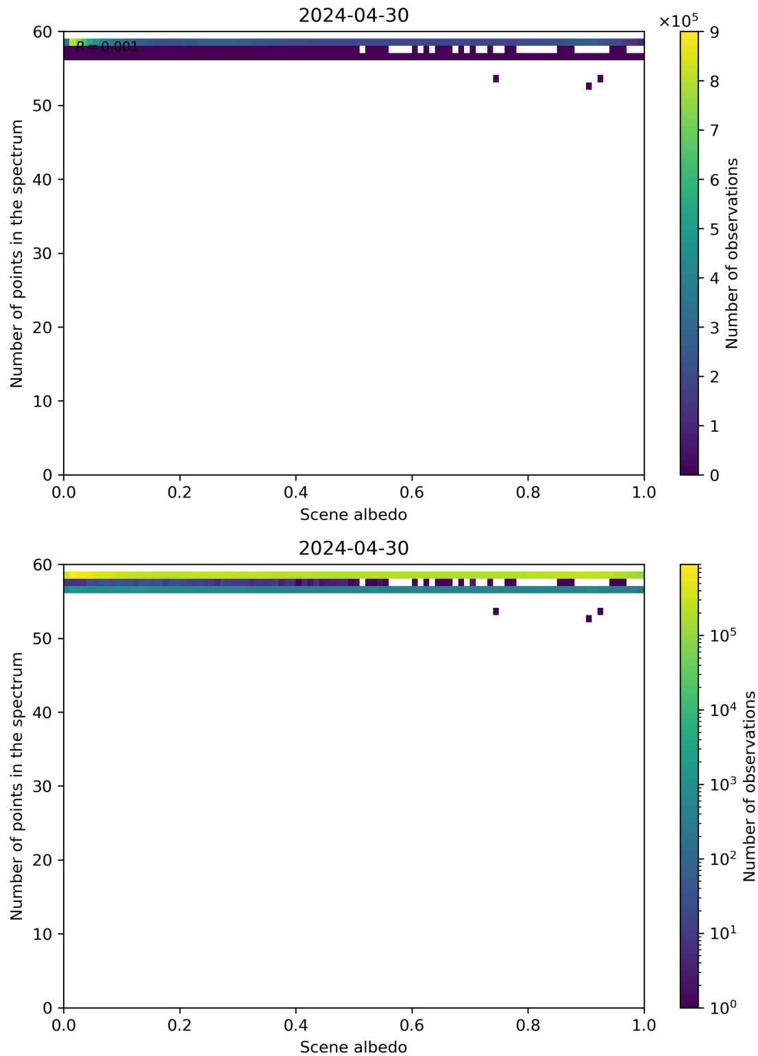
Figure 106: Scatter density plot of “Scene albedo” against “Number of points in the spectrum” for 2024-04-29 to 2024-05-01.
