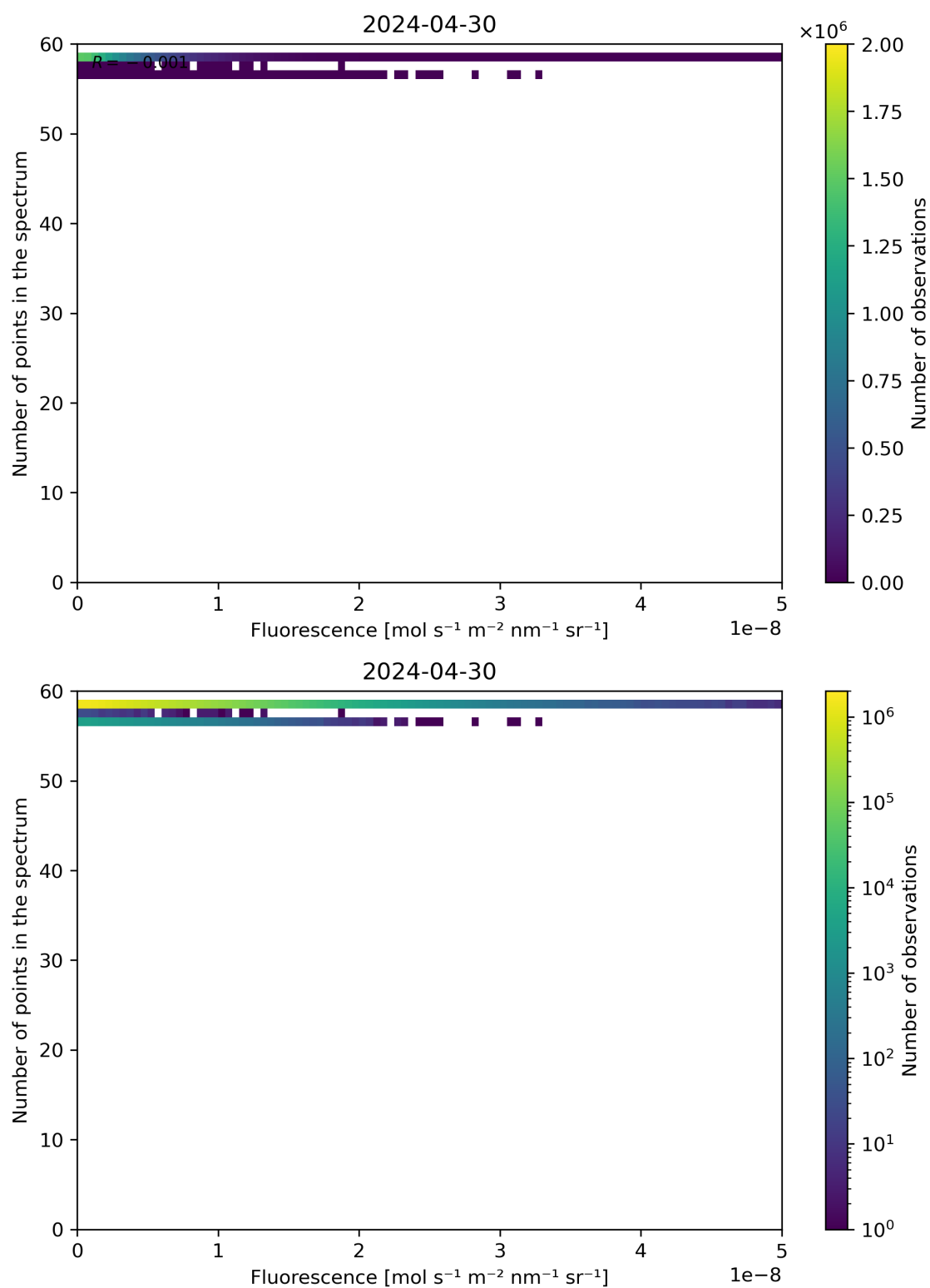
Figure 86: Scatter density plot of “Fluorescence” against “Number of points in the spectrum” for 2024-04-29 to 2024-05-01.
