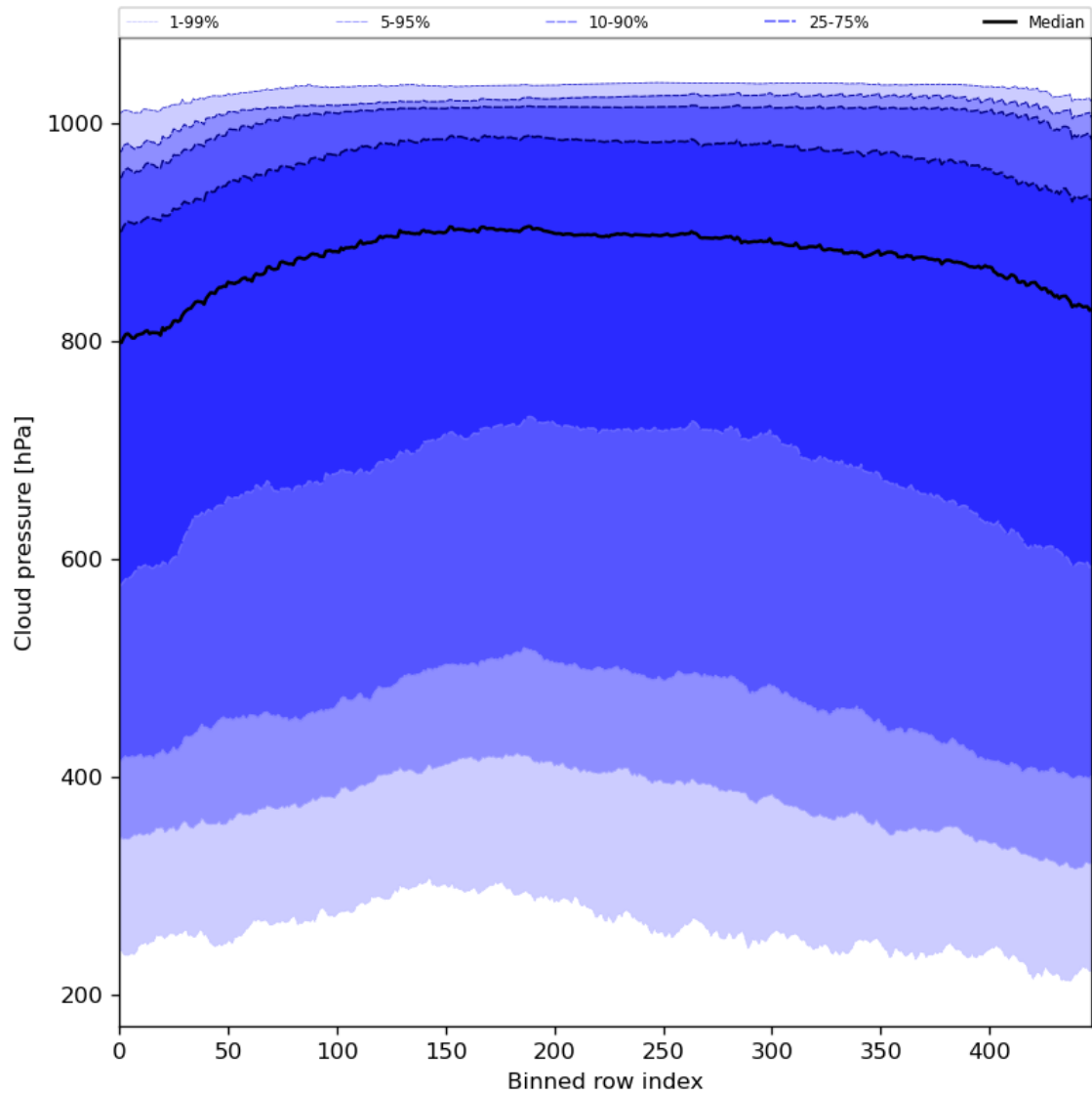
Figure 47: Along track statistics of “Cloud pressure” for 2024-04-30 to 2024-05-02
