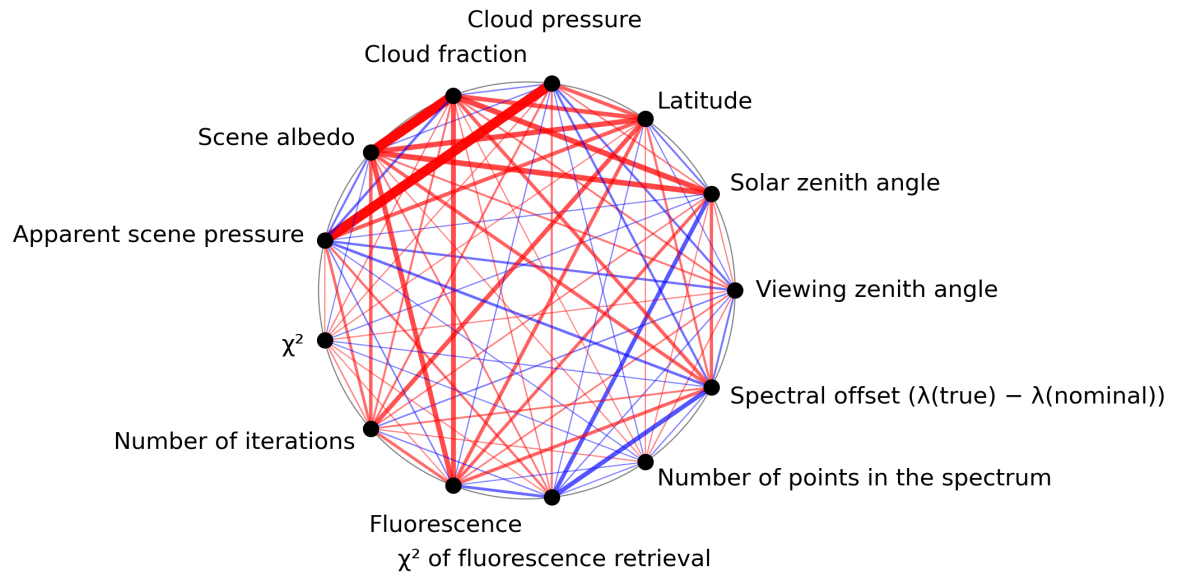
Figure 1: Map of correlation graph for 2024-04-30 to 2024-05-02.
