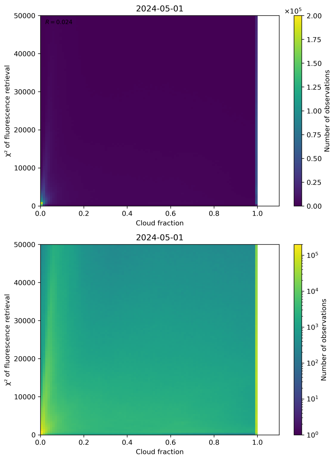
Figure 71: Scatter density plot of “Cloud fraction” against “ \chi^2 of fluorescence retrieval” for 2024-04-30 to 2024-05-02.
