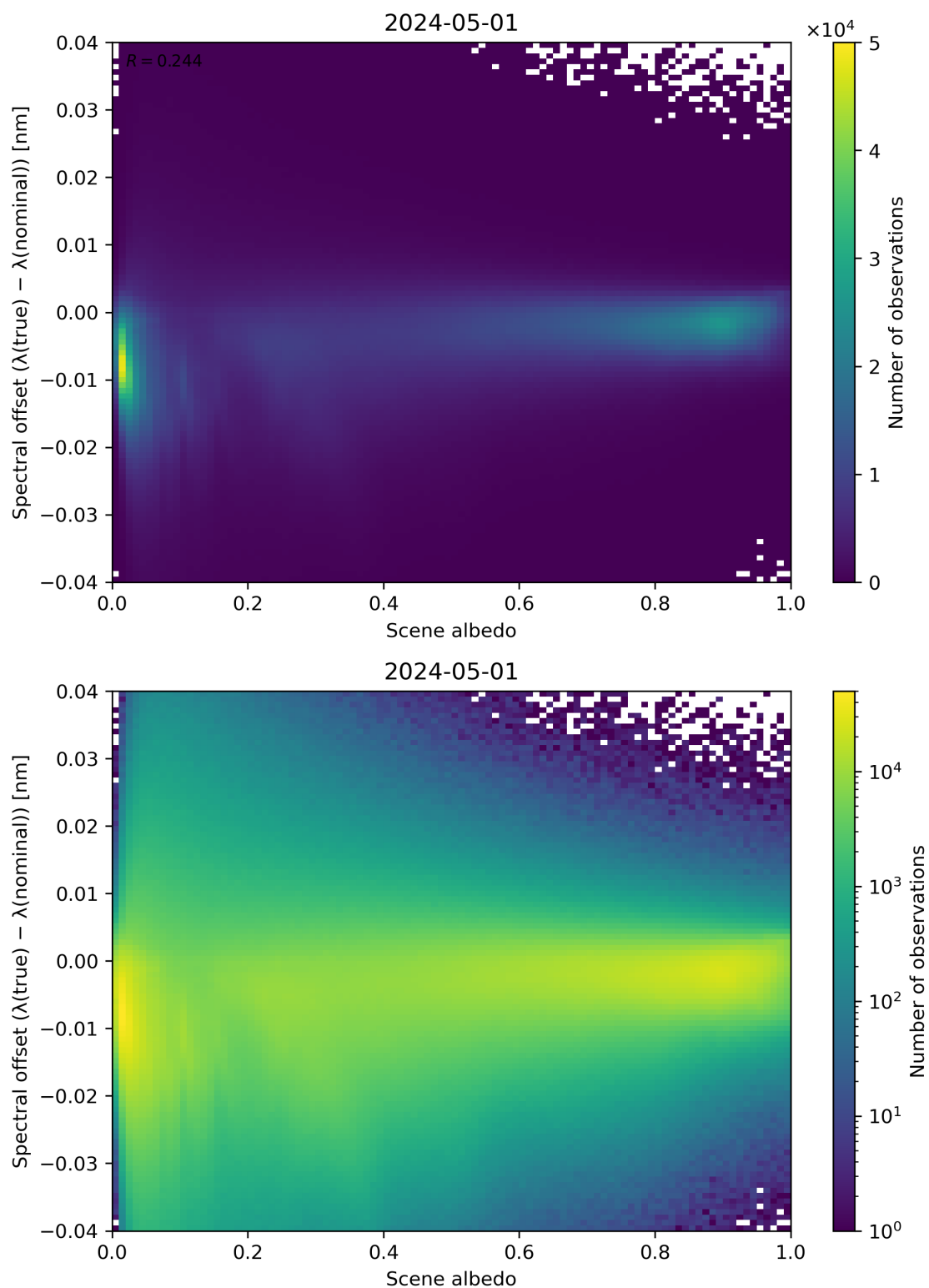
Figure 107: Scatter density plot of “Scene albedo” against “Spectral offset ( \lambda(\text{true}) - \lambda(\text{nominal}) )” for 2024-04-30 to 2024-05-02.
