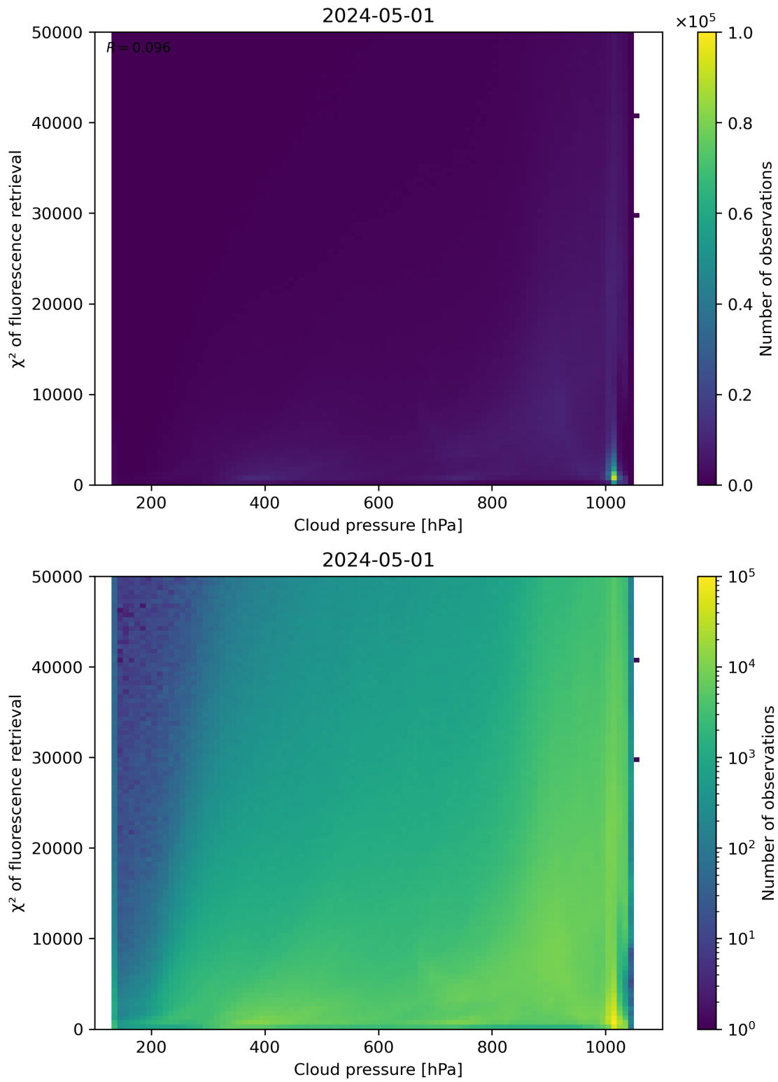
Figure 78: Scatter density plot of “Cloud pressure” against “ \chi^2 of fluorescence retrieval” for 2024-04-30 to 2024-05-02.
