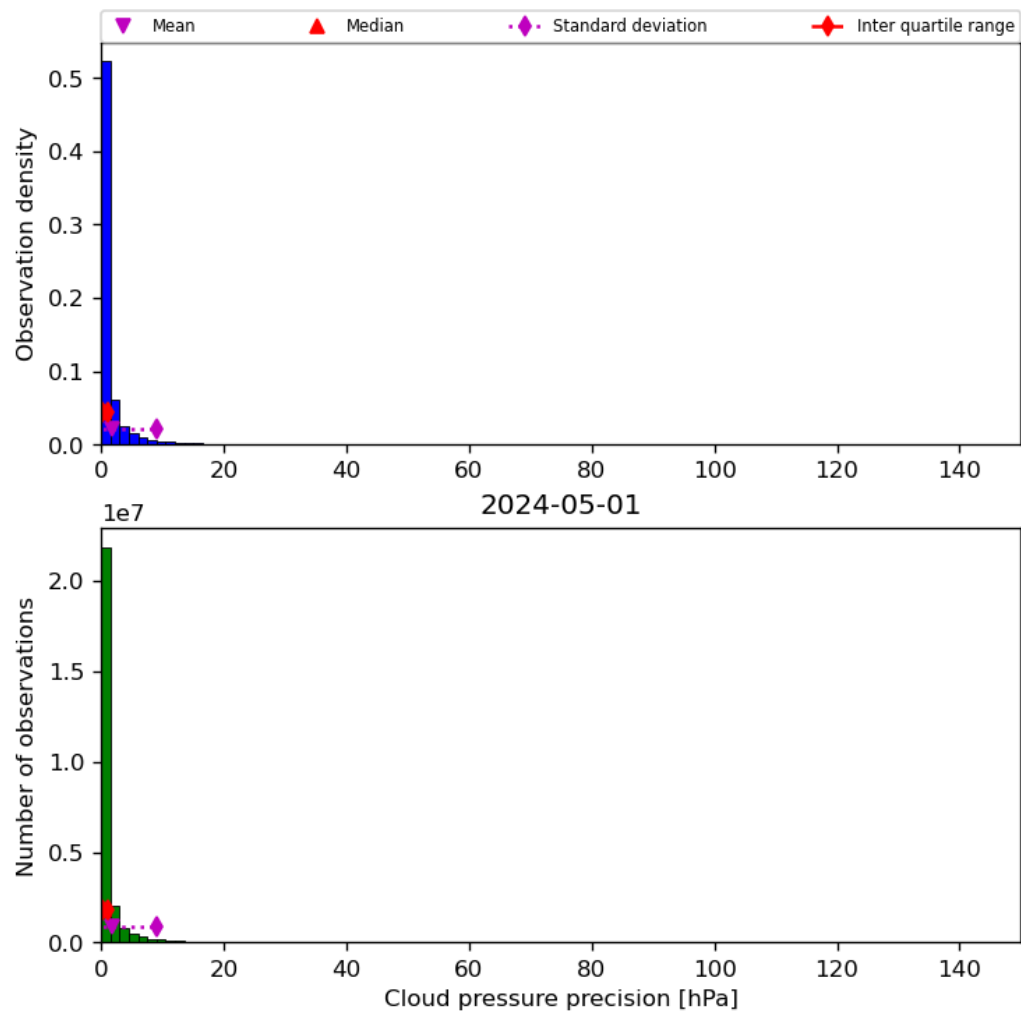
Figure 31: Histogram of “Cloud pressure precision” for 2024-04-30 to 2024-05-02
