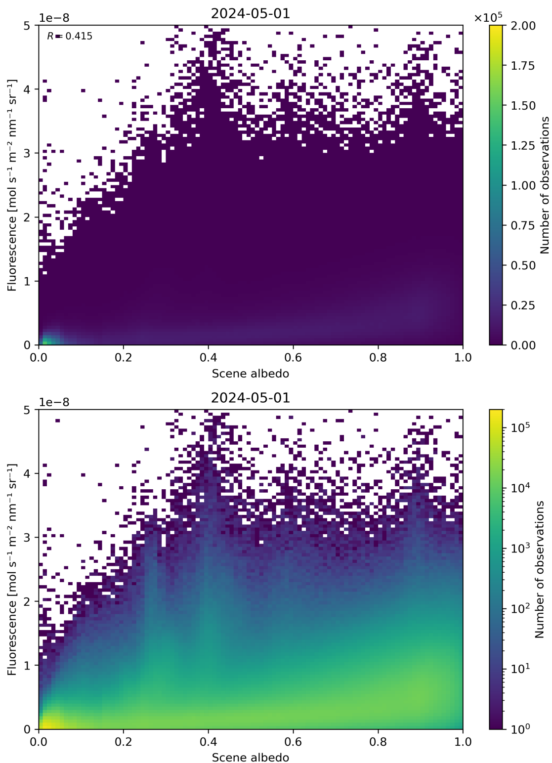
Figure 104: Scatter density plot of “Scene albedo” against “Fluorescence” for 2024-04-30 to 2024-05-02.
