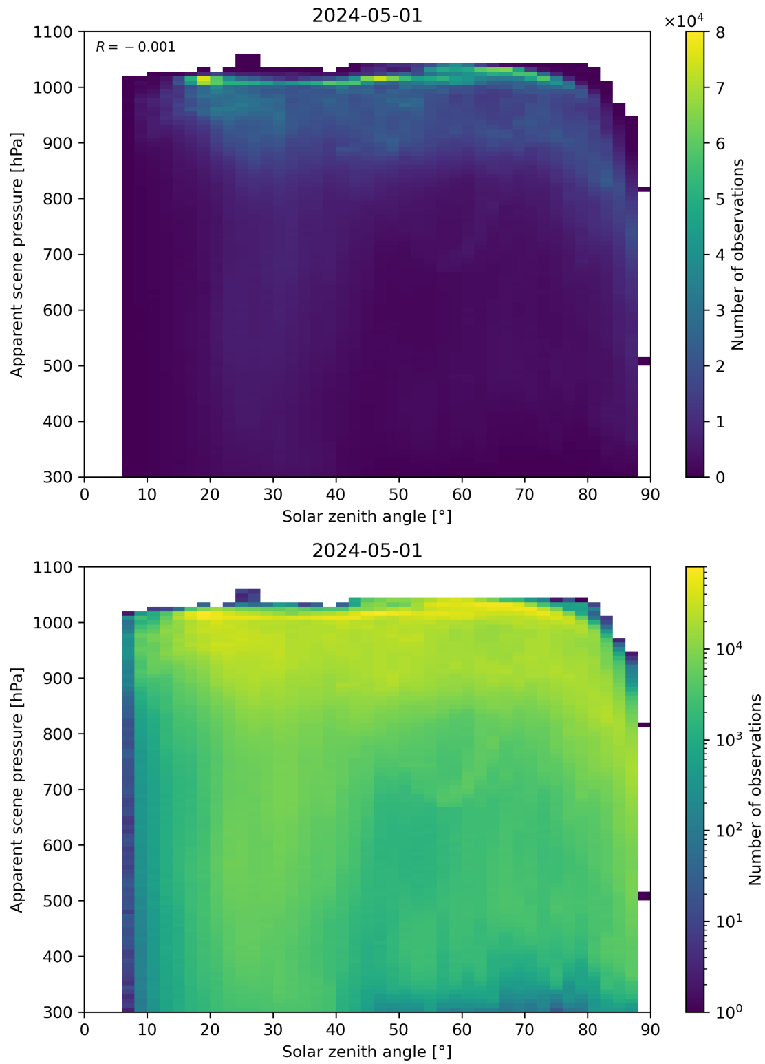
Figure 108: Scatter density plot of “Solar zenith angle” against “Apparent scene pressure” for 2024-04-30 to 2024-05-02.
