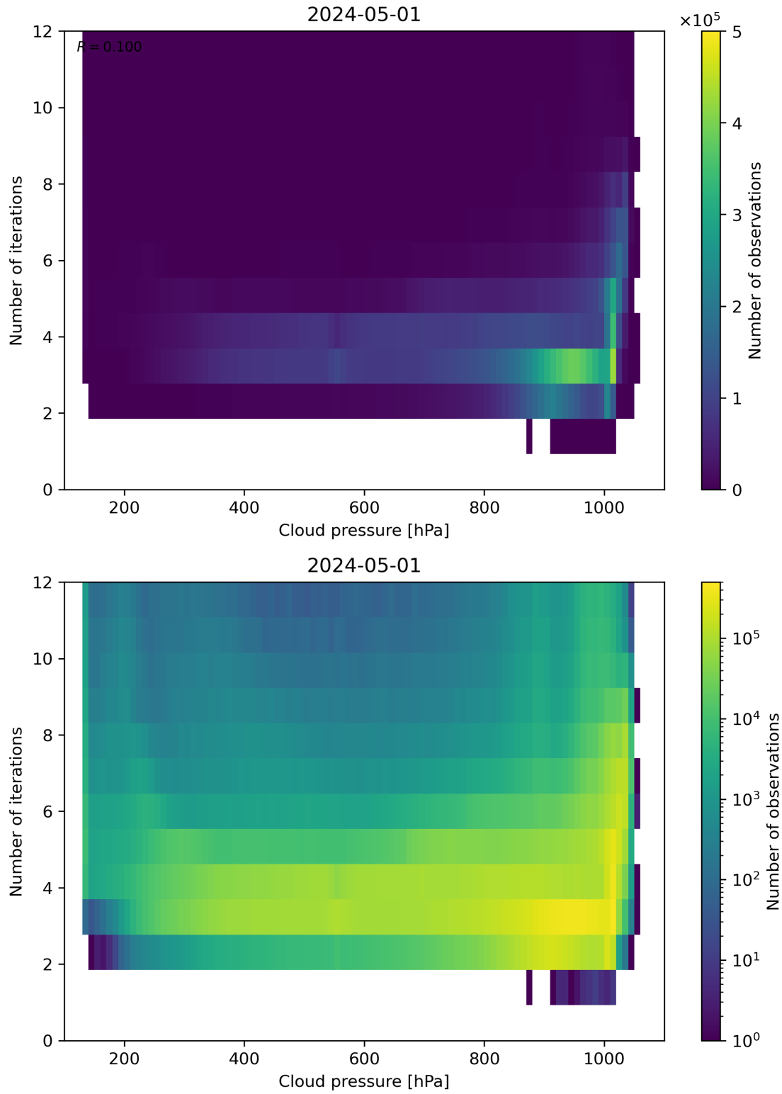
Figure 81: Scatter density plot of “Cloud pressure” against “Number of iterations” for 2024-04-30 to 2024-05-02.
