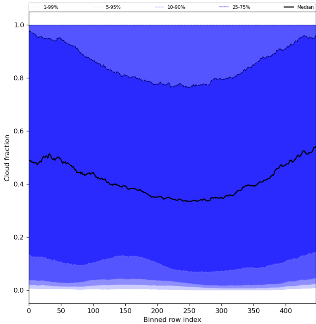
Figure 49: Along track statistics of “Cloud fraction” for 2024-04-30 to 2024-05-02
