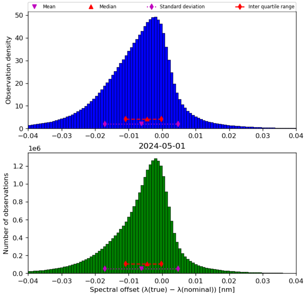
Figure 45: Histogram of “Spectral offset ( \lambda(\text{true}) - \lambda(\text{nominal}) )” for 2024-04-30 to 2024-05-02
