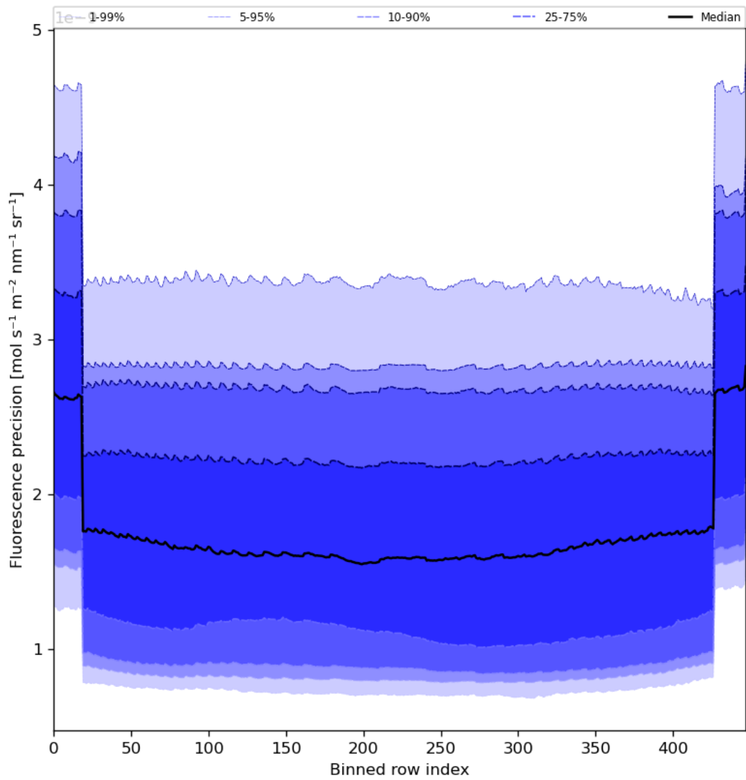
Figure 58: Along track statistics of "Fluorescence precision" for 2024-04-30 to 2024-05-02
