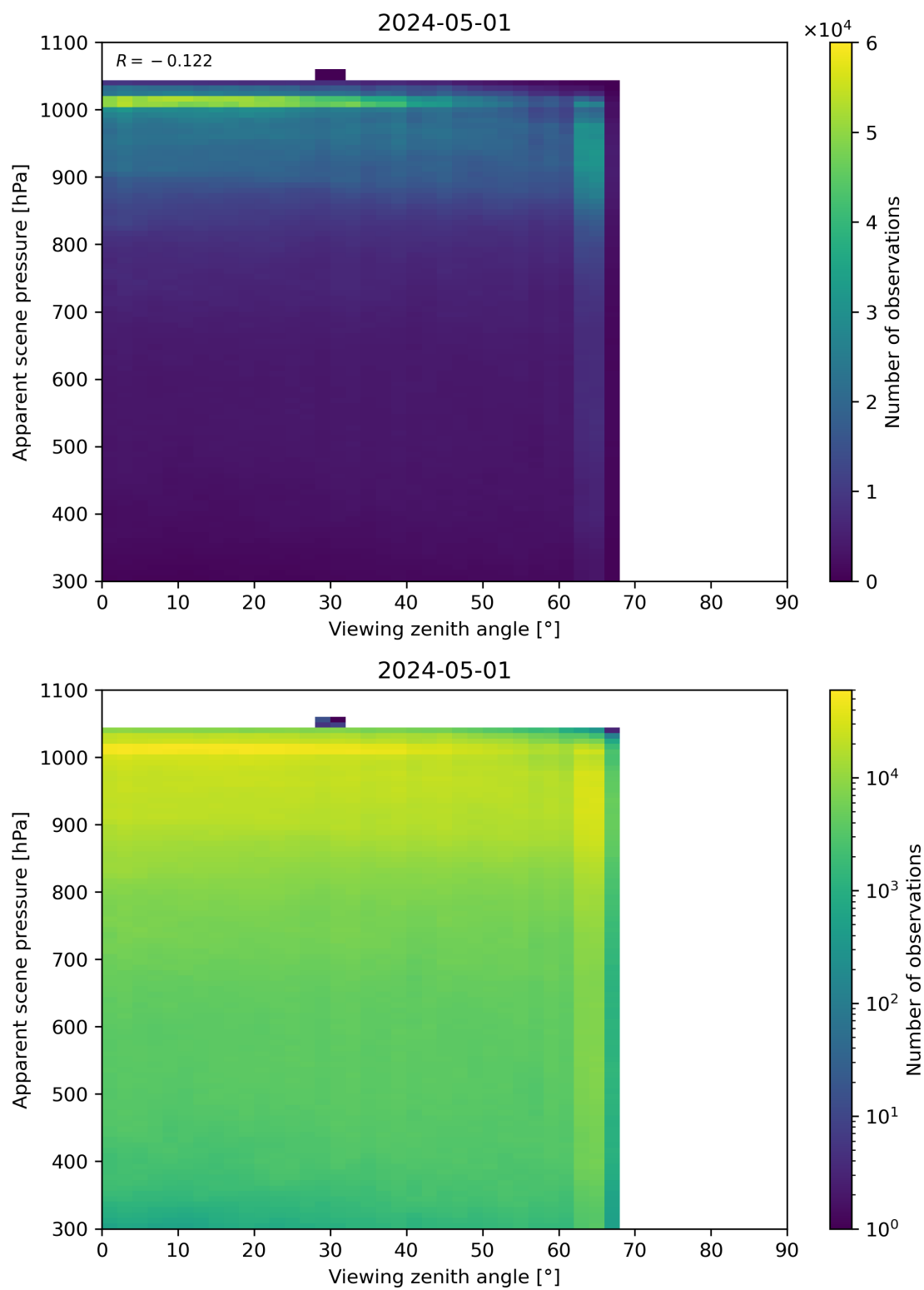
Figure 118: Scatter density plot of “Viewing zenith angle” against “Apparent scene pressure” for 2024-04-30 to 2024-05-02.
