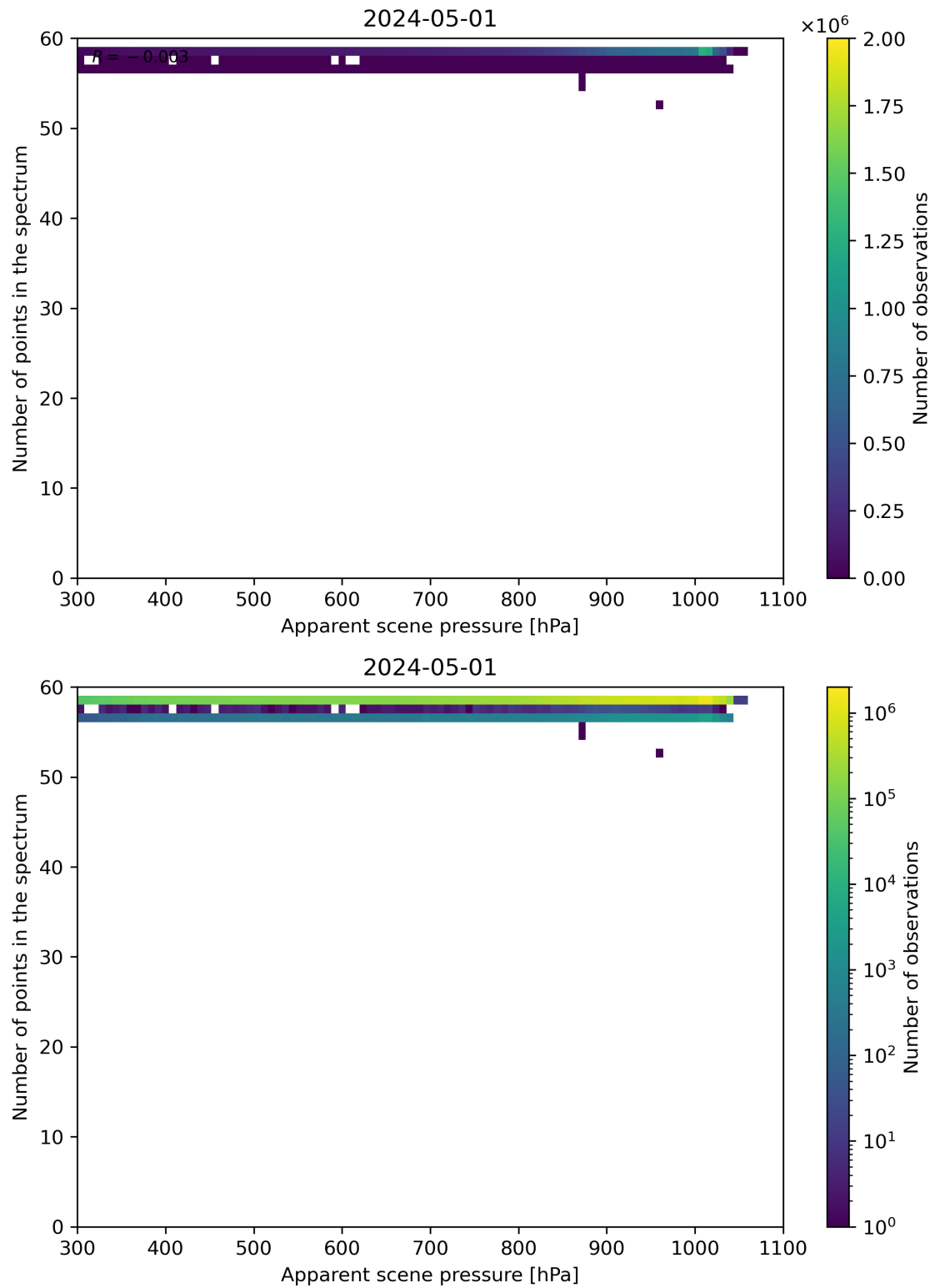
Figure 66: Scatter density plot of “Apparent scene pressure” against “Number of points in the spectrum” for 2024-04-30 to 2024-05-02.
