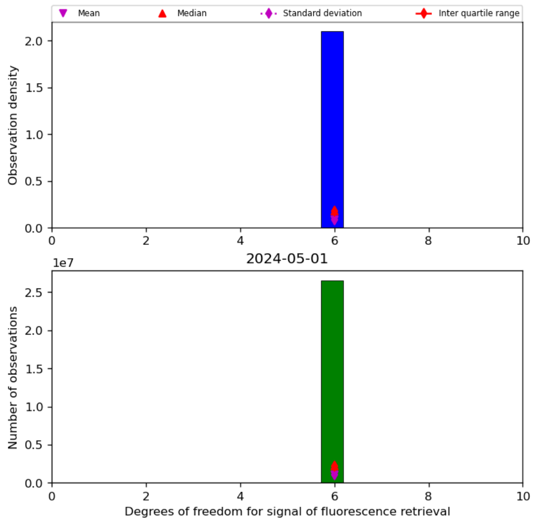
Figure 43: Histogram of “Degrees of freedom for signal of fluorescence retrieval” for 2024-04-30 to 2024-05-02
