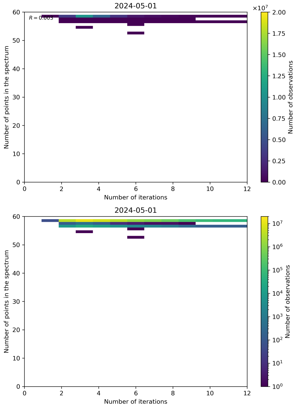
Figure 99: Scatter density plot of “Number of iterations” against “Number of points in the spectrum” for 2024-04-30 to 2024-05-02.
