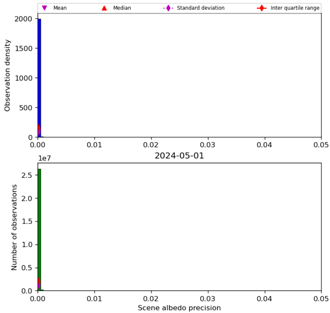
Figure 35: Histogram of “Scene albedo precision” for 2024-04-30 to 2024-05-02
