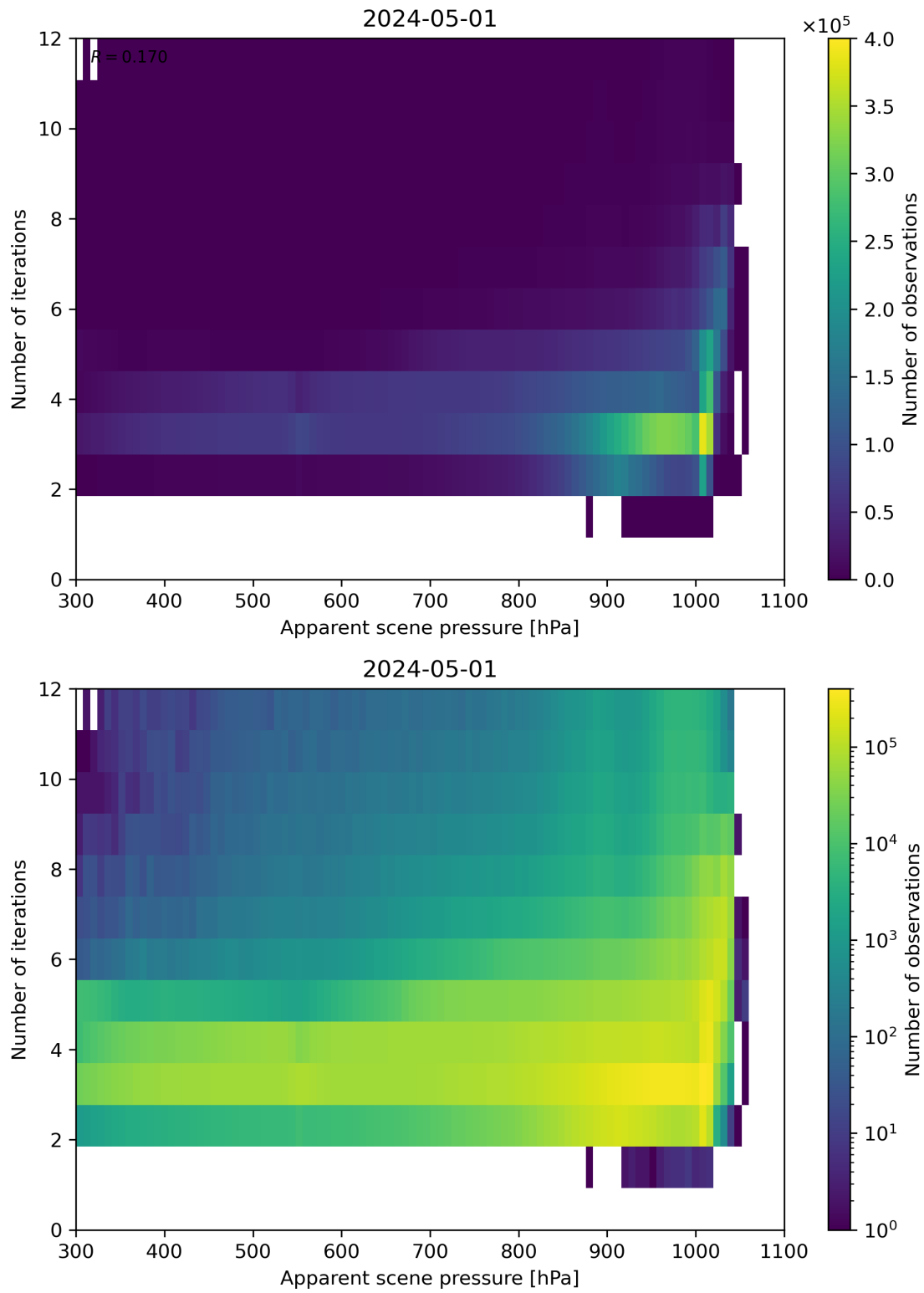
Figure 65: Scatter density plot of “Apparent scene pressure” against “Number of iterations” for 2024-04-30 to 2024-05-02.
