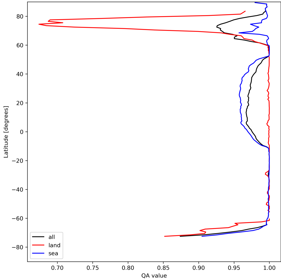
Figure 12: Zonal average of “QA value” for 2024-04-30 to 2024-05-02.
