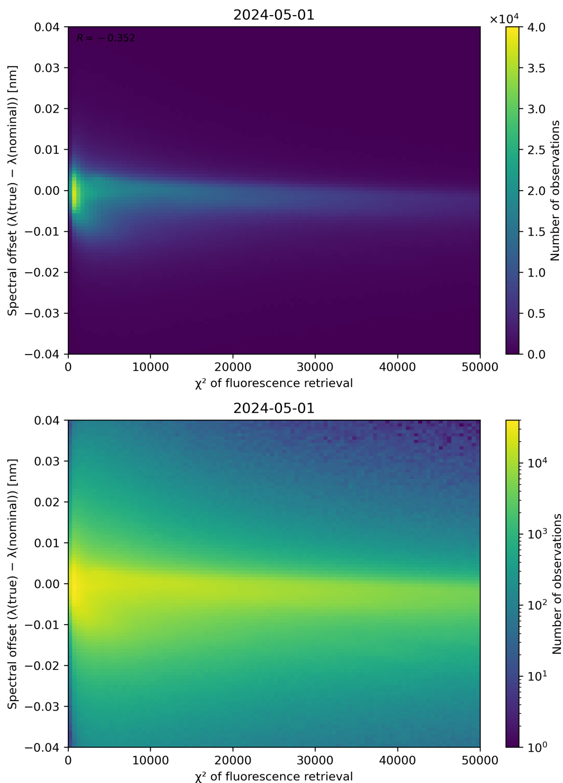
Figure 69: Scatter density plot of " \chi^2 of fluorescence retrieval" against "Spectral offset ( \lambda(\text{true}) - \lambda(\text{nominal})) " for 2024-04-30 to 2024-05-02.
