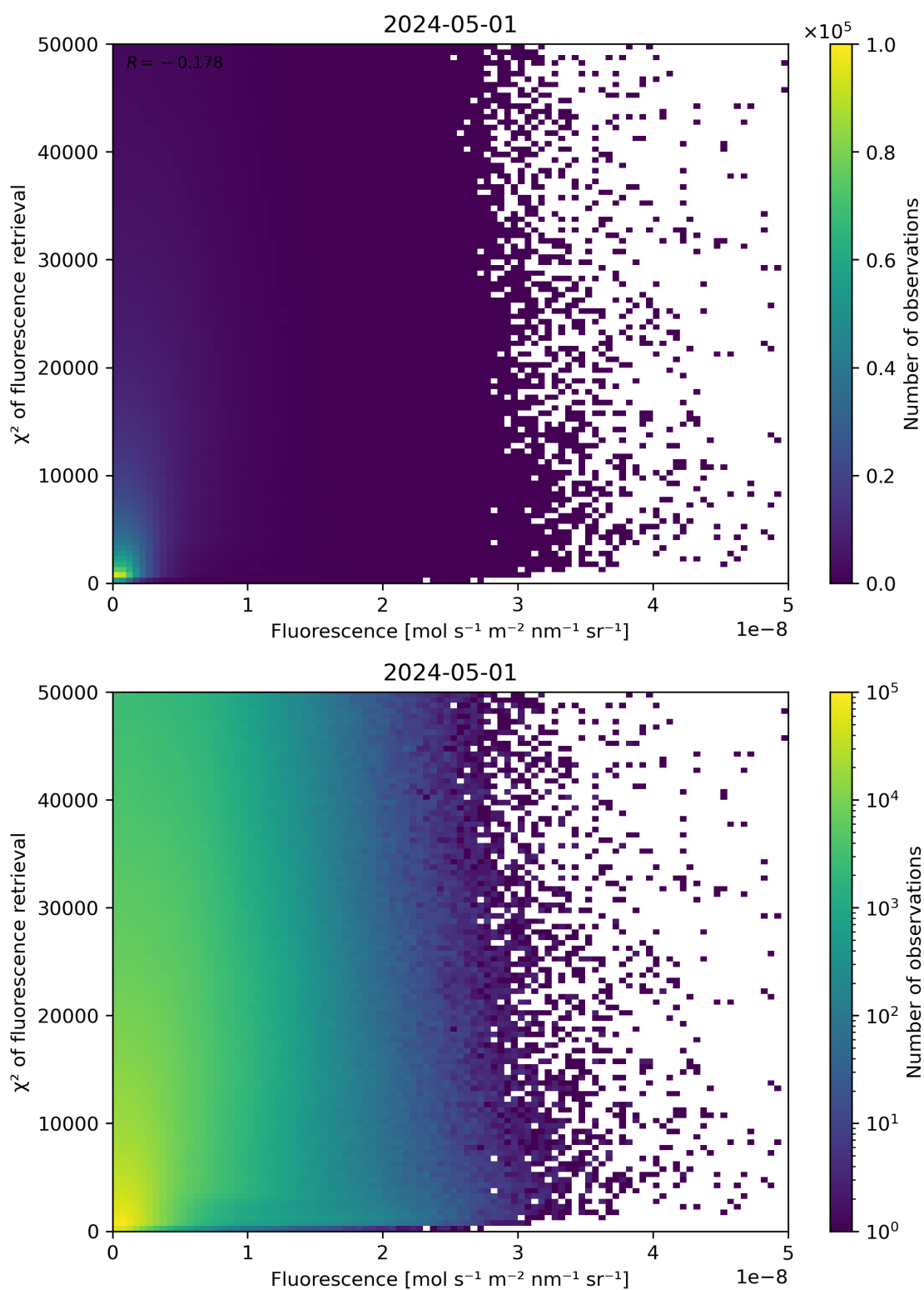
Figure 85: Scatter density plot of “Fluorescence” against “ \chi^2 of fluorescence retrieval” for 2024-04-30 to 2024-05-02.
