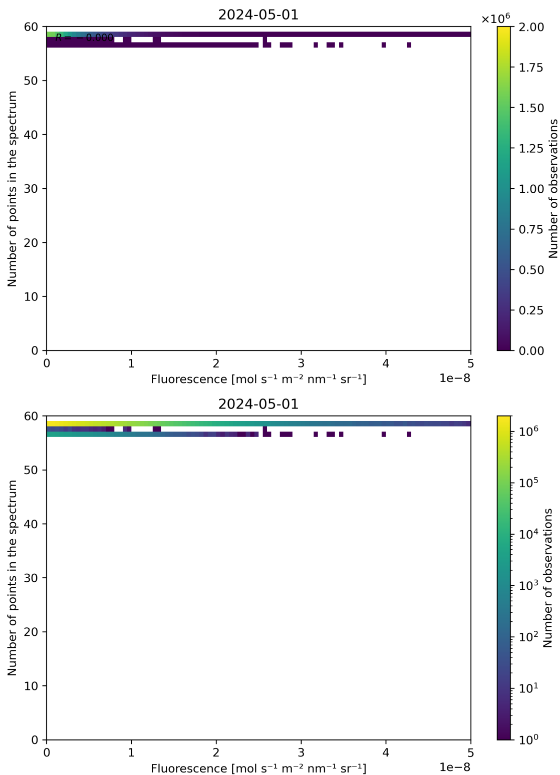
Figure 86: Scatter density plot of “Fluorescence” against “Number of points in the spectrum” for 2024-04-30 to 2024-05-02.
