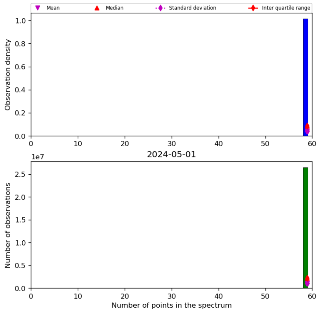
Figure 44: Histogram of “Number of points in the spectrum” for 2024-04-30 to 2024-05-02
