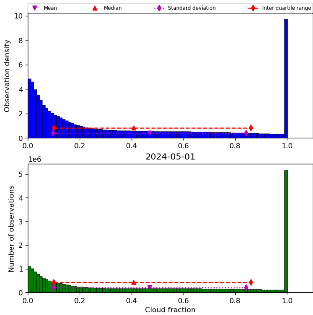
Figure 32: Histogram of “Cloud fraction” for 2024-04-30 to 2024-05-02
