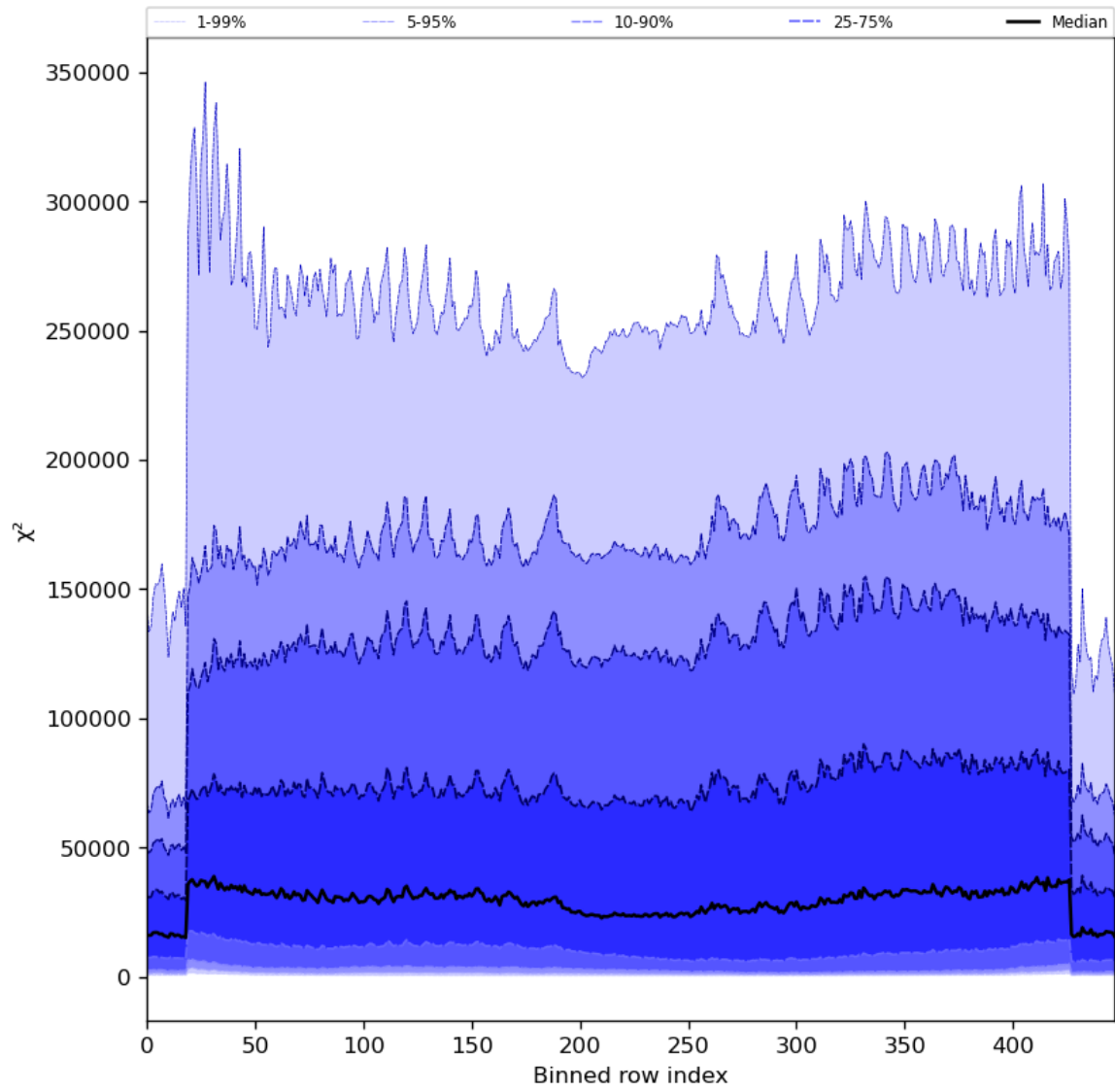
Figure 55: Along track statistics of “ \chi^2 ” for 2024-04-30 to 2024-05-02
