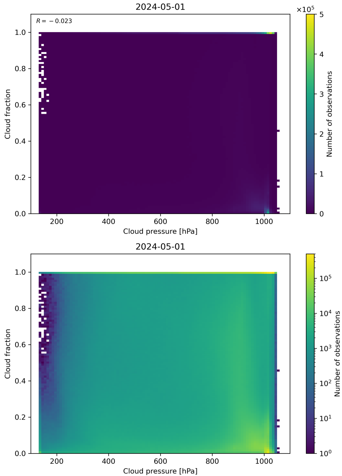
Figure 79: Scatter density plot of “Cloud pressure” against “Cloud fraction” for 2024-04-30 to 2024-05-02.
