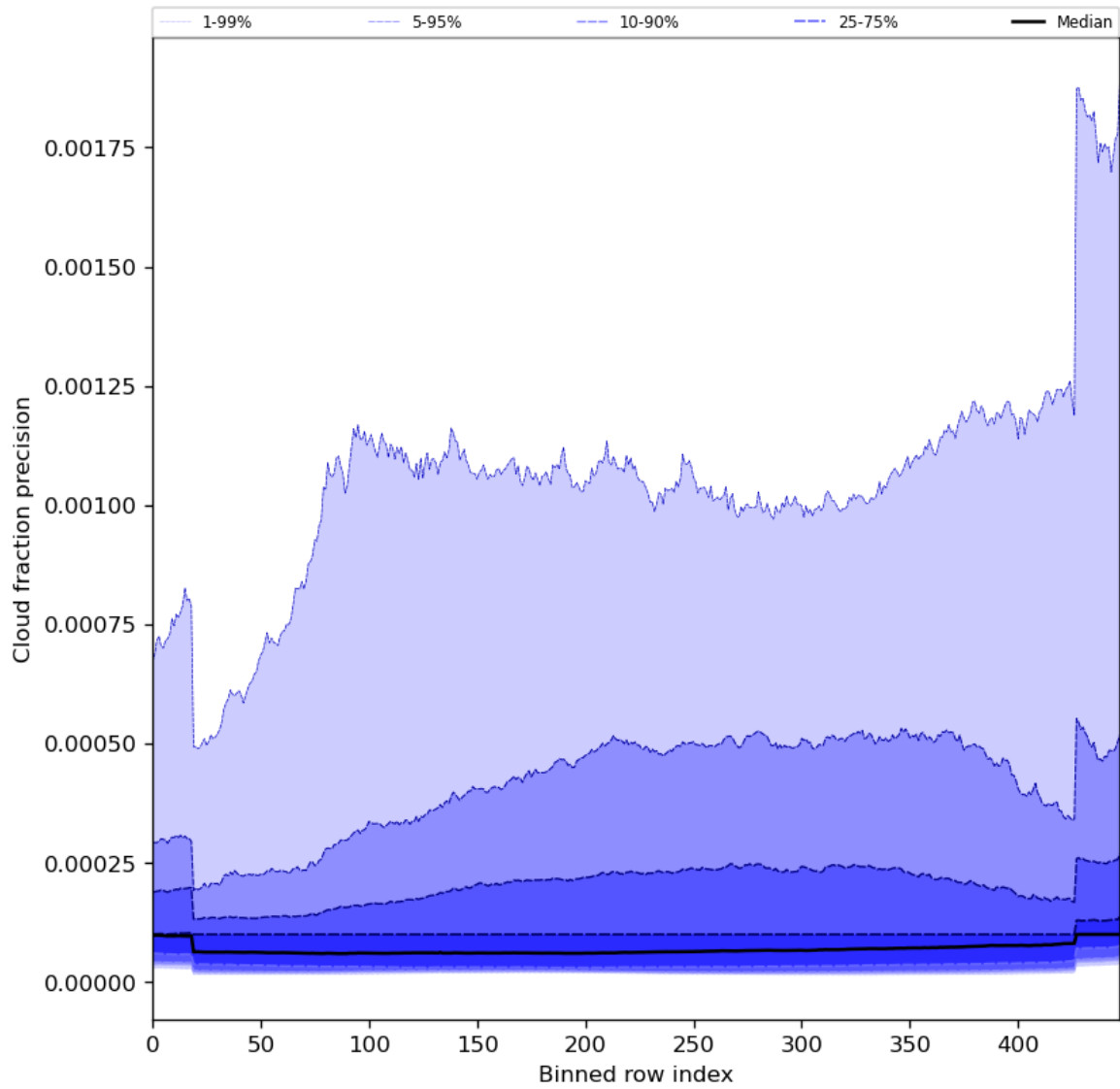
Figure 50: Along track statistics of “Cloud fraction precision” for 2024-04-30 to 2024-05-02
