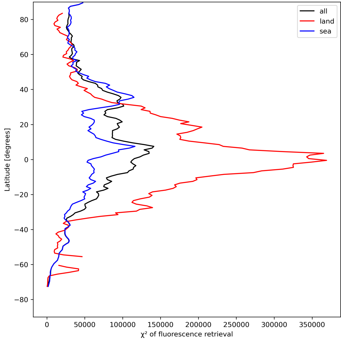
Figure 25: Zonal average of “ \chi^2 of fluorescence retrieval” for 2024-04-30 to 2024-05-02.
