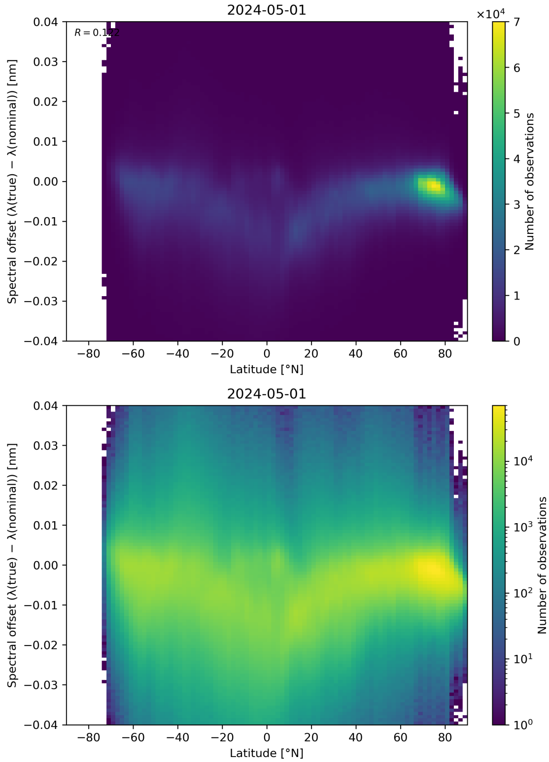
Figure 96: Scatter density plot of “Latitude” against “Spectral offset ( \lambda(\text{true}) - \lambda(\text{nominal}) )” for 2024-04-30 to 2024-05-02.
