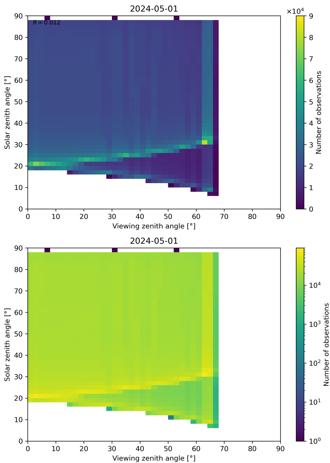
Figure 127: Scatter density plot of “Viewing zenith angle” against “Solar zenith angle” for 2024-04-30 to 2024-05-02.
