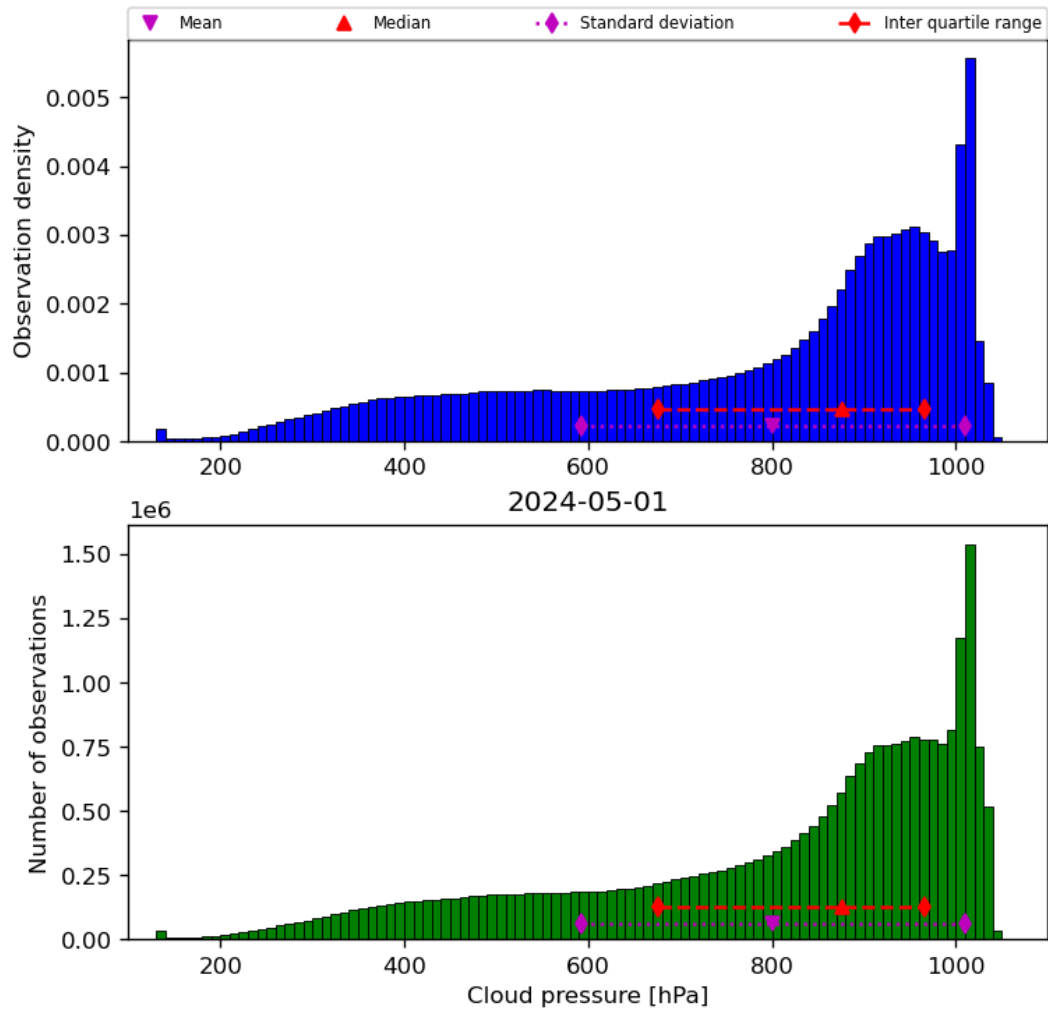
Figure 30: Histogram of “Cloud pressure” for 2024-04-30 to 2024-05-02
