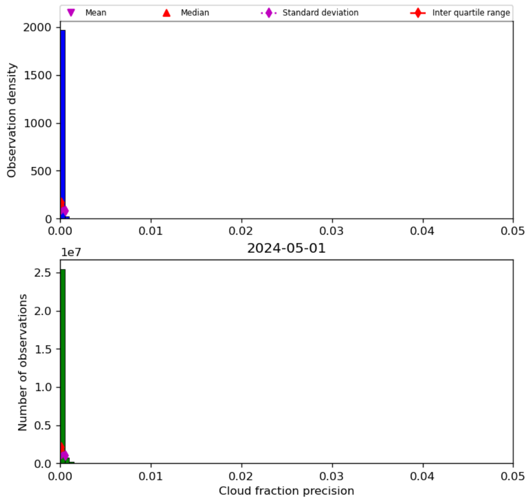
Figure 33: Histogram of “Cloud fraction precision” for 2024-04-30 to 2024-05-02
