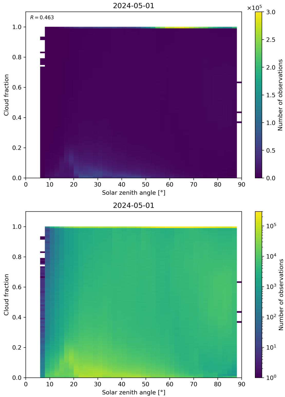
Figure 110: Scatter density plot of “Solar zenith angle” against “Cloud fraction” for 2024-04-30 to 2024-05-02.
