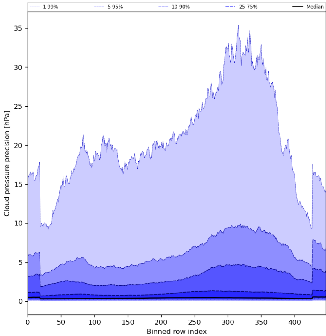
Figure 48: Along track statistics of “Cloud pressure precision” for 2024-04-30 to 2024-05-02
