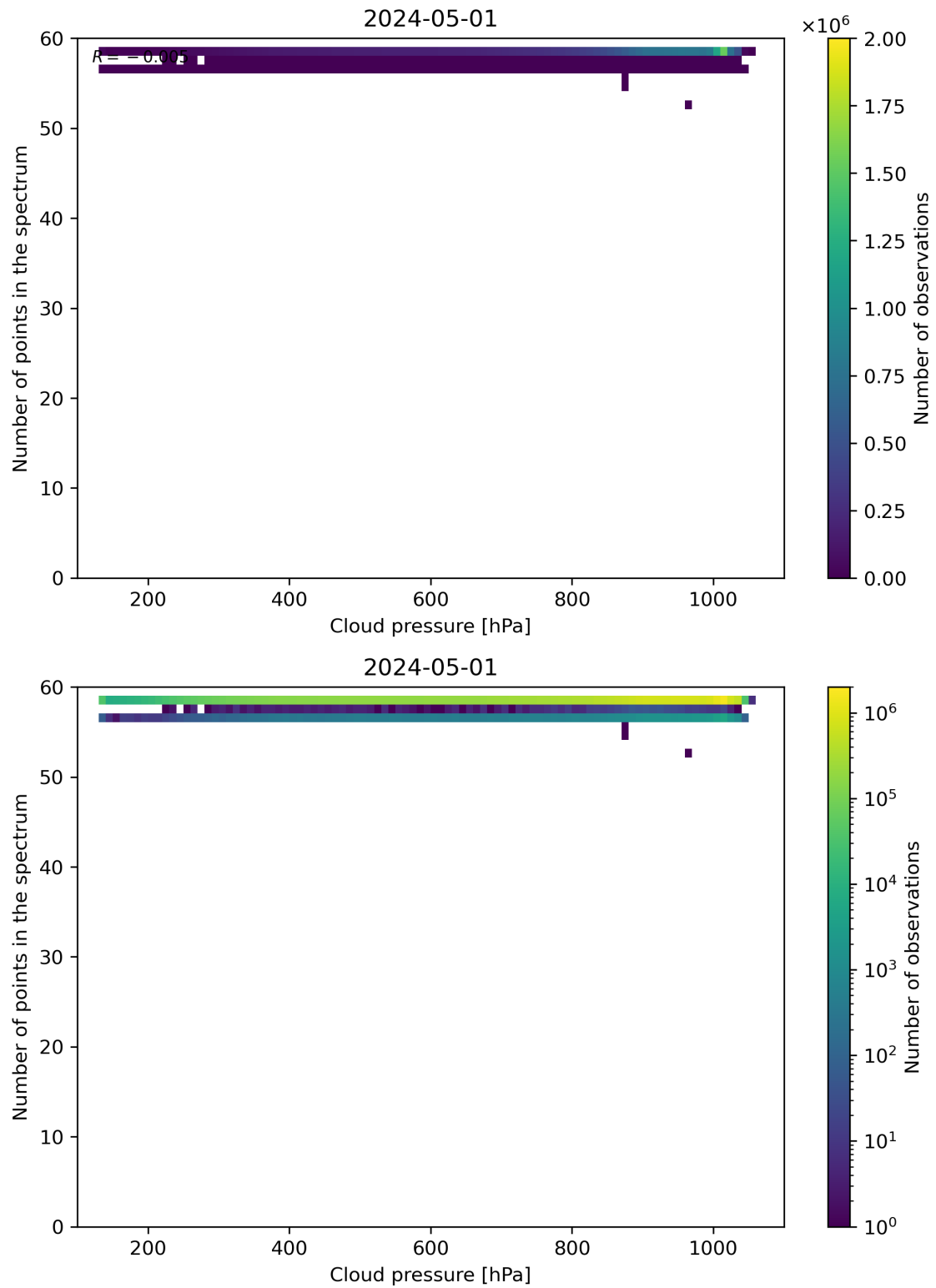
Figure 82: Scatter density plot of “Cloud pressure” against “Number of points in the spectrum” for 2024-04-30 to 2024-05-02.
