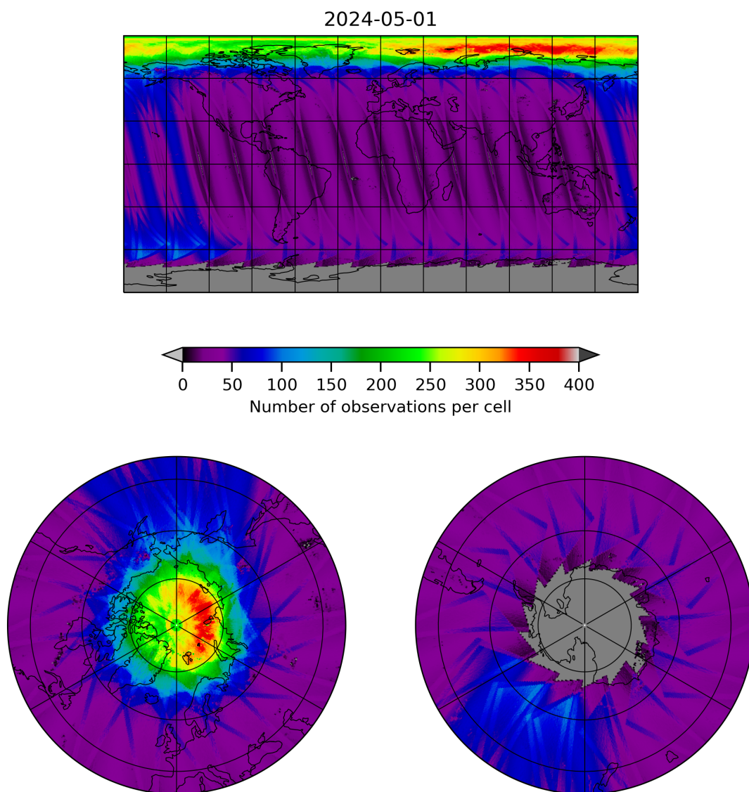
Figure 11: Map of the number of observations for 2024-04-30 to 2024-05-02
