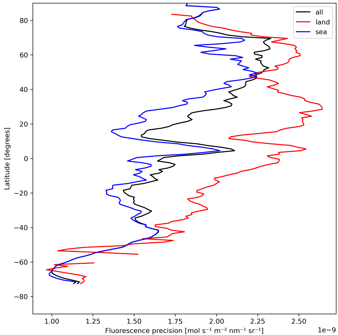
Figure 24: Zonal average of “Fluorescence precision” for 2024-04-30 to 2024-05-02.
