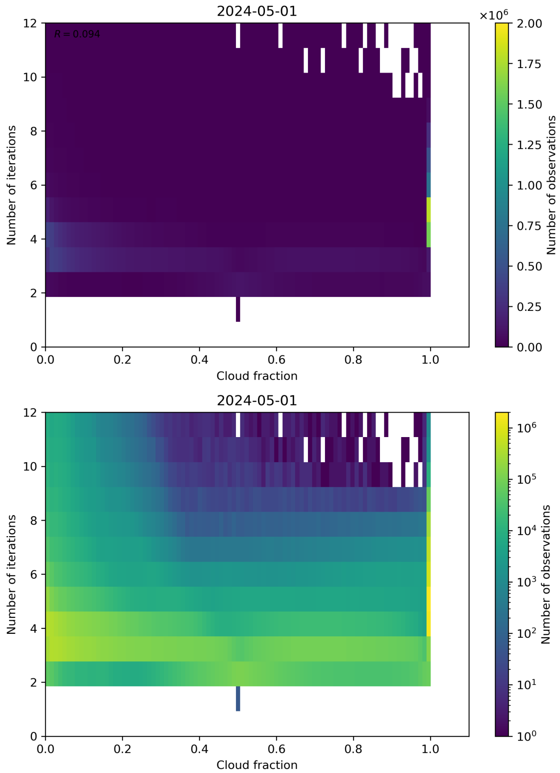
Figure 73: Scatter density plot of “Cloud fraction” against “Number of iterations” for 2024-04-30 to 2024-05-02.
