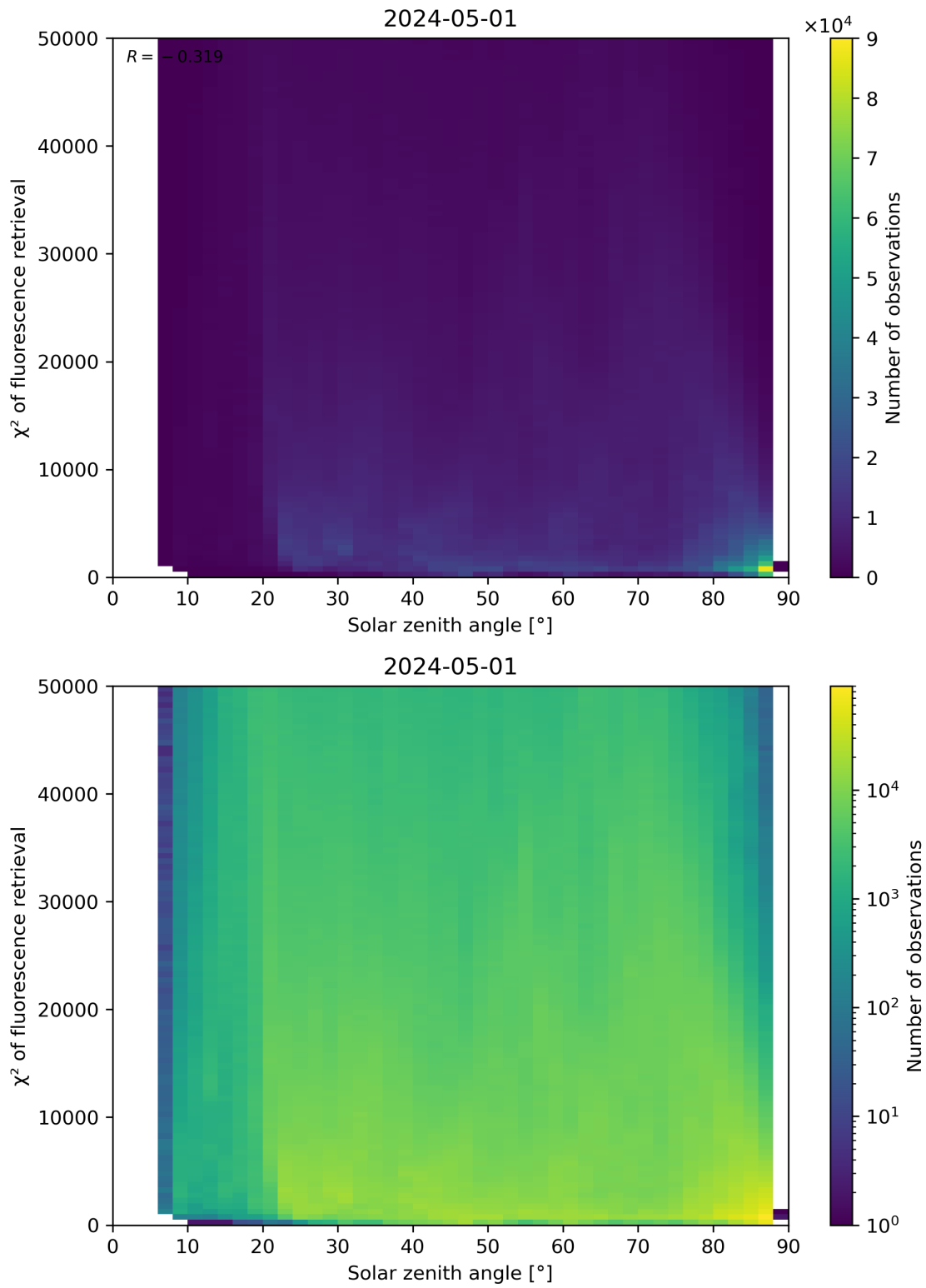
Figure 109: Scatter density plot of “Solar zenith angle” against “ \chi^2 of fluorescence retrieval” for 2024-04-30 to 2024-05-02.
