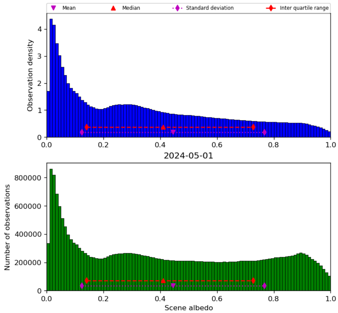
Figure 34: Histogram of “Scene albedo” for 2024-04-30 to 2024-05-02
