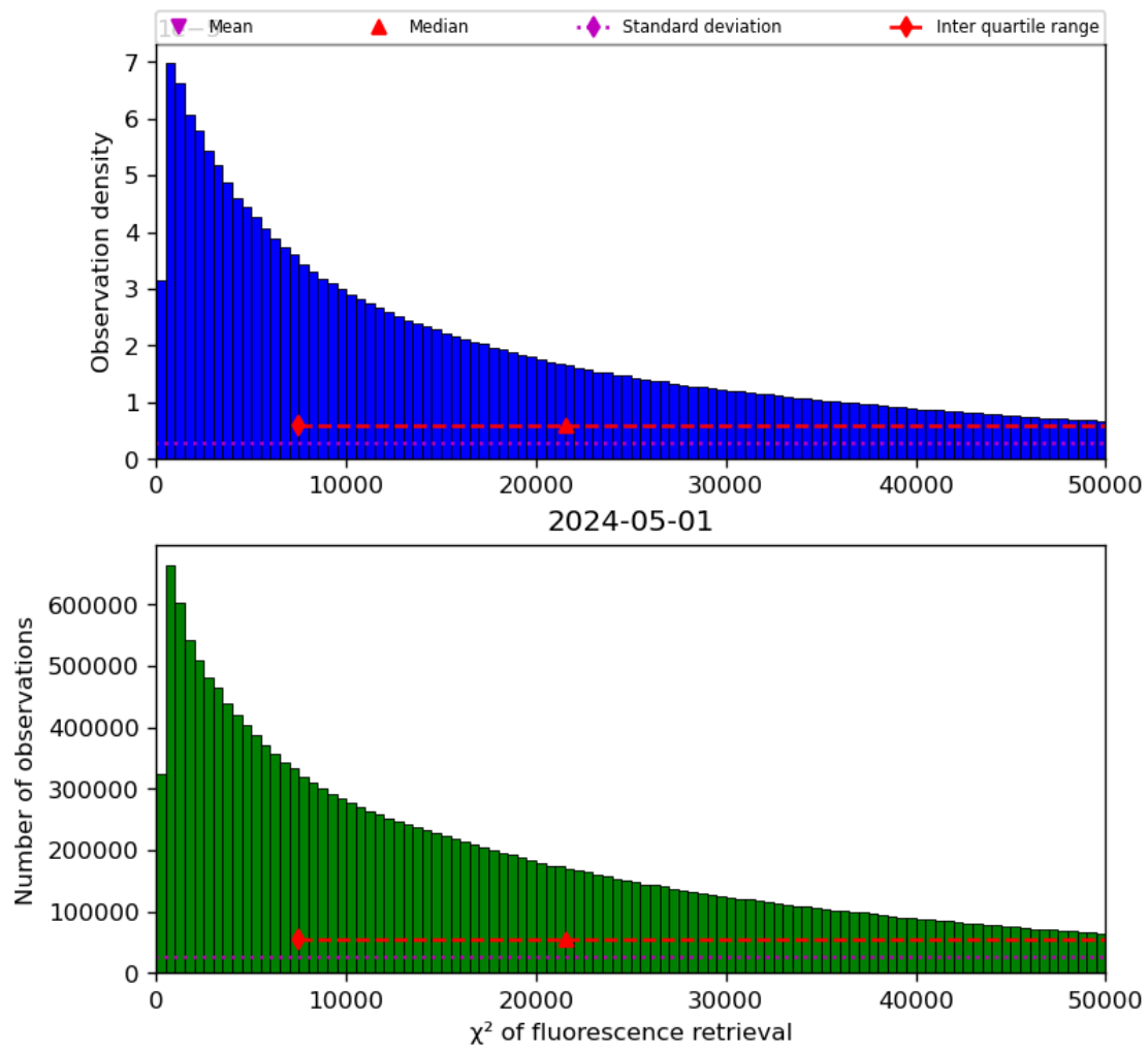
Figure 42: Histogram of “ \chi^2 of fluorescence retrieval” for 2024-04-30 to 2024-05-02
