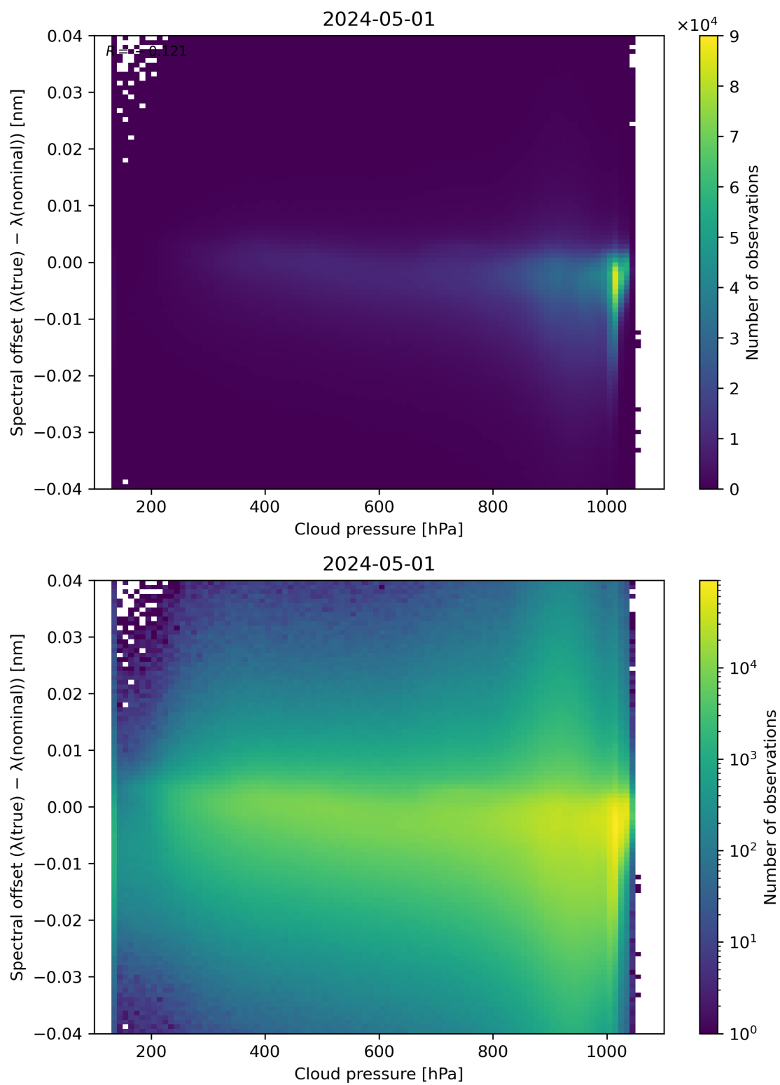
Figure 84: Scatter density plot of “Cloud pressure” against “Spectral offset ( \lambda(\text{true}) - \lambda(\text{nominal}) )” for 2024-04-30 to 2024-05-02.
