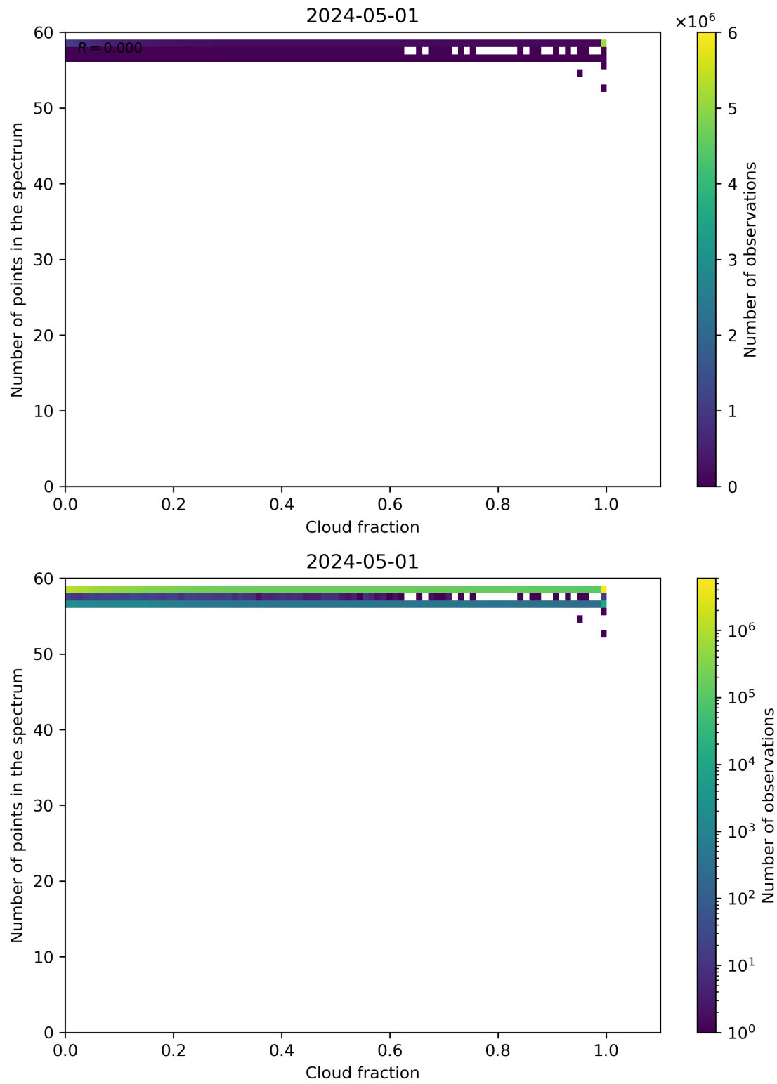
Figure 74: Scatter density plot of “Cloud fraction” against “Number of points in the spectrum” for 2024-04-30 to 2024-05-02.
