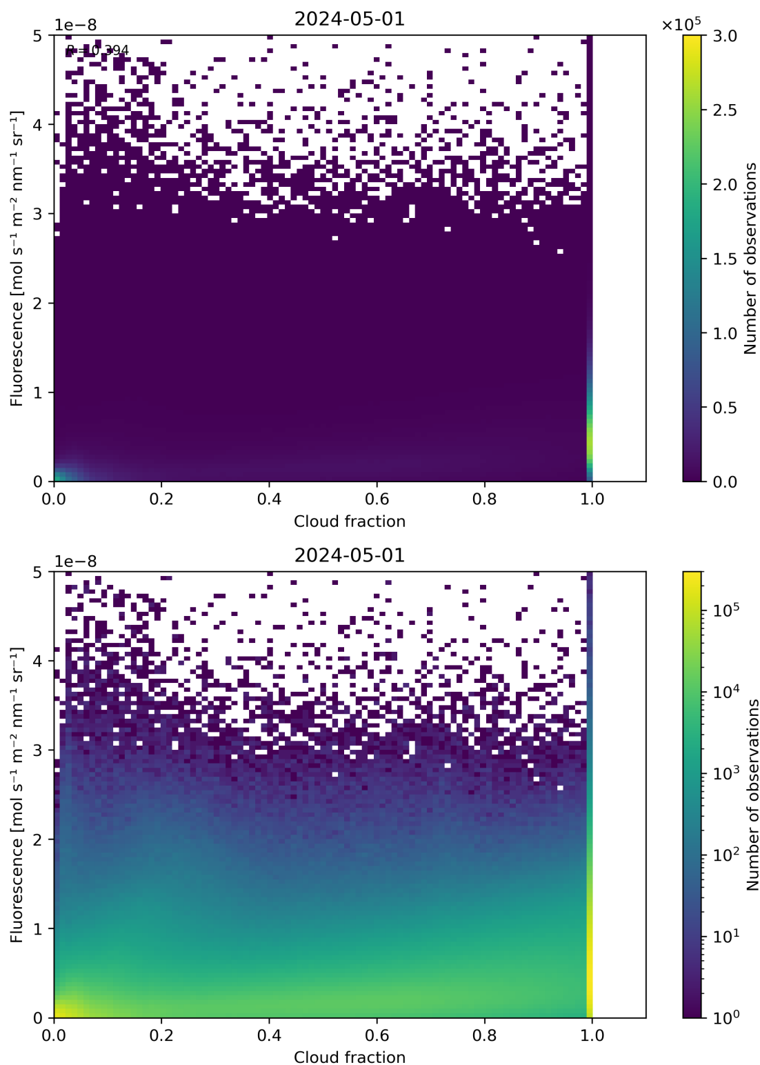
Figure 72: Scatter density plot of “Cloud fraction” against “Fluorescence” for 2024-04-30 to 2024-05-02.
