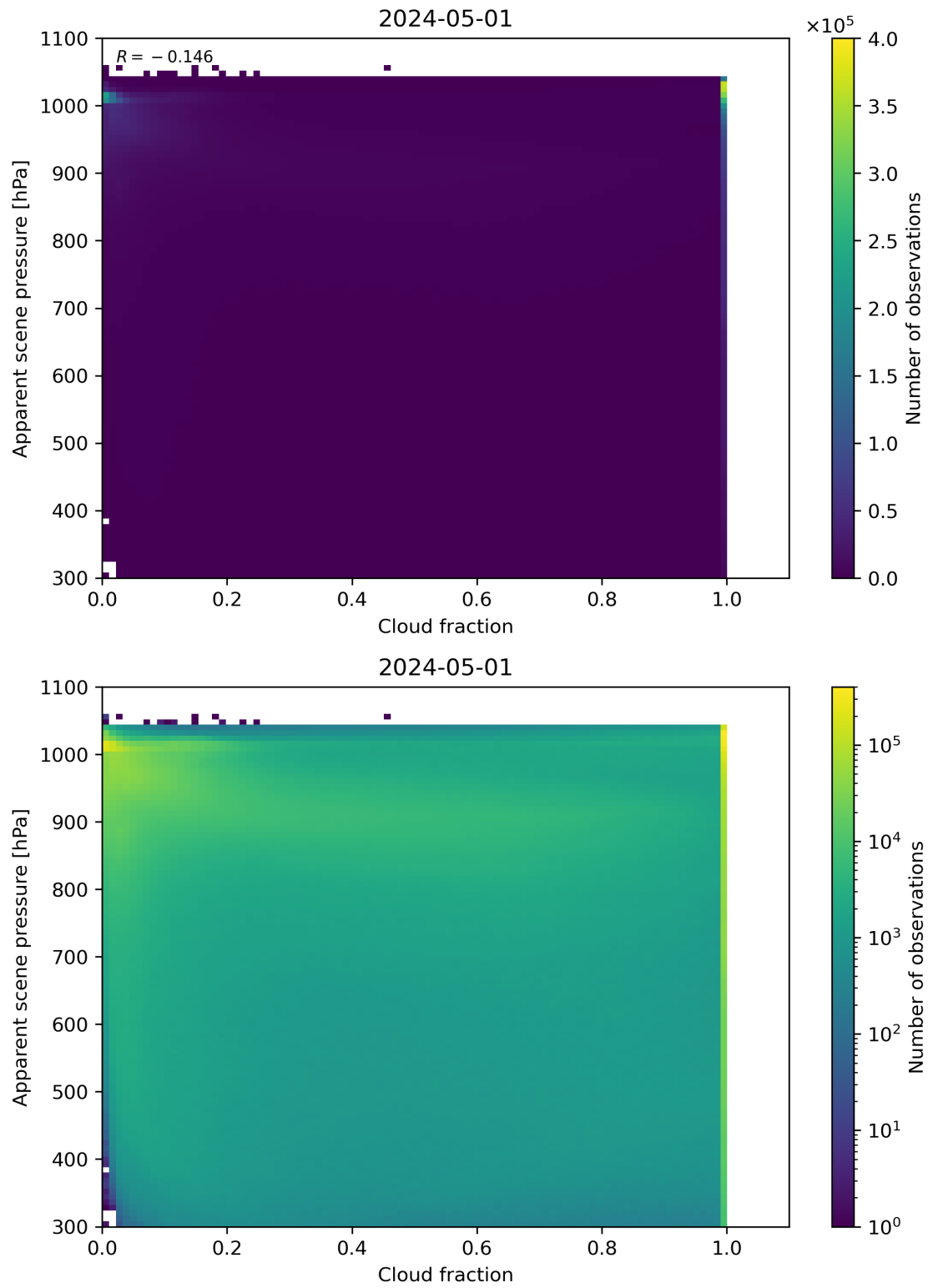
Figure 70: Scatter density plot of “Cloud fraction” against “Apparent scene pressure” for 2024-04-30 to 2024-05-02.
