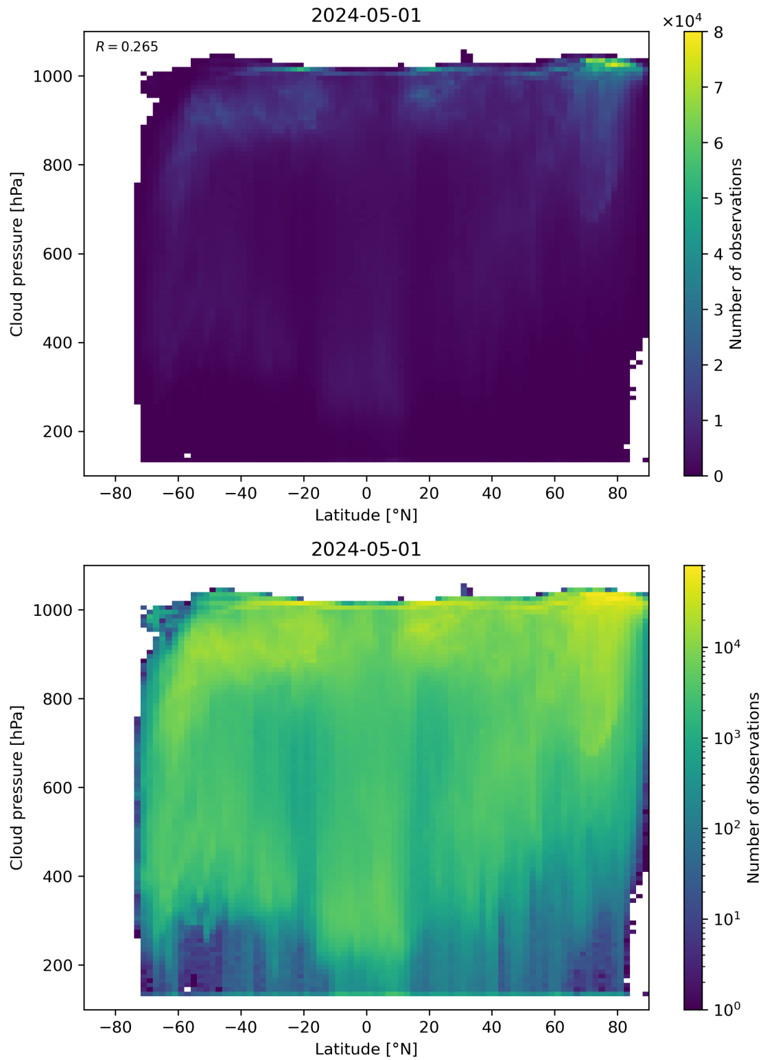
Figure 91: Scatter density plot of “Latitude” against “Cloud pressure” for 2024-04-30 to 2024-05-02.
