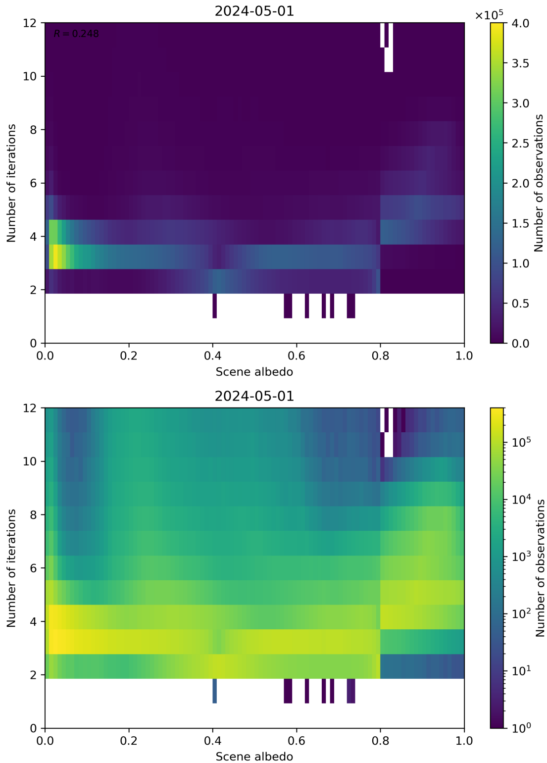
Figure 105: Scatter density plot of “Scene albedo” against “Number of iterations” for 2024-04-30 to 2024-05-02.
