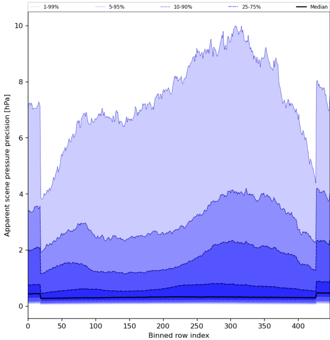
Figure 54: Along track statistics of “Apparent scene pressure precision” for 2024-04-30 to 2024-05-02
