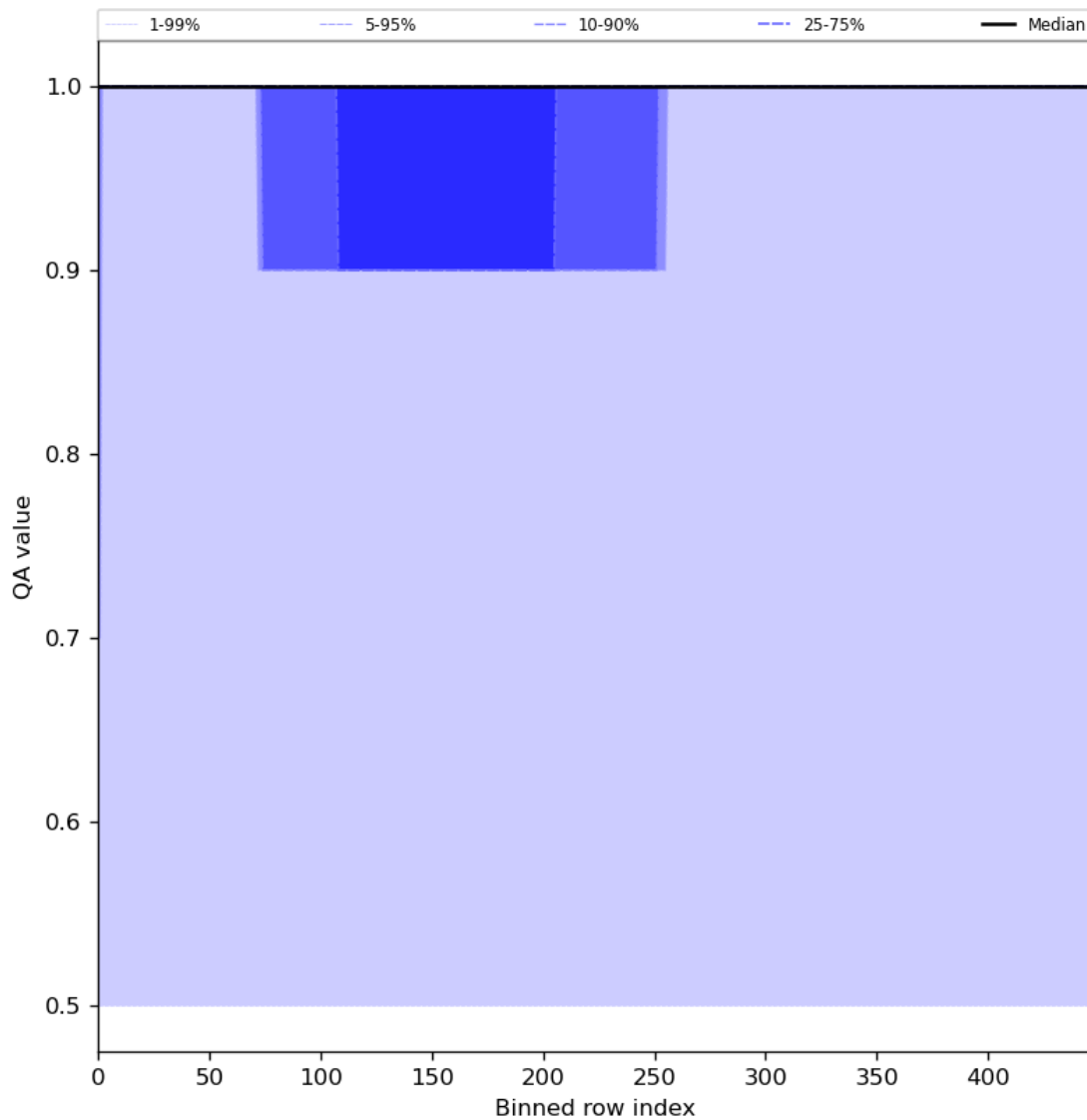
Figure 46: Along track statistics of “QA value” for 2024-04-30 to 2024-05-02
