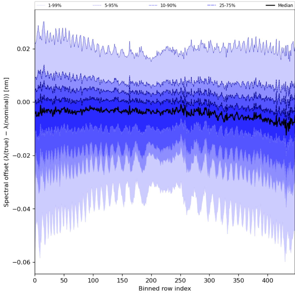
Figure 62: Along track statistics of “Spectral offset ( \lambda(\text{true}) - \lambda(\text{nominal}) )” for 2024-04-30 to 2024-05-02
