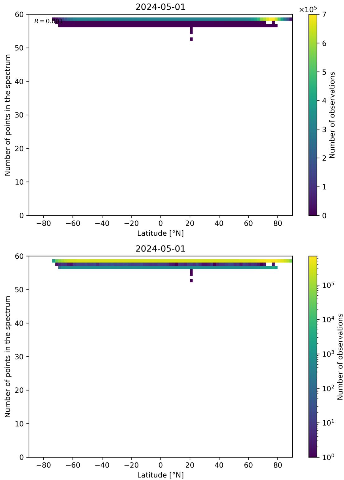
Figure 94: Scatter density plot of “Latitude” against “Number of points in the spectrum” for 2024-04-30 to 2024-05-02.
