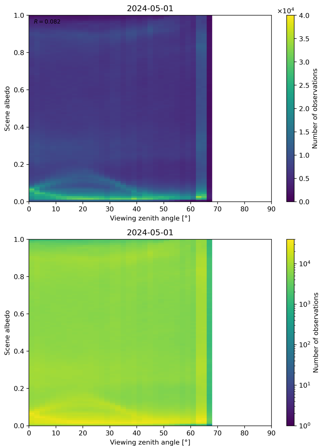
Figure 126: Scatter density plot of “Viewing zenith angle” against “Scene albedo” for 2024-04-30 to 2024-05-02.
