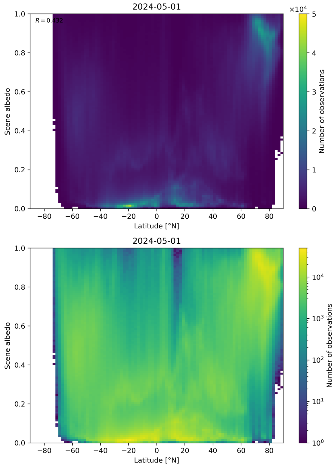
Figure 95: Scatter density plot of “Latitude” against “Scene albedo” for 2024-04-30 to 2024-05-02.
