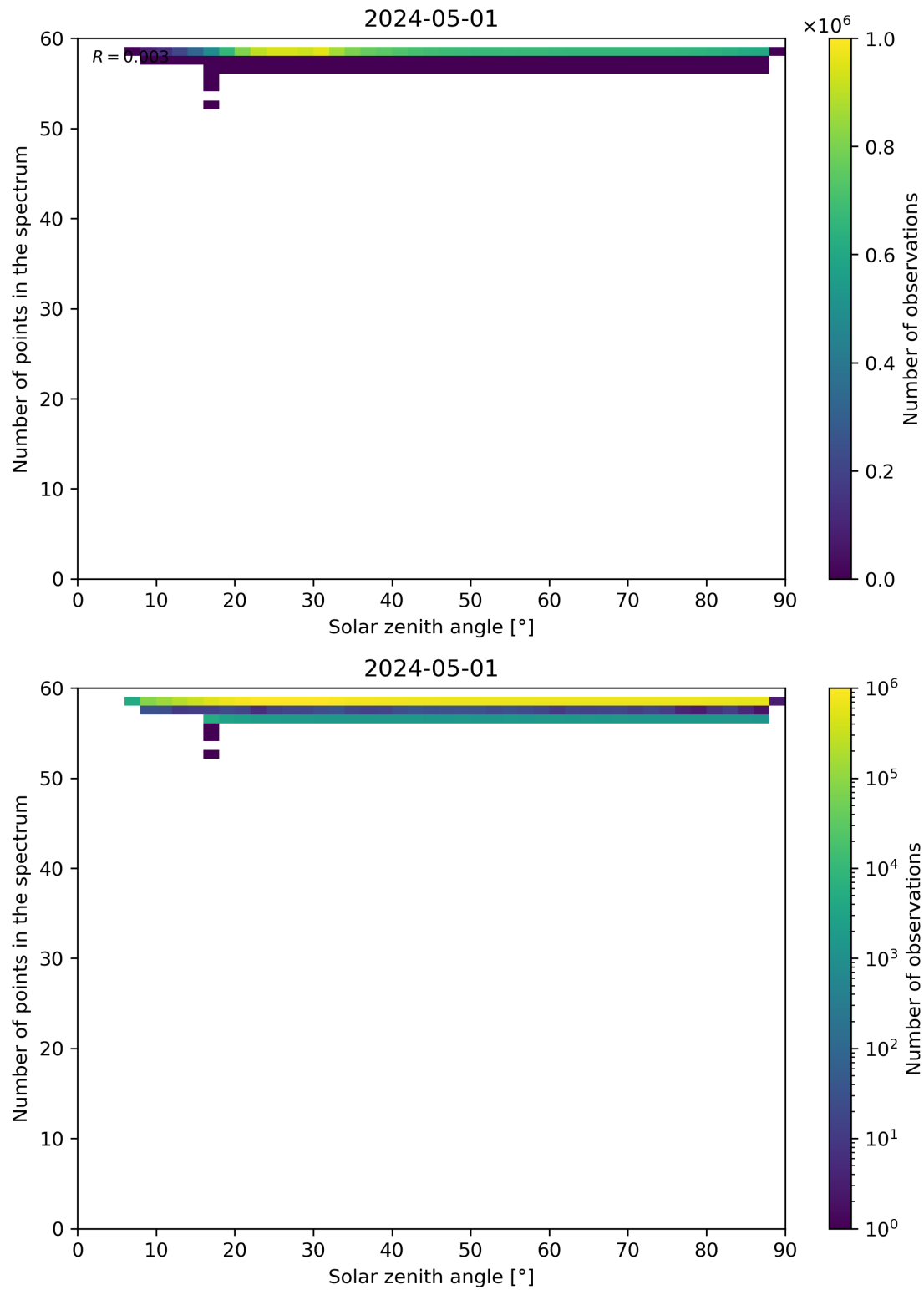
Figure 115: Scatter density plot of “Solar zenith angle” against “Number of points in the spectrum” for 2024-04-30 to 2024-05-02.
