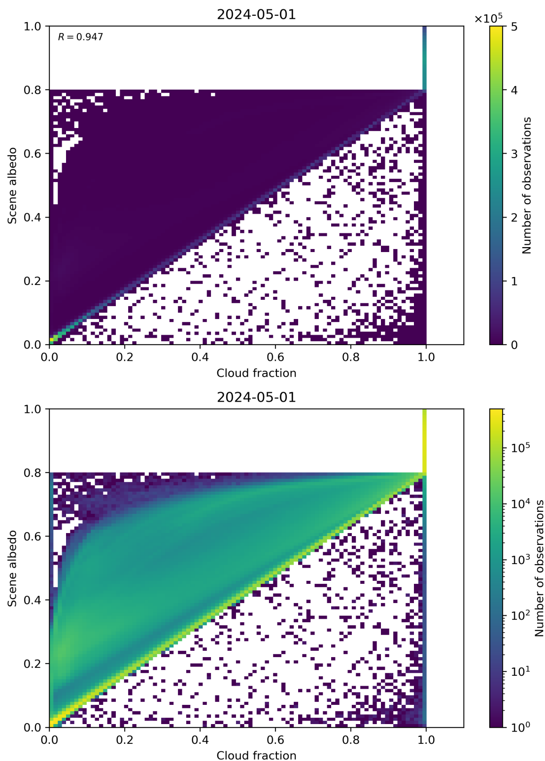
Figure 75: Scatter density plot of “Cloud fraction” against “Scene albedo” for 2024-04-30 to 2024-05-02.
