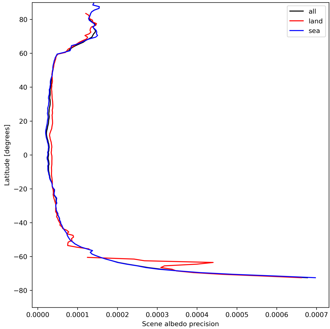
Figure 18: Zonal average of “Scene albedo precision” for 2024-04-30 to 2024-05-02.
