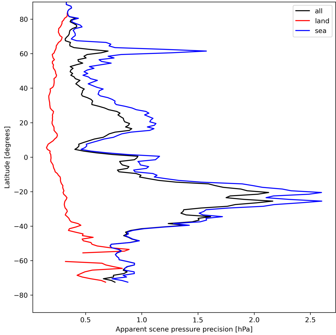
Figure 20: Zonal average of “Apparent scene pressure precision” for 2024-04-30 to 2024-05-02.
