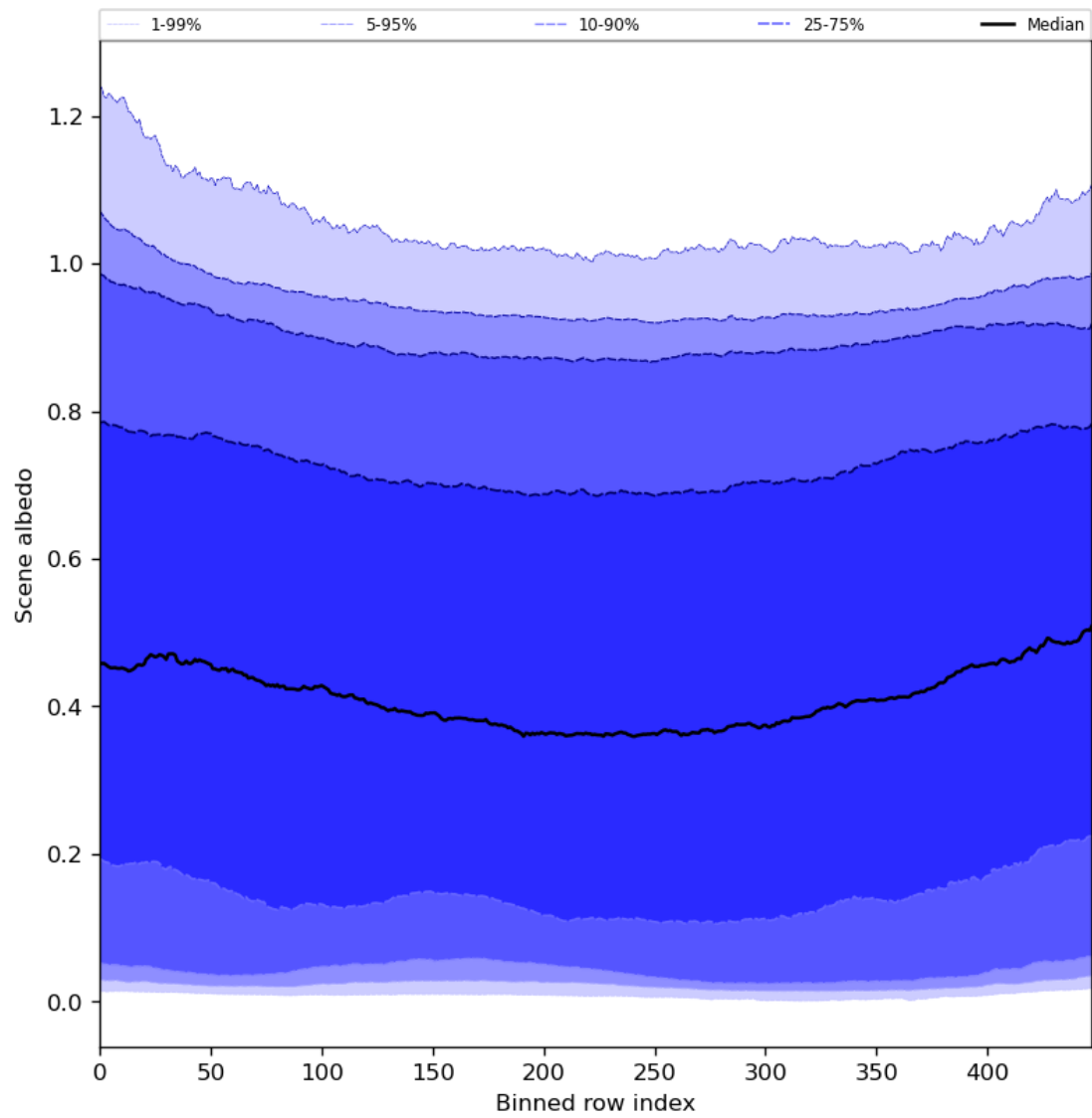
Figure 51: Along track statistics of “Scene albedo” for 2024-04-30 to 2024-05-02
