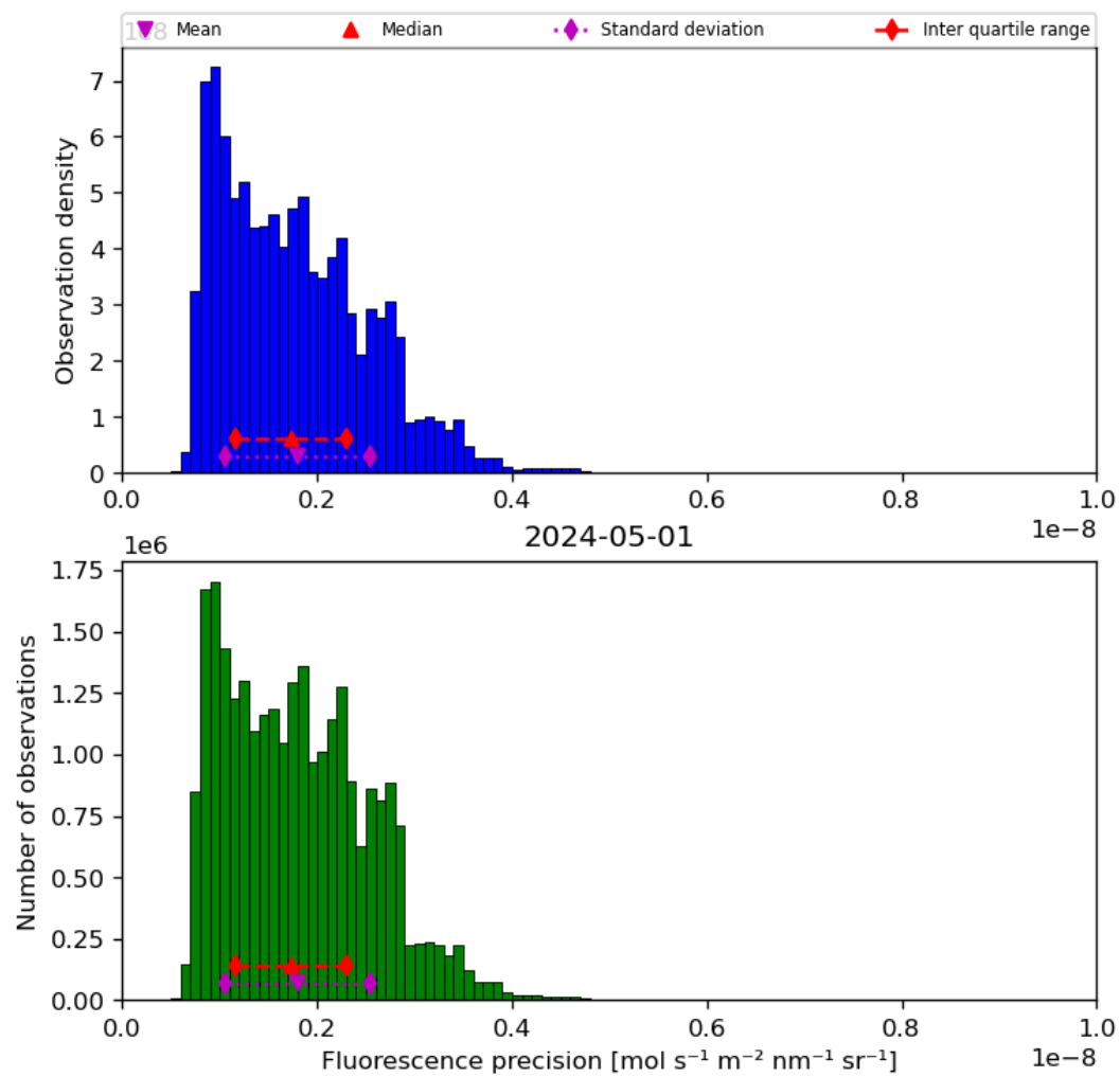
Figure 41: Histogram of “Fluorescence precision” for 2024-04-30 to 2024-05-02
