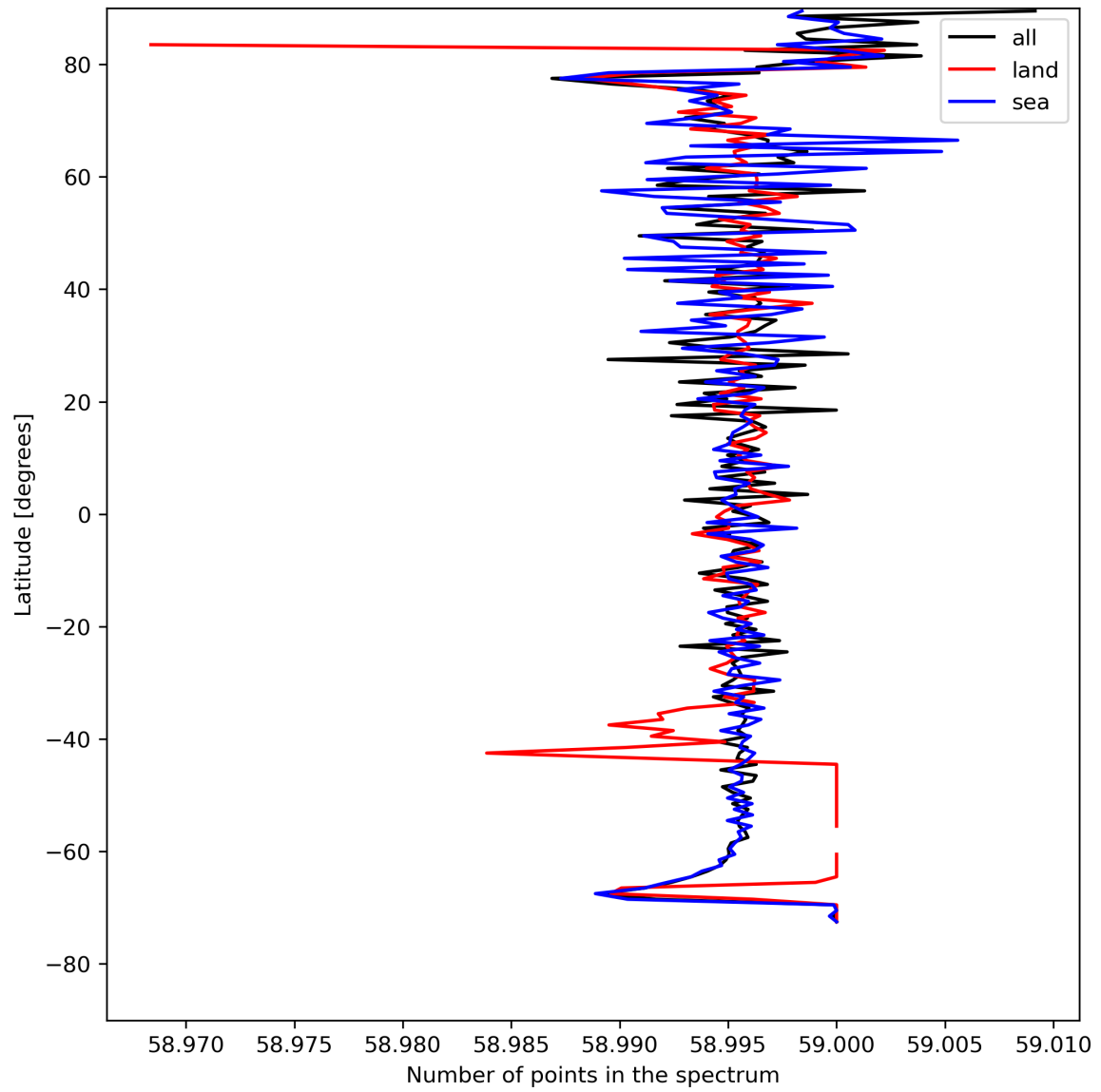
Figure 27: Zonal average of “Number of points in the spectrum” for 2024-04-30 to 2024-05-02.
