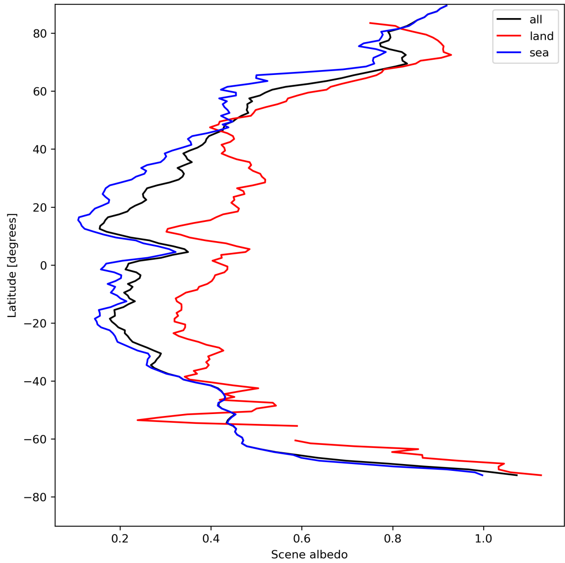
Figure 17: Zonal average of “Scene albedo” for 2024-04-30 to 2024-05-02.
