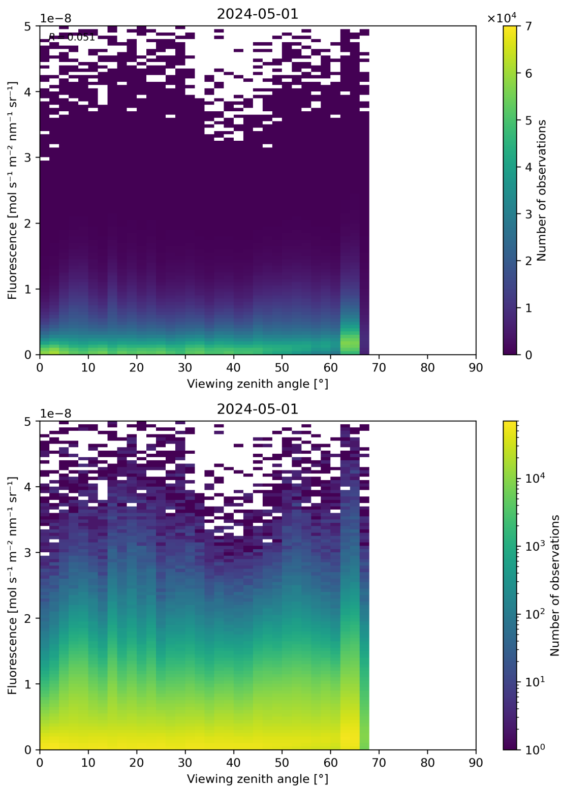
Figure 122: Scatter density plot of “Viewing zenith angle” against “Fluorescence” for 2024-04-30 to 2024-05-02.
