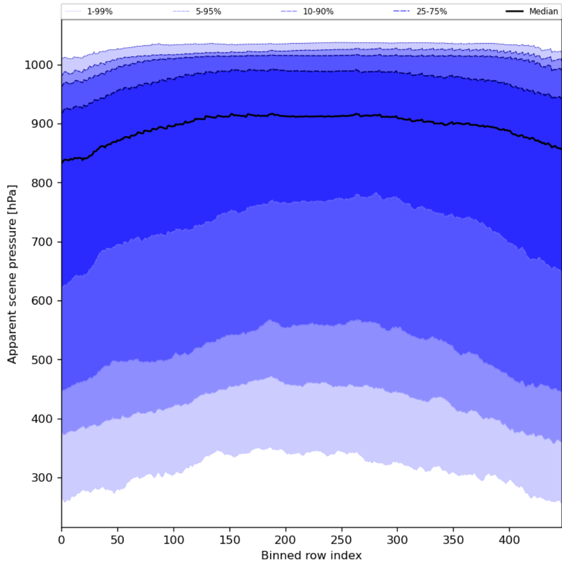
Figure 53: Along track statistics of “Apparent scene pressure” for 2024-04-30 to 2024-05-02
