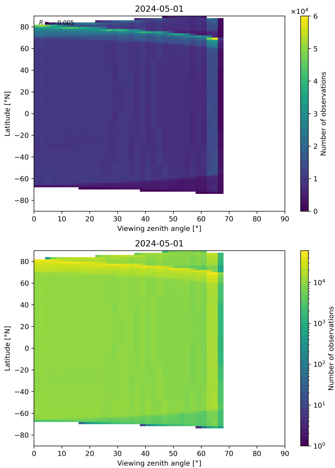
Figure 123: Scatter density plot of “Viewing zenith angle” against “Latitude” for 2024-04-30 to 2024-05-02.
