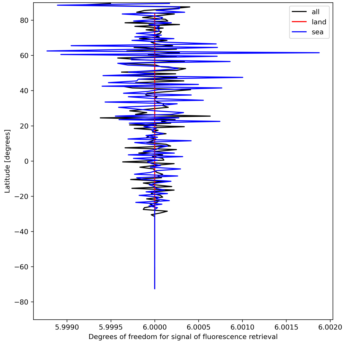
Figure 26: Zonal average of “Degrees of freedom for signal of fluorescence retrieval” for 2024-04-30 to 2024-05-02.
