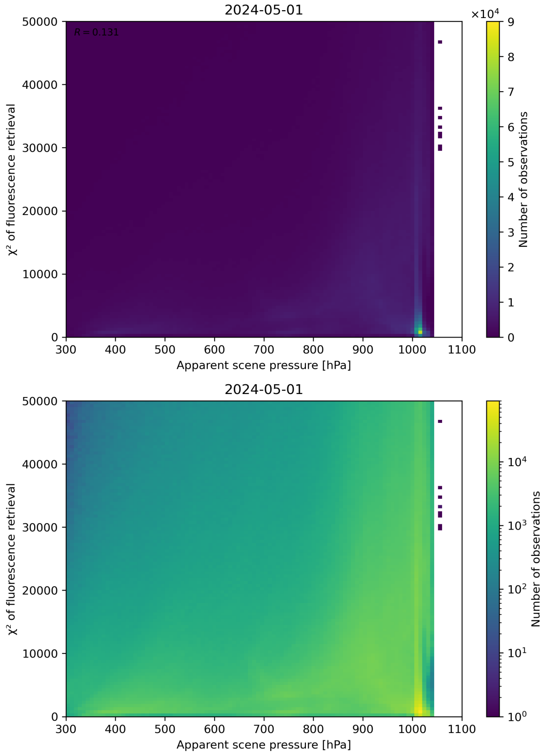
Figure 63: Scatter density plot of “Apparent scene pressure” against “ \chi^2 of fluorescence retrieval” for 2024-04-30 to 2024-05-02.
