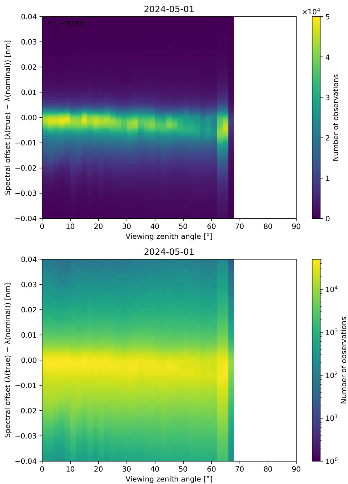
Figure 128: Scatter density plot of “Viewing zenith angle” against “Spectral offset ( \lambda(\text{true}) - \lambda(\text{nominal}) )” for 2024-04-30 to 2024-05-02.
