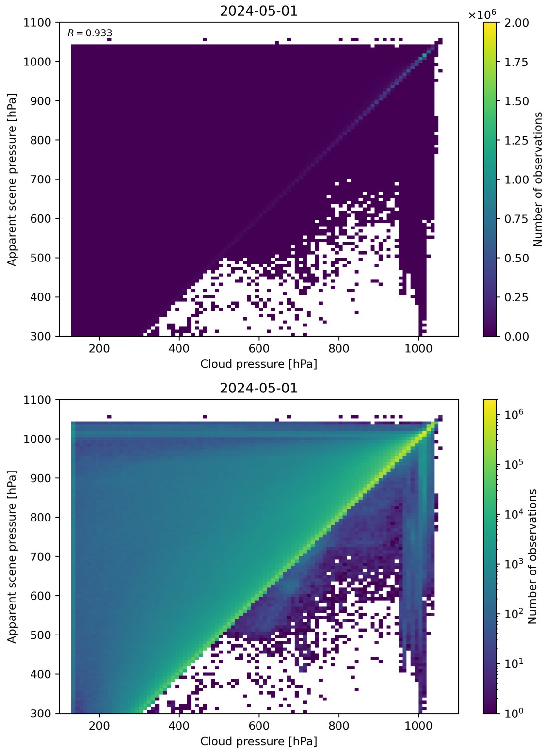
Figure 77: Scatter density plot of “Cloud pressure” against “Apparent scene pressure” for 2024-04-30 to 2024-05-02.
