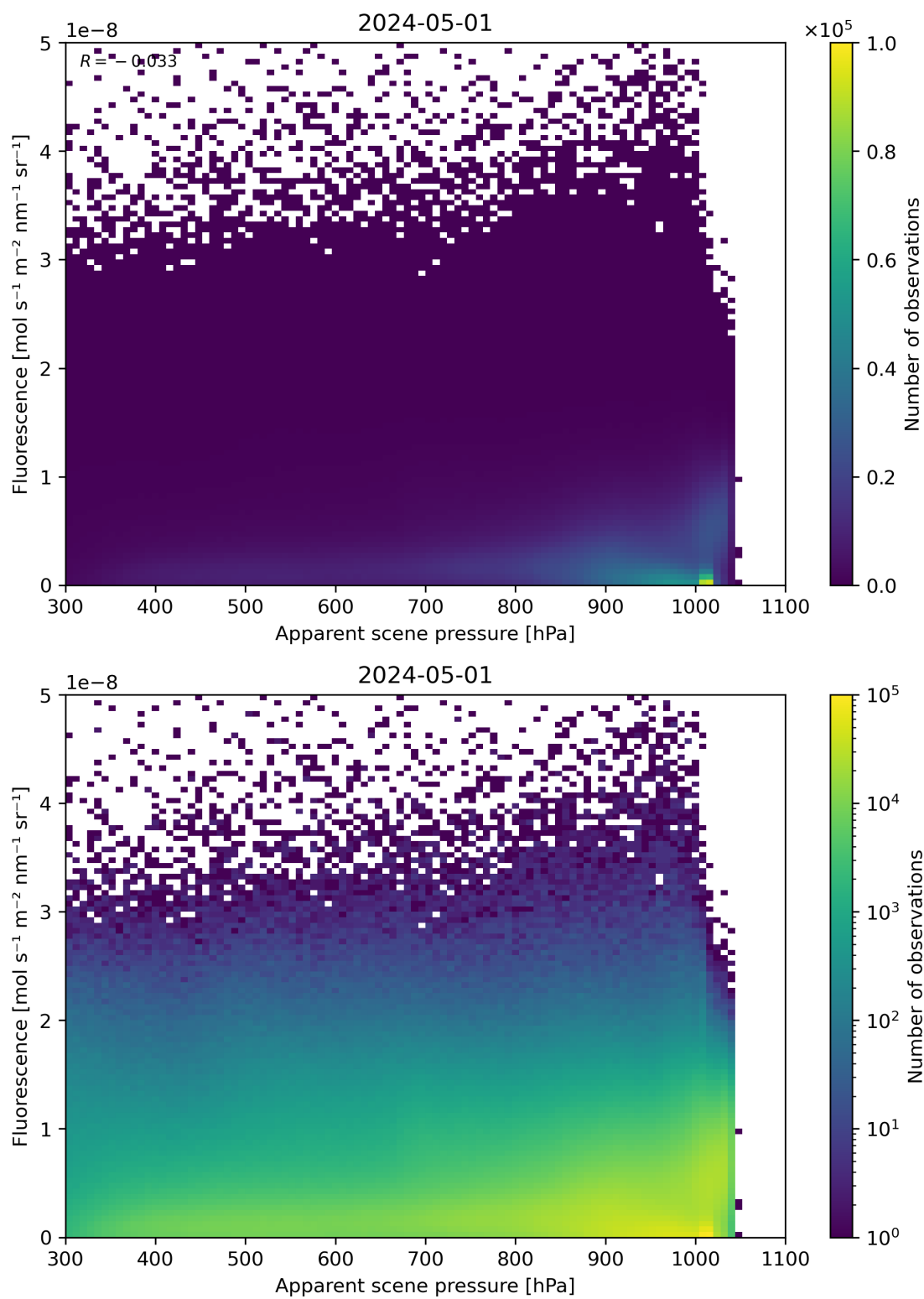
Figure 64: Scatter density plot of “Apparent scene pressure” against “Fluorescence” for 2024-04-30 to 2024-05-02.
