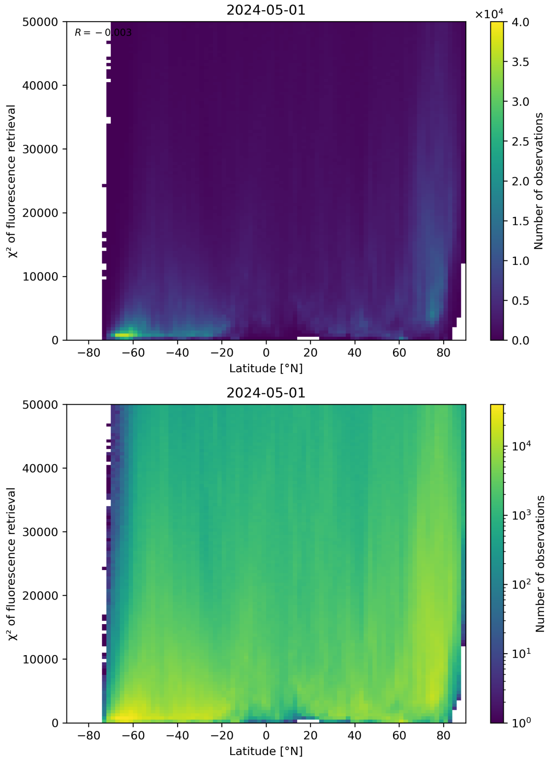
Figure 89: Scatter density plot of “Latitude” against “ \chi^2 of fluorescence retrieval” for 2024-04-30 to 2024-05-02.
