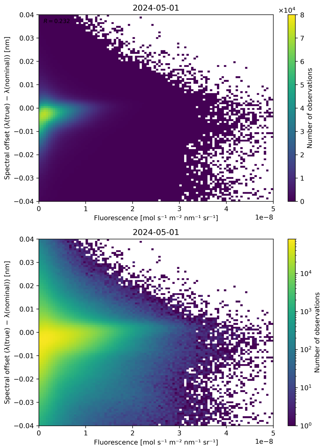
Figure 87: Scatter density plot of “Fluorescence” against “Spectral offset ( \lambda(\text{true}) - \lambda(\text{nominal}) )” for 2024-04-30 to 2024-05-02.
