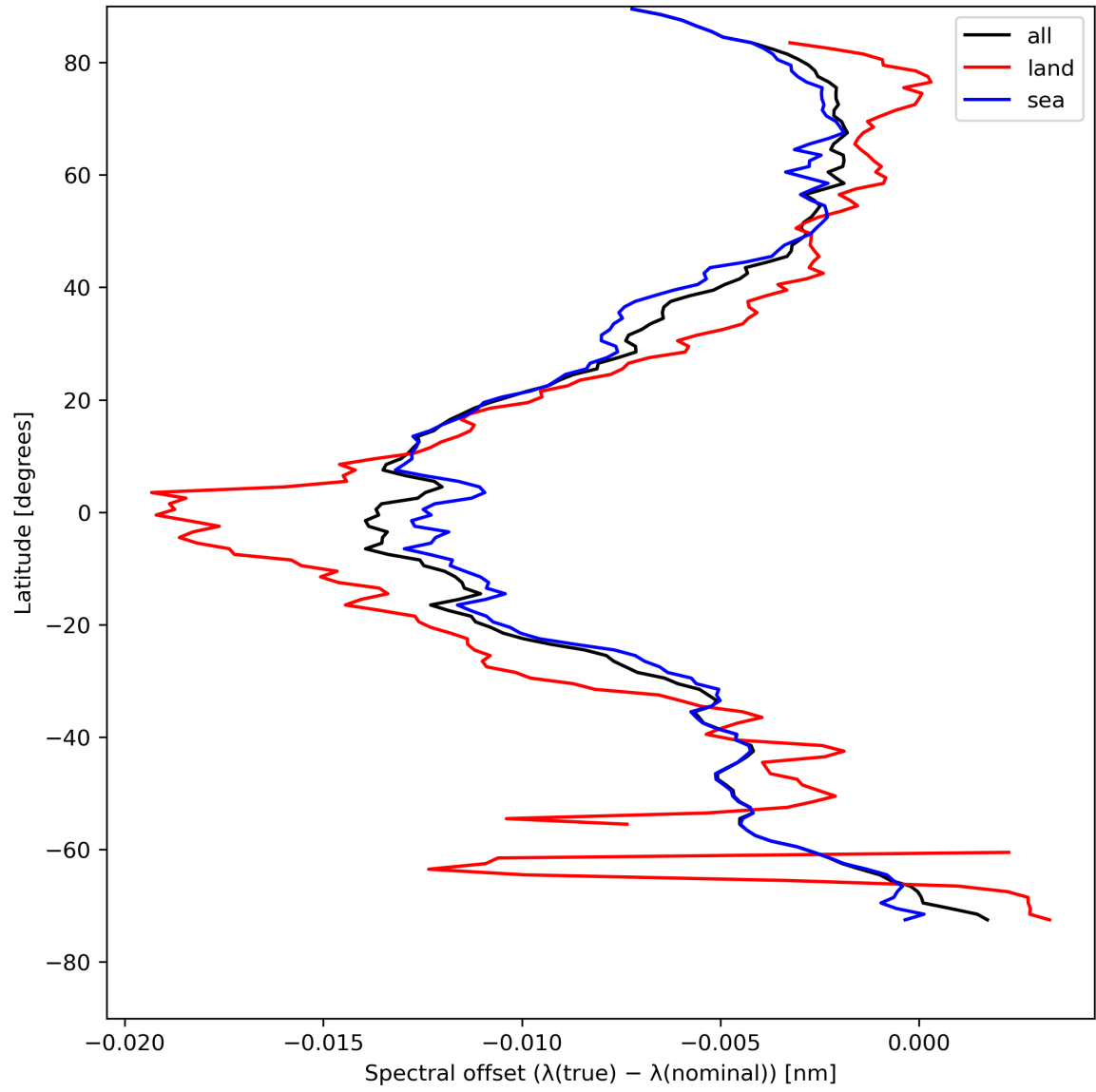
Figure 28: Zonal average of “Spectral offset ( \lambda(\text{true}) - \lambda(\text{nominal}) )” for 2024-04-30 to 2024-05-02.
