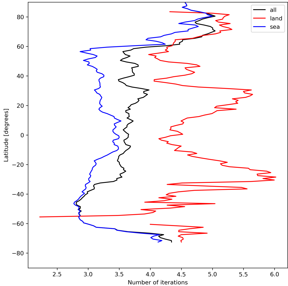
Figure 22: Zonal average of “Number of iterations” for 2024-04-30 to 2024-05-02.
