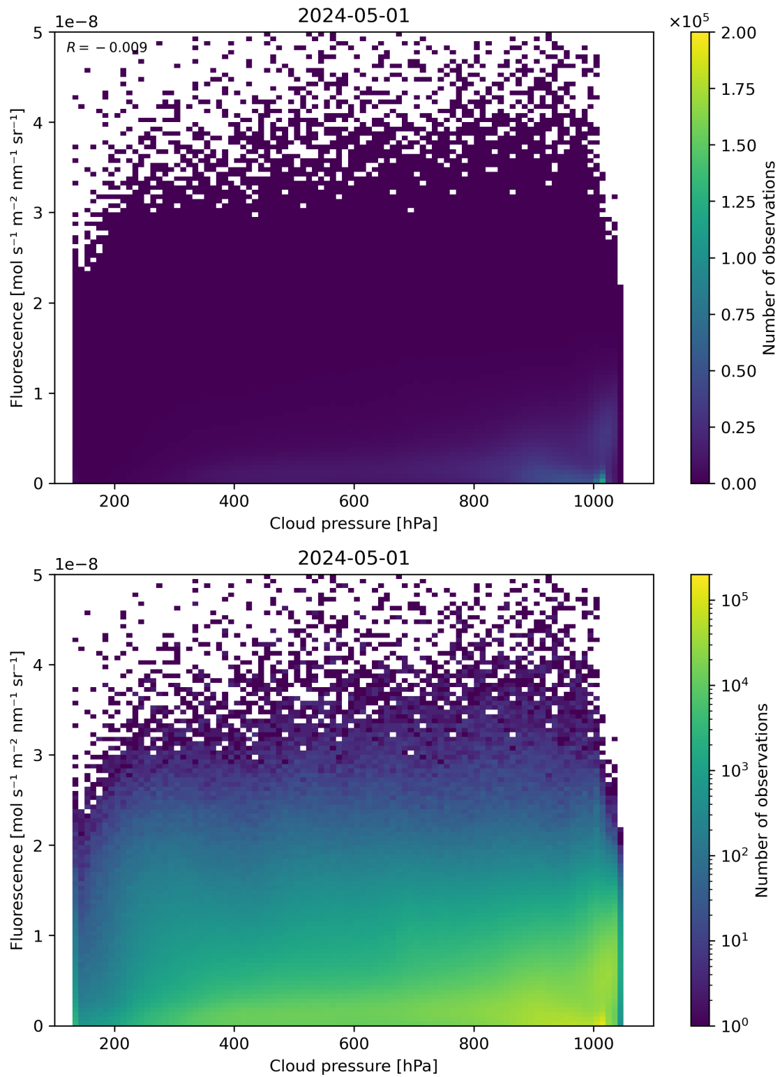
Figure 80: Scatter density plot of “Cloud pressure” against “Fluorescence” for 2024-04-30 to 2024-05-02.
