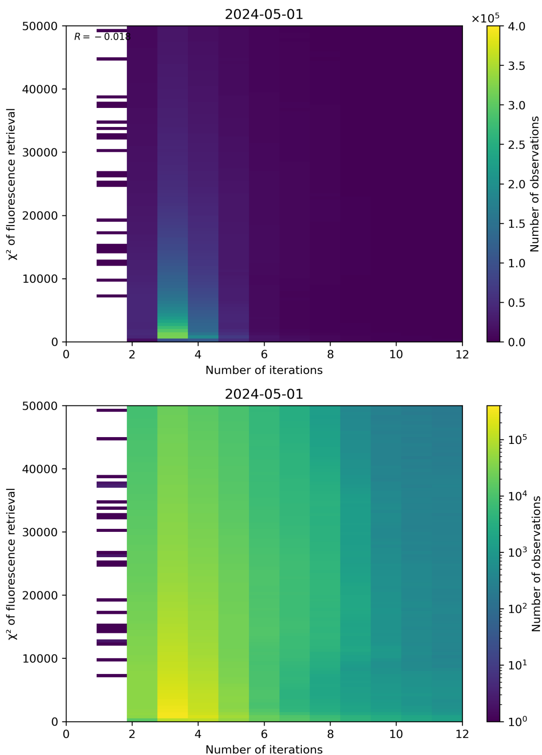
Figure 97: Scatter density plot of “Number of iterations” against “ \chi^2 of fluorescence retrieval” for 2024-04-30 to 2024-05-02.
