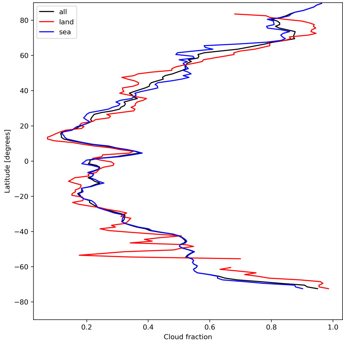
Figure 15: Zonal average of “Cloud fraction” for 2024-04-30 to 2024-05-02.
