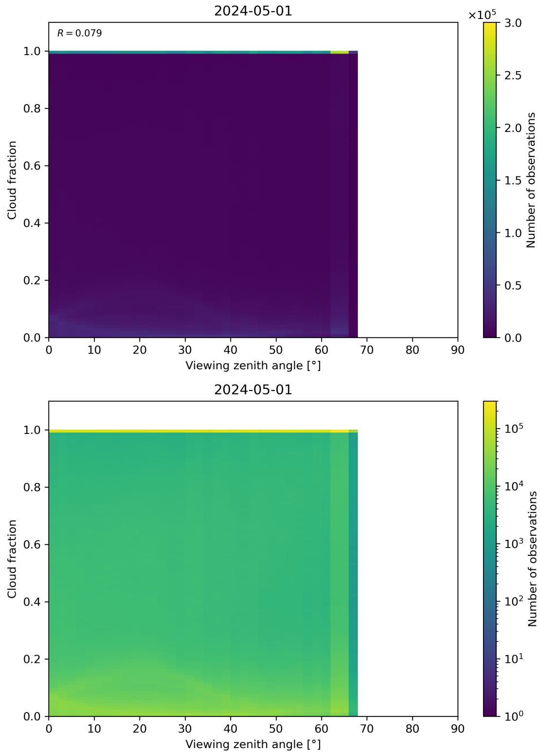
Figure 120: Scatter density plot of “Viewing zenith angle” against “Cloud fraction” for 2024-04-30 to 2024-05-02.
