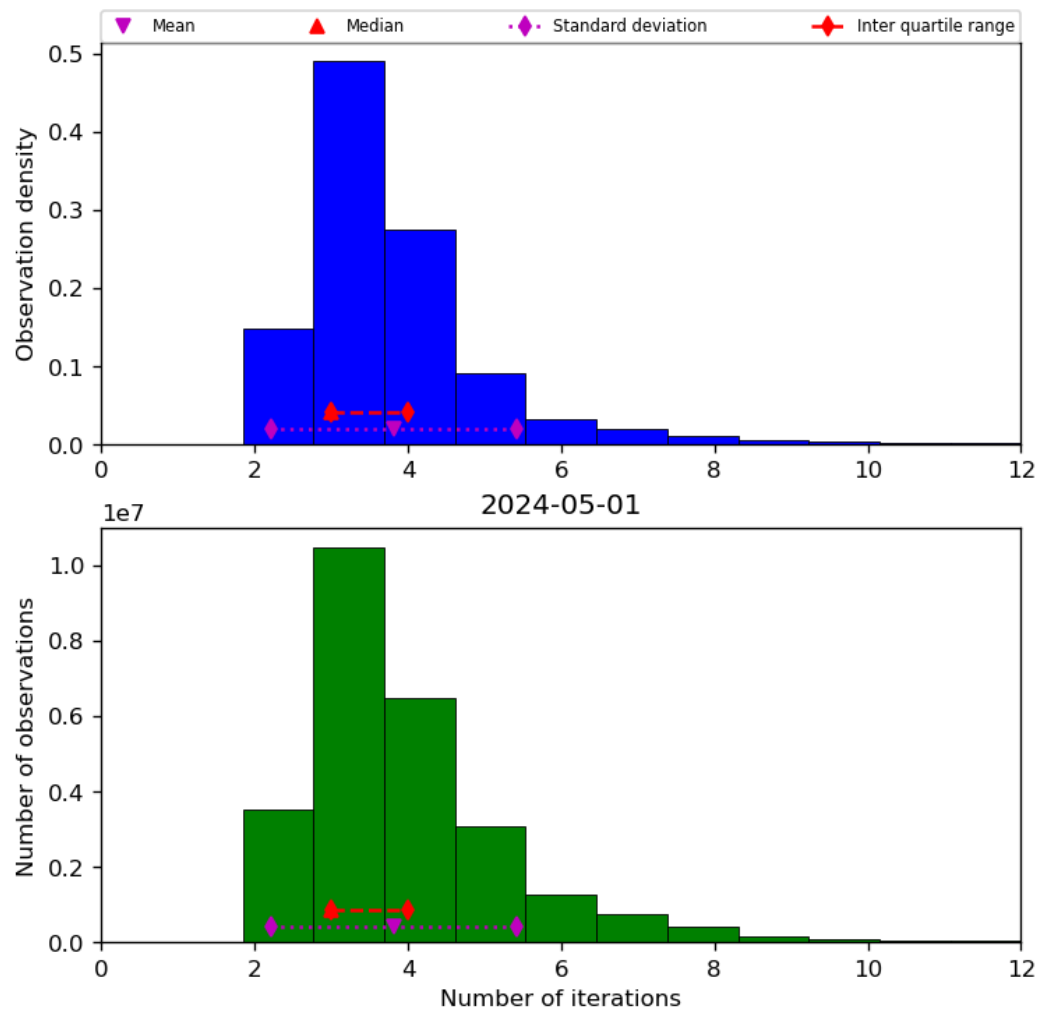
Figure 39: Histogram of “Number of iterations” for 2024-04-30 to 2024-05-02
