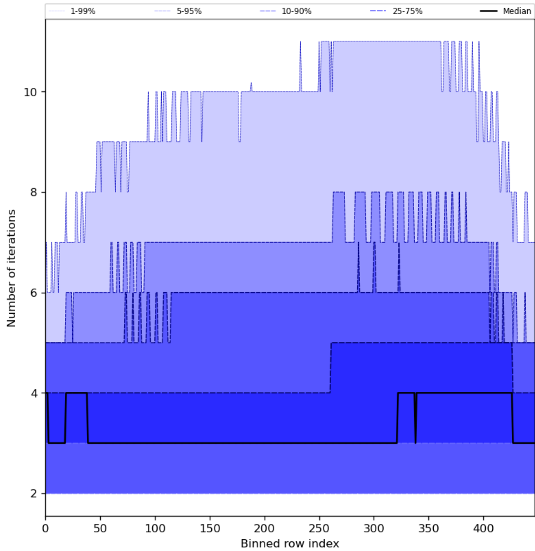
Figure 56: Along track statistics of “Number of iterations” for 2024-04-30 to 2024-05-02
