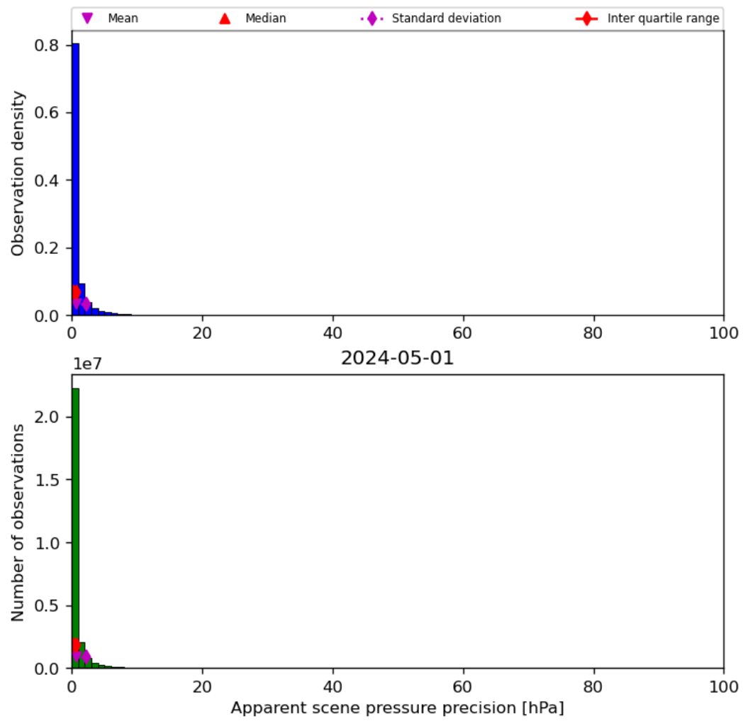
Figure 37: Histogram of “Apparent scene pressure precision” for 2024-04-30 to 2024-05-02
