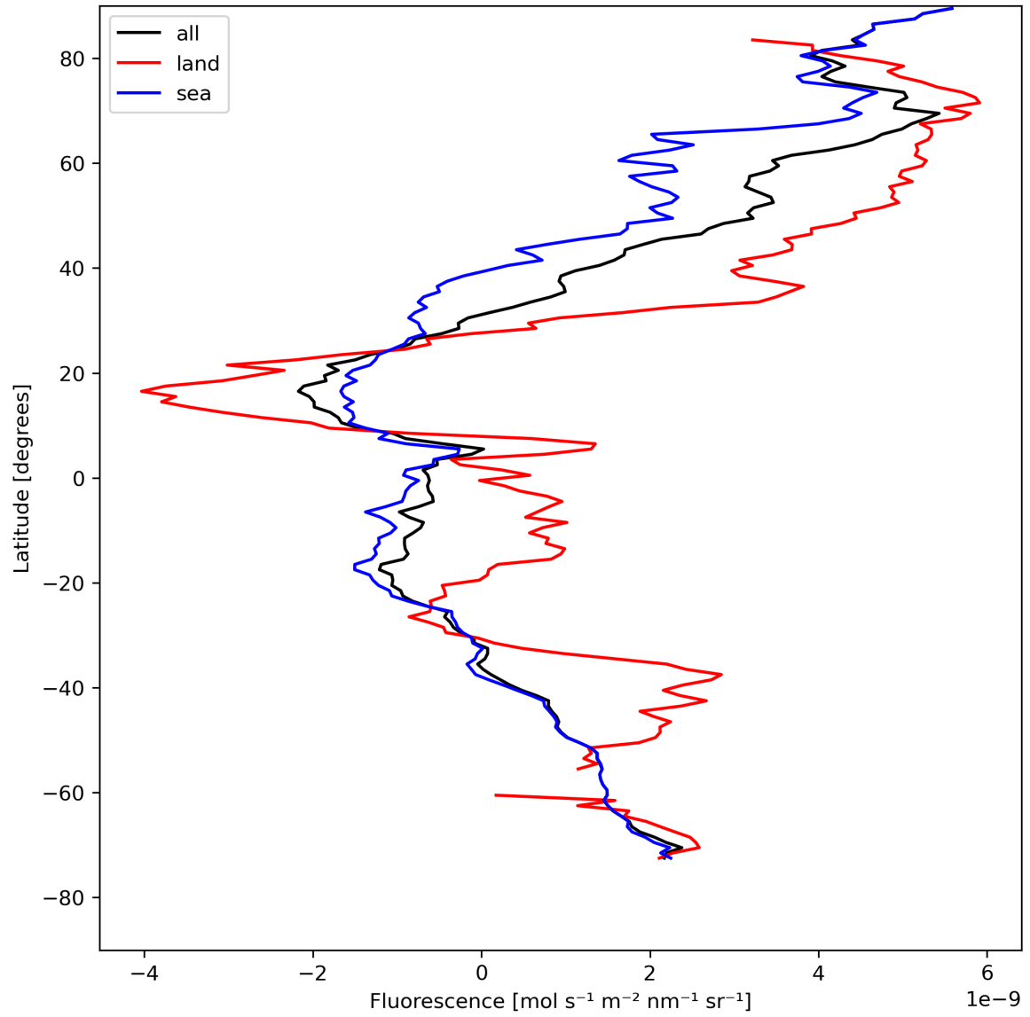
Figure 23: Zonal average of “Fluorescence” for 2024-04-30 to 2024-05-02.
