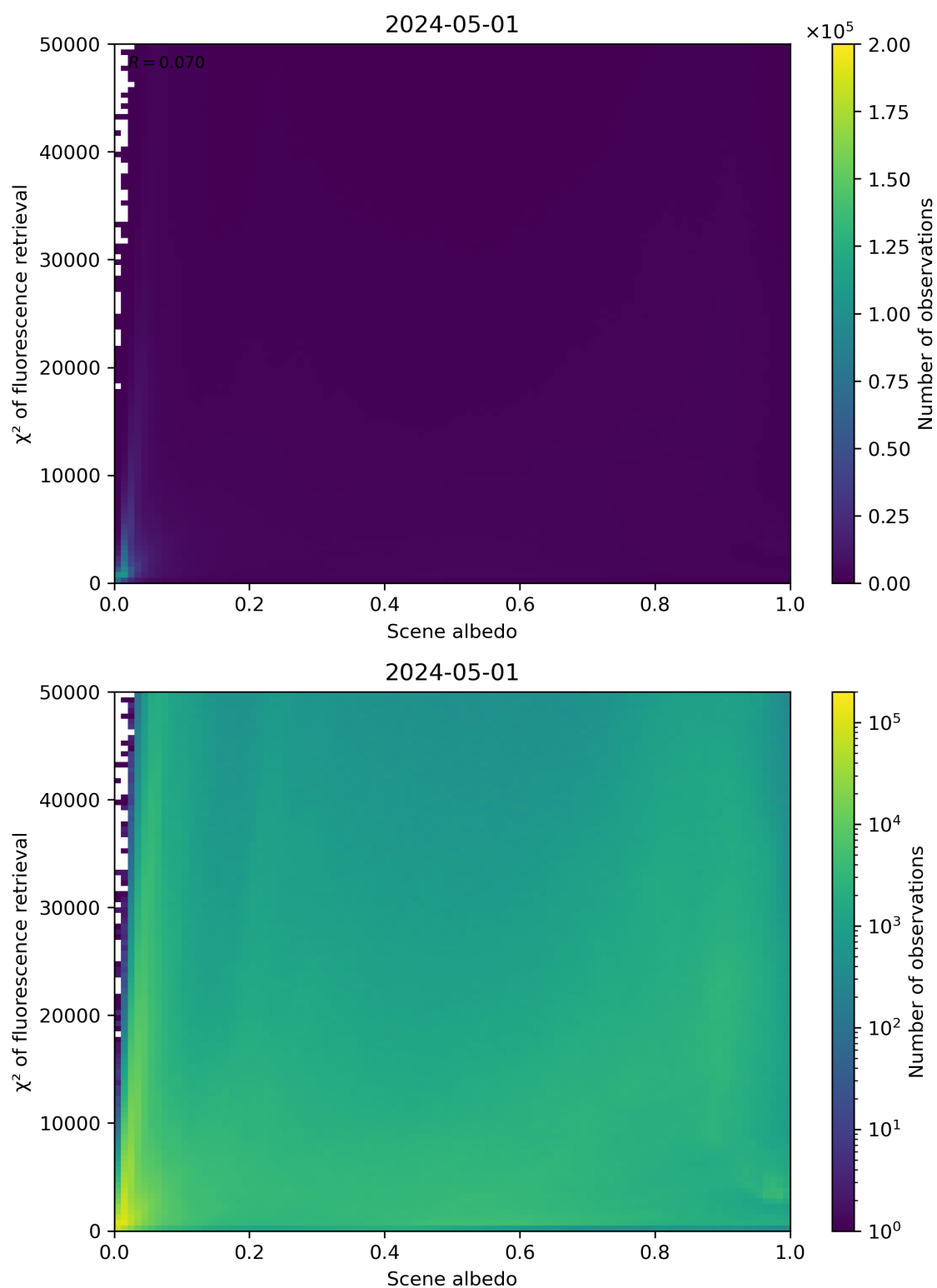
Figure 103: Scatter density plot of “Scene albedo” against “ \chi^2 of fluorescence retrieval” for 2024-04-30 to 2024-05-02.
