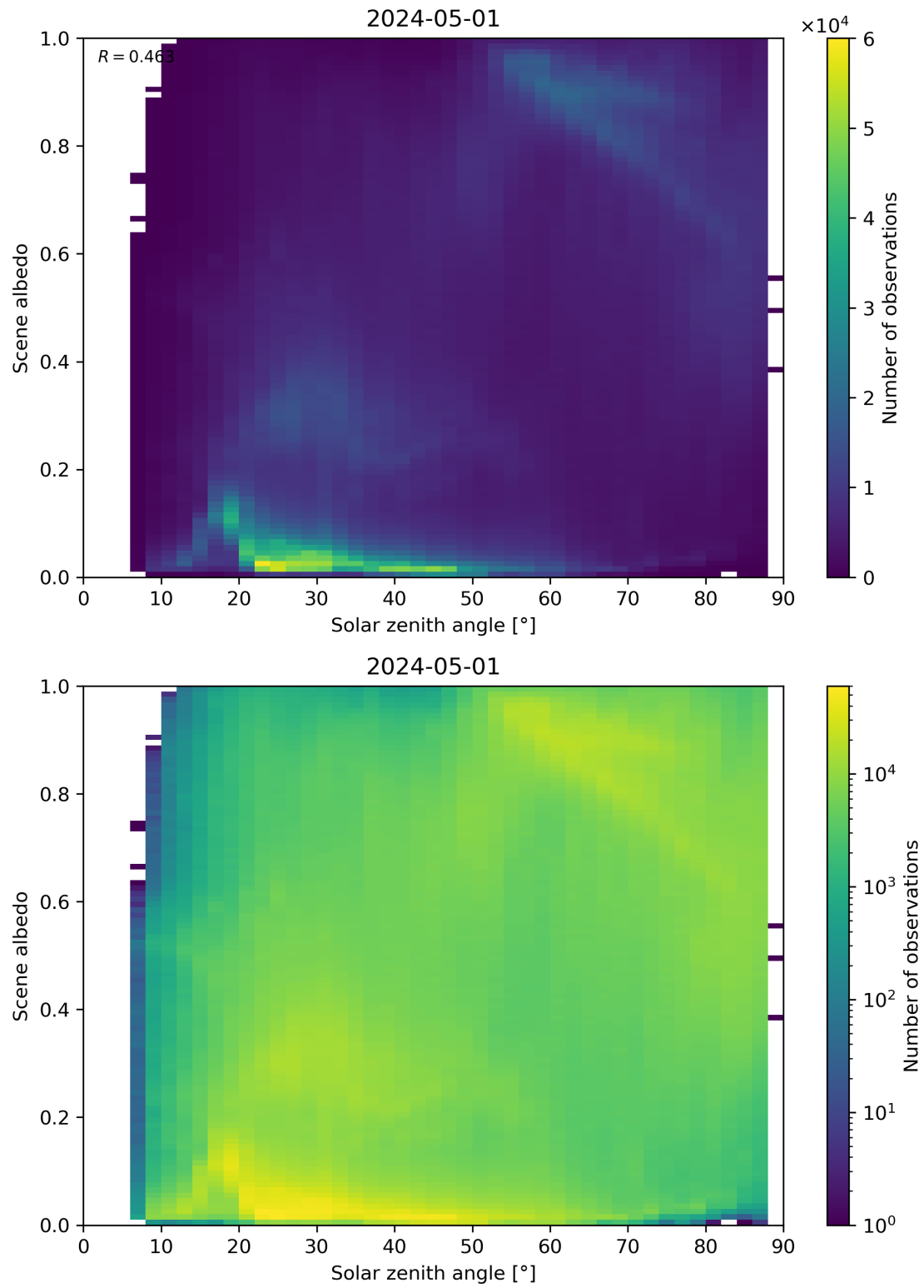
Figure 116: Scatter density plot of “Solar zenith angle” against “Scene albedo” for 2024-04-30 to 2024-05-02.
