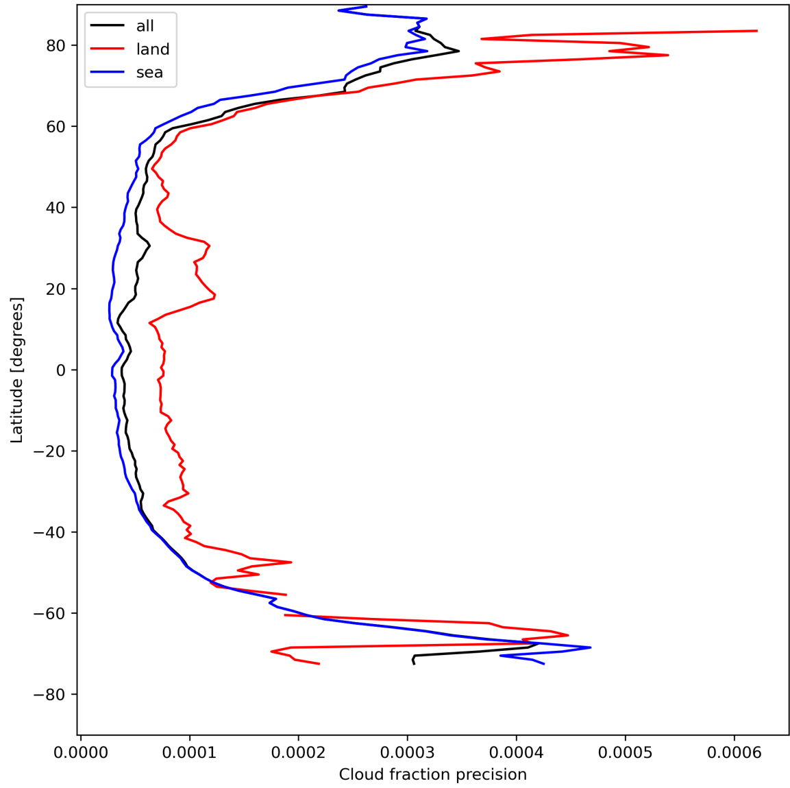
Figure 16: Zonal average of “Cloud fraction precision” for 2024-04-30 to 2024-05-02.
