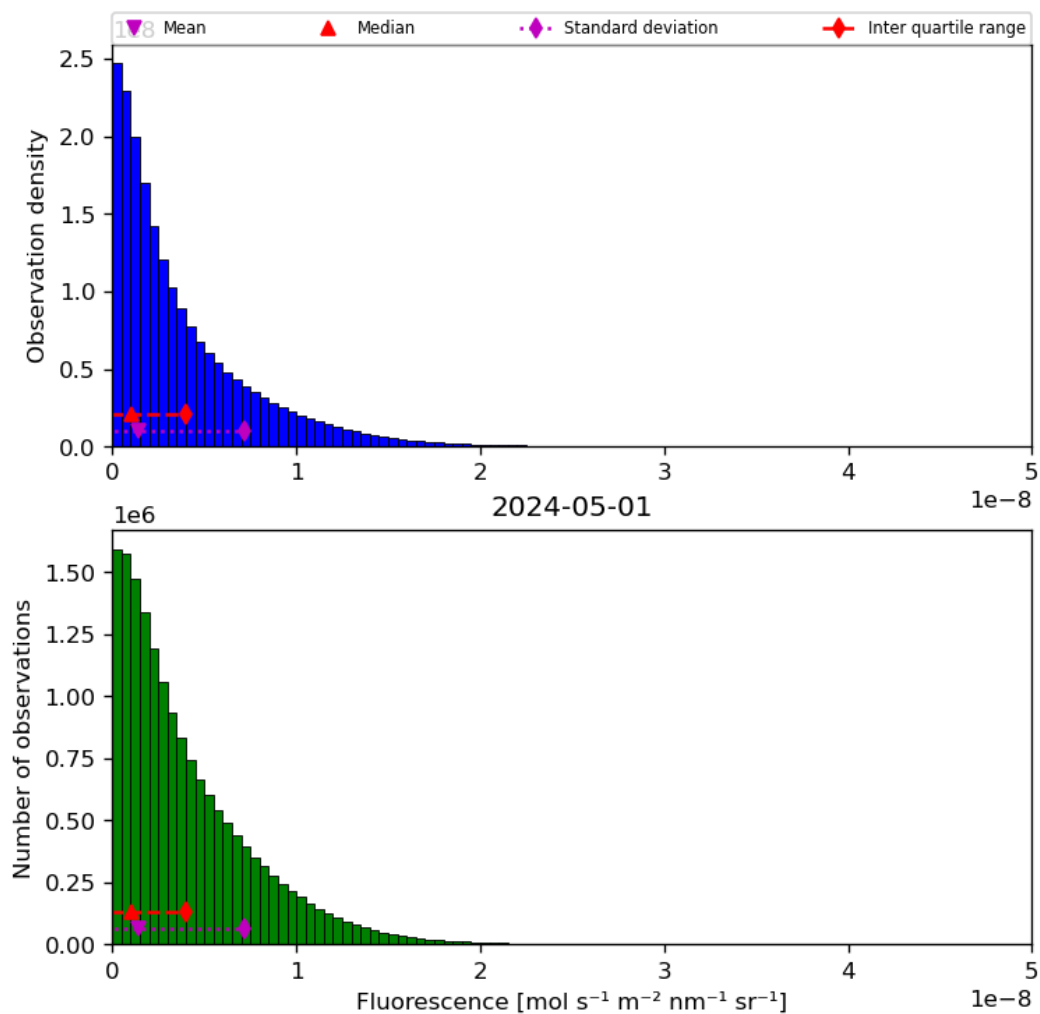
Figure 40: Histogram of “Fluorescence” for 2024-04-30 to 2024-05-02
