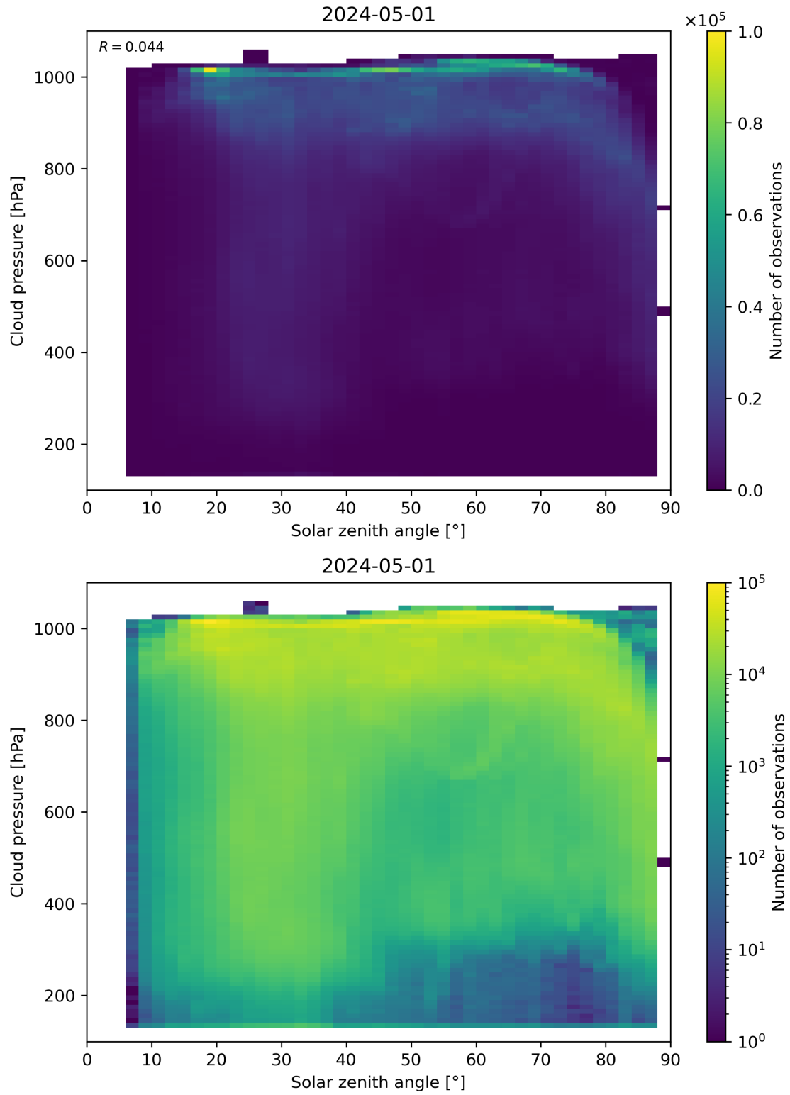
Figure 111: Scatter density plot of “Solar zenith angle” against “Cloud pressure” for 2024-04-30 to 2024-05-02.
