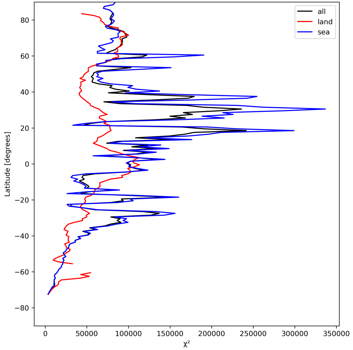
Figure 21: Zonal average of “ \chi^2 ” for 2024-04-30 to 2024-05-02.
