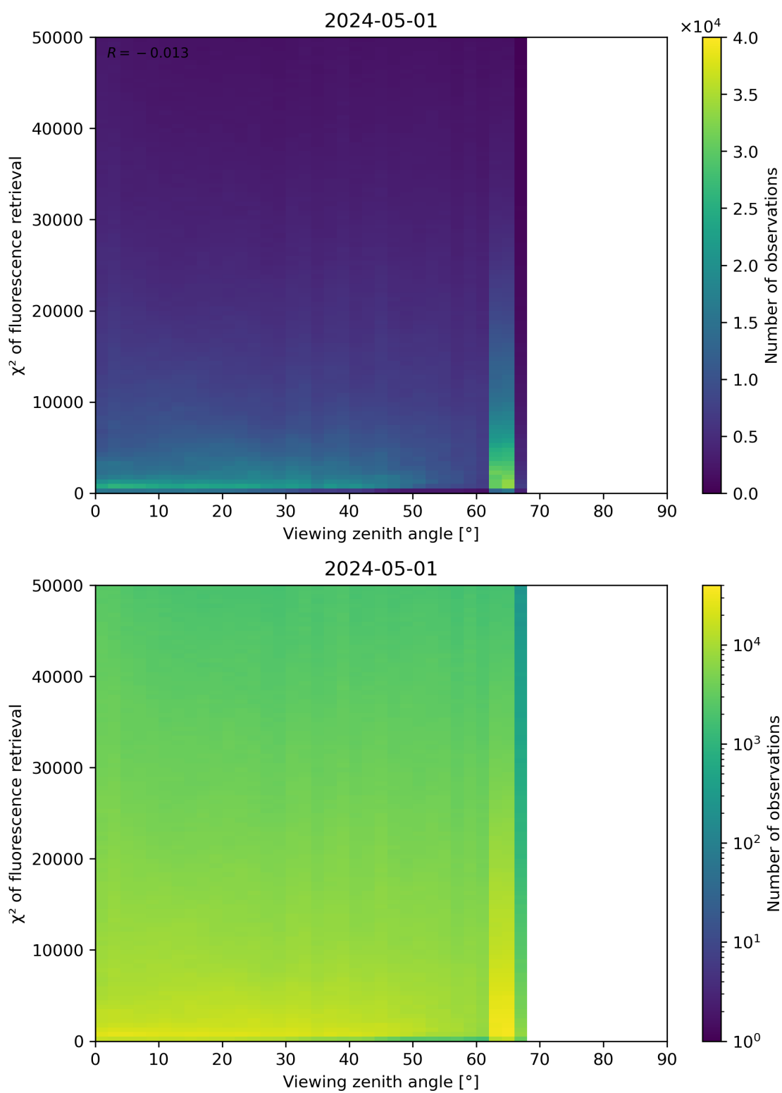
Figure 119: Scatter density plot of “Viewing zenith angle” against “ \chi^2 of fluorescence retrieval” for 2024-04-30 to 2024-05-02.
