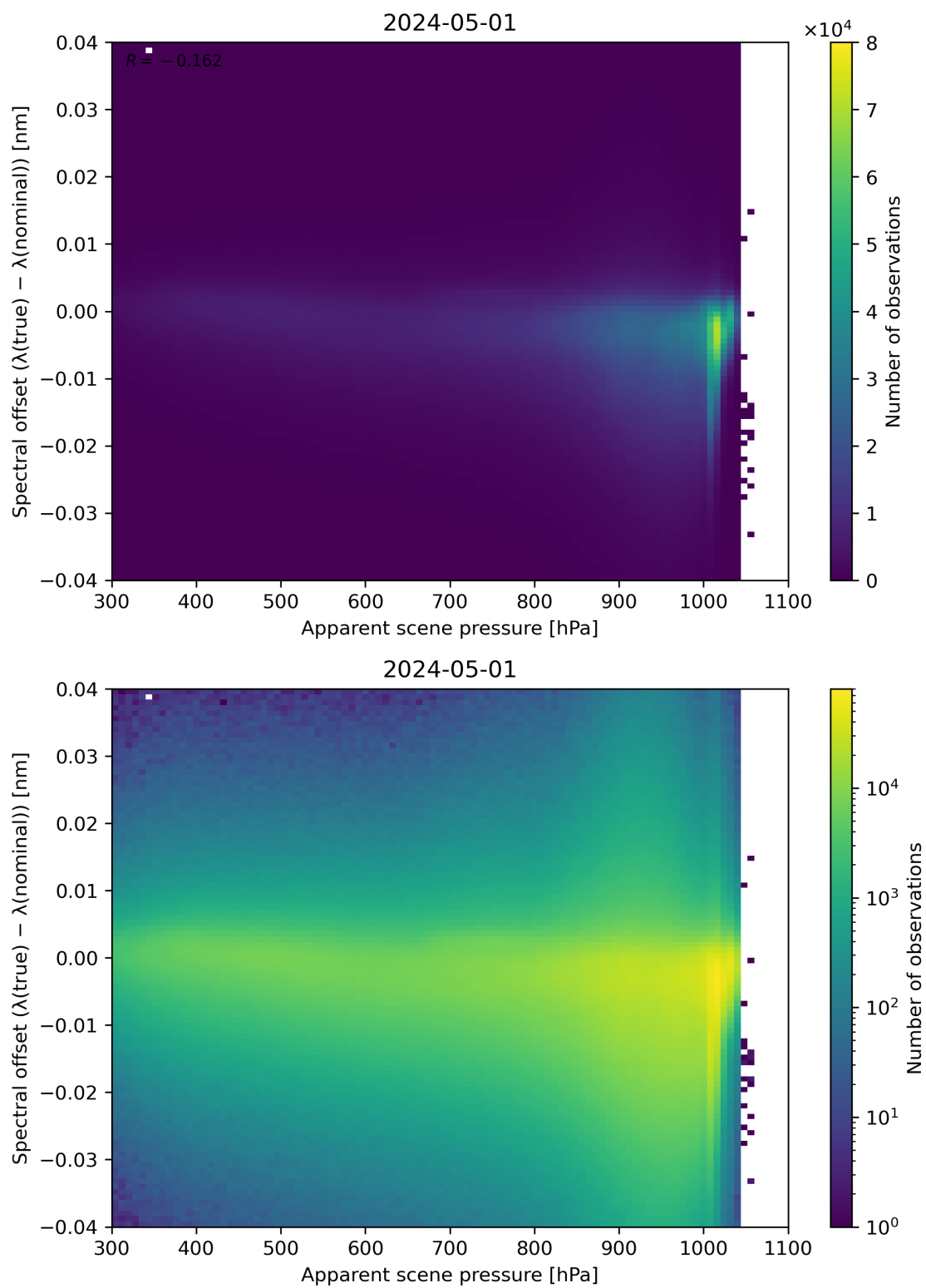
Figure 67: Scatter density plot of “Apparent scene pressure” against “Spectral offset ( \lambda(\text{true}) - \lambda(\text{nominal}) )” for 2024-04-30 to 2024-05-02.
