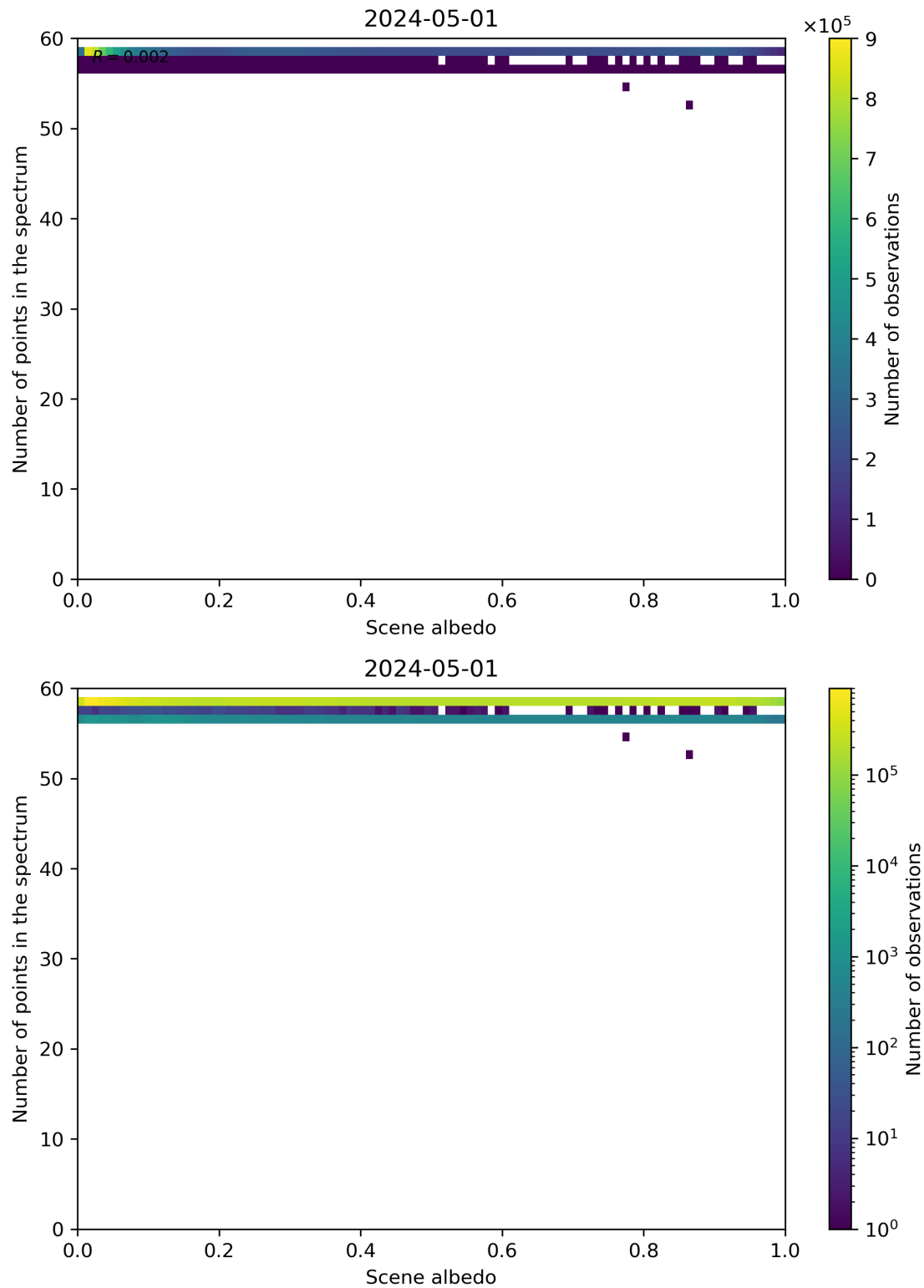
Figure 106: Scatter density plot of “Scene albedo” against “Number of points in the spectrum” for 2024-04-30 to 2024-05-02.
