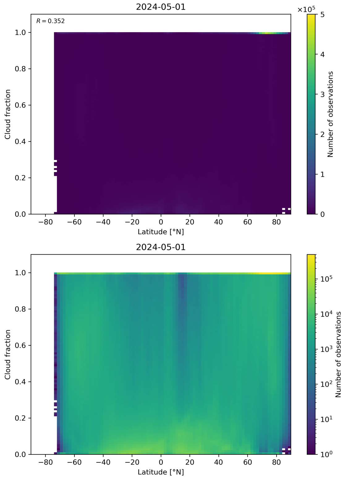
Figure 90: Scatter density plot of “Latitude” against “Cloud fraction” for 2024-04-30 to 2024-05-02.
