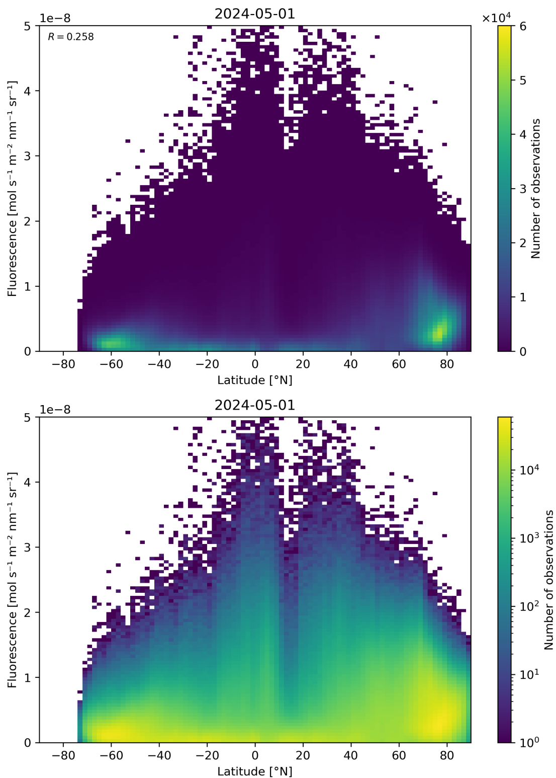
Figure 92: Scatter density plot of “Latitude” against “Fluorescence” for 2024-04-30 to 2024-05-02.
