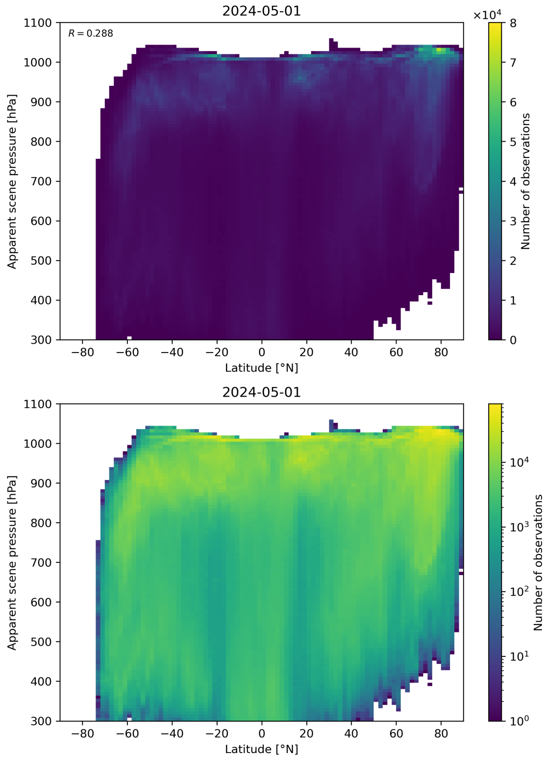
Figure 88: Scatter density plot of “Latitude” against “Apparent scene pressure” for 2024-04-30 to 2024-05-02.
