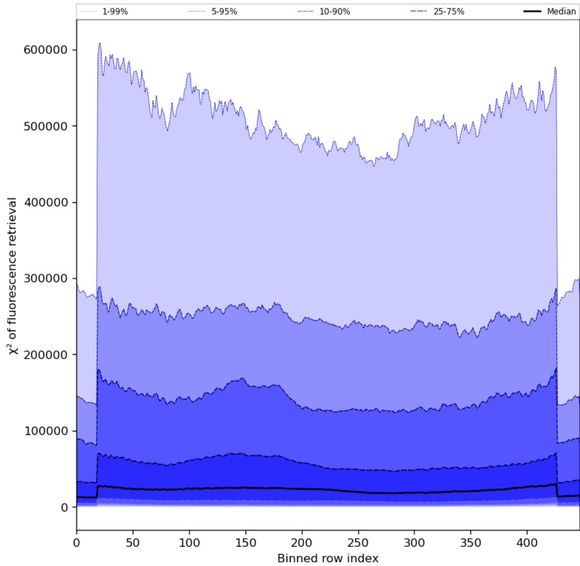
Figure 59: Along track statistics of “ \chi^2 of fluorescence retrieval” for 2024-04-30 to 2024-05-02
