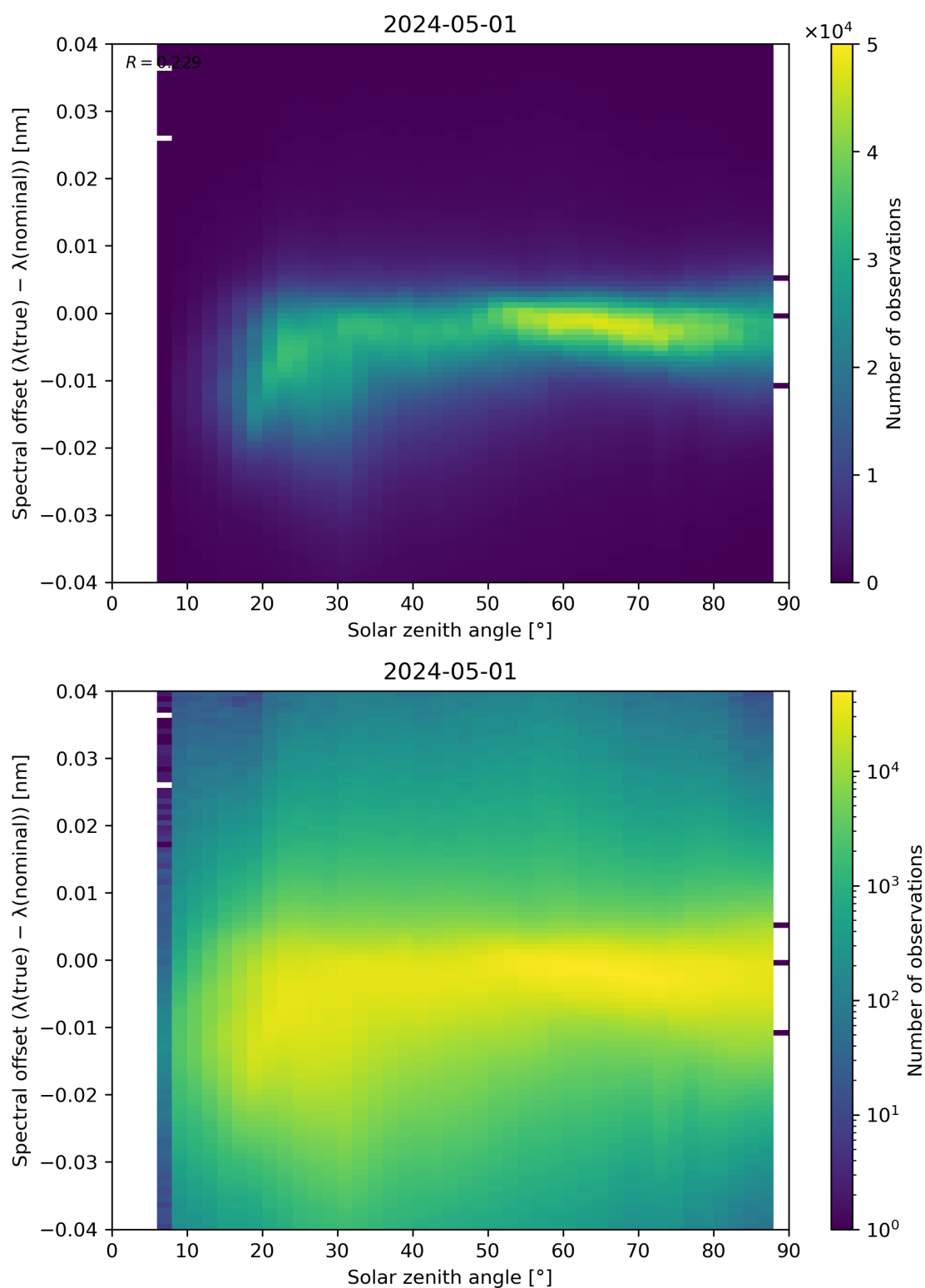
Figure 117: Scatter density plot of “Solar zenith angle” against “Spectral offset ( \lambda(\text{true}) - \lambda(\text{nominal}) )” for 2024-04-30 to 2024-05-02.
