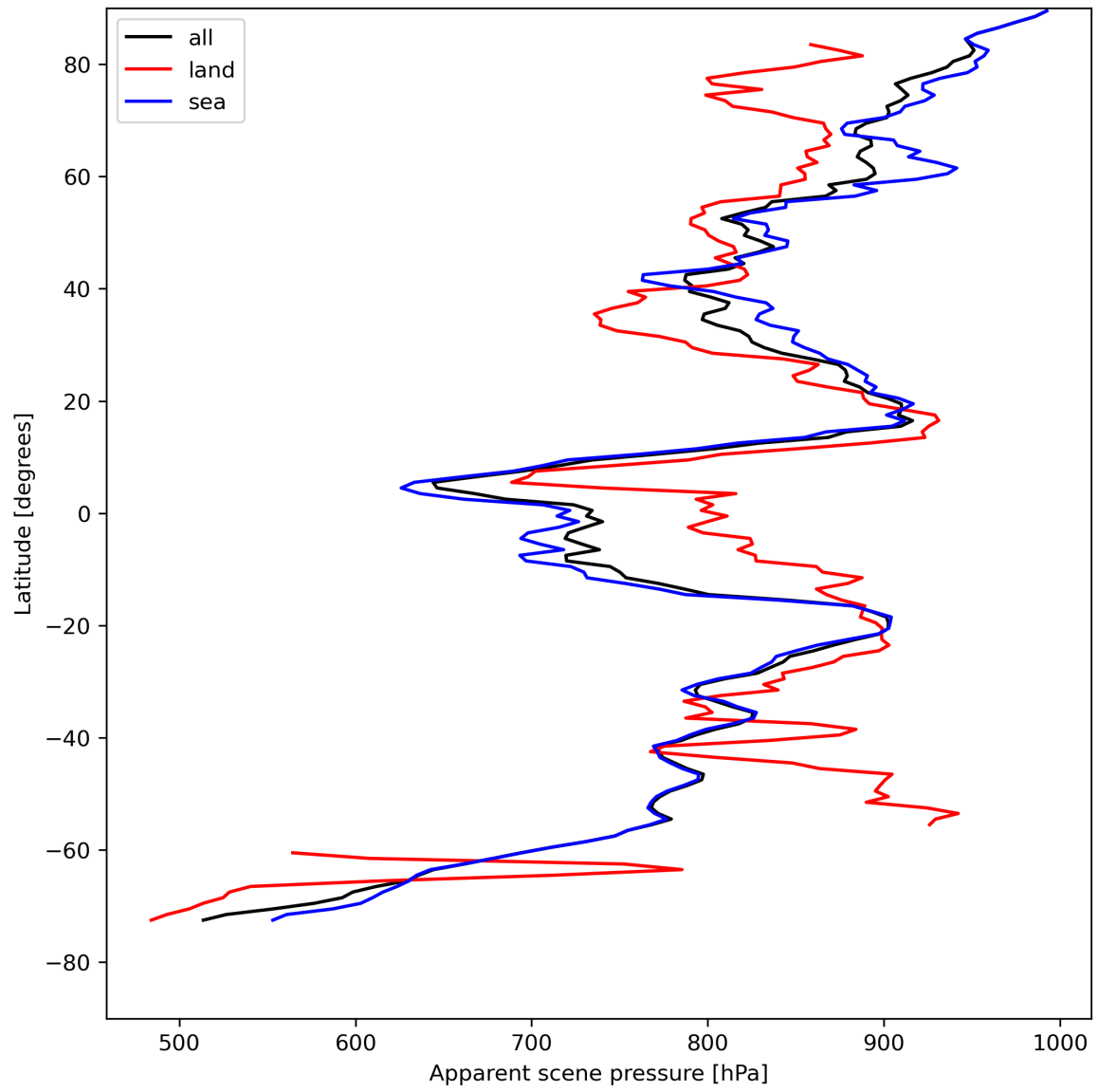
Figure 19: Zonal average of “Apparent scene pressure” for 2024-04-30 to 2024-05-02.
