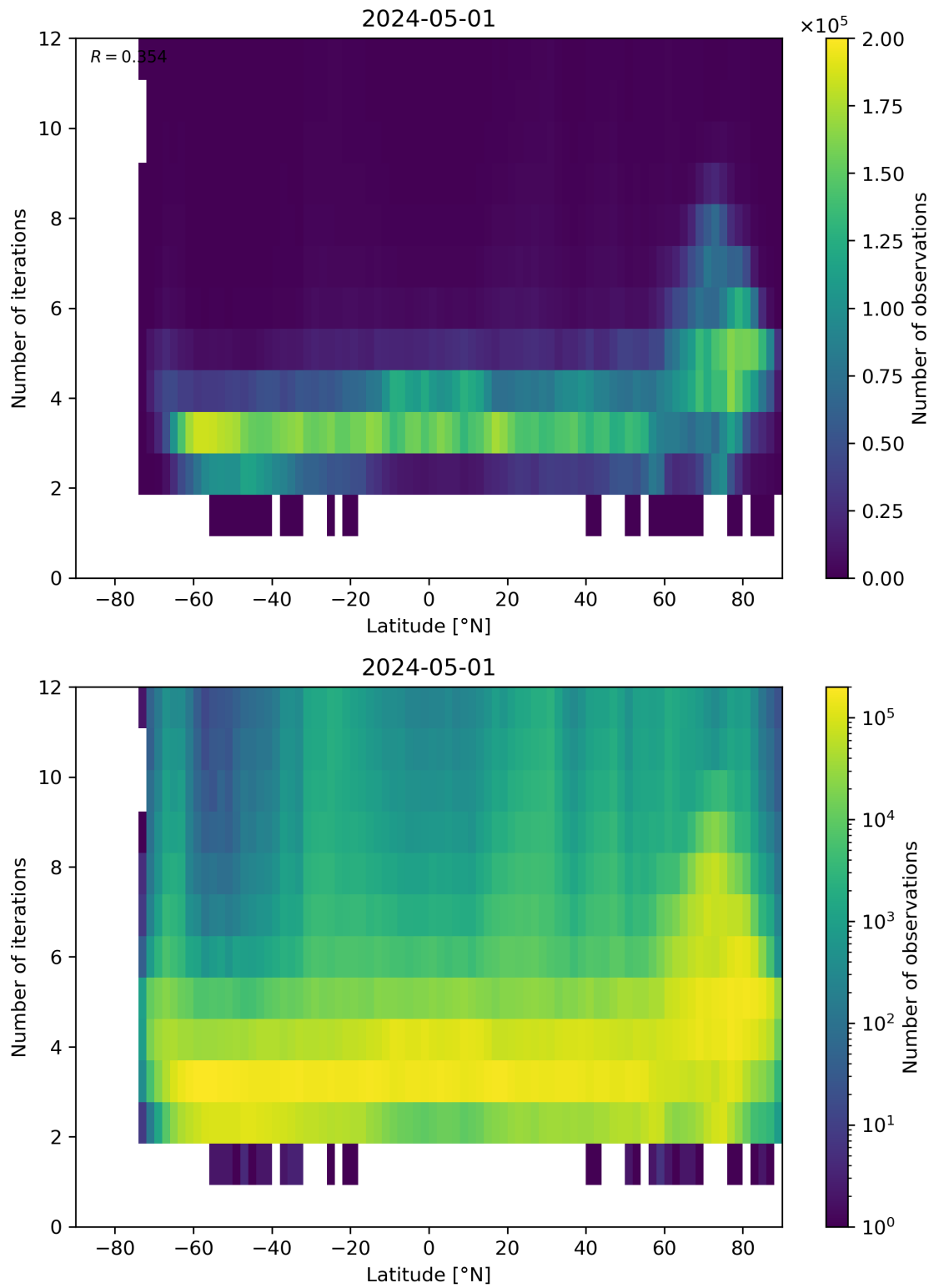
Figure 93: Scatter density plot of “Latitude” against “Number of iterations” for 2024-04-30 to 2024-05-02.
