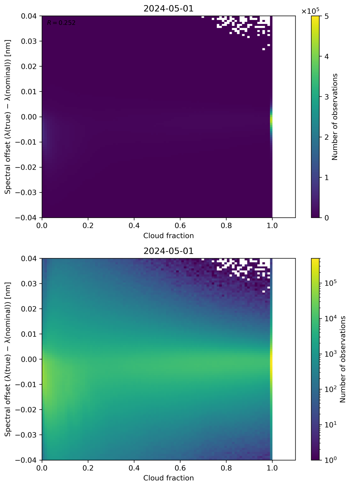
Figure 76: Scatter density plot of “Cloud fraction” against “Spectral offset ( \lambda(\text{true}) - \lambda(\text{nominal}) )” for 2024-04-30 to 2024-05-02.
