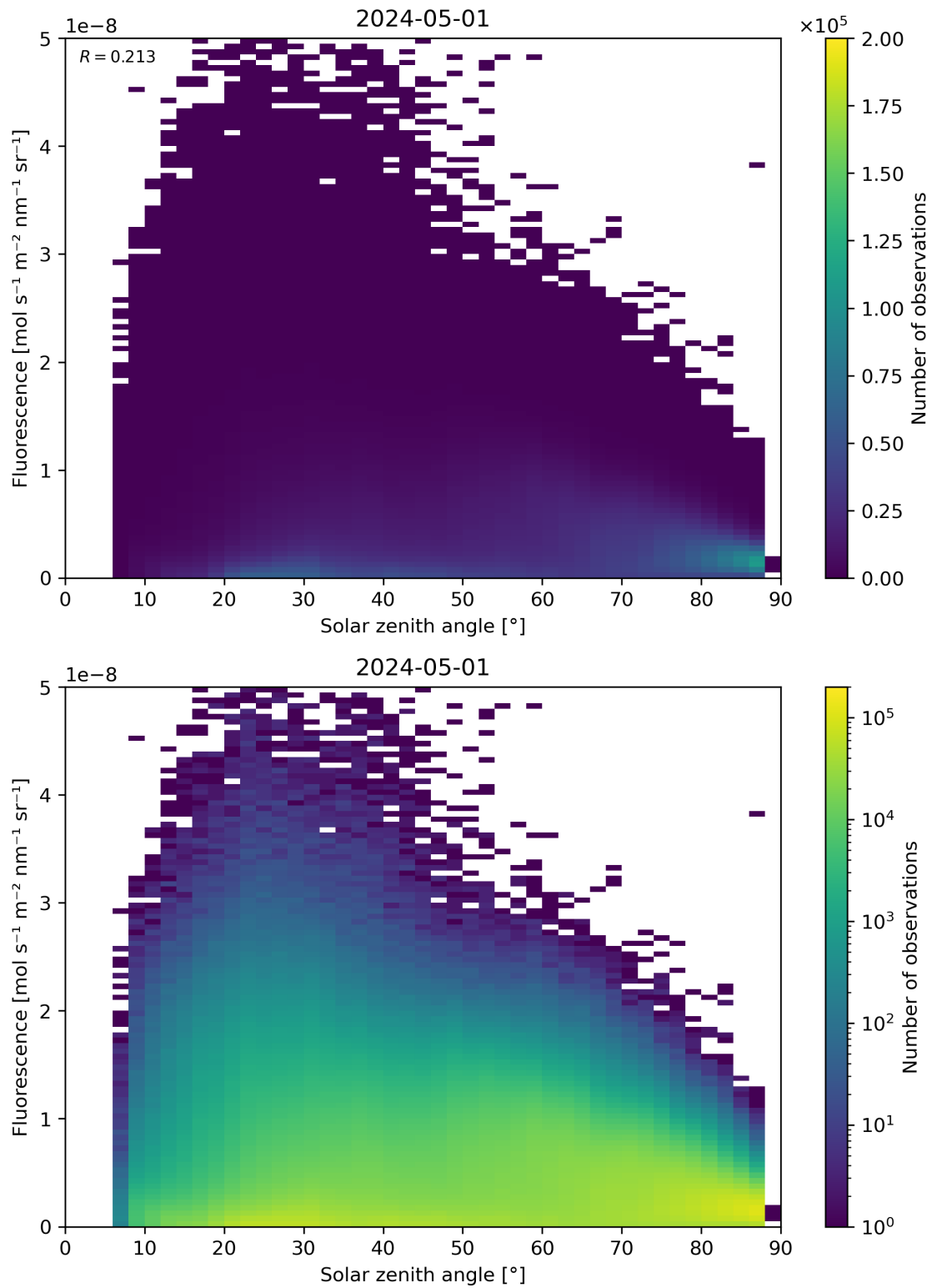
Figure 112: Scatter density plot of “Solar zenith angle” against “Fluorescence” for 2024-04-30 to 2024-05-02.
