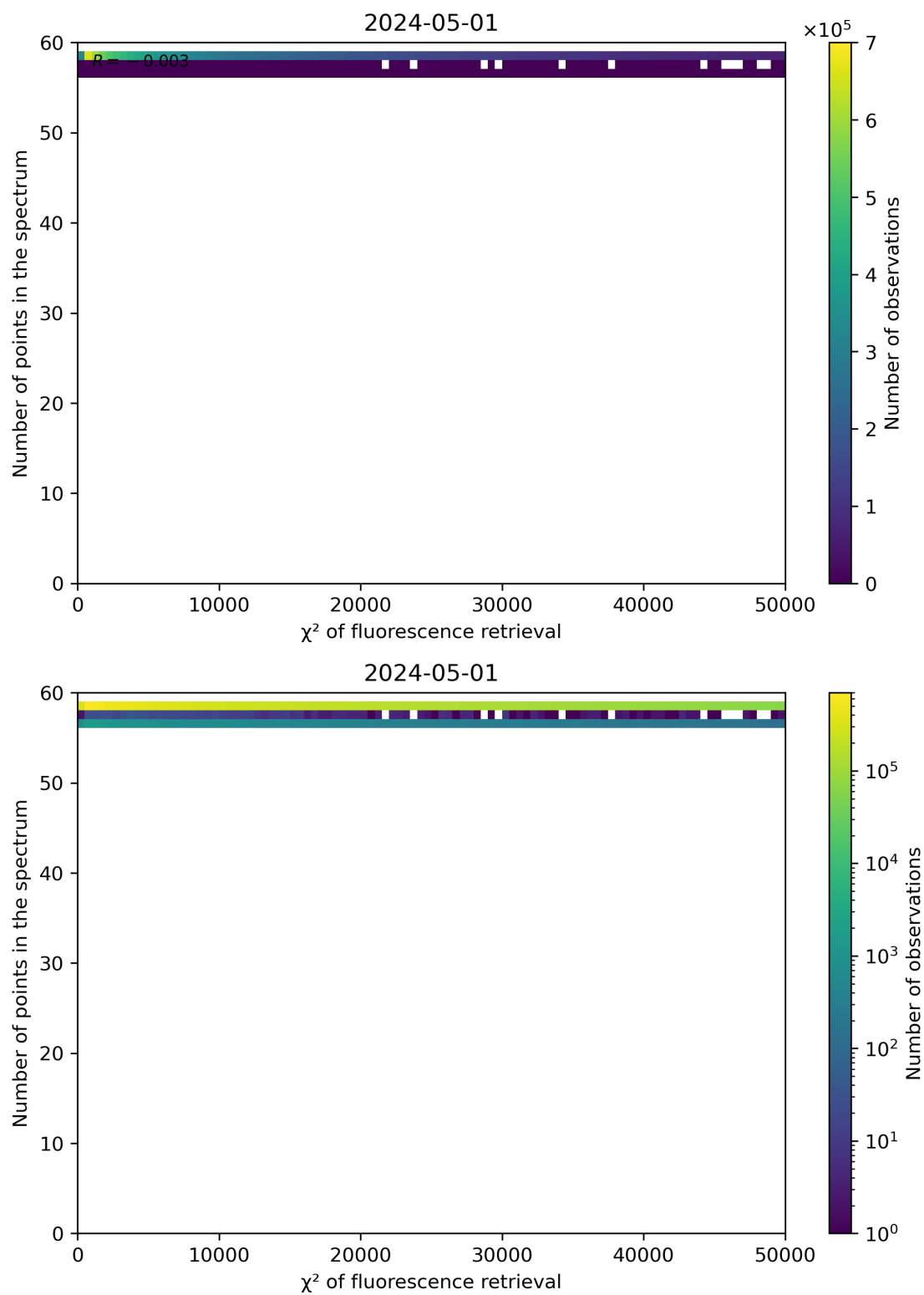
Figure 68: Scatter density plot of " \chi^2 of fluorescence retrieval" against "Number of points in the spectrum" for 2024-04-30 to 2024-05-02.
