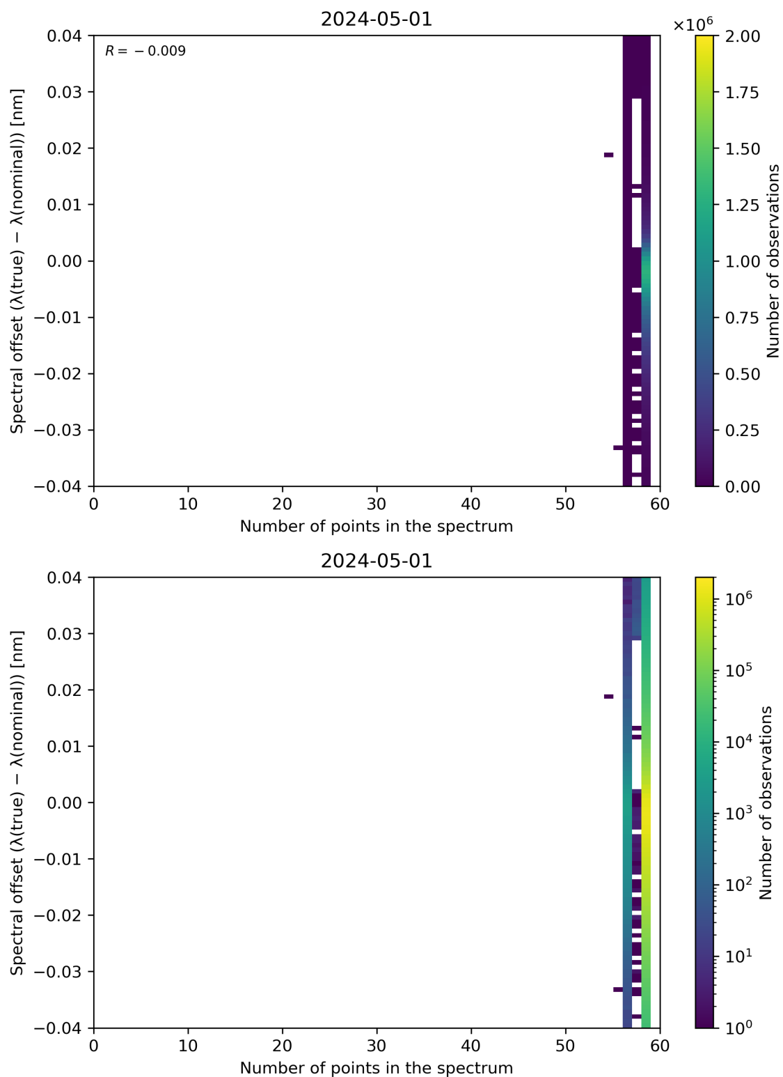
Figure 101: Scatter density plot of “Number of points in the spectrum” against “Spectral offset ( \lambda(\text{true}) - \lambda(\text{nominal}) )” for 2024-04-30 to 2024-05-02.
