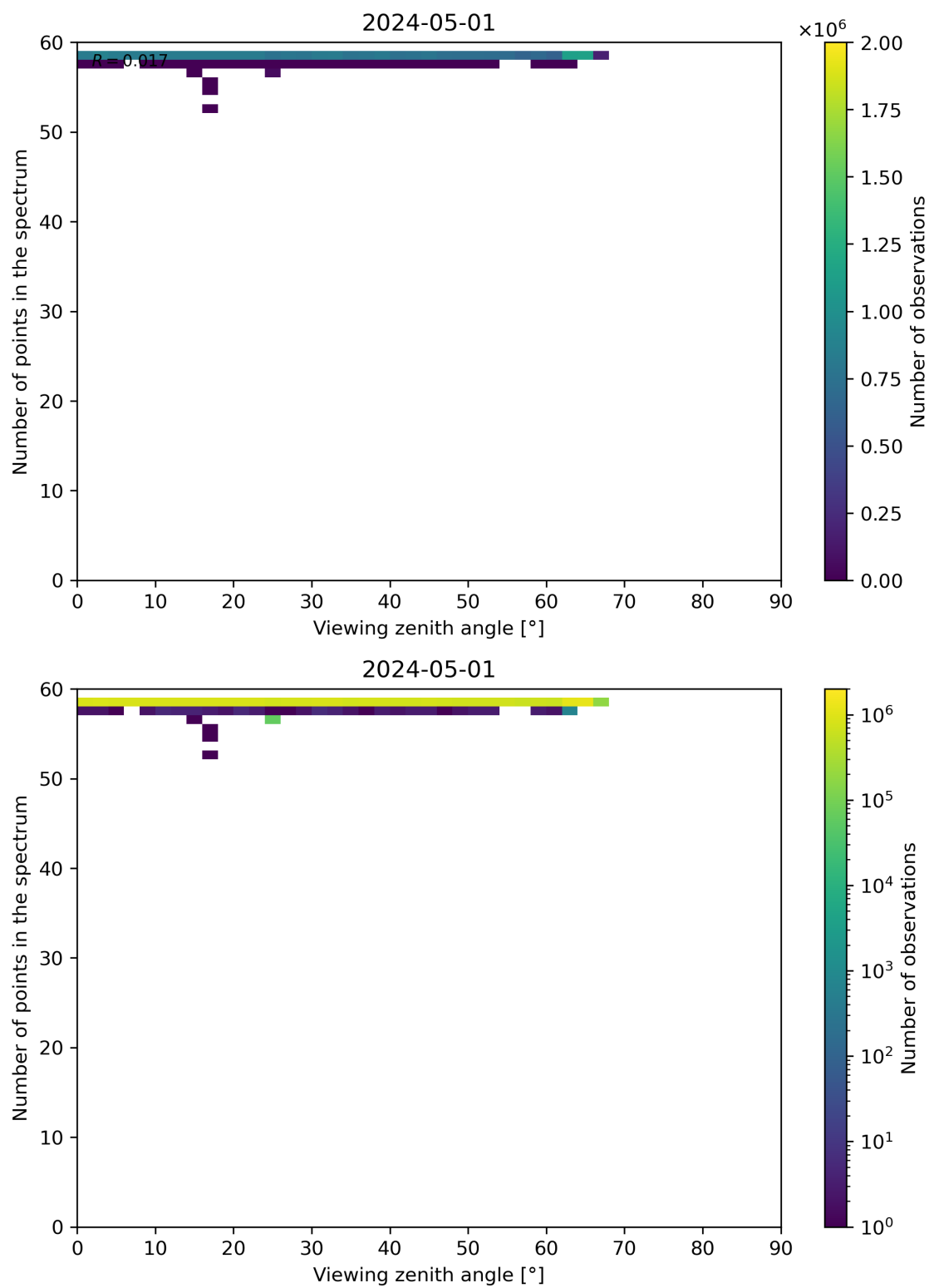
Figure 125: Scatter density plot of “Viewing zenith angle” against “Number of points in the spectrum” for 2024-04-30 to 2024-05-02.
