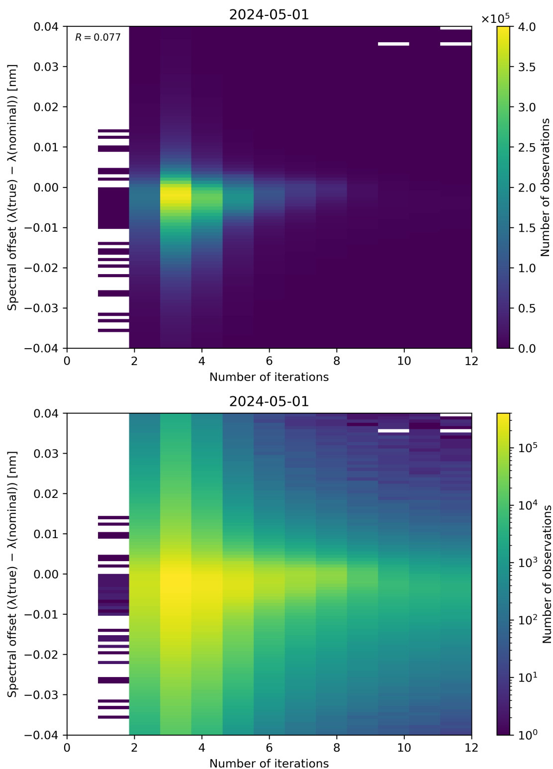
Figure 100: Scatter density plot of “Number of iterations” against “Spectral offset ( \lambda(\text{true}) - \lambda(\text{nominal}) )” for 2024-04-30 to 2024-05-02.
