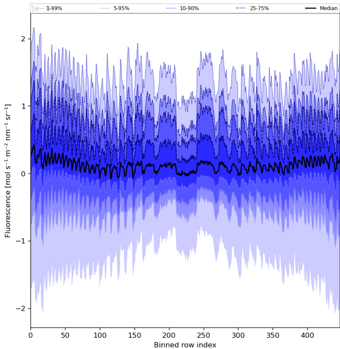
Figure 57: Along track statistics of “Fluorescence” for 2024-04-30 to 2024-05-02
