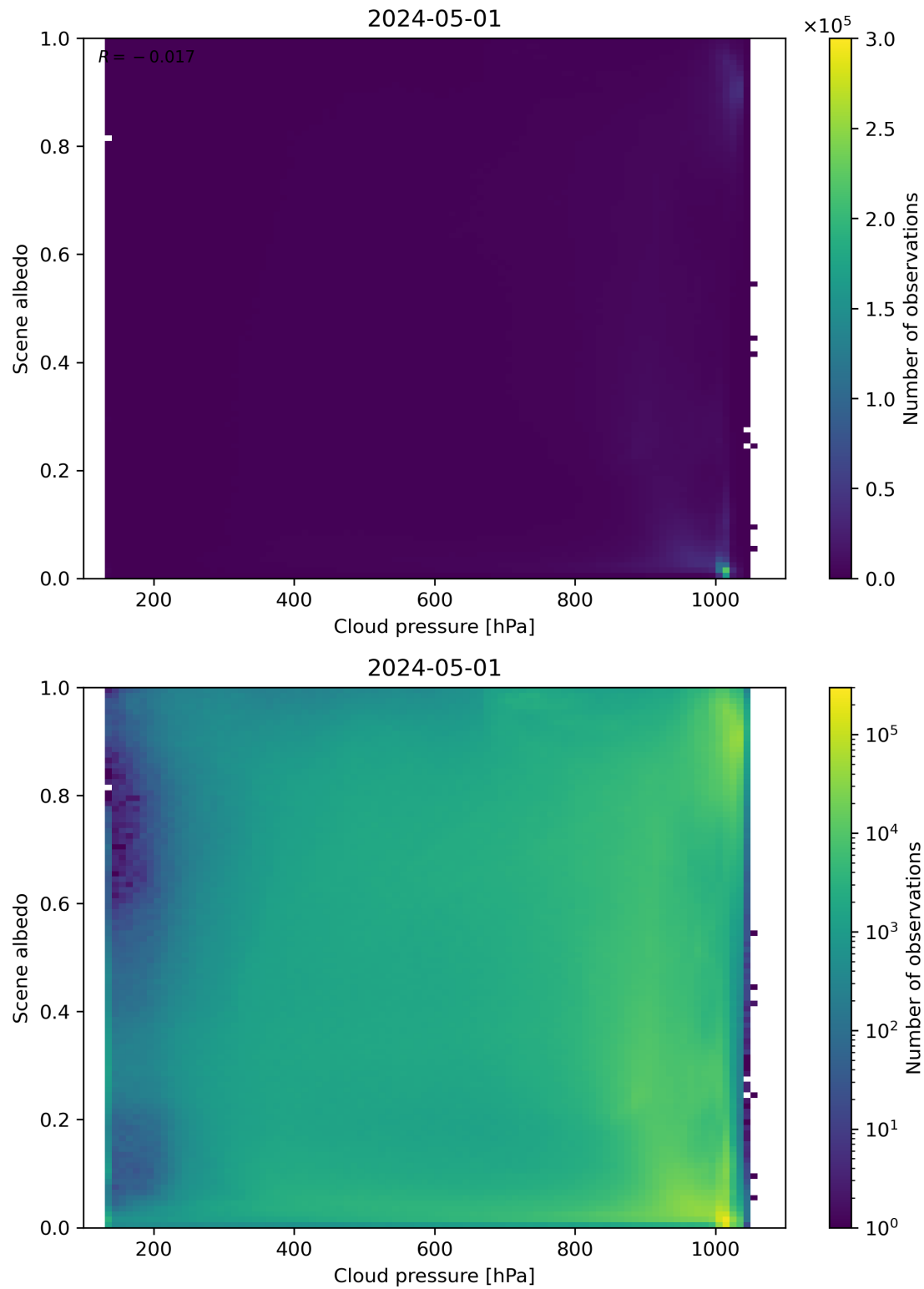
Figure 83: Scatter density plot of “Cloud pressure” against “Scene albedo” for 2024-04-30 to 2024-05-02.
