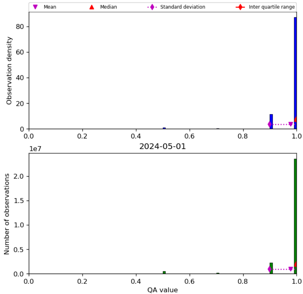
Figure 29: Histogram of “QA value” for 2024-04-30 to 2024-05-02
