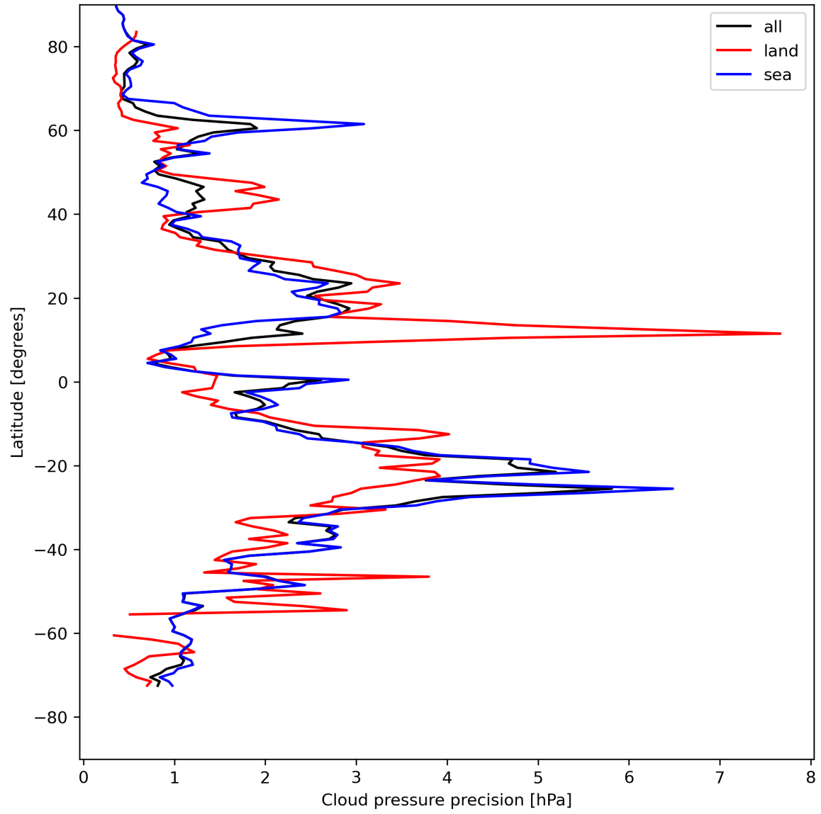
Figure 14: Zonal average of "Cloud pressure precision" for 2024-04-30 to 2024-05-02.
