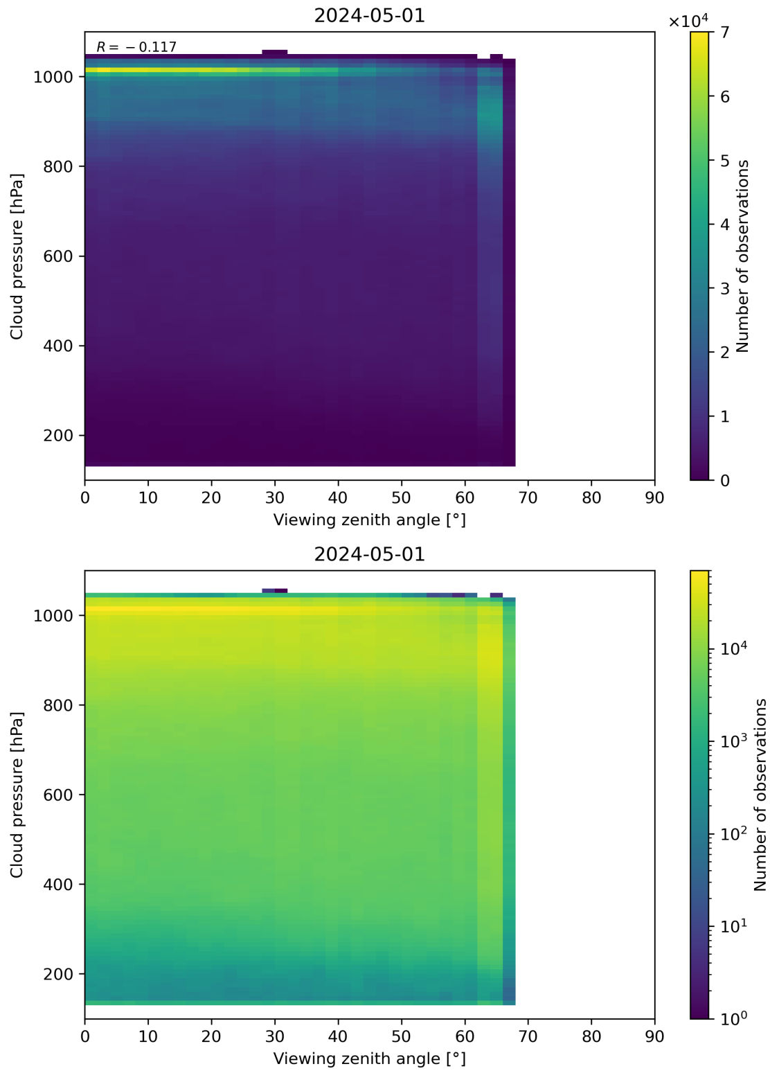
Figure 121: Scatter density plot of “Viewing zenith angle” against “Cloud pressure” for 2024-04-30 to 2024-05-02.
