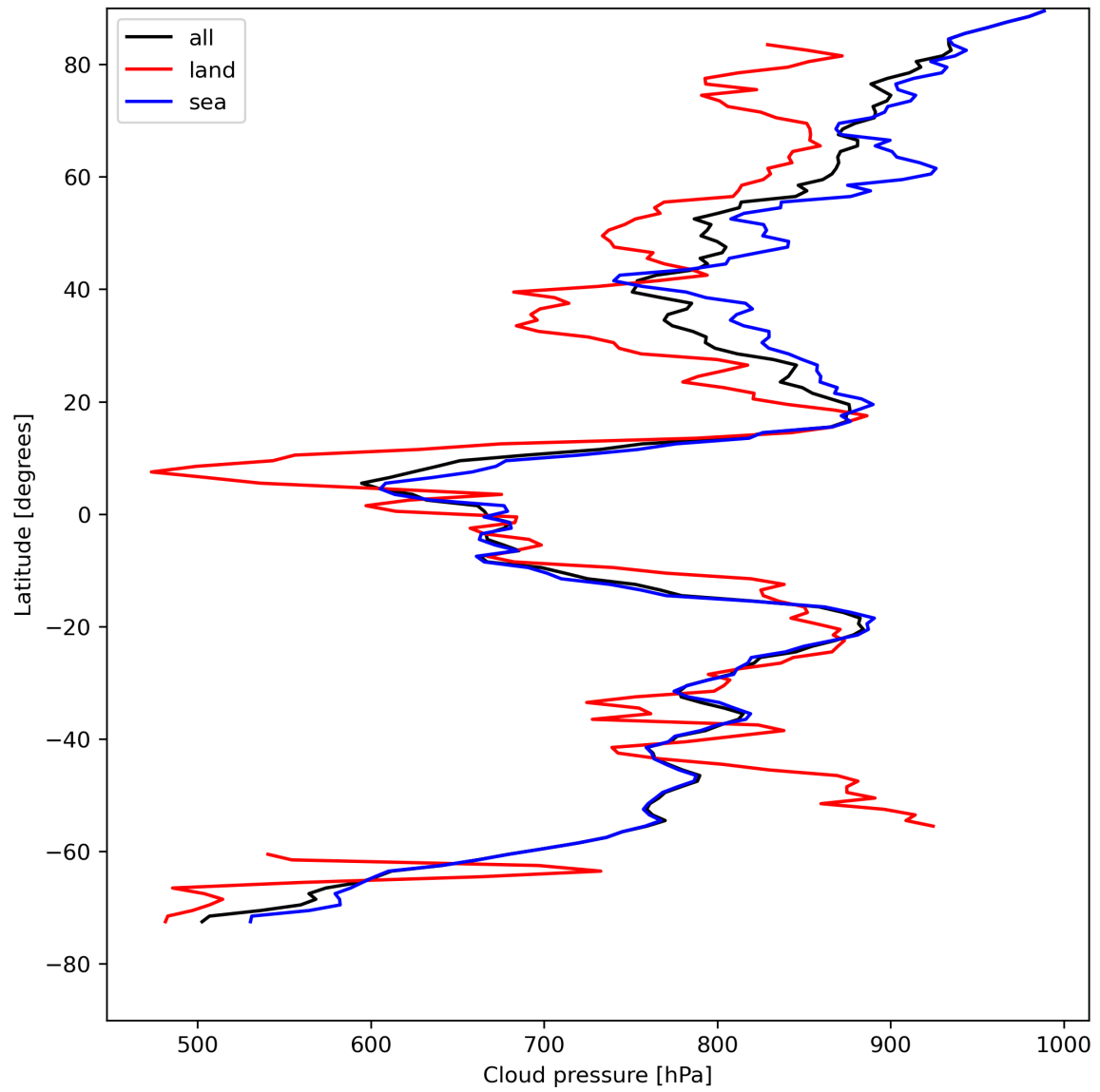
Figure 13: Zonal average of “Cloud pressure” for 2024-04-30 to 2024-05-02.
