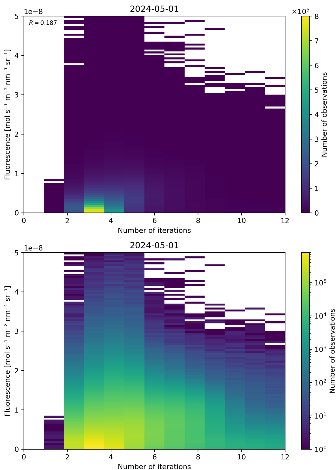
Figure 98: Scatter density plot of “Number of iterations” against “Fluorescence” for 2024-04-30 to 2024-05-02.
