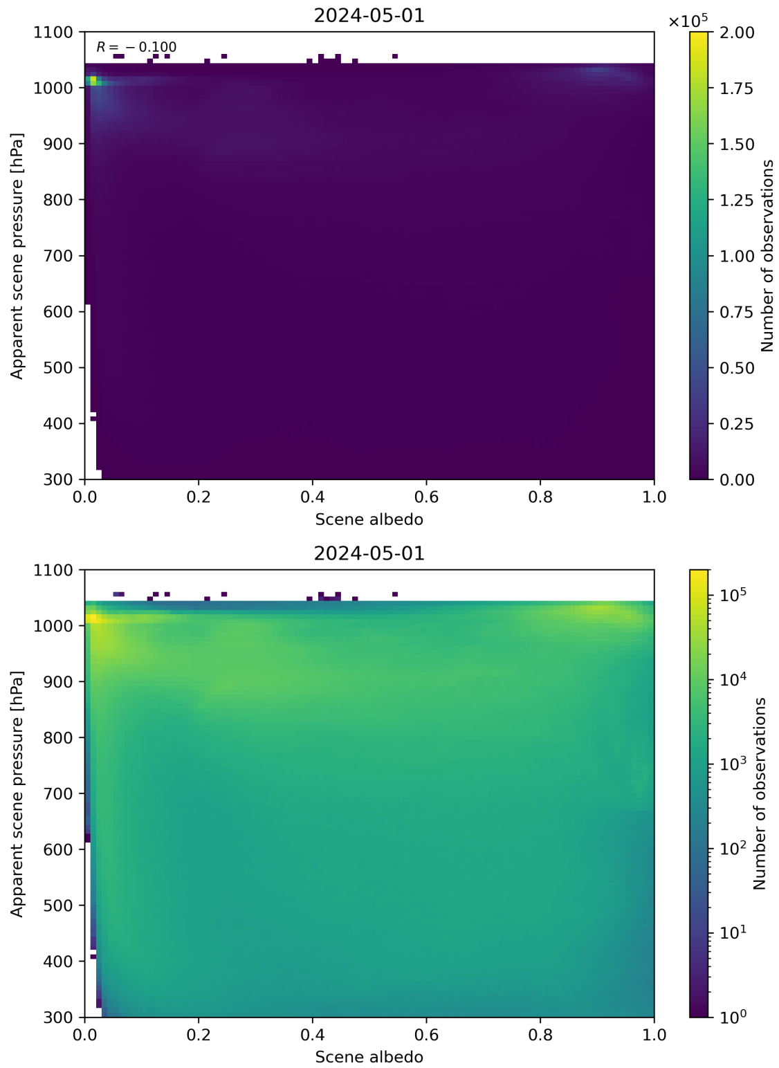
Figure 102: Scatter density plot of “Scene albedo” against “Apparent scene pressure” for 2024-04-30 to 2024-05-02.
