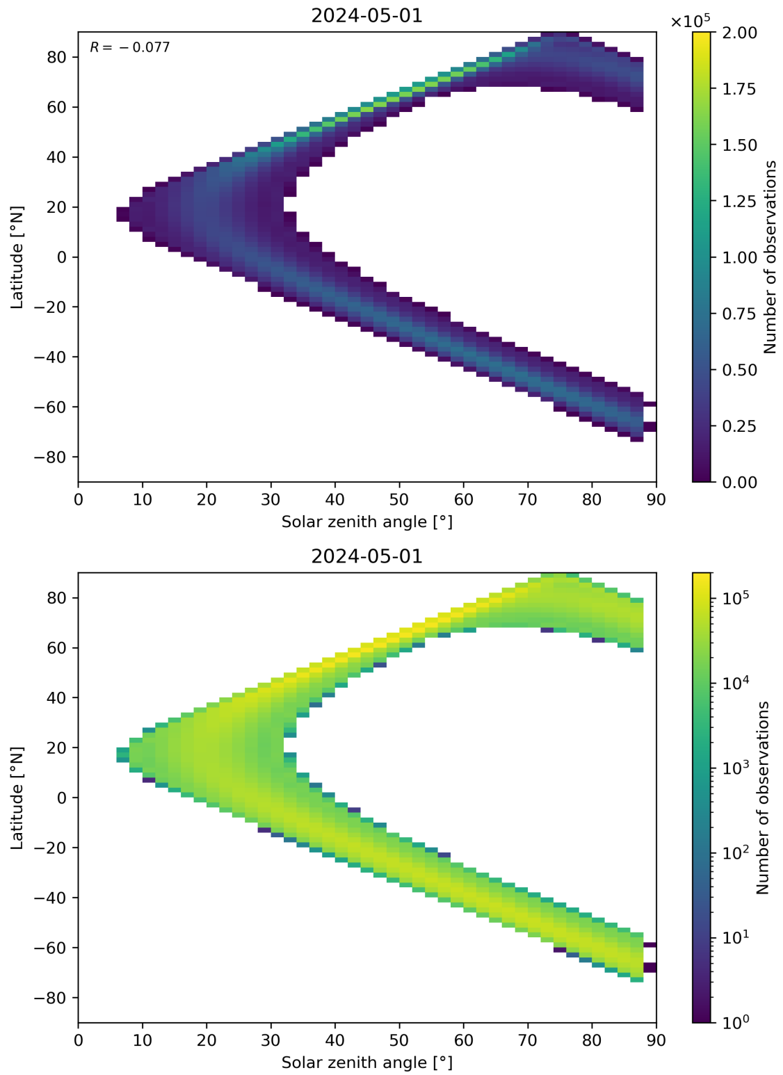
Figure 113: Scatter density plot of “Solar zenith angle” against “Latitude” for 2024-04-30 to 2024-05-02.
