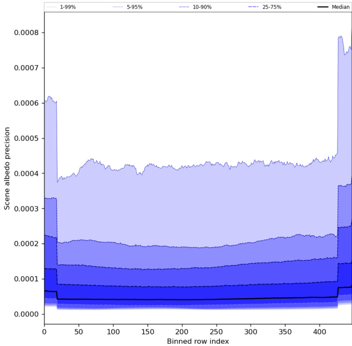
Figure 52: Along track statistics of “Scene albedo precision” for 2024-04-30 to 2024-05-02
