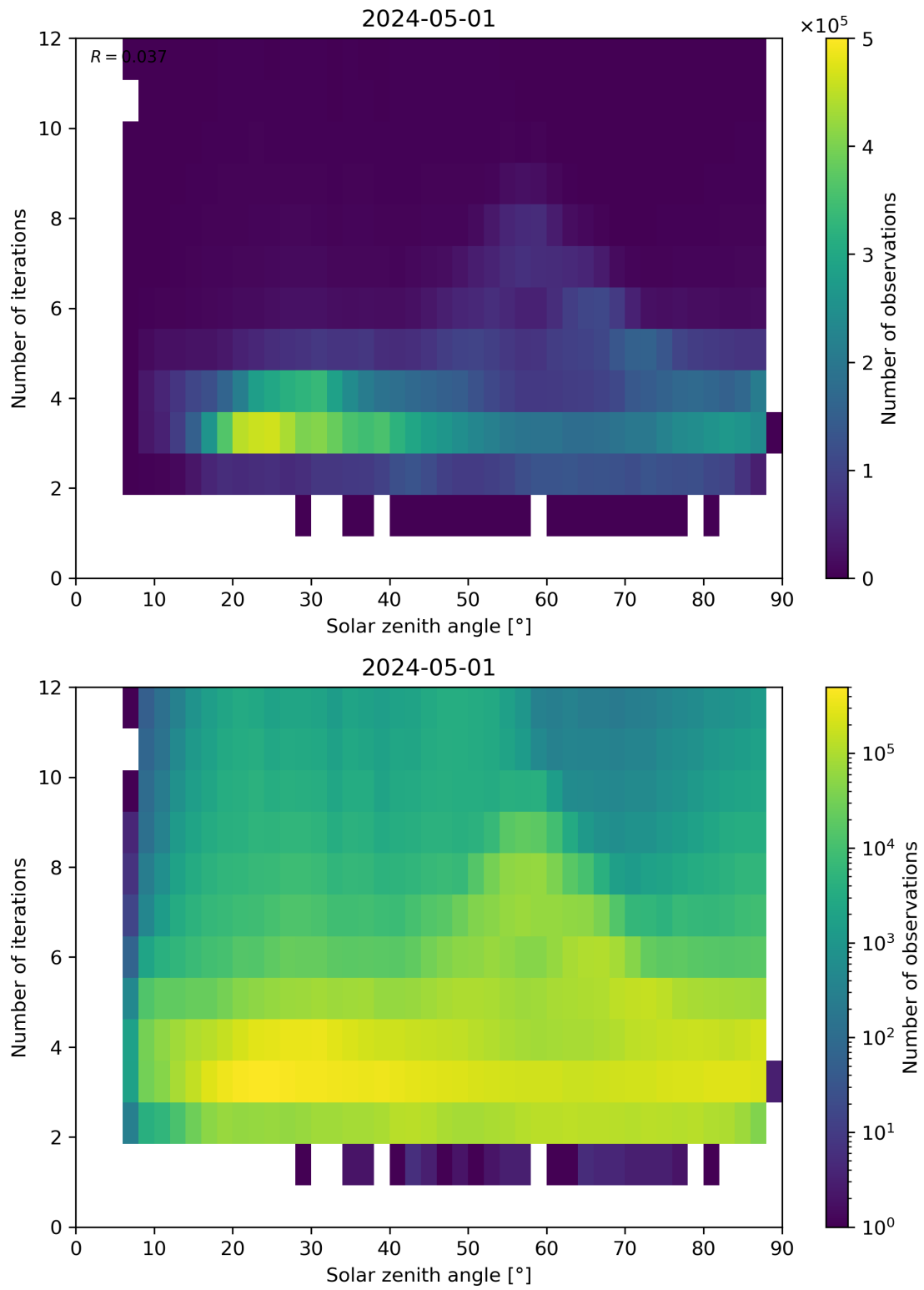
Figure 114: Scatter density plot of “Solar zenith angle” against “Number of iterations” for 2024-04-30 to 2024-05-02.
