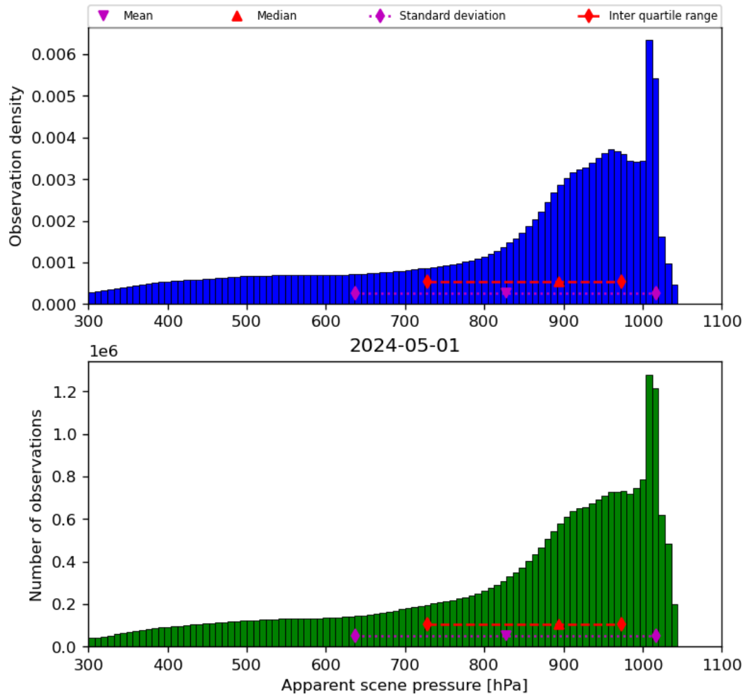
Figure 36: Histogram of “Apparent scene pressure” for 2024-04-30 to 2024-05-02
